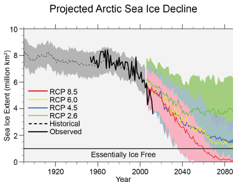
Figure 1. The current sea ice extent record and model projections. The Arctic sea ice extent declined more than 60% during the satellite era (1979–present). The colored lines and shaded regions represent the sea ice extent predictions and variances for several Representative Concentration Pathways (RCP). RCP 8.5 represents a scenario with high greenhouse gas emissions and predicts an essentially ice free Arctic by 2060. Note that ice extents predicted under the RCP 8.5 scenario under predicts extent compared to observations for recent years (Melillo et al. 2014).
