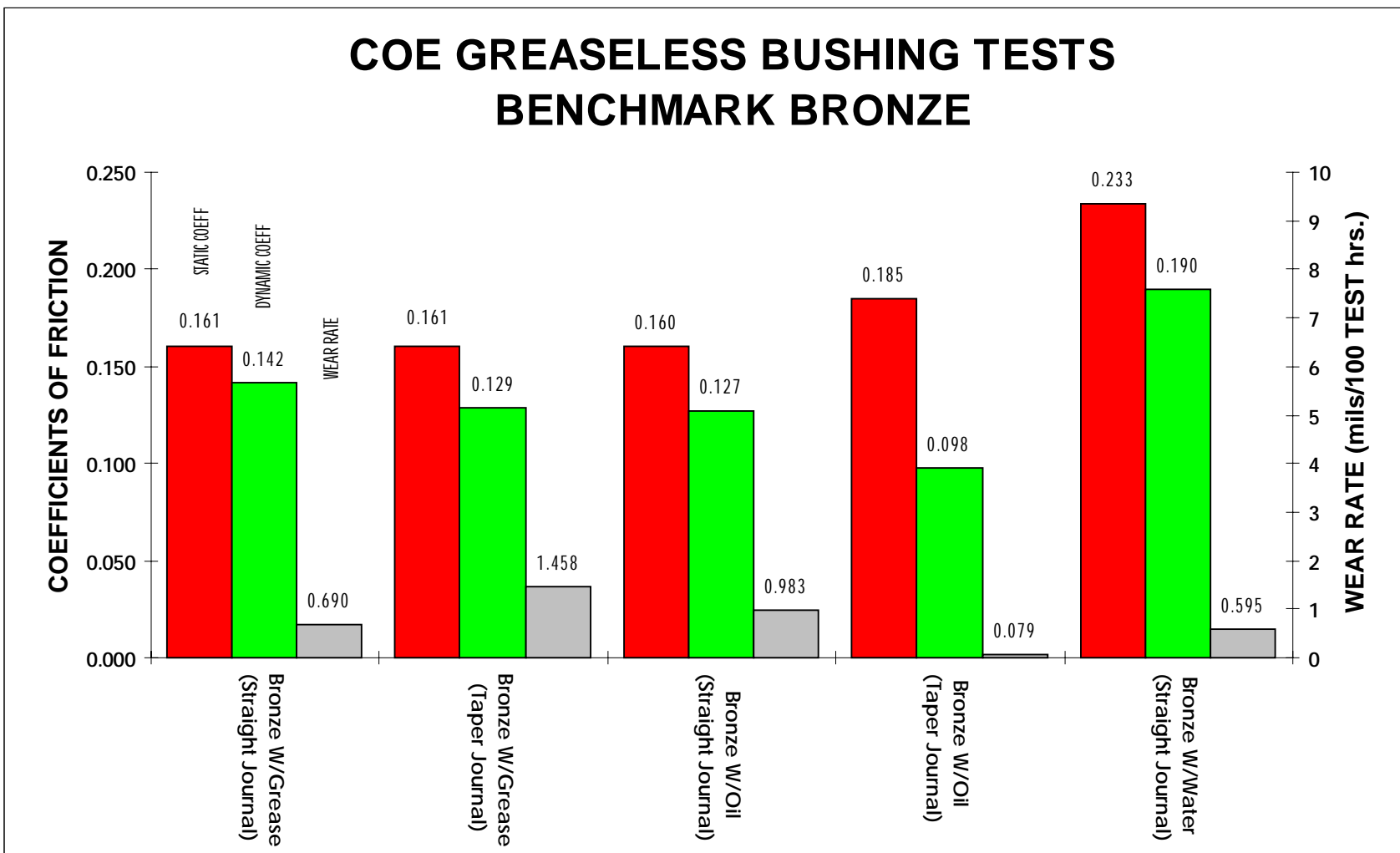
Figure B1. Greaseless bushing tests — benchmark bronze.
