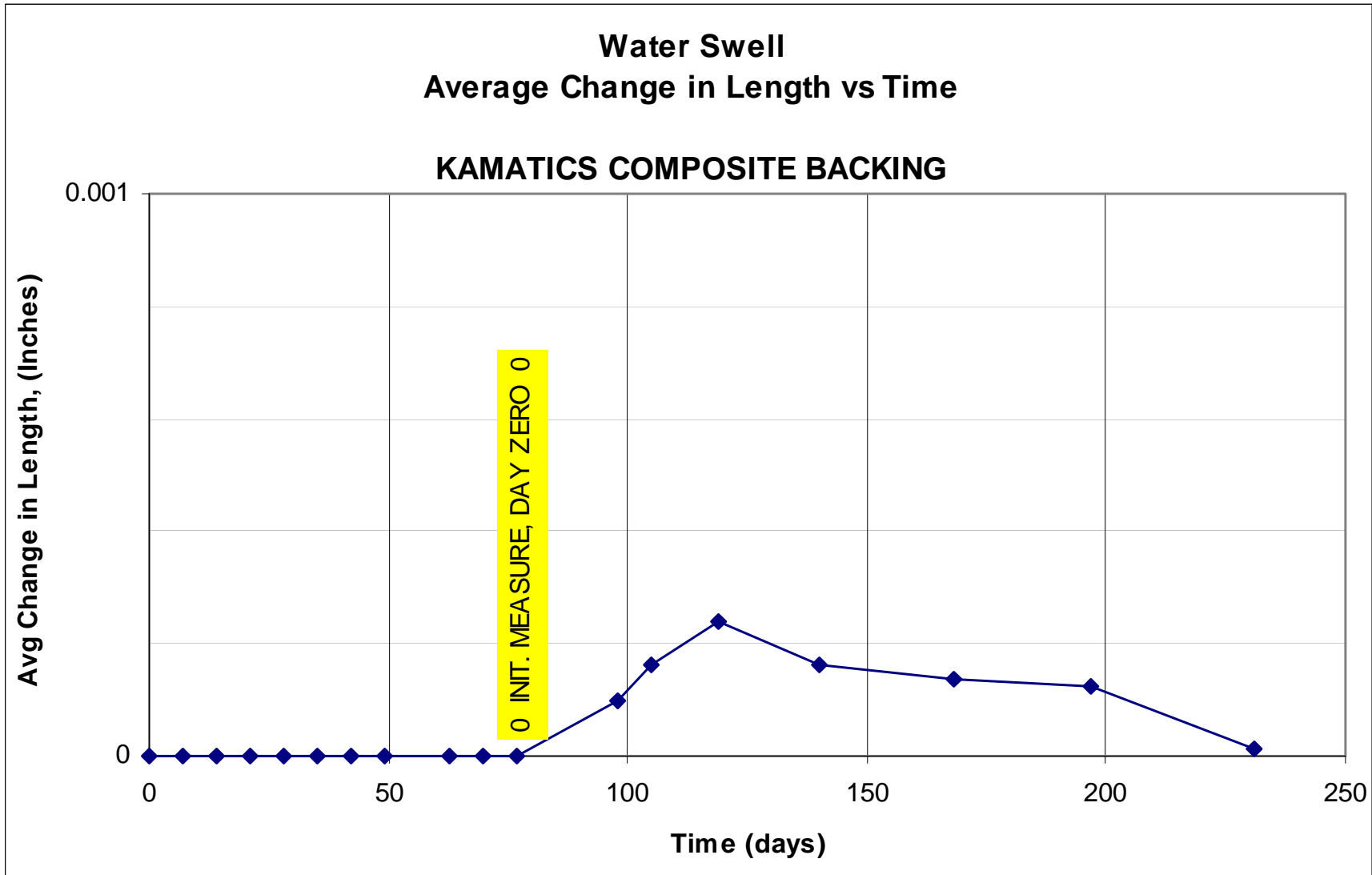
Figure E15. Average change in water swell length vs time using a Kamatics composite backing.
