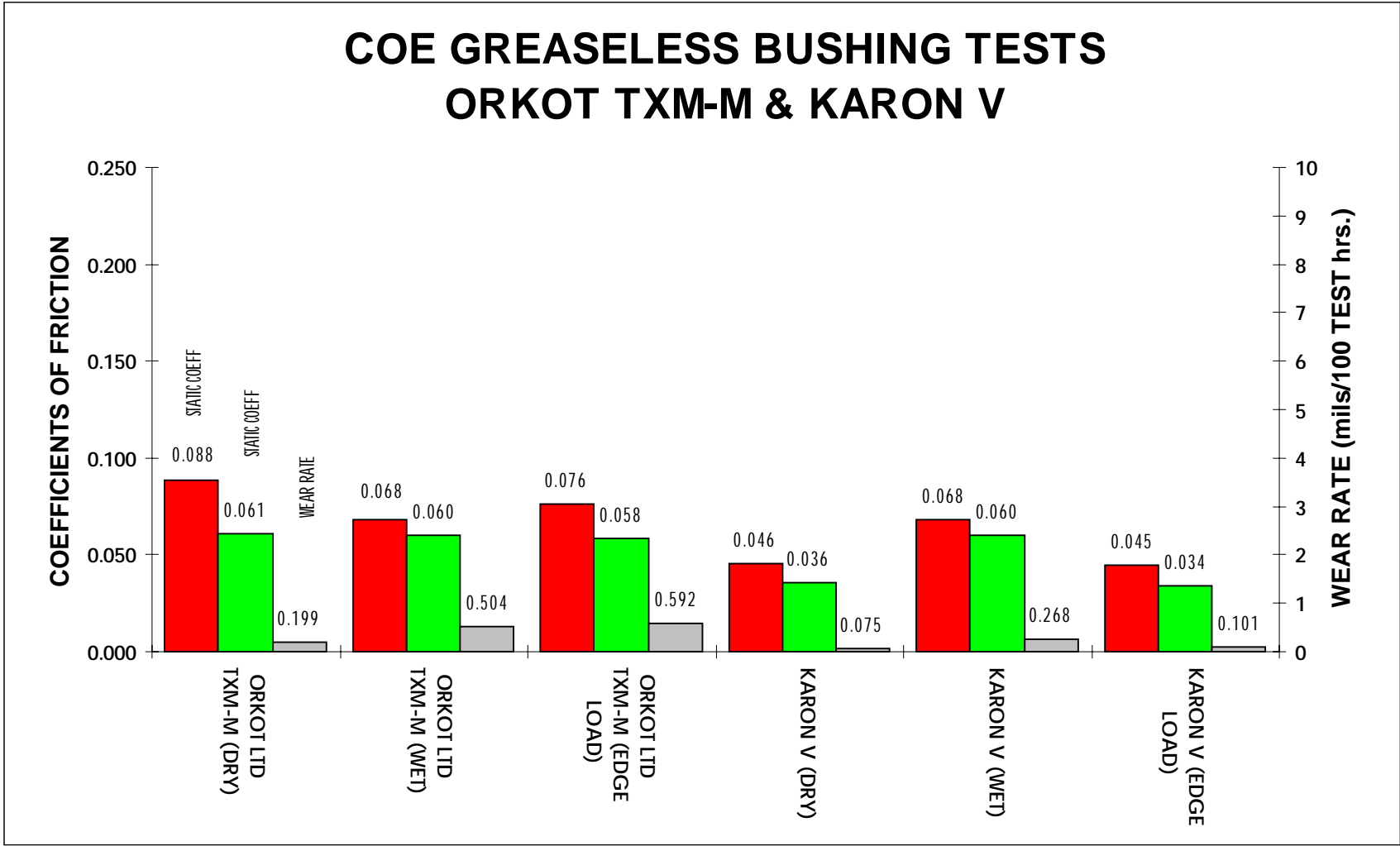
Figure B4. Greaseless bushing tests — Orkot TXM-M and Karon V.
