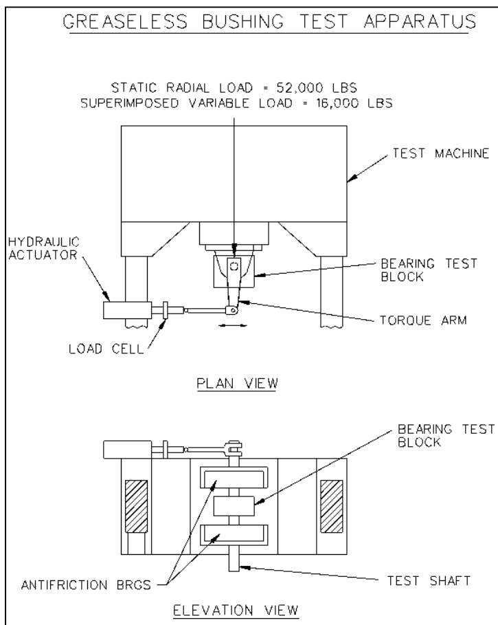
Figure A1. Greaseless bushing test apparatus.
