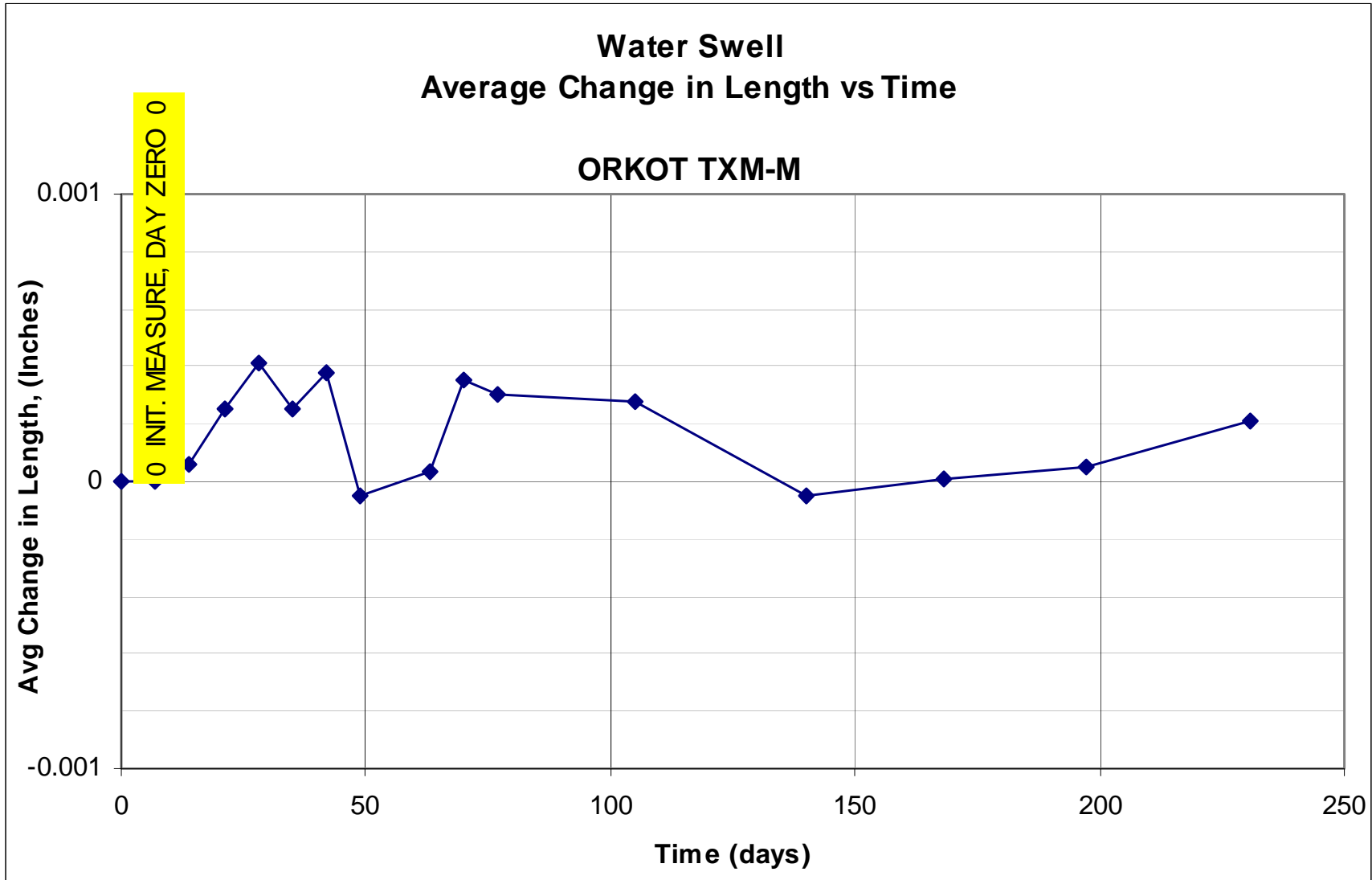
Figure E19. Average change in water swell length vs time using Orkot TXM-M.
