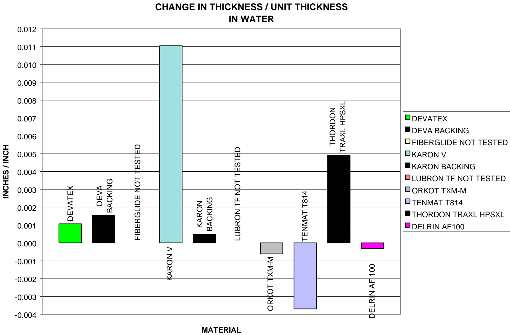
Figure E36. Change in material thickness per unit thickness in water.
