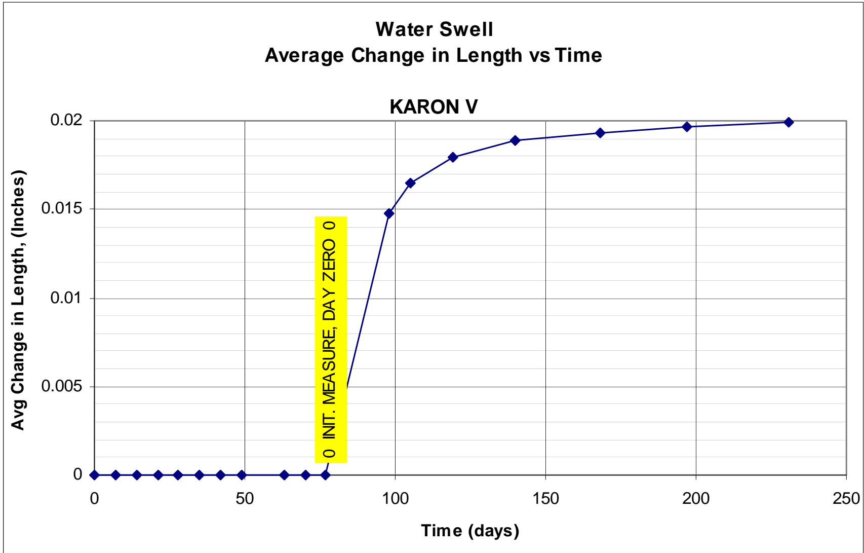
Figure E11. Average change in water swell length vs time using Karon V.
