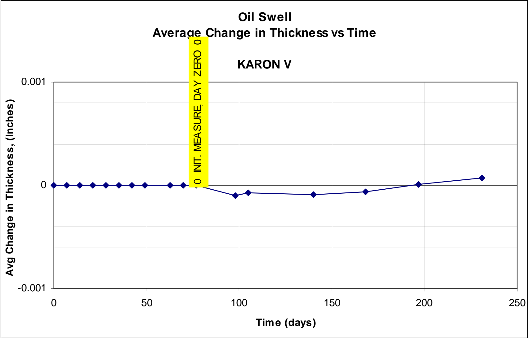
Figure E14. Average change in oil swell thickness vs time using Karon V.
