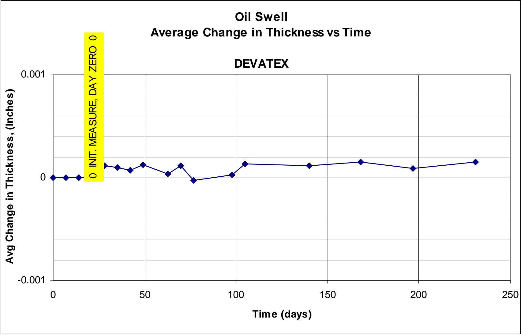
Figure E6. Average change in oil swell thickness vs time using Devatex.
