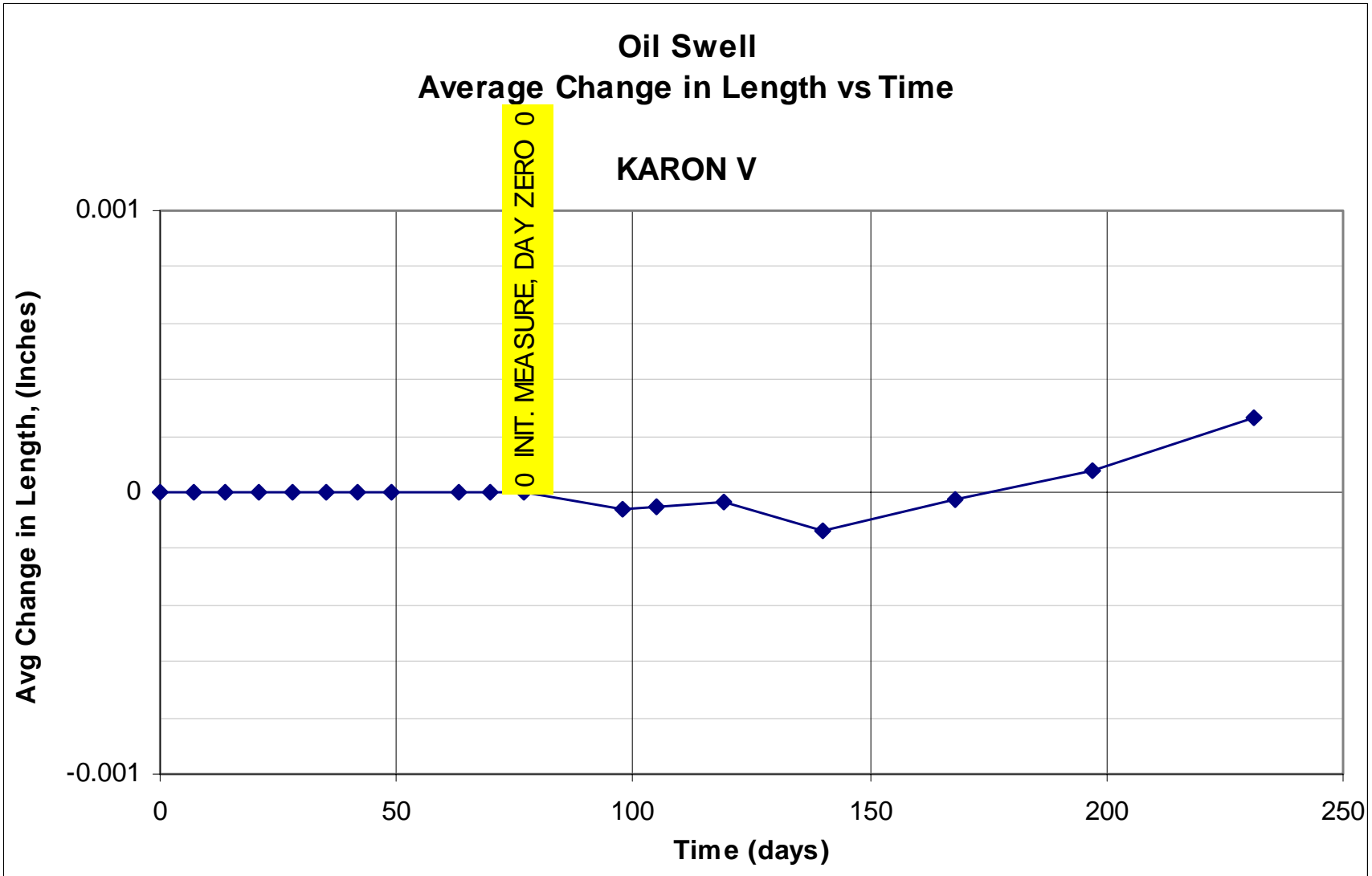
Figure E13. Average change in oil swell length vs time using Karon V.
