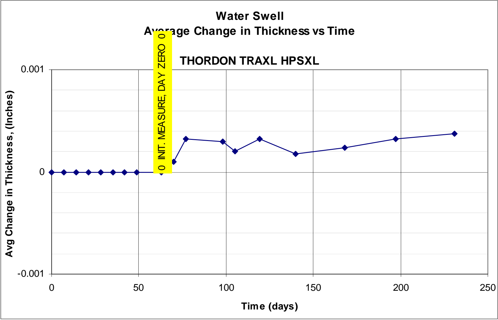
Figure E28. Average change in water swell thickness vs time using Thordon TRAXL HPSXL.
