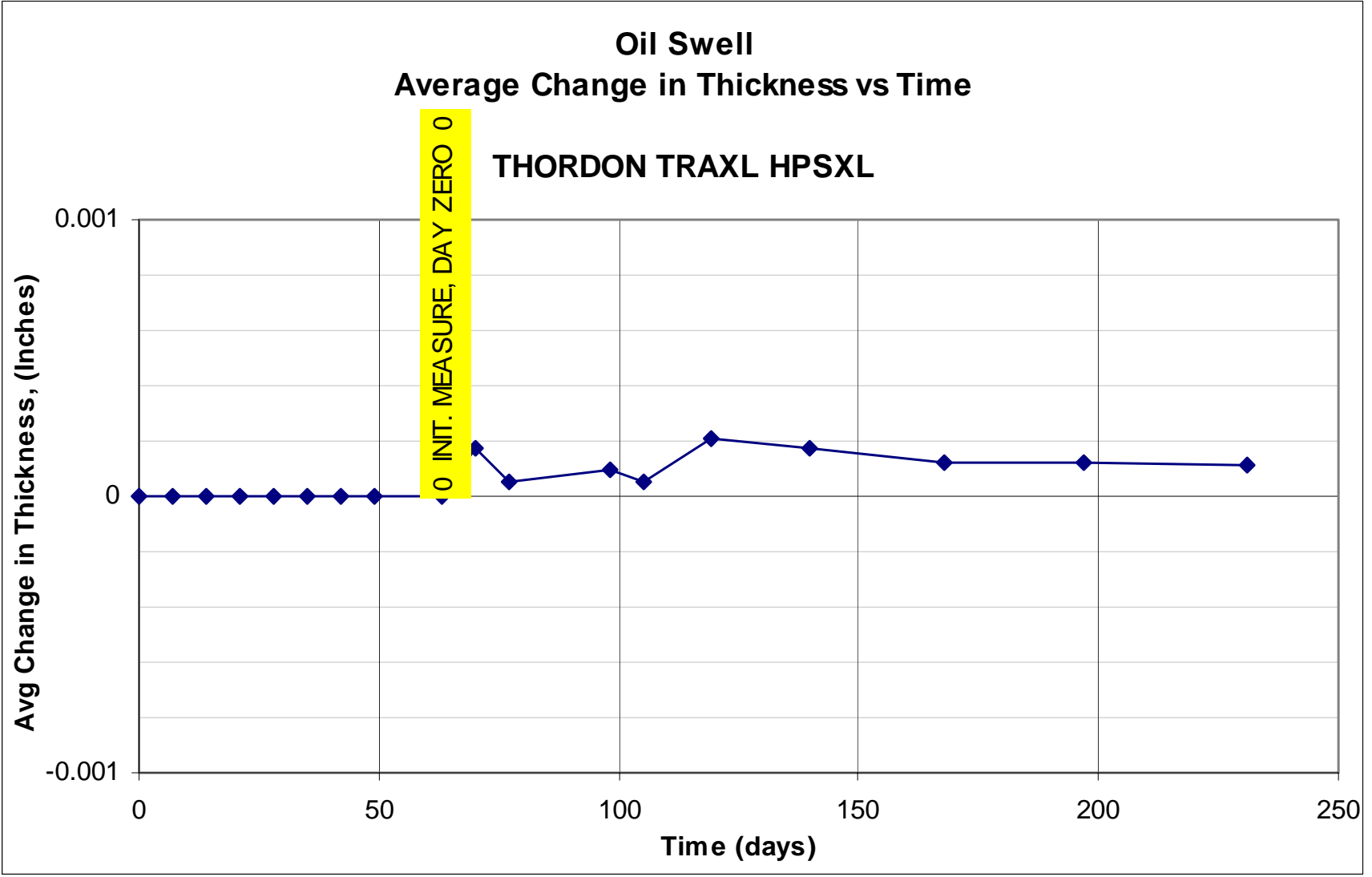
Figure E30. Average change in oil swell thickness vs time using Thordon TRAXL HPSXL.
