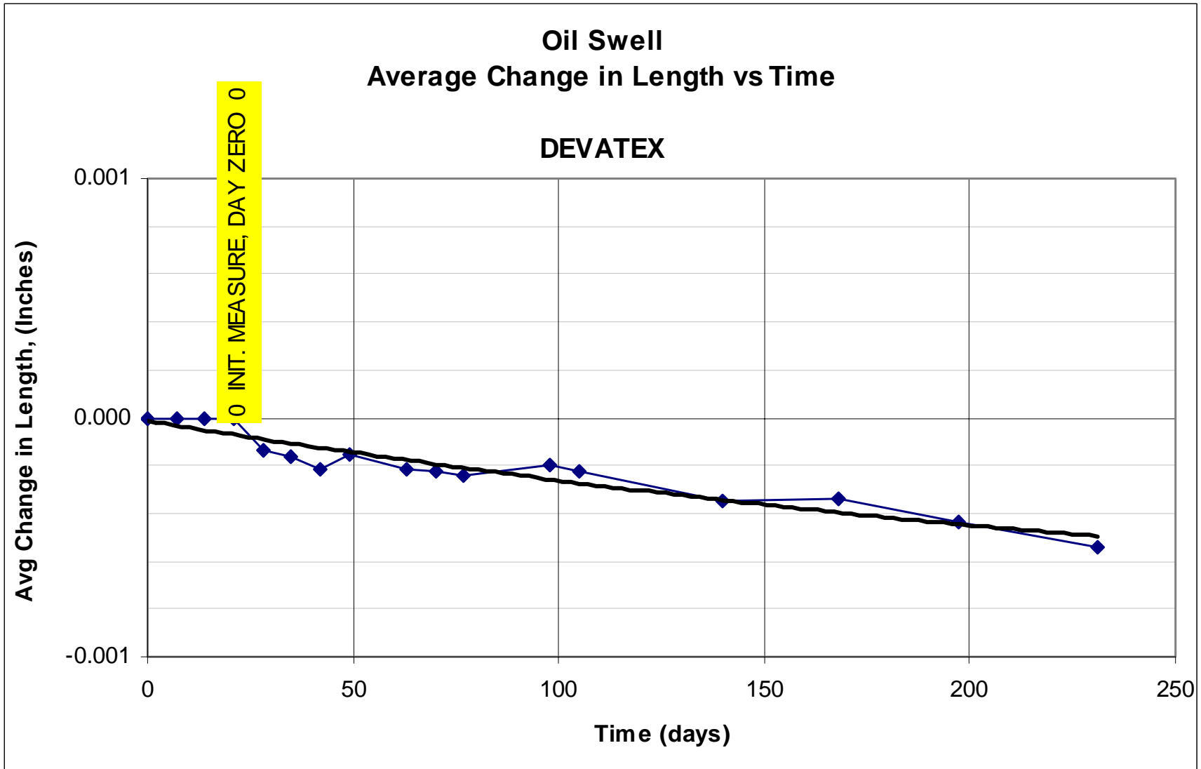
Figure E5. Average change in oil swell length vs time using Devatex.
