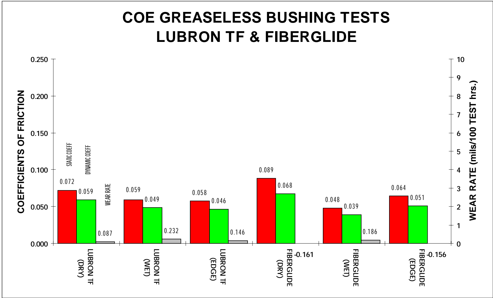
Figure B3. Greaseless bushing tests — Lubron TF and Fiberglide.
