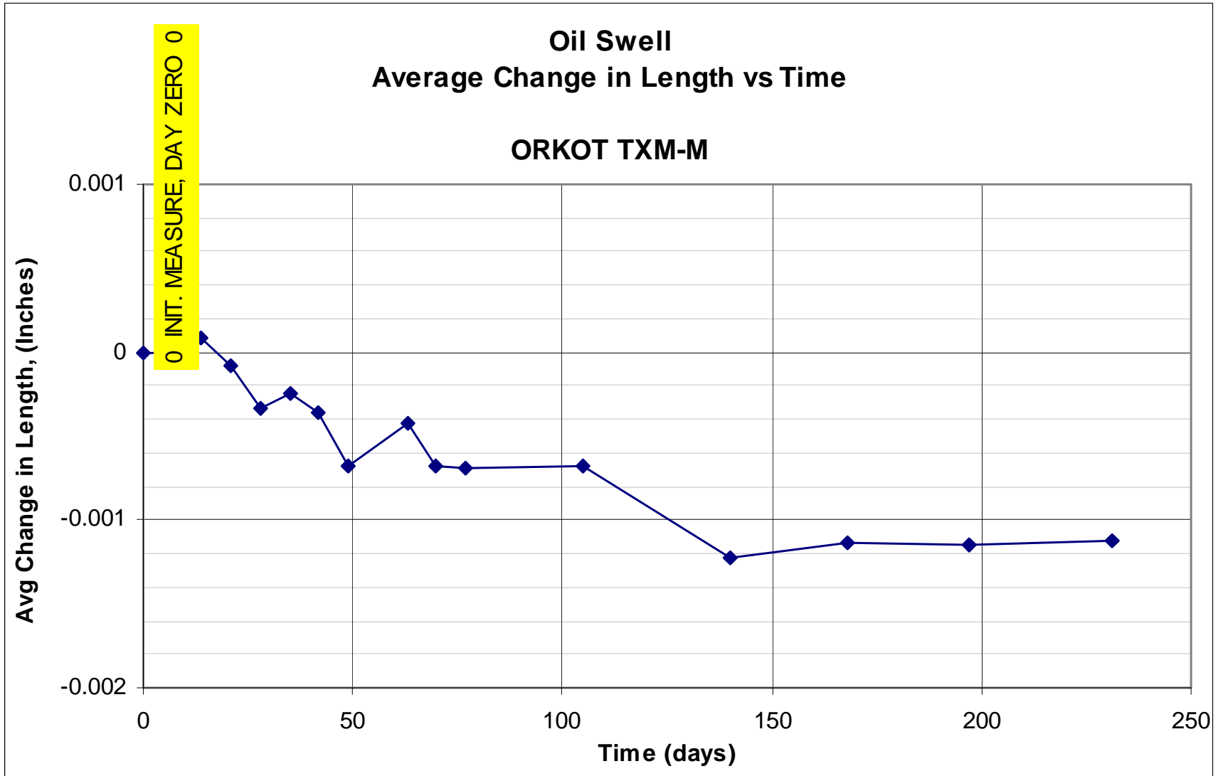
Figure E21. Average change in oil swell length vs time using Orkot TXM-M.
