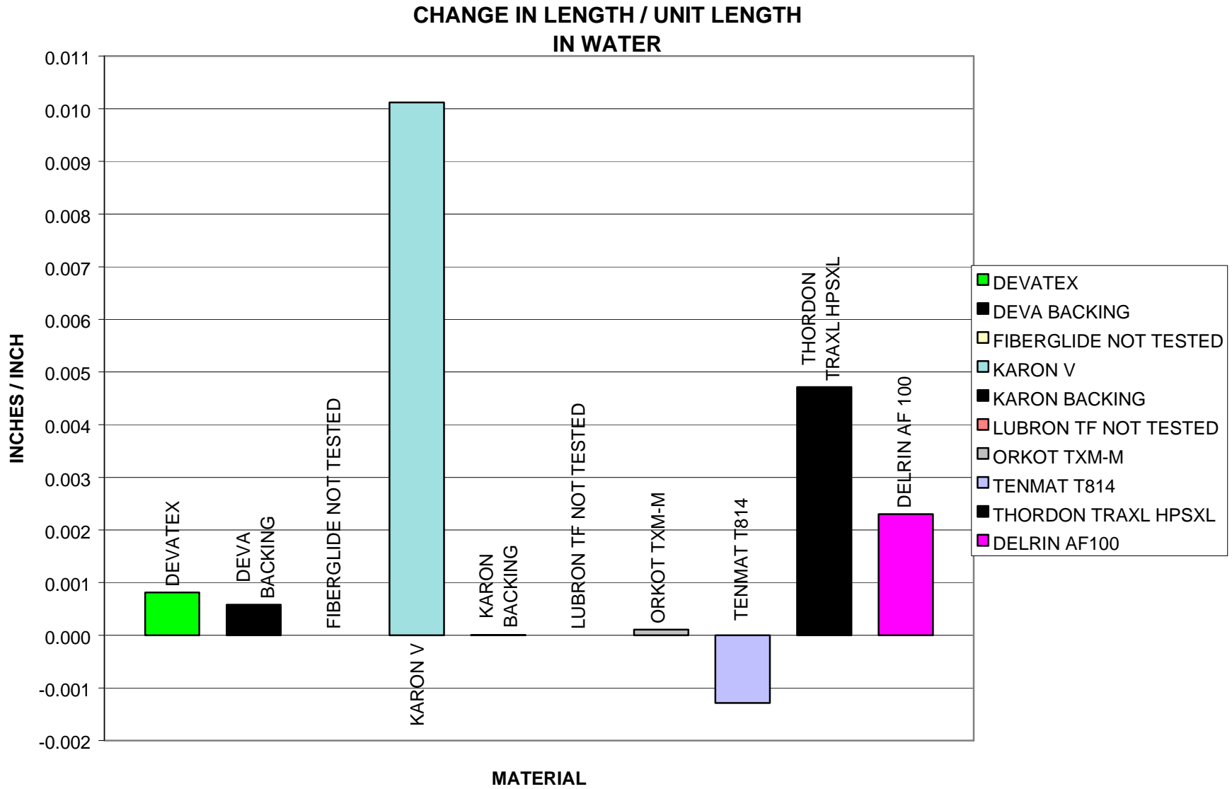
Figure E35. Change in material length per unit length in water.
