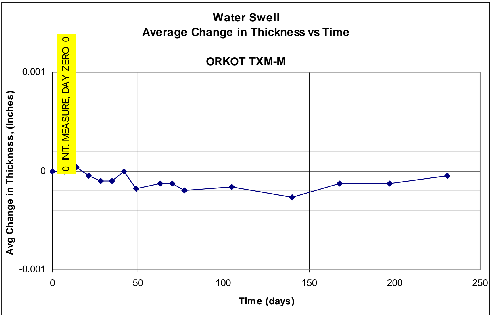
Figure E20. Average change in water swell thickness vs time using Orkot TXM-M.
