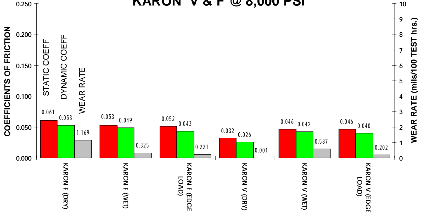
Figure B5. Greaseless bushing tests — Karon V and F@8,000 psi.
