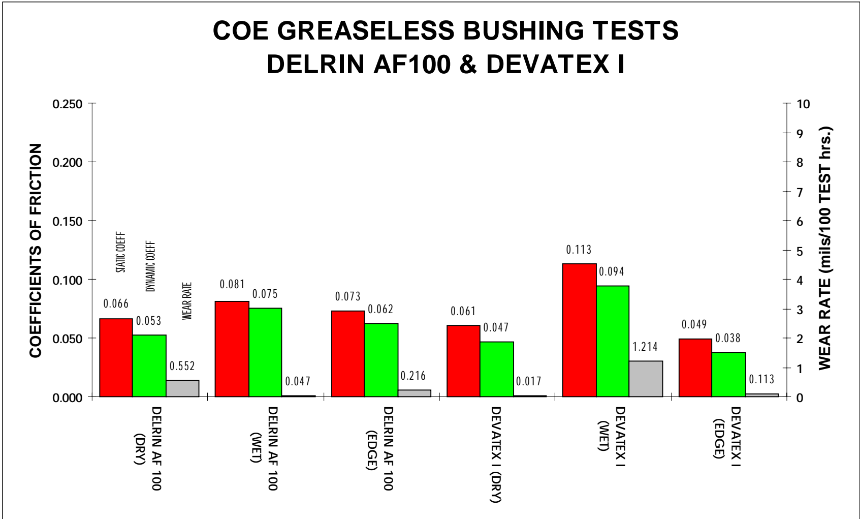
Figure B2. Greaseless bushing tests — Delrin AF100 and Devatex I.
