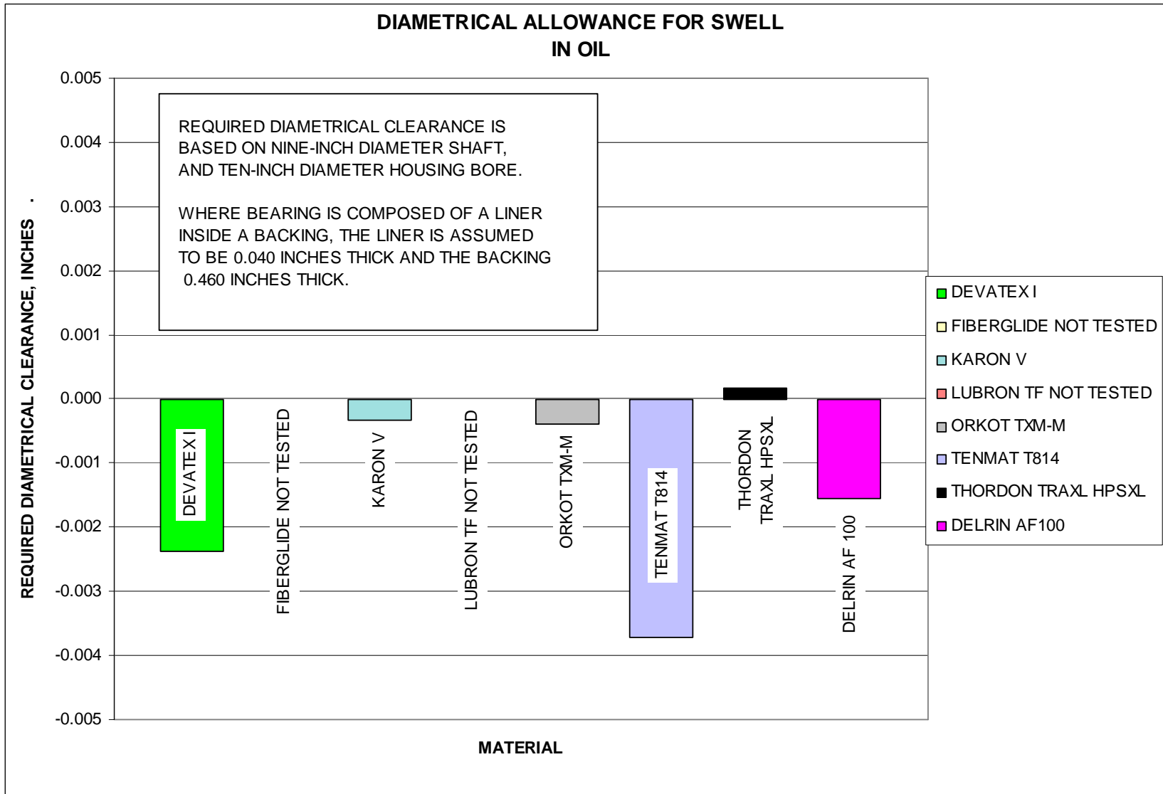
Figure E2. Diametrical allowance for swell in oil.
