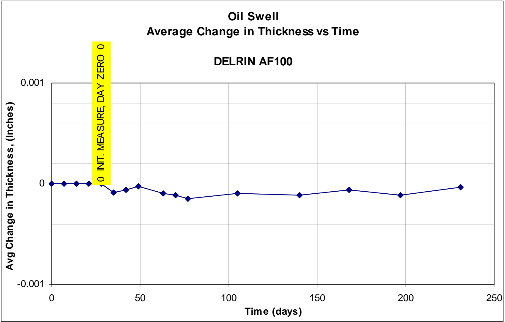
Figure E34. Average change in oil swell thickness vs time using Delrin AF100.
