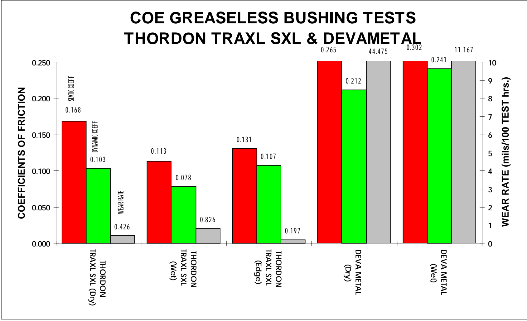
Figure B8. Greaseless bushing tests — Thordon TRAXL SXL and Deva Metal.
