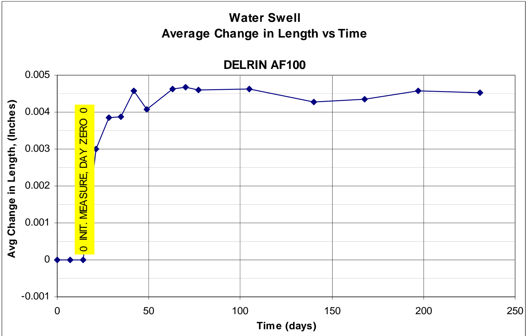
Figure E31. Average change in water swell length vs time using Delrin AF100.
