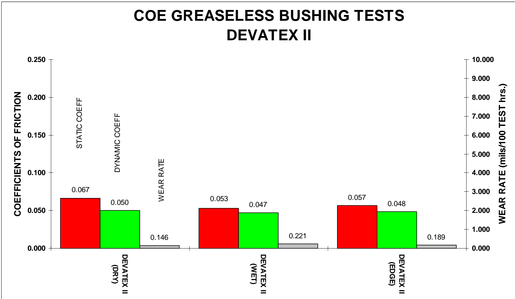
Figure B9. Greaseless bushing tests — Devatex II.
