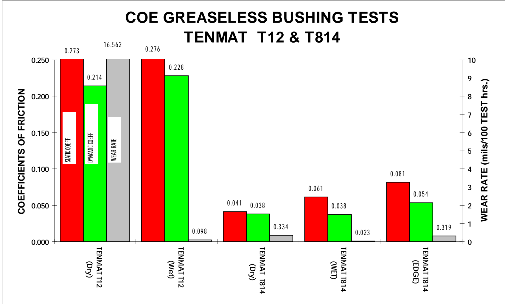
Figure B6. Greaseless bushing tests — Tenmat T12 and T814.
