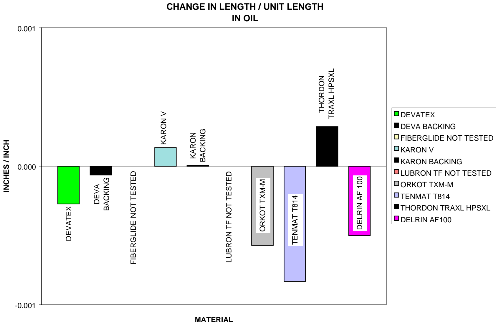
Figure E37. Change in material length per unit length in oil.
