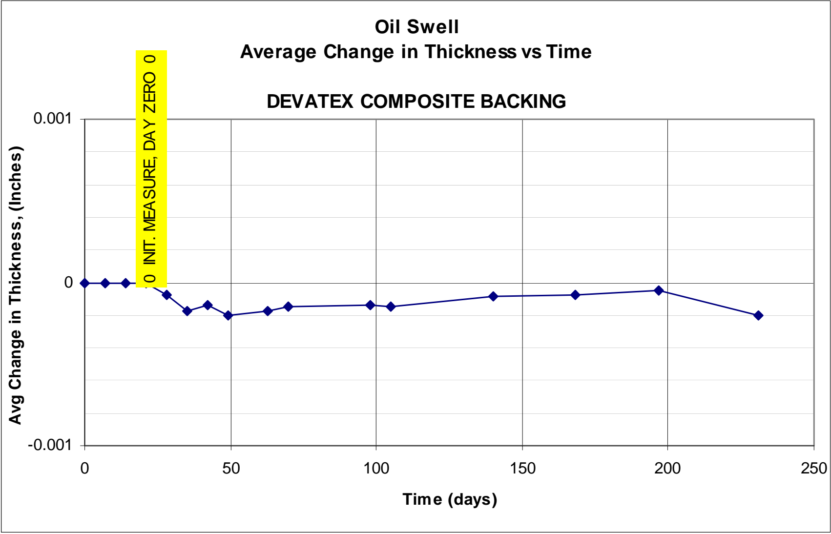
Figure E10. Average change in oil swell thickness vs time using a Devatex composite backing.
