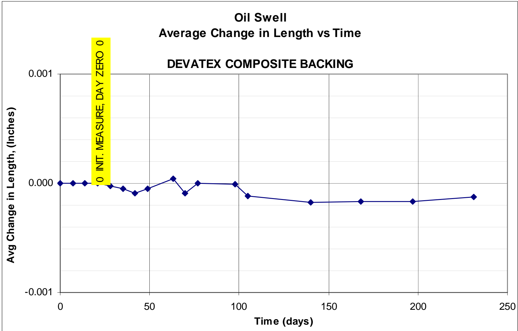
Figure E9. Average change in oil swell length vs time using a Devatex composite backing.
