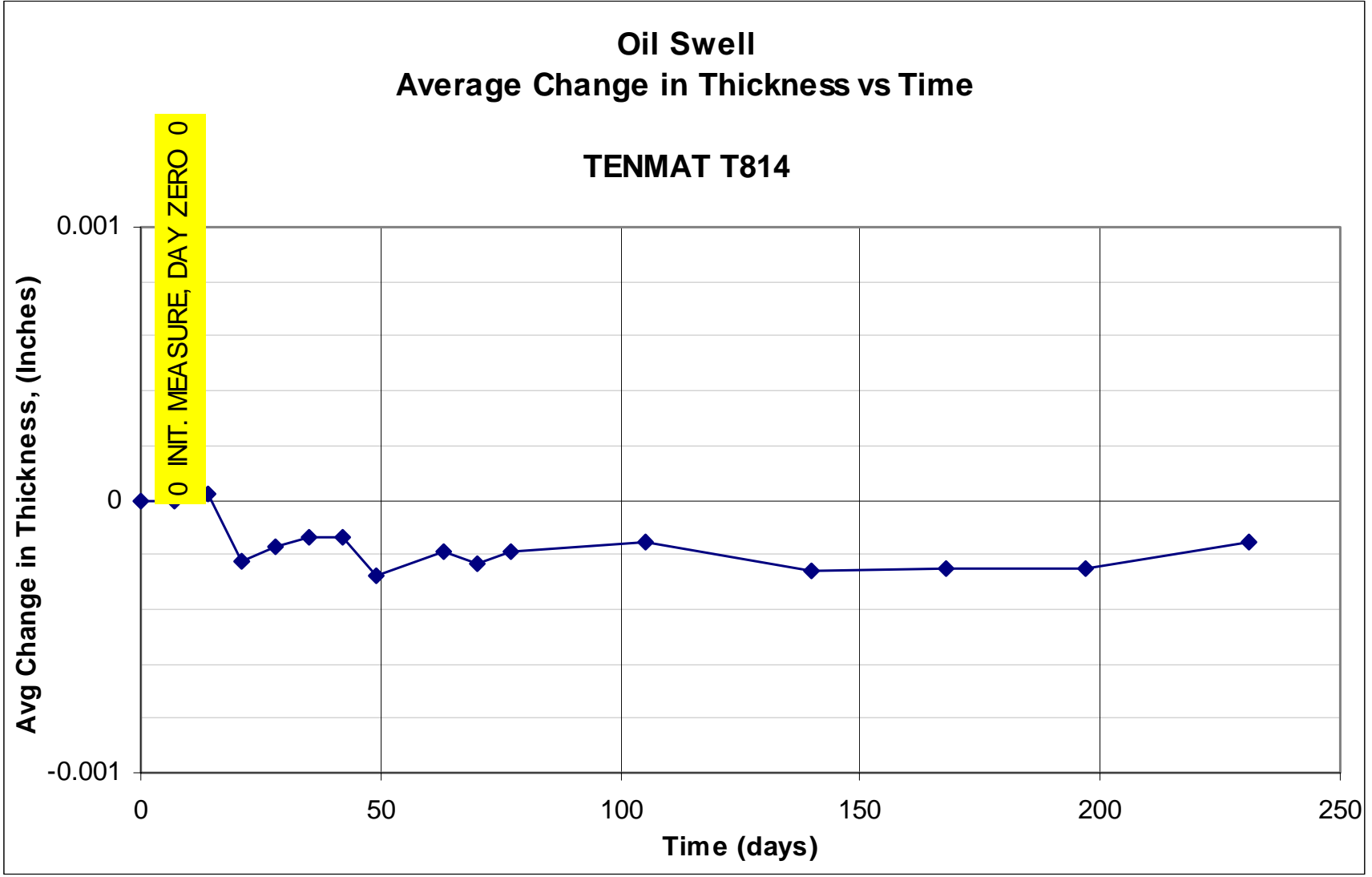
Figure E26. Average change in oil swell thickness vs time using Tenmat T814.
