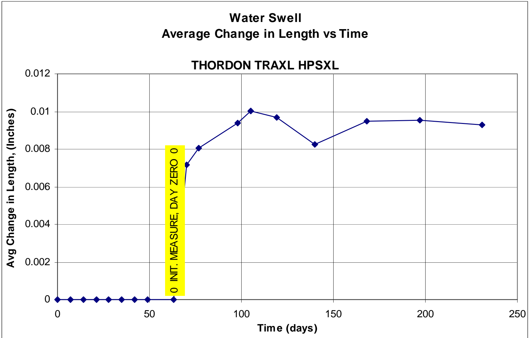
Figure E27. Average change in water swell length vs time using Thordon TRAXL HPSXL.
