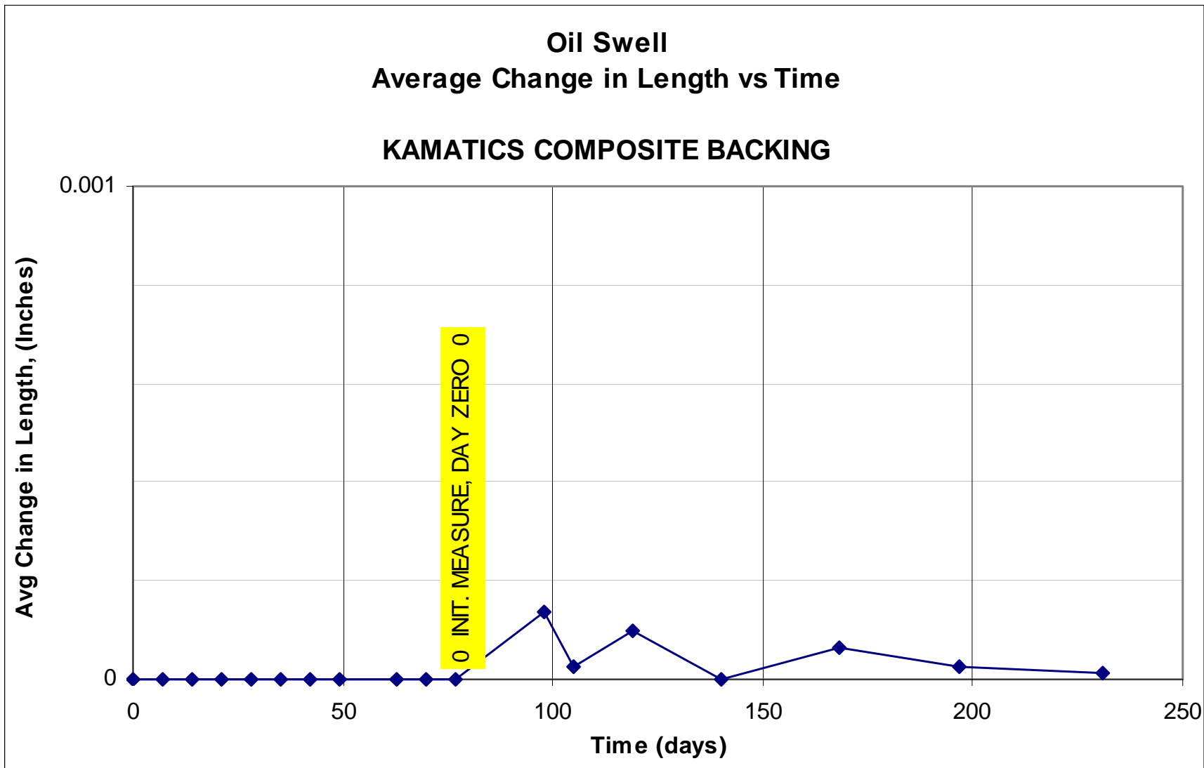
Figure E17. Average change in oil swell length vs time using a Kamatics composite backing.
