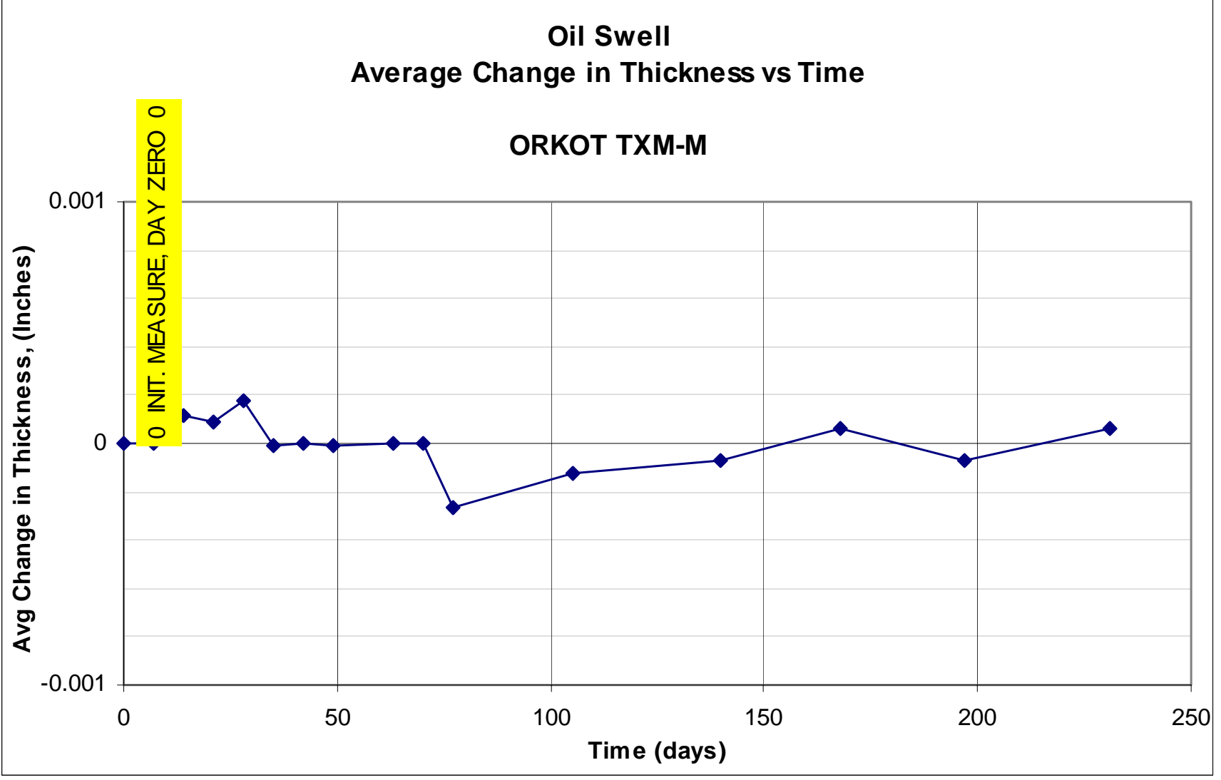
Figure E22. Average change in oil swell thickness vs time using OrkotTXM-M.
