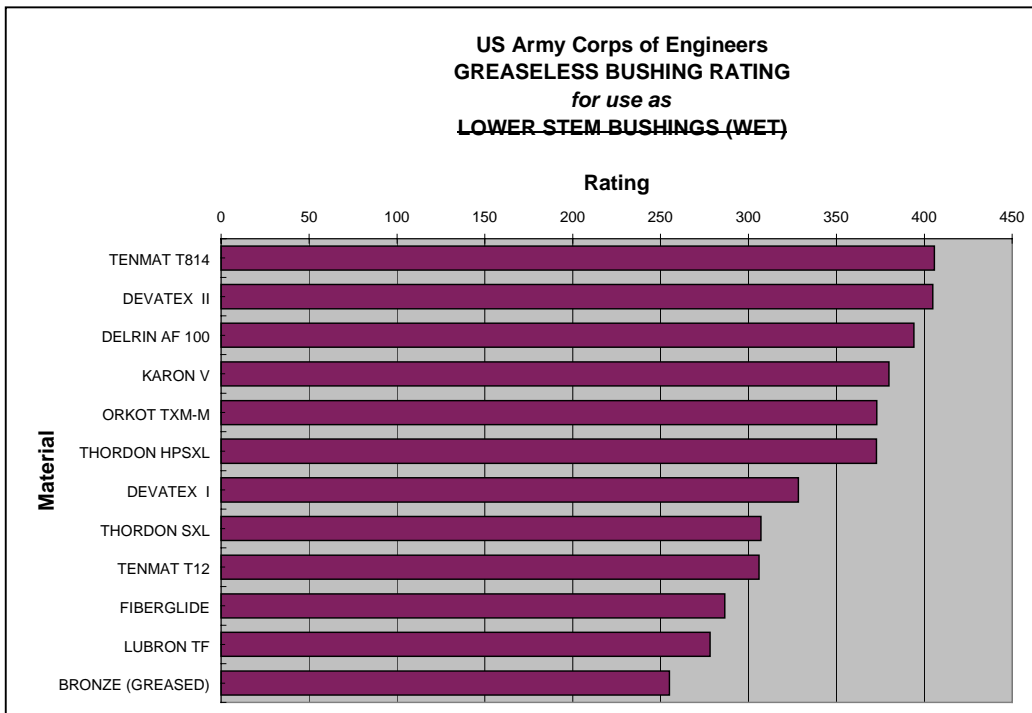
Figure G4. Greaseless bushing rating for use as lower stem bushings (wet).
