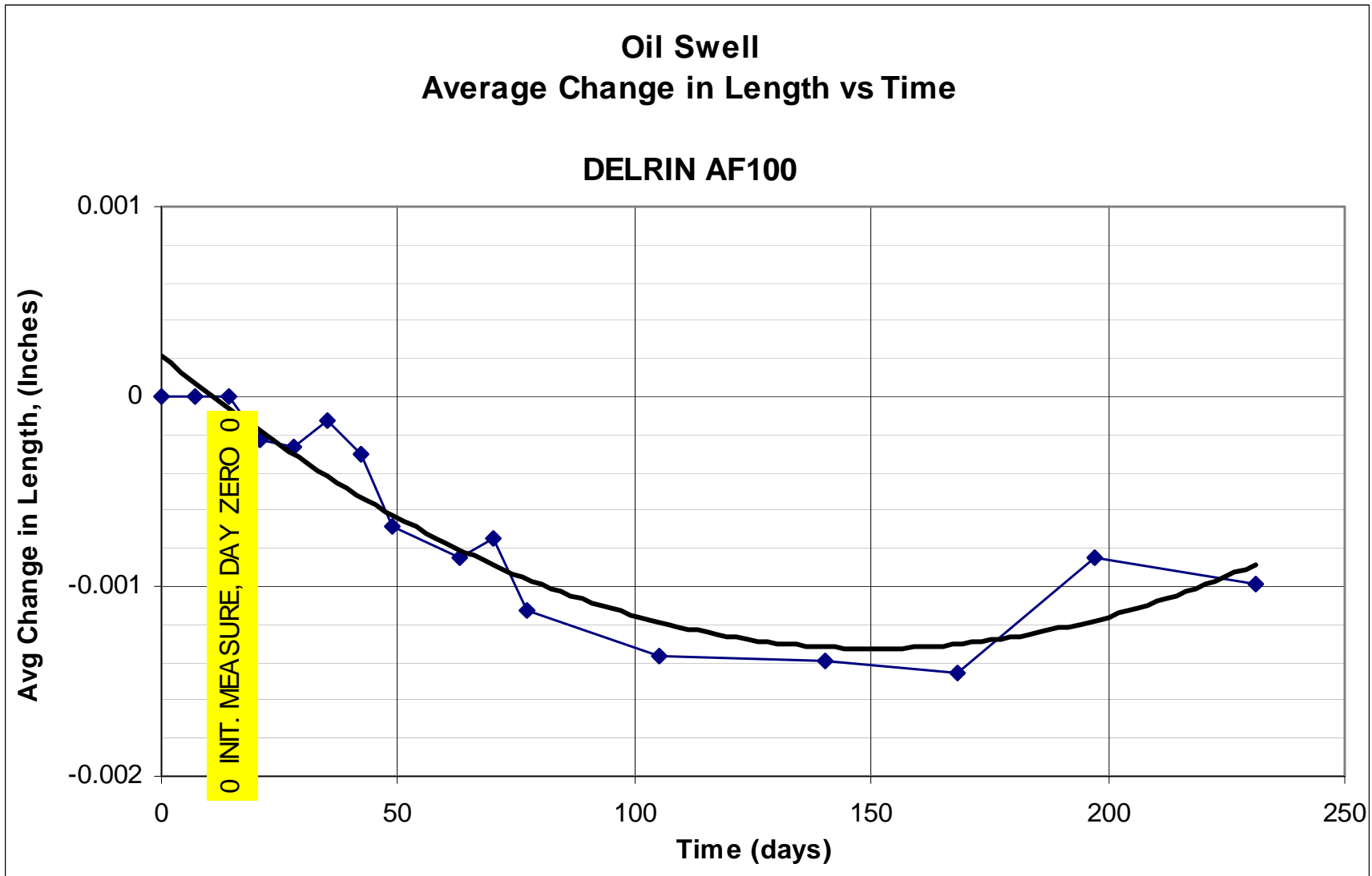
Figure E33. Average change in oil swell length vs time using Delrin AF100.
