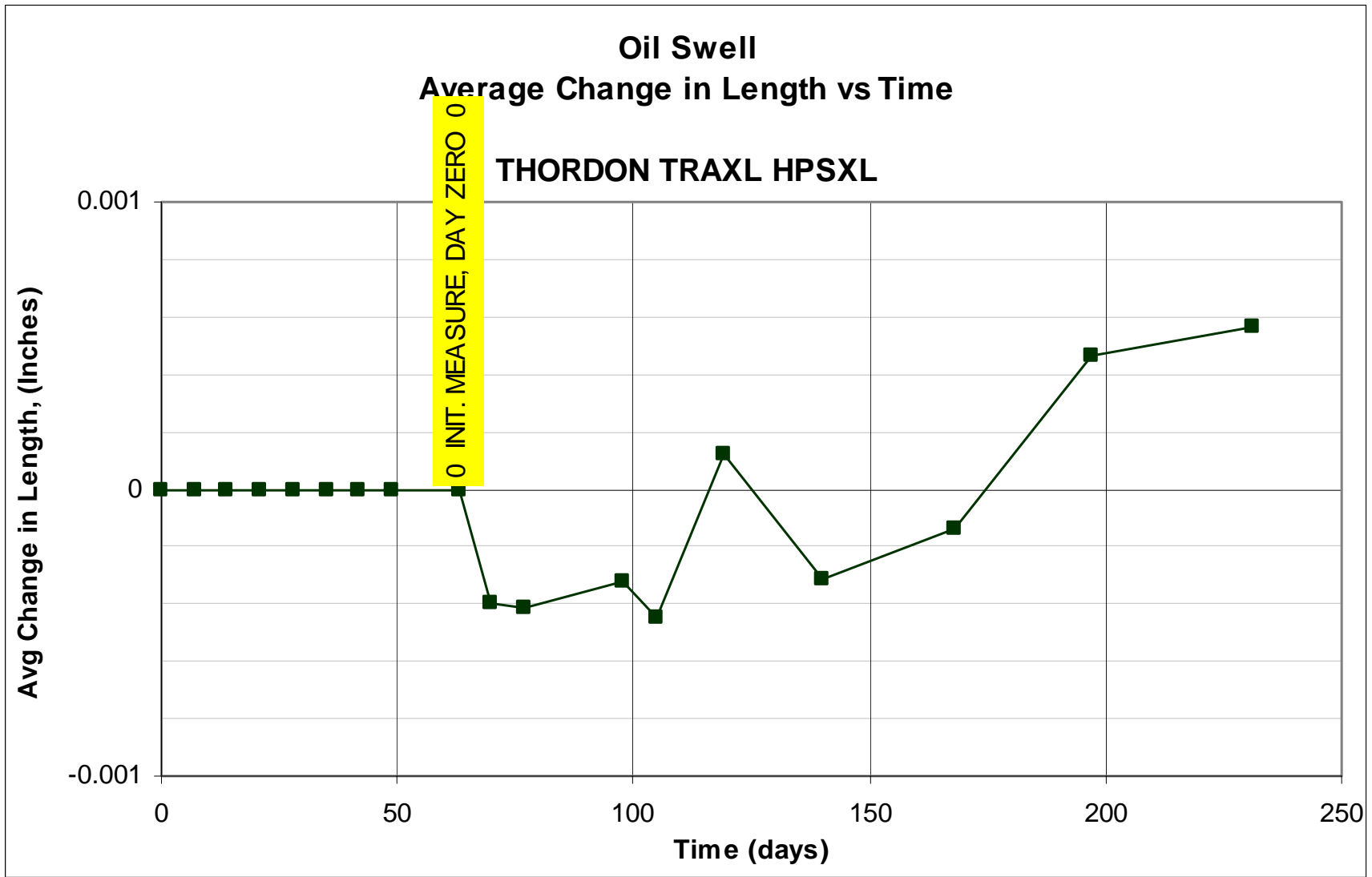
Figure E29. Average change in oil swell length vs time using Thordon TRAXL HPSXL.
