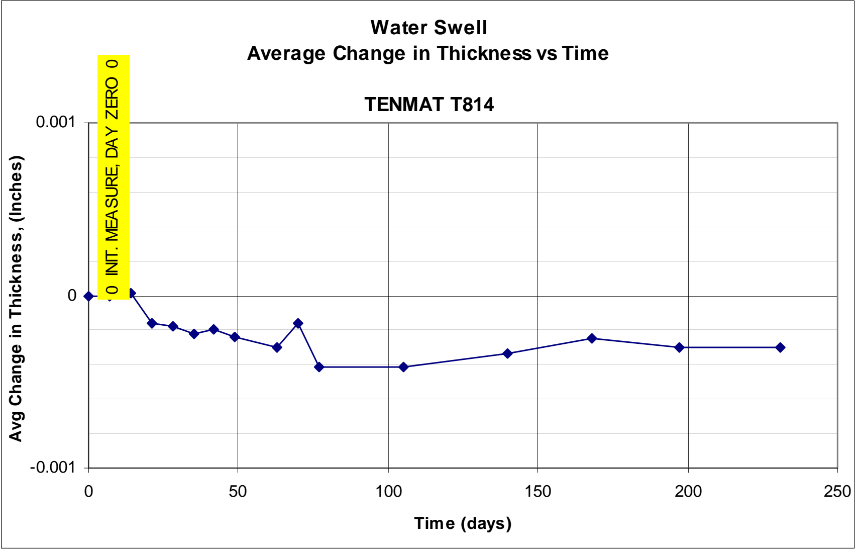
Figure E24. Average change in water swell thickness vs time using Tenmat T814.
