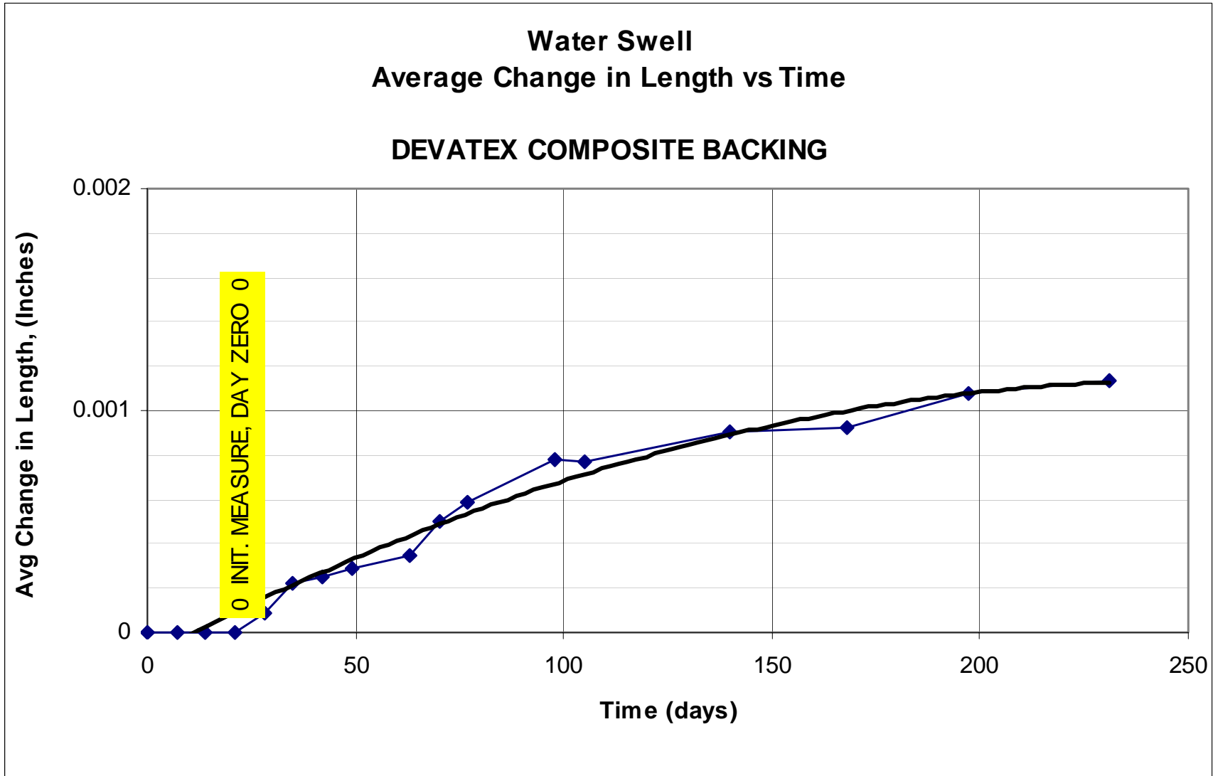
Figure E7. Average change in water swell length vs time using a Devatex composite backing.
