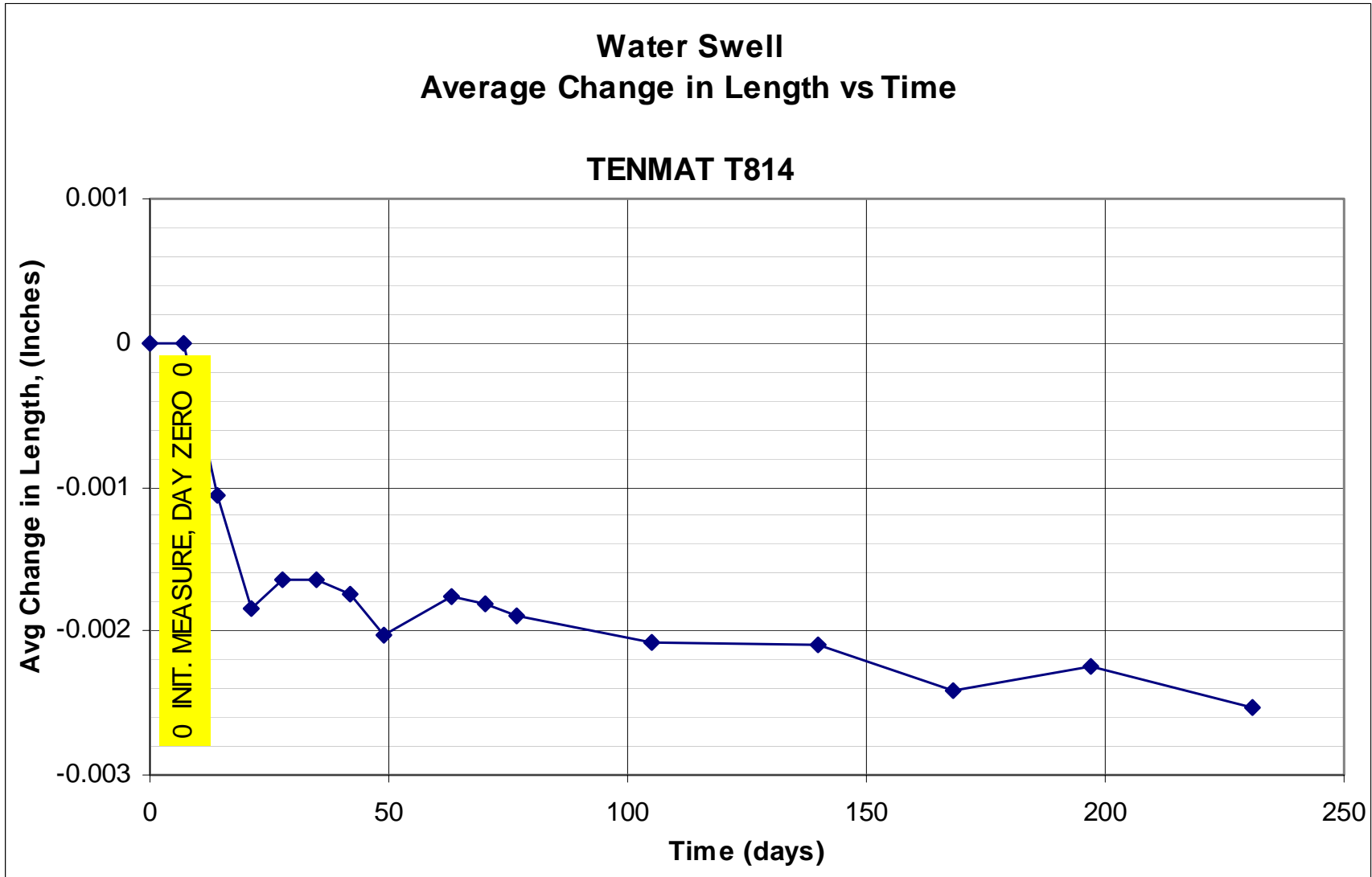
Figure E23. Average change in water swell length vs time using Tenmat T814.
