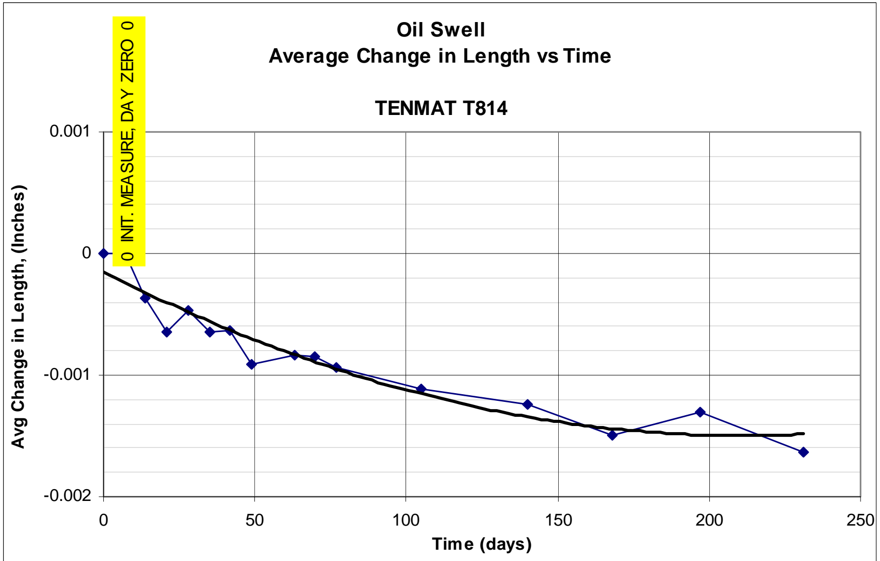
Figure E25. Average change in oil swell length vs time using Tenmat T814.
