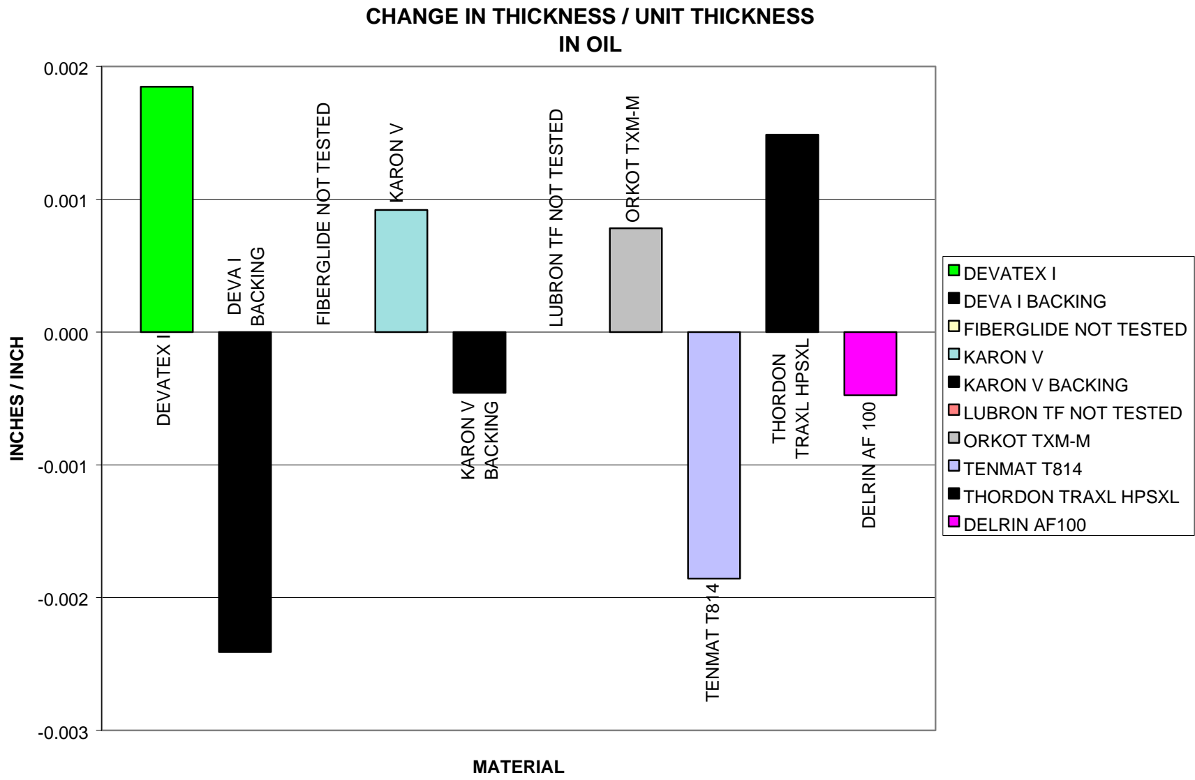
Figure E38. Change in material thickness per unit thickness in oil.
