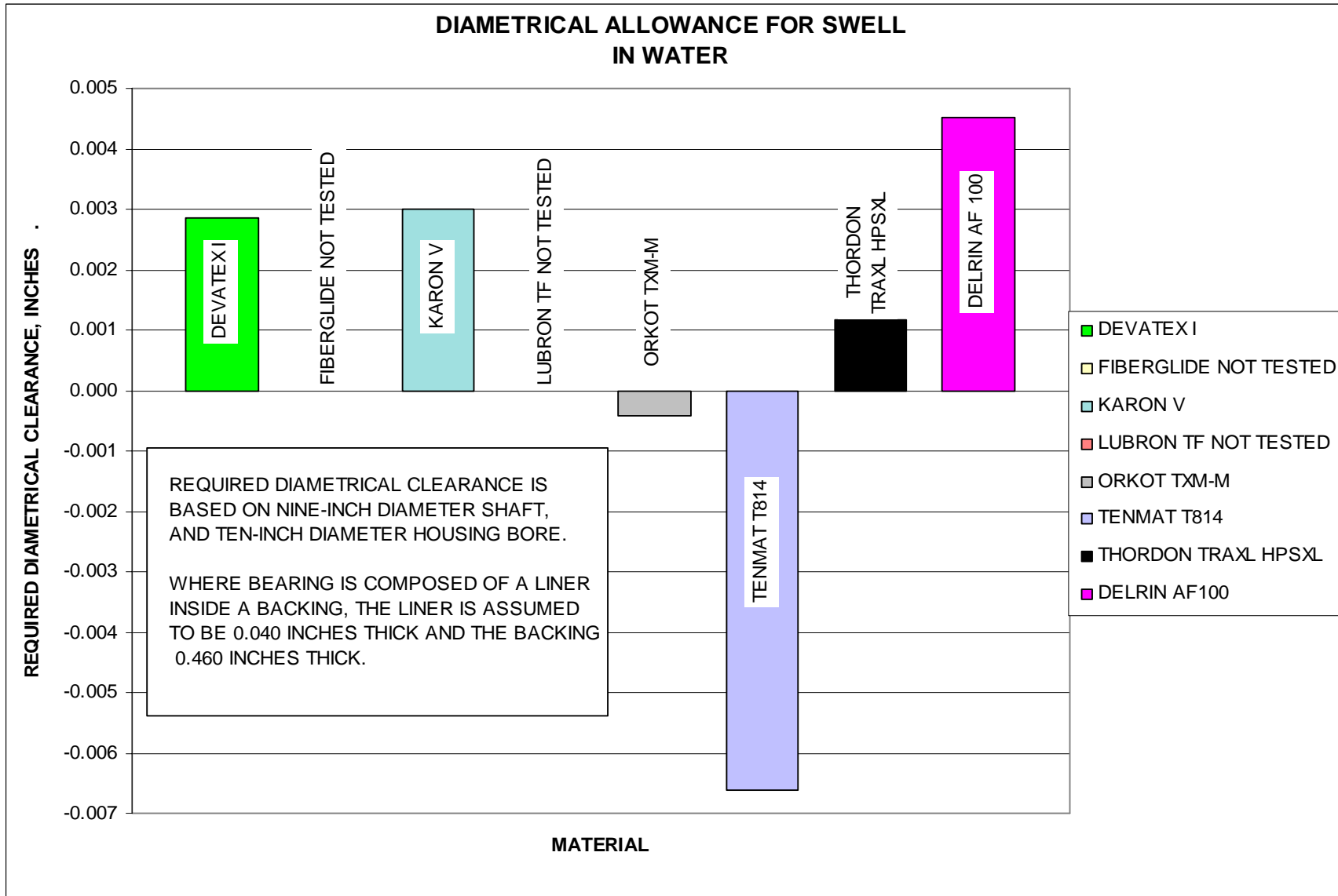
Figure E1. Diametrical allowance for swell in water.
