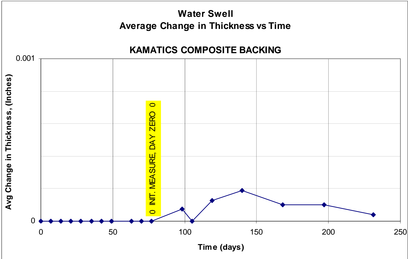
Figure E16. Average change in water swell thickness vs time using a Kamatics composite backing.
