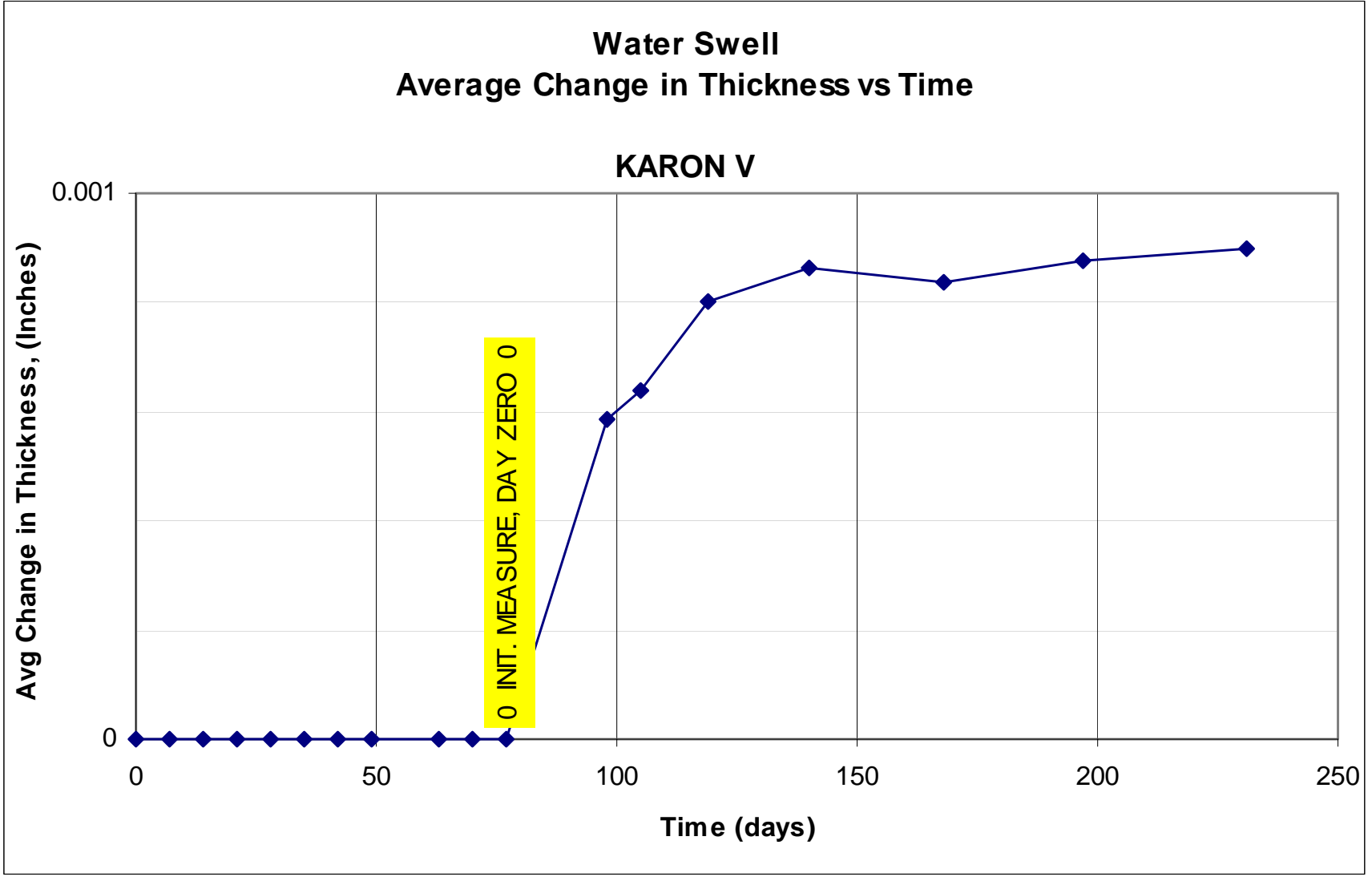
Figure E12. Average change in water swell thickness vs time using Karon V.
