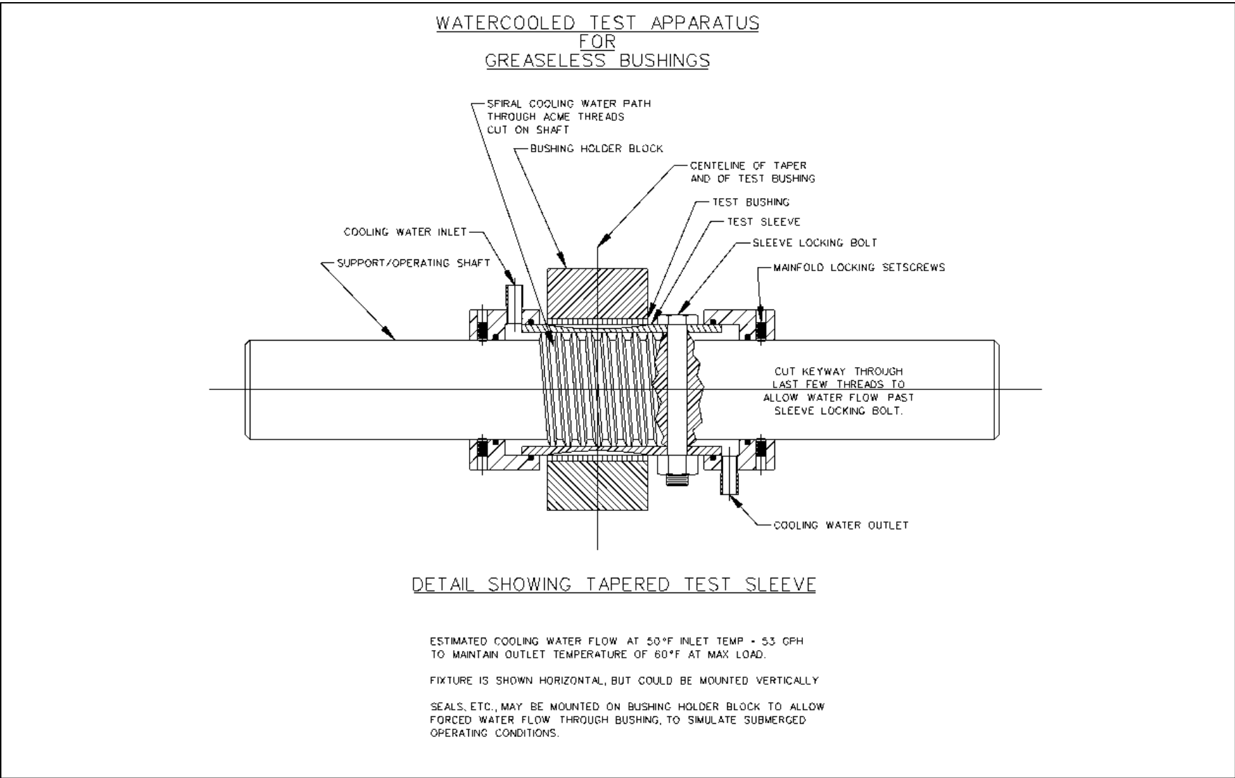
Figure A2. Apparatus detail showing water-cooled test sleeve.
