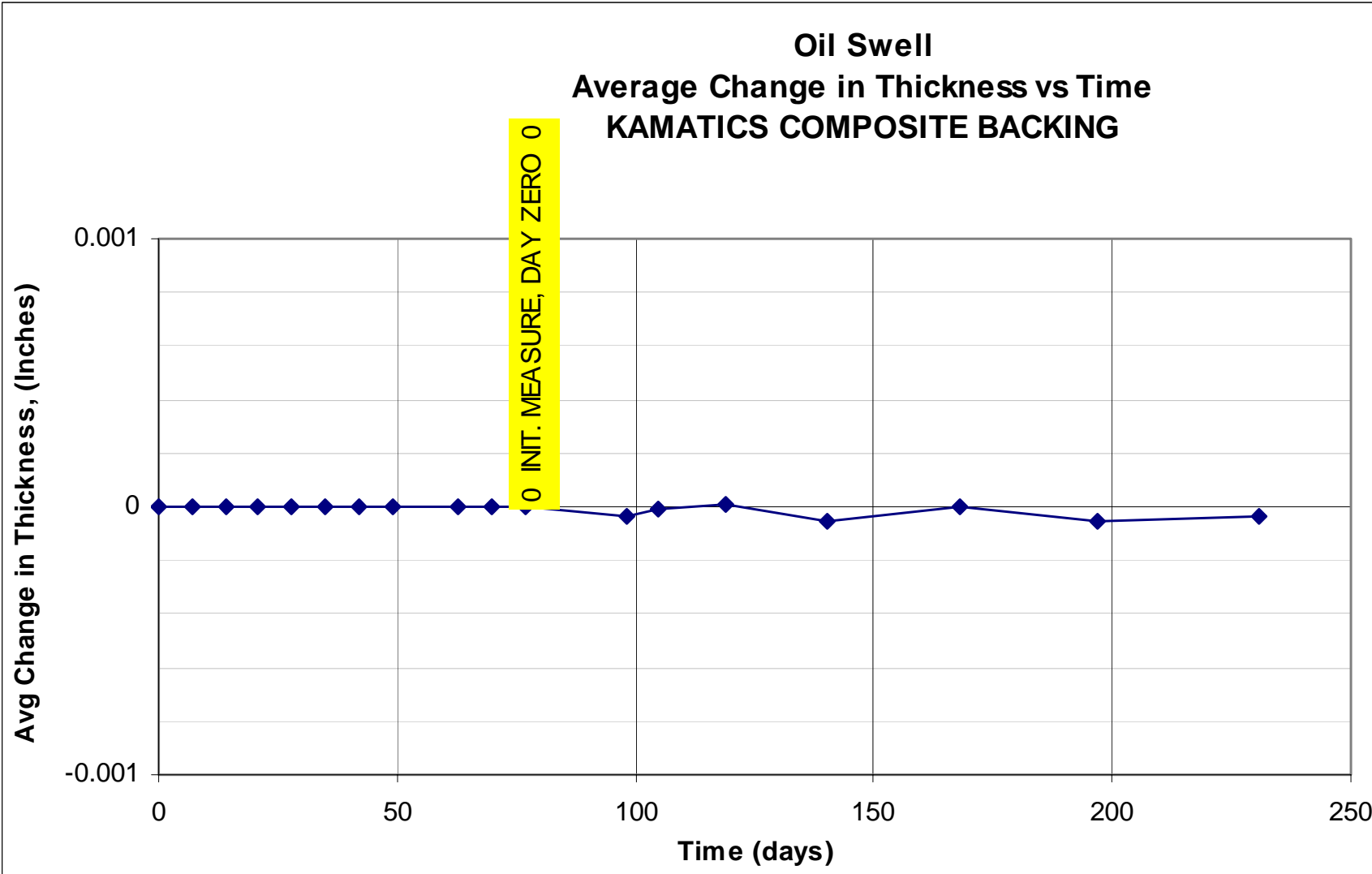
Figure E18. Average change in oil swell thickness vs time using a Kamatics composite backing.
