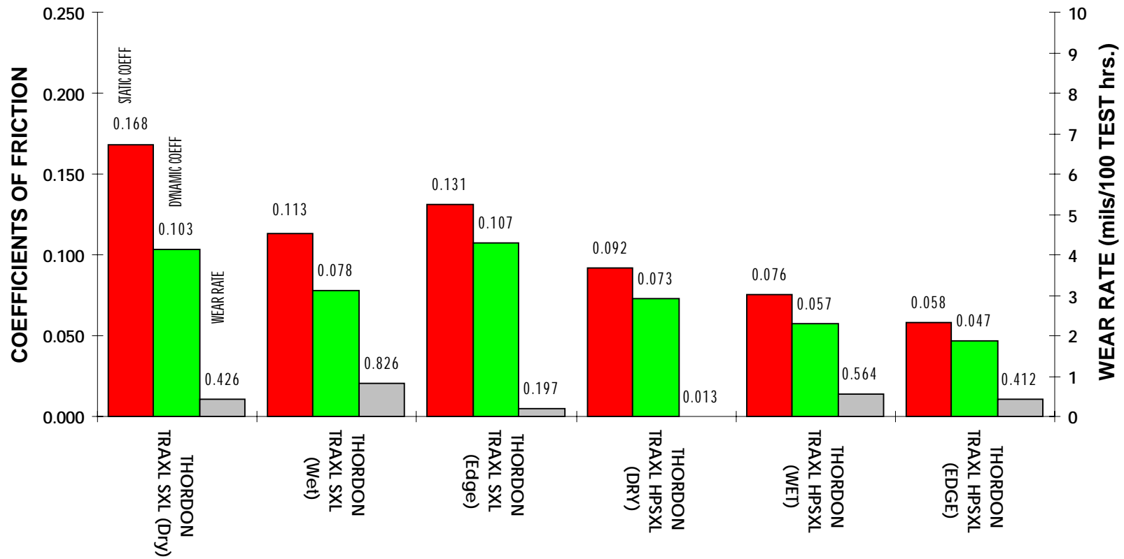
Figure B7. Greaseless bushing tests — Thordon TRAXL SXL and HPSXL.
