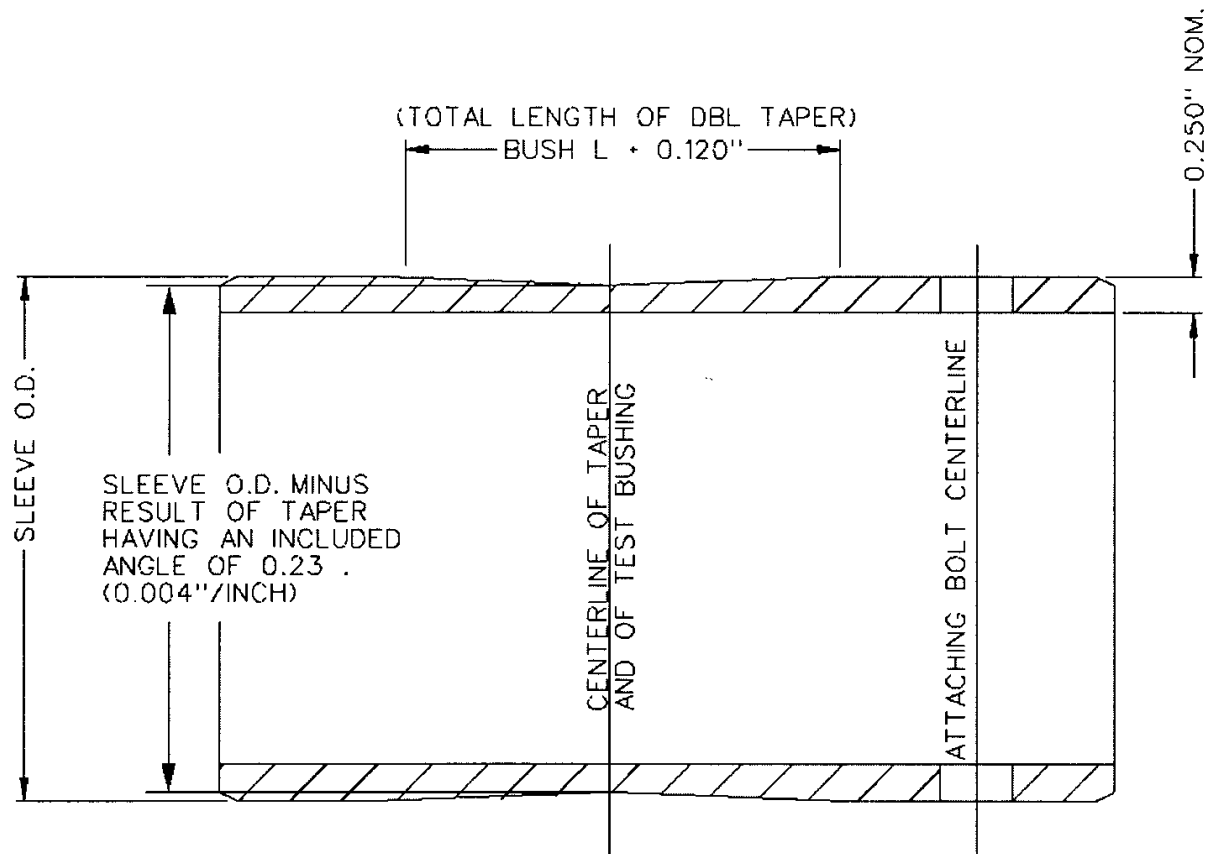
Figure A3. Detail showing tapered test sleeve.
