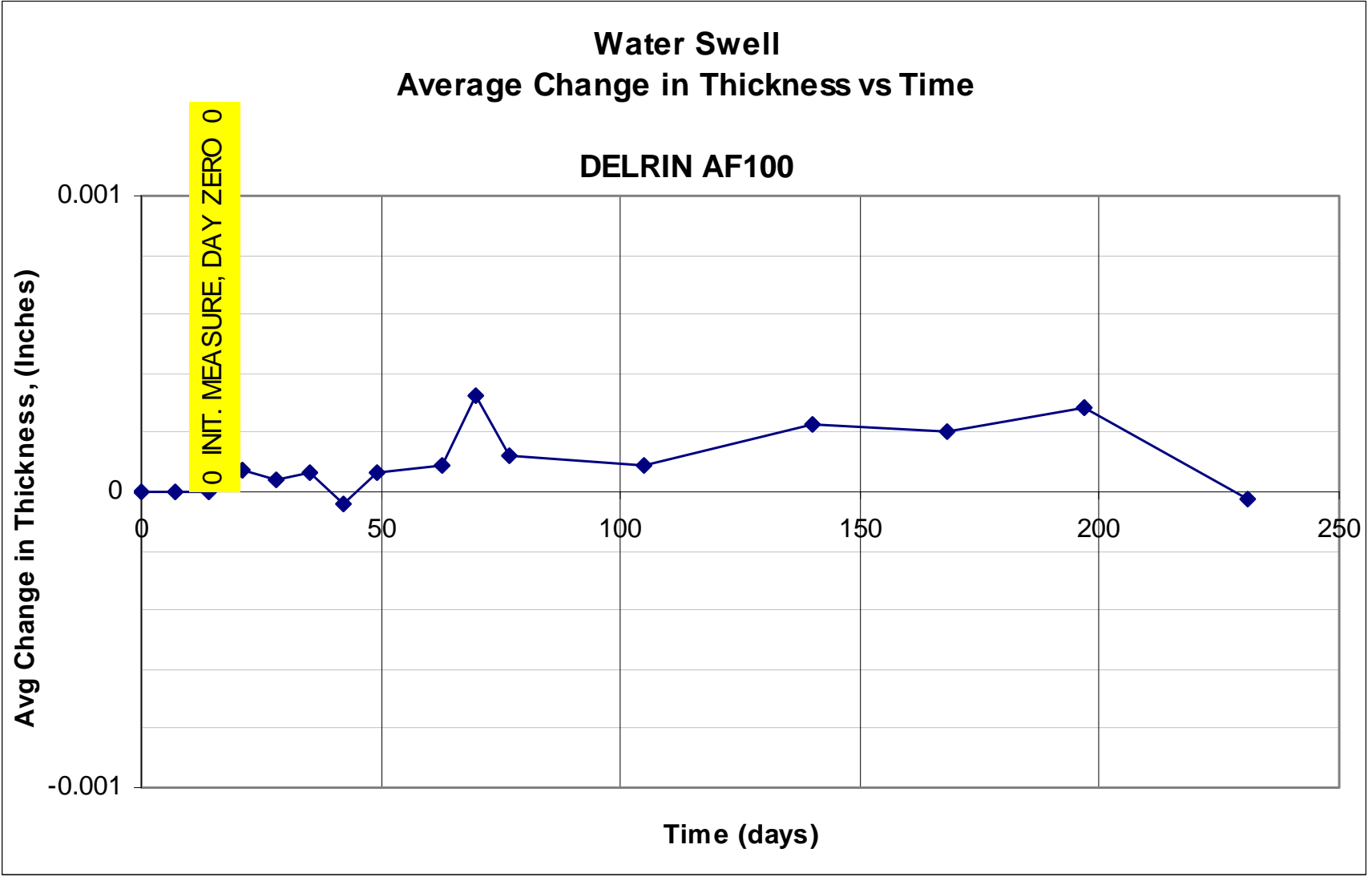
Figure E32. Average change in water swell thickness vs time using Delrin AF100.
