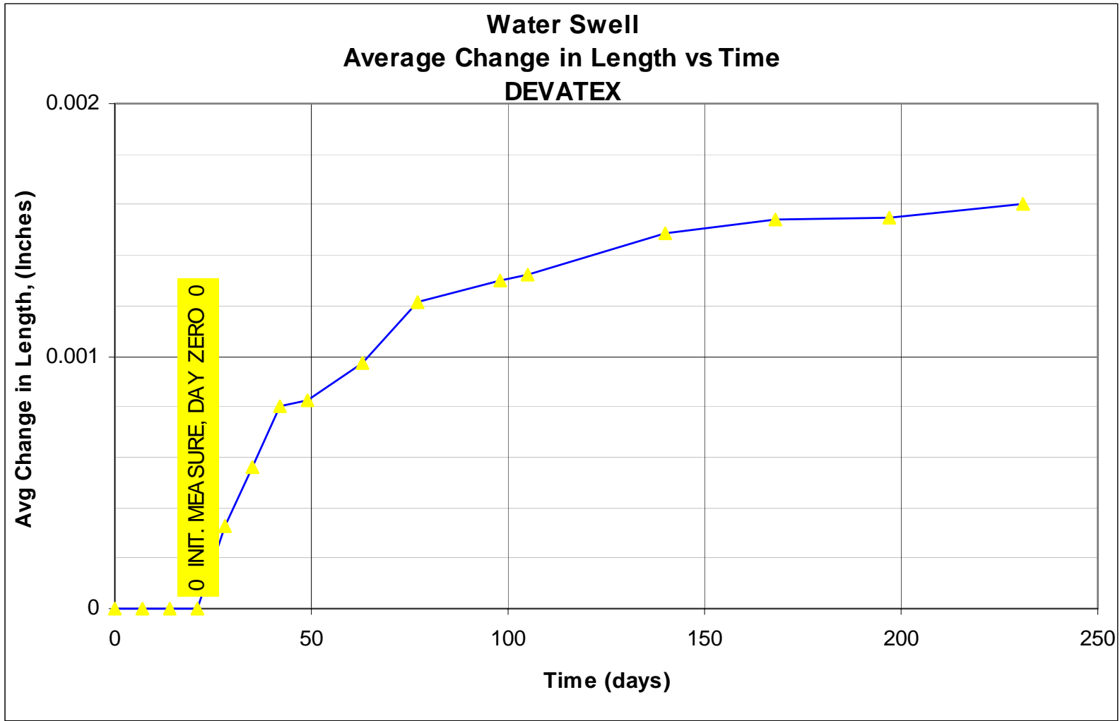
Figure E3. Average change in water swell length vs time using Devatex.
