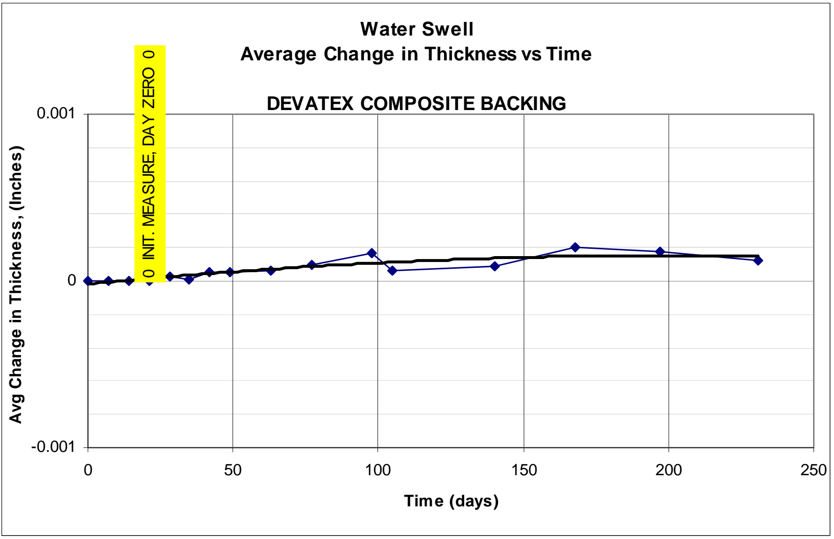
Figure E8. Average change in water swell thickness vs time using a Devatex composite backing.
