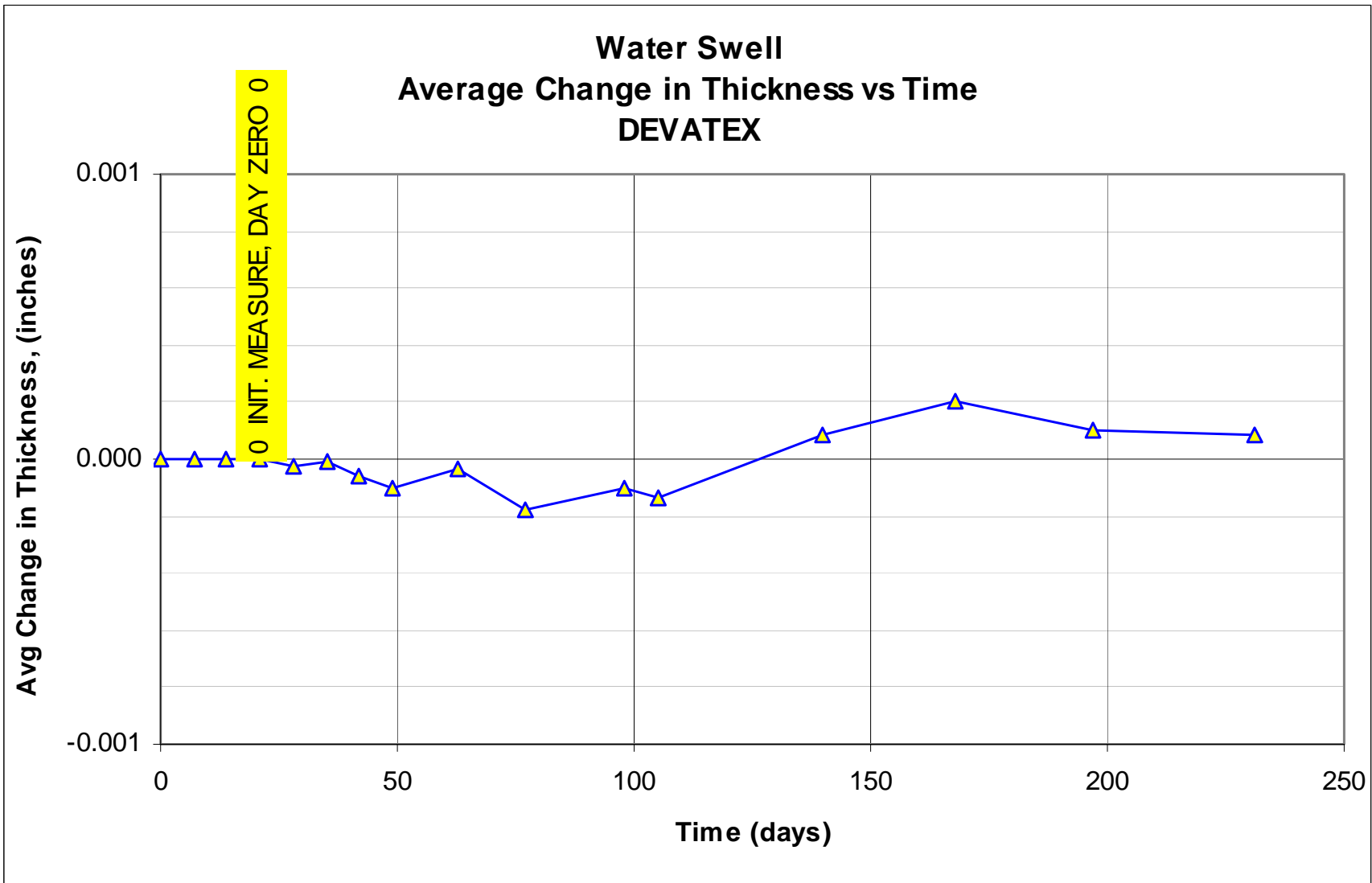
Figure E4. Average change in water swell thickness vs time using Devatex.
