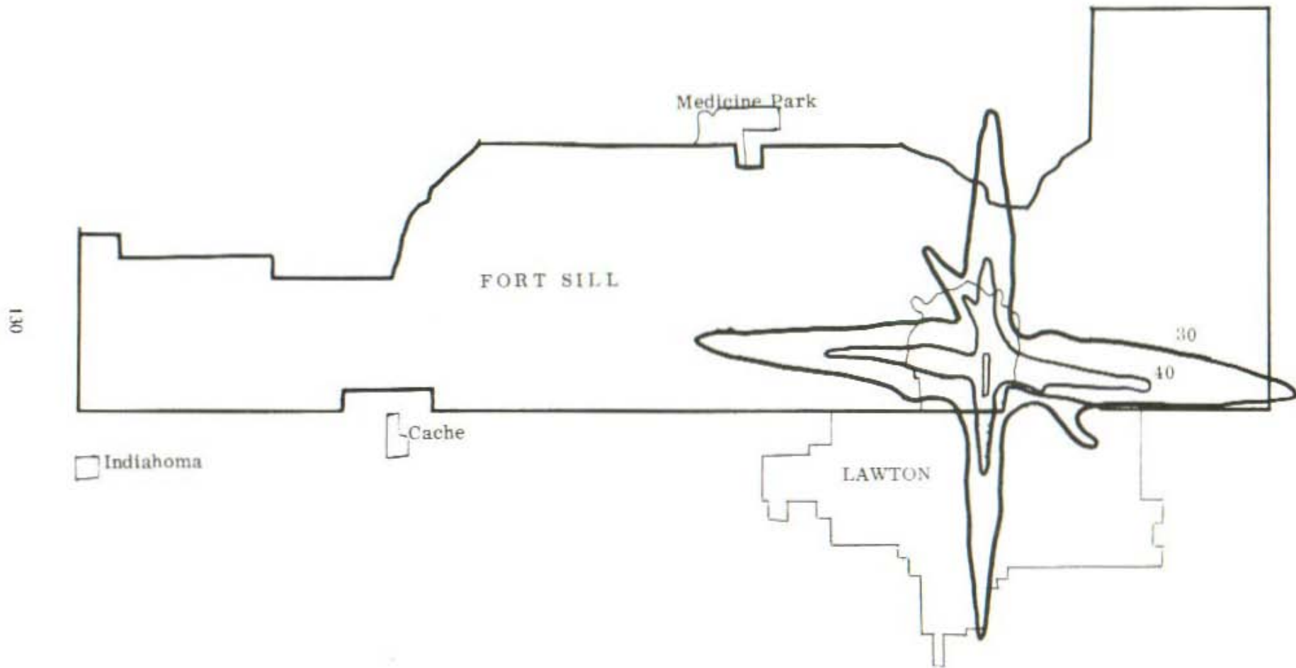
Figure B1. Base and plan map with NEF contours.
