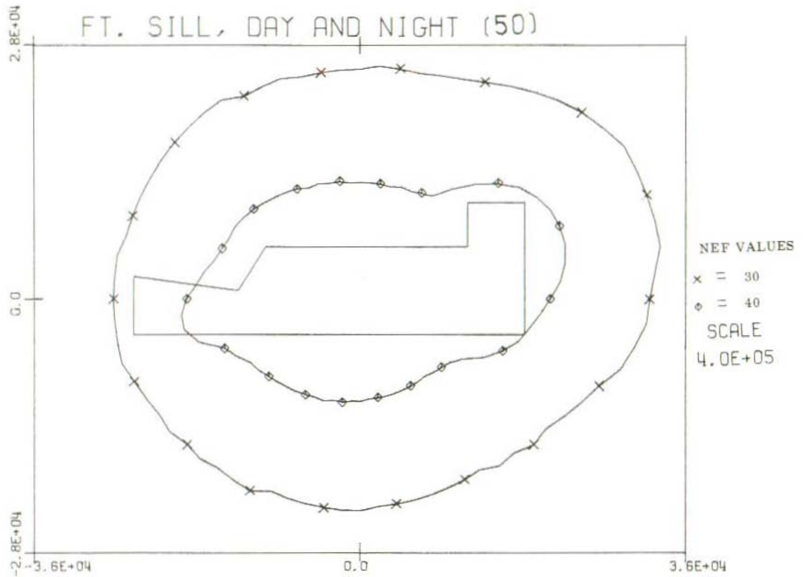
Figure B3. NEF contour for 50% inversion condition.
