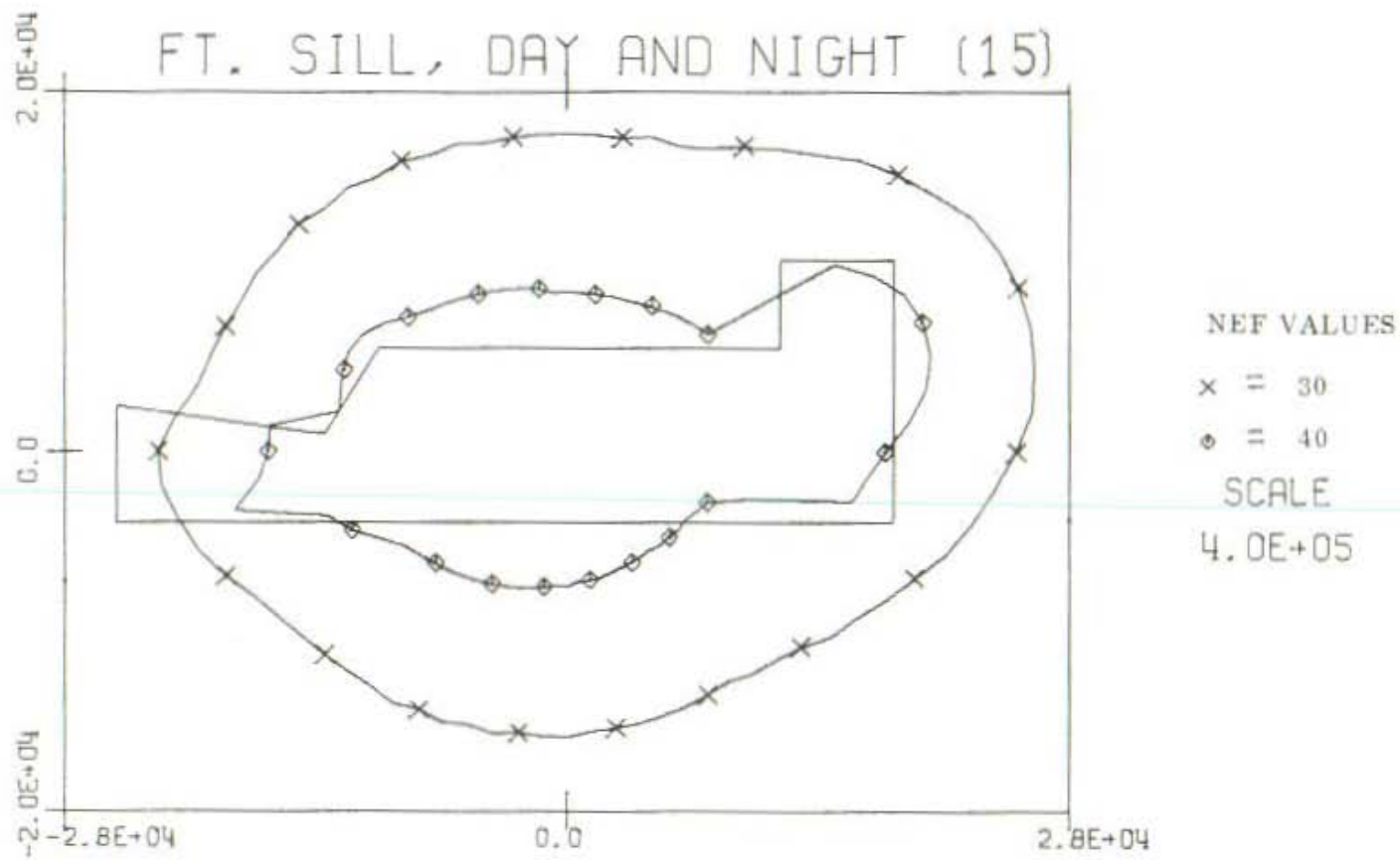
Figure B6. Firing during non-inversion daylight hours.
