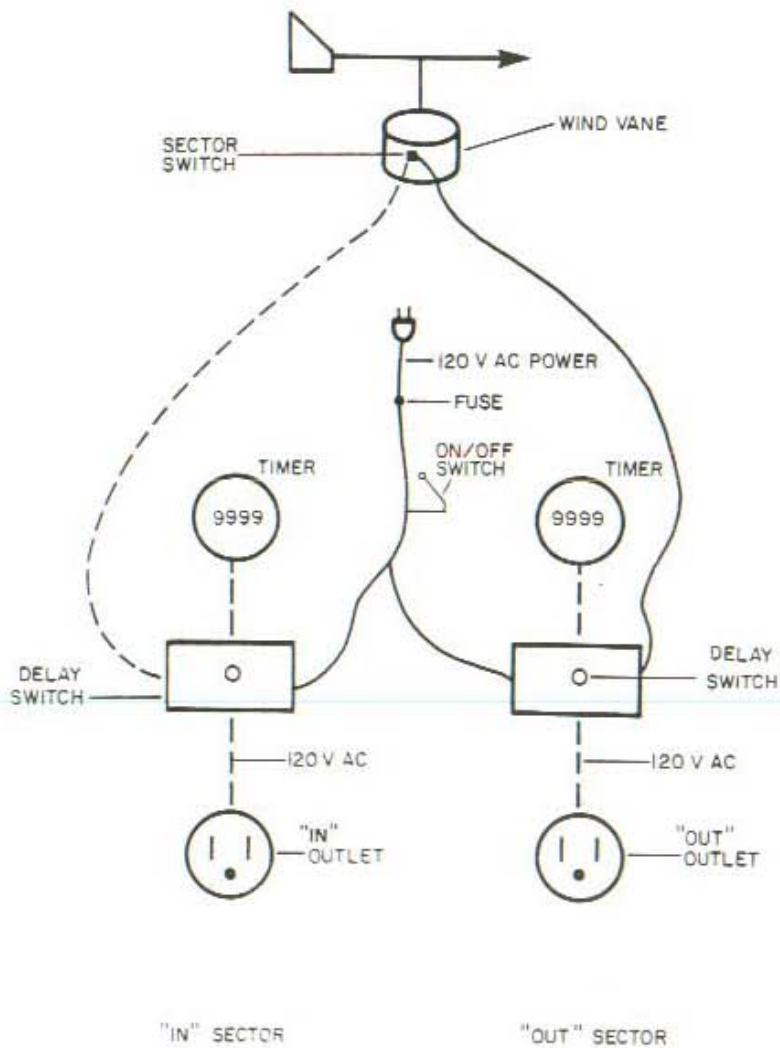
Figure 3. Wind direction controller system schematic.
