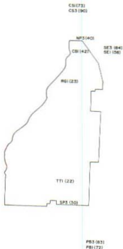
Figure 10. Station annual geometric mean concentrations.
