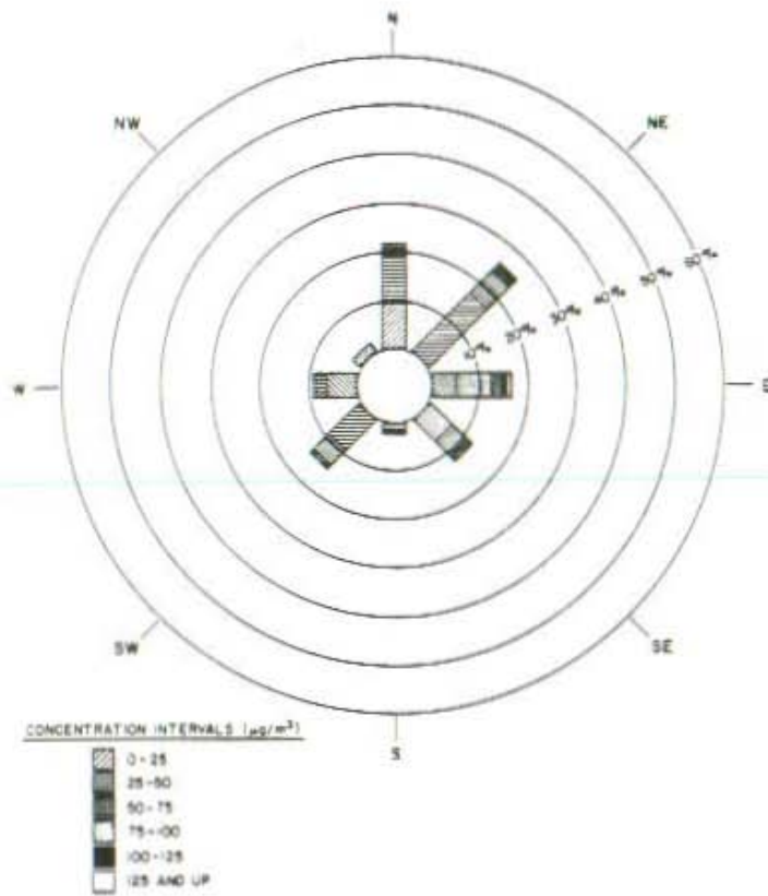
Figure 14. Concentration distribution for the Fort Carson Training Area station.
