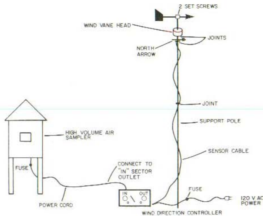
Figure 4. Three-day, high-volume sampling station schematic (North Post, South Post, El Paso Health Department, Security and Pueblo Health Department sites).
