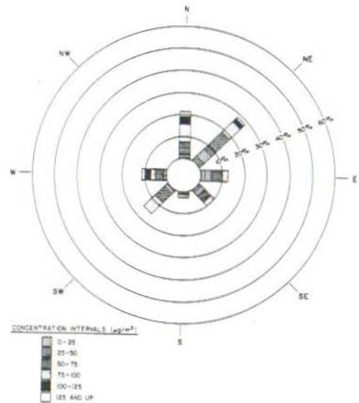
Figure 13. Concentration distribution for Pueblo County Health Department station.
