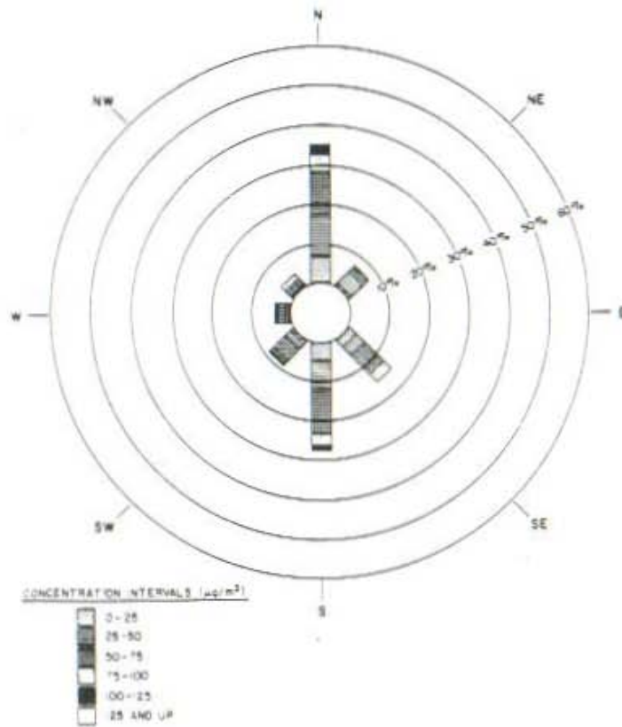
Figure 12. Concentration distribution for Security Volunteer Fire Department station.
