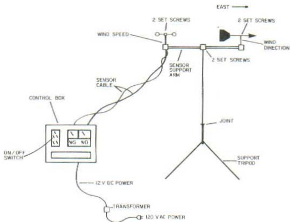
Figure 5. Climatronics wind monitoring system schematic.
