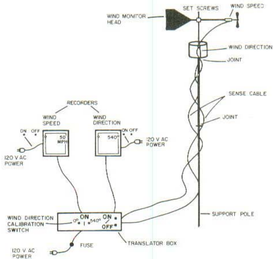
Figure 6. R. M. Young wind monitoring system schematic.
