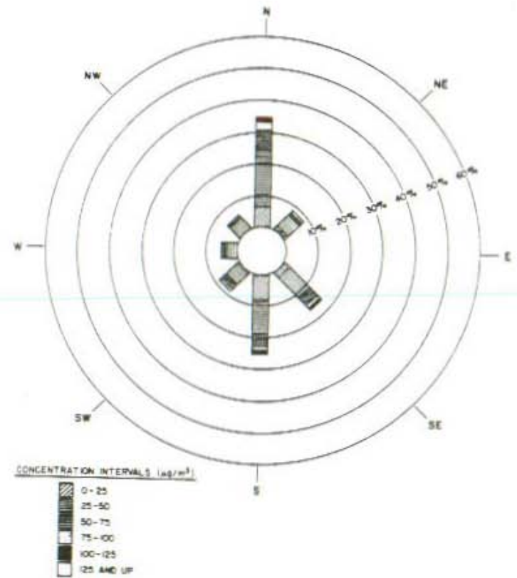
Figure 15. Concentration distribution for the Fort Carson Cantonment Area station.
