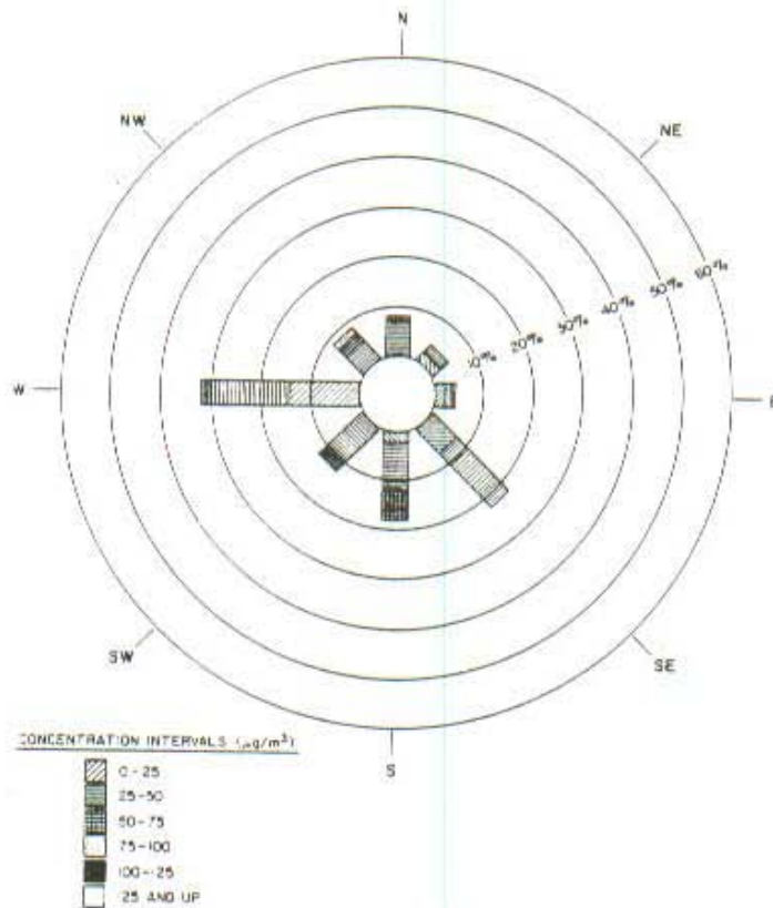
Figure 16. Concentration distribution for the background station.
