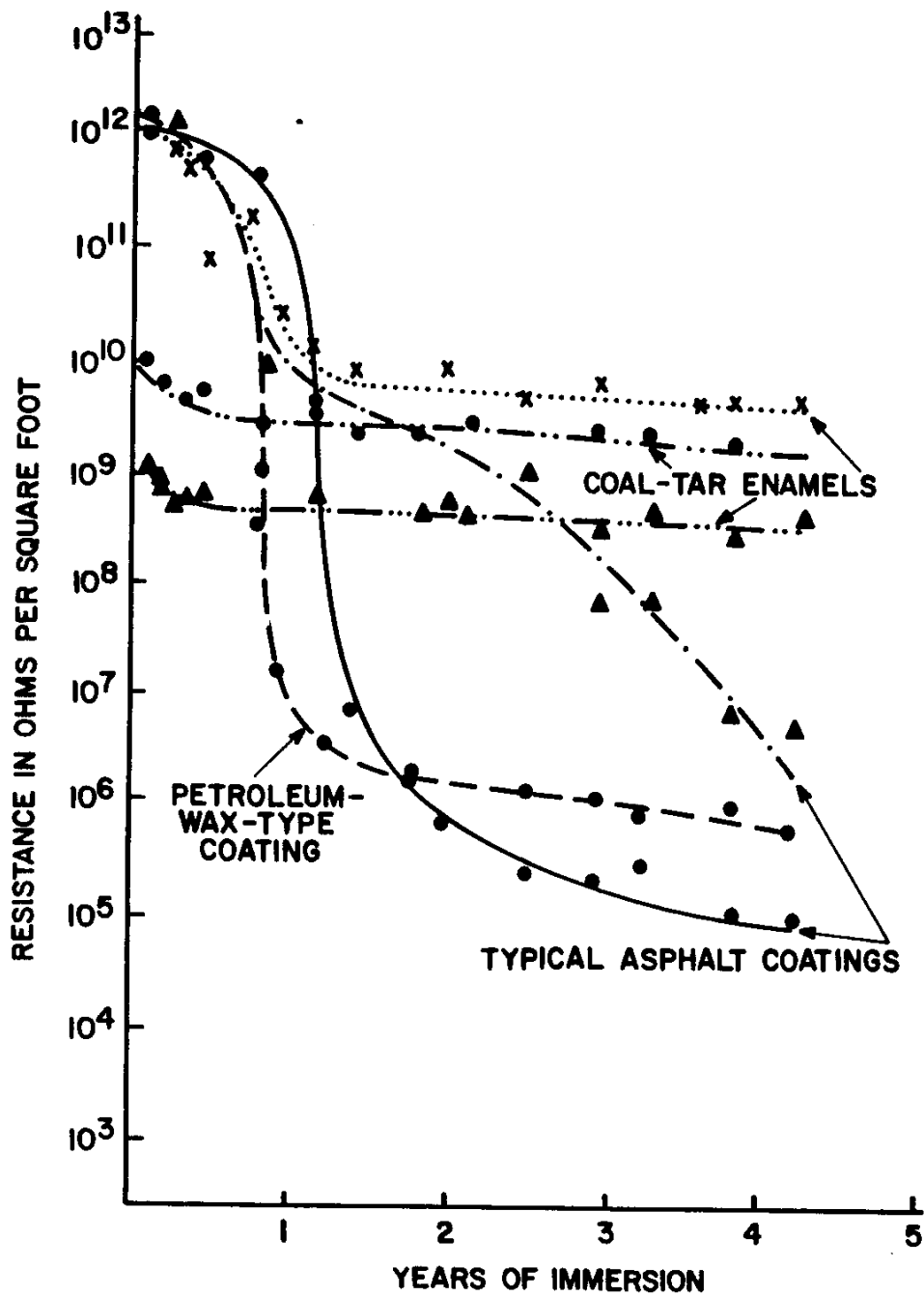
Figure 15. Effect of immersion time on the electrical resistance of selected coatings for steel in underground environments.
