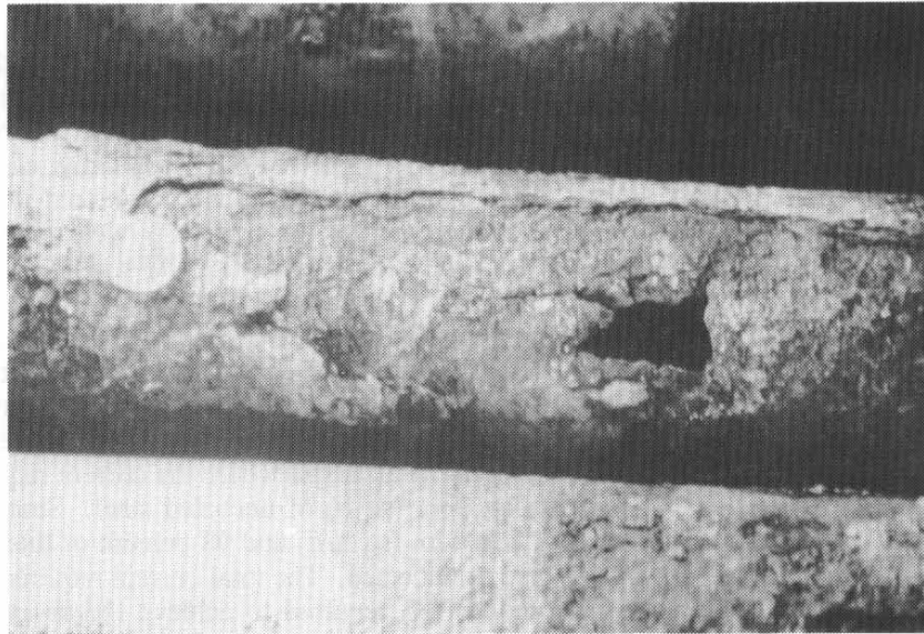
Figure 3. Corroded carrier pipe from a concrete trench. (Magnification: 0.6X)
