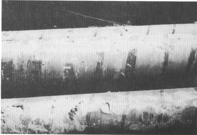
Figure 13. Damage to the bitumen coating was present before installation.
