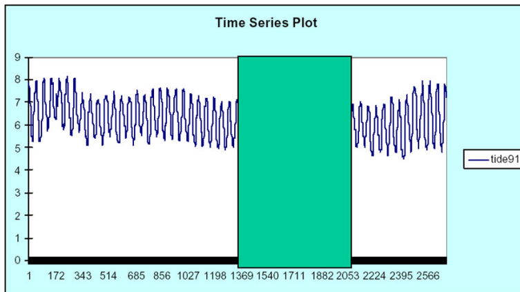
b. Output series for surface elevation at lagoon entrance (ft)
