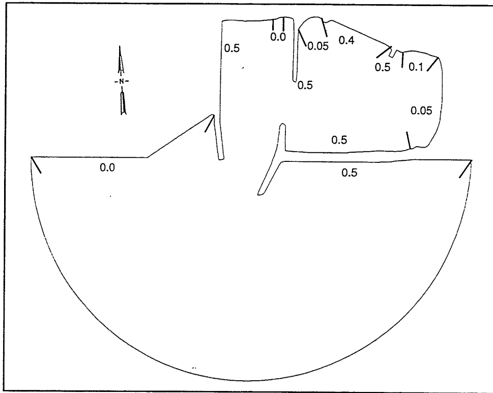
Figure 17. Wave reflection coefficient values, short waves, existing harbor
