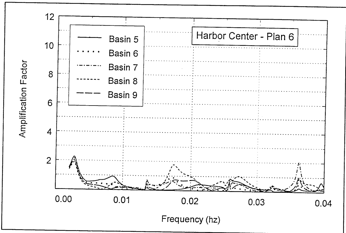
Figure C4. Long wave response, harbor center, Plan 6
