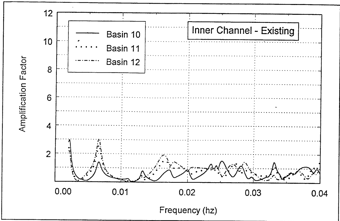
Figure C5. Long wave response, inner channel, existing harbor
