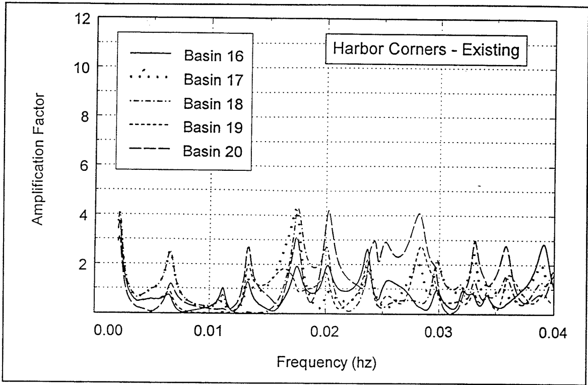
Figure C9. Long wave response, harbor corners, existing harbor
