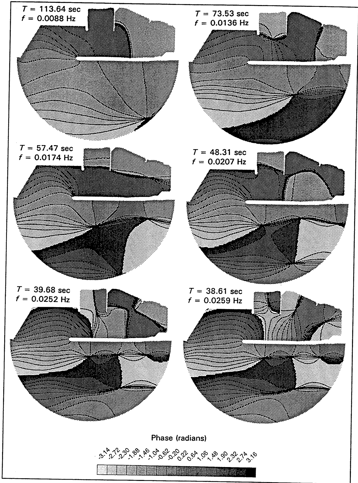
Figure 26. Resonant long wave phase contours, Plan 6
