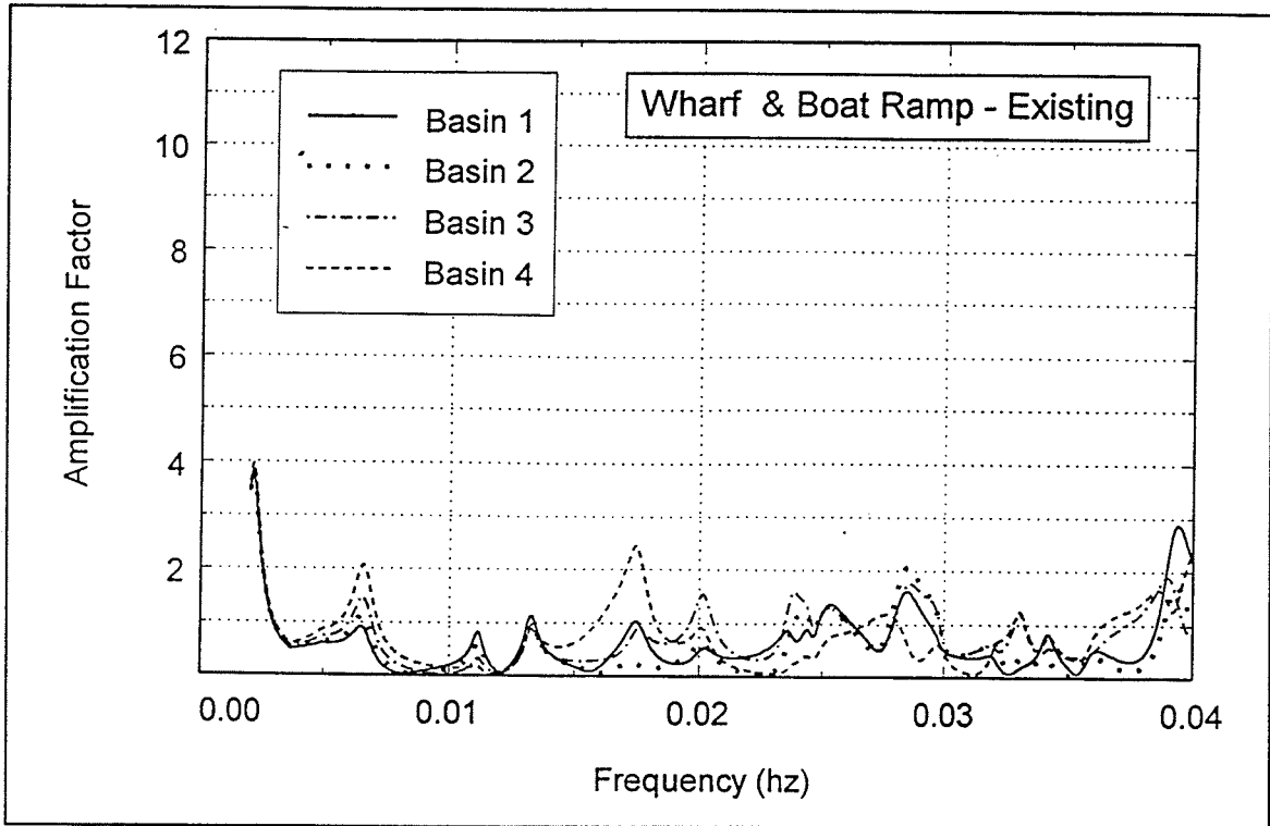
Figure C1. Long wave response, wharf and boat ramp, existing harbor
