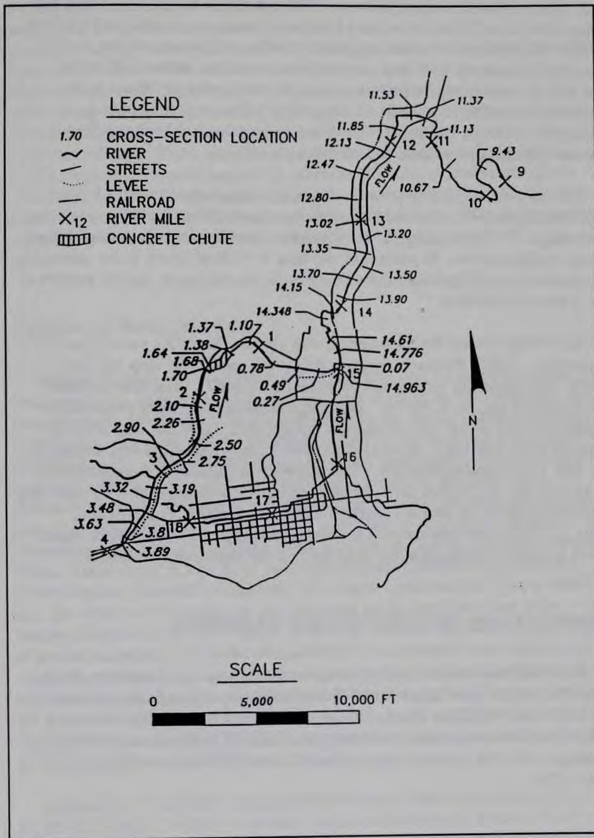
Figure 3. Cross-section locations
