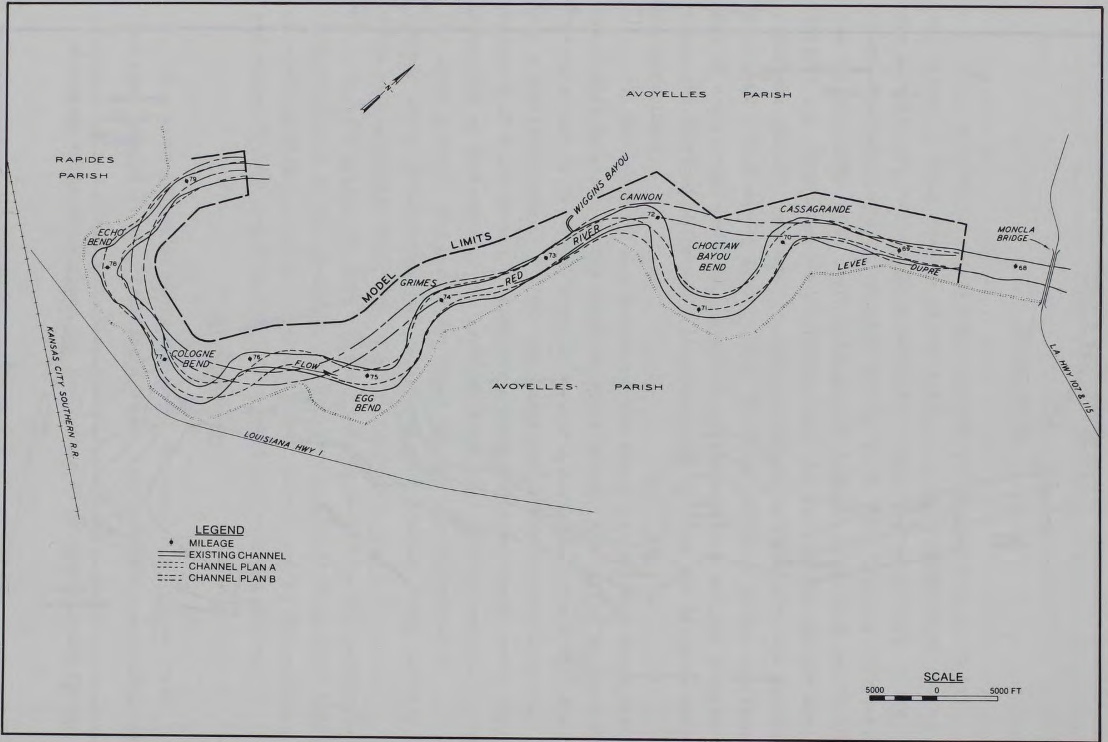
Figure 3. Channel alignment
