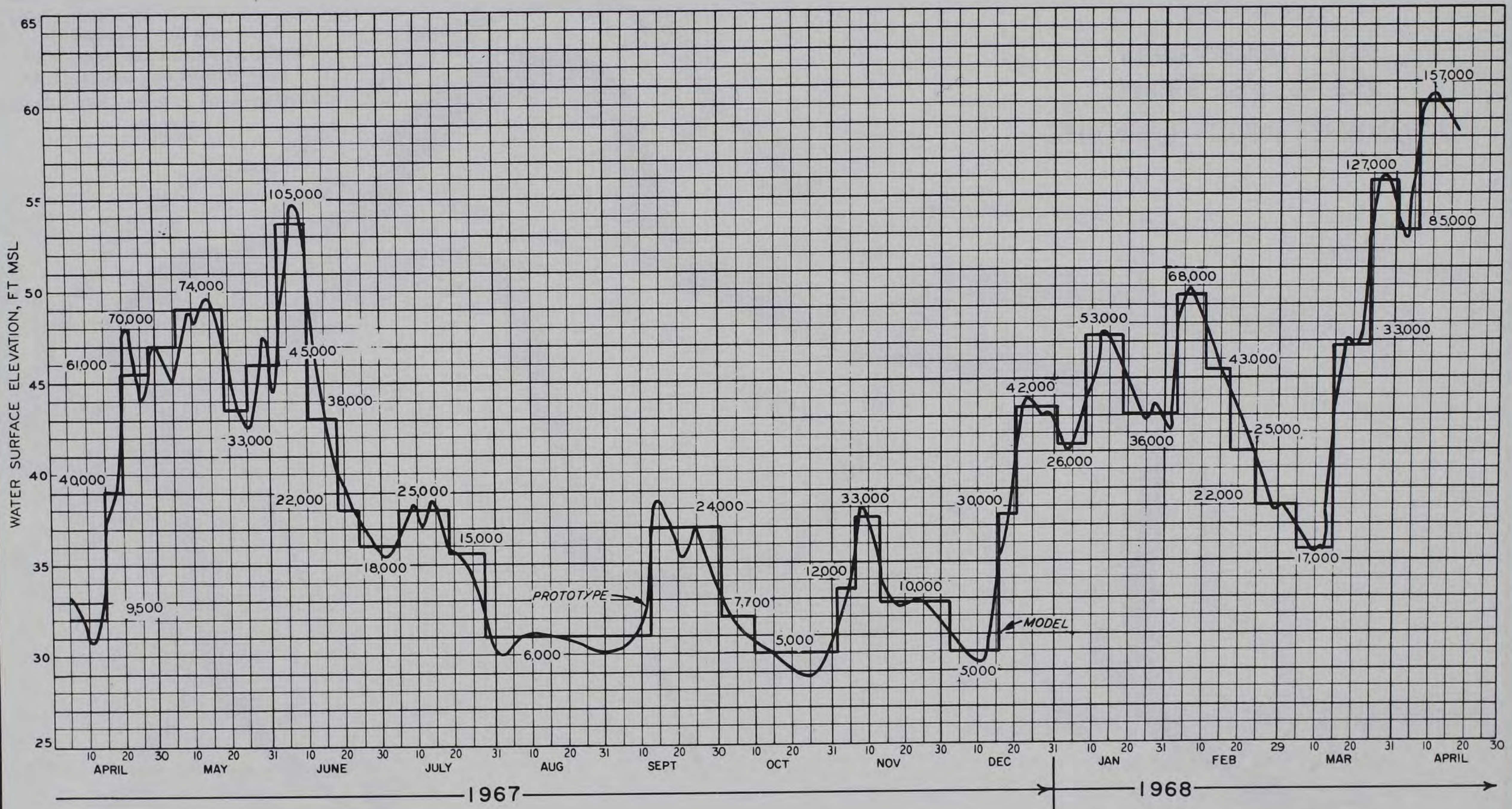
1967-1968 STAGE HYDROGRAPH
