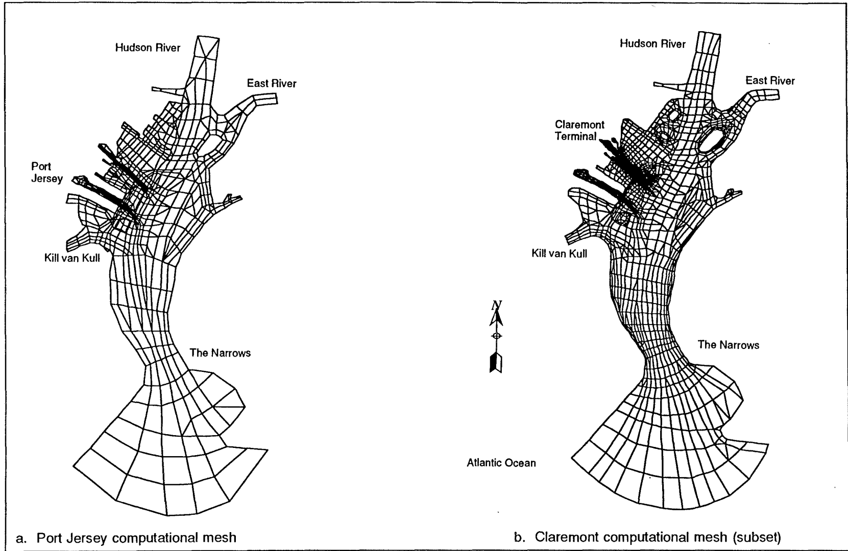
Figure A4. Comparison of the Claremont mesh and the predecessor Port Jersey mesh
