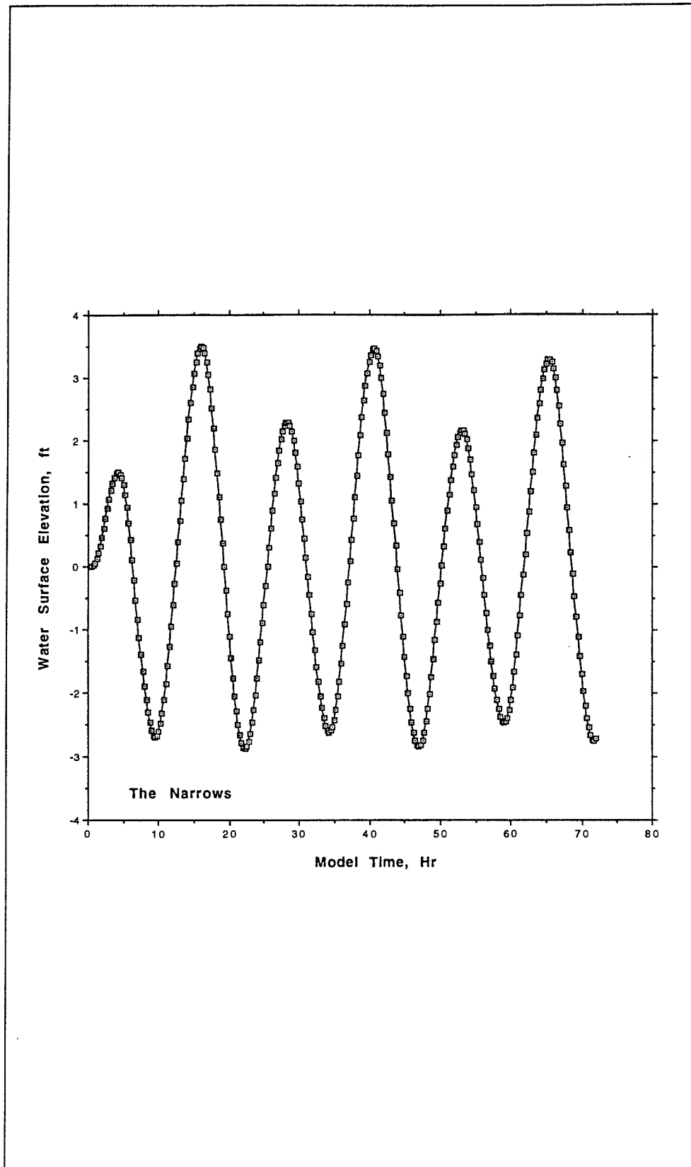
Figure A20. Water surface elevation at the Narrows, existing condition
