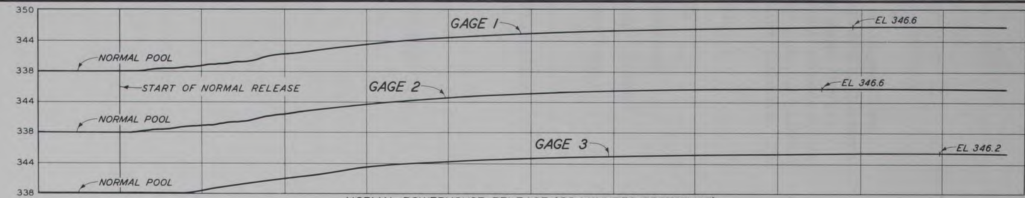
NORMAL POWERHOUSE RELEASE (25 MINUTES PROTOTYPE) FLOW FROM 0 TO 50,000 CFS
