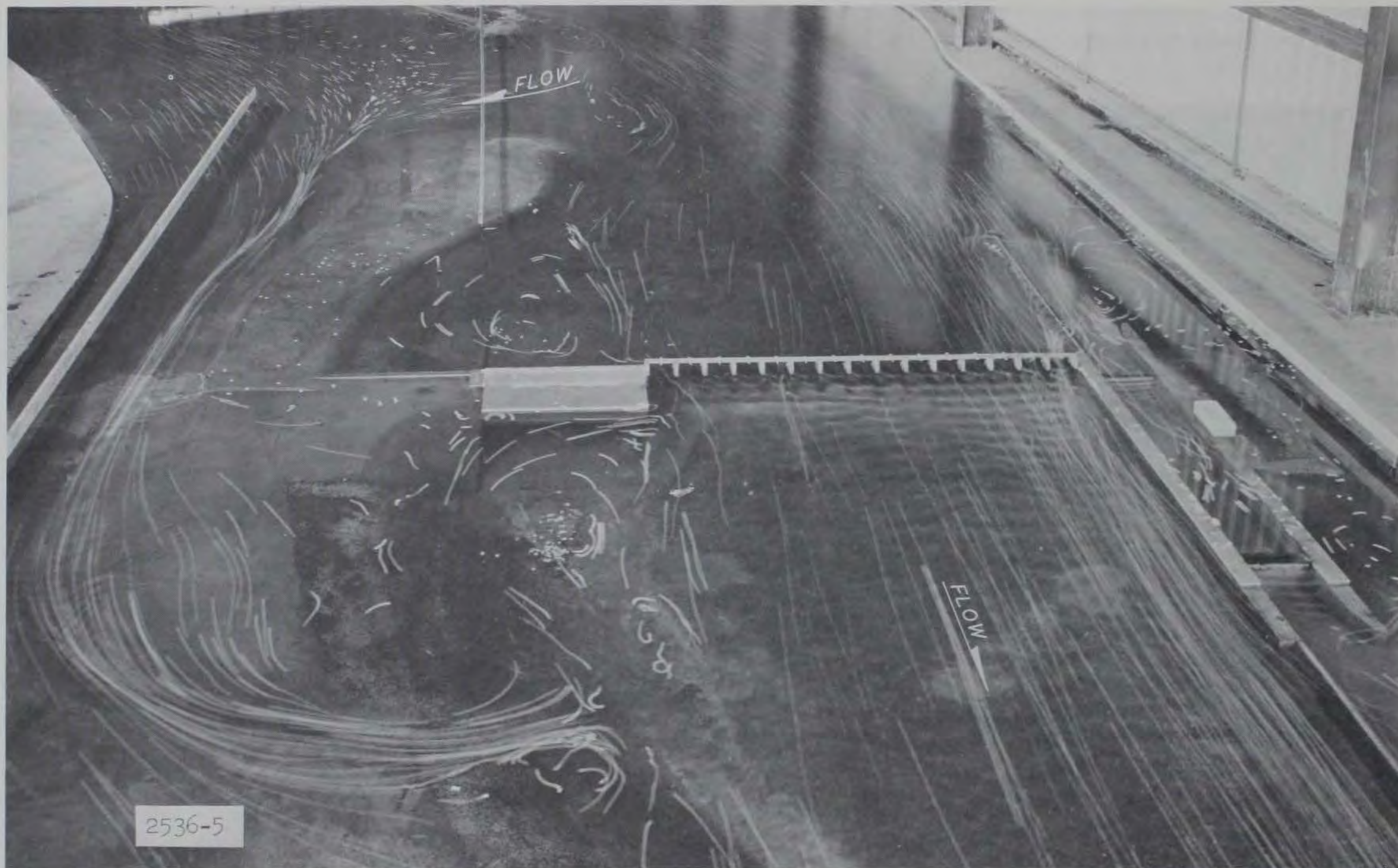
Photograph 14. Discharge 920,000 cfs; surface currents in vicinity of the structures with the right bank access road removed
