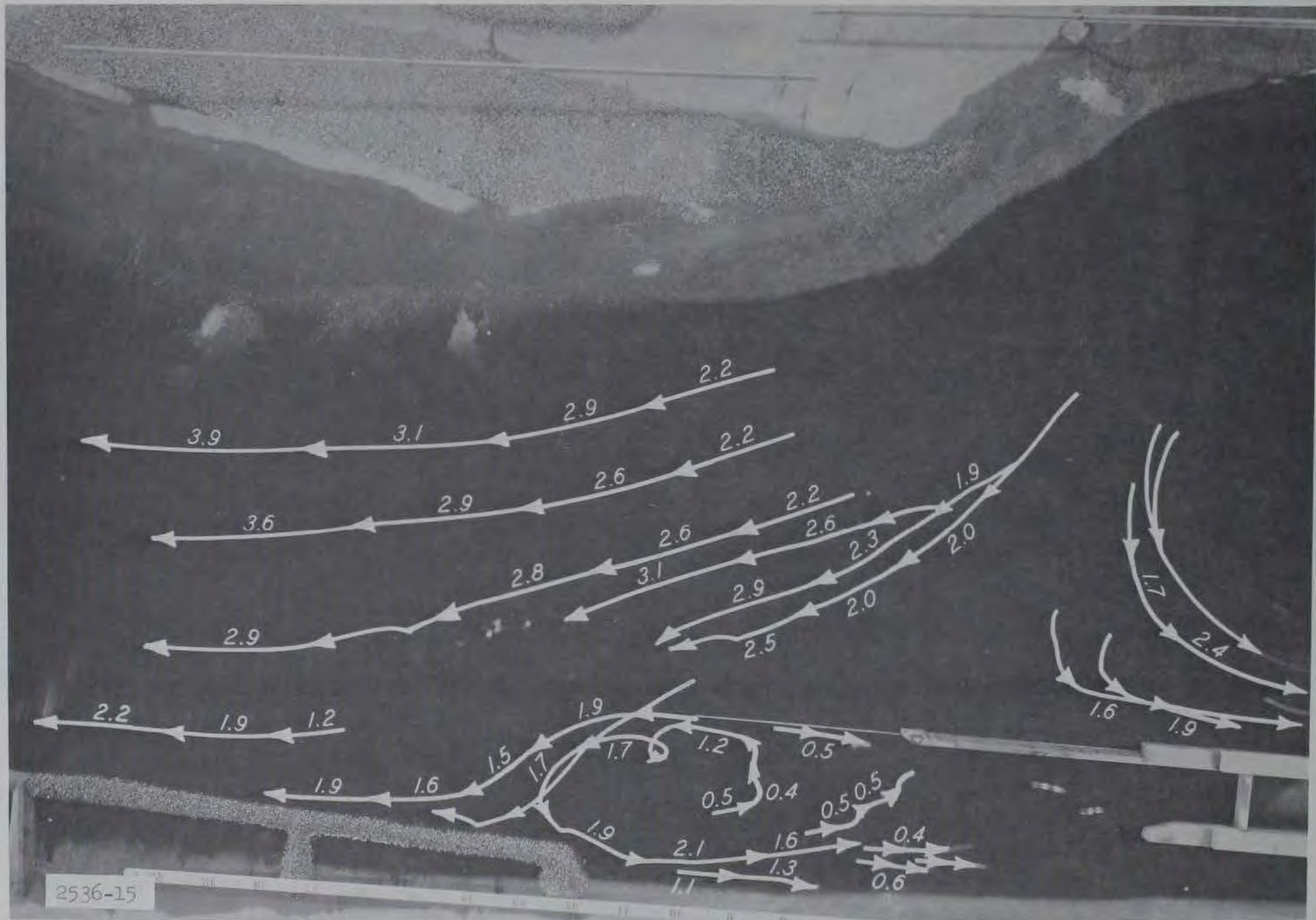
Photograph 9. Paths of floats (submerged 9 ft) during the period 11-22 min after start of powerhouse release. Powerhouse discharge increased from 0 to 50,000 cfs in 25 min (prototype). Numbers indicate average velocity in feet per second during 11-min period
