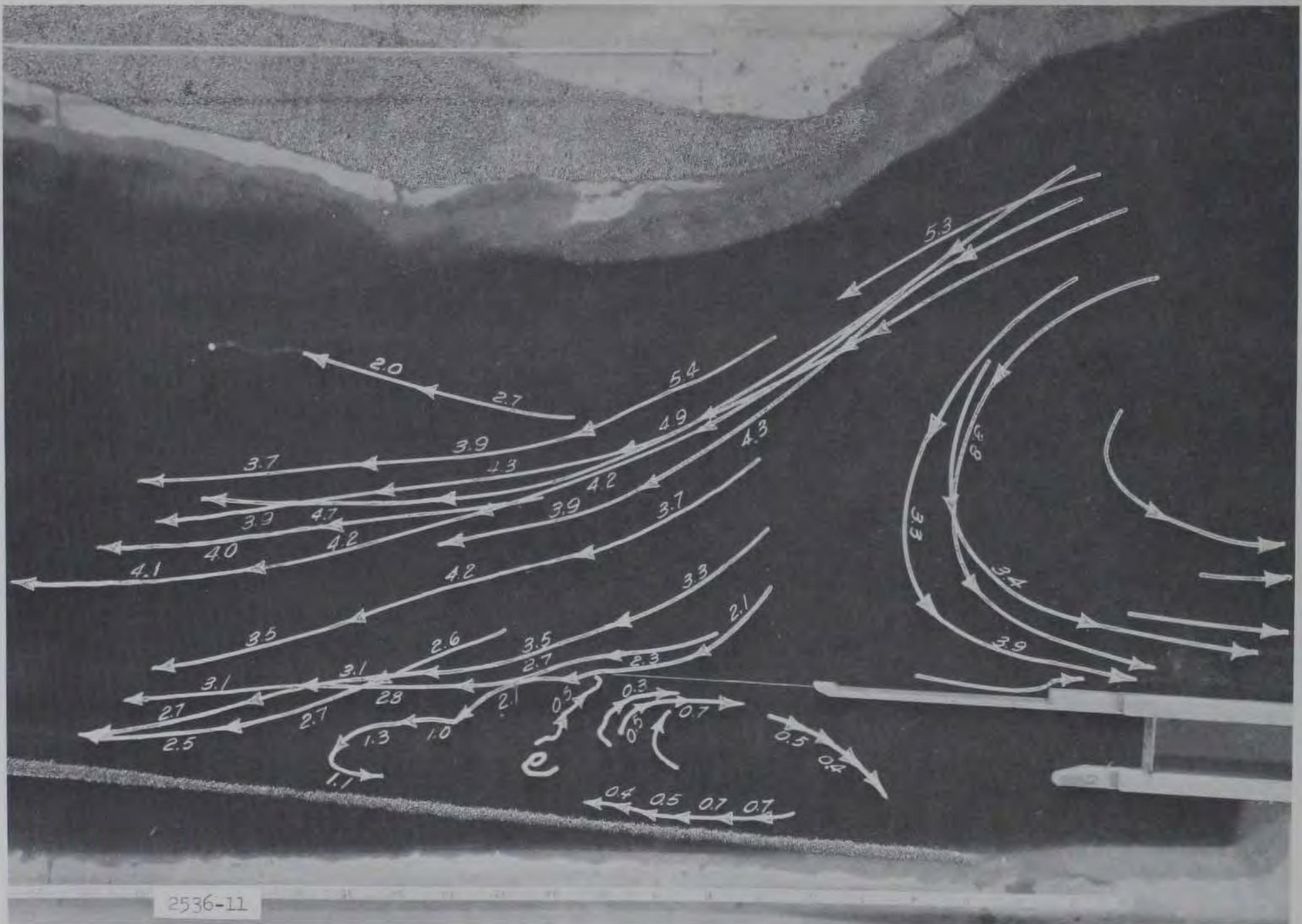
Photograph 3. Paths of floats (submerged 9 ft) during period 44-55 min after start of powerhouse release. Powerhouse discharge increased from 0 to 50,000 cfs in 6 sec (prototype). Numbers indicate average velocity in feet per second during 11-min period
