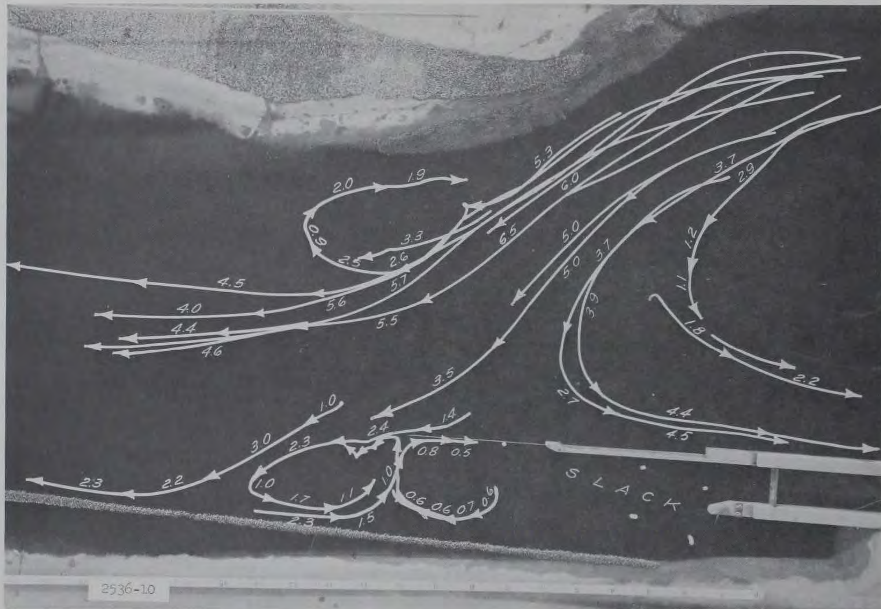
Photograph 6. Paths of floats (submerged 9 ft) during the period 44-55 min after start of powerhouse release. Powerhouse discharge increased from 0 to 50,000 cfs in 25 min (prototype). Numbers indicate average velocity in feet per second during 11-min period
