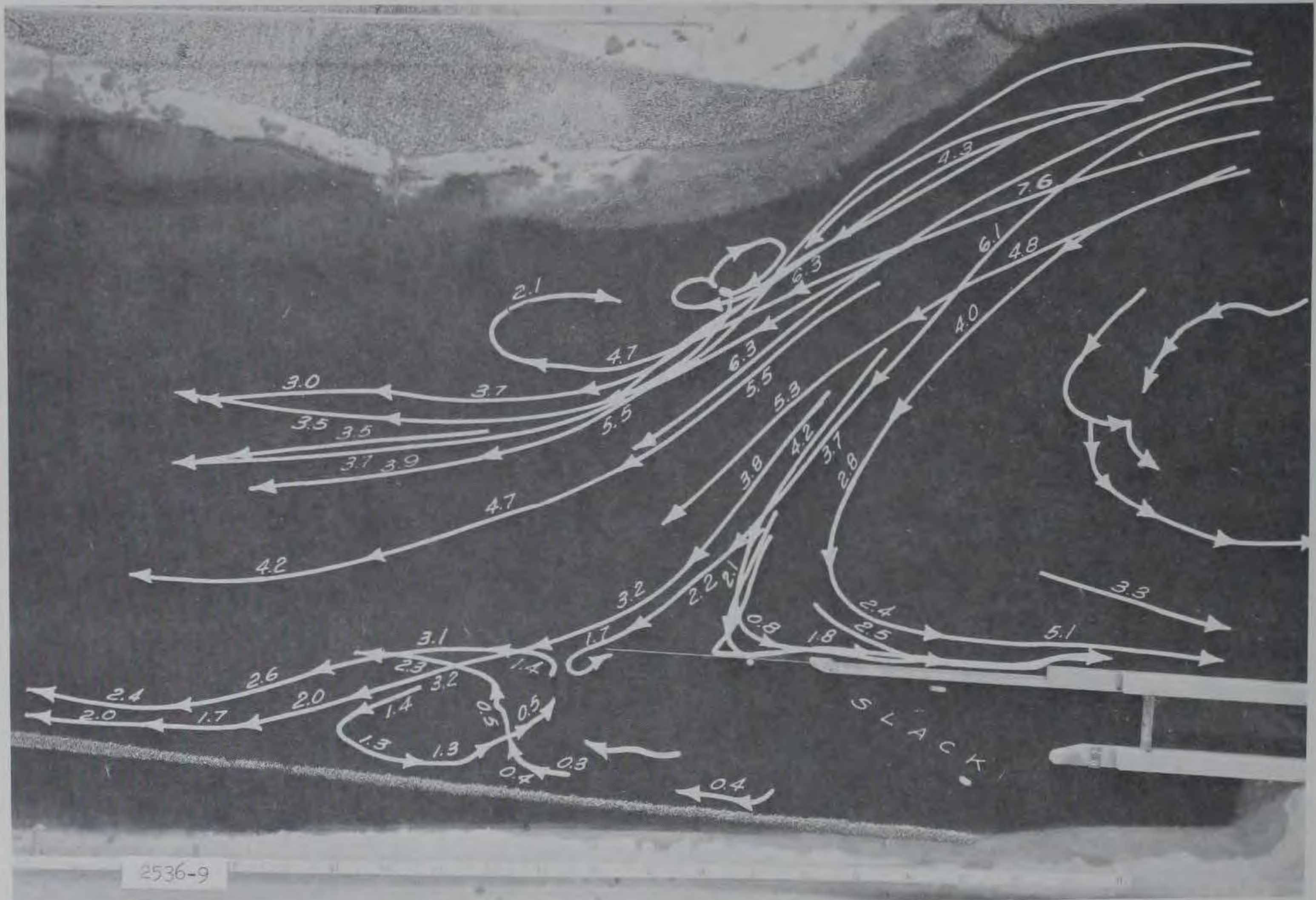
Photograph 7. Paths of floats (submerged 9 ft) during the period 66-77 min after start of powerhouse release. Powerhouse discharge increased from 0 to 50,000 cfs in 25 min (prototype). Numbers indicate average velocity in feet per second during 11-min period
