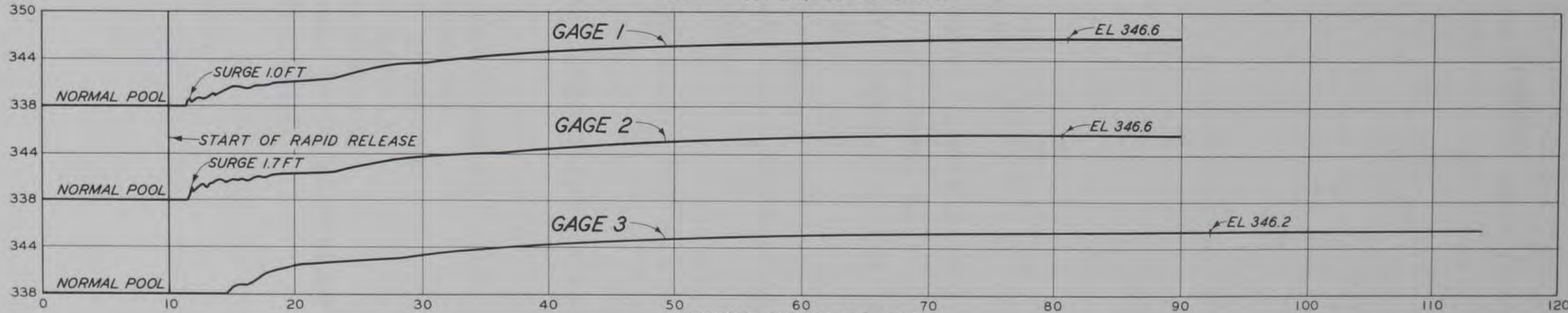
RAPID POWERHOUSE RELEASE (6 SECONDS PROTOTYPE) FLOW FROM 0 TO 50,000 CFS
