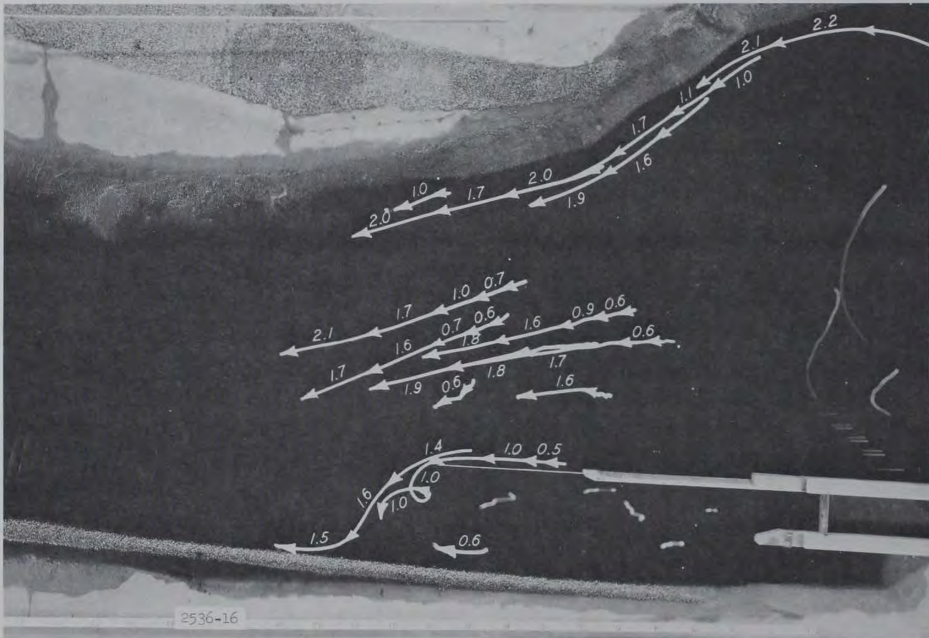
Photograph 4. Paths of floats (submerged 9 ft) during the period 0-11 min after start of powerhouse release. Powerhouse discharge increased from 0 to 50,000 cfs in 25 min (prototype). Numbers indicate average velocity in feet per second during 11-min period
