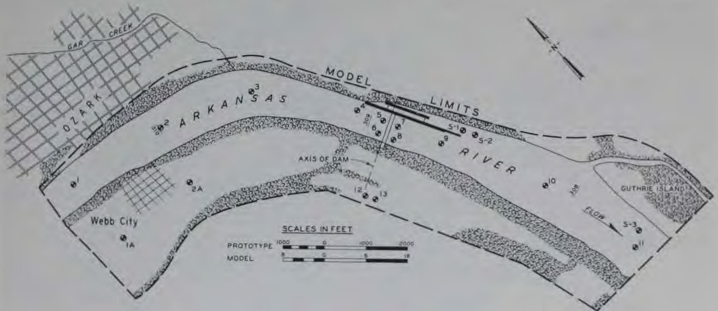
Fig. 3. Model layout and locations of gages
