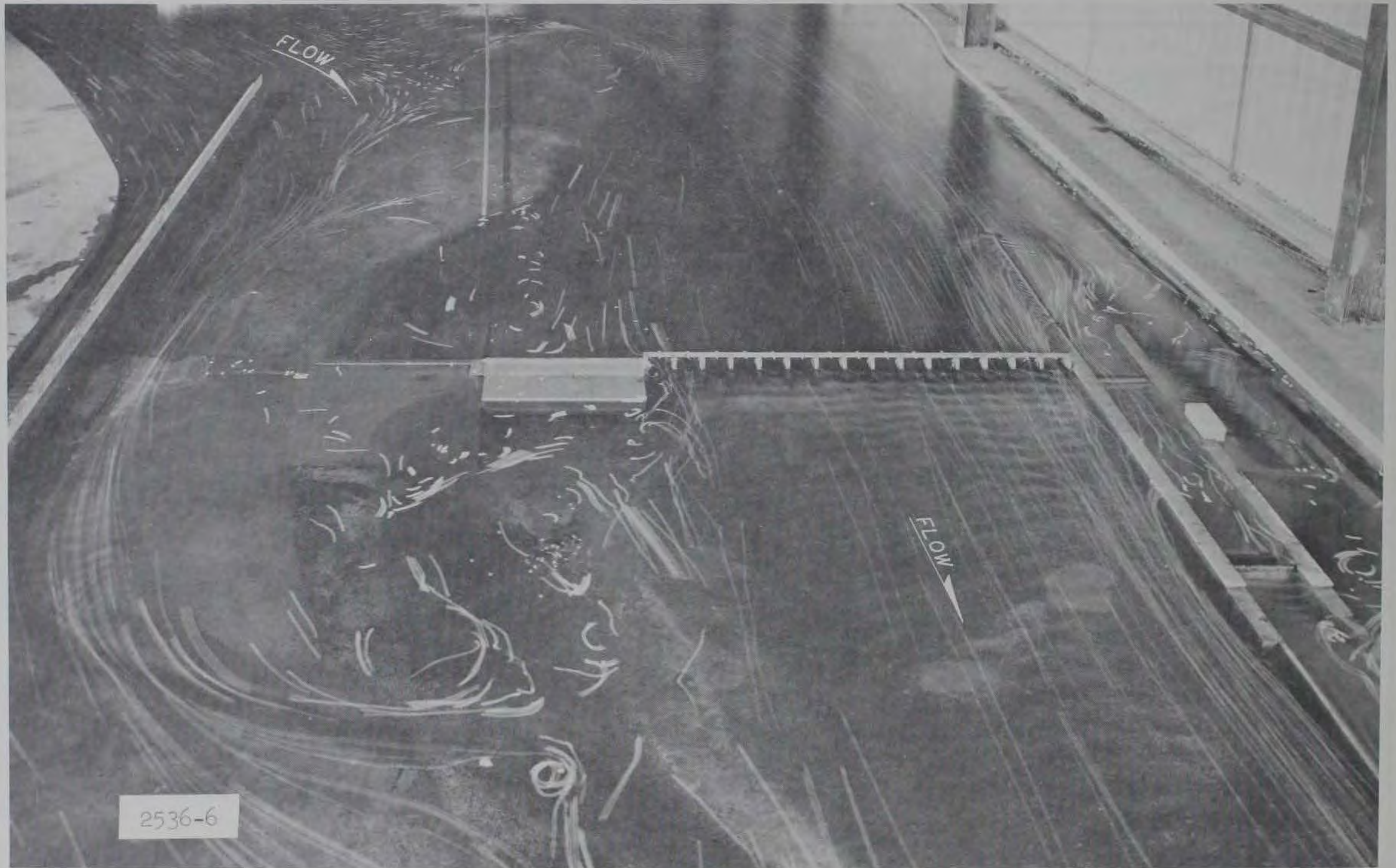
Photograph 15. Discharge 1,000,000 cfs; surface currents in vicinity of the structures with the right bank access road removed
