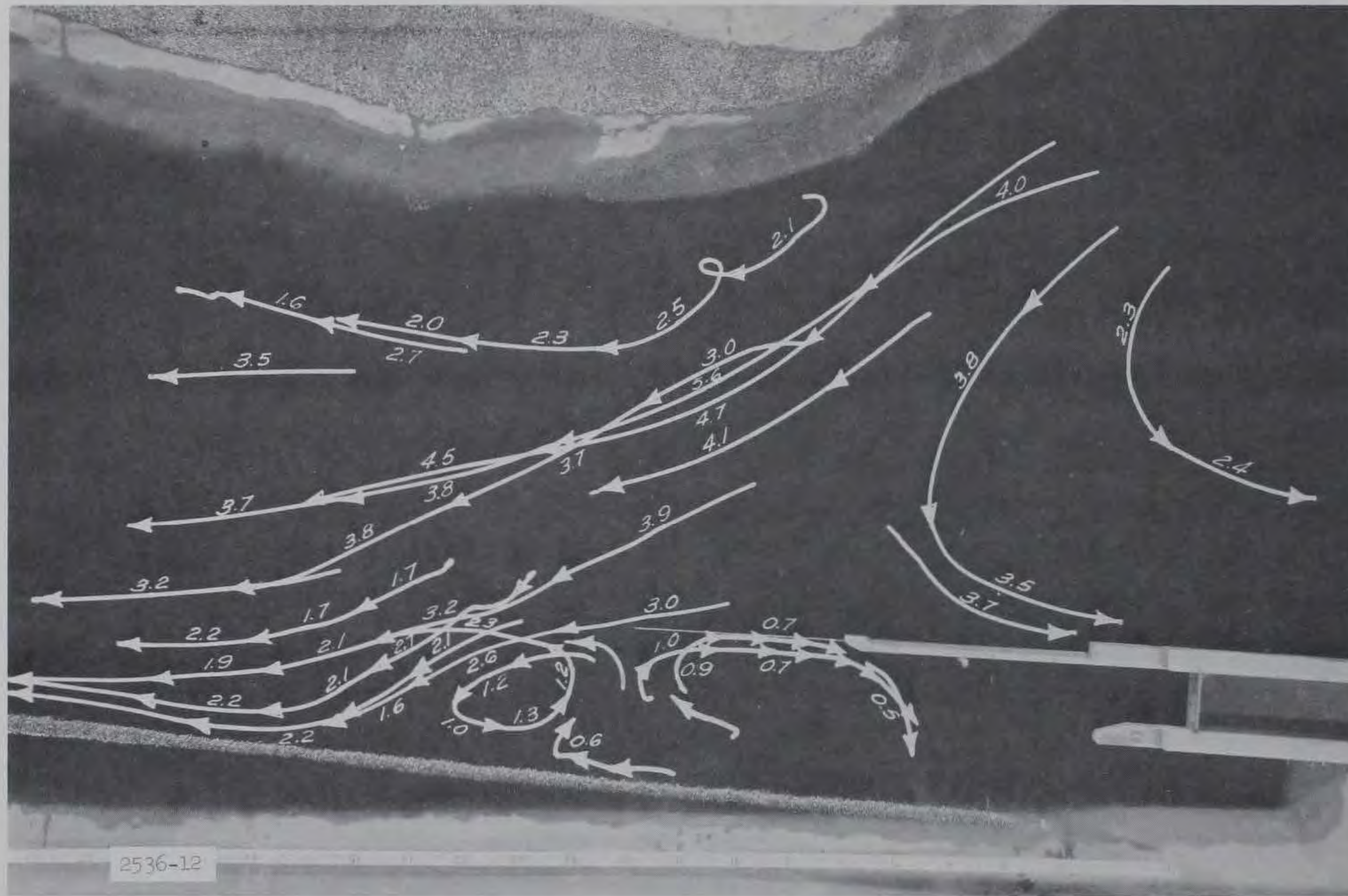
Photograph 2. Paths of floats (submerged 9 ft) during period 22-33 min after start of powerhouse release. Powerhouse discharge increased from 0 to 50,000 cfs in 6 sec (prototype). Numbers indicate average velocity in feet per second during 11-min period
