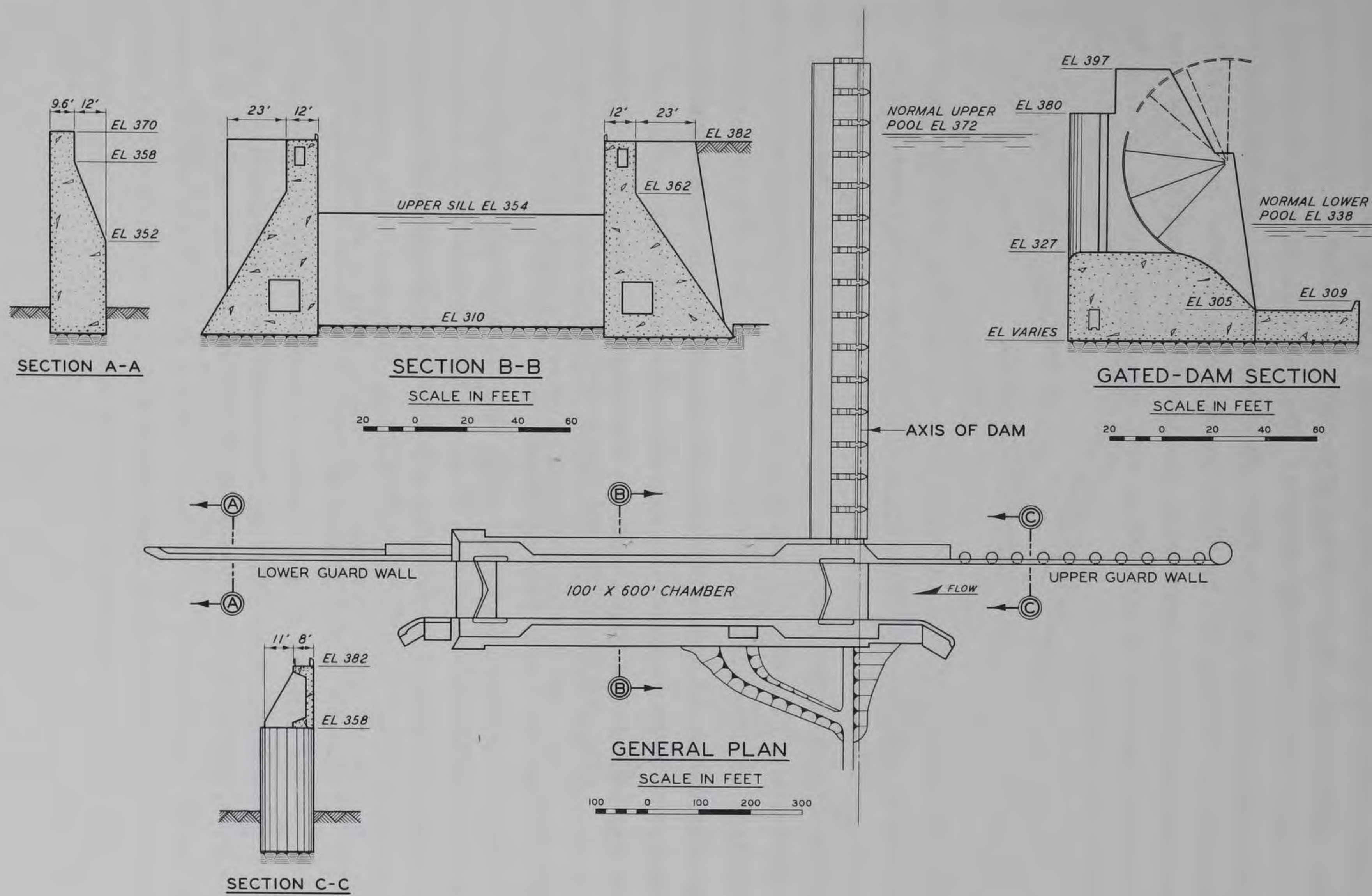
Fig. 2. General plan of lock and dam
