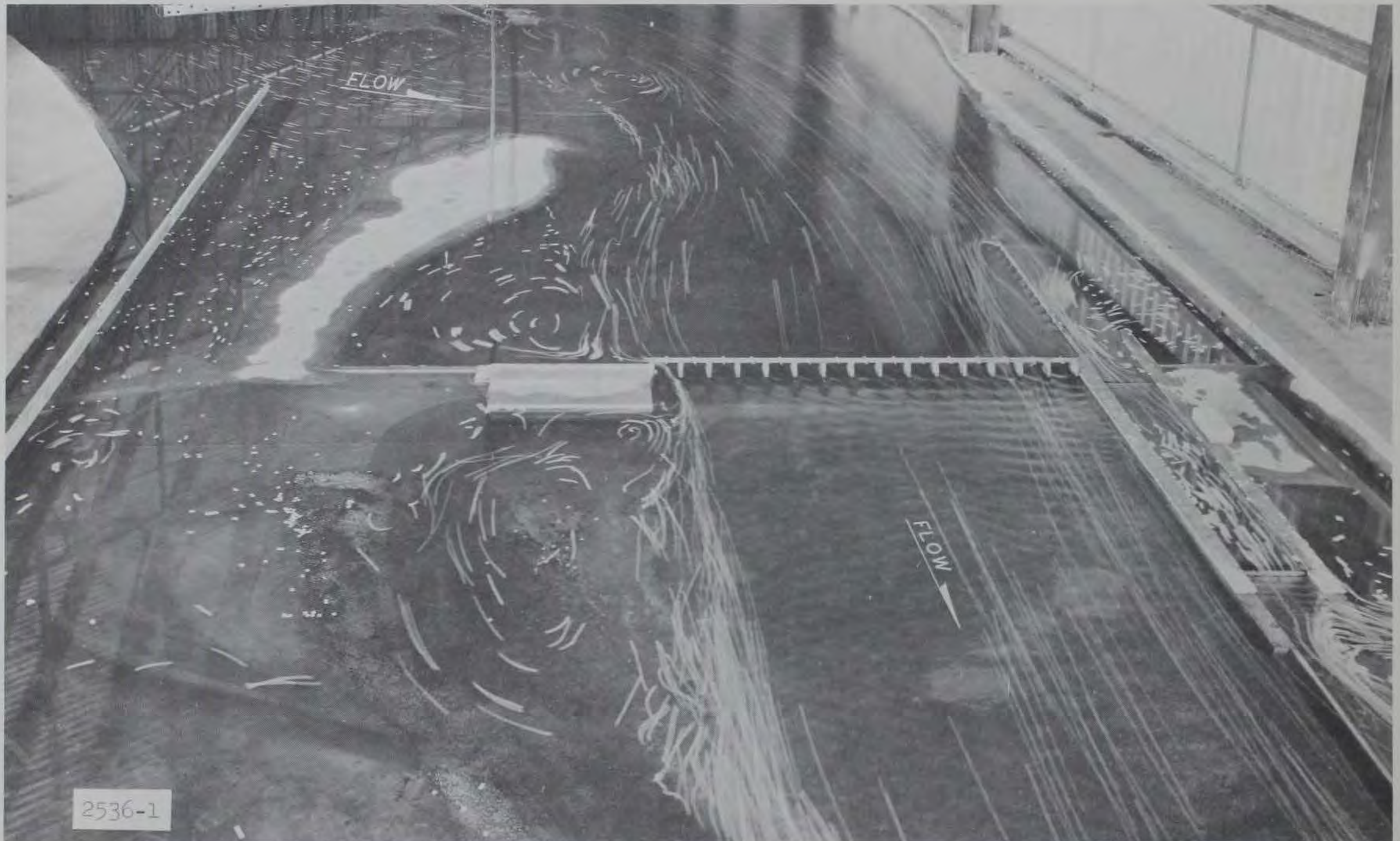
Photograph 10. Discharge 800,000 cfs; surface currents in vicinity of the structures with the right bank access road in place
