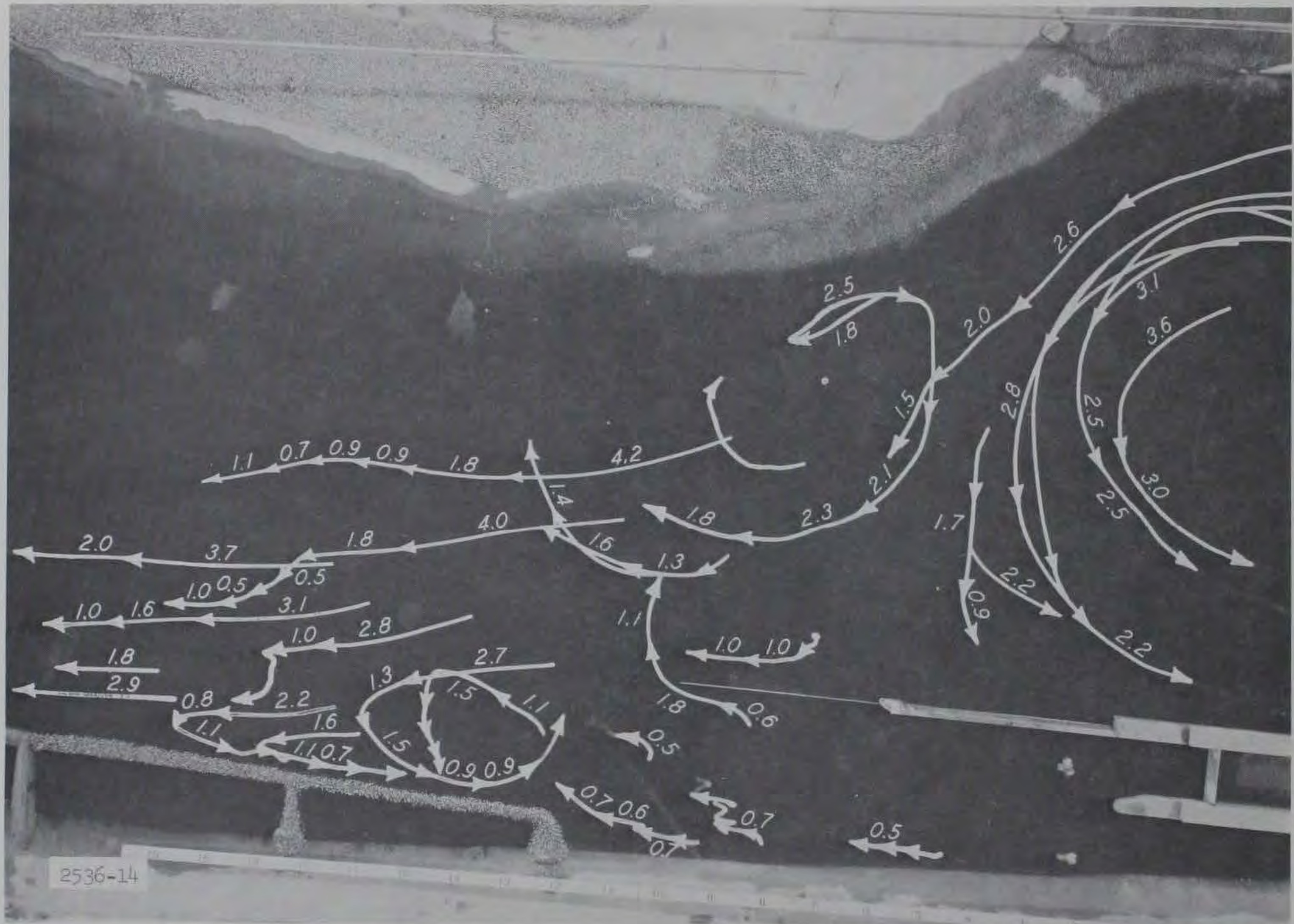
Photograph 8. Paths of floats (submerged 9 ft) during the period 0-11 min after start of cut-off of powerhouse release. Powerhouse discharge decreased from 50,000 to 0 cfs in 6 sec (prototype). Numbers indicate average velocity in feet per second during 11-min period
