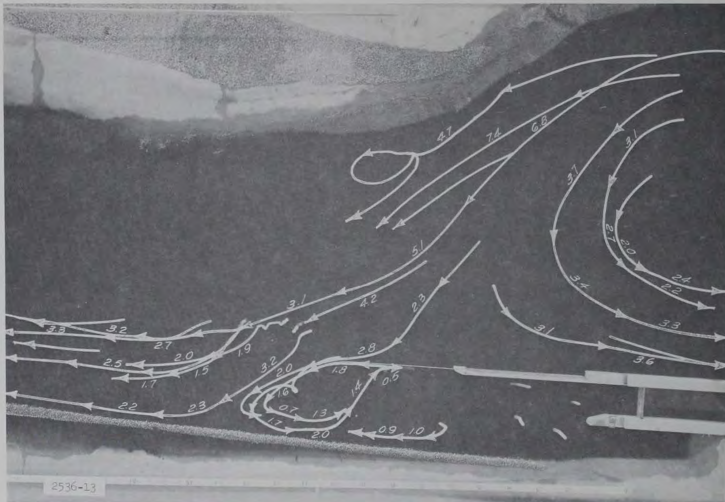
Photograph 5. Paths of floats (submerged 9 ft) during the period 22-33 min after start of powerhouse release. Powerhouse discharge increased from 0 to 50,000 cfs in 25 min (prototype). Numbers indicate average velocity in feet per second during 11-min period
