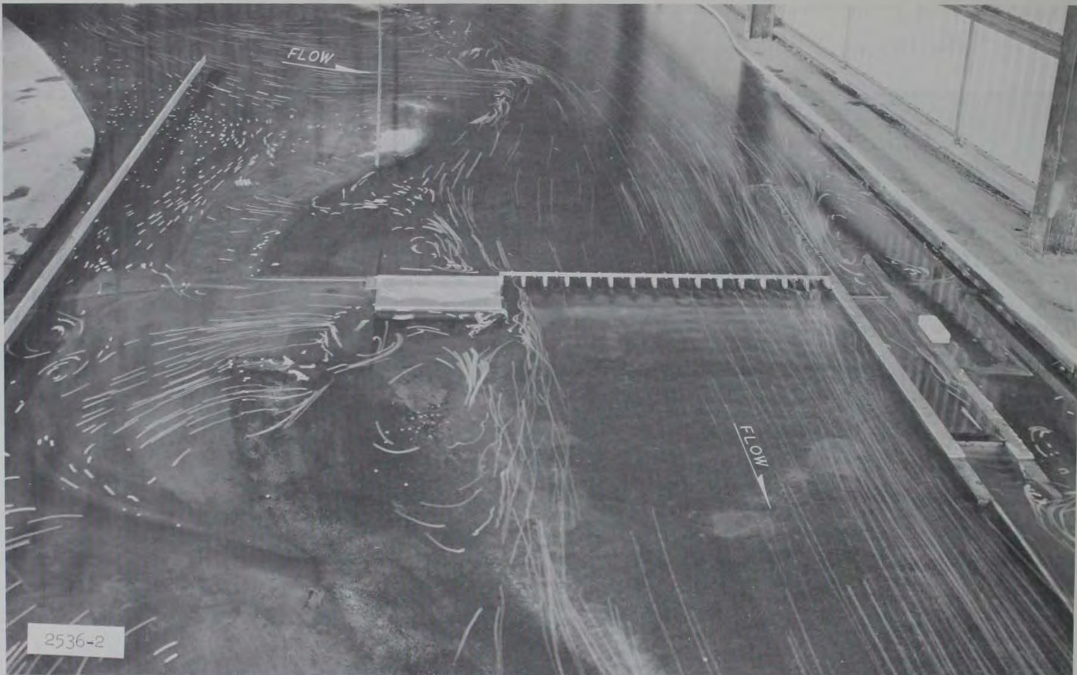
Photograph 11. Discharge 920,000 cfs; surface currents in vicinity of the structures with the right bank access road in place
