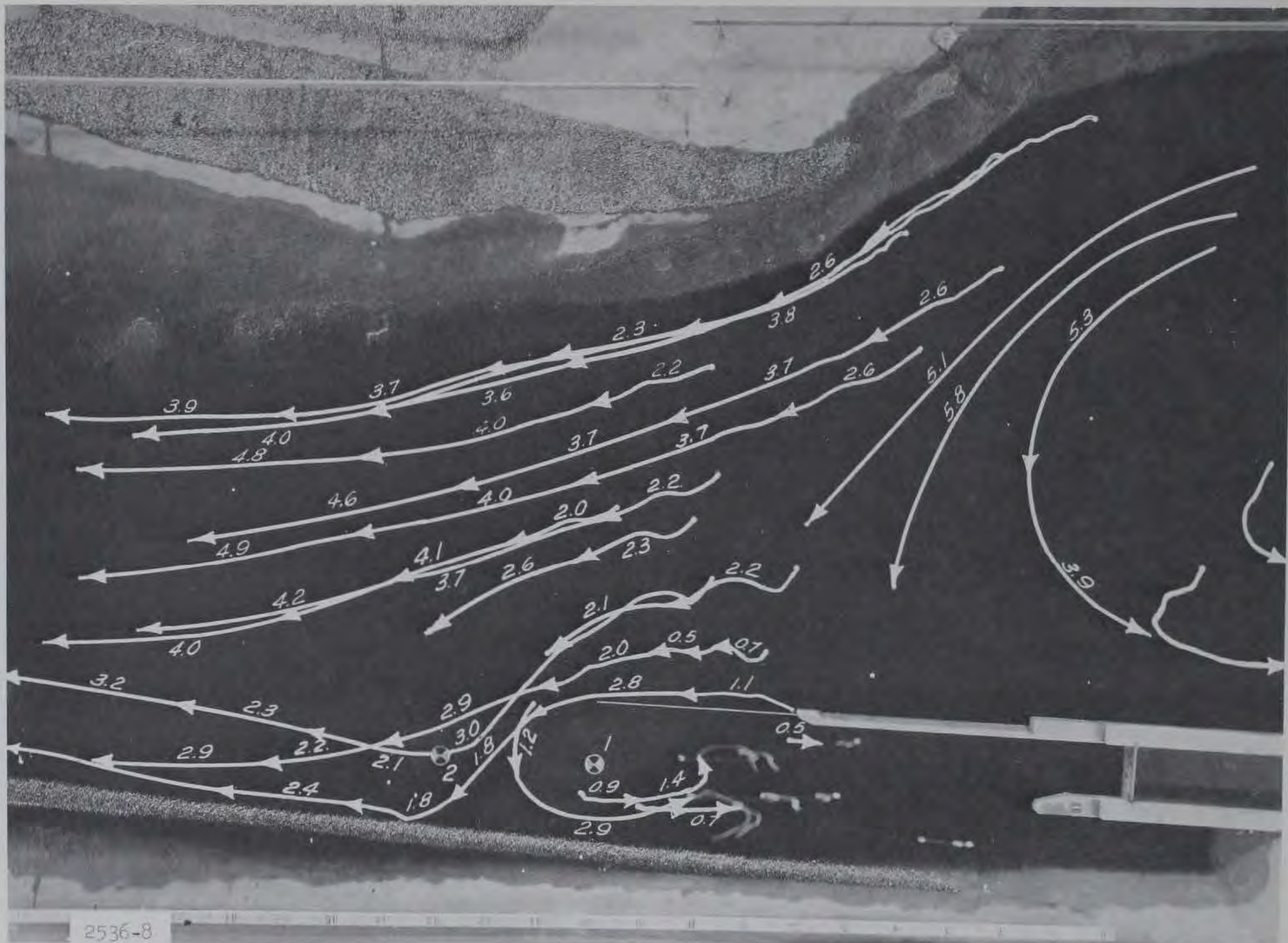
Photograph 1. Paths of floats (submerged 9 ft) during period 0-11 min after start of powerhouse release. Powerhouse discharge increased from 0 to 50,000 cfs in 6 sec (prototype). Numbers indicate average velocity in feet per second during 11-min period
