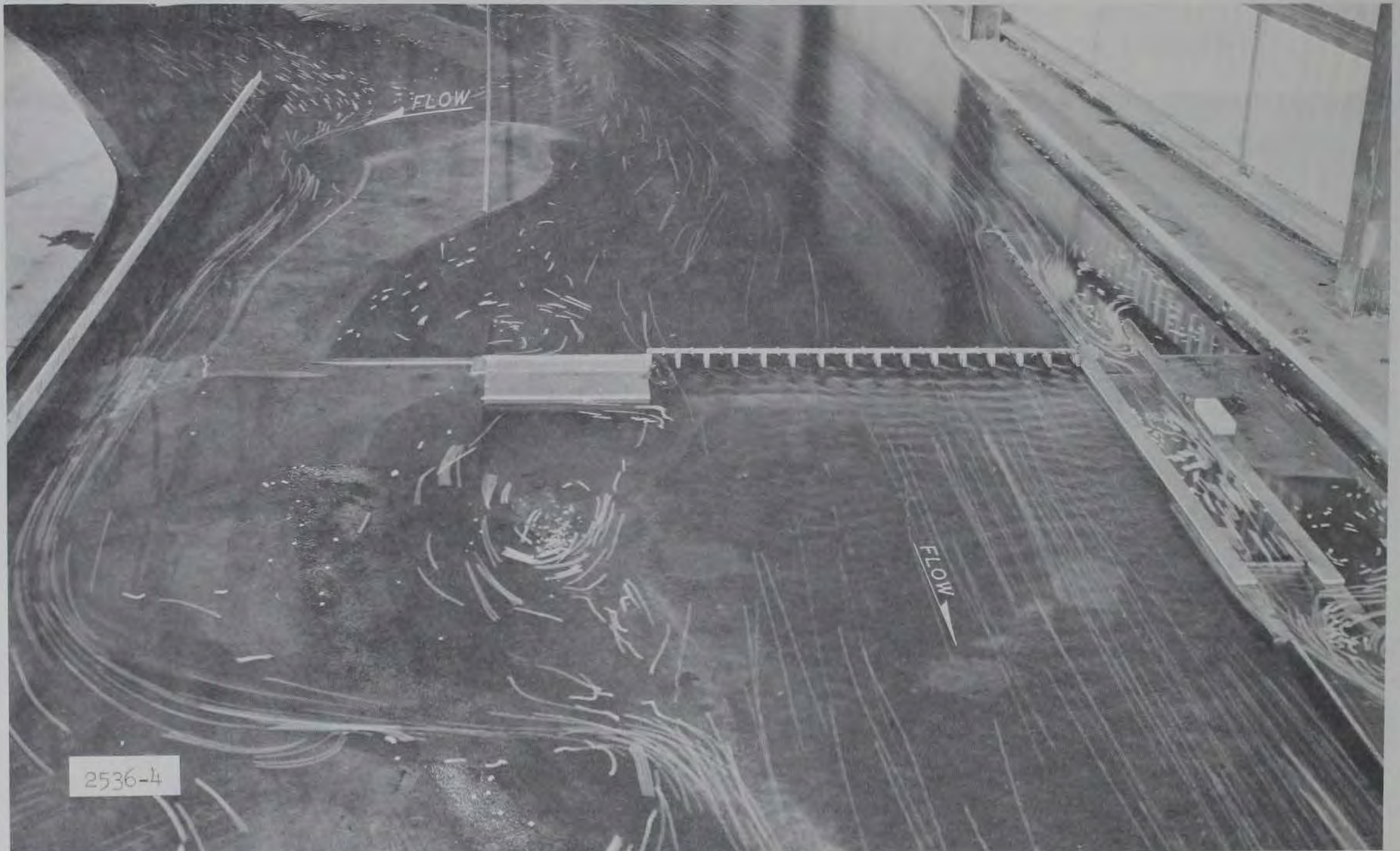
Photograph 13. Discharge 800,000 cfs; surface currents in vicinity of the structures with the right bank access road removed
