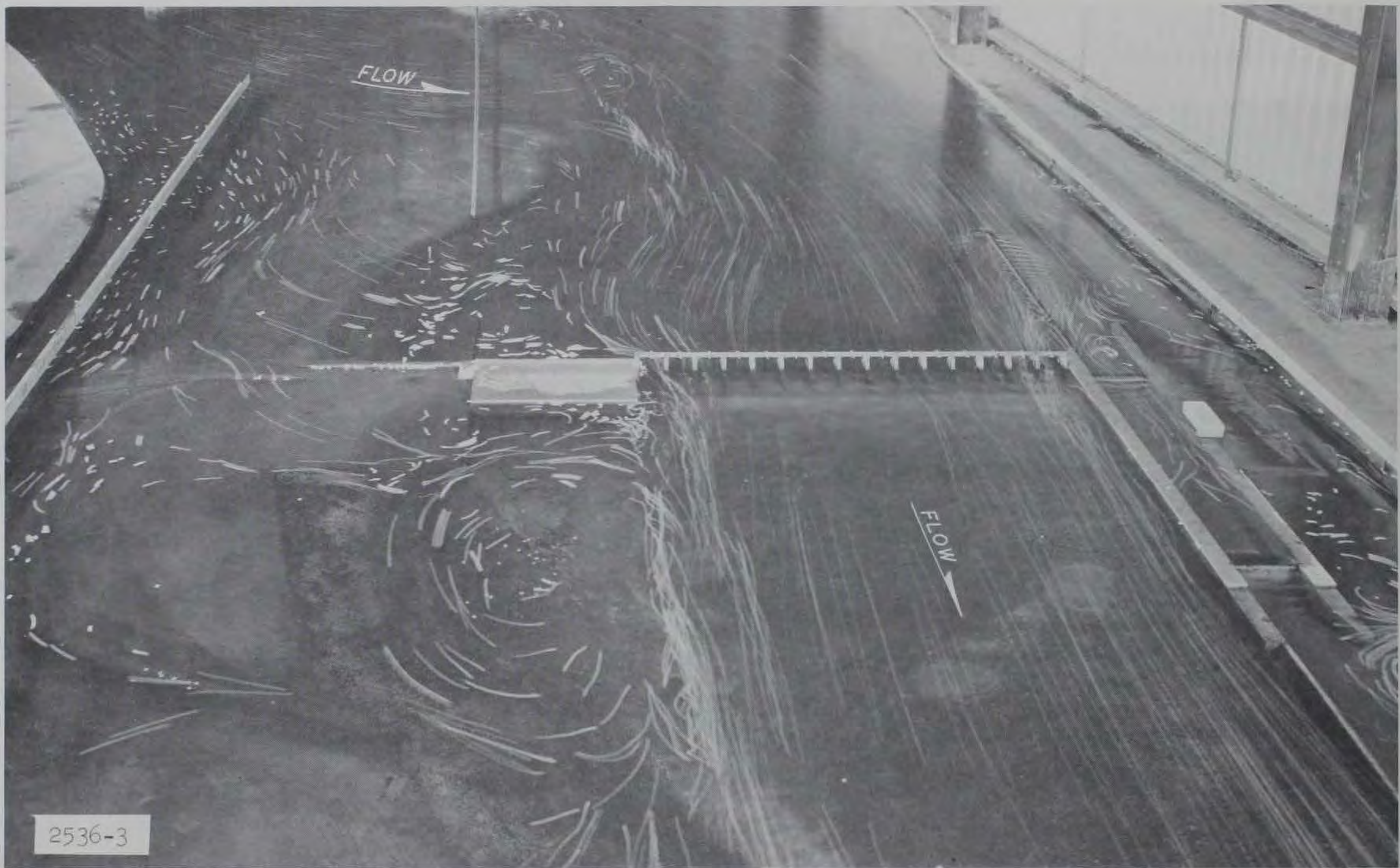
Photograph 12. Discharge 1,000,000 cfs; surface currents in vicinity of the structures with the right bank access road in place
