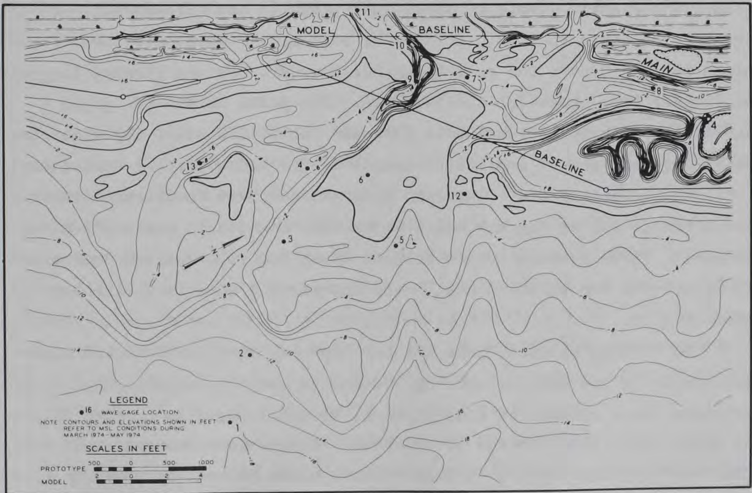
Figure 23. Wave gage locations, base conditions, plan 7
