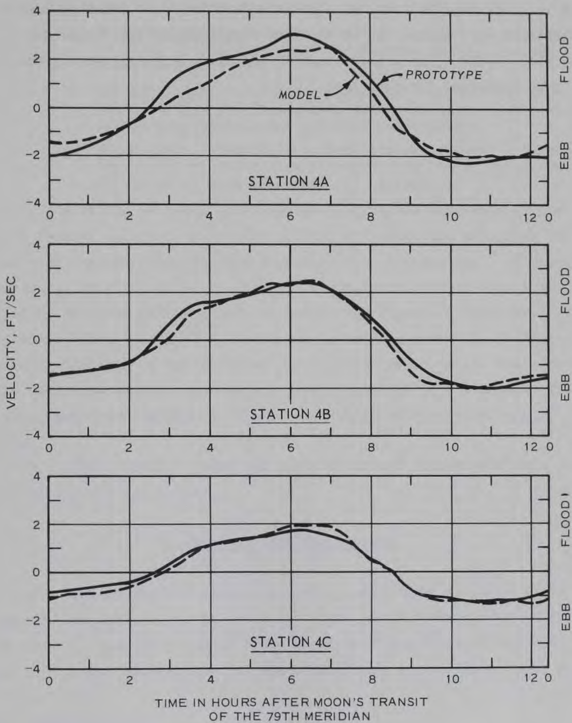
Figure 16. Verification of model velocities, middepth
