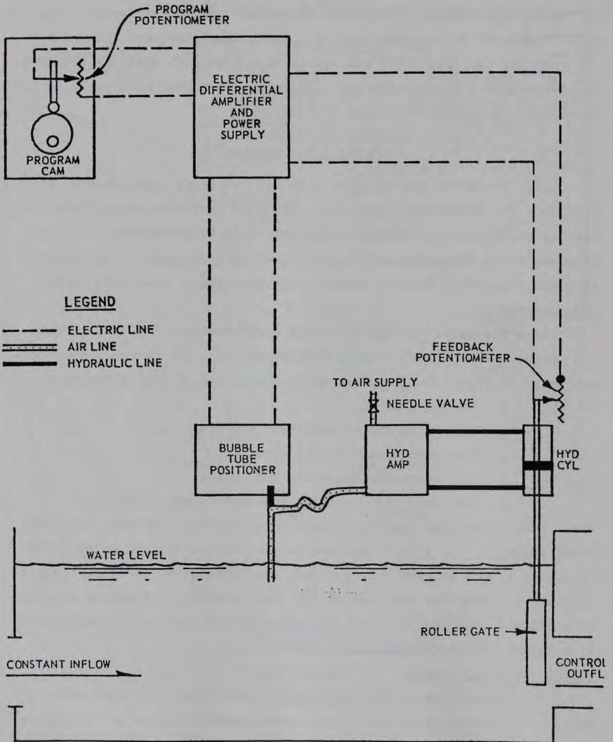
Figure 8. Automatic tide generator
