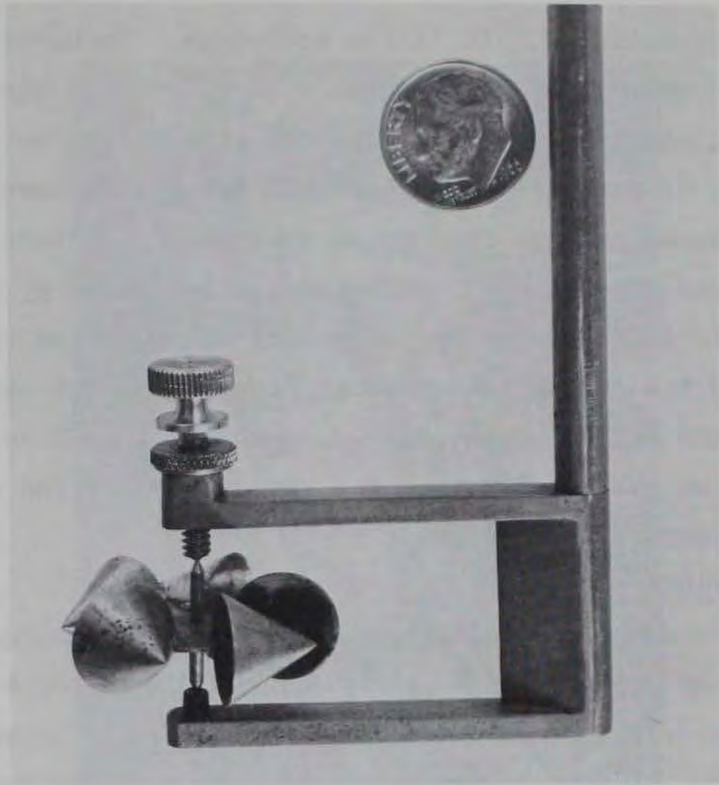
Figure 9. Miniature current velocity meter
