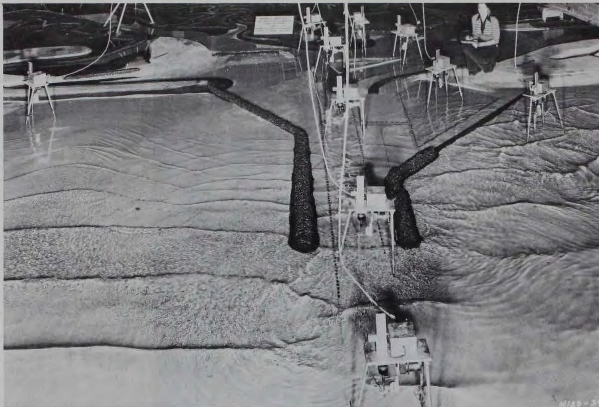
Figure 12. Wave gages
