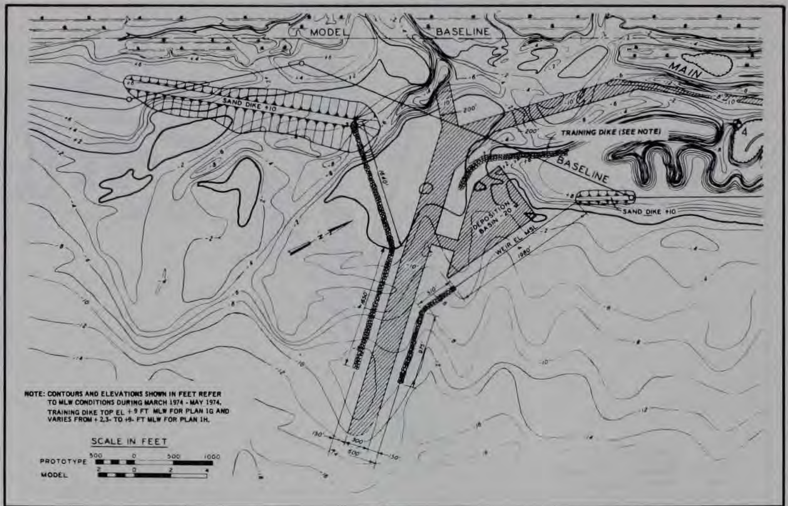
Figure 30. Plans 1G and 1H
