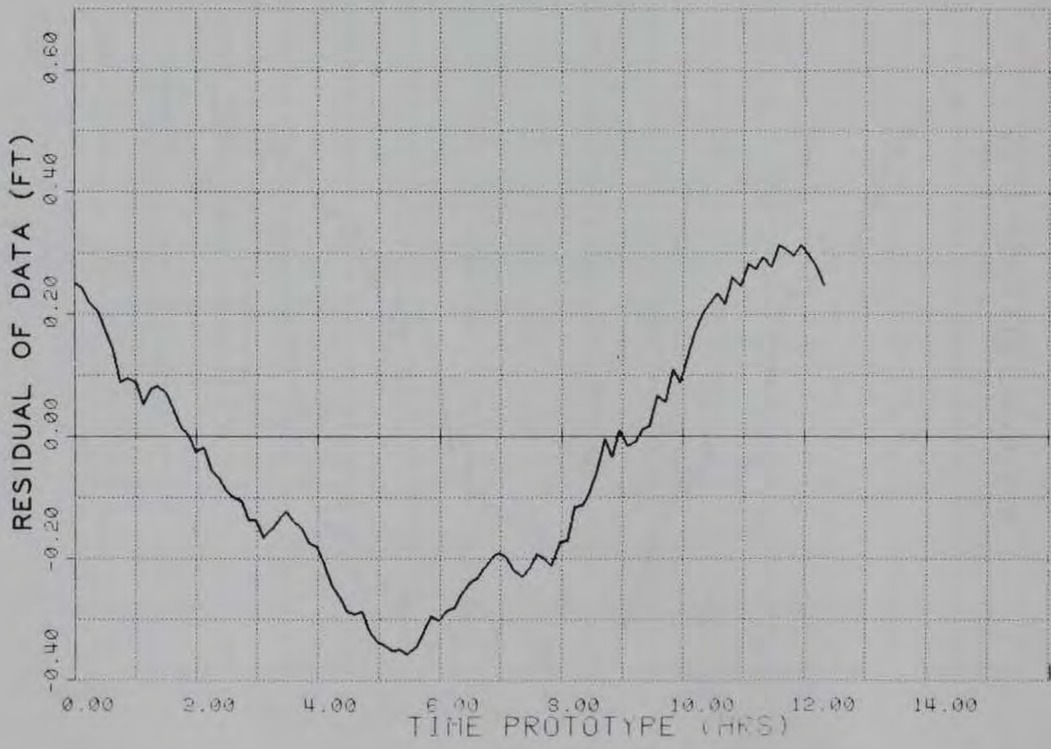
TIDAL ELEVATIONS COMPARISON OF PLAN 1 TO BASE GAGE 3
