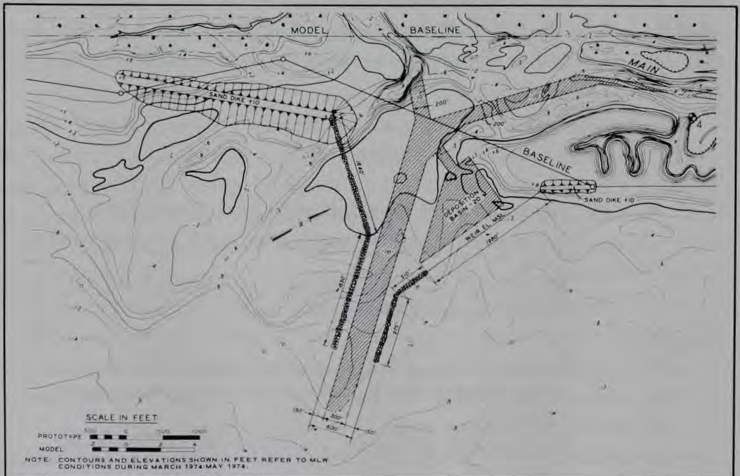
Figure 24. Plan 1D
