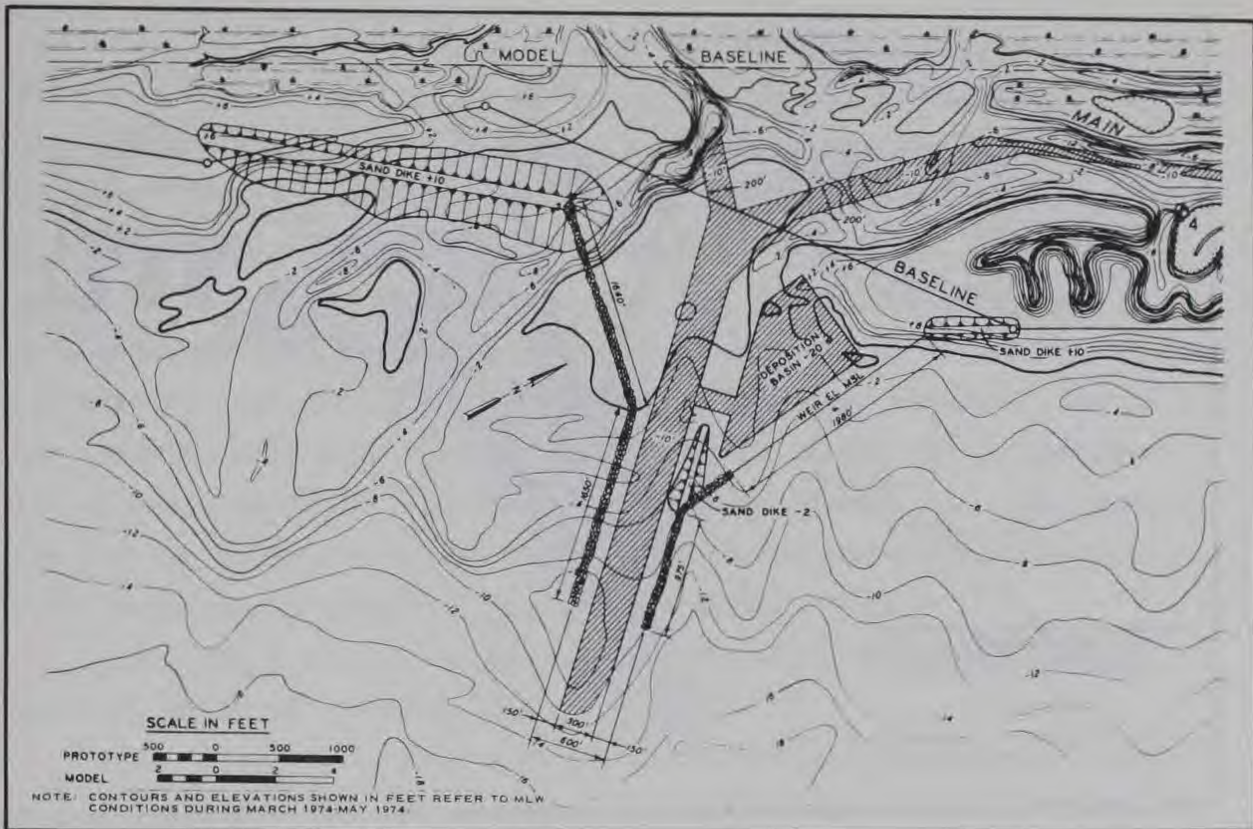
Figure 29. Plan 1F
