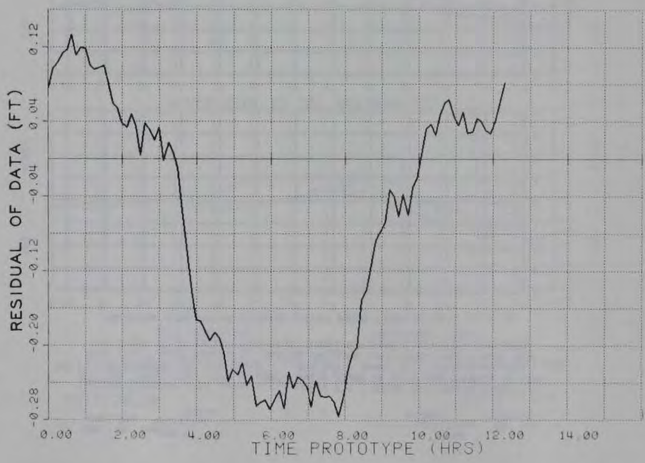
TIDAL ELEVATIONS COMPARISON OF PLAN 1 TO BASE GAGE 1
