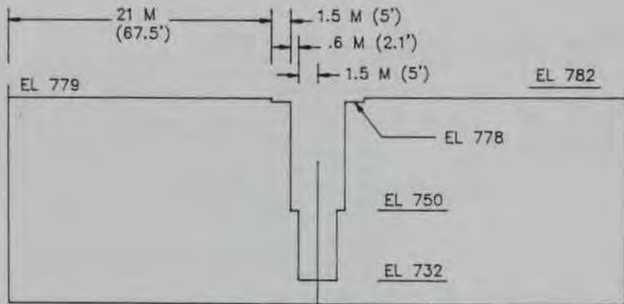
TYPE 6 WEIR - ELEVATION
