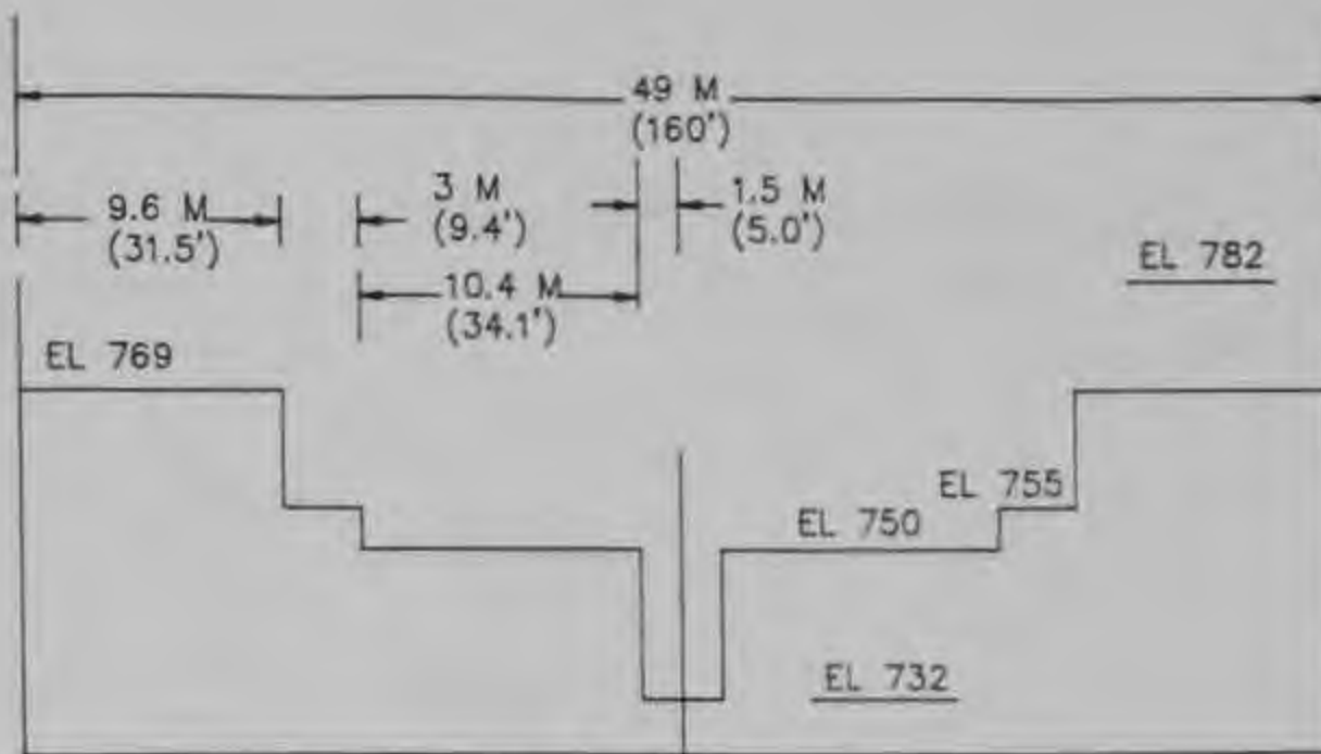
TYPE 8 WEIR - ELEVATION
