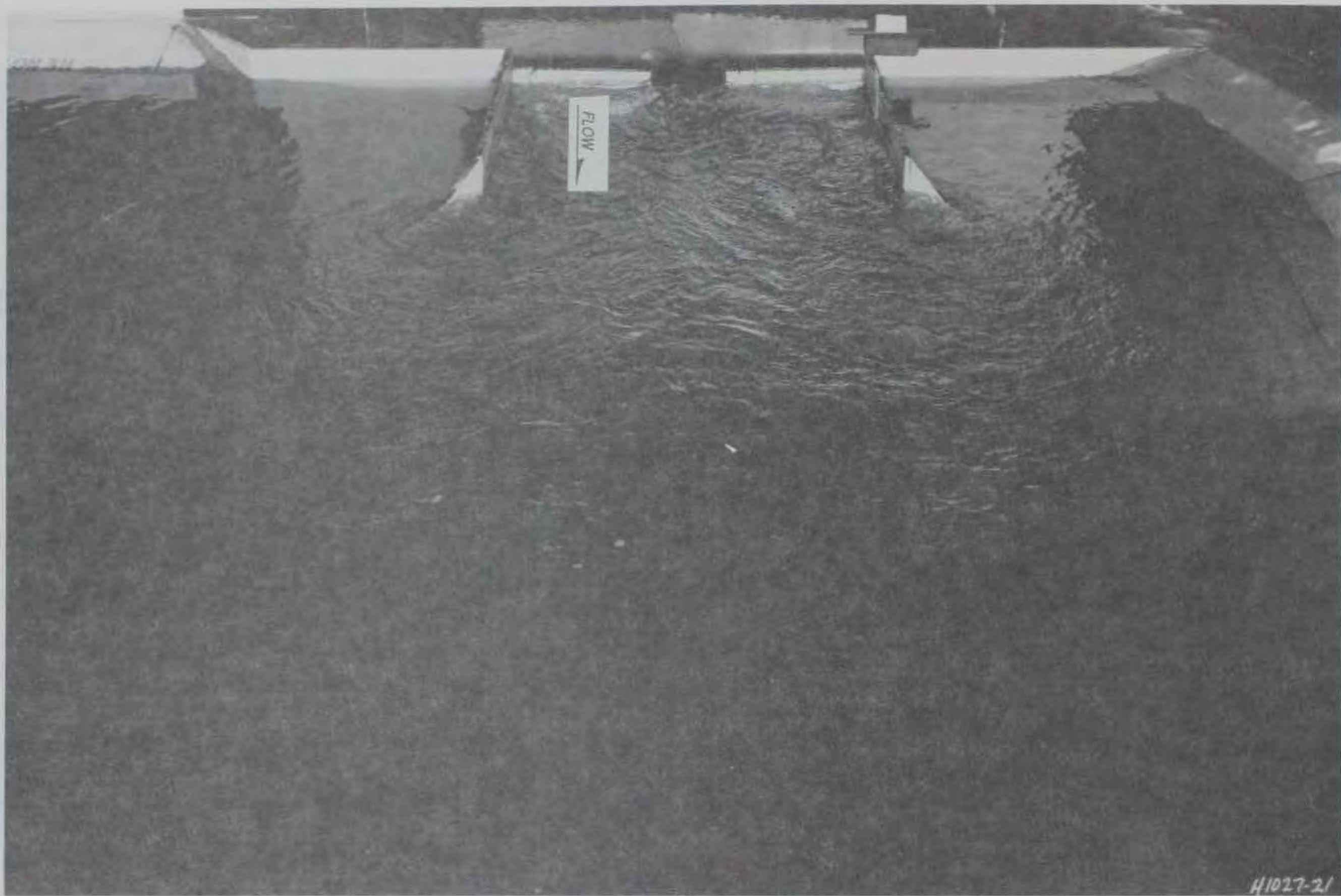
Photo 2. Type 23 weir, discharge 1,557 cu m/sec (55,000 cfs), tailwater el 766.71
