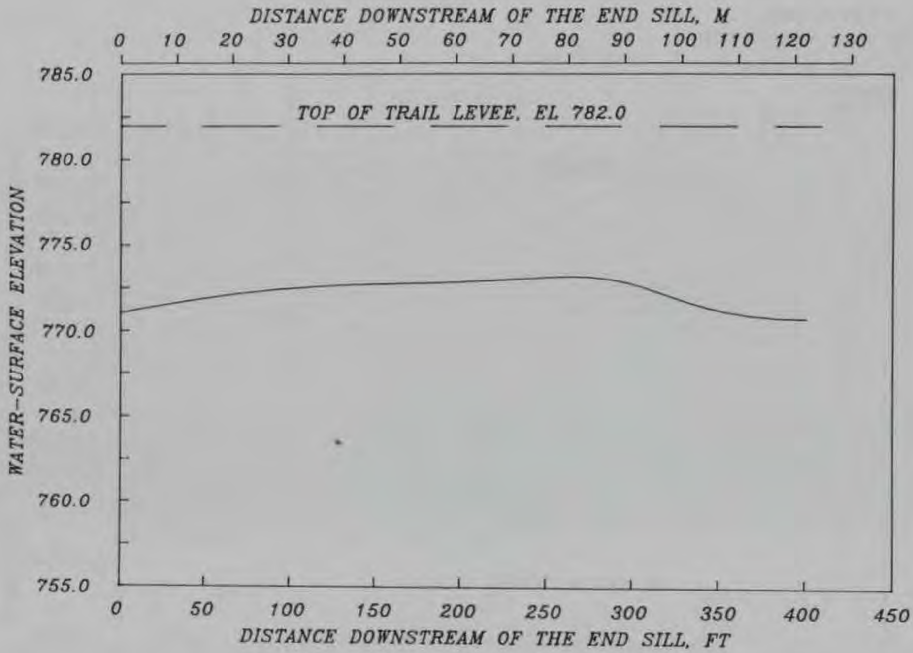
TRAIL LEVEE - WATER-SURFACE PROFILE DISCHARGE 1,557 CU M/SEC (55,000 CFS) TAILWATER EL 766.71
