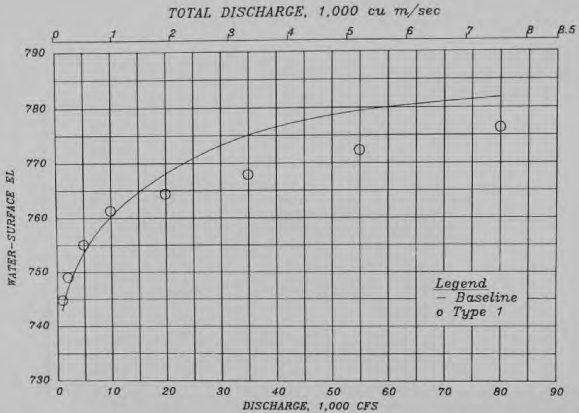
TYPE 1 WEIR STAGE-DISCHARGE CURVE STA 113+50
