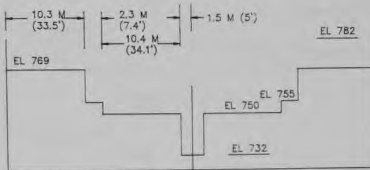
TYPE 9 WEIR - ELEVATION
