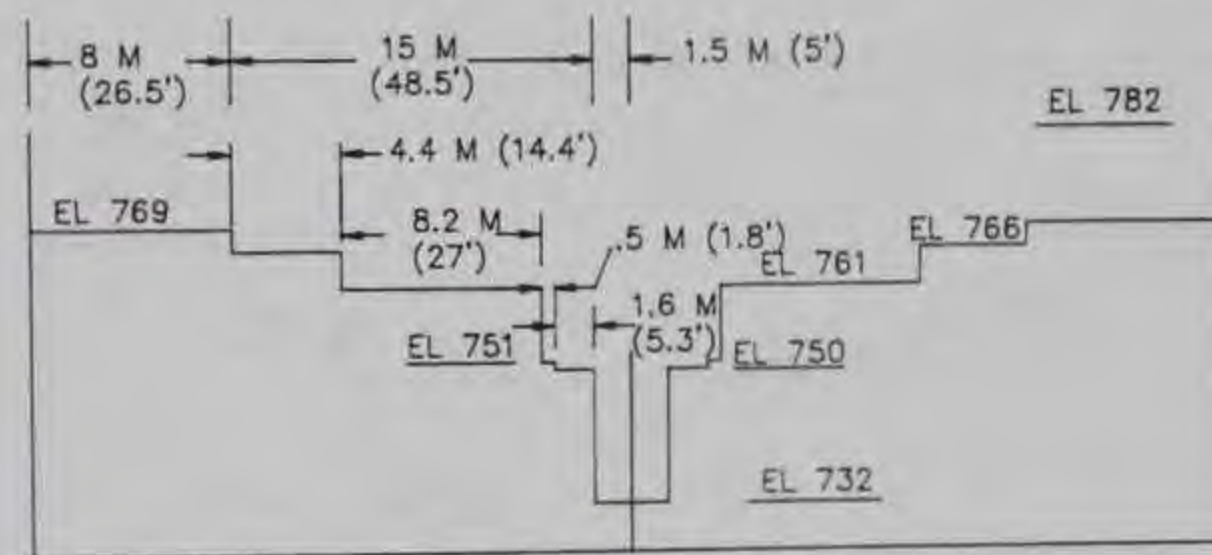
TYPE 4 WEIR - ELEVATION
