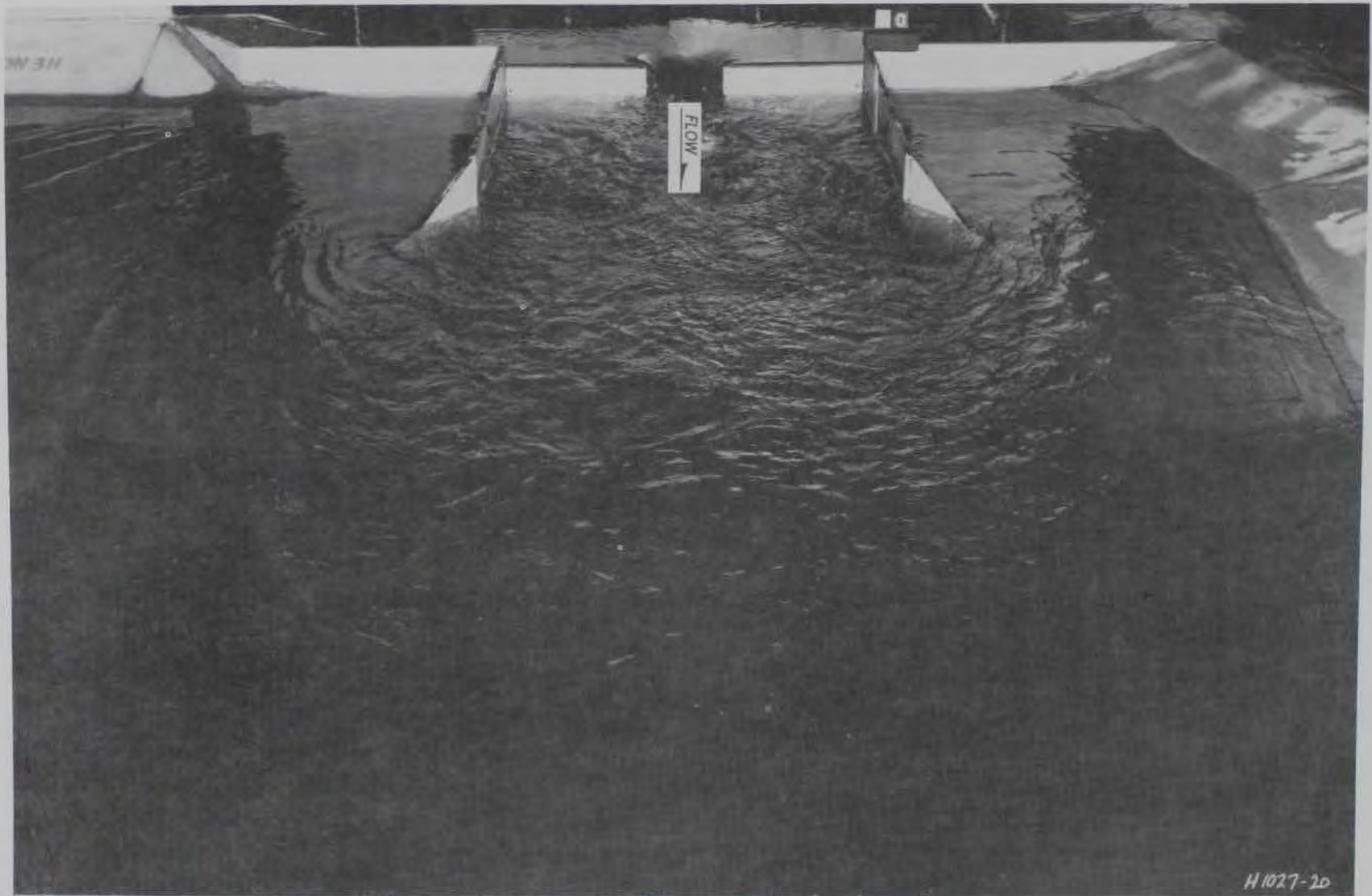
Photo 1. Type 23 weir, discharge 991 cu m/sec (35,000 cfs), tailwater el 759.71
