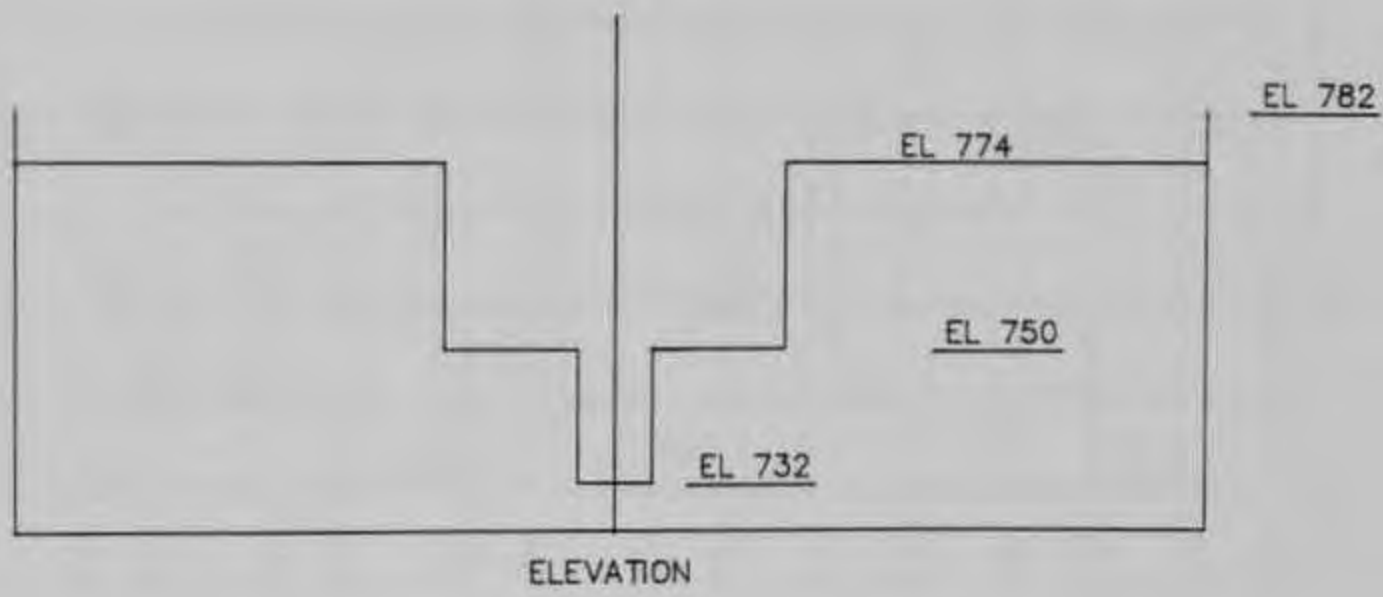
TYPE 21 WEIR DESIGN
