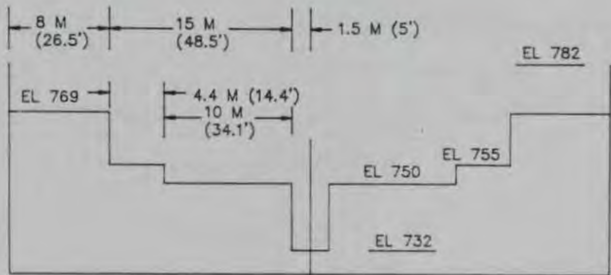
TYPE 7 WEIR - ELEVATION
