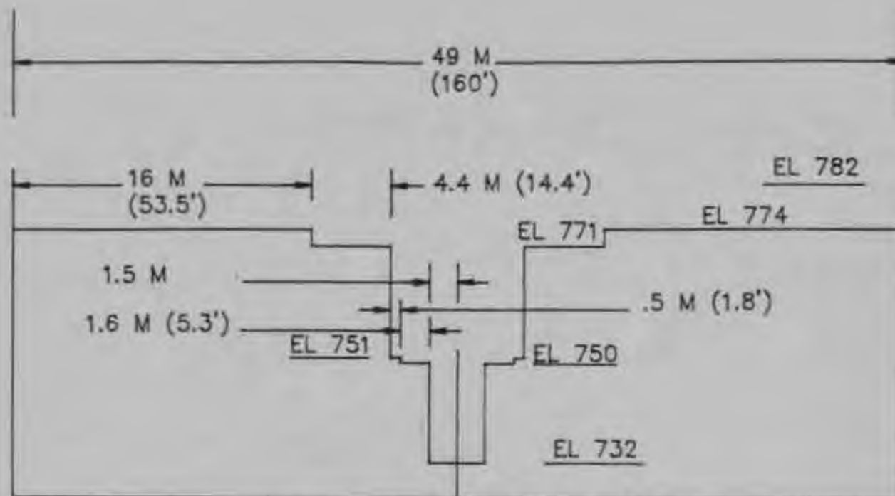
TYPE 5 WEIR - ELEVATION
