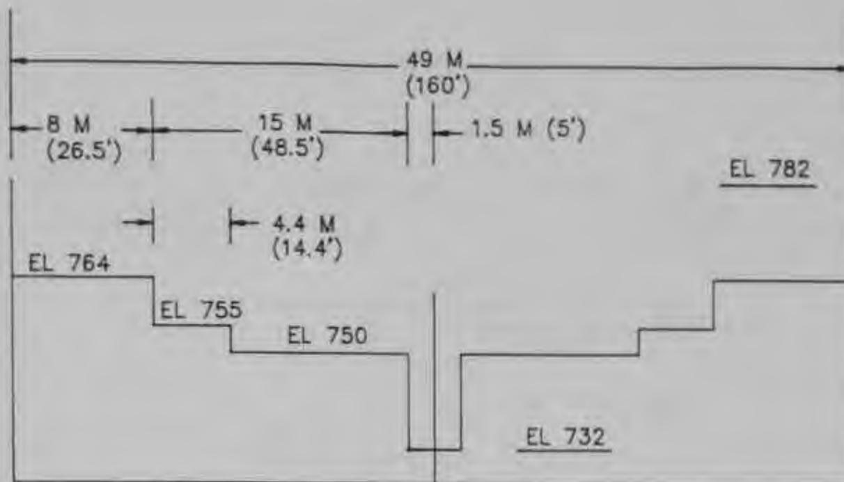
TYPE 2 WEIR - ELEVATION
