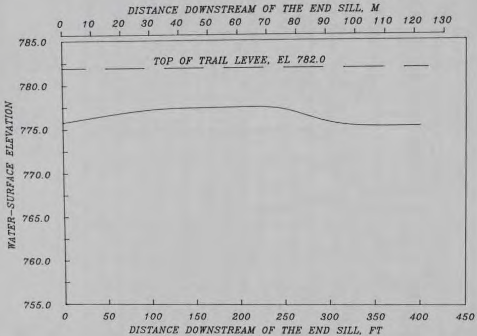
TRAIL LEVEE WATER-SURFACE PROFILE DISCHARGE 2,265 CU M/SEC (80,000 CFS) TAILWATER EL 772.28
