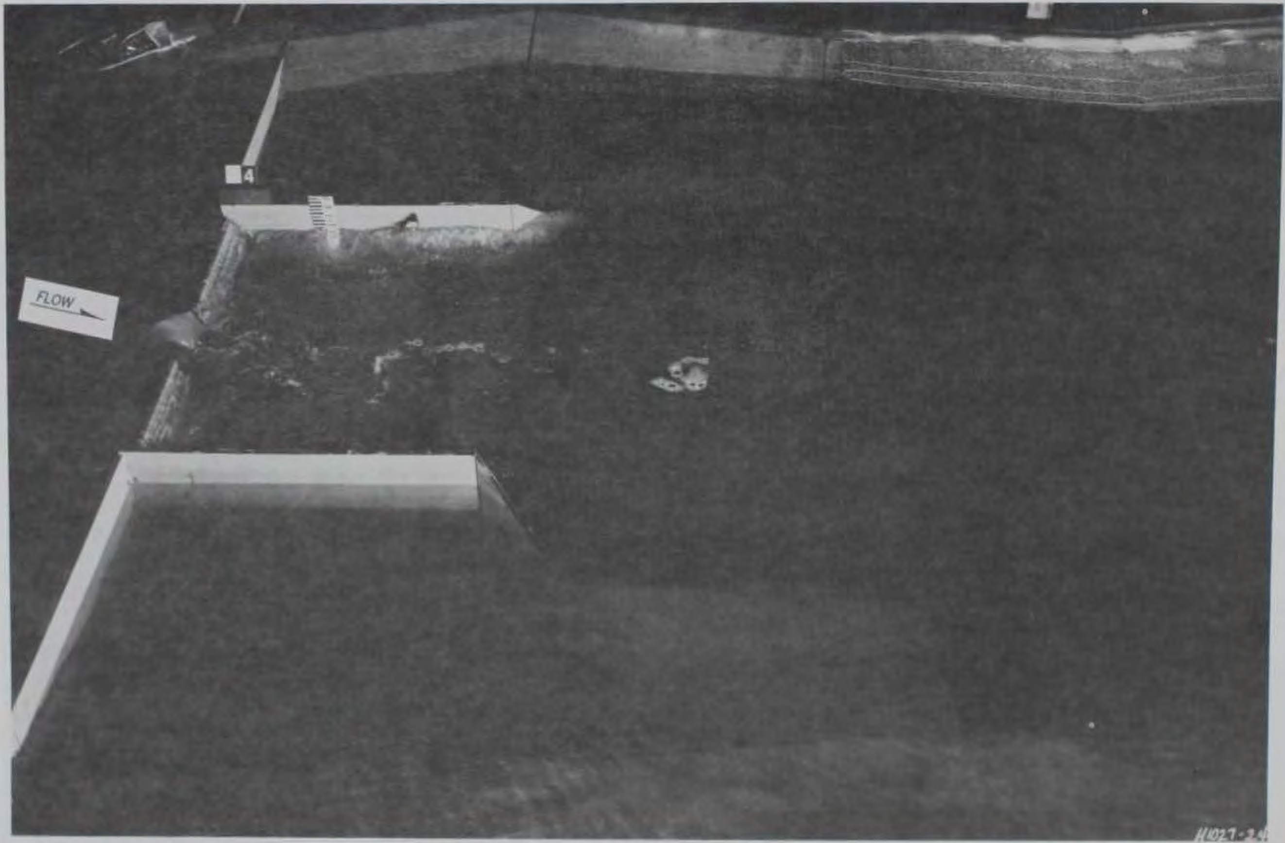
Photo 5. Type 23 weir, basin flow, discharge 1,557 cu m/sec (55,000 cfs), tailwater el 766.71
