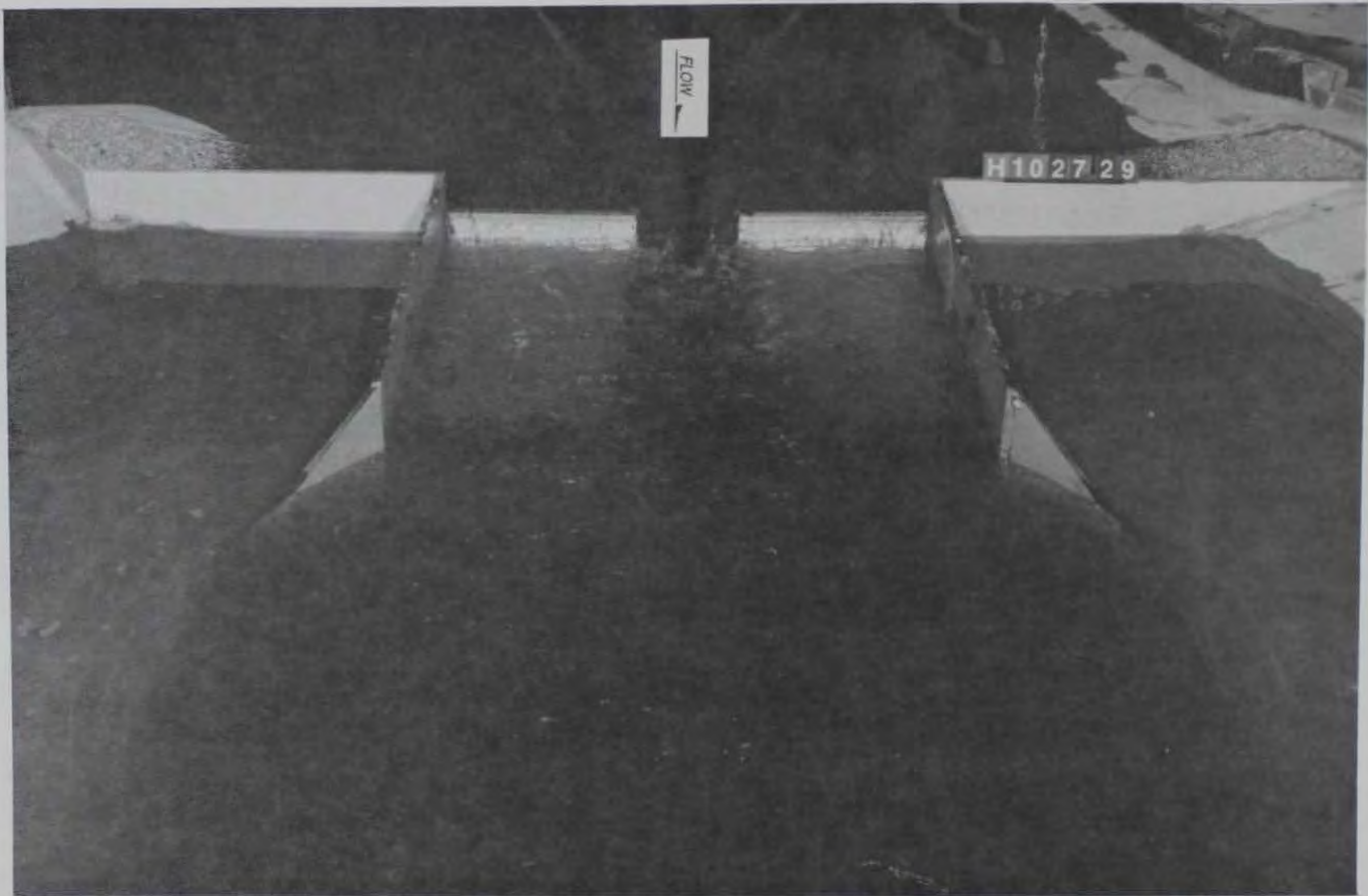
Photo 7. Type 25 weir, weir flow, discharge 991 cu m/sec (35,000 cfs), tailwater el 759.71
