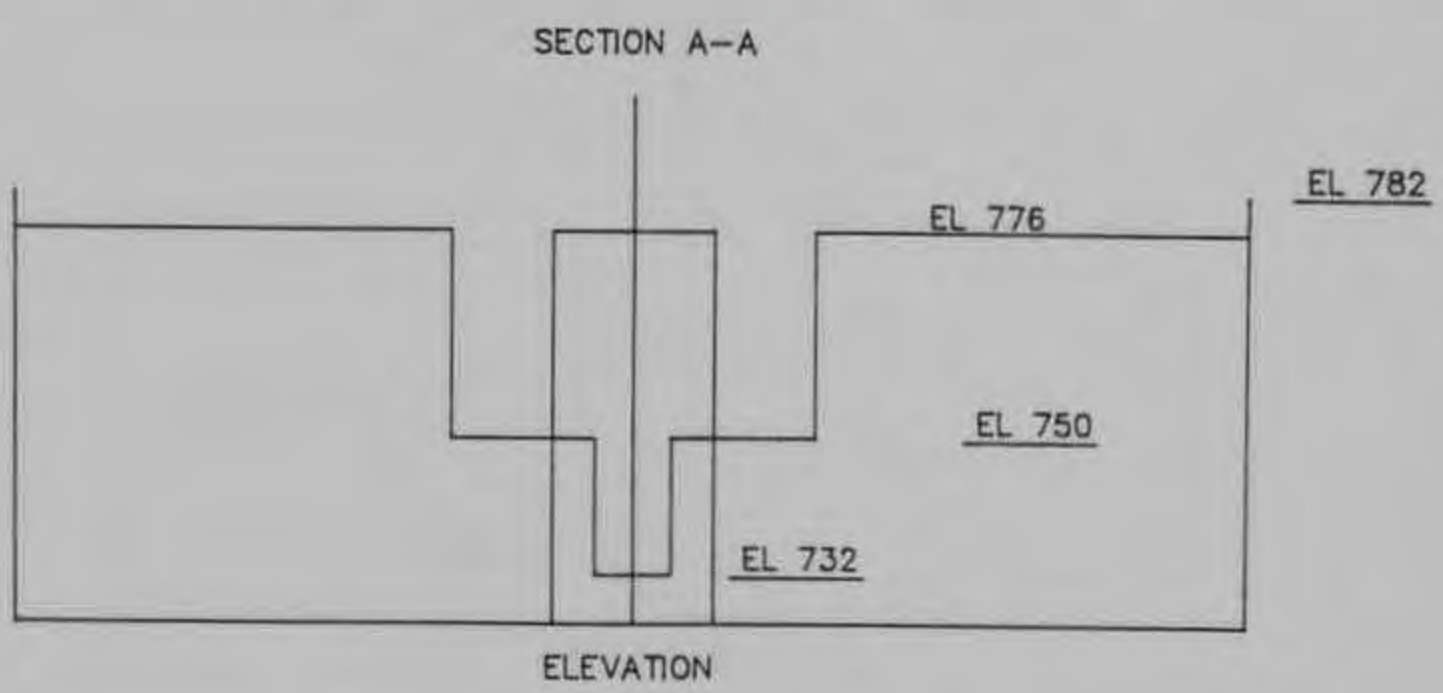
TYPE 18 WEIR DESIGN
