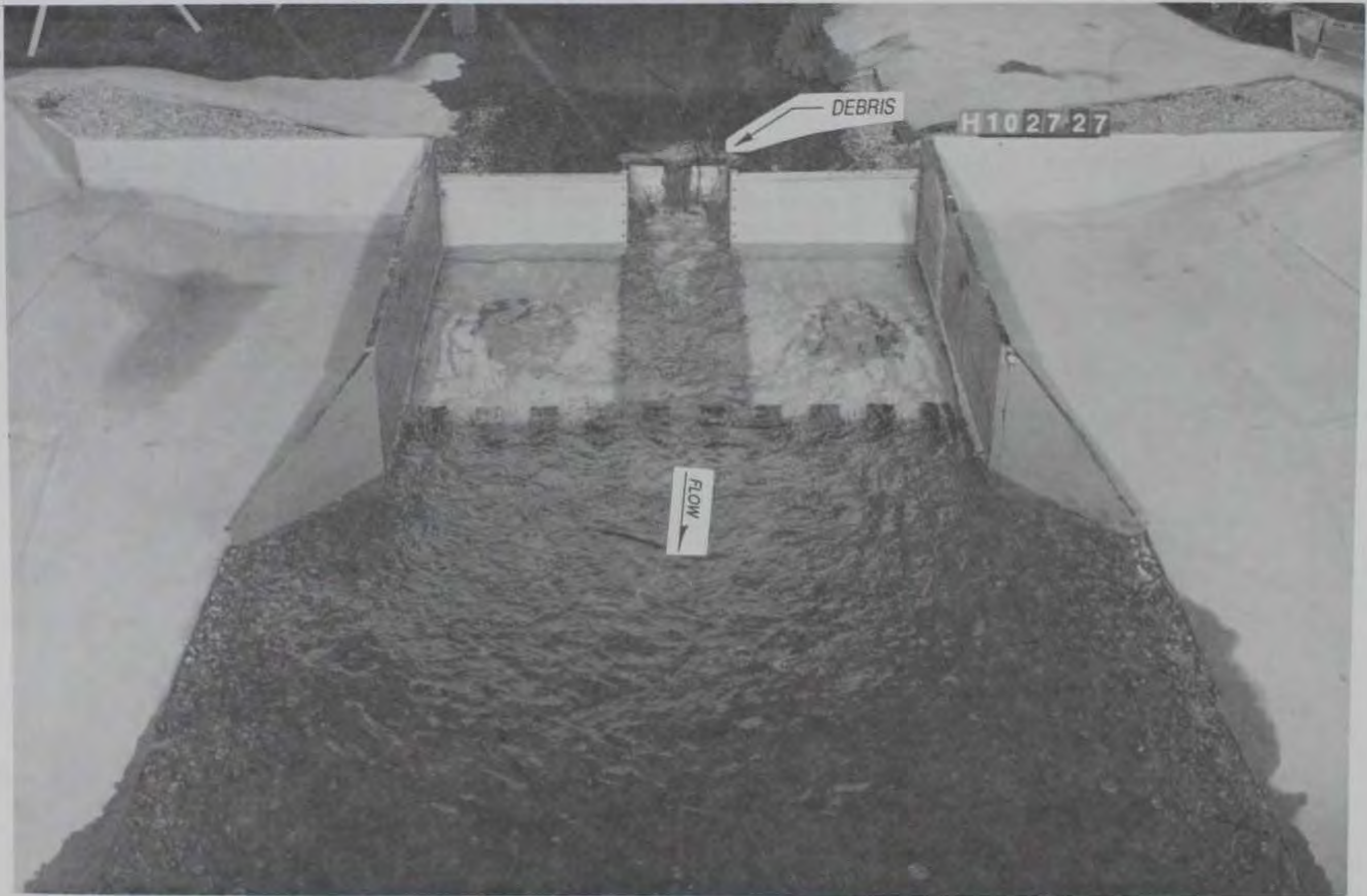
Photo 11. Type 2 debris deflectors, debris passage looking upstream, discharge 142 cu m/sec (5,000 cfs), tailwater el 741.44
