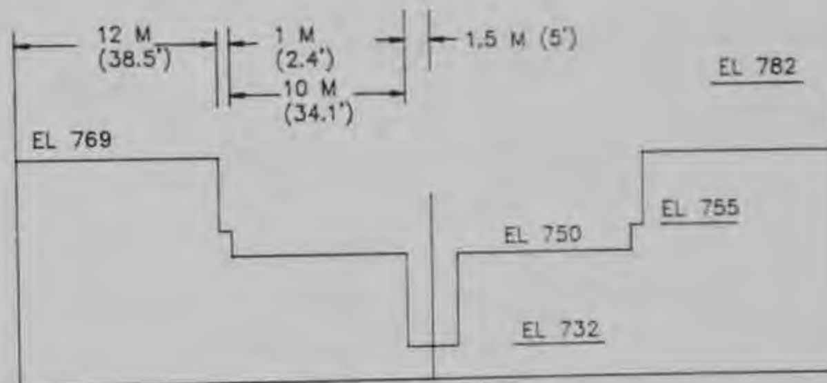
TYPE 10 WEIR - ELEVATION
