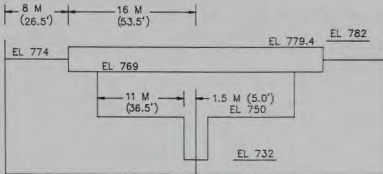
TYPE 12 WEIR - ELEVATION
