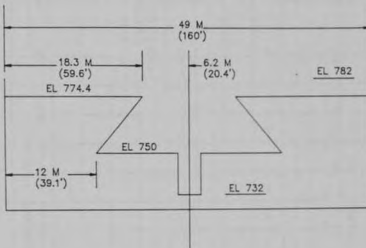
TYPE 14 WEIR - ELEVATION
