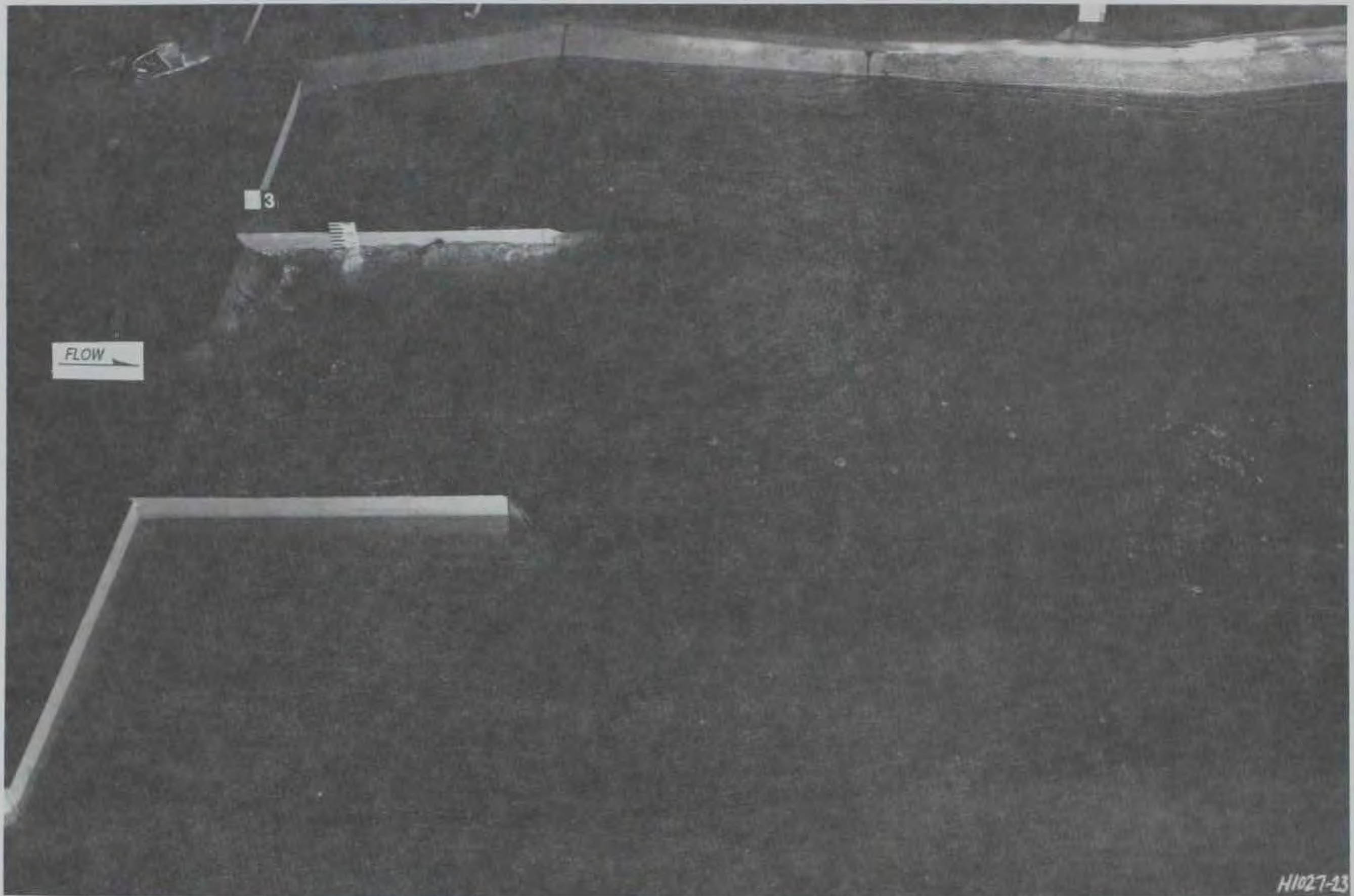
Photo 6. Type 23 weir, basin flow, discharge 2,265 cu m/sec (80,000 cfs), tailwater el 772.28
