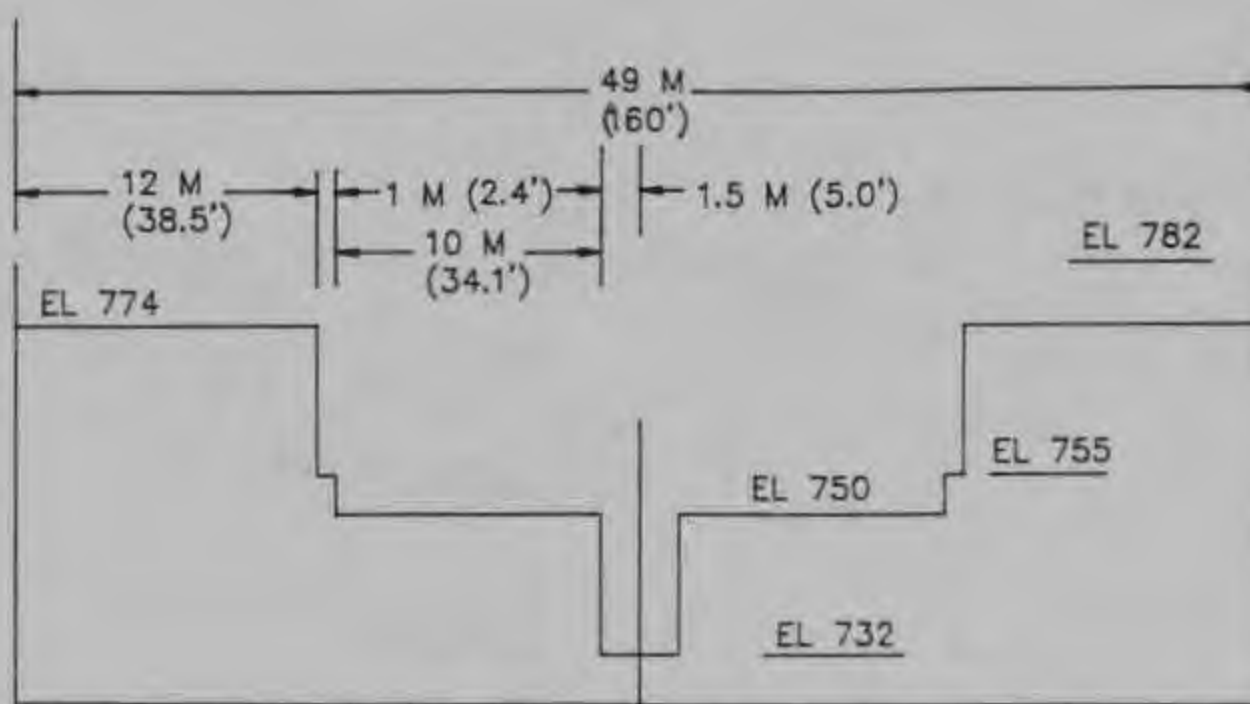
TYPE 11 WEIR - ELEVATION
