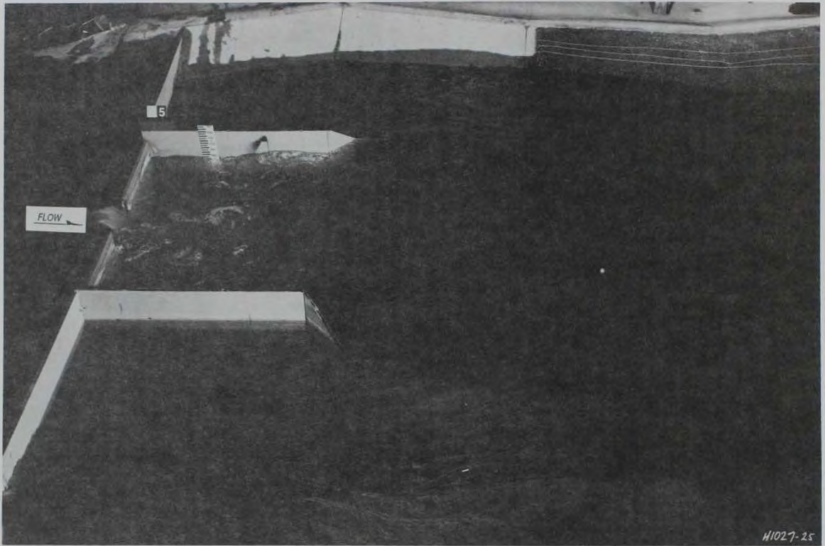
Photo 4. Type 23 weir, basin flow, discharge 991 cu m/sec (35,000 cfs), tailwater el 759.71
