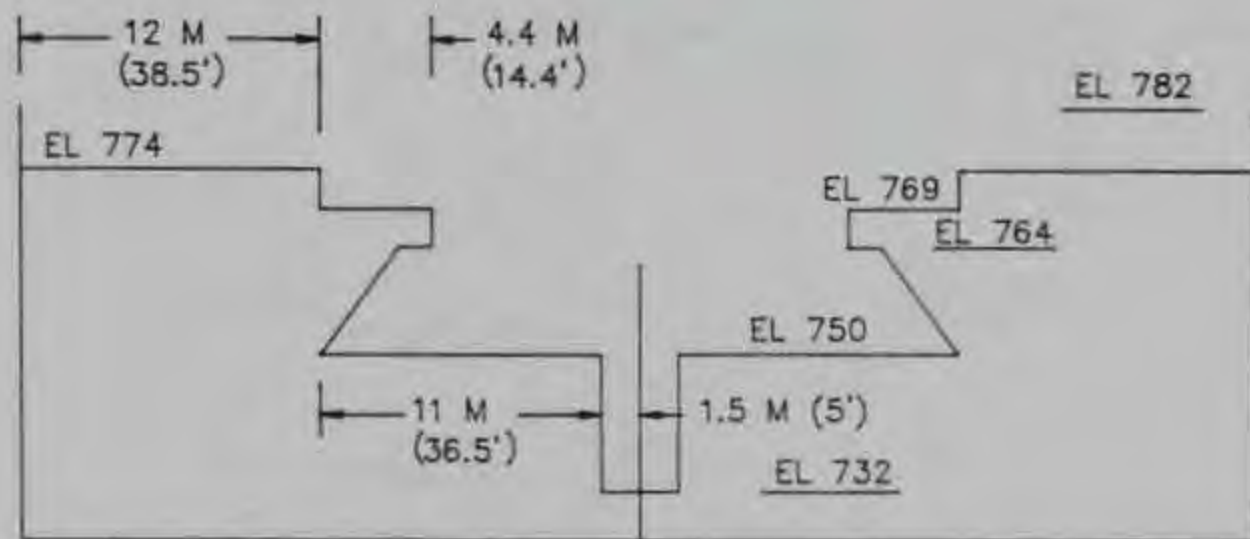
TYPE 13 WEIR - ELEVATION
