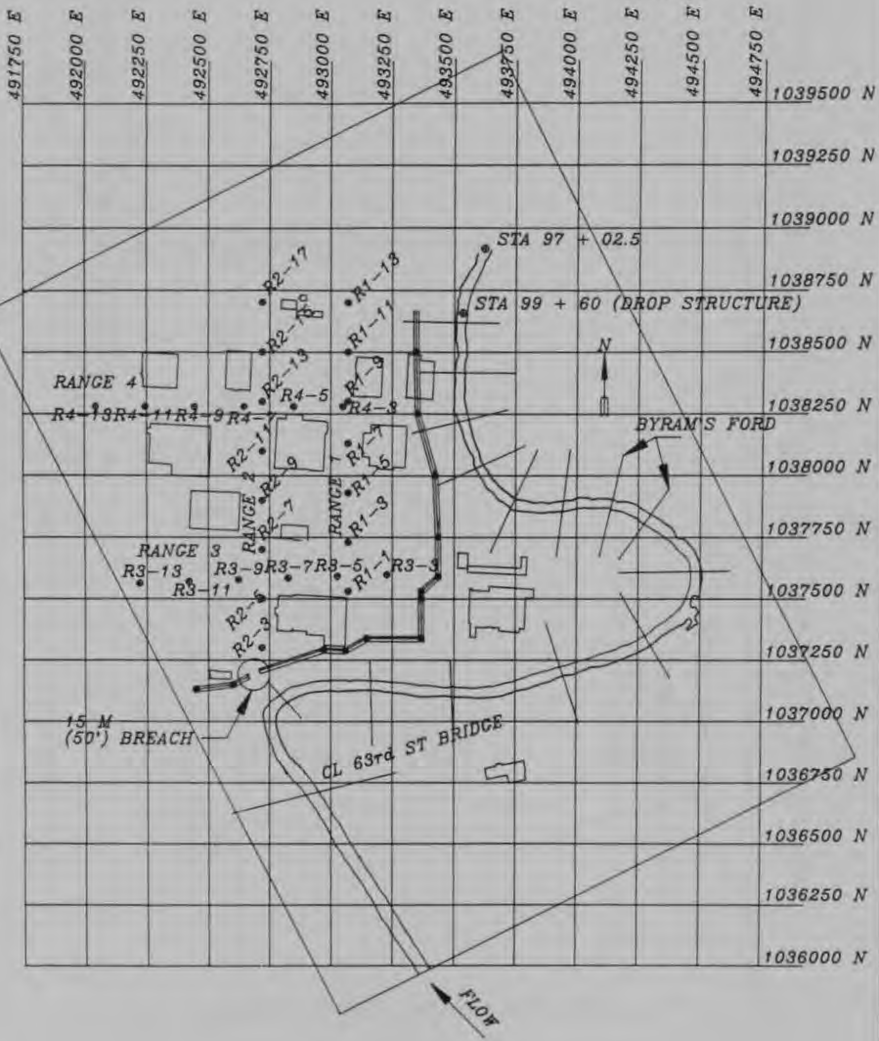
LOCATION OF 15-M (50-FT) BREACHED SECTION
