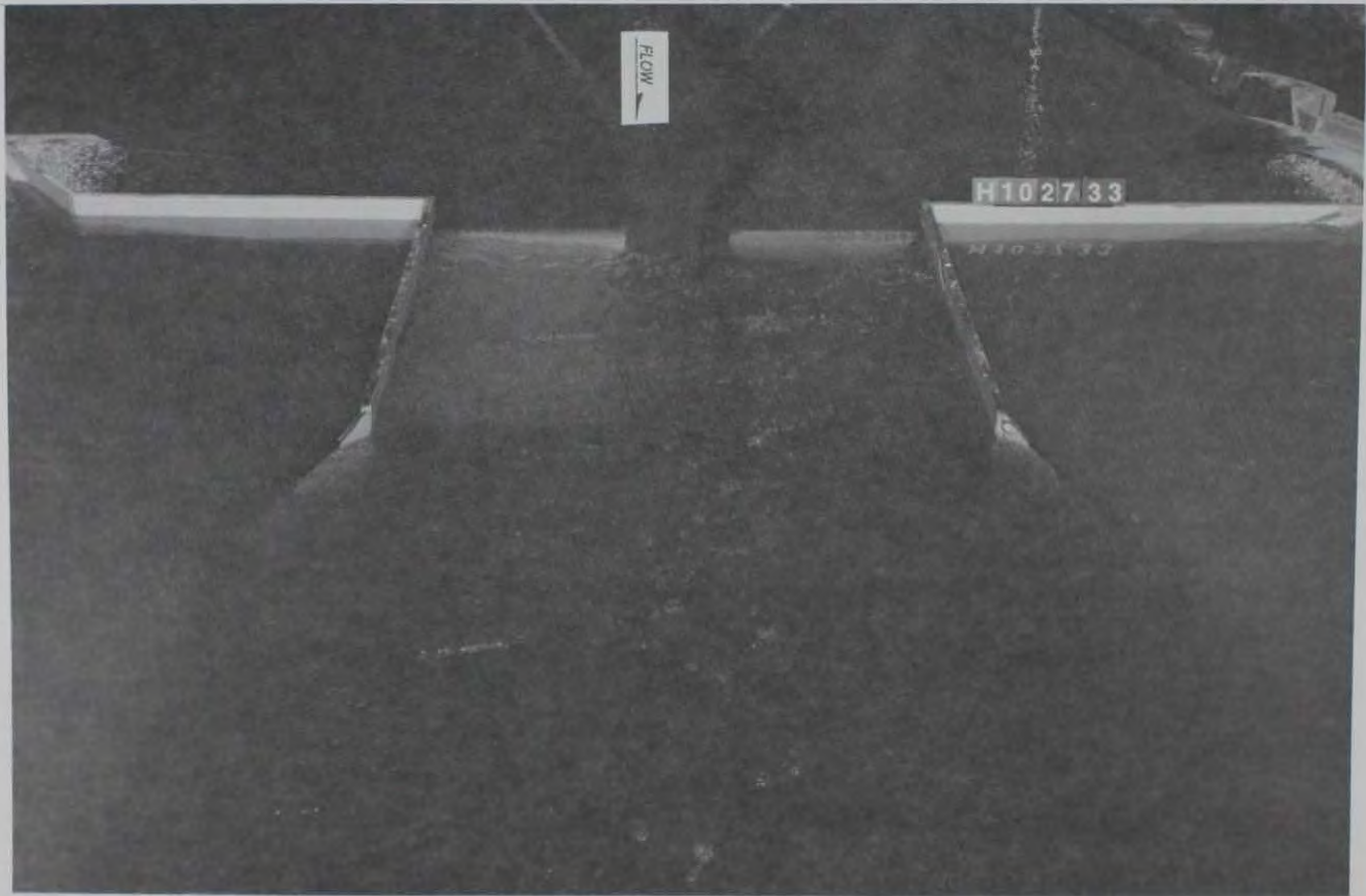
Photo 9. Type 25 weir, weir flow, discharge 2,265 cu m/sec (80,000 cfs), tailwater el 772.28
