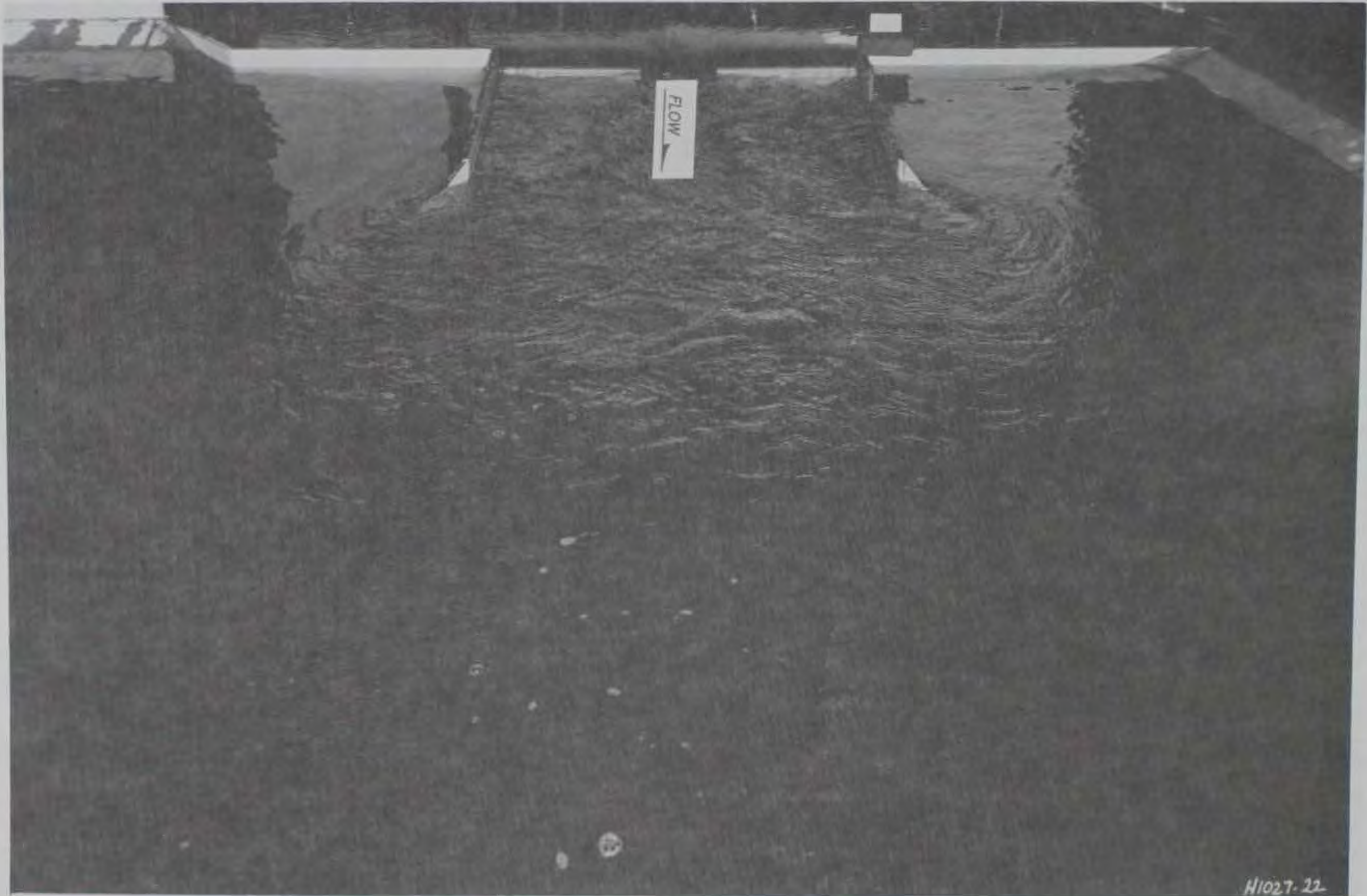
Photo 3. Type 23 weir, discharge 2,265 cu m/sec (80,000 cfs), tailwater el 772.28
