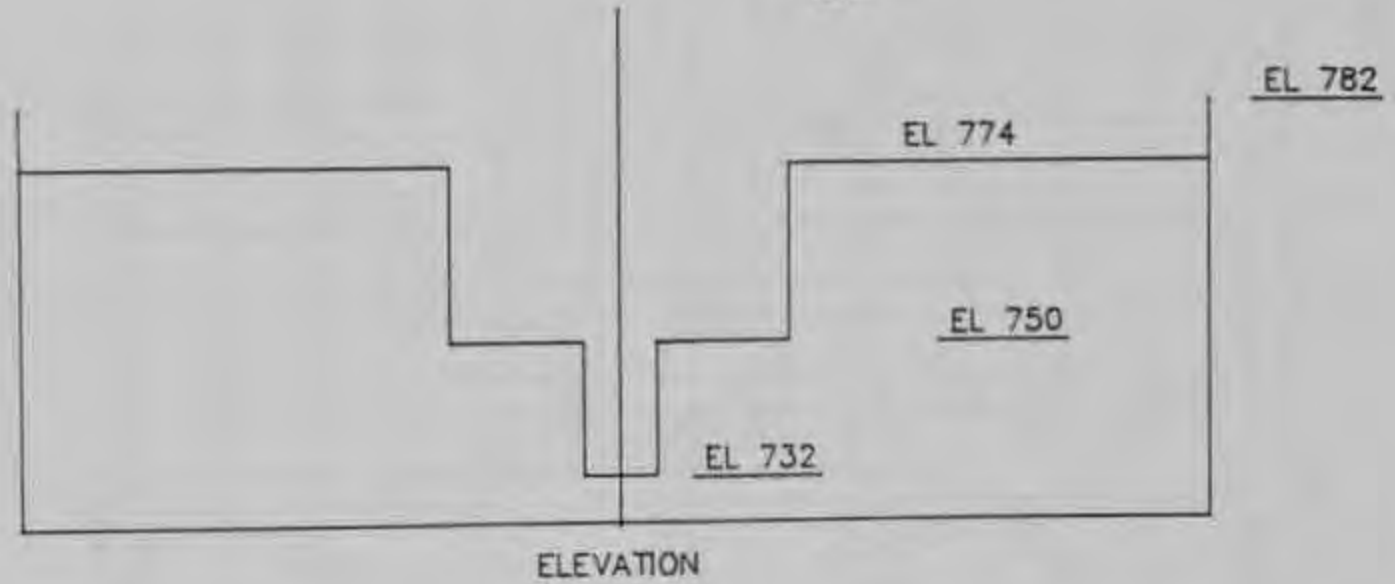
TYPE 23 WEIR DESIGN
