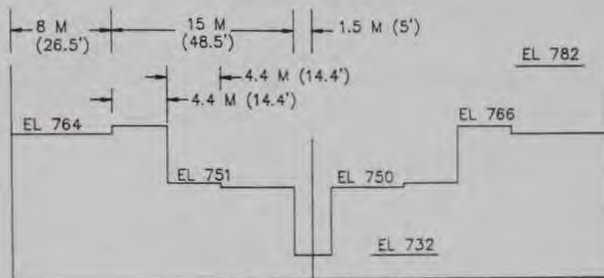
TYPE 3 WEIR - ELEVATION
