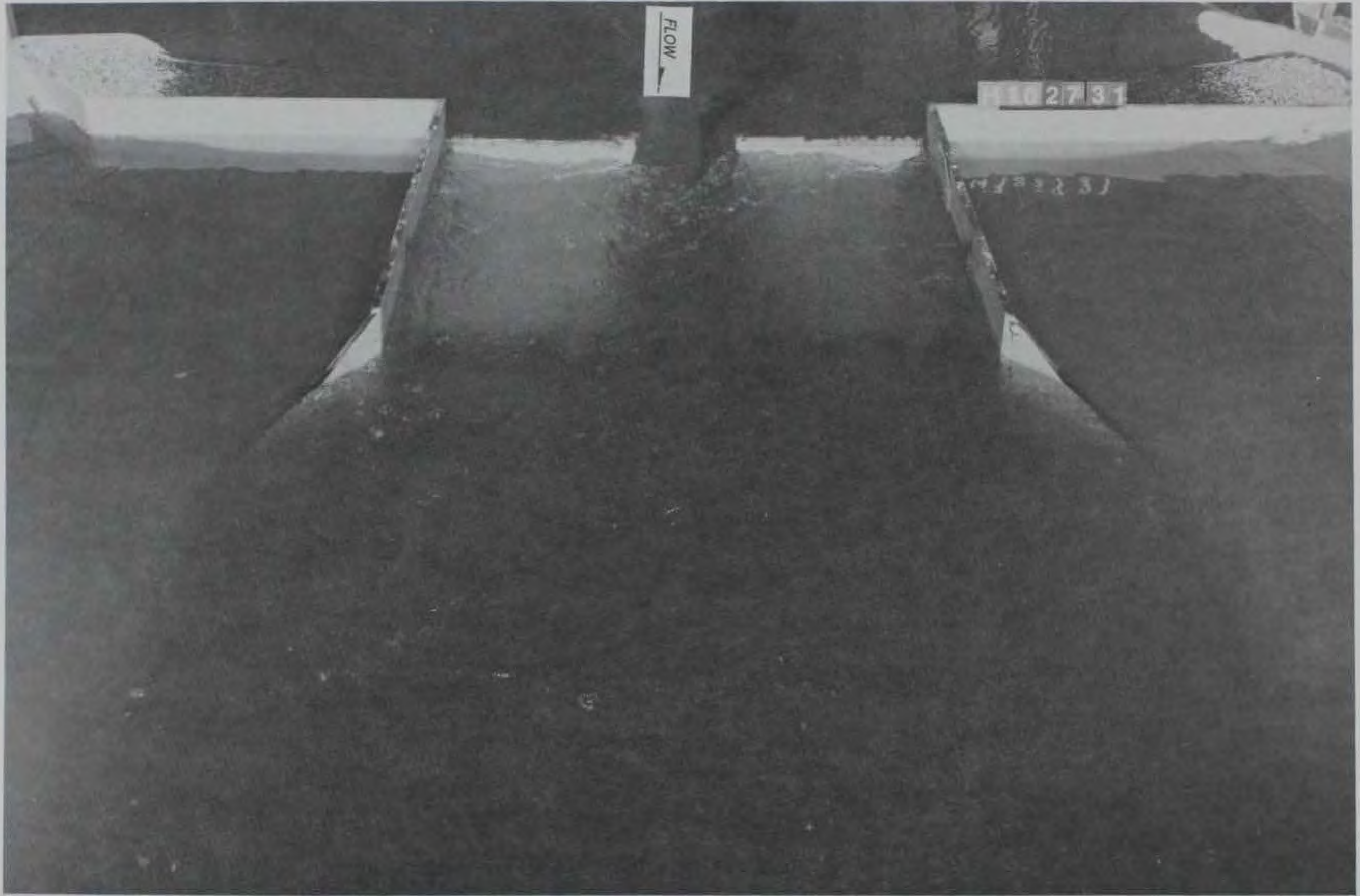
Photo 8. Type 25 weir, weir flow, discharge 991 cu m/sec (55,000 cfs), tailwater el 766.71
