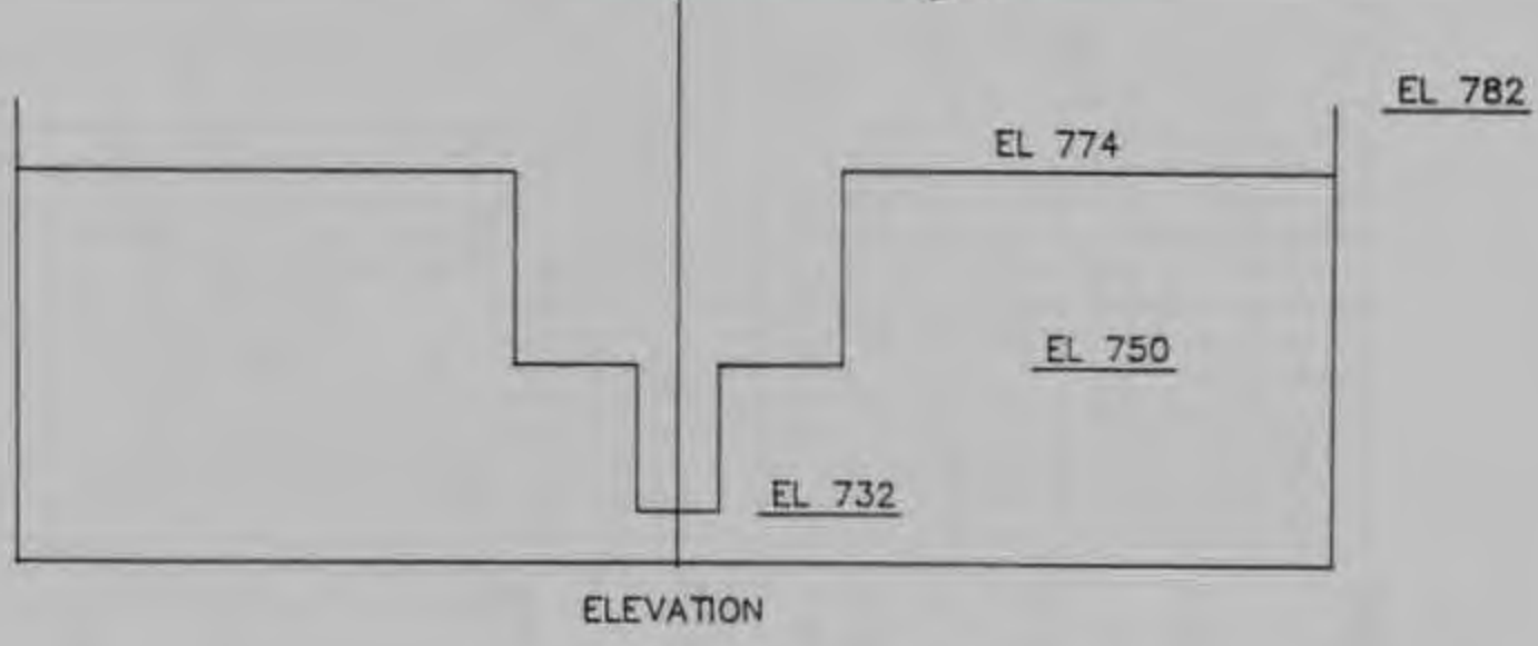
TYPE 22 WEIR DESIGN
