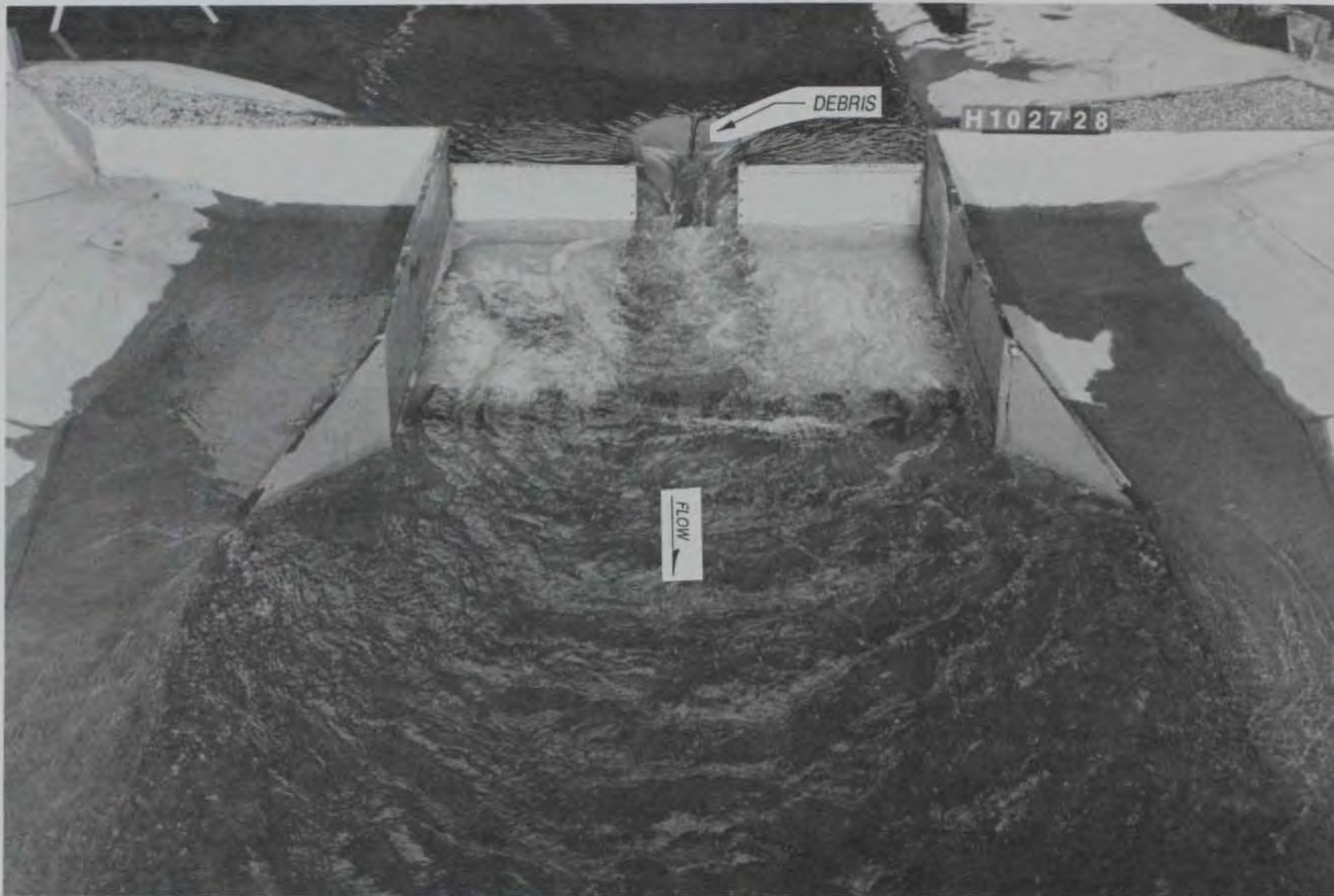
Photo 12. Type 2 debris deflectors, debris passage looking upstream, discharge 283 cu m/sec (10,000 cfs), tailwater el 747.01
