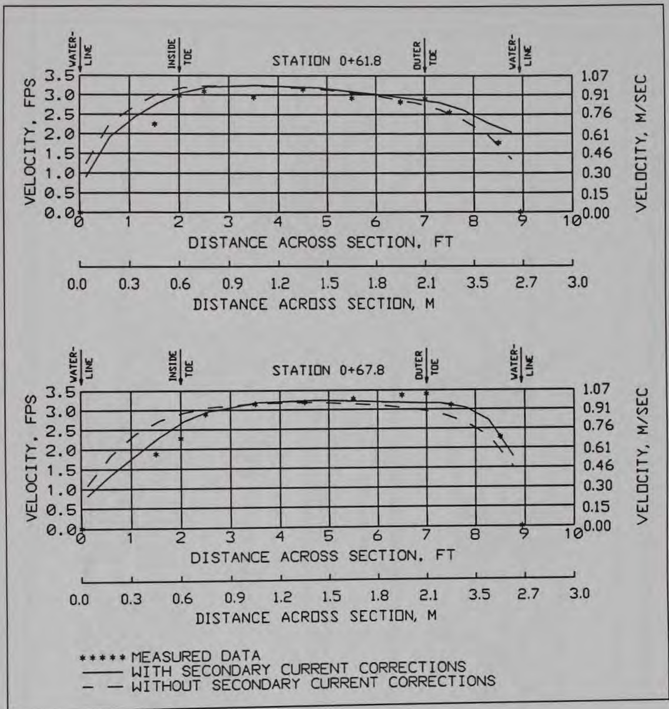
Figure 7. Computed versus measured velocity, 0.5-rad (30-deg) bend
