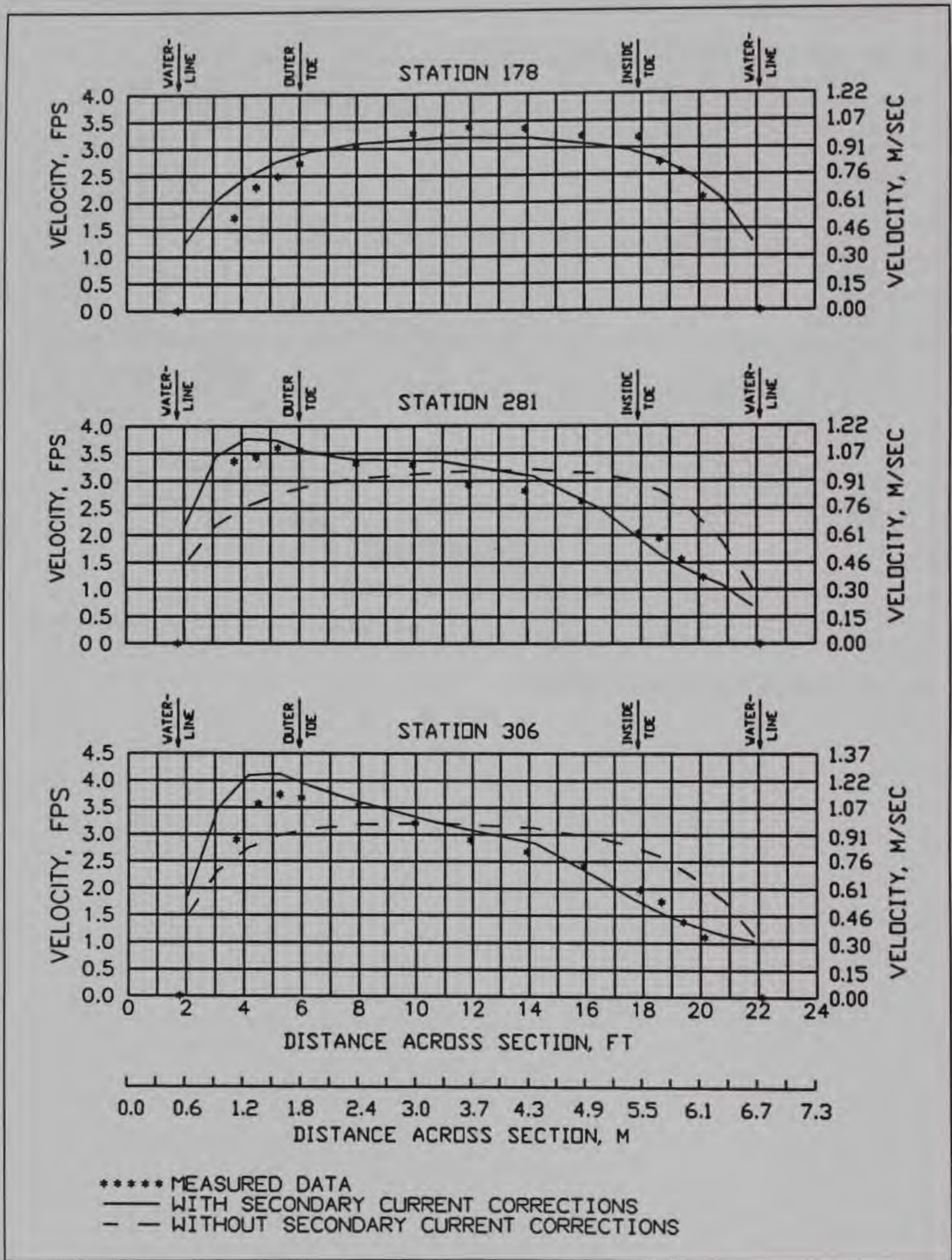
Figure 2. Predicted versus observed velocities, RTF, discharge 2.9 cu m/sec (101 cfs)
