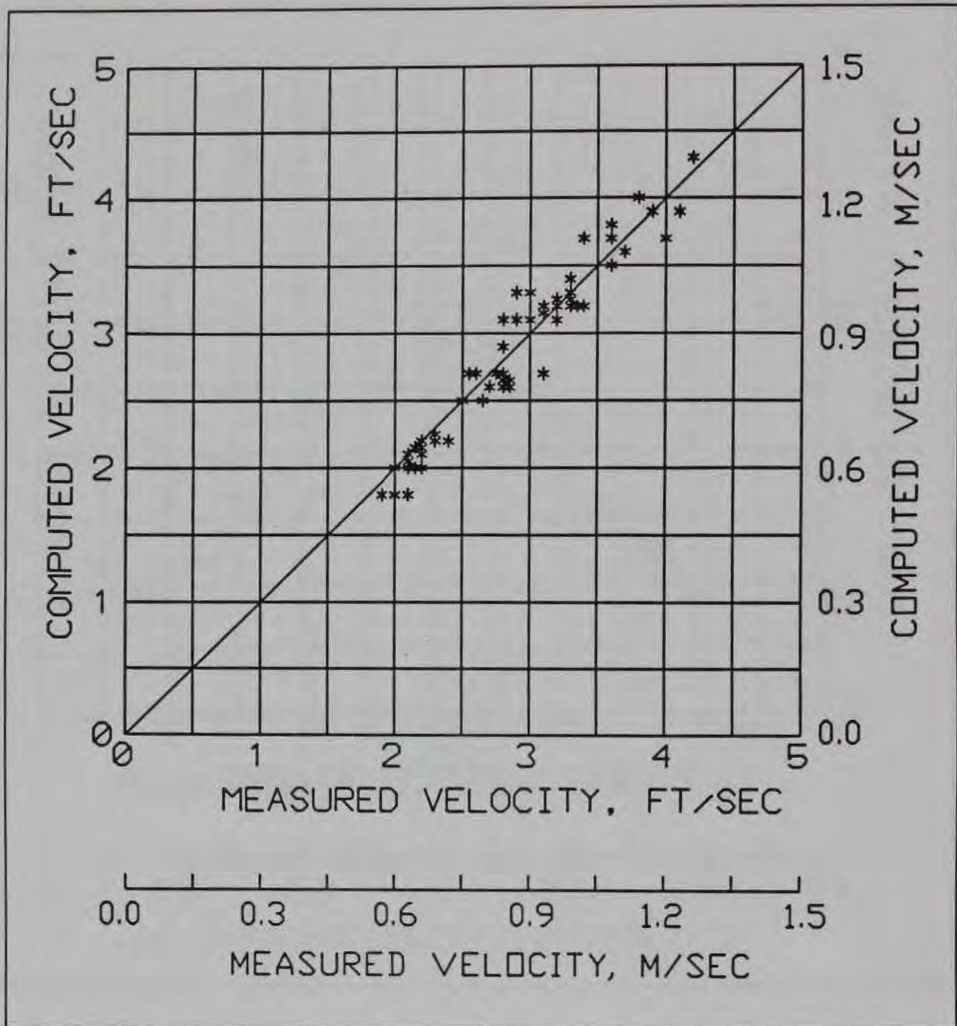
Figure 17. Scatter plot, 1V:2H side slope, channel bottom
