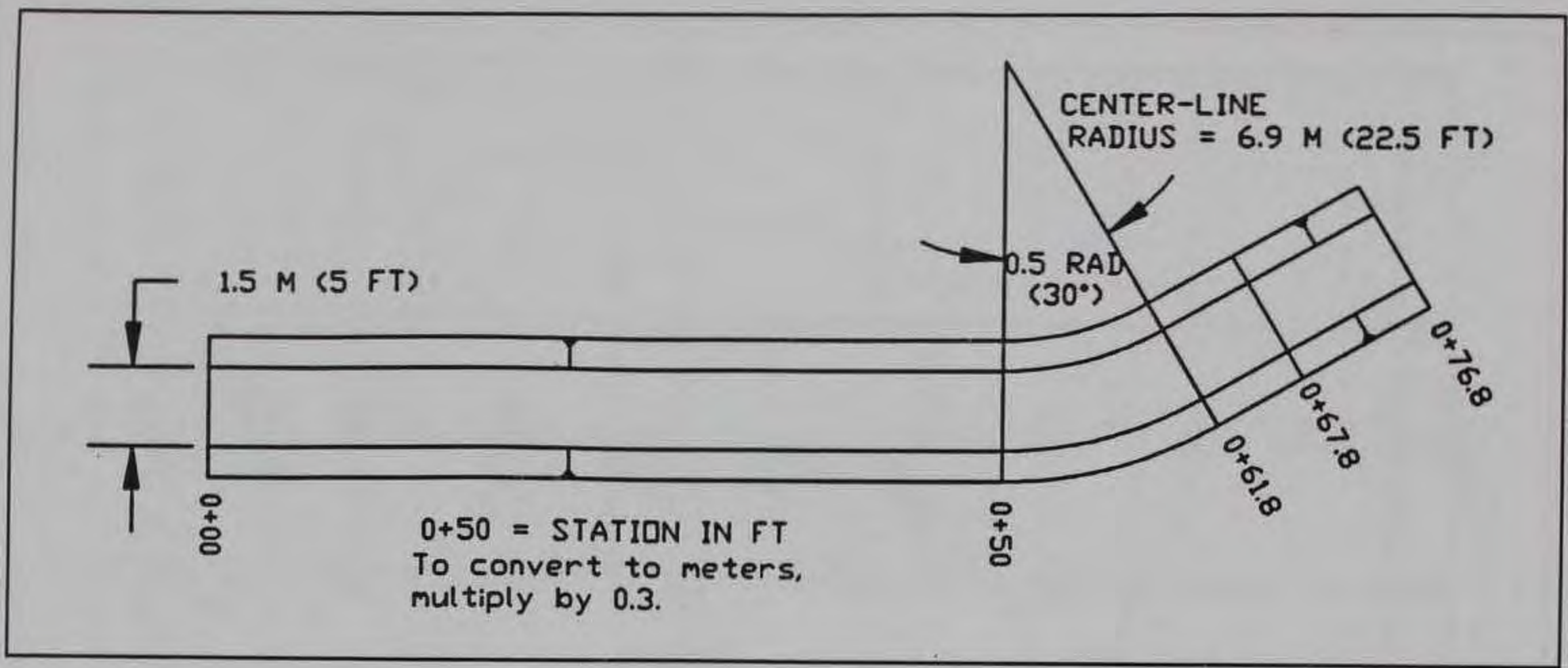
Figure 6. Schematic of 0.5-rad (30-deg) bend
