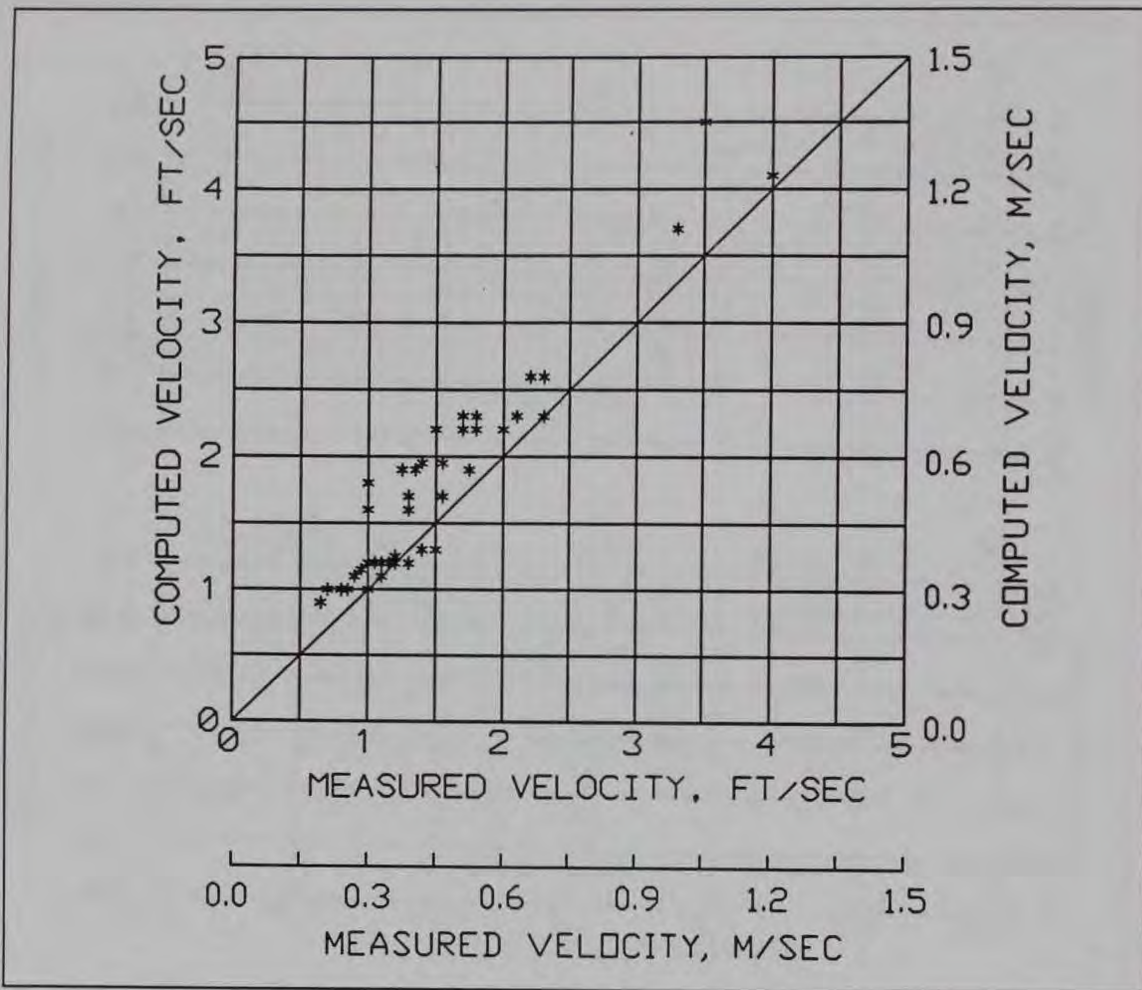
Figure 15. Scatter plot, 1V:2H side slope, upper bank
