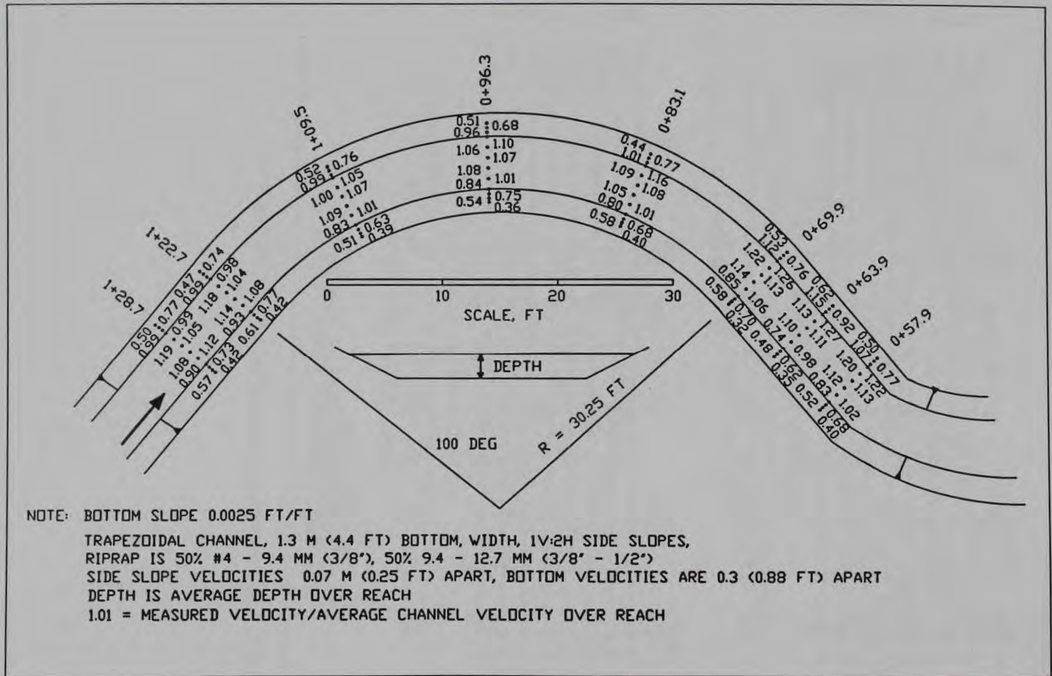
Figure 8. Dimensionless velocities, 1.7-rad (100-deg) bend, discharge 0.15 cu m/sec (5.3 cfs), depth 152 mm (0.50 ft)
