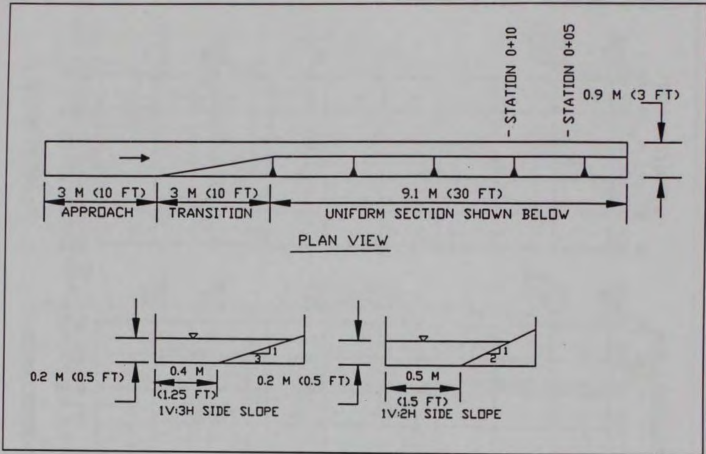
Figure 13. Schematic of straight channel
