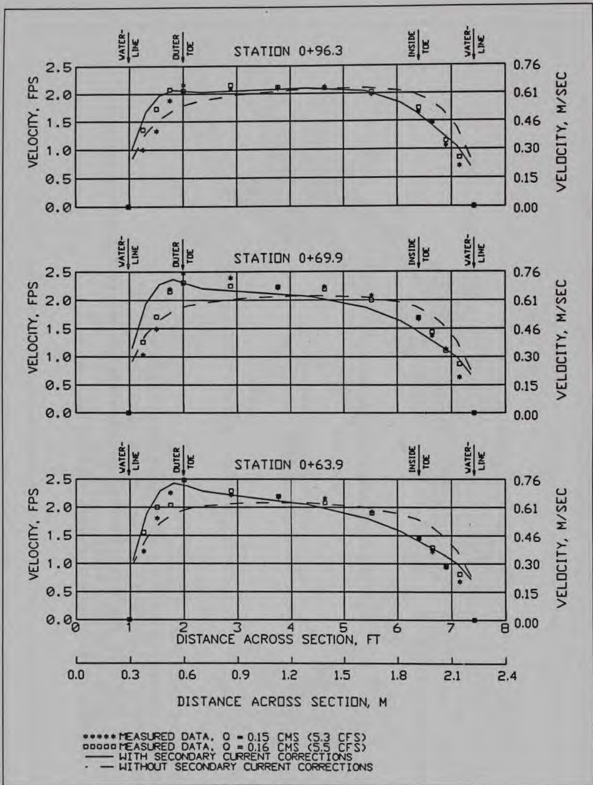
Figure 10. Computed versus measured velocity, 1.7-rad (100-deg) bend
