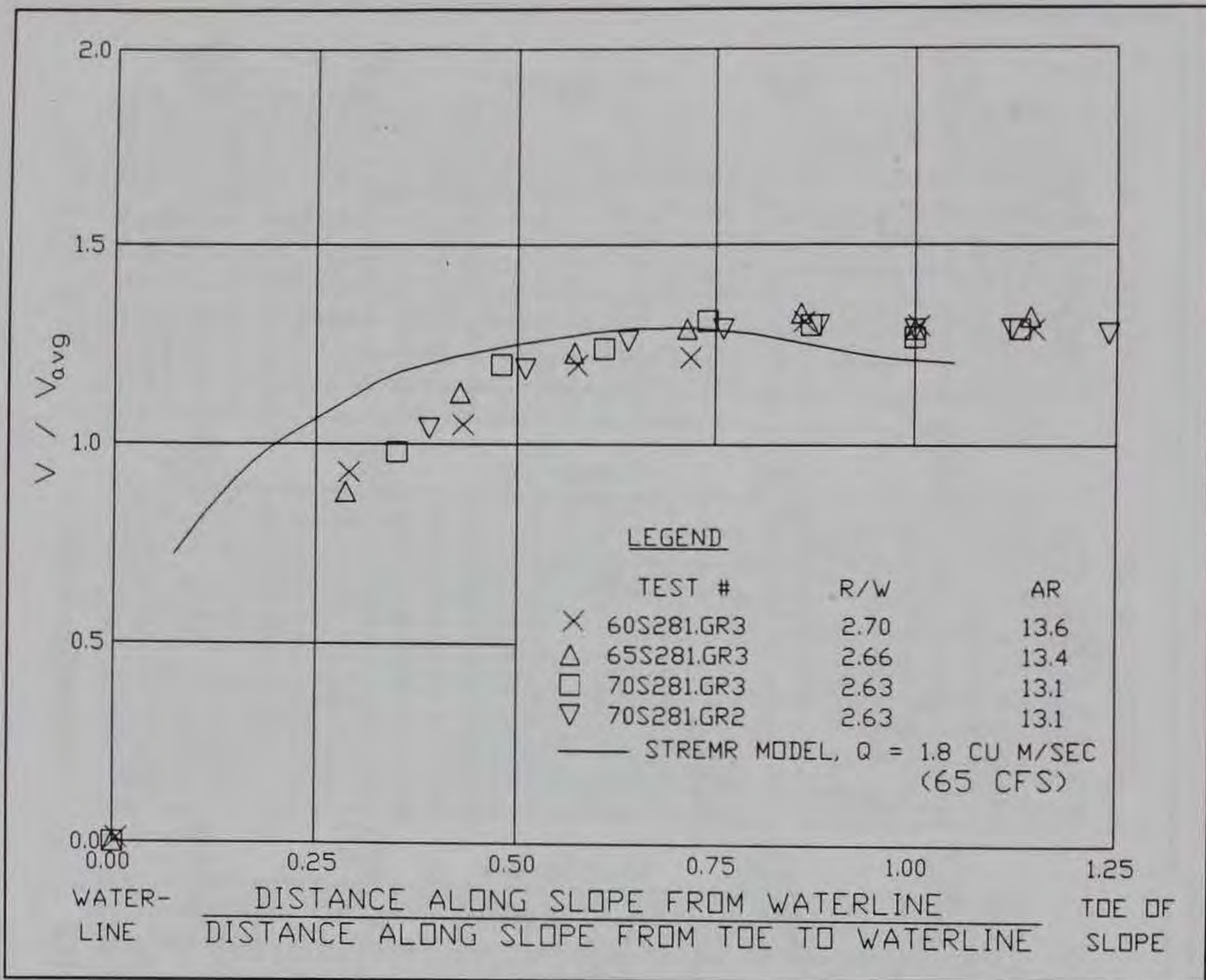
Figure 4. Predicted versus observed velocity, RTF, 1V:2H side slope, station 2+81, discharge 1.7 to 1.9 cu m/sec (60 to 70 cfs)
