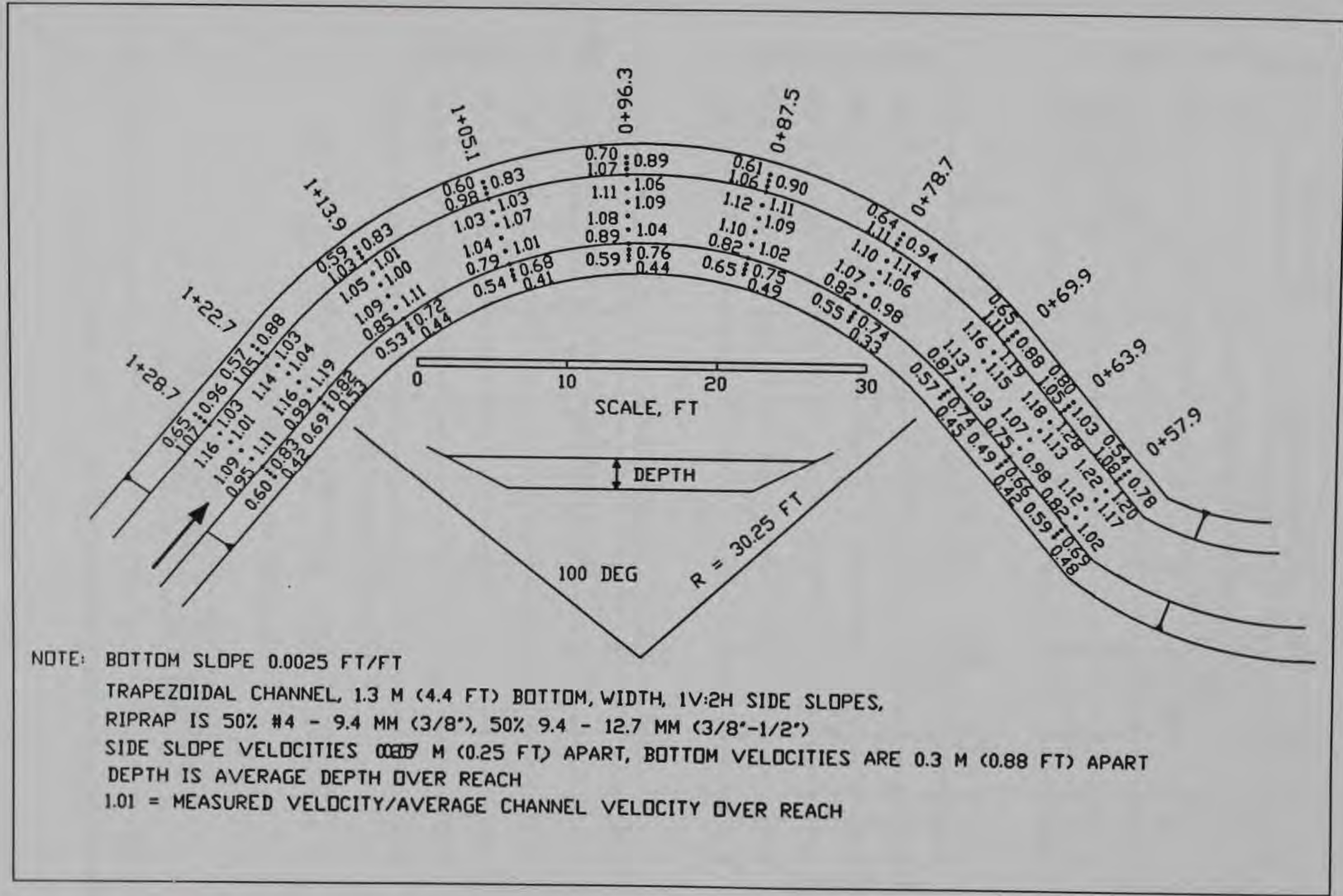
Figure 9. Dimensionless velocities, 1.7-rad (100-deg) bend, discharge 0.16 cu m/sec (5.5 cfs), depth 158 mm (0.52 ft)
