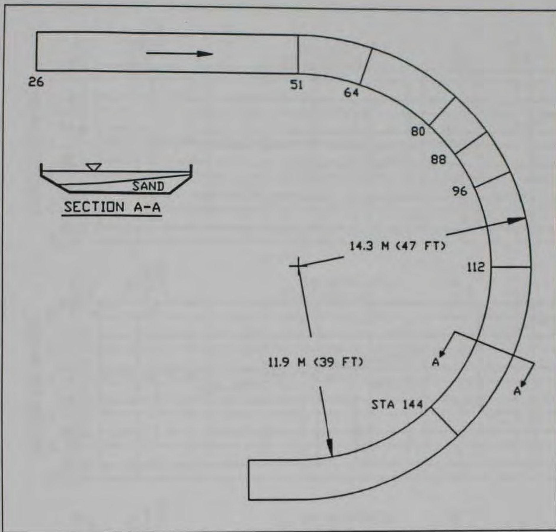
Figure 11. Schematic of 3.1-rad (180-deg) bend
