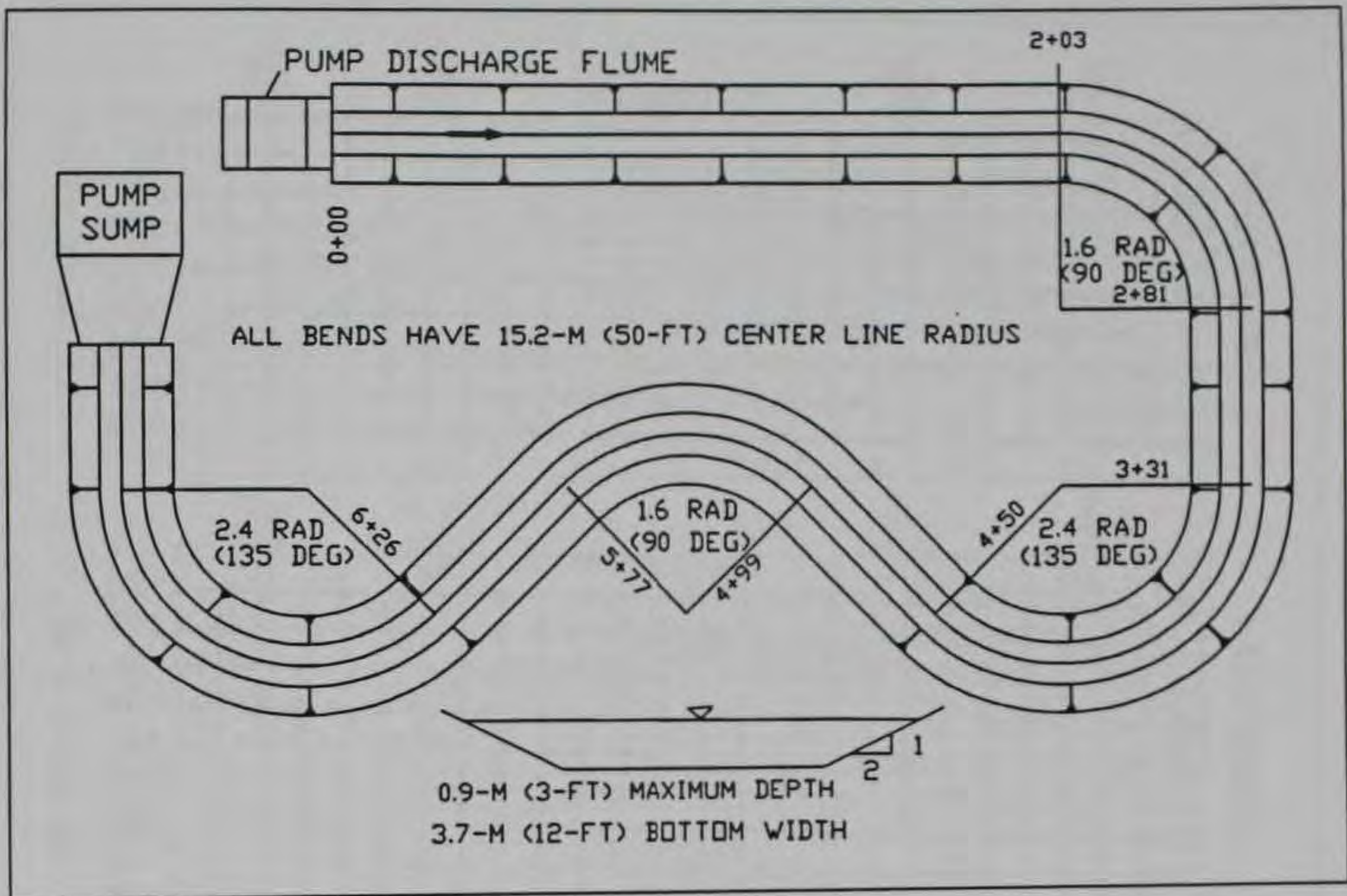
Figure 1. Riprap Test Facility schematic
