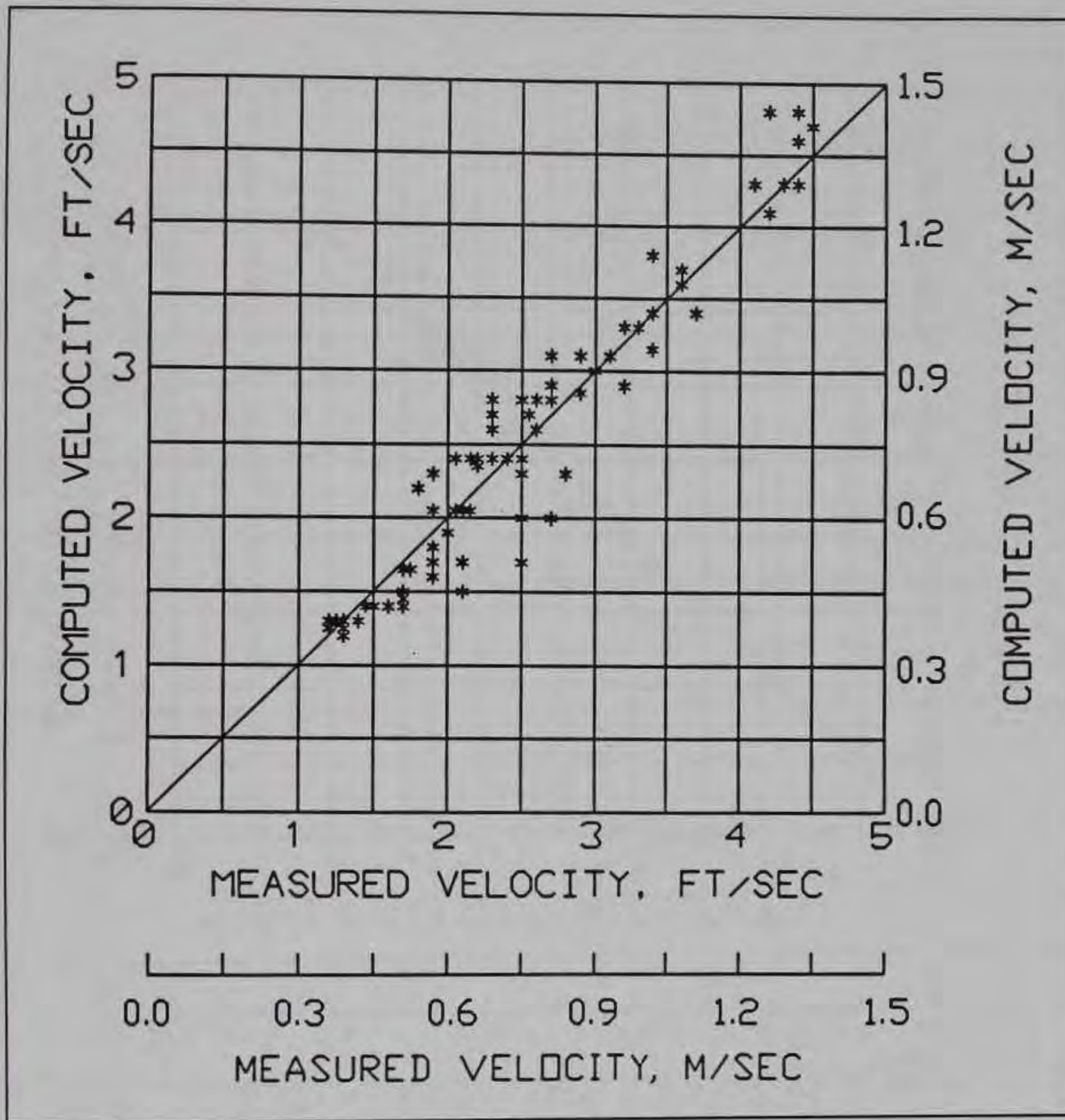
Figure 16. Scatter plot, 1V:2H side slope, lower bank
