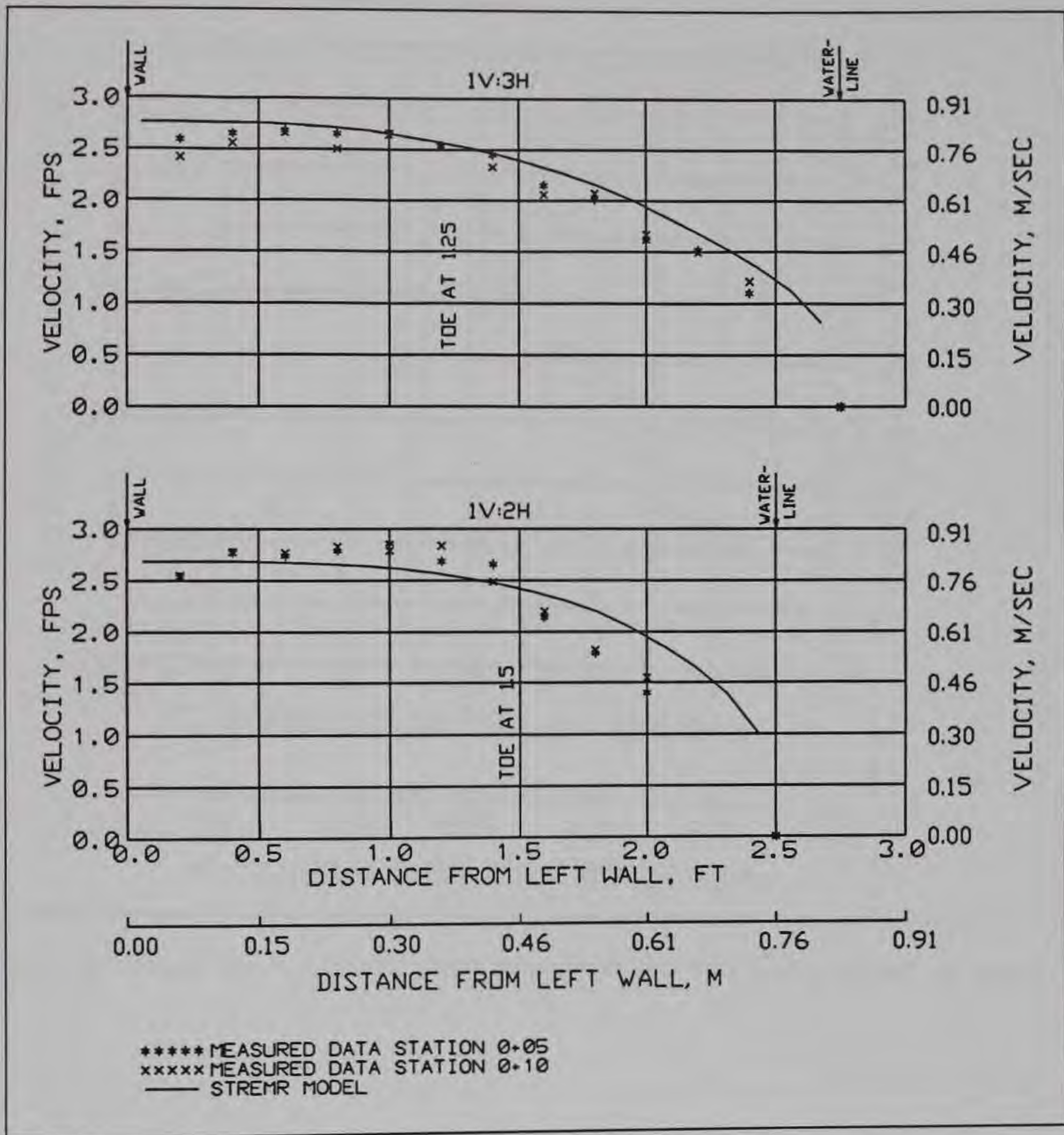
Figure 14. Computed versus measured velocity, straight channel
