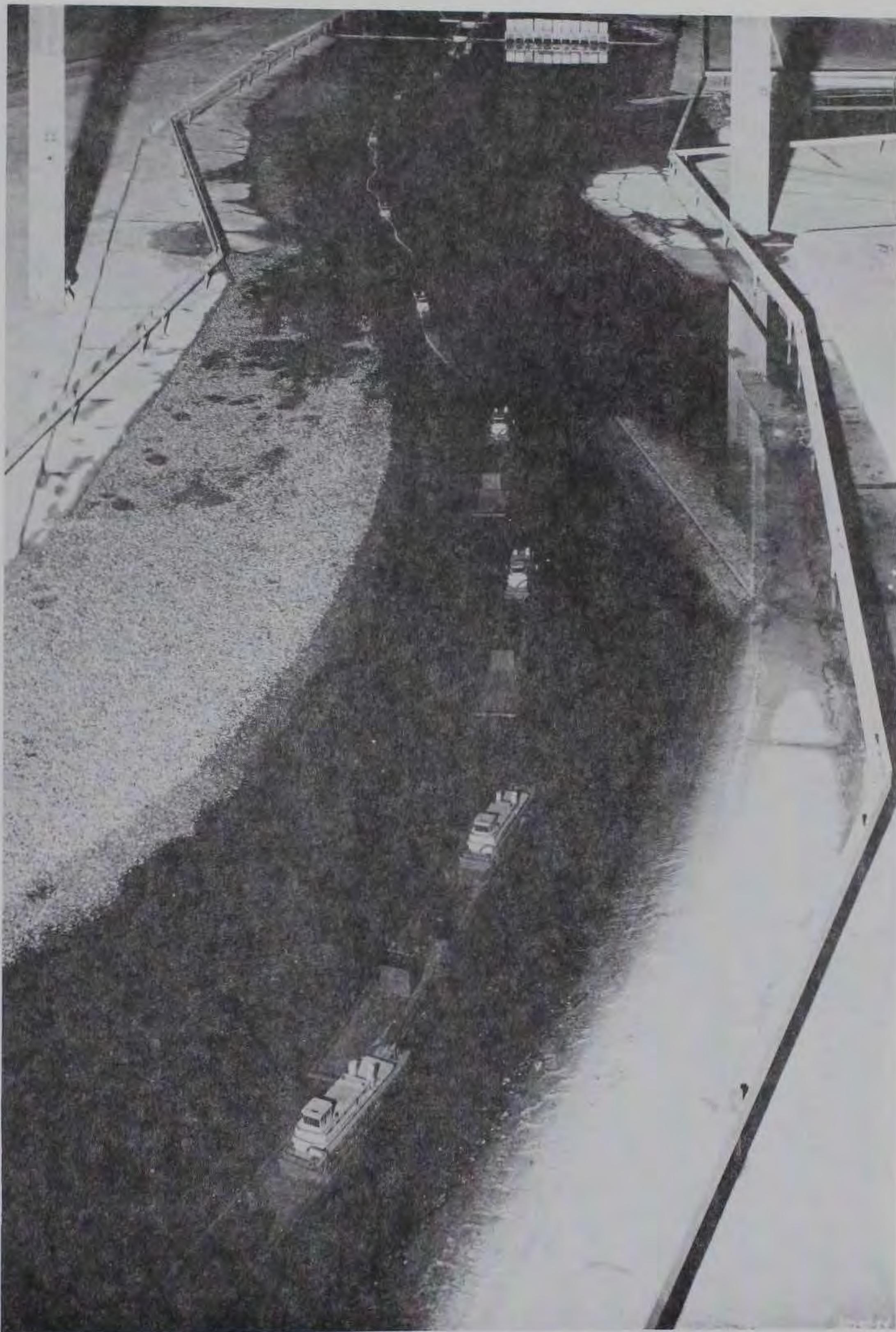
Photo 7. Plan B-34, upbound tow crossing to the right bank upstream of the longitudinal dike in the upper pool; discharge 145,000 cfs, tailwater el 57.5 (normal)
