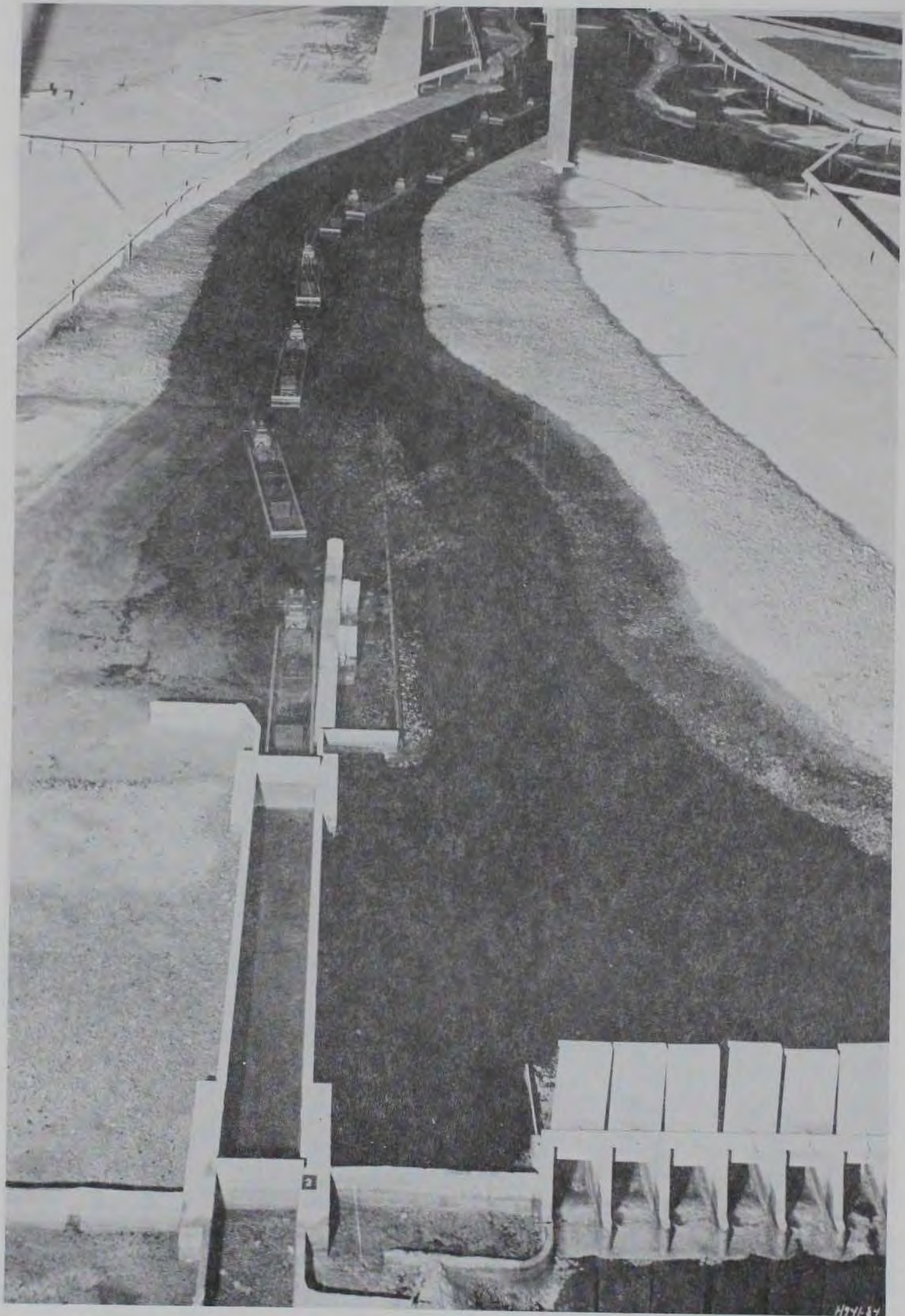
Photo 16. Plan B-35, Upbound tow approaching the lock; discharge 145,000 cfs, tailwater el 42.9 (minimum)
