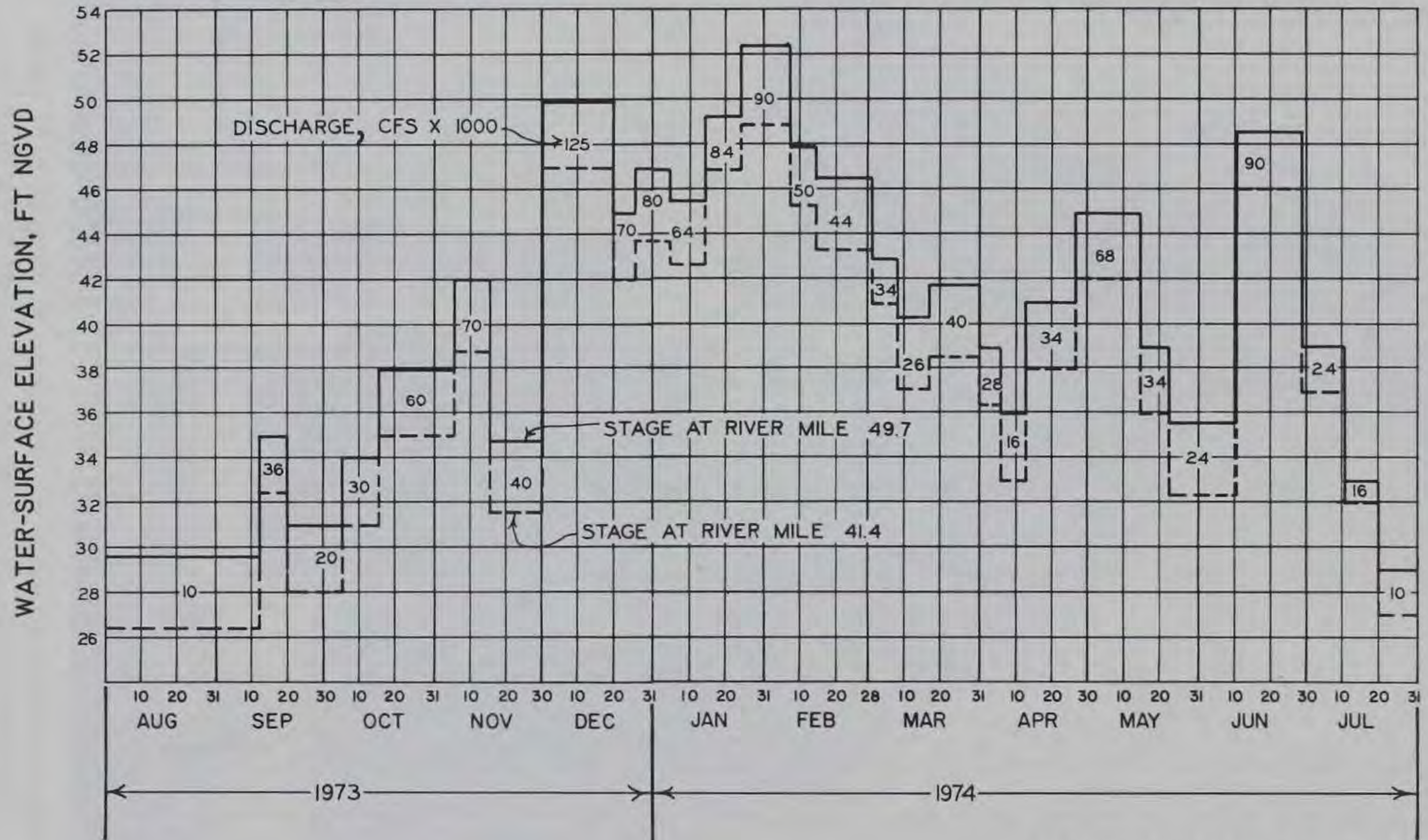
ADJUSTMENT HYDROGRAPH
