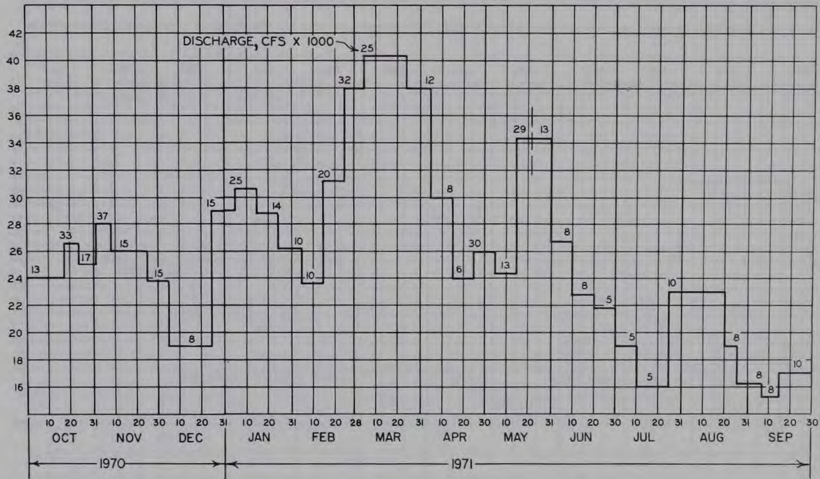
LOW-WATER HYDROGRAPH
