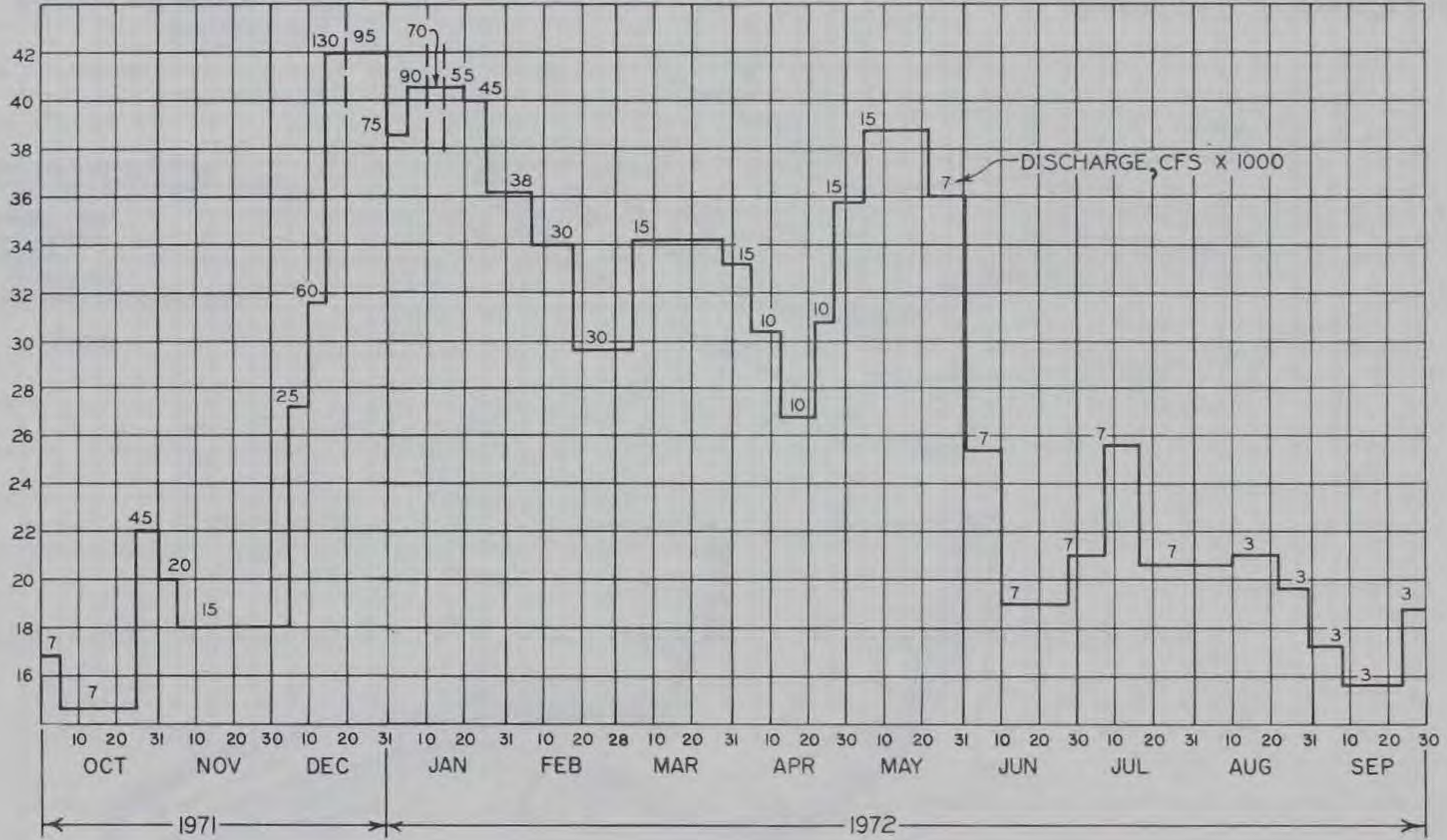
AVERAGE HYDROGRAPH
