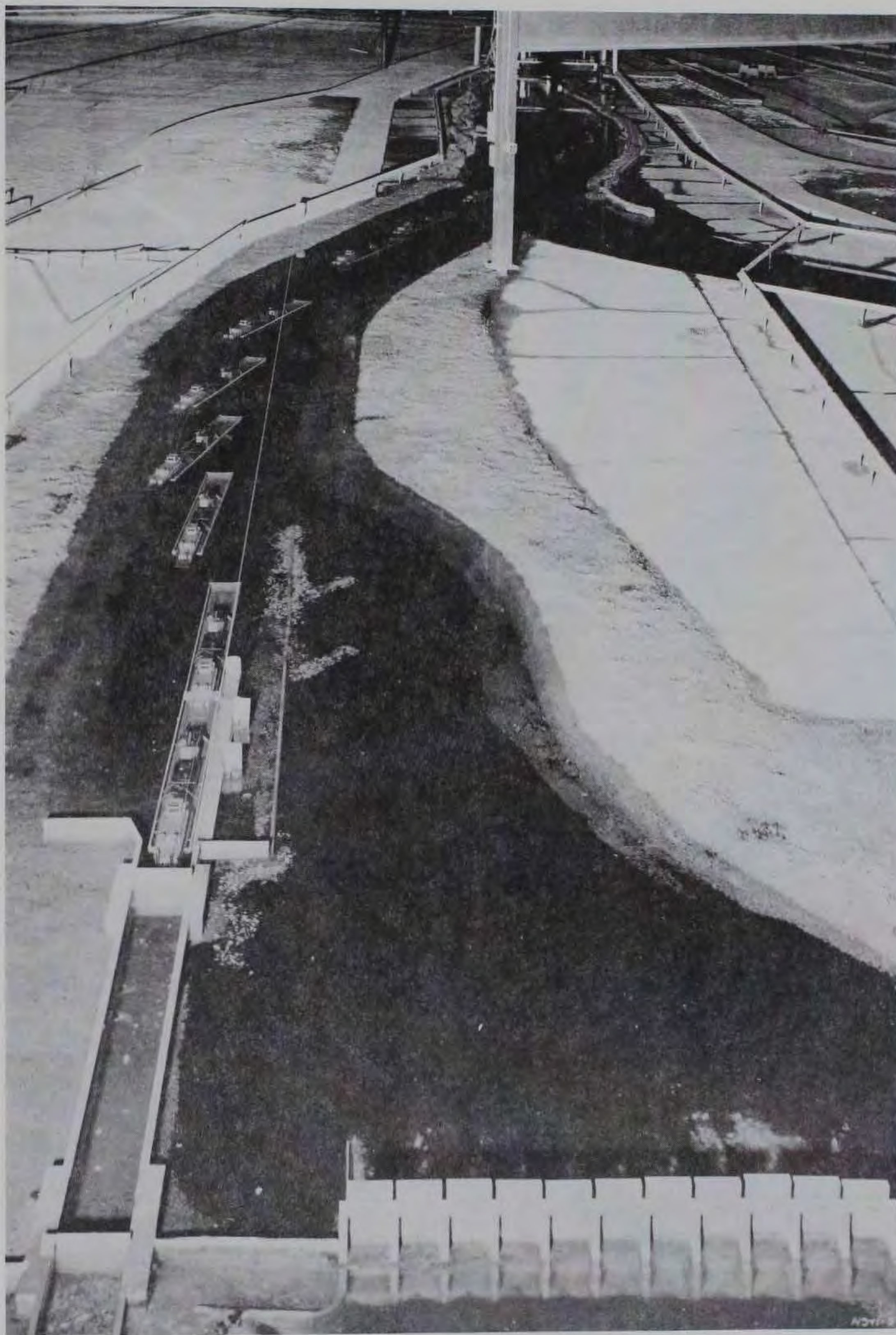
Photo 11. Plan B-34, downbound tow leaving the lock; discharge 145,000 cfs, tailwater el 42.9 (minimum)
