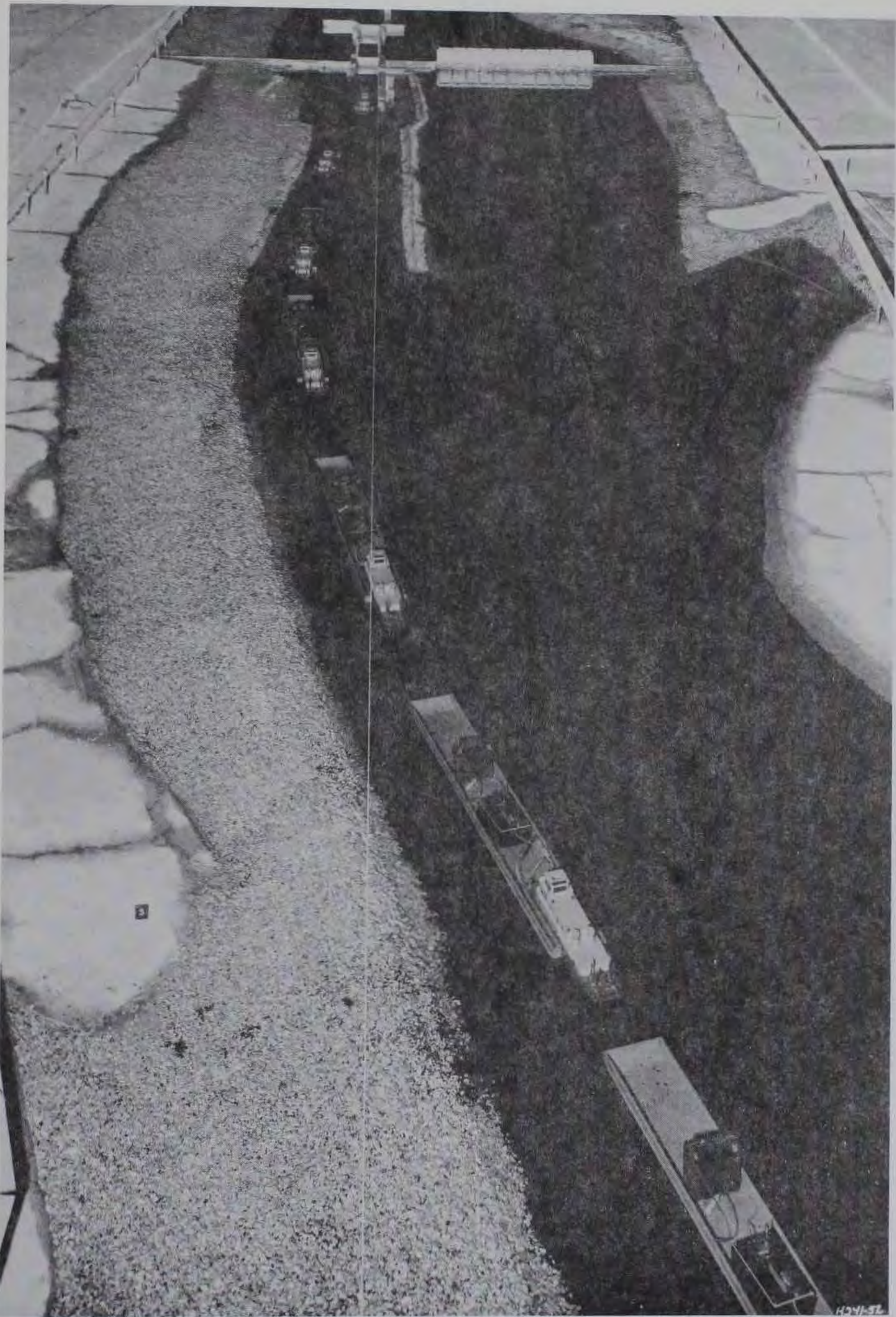
Photo 5. Plan B-34, downbound tow approaching the canal and lock from upstream; discharge 31,000 cfs, tailwater el 21.0 (normal)
