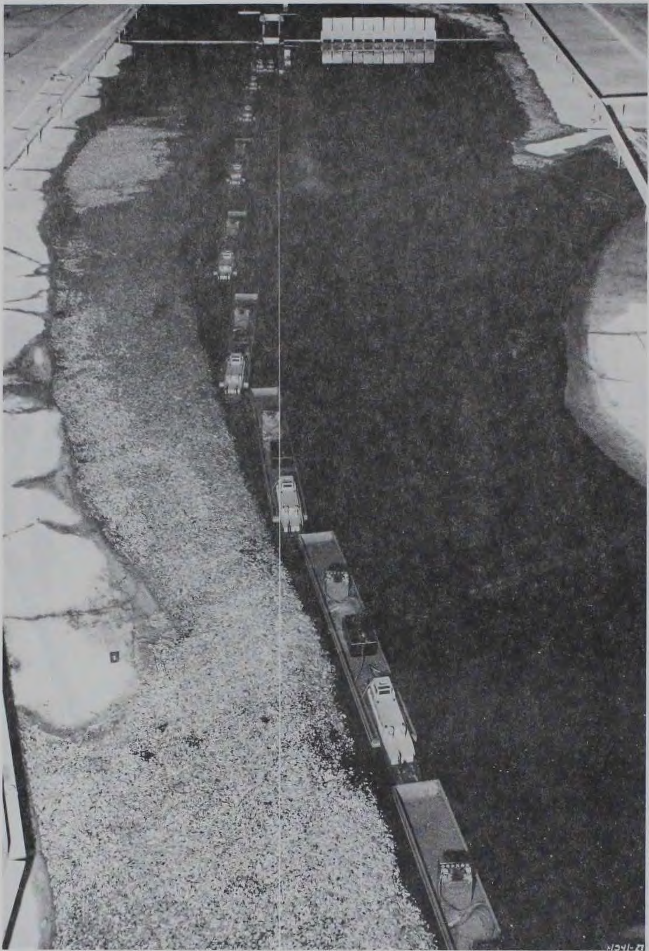
Photo 2. Plan B-34, downbound tow approaching the canal and lock from upstream; discharge 145,000 cfs, tailwater el 57.5 (normal)
