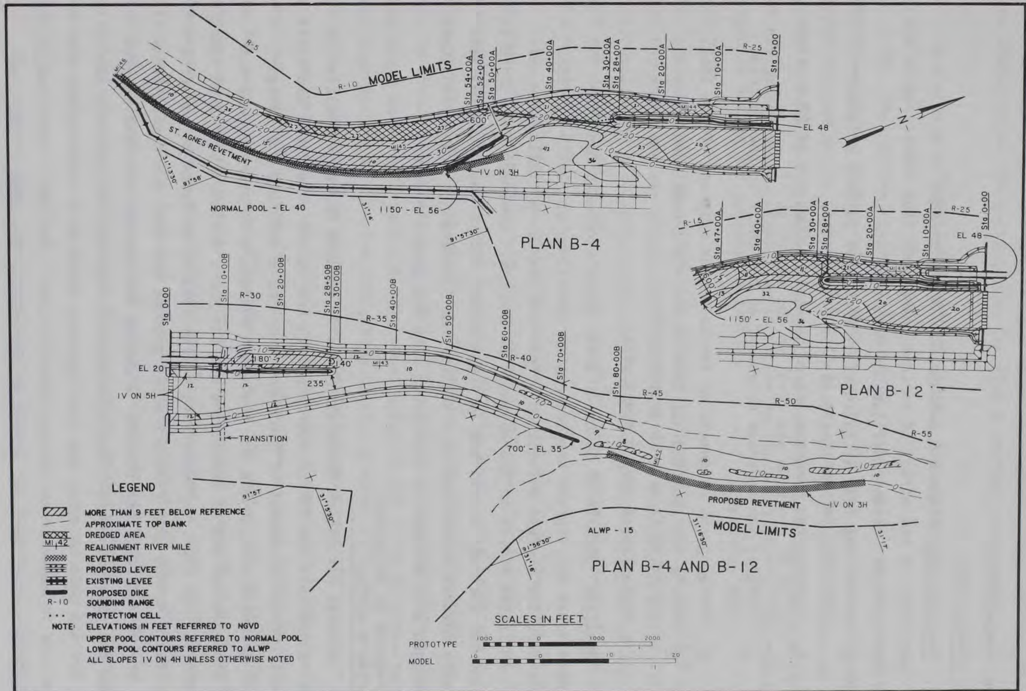
Figure 10. Plans B-4 and B-12
