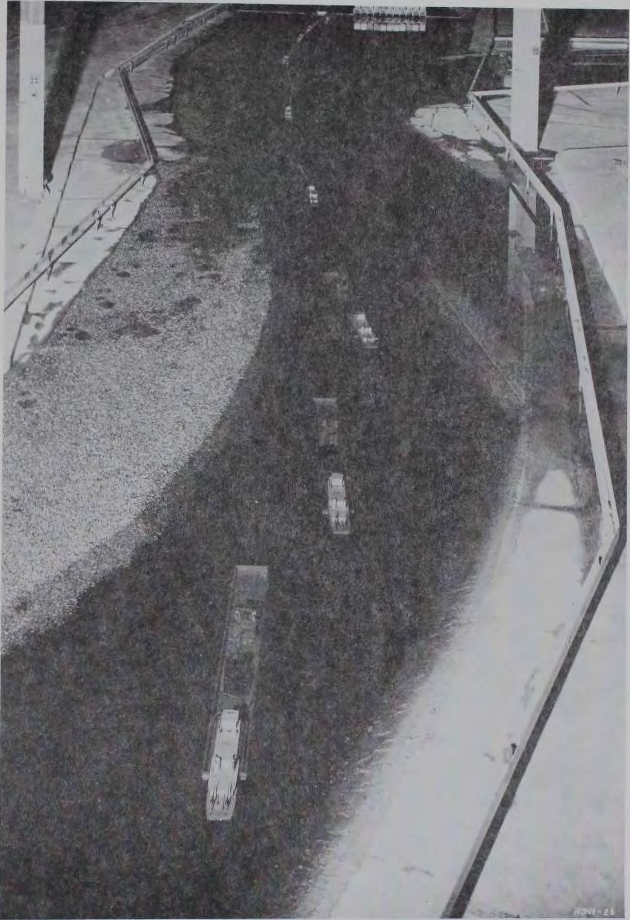
Photo 1. Plan B-34, downbound tow crossing to the left bank upstream of the longitudinal dike; discharge 145,000 cfs, tailwater el 57.5 (normal)
