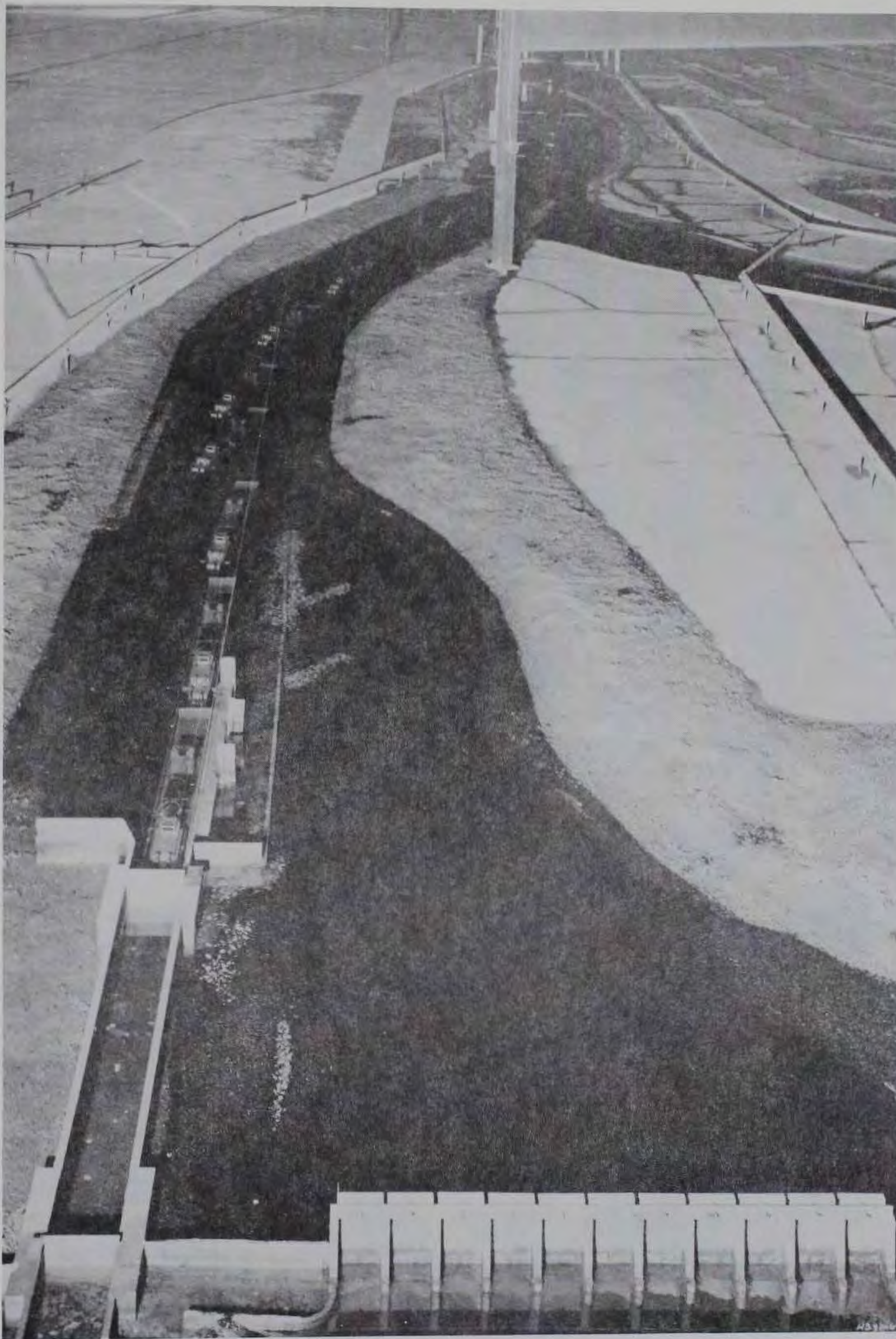
Photo 13. Plan B-34, downbound tow leaving the lock; discharge 31,000 cfs, tailwater el 21.0 (normal)
