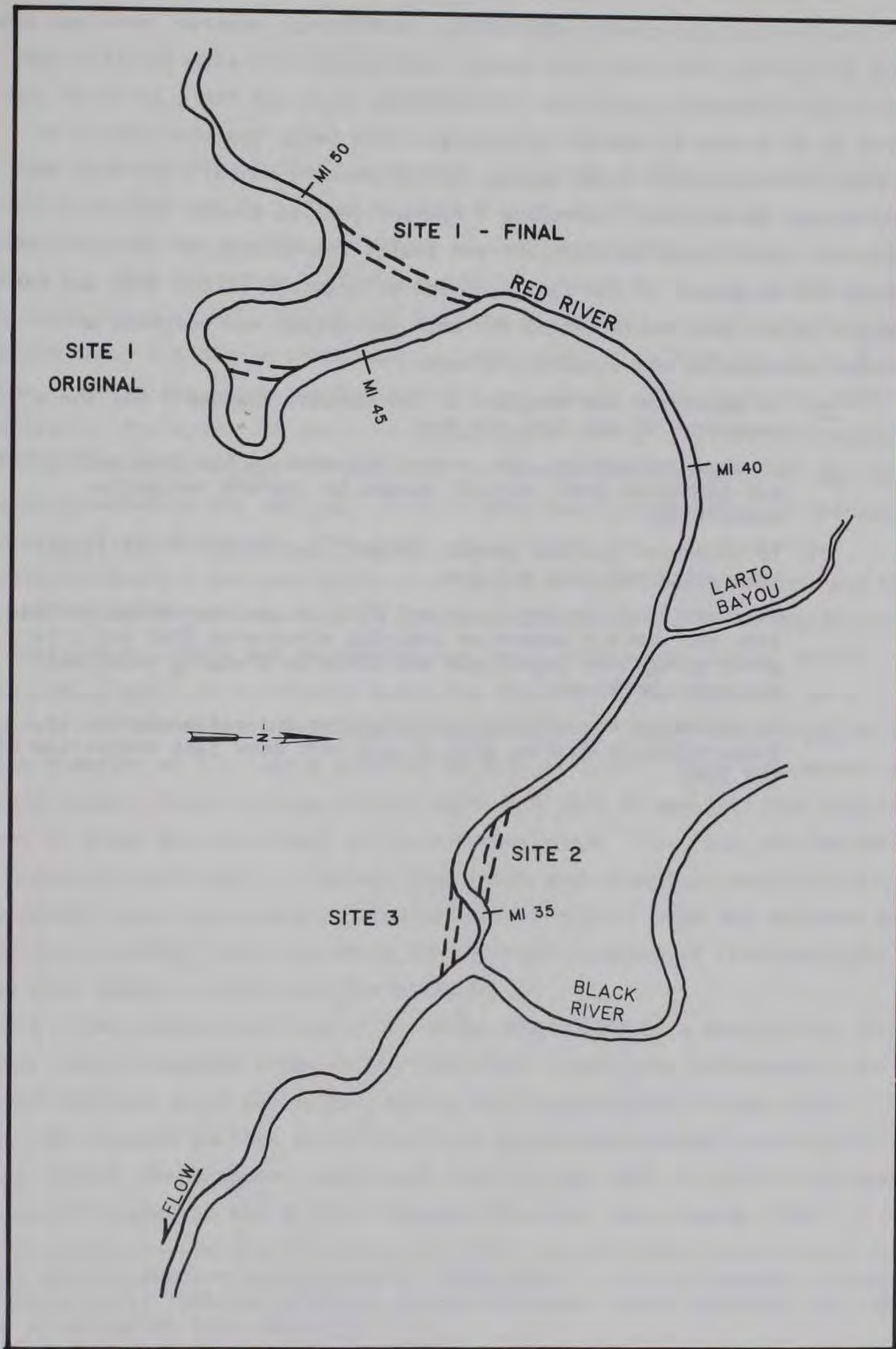
Figure 2. Alternate sites for Lock and Dam 1
