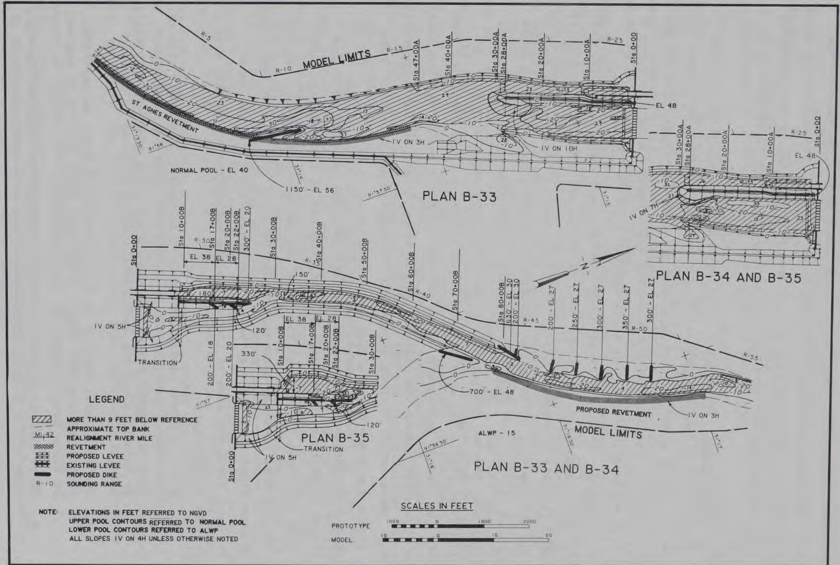
Figure 13. Plans B-33, B-34, and B-35
