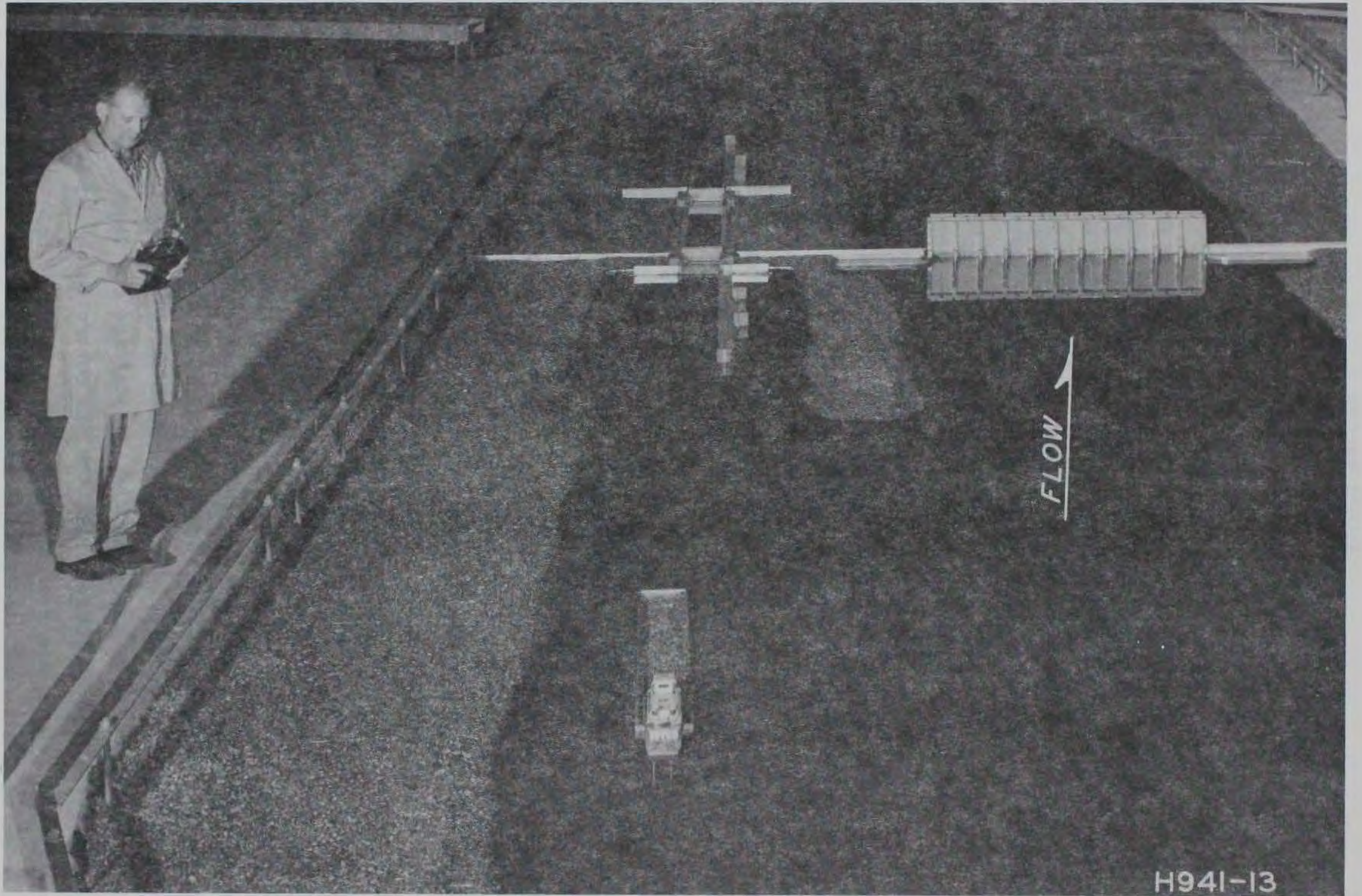
Figure 4. Remote-controlled towboat and tow in upper lock approach
