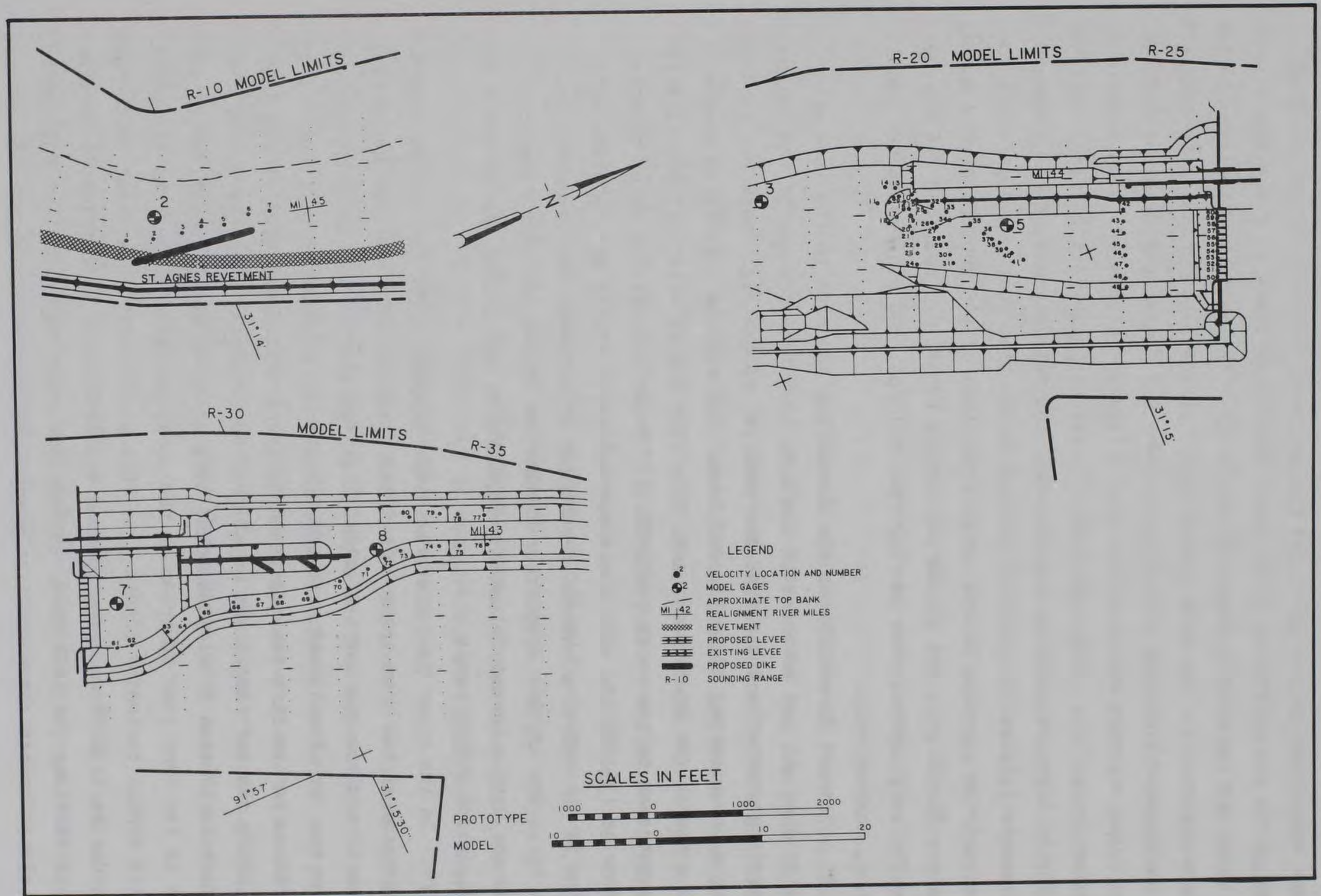
Figure 14. Location of point velocities
