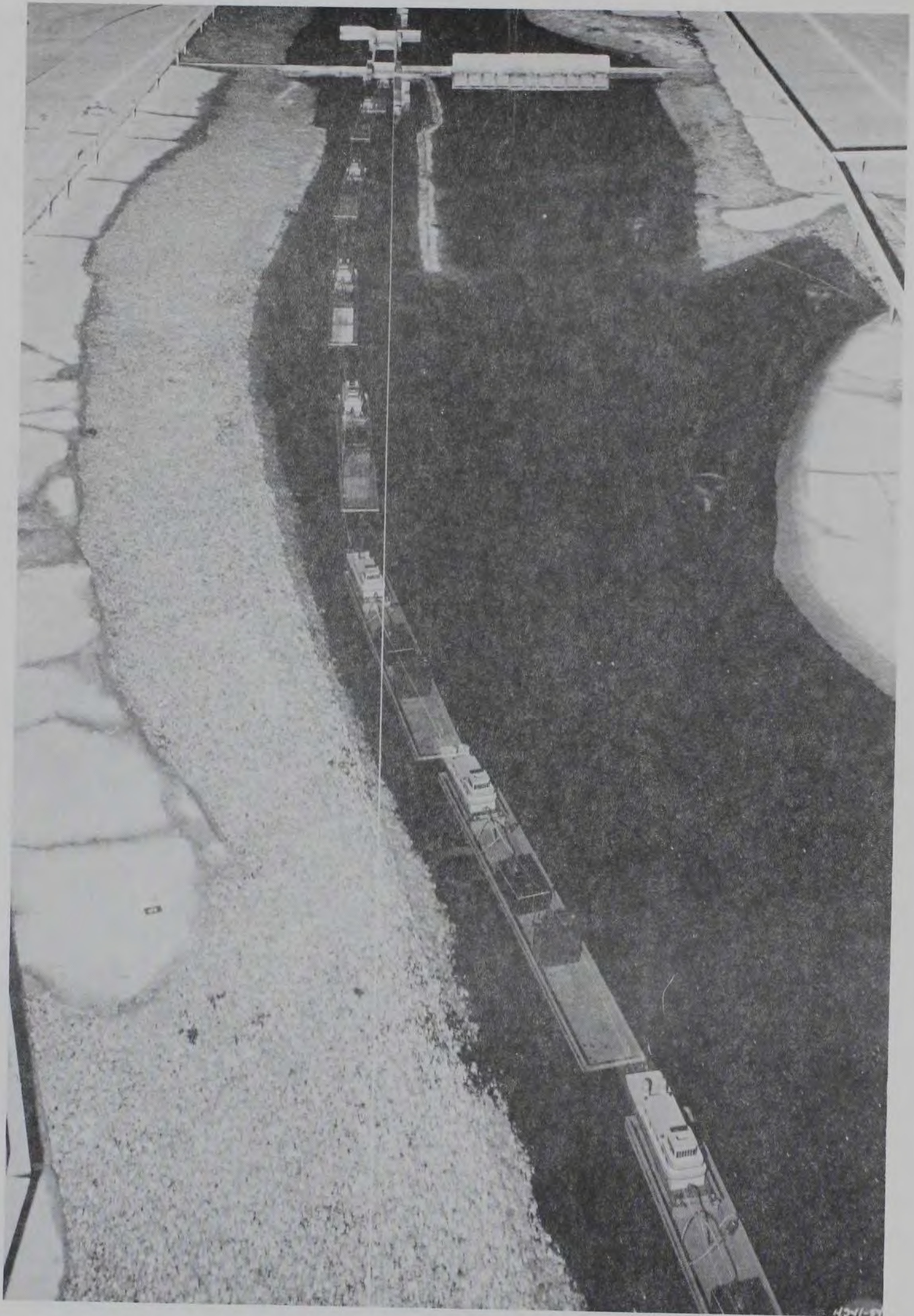
Photo 10. Plan B-34, upbound tow leaving the lock and canal; discharge 31,000 cfs, tailwater el 21.0 (normal)
