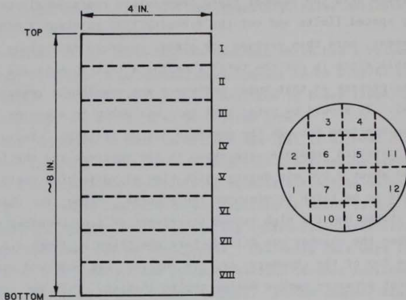
Figure 11. Specimen dissection pattern
