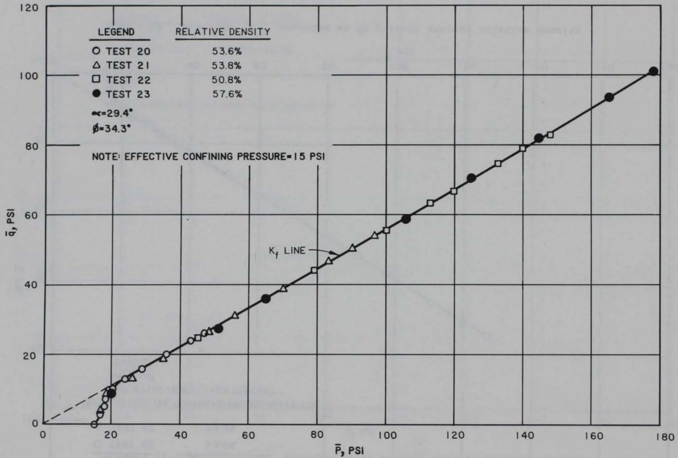
Figure 23. Specimen \bar{p} - \bar{q} response at 54 percent average relative density
