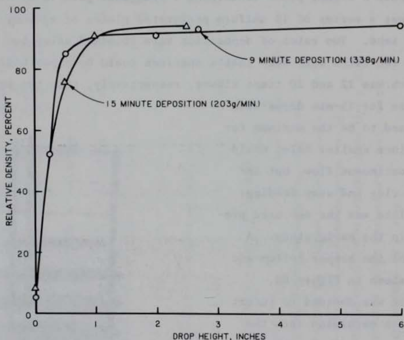
Figure D9. Relative density versus drop height
