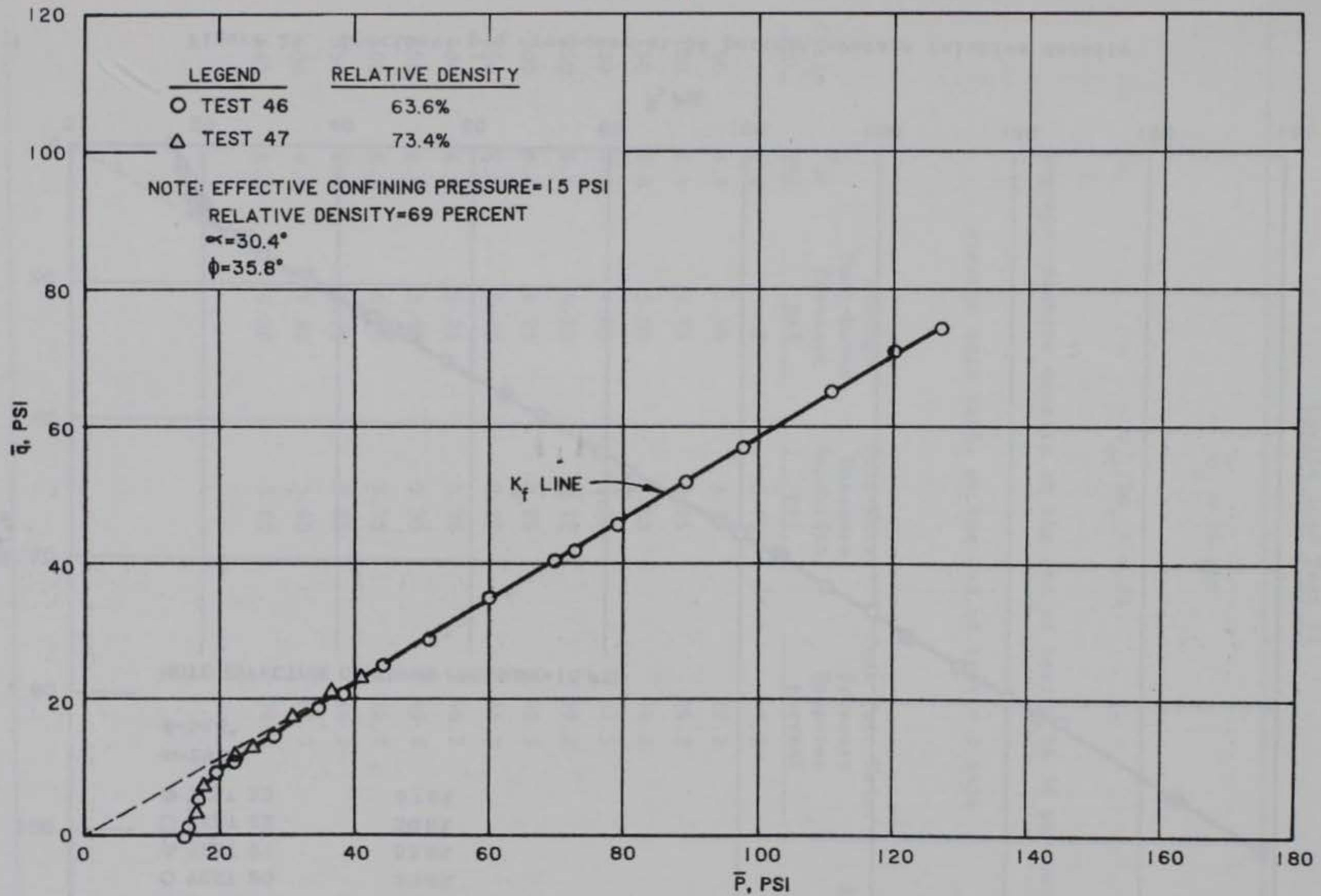
Figure 22. Specimen \bar{p} - \bar{q} response at 69 percent average relative density
