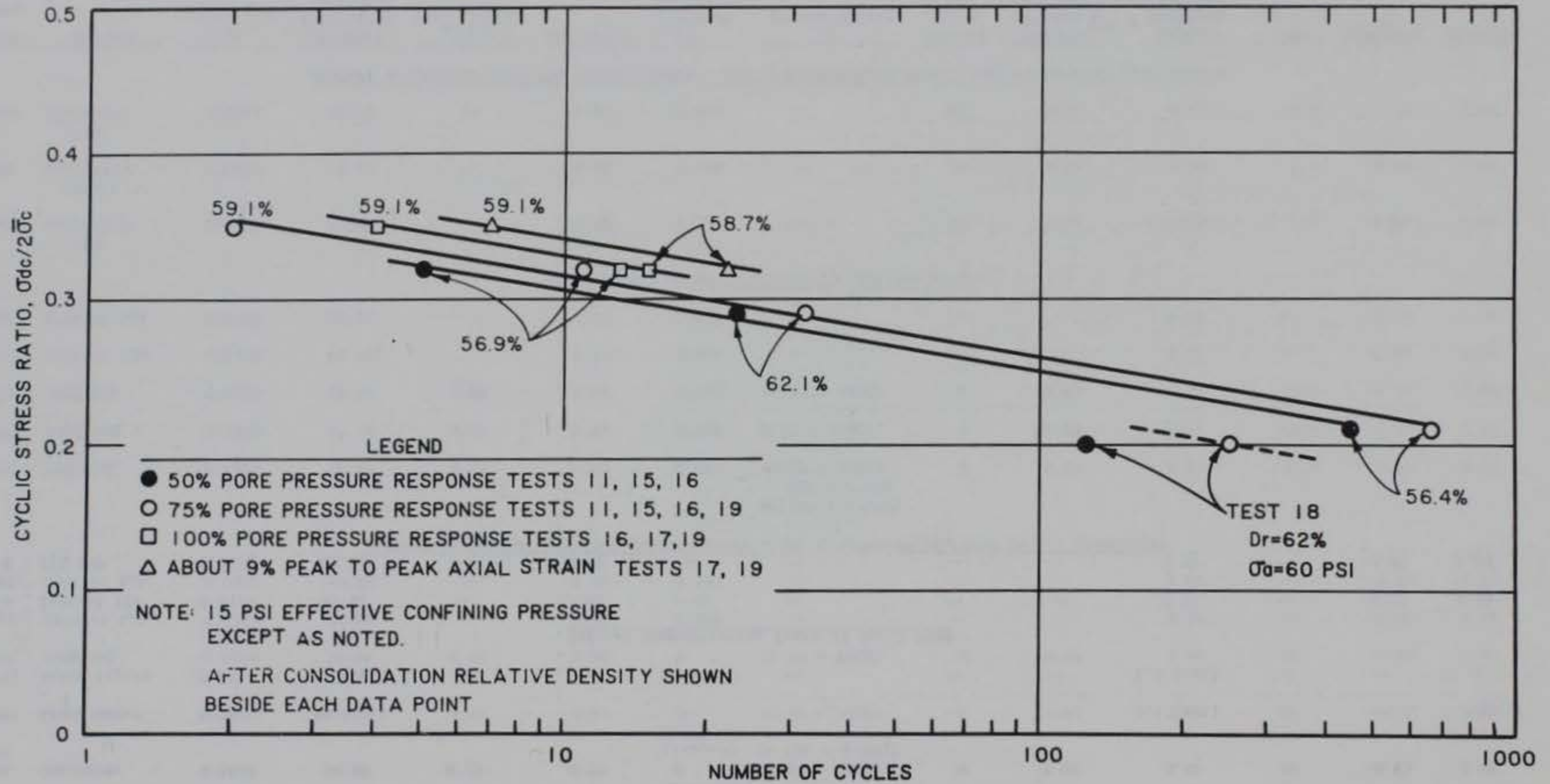
Figure 13. Summary of cyclic triaxial tests at nominal 60 percent average relative density
