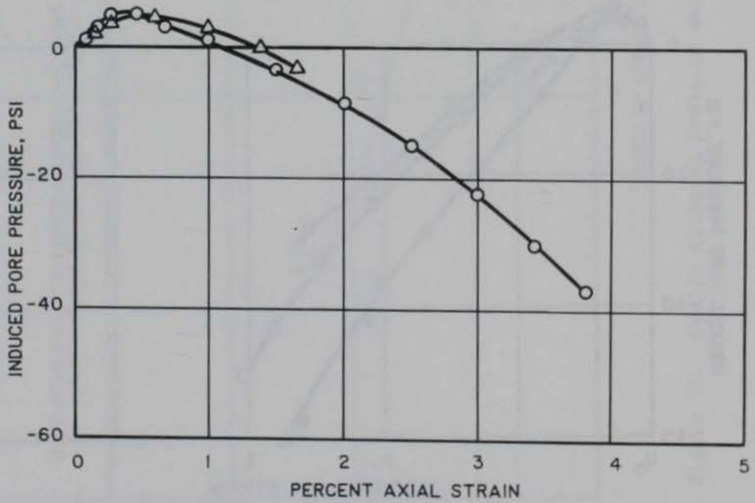
Figure 19. Specimen monotonic load response at nominal 70 percent average relative density
