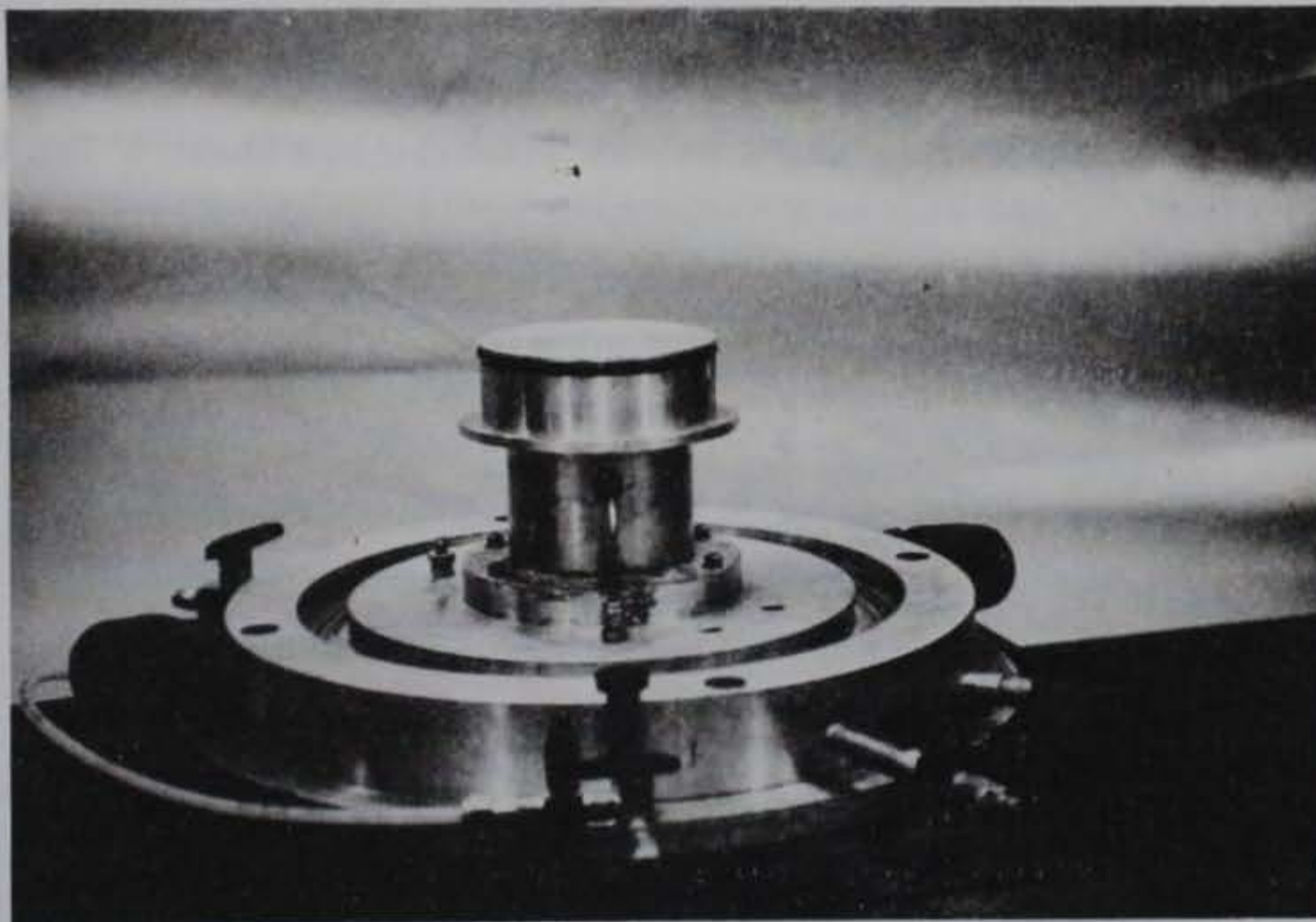
Figure 6. Triaxial baseplate showing oversize adapter
