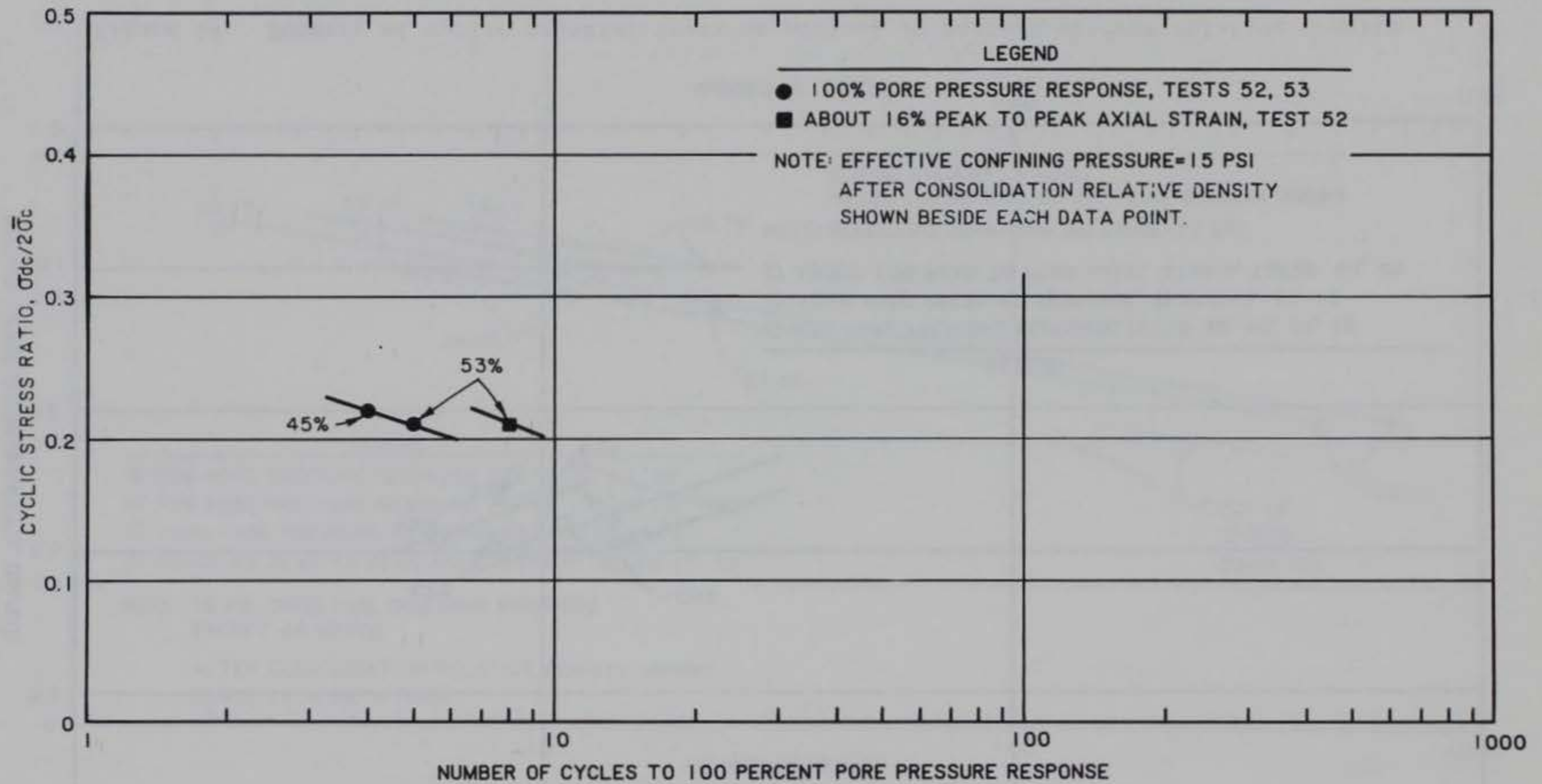
Figure 15. Summary of cyclic triaxial tests at nominal 45 percent average relative density
