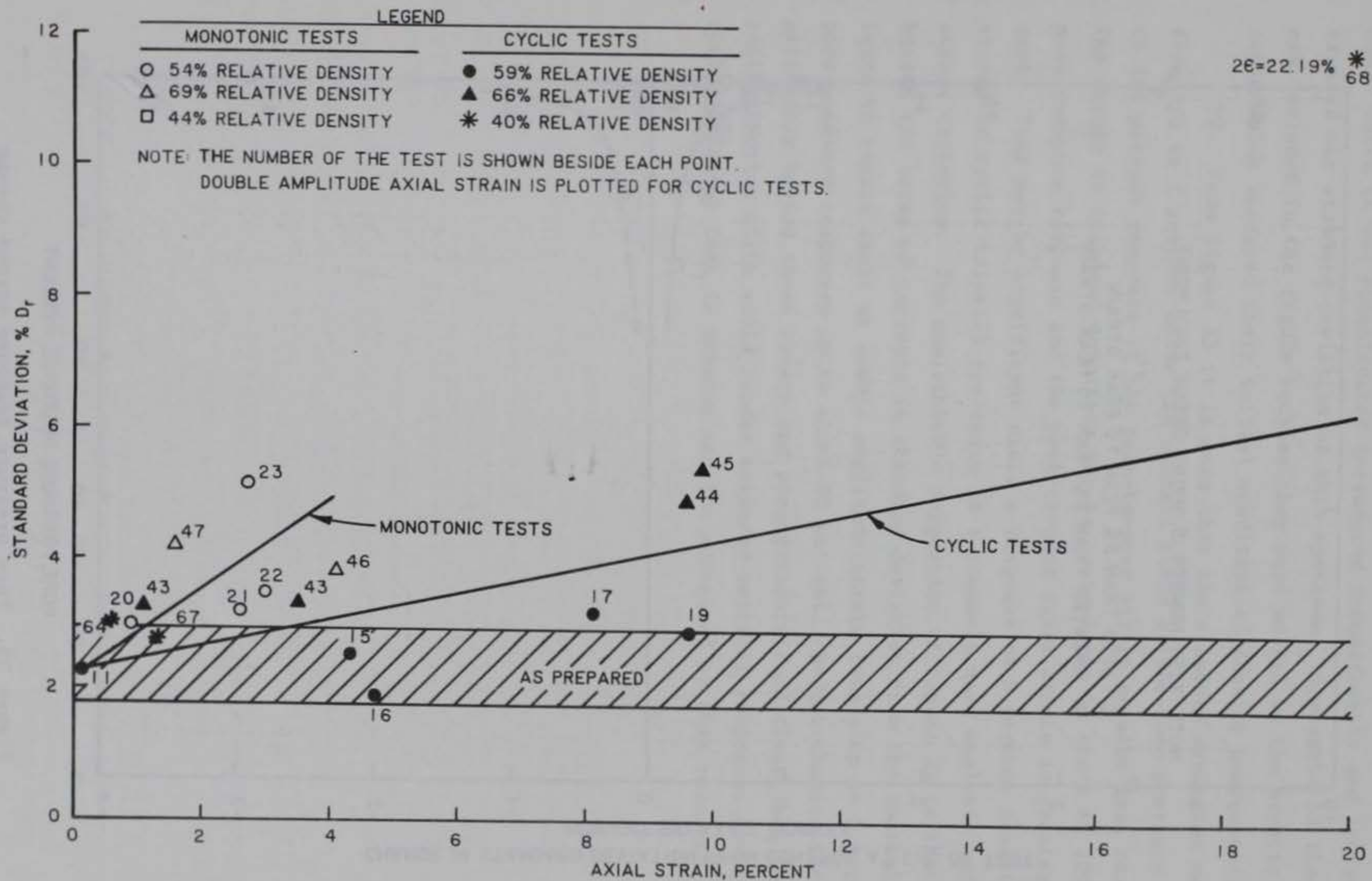
Figure 32. Axial strain versus standard deviation for cyclic and monotonic load tests
