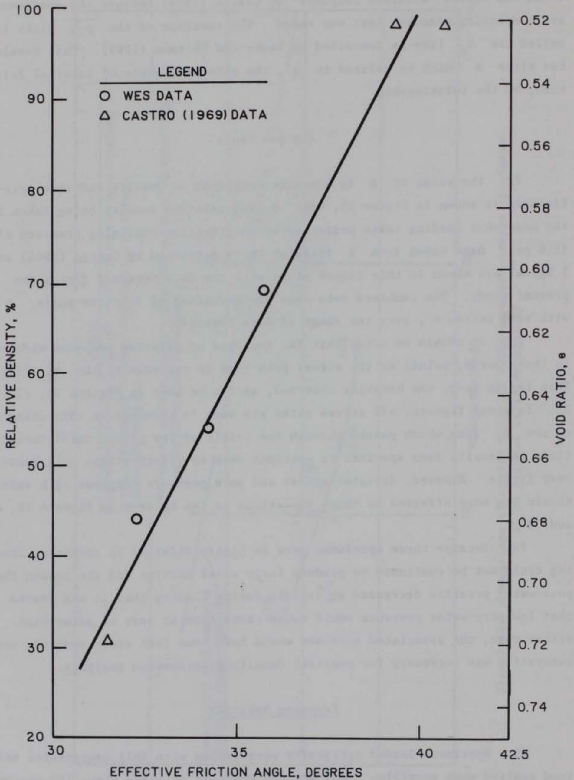
Figure 25. Relative density versus effective friction angle
