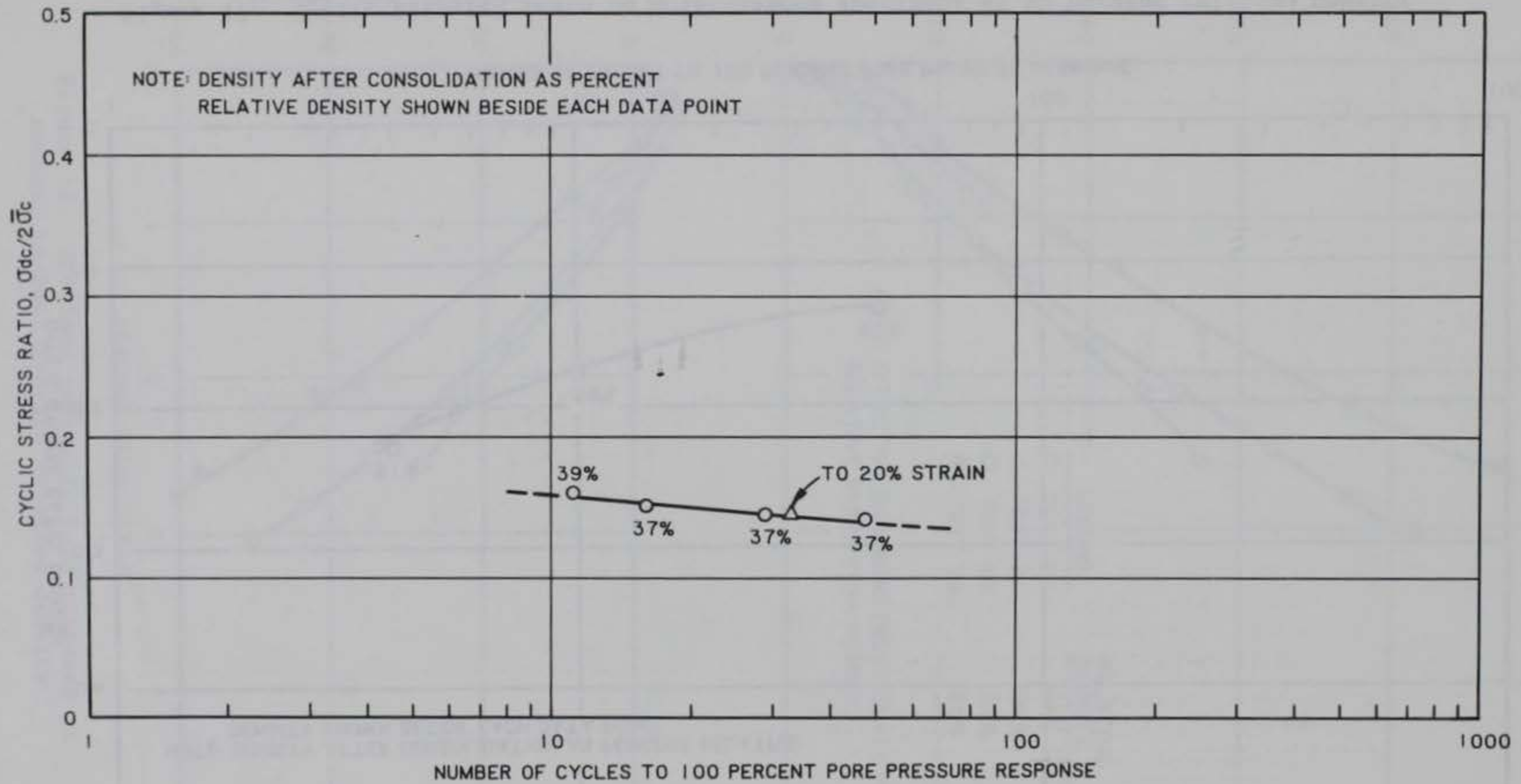
Figure 16. Cyclic triaxial tests on water-pluviated specimens at nominal 40 percent relative density
