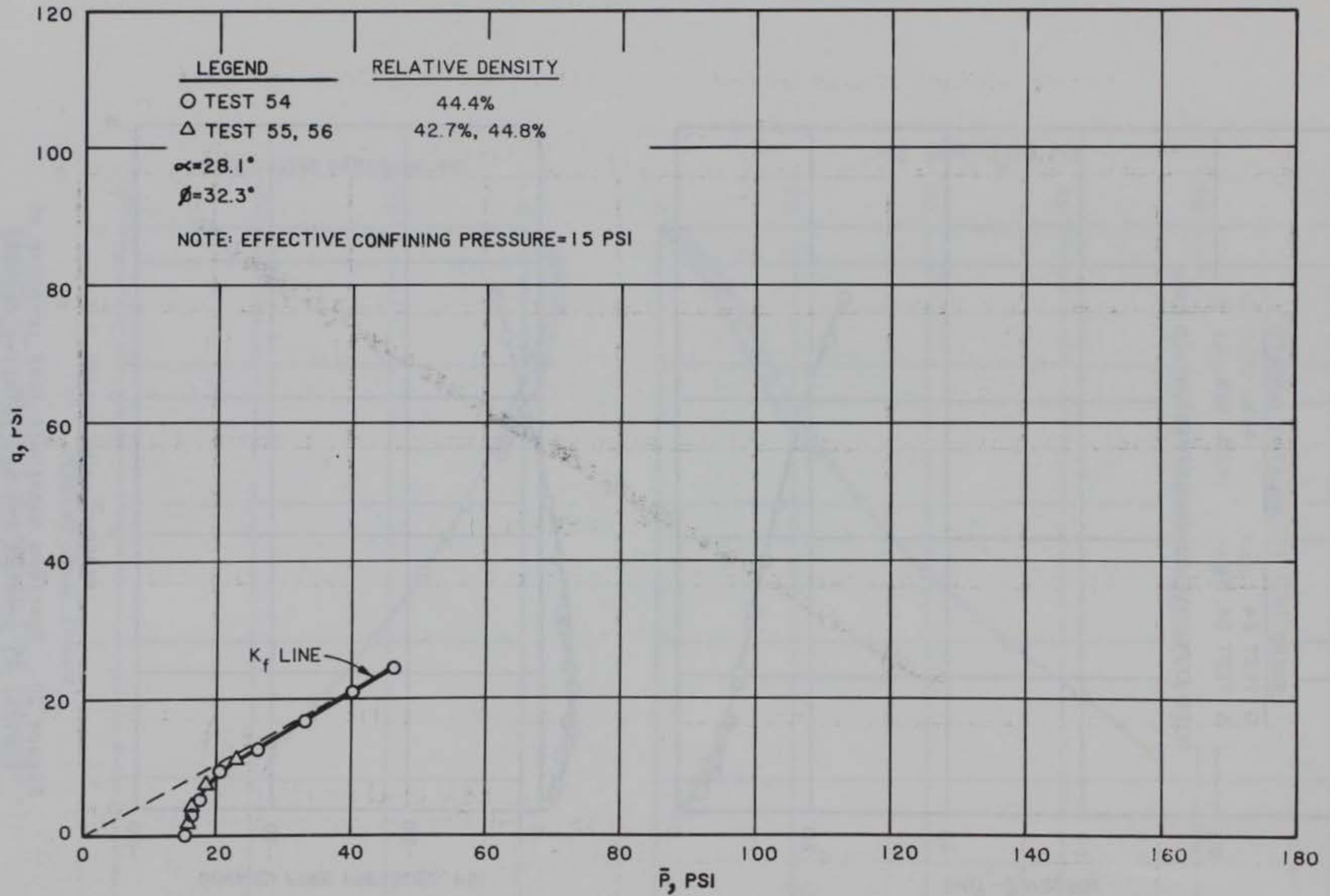
Figure 21. Specimen \bar{p} - \bar{q} response at 44 percent average relative density
