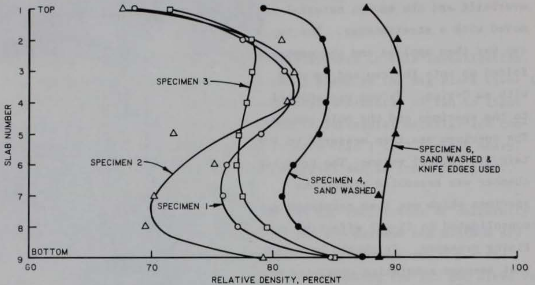
Figure D2. Vertical density patterns in early sand specimens
