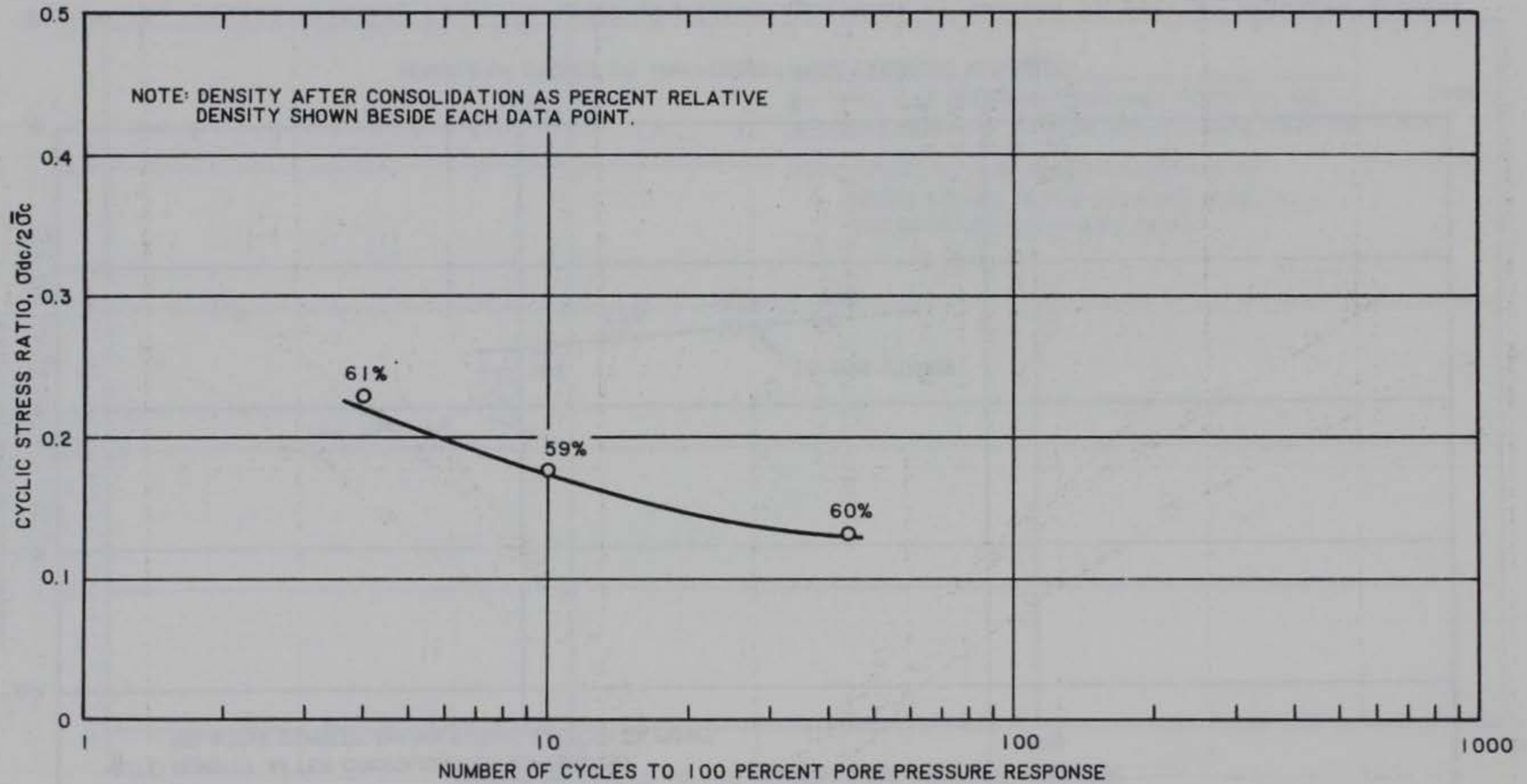
Figure 17. Cyclic triaxial tests on moist-tamped specimens at 60 percent relative density
