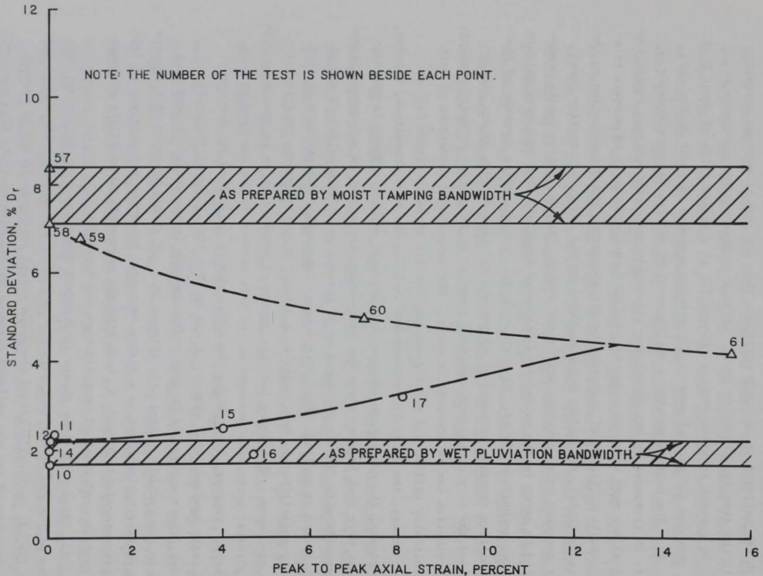
Figure 31. Redistribution in specimens at 60 percent relative density
