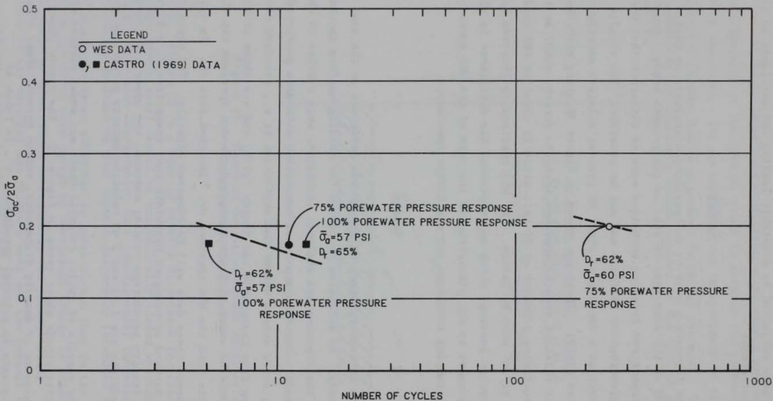
Figure 36. Comparison of Harvard and WES triaxial specimens subjected to cyclic loading
