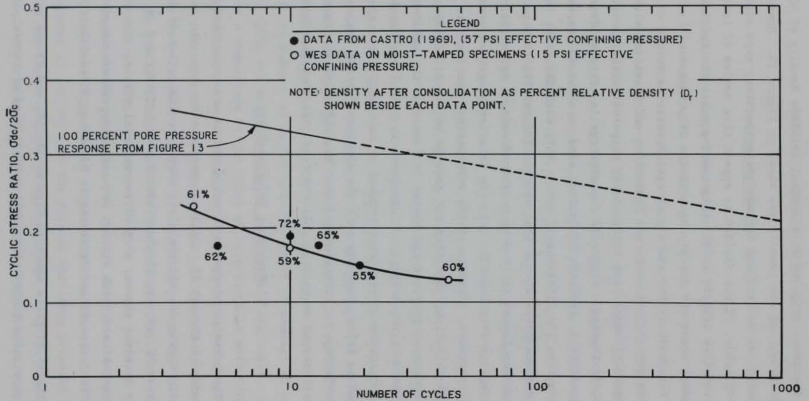
Figure 24. Comparison of cyclic triaxial tests on moist-tamped specimens at 60 percent relative density
