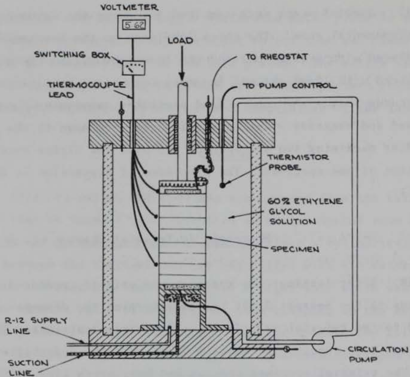
Figure 8. Schematic of triaxial equipment
