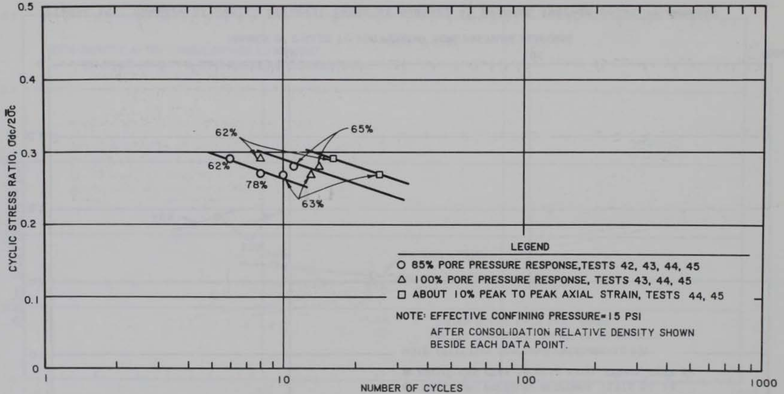
Figure 14. Summary of cyclic triaxial tests at nominal 70 percent average relative density
