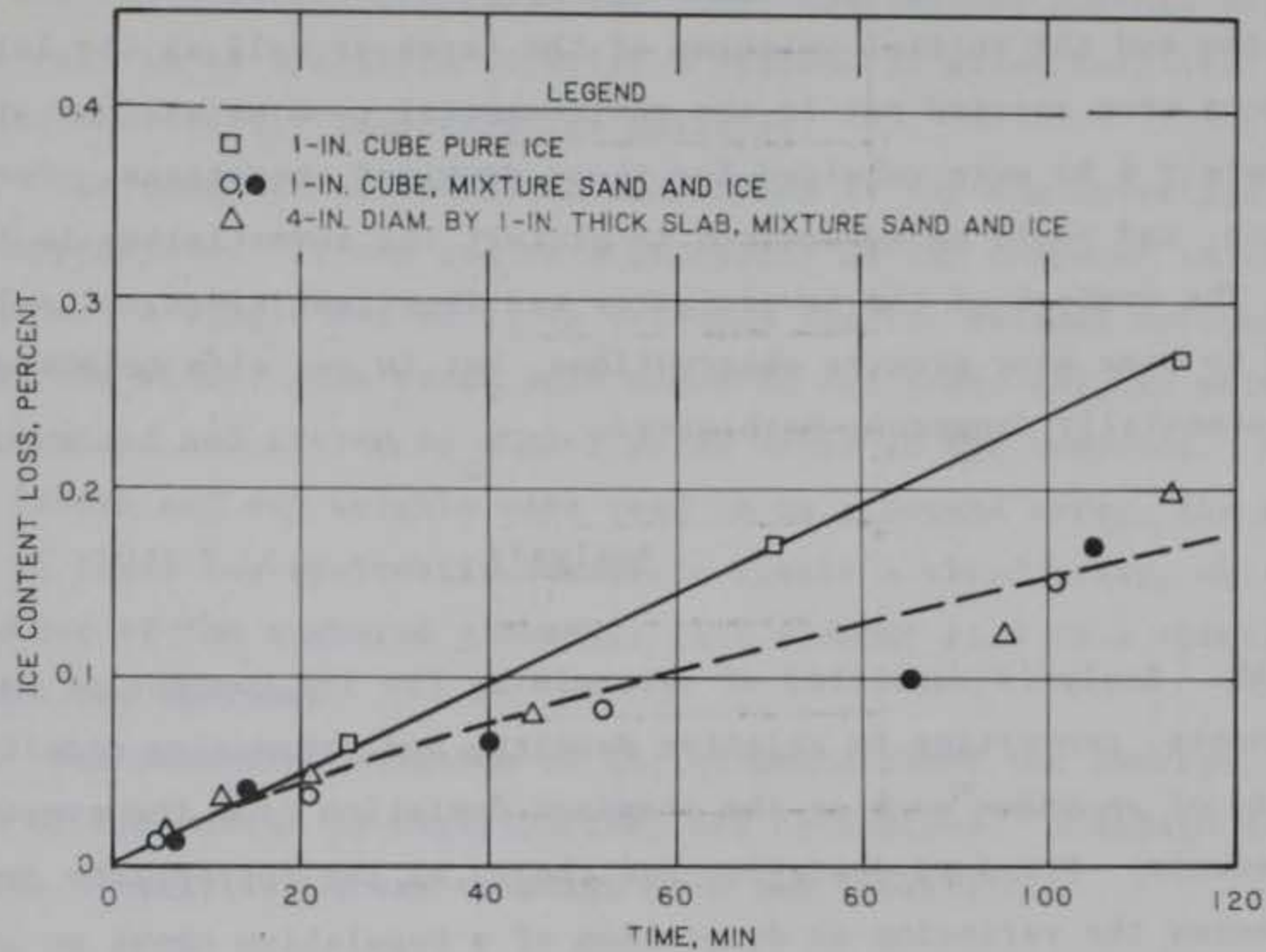
Figure 12. Sublimation versus time study
