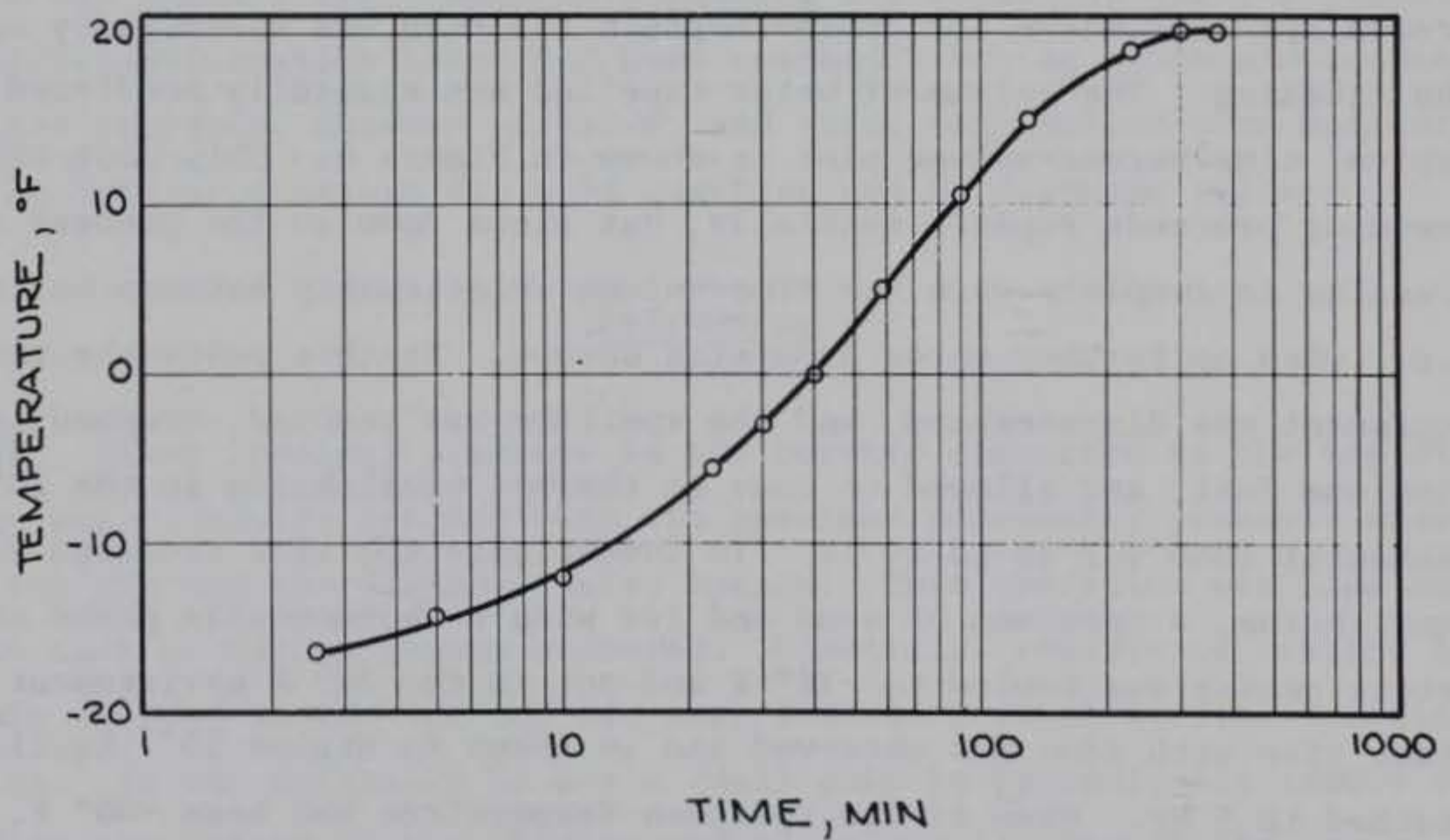
Figure 10. Temperature decay versus time
