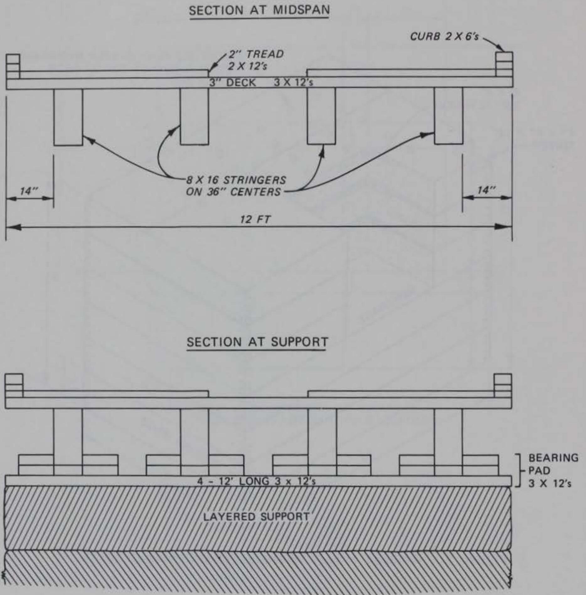
Figure 3. Bridge cross sections
