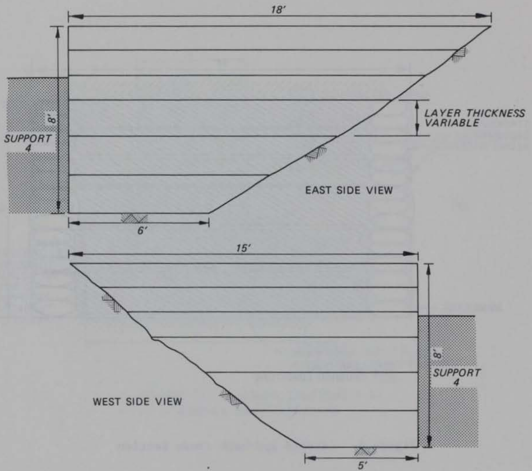
Figure 7. Layered approach side views
