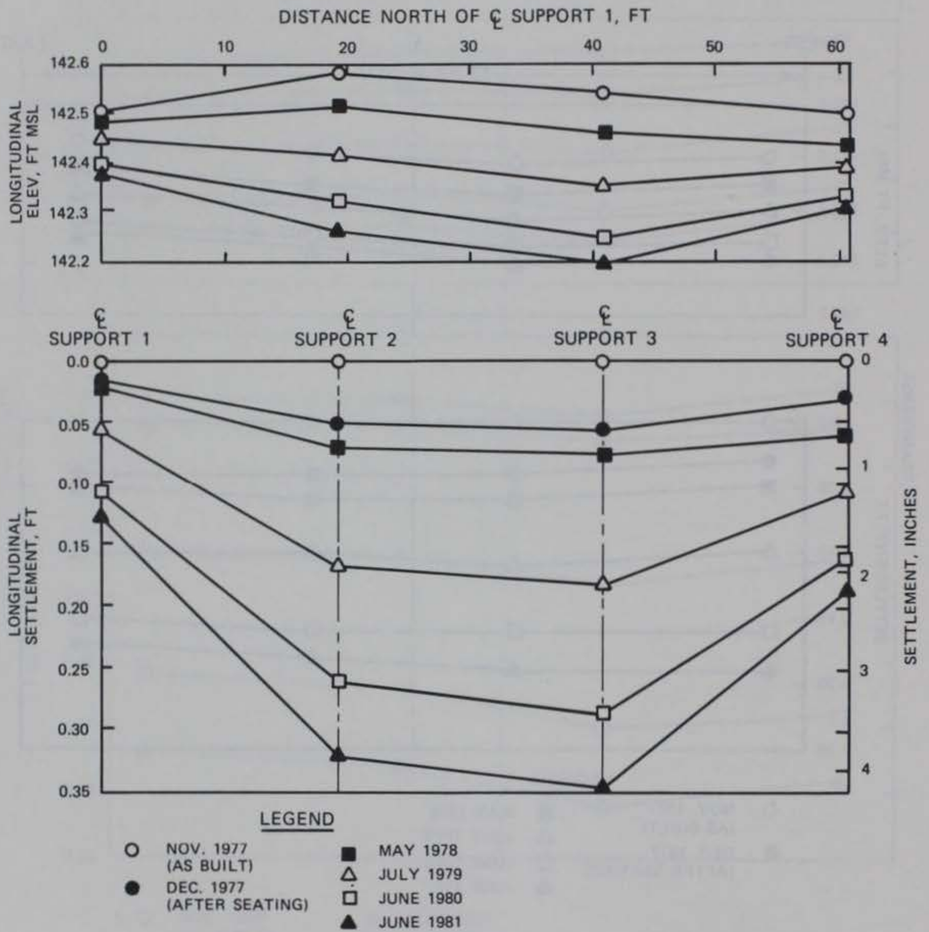
Figure 19. Summary of vertical bridge deck movement
