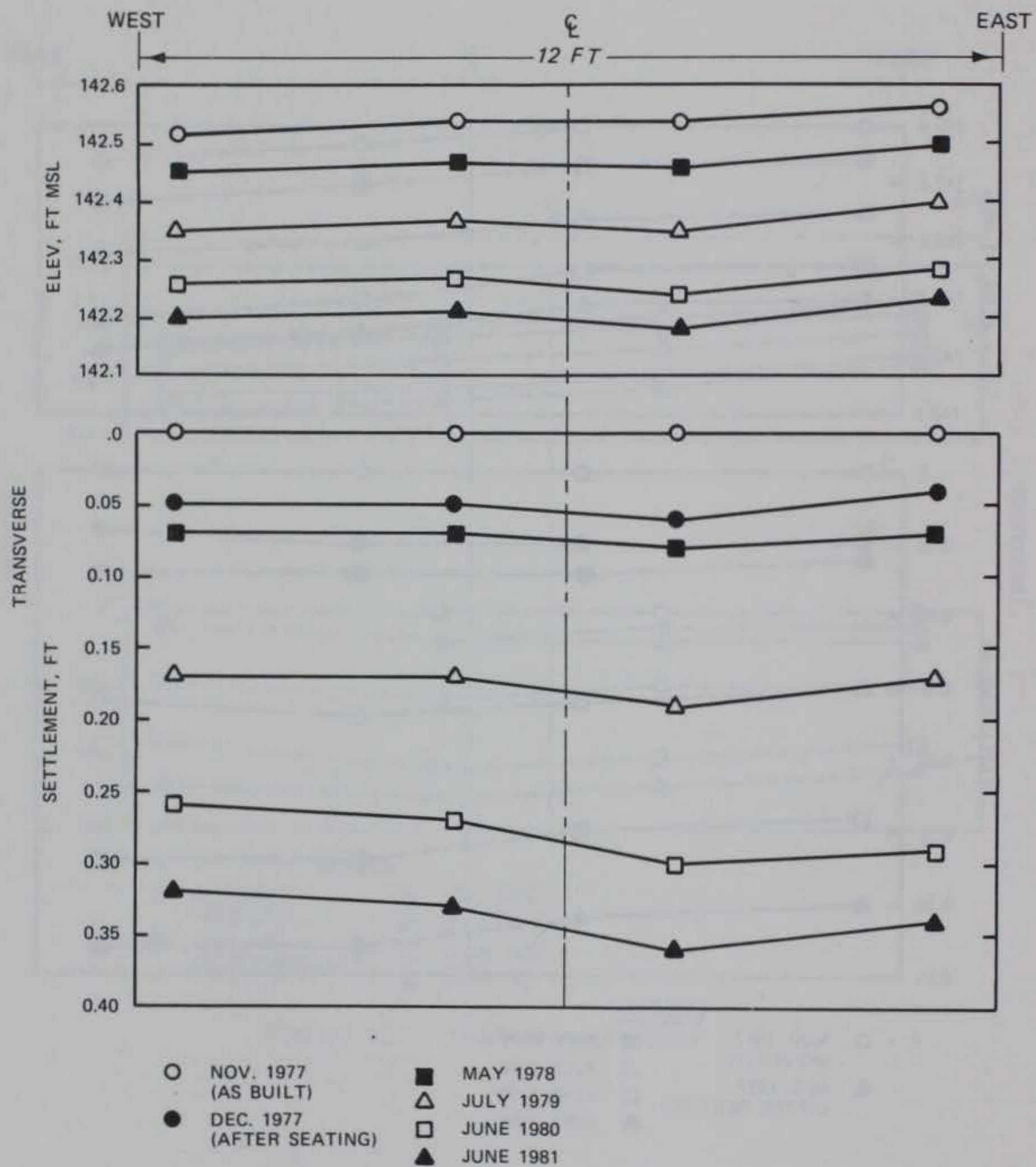
Figure 17. Tread above support 3
