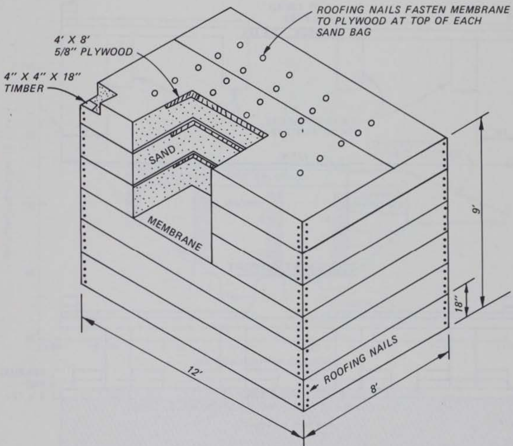
Figure 2. Sandbag bridge abutment (from Webster 1975)
