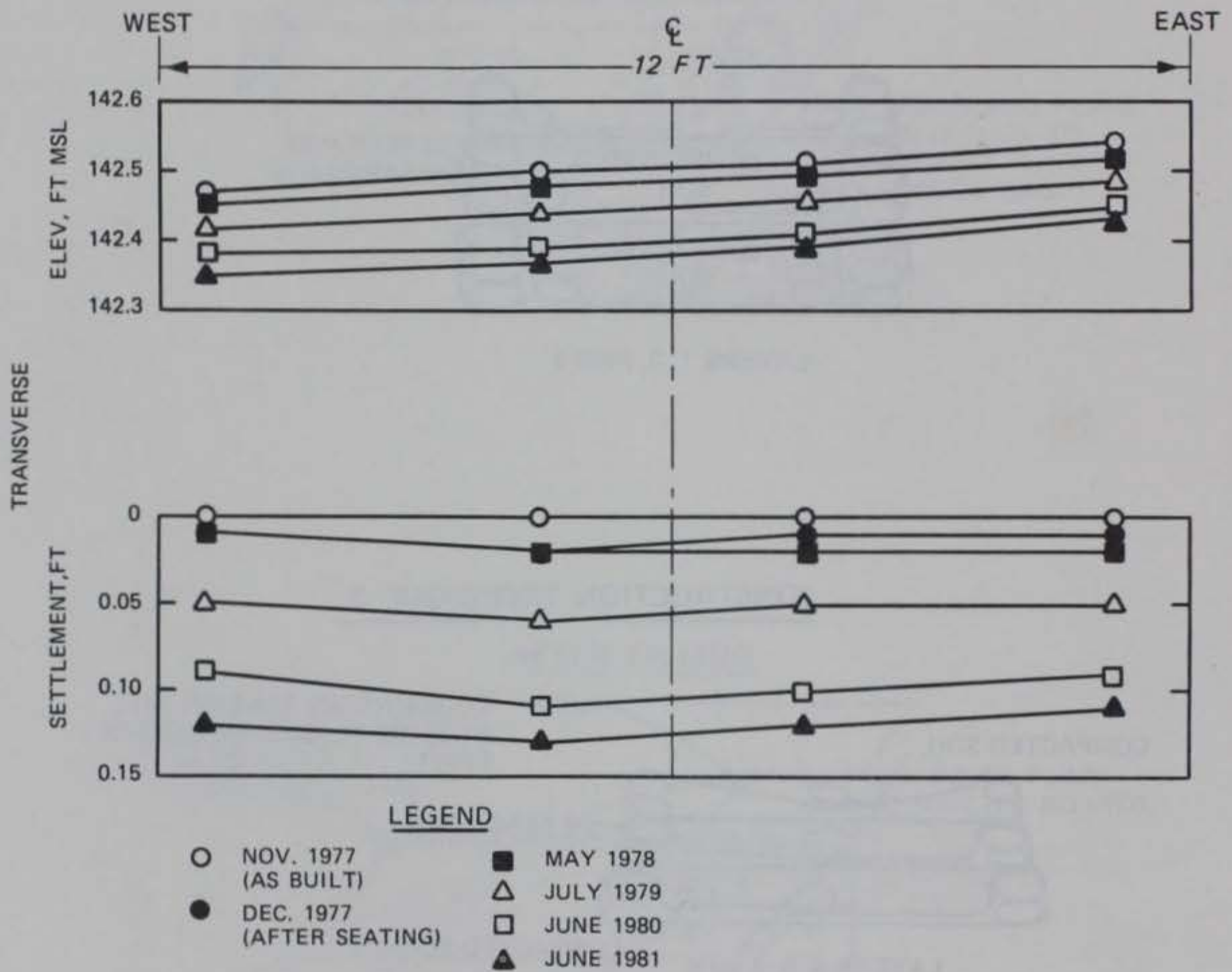
Figure 15. Tread above support 1
