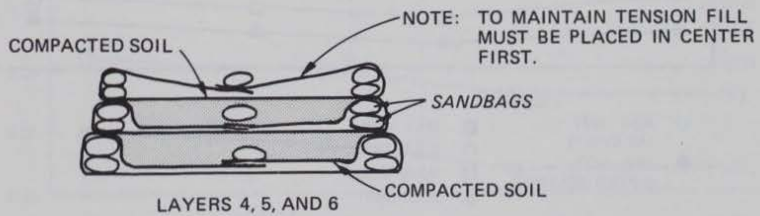
Figure 14. Approach construction techniques used
