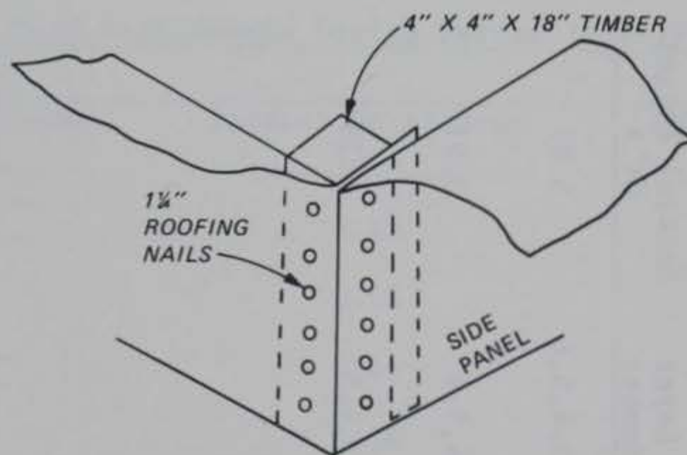
ASSEMBLED CORNER DETAIL
