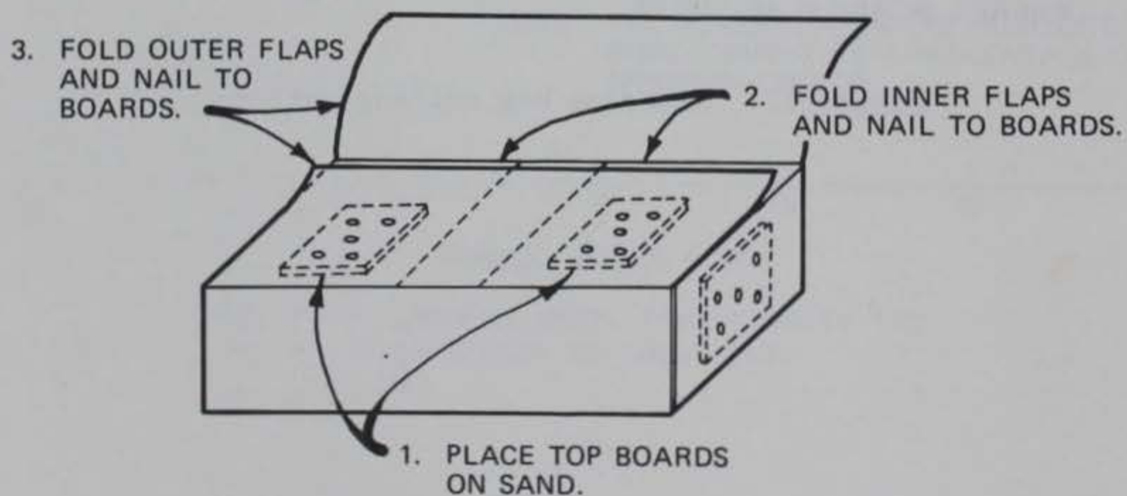
Figure 13. Membrane bag construction details
