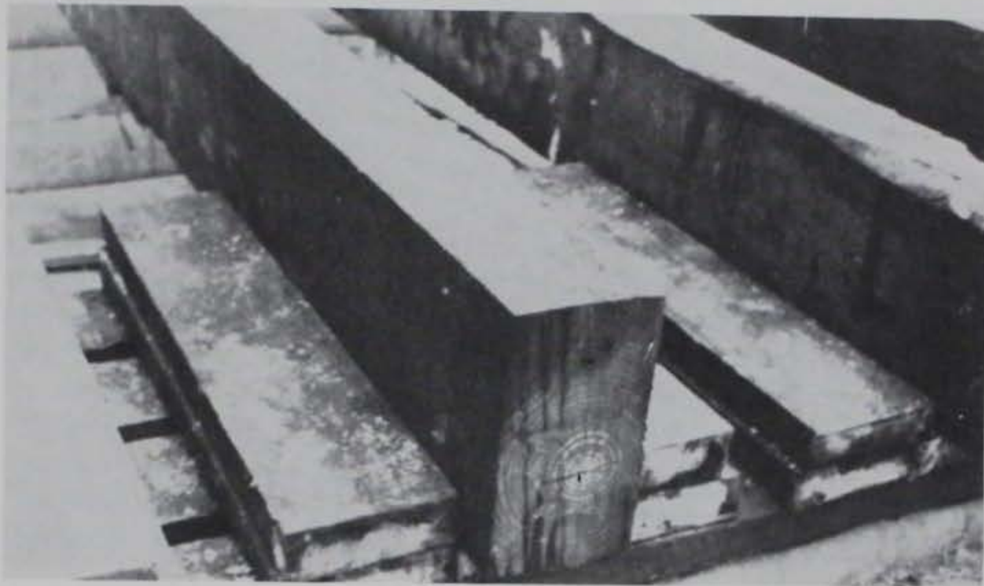
Photo 19. Stringer with lateral restraint above support
