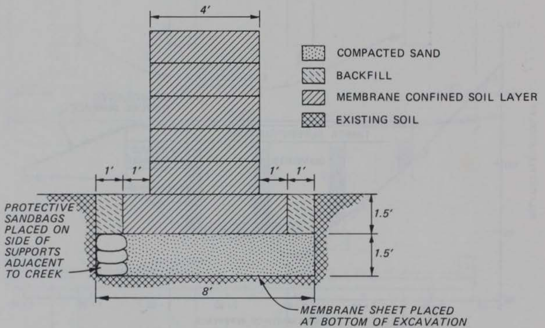
Figure 5. Membrane confined soil support and foundation
