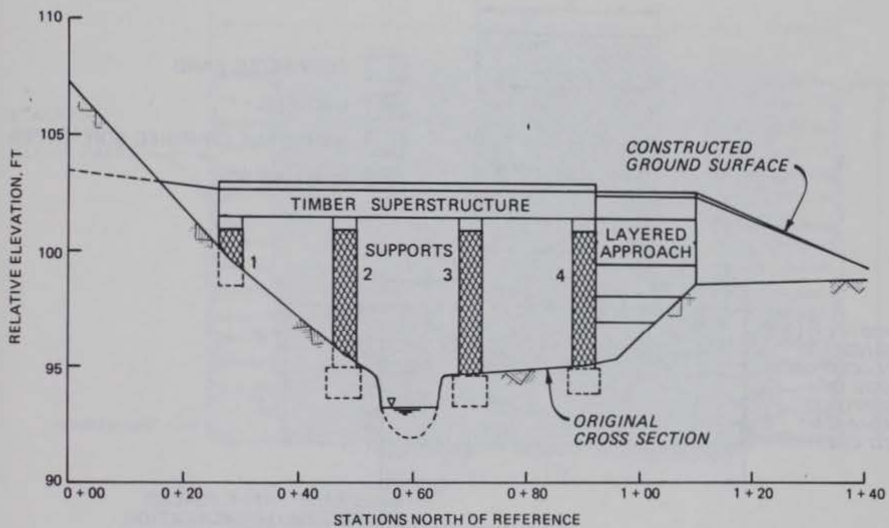
Figure 4. Original cross section along bridge centerline showing support locations
