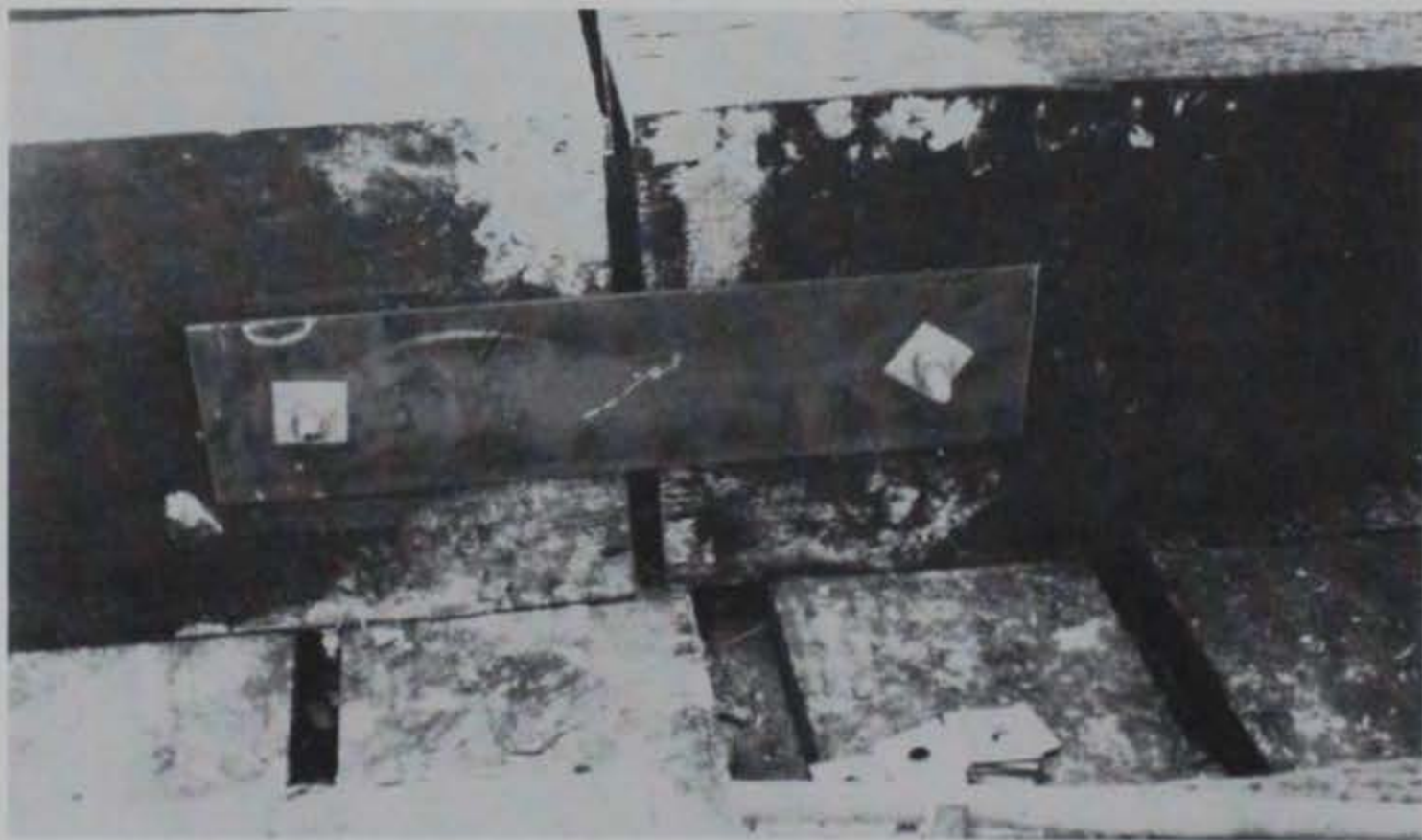
Photo 18. Stringer connection at interior supports
