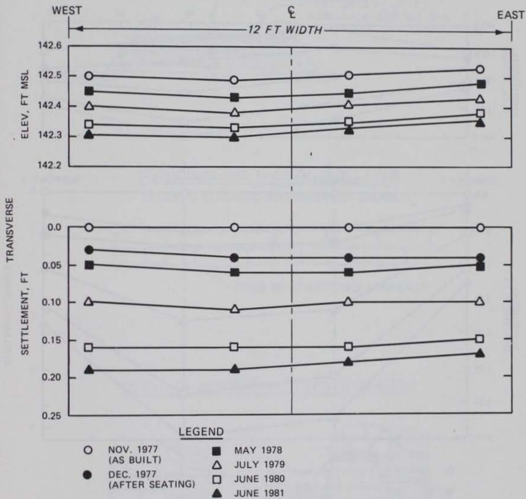
Figure 18. Tread above support 4
