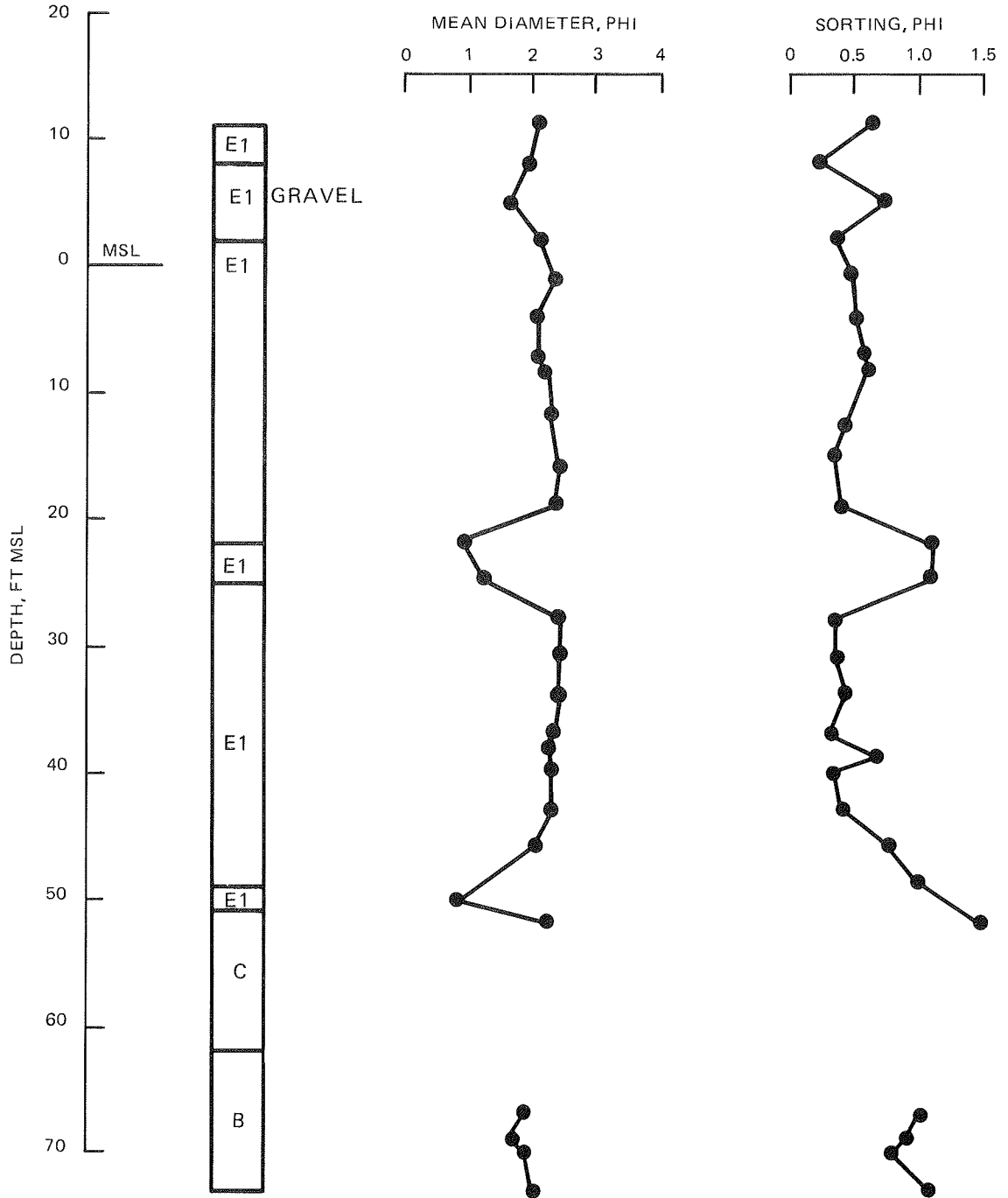
Figure 4. Sediment unit distribution, mean grain size, and sorting for Boring 2 (number 1 following unit designation denotes gravelly facies)
