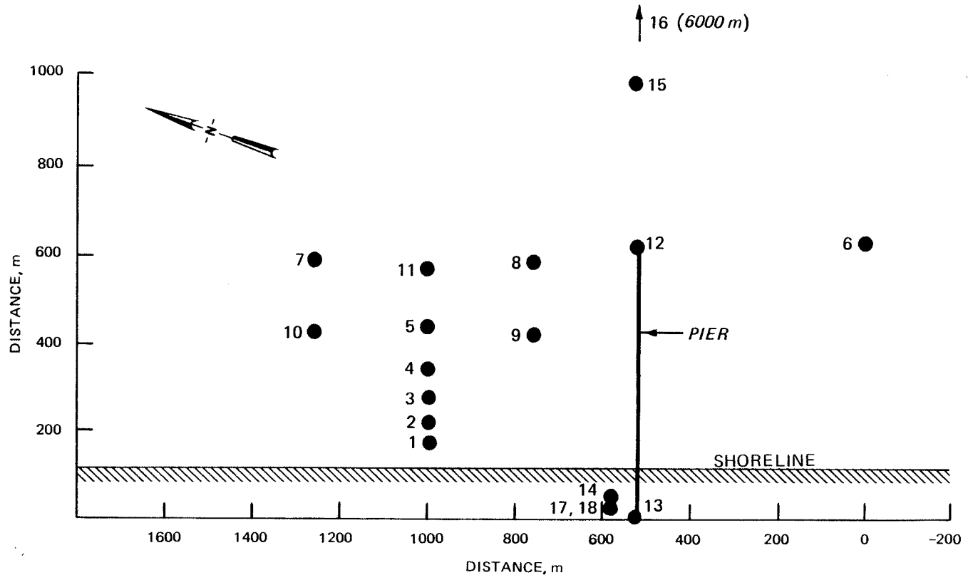
Figure 1. Nearshore waves and currents experiment station locations during DUCK '85
