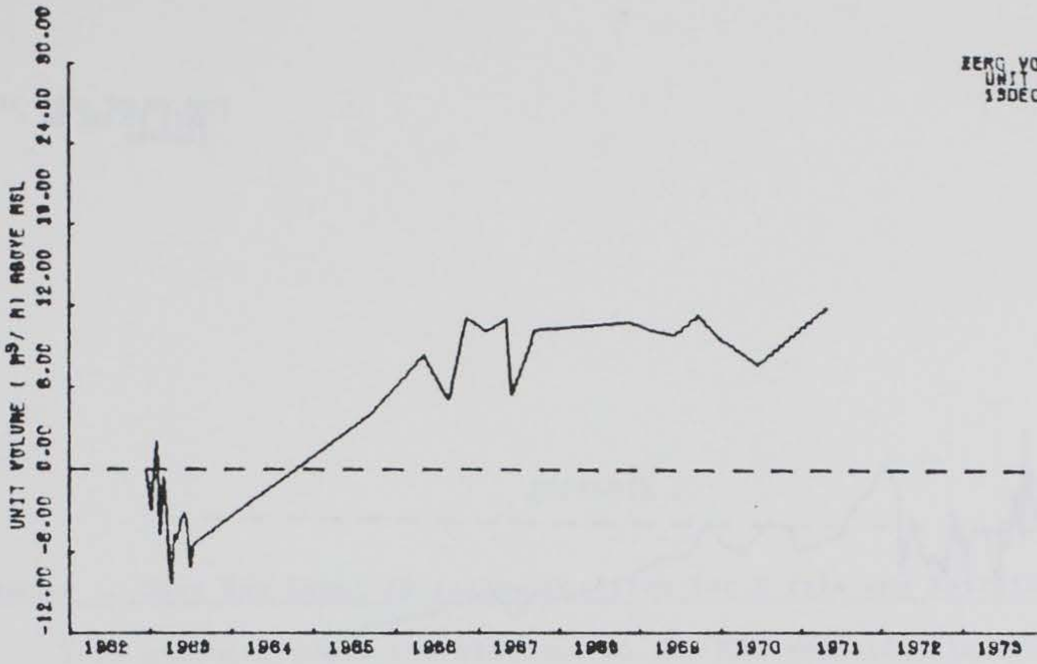
UNIT VOLUME CHANGES FOR PROFILE LINE 1 AT FAIRFIELD BEACH, CONNECTICUT
