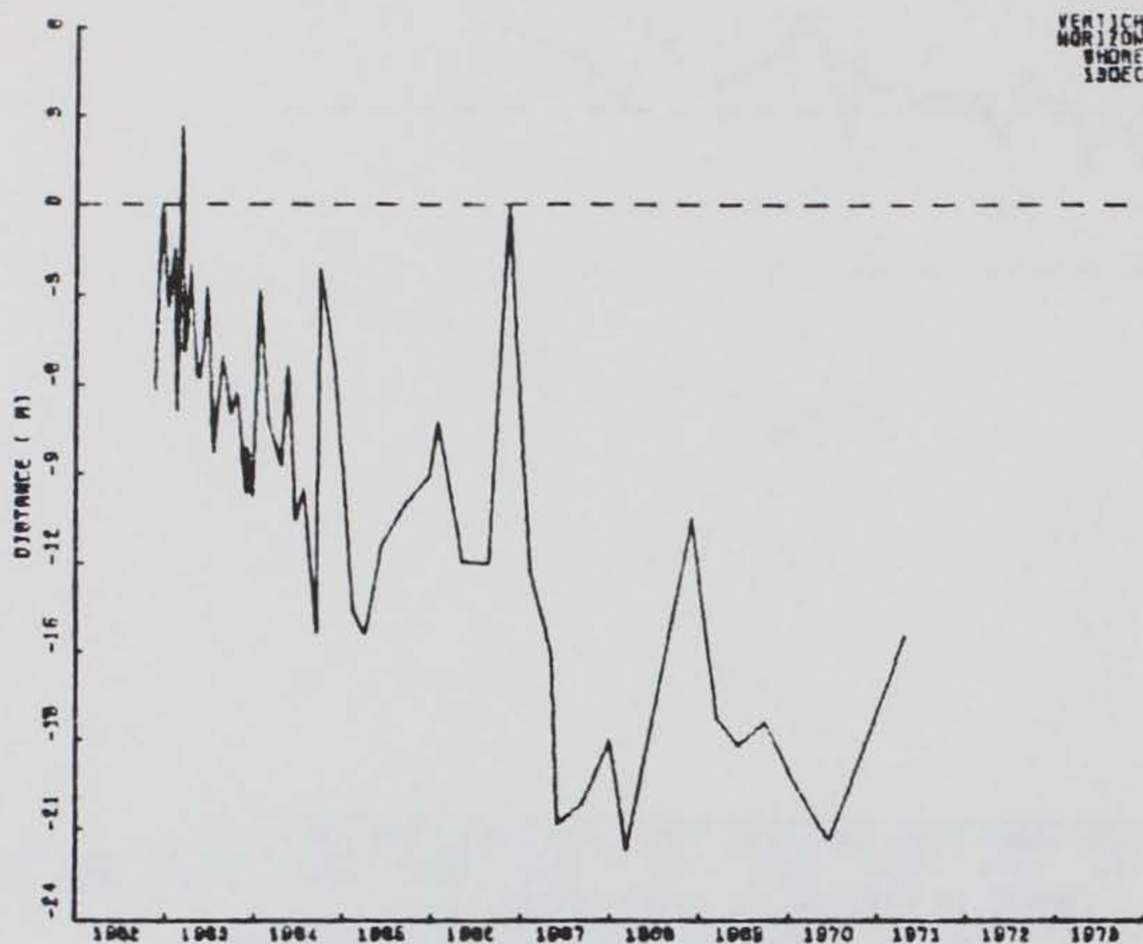
CHANGE IN DISTANCE TO SHORELINE AT PROFILE LINE 3 FAIRFIELD BEACH, CONNECTICUT
