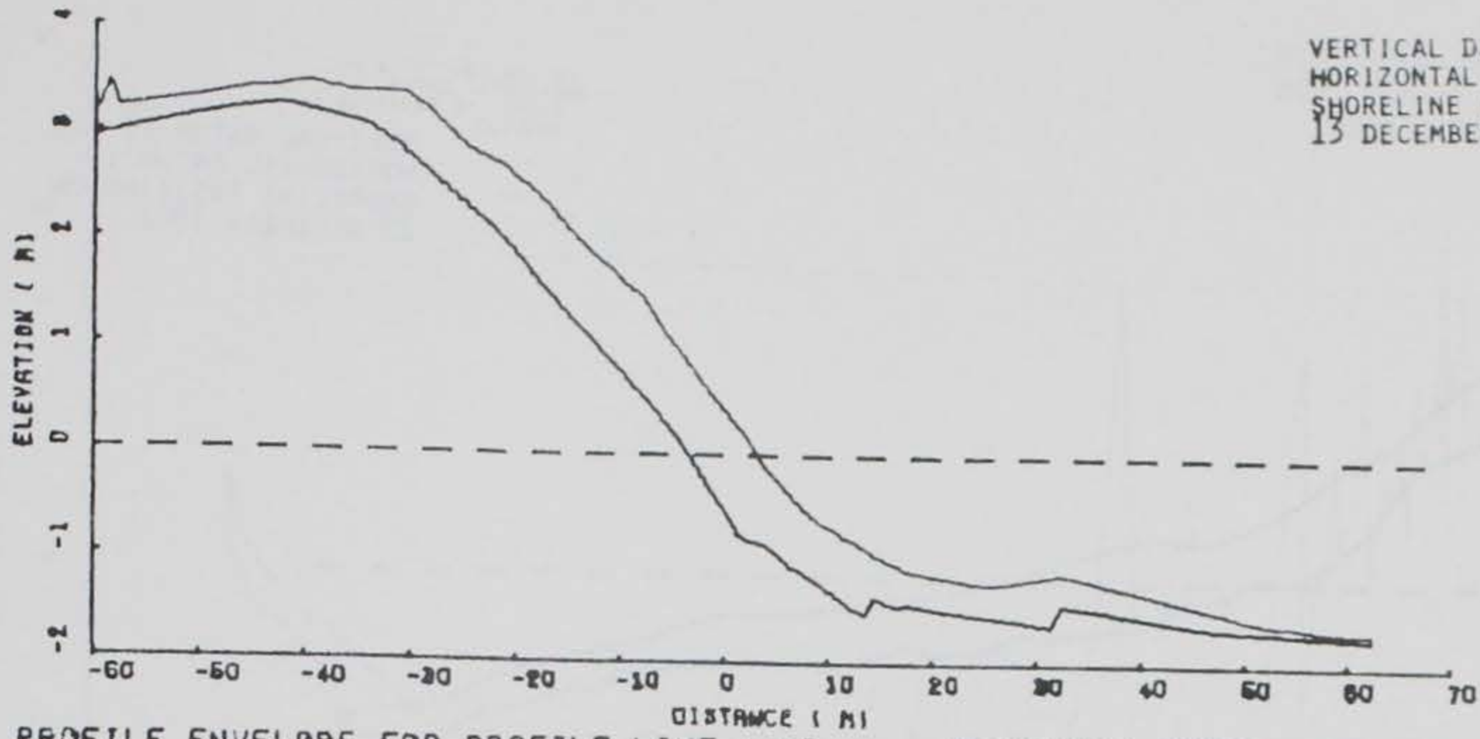
PROFILE ENVELOPE FOR PROFILE LINE 1 AT FAIRFIELD BEACH, CONNECTICUT 13DEC62 - 20APR71
