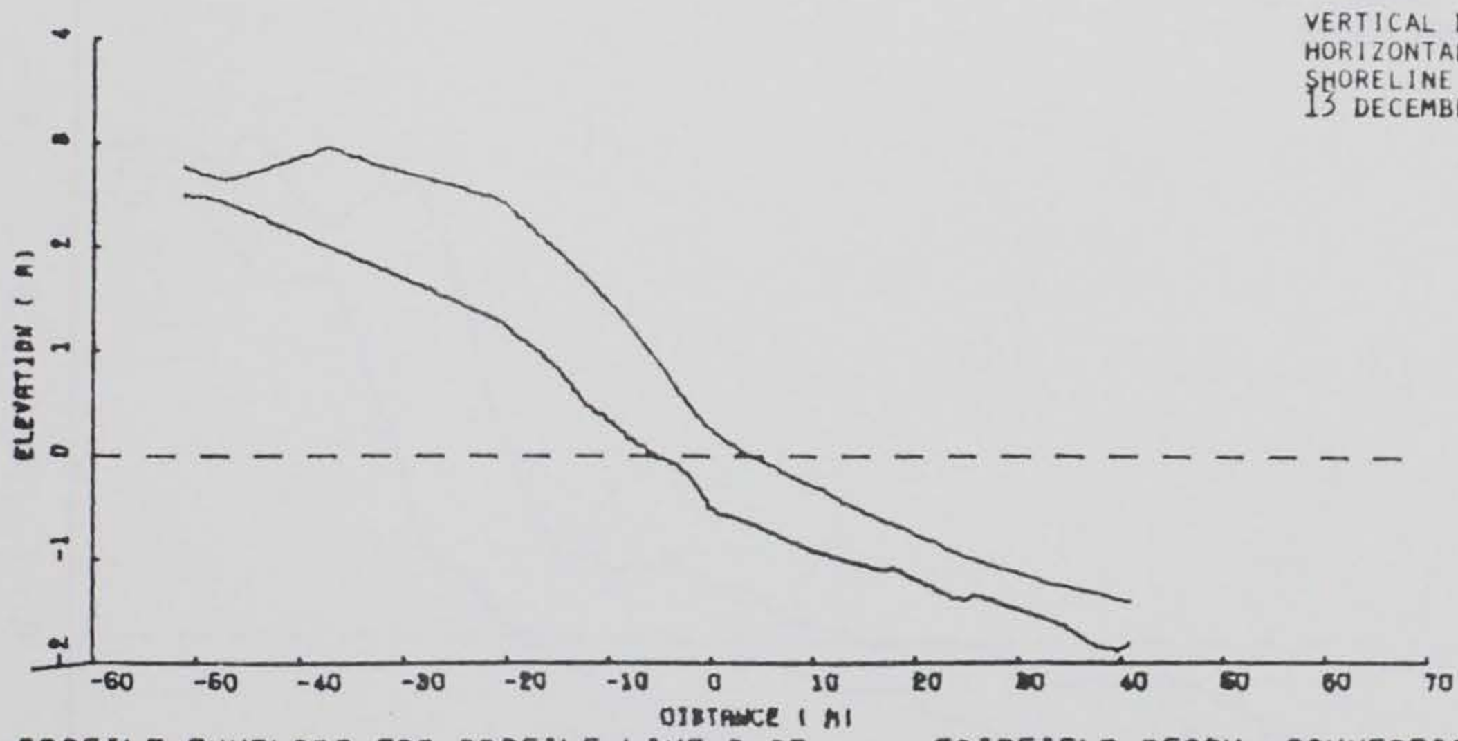
PROFILE ENVELOPE FOR PROFILE LINE 2 AT FAIRFIELD BEACH, CONNECTICUT 13NOV62 - 20APR71
