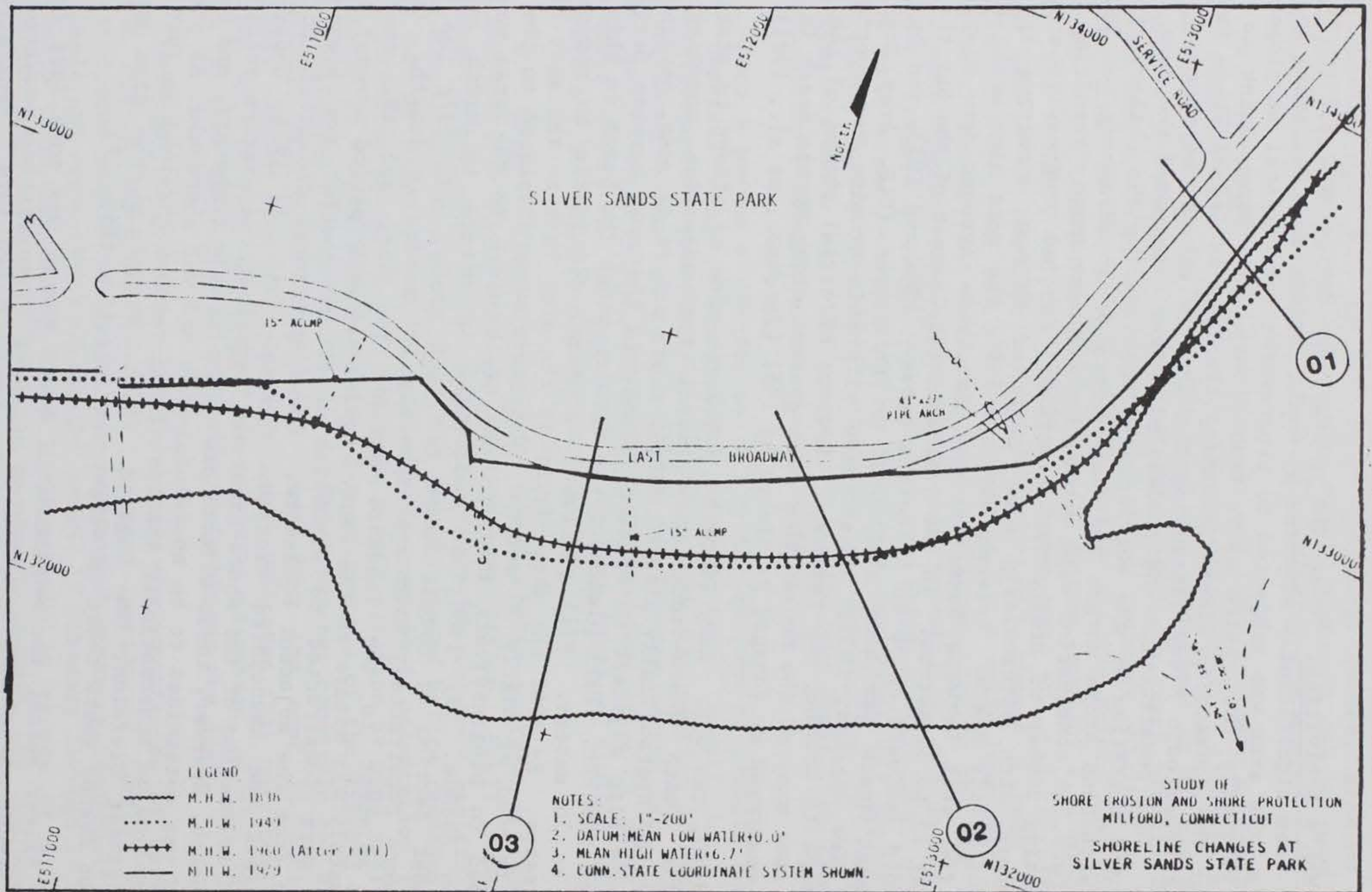
Figure 7. Silver Beach MHW positions as a function of time.
