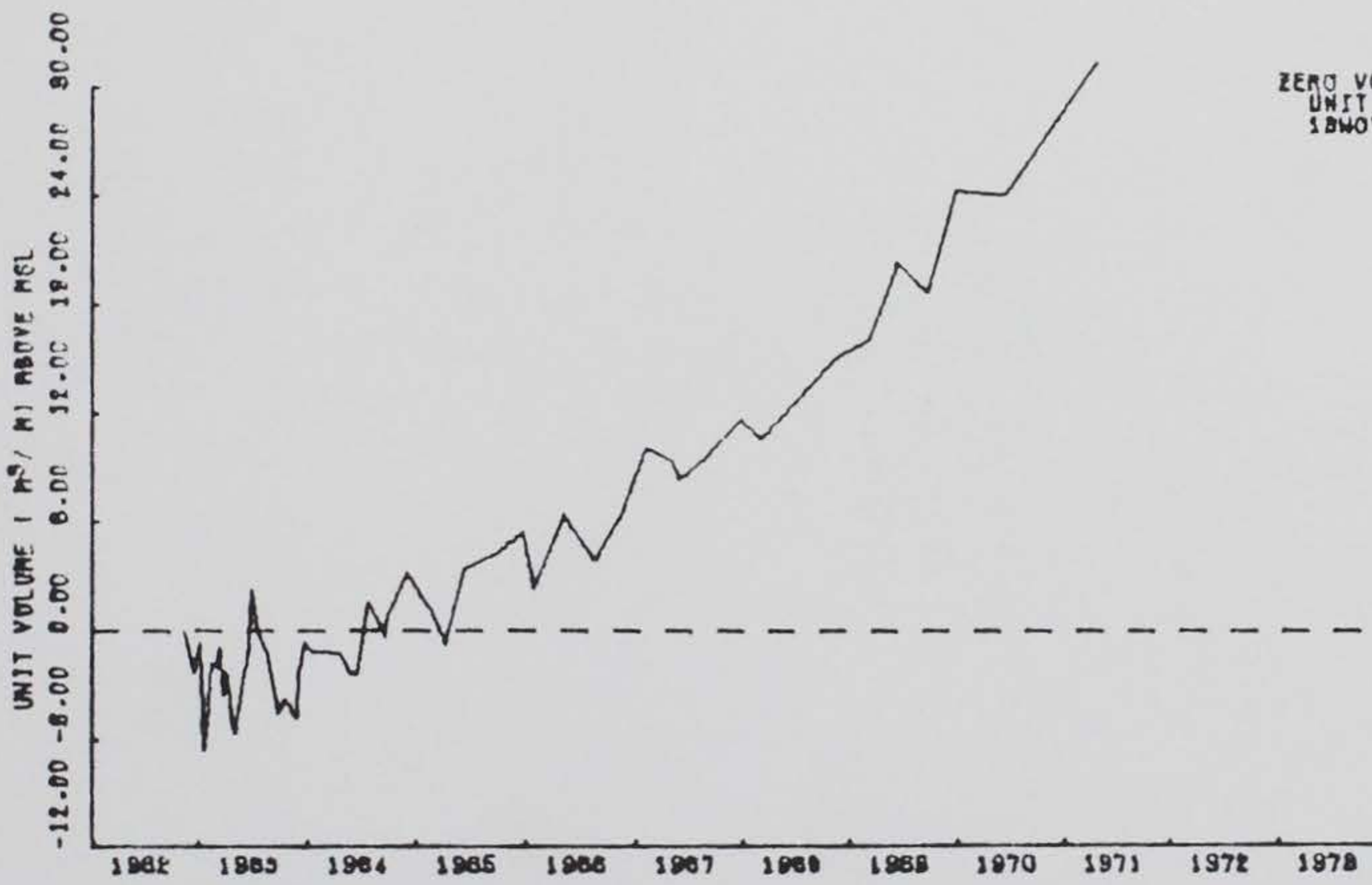
UNIT VOLUME CHANGES FOR PROFILE LINE 2 AT FAIRFIELD BEACH, CONNECTICUT
