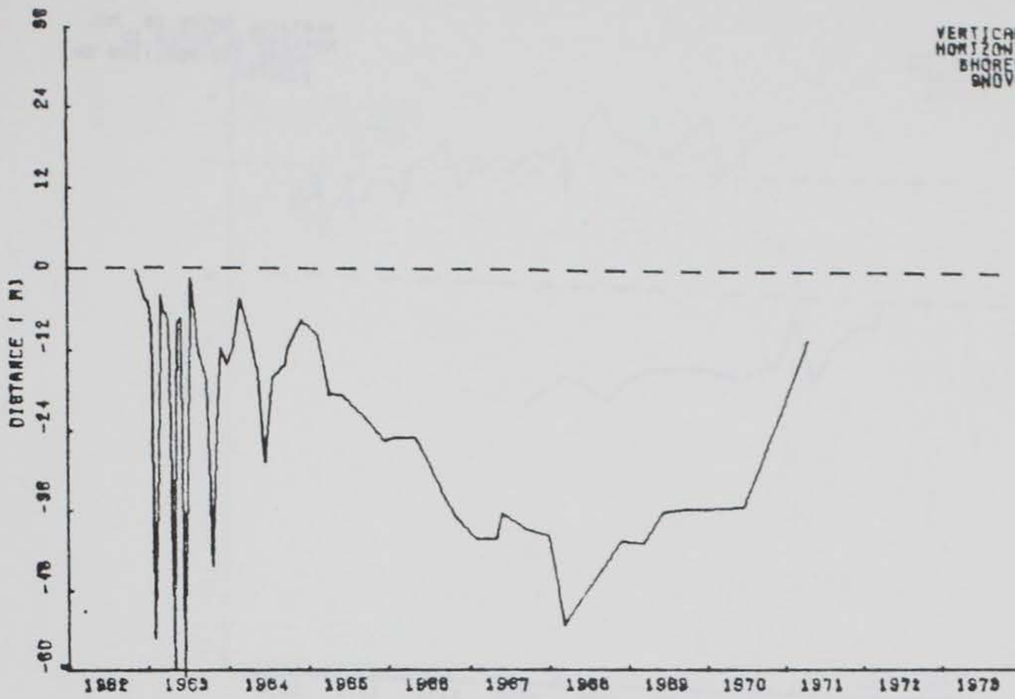
CHANGE IN DISTANCE TO SHOBE LINE AT PROFILE LINE 1 BEACH PROFILES MYRTLE BEACH CONN.
