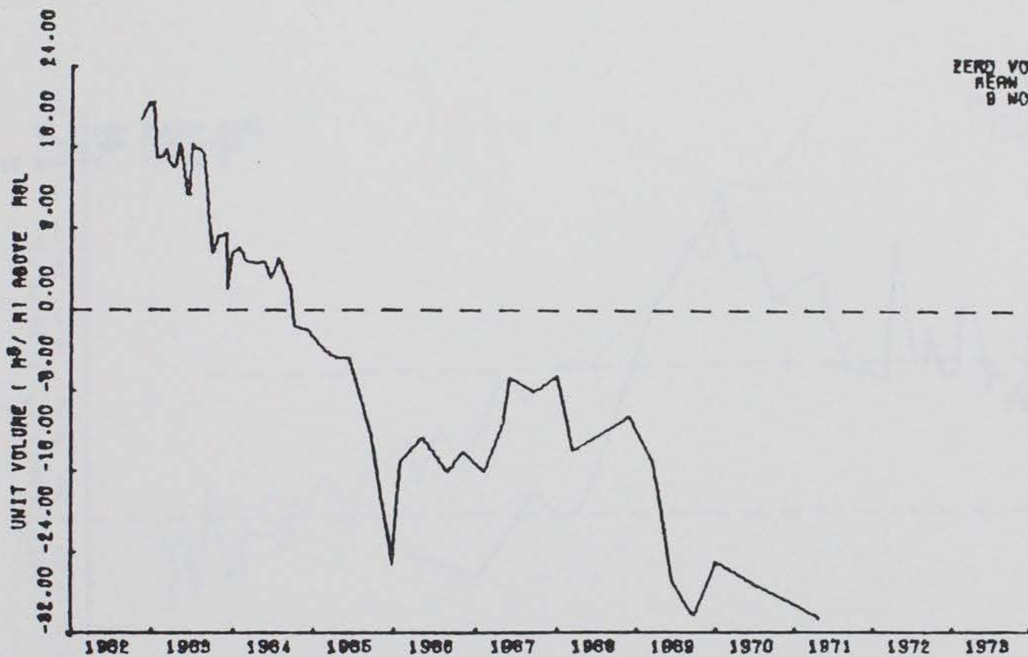
UNIT VOLUME CHANGES FOR PROFILE LINE 2 AT BEACH PROFILES MYRTLE BEACH CONNECTICUT
