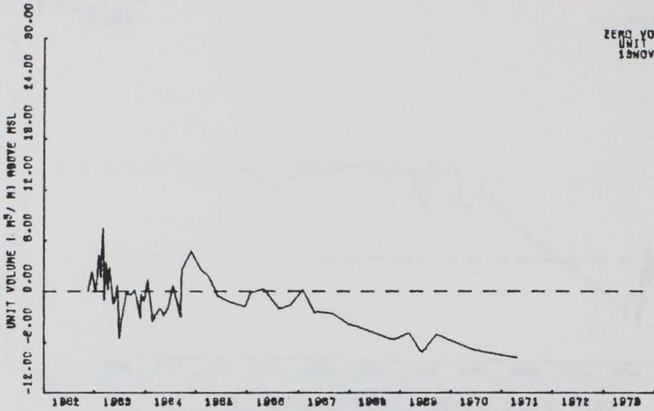
UNIT VOLUME CHANGES FOR PROFILE LINE 3 AT FAIRFIELD BEACH, CONNECTICUT
