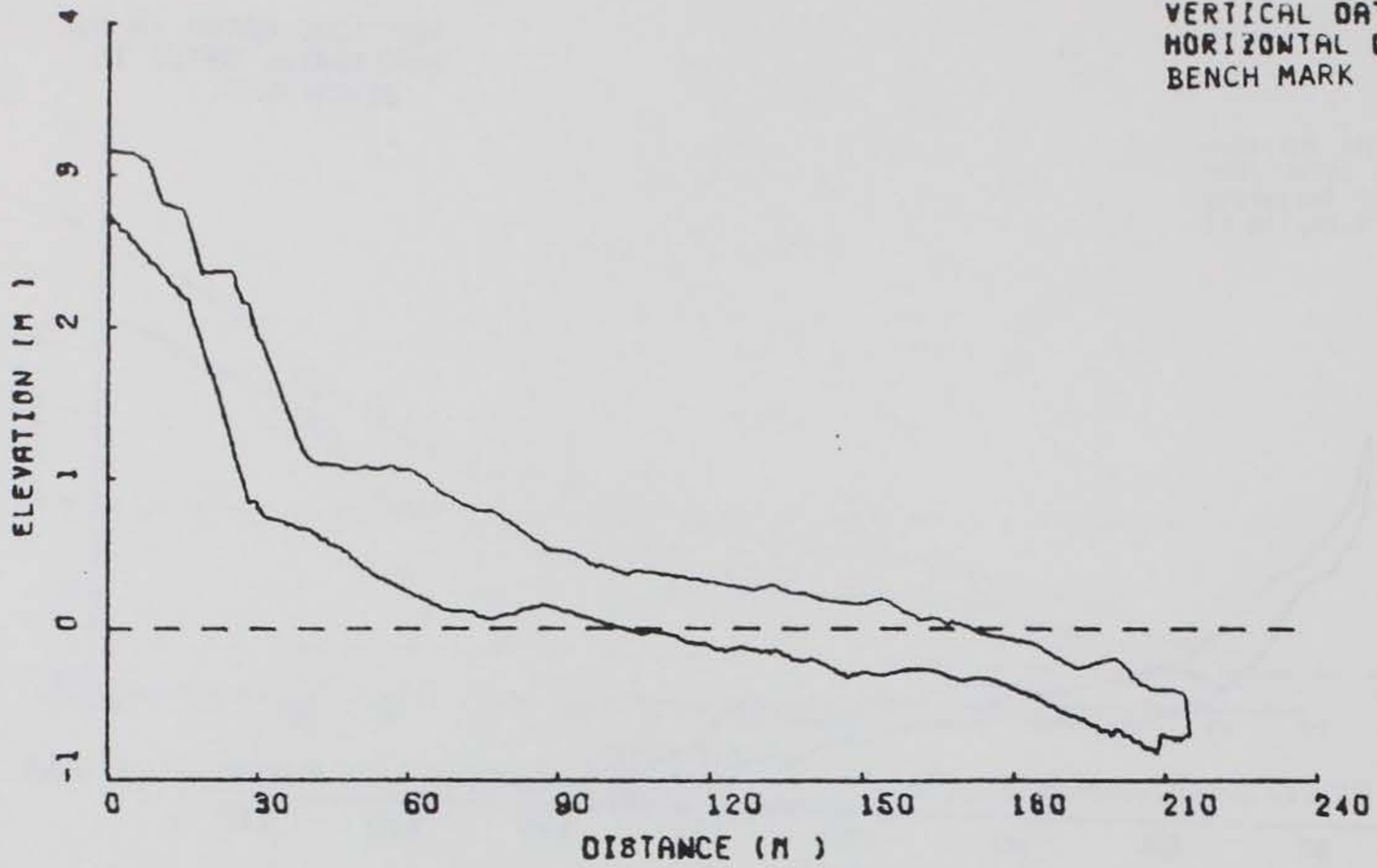
PROFILE ENVELOPE FOR PROFILE LINE 1 AT BEACH PROFILES MYRTLE BEACH, CONNECTICUT. 9 NOVEMBER 1962 - 19 APRIL 1971
