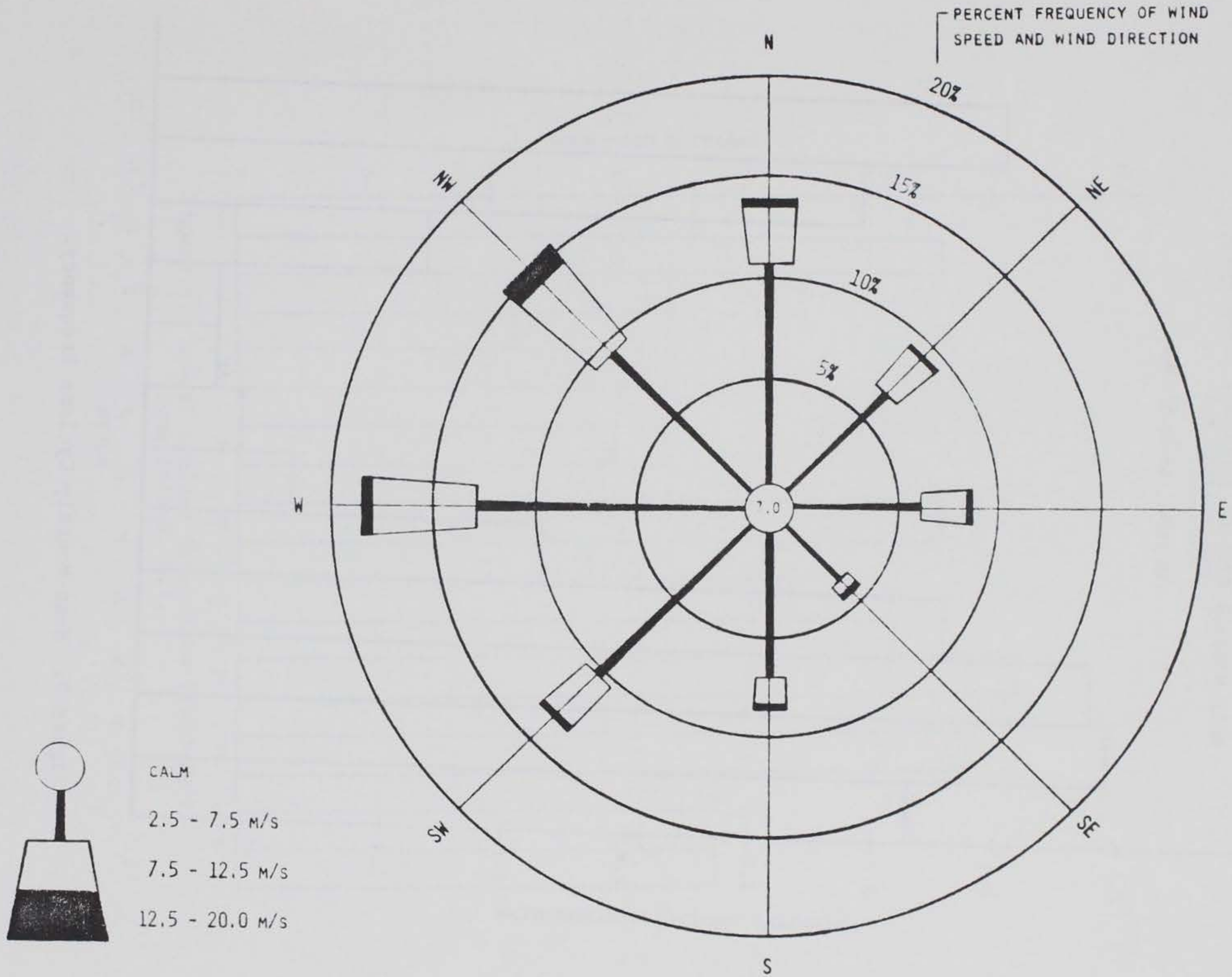
Figure 4. Wind rose (Bridgeport, Connecticut) for the period 1 January 1962 through 31 December 1971.
