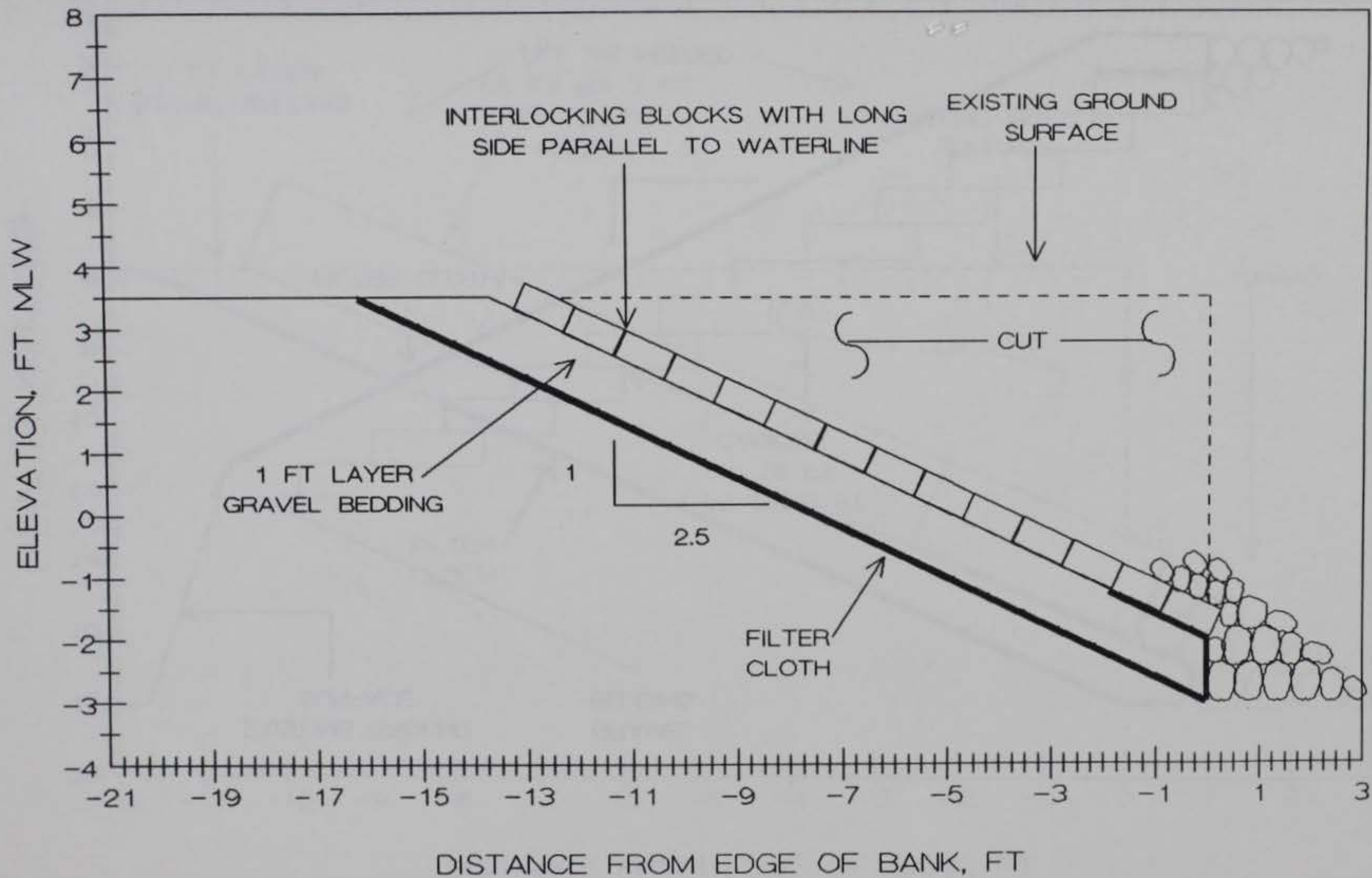
FIGURE 42. INTERLOCKING CONCRETE BLOCK REVETMENT PROPOSED FOR SITE 10
