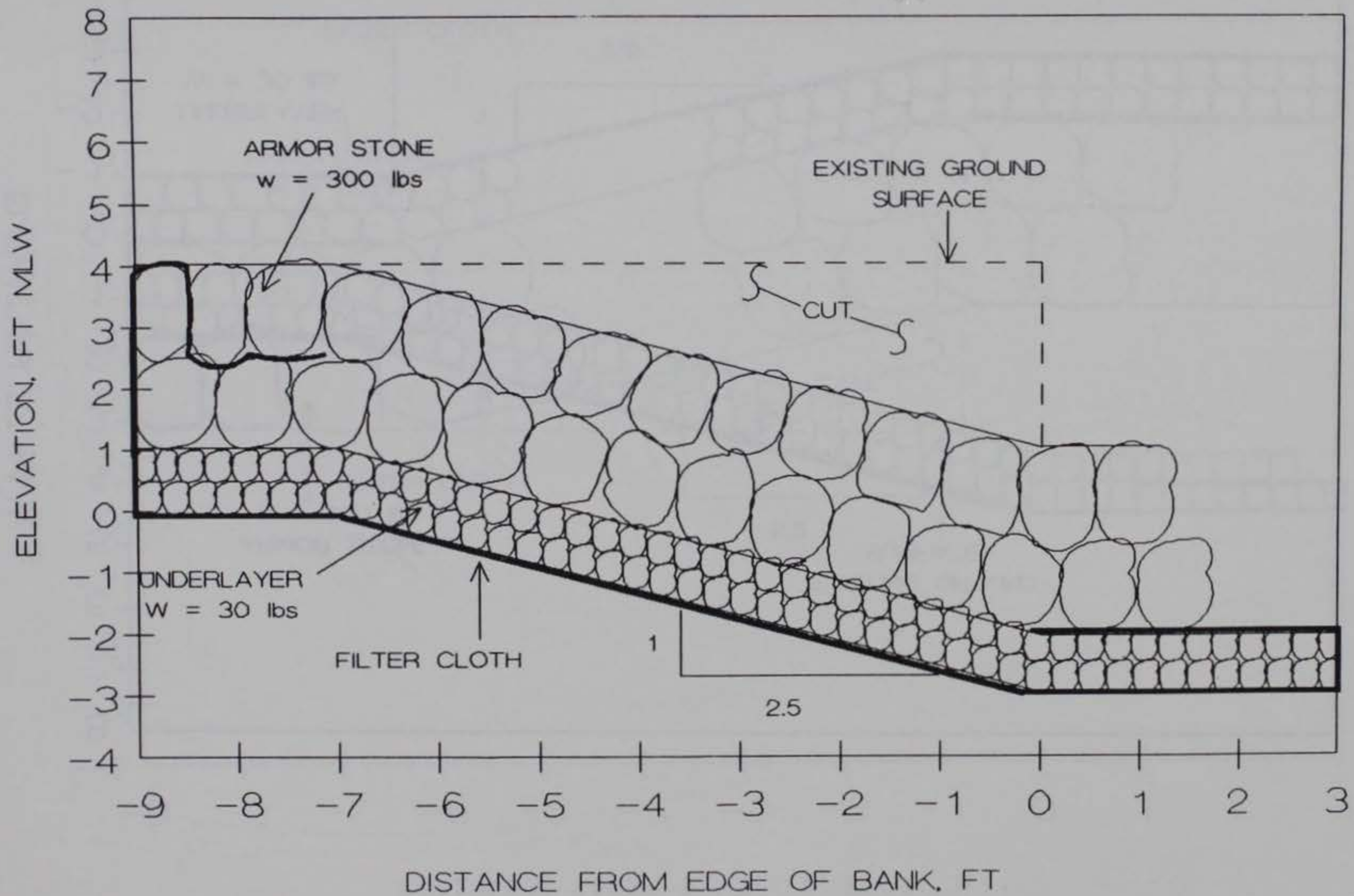
FIGURE 26. PLACED RIPRAP REVETMENT PROPOSED FOR SITE 7
