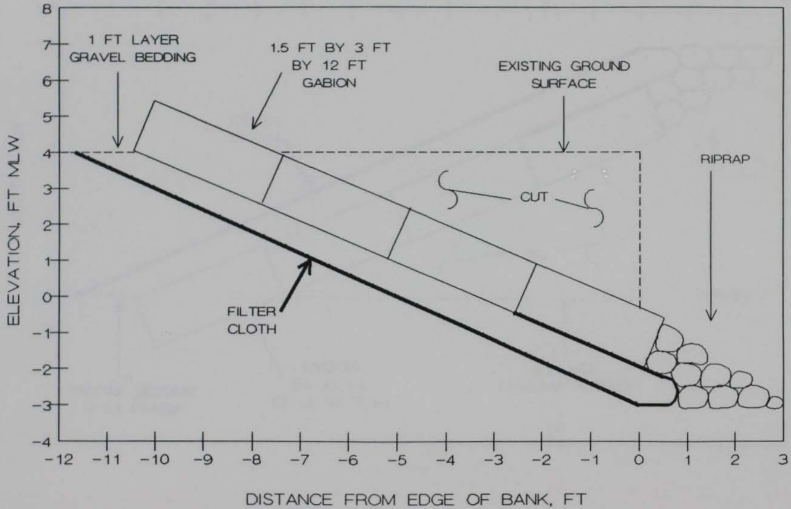
FIGURE 47. GABION REVETMENT PROPOSED FOR SITE 4
