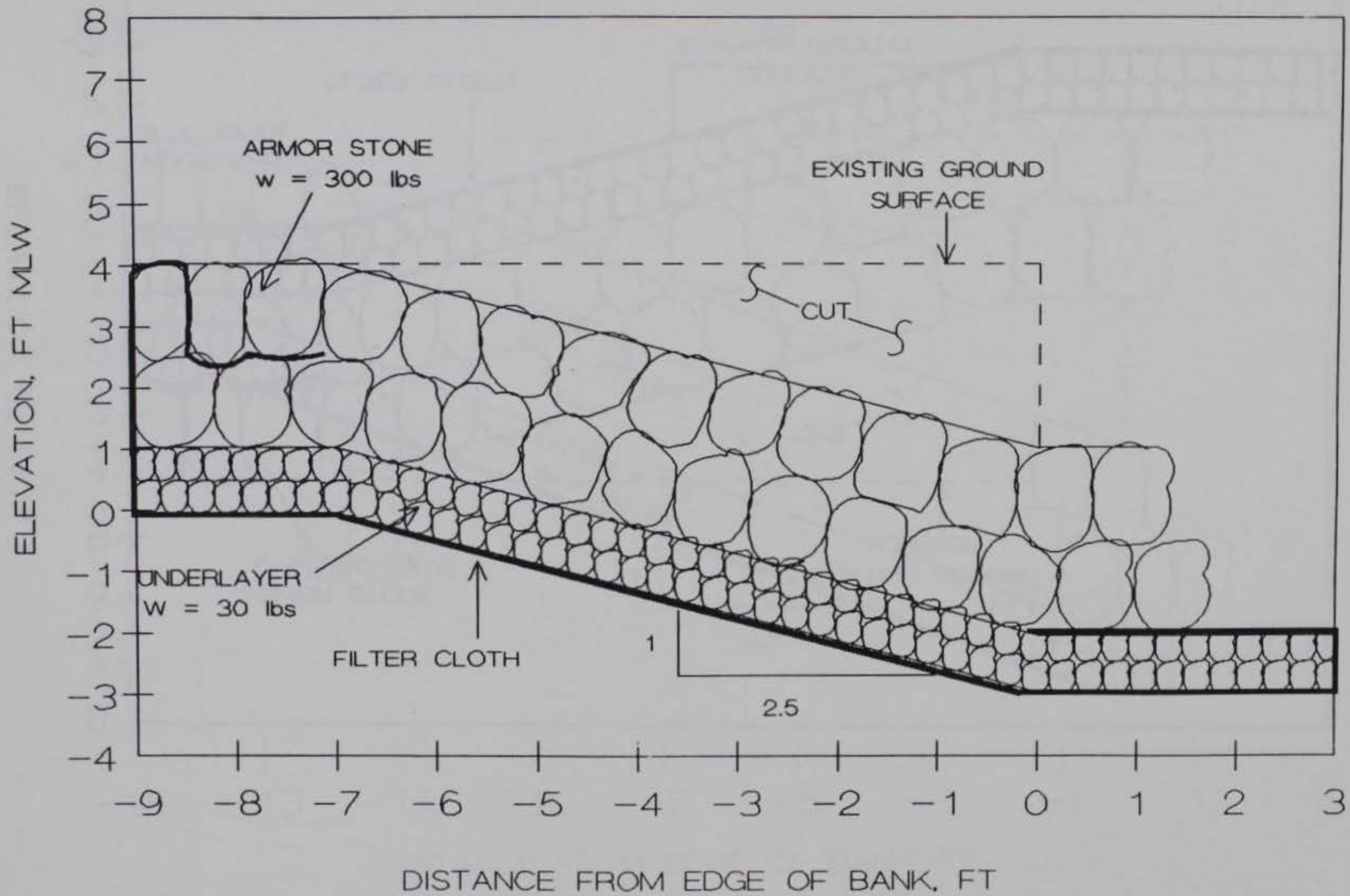
FIGURE 22. PLACED RIPRAP REVETMENT PROPOSED FOR SITE 3
