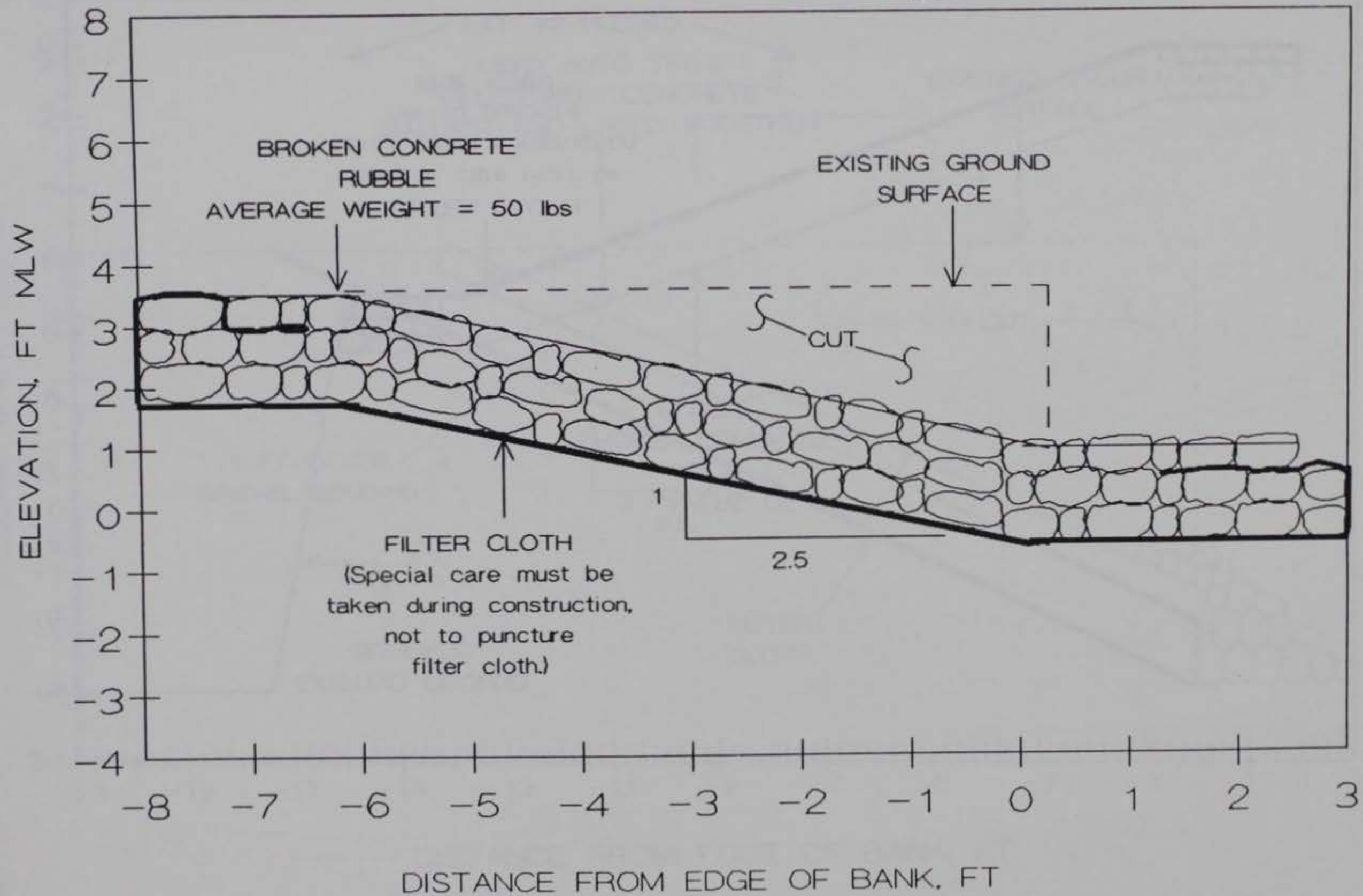
FIGURE 32. BROKEN CONCRETE REVETMENT PROPOSED FOR SITE 10
