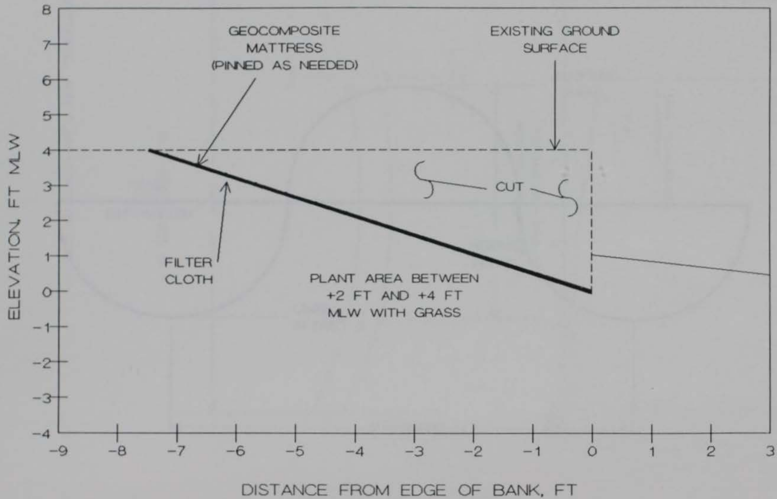
FIGURE 17. GEOCOMPOSITE MATTRESS PROPOSED FOR SITE 9
