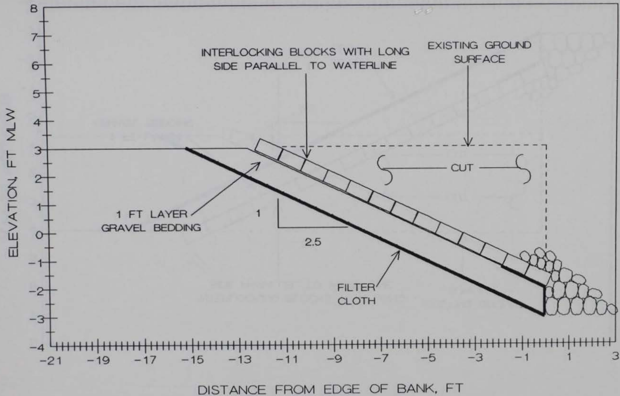
FIGURE 40. INTERLOCKING CONCRETE BLOCK REVETMENT PROPOSED FOR SITE 8
