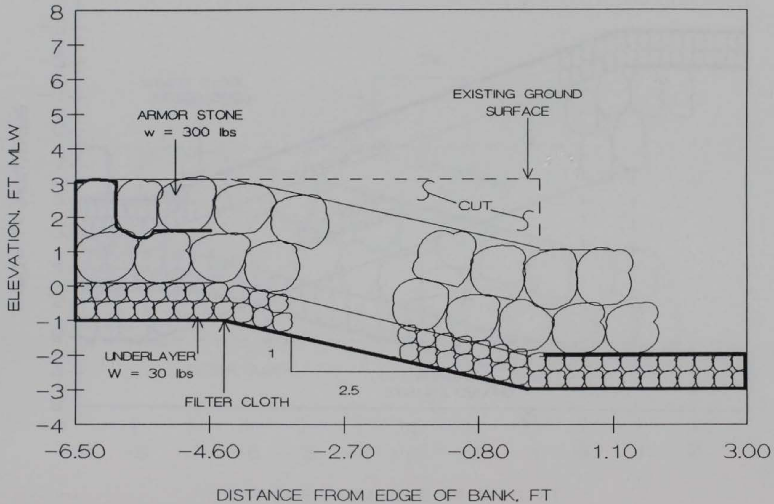
FIGURE 25. PLACED RIPRAP REVETMENT PROPOSED FOR SITE 6
