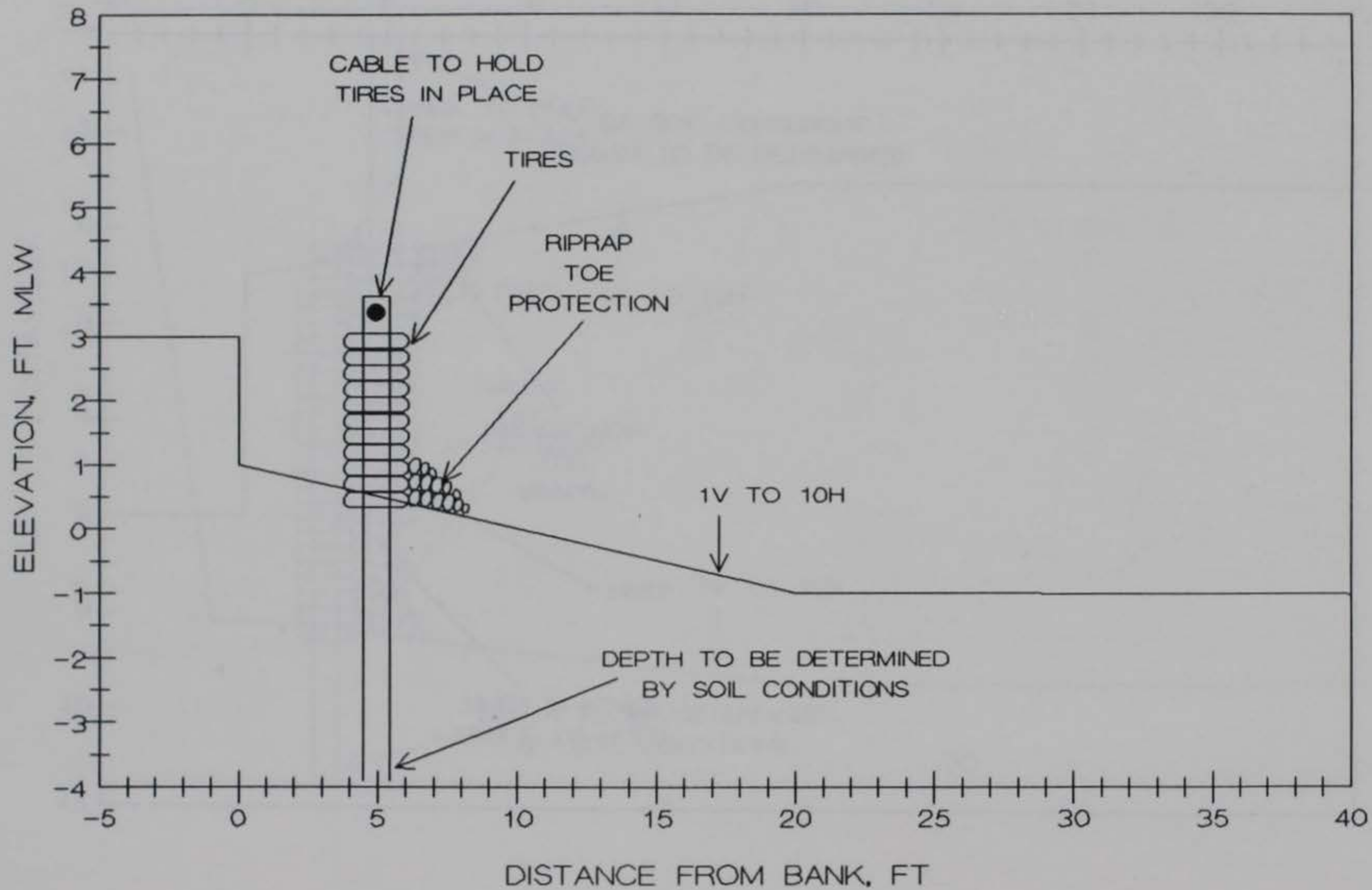
FIGURE 61. USE AUTO TIRE POST RETARD PROPOSED FOR SITE 6
