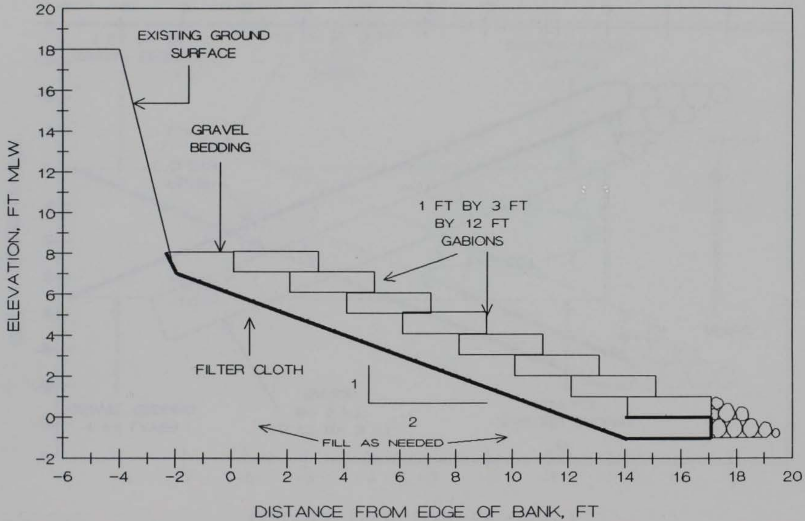
FIGURE 53. GABION REVETMENT PROPOSED FOR SITE 11
