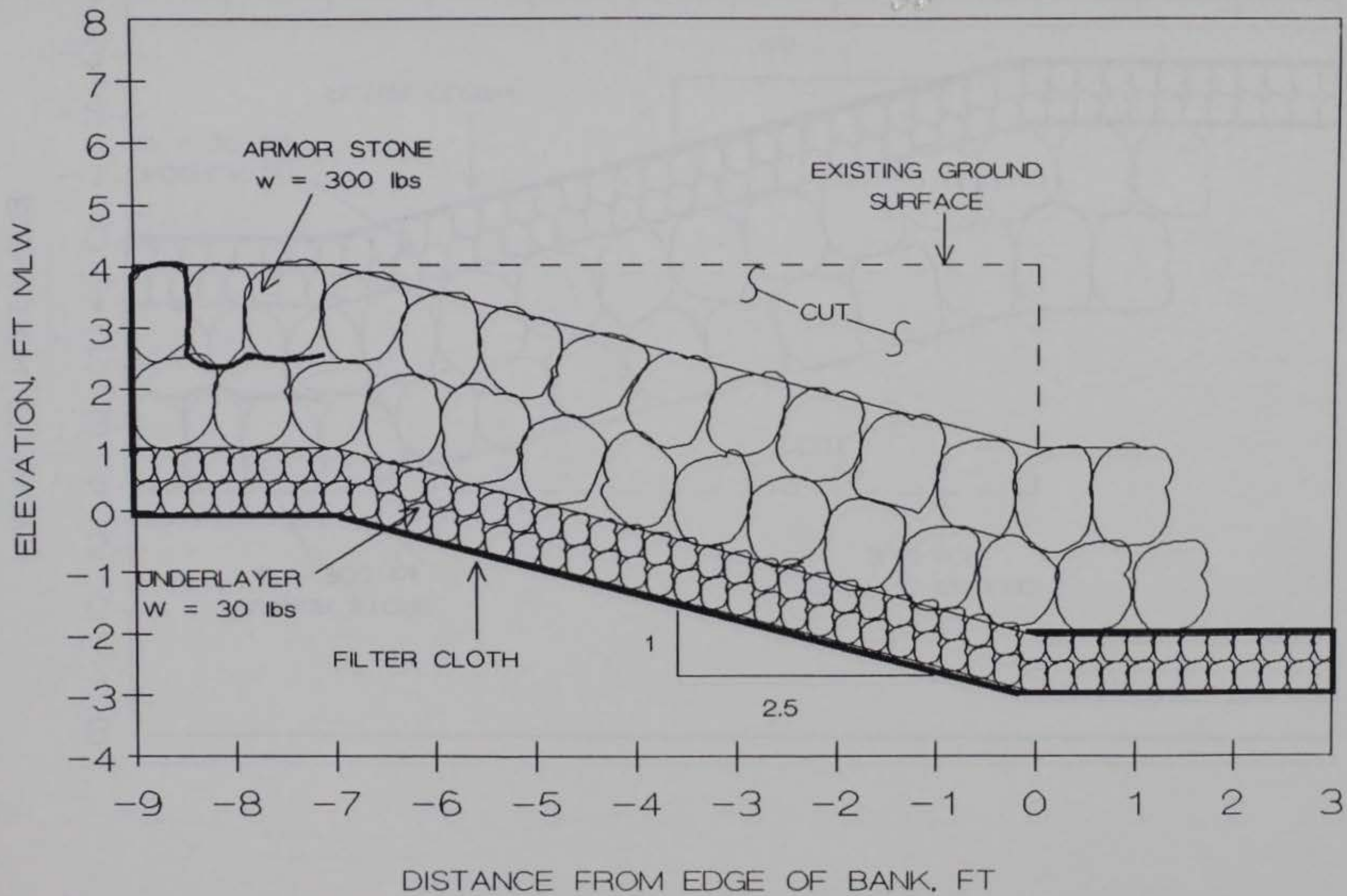
FIGURE 20. PLACED RIPRAP REVETMENT PROPOSED FOR SITE 2
