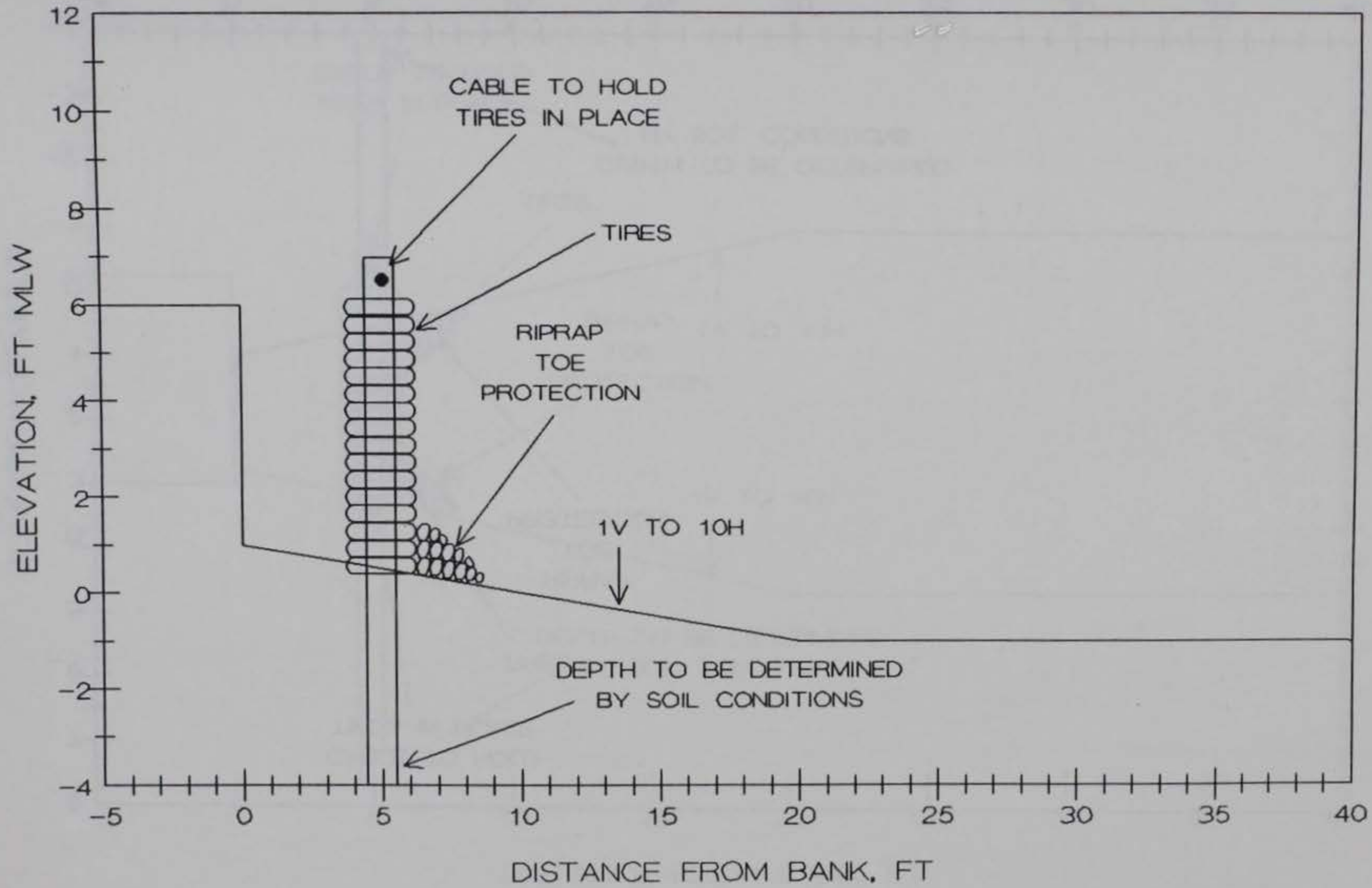
FIGURE 60. USED AUTO TIRE POST RETARD PROPOSED FOR SITE 5
