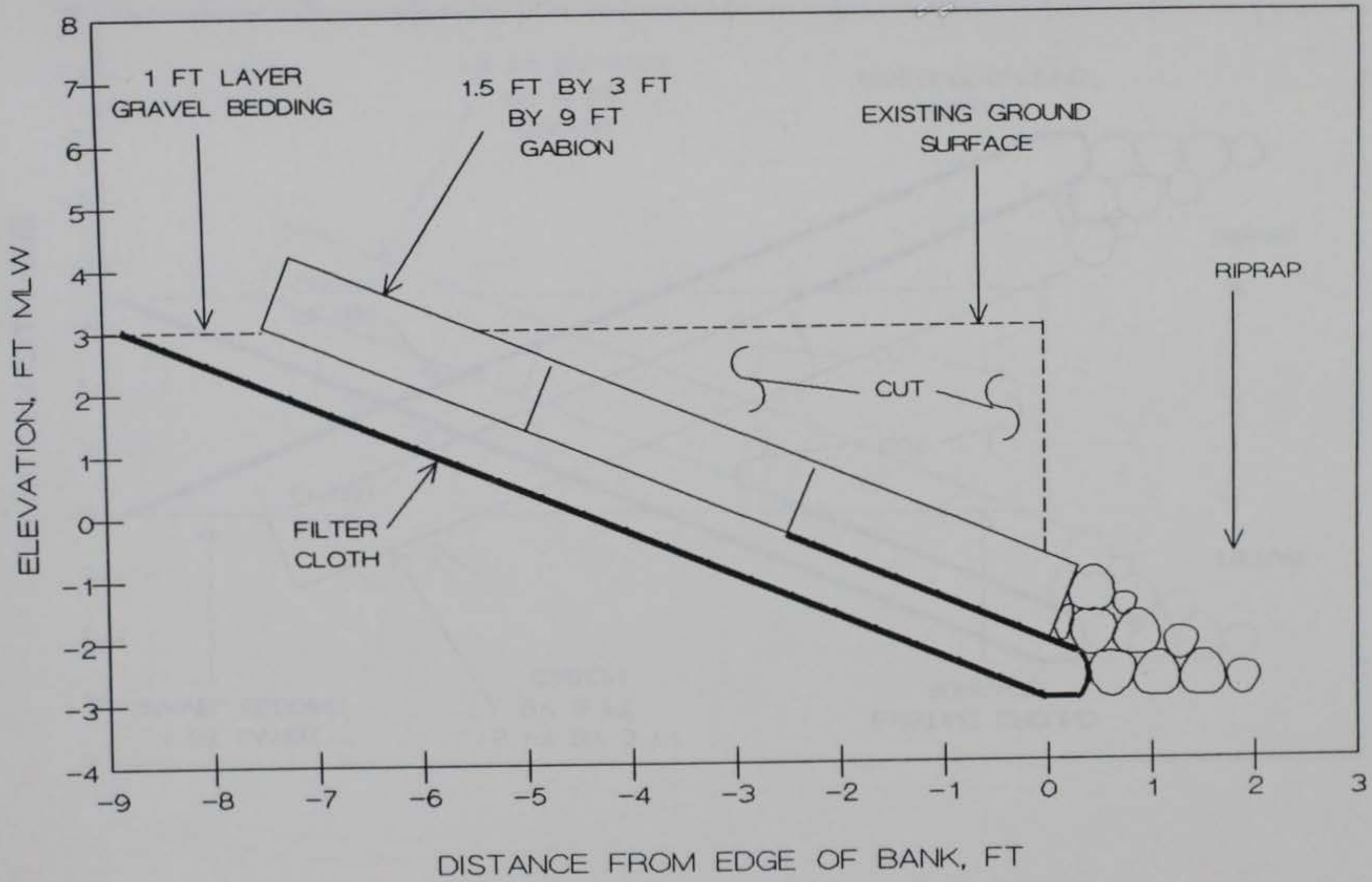
FIGURE 50. GABION REVETMENT PROPOSED FOR SITE 8
