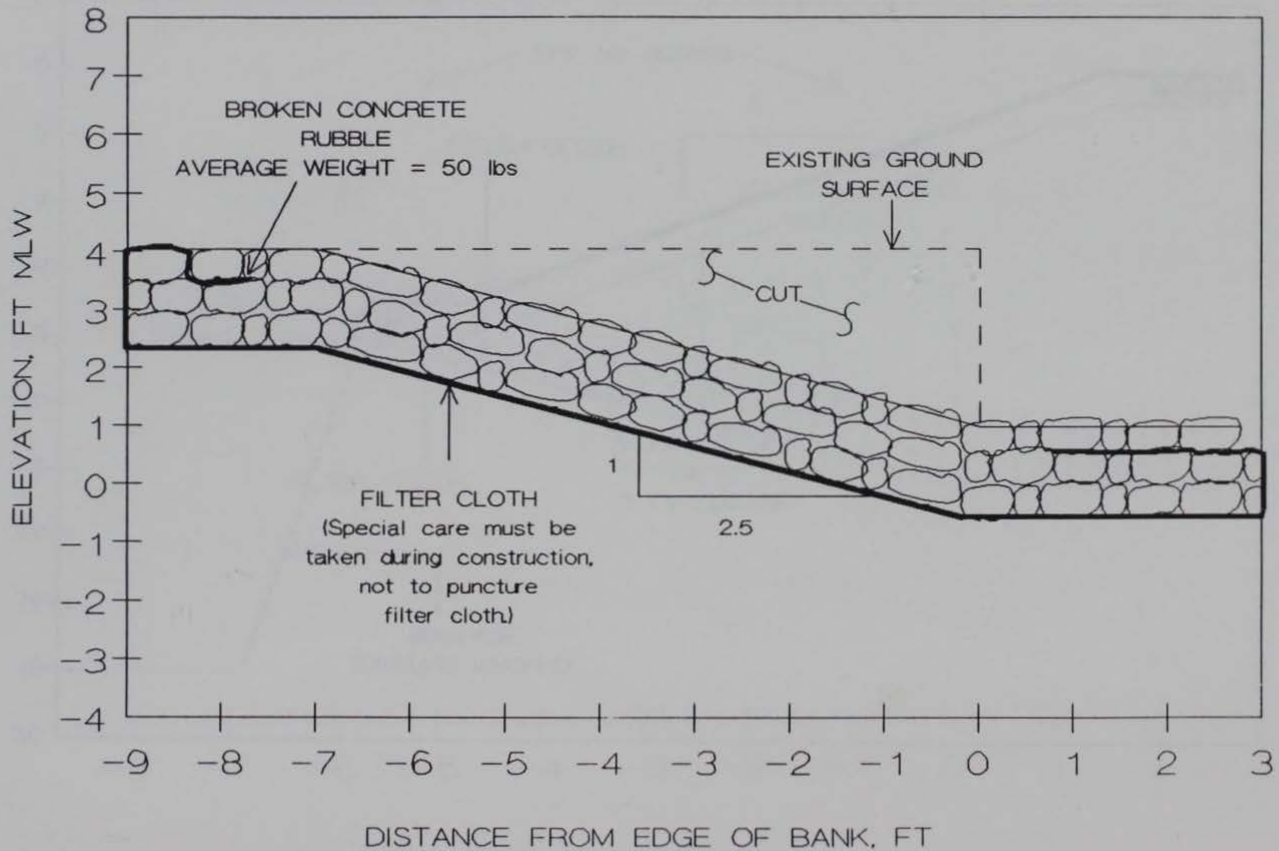
FIGURE 31. BROKEN CONCRETE REVETMENT PROPOSED FOR SITE 9
