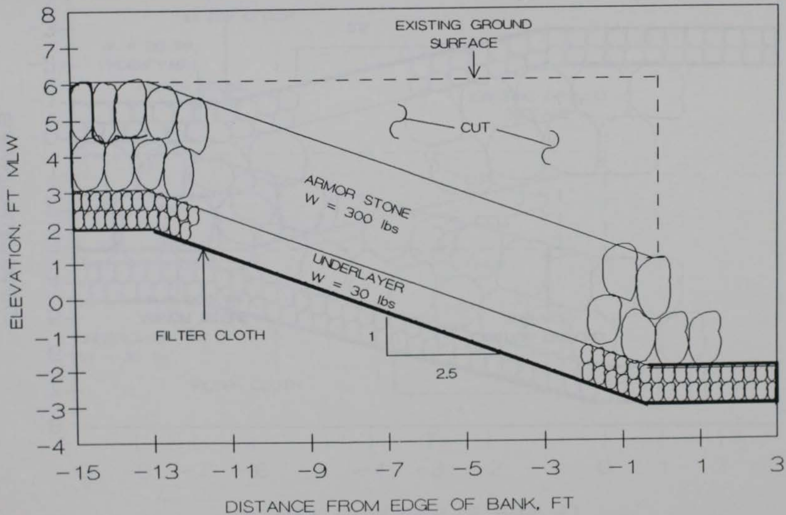
FIGURE 24. PLACED RIPRAP REVETMENT PROPOSED FOR SITE 5
