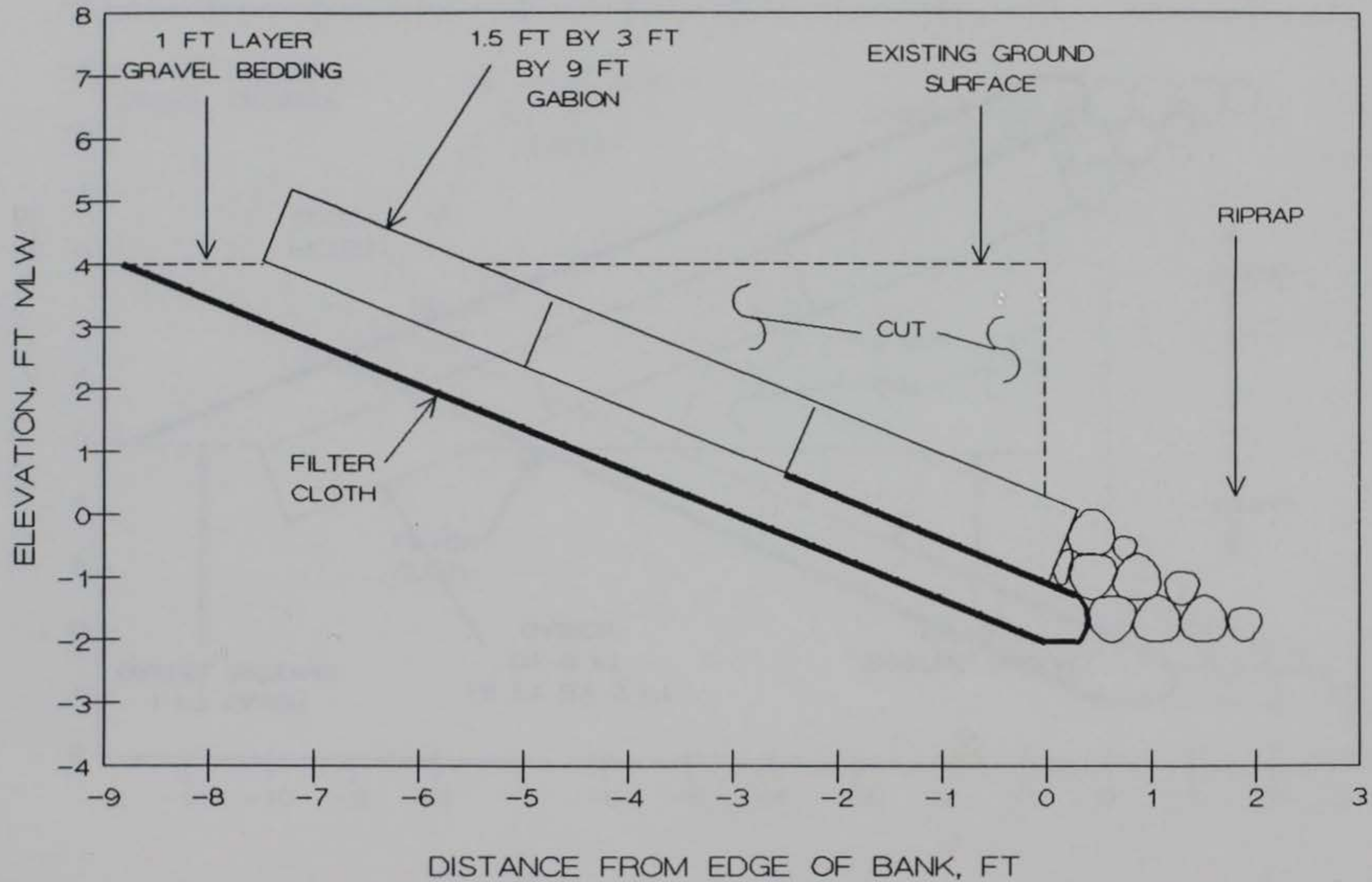
FIGURE 51. GABION REVETMENT PROPOSED FOR SITE 9
