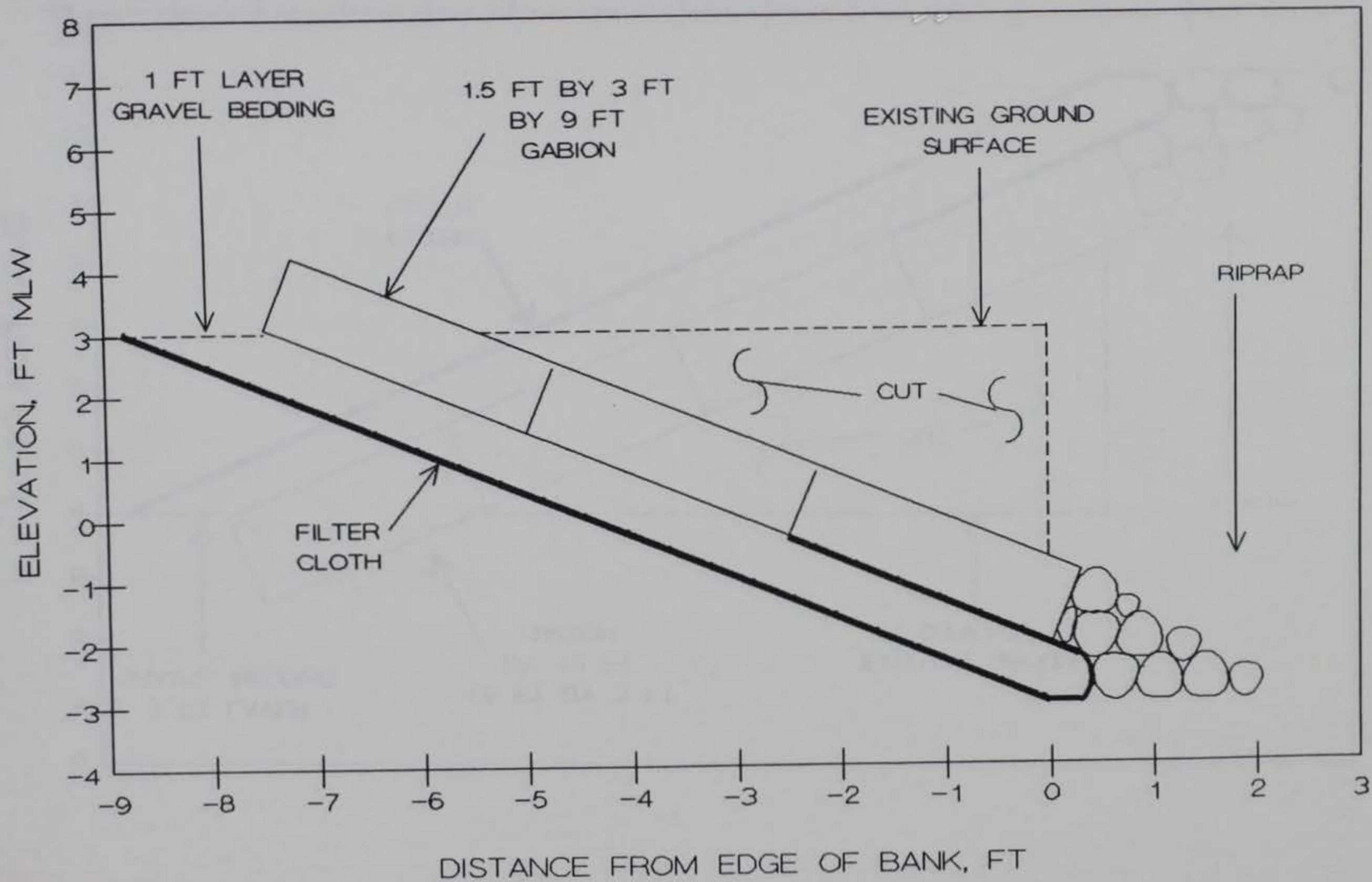
FIGURE 48. GABION REVETMENT PROPOSED FOR SITE 6
