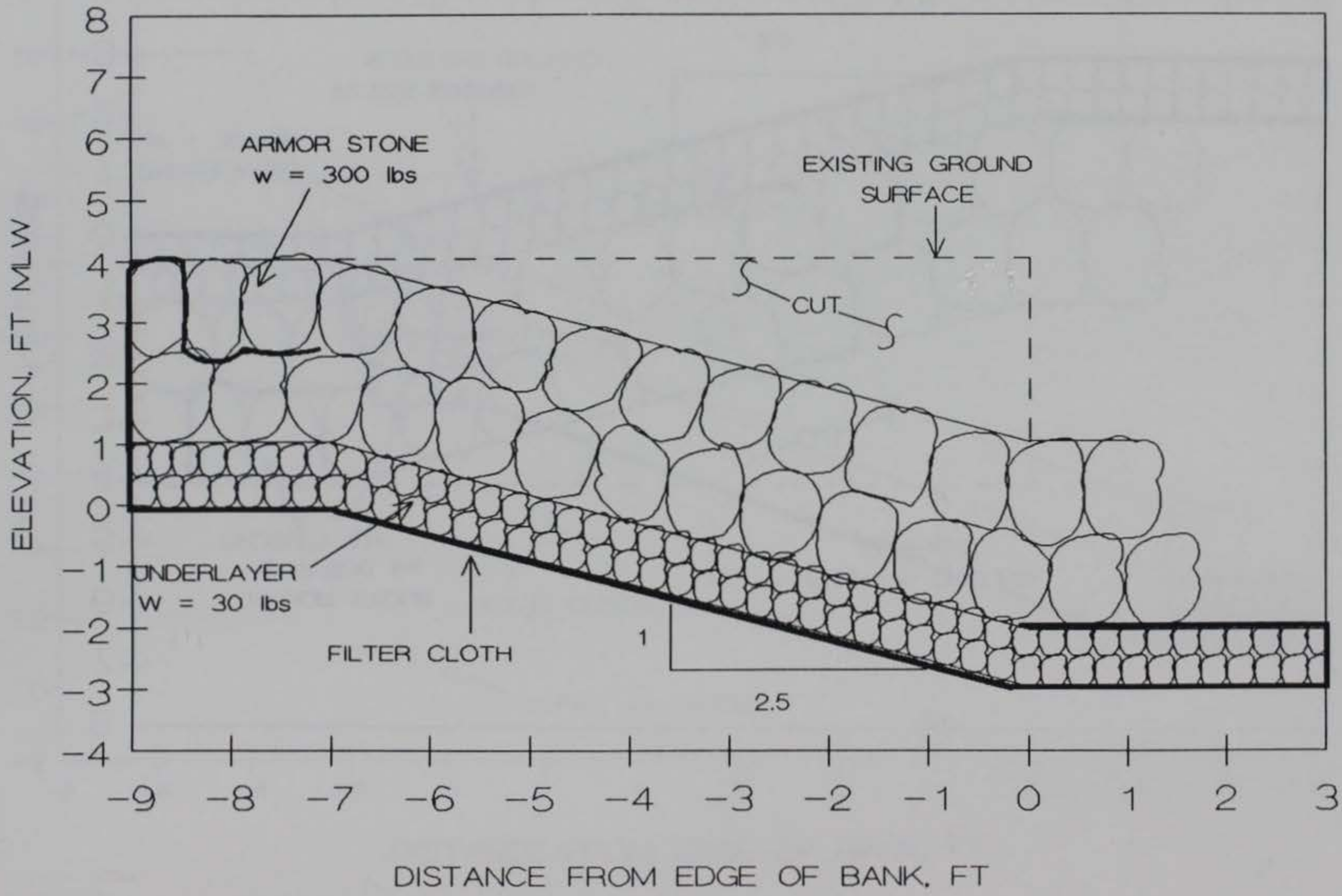
FIGURE 21. PLACED RIPRAP REVETMENT PROPOSED FOR SITE 2A
