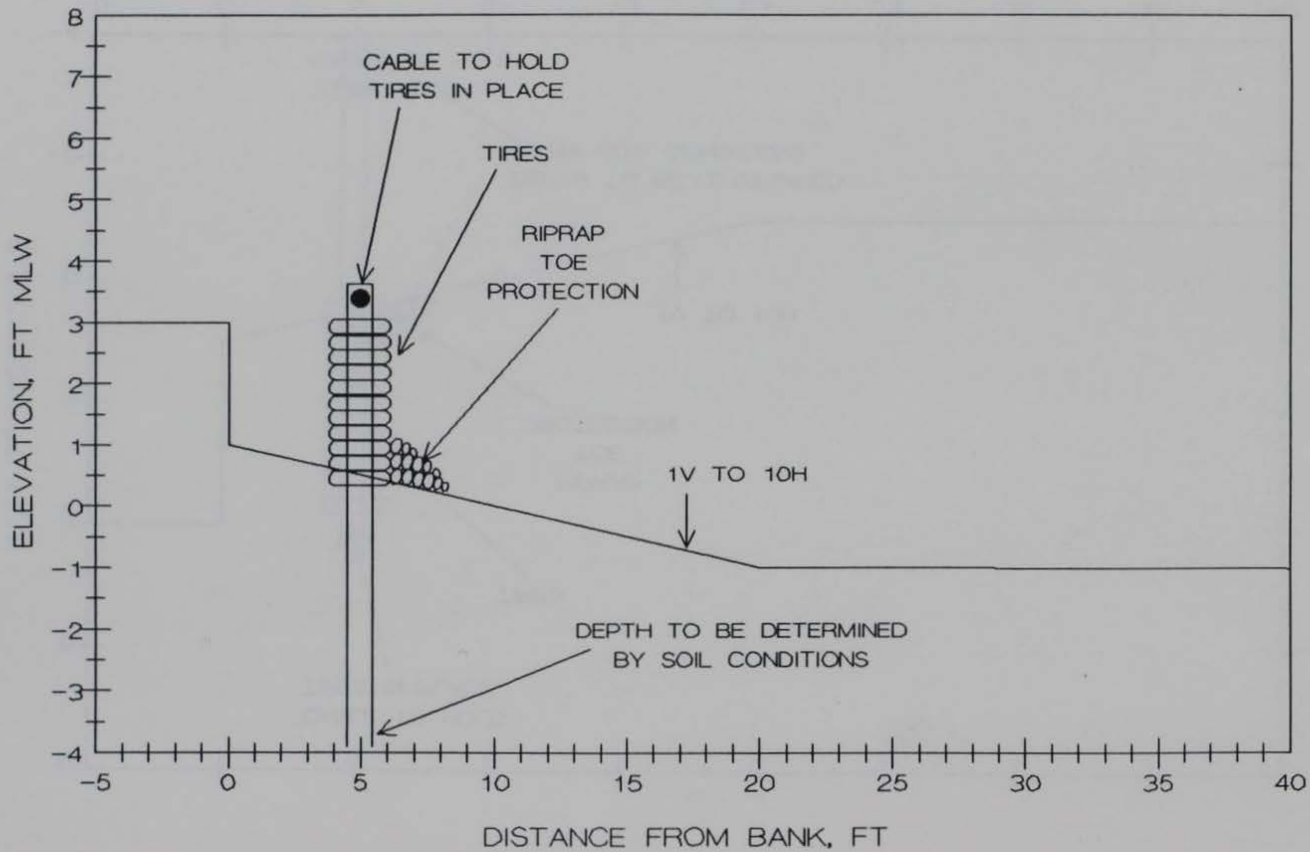
FIGURE 63. USED AUTO TIRE POST RETARD PROPOSED FOR SITE 8
