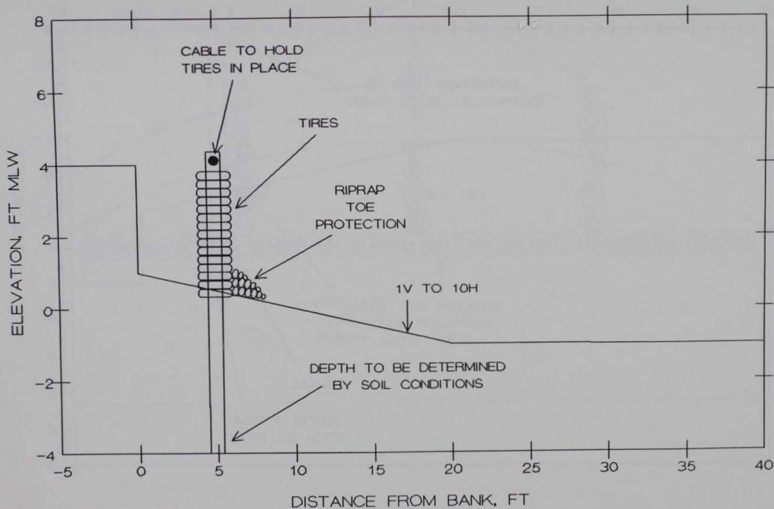
FIGURE 62. USED AUTO TIRE POST RETARD PROPOSED FOR SITE 7
