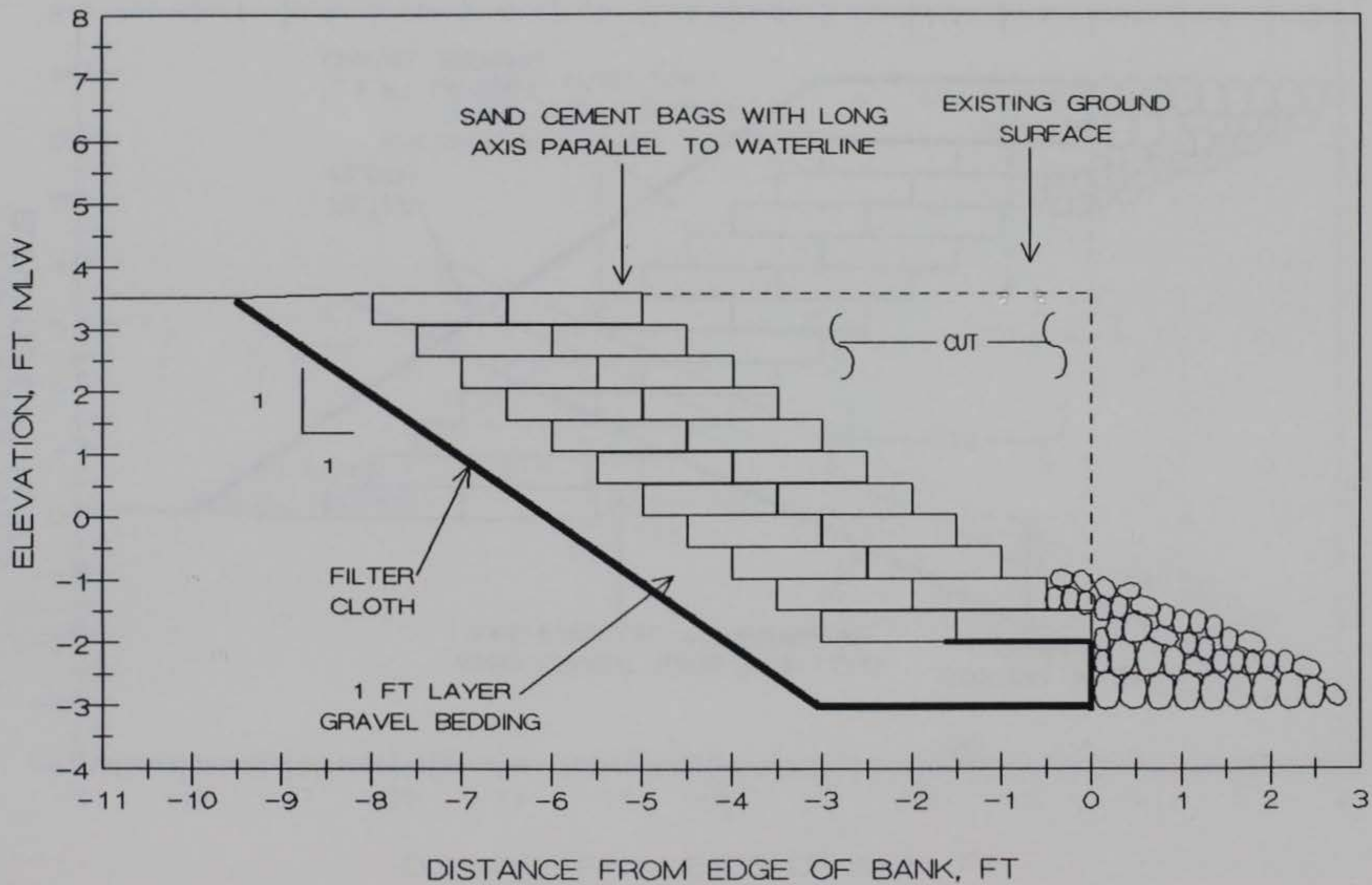
FIGURE 37. SAND-CEMENT SACK REVETMENT PROPOSED FOR SITE 10
