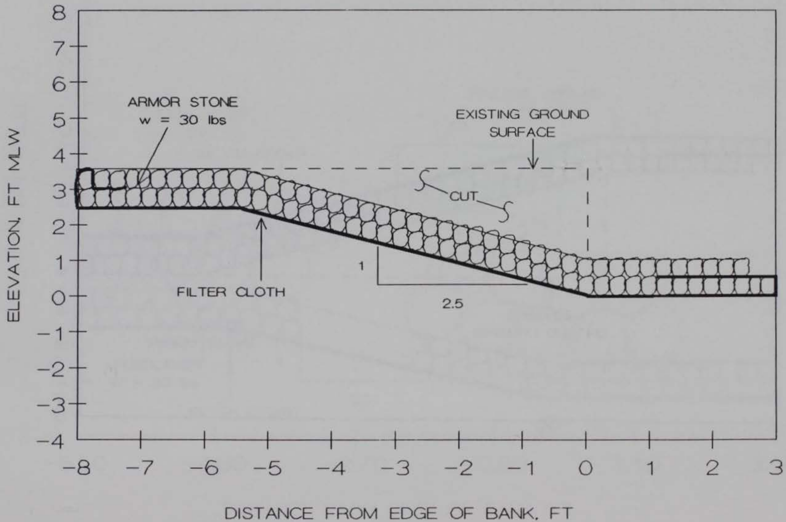
FIGURE 29. PLACED RIPRAP REVETMENT PROPOSED FOR SITE 10
