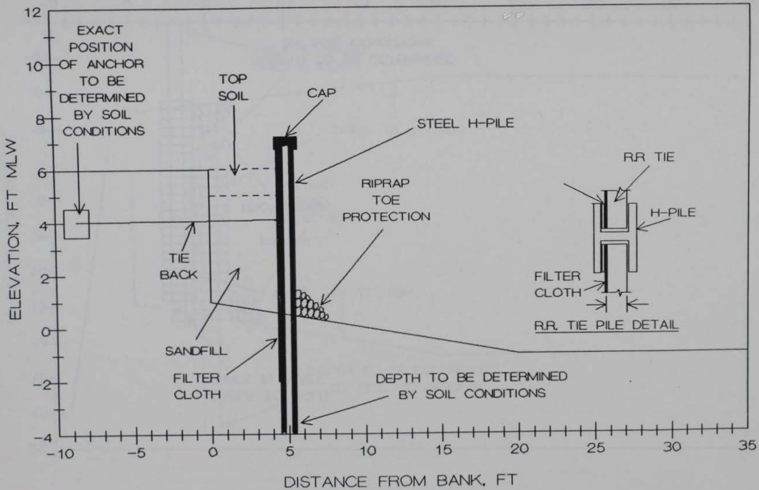
FIGURE 58. STEEL H-PILE AND RAILROAD TIES BULKHEAD PROPOSED FOR SITE 5
