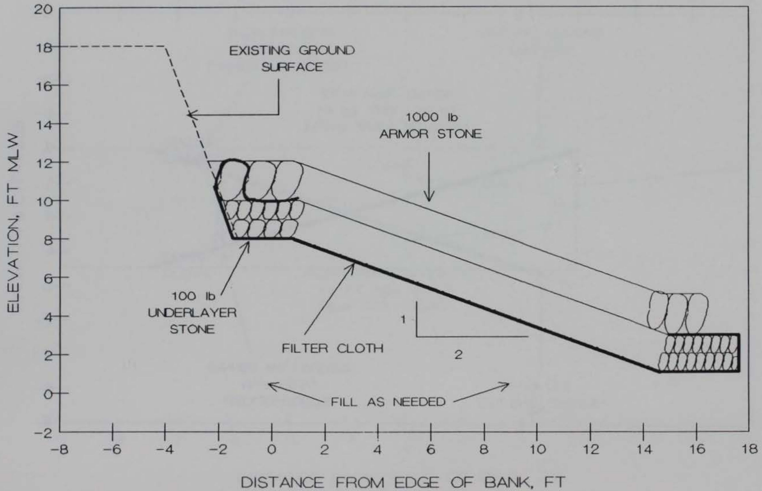
FIGURE 19. PLACED RIPRAP REVETMENT PROPOSED FOR SITE 1
