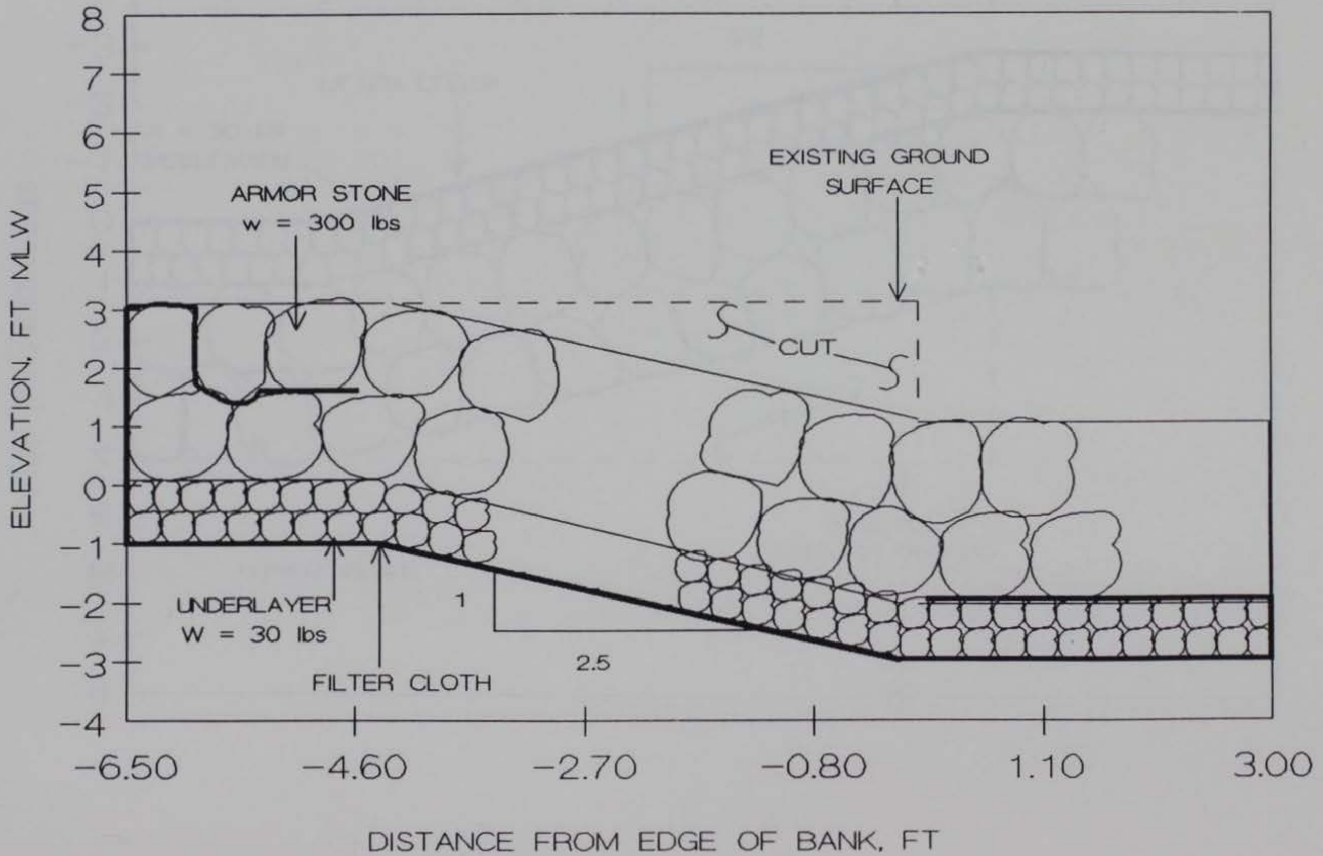
FIGURE 27. PLACED RIPRAP REVETMENT PROPOSED FOR SITE 8
