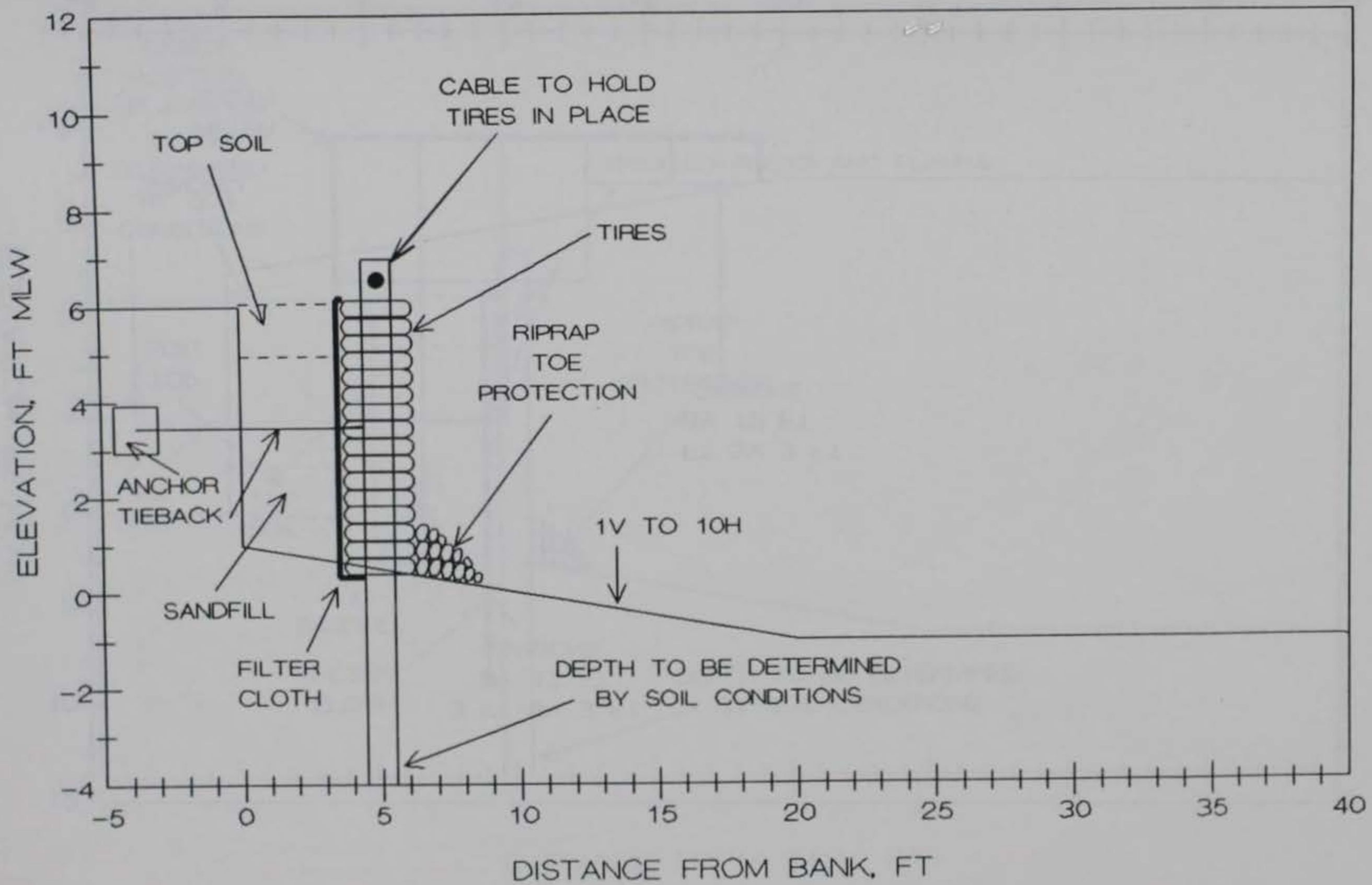
FIGURE 54. USED AUTO TIRE POST BULKHEAD PROPOSED FOR SITE 5
