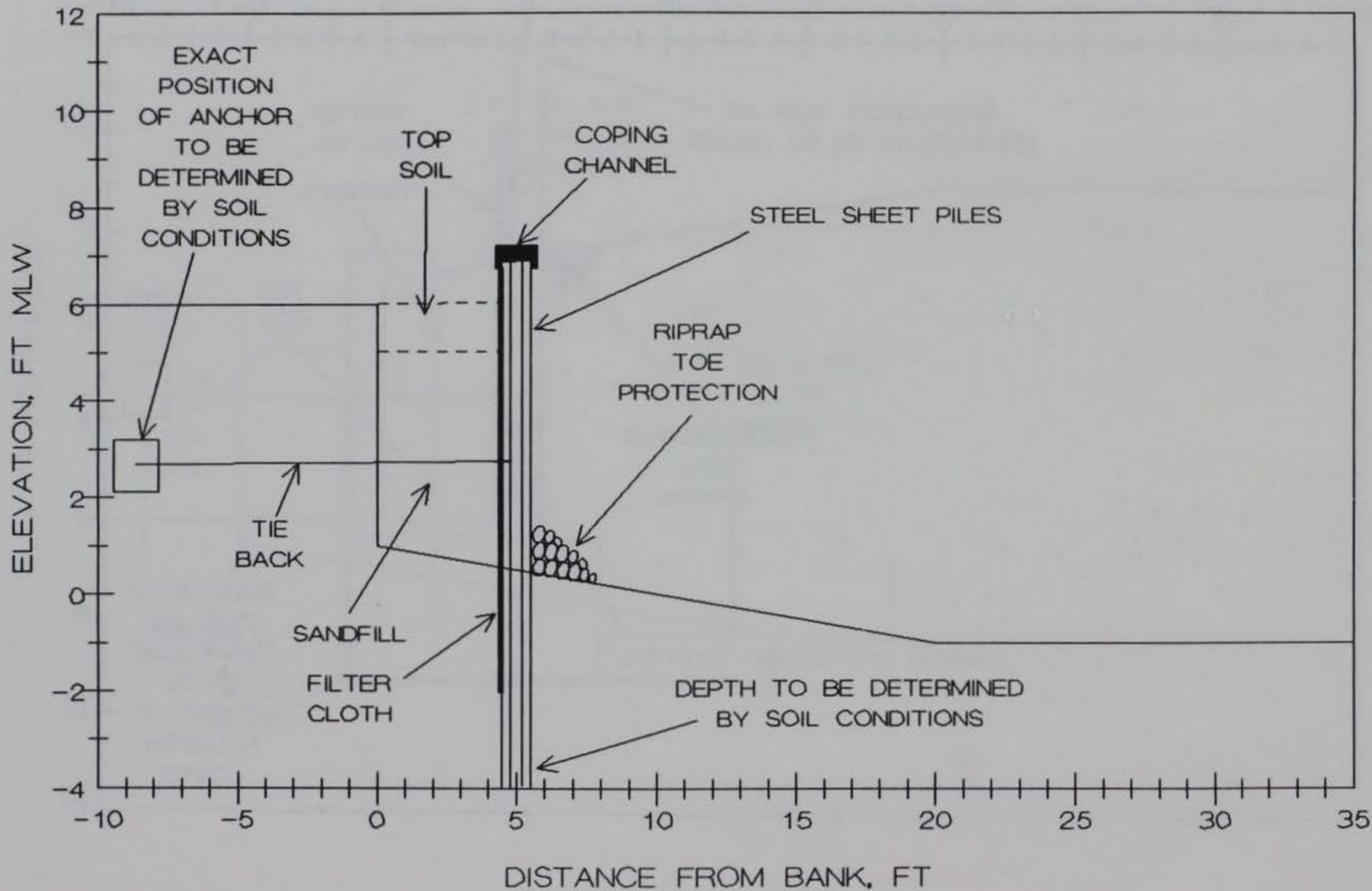
FIGURE 57. STEEL SHEETPILE BULKHEAD PROPOSED FOR SITE 5
