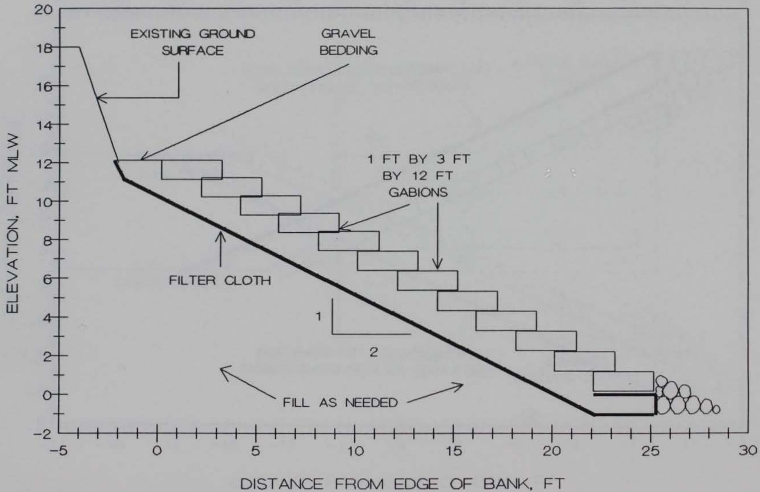
FIGURE 43. GABION REVETMENT PROPOSED FOR SITE 1
