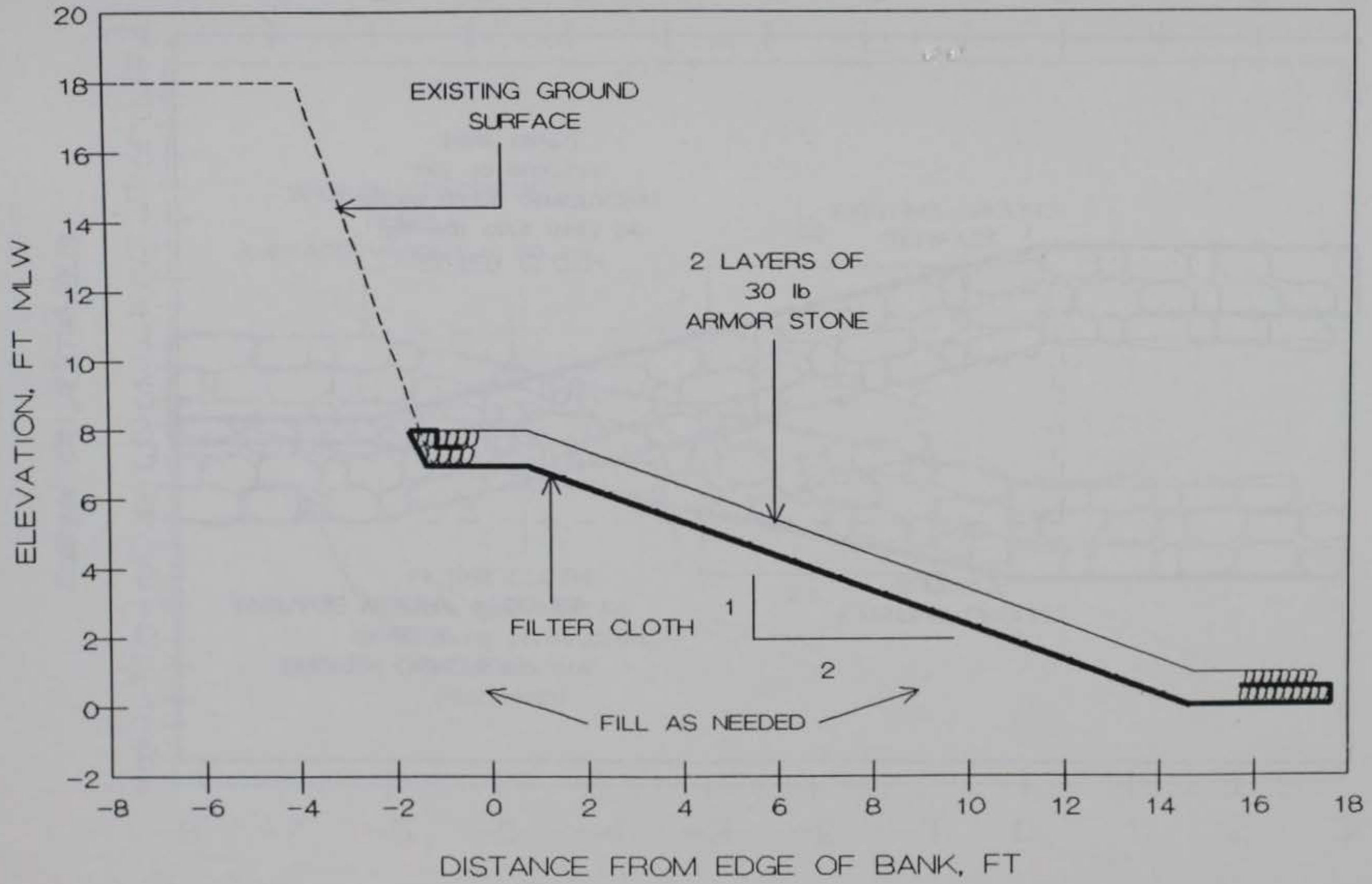
FIGURE 30. PLACED RIPRAP REVETMENT PROPOSED FOR SITE 11
