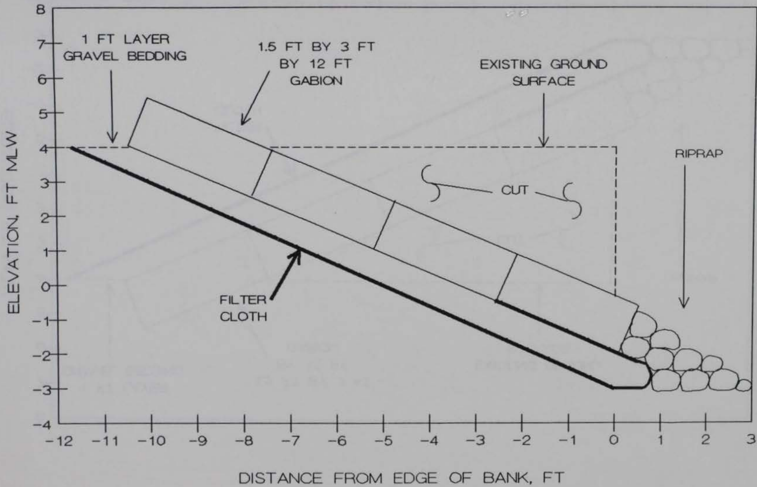
FIGURE 44. GABION REVETMENT PROPOSED FOR SITE 2
