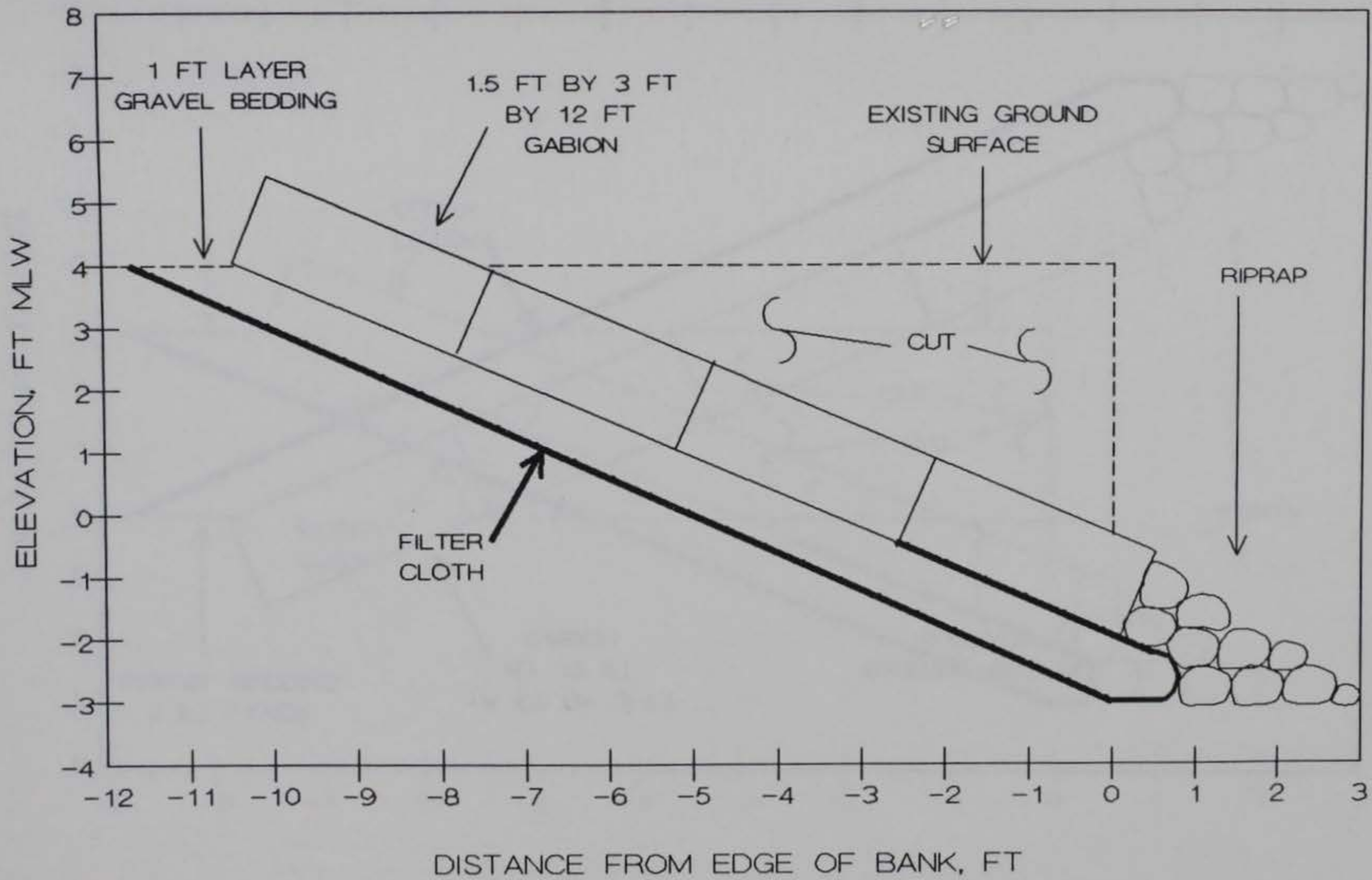
FIGURE 46. GABION REVETMENT PROPOSED FOR SITE 3
