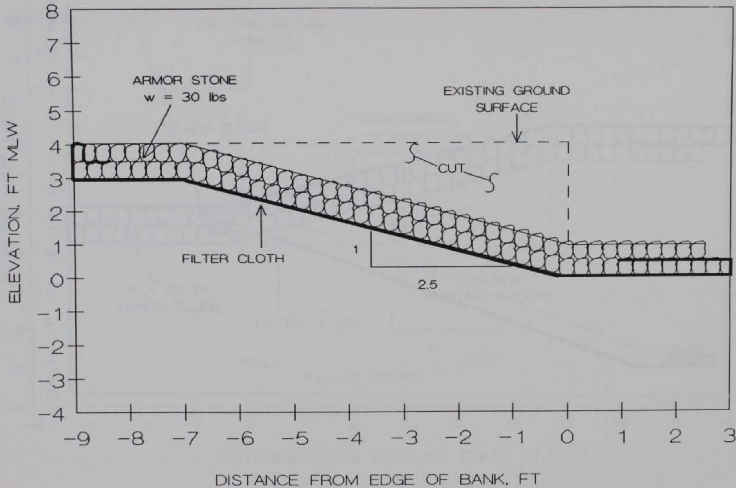
FIGURE 28. PLACED RIPRAP REVETMENT PROPOSED FOR SITE 9
