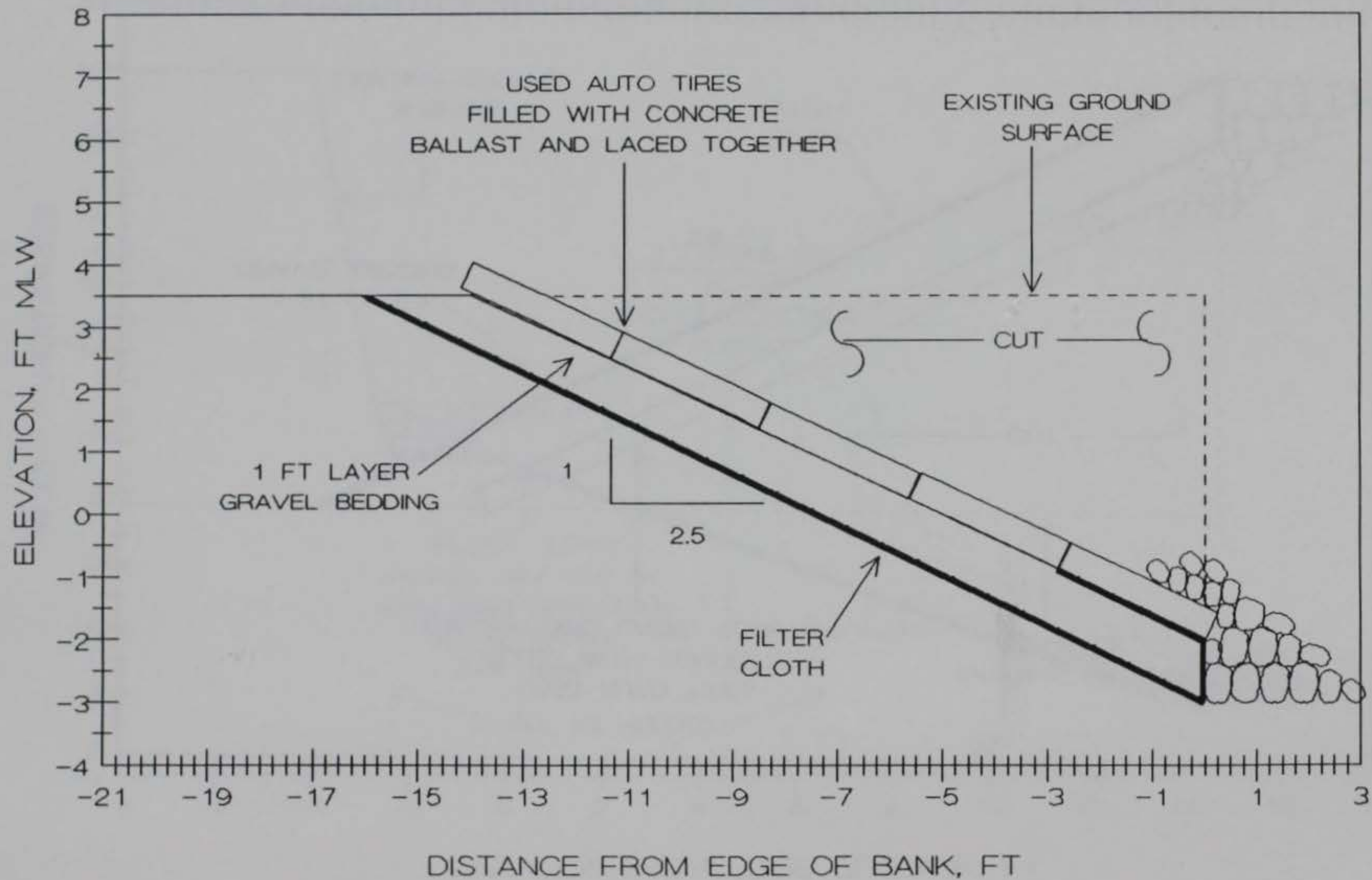
FIGURE 35. USED AUTO TIRE MATTRESS REVETMENT PROPOSED FOR SITE 10
