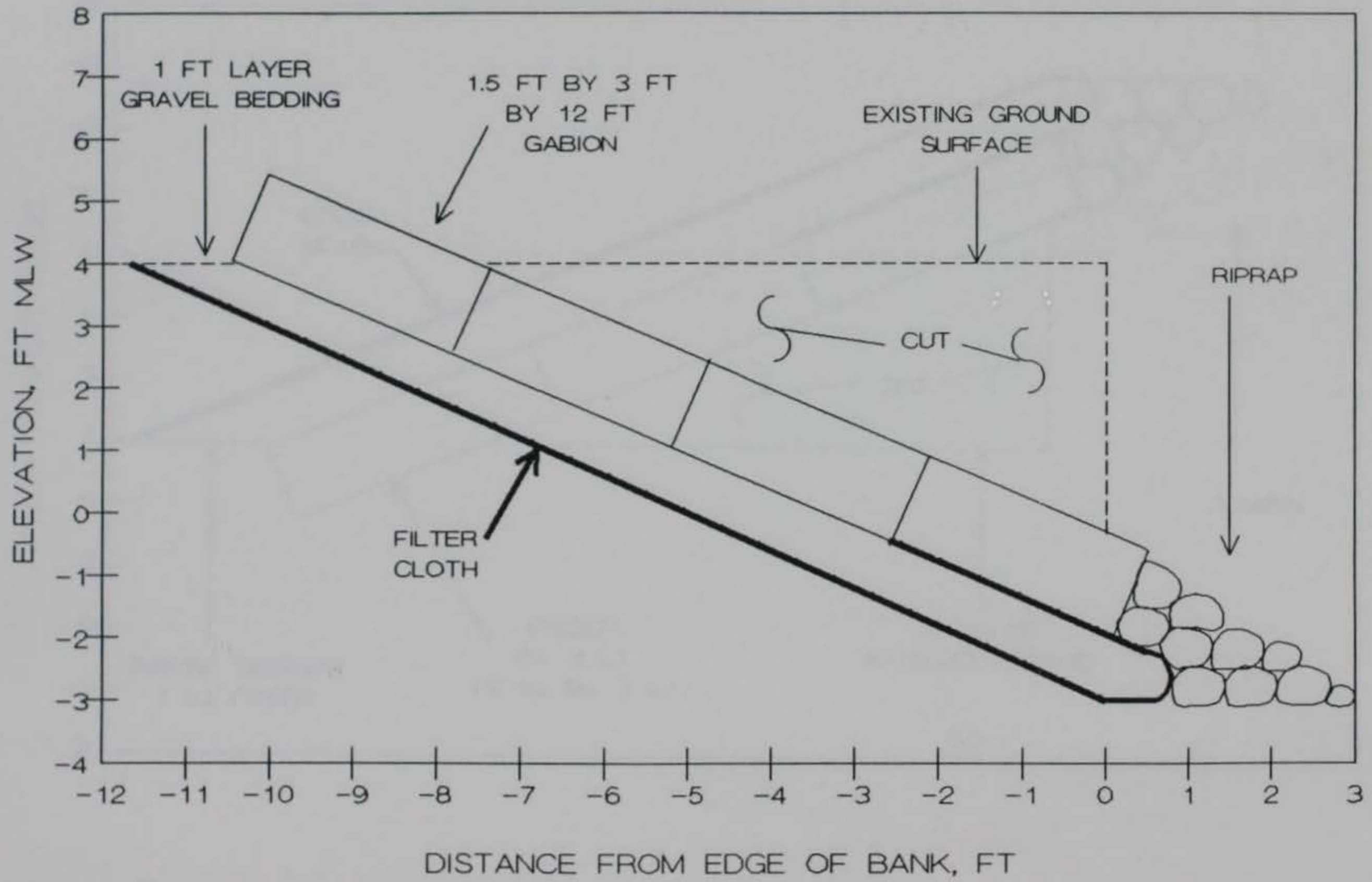
FIGURE 49. GABION REVETMENT PROPOSED FOR SITE 7
