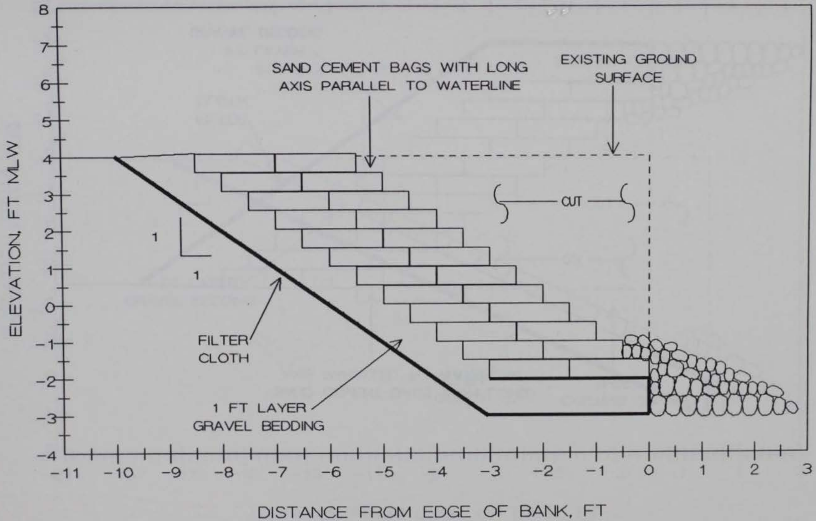
FIGURE 36. SAND-CEMENT SACK REVETMENT PROPOSED FOR SITE 9
