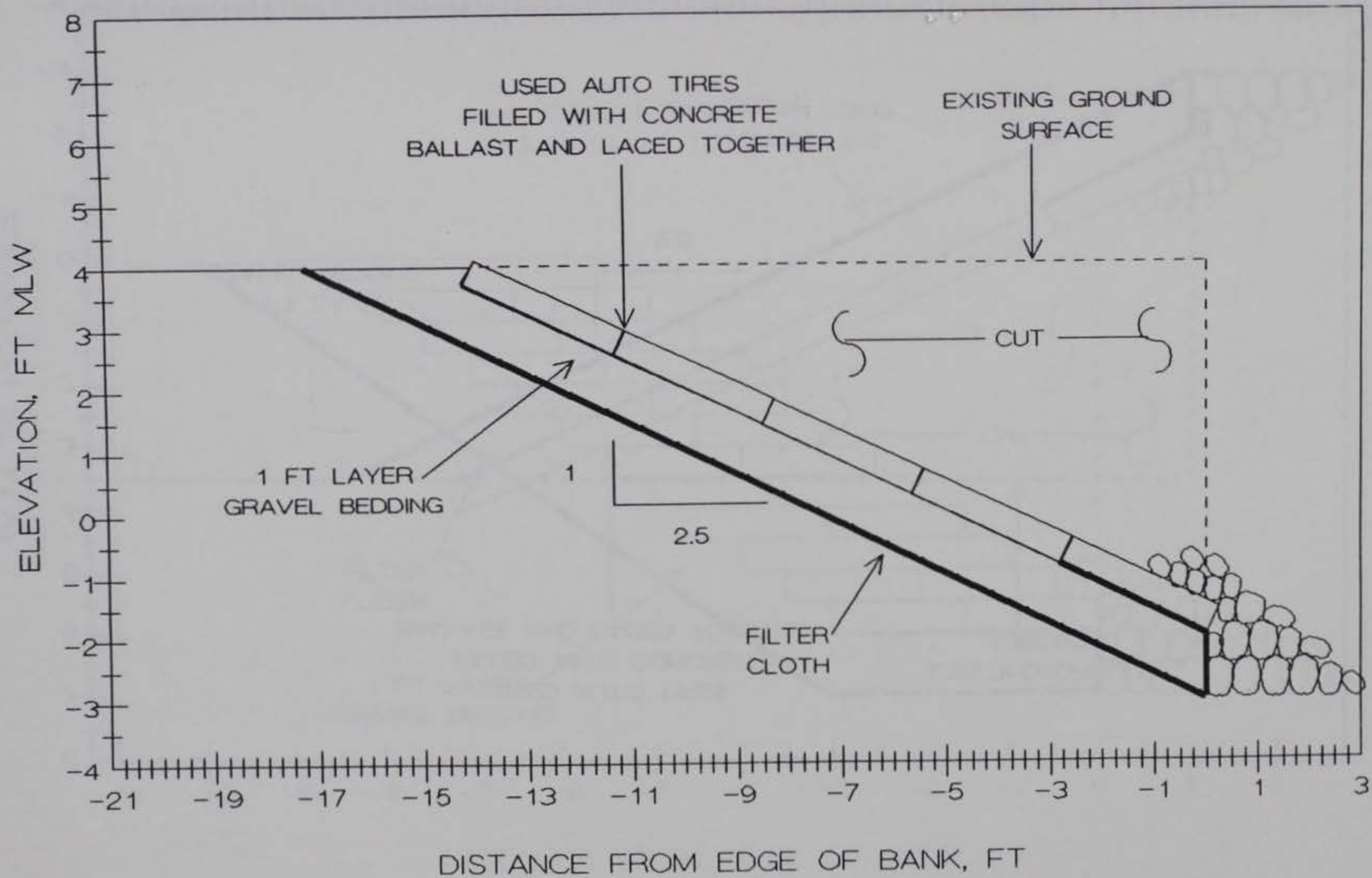
FIGURE 34. USED AUTO TIRE MATTRESS REVETMENT PROPOSED FOR SITE 9
