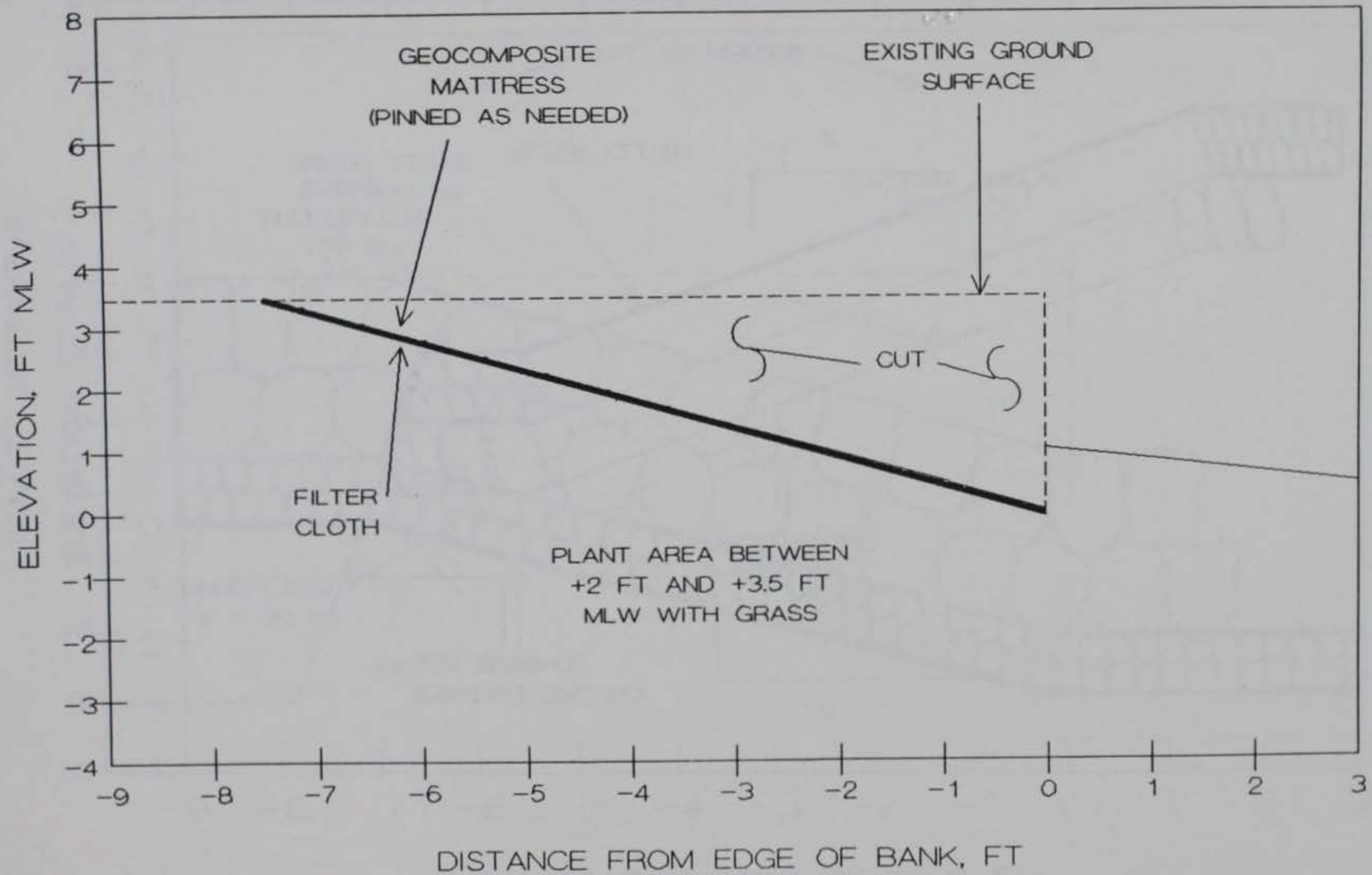
FIGURE 18. GEOCOMPOSITE MATTRESS PROPOSED FOR SITE 10
