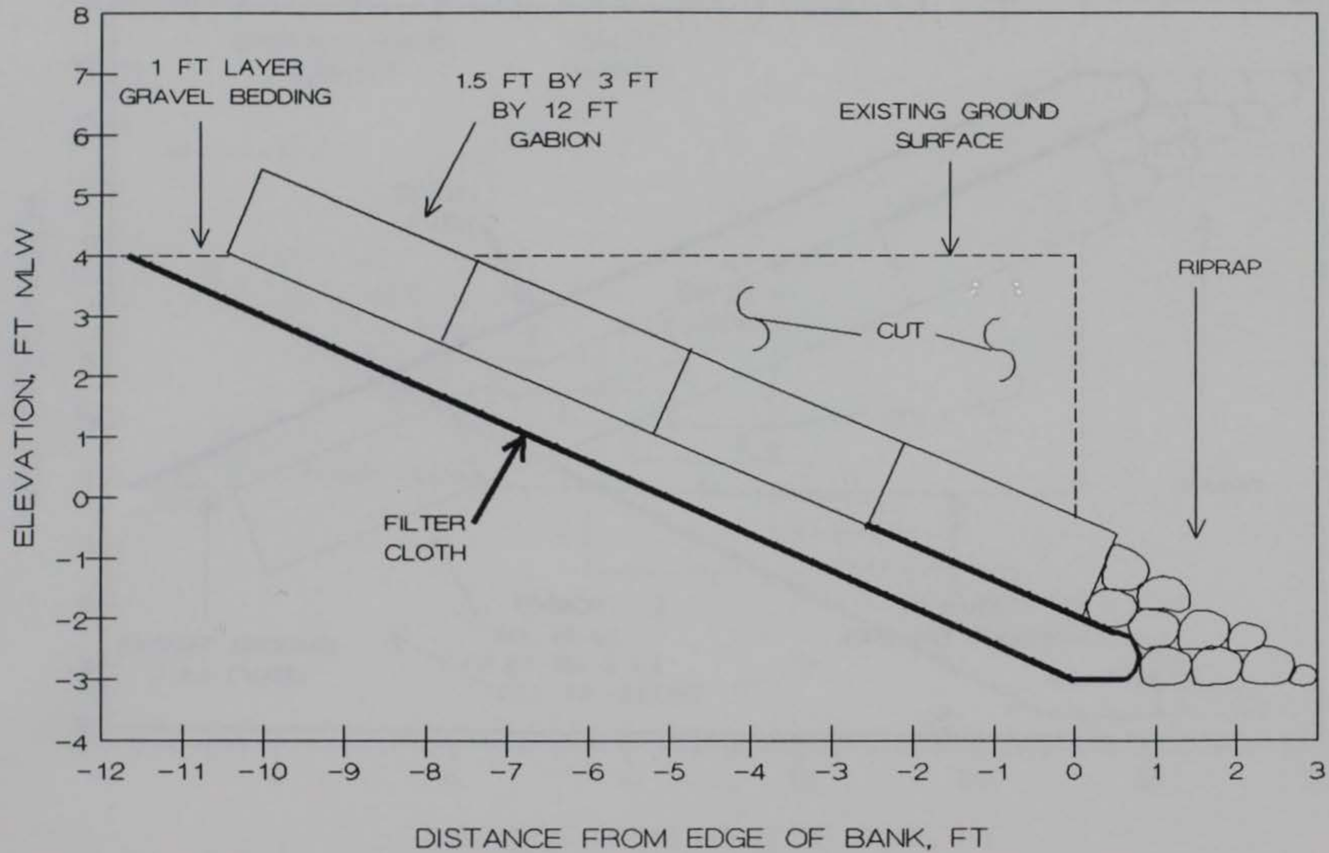
FIGURE 45. GABION REVETMENT PROPOSED FOR SITE 2A
