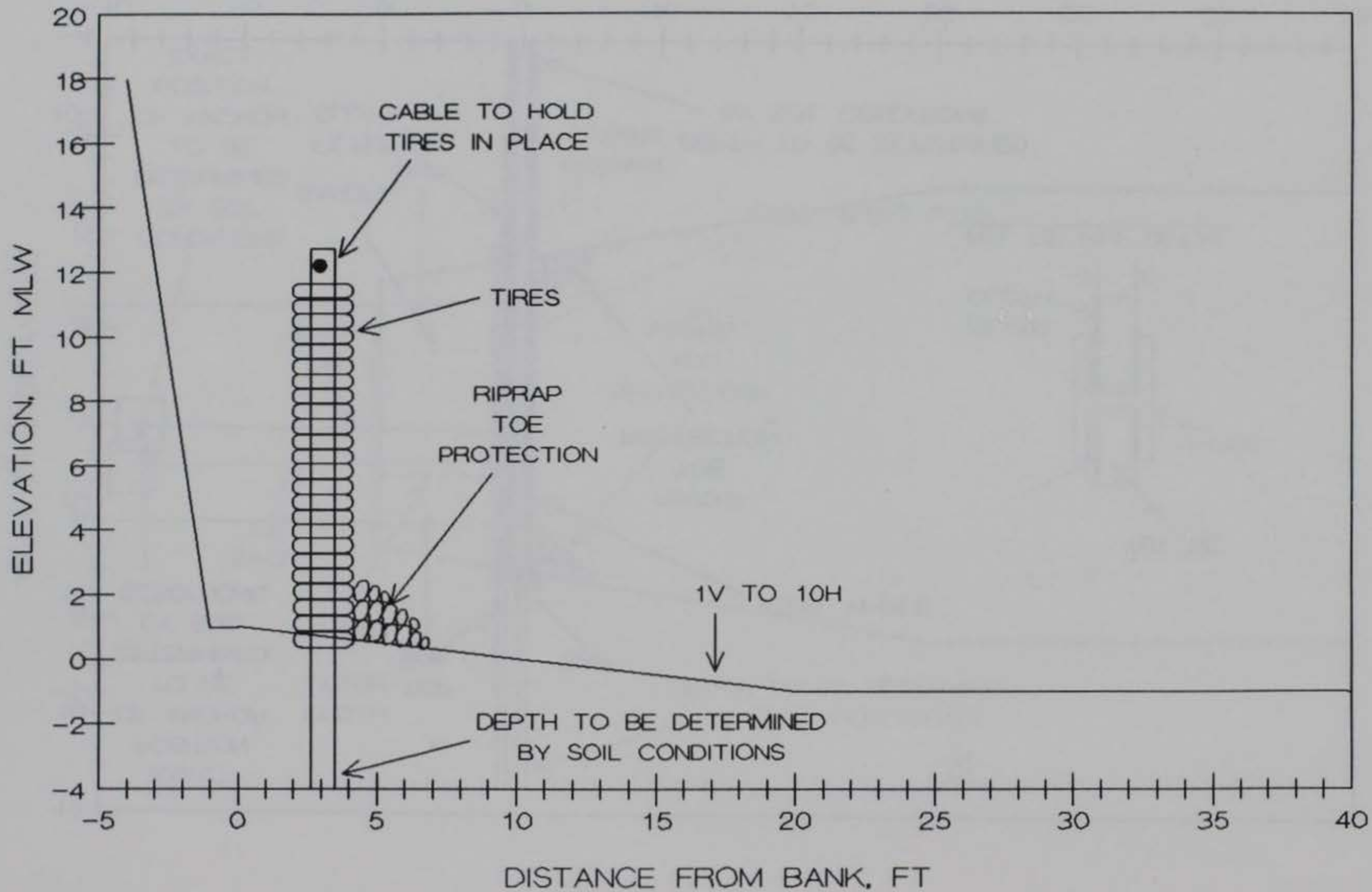
FIGURE 59. USED AUTO TIRE POST RETARD PROPOSED FOR SITE 1
