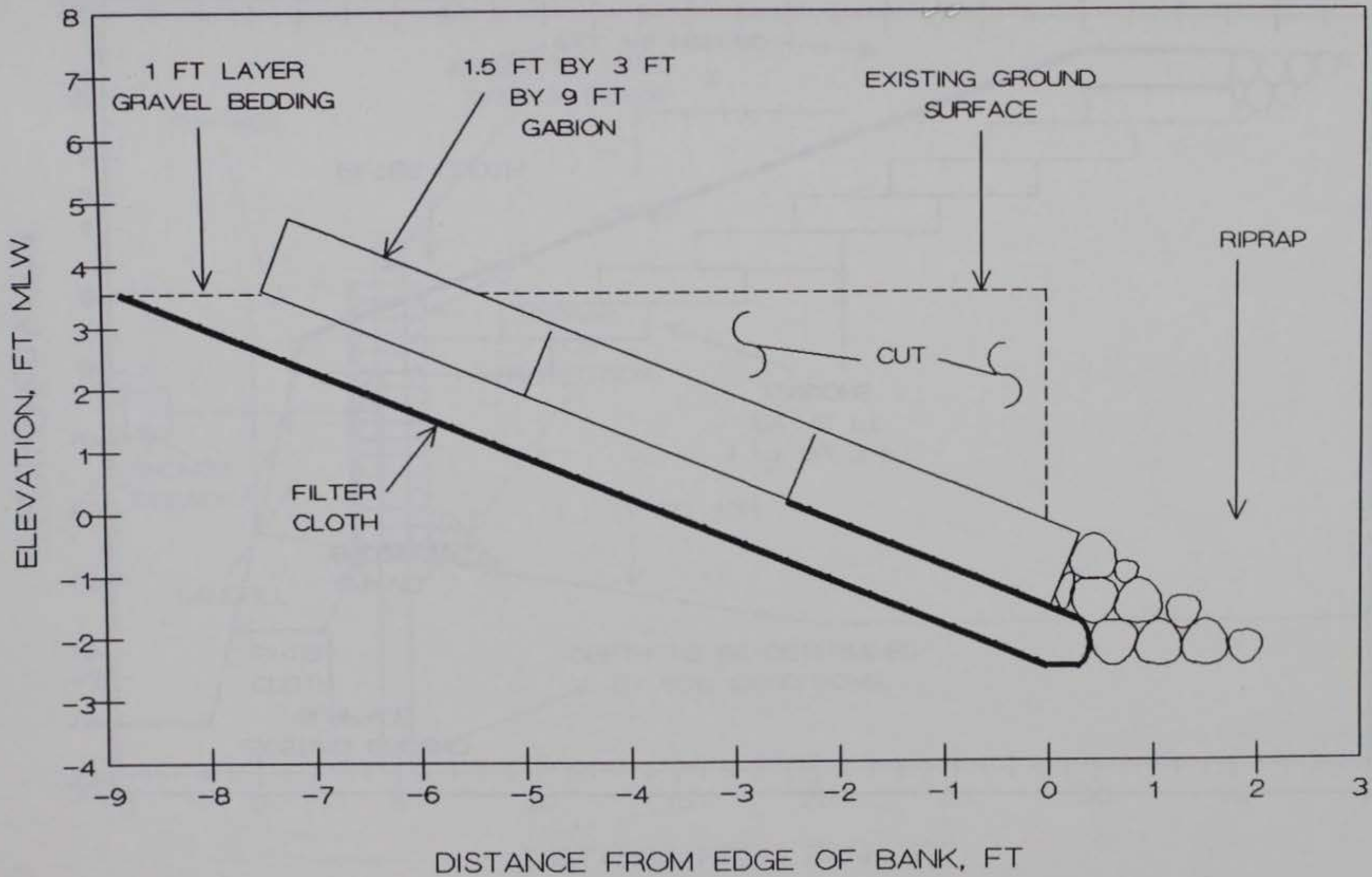
FIGURE 52. GABION REVETMENT PROPOSED FOR SITE 10
