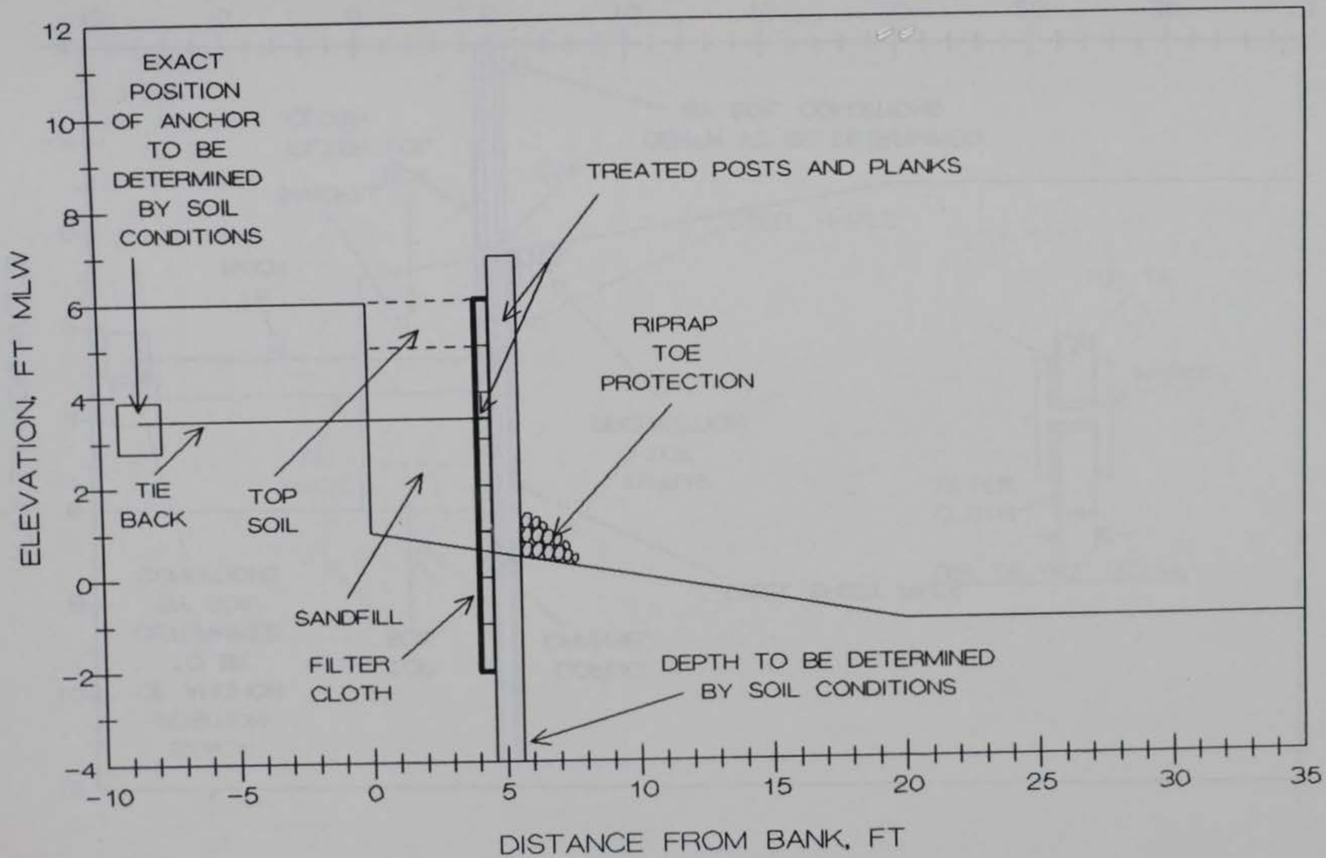
FIGURE 56. TREATED TIMBER BULKHEAD PROPOSED SITE 5
