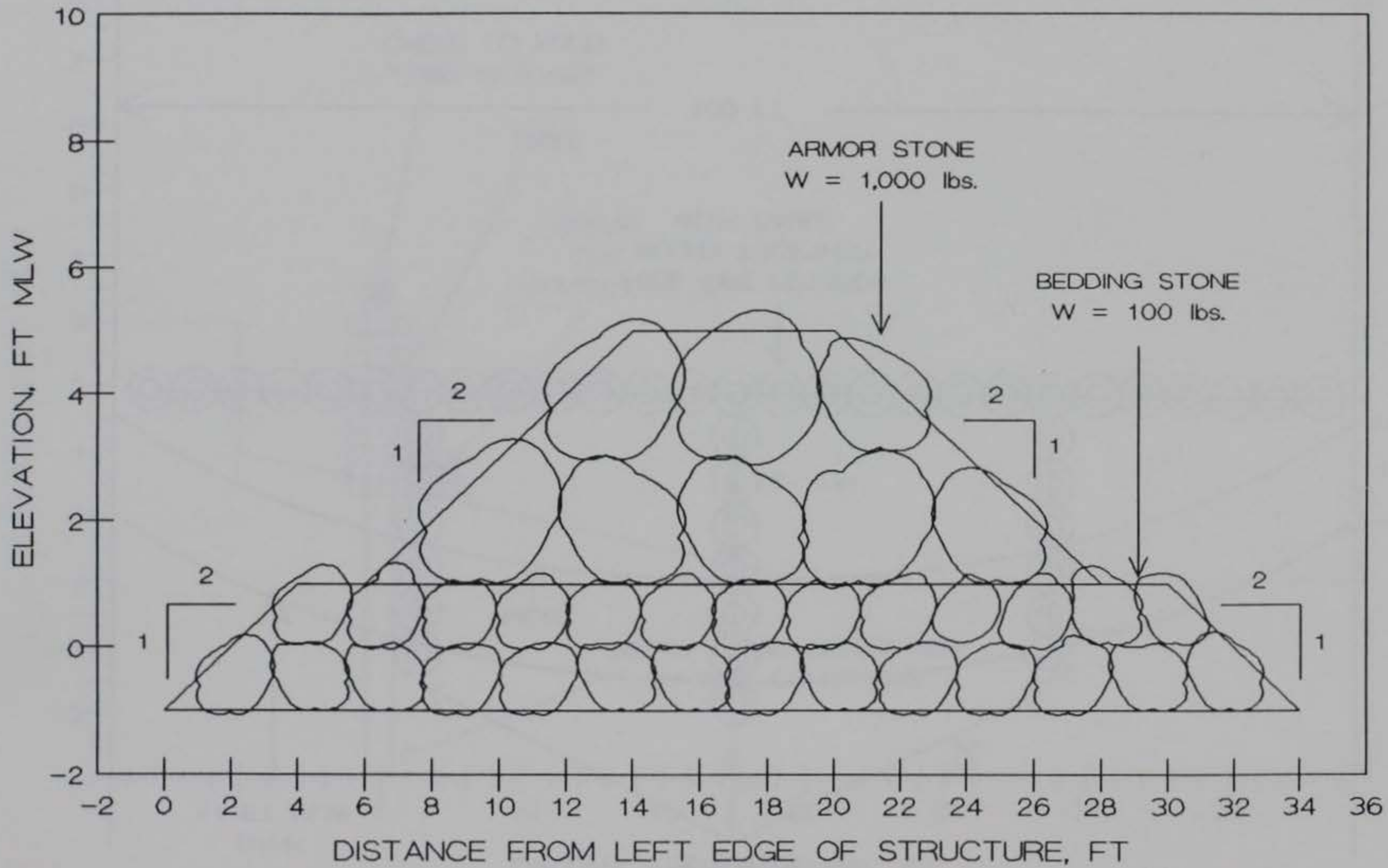
FIGURE 65. SEGMENTED LOW CRESTED BREAKWATER PROPOSED FOR SITE 3
