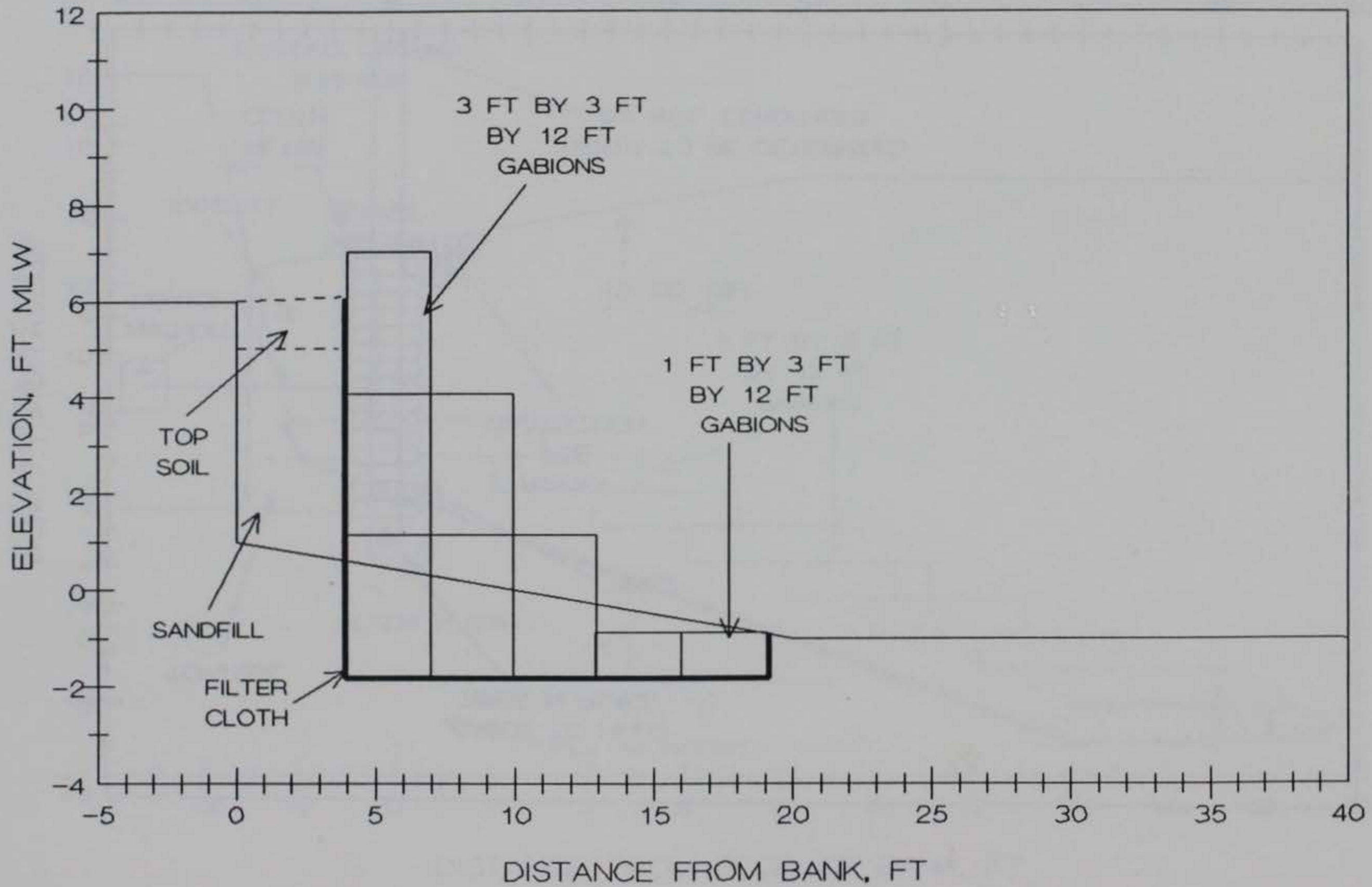
FIGURE 55. GABION BULKHEAD PROPOSED FOR SITE 5
