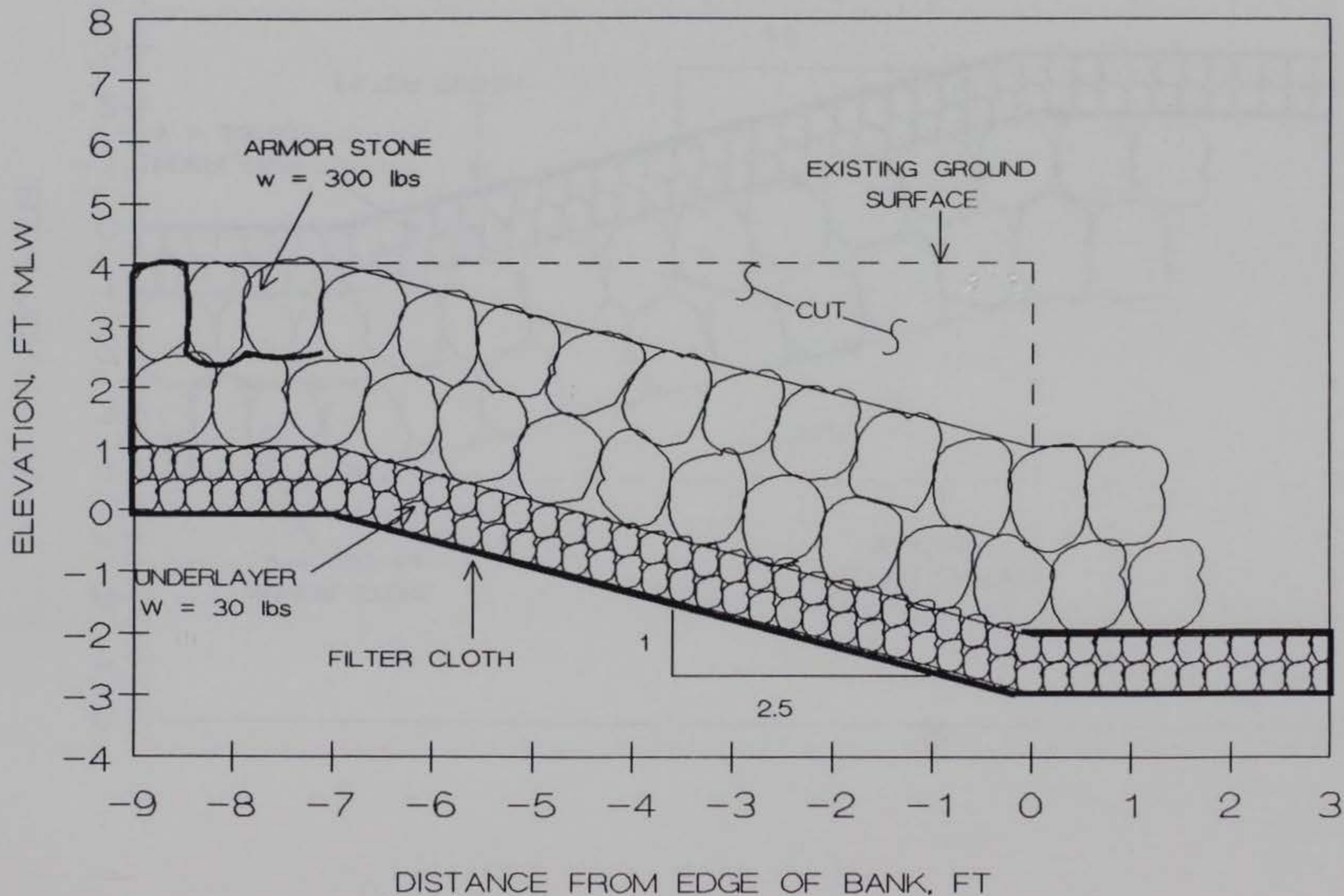
FIGURE 23. PLACED RIPRAP REVETMENT PROPOSED FOR SITE 4
