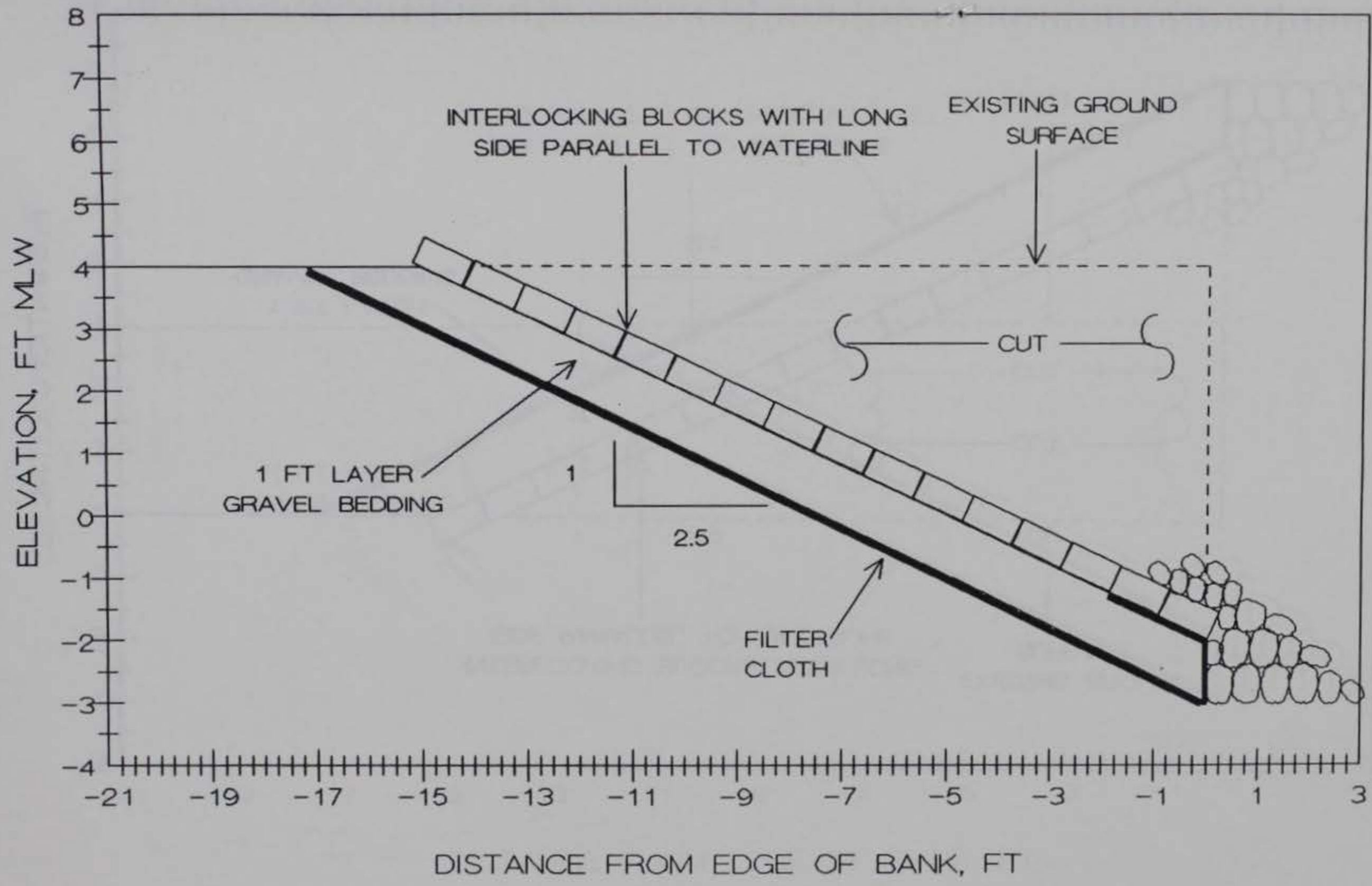
FIGURE 38. INTERLOCKING CONCRETE BLOCK REVETMENT PROPOSED FOR SITE 2
