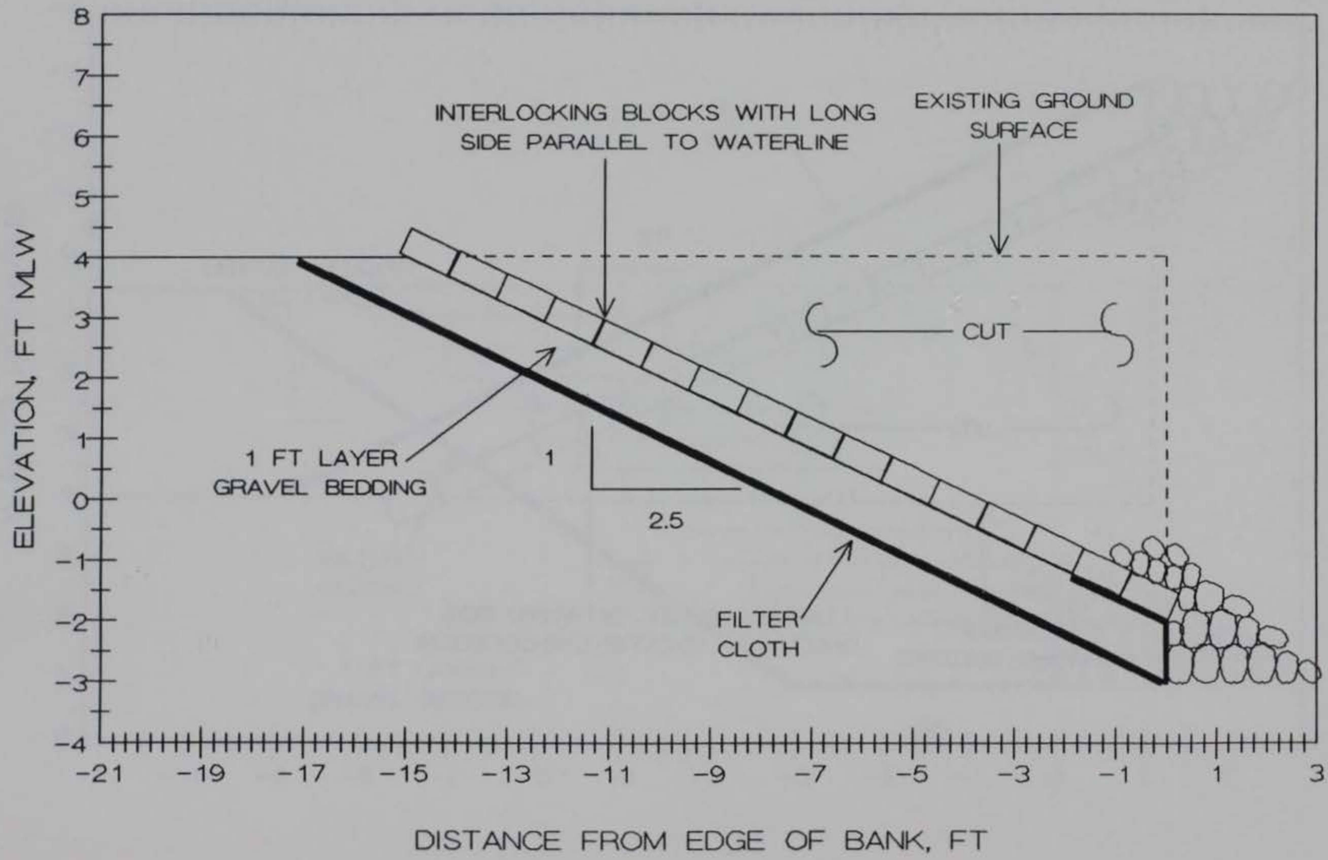
FIGURE 39. INTERLOCKING CONCRETE BLOCK REVETMENT PROPOSED FOR SITE 2A
