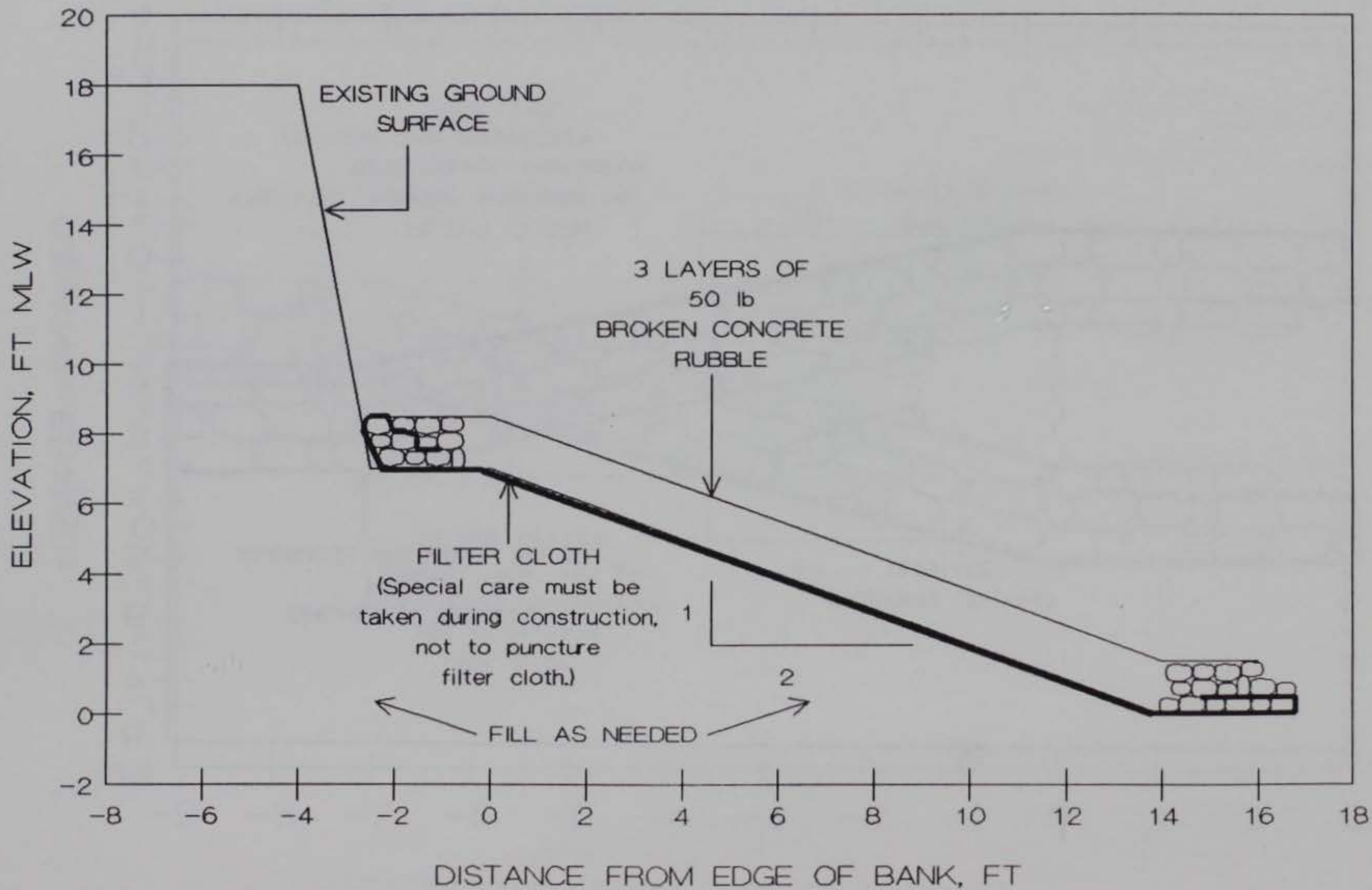
FIGURE 33. BROKEN CONCRETE REVETMENT PROPOSED FOR SITE 11
