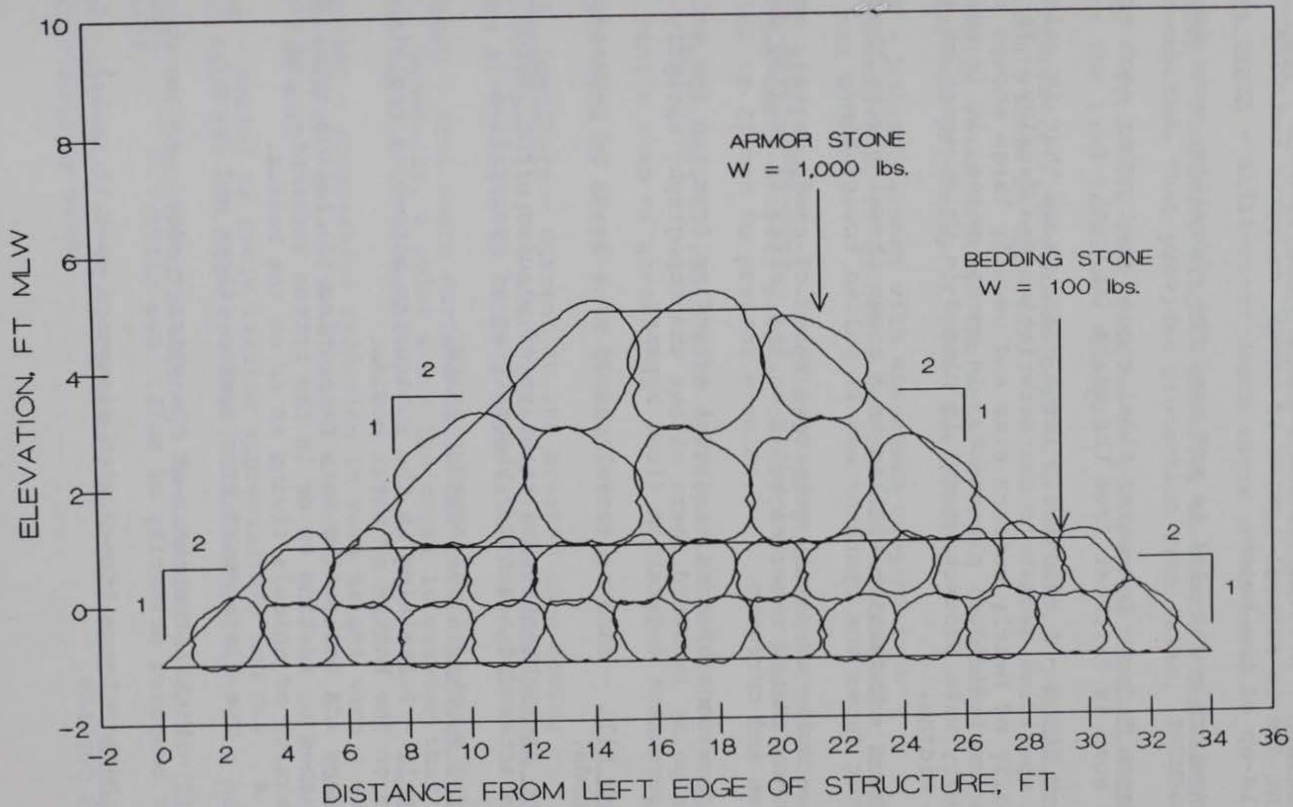
FIGURE 66. SEGMENTED LOW CRESTED BREAKWATER PROPOSED FOR SITE 4
