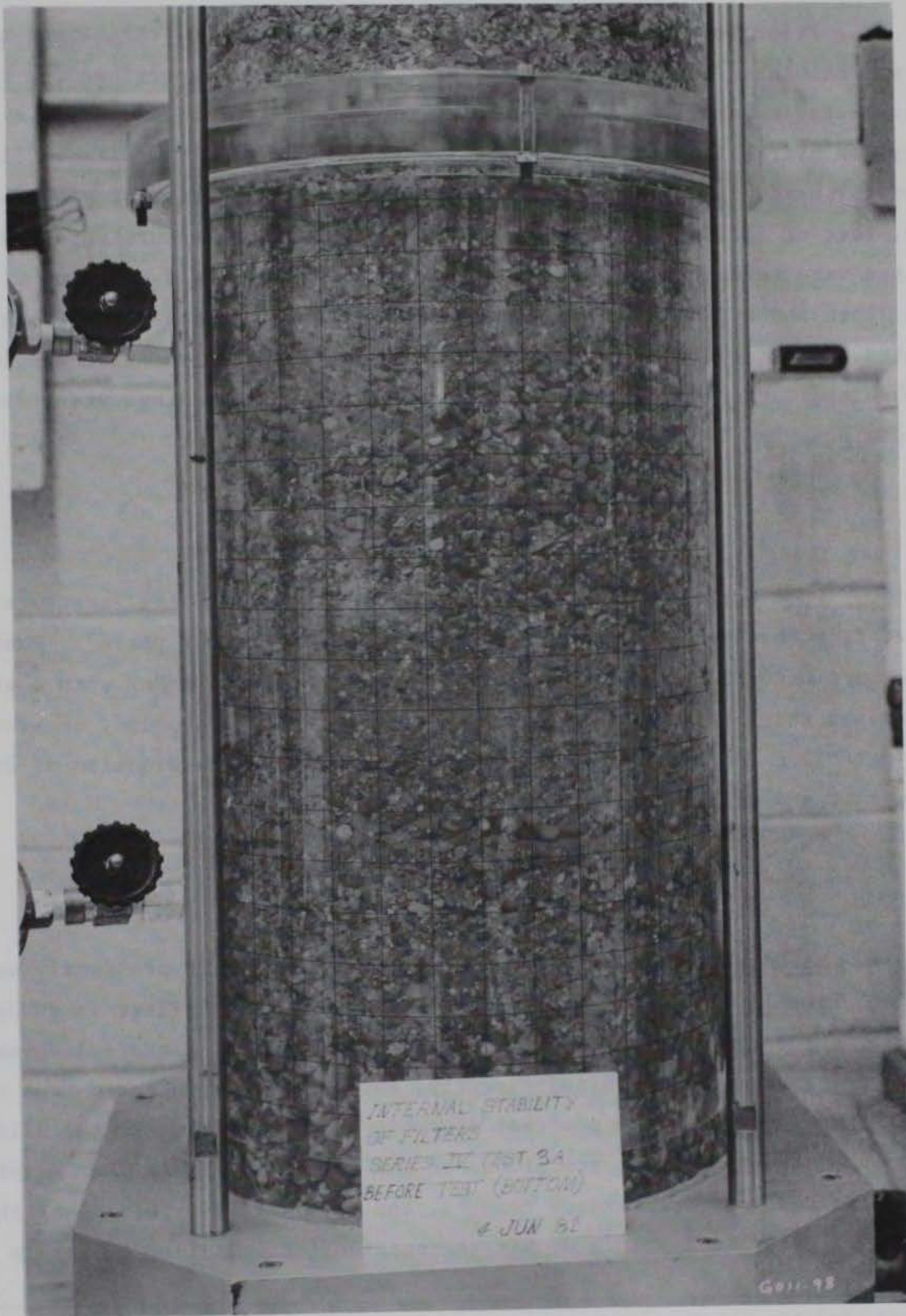
Figure 54. Bottom cylinder with grid before test
