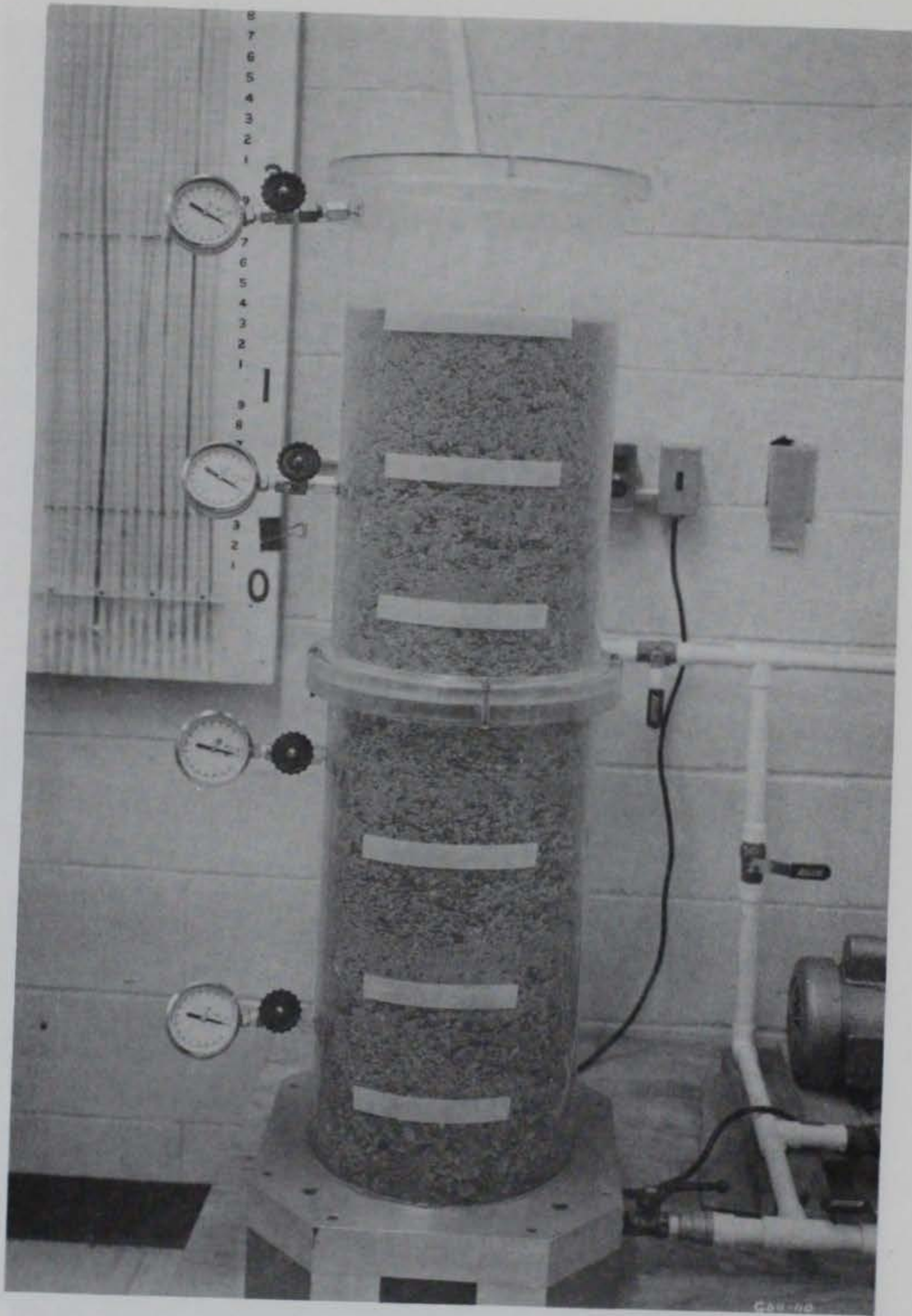
Figure 24. First increment of filter material removed from middle cylinder during posttest sampling (no base material for this test)
