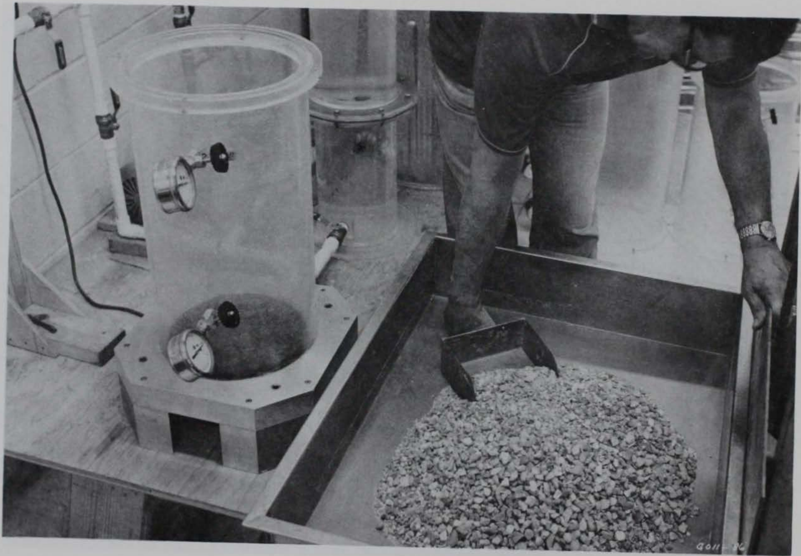
Figure 12. Mixing filter material prior to placement (Material shown is a poorly-graded sandy gravel used in Test No. 3A as discussed in Part IV.)
