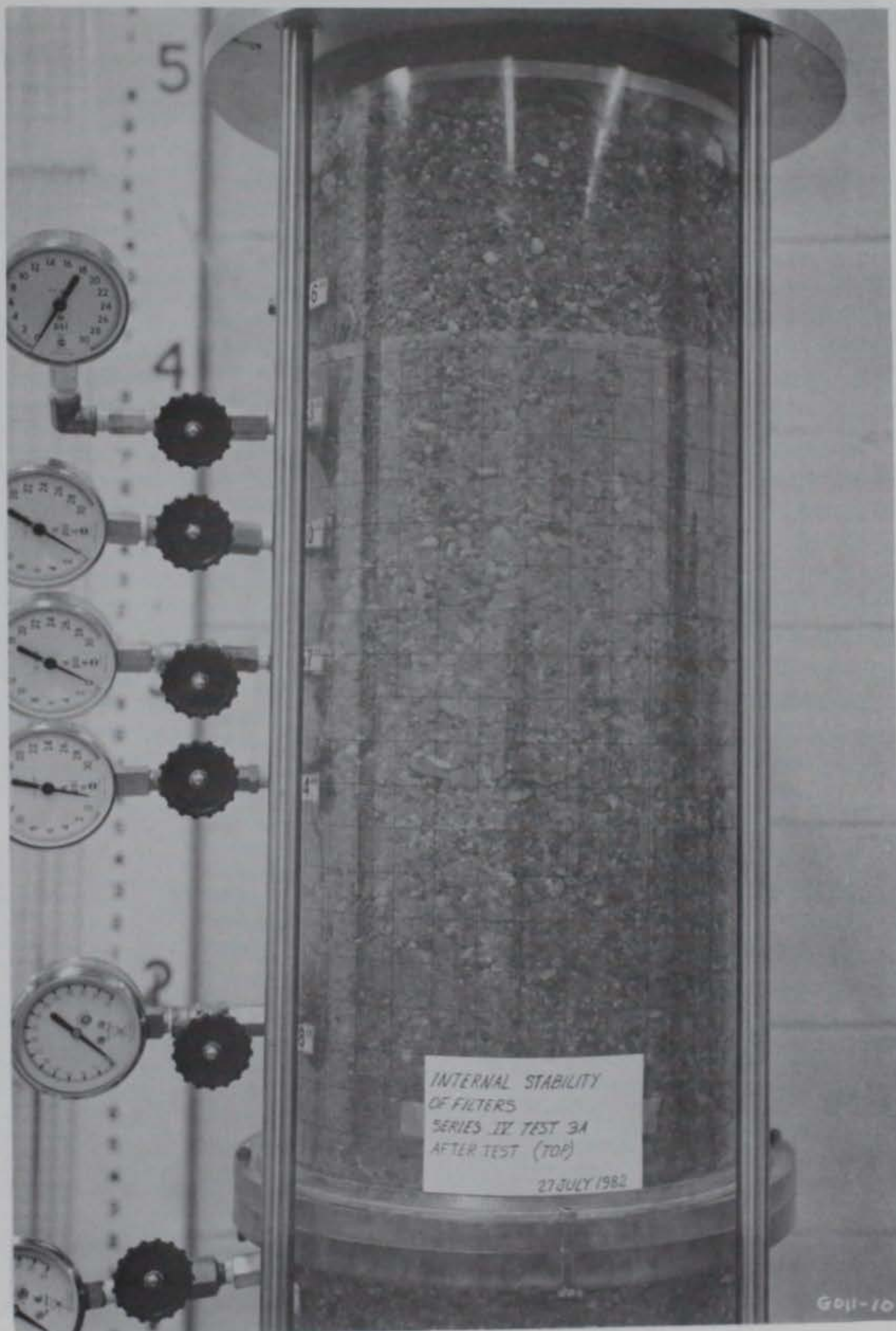
Figure 57. Top cylinder with grid after test
