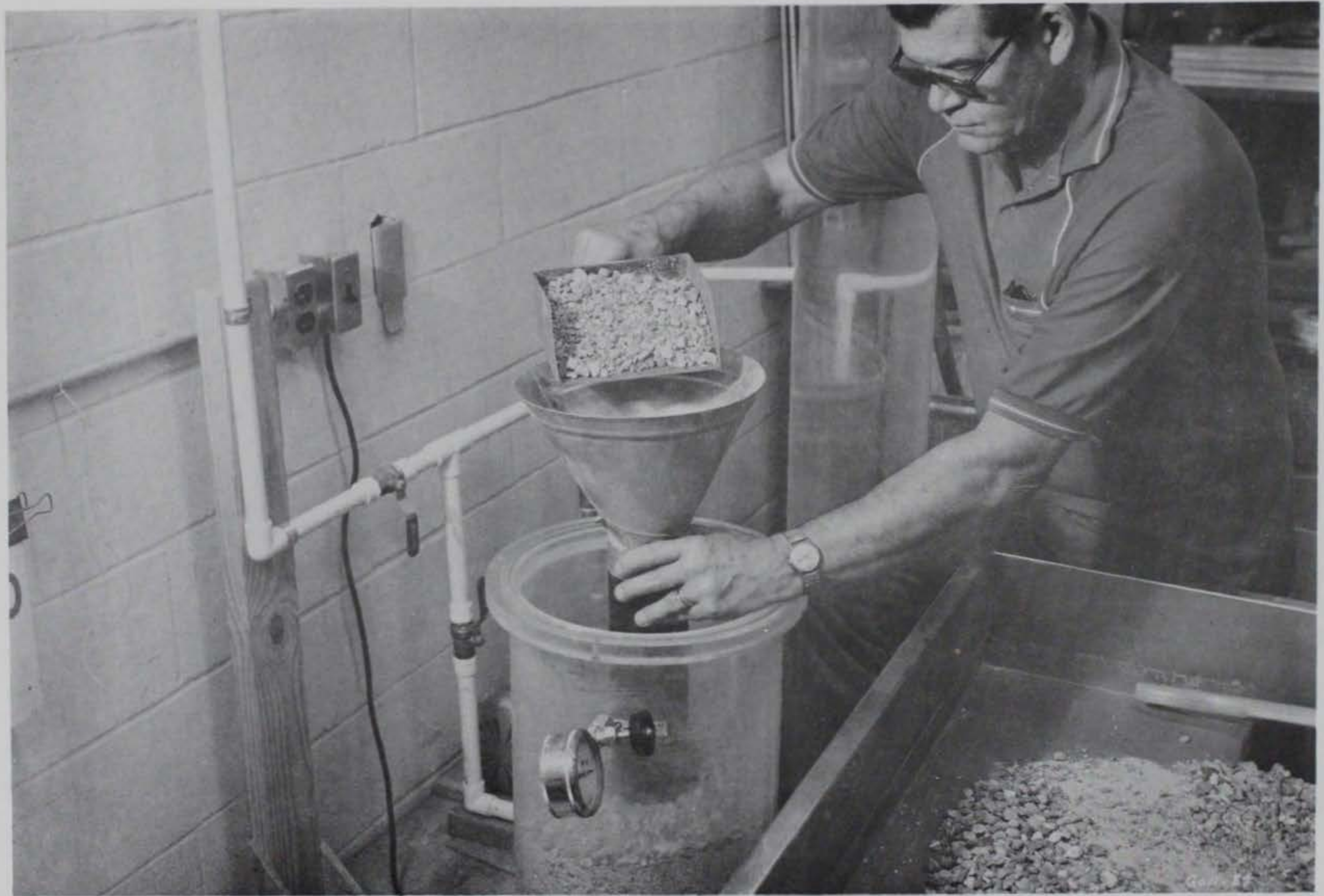
Figure 13. Placing filter material with funnel and open hose (Material shown is a poorly-graded sandy gravel used in Test No. 3A as discussed in Part IV.)
