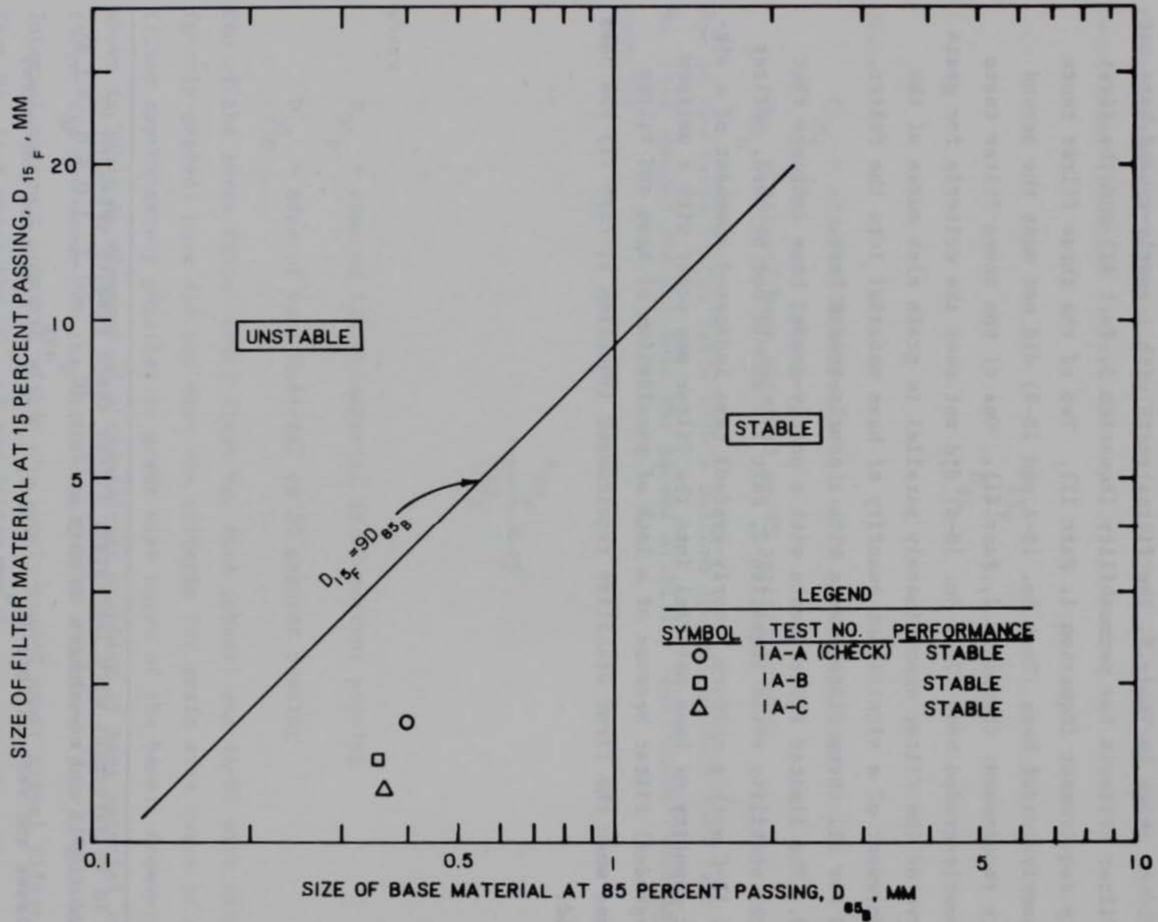
Figure 49. Filter stability for very uniform ( C_{u,avg} = 1.1 , 1.0 \leq C_u \leq 1.4 ) sand bases (after Sherard, Dunnigan, and Talbot 1984)
