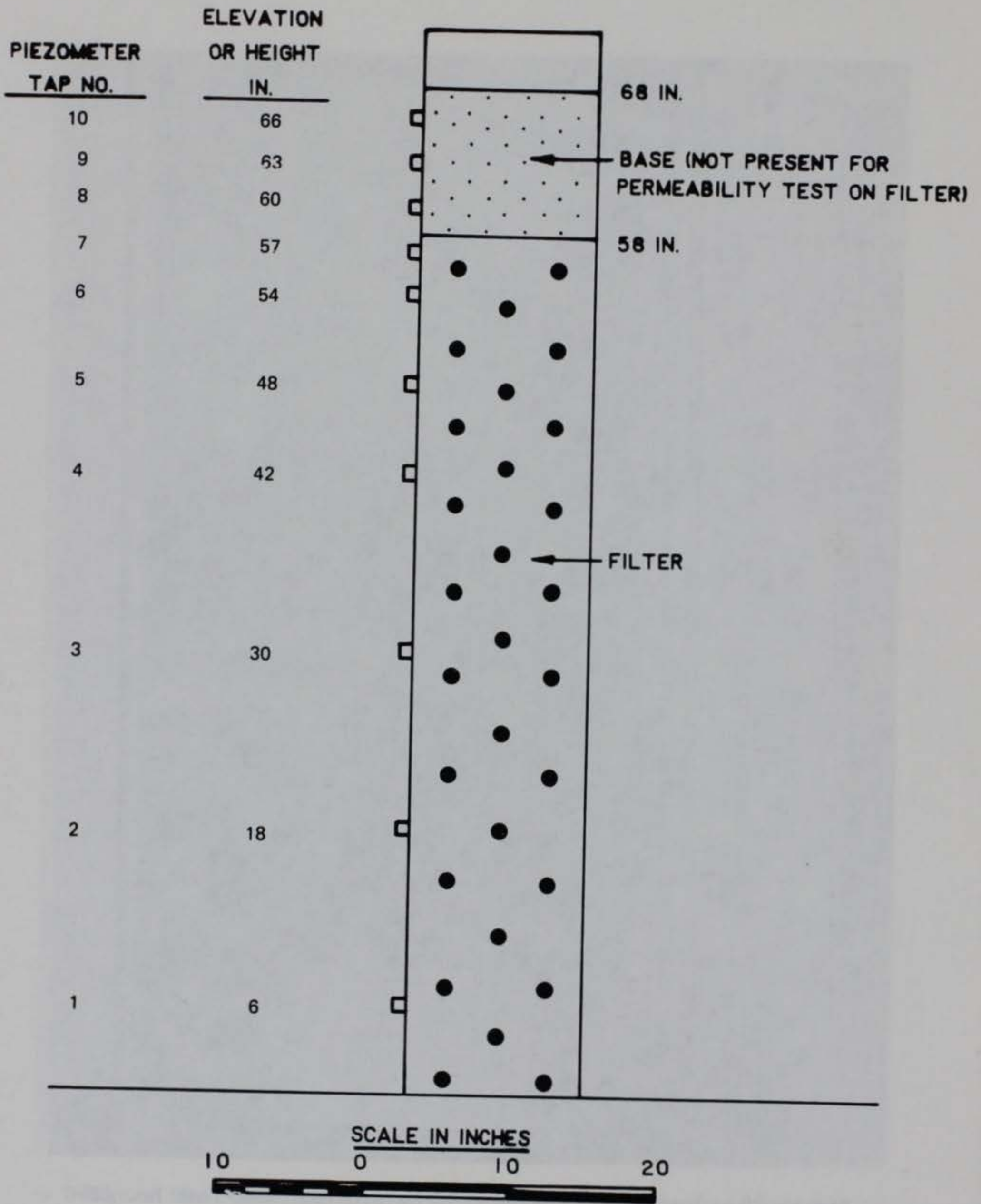
Figure 21. Schematic diagram showing location of piezometer taps
