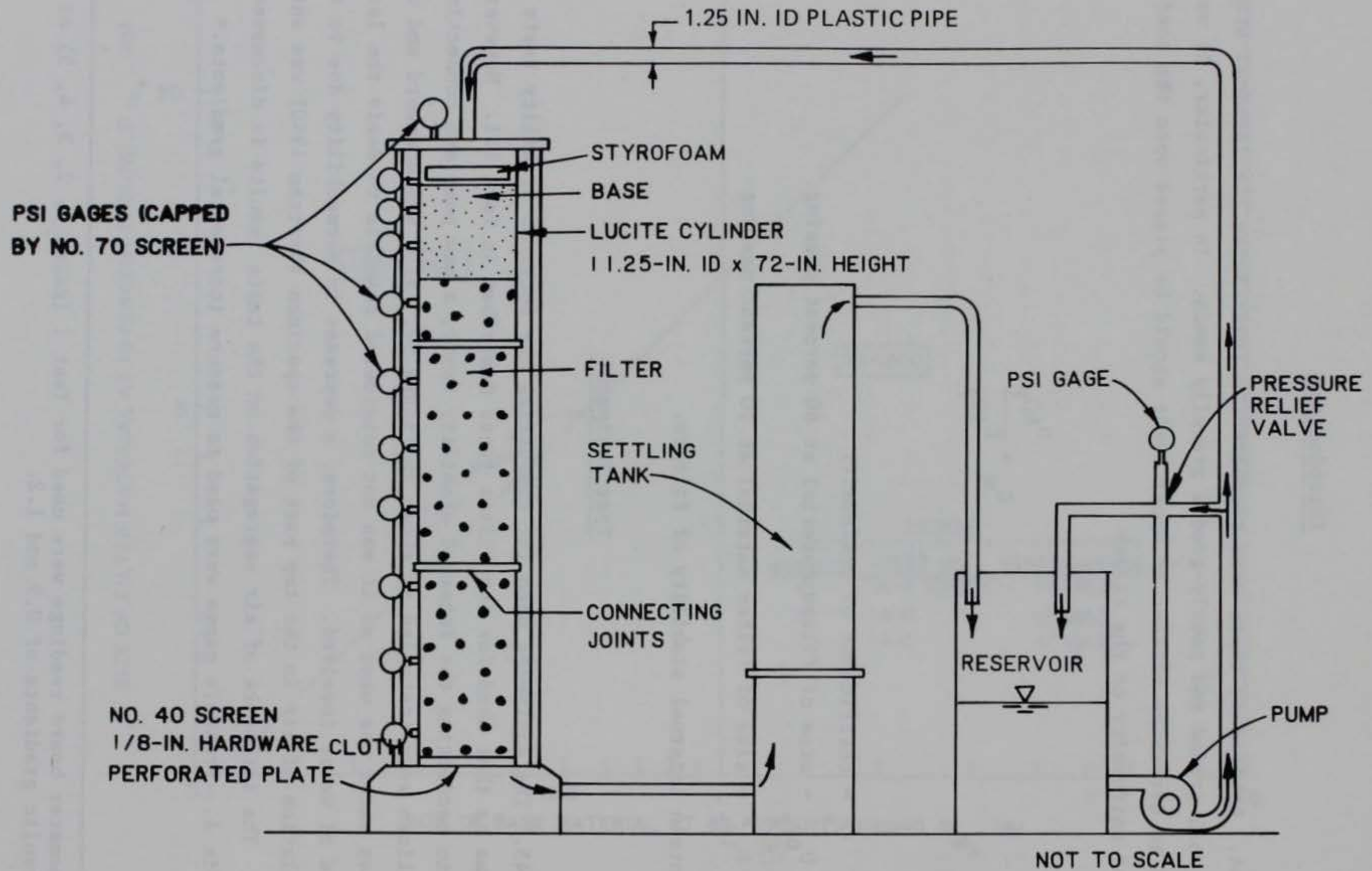
Figure 50. Schematic diagram of test apparatus used for internal stability of filters
