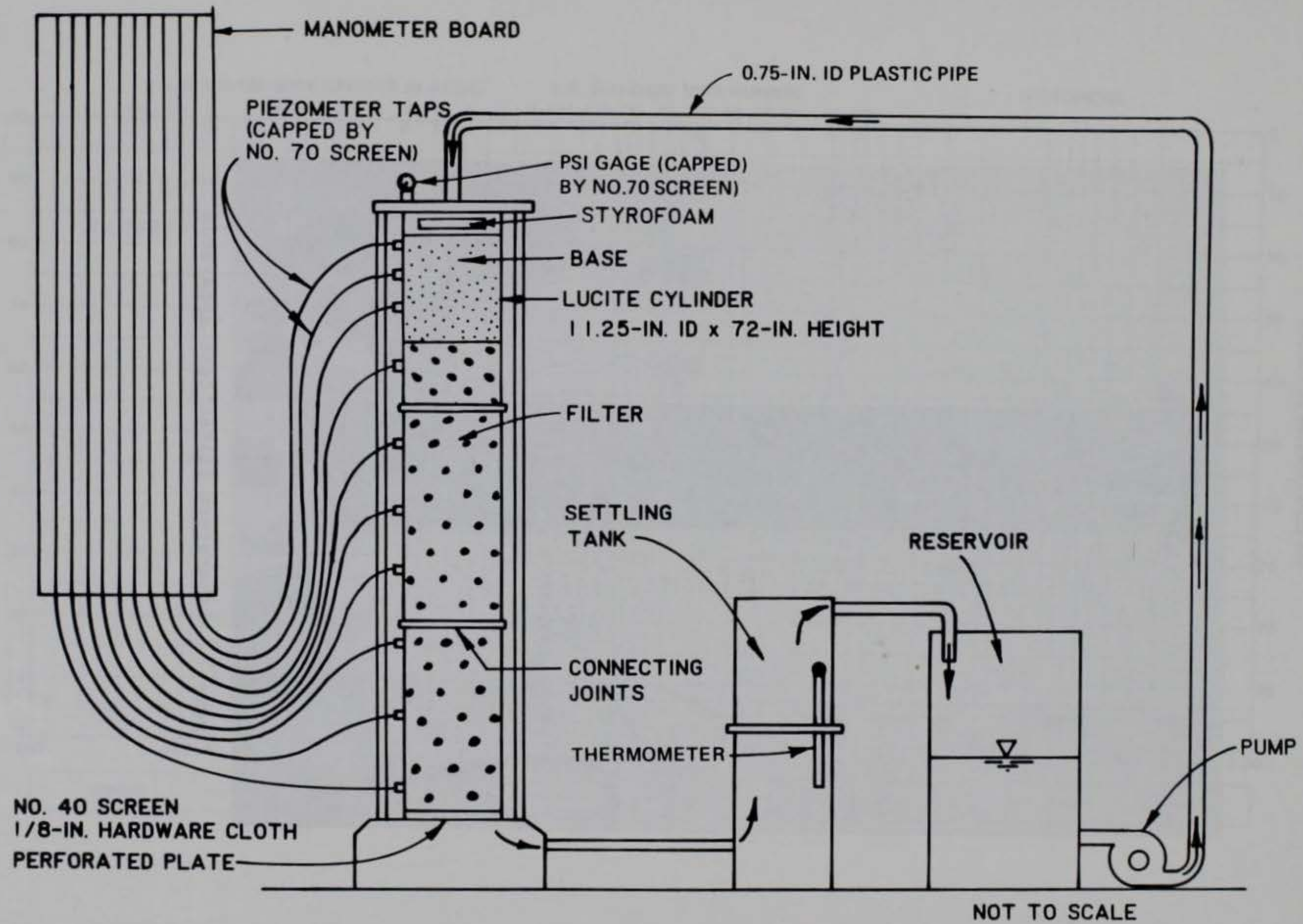
Figure 6. Schematic diagram of laboratory filter apparatus
