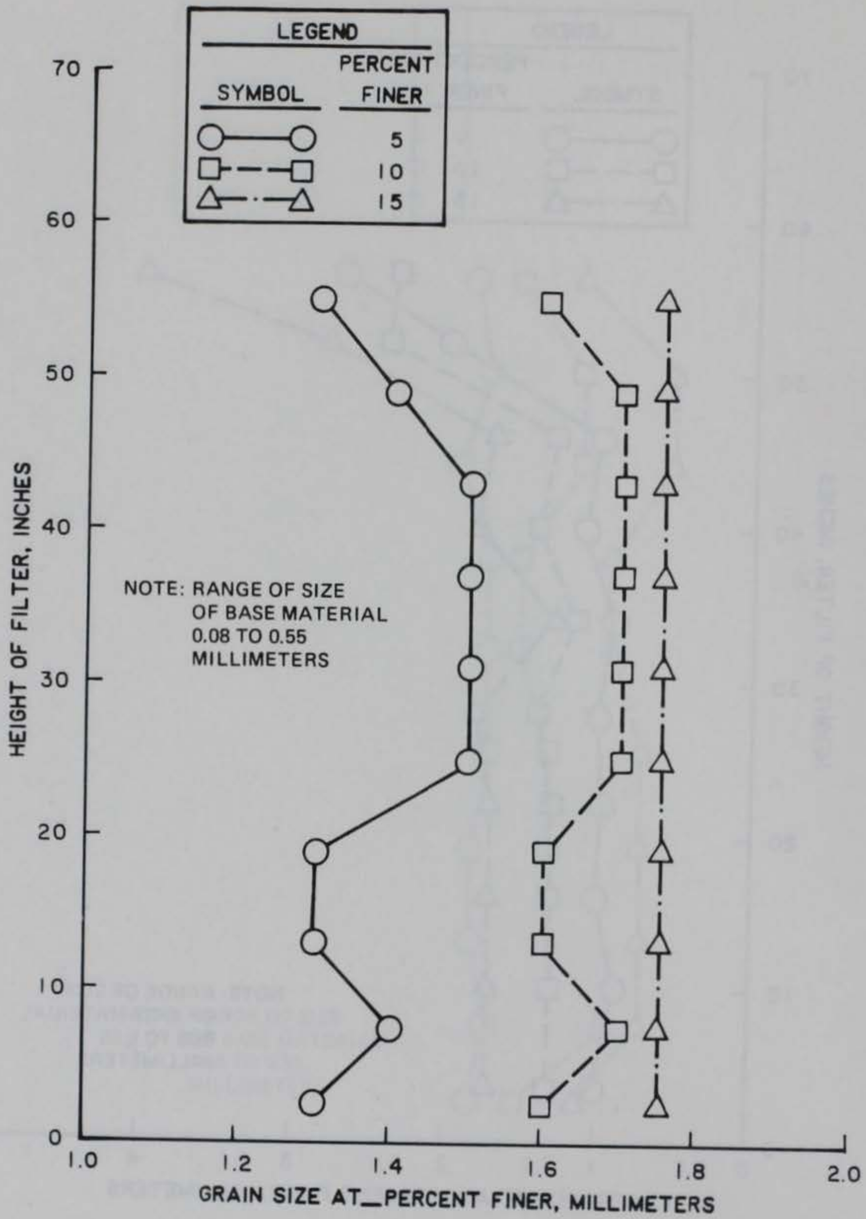
Figure 30. Posttest grain size of fine particles profile of filter for Test No. 1A-C
