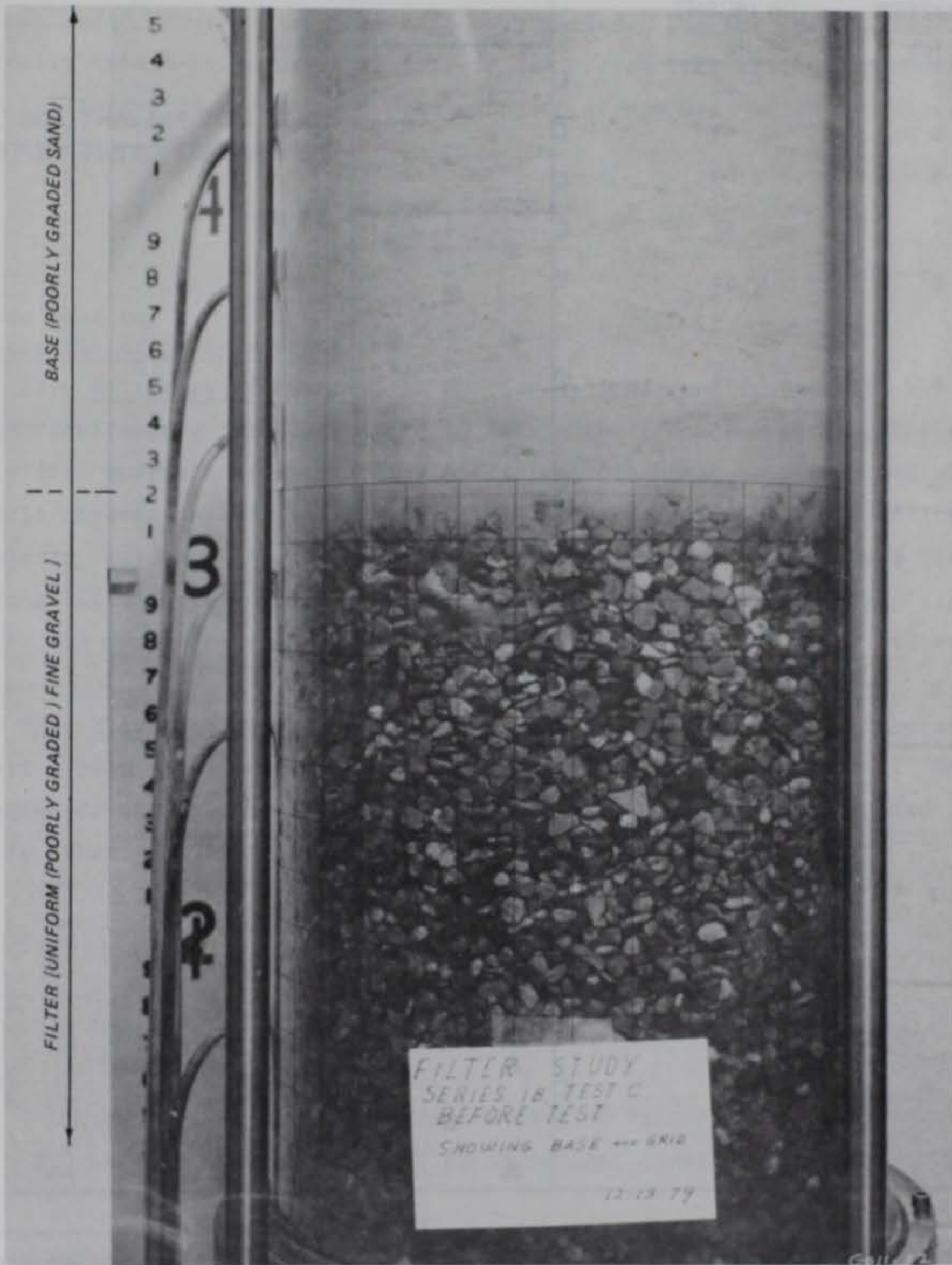
Figure 20. Top cylinder with grid before test for Test No. 1B-C
