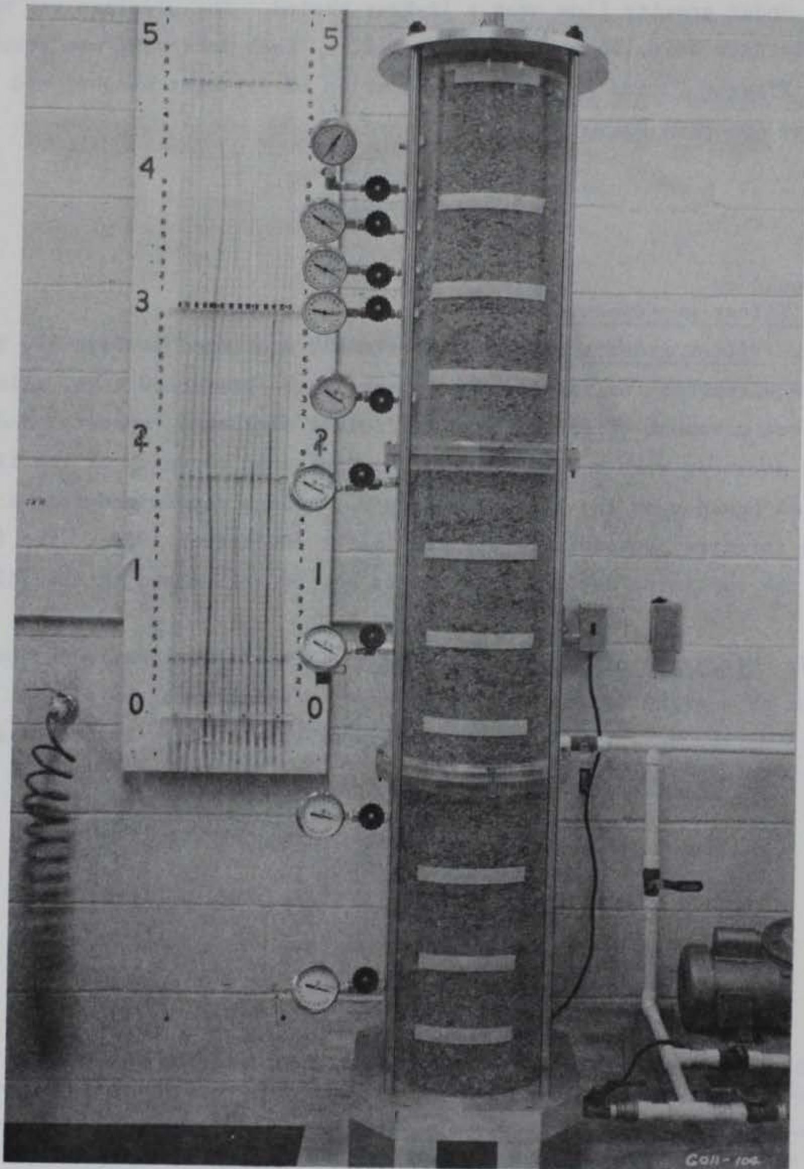
Figure 22. Overall view of specimen prior to posttest sampling (no base material for this test)
