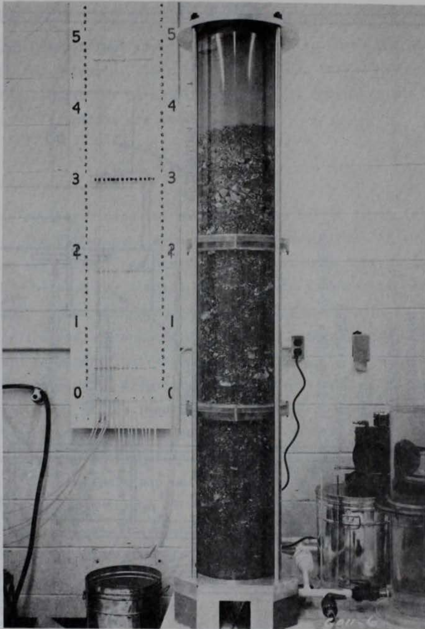
Figure 7. Laboratory filter test apparatus
