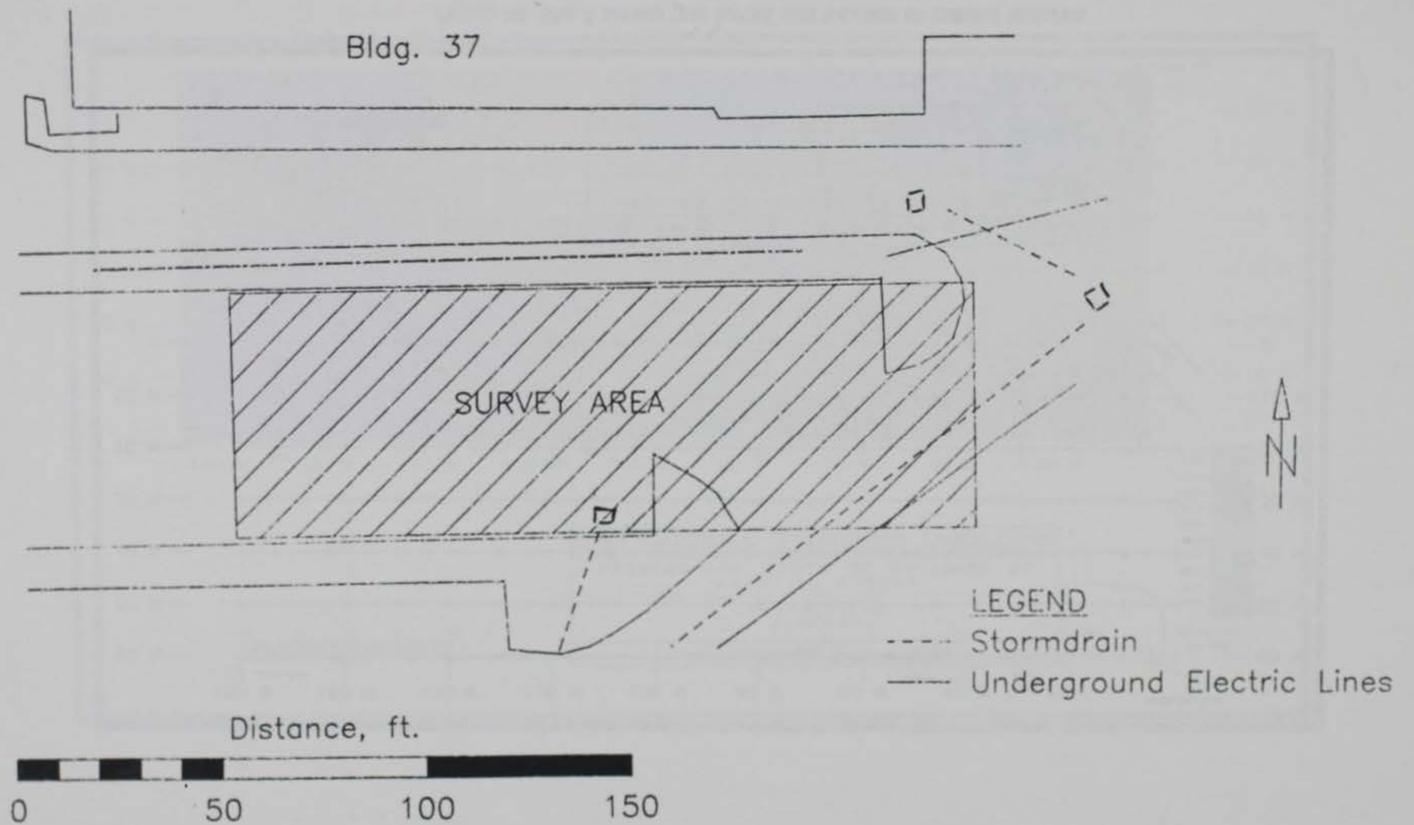
Figure 19. Map of Site 3 showing the area surveyed and location of underground utilities
