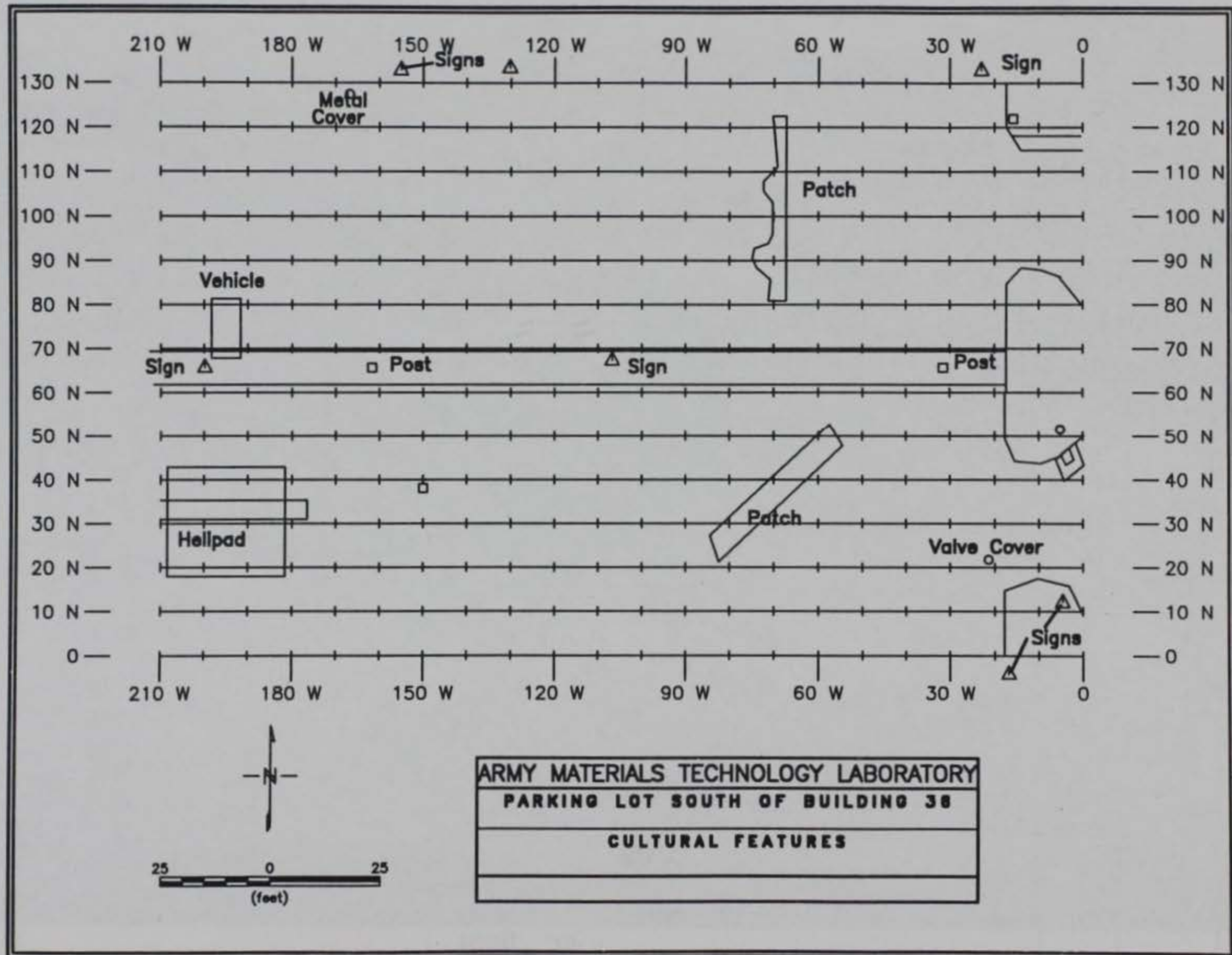
Figure 8. Site 1 survey grid layout and location of cultural features
