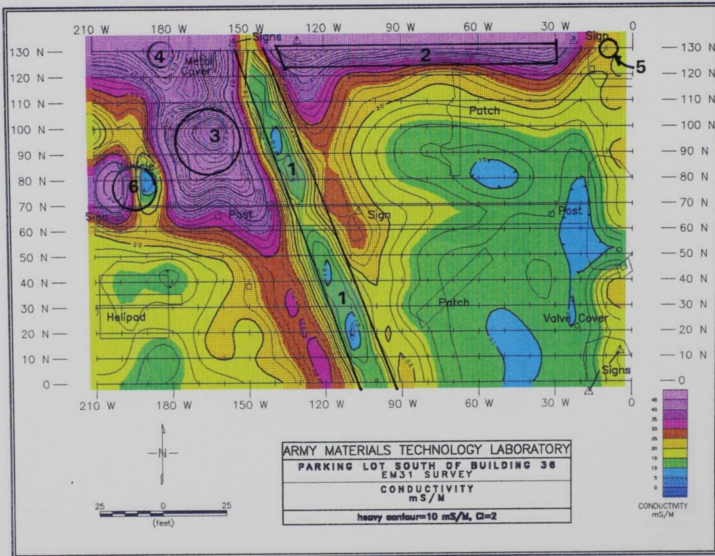
Figure 11. Results of EM-31 conductivity survey, Site 1
