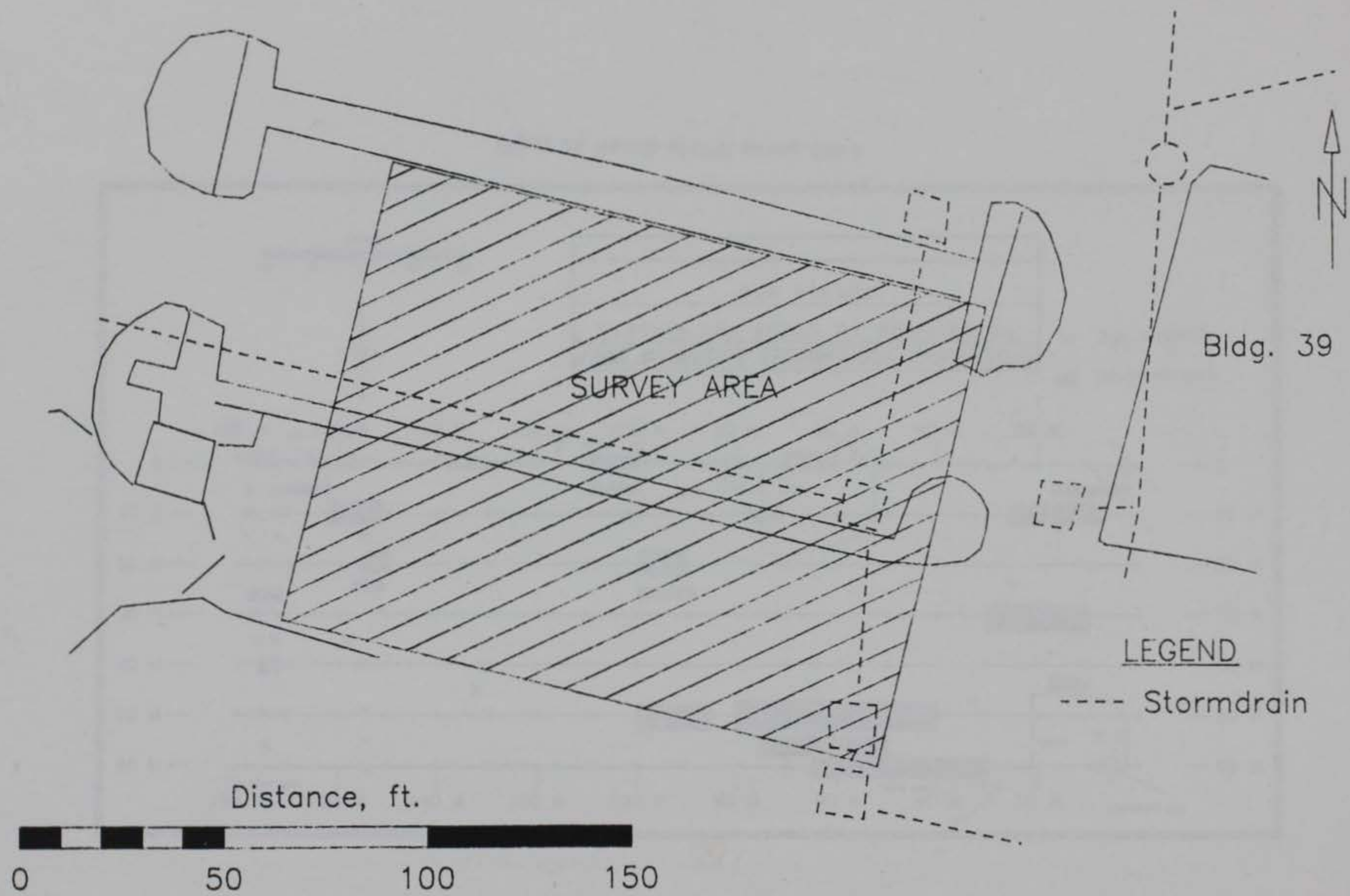
Figure 26. Map of Site 4 showing the area surveyed and location of underground utilities
