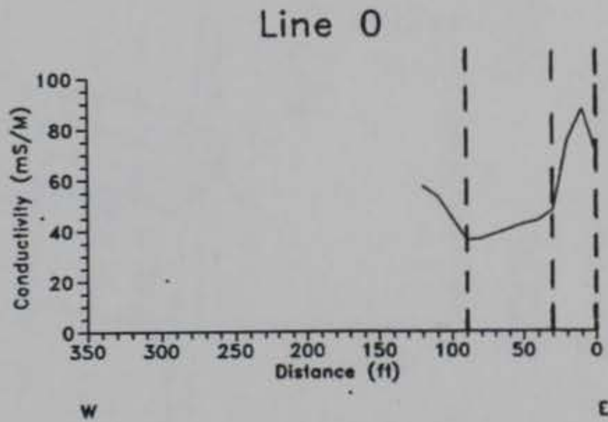
Figure 16. Results of EM-31 conductivity survey, Site 2
