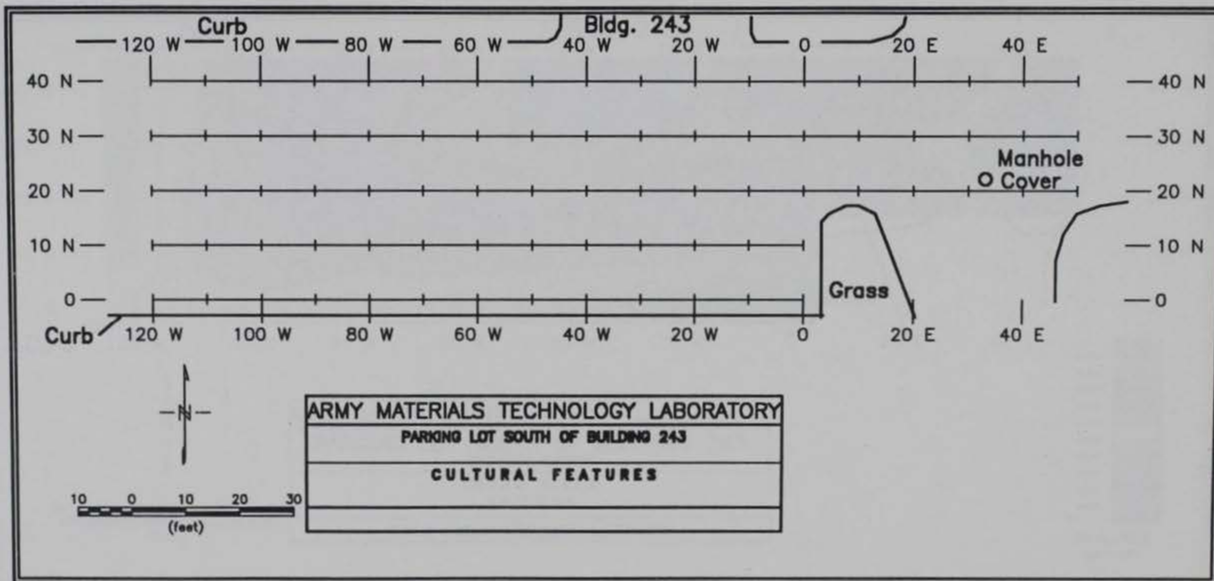
Figure 33. Site 5 survey grid layout and location of cultural features
