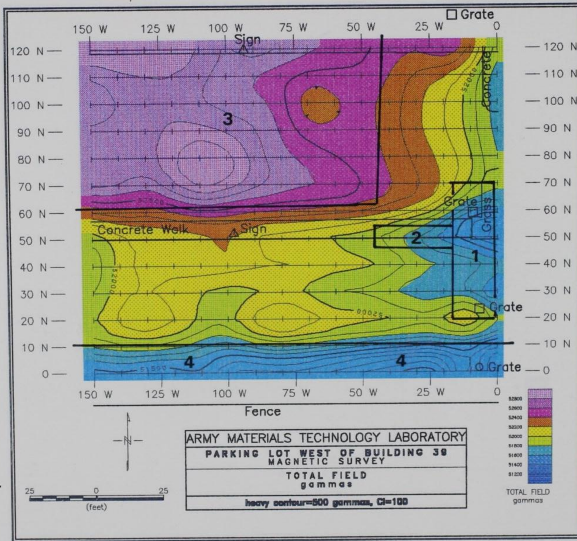
Figure 28. Results of magnetic total field survey, Site 4
