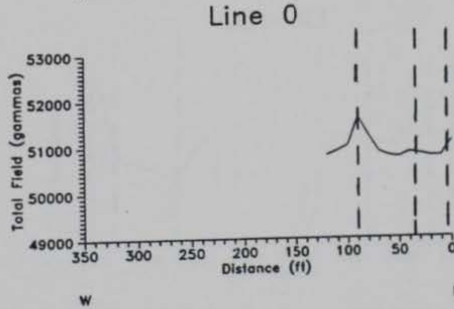
Figure 15. Results of magnetic total field survey, Site 2
