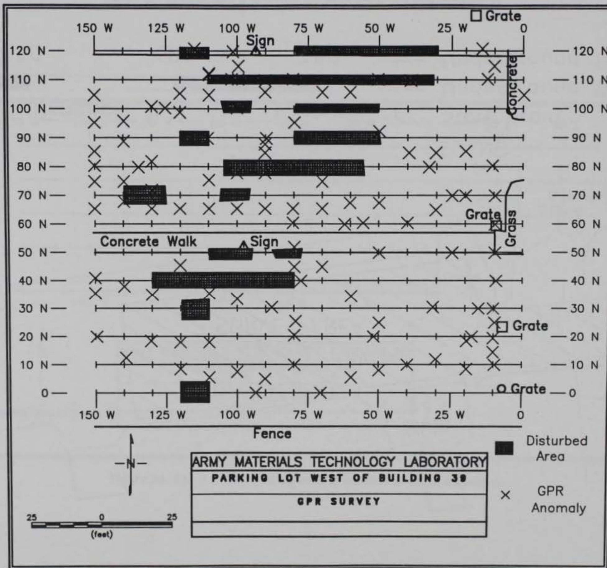
Figure 31. Results of GPR survey, Site 4
