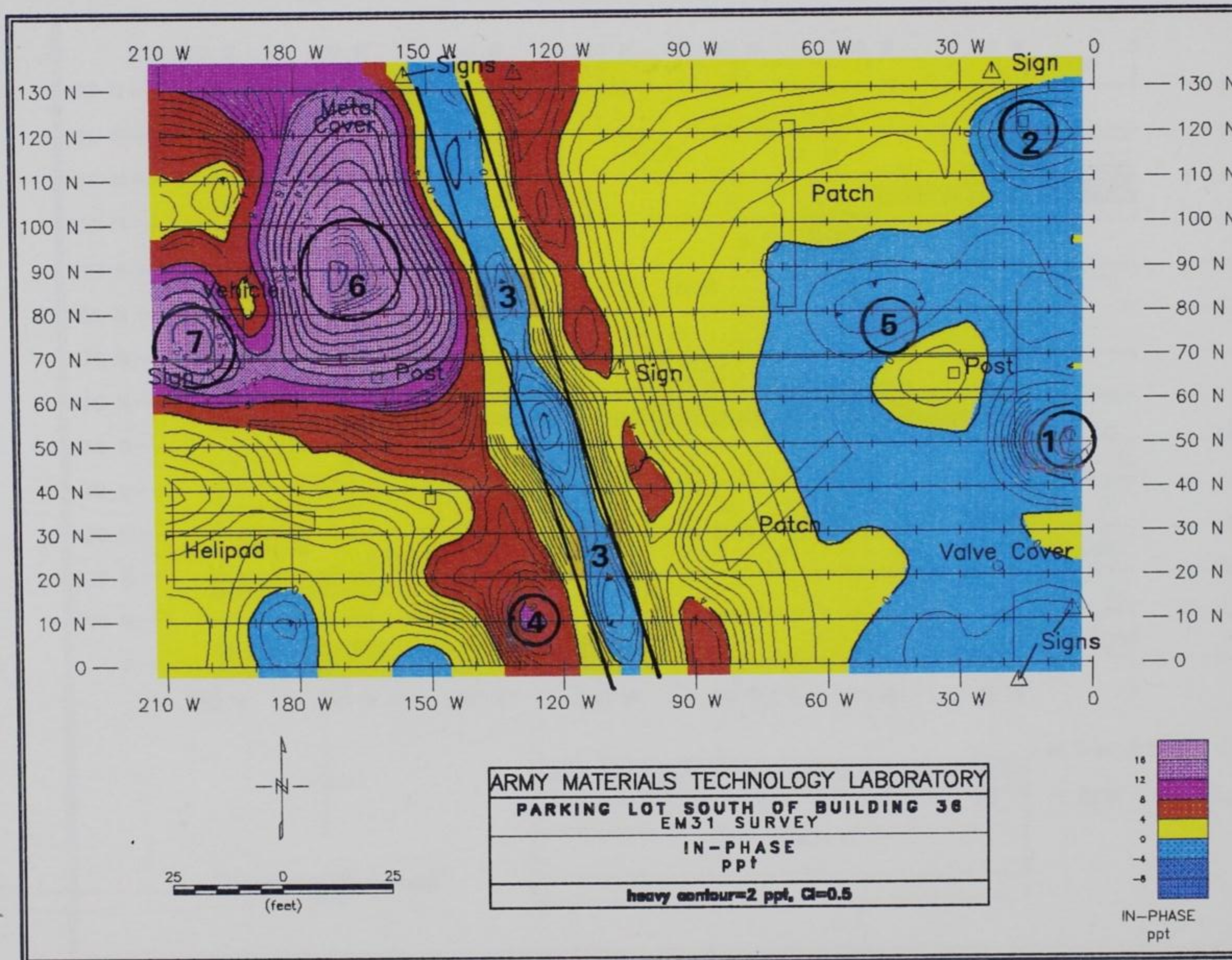
Figure 12. Results of EM-31 in-phase survey, Site 1
