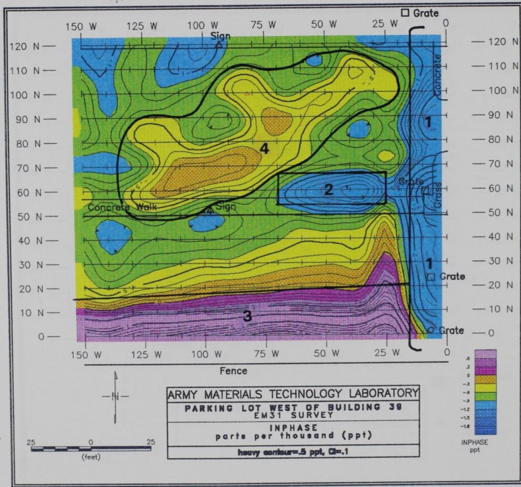
Figure 30. Results of EM-31 in-phase survey, Site 4
