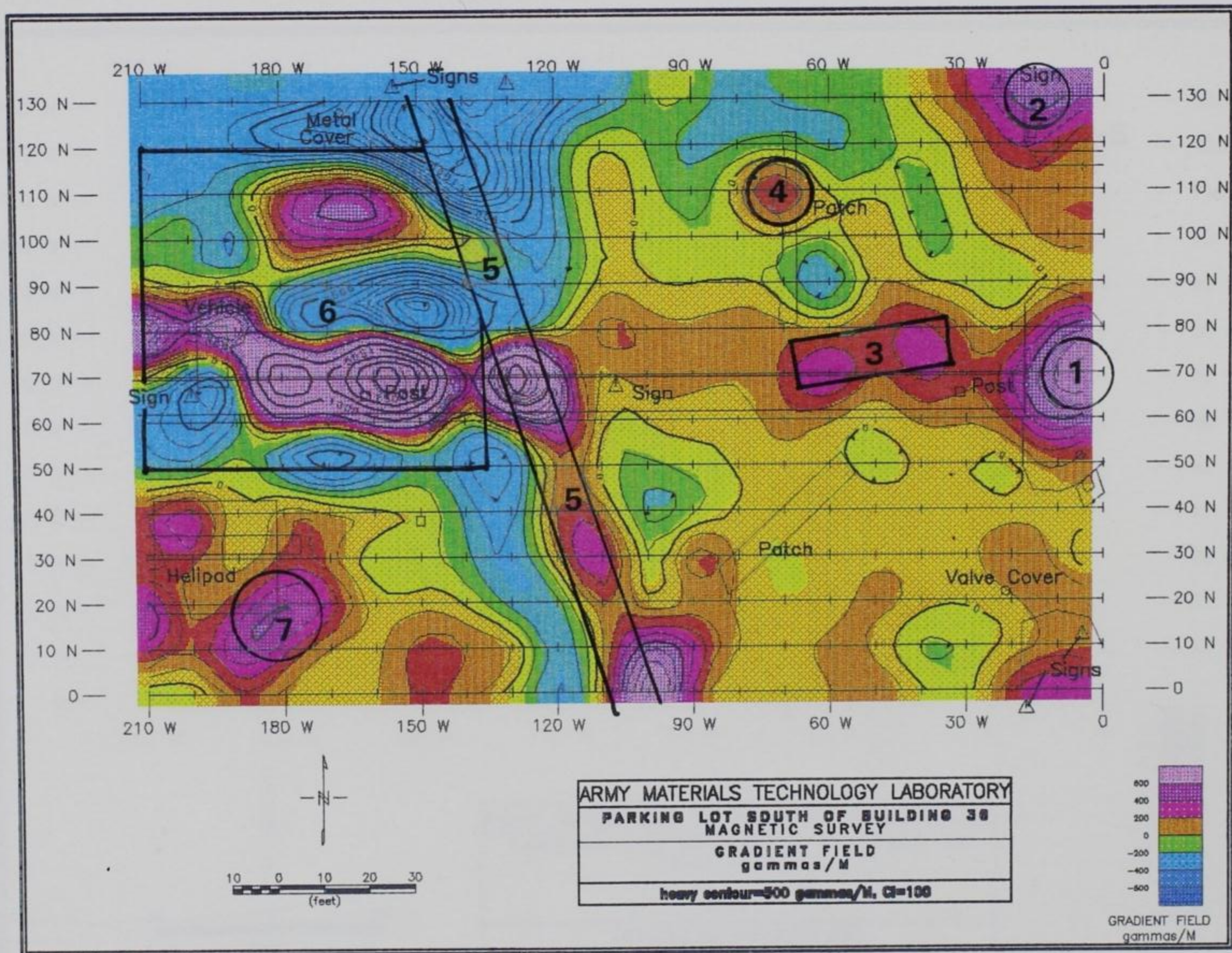
Figure 10. Results of magnetic gradient survey, Site 1
