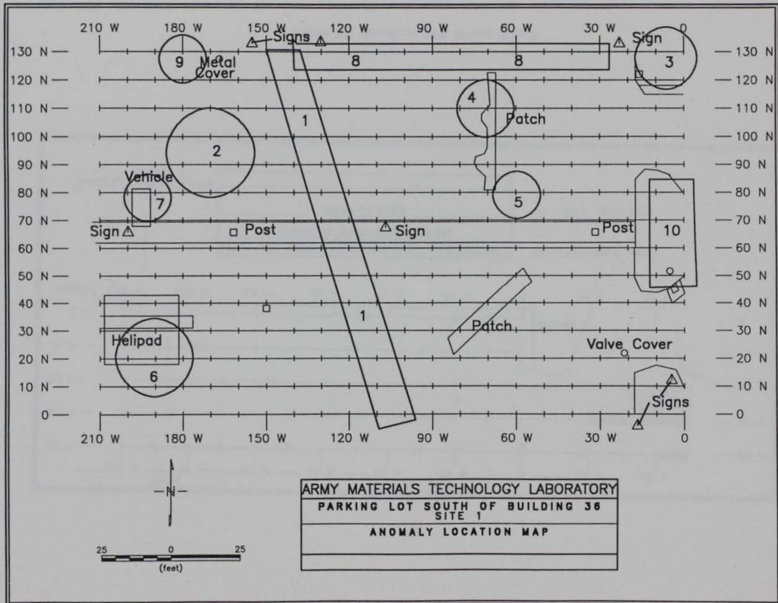
Figure 38. Anomaly location map, Site 1
