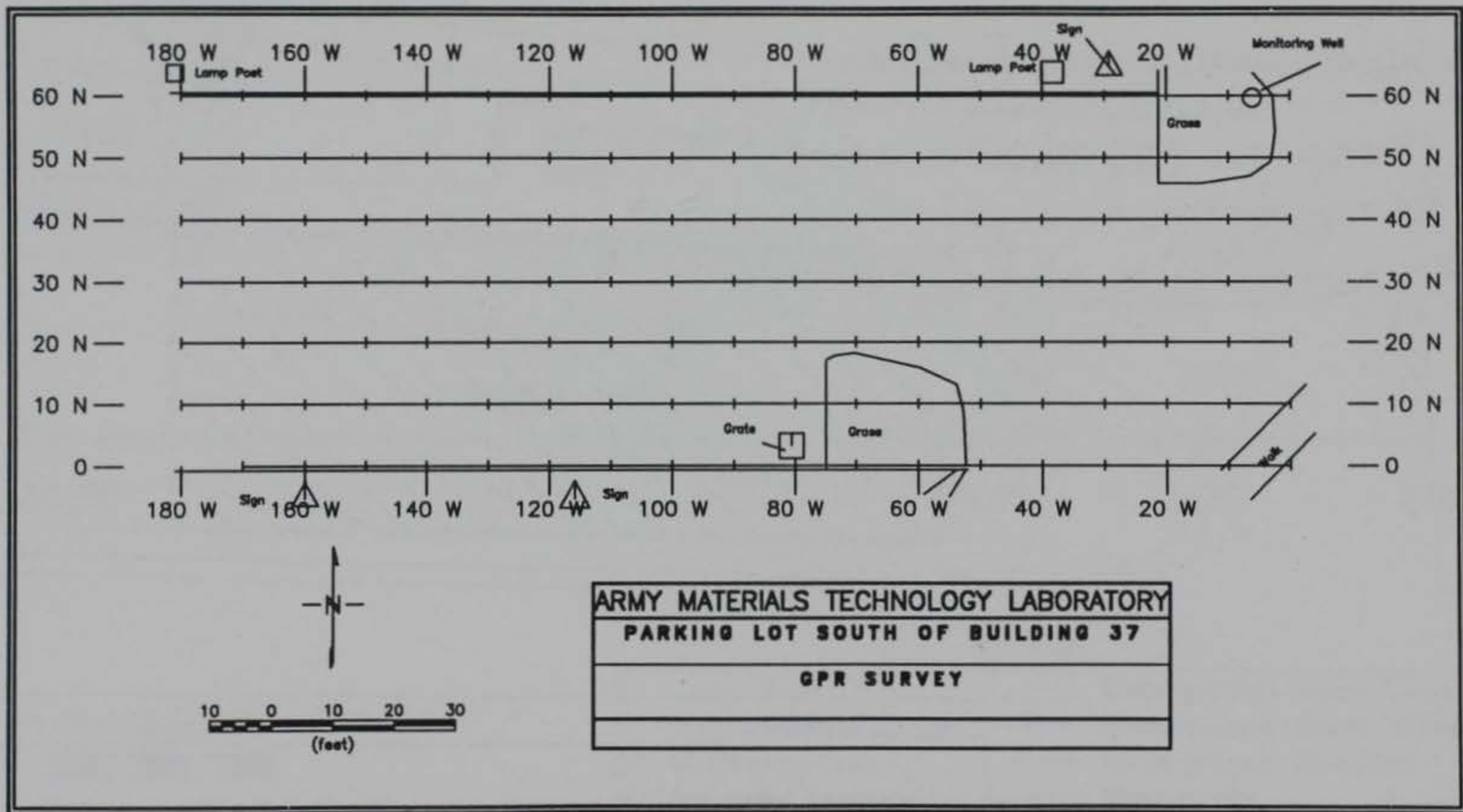
Figure 20. Site 3 survey grid layout and location of cultural features
