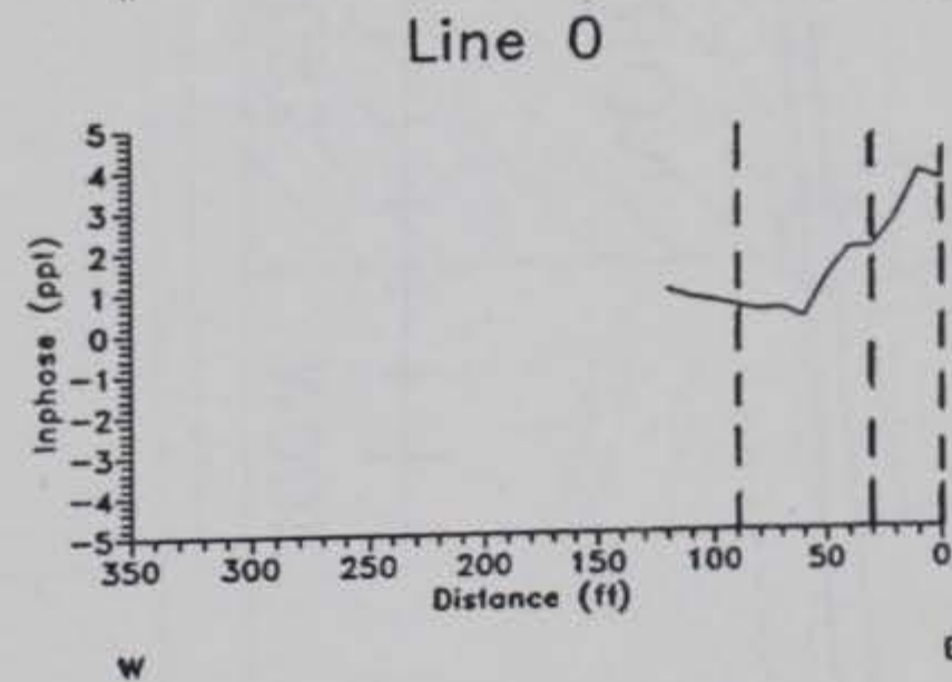
Figure 17. Results of EM-31 in-phase survey, Site 2
