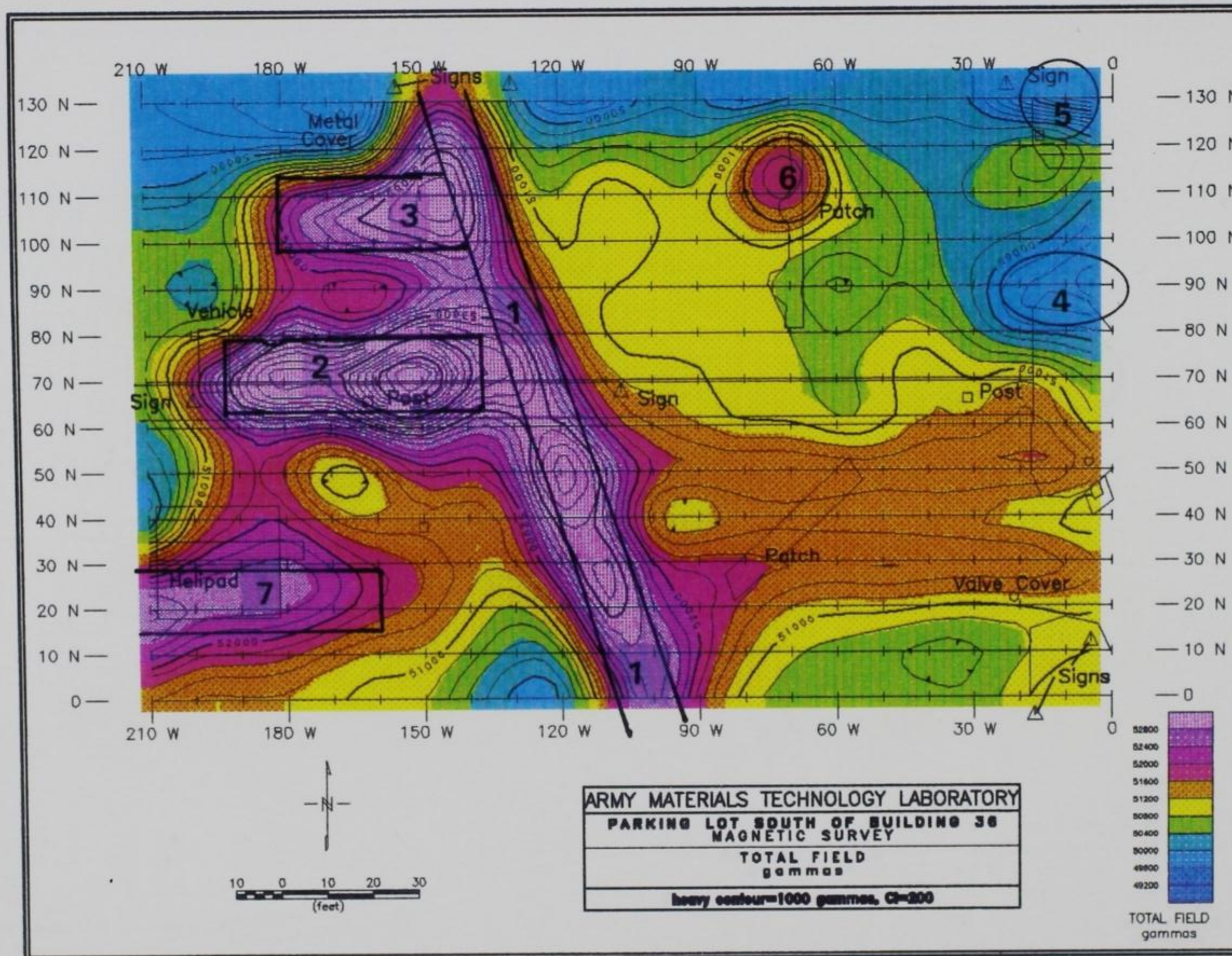
Figure 9. Results of magnetic total field survey, Site 1
