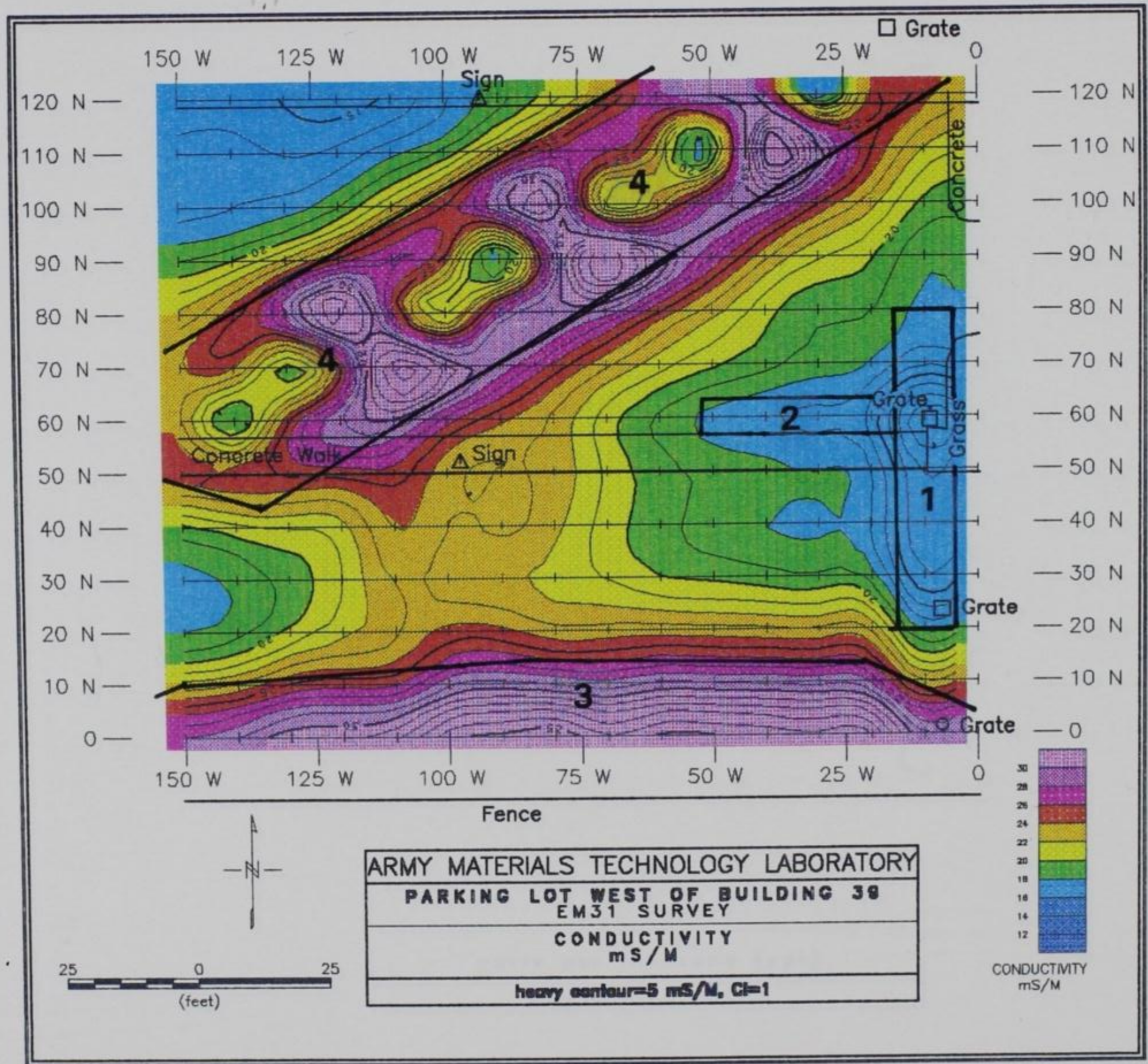
Figure 29. Results of EM-31 conductivity survey, Site 4
