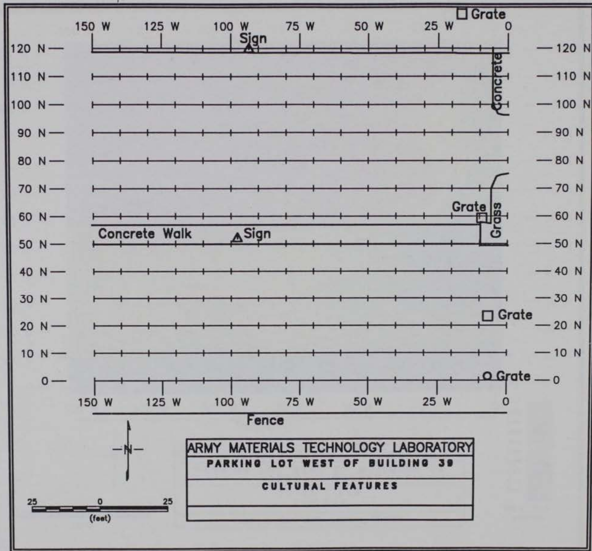
Figure 27. Site 4 survey grid layout and location of cultural features
