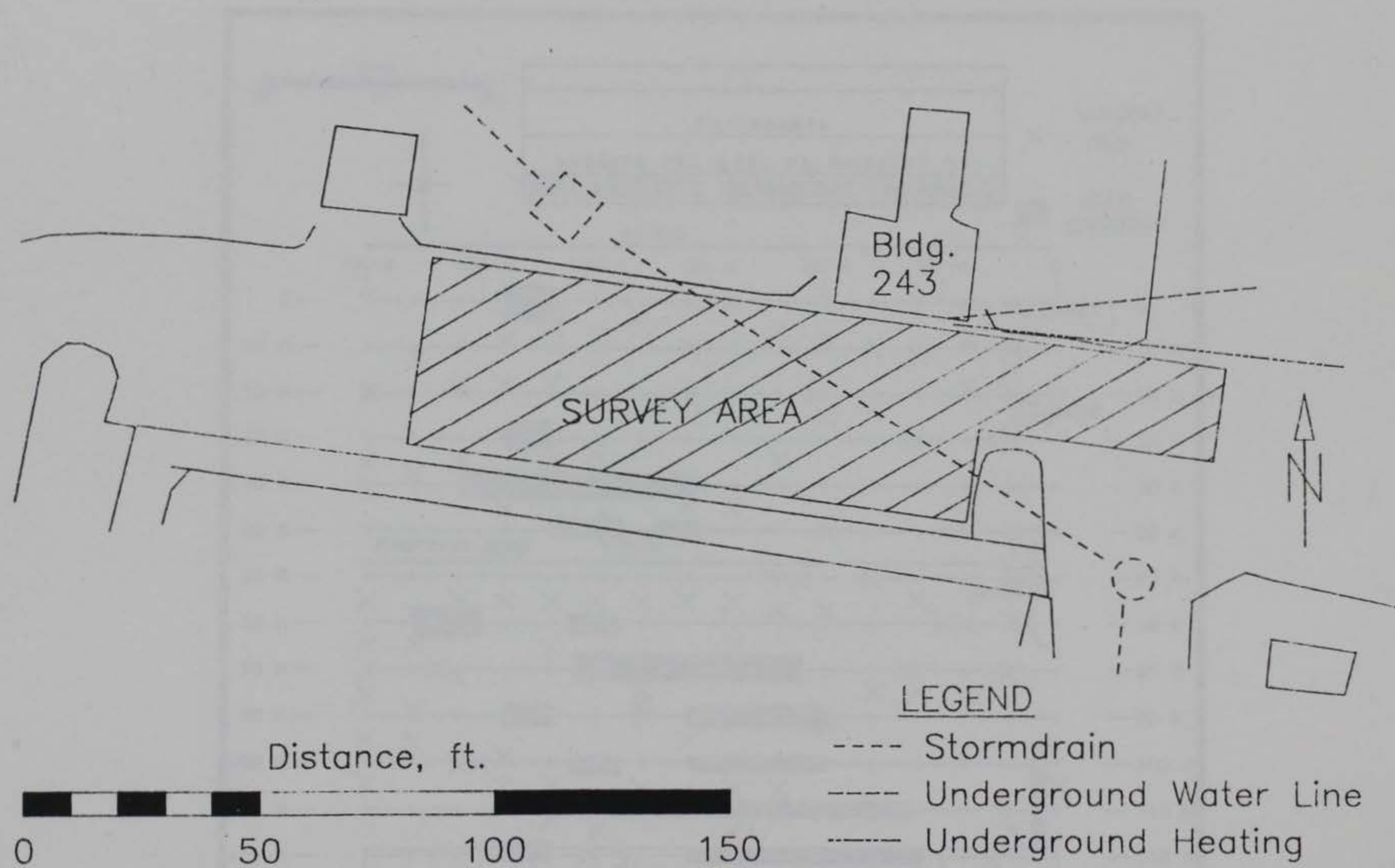
Figure 32. Map of Site 5 showing the area surveyed and location of underground utilities
