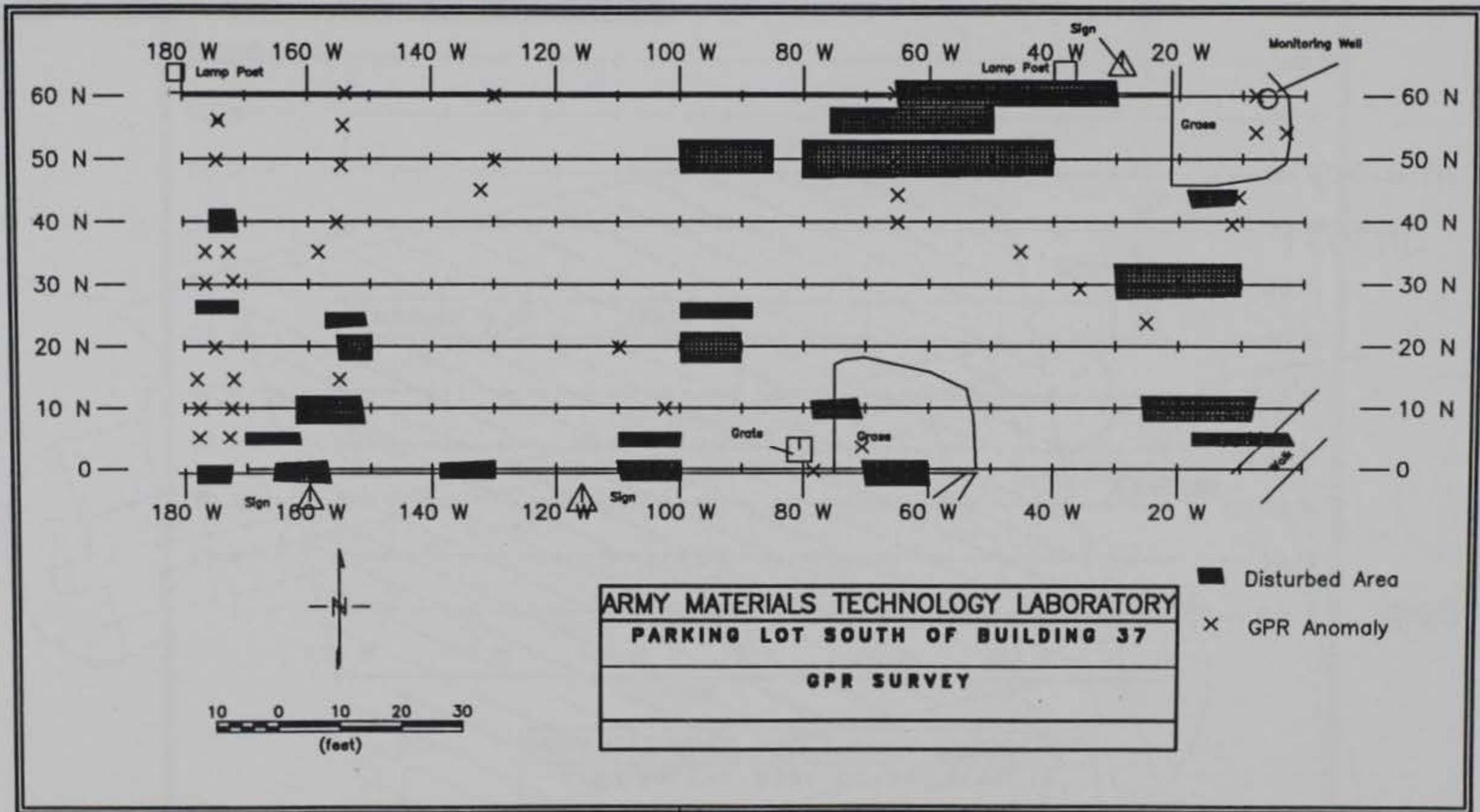
Figure 25. Results of GPR survey, Site 3
