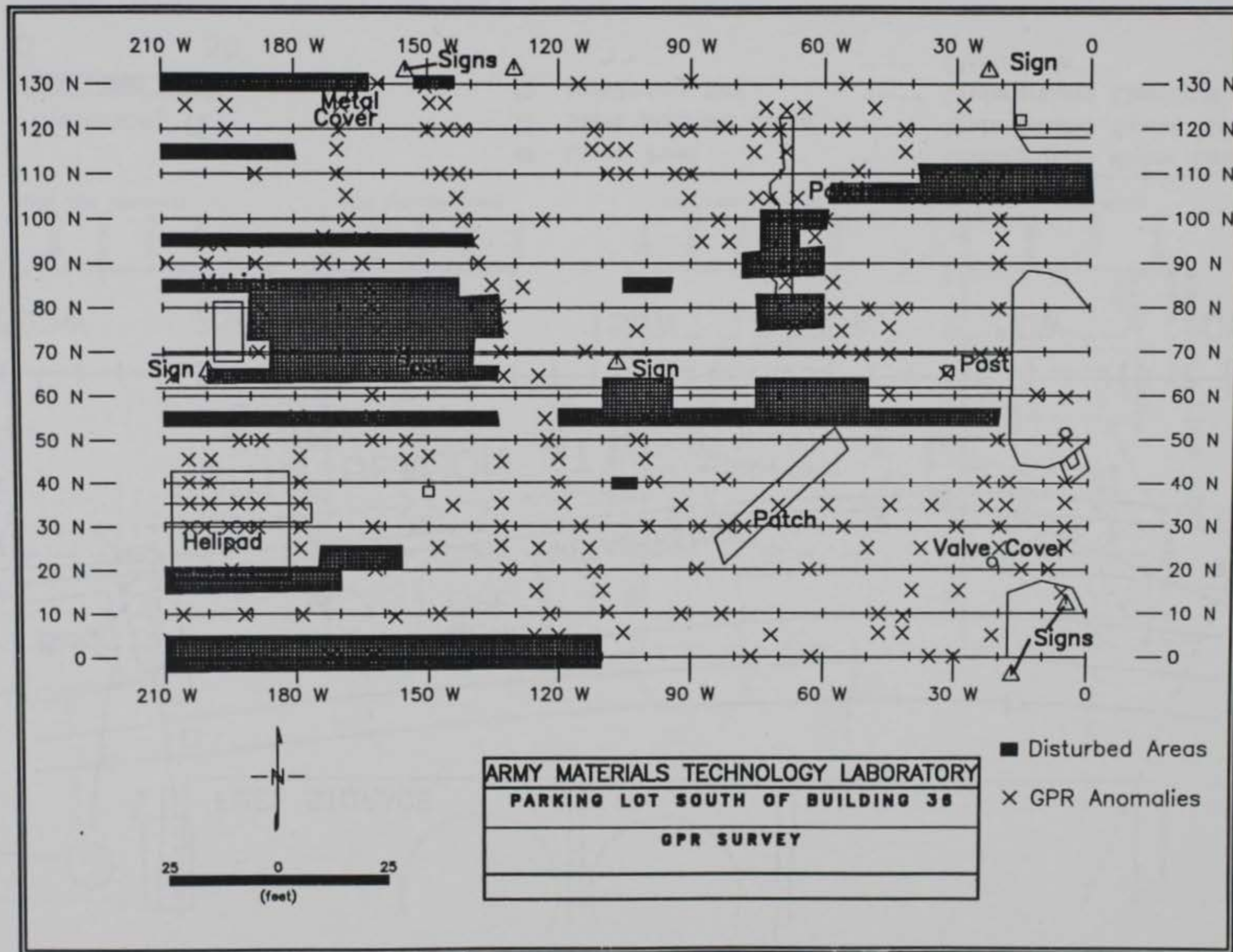
Figure 13. Results of GPR survey, Site 1
