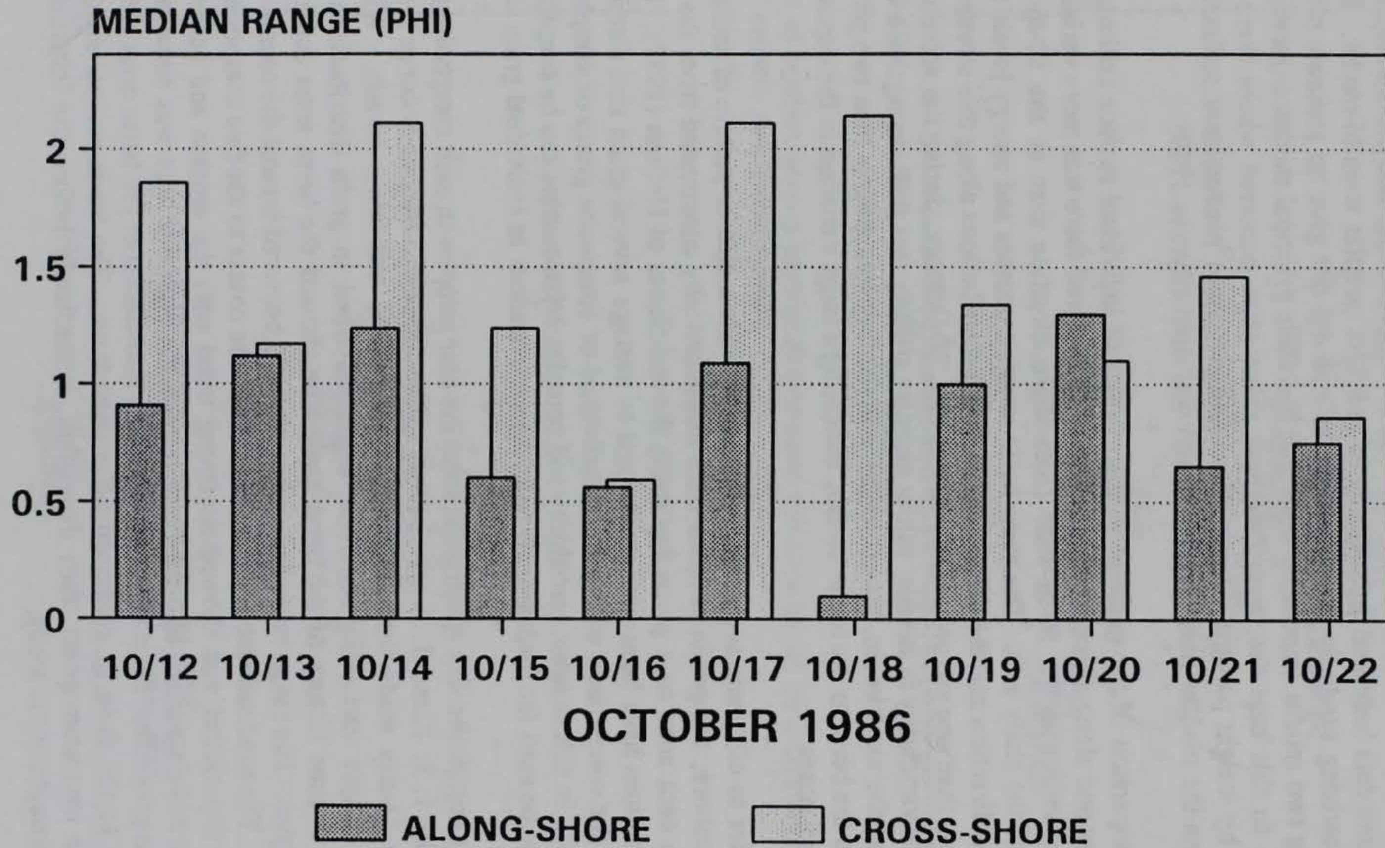
Figure 15. Cross-shore versus alongshore variability in median range of foreshore sediment samples
