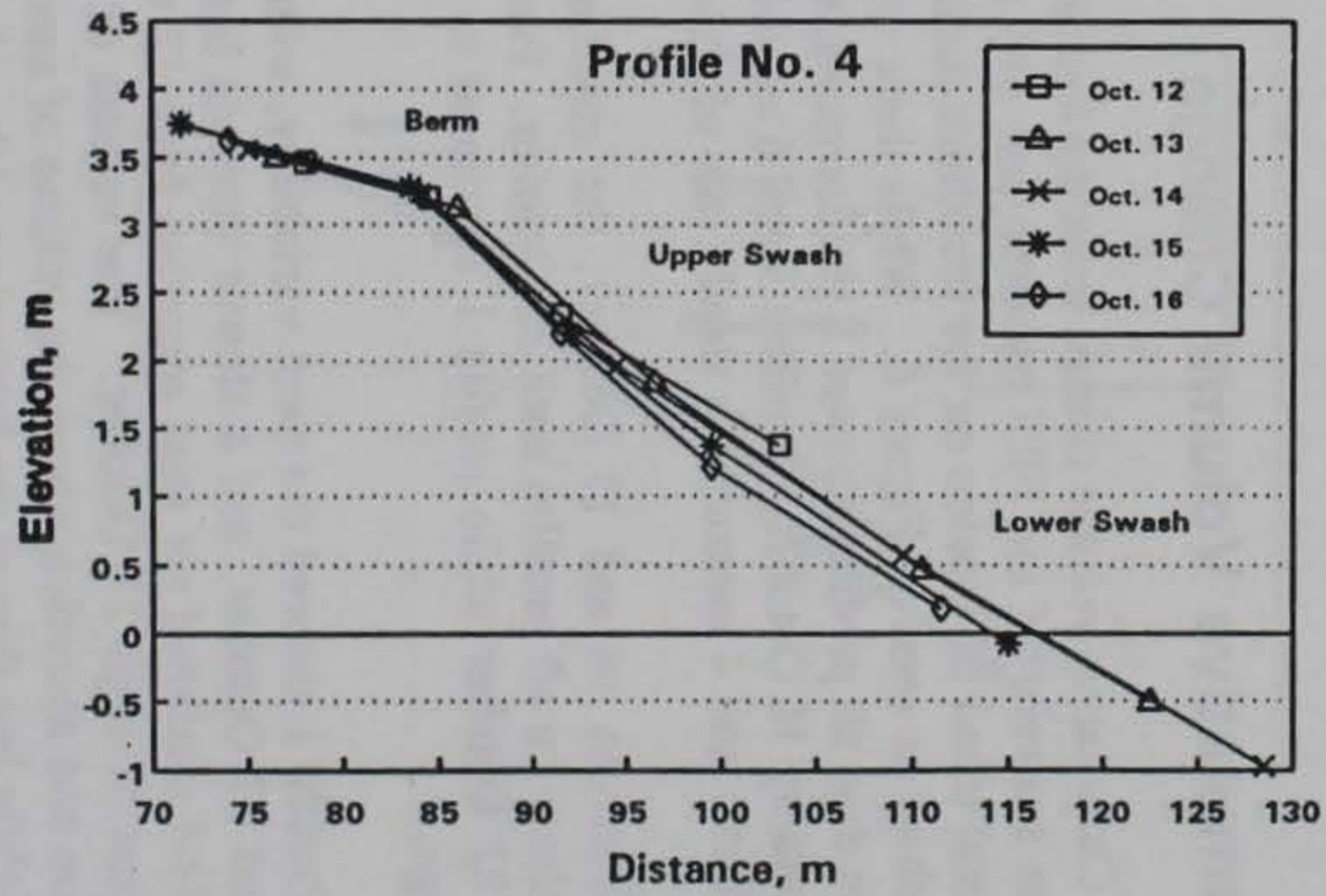
Figure 4. Foreshore cross-shore profile variation during the erosional sequence
