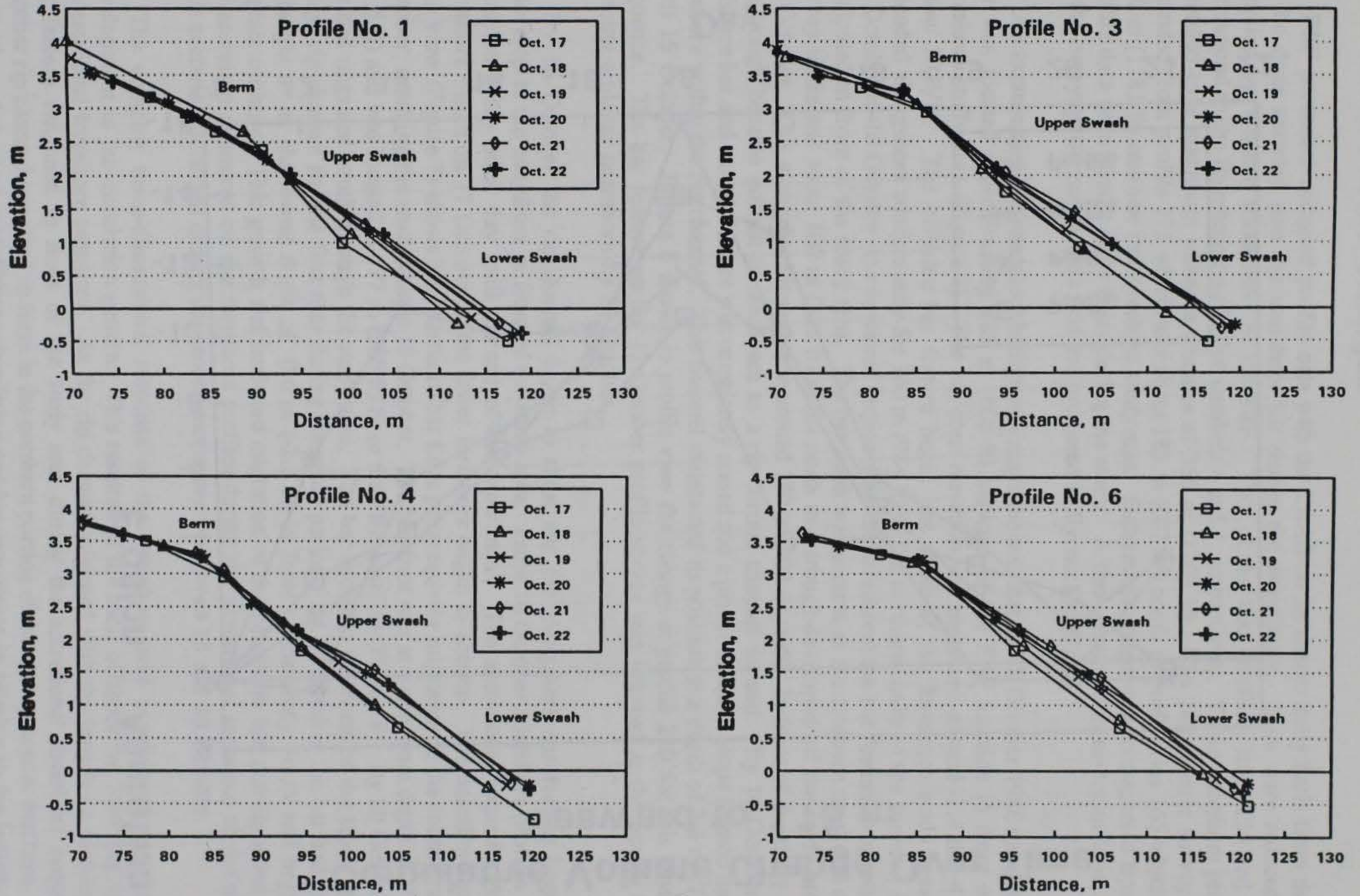
Figure 5. Foreshore cross-shore profile variation during the accretional sequence
