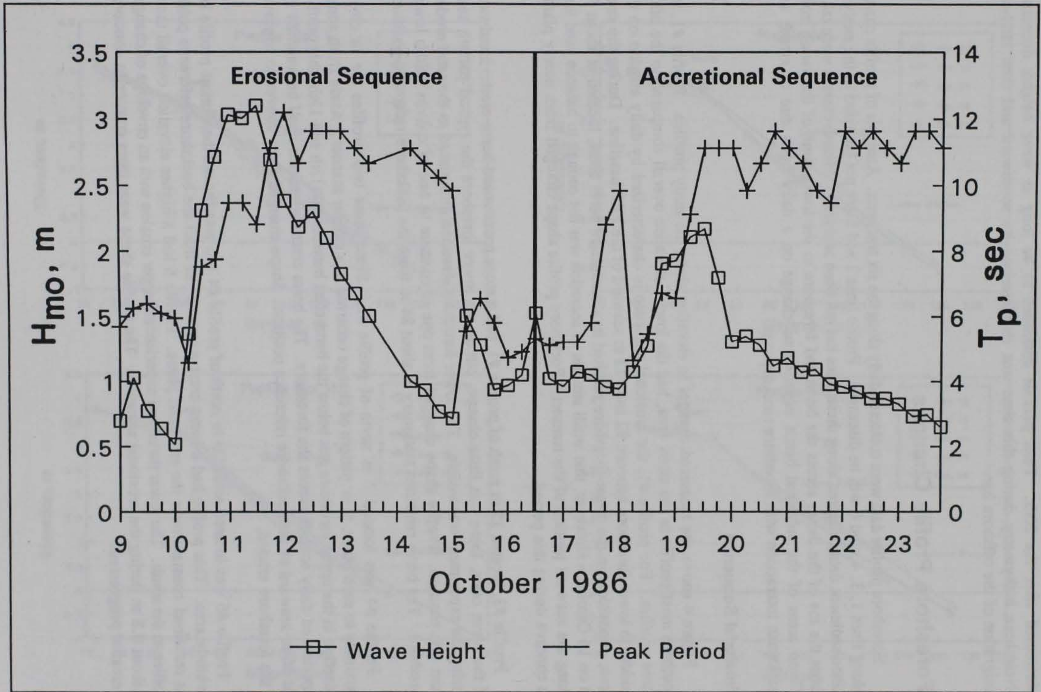
Figure 3. Plot of root mean wave height and peak period measured at 0.8 km seaward of foreshore study area in 8-m water depth at gage 191 (after Byrnes 1989)
