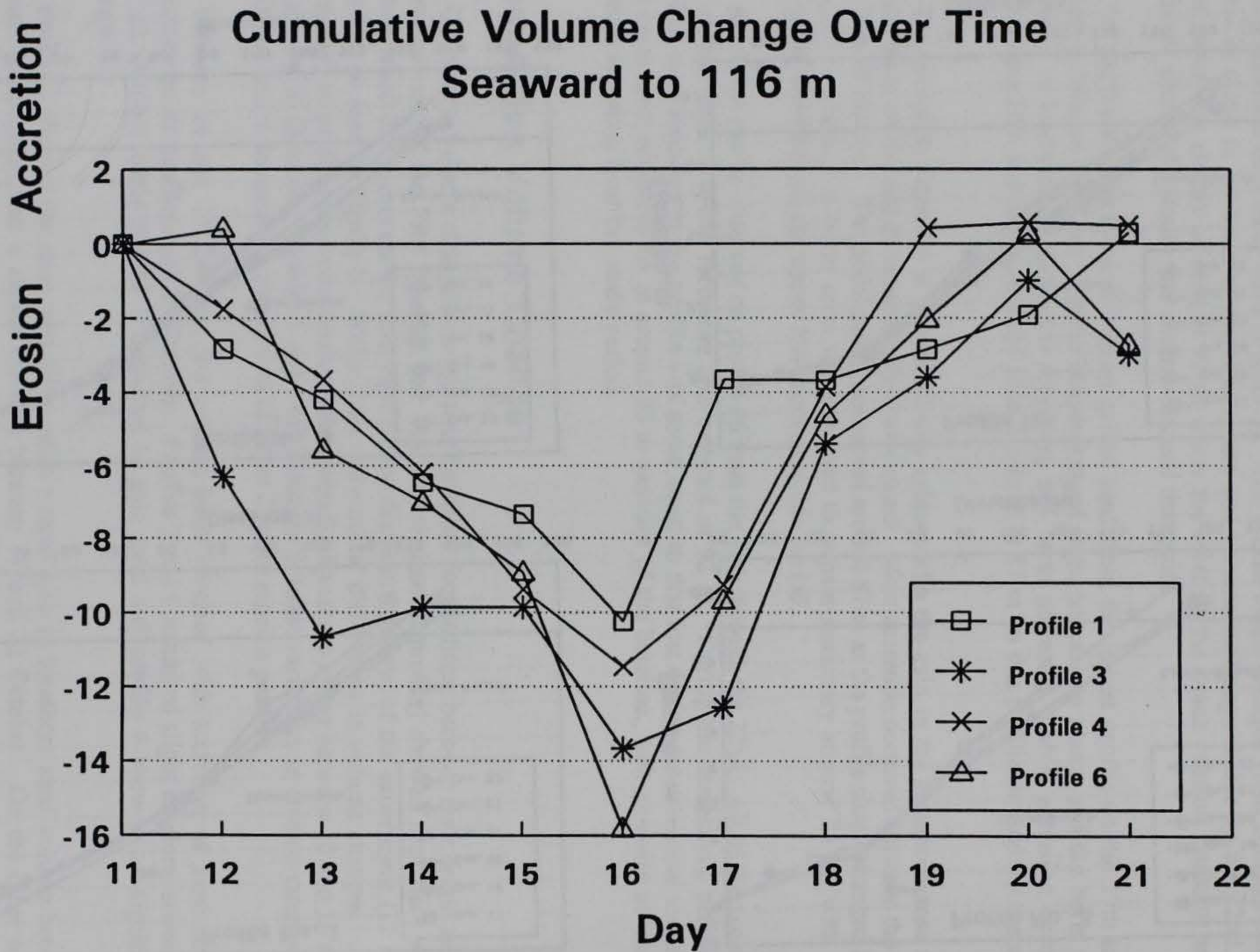
Figure 6. Cumulative volume change on the four foreshore profiles during the 11-day experimental period
