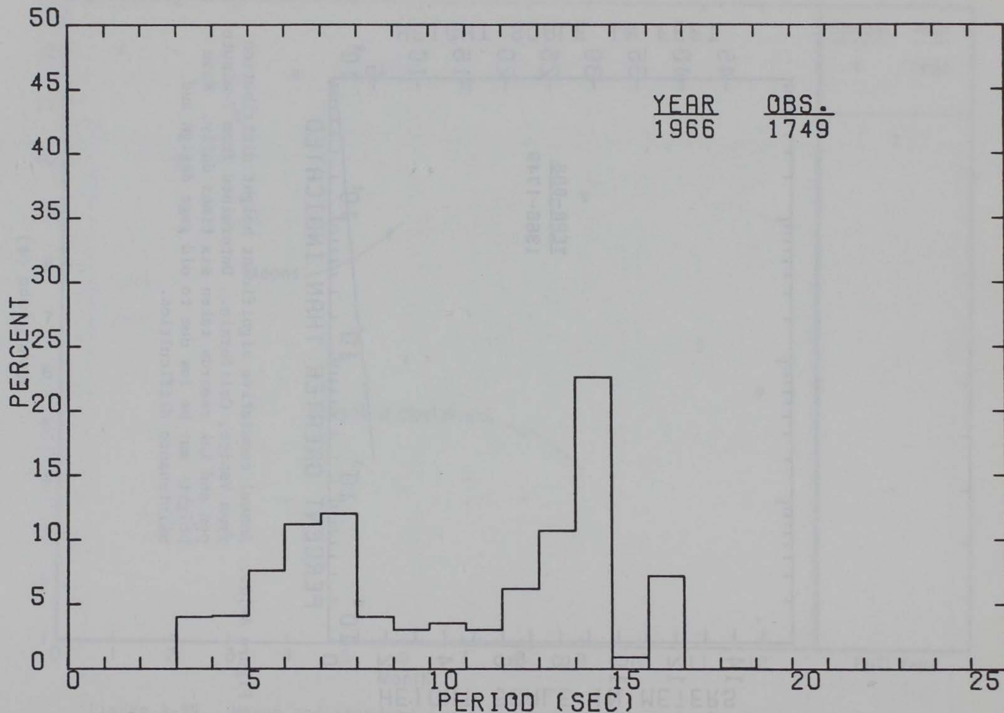
Figure A-101. Annual significant period distributions from Venice, California; determined from 7-minute pen and ink records taken six times daily.
