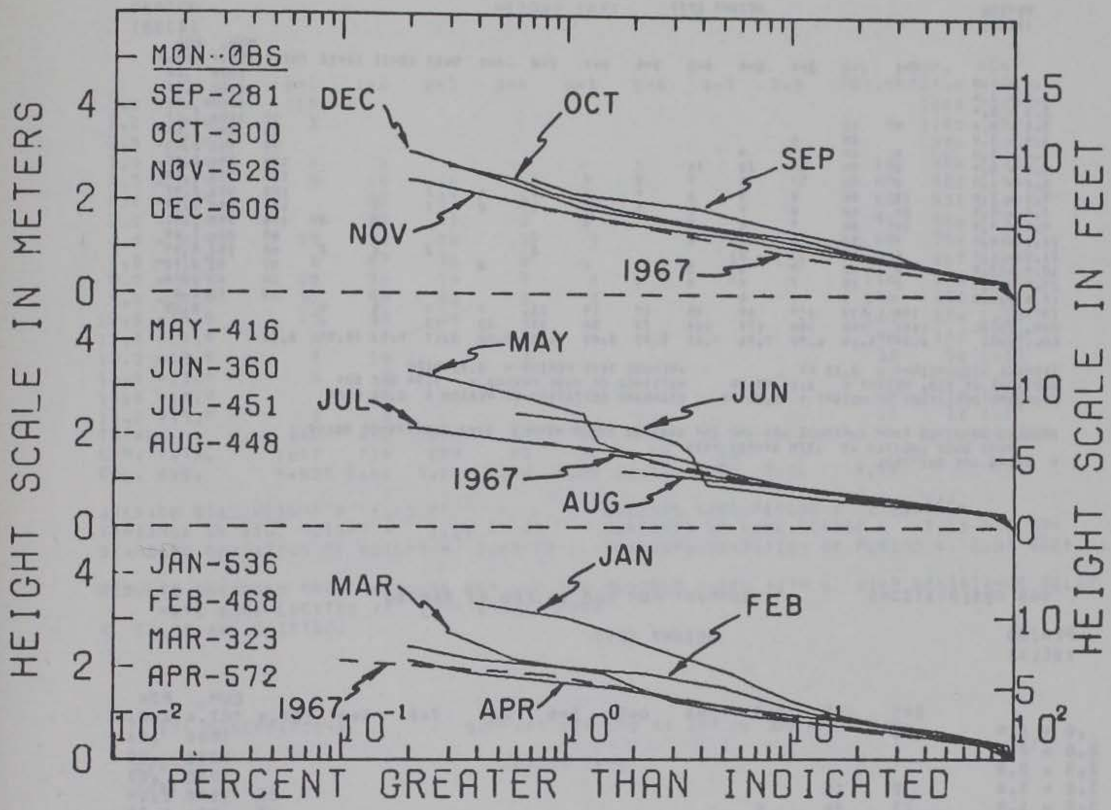
Figure A-27. Seasonal summaries of cumulative significant height distributions from Virginia Beach, Virginia; determined from 7-minute pen and ink records taken six times daily.
