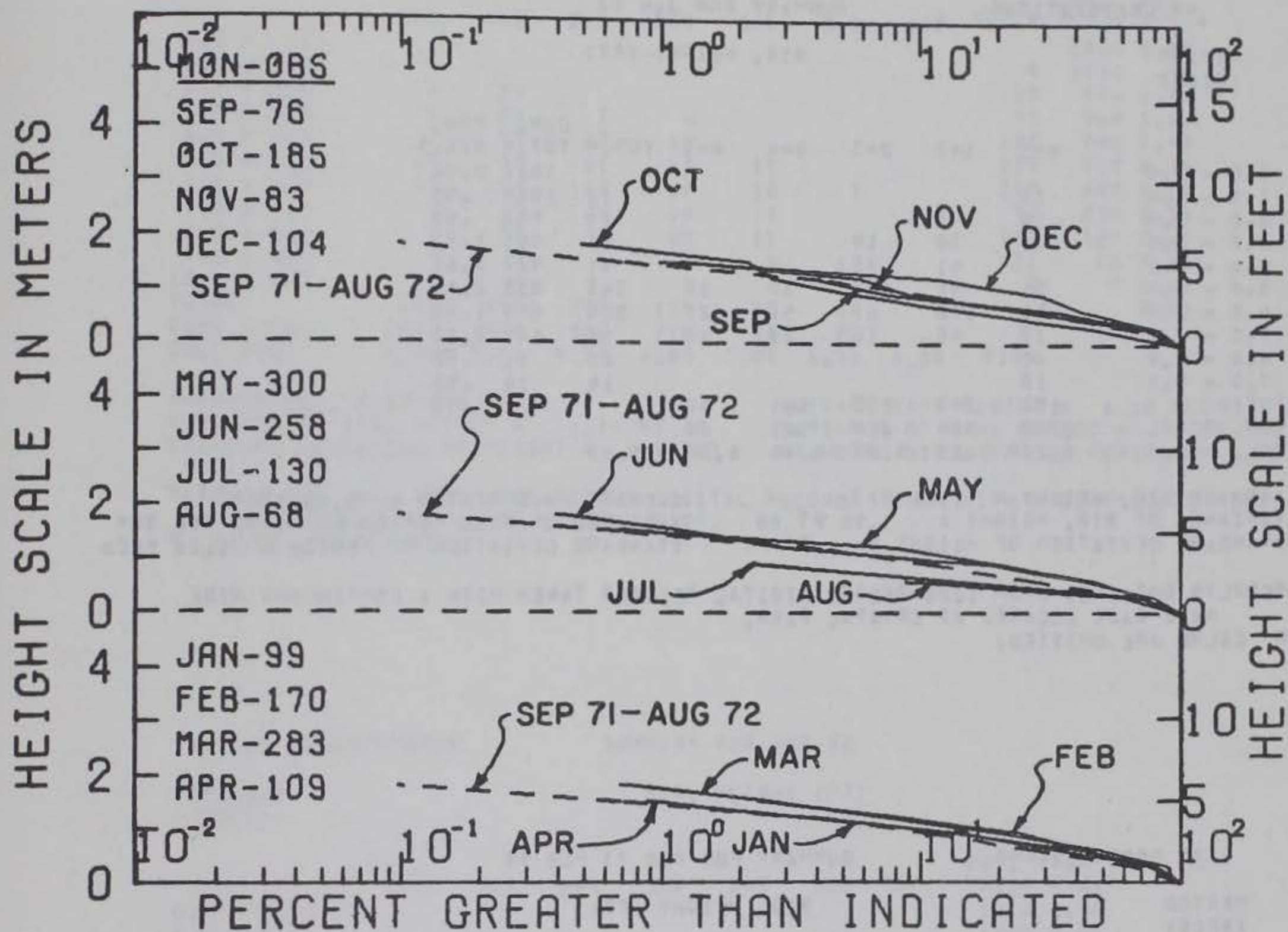
Figure A-73. Seasonal summaries of cumulative significant height distributions from Destin, Florida; computed from 1,024-second digital wave records taken four times daily.
