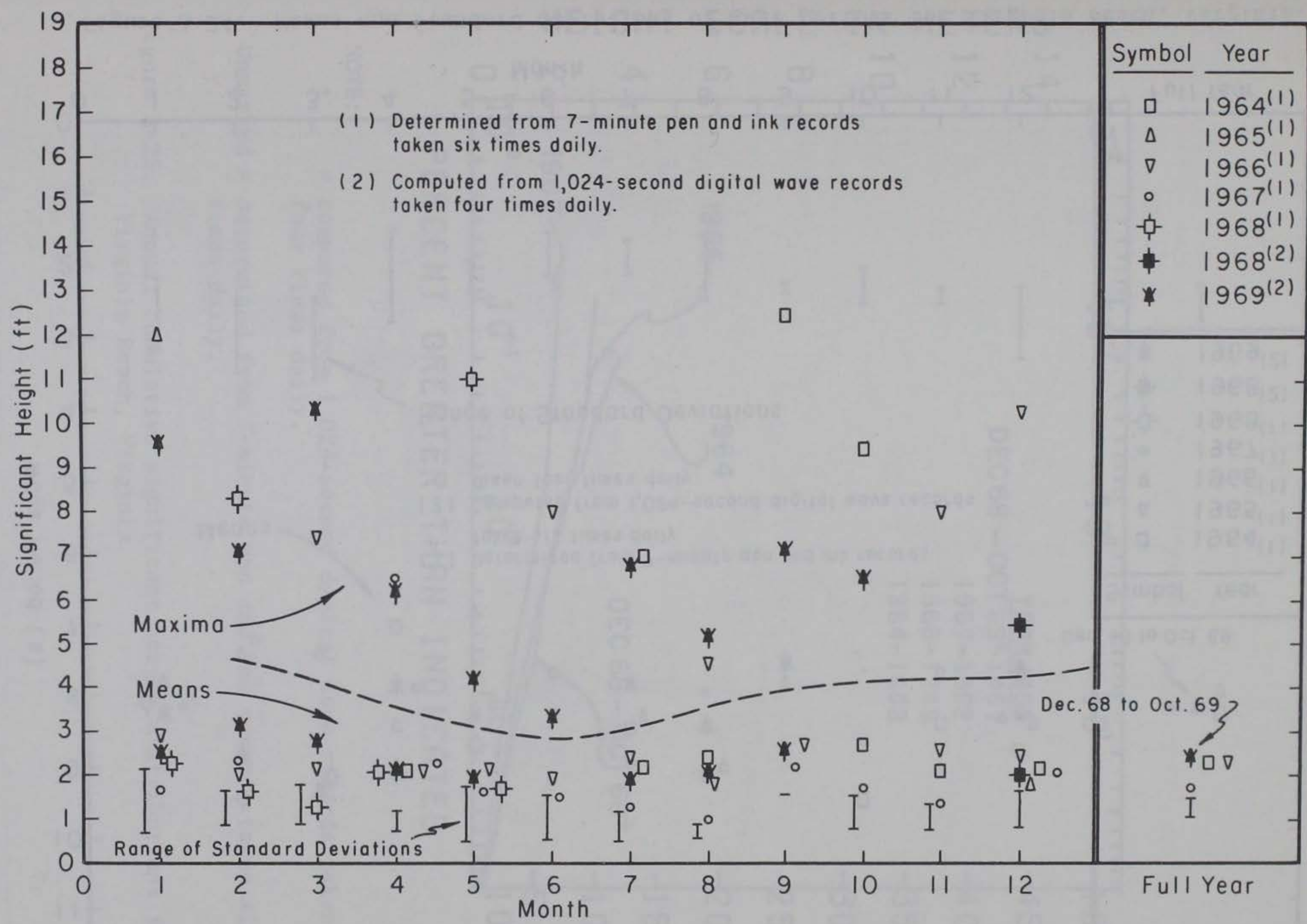
Figure A-23. Maxima, means, and standard deviations of significant height from Virginia Beach, Virginia.
