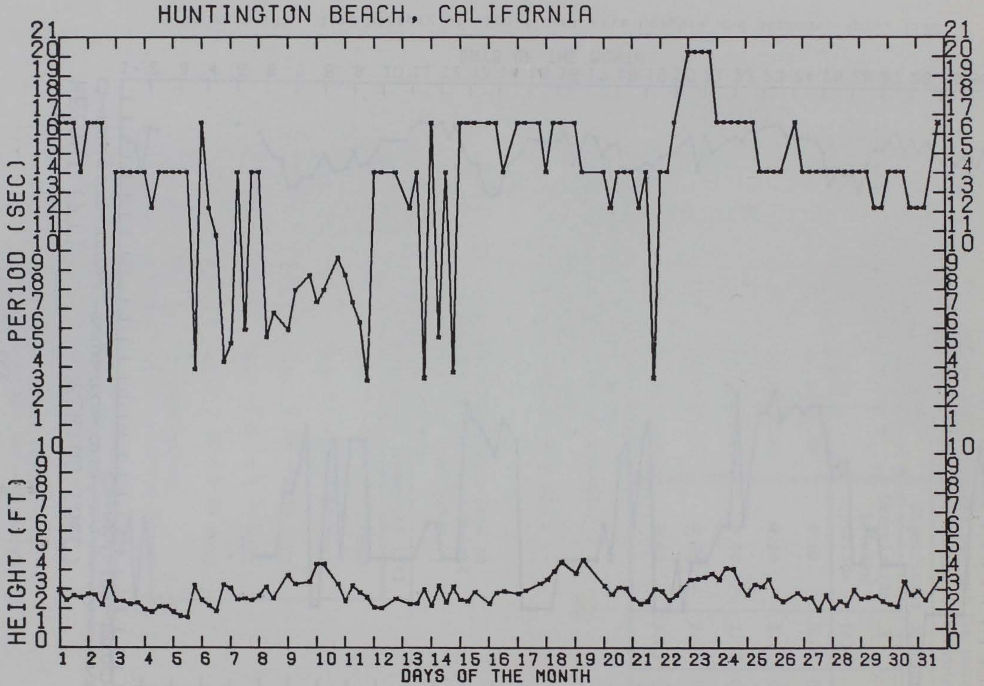
Figure A-109. Time history of significant wave heights and periods, May 1972.
