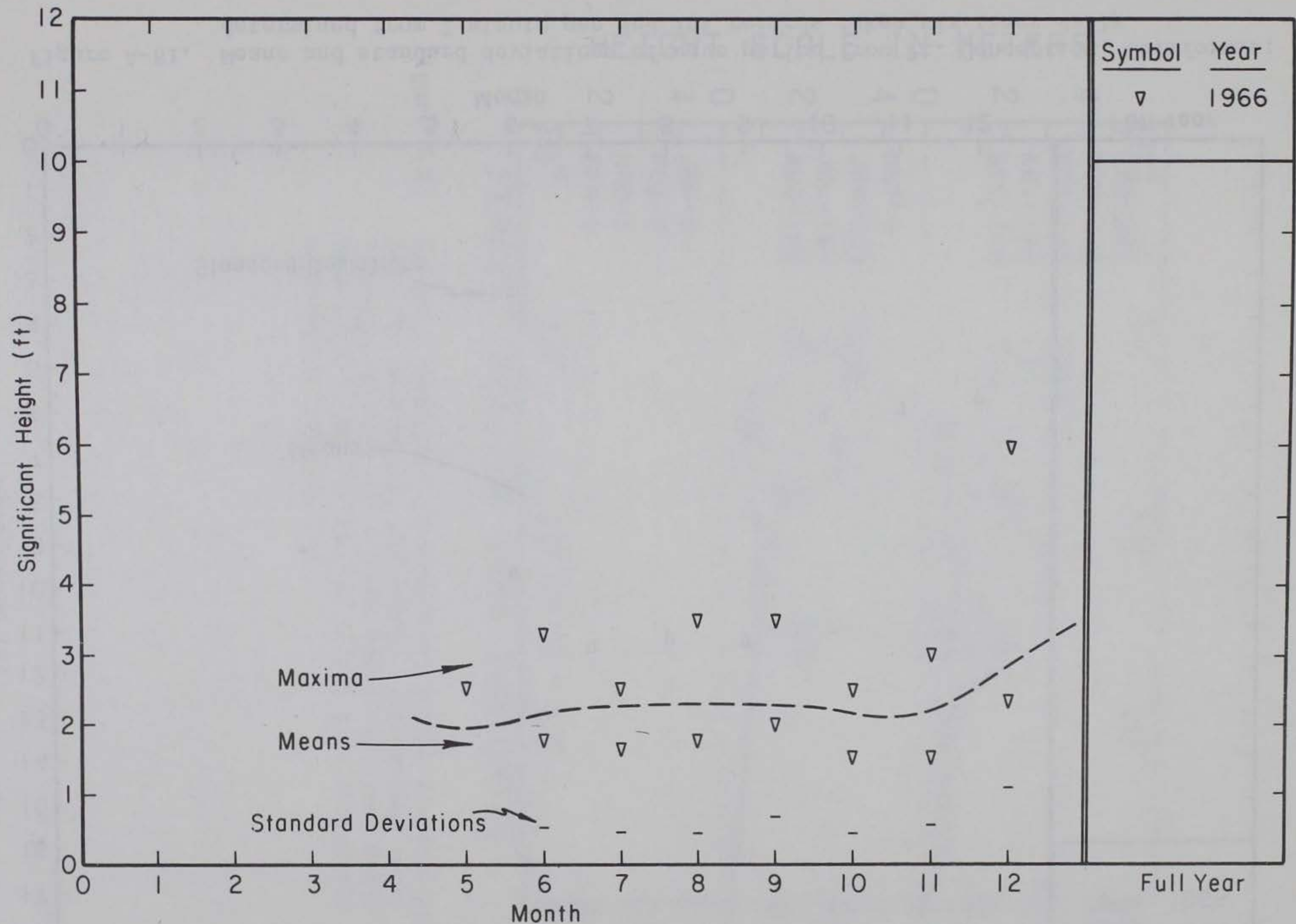
Figure A-80. Maxima, means, and standard deviation of significant height from Pt. Conception, California. Determined from 7-minute pen and ink records taken six times daily. Wave heights may be low due to old gage design and maintenance difficulties.
