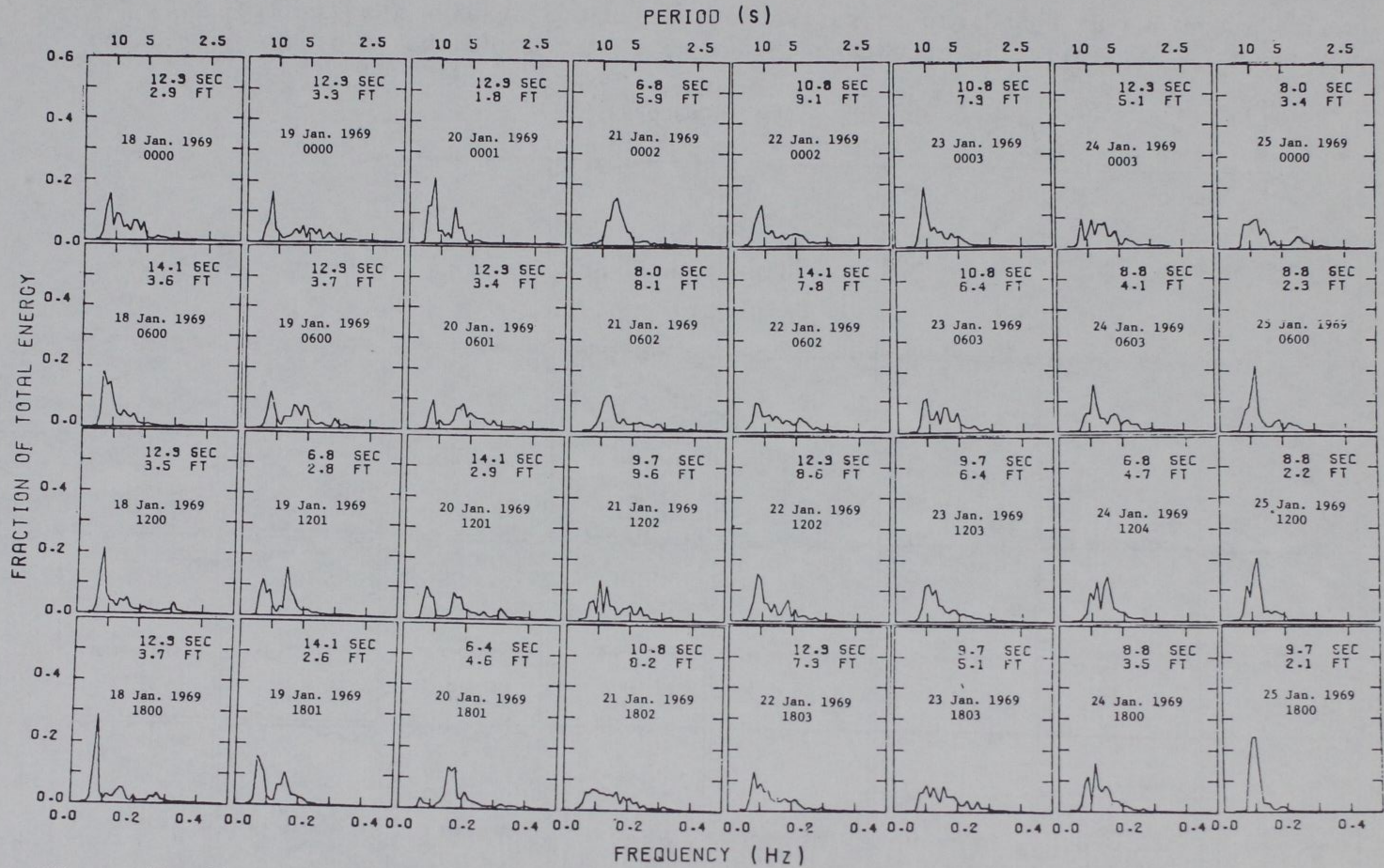
Figure 3. Example of energy spectra from the CERC gage at Atlantic City, New Jersey. --Continued
