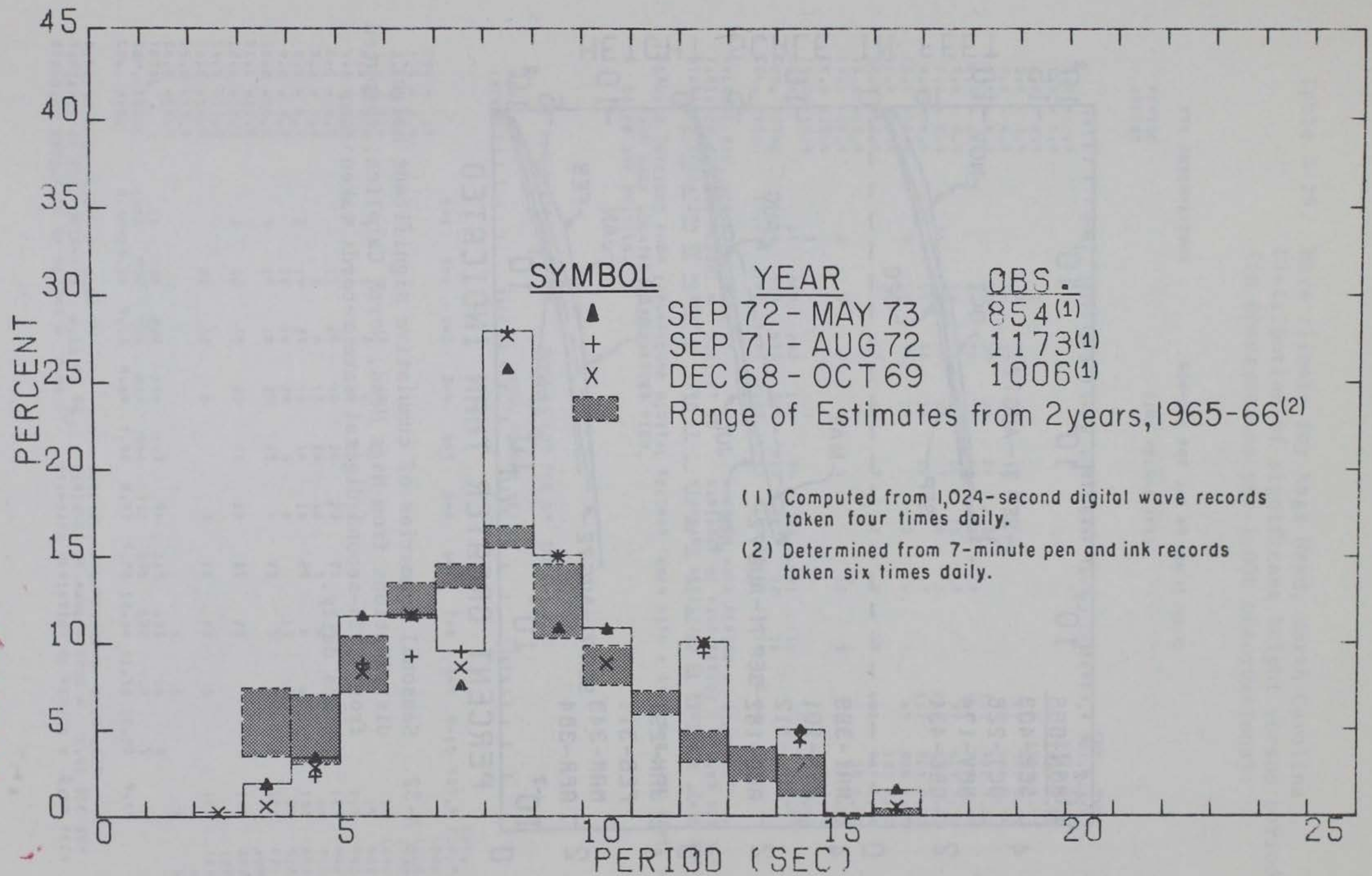
Figure A-31. Annual significant period distributions from Nags Head, North Carolina.
