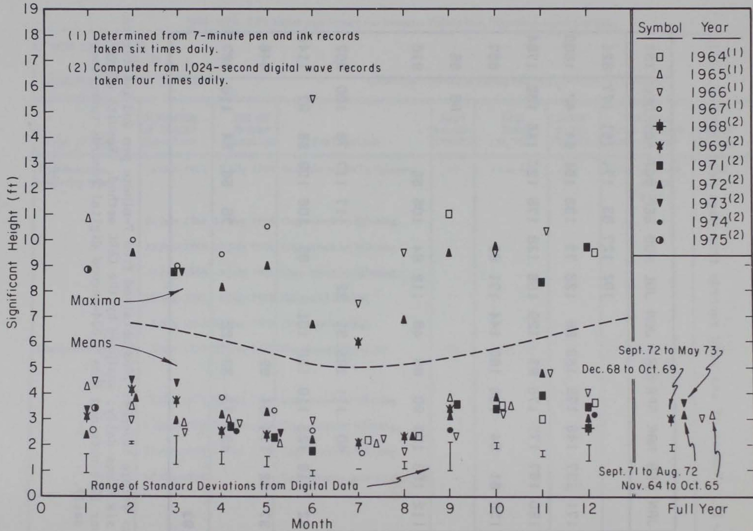
Figure A-28. Maxima, means, and standard deviations of significant height from Nags Head, North Carolina.
