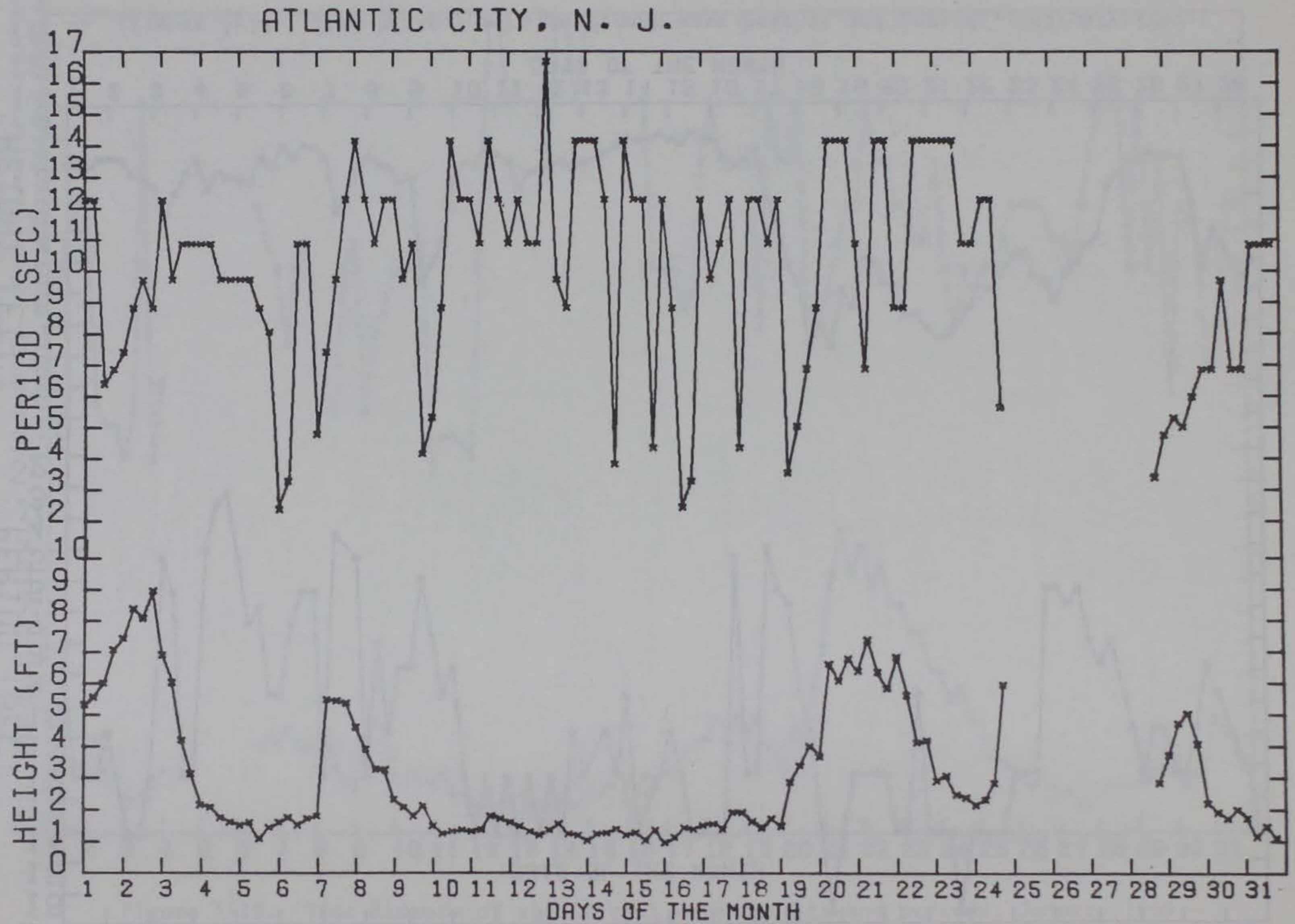
Figure A-15. Time history of significant wave heights and periods, March 1969.
