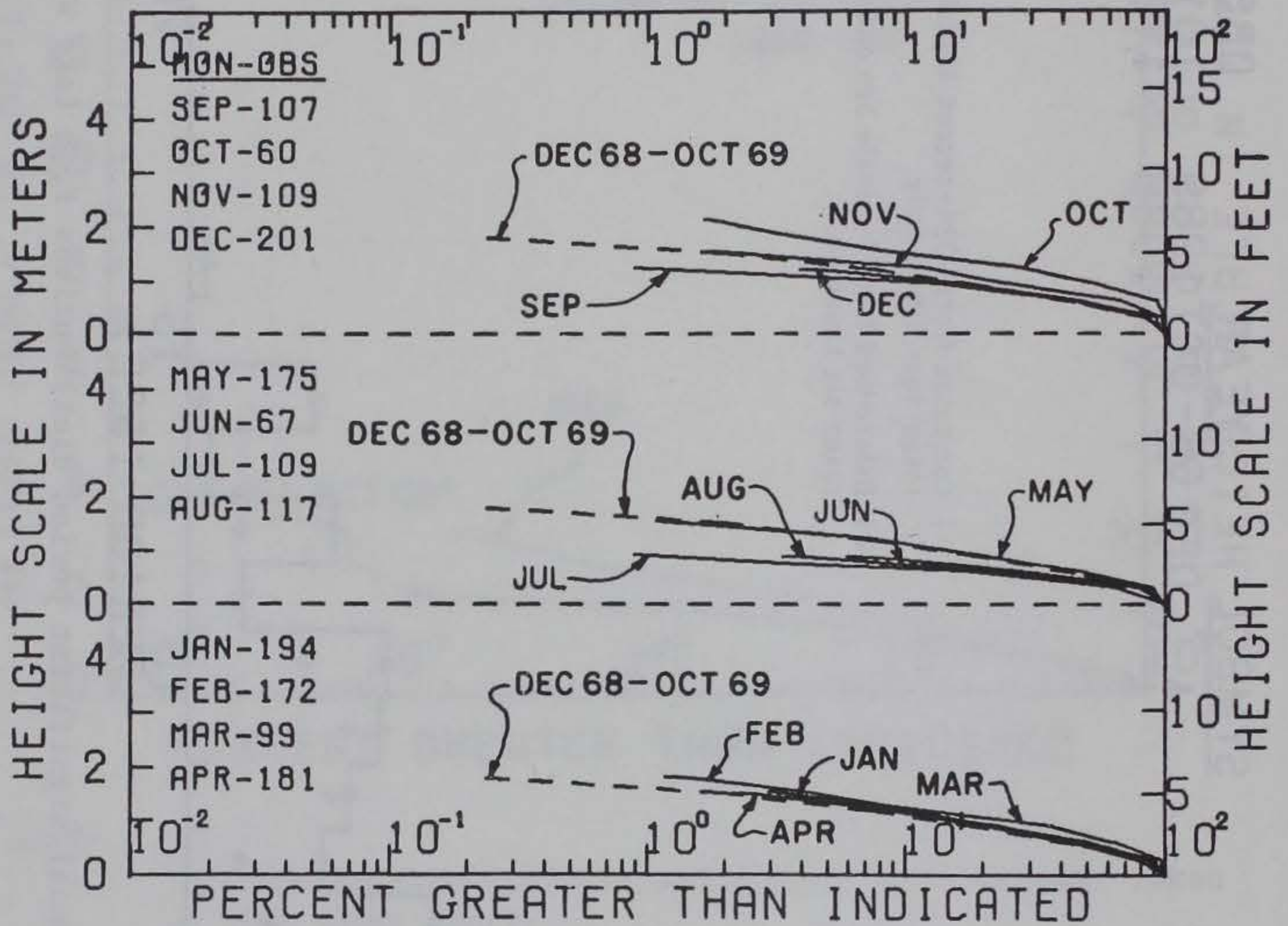
Figure A-62. Seasonal summaries of cumulative significant height distributions from Lake Worth, Florida; computed from 1,024-second digital wave records taken four times daily.
