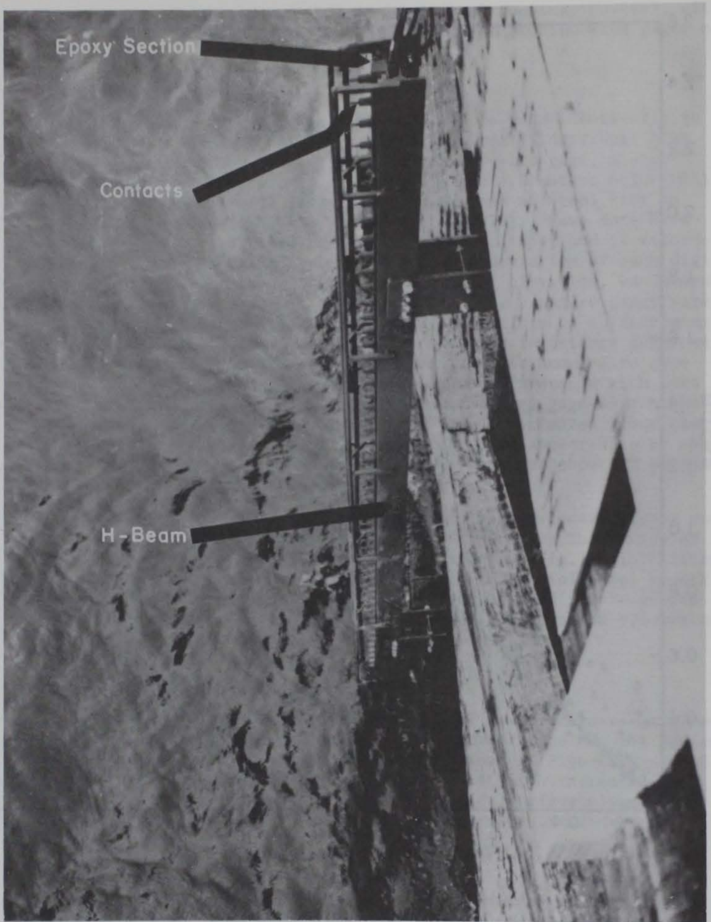
Figure 8. Oblique photo of step-resistance gage near Chesapeake Beach, Maryland.
