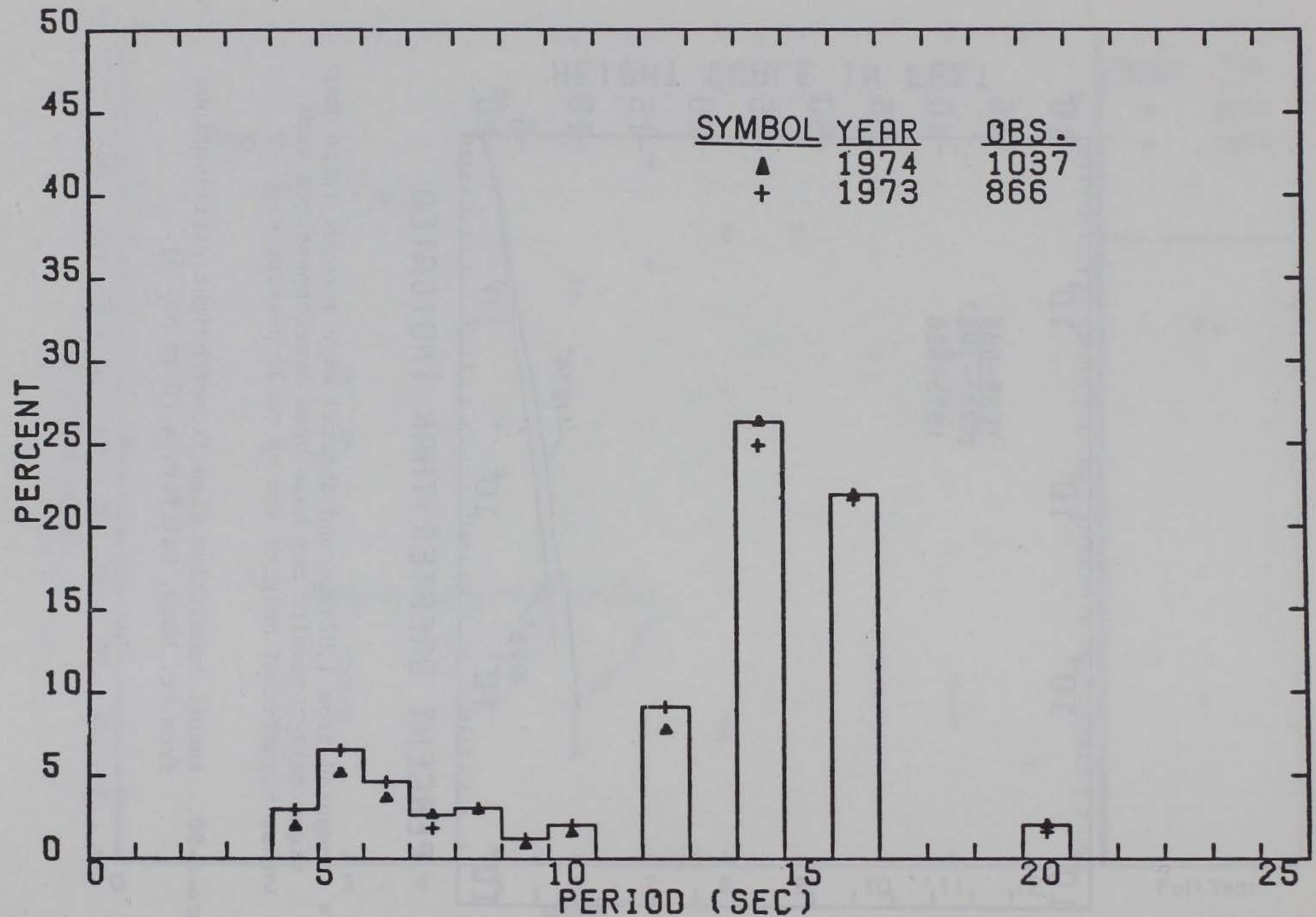
Figure A-91. Annual significant period distributions from Pt. Mugu, California (Gage No. 3). Computed from 1,024-second digital wave records taken four times daily. Results may have been overcompensated such that wave periods tend to be too short; periods less than 4 seconds have been omitted.
