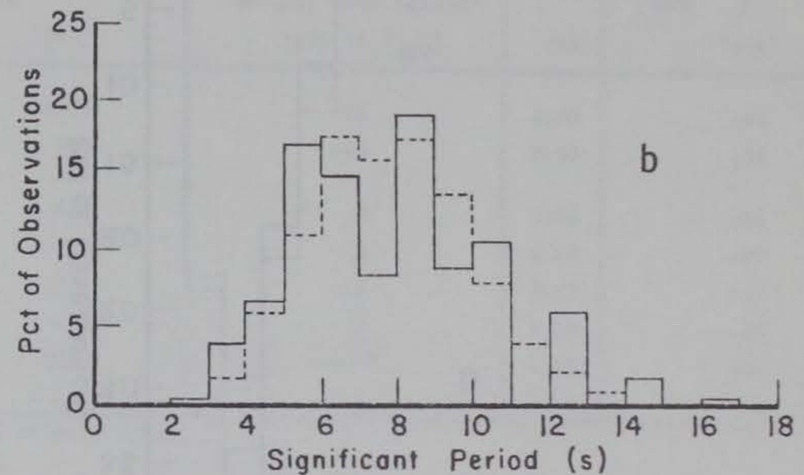
Figure 16. Comparison of distribution functions of wave period estimated from digital (solid line) and pen and ink records (dashline) taken during September 1971 to April 1972. (a) Savannah Light Tower, Georgia (499 observations); (b) Wrightsville Beach, North Carolina (755 observations).
