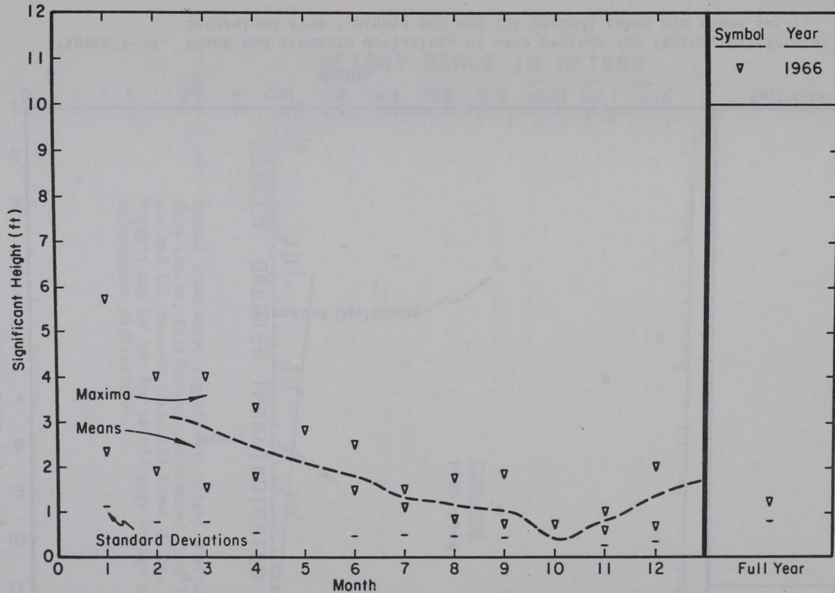
Figure A-98. Maxima, means, and standard deviations of significant height from Venice, California. Determined from 7-minute pen and ink records taken six times daily. Wave heights may be low due to old gage design and maintenance difficulties.
