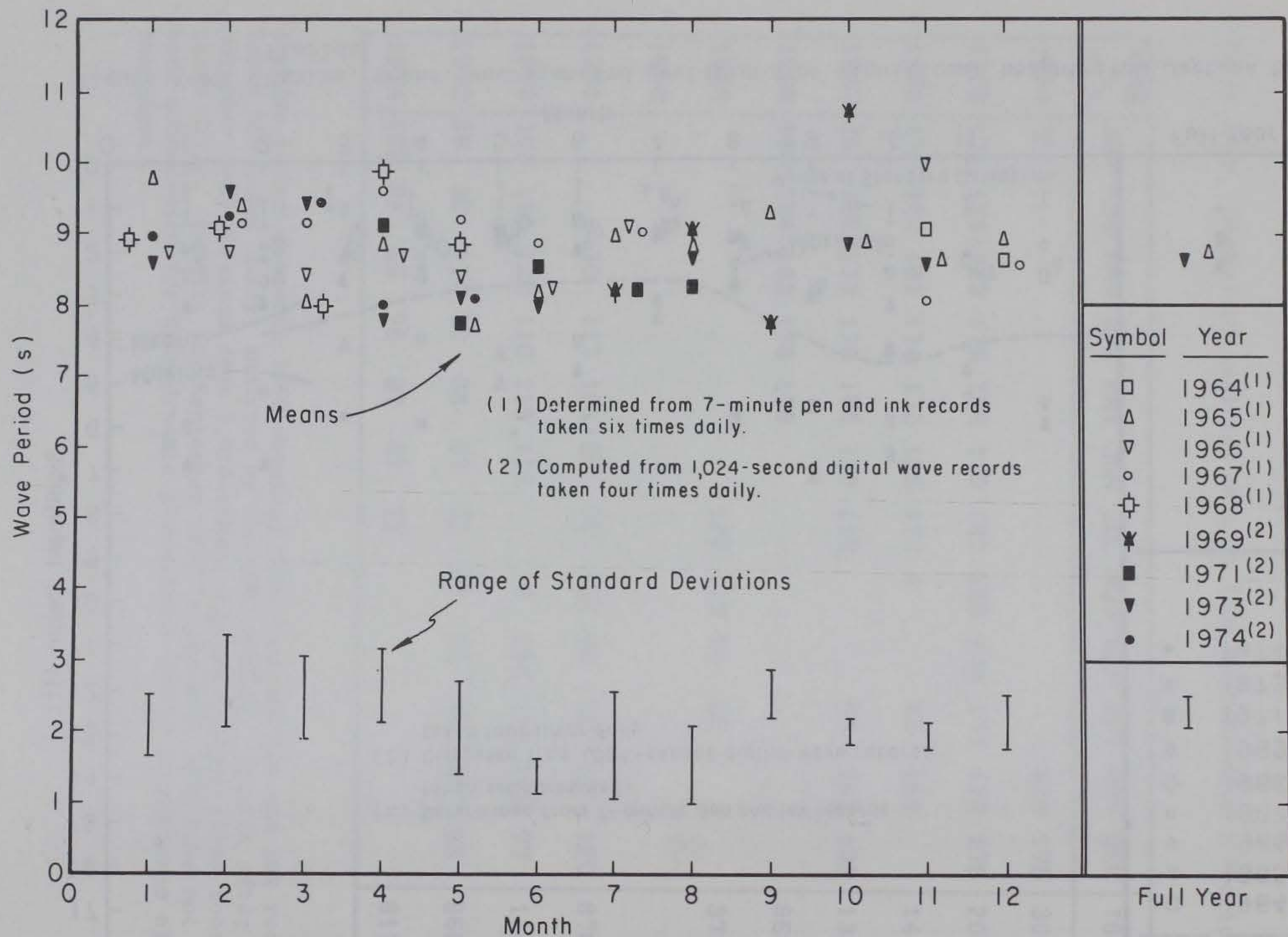
Figure A-49. Means and standard deviations of wave periods for Daytona Beach, Florida.
