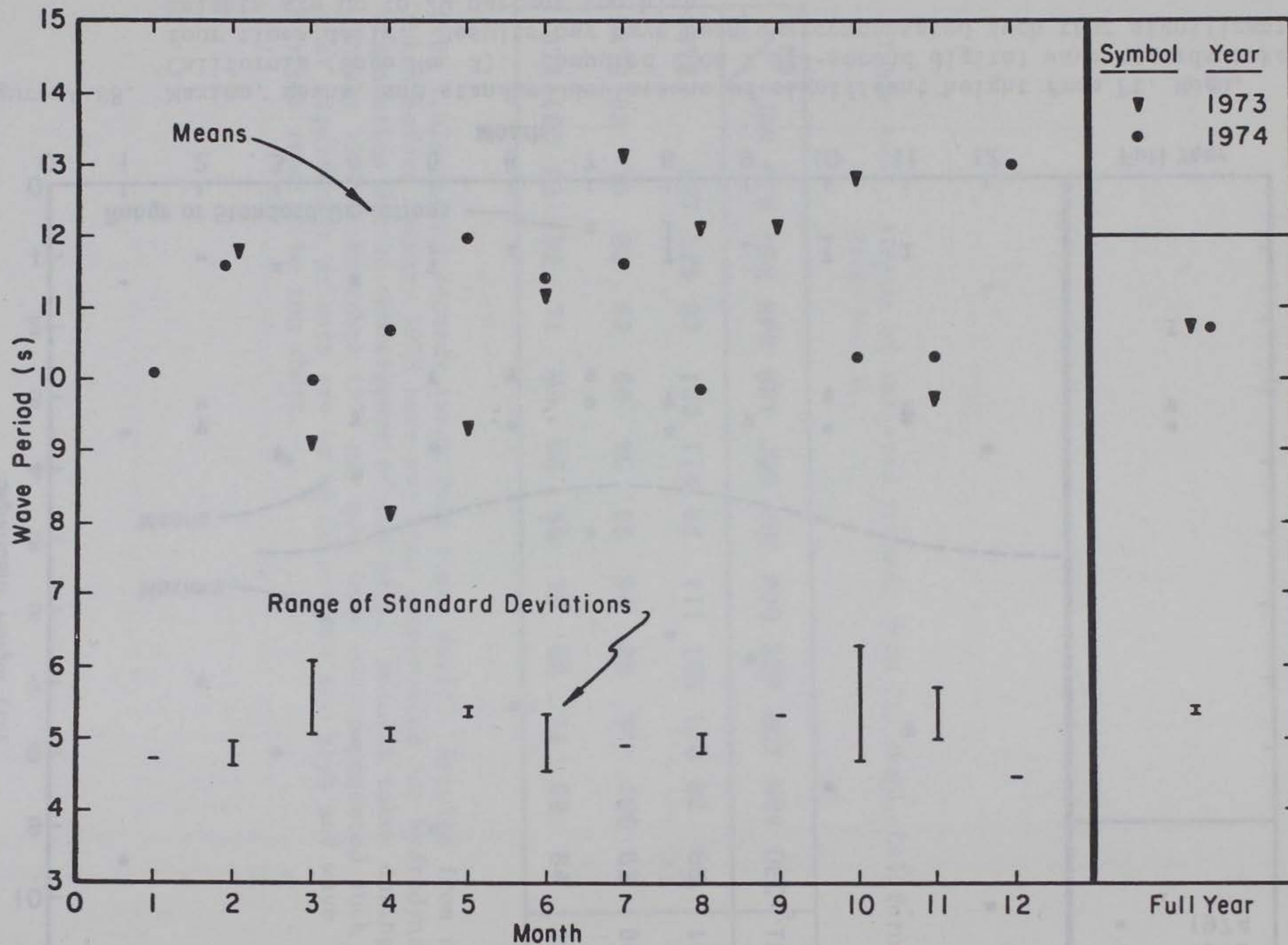
Figure A-89. Means and standard deviations of wave periods for Pt. Mugu, California (Gage No. 3). Computed from 1,024-second digital wave records taken four times daily. Results may have been overcompensated such that wave periods tend to be too short.
