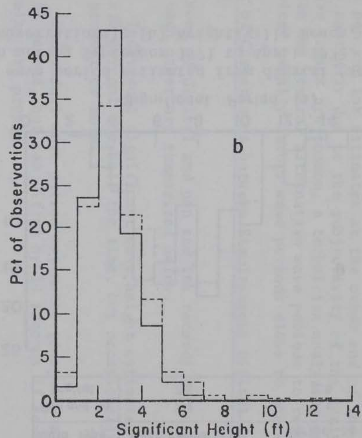
Figure 15. Comparison of distribution functions of significant wave height estimated from digital (solid line) and pen and ink records (dashline) taken during September 1971 to April 1972. (a) Savannah Light Tower, Georgia (499 observations); (b) Wrightsville Beach, North Carolina (764 observations).
