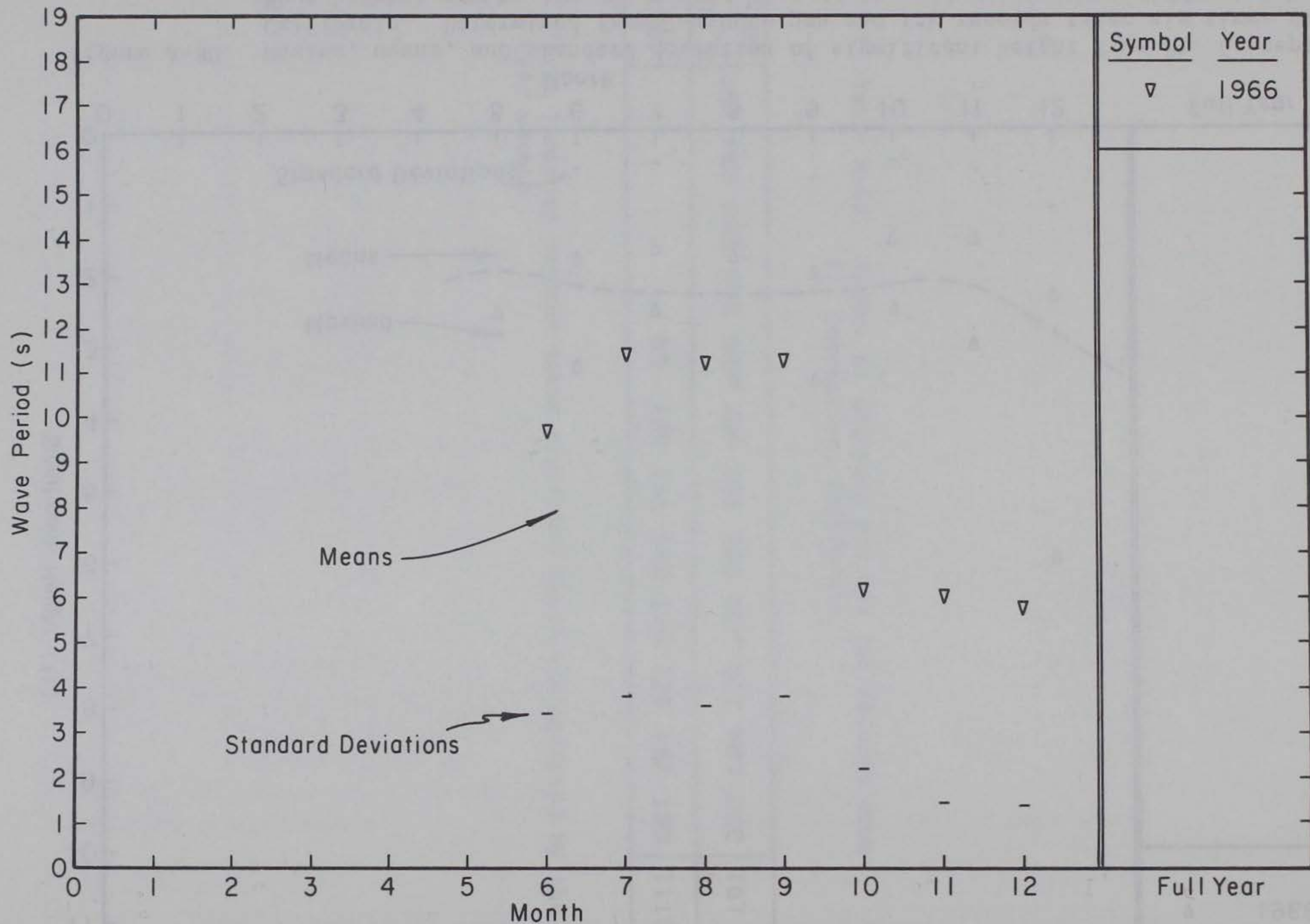
Figure A-81. Means and standard deviations of wave period from Pt. Conception, California; determined from 7-minute pen and ink records taken six times daily.
