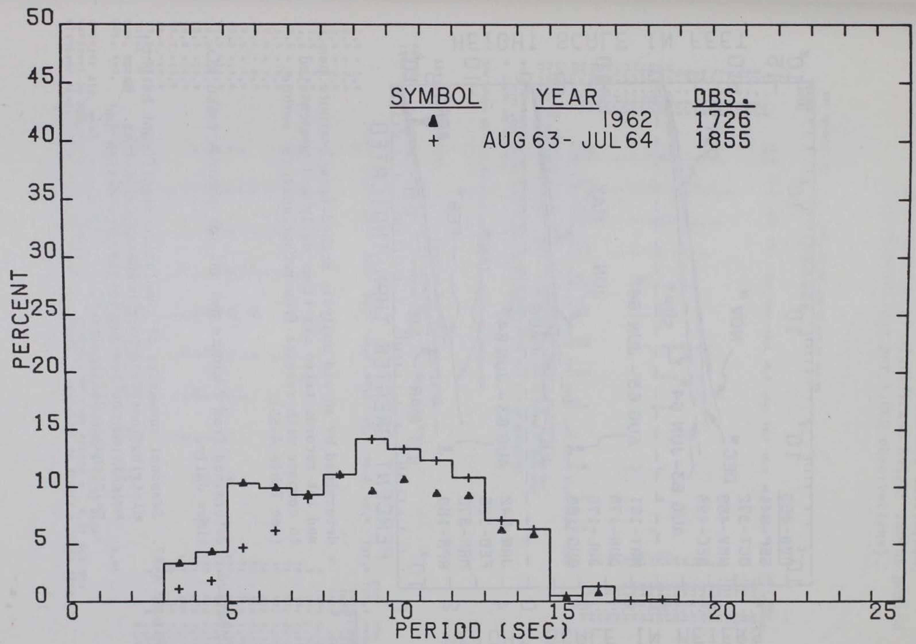
Figure A-86. Annual significant period distributions from Port Hueneme, California; determined by an old analysis method from 7-minute pen and ink records taken six times daily.
