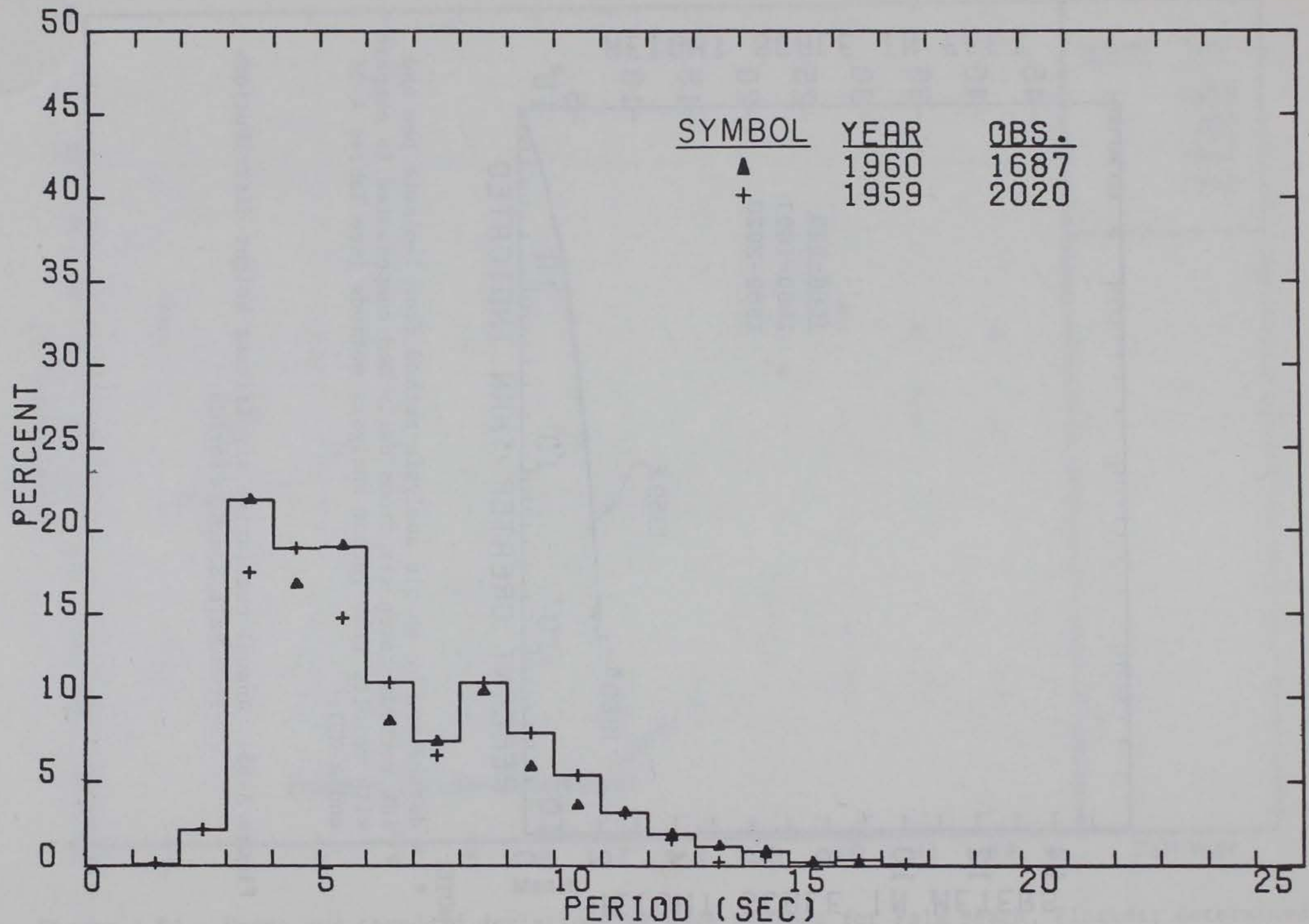
Figure A-56. Annual significant period distributions from Palm Beach, Florida; determined by an old analysis method from 7-minute pen and ink records taken six times daily.
