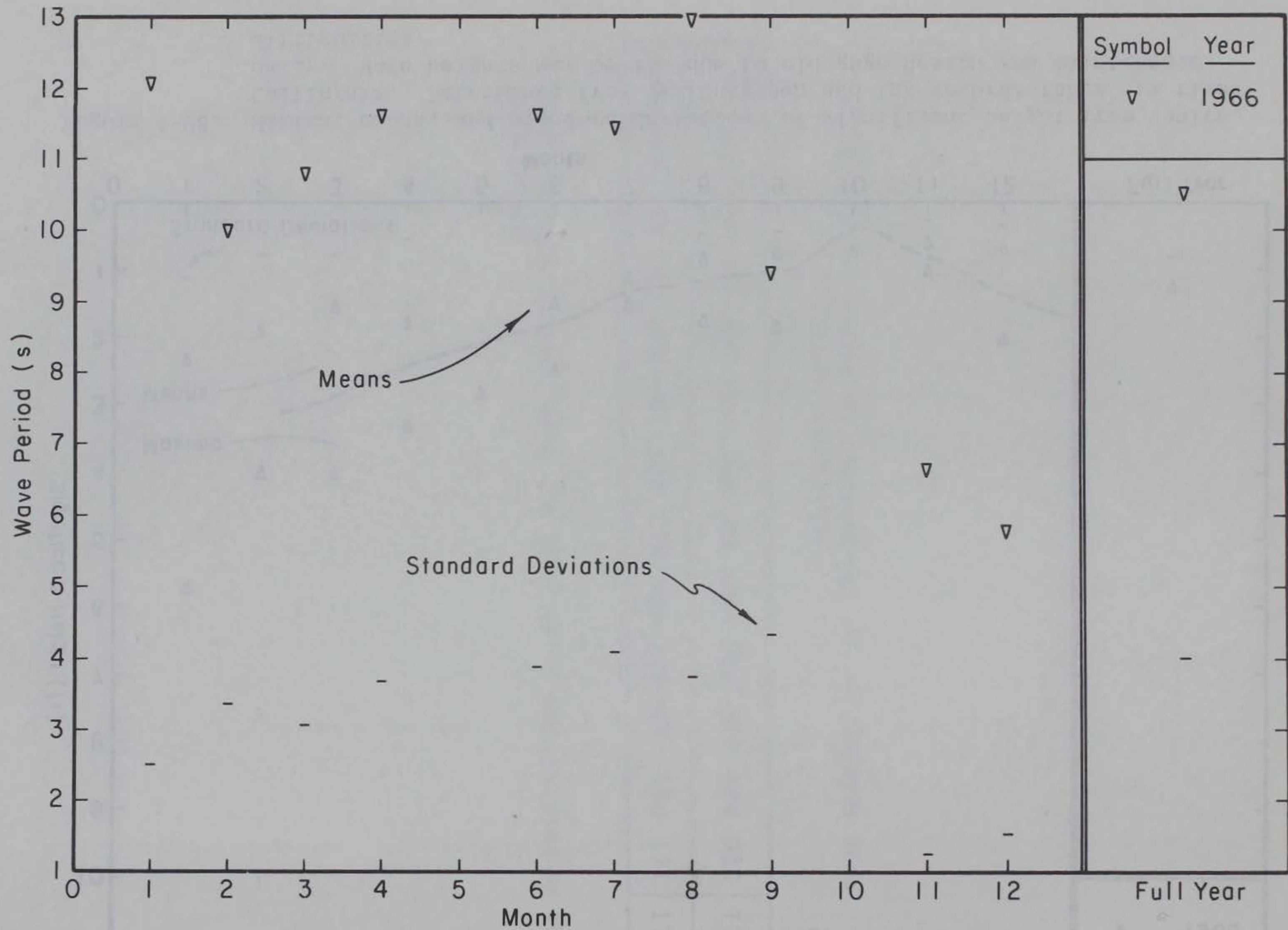
Figure A-99. Means and standard deviations of wave periods for Venice, California; determined from 7-minute pen and ink records taken six times daily.
