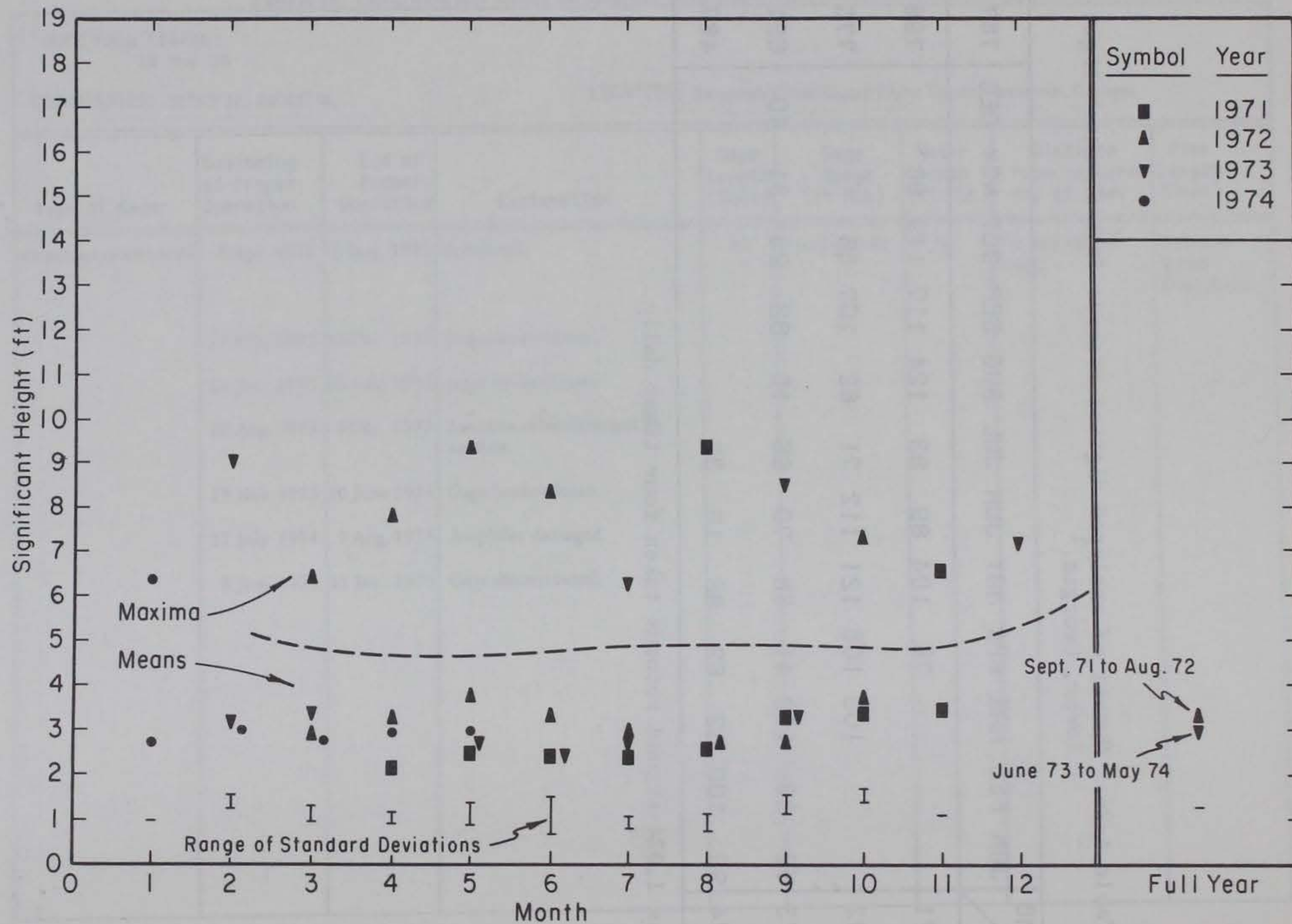
Figure A-43. Maxima, means, and standard deviations of significant height from Savannah Light Tower, Georgia; computed from 1,024-second digital wave records taken four times daily.
