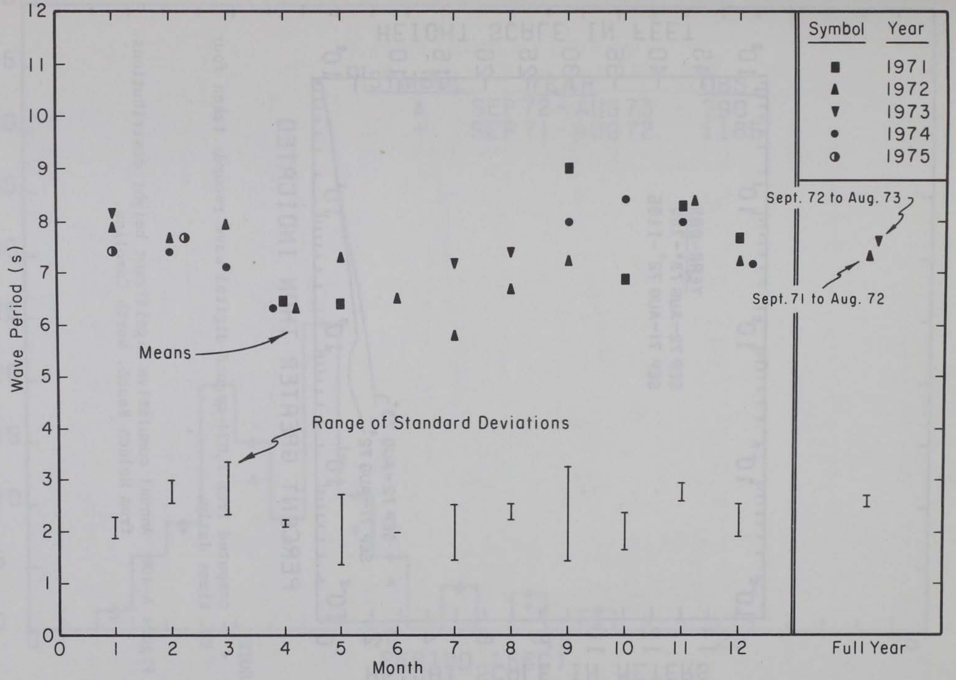
Figure A-39. Means and standard deviations of wave periods for Holden Beach, North Carolina; computed from 1,024-second digital wave records taken four times daily.
