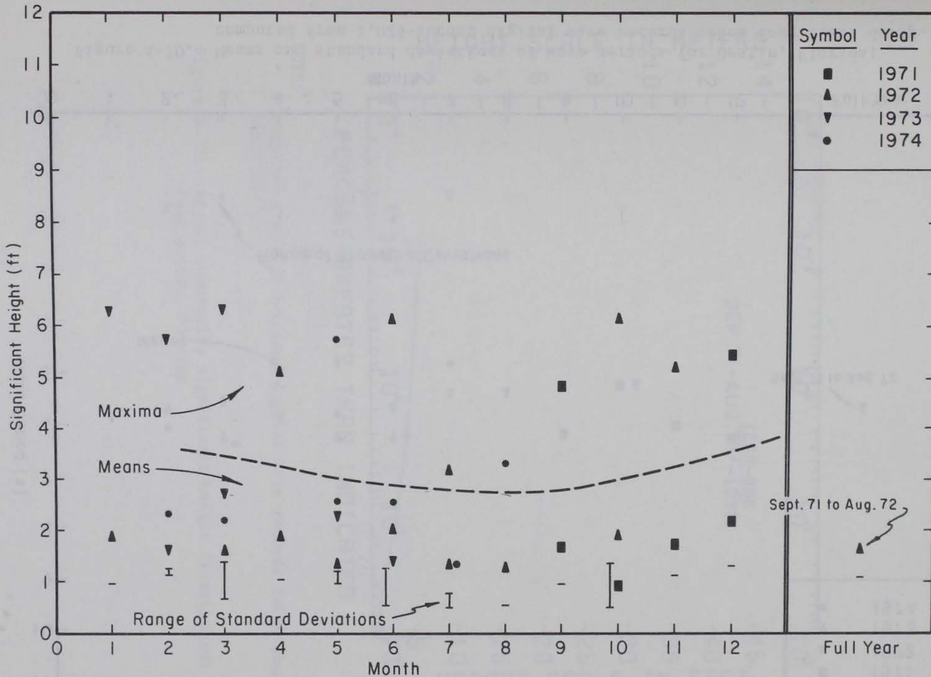
Figure A-69. Maxima, means, and standard deviations of significant height from Destin, Florida; computed from 1,024-second digital wave records taken four times daily.
