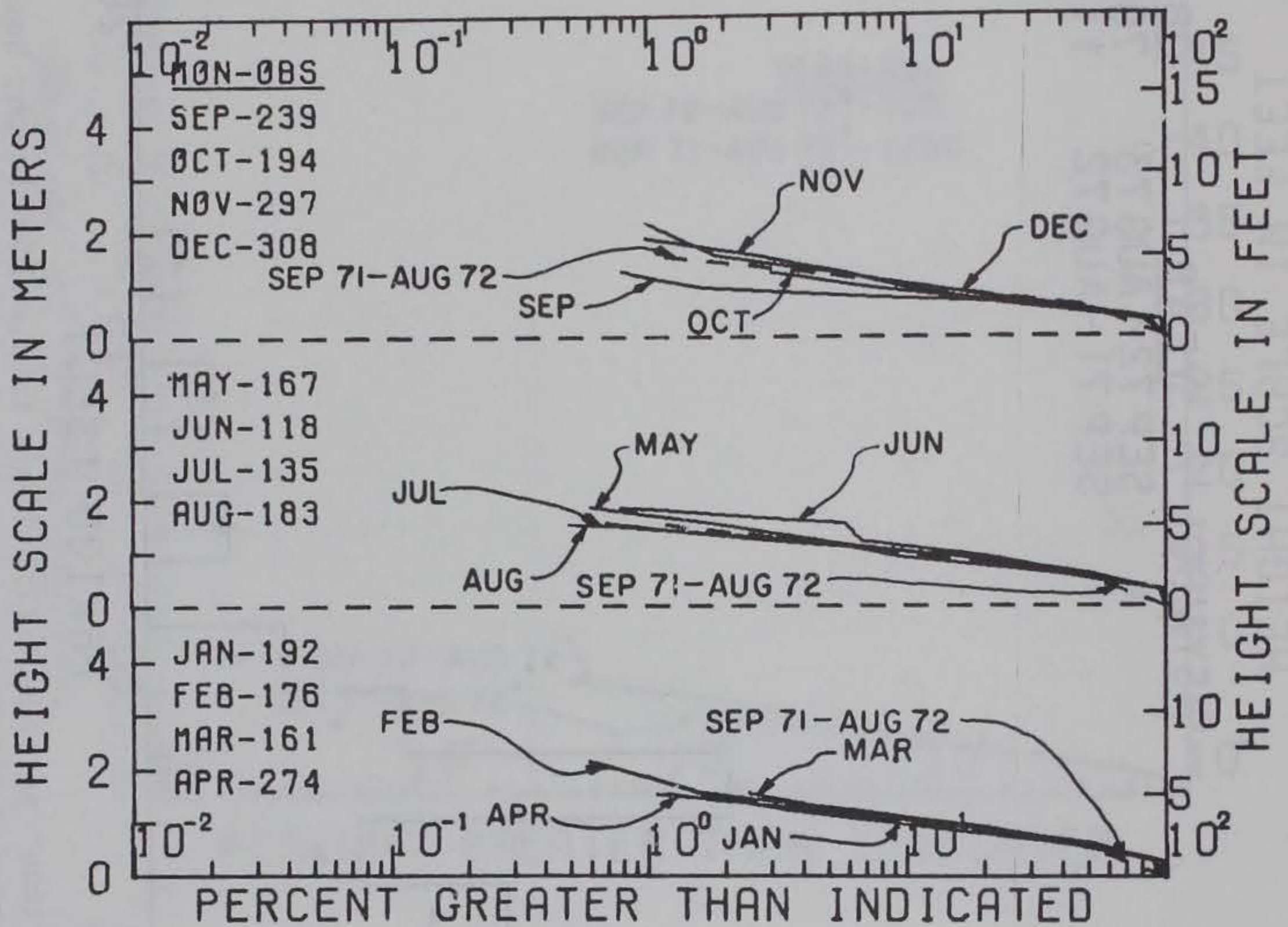
Figure A-42. Seasonal summaries of cumulative significant height distributions from Holden Beach, North Carolina; computed from 1,024-second digital wave records taken four times daily.
