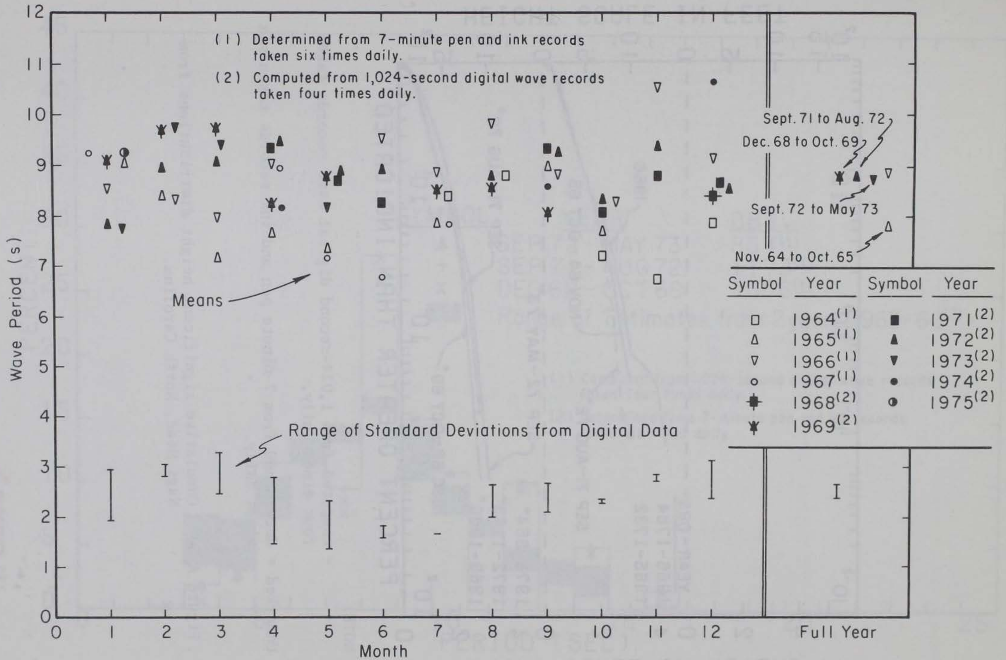
Figure A-29. Means and standard deviations of wave periods for Nags Head, North Carolina
