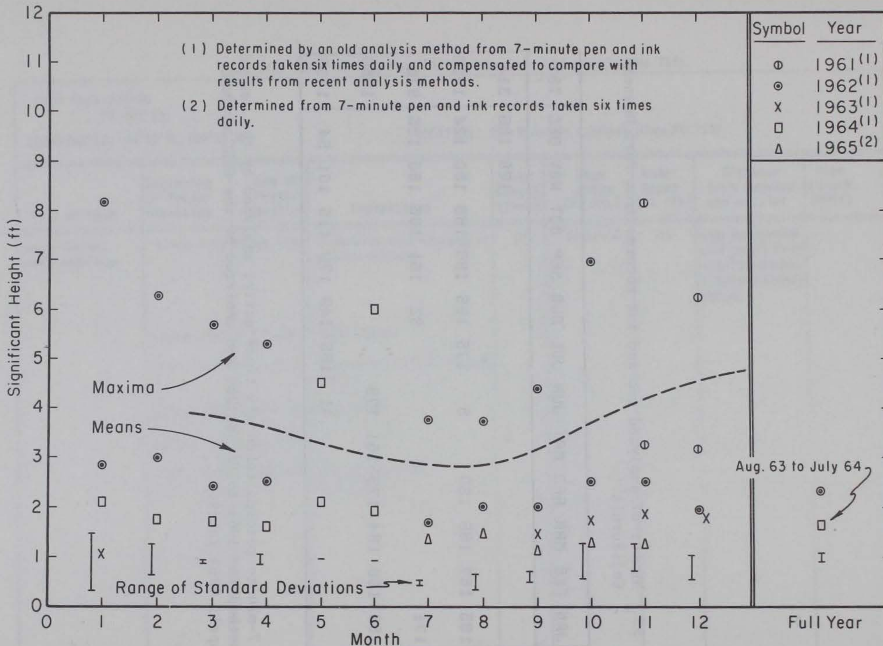
Figure A-83. Maxima, means, and standard deviation of significant height from Port Hueneme, California. Wave heights may be low due to old gage design and maintenance difficulties.
