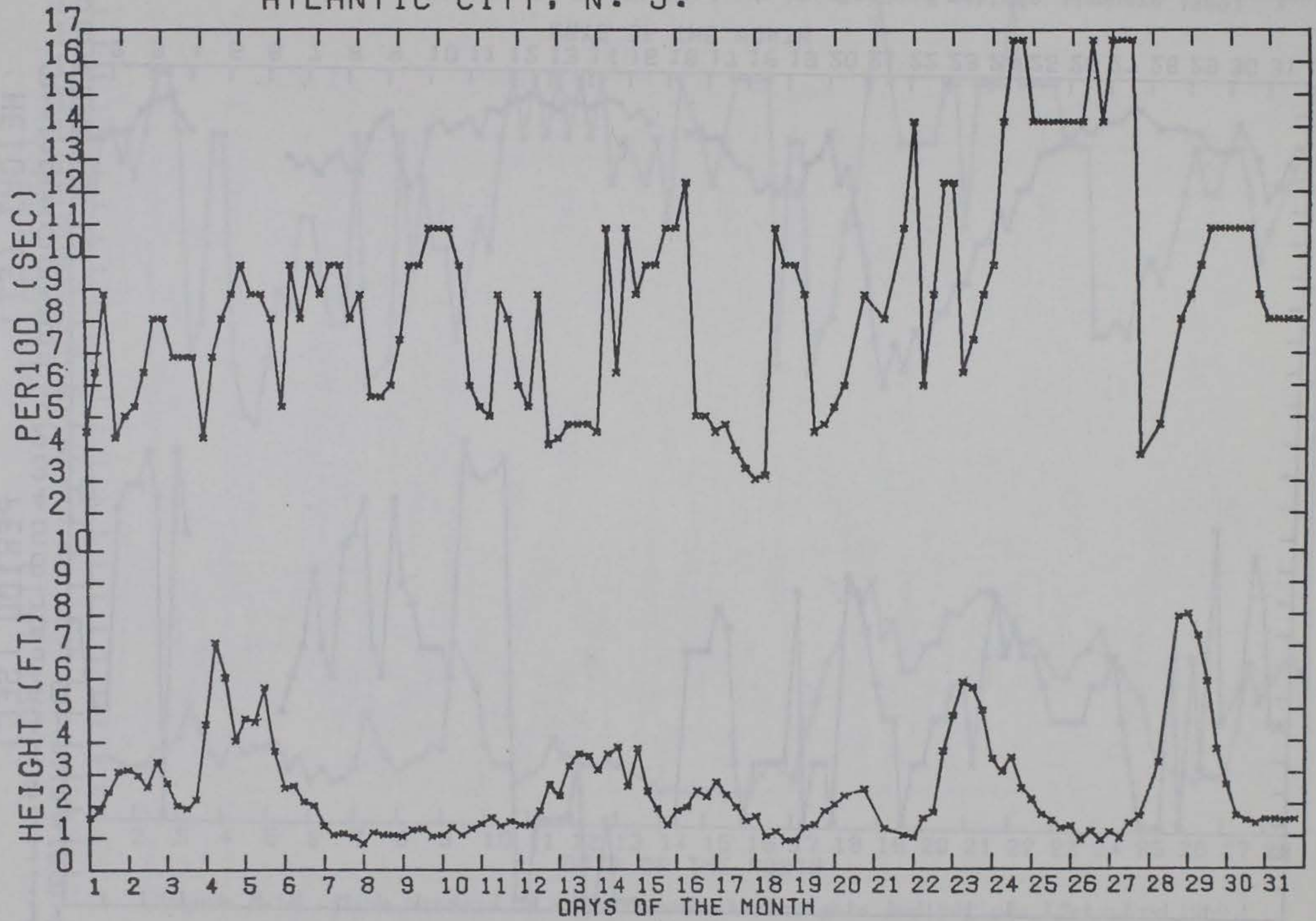
Figure A-12. Time history of significant wave heights and periods, December 1968.
