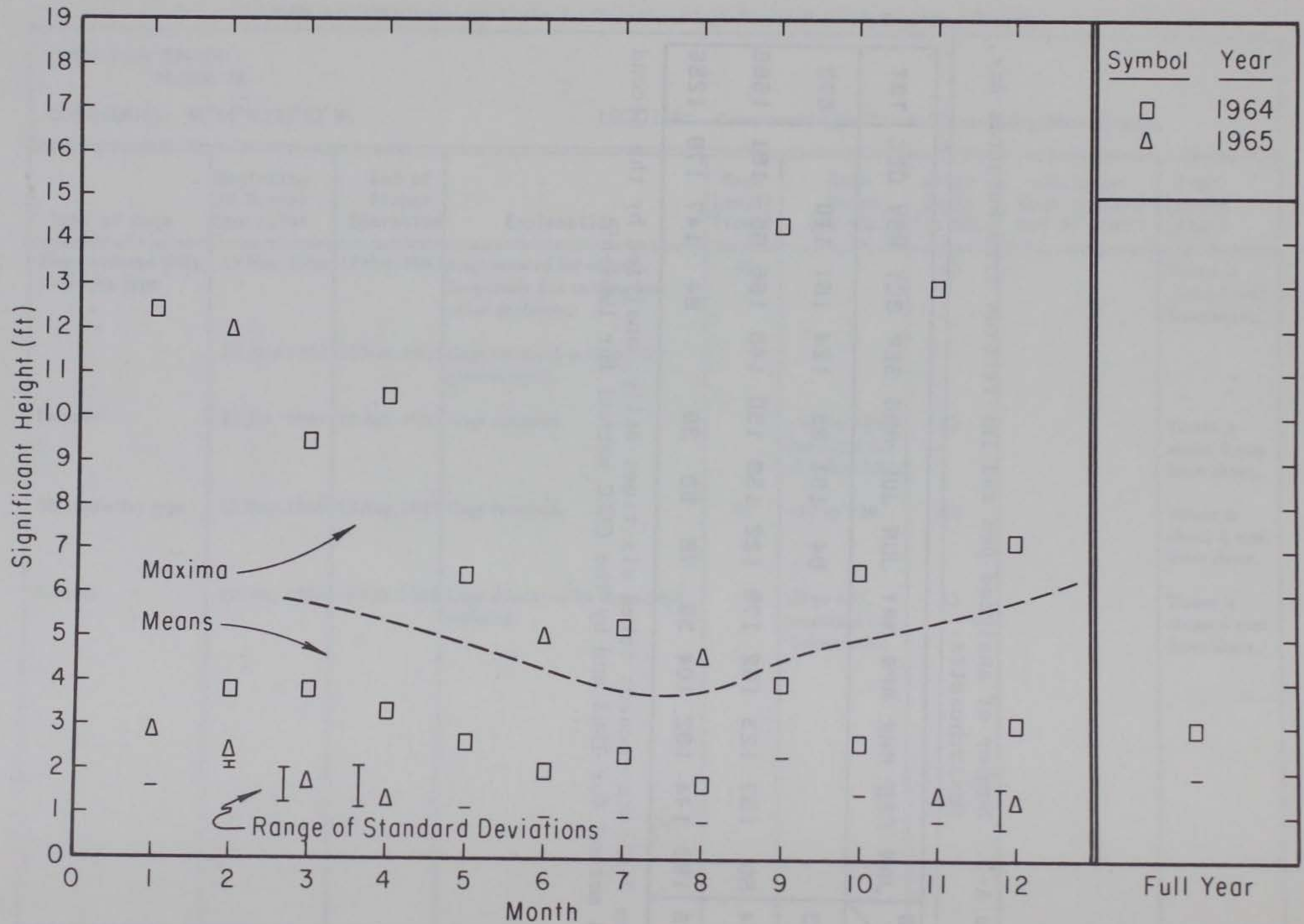
Figure A-2. Maxima, means, and standard deviations of significant height from Buzzards Bay, Massachusetts; determined from 7-minute pen and ink records taken six times daily.
