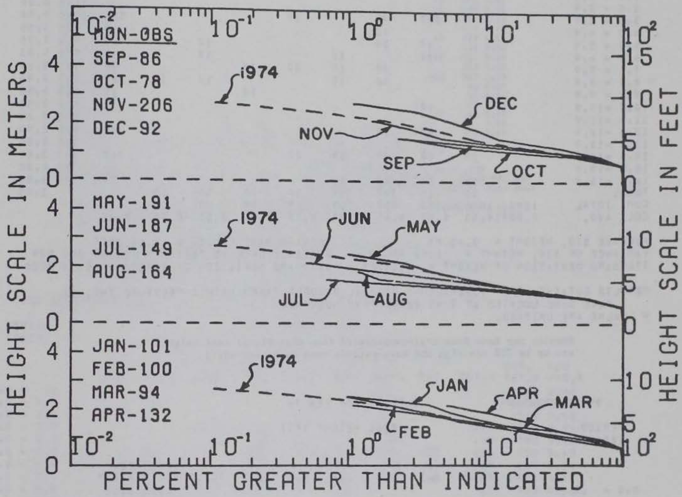
Figure A-97. Seasonal summaries of cumulative significant height distributions from Pt. Mugu, California (Gage No. 4). Computed from 1,024-second digital wave records taken four times daily. Results may have been overcompensated such that significant heights are up to 20 percent too high.
