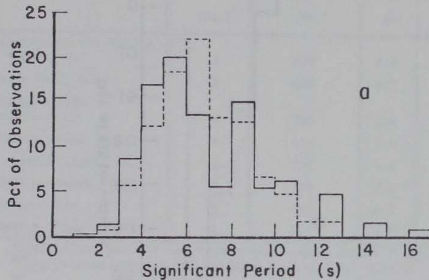
Figure 16. Comparison of distribution functions of wave period estimated from digital (solid line) and pen and ink records (dashline) taken during September 1971 to April 1972. (a) Savannah Light Tower, Georgia (499 observations); (b) Wrightsville Beach, North Carolina (755 observations).
