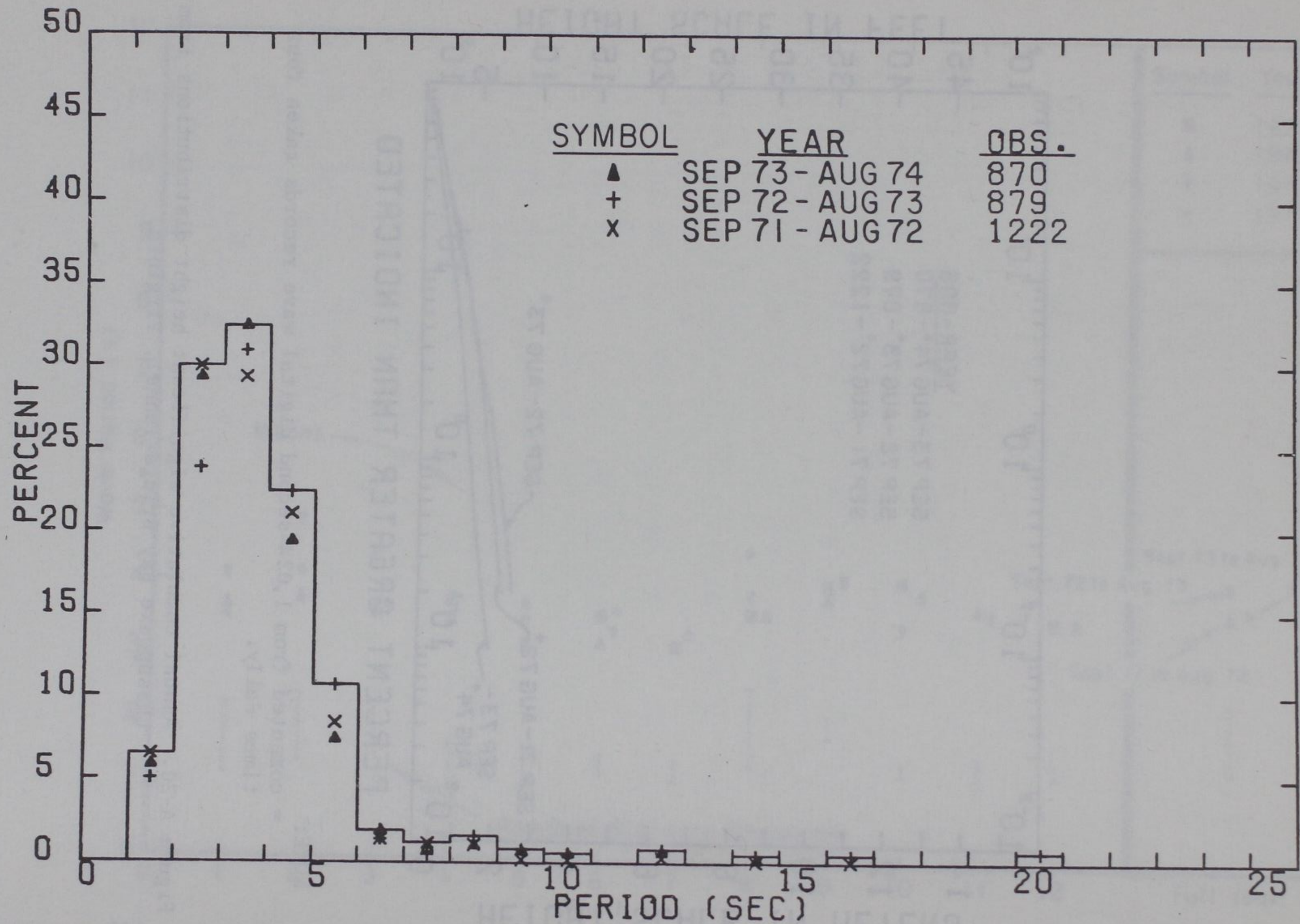
Figure A-21. Annual significant period distributions from Chesapeake Bay Bridge-Tunnel, Virginia; computed from 1,024-second digital wave records taken four times daily.
