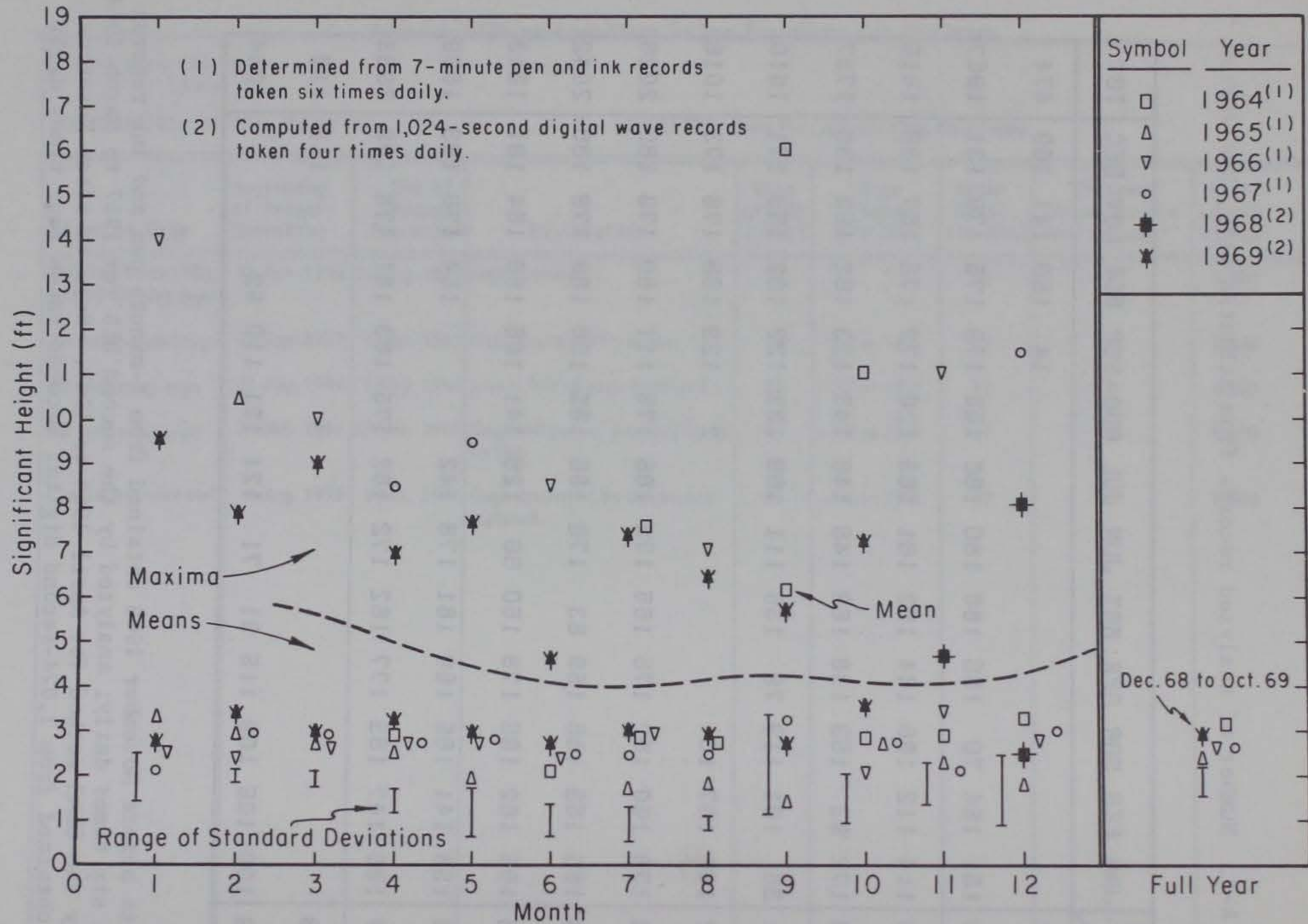
Figure A-7. Maxima, means, and standard deviations of significant height from Atlantic City, New Jersey.
