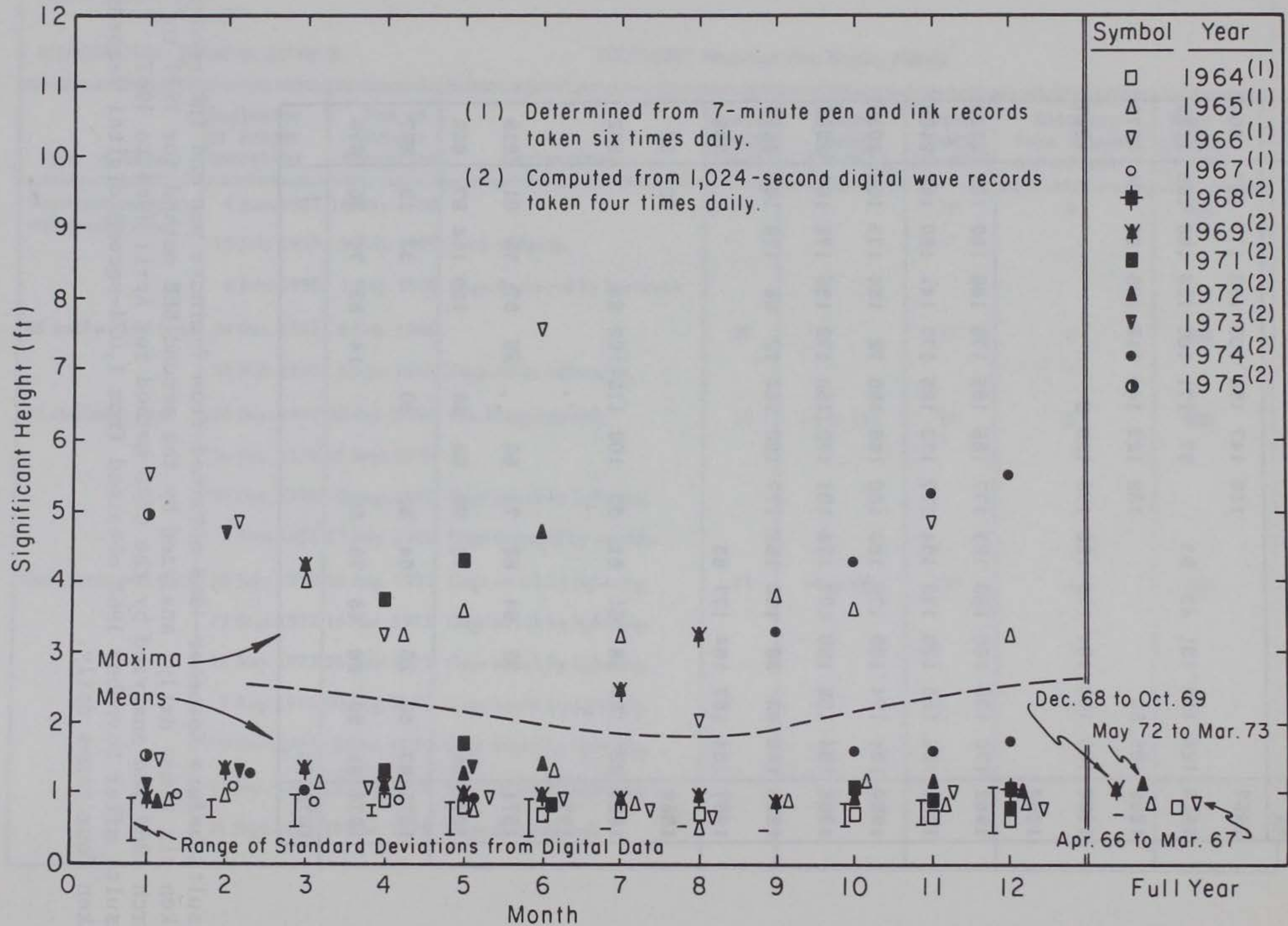
Figure A-64. Maxima, means, and standard deviations of significant height from Naples, Florida.
