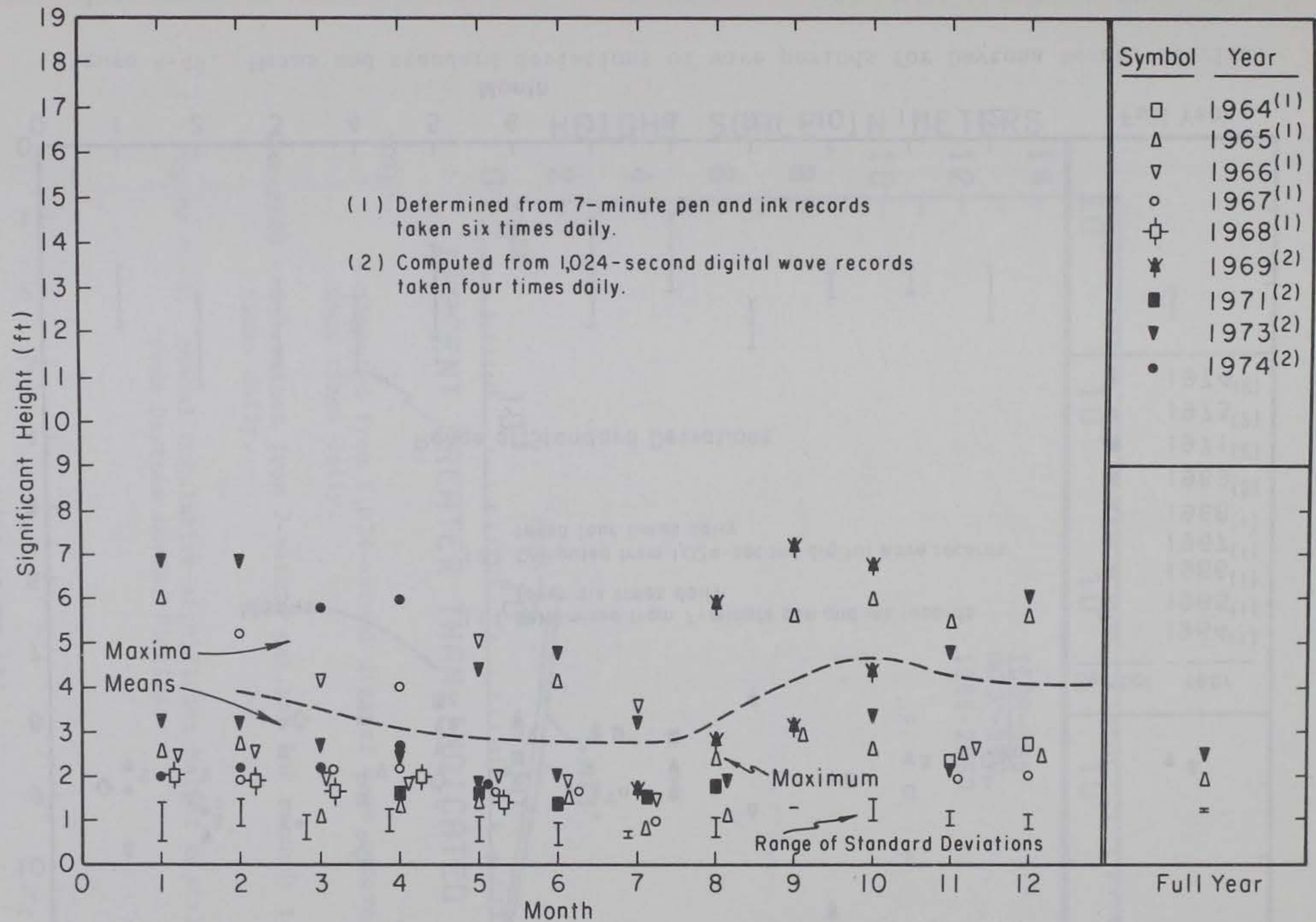
Figure A-48. Maxima, means, and standard deviations of significant height from Daytona Beach, Florida.
