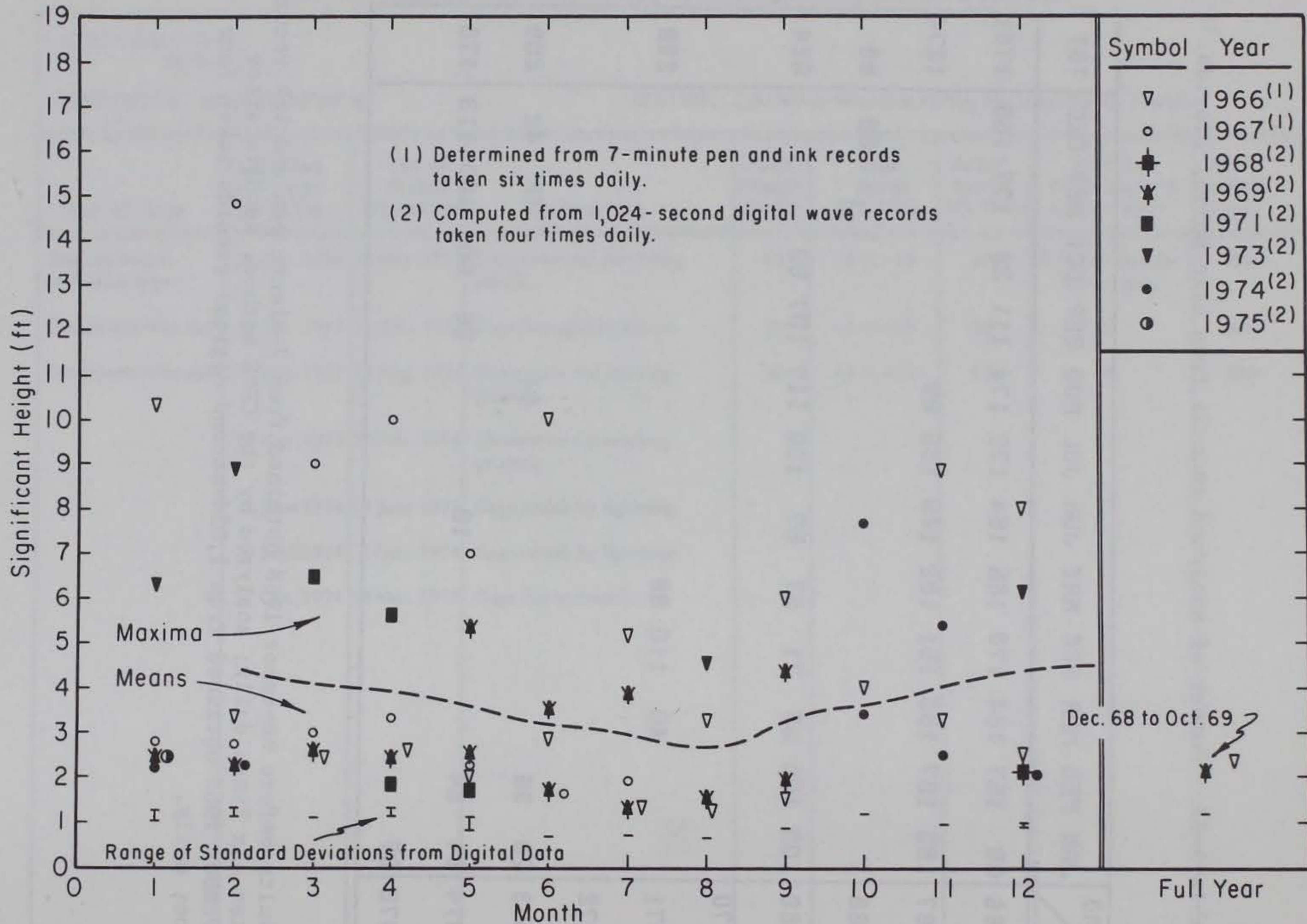
Figure A-58. Maxima, means, and standard deviations of significant height from Lake Worth, Florida.
