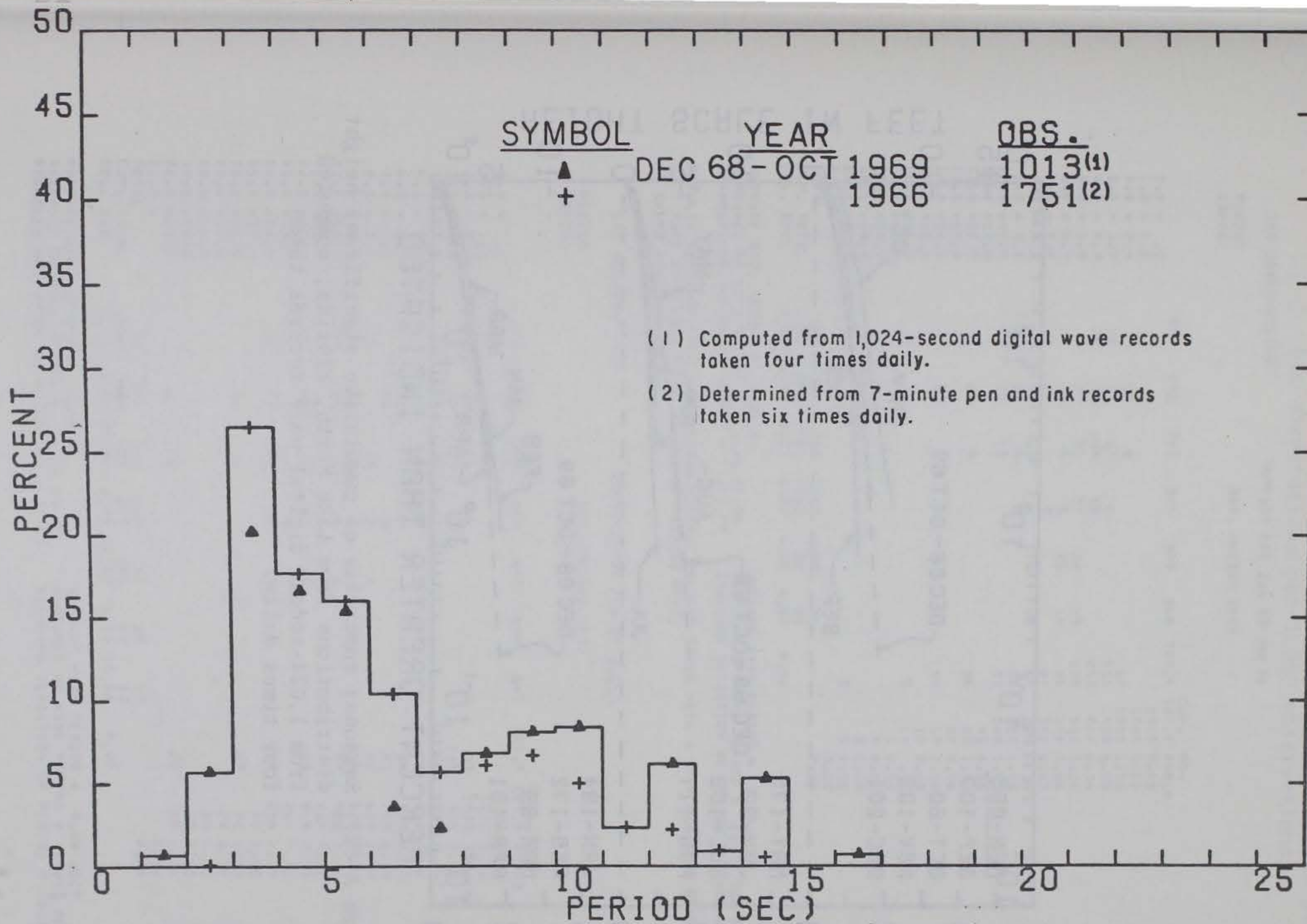
Figure A-61. Annual significant period distributions from Lake Worth, Florida.
