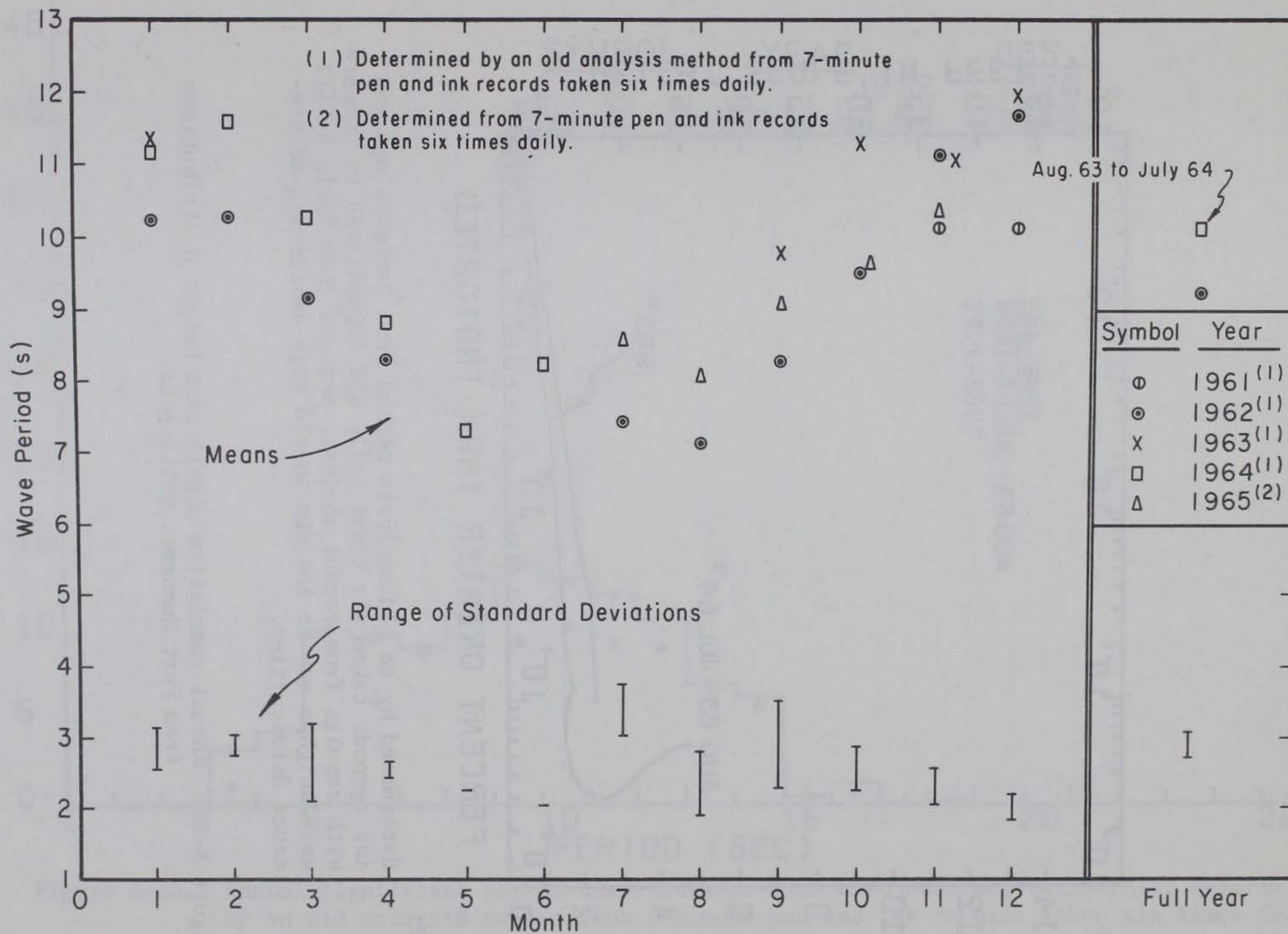
Figure A-84. Means and standard deviations of wave periods for Port Hueneme, California.
