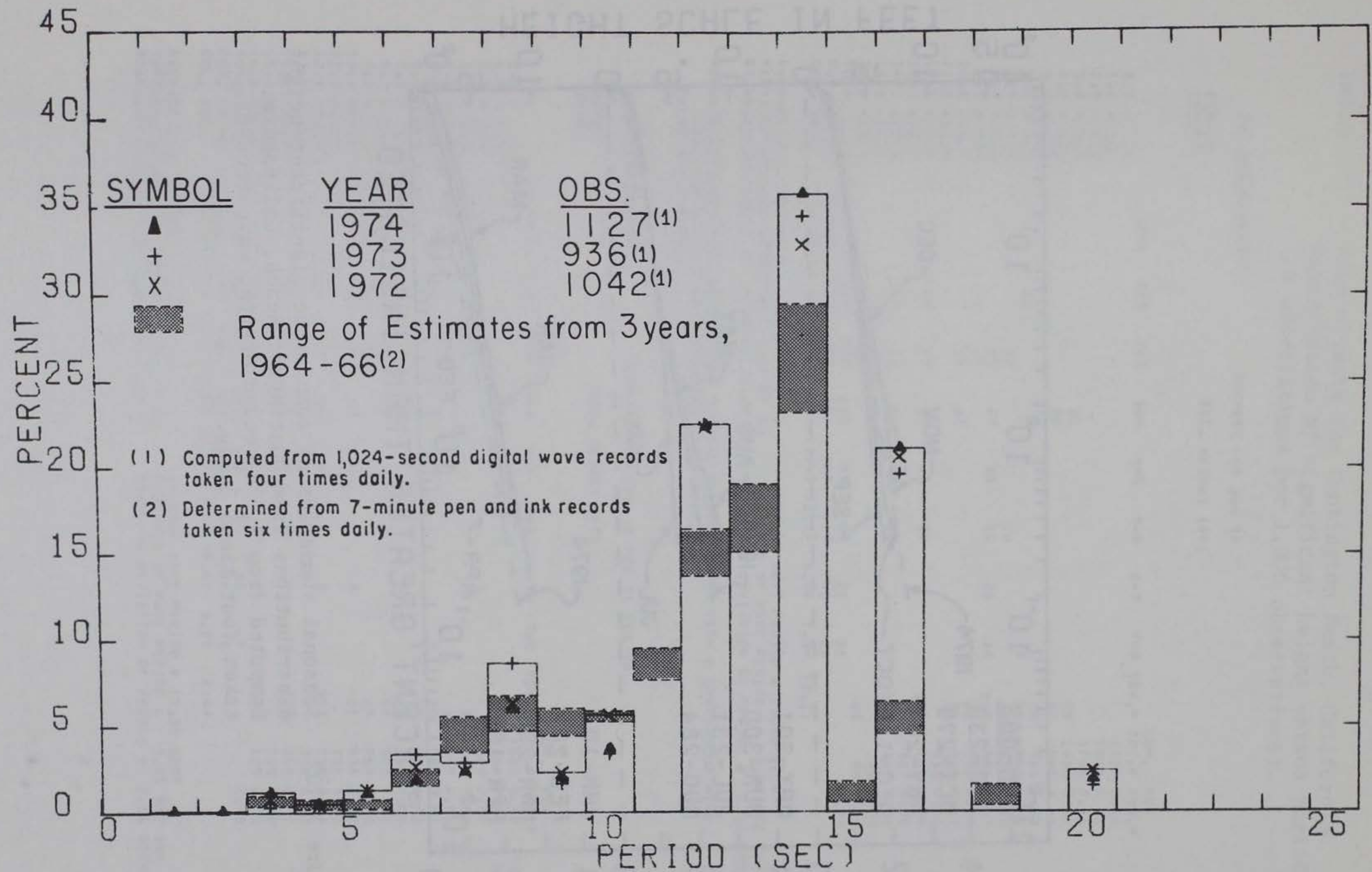
Figure A-106. Annual significant period distributions from Huntington Beach, California.
