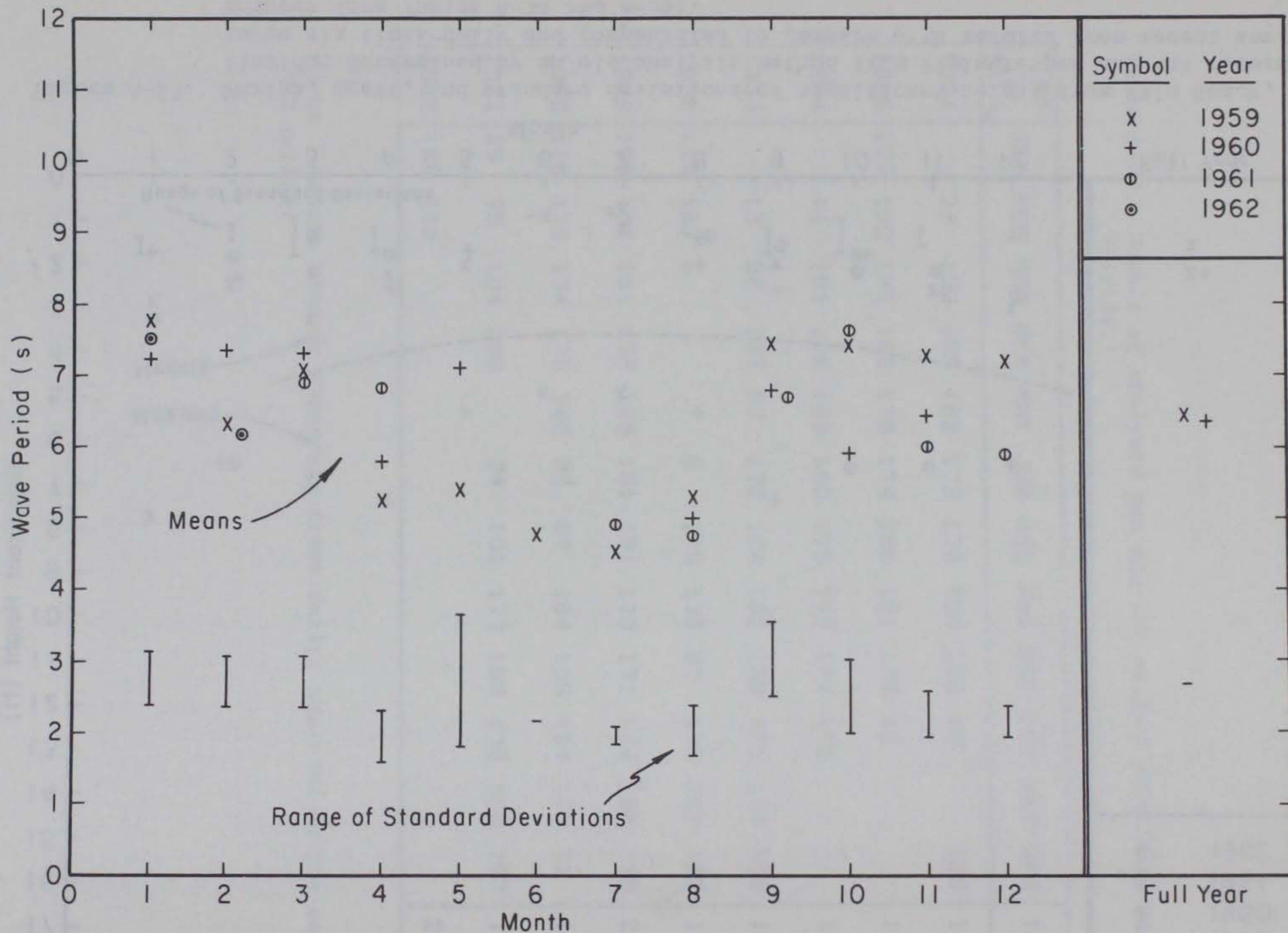
Figure A-54. Means and standard deviations of wave periods for Palm Beach, Florida; determined by an old analysis method from 7-minute pen and ink records taken six times daily
