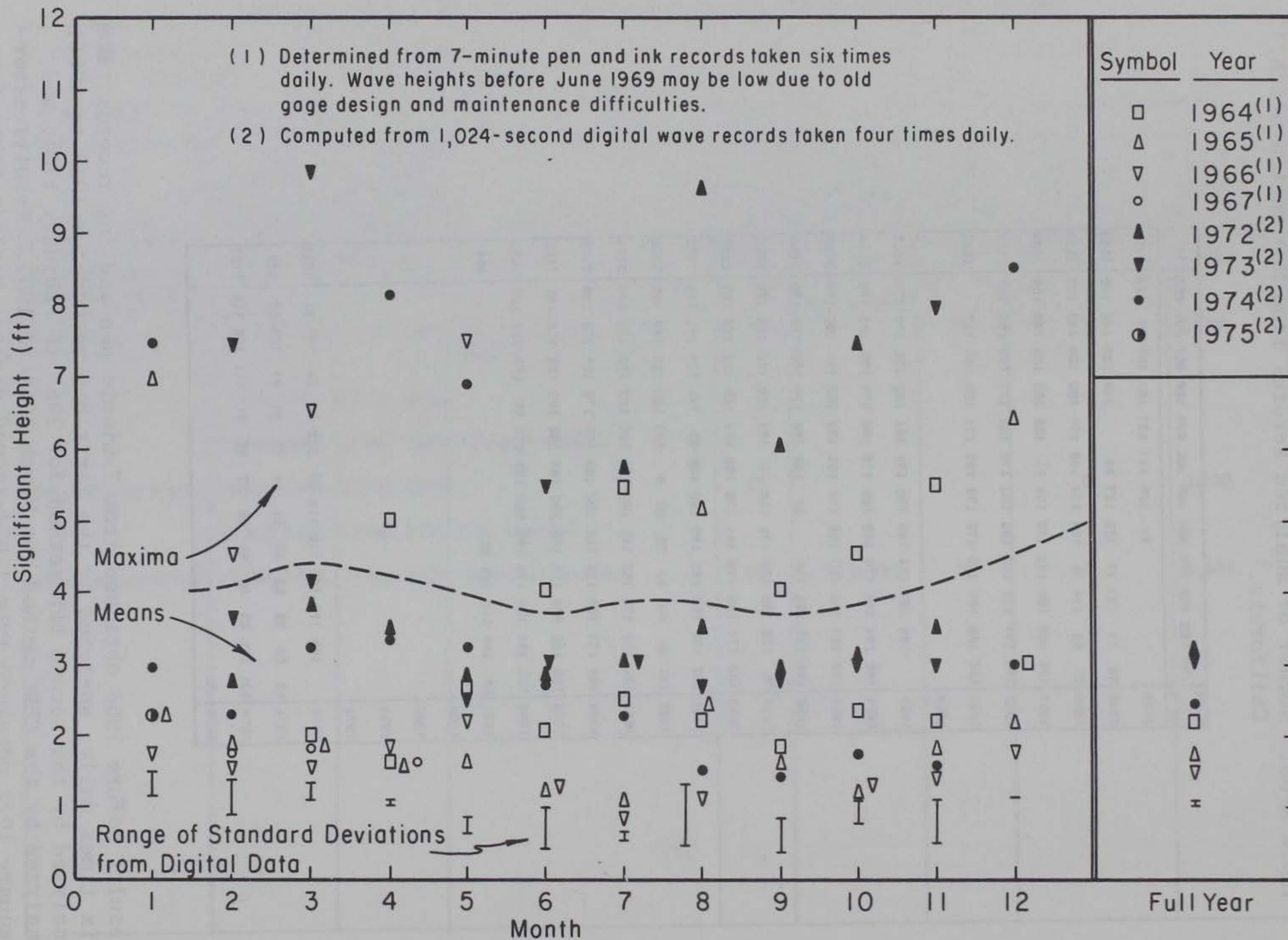
Figure A-103. Maxima, means, and standard deviations of significant height from Huntington Beach, California.
