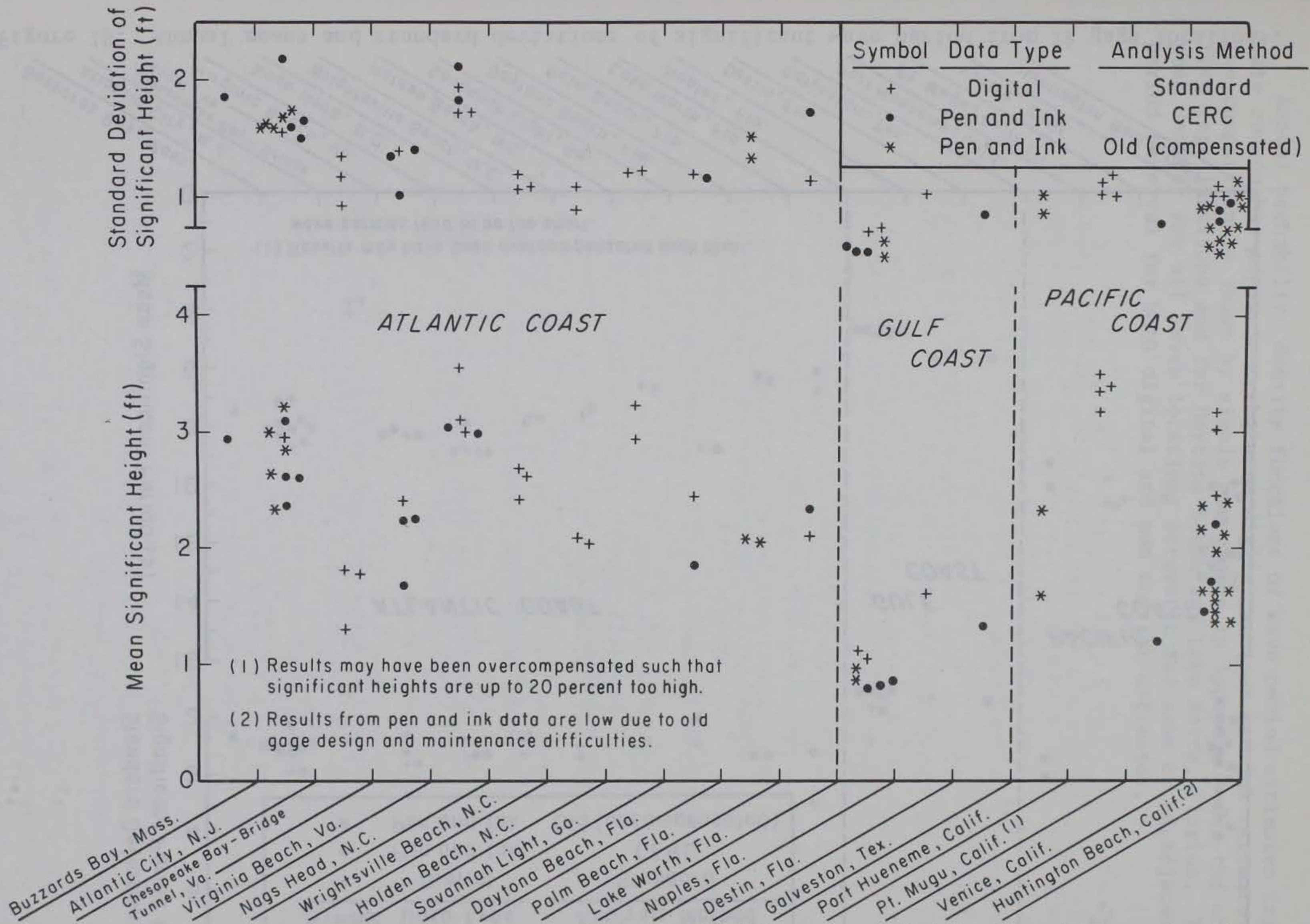
Figure 17. Annual means and standard deviations of significant wave height from 19 gage locations.
