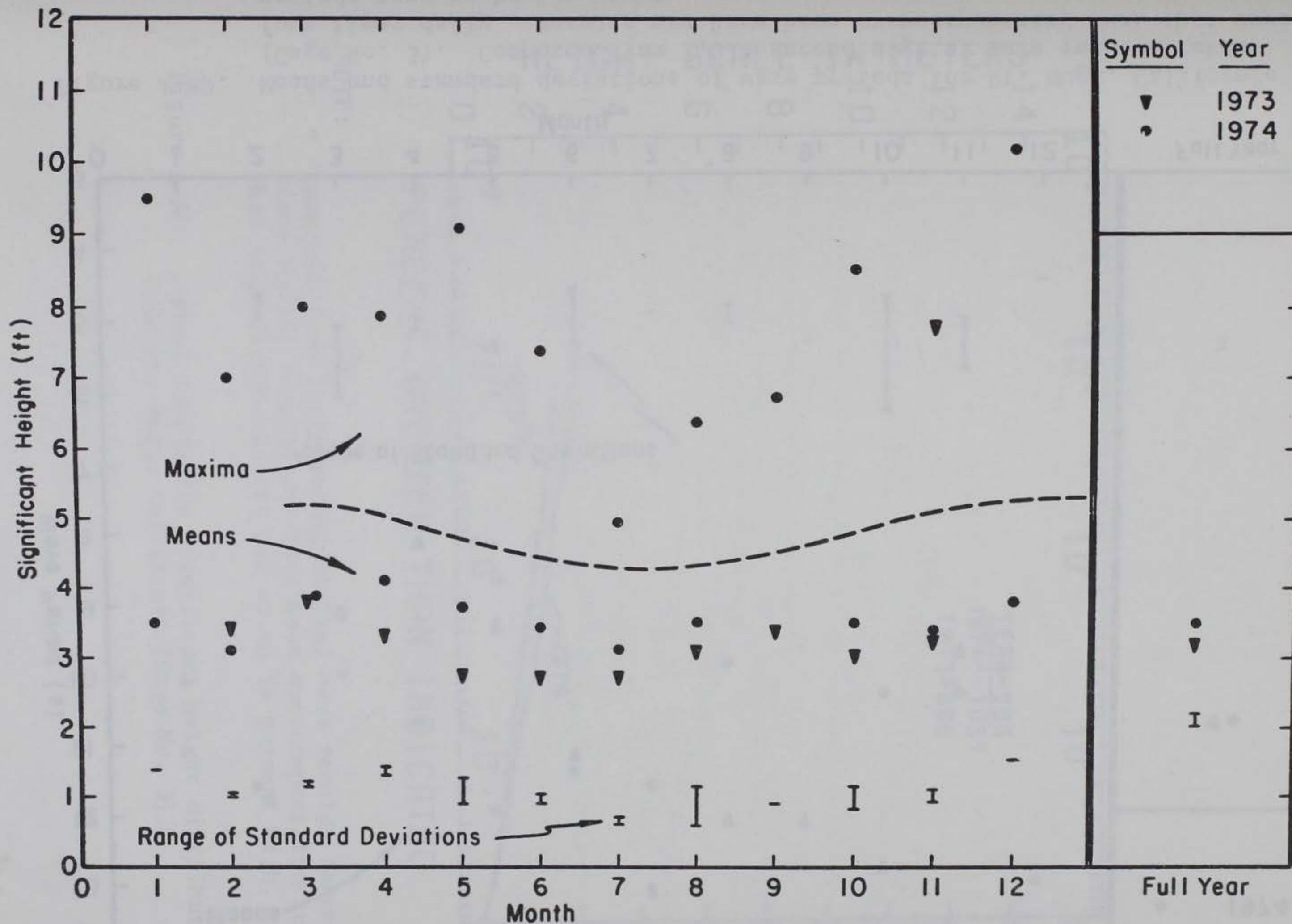
Figure A-88. Maxima, means, and standard deviations of significant height from Pt. Mugu, California (Gage No. 3). Computed from 1,024-second digital wave records taken four times daily. Results may have been overcompensated such that significant heights are up to 20 percent too high.
