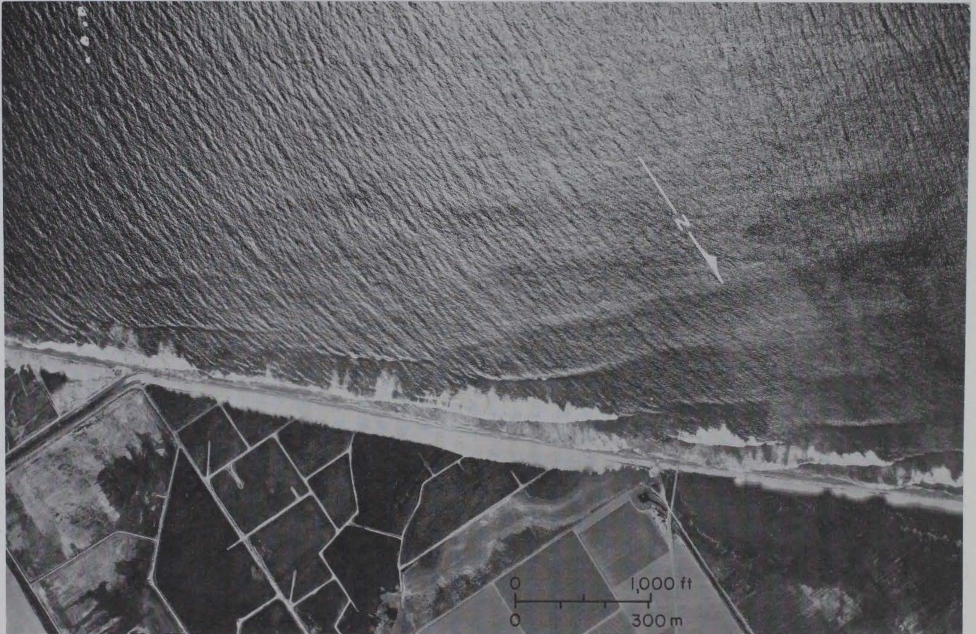
Figure 6. Aerial photo showing superimposed trains of sea and swell waves south of Port Hueneme, California, on 3 August 1960. The train of swell waves is nearly invisible offshore but is dominating the breaker zone.
