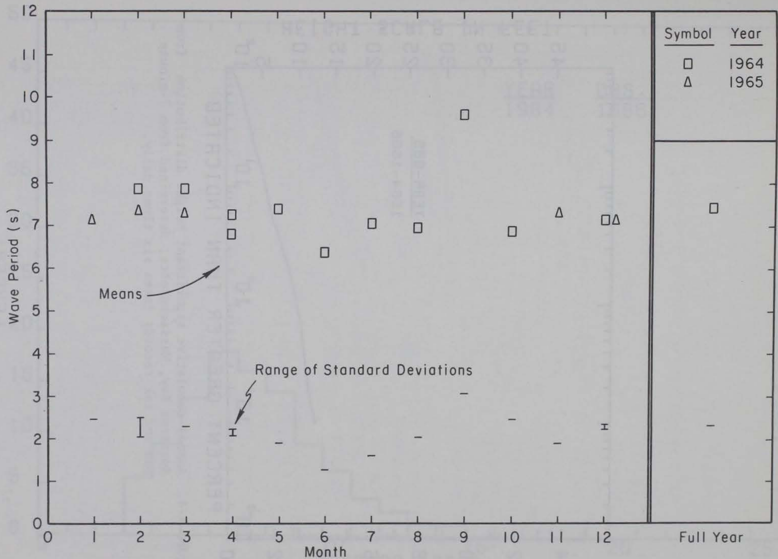
Figure A-3. Means and standard deviations of wave period from Buzzards Bay, Massachusetts; determined from 7-minute pen and ink records taken six times daily.
