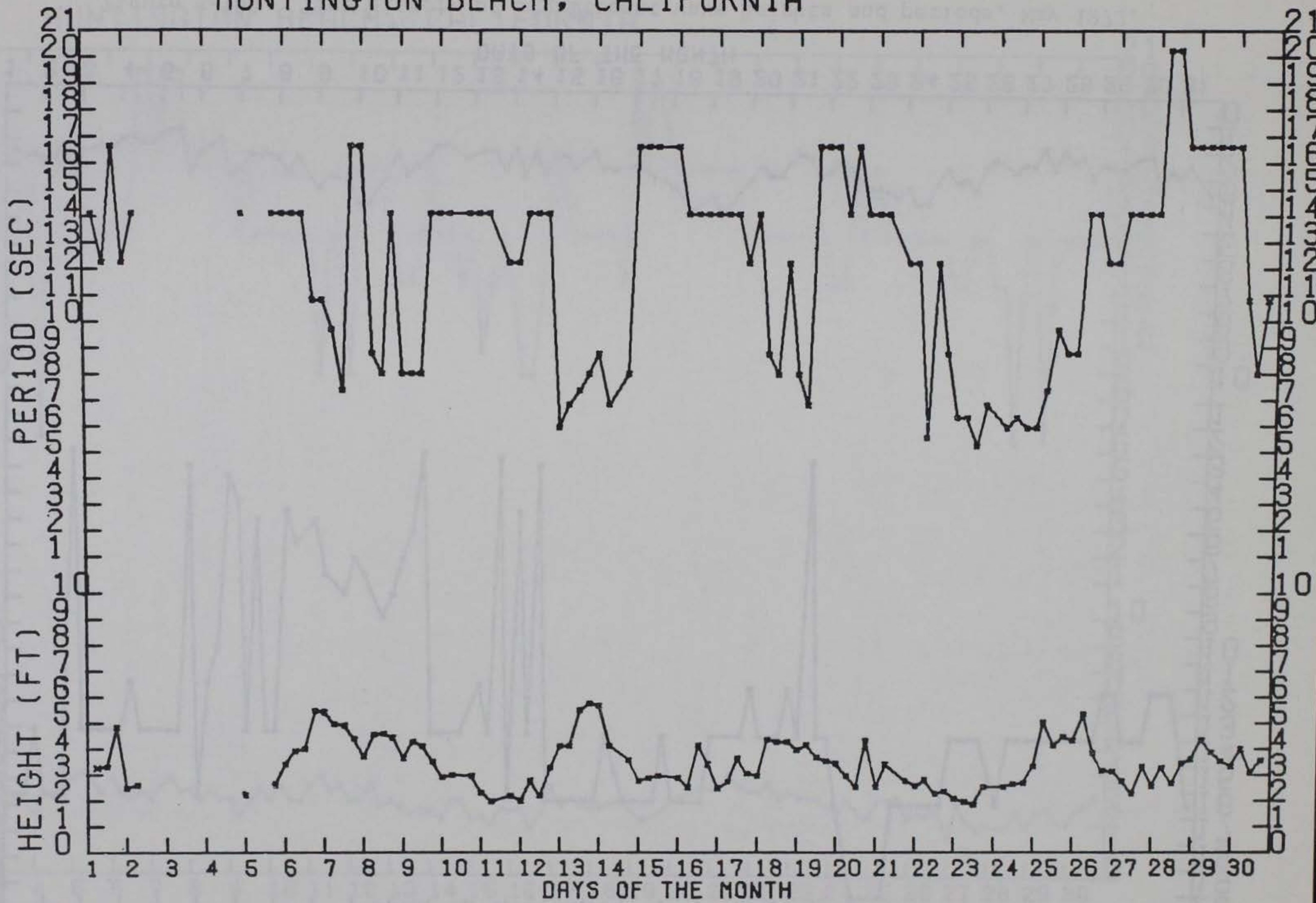
Figure A-108. Time history of significant wave heights and periods, April 1972.
