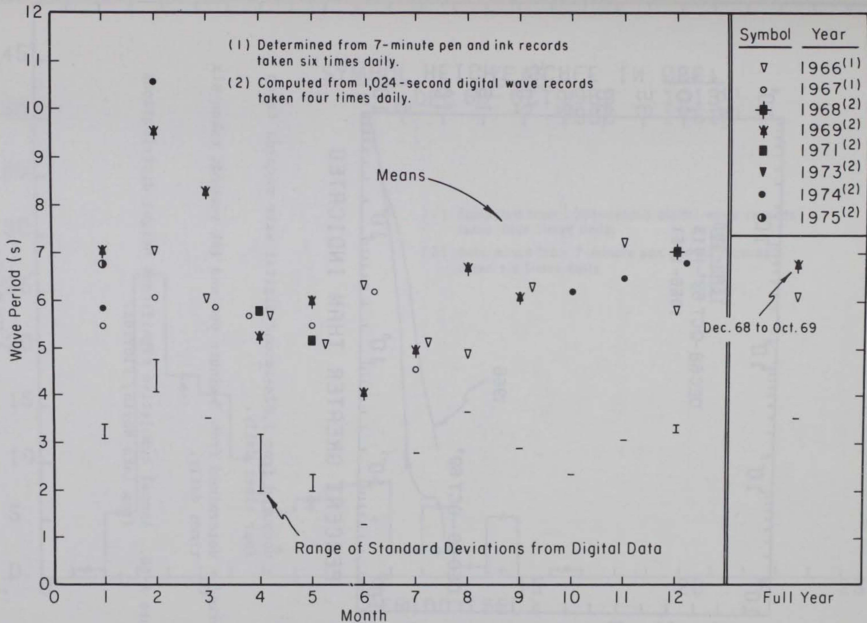
Figure A-59. Means and standard deviations of wave periods for Lake Worth, Florida.
