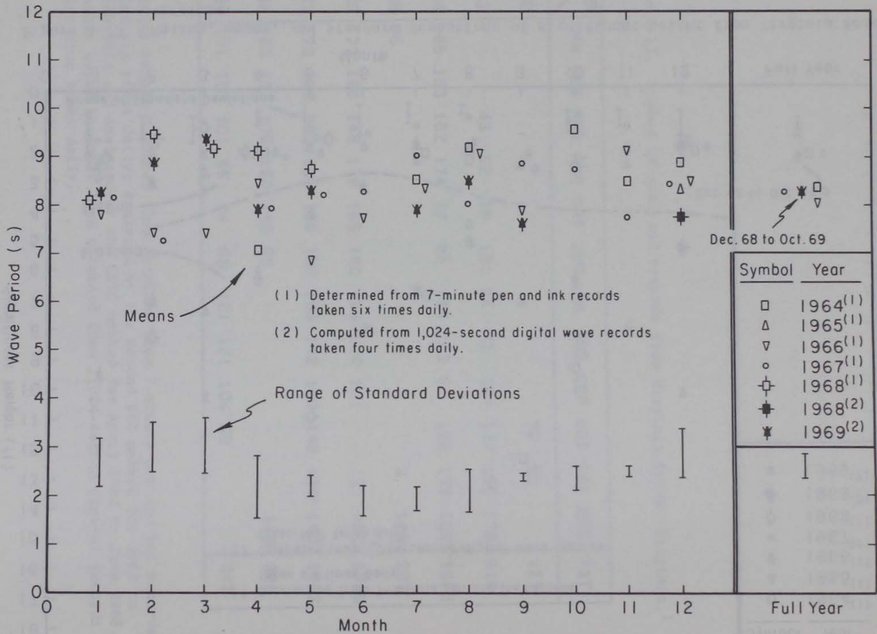
Figure A-24. Means and standard deviations of wave periods for Virginia Beach, Virginia.
