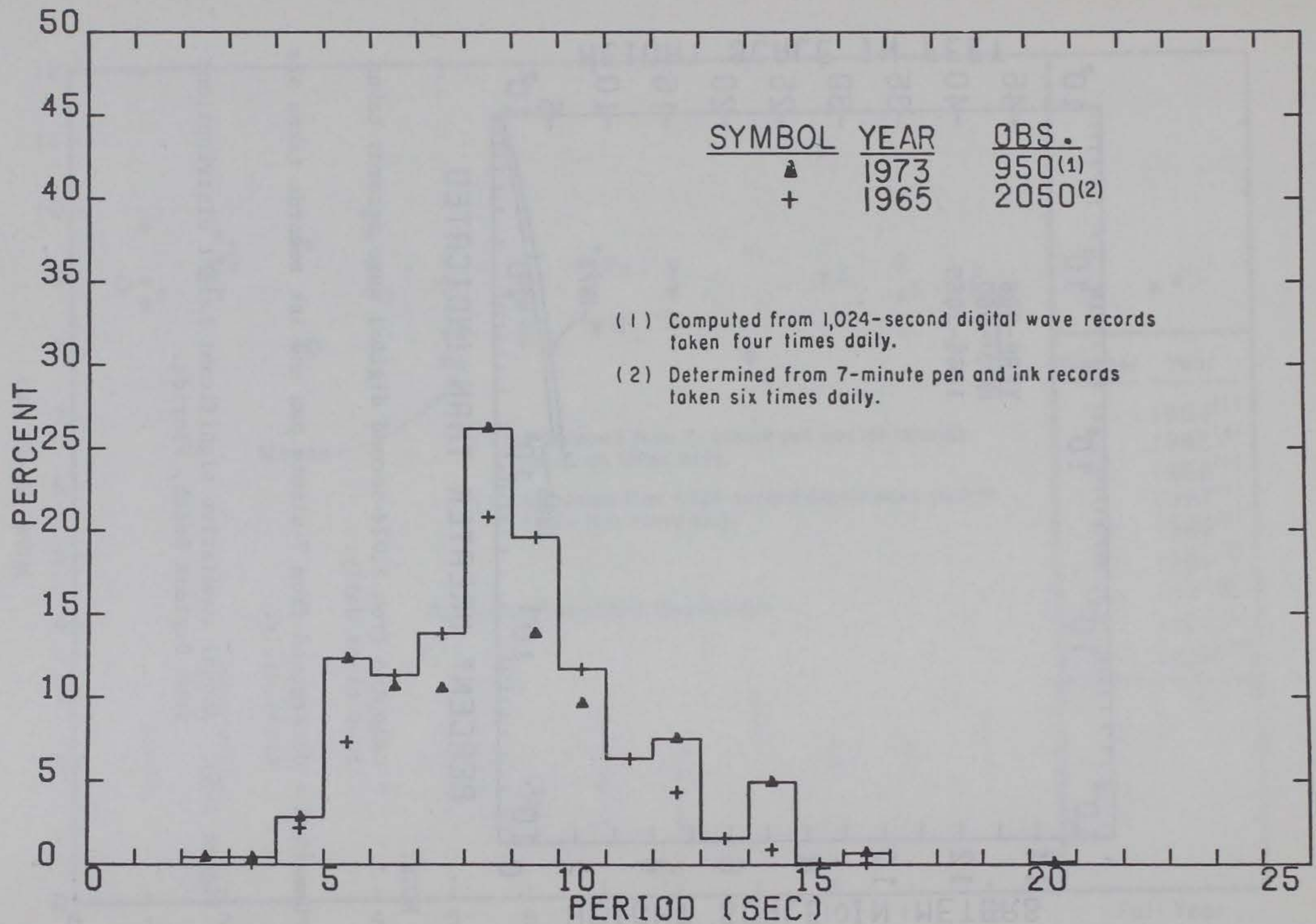
Figure A-51. Annual significant period distributions from Daytona Beach, Florida.
