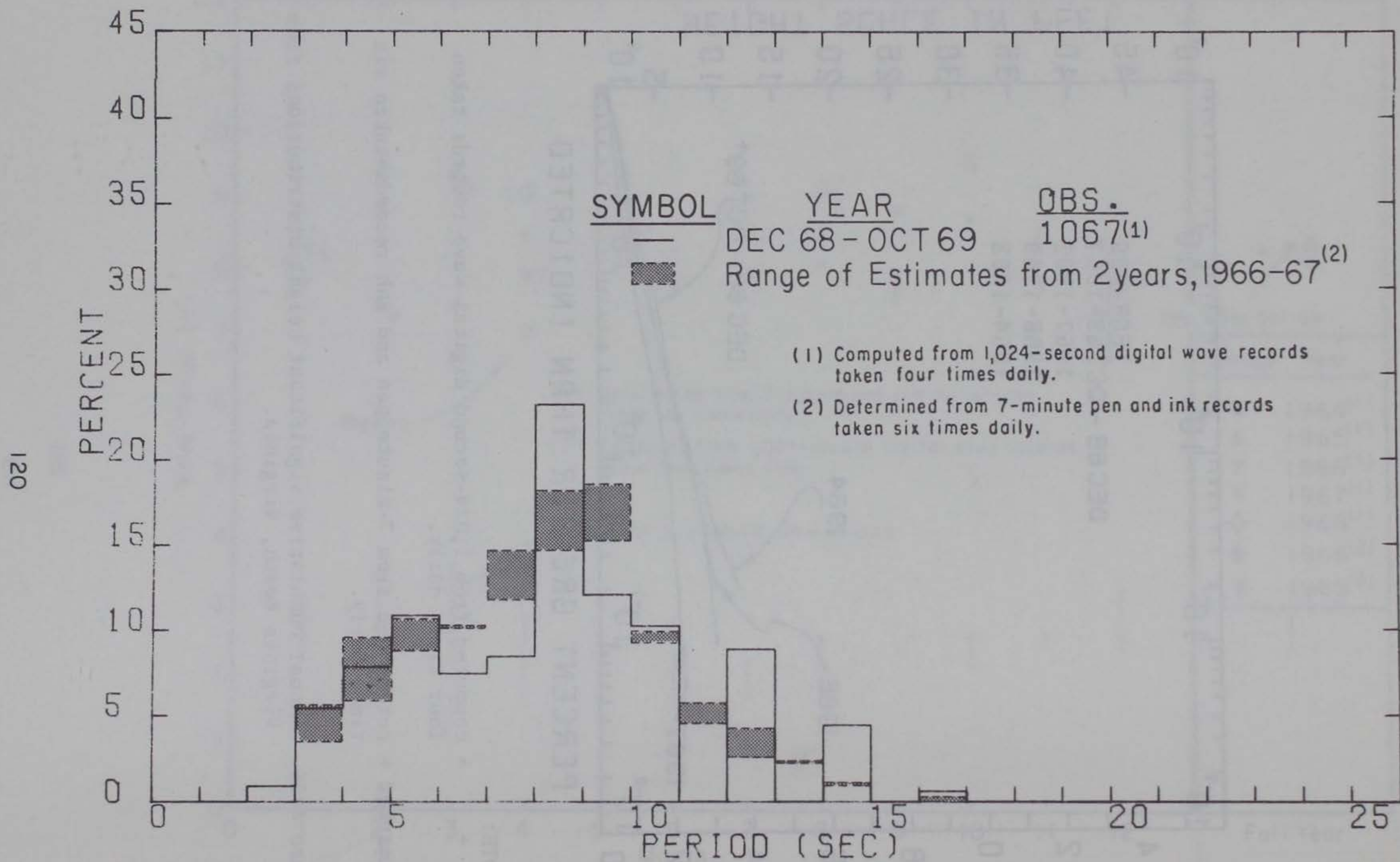
Figure A-26. Annual significant period distributions from Virginia Beach, Virginia.
