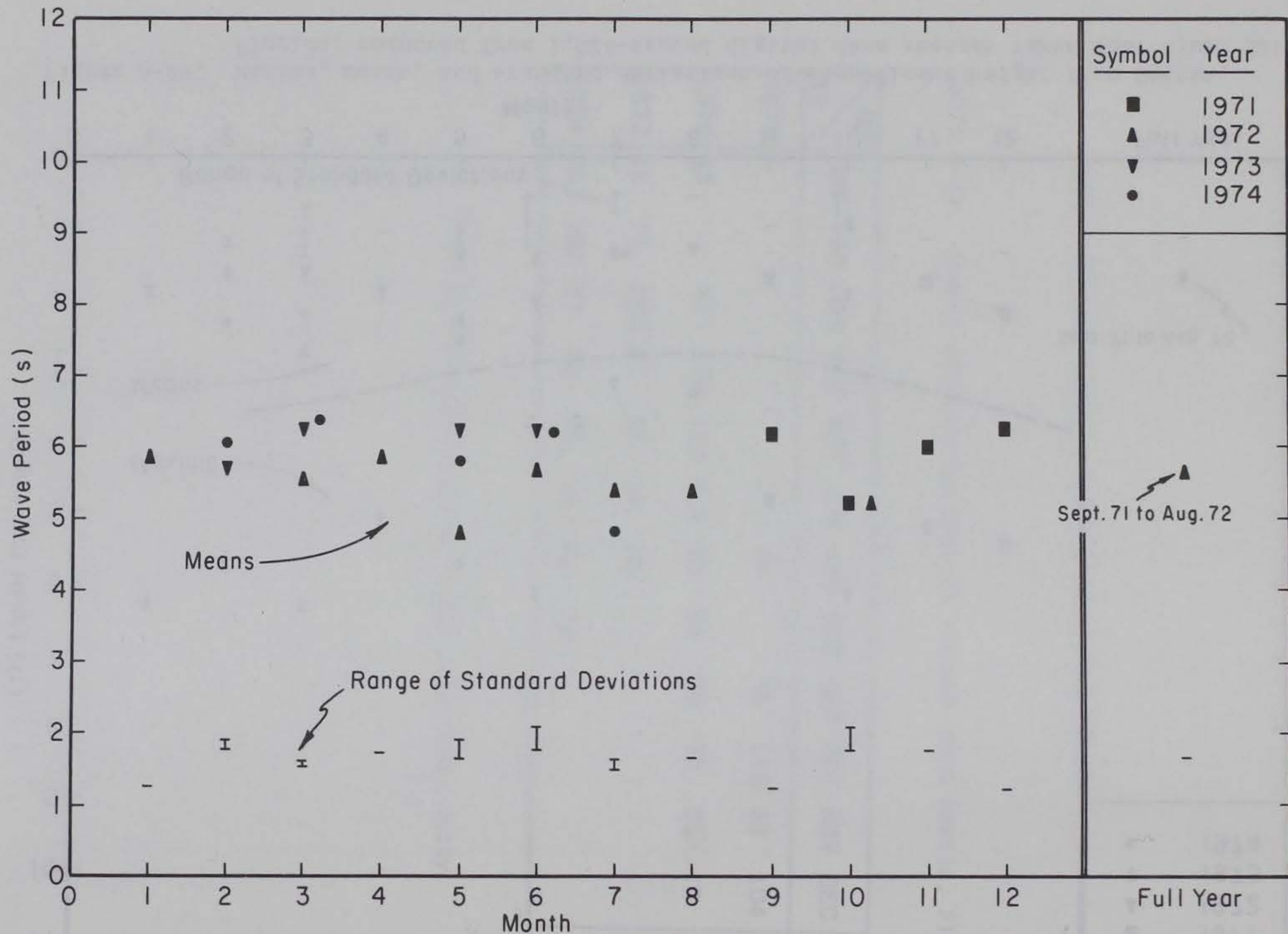
Figure A-70. Means and standard deviations of wave periods for Destin, Florida; computed from 1,024-second digital wave records taken four times daily.
