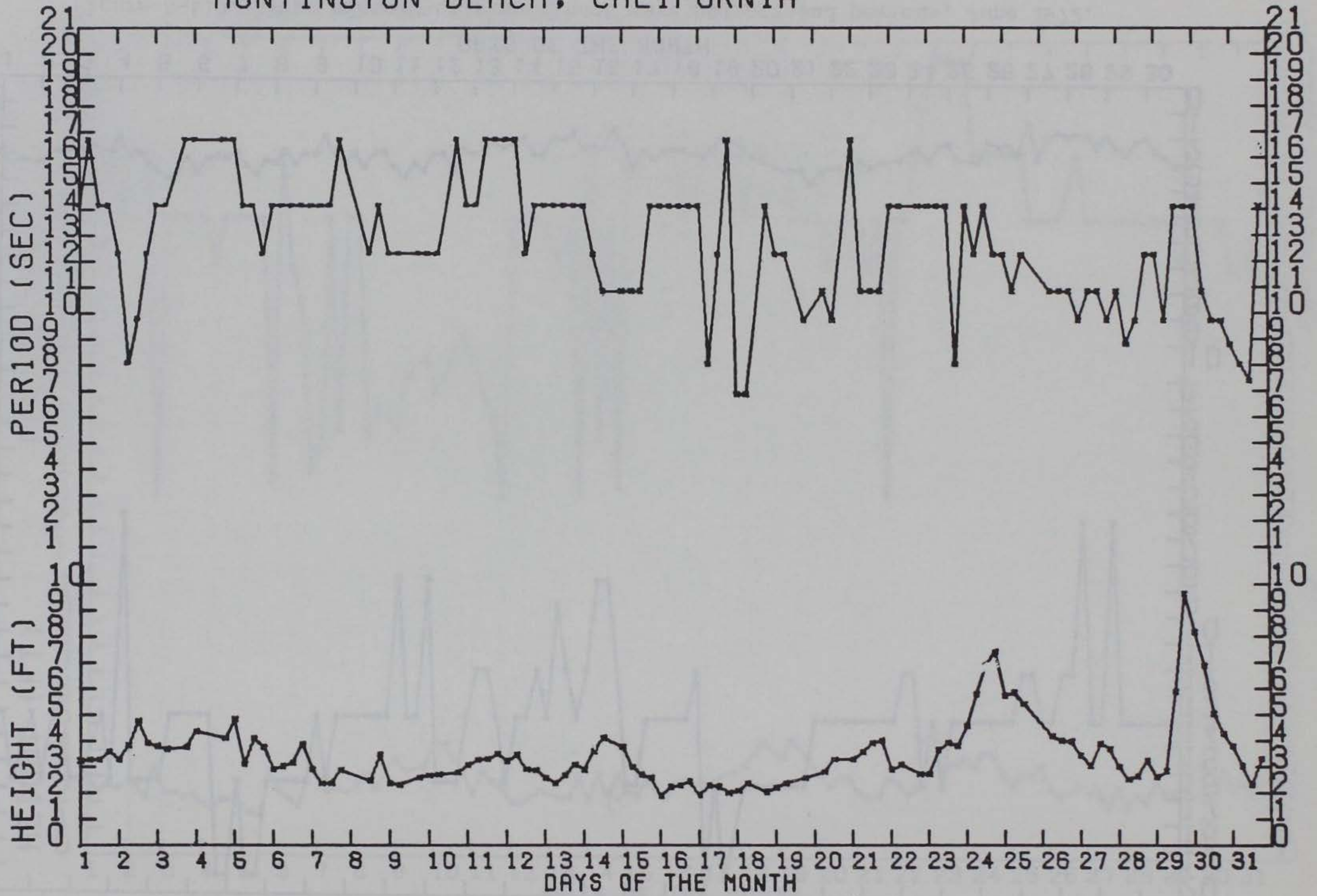
Figure A-111. Time history of significant wave heights and periods, July 1972.
