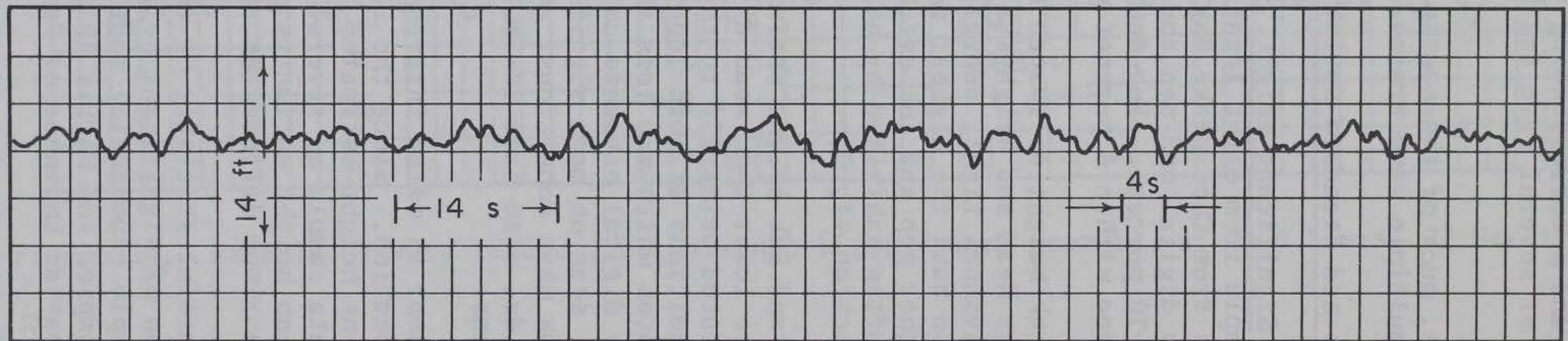
Figure 13. Example of wave record from Savannah Light Tower, Georgia, at 0042 hours, 22 September 1971.
