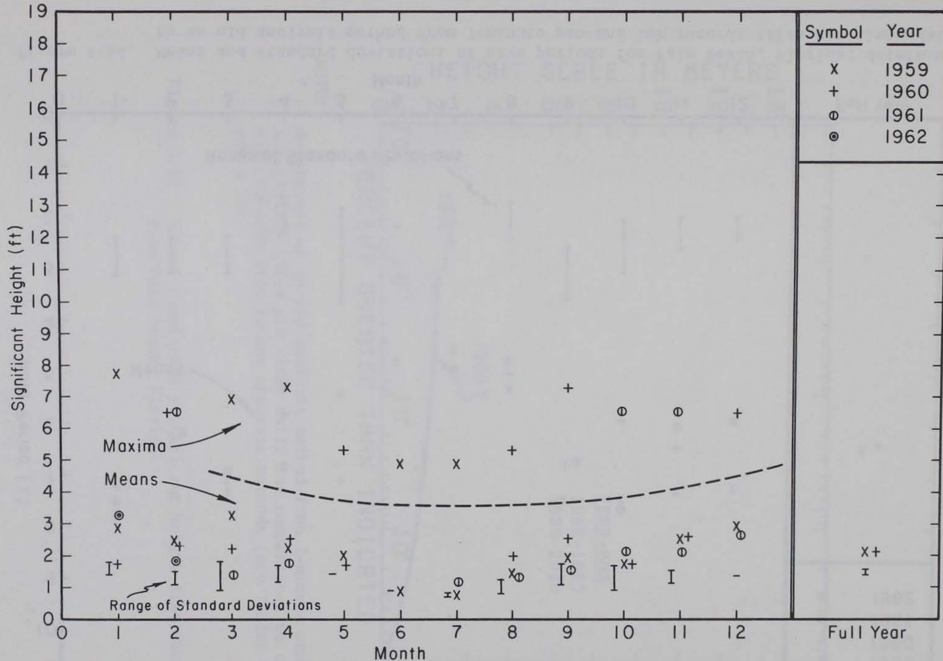
Figure A-53. Maxima, means, and standard deviations of significant height from Palm Beach, Florida; determined by an old analysis method from 7-minute pen and ink records taken six times daily and compensated to compare with results from recent analysis methods (see Tables A-34 and A-35).
