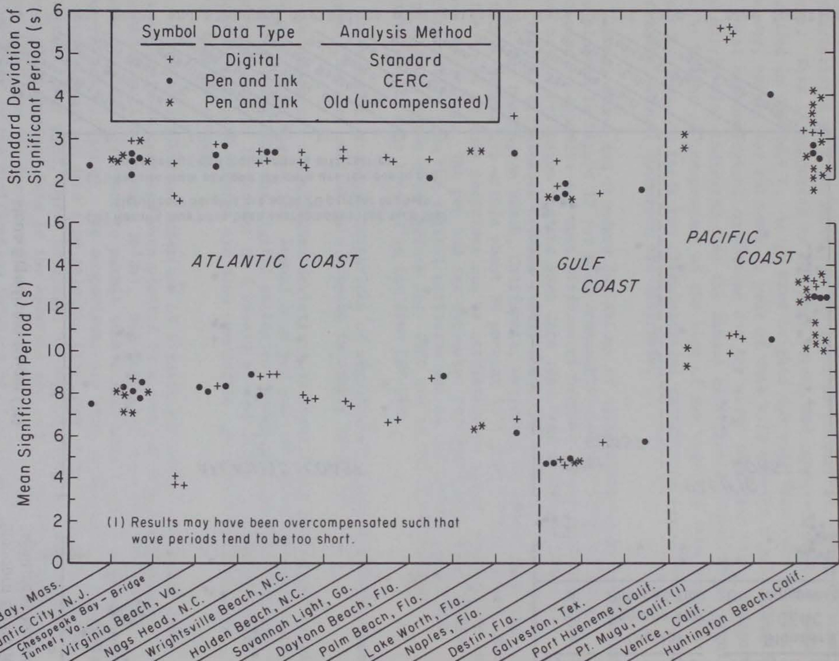
Figure 18. Annual means and standard deviations of significant wave period from 19 gage locations.
