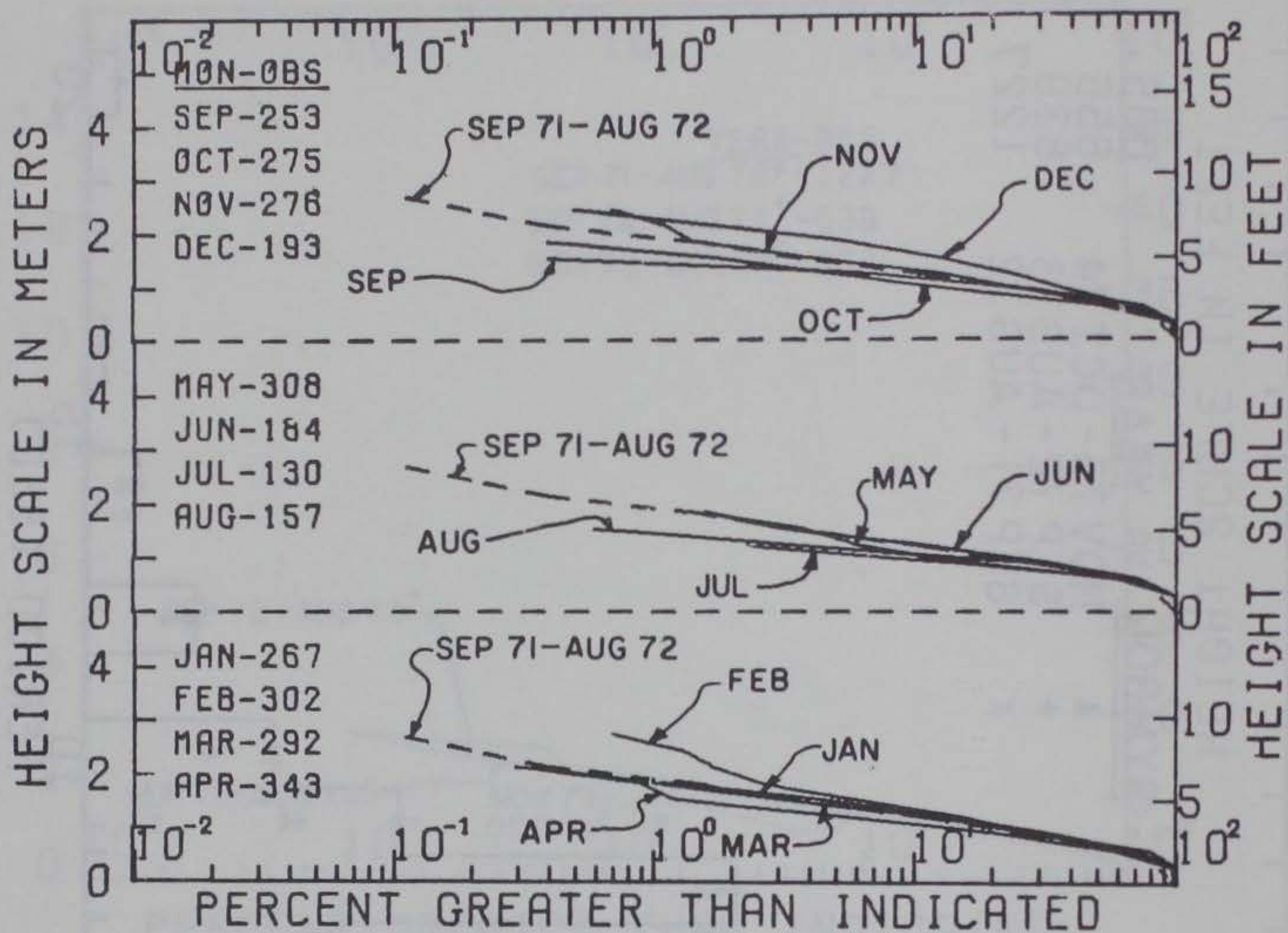
Figure A-37. Seasonal summaries of cumulative significant height distributions from Wrightsville Beach, North Carolina; computed from 1,024-second digital wave records taken four times daily.
