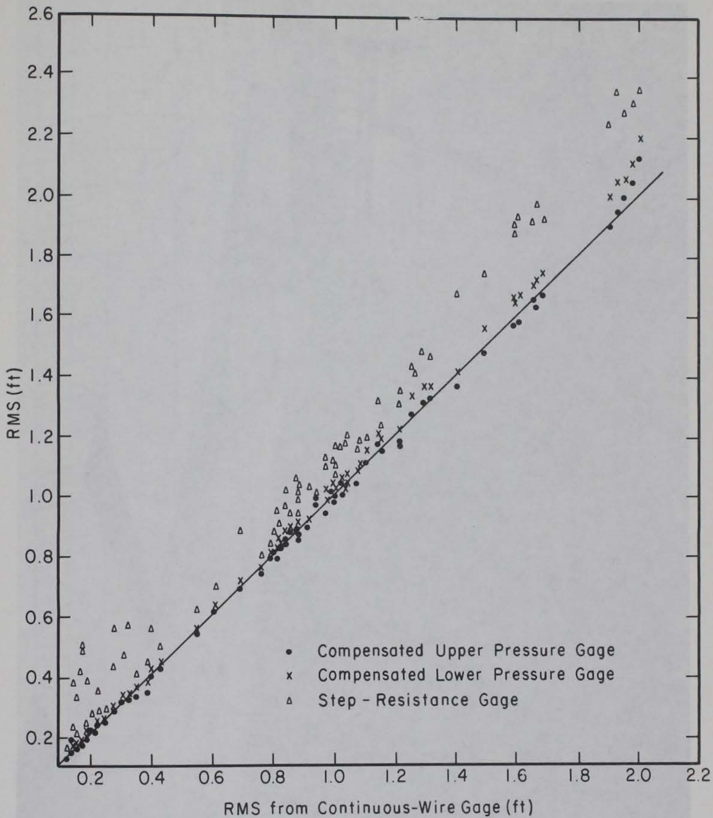
Figure 7. Comparison of root-mean-square (RMS) sea surface elevations from pressure- and step-resistance gage records with those from continuous-wire gage records (Esteva and Harris, 1970).
