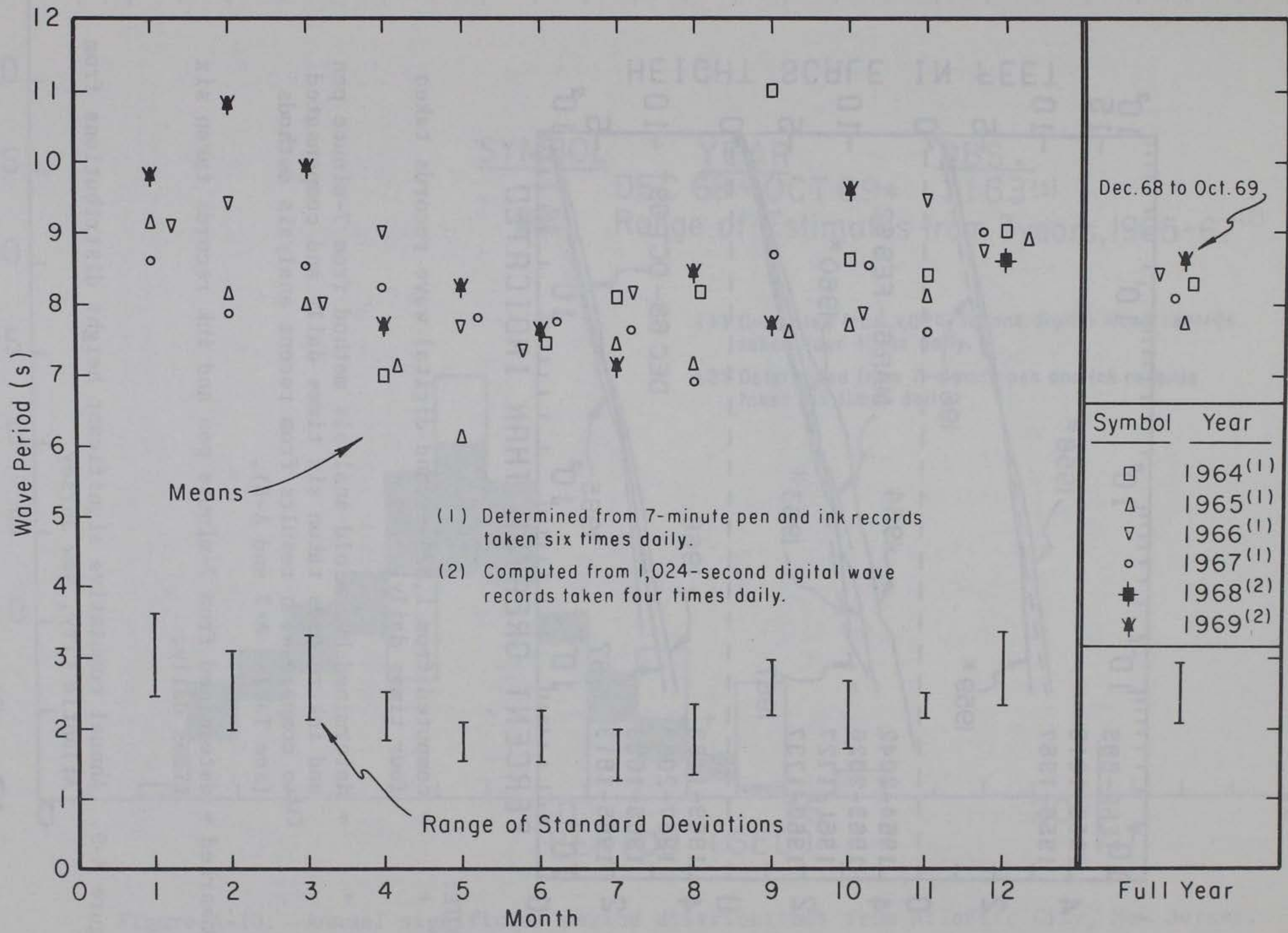
Figure A-8. Means and standard deviations of wave periods for Atlantic City, New Jersey.
