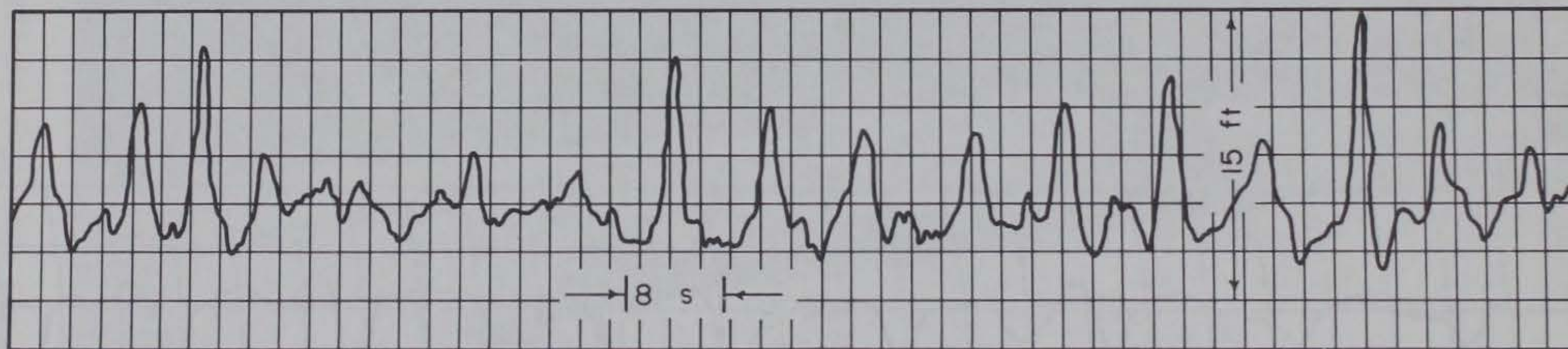
Figure 10. Example of wave record from Wrightsville Beach, North Carolina, at 0100 hours, 27 May 1972.
