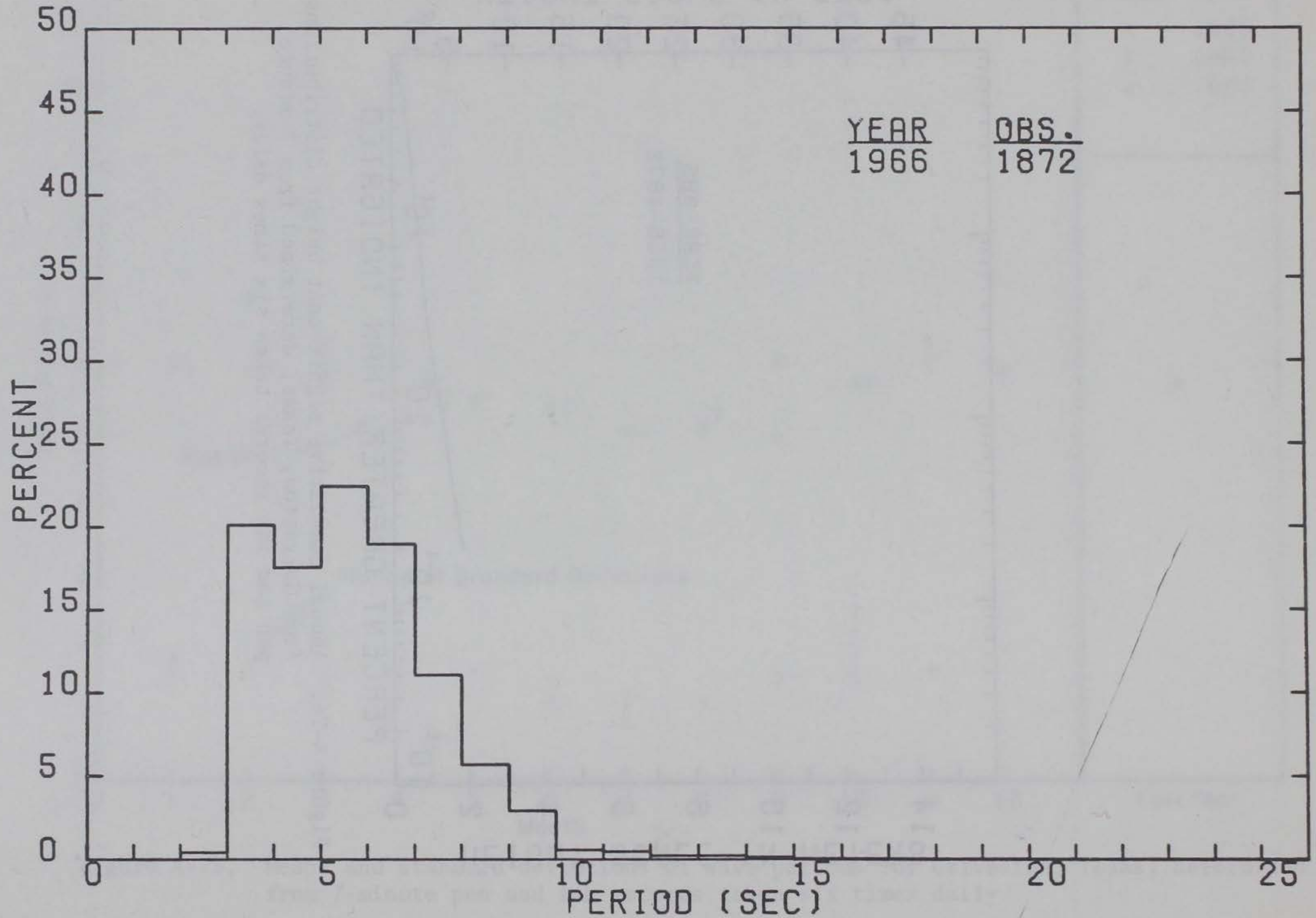
Figure A-77. Annual significant period distributions from Galveston, Texas; determined from 7-minute pen and ink records taken six times daily.
