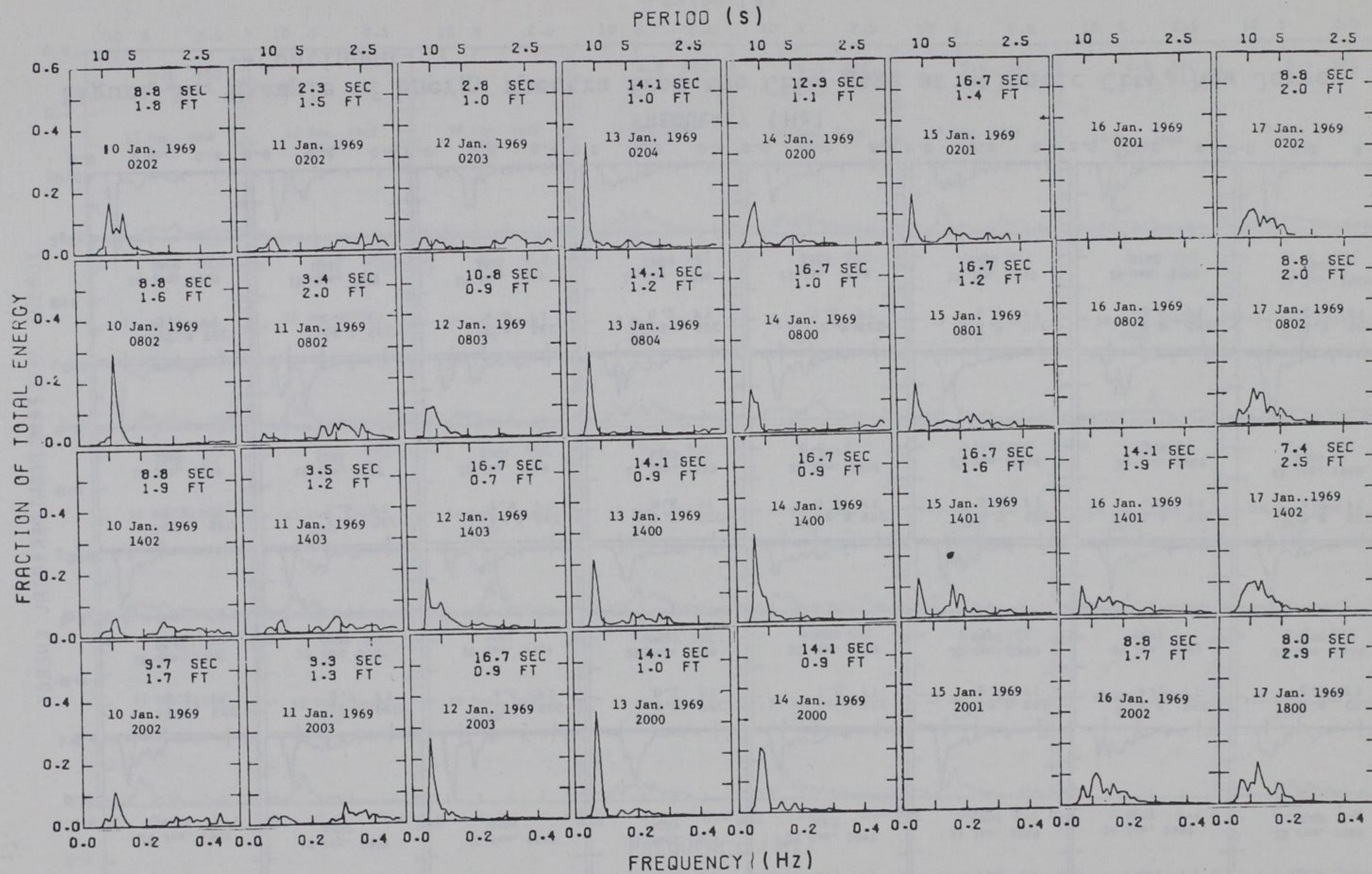
Figure 3. Example of energy spectra from the CERC gage at Atlantic City, New Jersey. Significant wave height and period estimates are given in the upper part of each spectrum.
