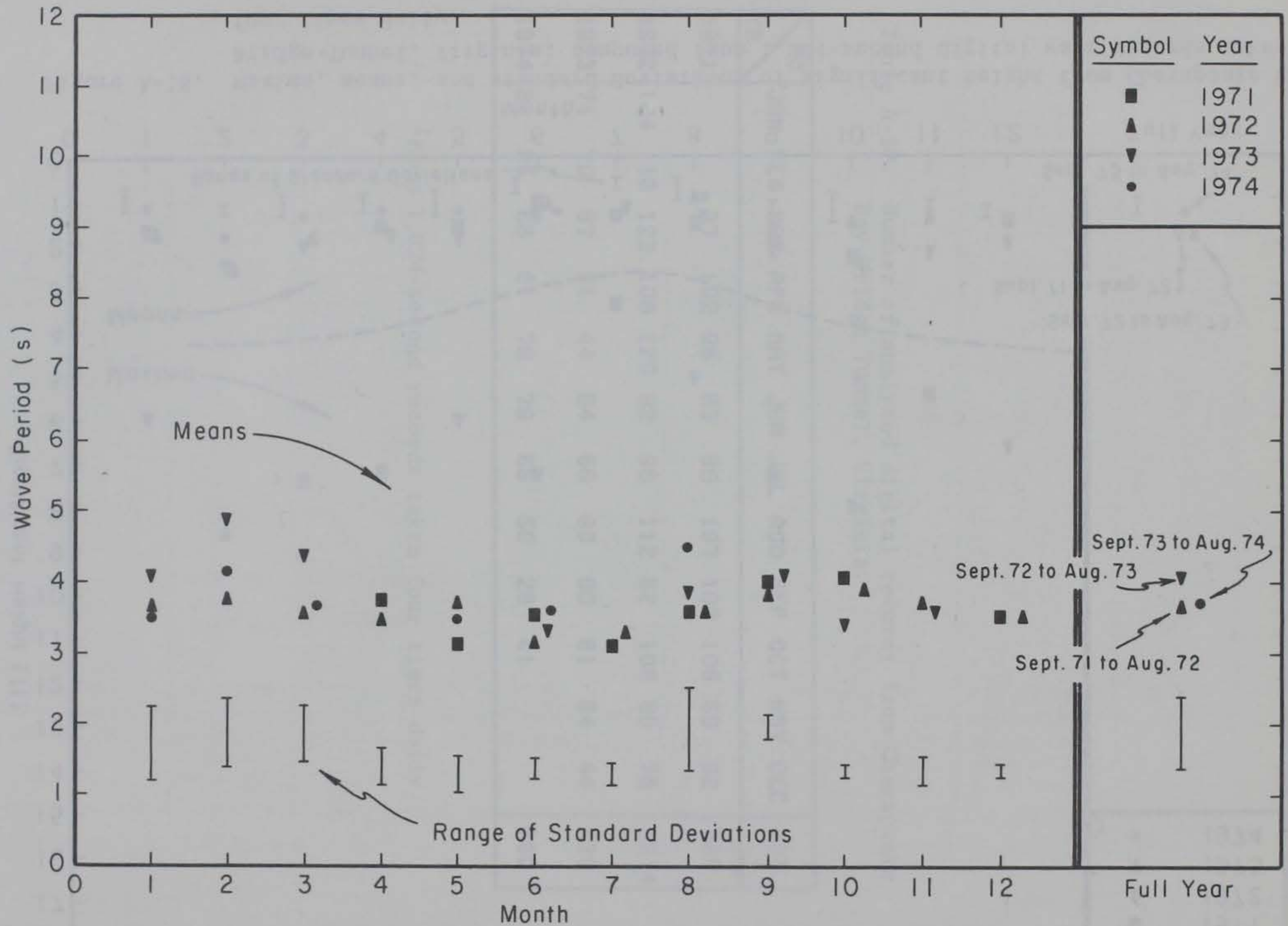
Figure A-19. Means and standard deviations of wave periods for Chesapeake Bay Bridge-Tunnel, Virginia; computed from 1,024-second digital wave records taken four times daily.
