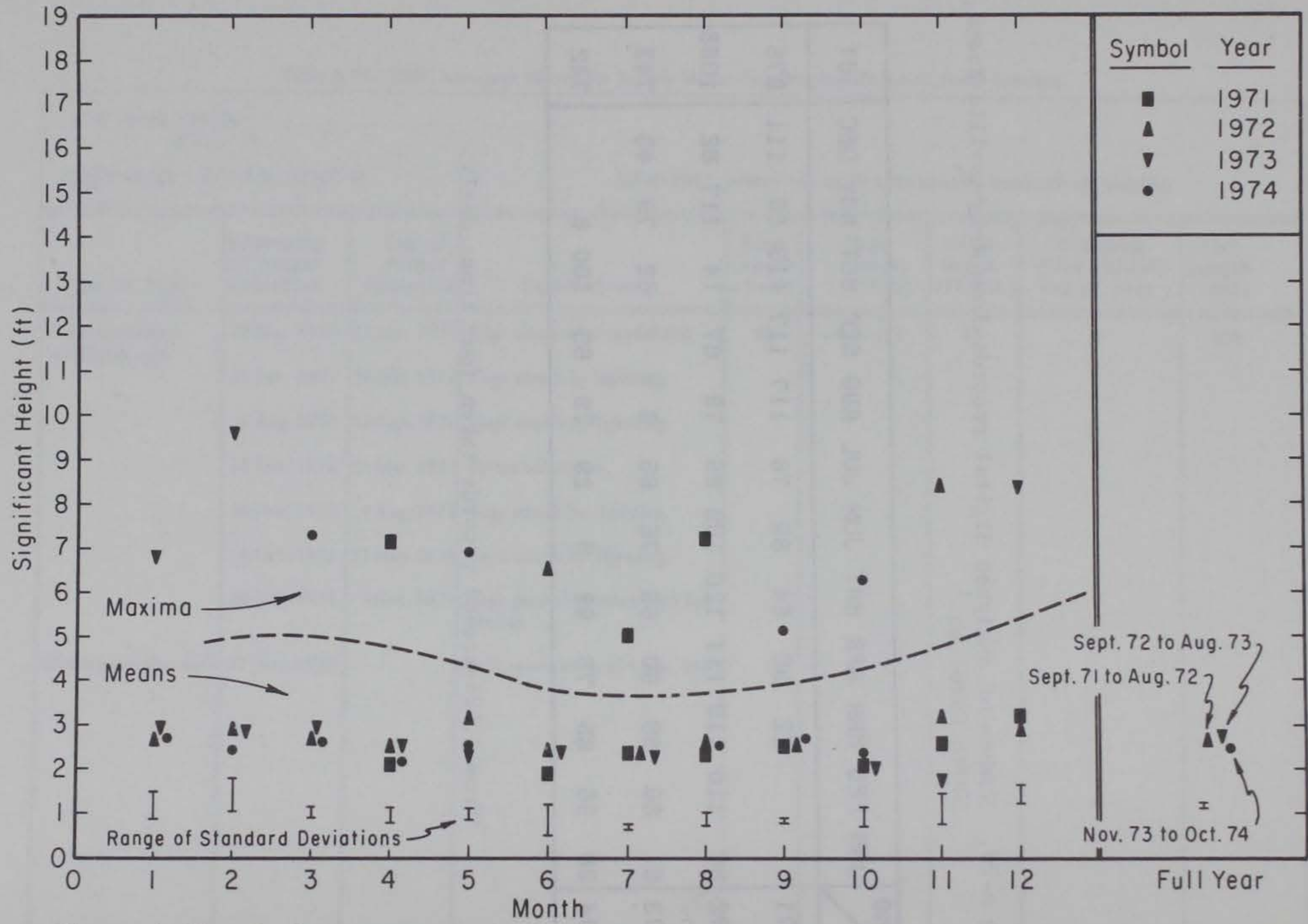
Figure A-33. Maxima, means, and standard deviations of significant height from Wrightsville Beach, North Carolina; computed from 1,024-second digital wave records taken four times daily.
