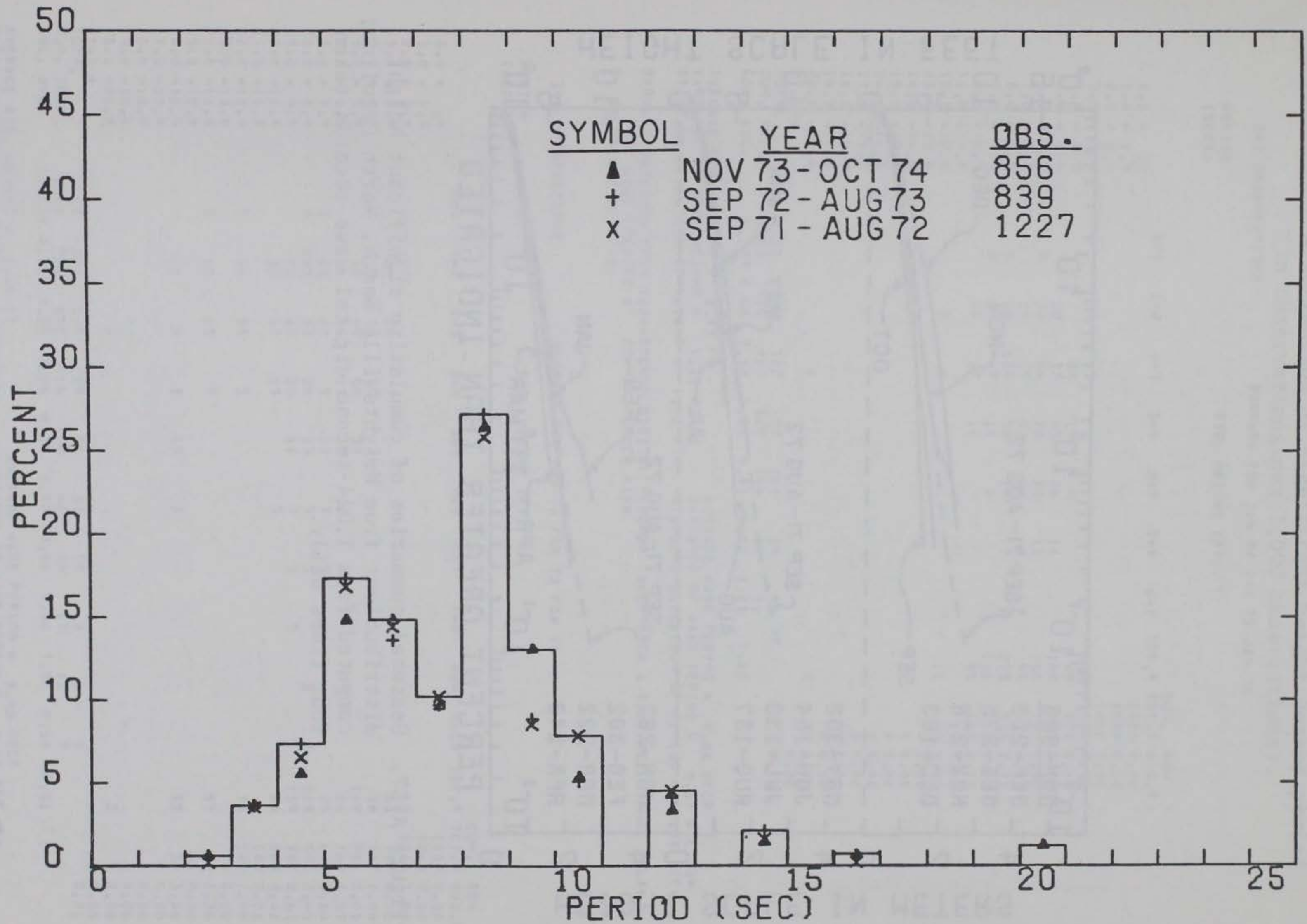
Figure A-36. Annual significant period distributions from Wrightsville Beach, North Carolina; computed from 1,024-second digital wave records taken four times daily.
