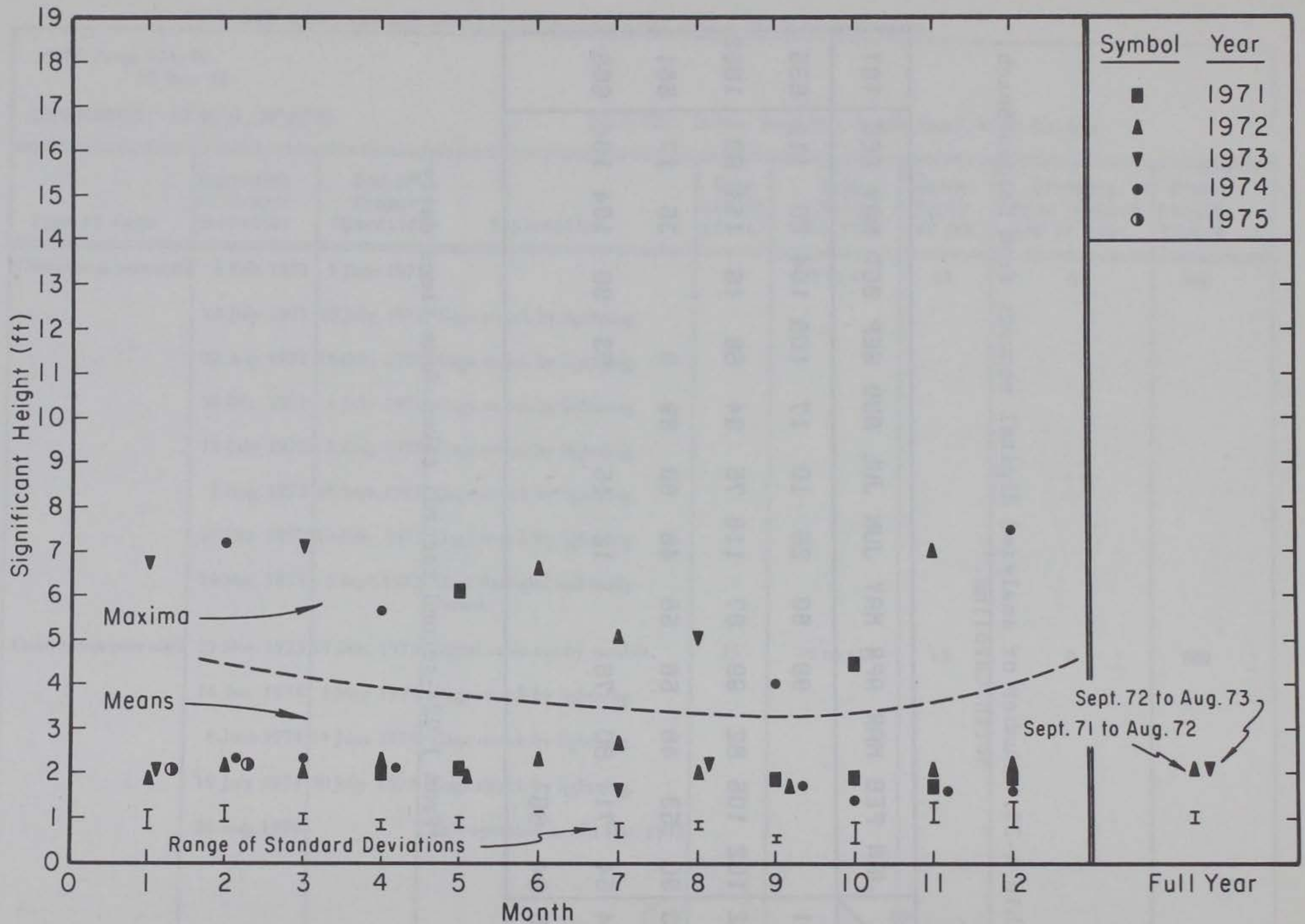
Figure A-38. Maxima, means, and standard deviations of significant height from Holden Beach, North Carolina; computed from 1,024-second digital wave records taken four times daily.
