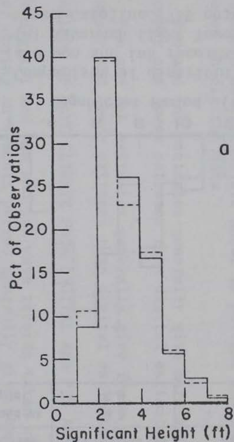
Figure 15. Comparison of distribution functions of significant wave height estimated from digital (solid line) and pen and ink records (dashline) taken during September 1971 to April 1972. (a) Savannah Light Tower, Georgia (499 observations); (b) Wrightsville Beach, North Carolina (764 observations).
