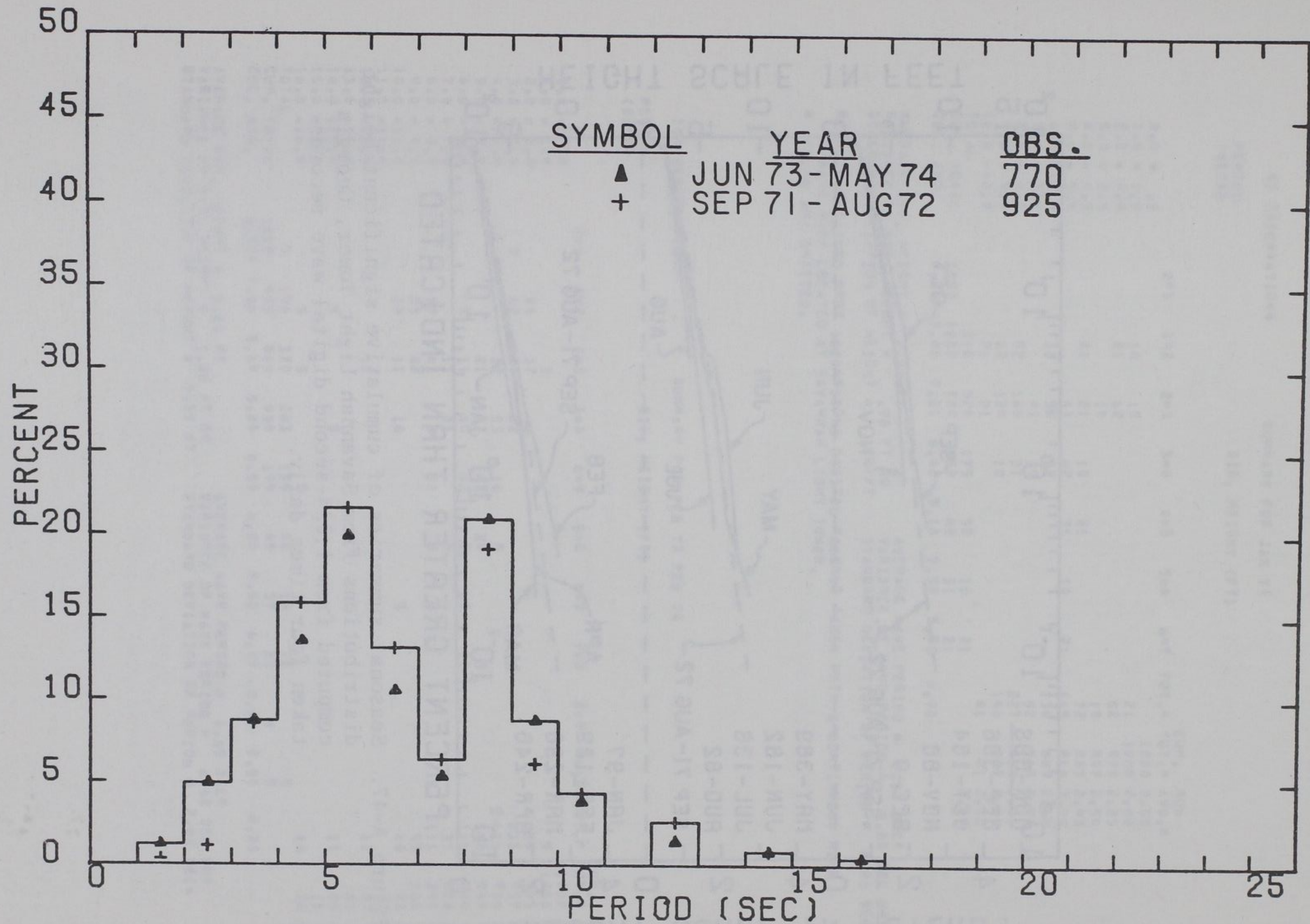
Figure A-46. Annual significant period distributions from Savannah Light Tower, Georgia; computed from 1,024-second digital wave records taken four times daily.
