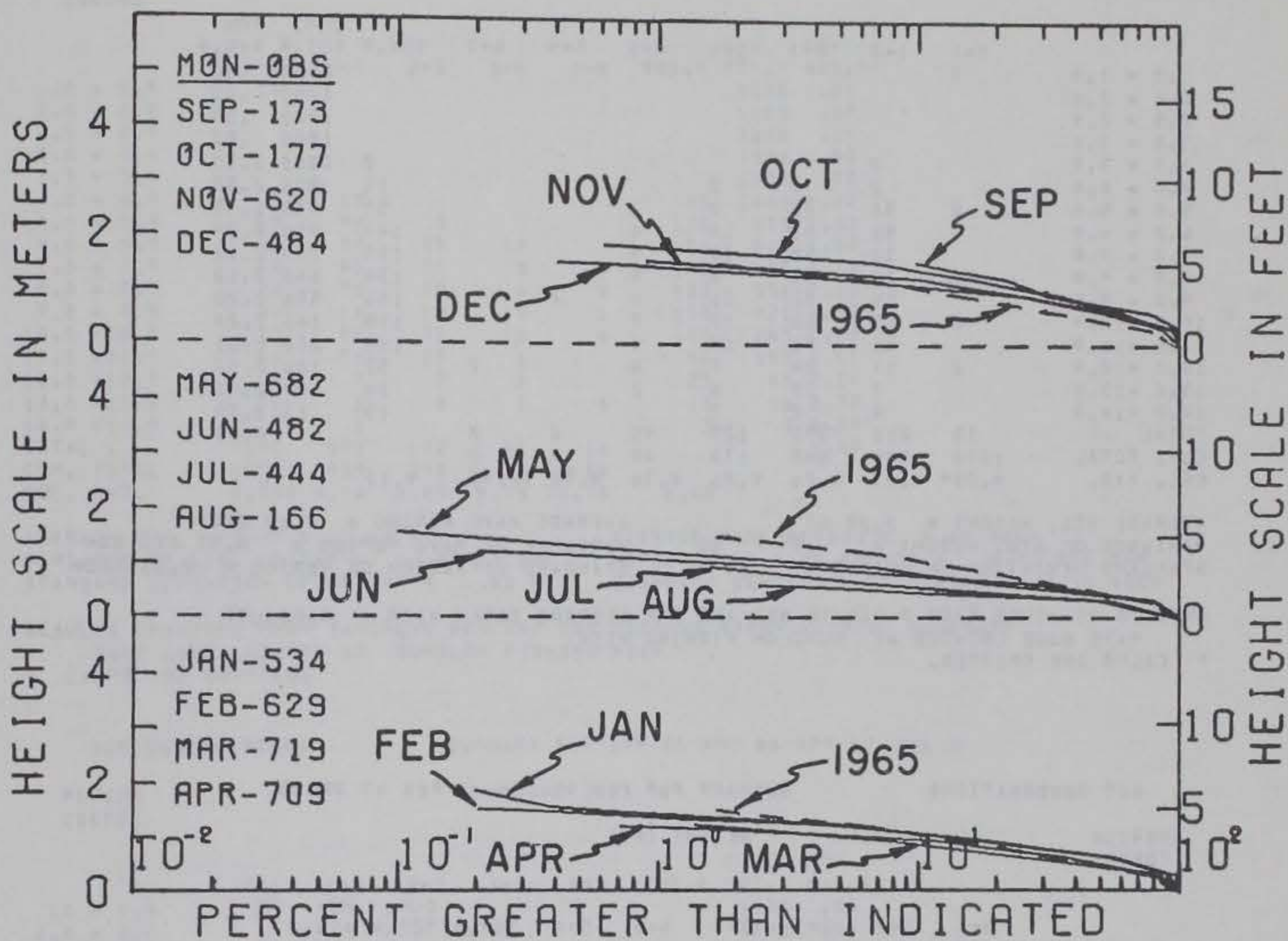
Figure A-52. Seasonal summaries of cumulative significant height distributions from Daytona Beach, Florida; determined from 7-minute pen and ink records taken six times daily.
