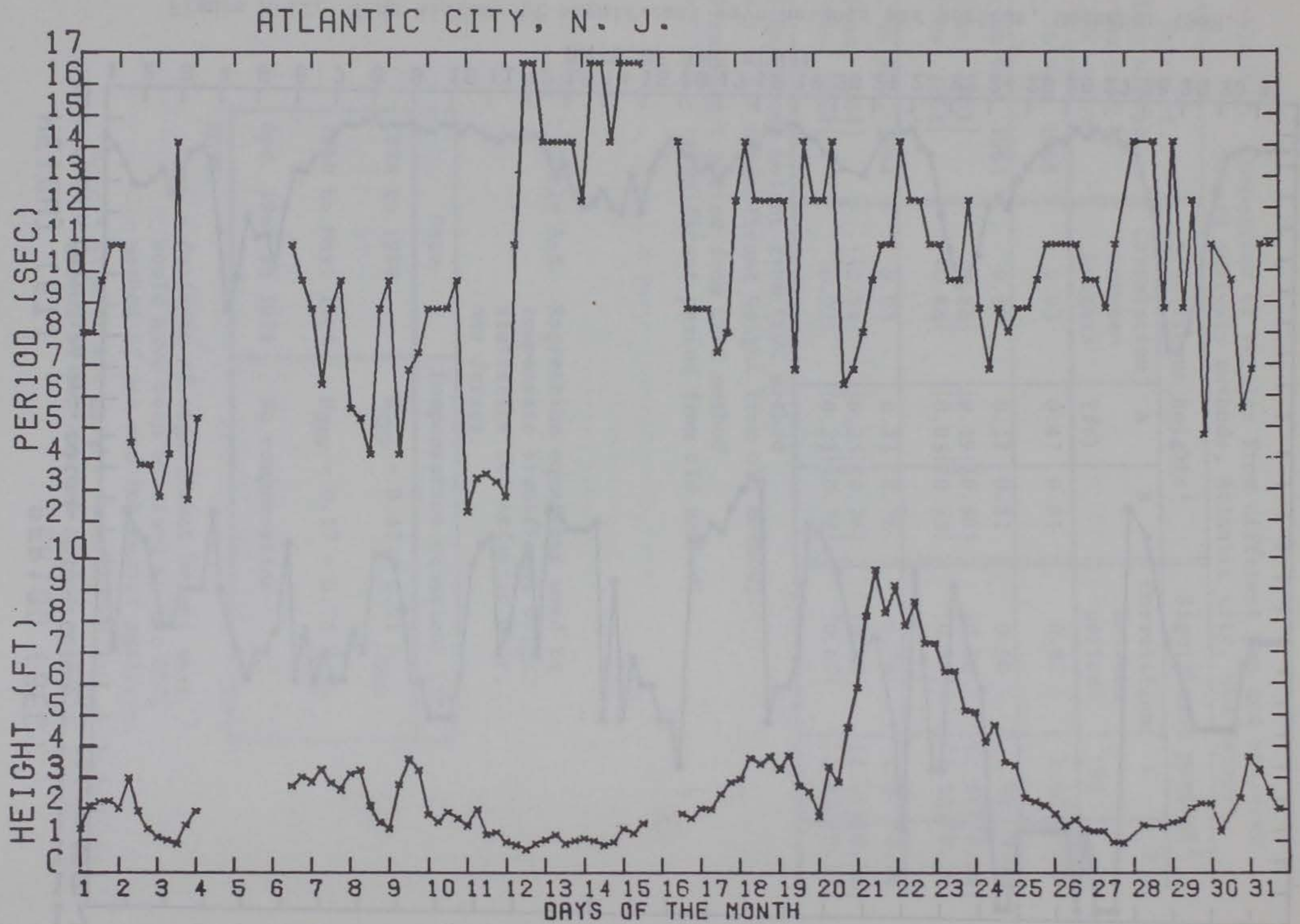
Figure A-13. Time history of significant wave heights and periods, January 1969.
