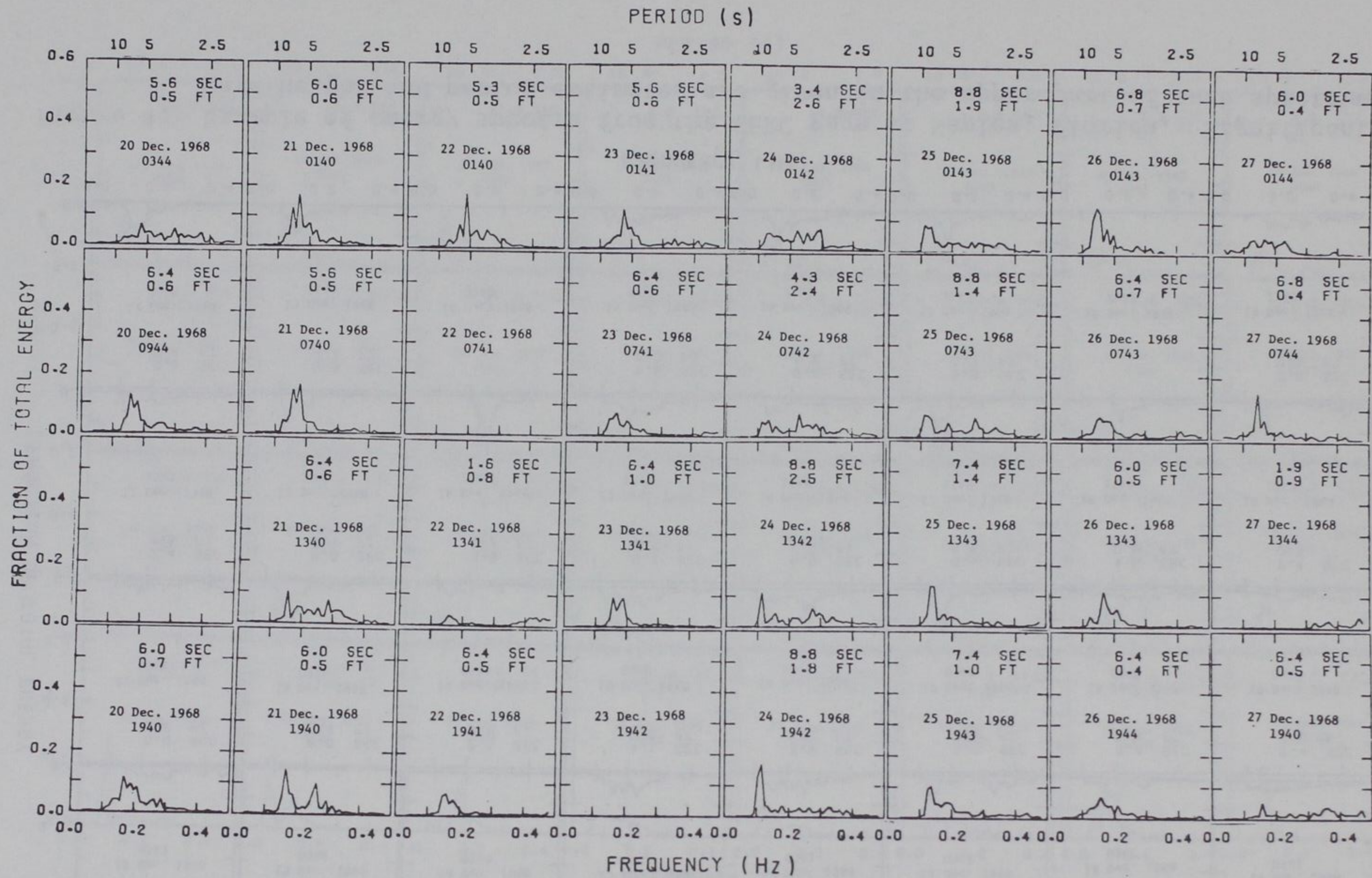
Figure 4. Example of energy spectra from the CERC gage at Naples, Florida.--Continued
