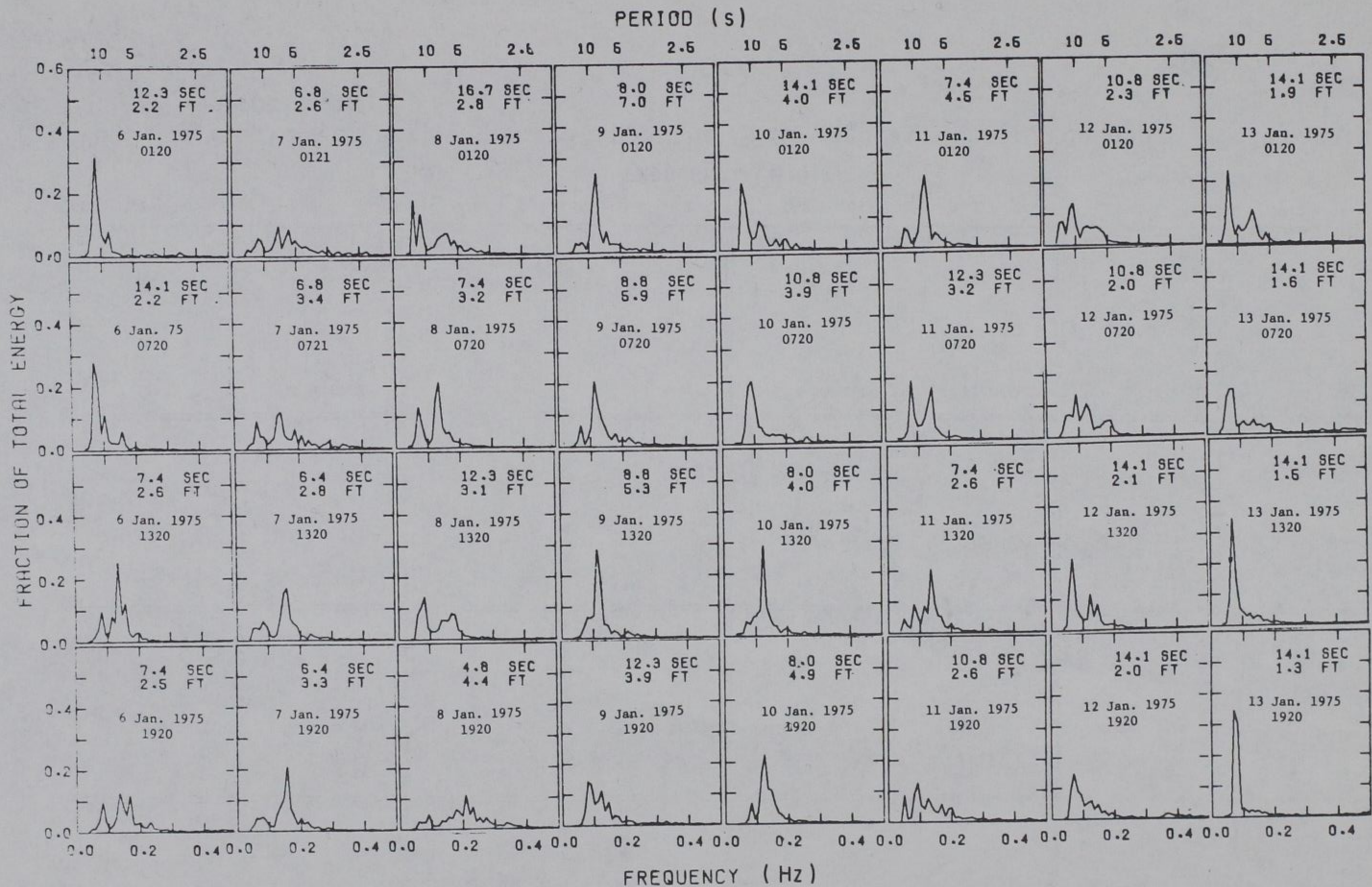
Figure 5. Example of energy spectra from the CERC gage at Huntington Beach, California. Significant wave height and period estimates are given in the upper part of each spectrum.
