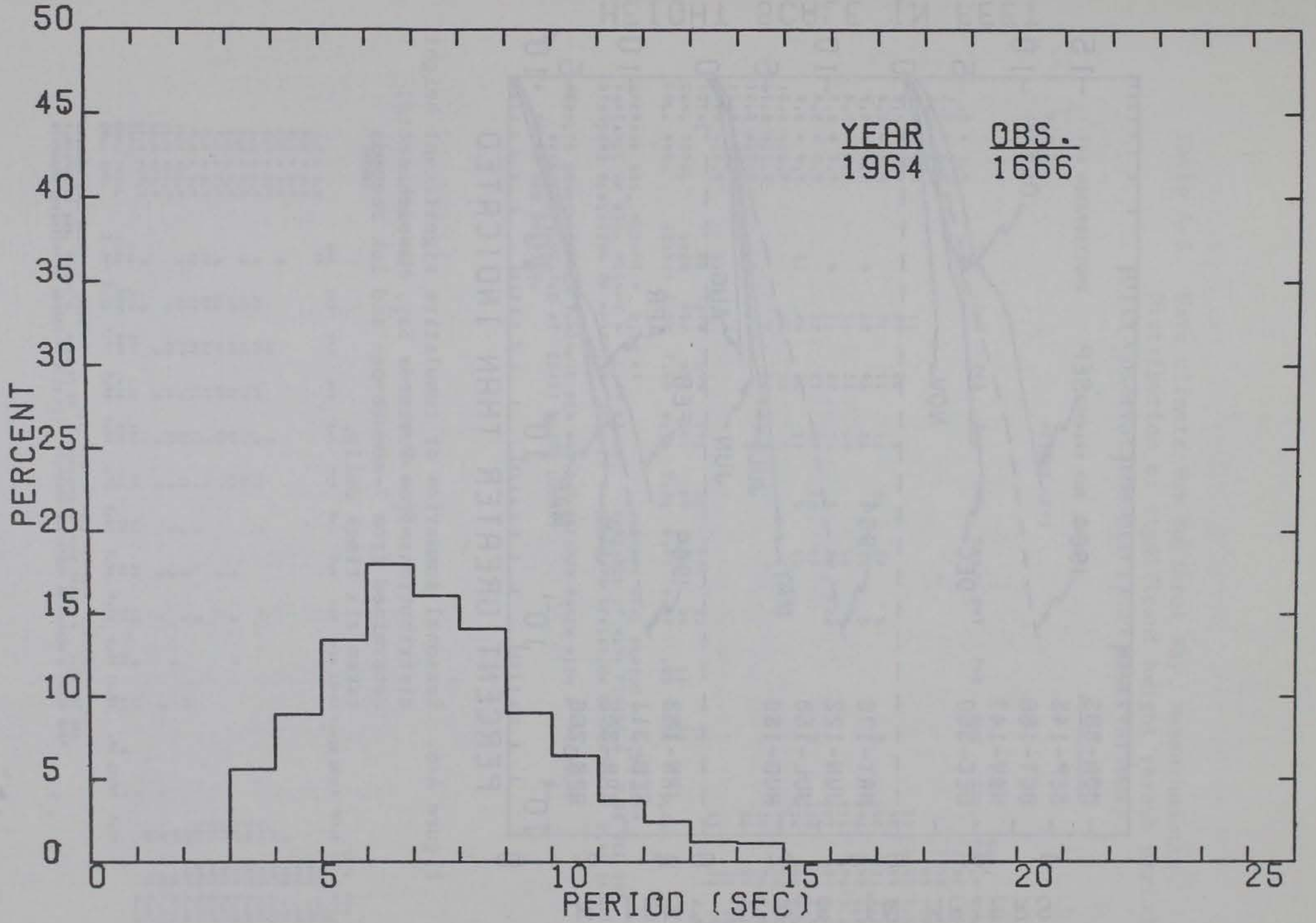
Figure A-5. Annual significant period distributions from Buzzards Bay, Massachusetts; determined from 7-minute pen and ink records taken six times daily.
