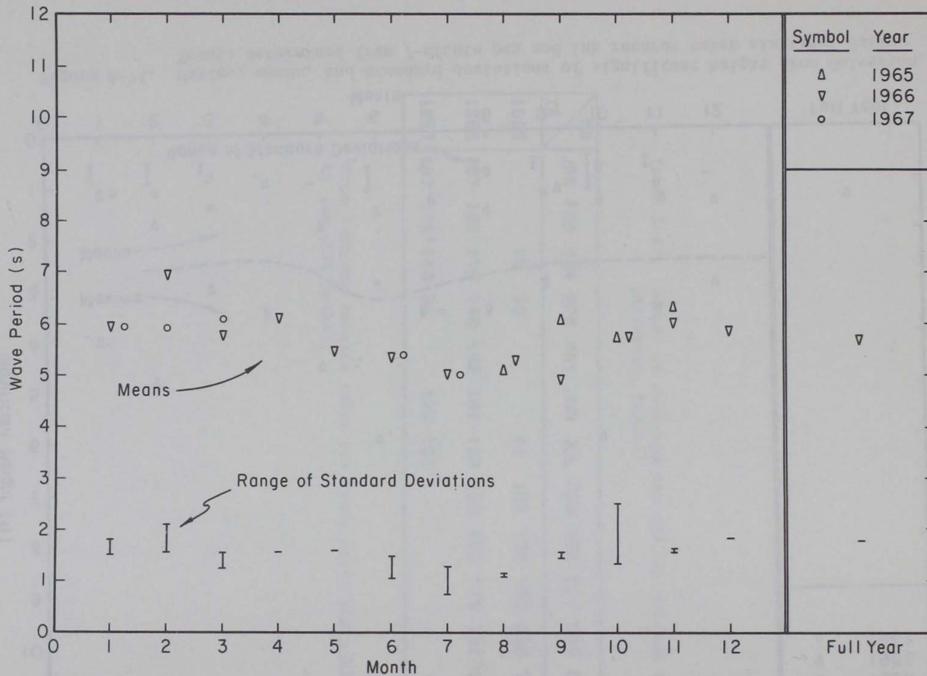
Figure A-75. Means and standard deviations of wave periods for Galveston, Texas; determined from 7-minute pen and ink records taken six times daily.
