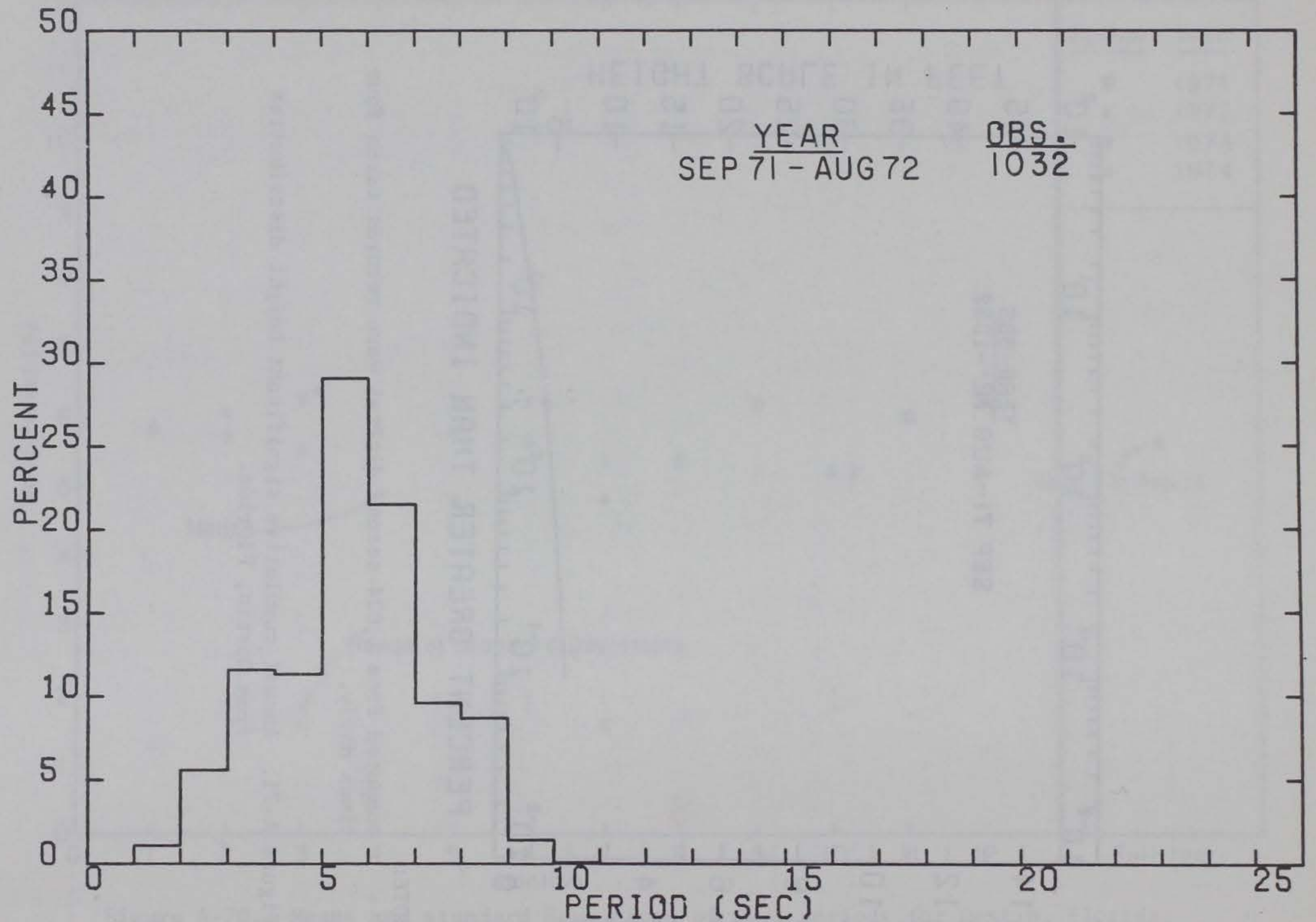
Figure A-72. Annual significant period distributions from Destin, Florida; computed from 1,024-second digital wave records taken four times daily.
