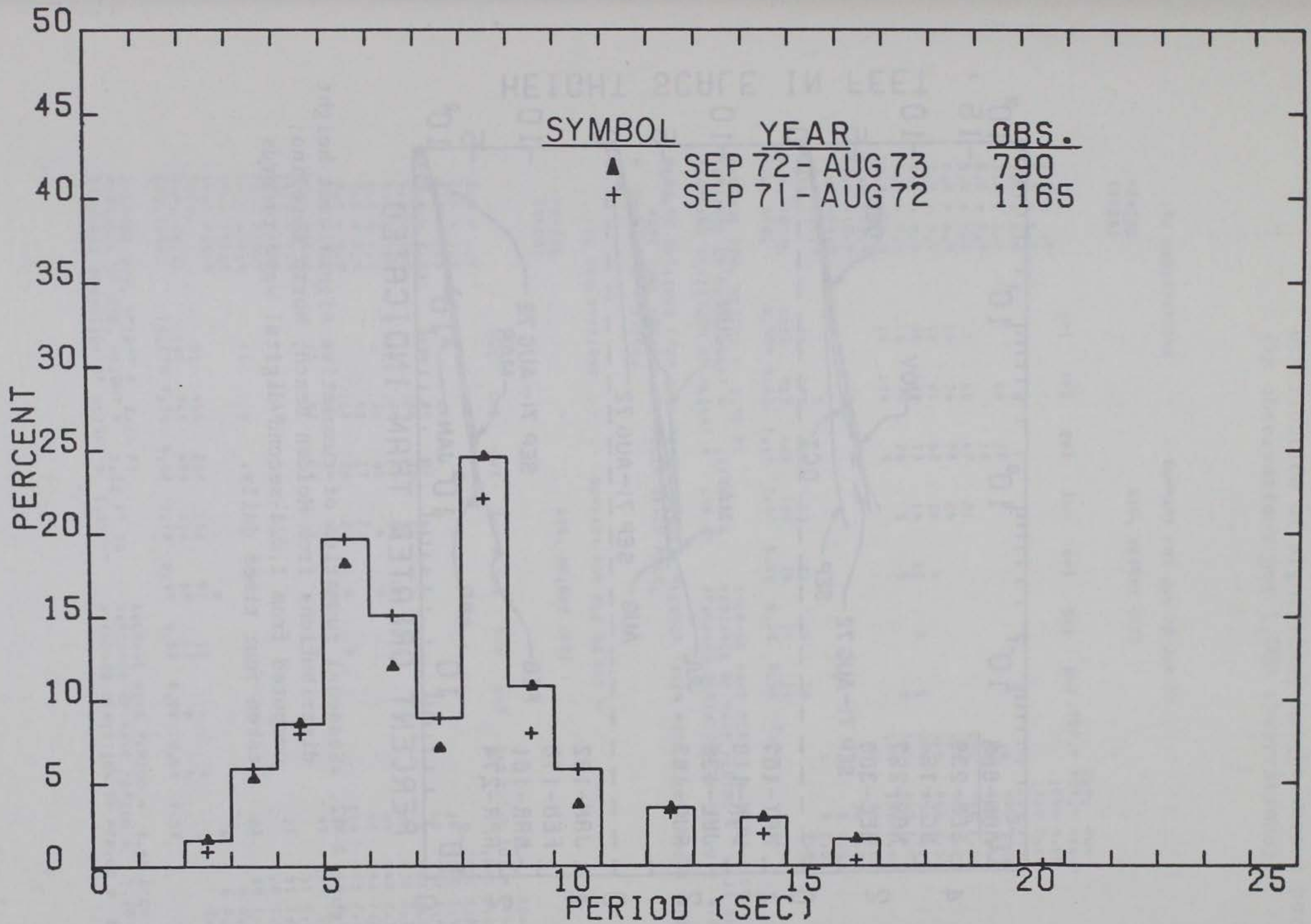
Figure A-41. Annual significant period distributions from Holden Beach, North Carolina; computed from 1,024-second digital wave records taken four times daily.
