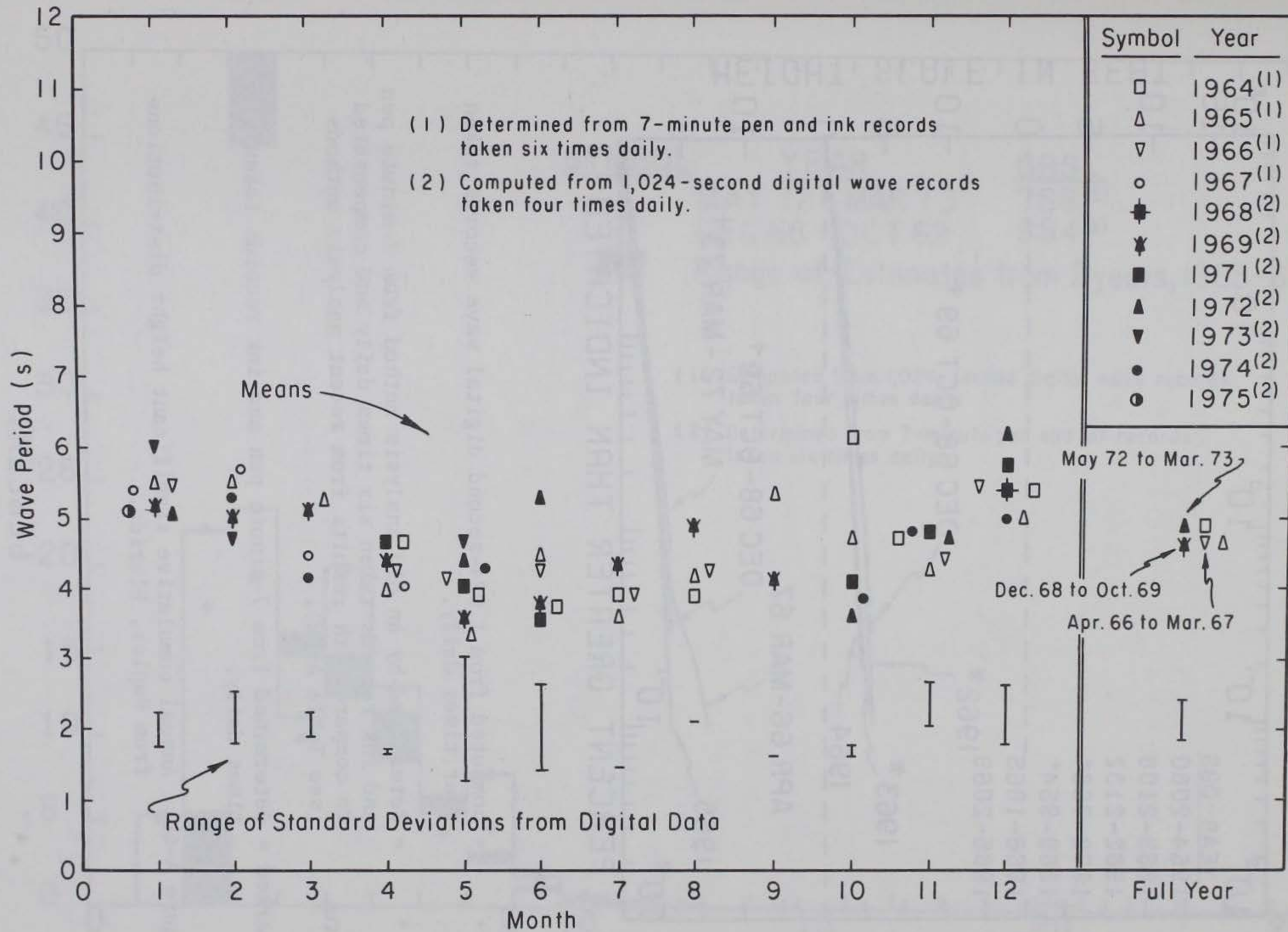
Figure A-65. Means and standard deviations of wave periods for Naples, Florida.
