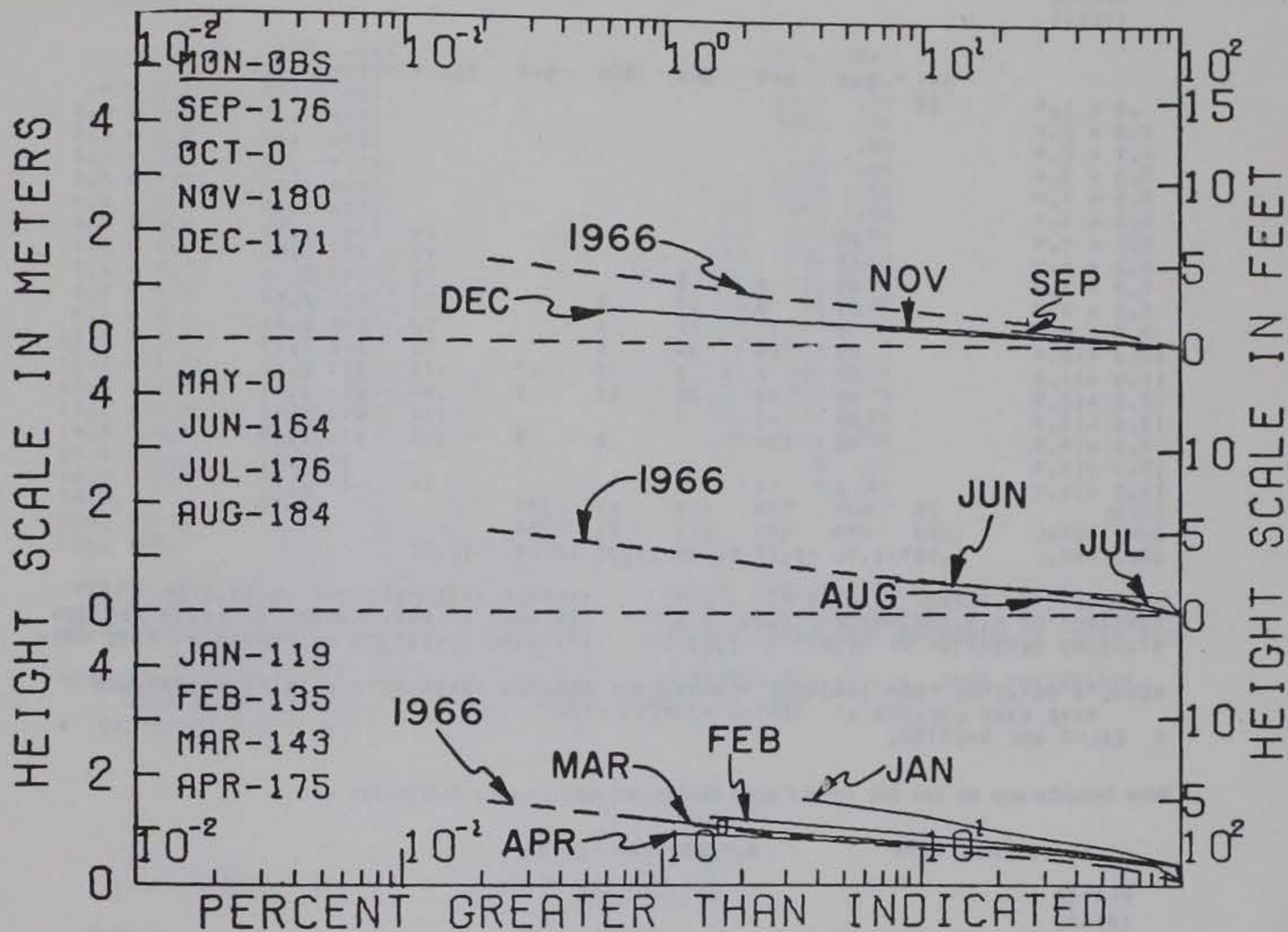
Figure A-102. Seasonal summaries of cumulative significant height distributions from Venice, California. Determined from 7-minute pen and ink records taken six times daily. Wave heights may be low due to old gage design and maintenance difficulties.
