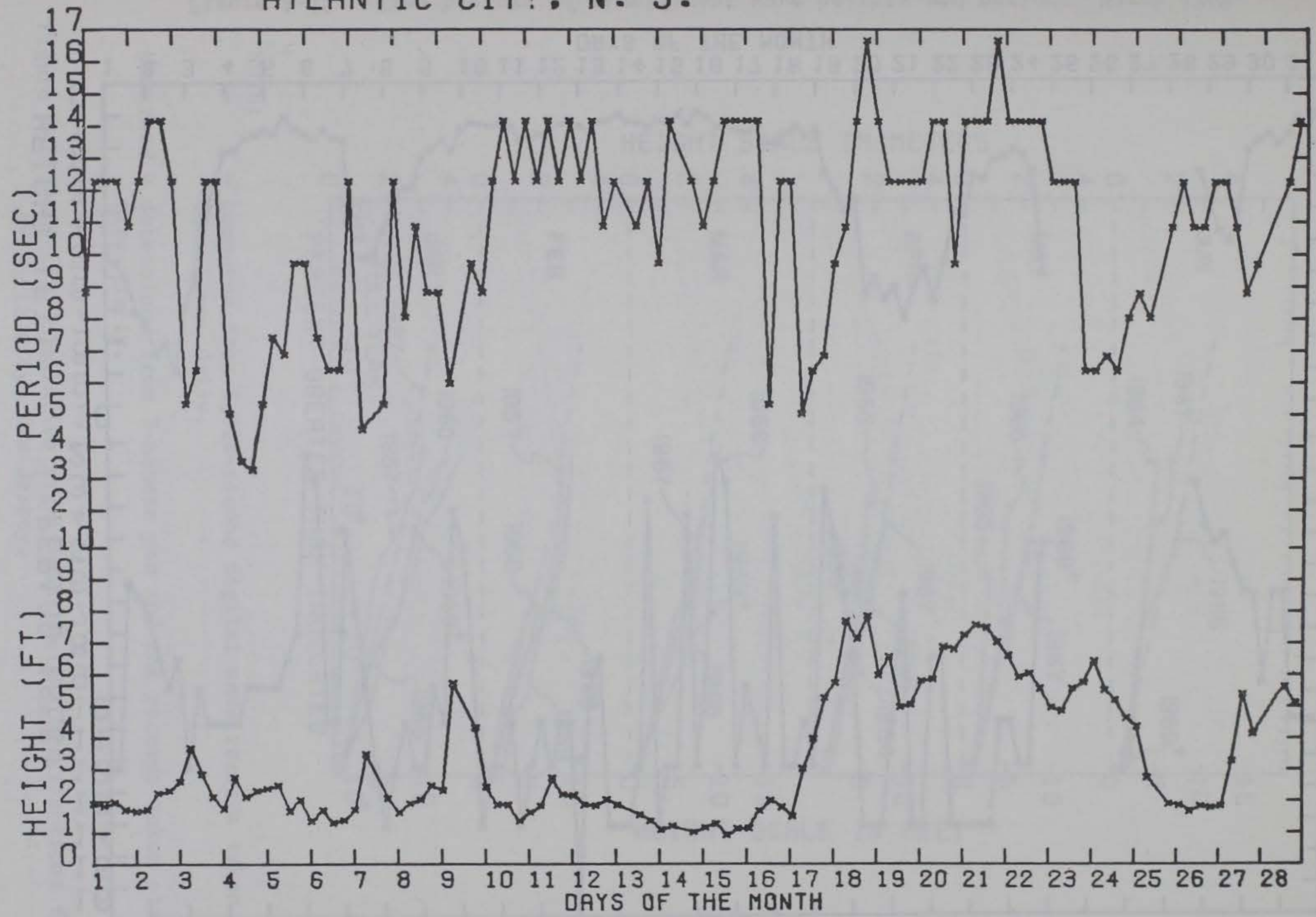
Figure A-14. Time history of significant wave heights and periods, February 1969.
