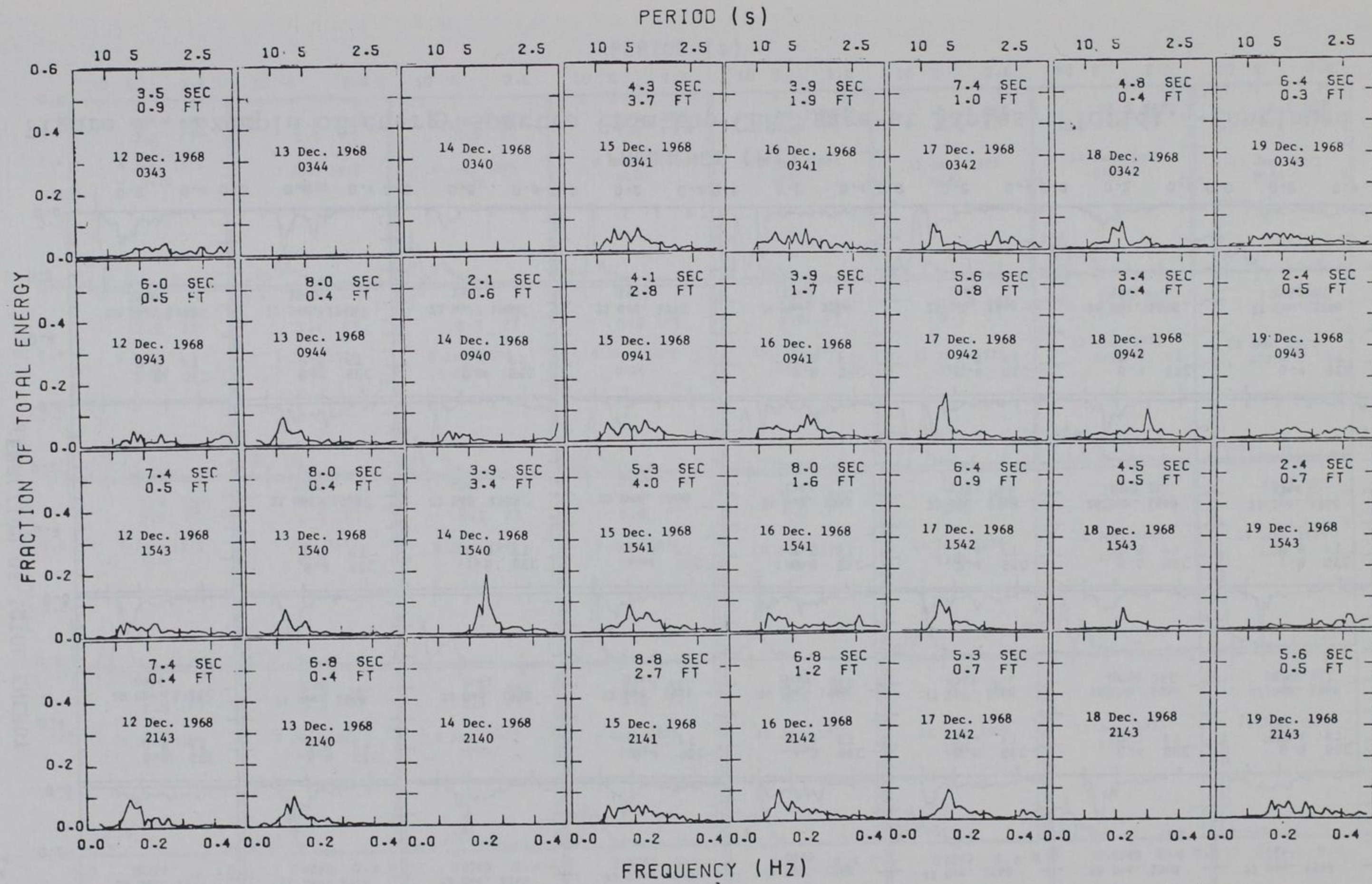
Figure 4. Example of energy spectra from the CERC gage at Naples, Florida. Significant wave height and period estimates are given in the upper part of each spectrum.
