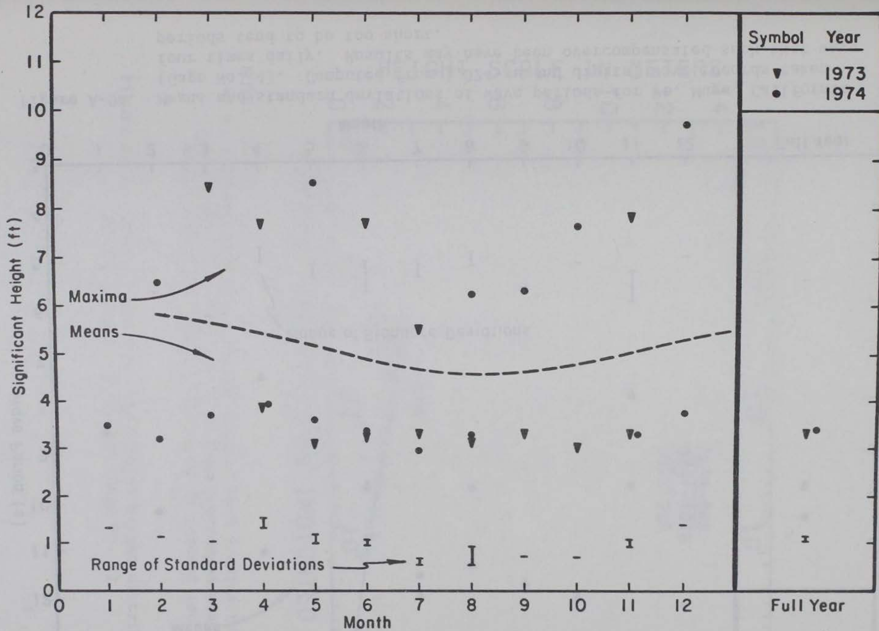
Figure A-93. Maxima, means, and standard deviations of significant height from Pt. Mugu, California (Gage No. 4). Computed from 1,024-second digital wave records taken four times daily. Results may have been overcompensated such that significant heights are up to 20 percent too high.
