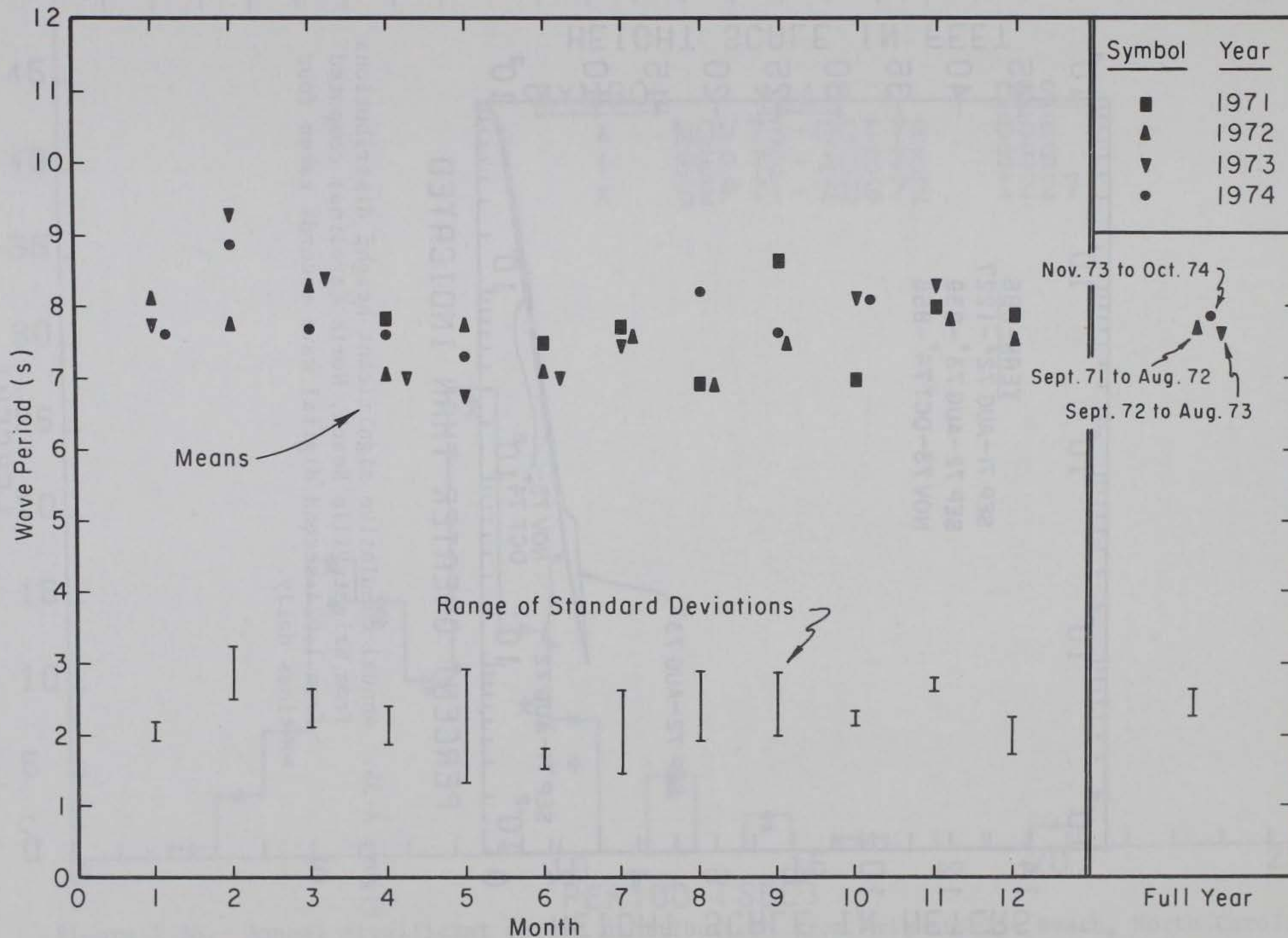
Figure A-34. Means and standard deviations of wave periods for Wrightsville Beach, North Carolina; computed from 1,024-second digital wave records taken four times daily.
