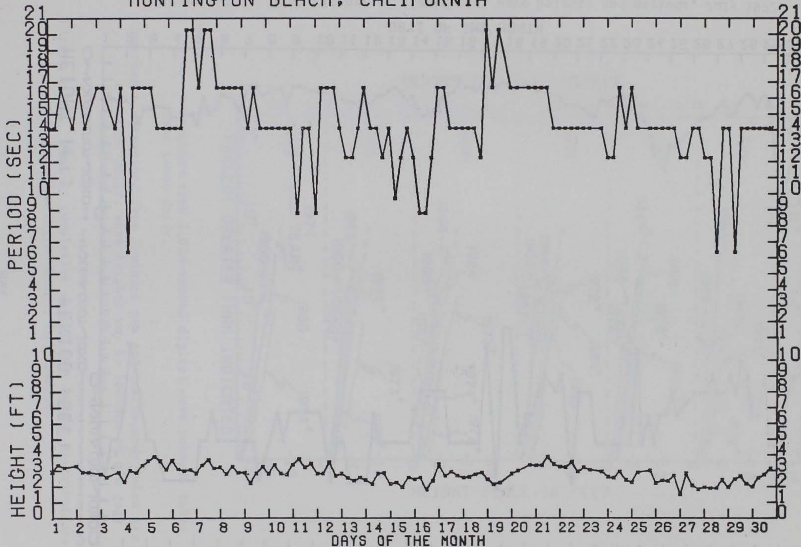
Figure A-110. Time history of significant wave heights and periods, June 1972.
