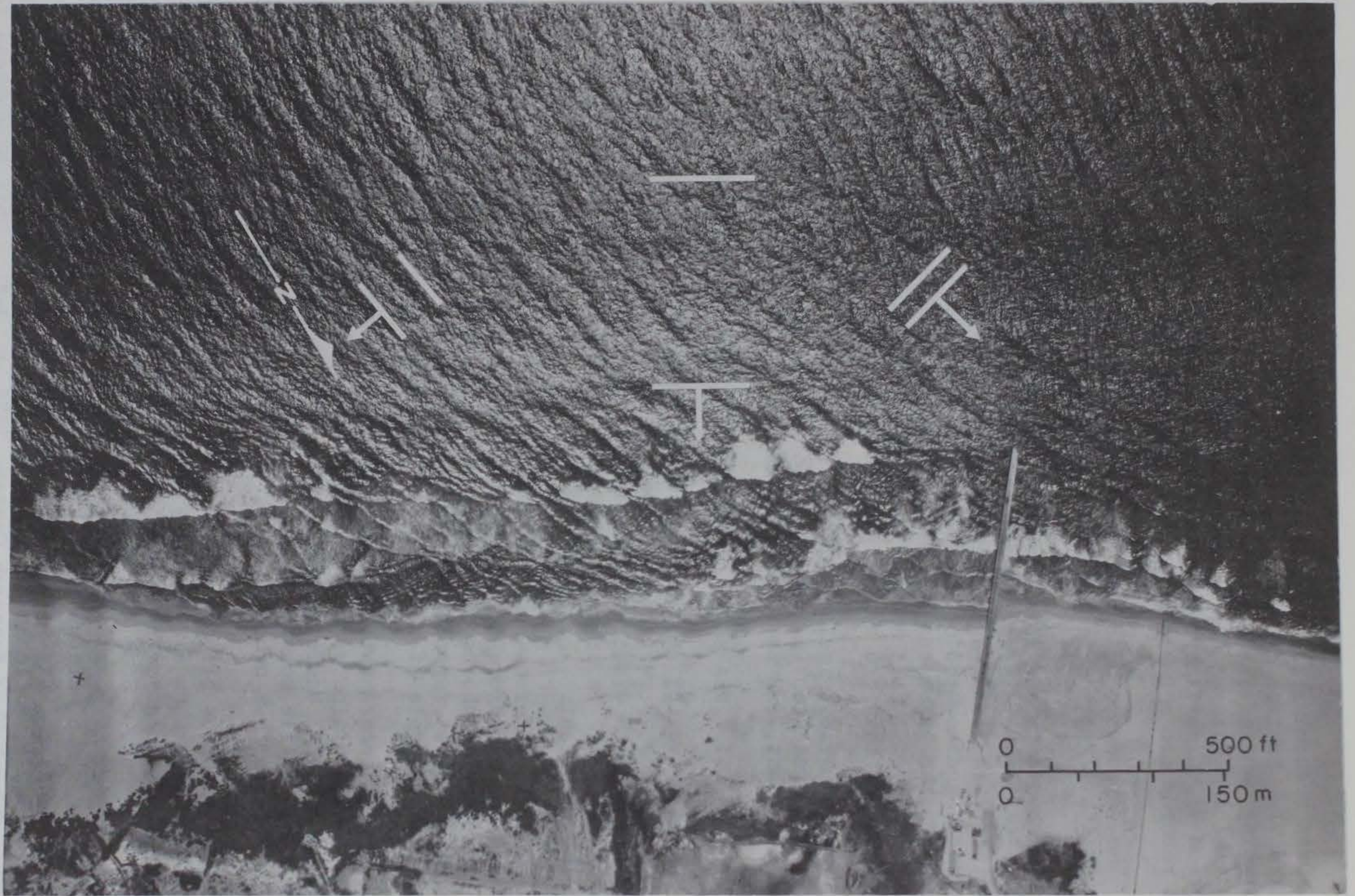
Figure 2. Aerial photo of several wave trains along the California coast north of Pt. Mugu, at 1300 hours, 9 August 1973.
