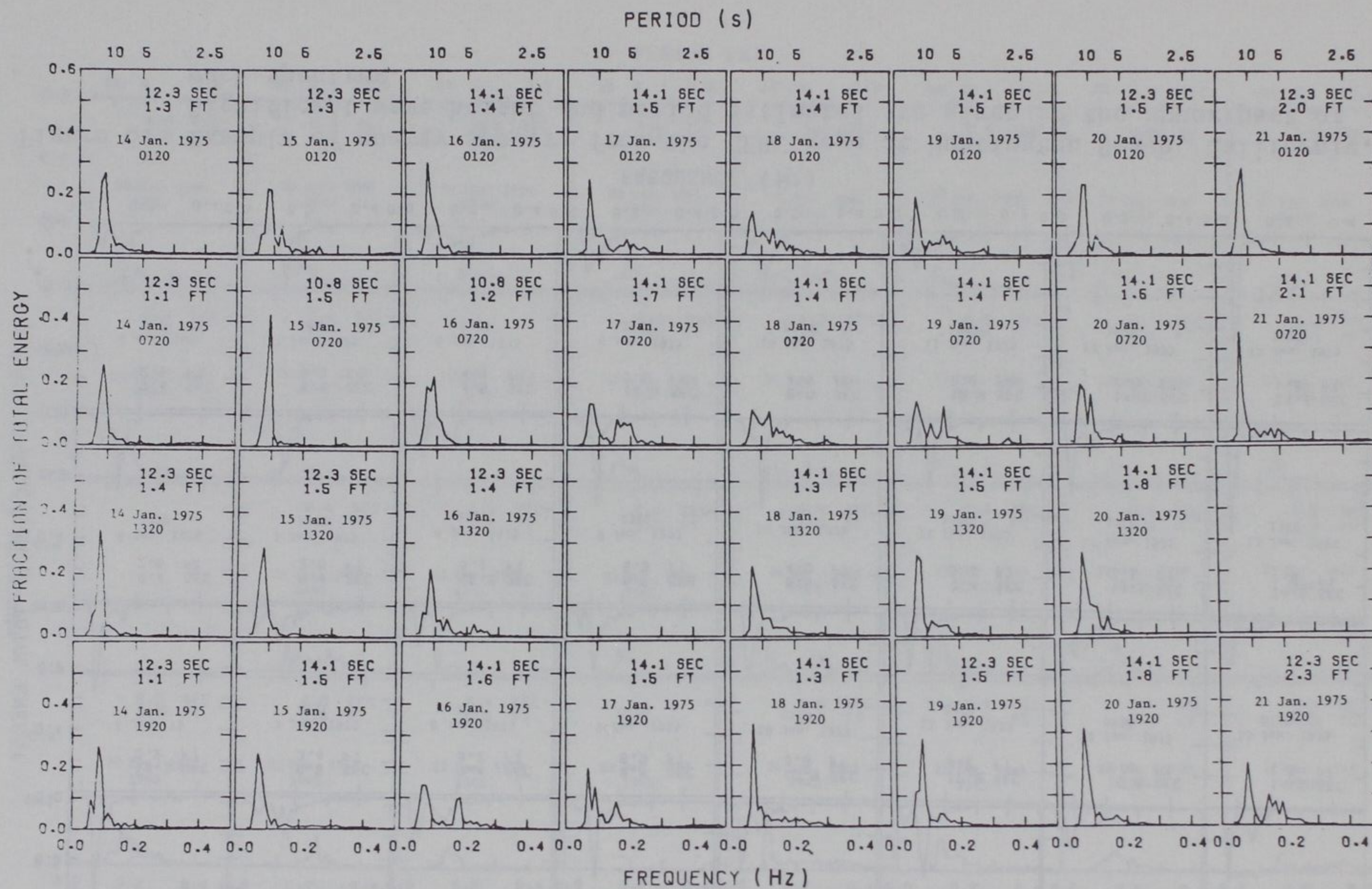
Figure 5. Example of energy spectra from the CERC gage at Huntington Beach, California. --Continued
