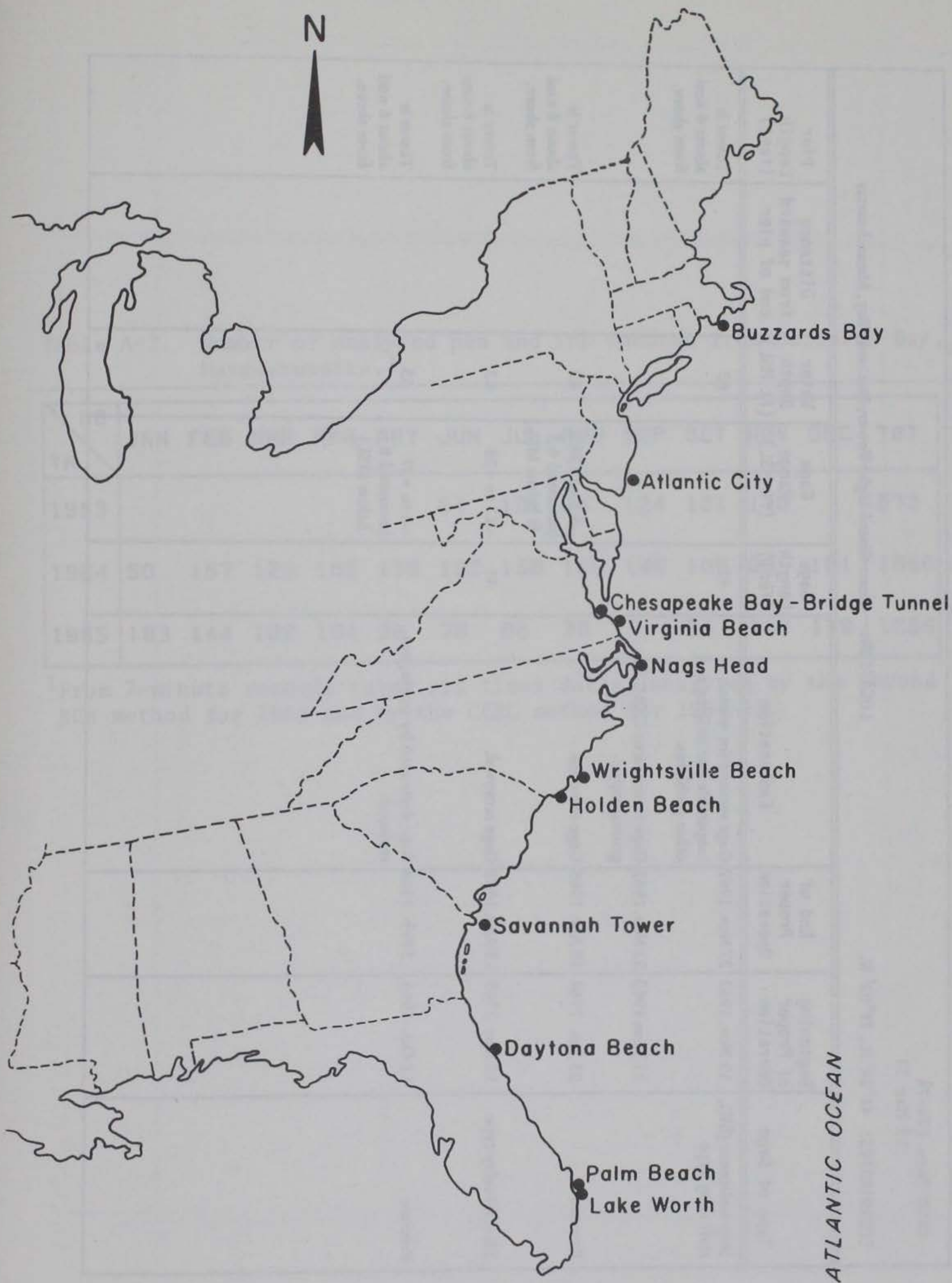
Figure A-1. Location of BEB-CERC wave gages along the U.S. Atlantic coast.
