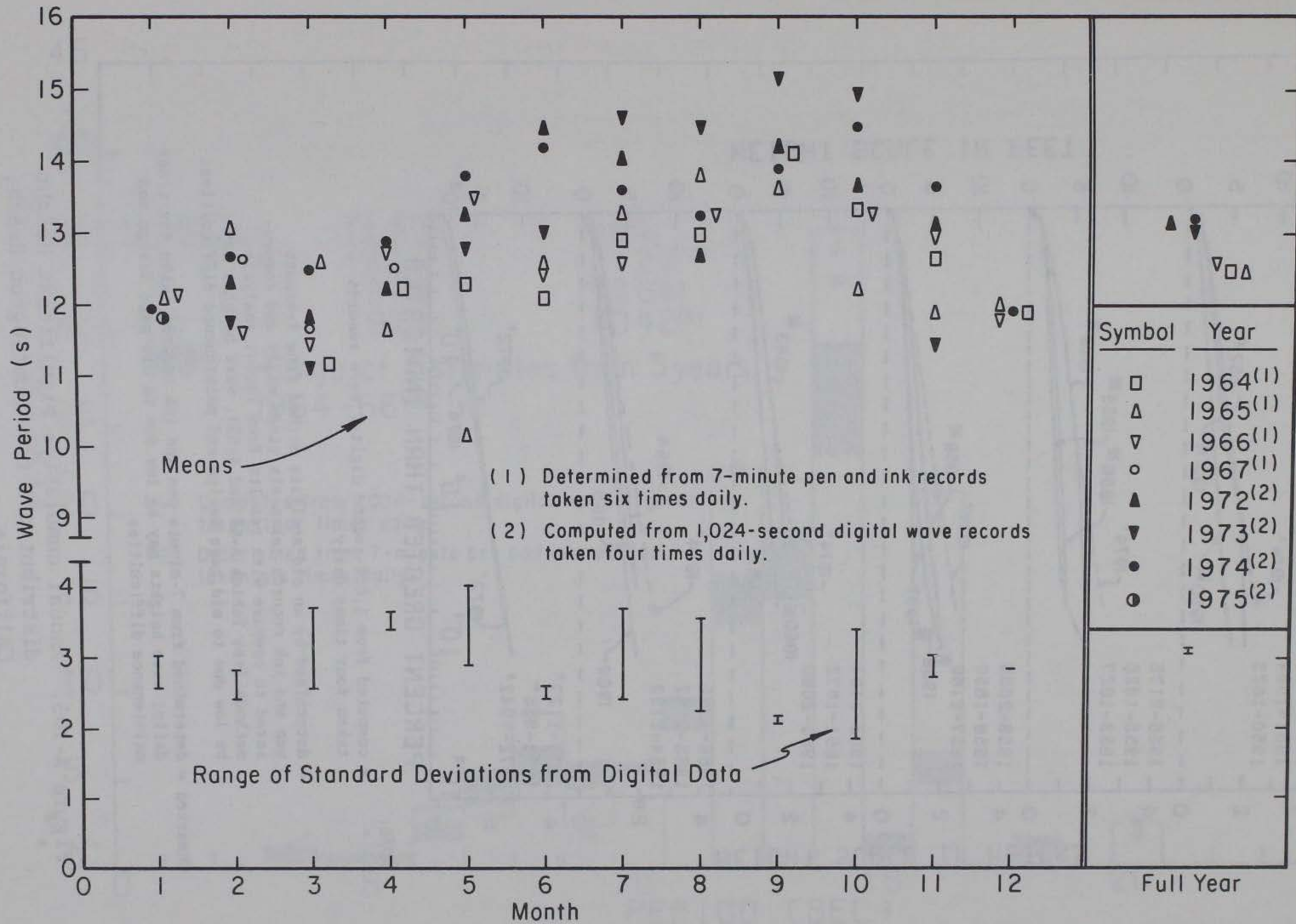
Figure A-104. Means and standard deviations of wave periods for Huntington Beach, California.
