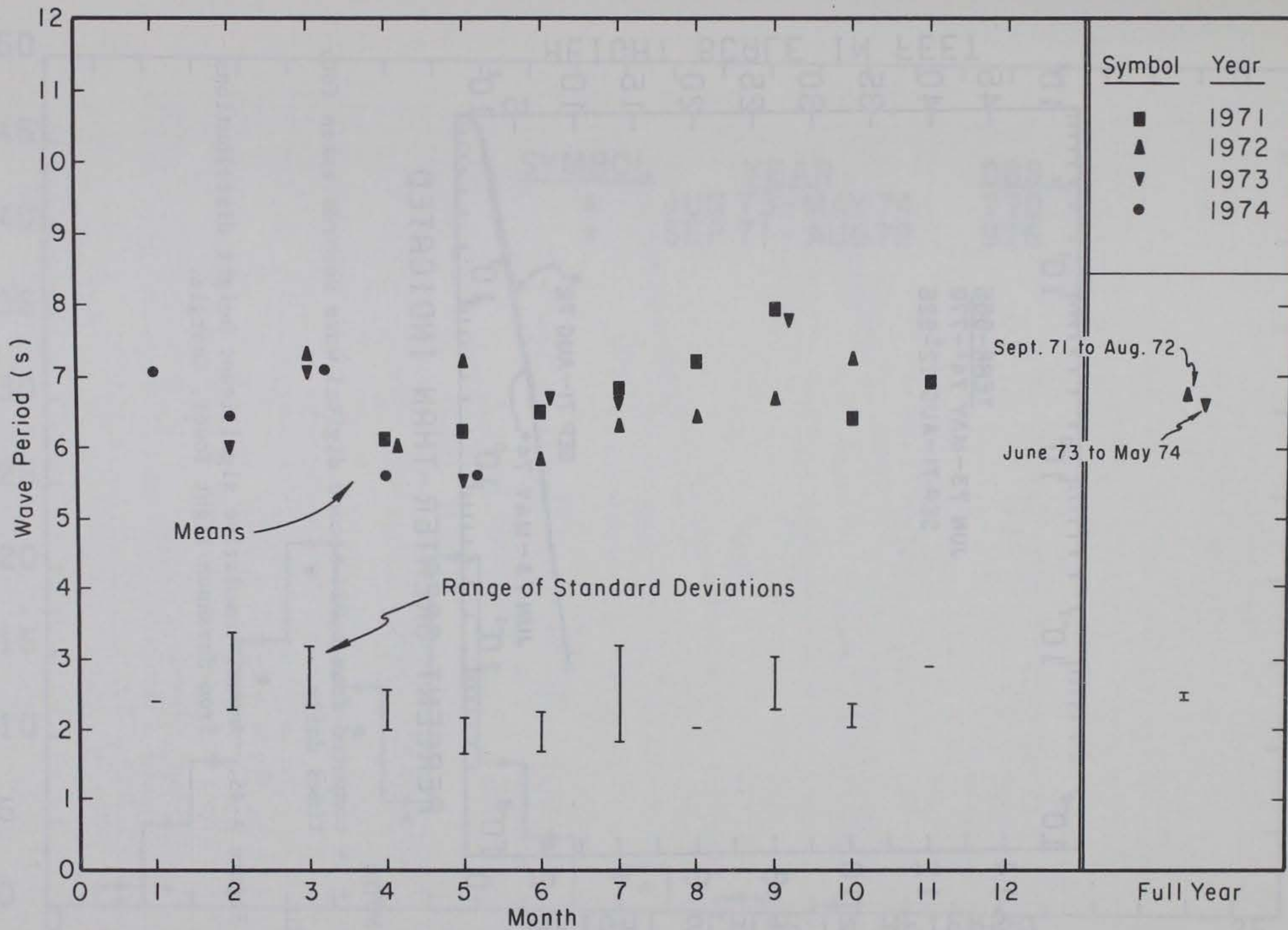
Figure A-44. Means and Standard deviations of wave periods for Savannah Light Tower, Georgia; computed from 1,024-second digital wave records taken four times daily.
