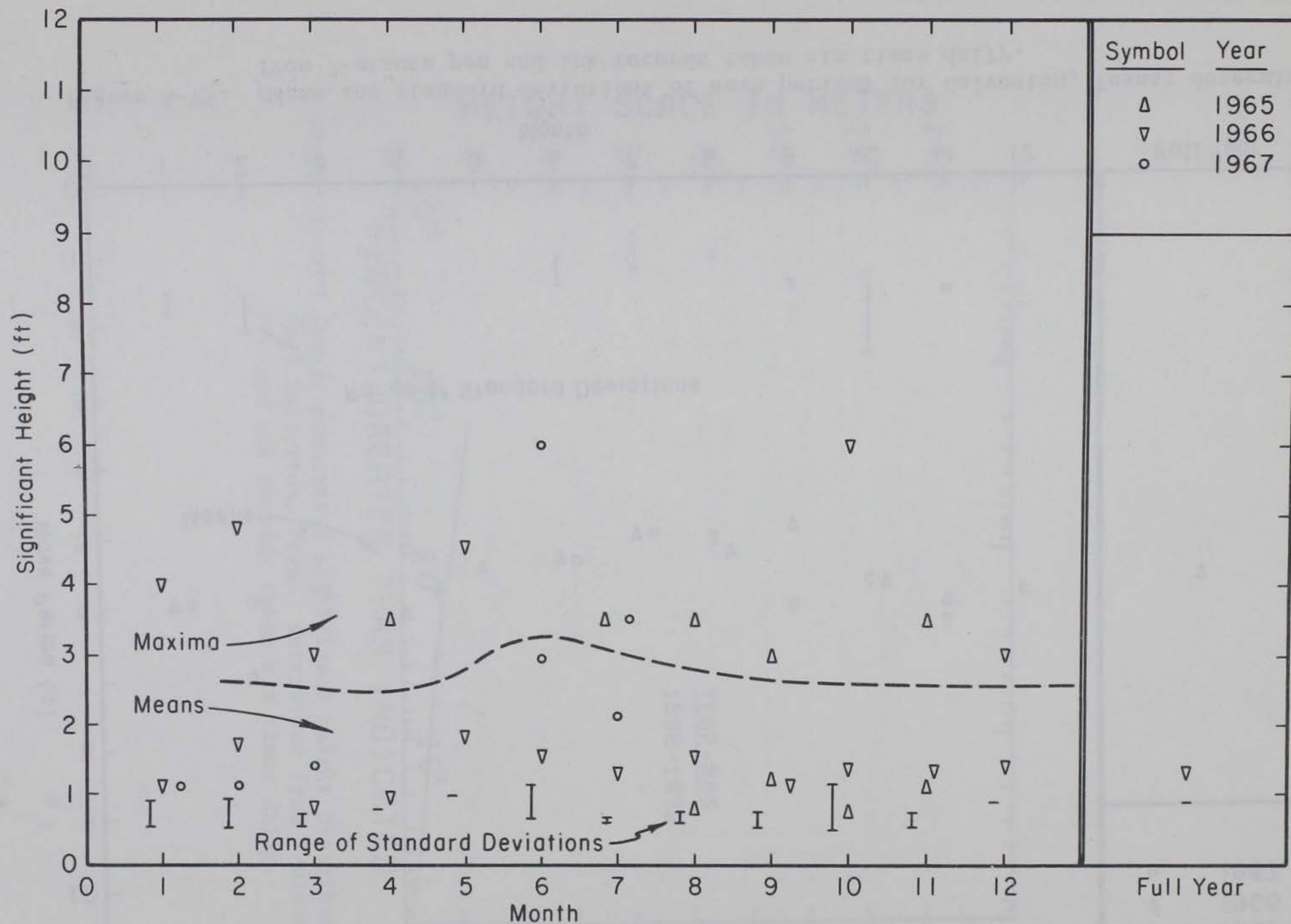
Figure A-74. Maxima, means, and standard deviations of significant height from Galveston, Texas; determined from 7-minute pen and ink records taken six times daily.
