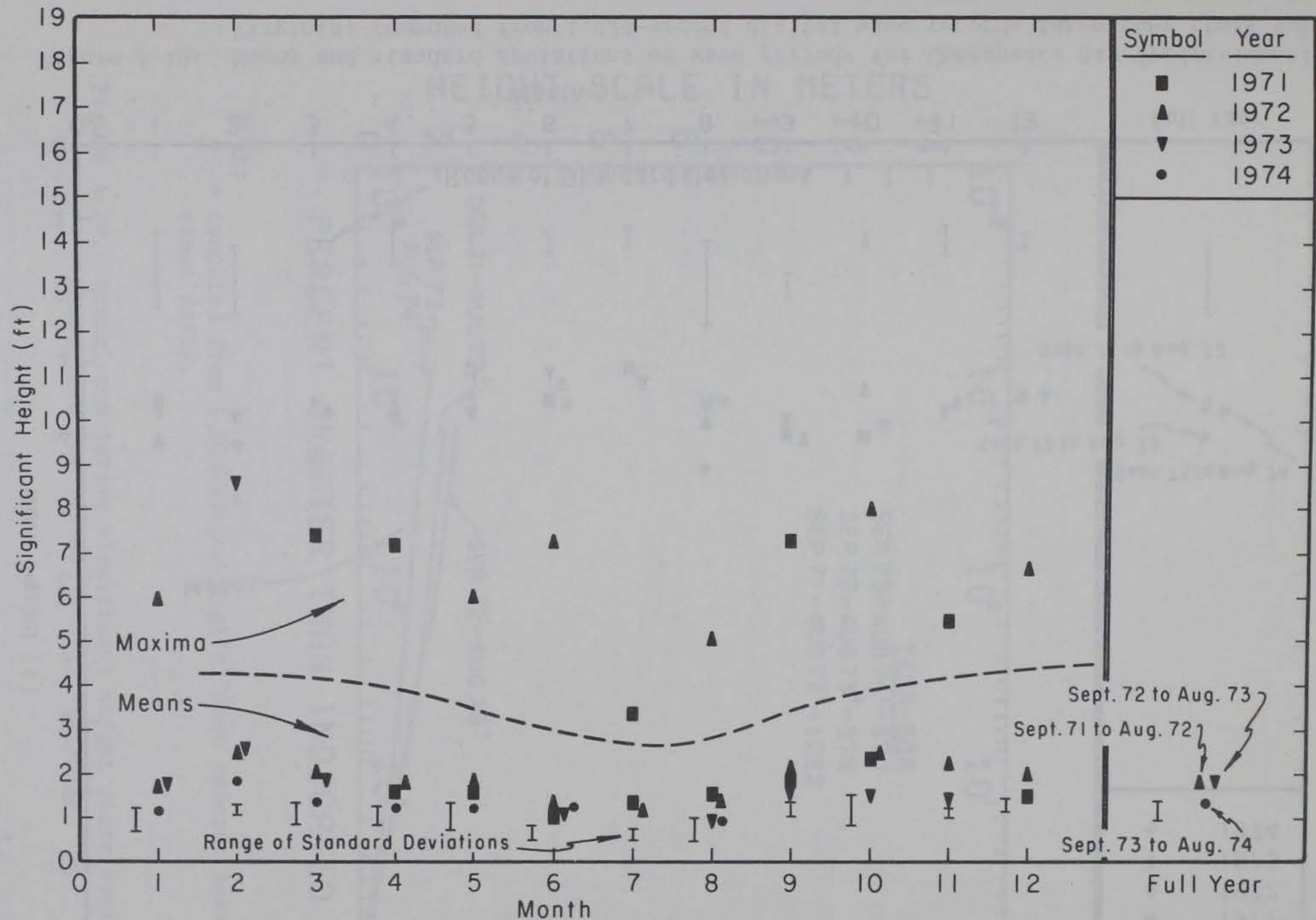
Figure A-18. Maxima, means, and standard deviations of significant height from Chesapeake Bay Bridge-Tunnel, Virginia; computed from 1,024-second digital wave records taken four times daily.
