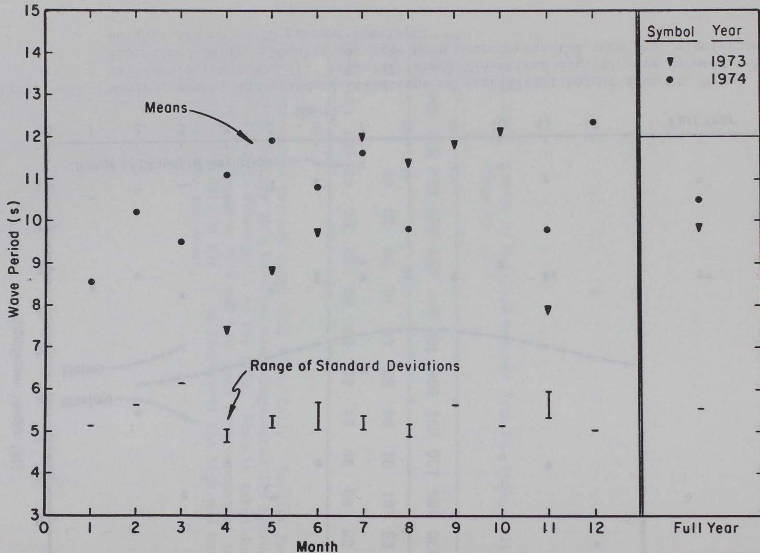
Figure A-94. Means and standard deviations of wave periods for Pt. Mugu, California (Gage No. 4). Computed from 1,024-second digital wave records taken four times daily. Results may have been overcompensated such that wave periods tend to be too short.
