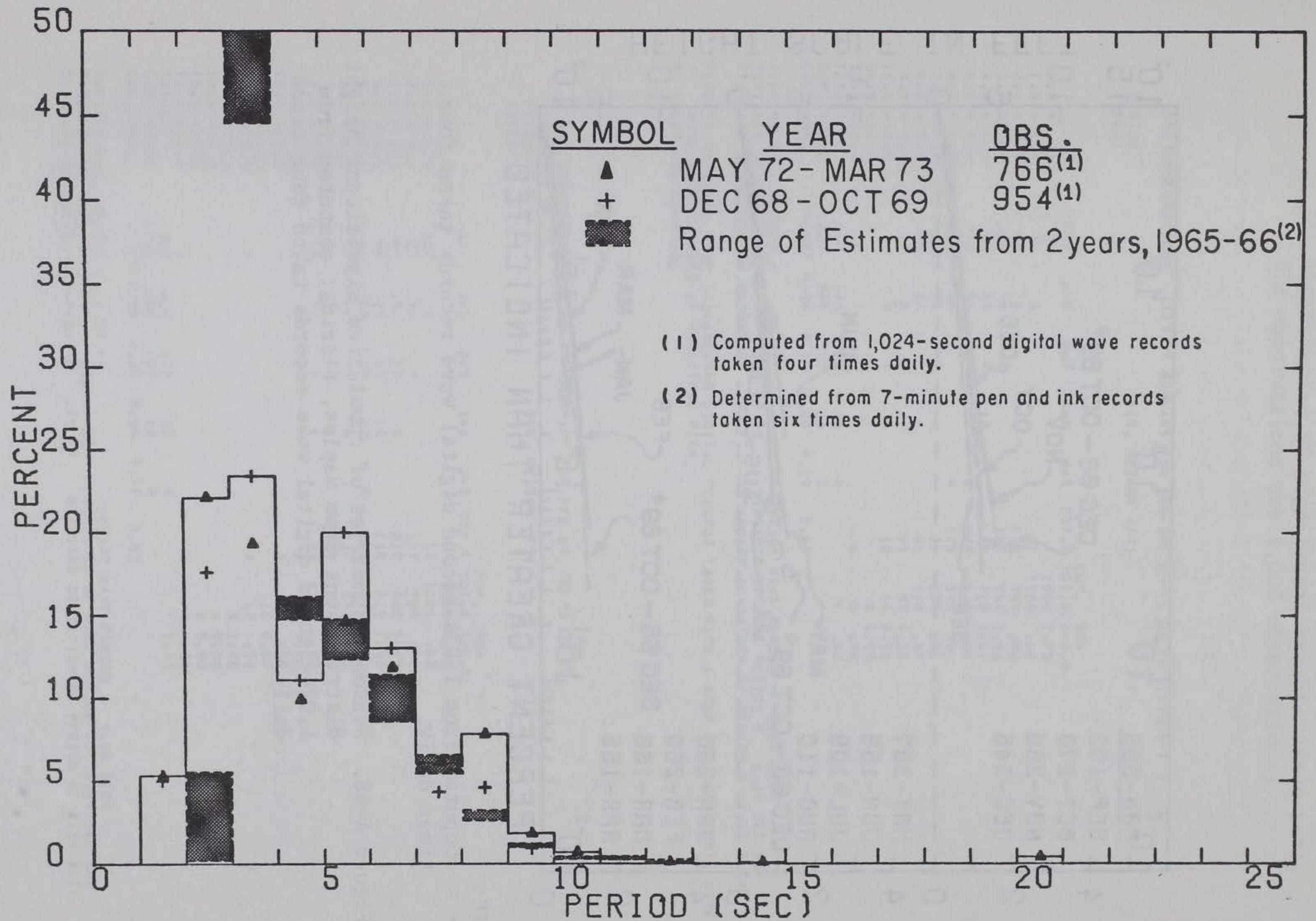
Figure A-67. Annual significant period distributions from Naples, Florida.
