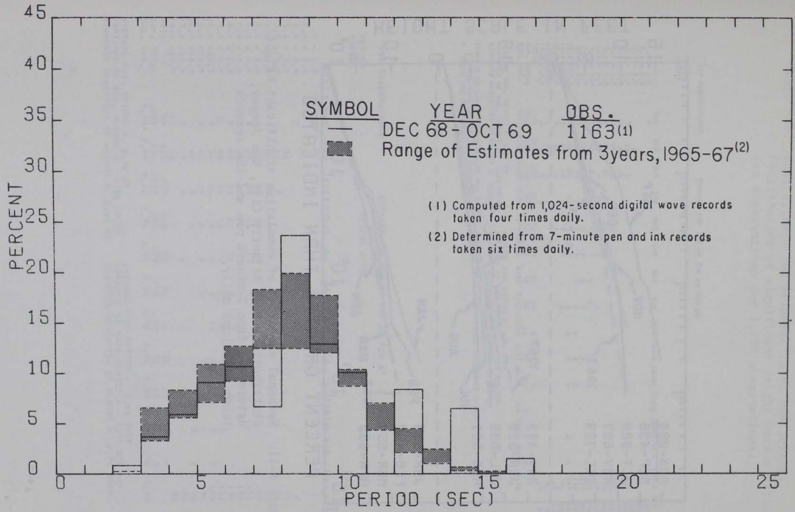
Figure A-10. Annual significant period distributions from Atlantic City, New Jersey.
