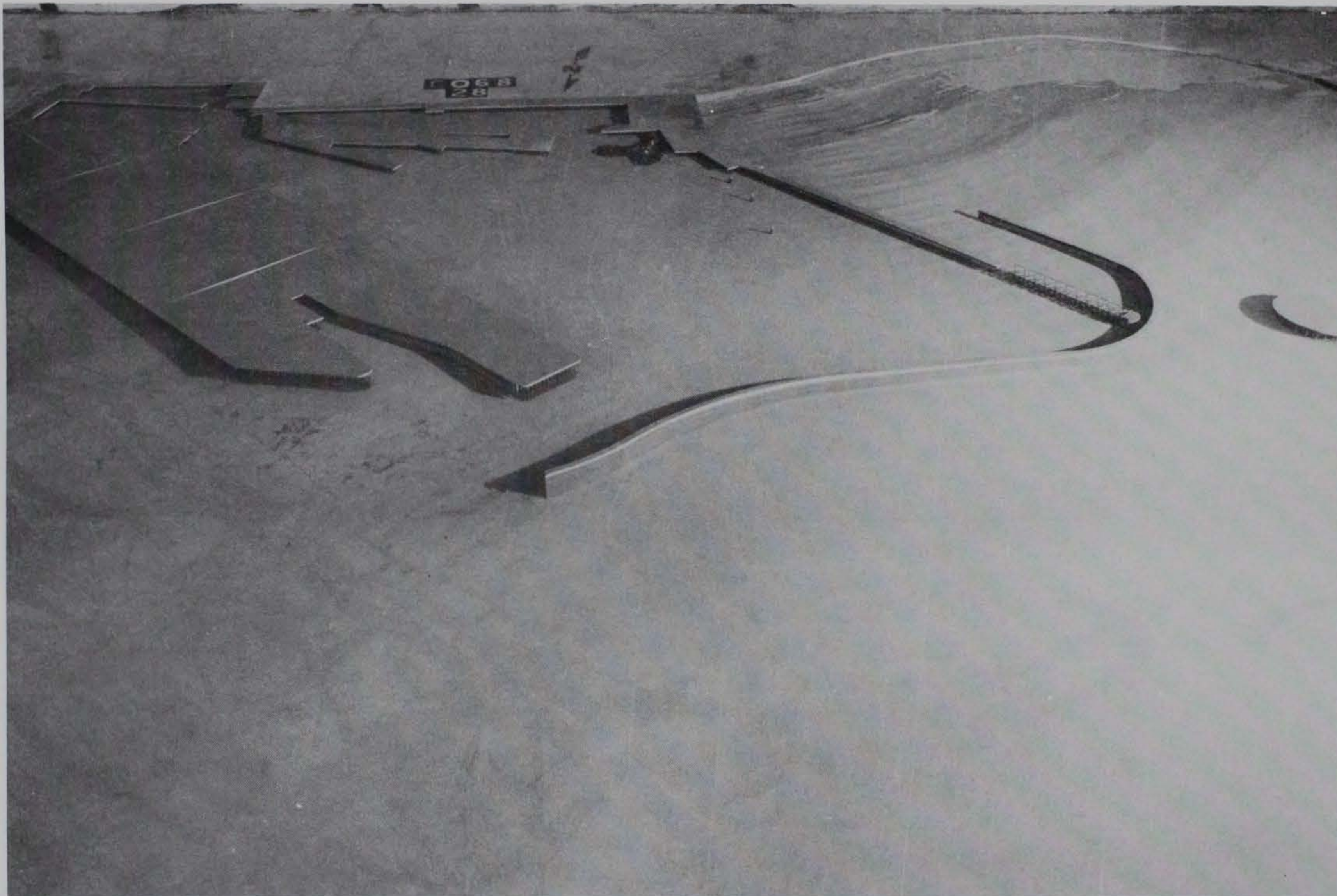
Photo 33. Typical wave patterns for Plan 2; 10-sec, 2-ft waves from west-northwest; +5.7 ft swl
