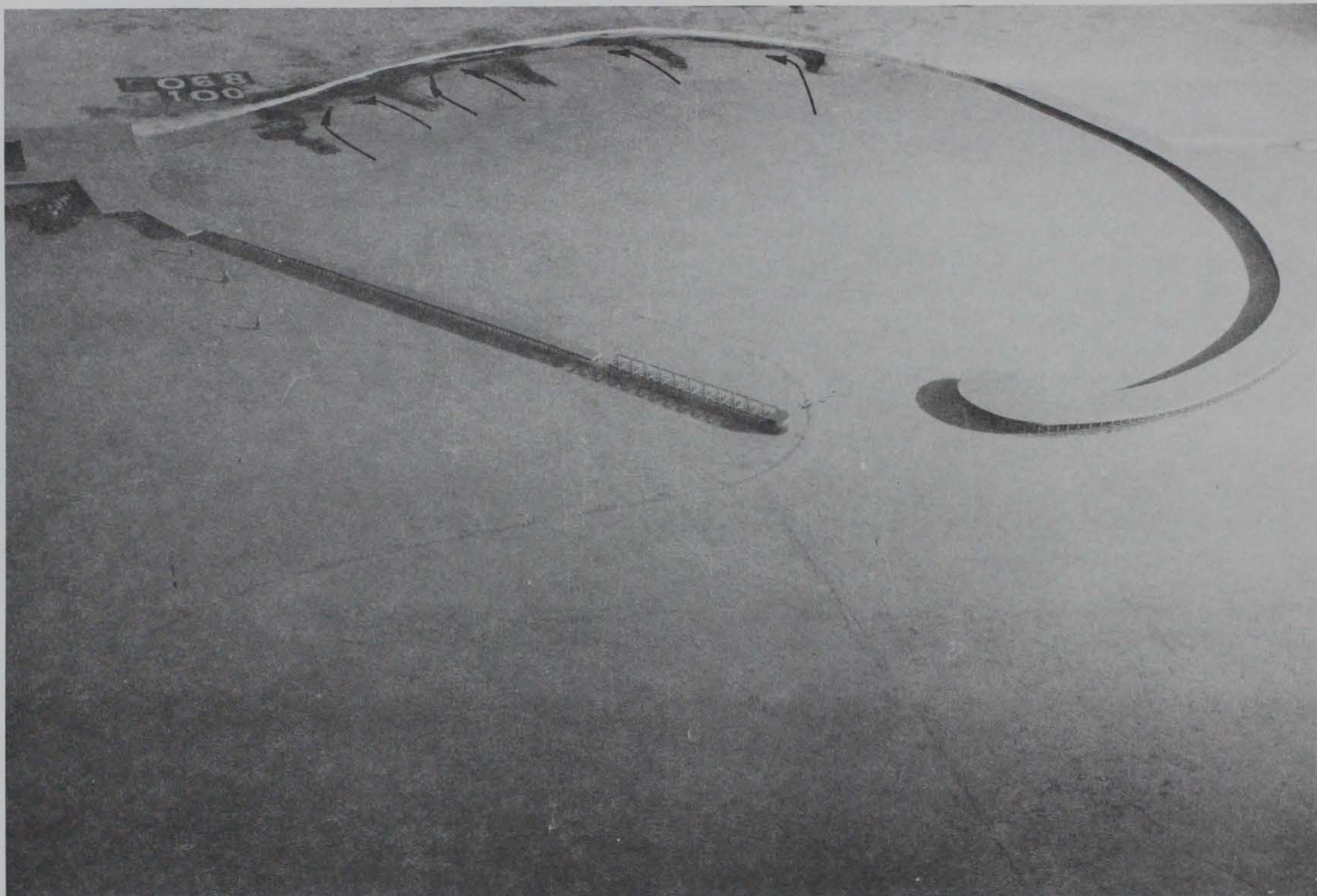
Photo 30. General movement of tracer material for existing conditions; 10-sec, 3-ft waves from west-northwest; +5.7 ft swl
