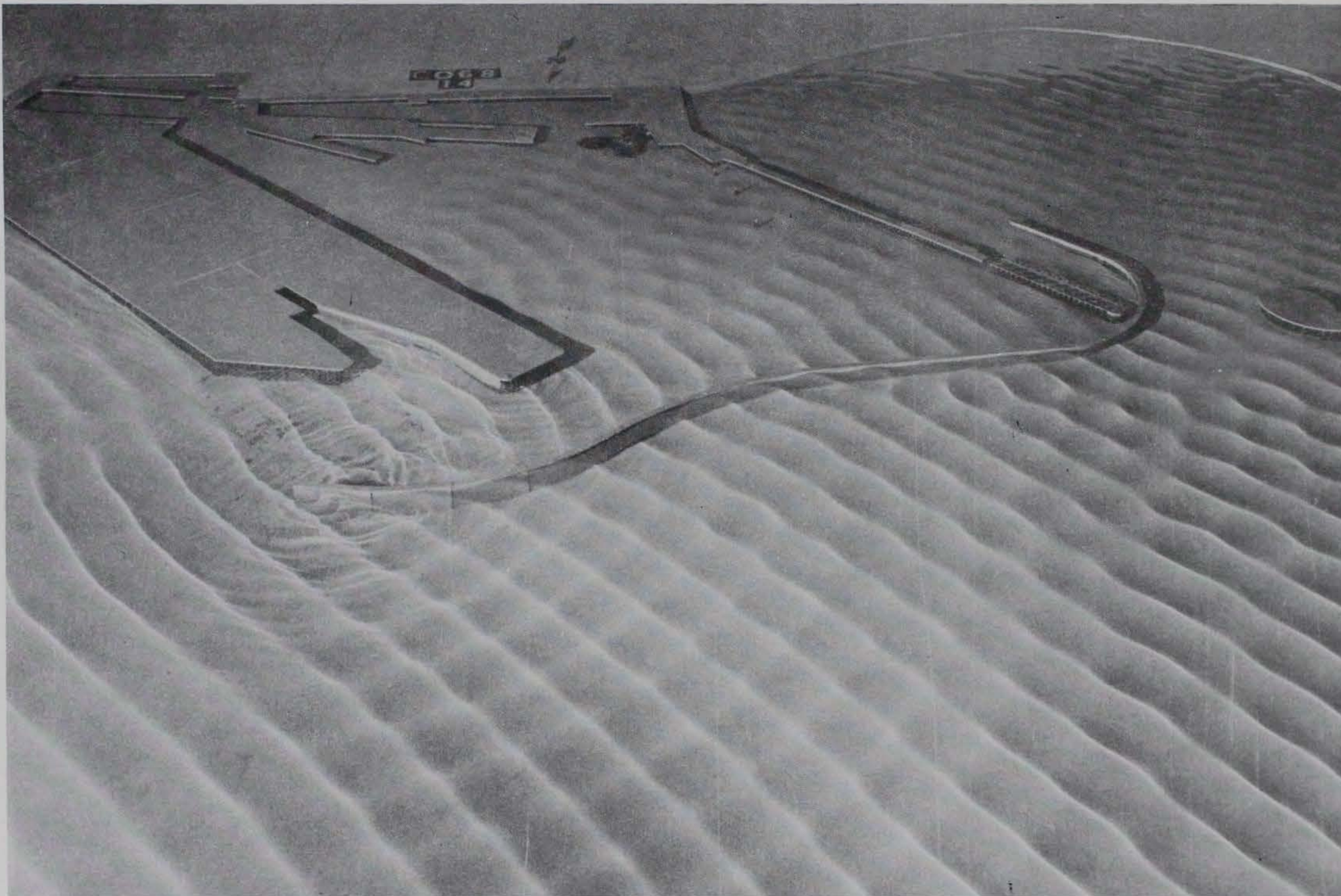
Photo 39. Typical wave patterns for Plan 8; 3.9-sec, 3.3-ft waves from northeast; +5.7 ft swl
