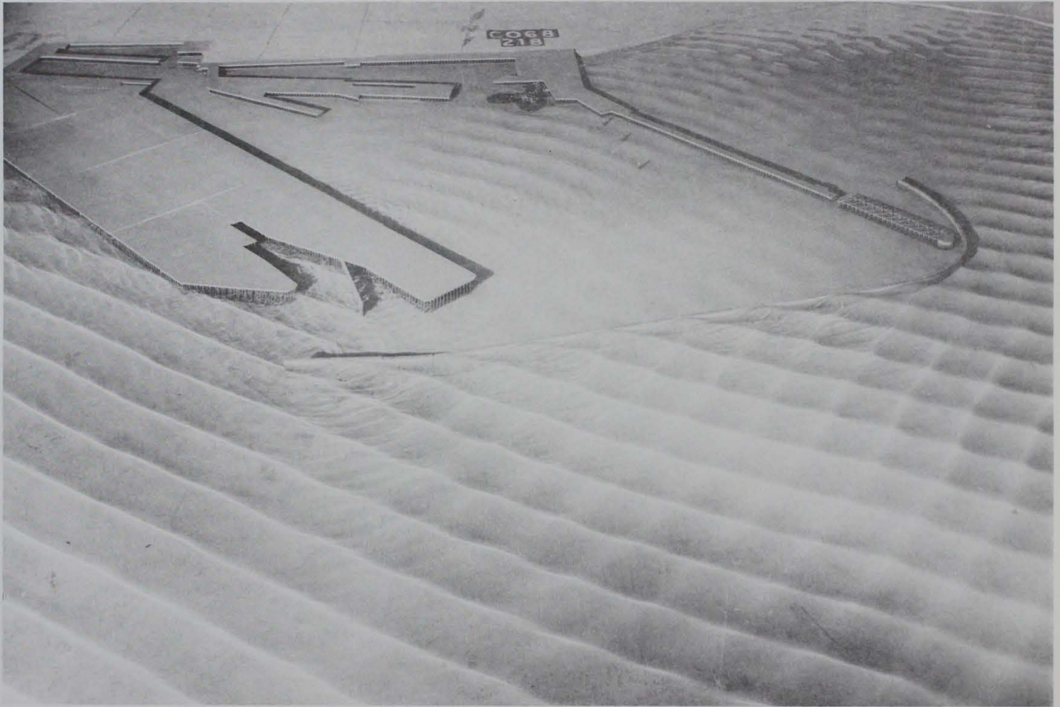
Photo 154. Typical wave patterns for Plan 78; 4.2-sec, 4.8-ft waves from north-northeast; +5.7 ft swl
