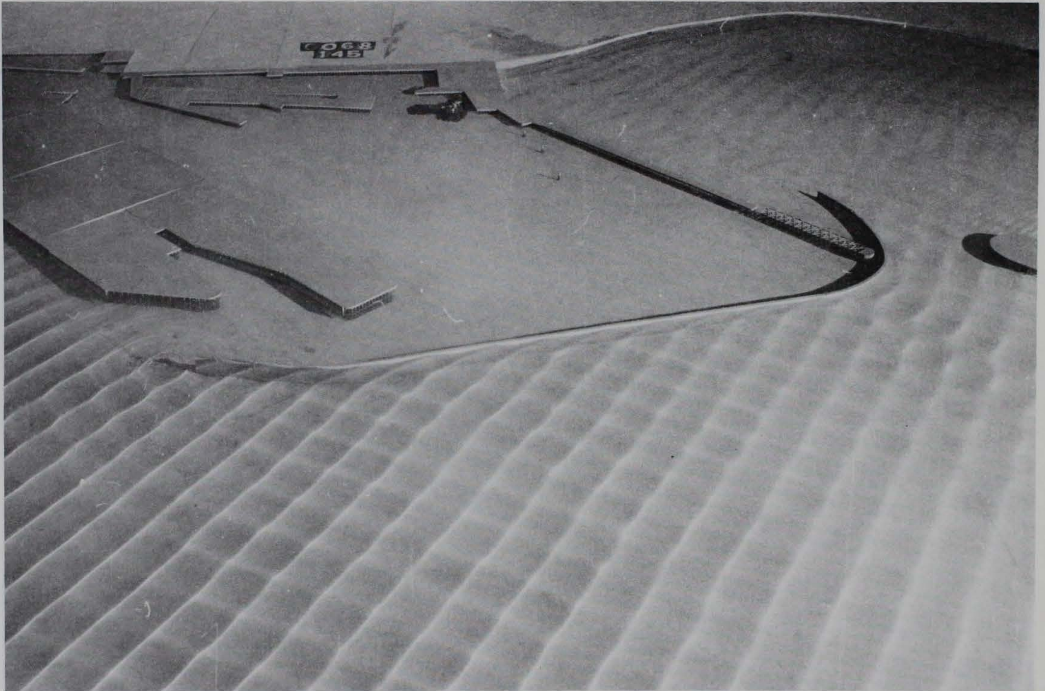
Photo 81. Typical wave patterns for Plan 38; 3.6-sec, 2-ft waves from west-northwest; +5.7 ft swl
