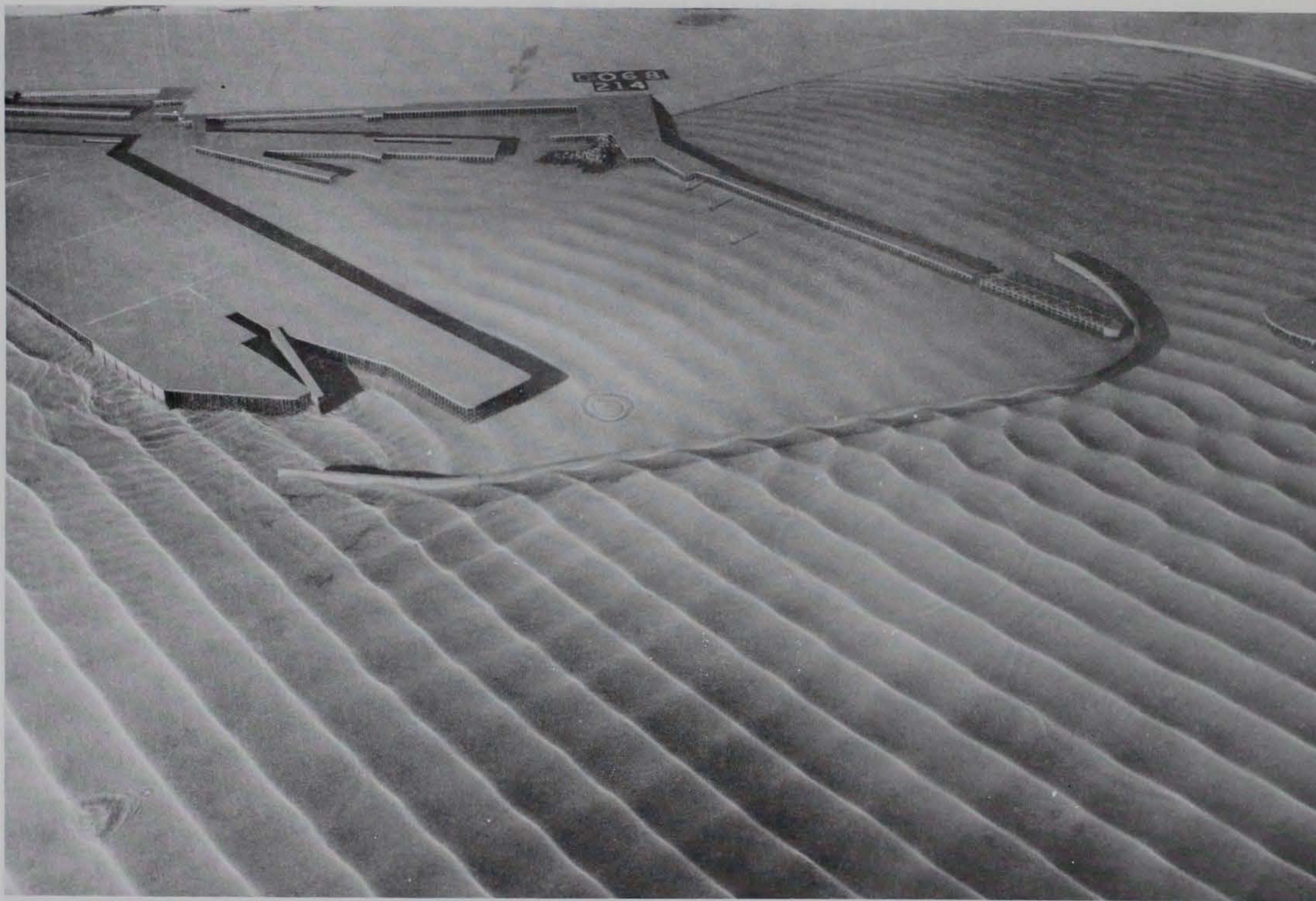
Photo 119. Typical wave patterns for Plan 59; 3.9-sec, 3.3-ft waves from northeast; 0.0-ft swl
