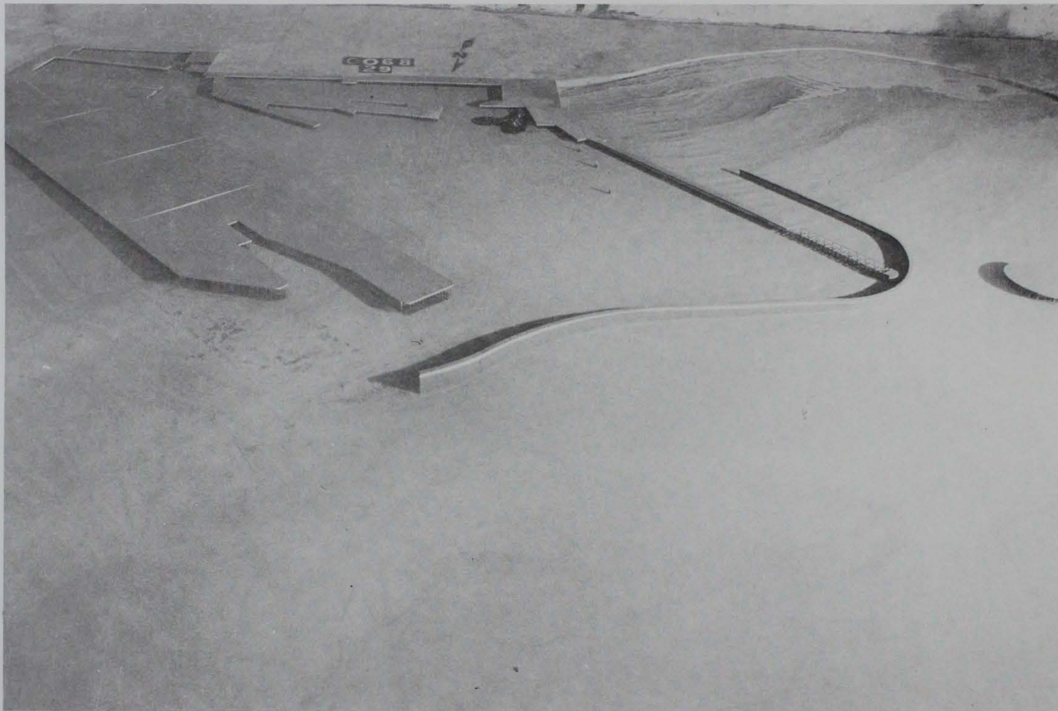
Photo 34. Typical wave patterns for Plan 3; 10-sec, 2-ft waves from west-northwest; +5.7 ft swl
