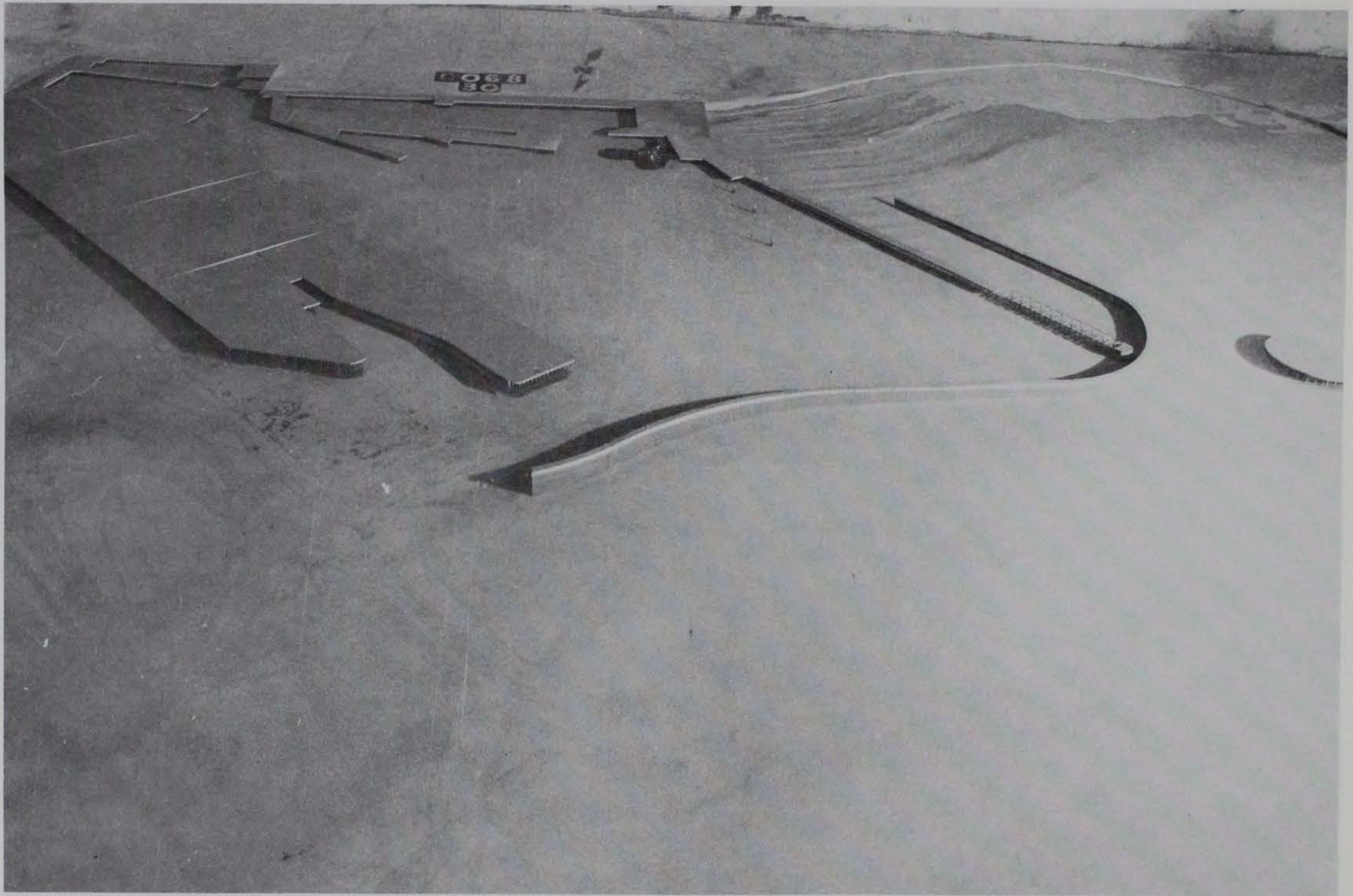
Photo 35. Typical wave patterns for Plan 4; 10-sec, 2-ft waves from west-northwest; +5.7 ft swl
