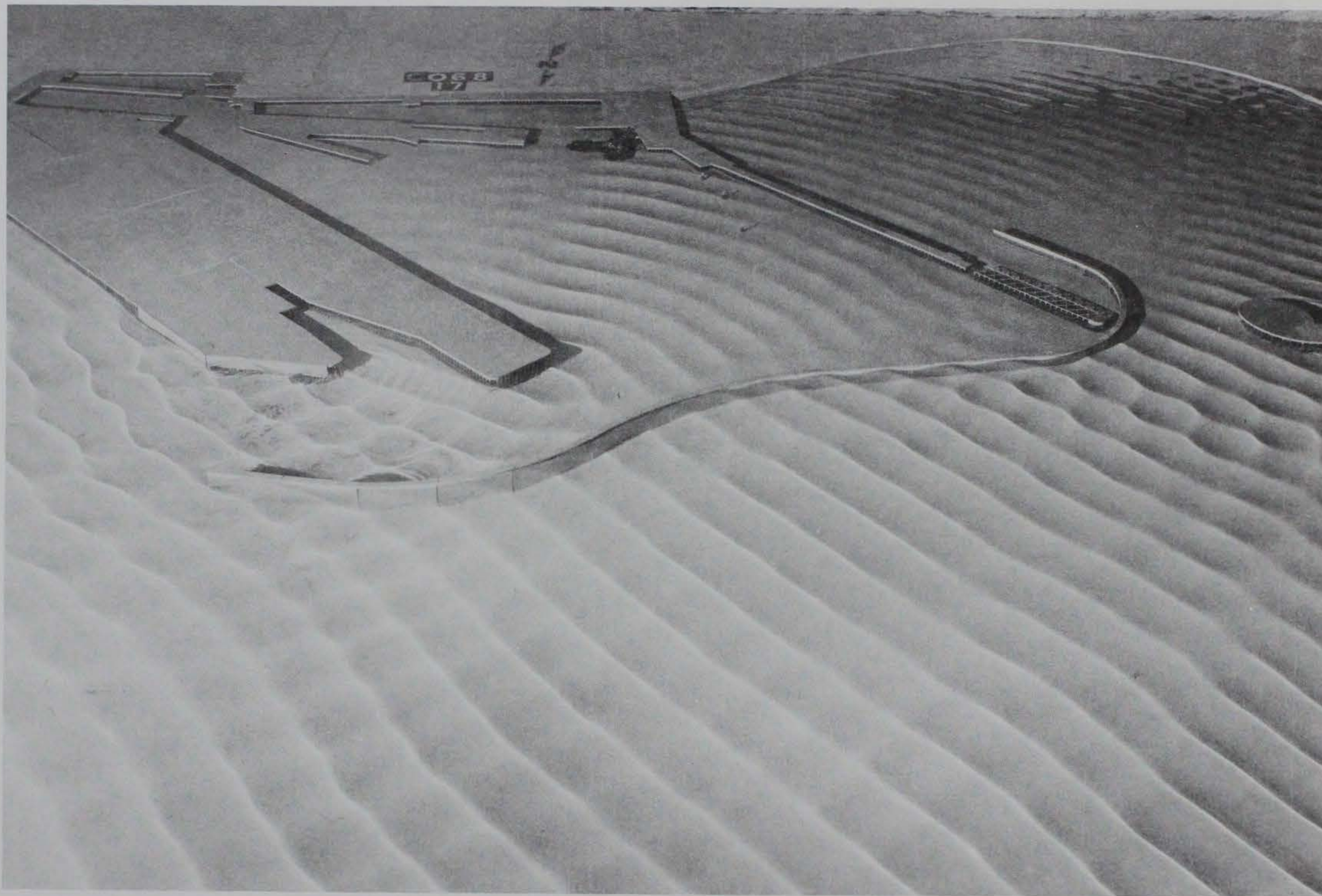
Photo 42. Typical wave patterns for Plan 11; 3.9-sec, 3.3-ft waves from northeast; +5.7 ft swl
