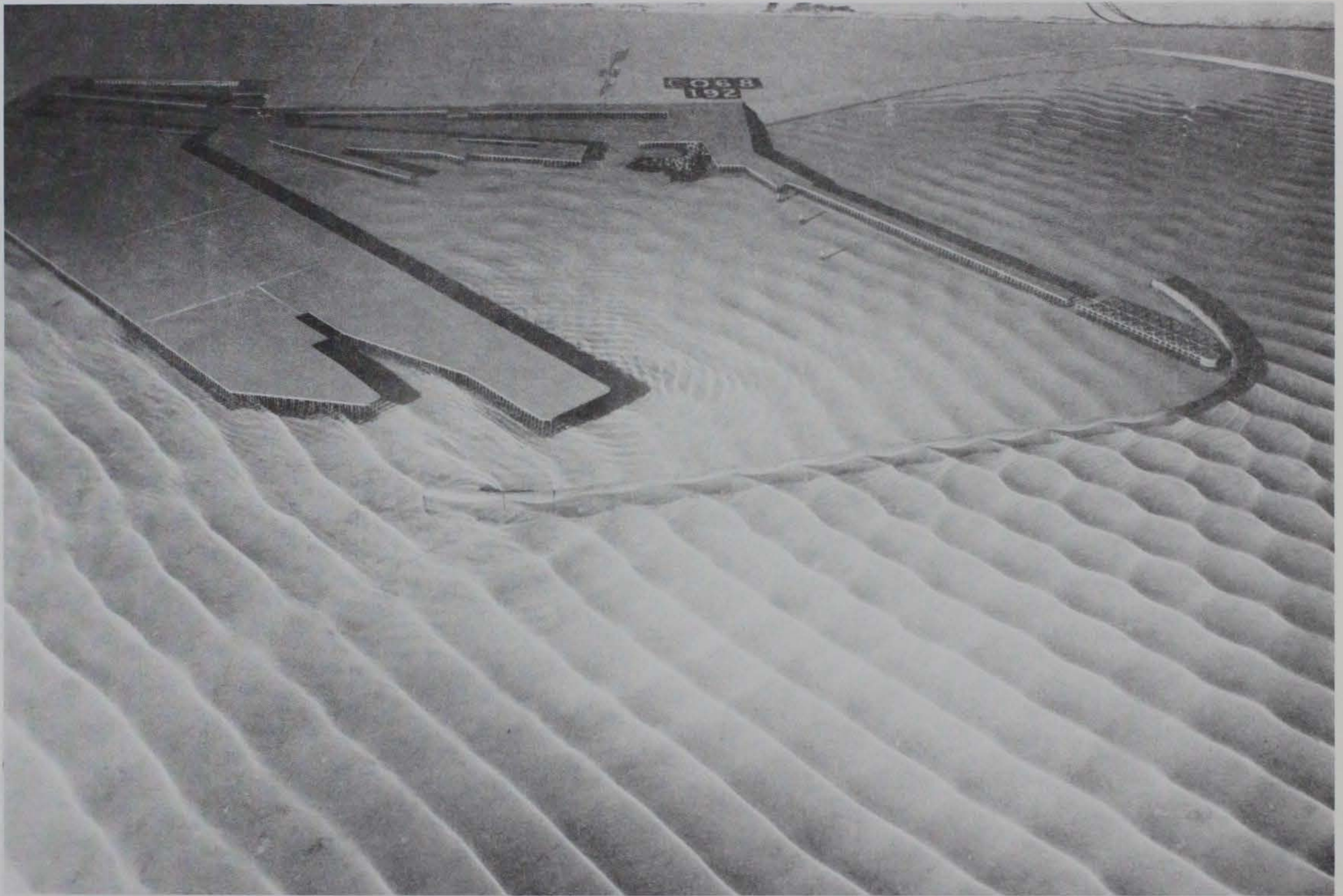
Photo 130. Typical wave patterns for Plan 70; 3.9-sec, 3.3-ft waves from northeast; 0.0-ft swl
