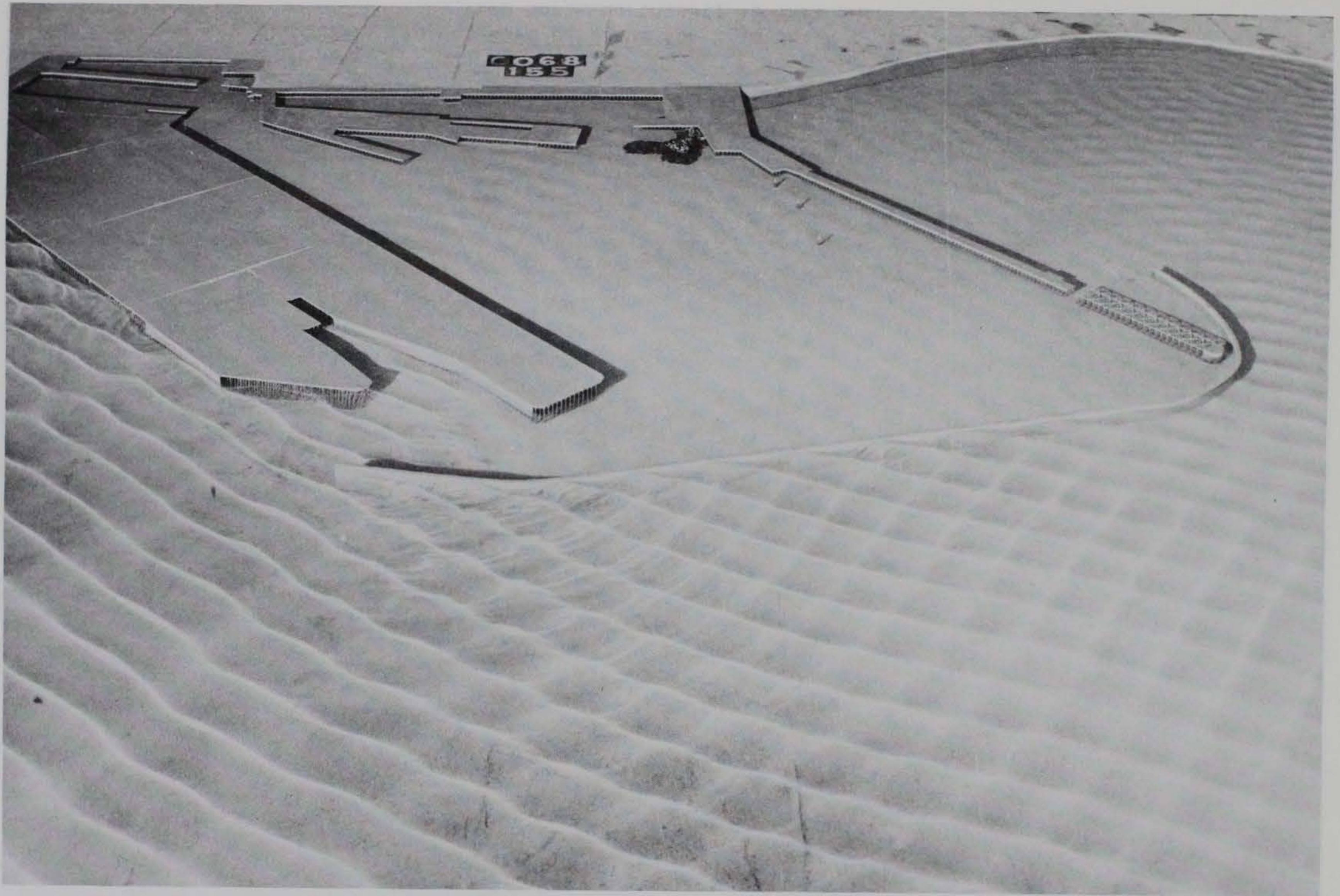
Photo 73. Typical wave patterns for Plan 38; 3.6-sec, 2.5-ft waves from north-northeast; +5.7 ft swl
