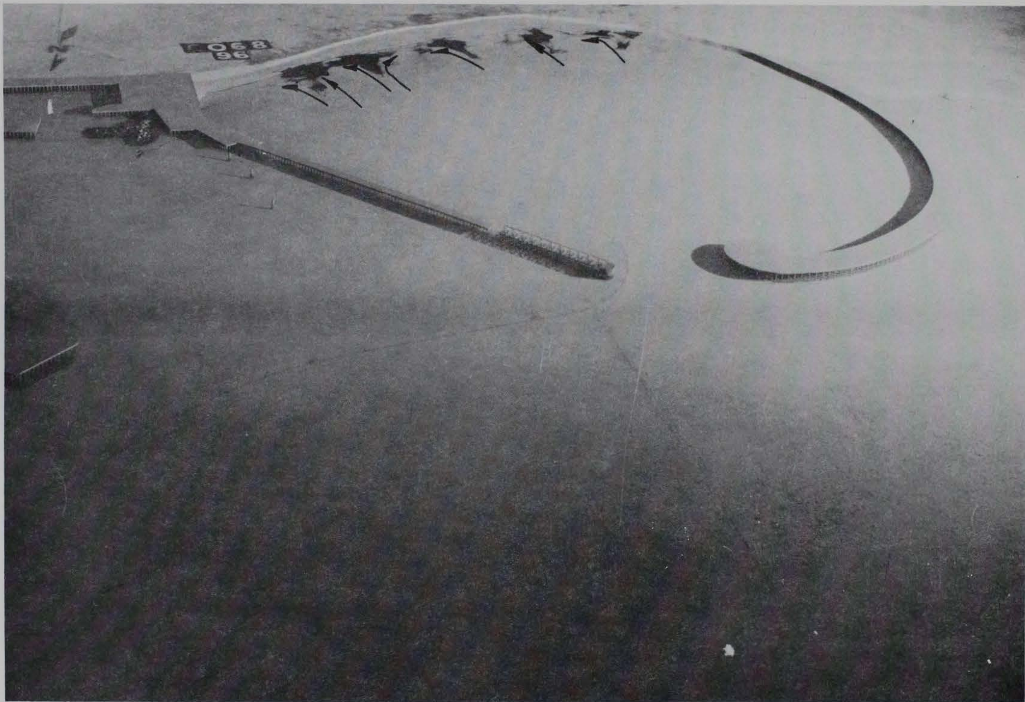
Photo 27. General movement of tracer material for existing conditions; 10-sec, 2-ft waves from west-northwest; 0.0-ft swl
