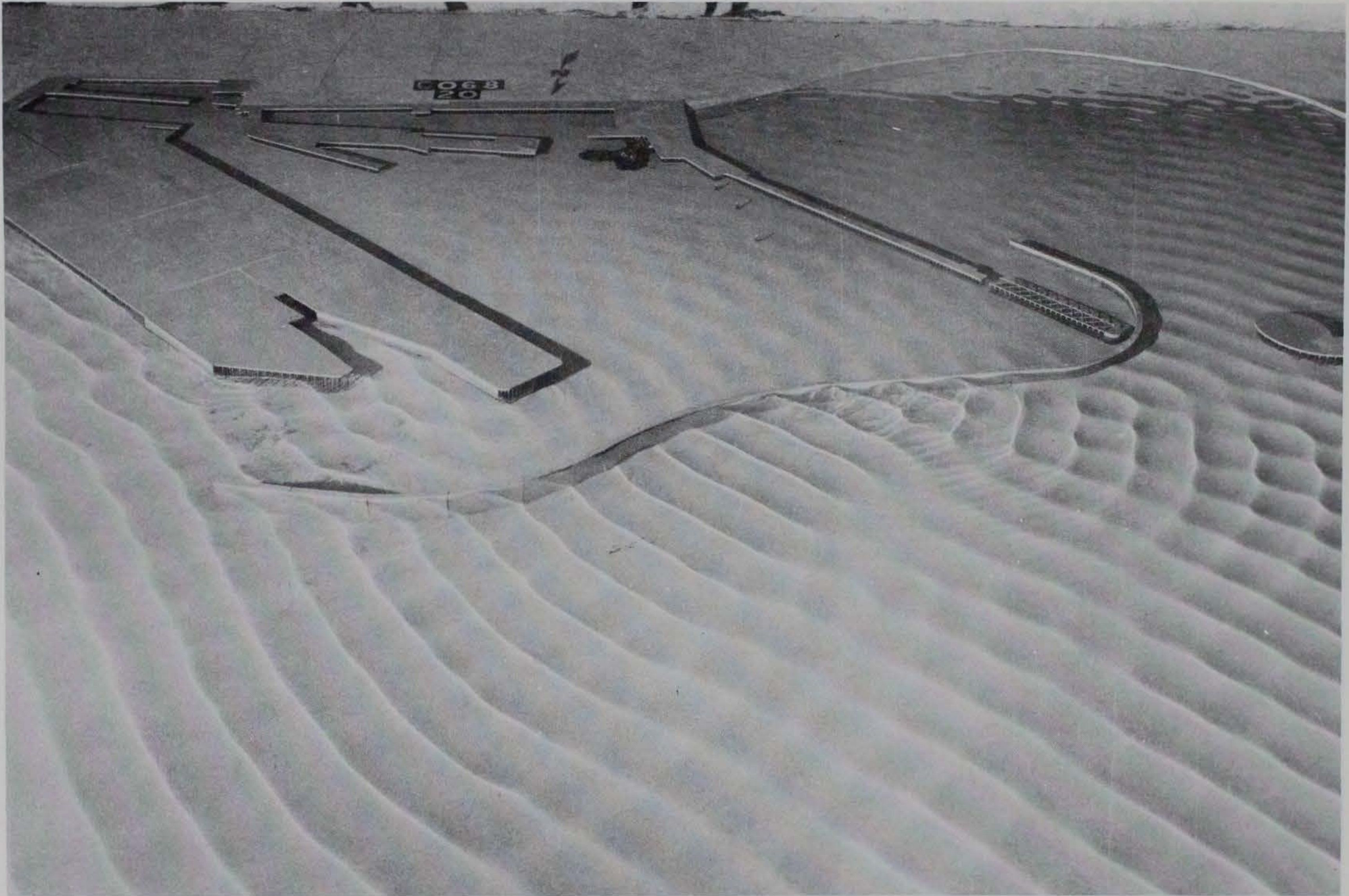
Photo 45. Typical wave patterns for Plan 14; 3.9-sec, 3.3-ft waves from northeast; +5.7 ft swl
