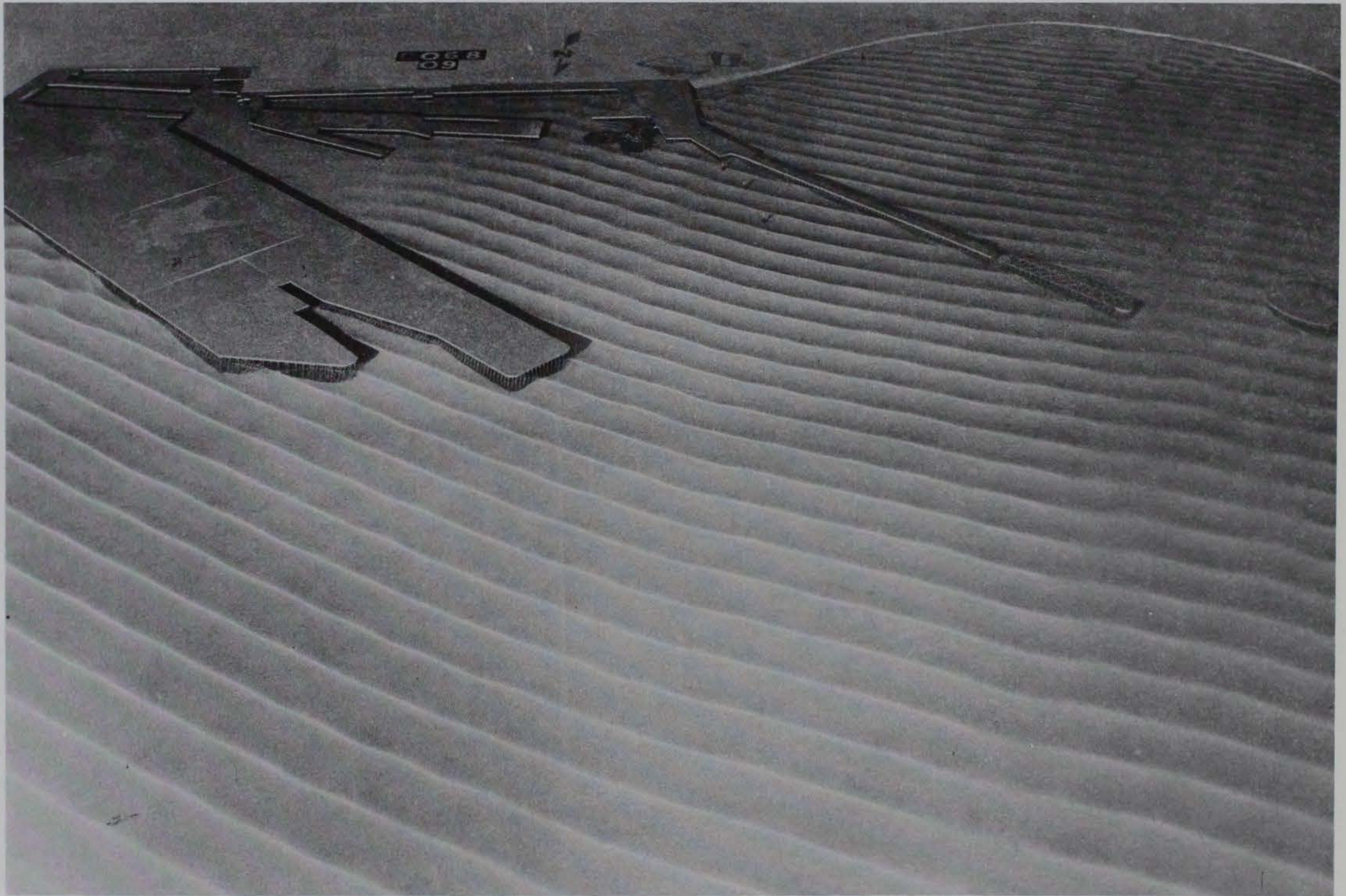
Photo 3. Typical wave patterns for existing conditions; 3.6-sec, 2.5-ft waves from north-northeast; +5.7 ft swl
