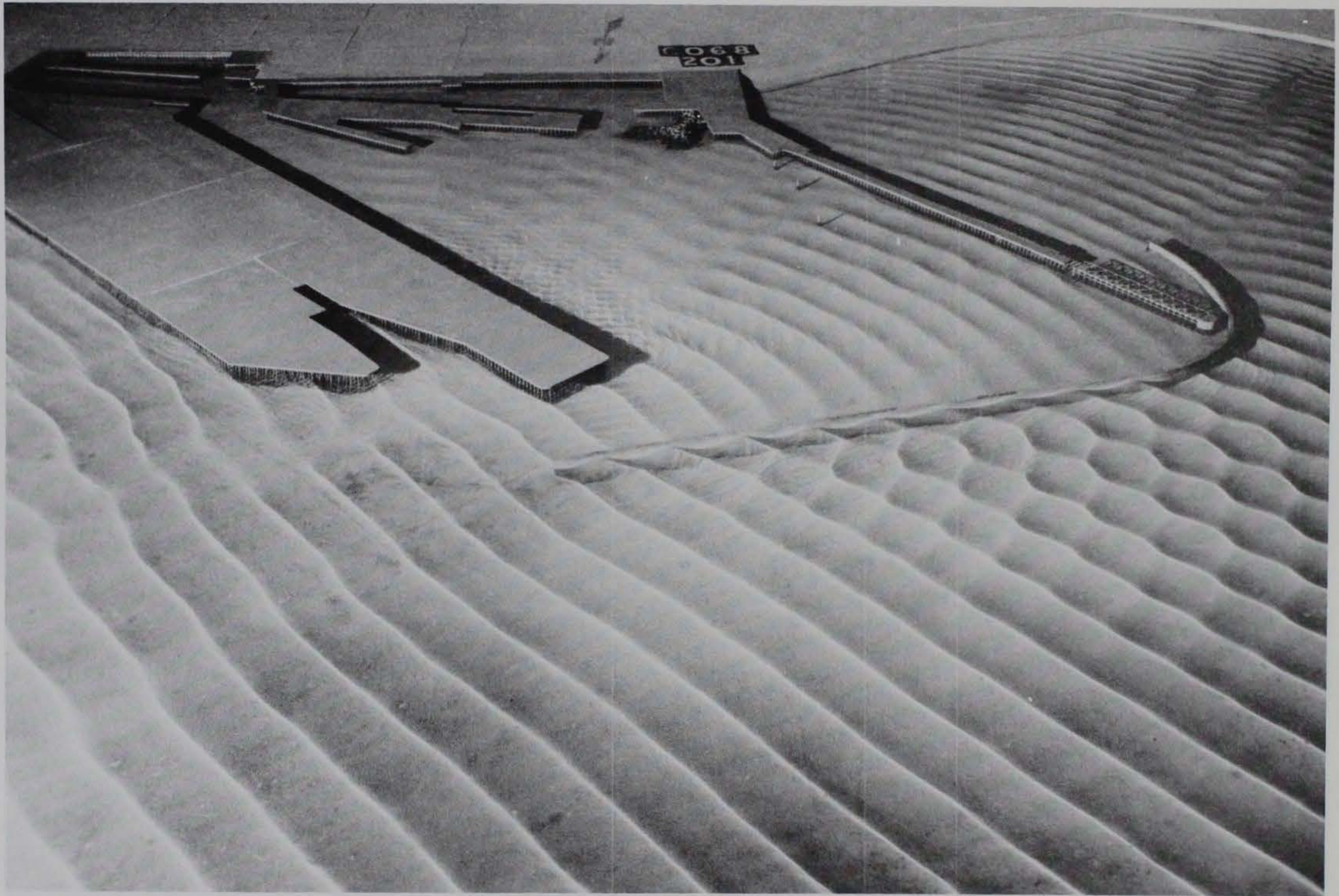
Photo 129. Typical wave patterns for Plan 69; 3.9-sec, 3.3-ft waves from northeast; 0.0-ft swl
