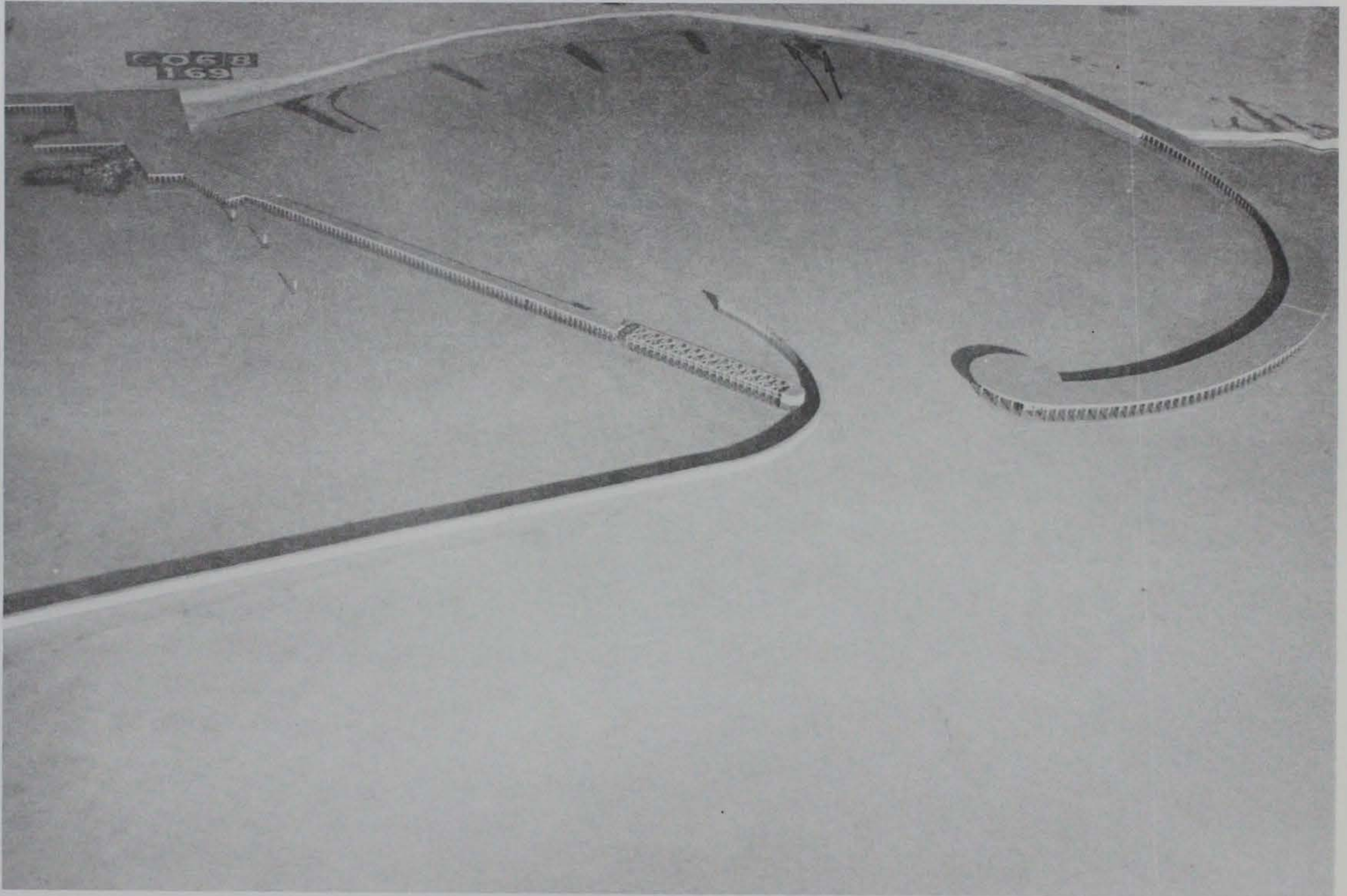
Photo 90. General movement of tracer material for Plan 38; 3.6-sec, 3.1-ft waves from north; 0.0-ft swl
