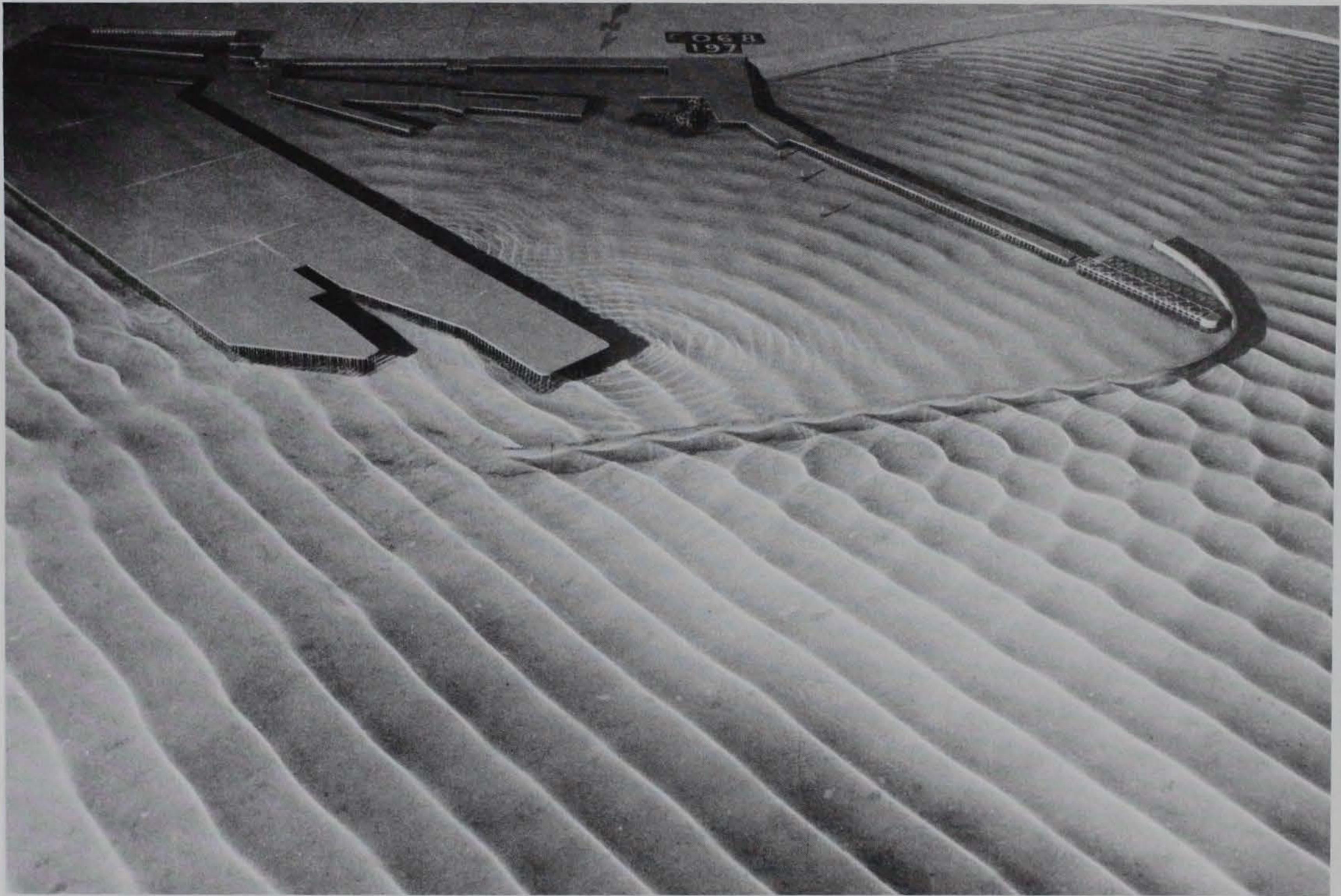
Photo 131. Typical wave patterns for Plan 71; 3.9-sec, 3.3-ft waves from northeast; 0.0-ft swl
