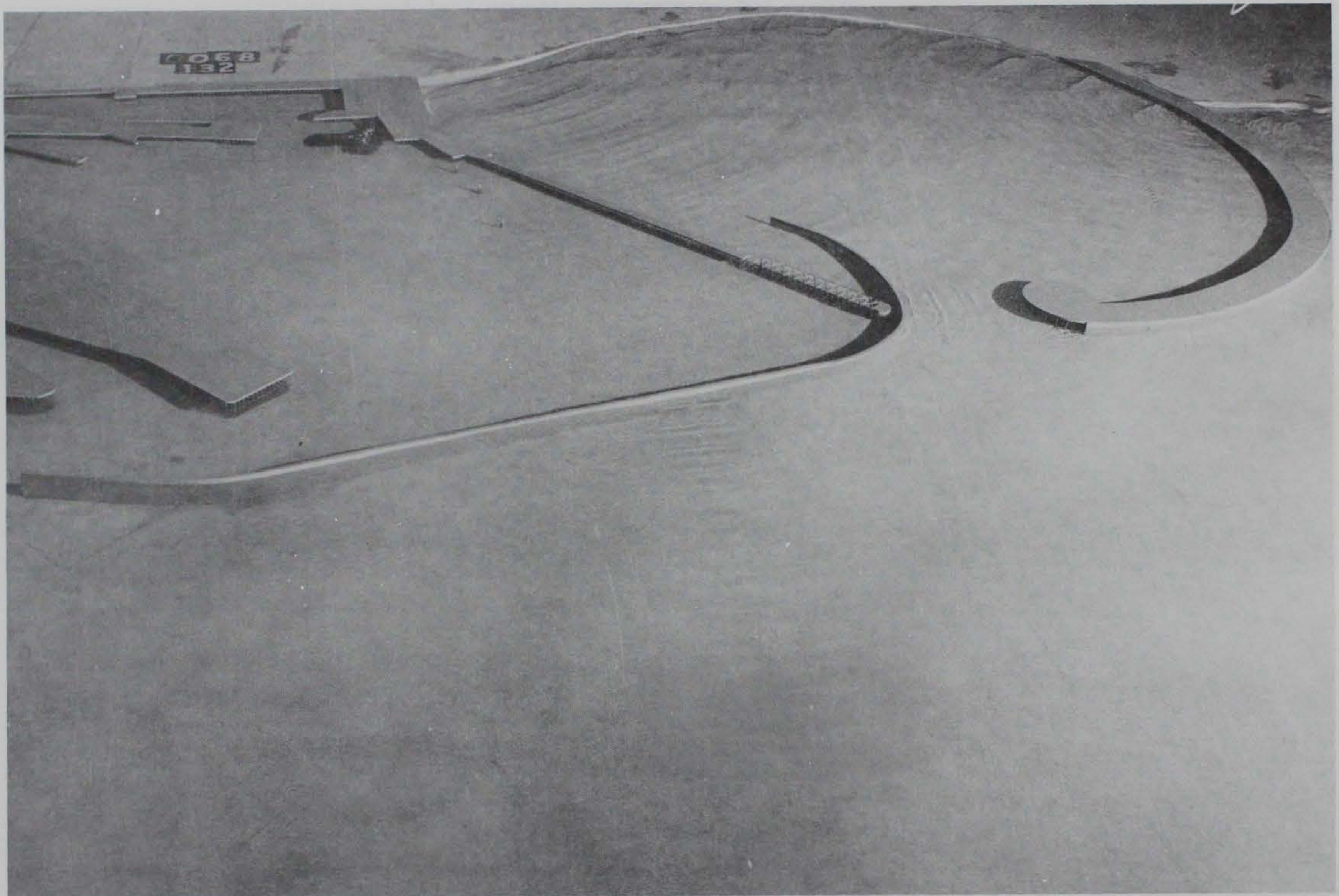
Photo 60. Typical wave patterns for Plan 29; 10-sec, 3-ft waves from west-northwest; +5.7 ft swl
