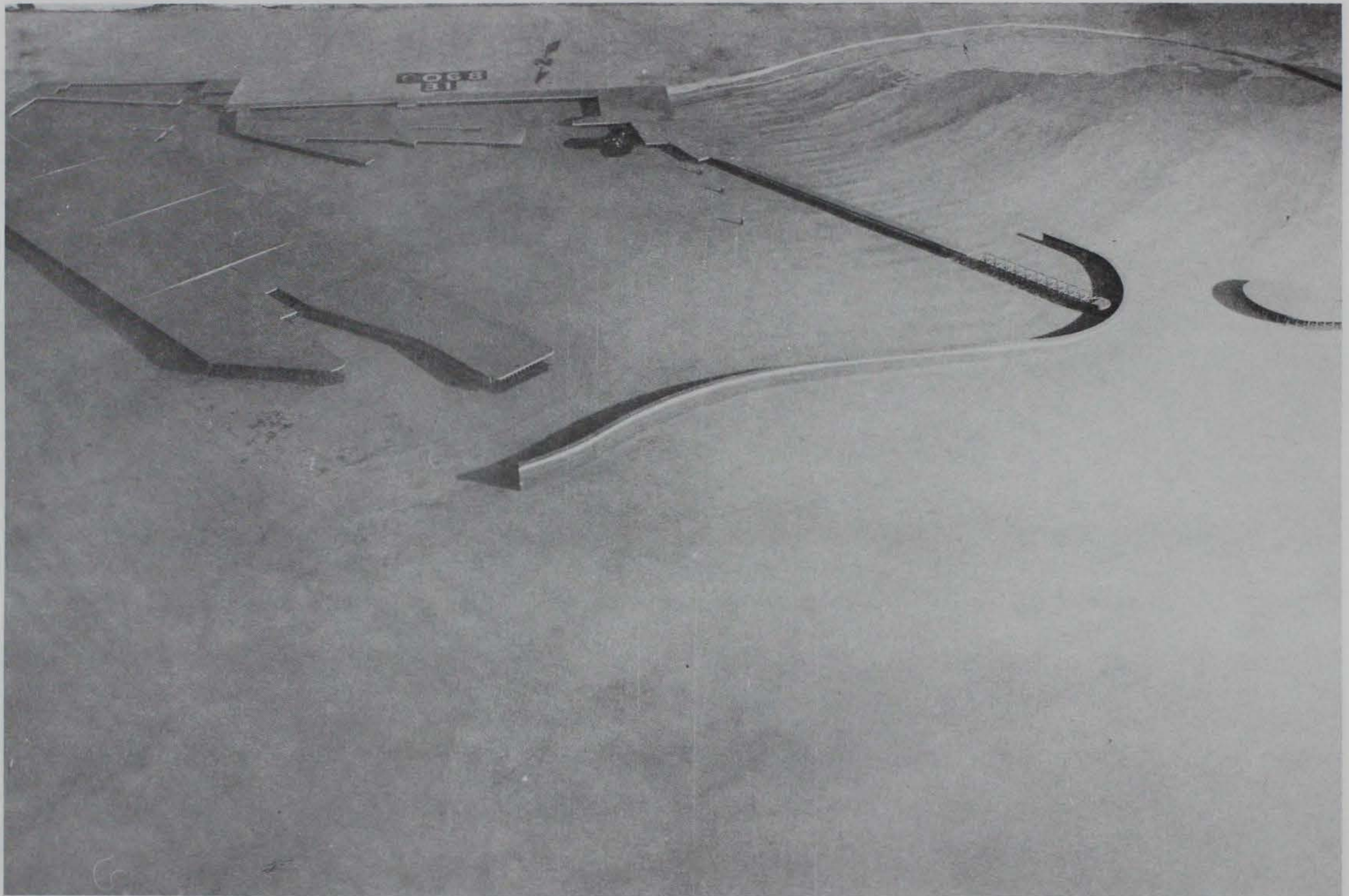
Photo 36. Typical wave patterns for Plan 5; 10-sec, 2-ft waves from west-northwest; +5.7 ft swl
