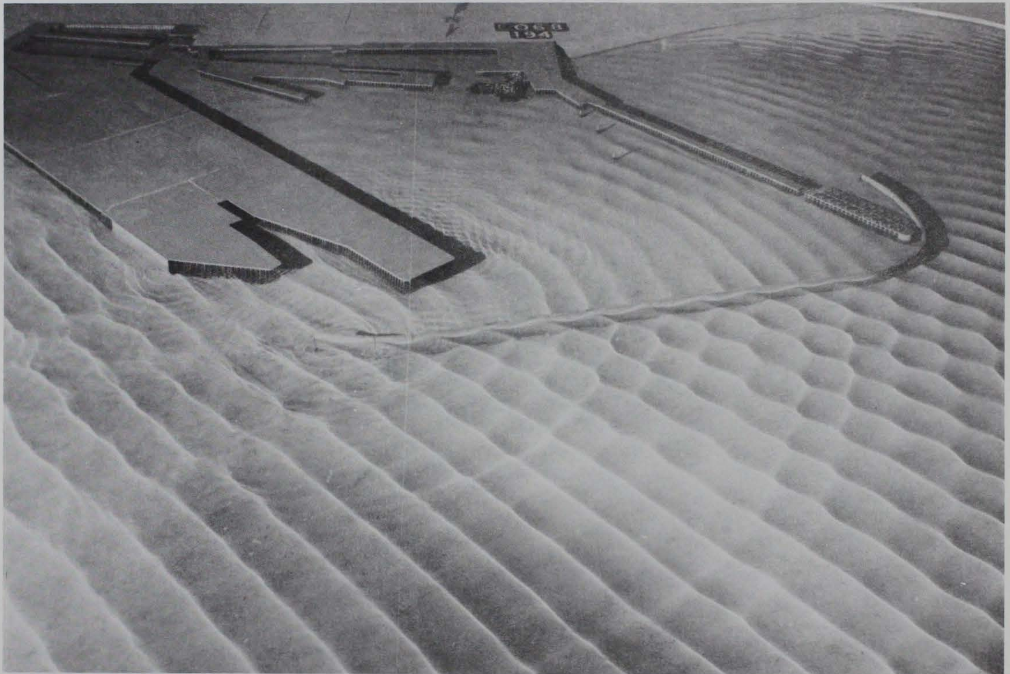
Photo 124. Typical wave patterns for Plan 64; 3.9-sec, 3.3-ft waves from northeast; 0.0-ft swl
