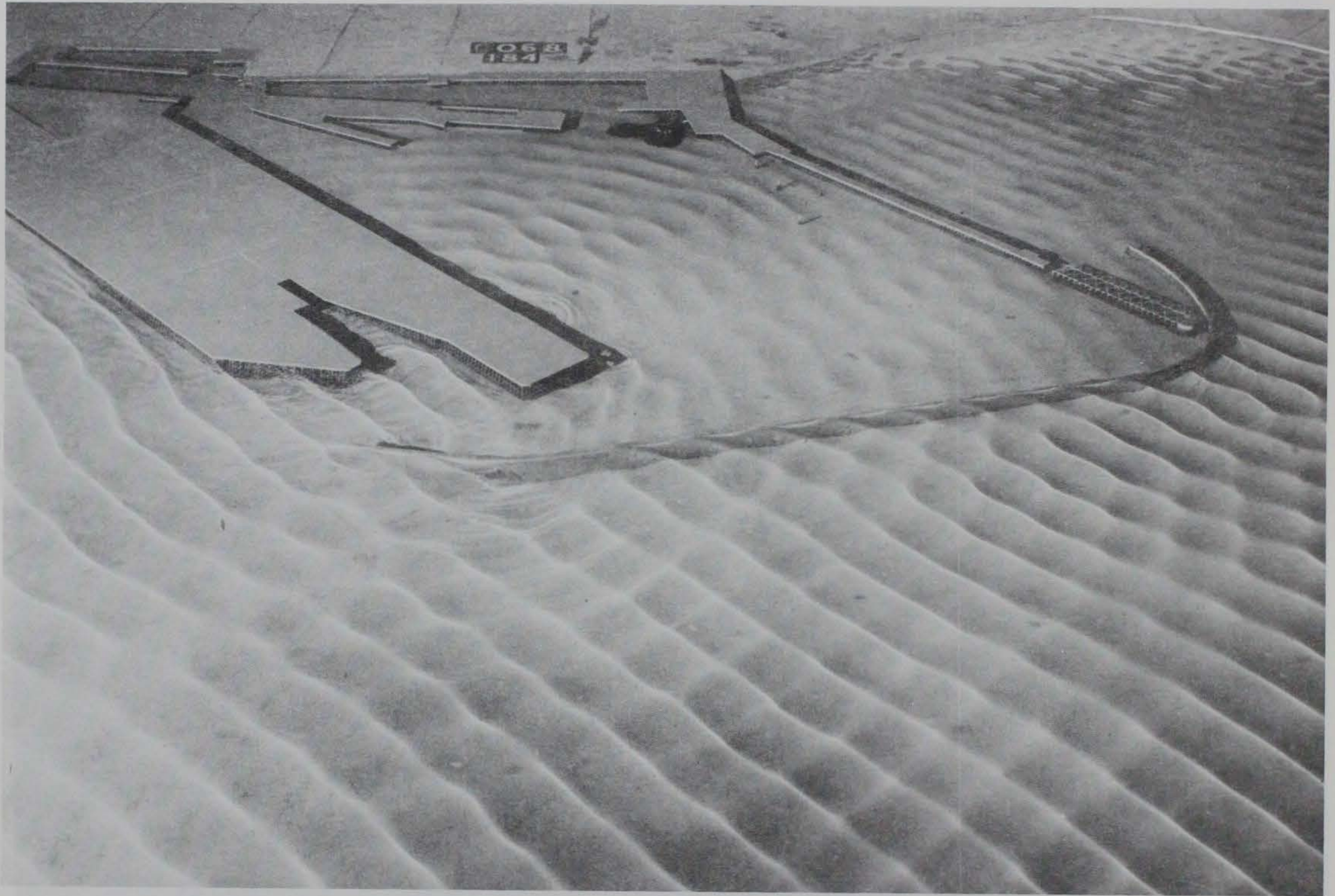
Photo 102. Typical wave patterns for Plan 41; 3.9-sec, 3.3-ft waves from northeast; +5.7 ft swl
