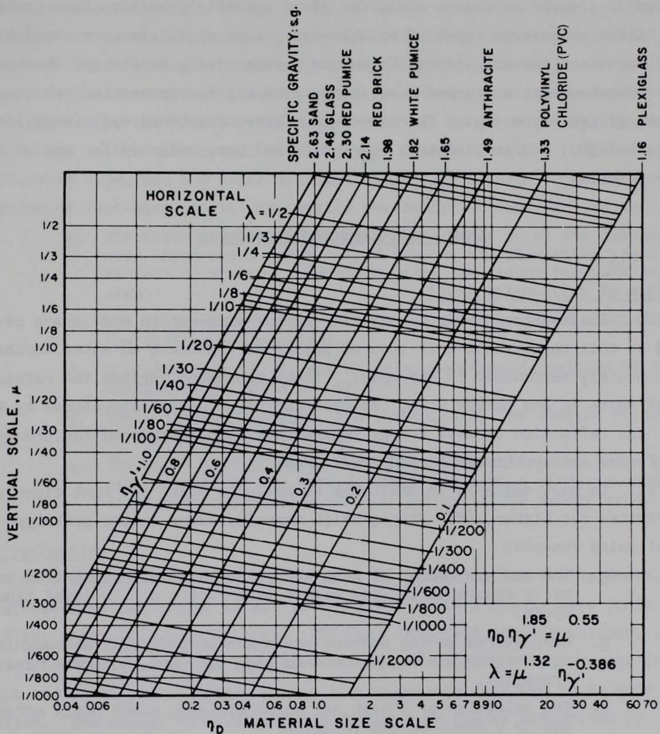
Figure 6. Graphic representation of model law (from Noda 1972)
