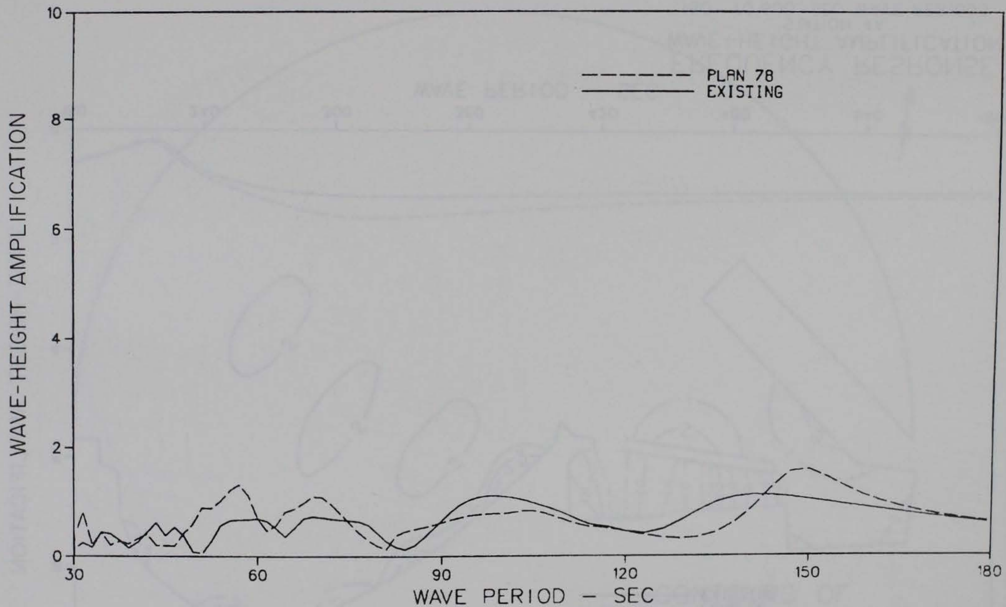
FREQUENCY RESPONSE WAVE-HEIGHT AMPLIFICATION STATION 4A 30 - TO 180-SEC WAVE PERIODS
