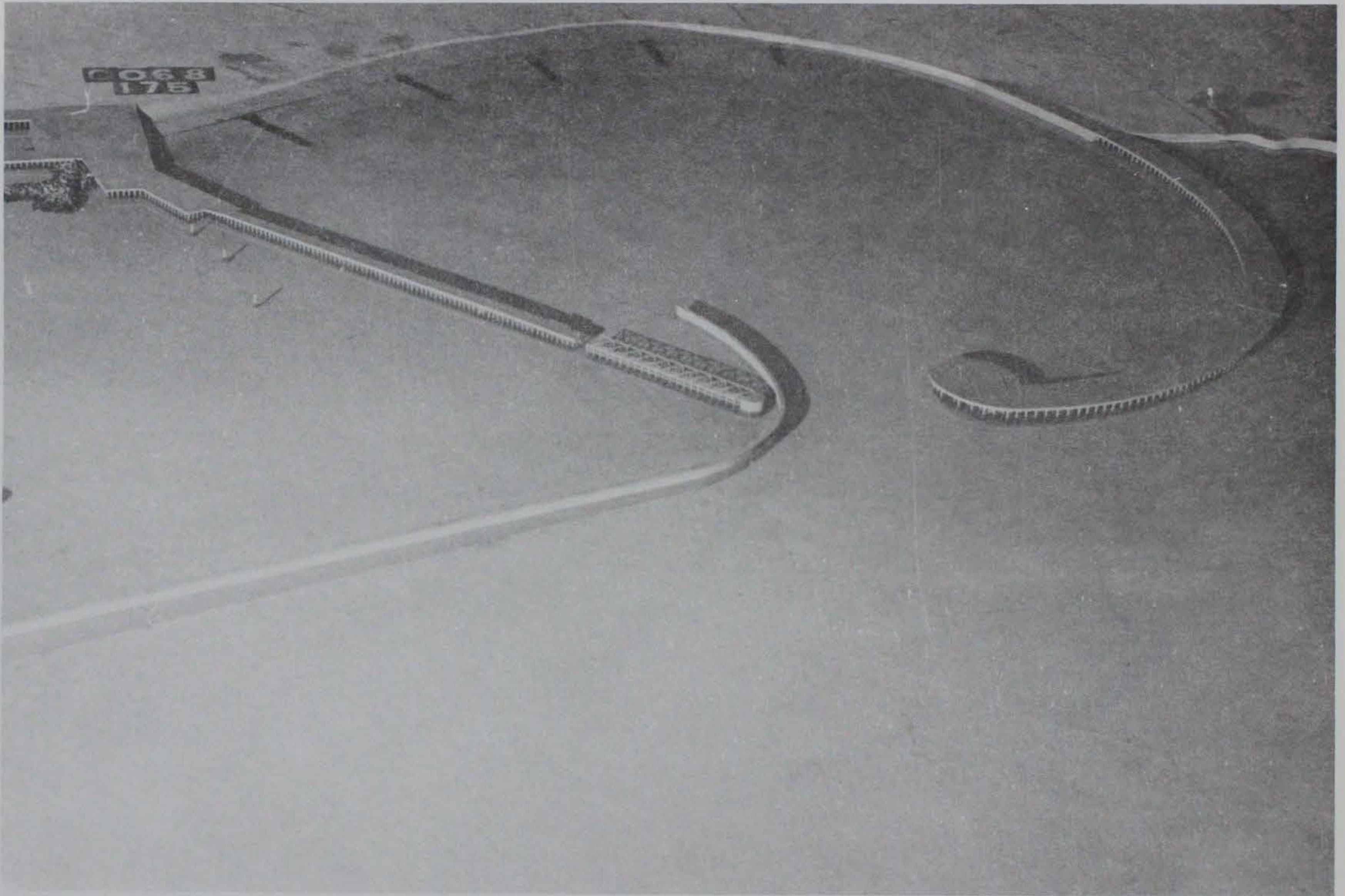
Photo 86. General movement of tracer material for Plan 38; 3.9-sec, 3.3-ft waves from northeast; 0.0-ft swl
