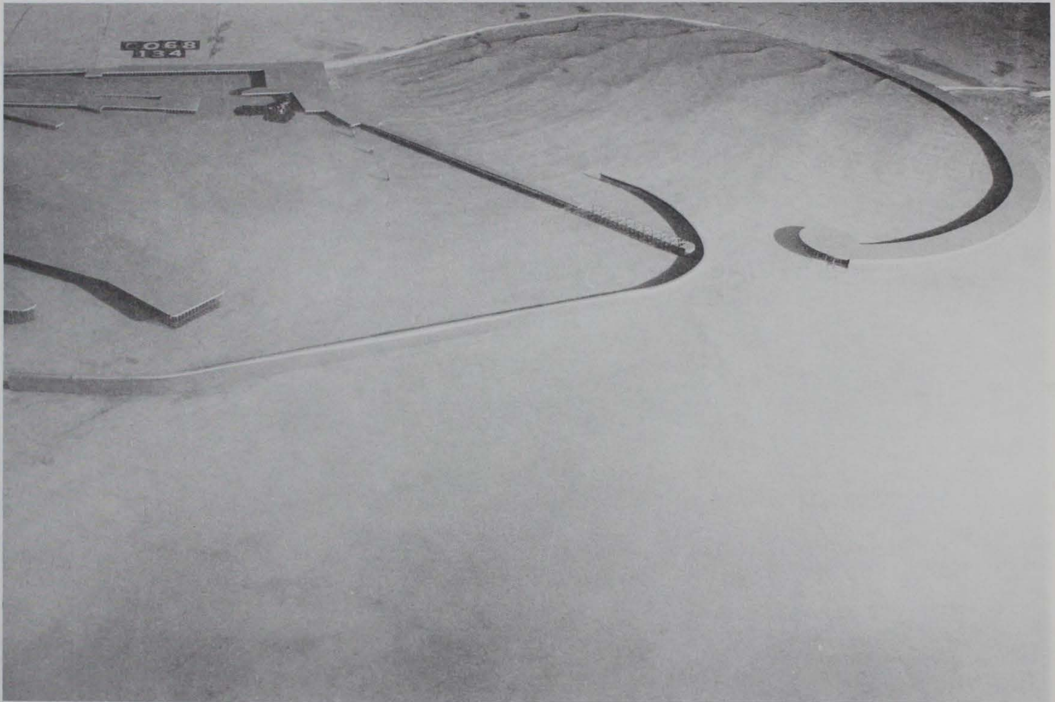
Photo 58. Typical wave patterns for Plan 27; 10-sec, 3-ft waves from west-northwest; +5.7 ft swl
