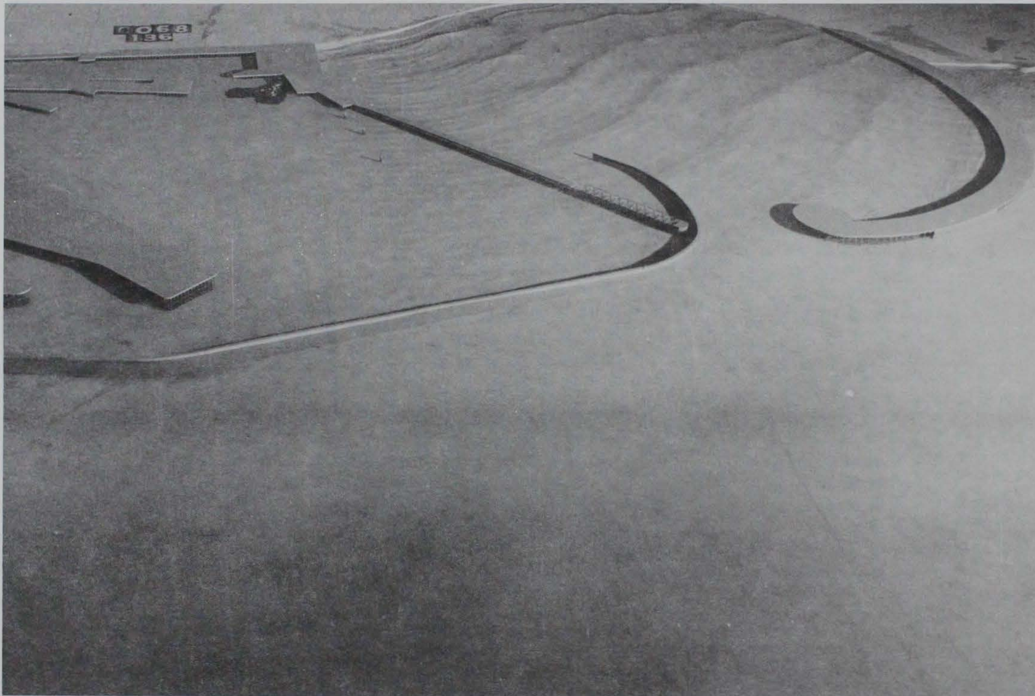
Photo 56. Typical wave patterns for Plan 25; 10-sec, 3-ft waves from west-northwest; +5.7 ft swl
