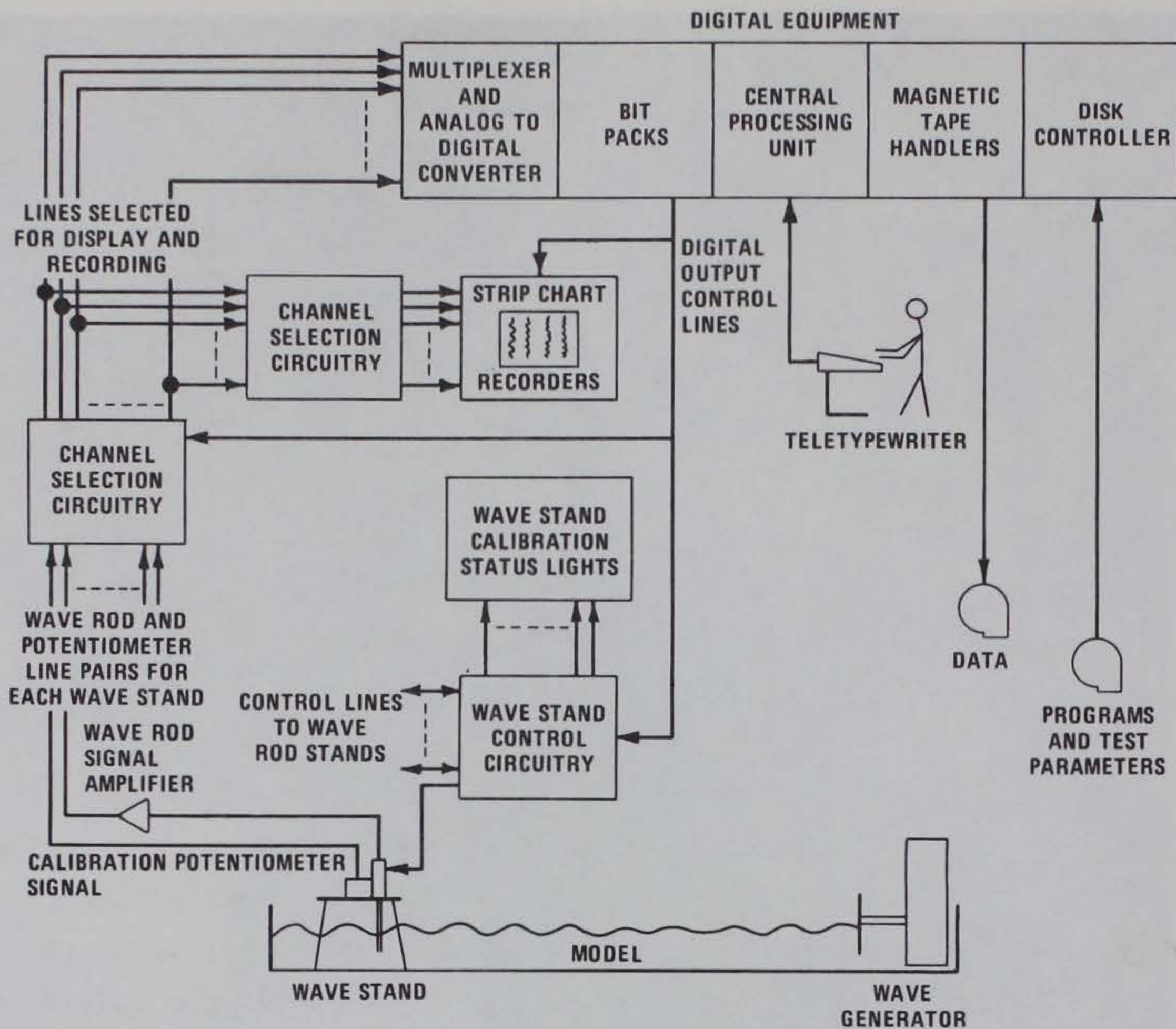
Figure 5. Automated Data Acquisition and Control System (ADACS)
