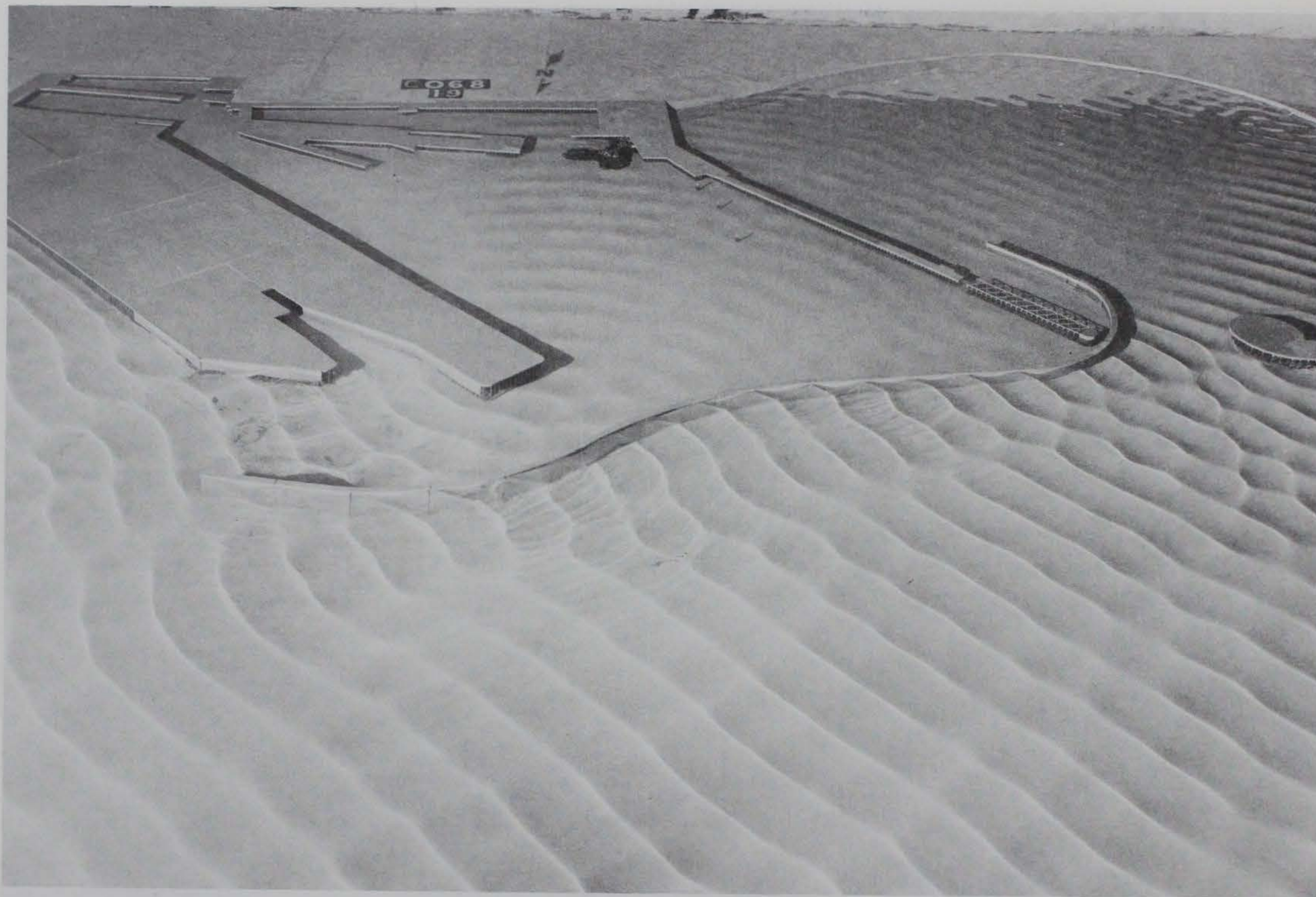
Photo 44. Typical wave patterns for Plan 13; 3.9-sec, 3.3-ft waves from northeast; +5.7 ft swl
