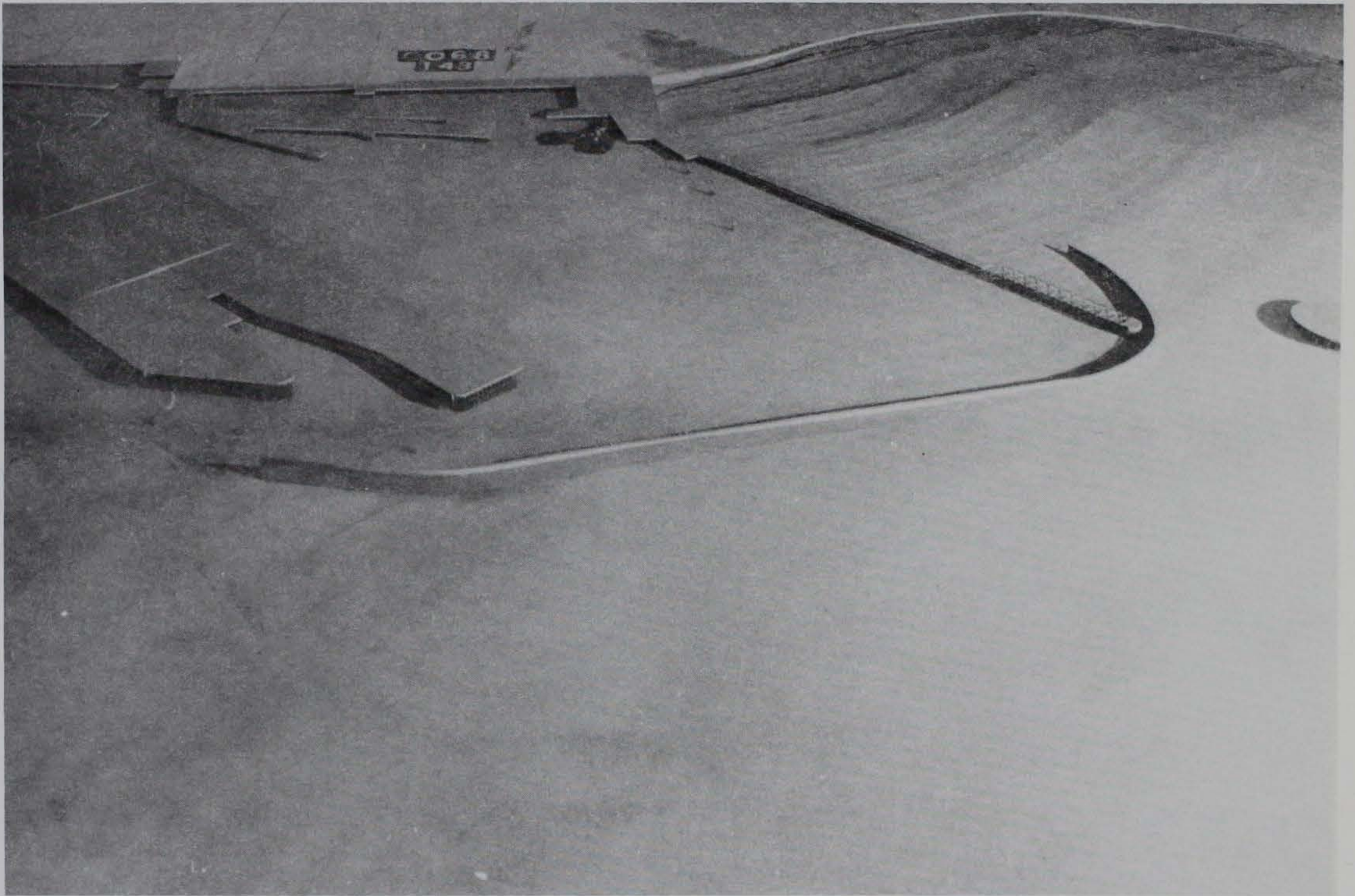
Photo 83. Typical wave patterns for Plan 38; 10-sec, 2-ft waves from west-northwest; +5.7 ft swl
