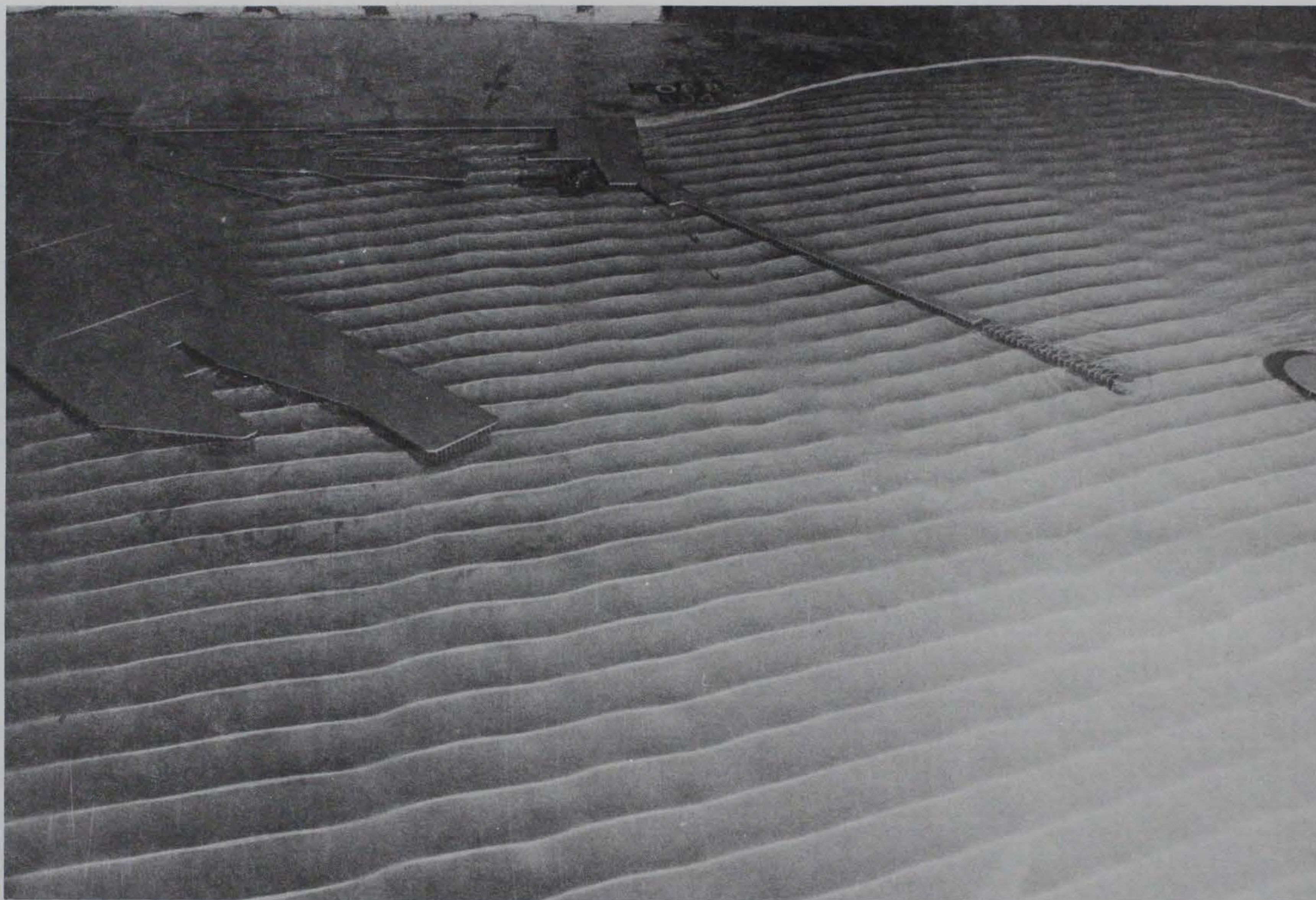
Photo 8. Typical wave patterns for existing conditions; 3.6-sec, 3.3-ft waves from north-northwest; +5.7 ft swl
