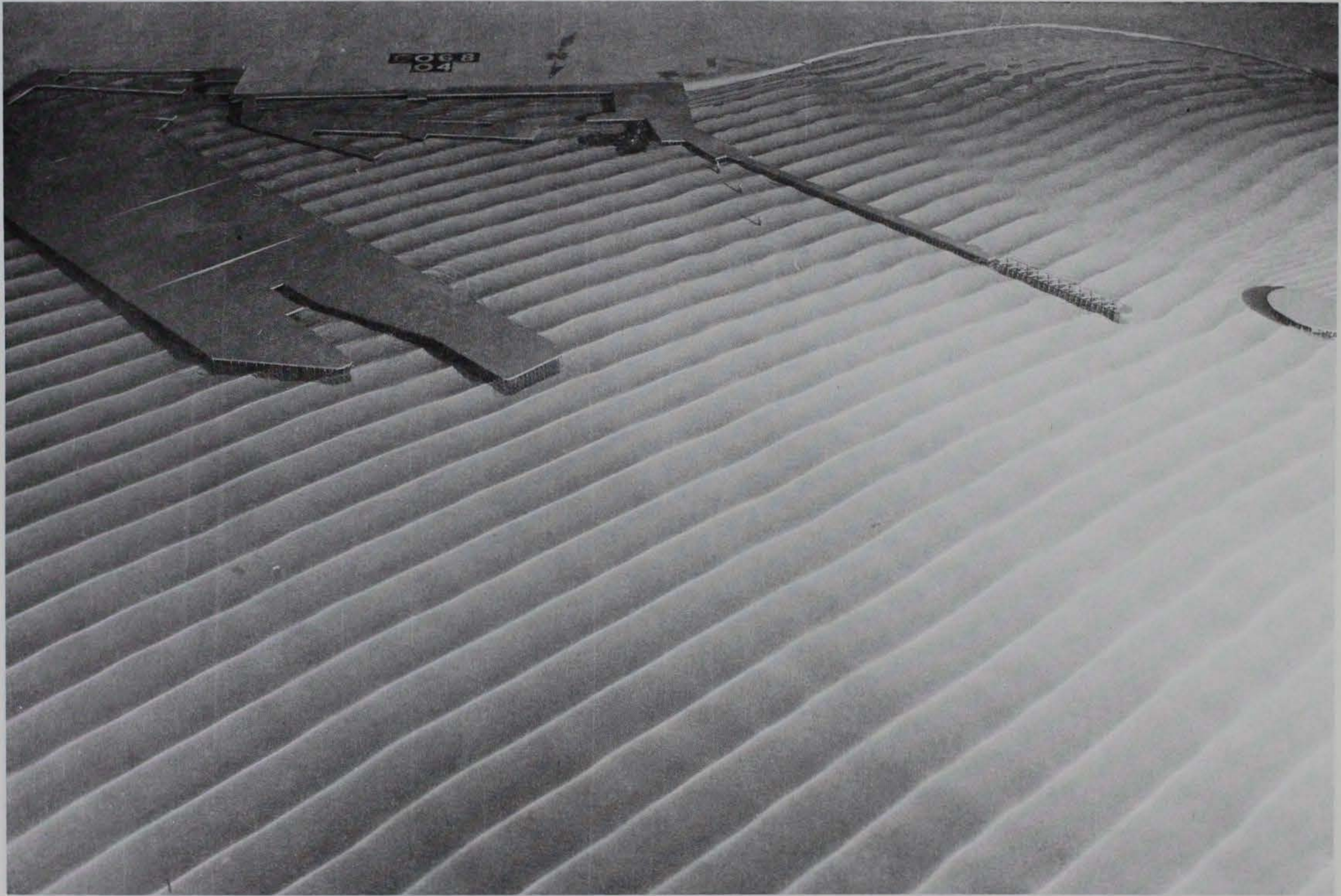
Photo 9. Typical wave patterns for existing conditions; 3.6-sec, 2-ft waves from northwest; +5.7 ft swl
