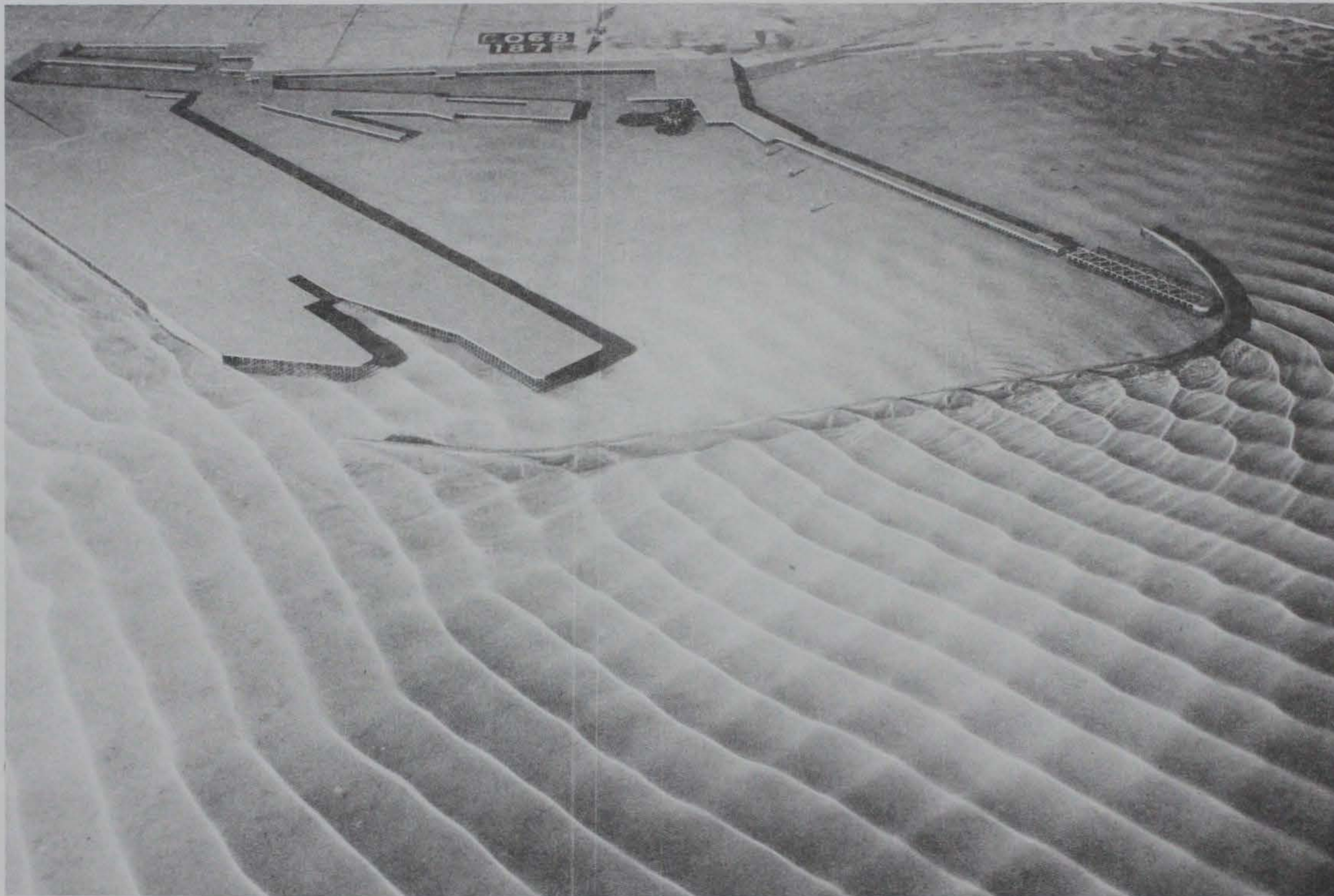
Photo 110. Typical wave patterns for Plan 50; 3.9-sec, 3.3-ft waves from northeast; +5.7 ft swl
