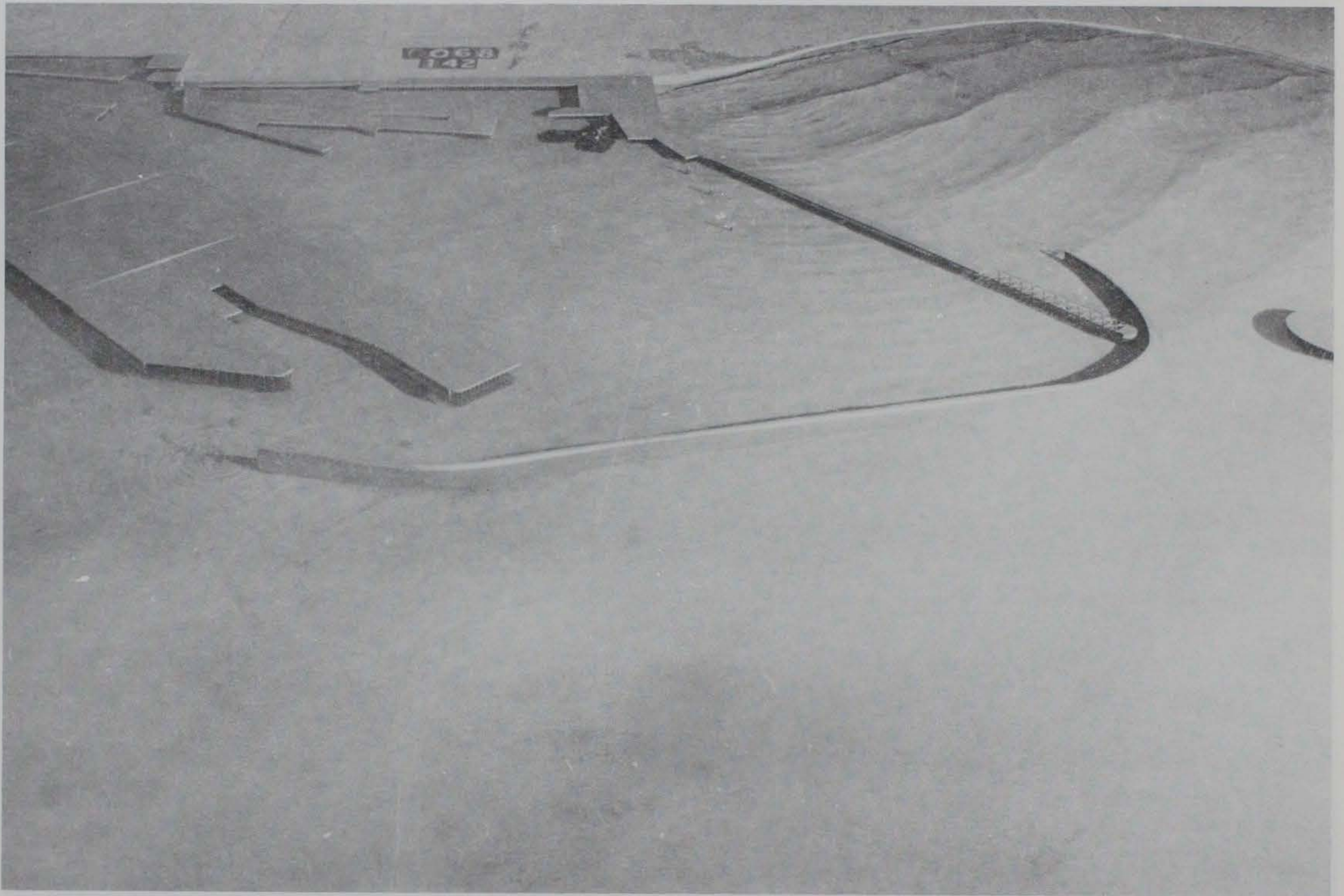
Photo 84. Typical wave patterns for Plan 38; 10-sec, 3-ft waves from west-northwest; +5.7 ft swl
