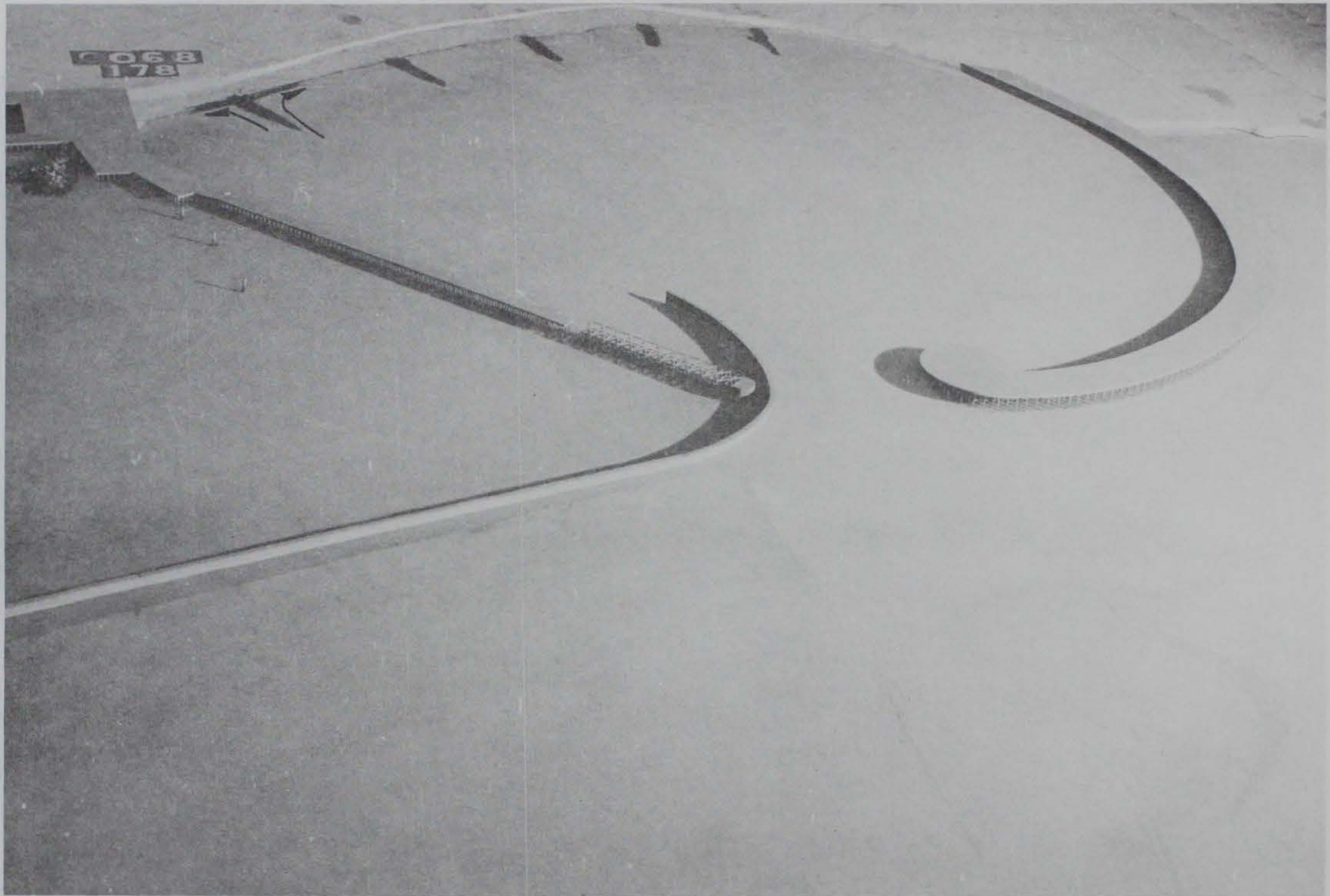
Photo 96. General movement of tracer material for Plan 38; 3.6-sec, 3.4-ft waves from west-northwest; 0.0-ft swl
