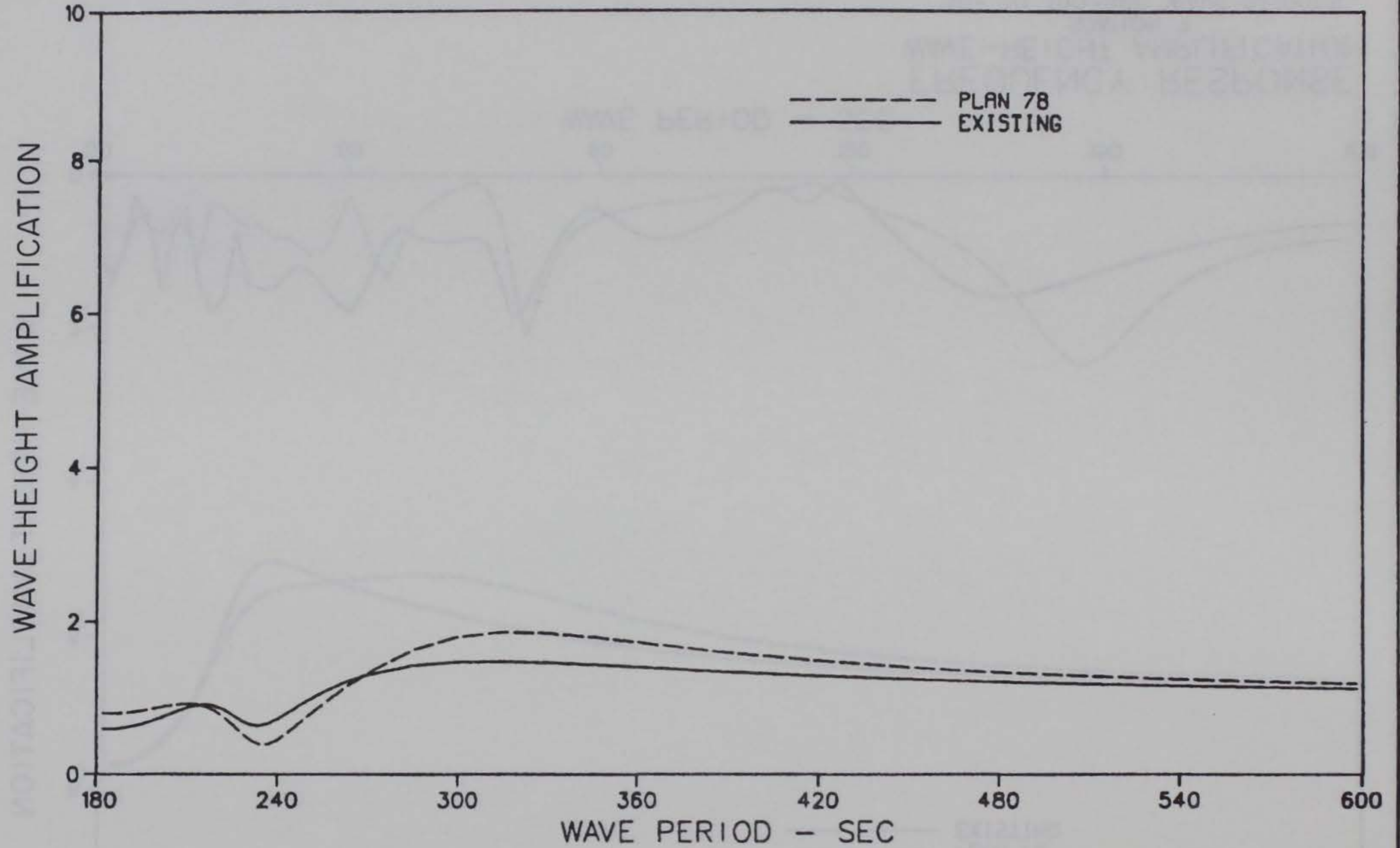
FREQUENCY RESPONSE WAVE-HEIGHT AMPLIFICATION STATION 7 180- TO 600-SEC WAVE PERIODS
