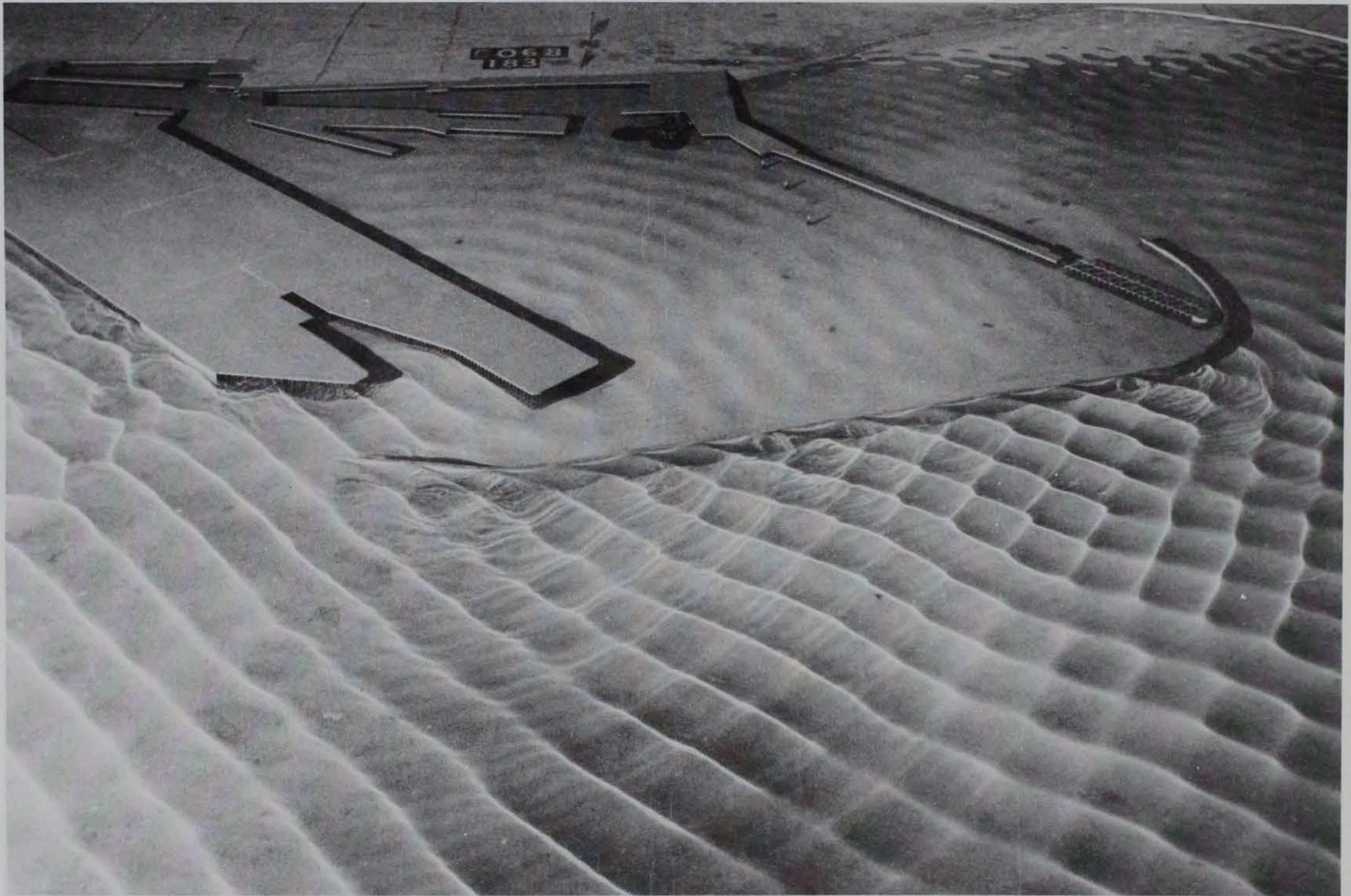
Photo 109. Typical wave patterns for Plan 49; 3.9-sec, 3.3-ft waves from northeast; +5.7 ft swl
