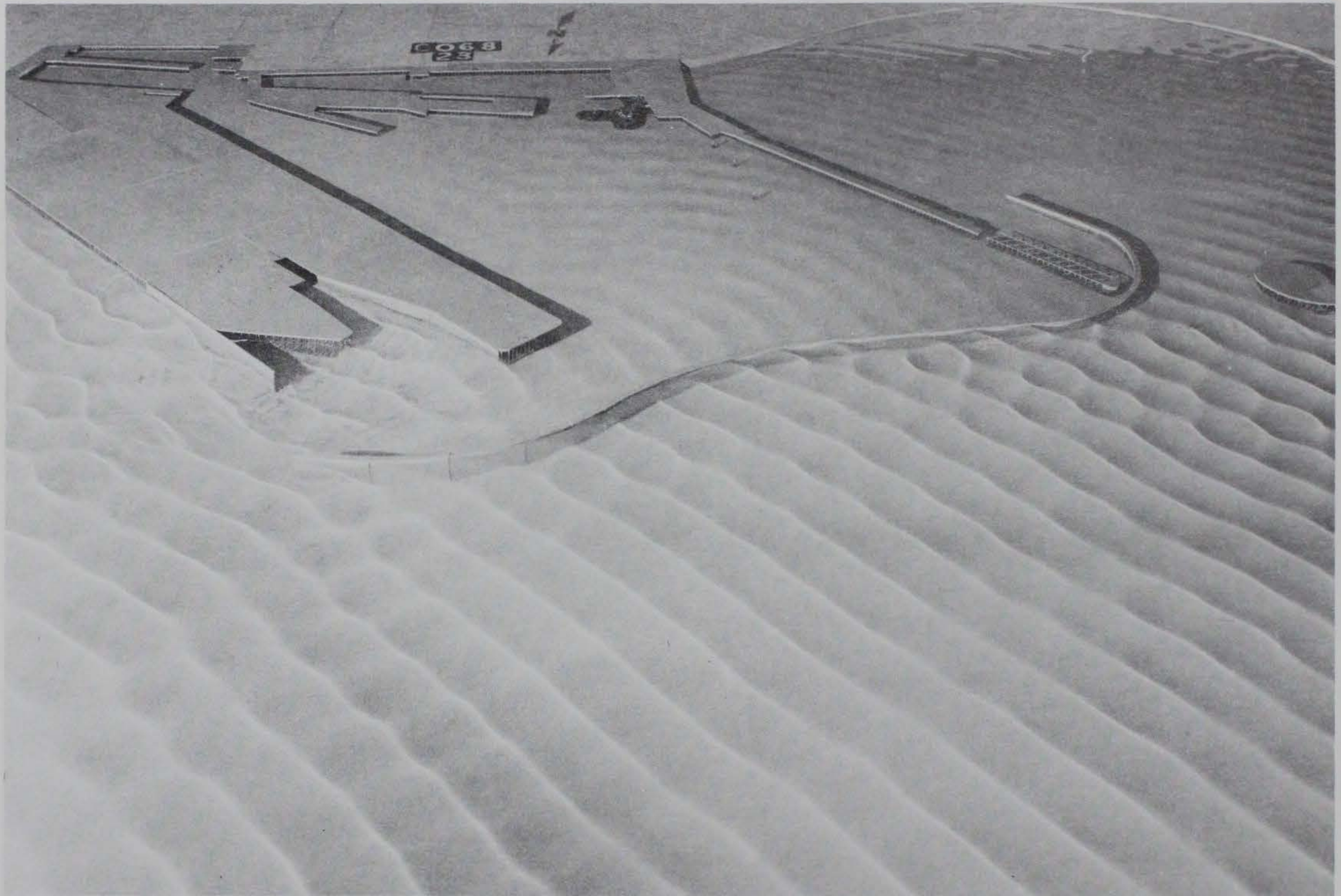
Photo 48. Typical wave patterns for Plan 17; 3.9-sec, 3.3-ft waves from northeast; +5.7 ft swl
