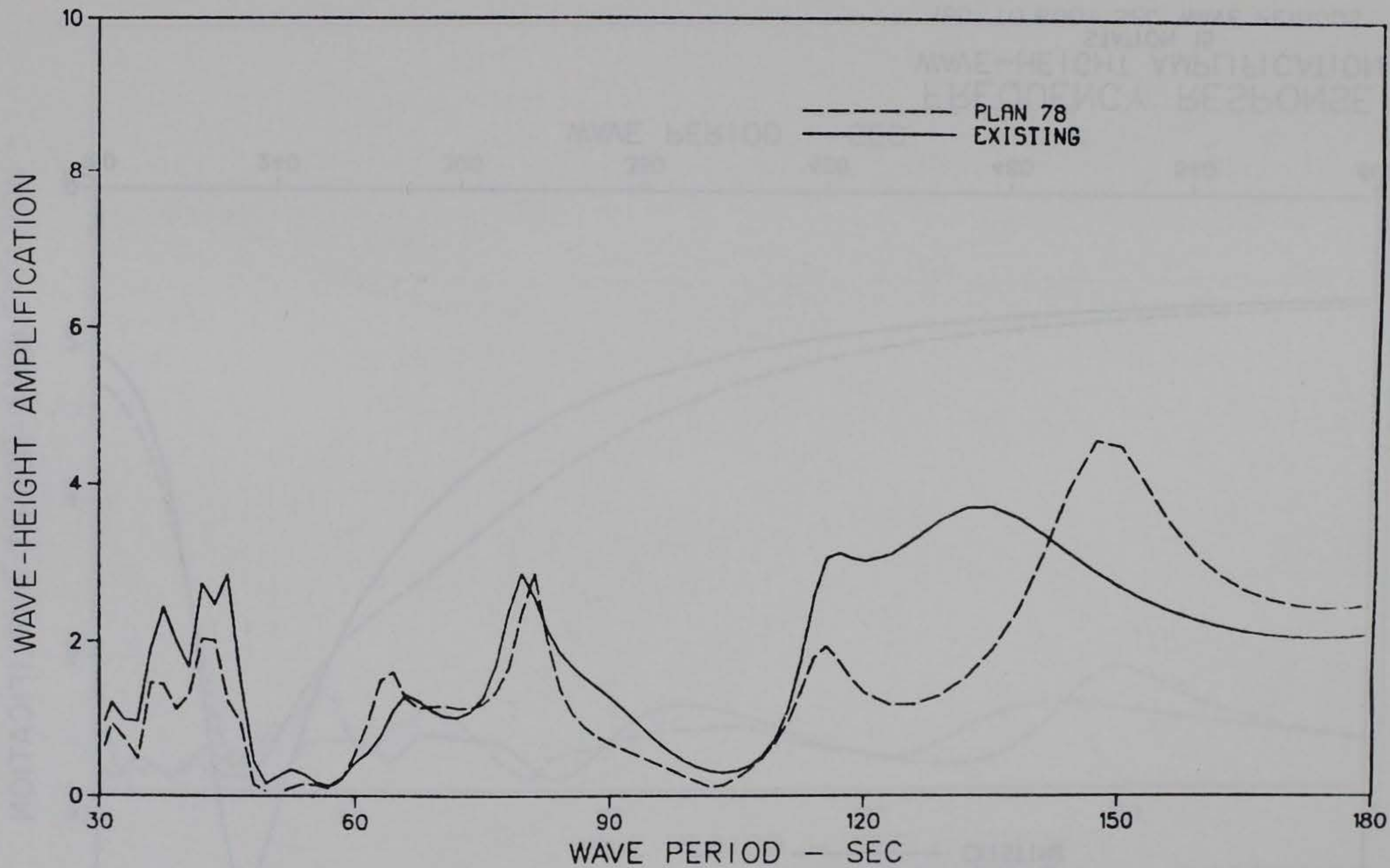
FREQUENCY RESPONSE WAVE-HEIGHT AMPLIFICATION STATION 15 30- TO 180-SEC WAVE PERIODS
