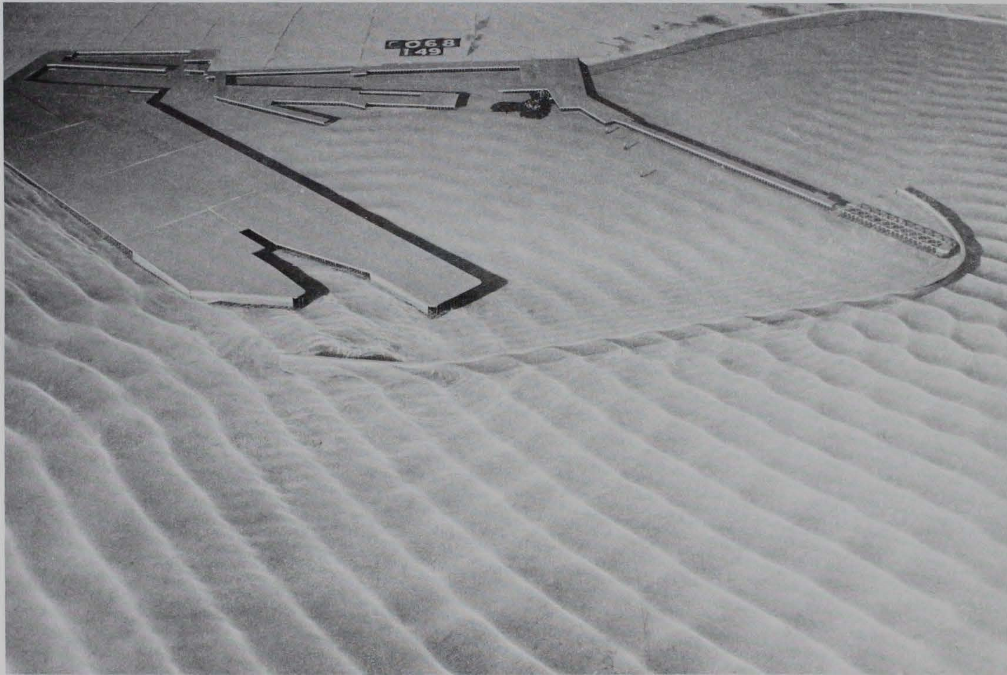
Photo 67. Typical wave patterns for Plan 35; 3.9-sec, 3.3-ft waves from northeast; +5.7 ft swl
