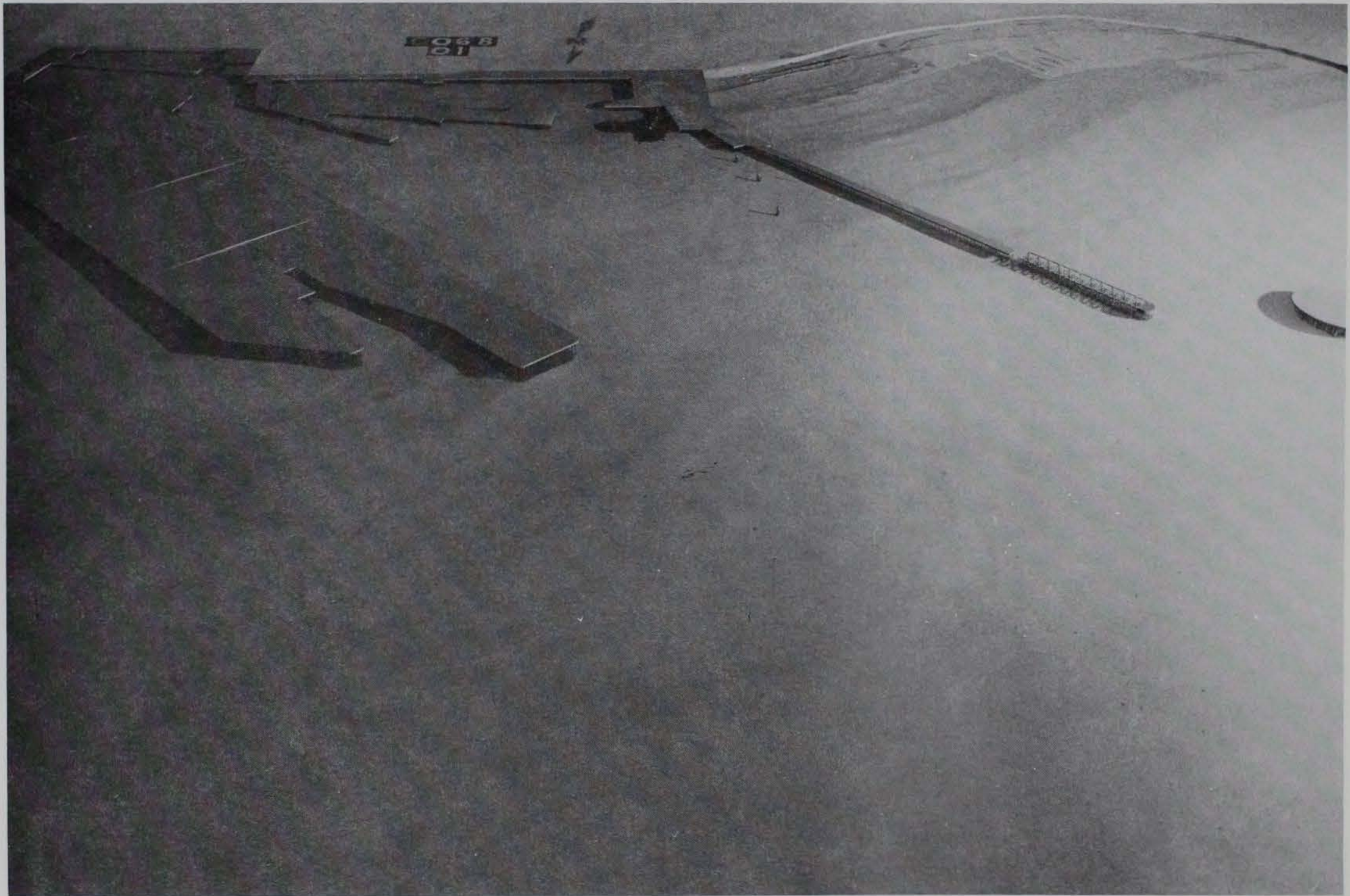
Photo 13. Typical wave patterns for existing conditions; 10-sec, 2-ft waves from west-northwest; +5.7 ft swl
