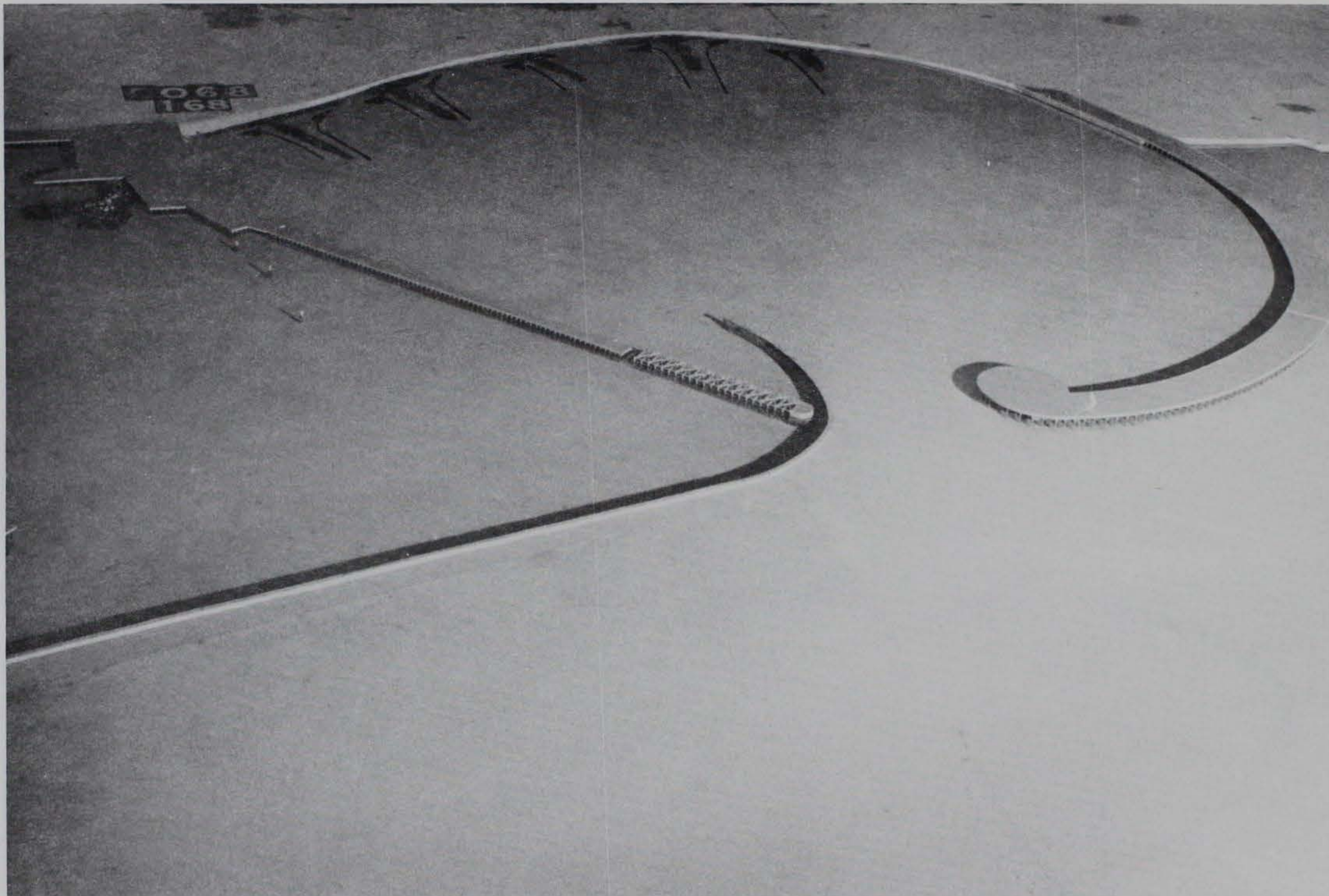
Photo 93. General movement of tracer material for Plan 38; 3.6-sec, 3.3-ft waves from north-northwest; +5.7 ft swl
