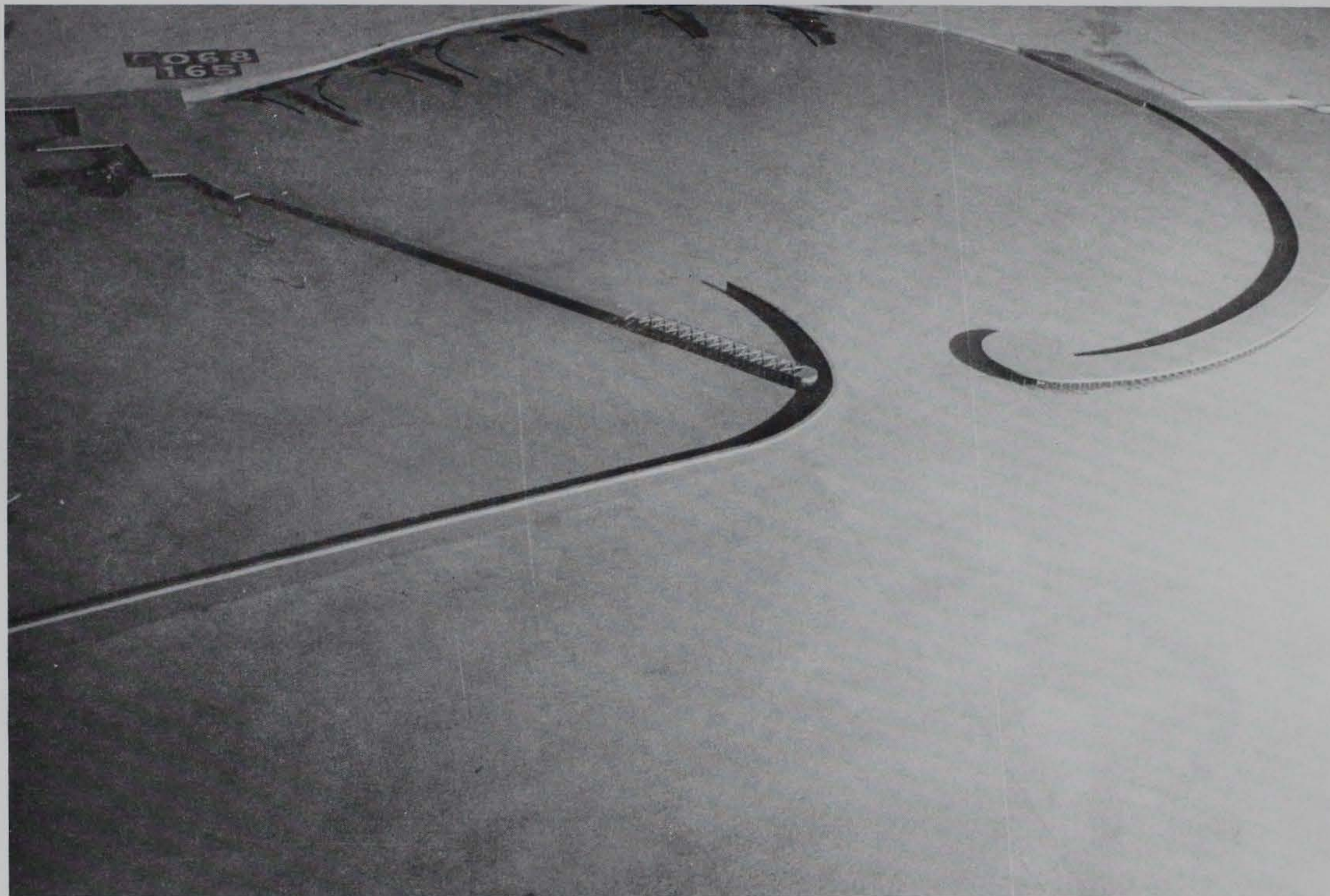
Photo 95. General movement of tracer material for Plan 38; 3.8-sec, 4.1-ft waves from northwest; +5.7 ft swl
