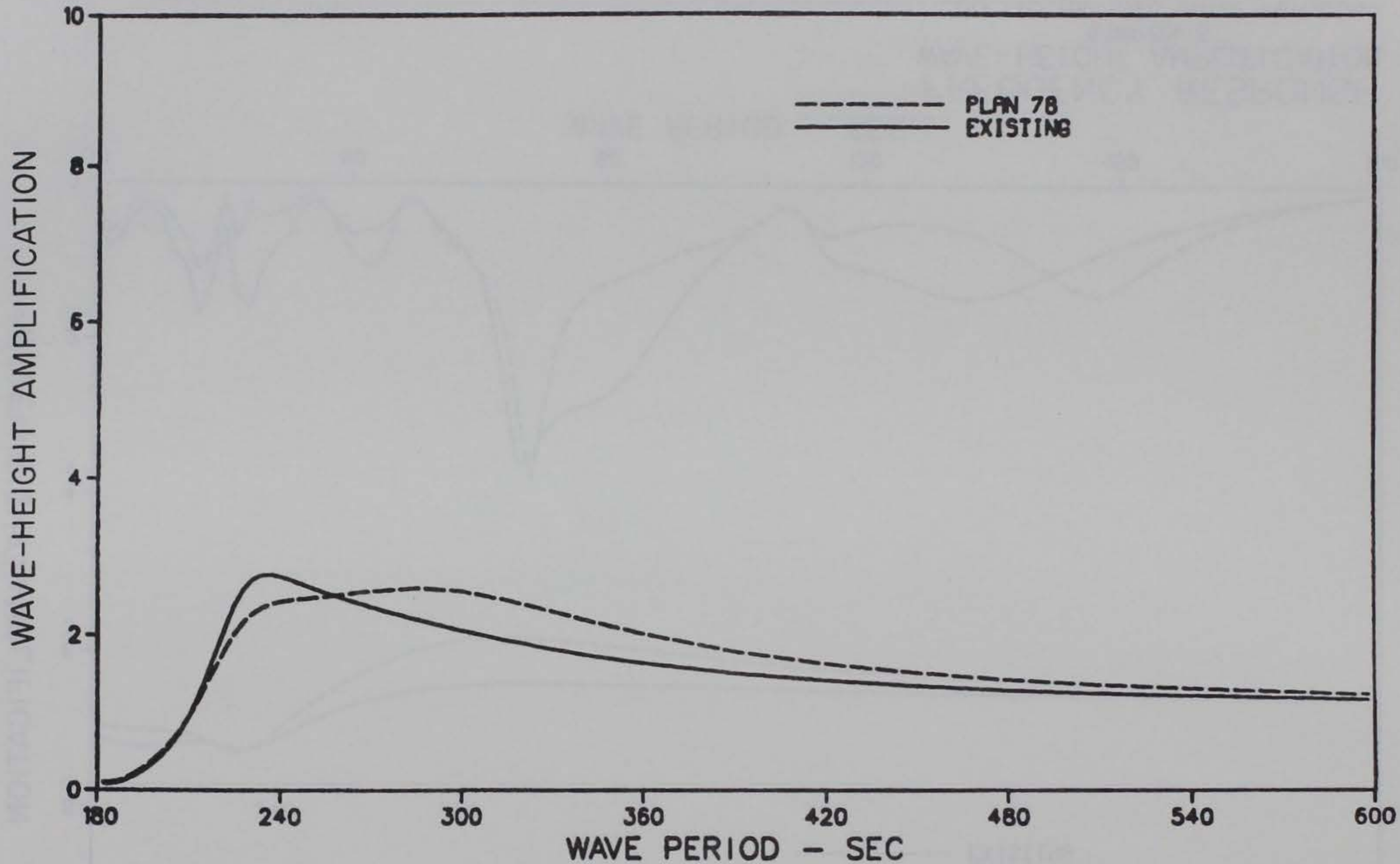
FREQUENCY RESPONSE WAVE-HEIGHT AMPLIFICATION STATION 5 180- TO 600-SEC WAVE PERIODS
