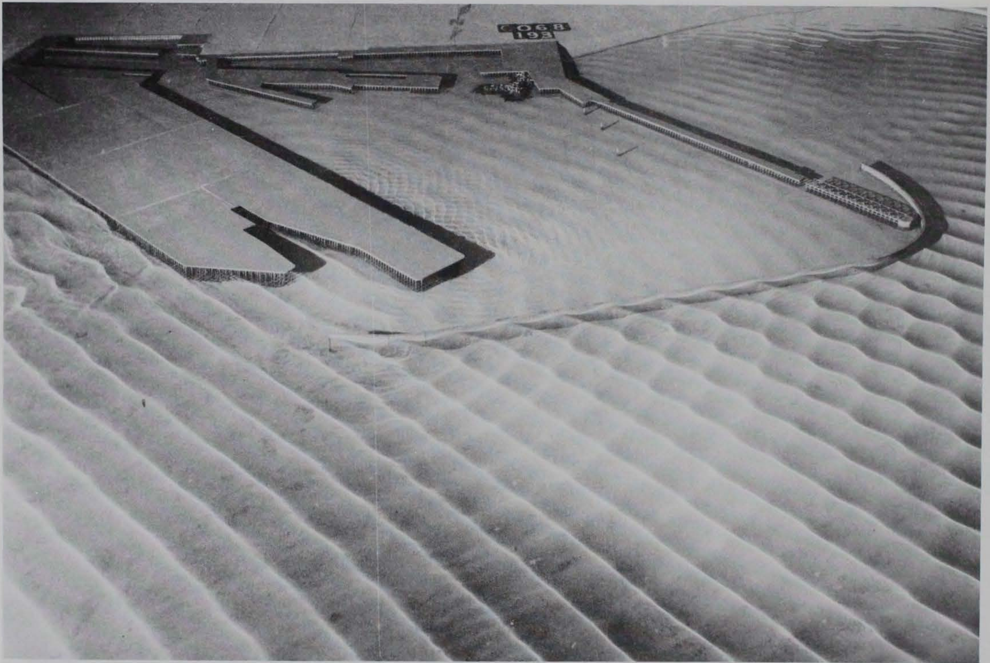
Photo 127. Typical wave patterns for Plan 67; 3.9-sec, 3.3-ft waves from northeast; 0.0-ft swl
