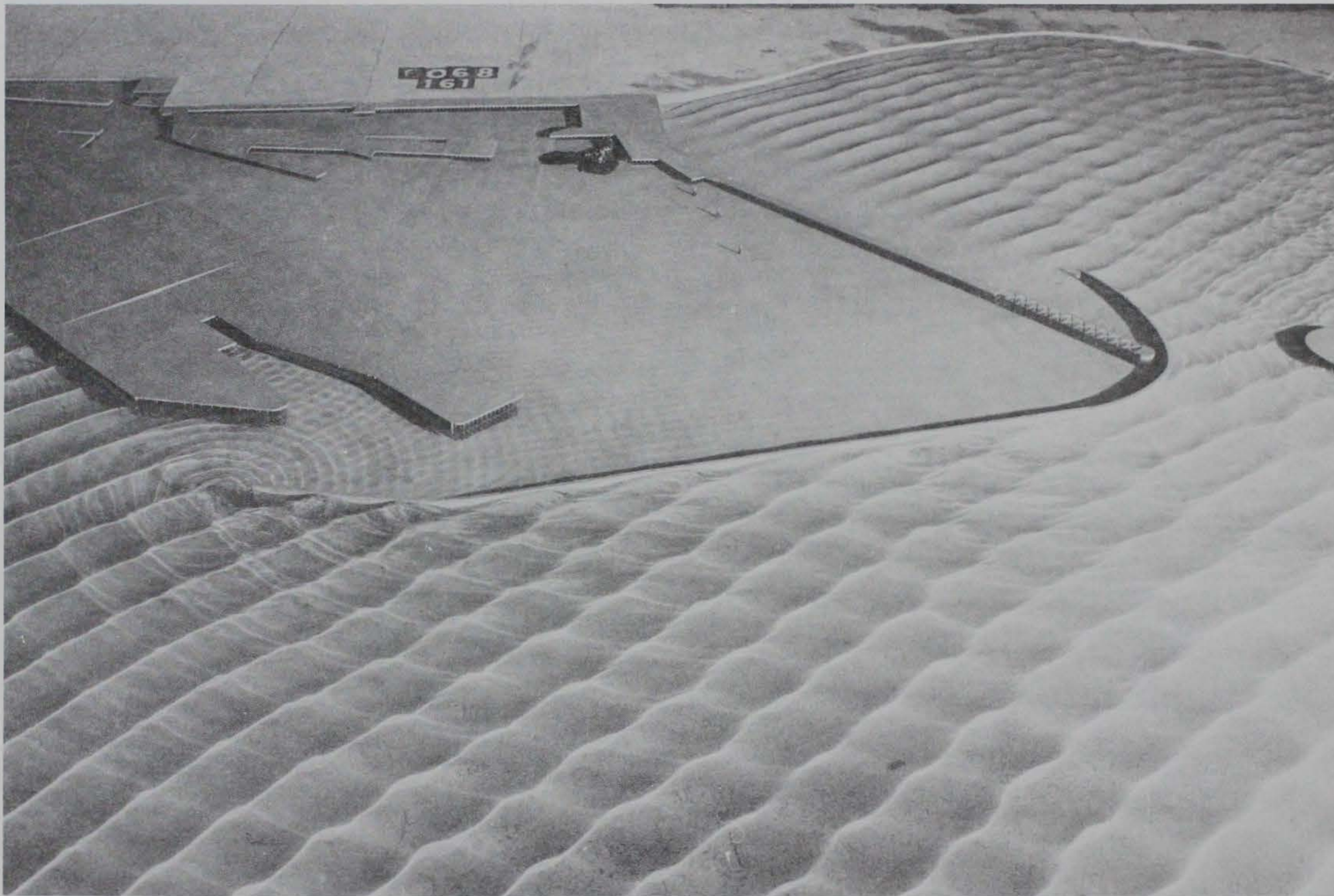
Photo 80 Typical wave patterns for Plan 38; 3.8-sec, 4.1-ft waves from northwest; +5.7 ft swl
