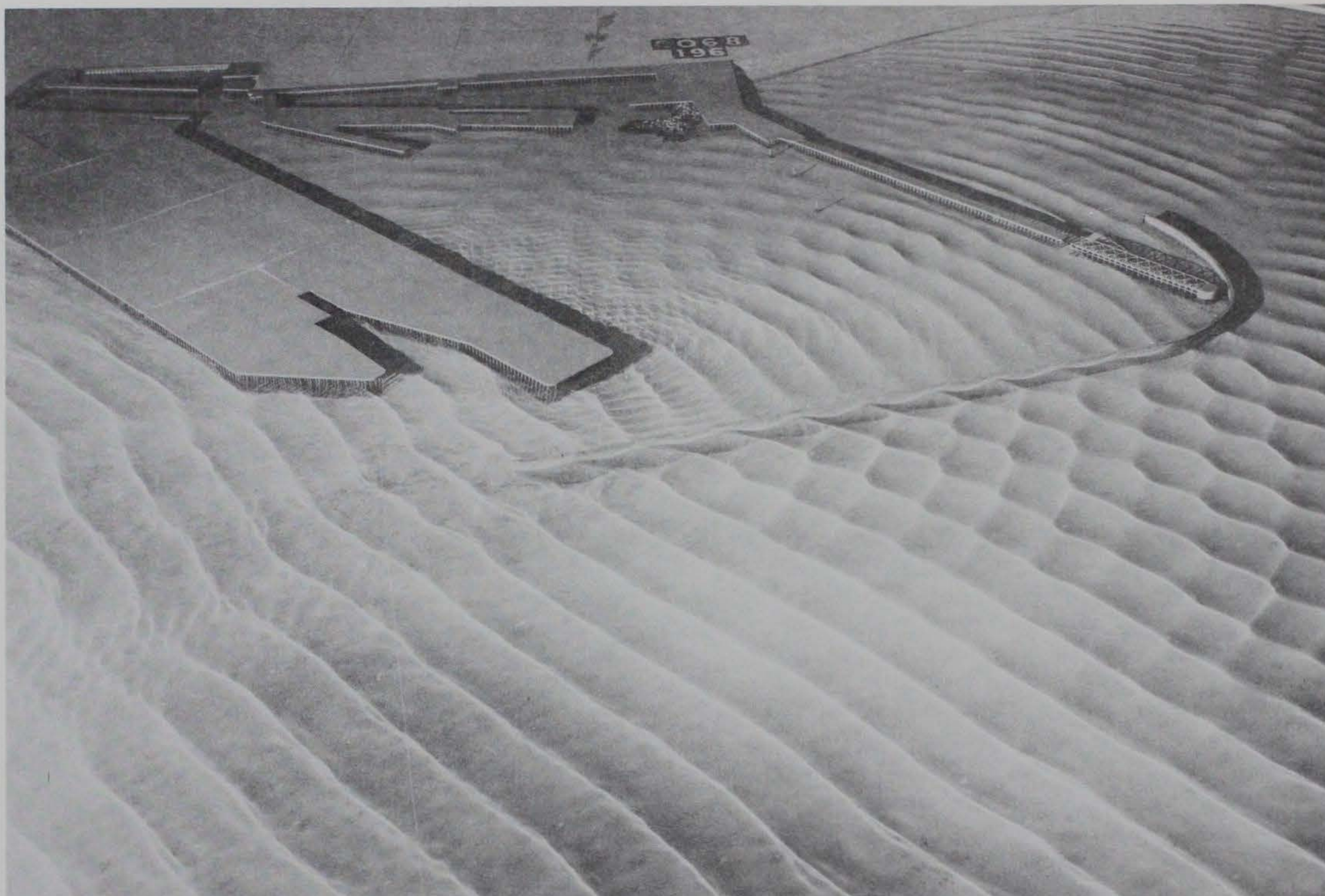
Photo 128. Typical wave patterns for Plan 68; 3.9-sec, 3.3-ft waves from northeast; 0.0-ft swl
