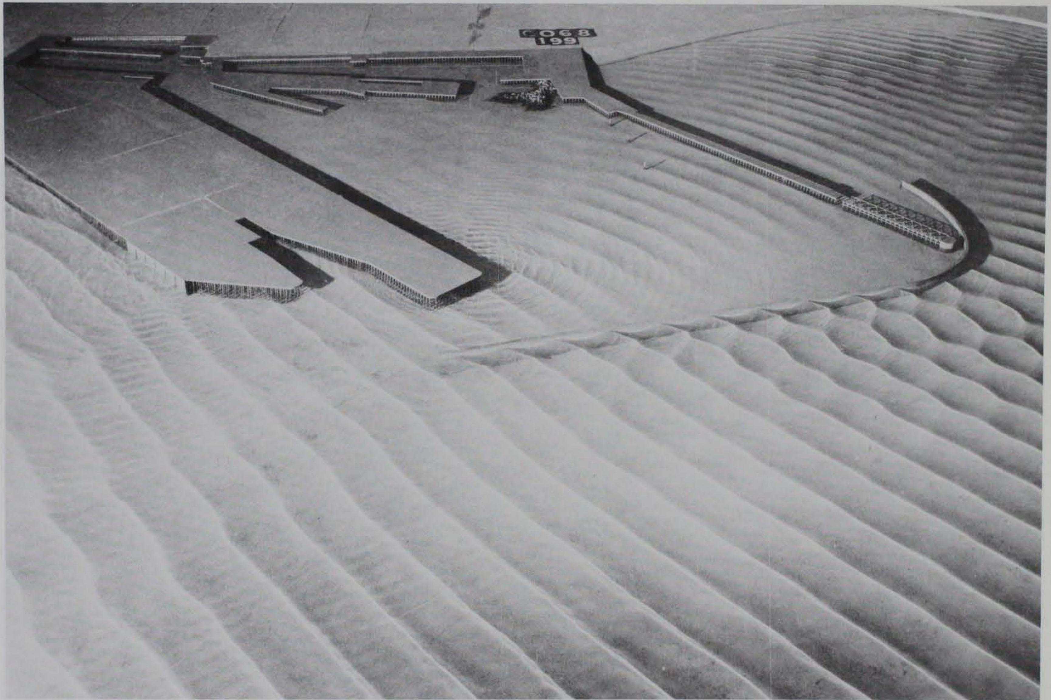
Photo 135. Typical wave patterns for Plan 75; 3.9-sec, 3.3-ft waves from northeast; 0.0-ft swl
