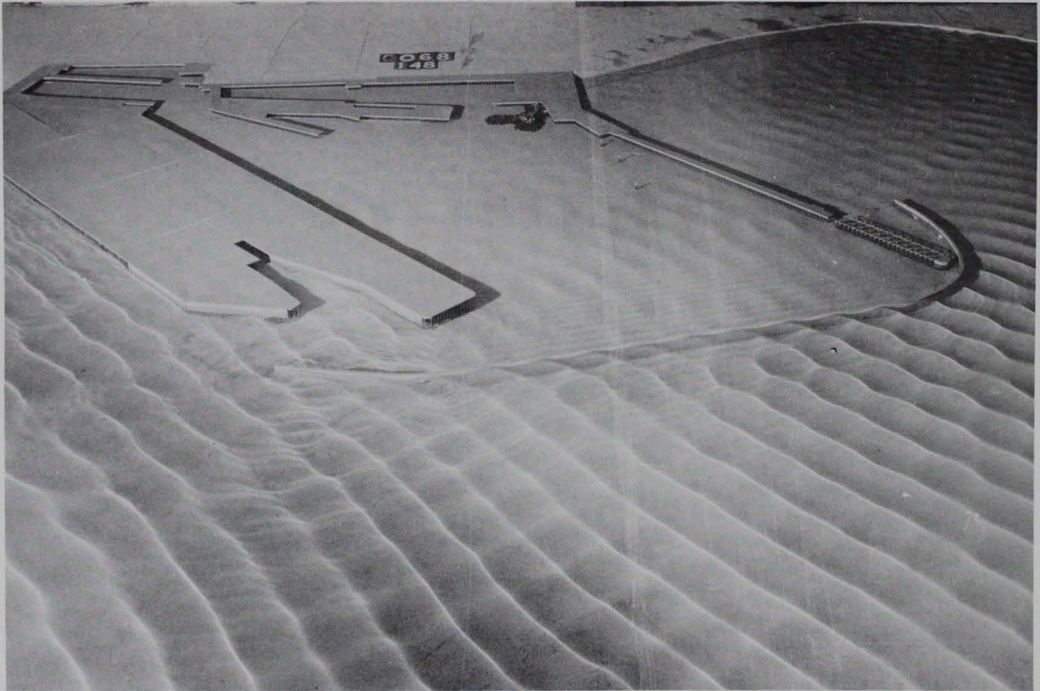
Photo 69. Typical wave patterns for Plan 37; 3.9-sec, 3.3-ft waves from northeast; +5.7 ft swl
