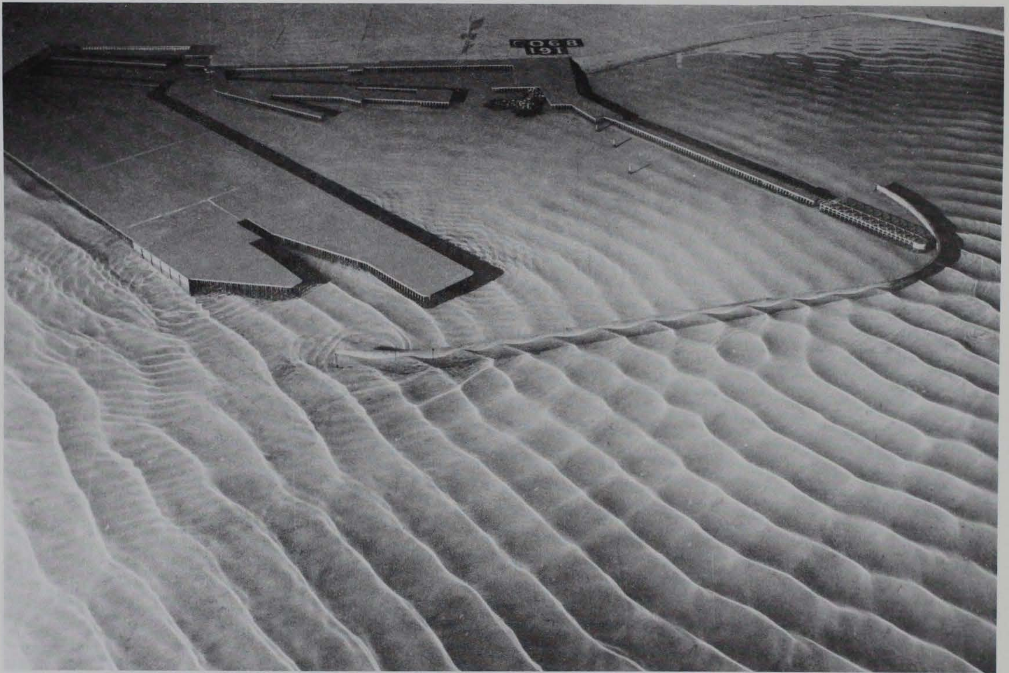
Photo 133. Typical wave patterns for Plan 73; 3.9-sec, 3.3-ft waves from northeast; 0.0-ft swl
