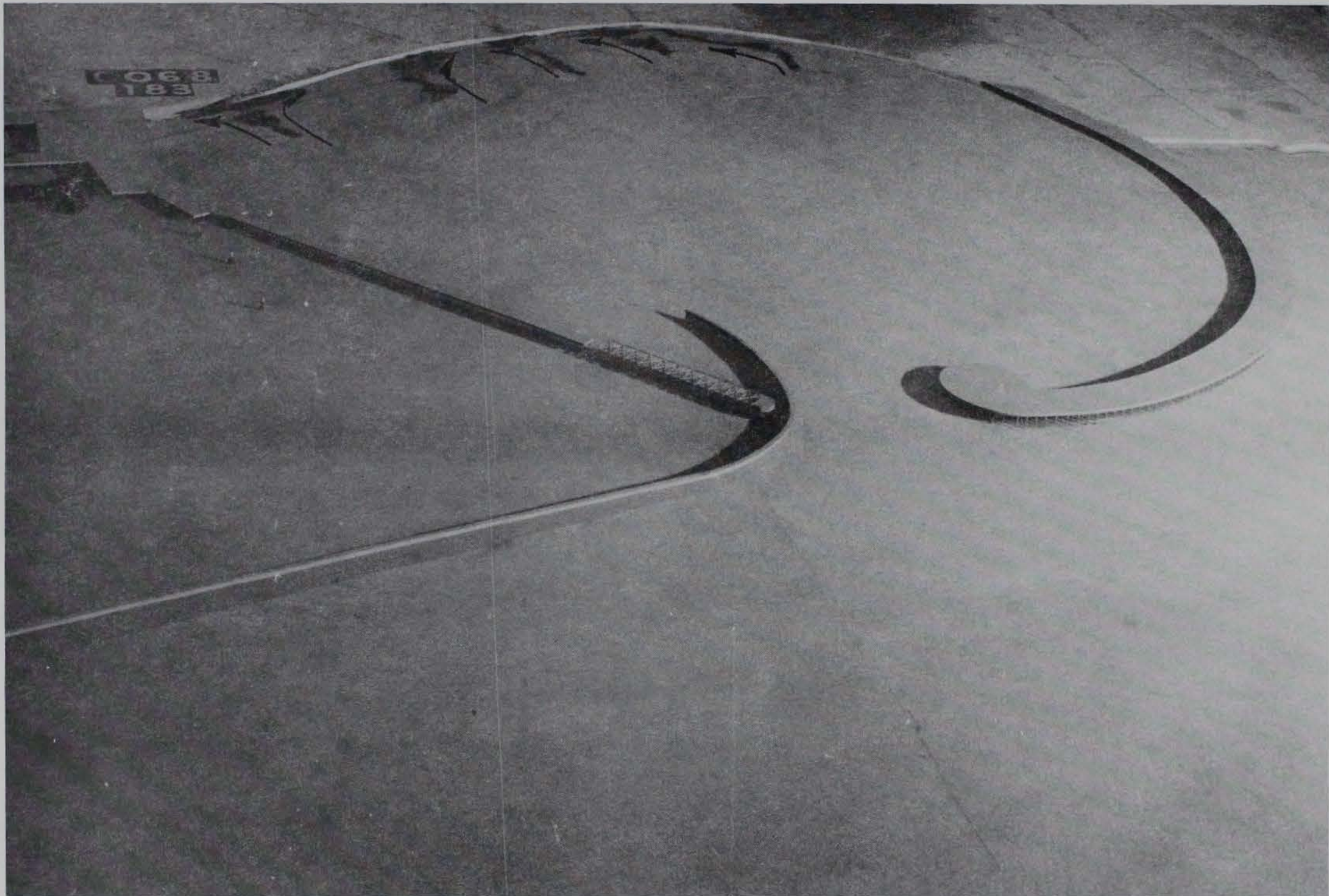
Photo 99. General movement of tracer material for Plan 38; 10-sec, 2-ft waves from west-northwest; +5.7 ft swl
