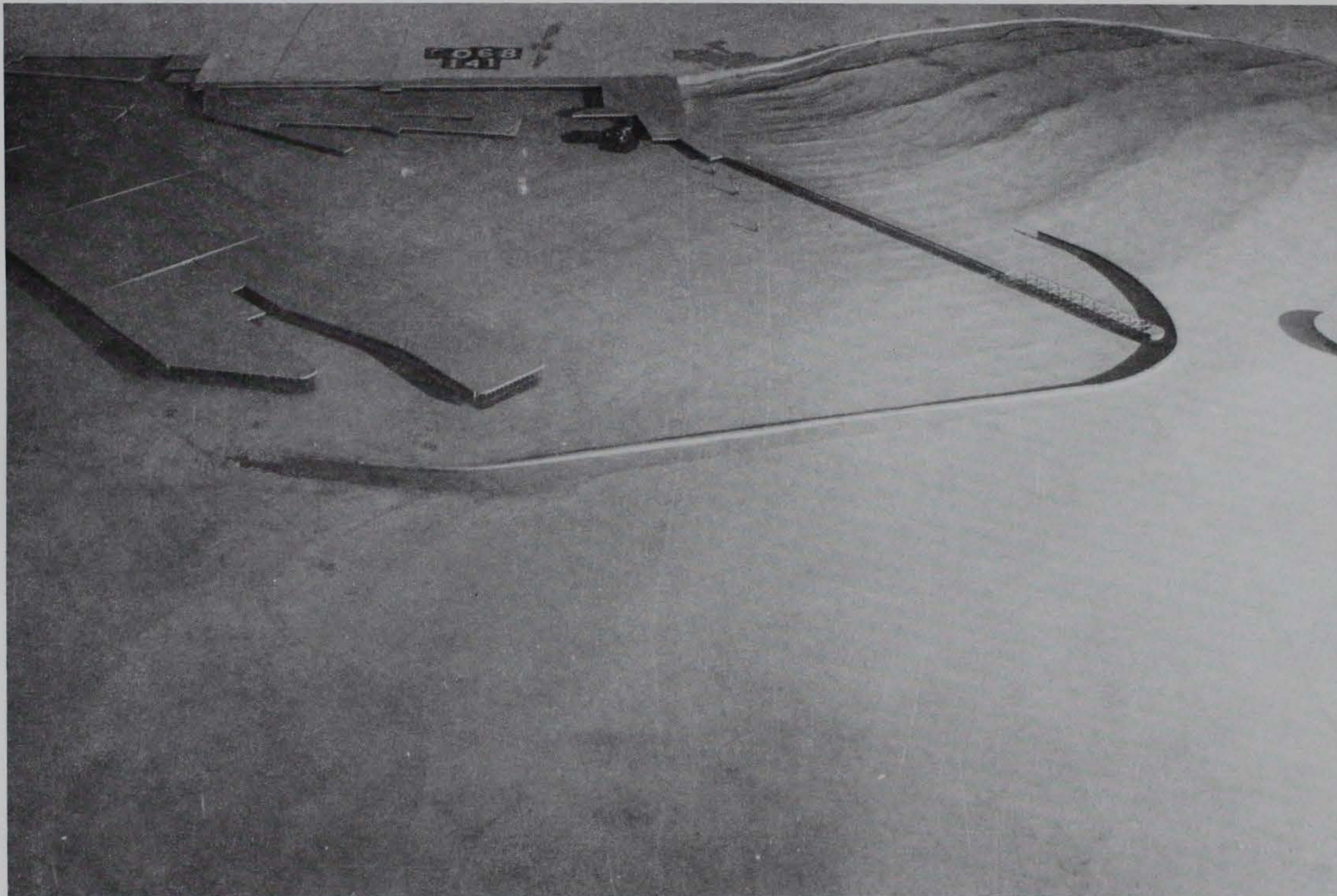
Photo 85. Typical wave patterns for Plan 40; 10-sec, 2.5-ft waves from west-northwest; +5.7 ft swl
