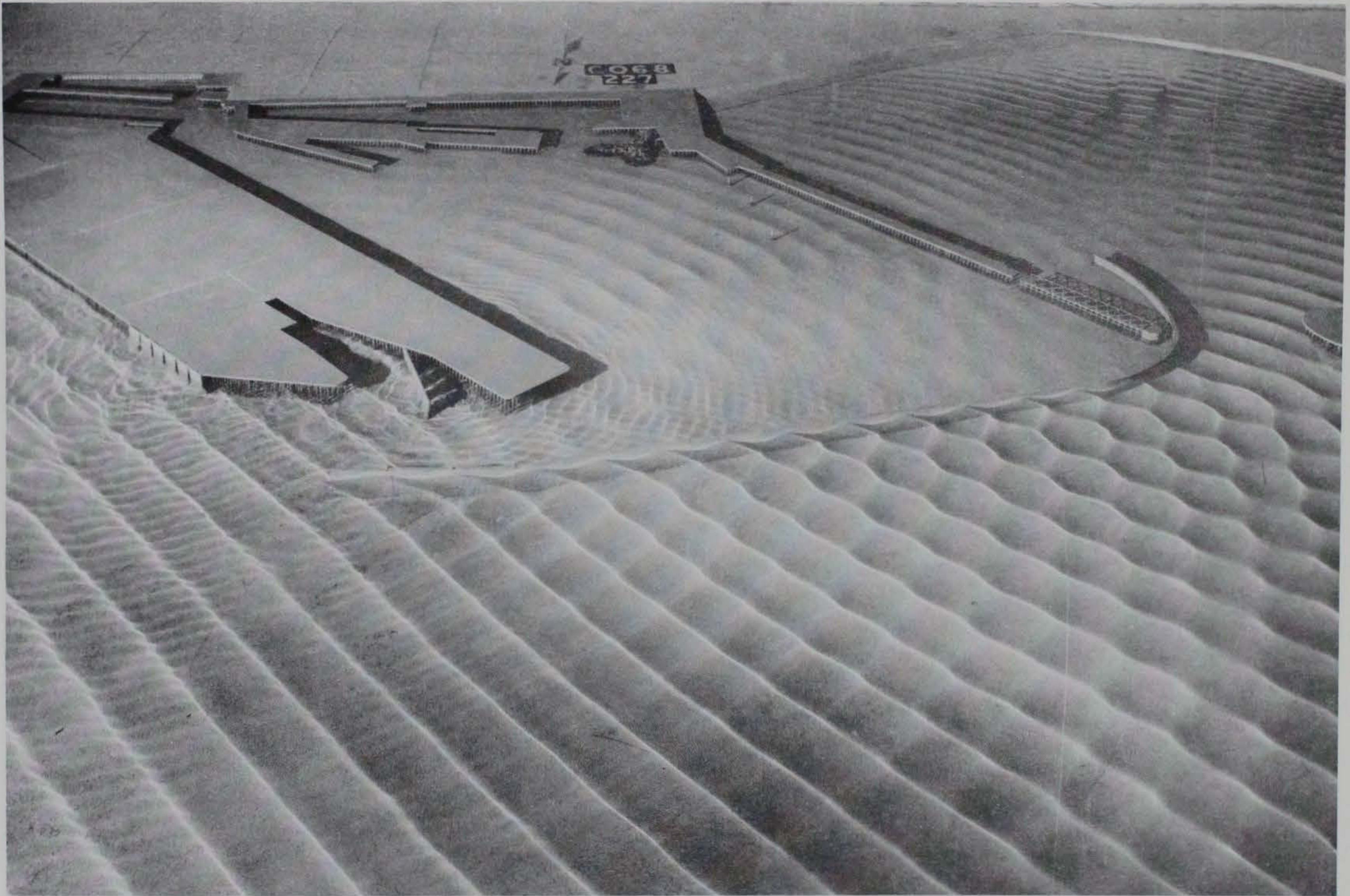
Photo 145. Typical wave patterns for Plan 85; 3.9-sec, 3.3-ft waves from northeast; 0:0-ft swl
