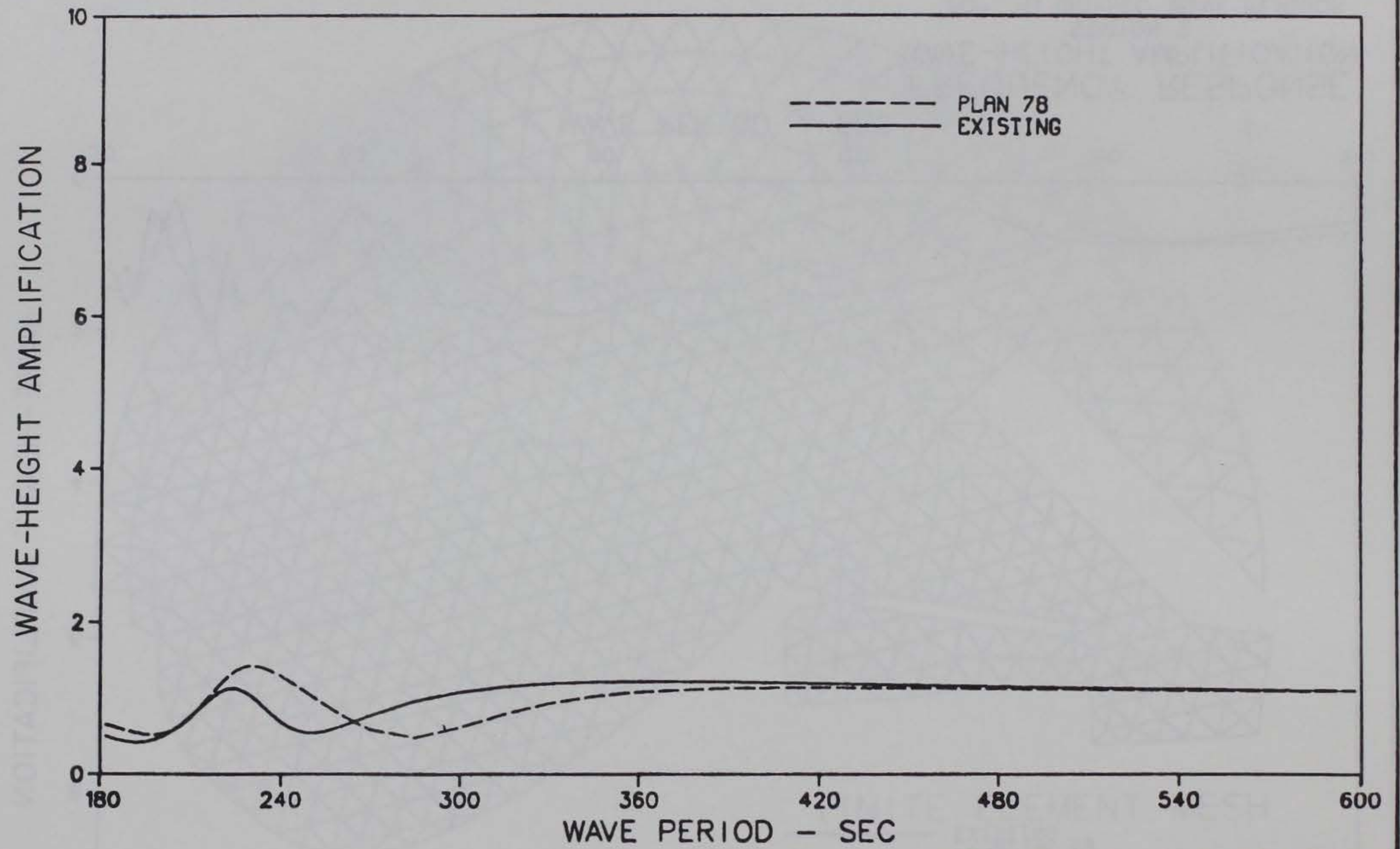
FREQUENCY RESPONSE WAVE-HEIGHT AMPLIFICATION STATION 2 180-TO 600-SEC WAVE PERIODS
