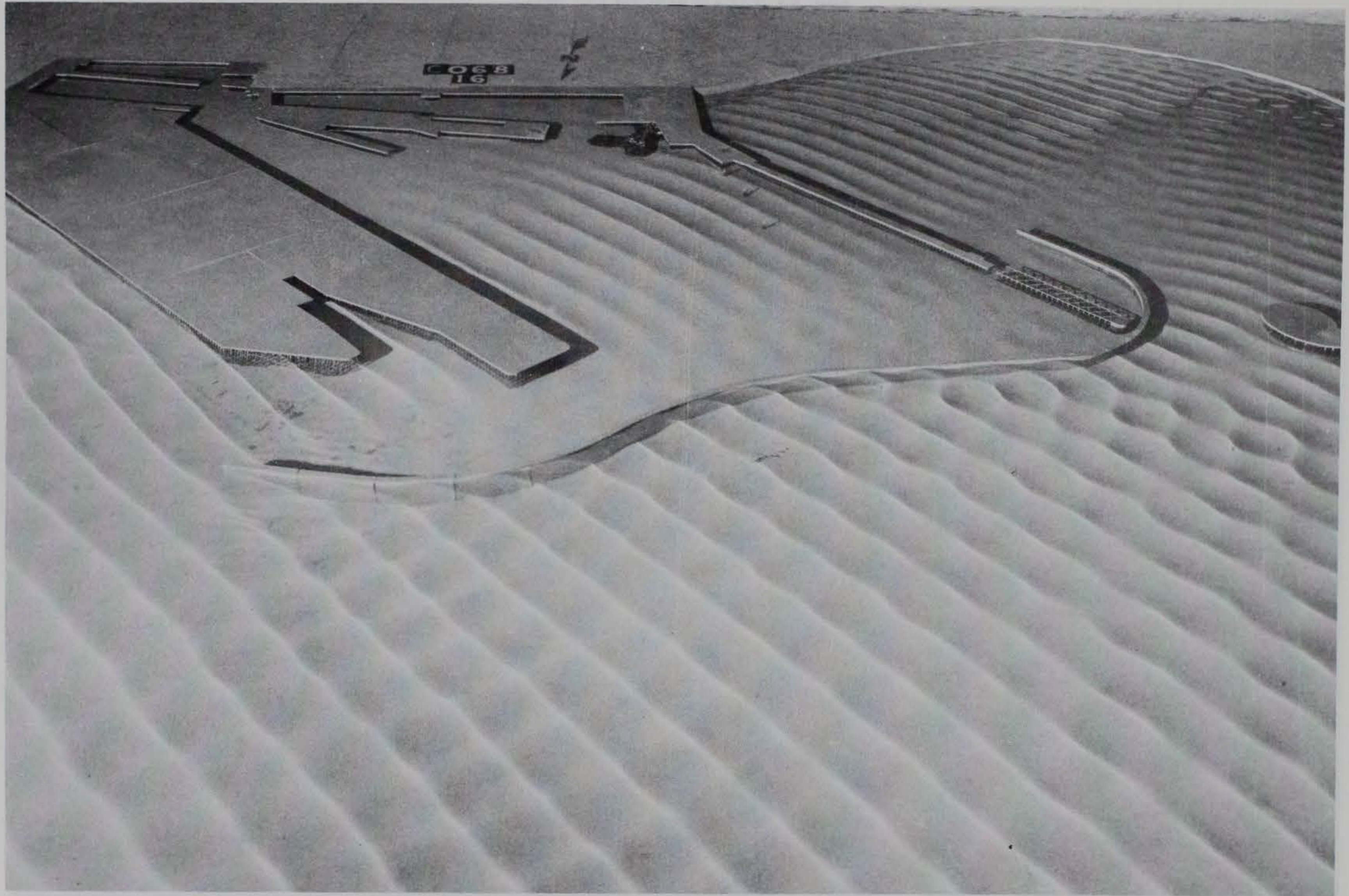
Photo 41. Typical wave patterns for Plan 10; 3.9-sec, 3.3-ft waves from northeast; +5.7 ft swl
