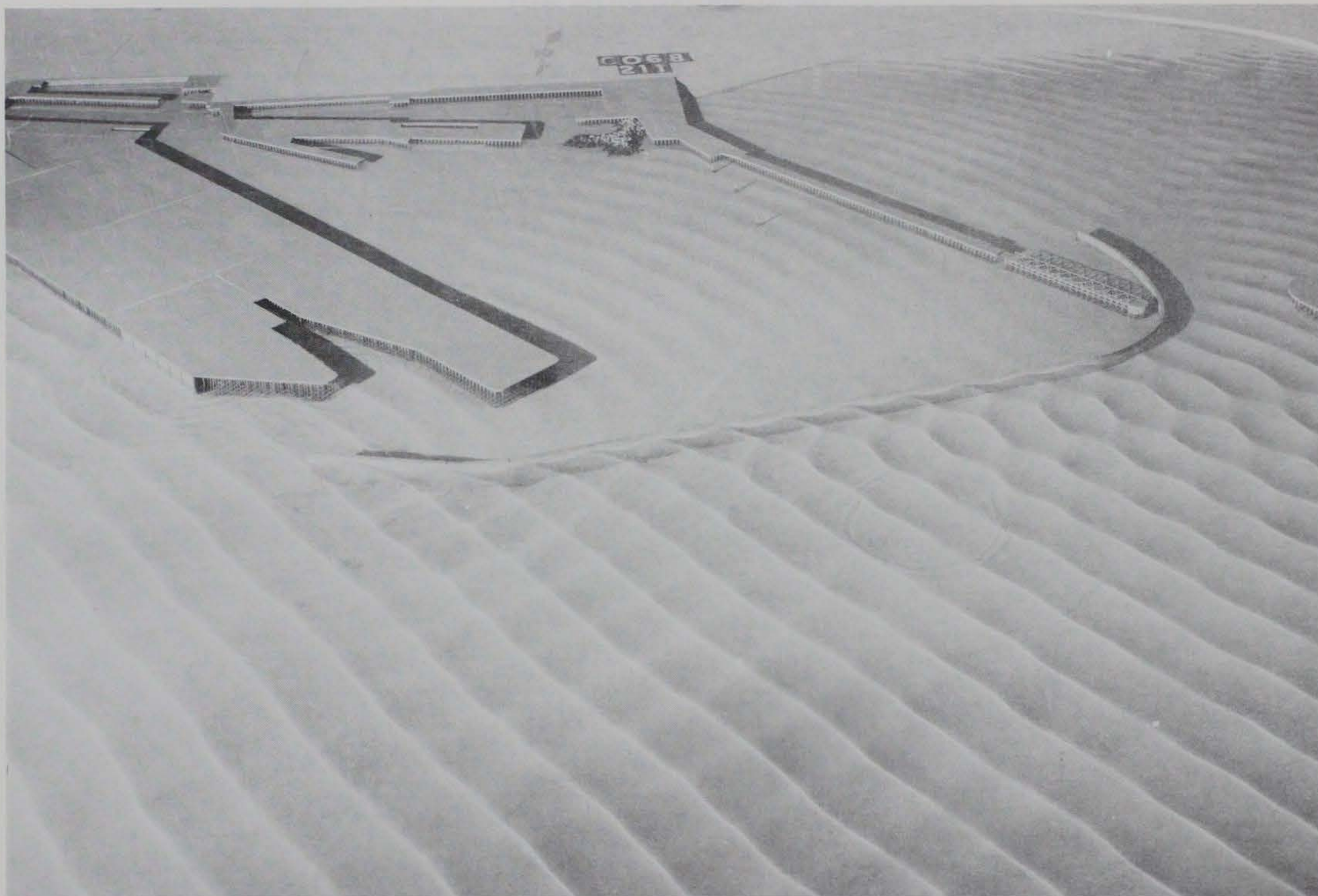
Photo 116. Typical wave patterns for Plan 56; 3.9-sec, 3.3-ft waves from northeast; 0.0-ft swl
