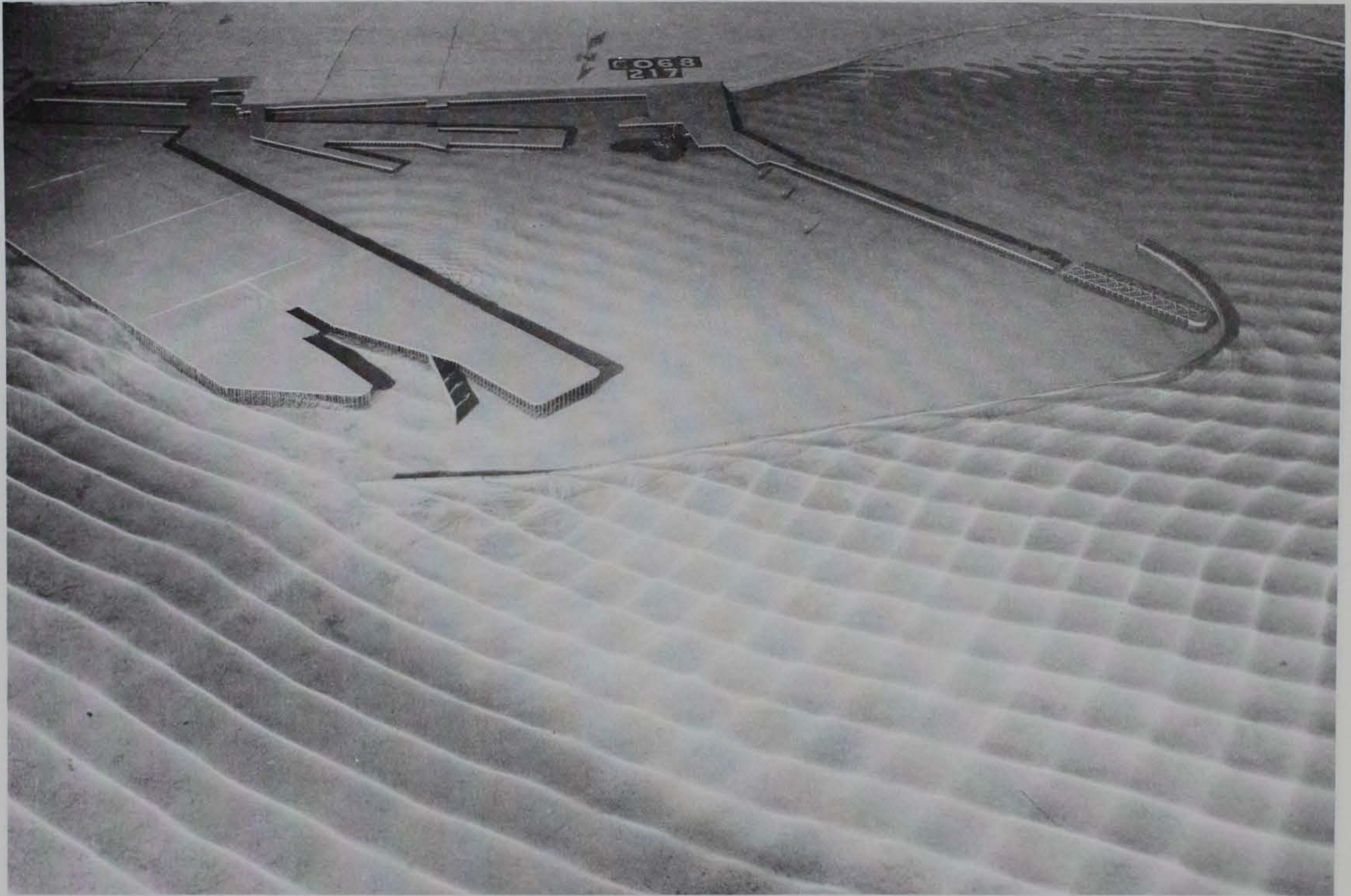
Photo 153. Typical wave patterns for Plan 78; 3.6-sec, 2.5-ft waves from north-northeast; +5.7 ft swl
