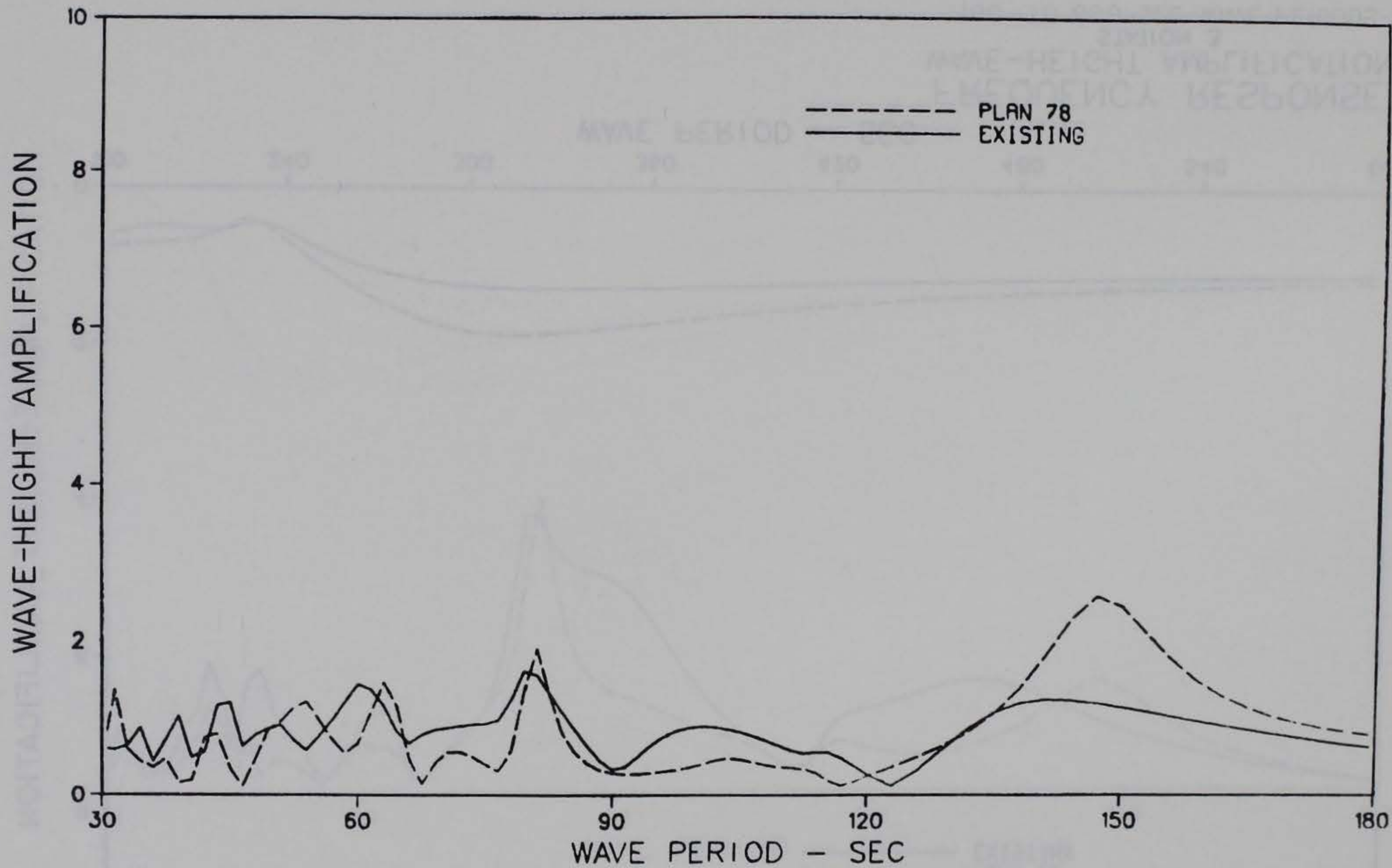
FREQUENCY RESPONSE WAVE-HEIGHT AMPLIFICATION STATION 3 30 - TO 180-SEC WAVE PERIODS
