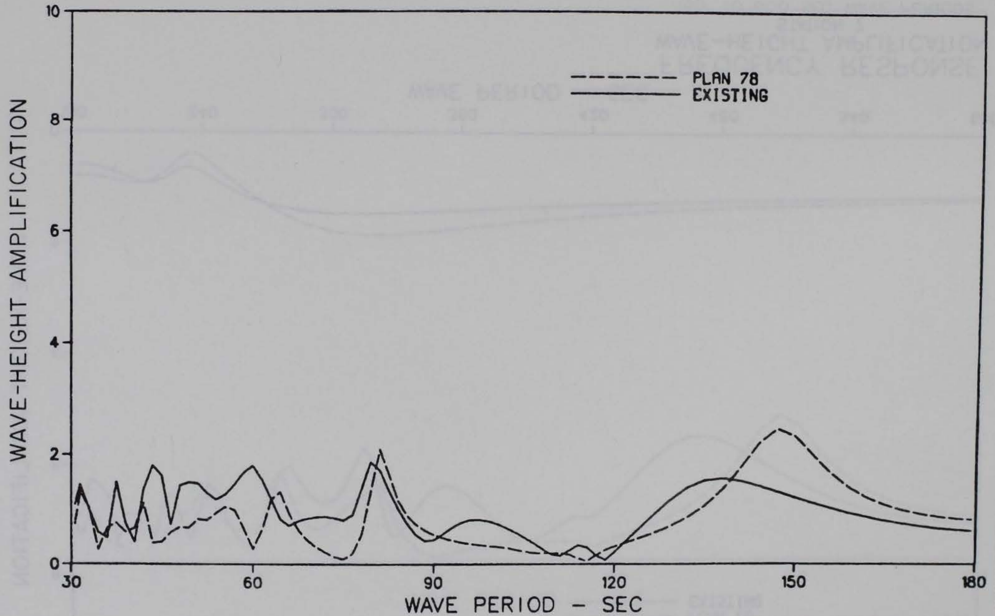
FREQUENCY RESPONSE WAVE-HEIGHT AMPLIFICATION STATION 7 30- TO 180-SEC WAVE PERIODS
