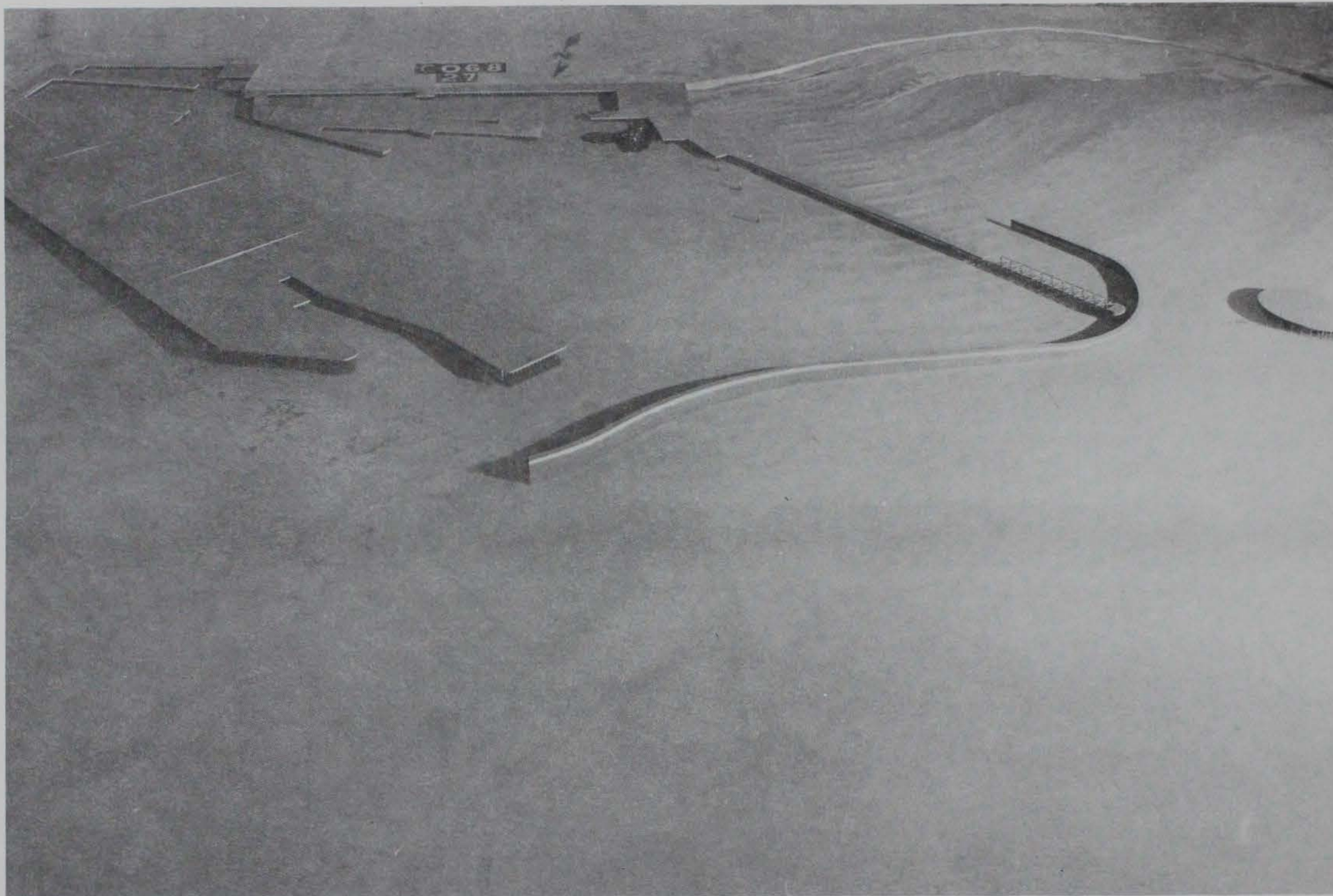
Photo 32. Typical wave patterns for Plan 1; 10-sec, 2-ft waves from west-northwest; +5.7 ft swl
