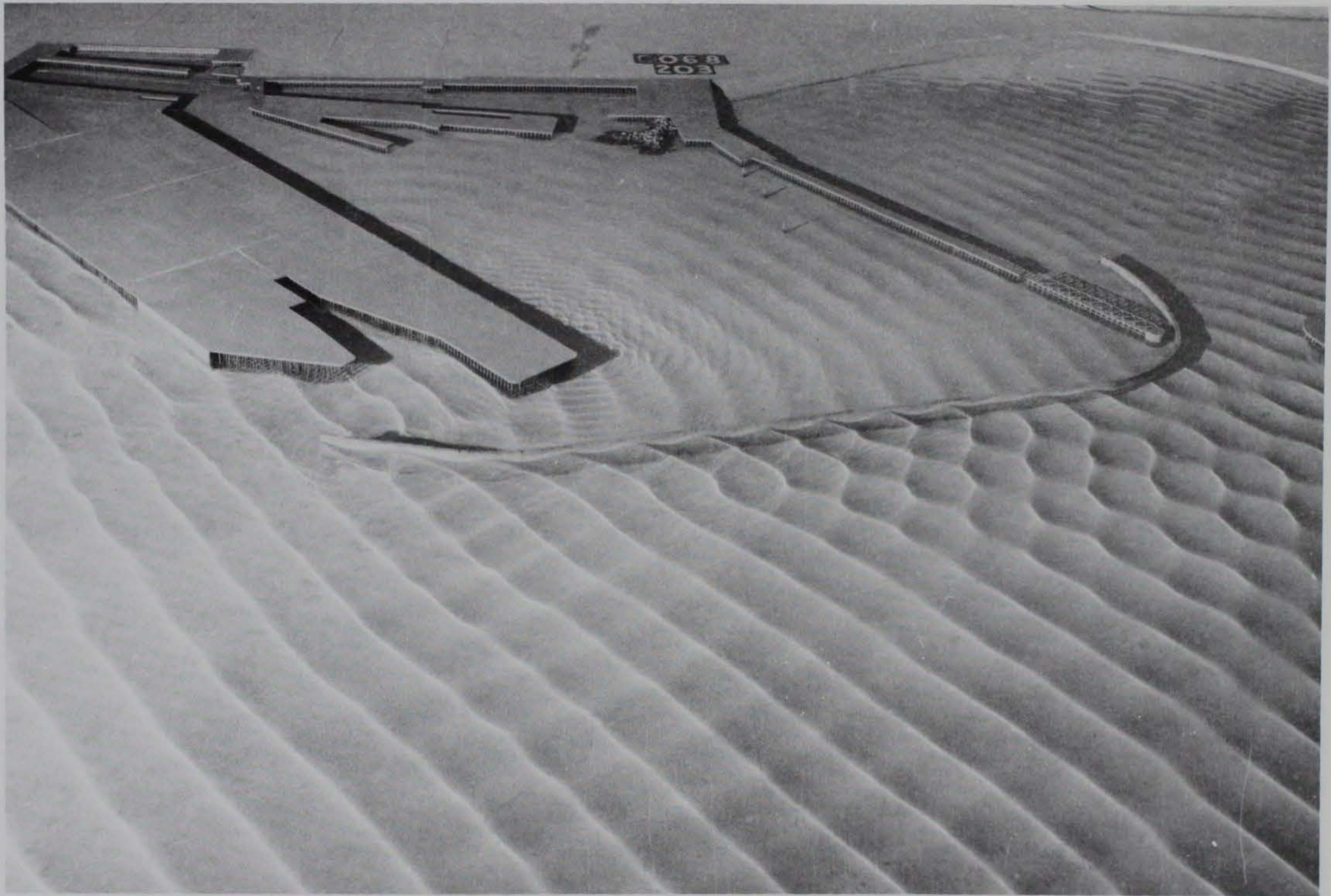
Photo 123. Typical wave patterns for Plan 63; 3.9-sec, 3.3-ft waves from northeast; 0.0-ft swl
