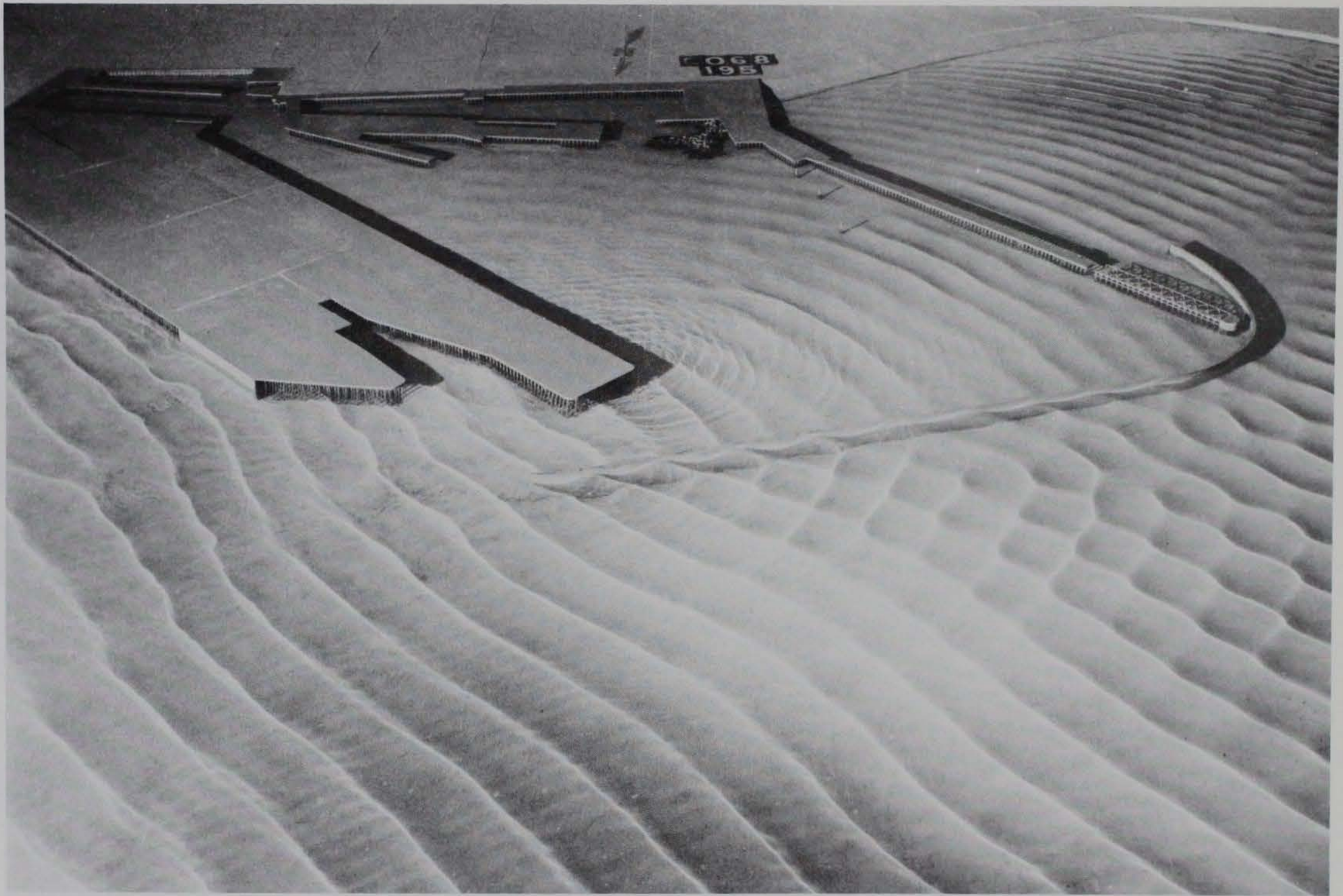
Photo 125. Typical wave patterns for Plan 65; 3.9-sec, 3.3-ft waves from northeast; 0.0-ft swl
