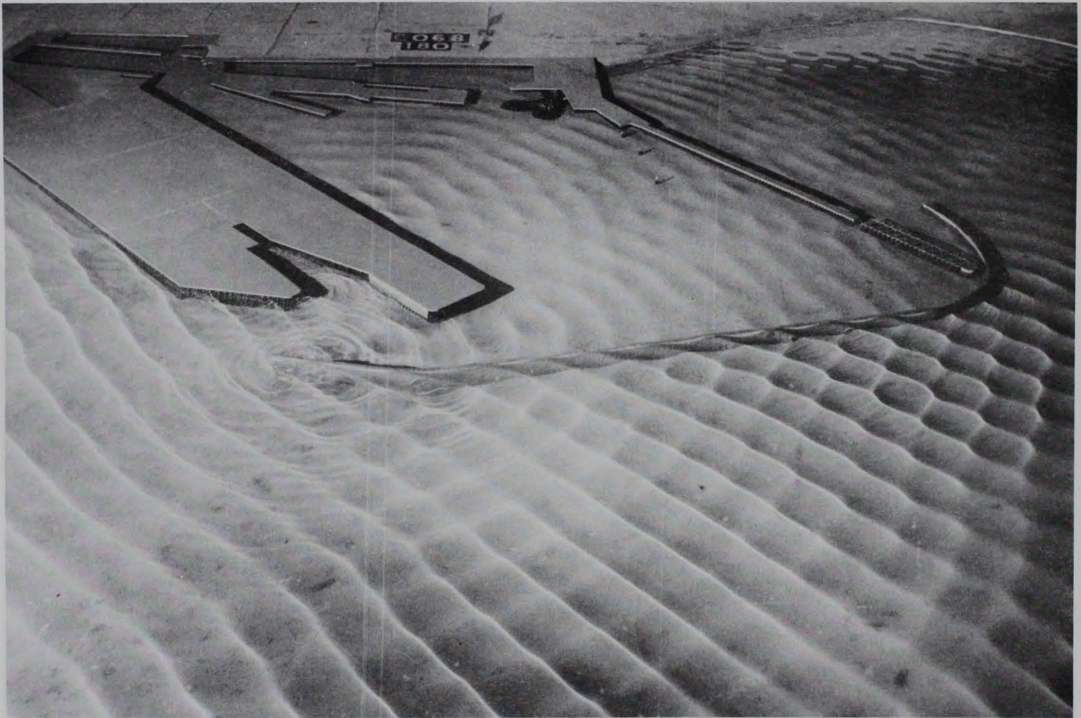
Photo 105. Typical wave patterns for Plan 44; 3.9-sec, 3.3-ft waves from northeast; +5.7 ft swl
