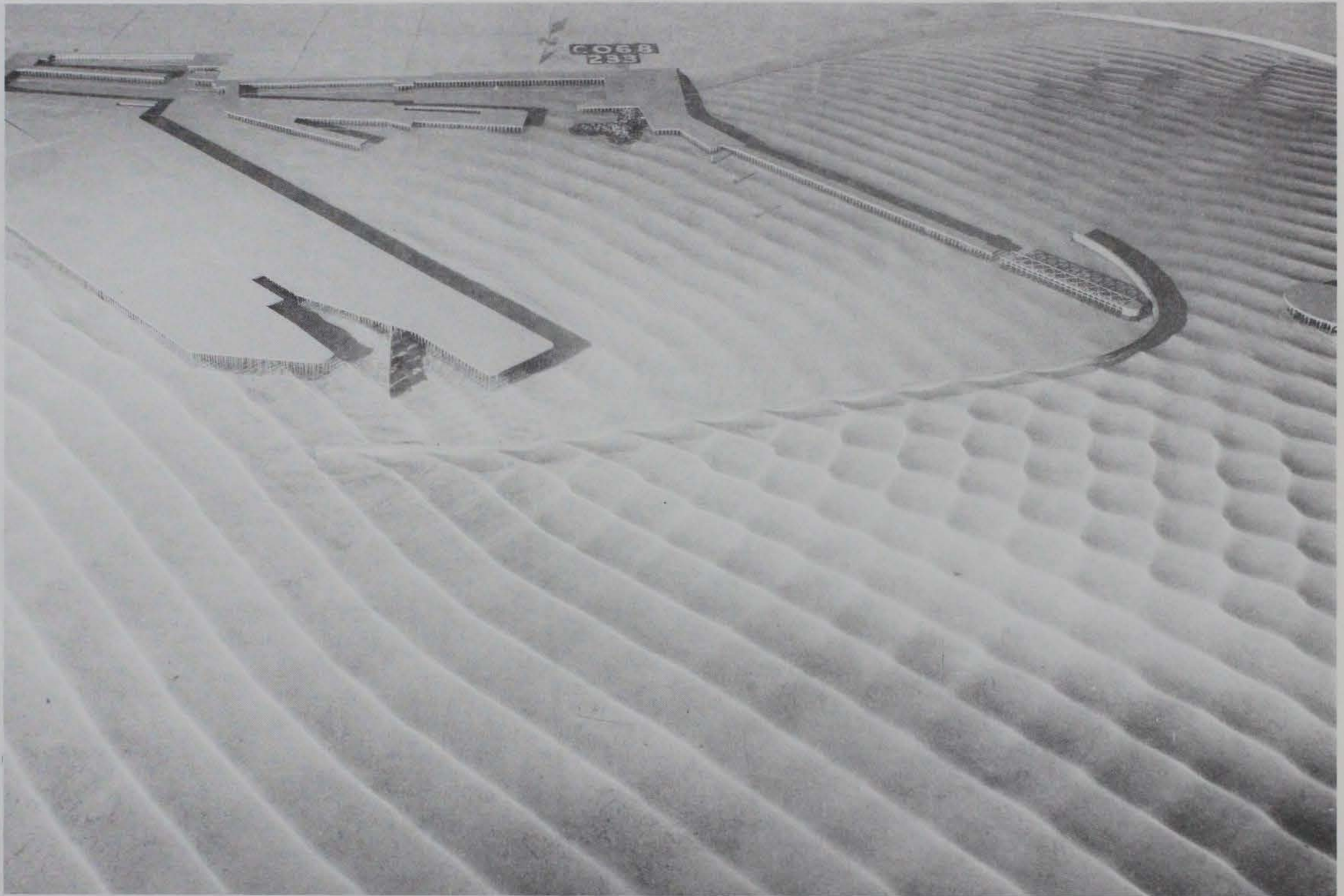
Photo 150. Typical wave patterns for Plan 90; 3.9-sec, 3.3-ft waves from northeast; 0.0-ft swl
