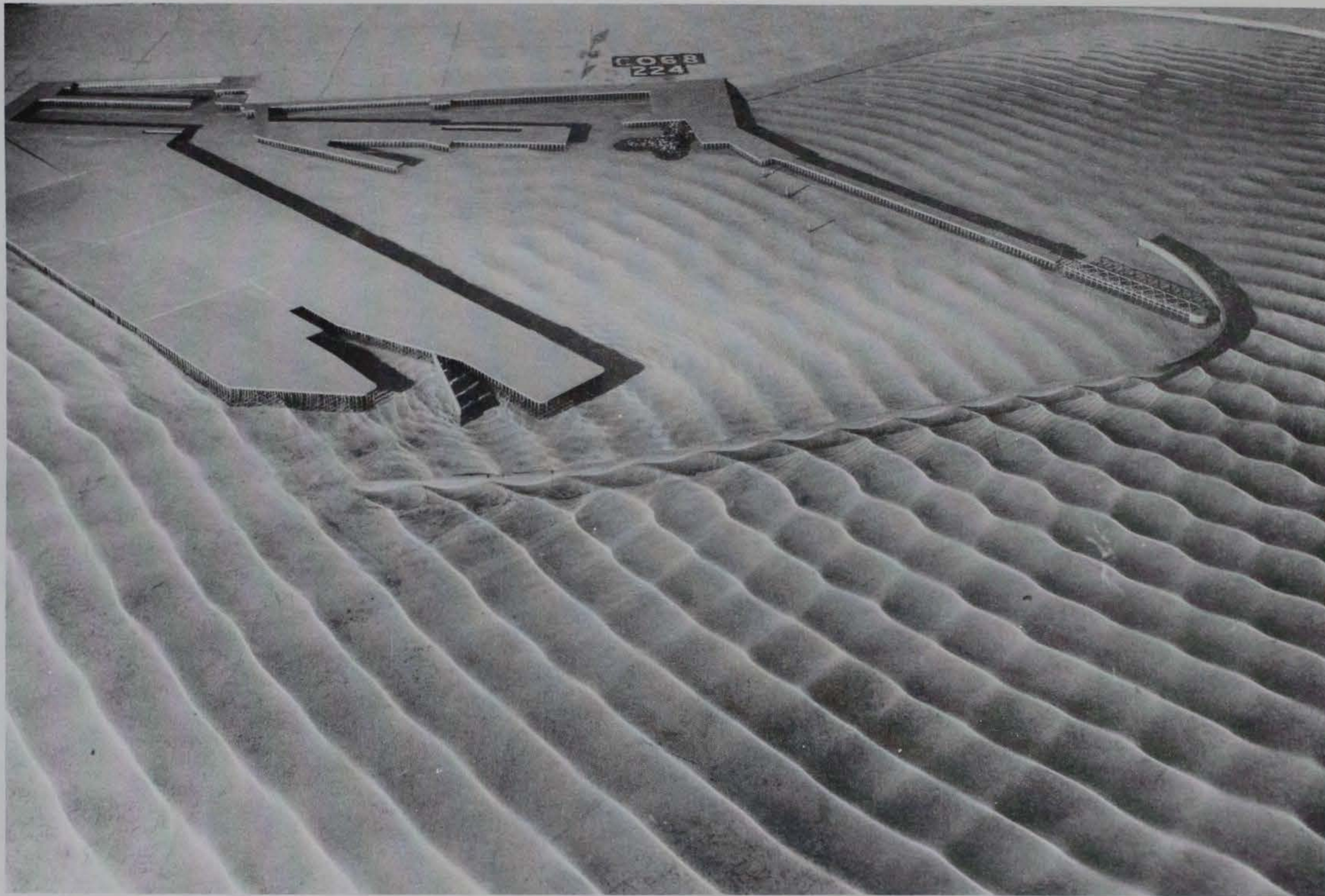
Photo 139. Typical wave patterns for Plan 79; 3.9-sec, 3.3-ft waves from northeast; 0.0-ft swl
