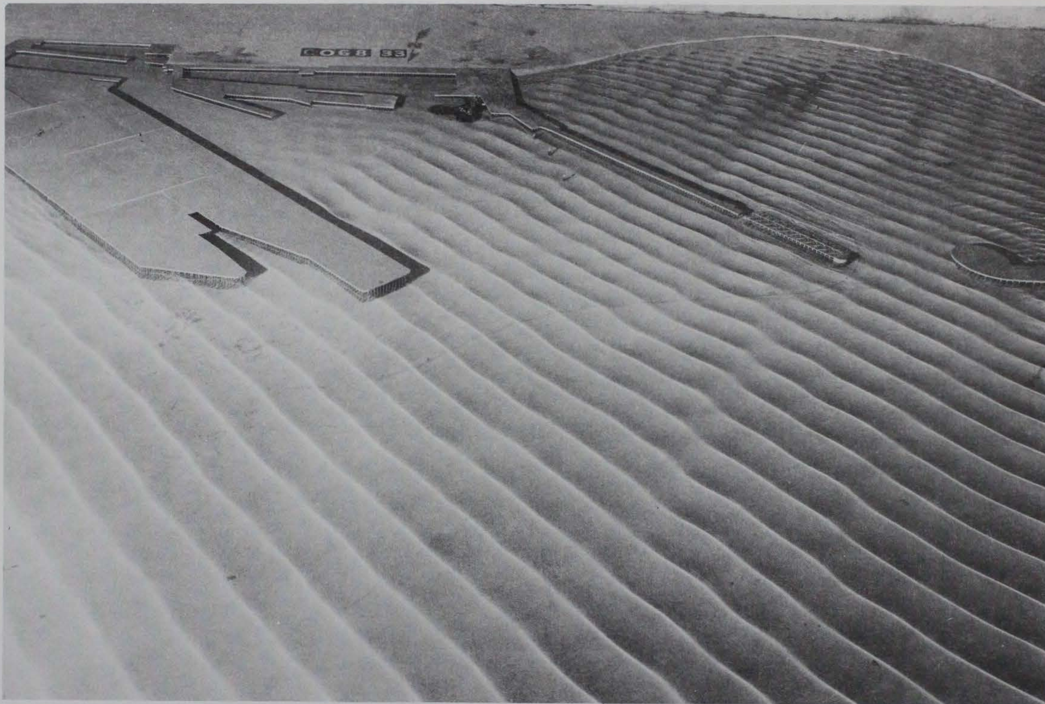
Photo 2. Typical wave patterns for existing conditions; 3.9-sec, 3.3-ft waves from northeast; +5.7 ft swl
