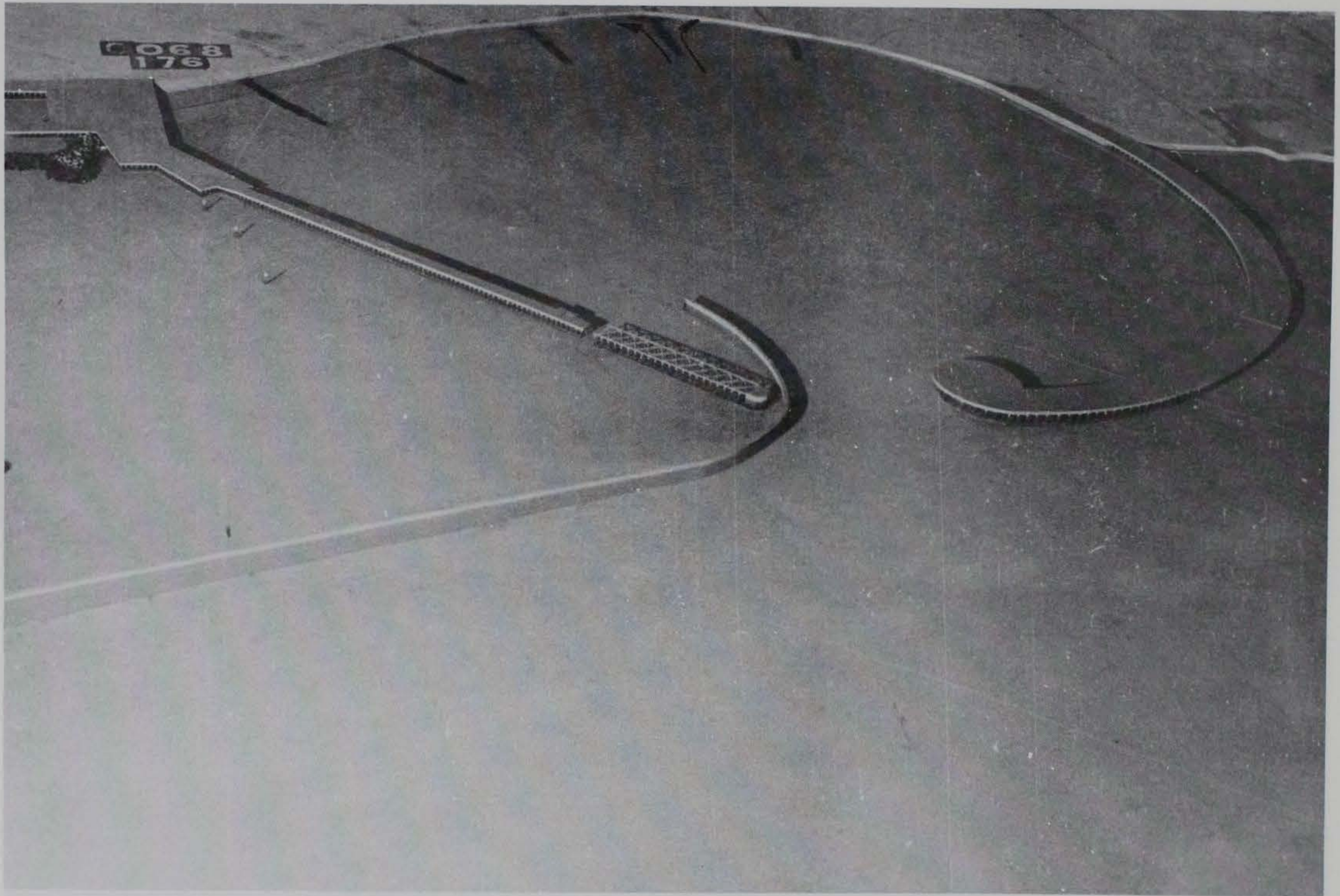
Photo 87. General movement of tracer material for Plan 38; 3.9-sec, 3.3-ft waves from northeast; +5.7 ft swl
