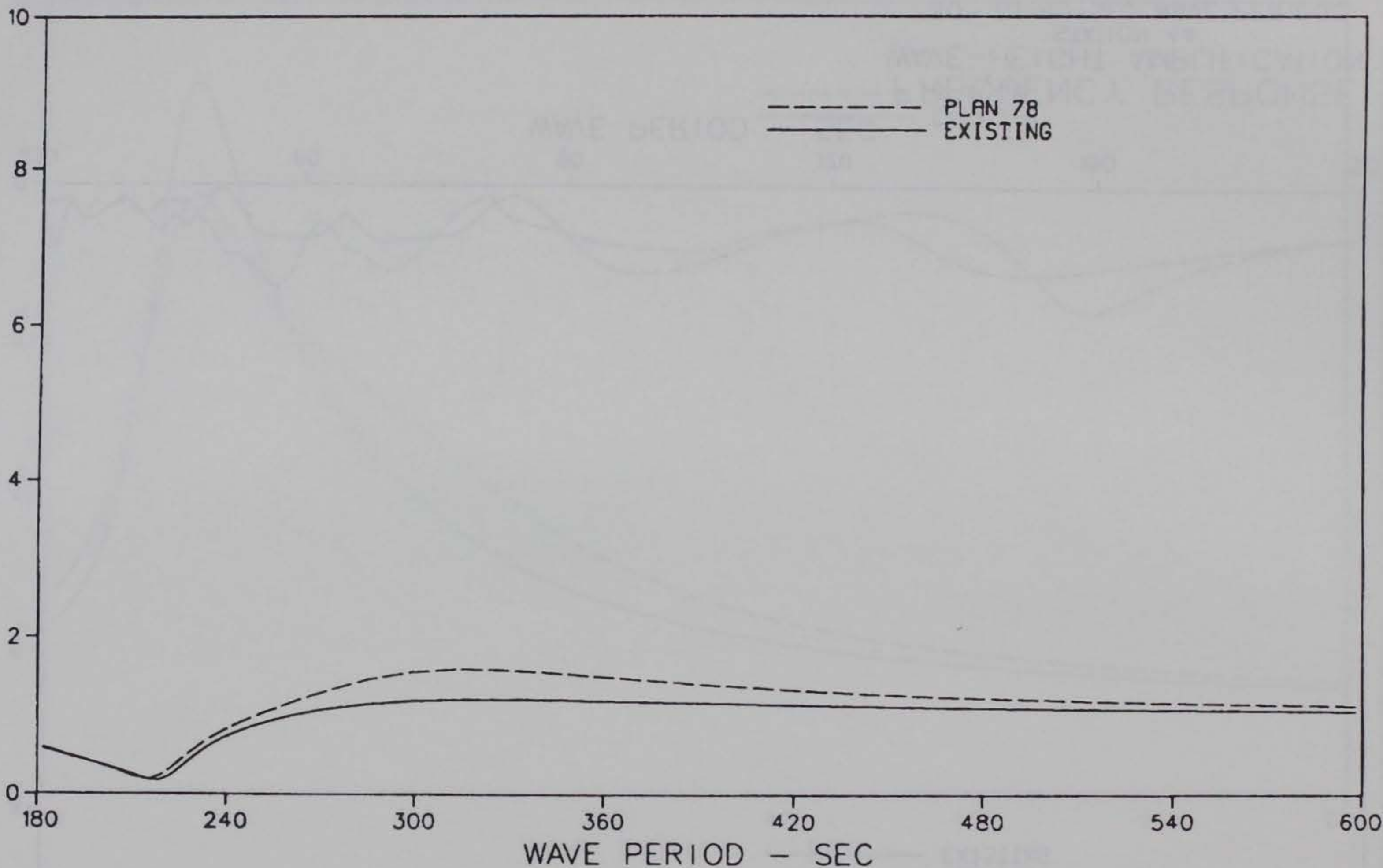
FREQUENCY RESPONSE WAVE-HEIGHT AMPLIFICATION STATION 4A 180 - TO 600 - SEC WAVE PERIODS
