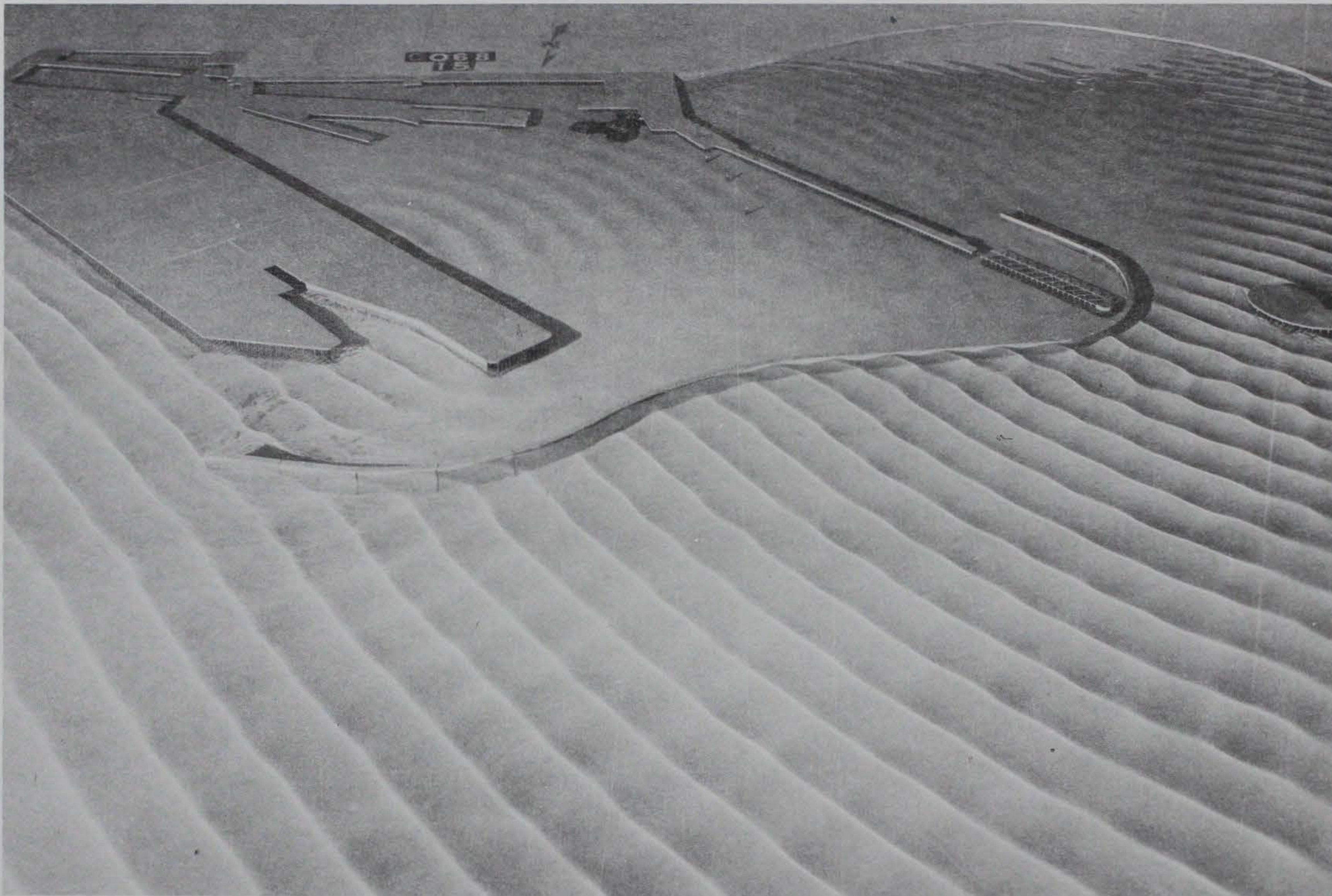
Photo 40. Typical wave patterns for Plan 9; 3.9-sec, 3.3-ft waves from northeast; +5.7 ft swl
