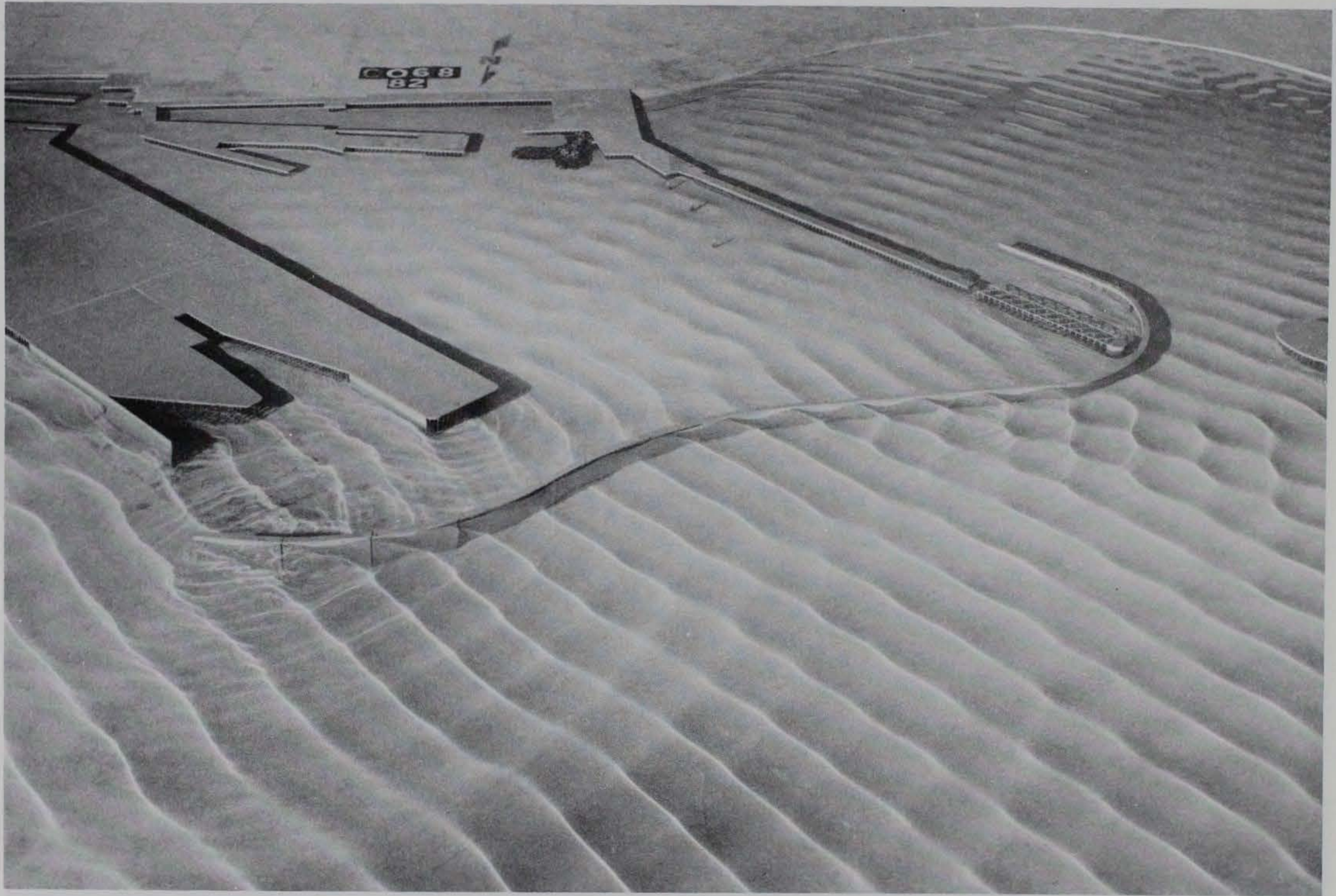
Photo 51. Typical wave patterns for Plan 20; 3.9-sec, 3.3-ft waves from northeast; +5.7 ft swl
