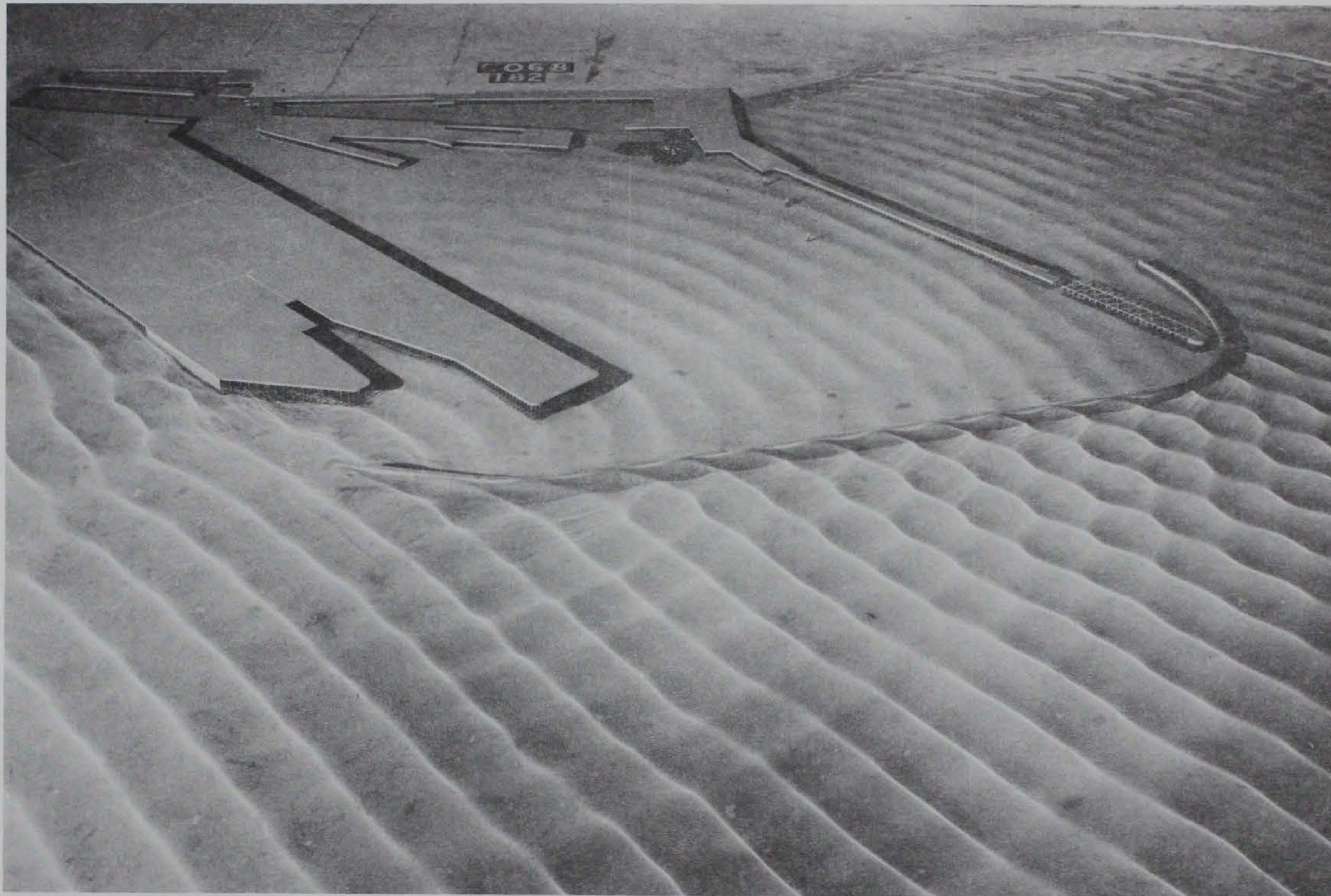
Photo 108. Typical wave patterns for Plan 48; 3.9-sec, 3.3-ft waves from northeast; +5.7 ft swl
