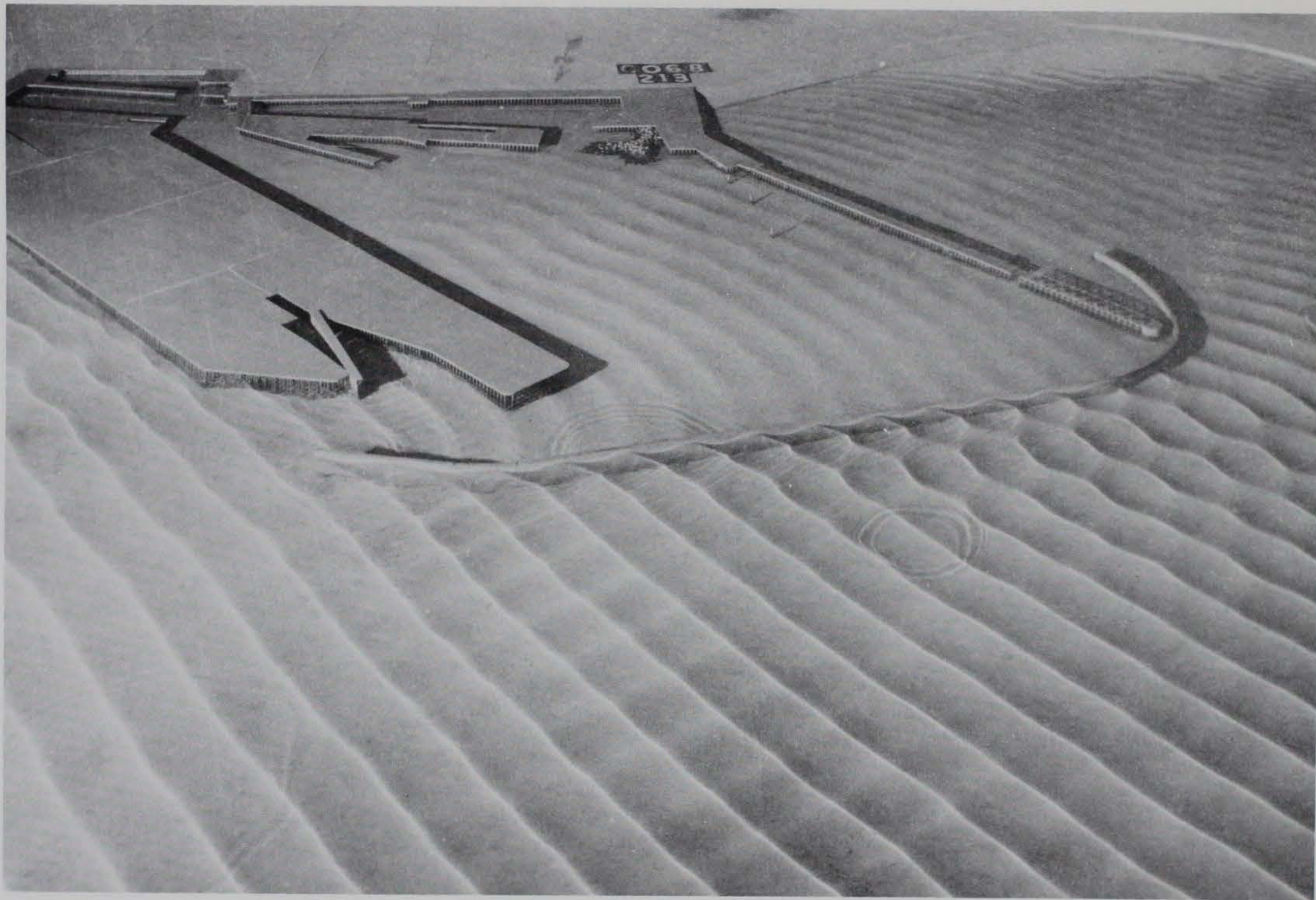
Photo 115. Typical wave patterns for Plan 55; 3.9-sec, 3.3-ft waves from northeast; 0.0-ft swl
