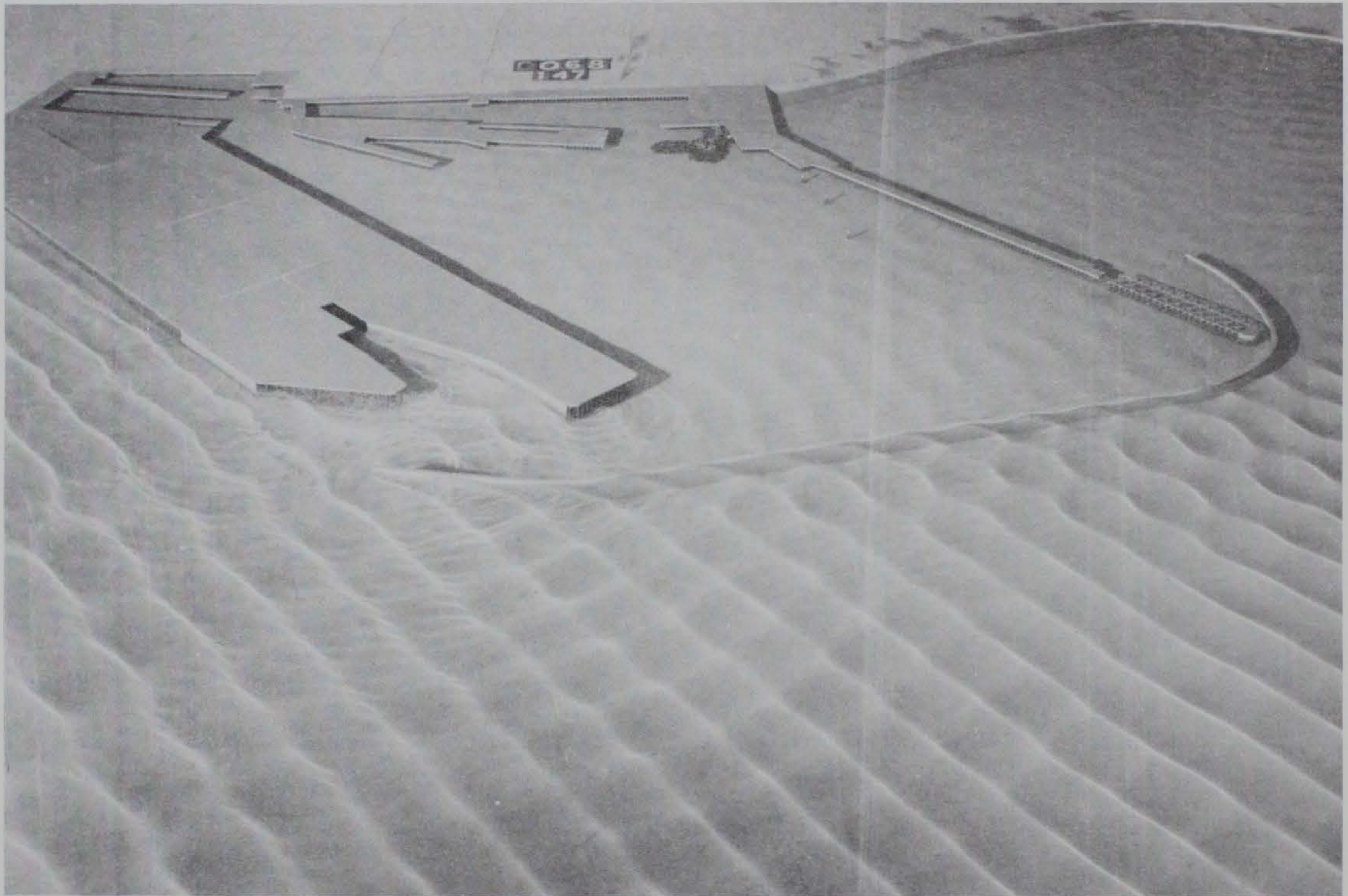
Photo 70. Typical wave patterns for Plan 38; 3.9-sec, 3.3-ft waves from northeast; +5.7 ft swl
