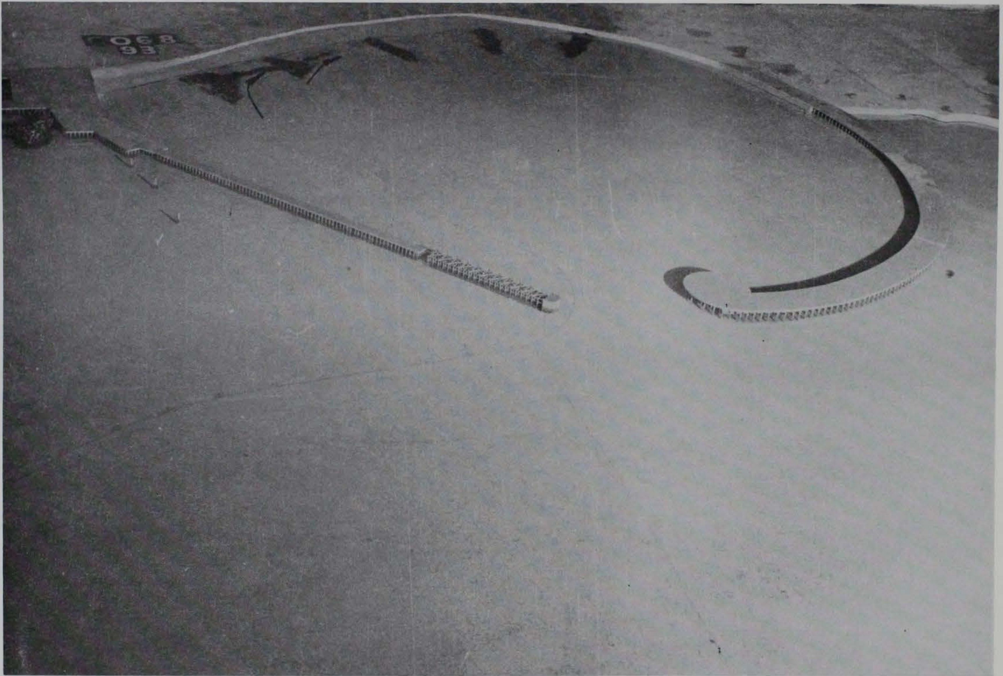
Photo 21. General movement of tracer material for existing conditions; 3.6-sec, 3.3-ft waves from north-northwest; 0.0-ft swl
