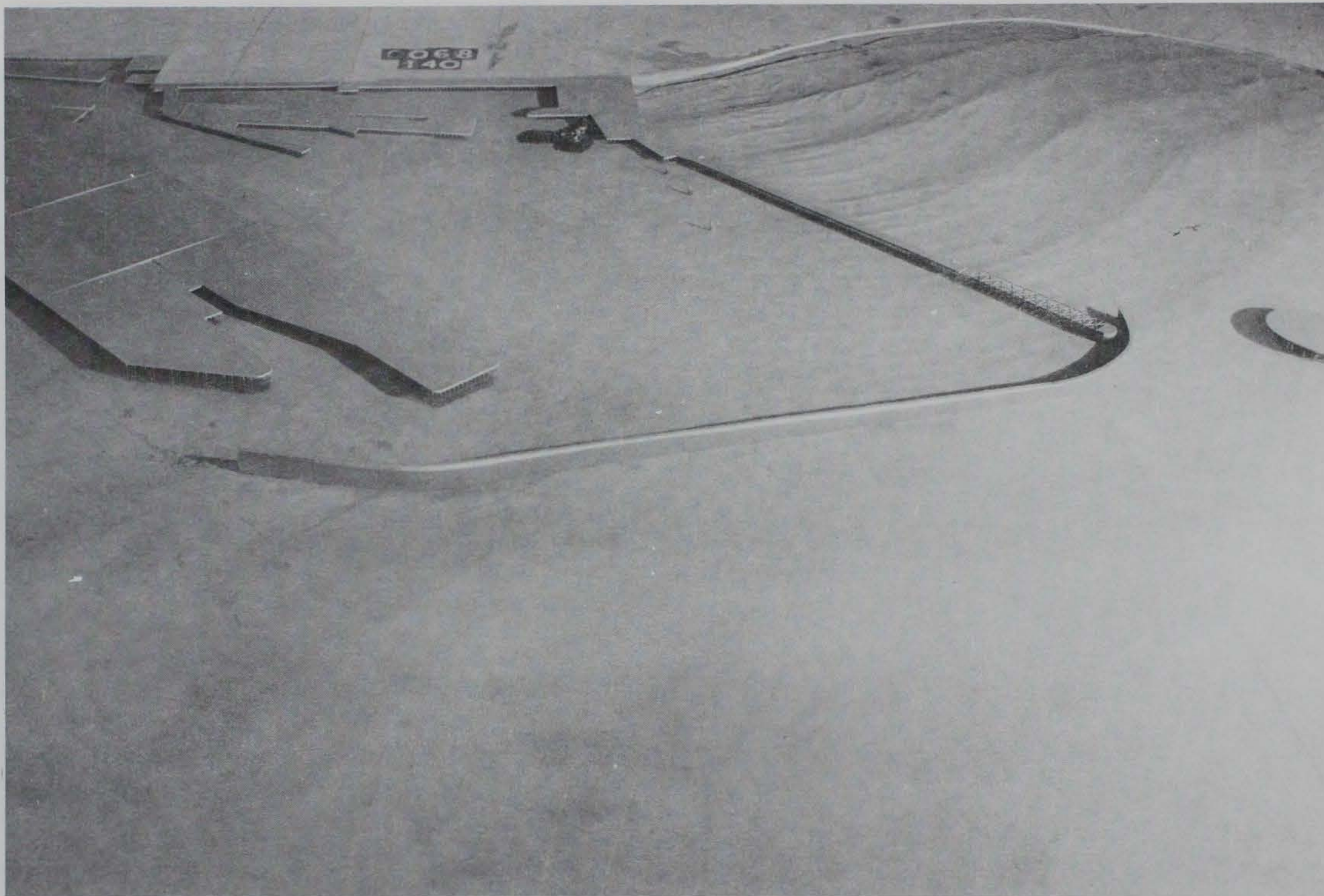
Photo 52. Typical wave patterns for Plan 21; 10-sec, 2-ft waves from west-northwest; +5.7 ft swl
