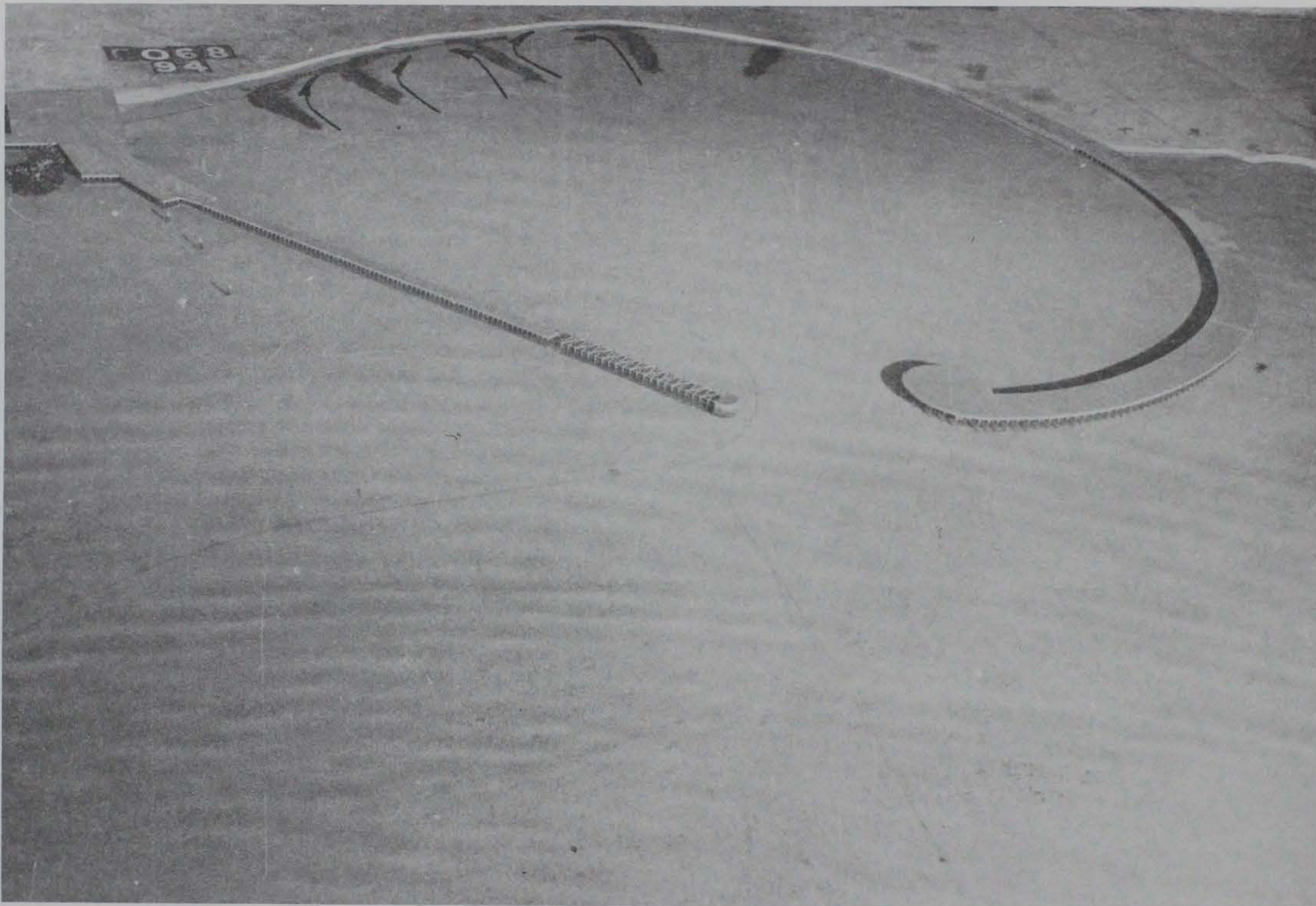
Photo 22. General movement of tracer material for existing conditions; 3.6-sec, 3.3-ft waves from north-northwest; +5.7 ft swl
