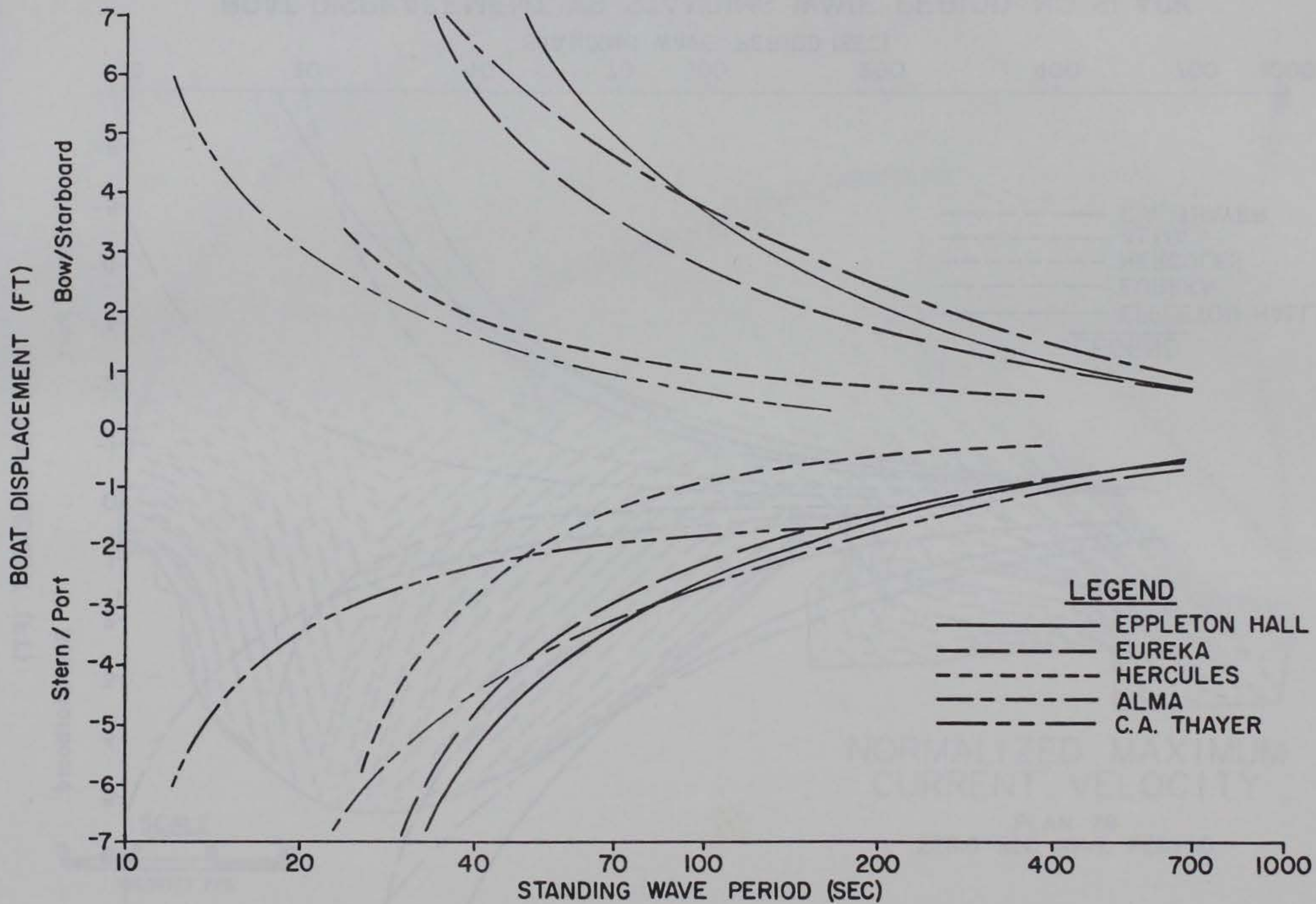
BOAT DISPLACEMENT VS. STANDING WAVE PERIOD: 1-FT SLACK
