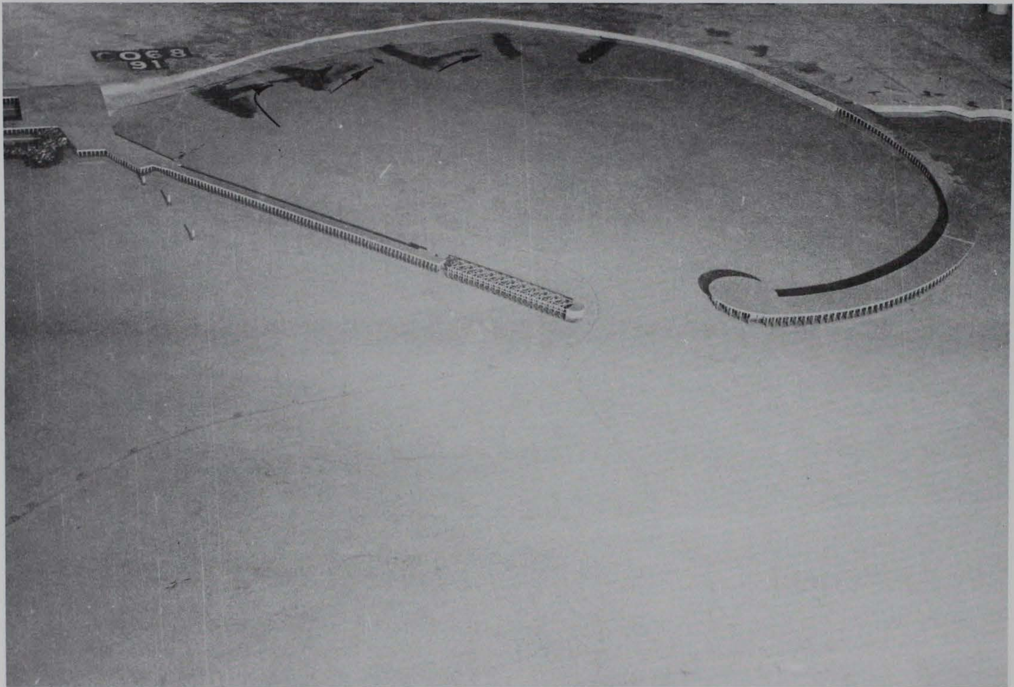
Photo 19. General movement of tracer material for existing conditions; 3.6-sec, 3.1-ft waves from north; 0.0-ft swl
