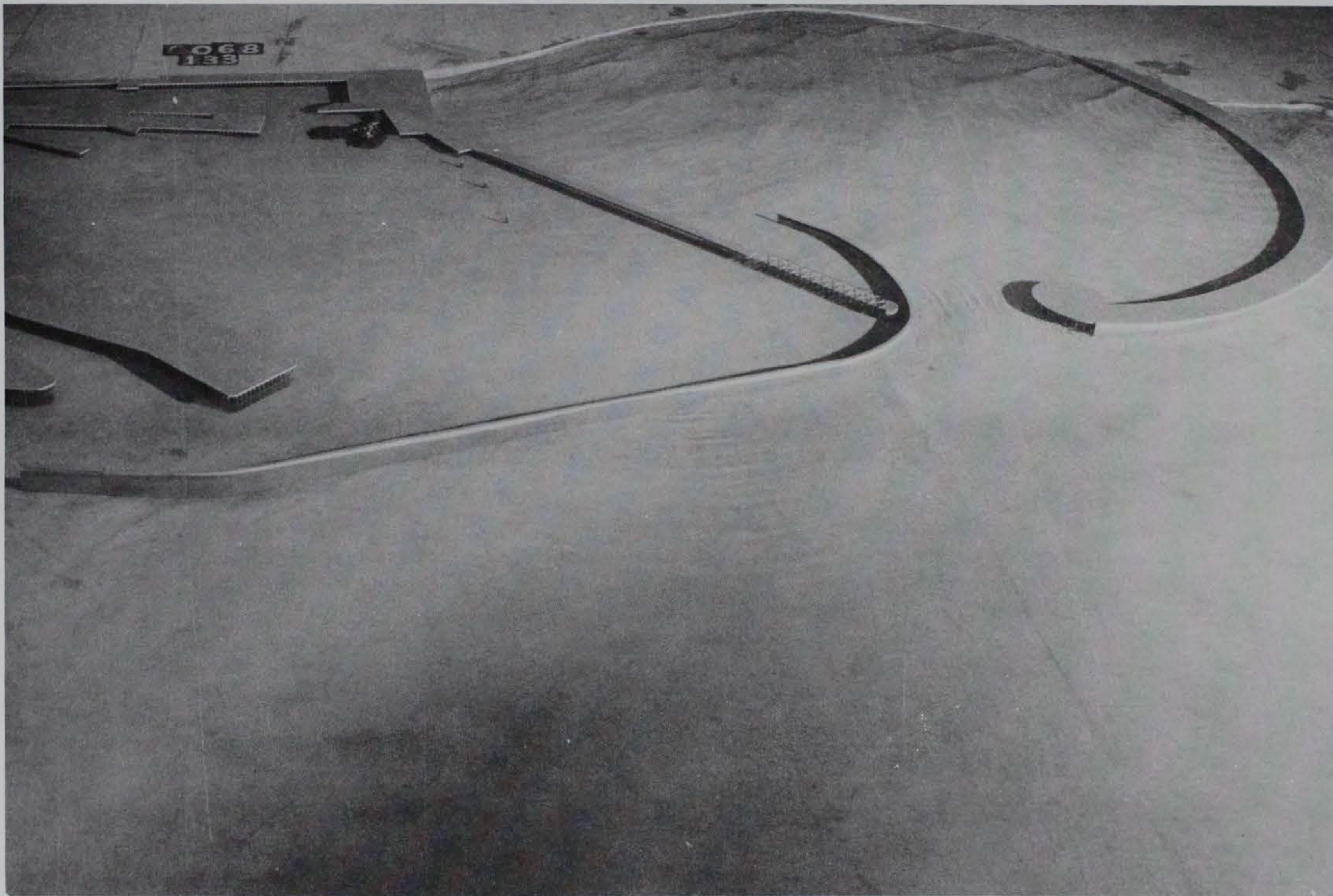
Photo 59. Typical wave patterns for Plan 28; 10-sec, 3-ft waves from west-northwest; +5.7 ft swl
