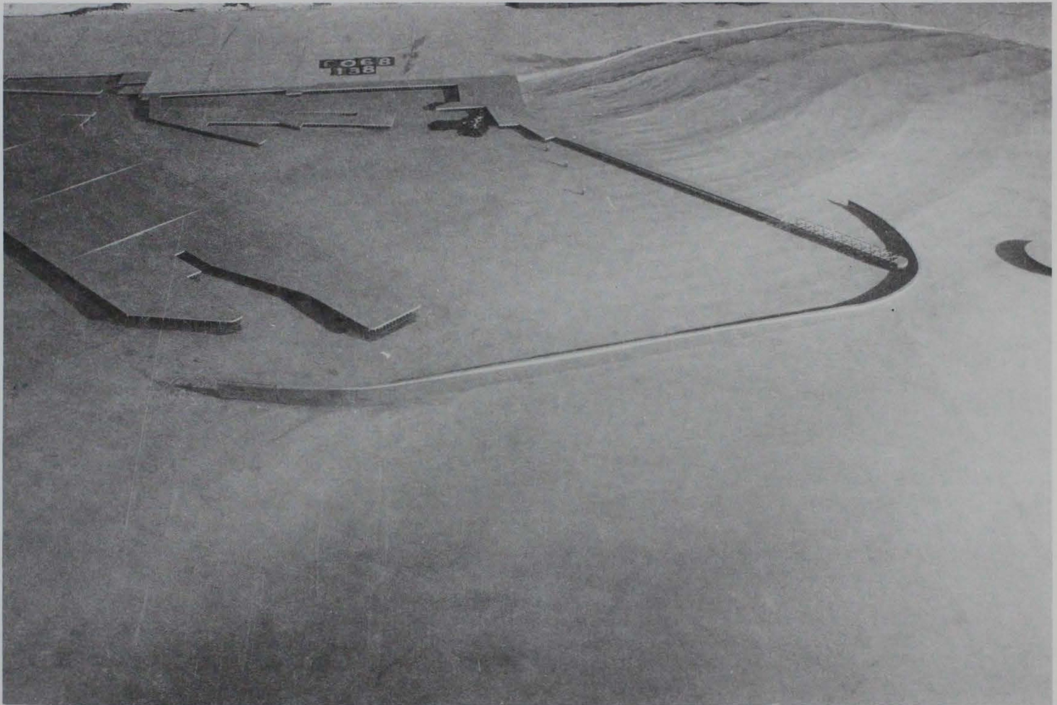
Photo 54. Typical wave patterns for Plan 23; 10-sec, 2-ft waves from west-northwest; +5.7 ft swl
