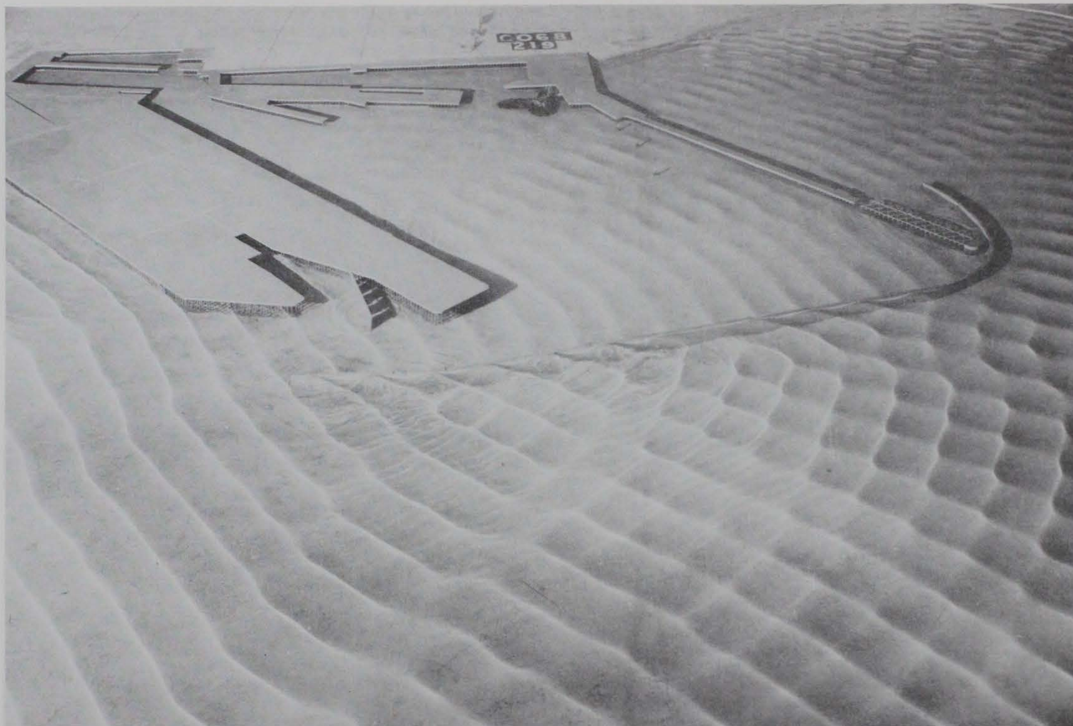
Photo 152. Typical wave patterns for Plan 78; 3.9-sec, 3.3-ft waves from northeast; +5.7 ft swl
