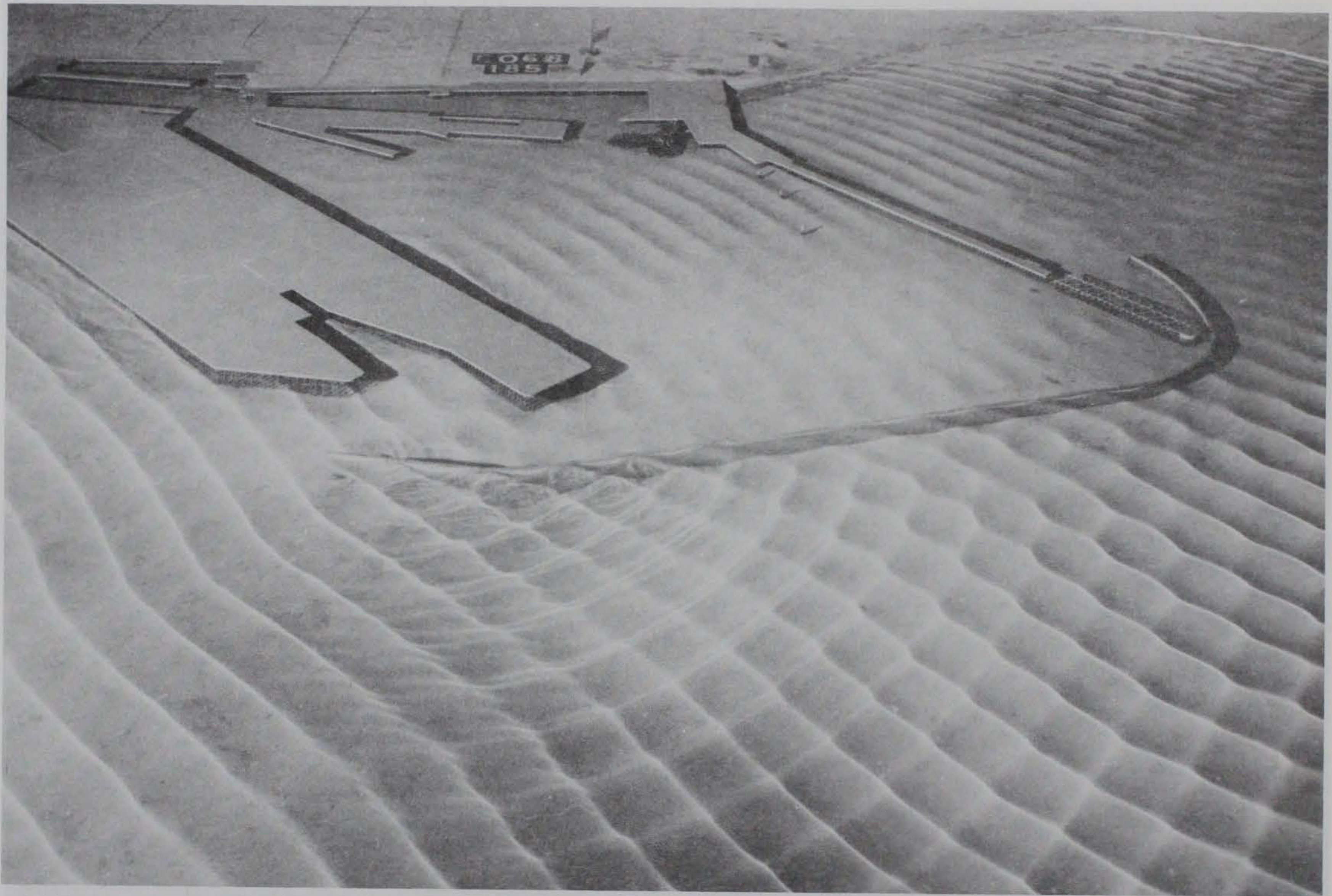
Photo 104. Typical wave patterns for Plan 43; 3.9-sec, 3.3-ft waves from northeast; +5.7 ft swl
