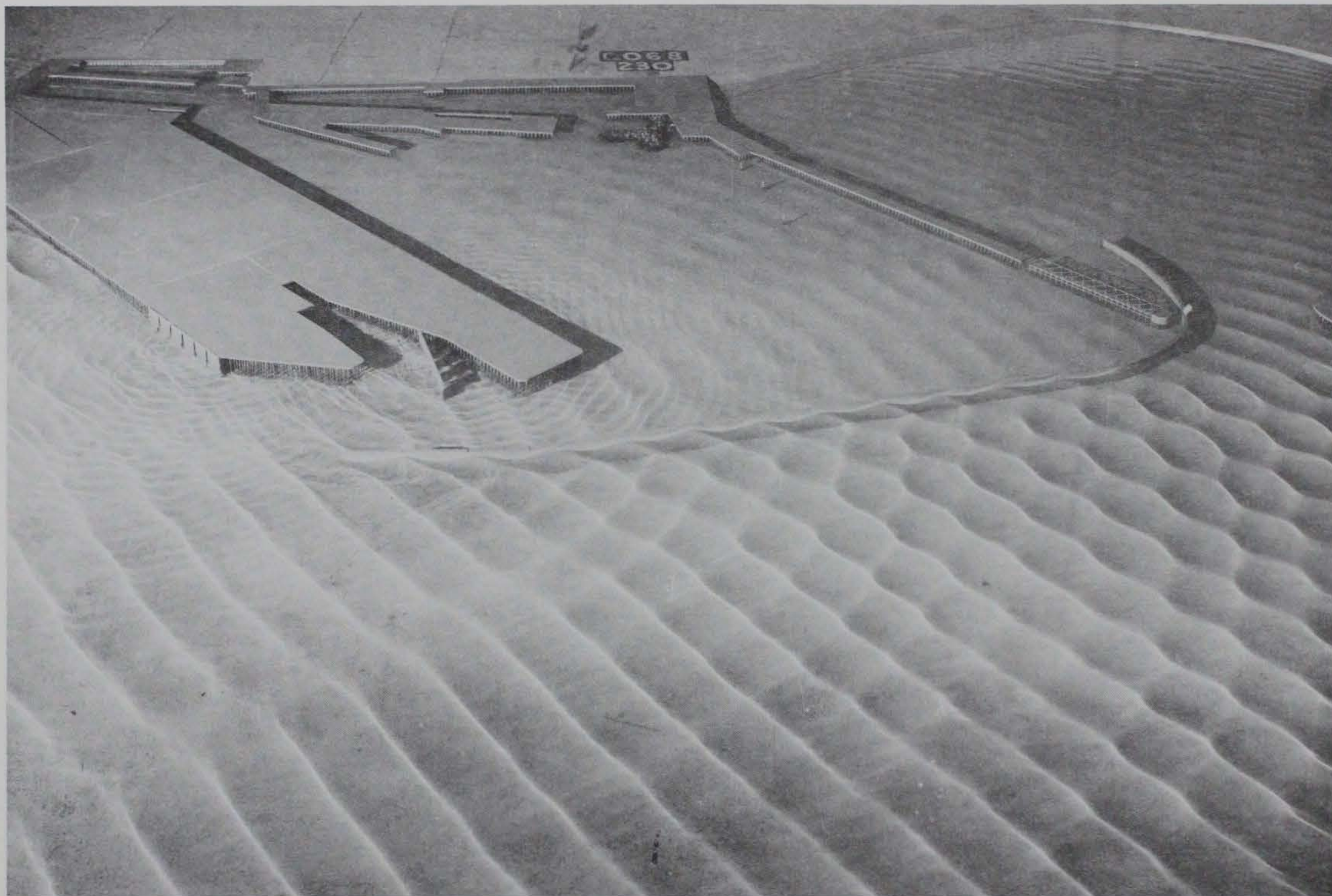
Photo 142. Typical wave patterns for Plan 82; 3.9-sec, 3.3-ft waves from northeast; 0.0-ft swl
