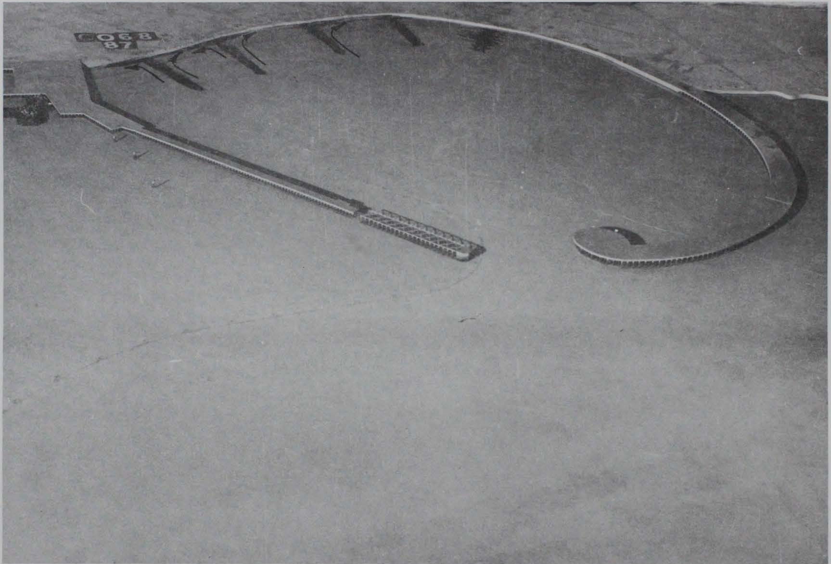
Photo 16. General movement of tracer material for existing conditions; 3.9-sec, 3.3-ft waves from northeast; +5.7 ft swl
