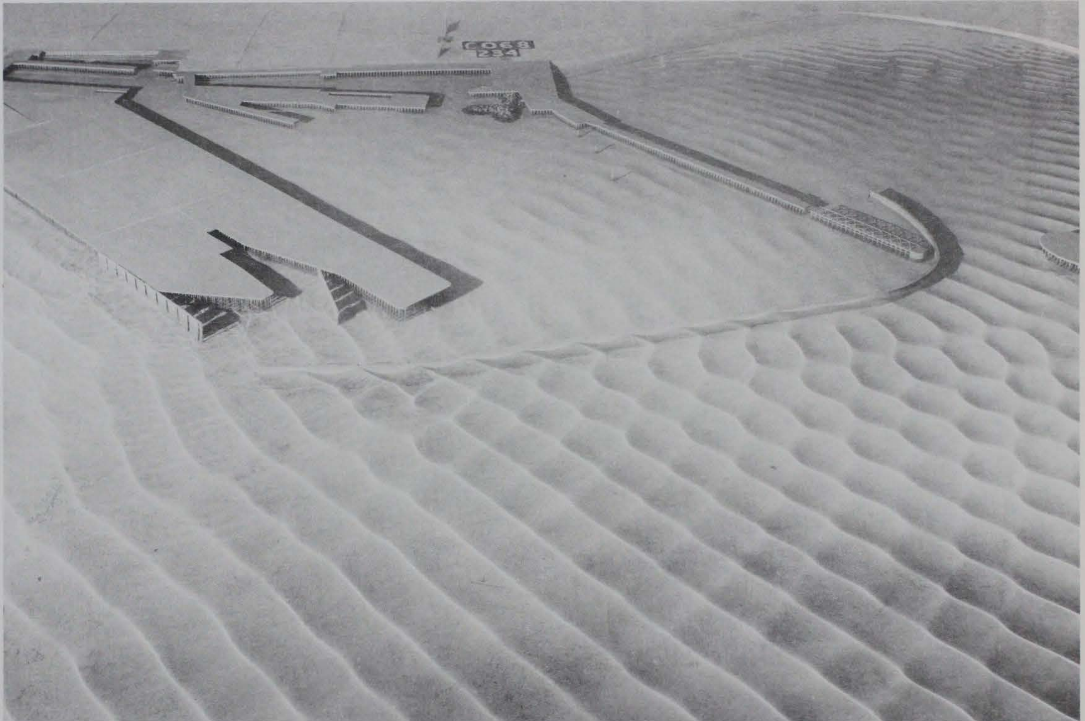
Photo 146. Typical wave patterns for Plan 86; 3.9-sec, 3.3-ft waves from northeast; 0.0-ft swl
