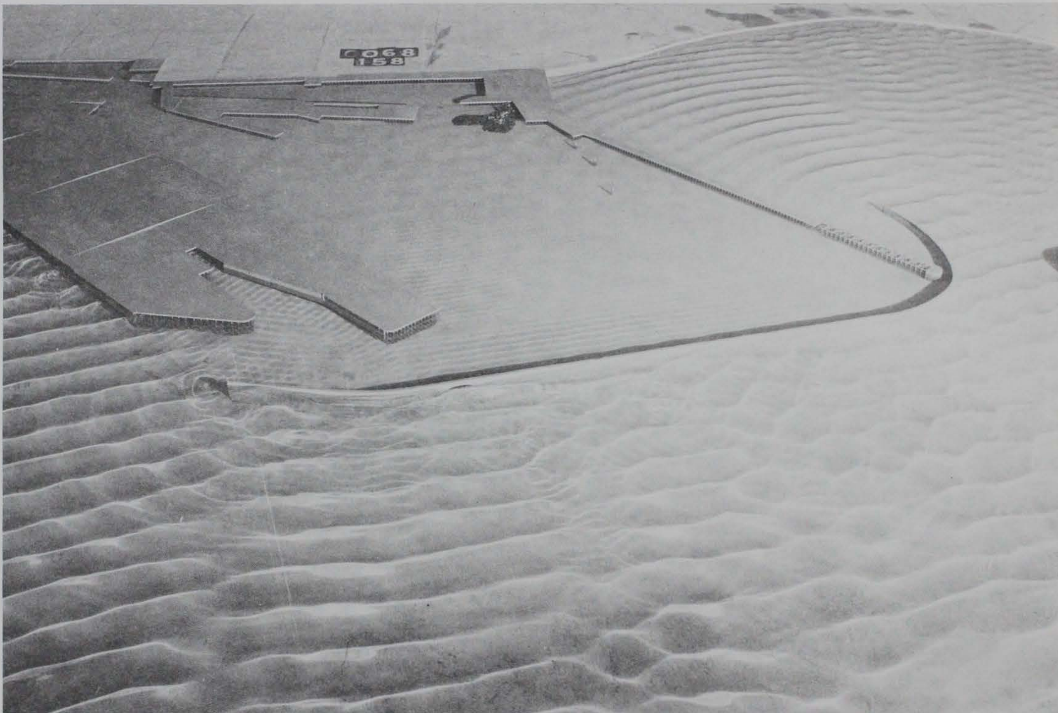
Photo 78. Typical wave patterns for Plan 38; 3.6-sec, 3.3-ft waves from north-northwest; +5.7 ft swl
