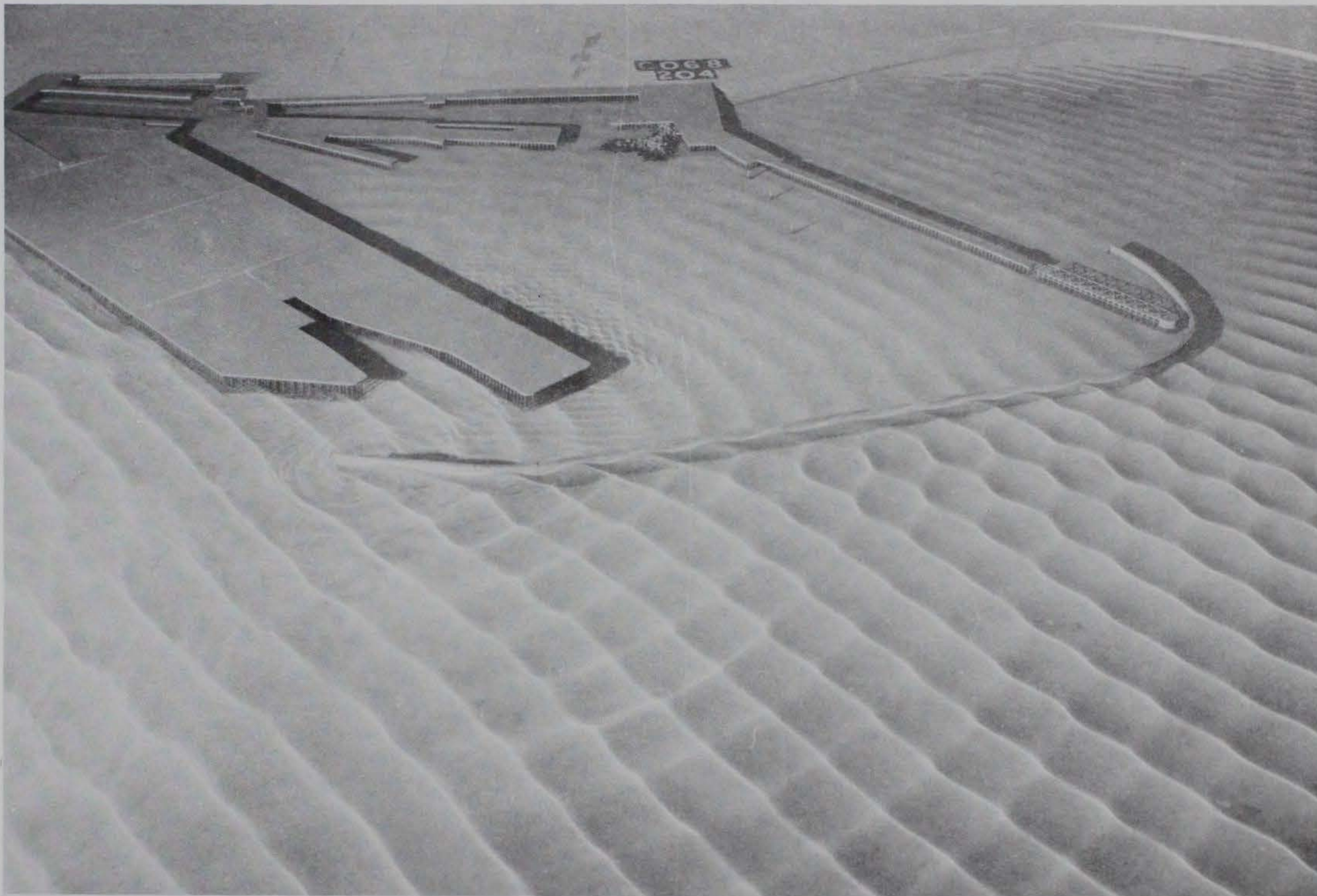
Photo 122. Typical wave patterns for Plan 62; 3.9-sec, 3.3-ft waves from northeast; 0.0-ft swl
