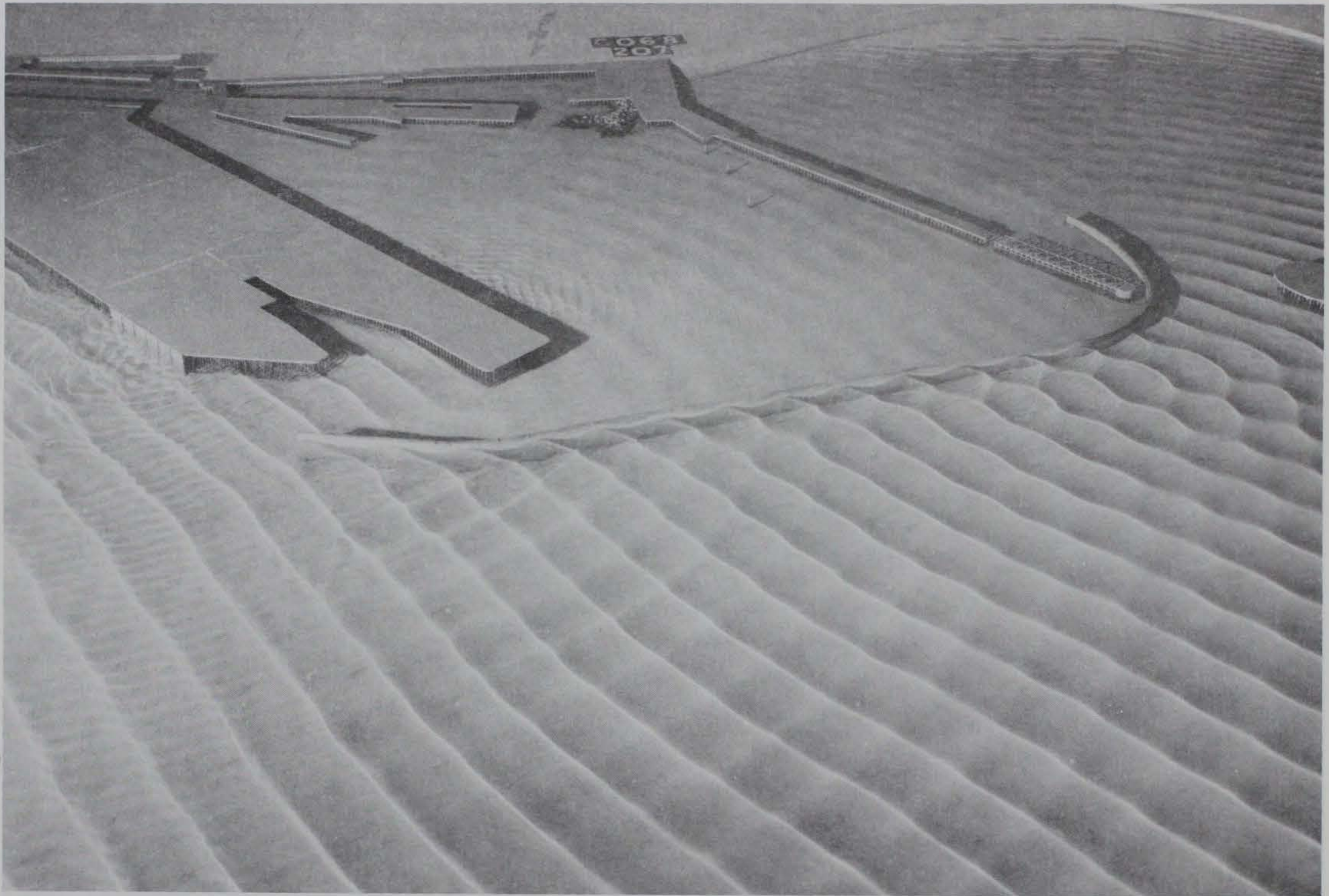
Photo 118. Typical wave patterns for Plan 58; 3.9-sec, 3.3-ft waves from northeast; 0.0-ft swl
