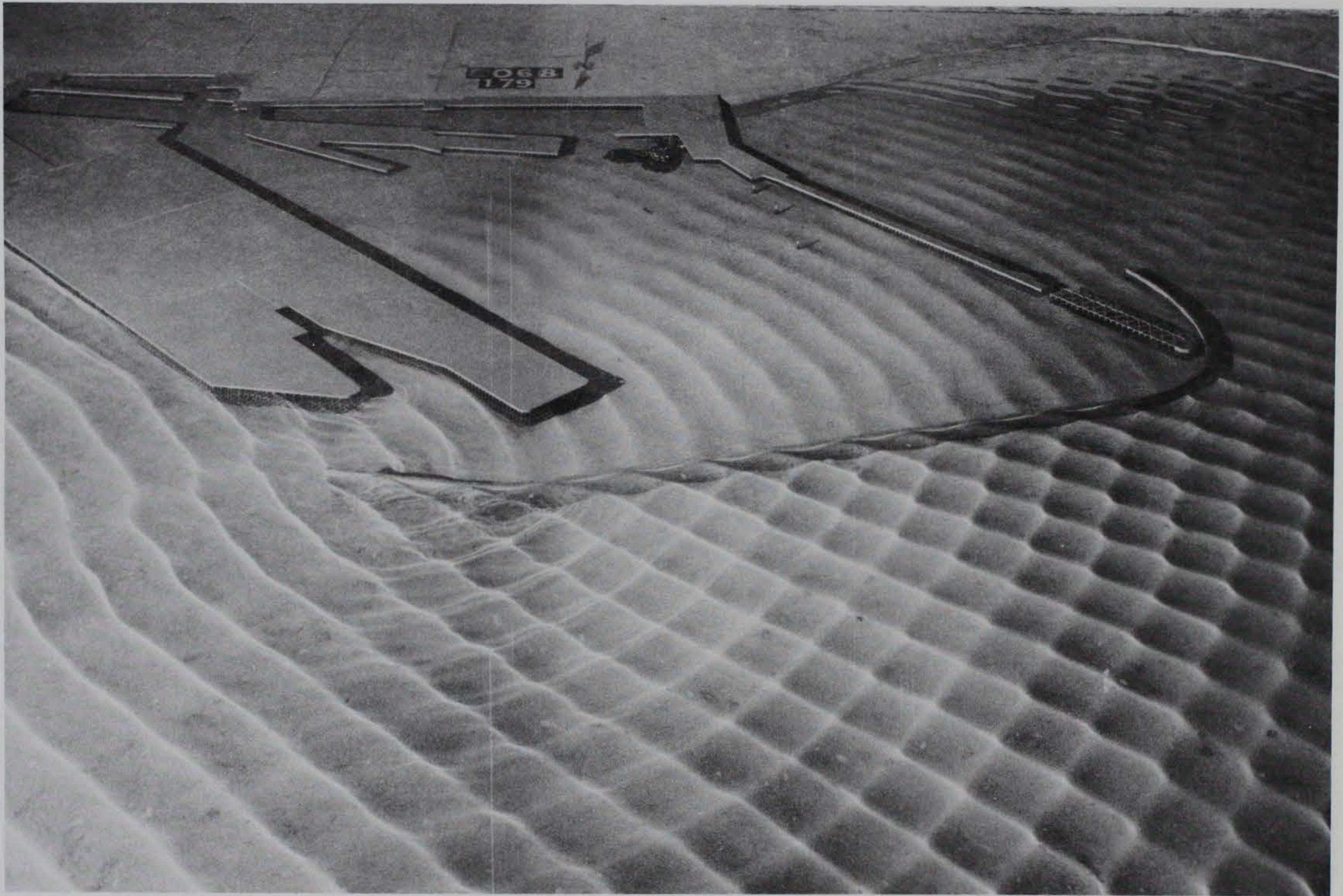
Photo 103. Typical wave patterns for Plan 42; 3.9-sec, 3.3-ft waves from northeast; +5.7 ft swl
