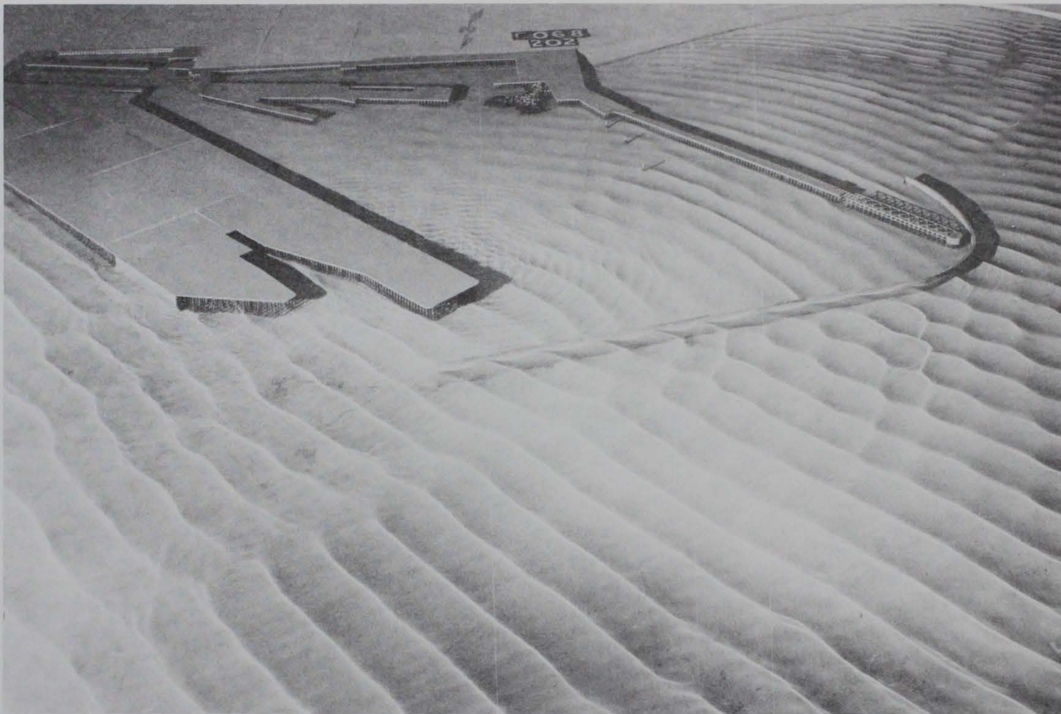
Photo 126. Typical wave patterns for Plan 66; 3.9-sec, 3.3-ft waves from northeast; 0.0-ft swl
