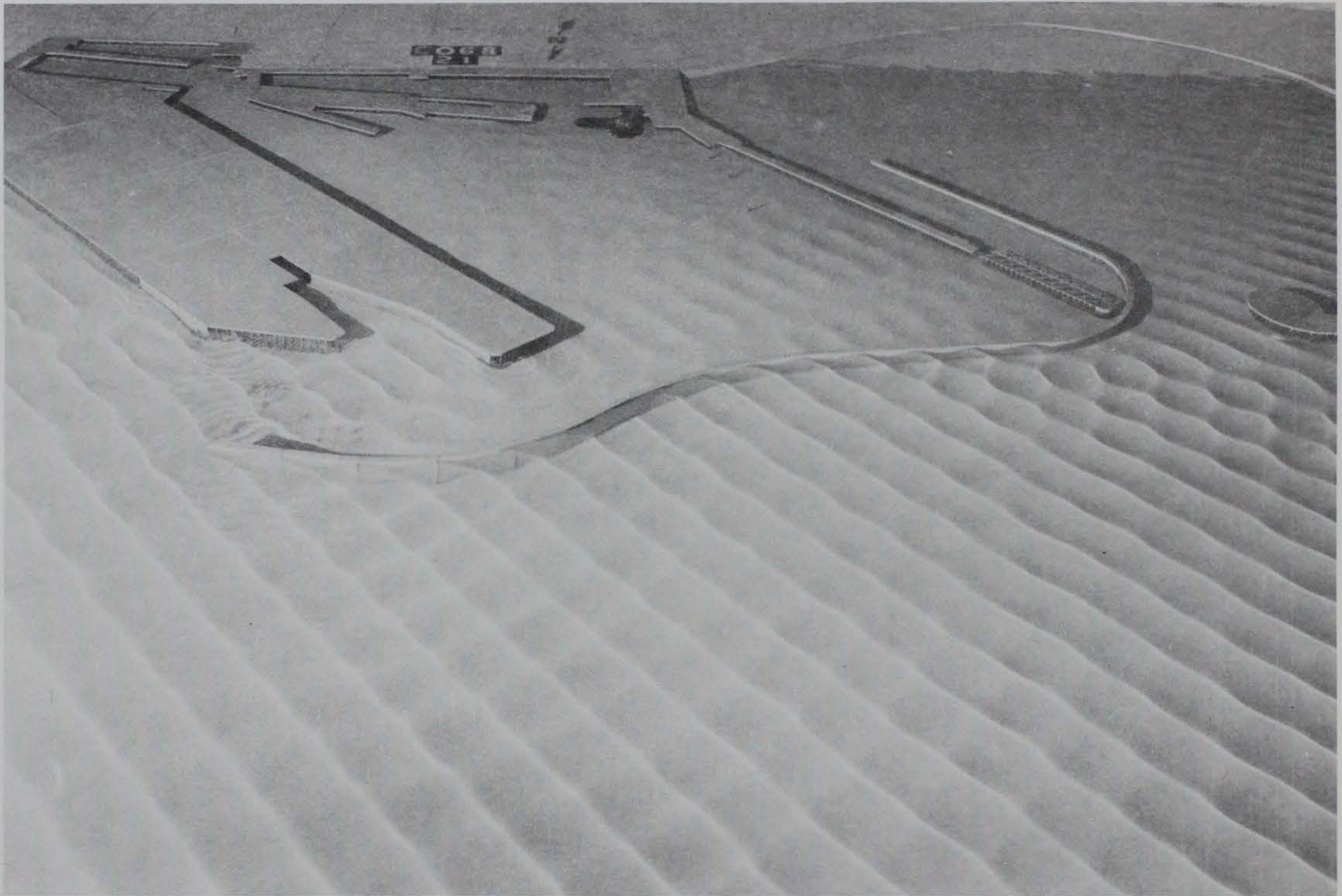
Photo 46. Typical wave patterns for Plan 15; 3.9-sec, 3.3-ft waves from northeast; +5.7 ft swl
