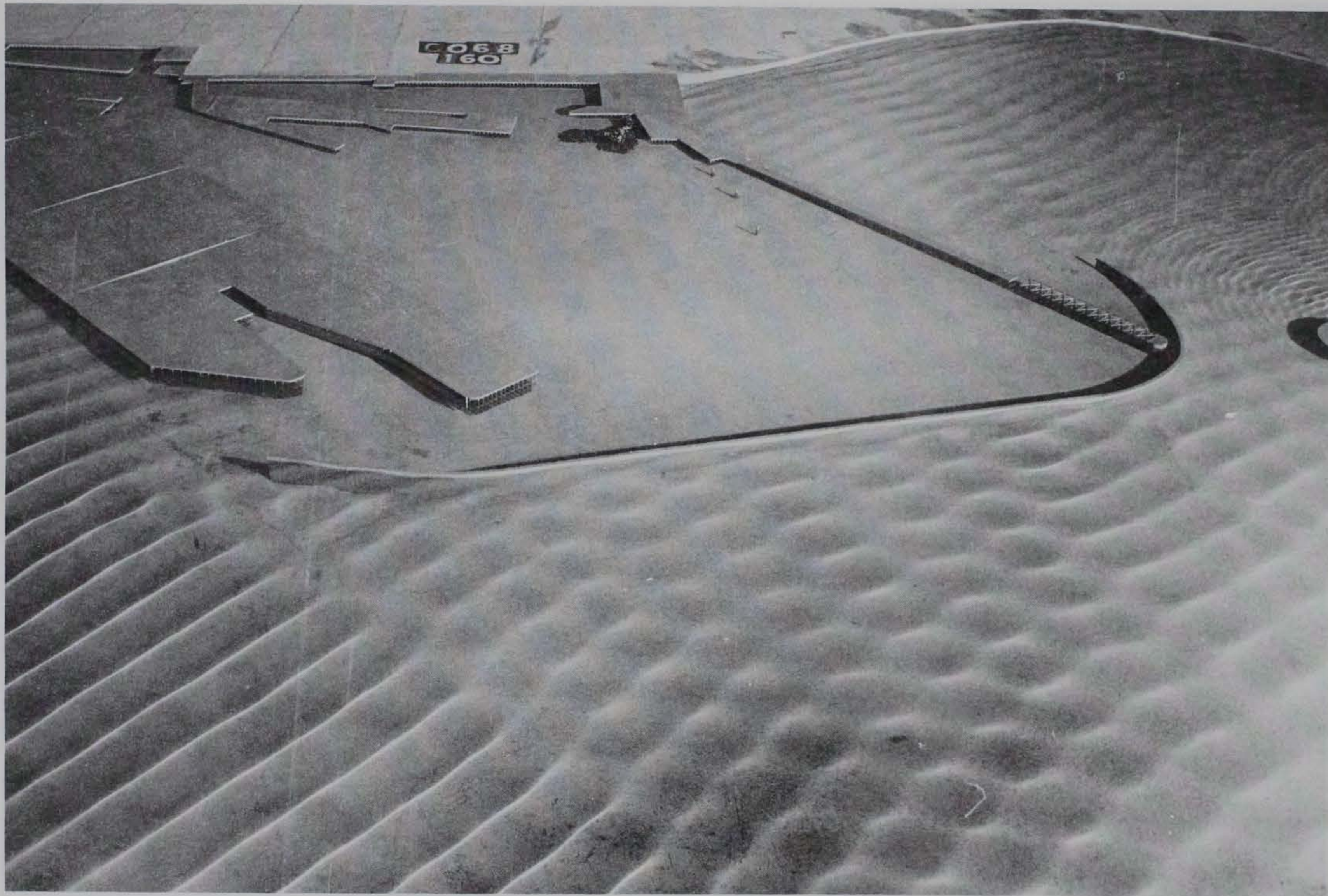
Photo 79. Typical wave patterns for Plan 38; 3.6-sec, 2-ft waves from northwest; +5.7 ft swl
