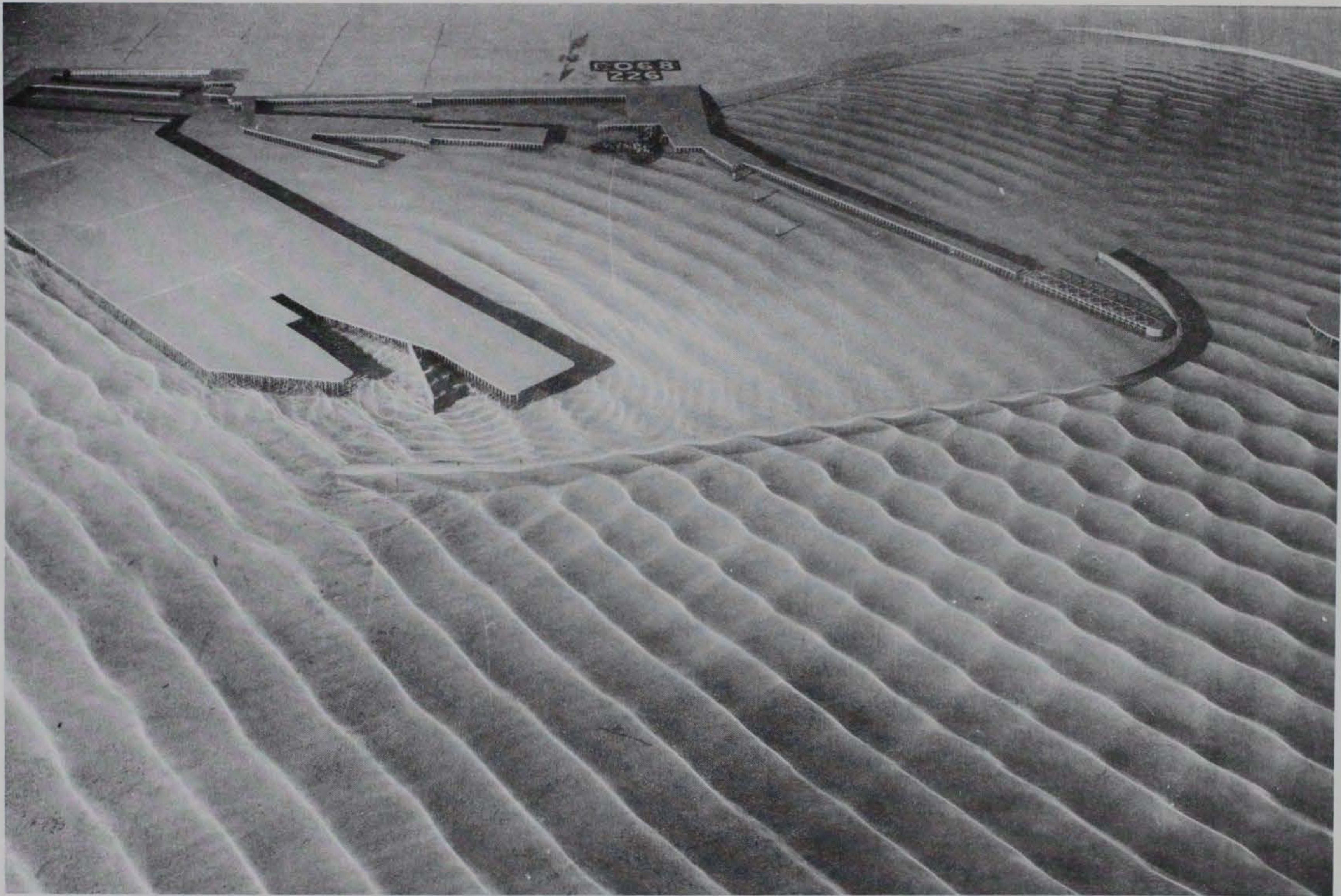
Photo 141. Typical wave patterns for Plan 81; 3.9-sec, 3.3-ft waves from northeast; 0.0-ft swl
