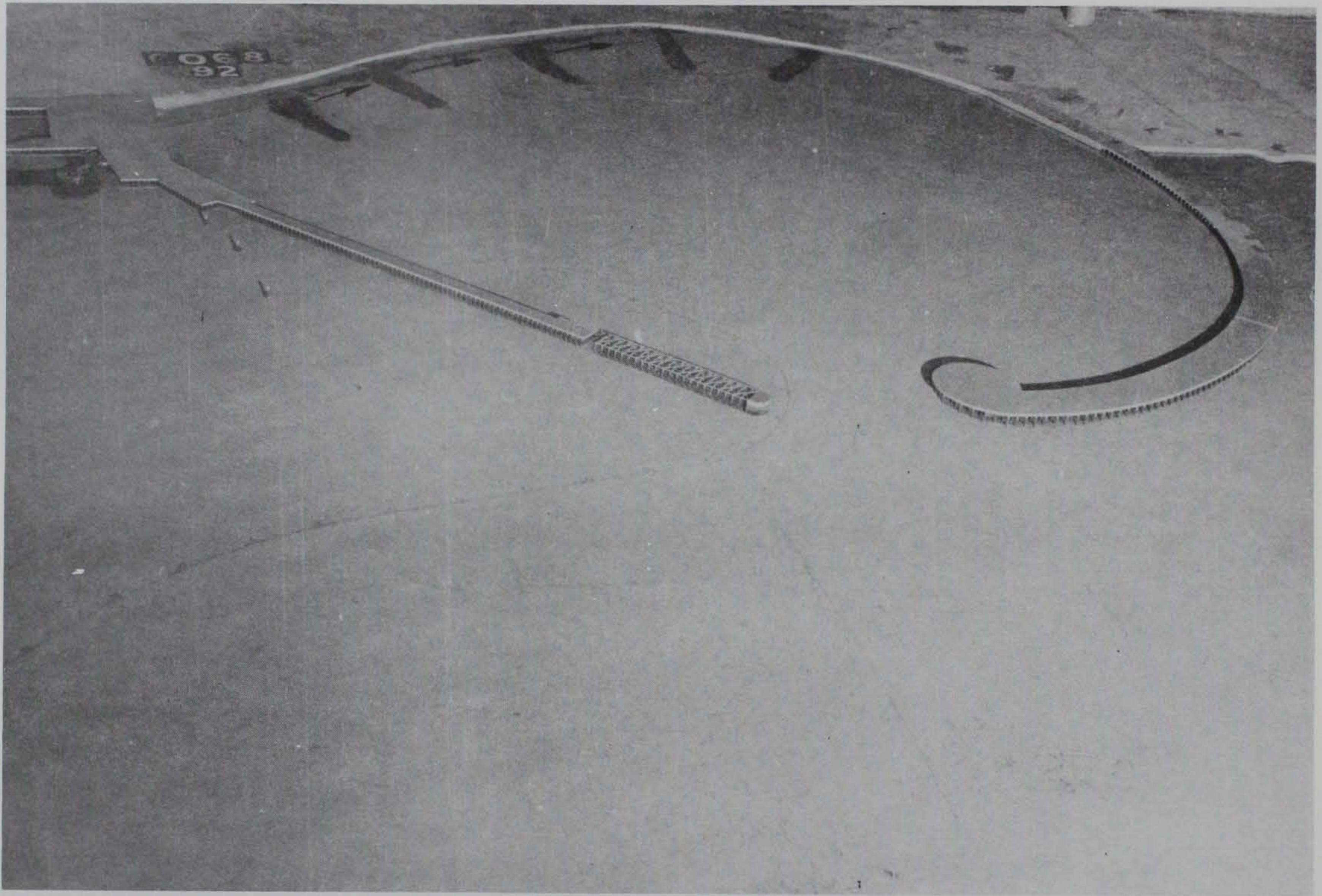
Photo 20. General movement of tracer material for existing conditions; 3.6-sec, 3.1-ft waves from north; +5.7 ft swl
