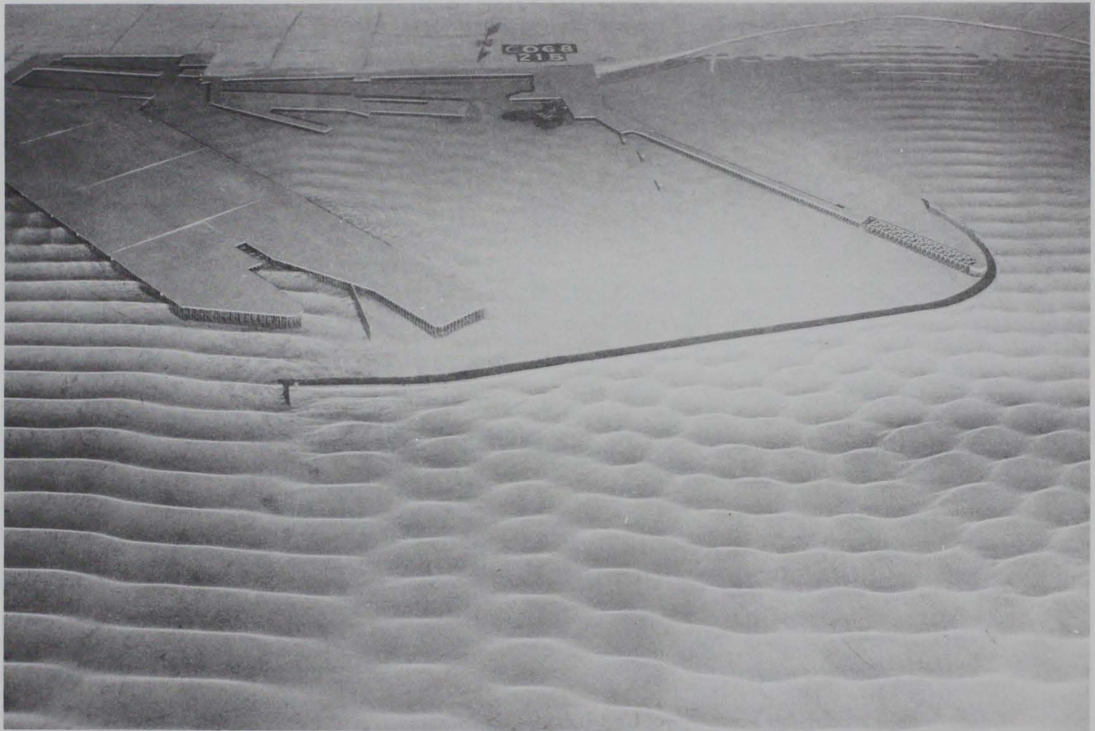
Photo 156. Typical wave patterns for Plan 78; 3.6-sec, 3.1-ft waves from north; +5.7 ft swl
