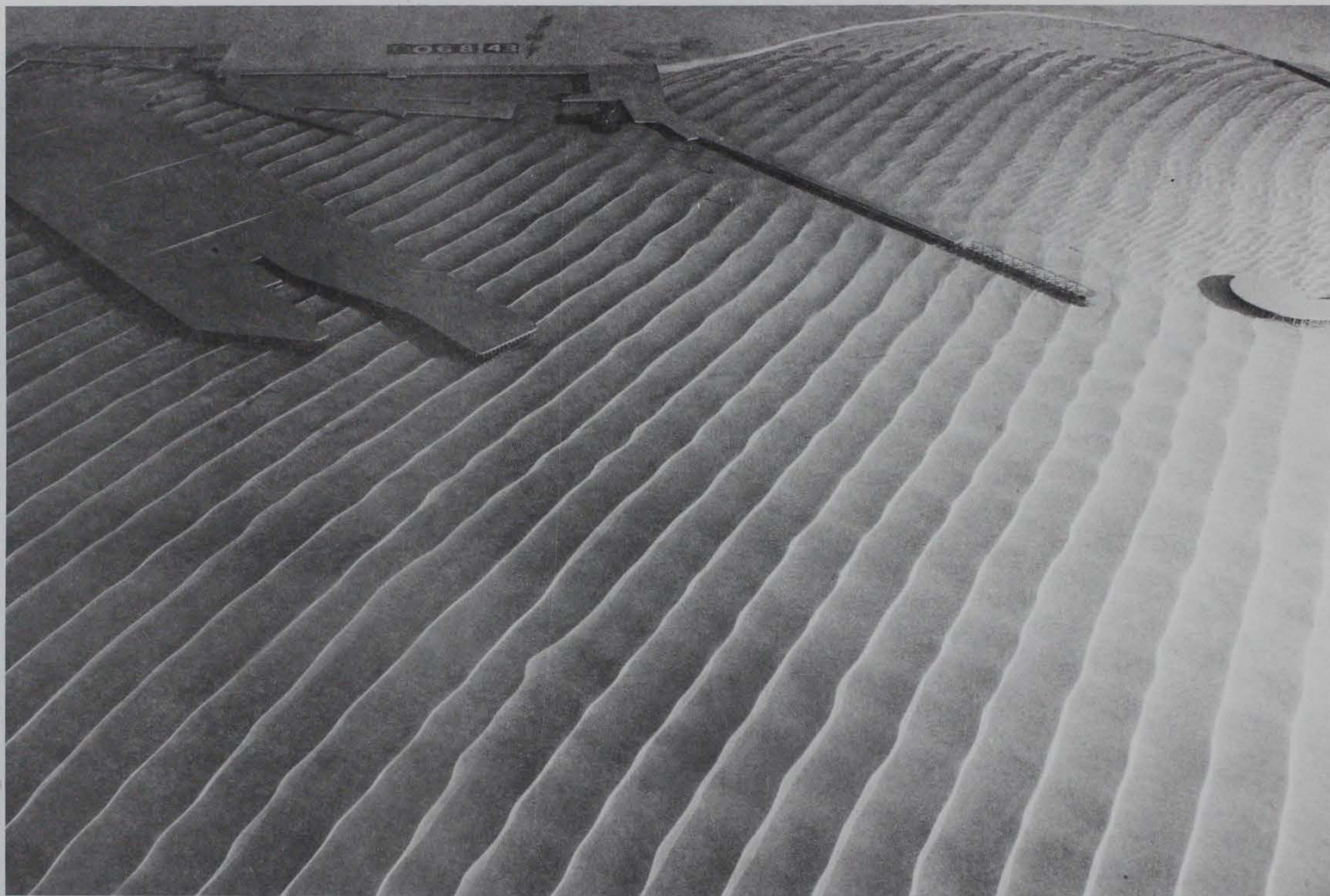
Photo 12. Typical wave patterns for existing conditions; 3.6-sec, 3.4-ft waves from west-northwest; +5.7 ft swl
