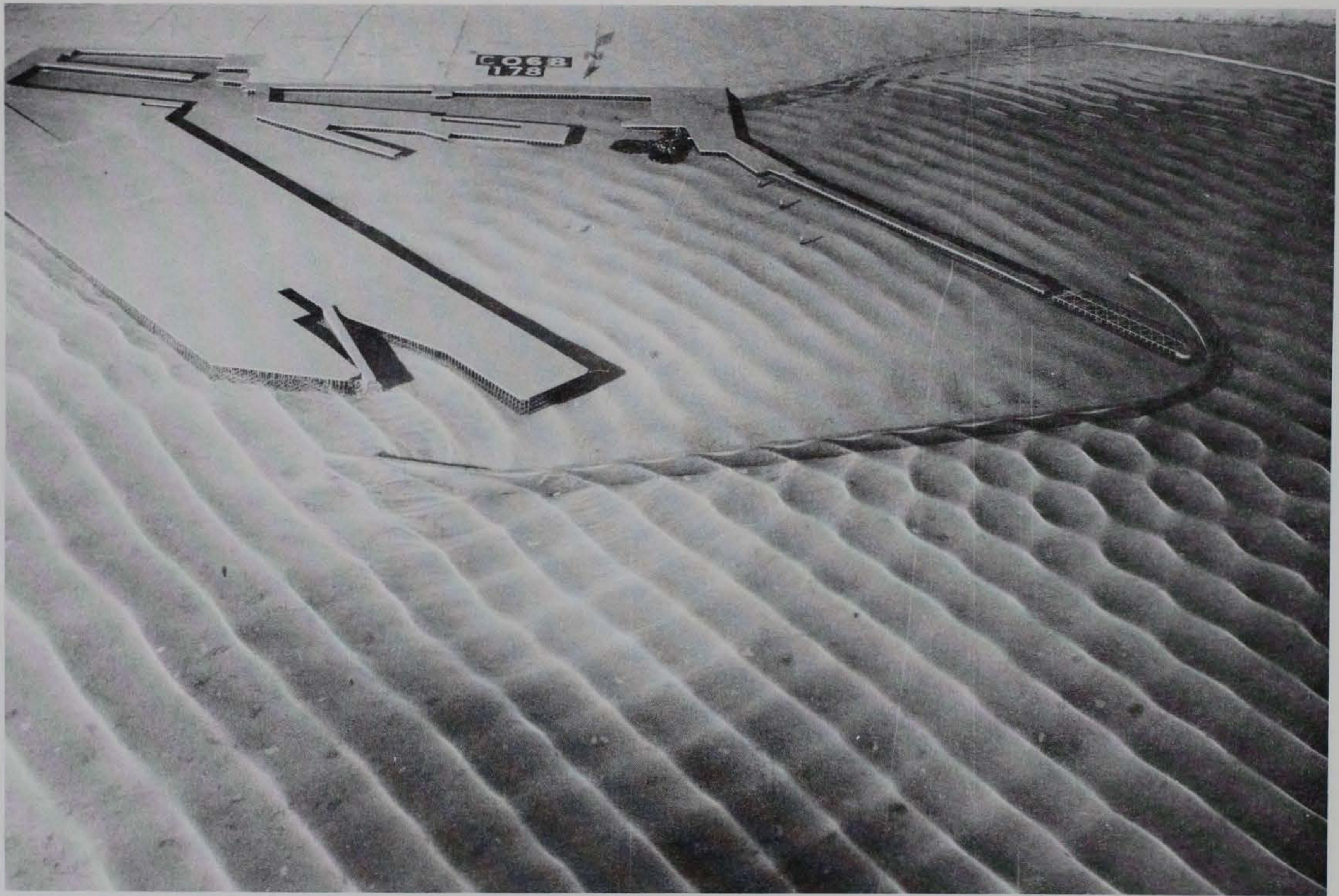
Photo 107. Typical wave patterns for Plan 46; 3.9-sec, 3.3-ft waves from northeast; +5.7 ft swl -
