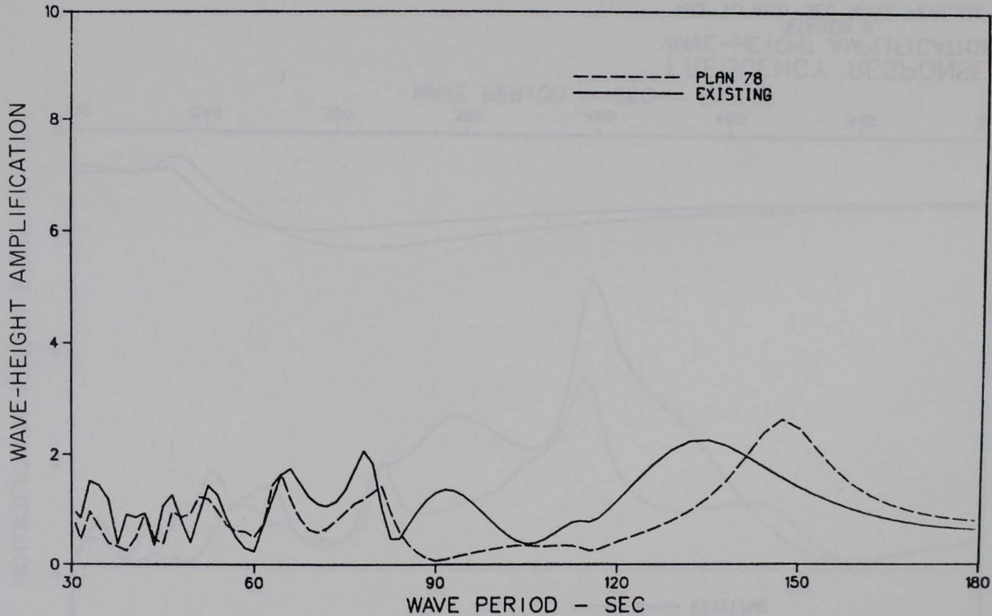
FREQUENCY RESPONSE WAVE-HEIGHT AMPLIFICATION STATION 9 30- TO 180-SEC WAVE PERIODS
