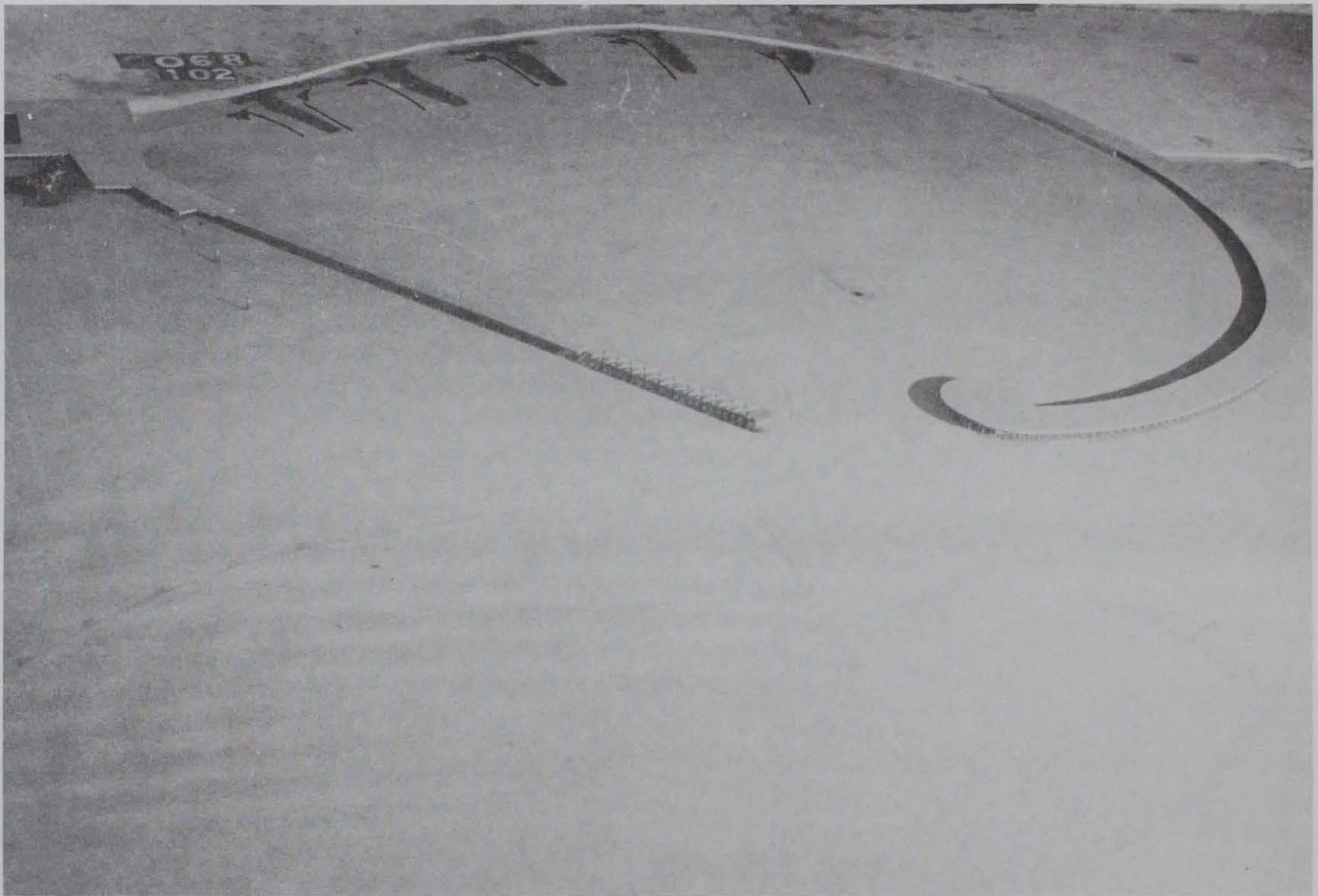
Photo 24. General movement of tracer material for existing conditions; 3.8-sec, 4.1-ft waves from northwest; +5.7 ft swl
