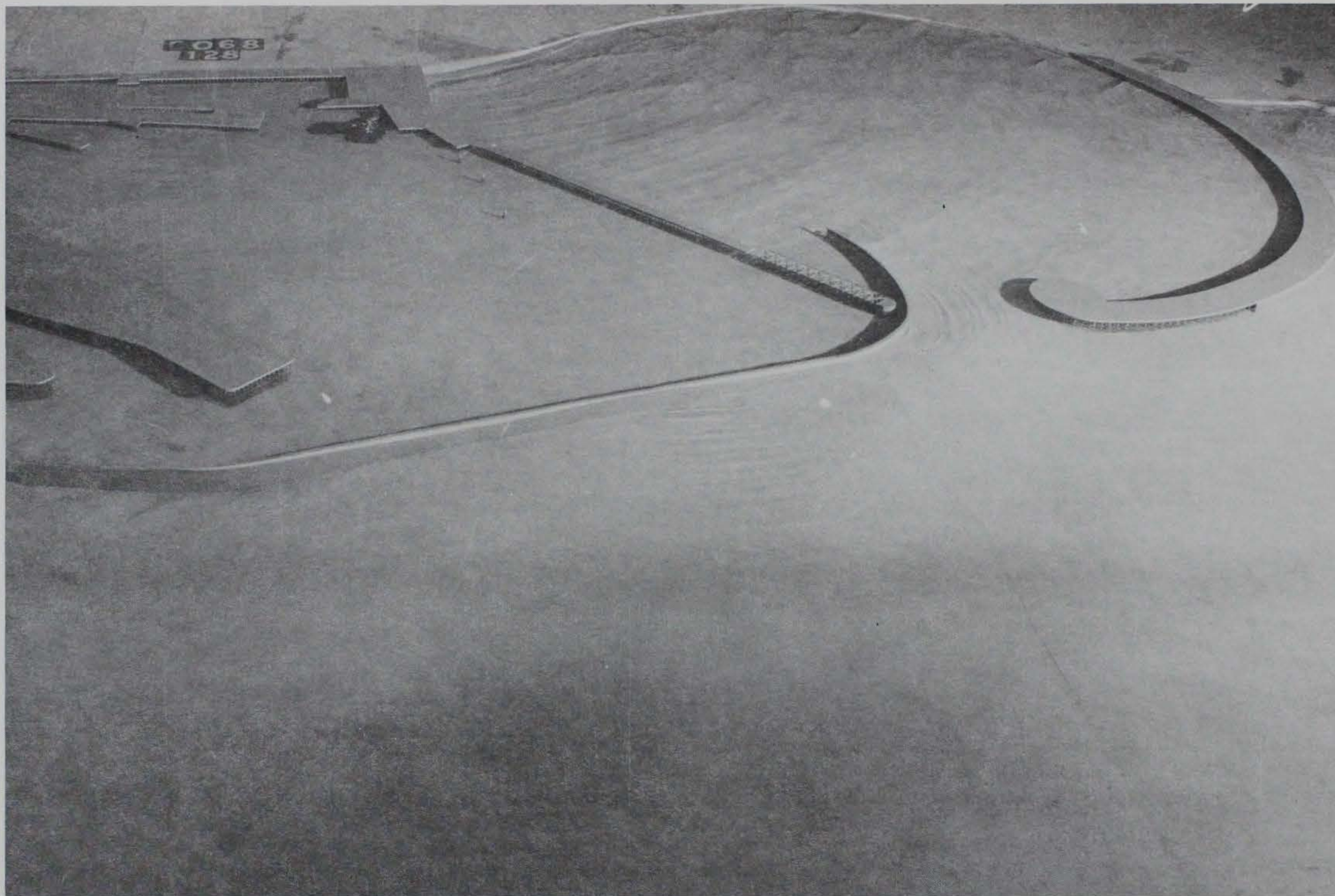
Photo 64. Typical wave patterns for Plan 33; 10-sec, 3-ft waves from west-northwest; +5.7 ft swl
