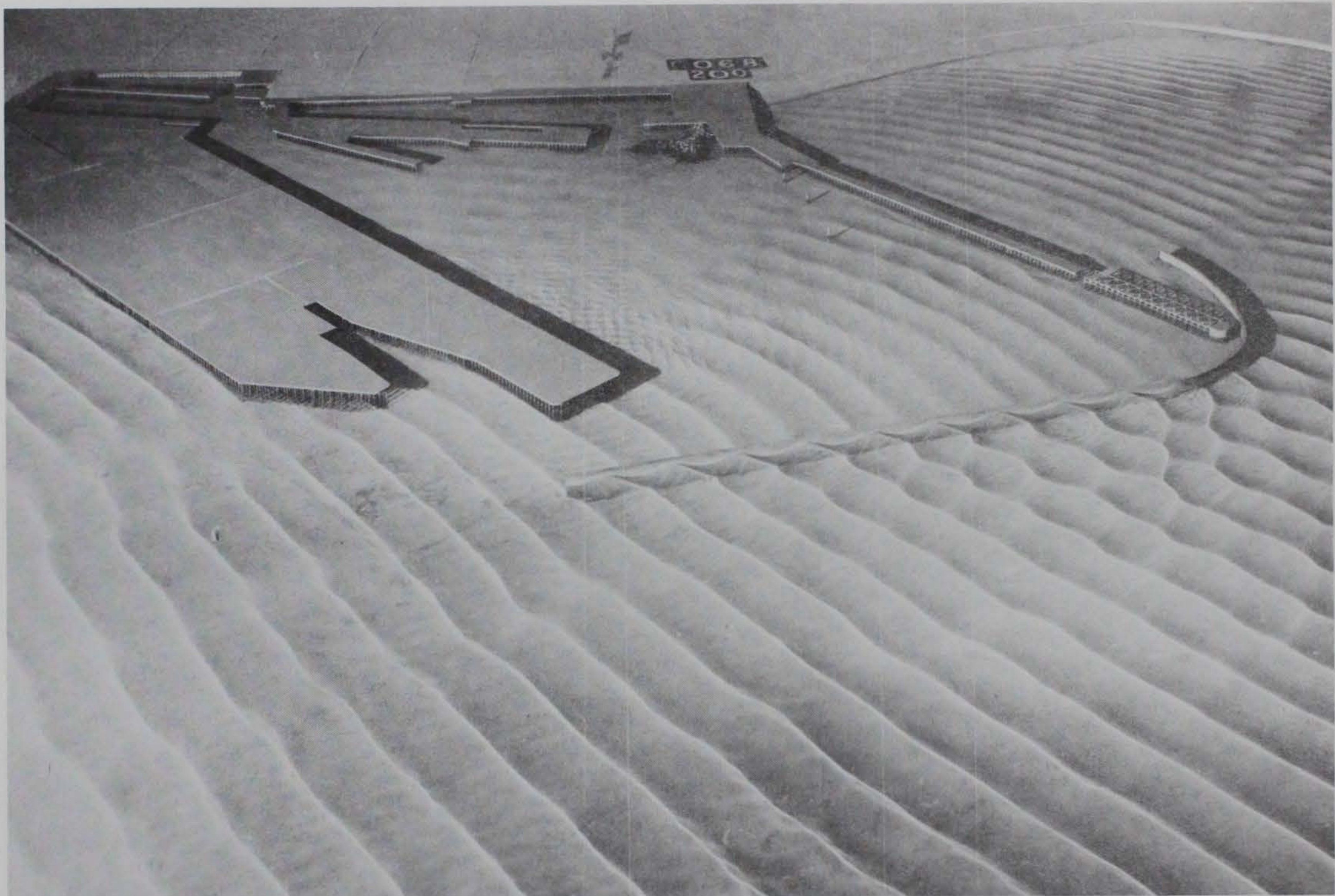
Photo 132. Typical wave patterns for Plan 72; 3.9-sec, 3.3-ft waves from northeast; 0.0-ft swl
