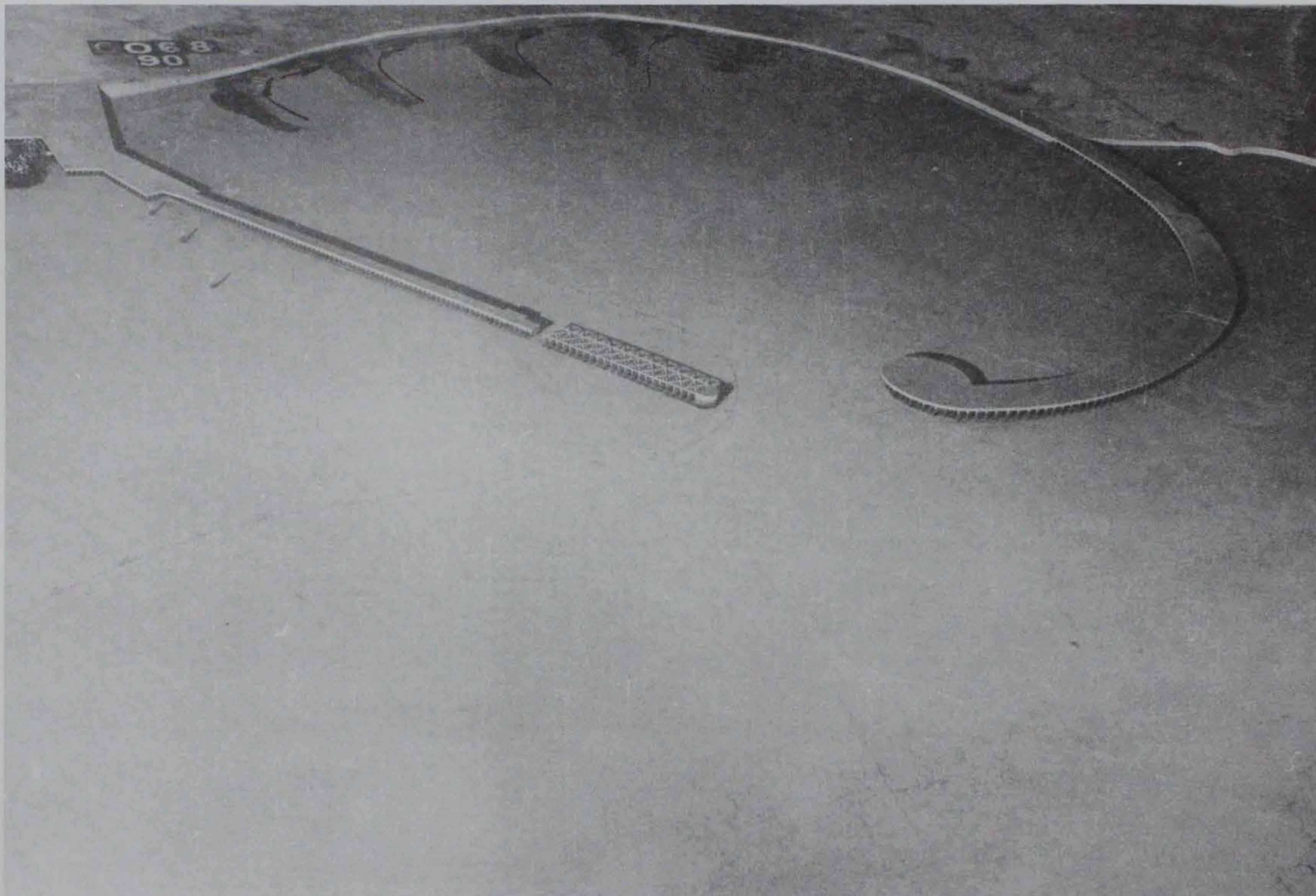
Photo 18. General movement of tracer material for existing conditions; 4.2-sec, 4.8-ft waves from north-northeast; +5.7 ft swl
