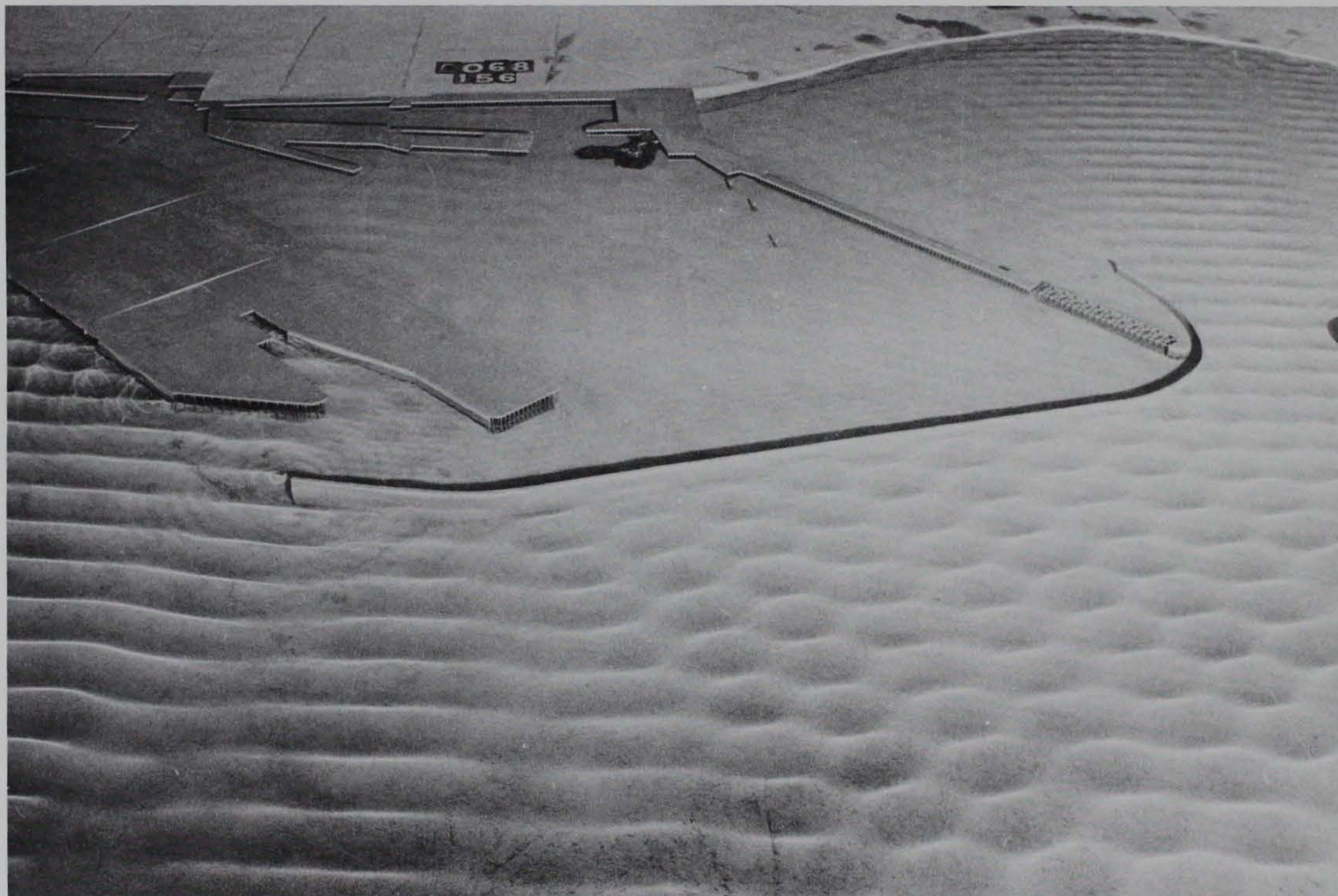
Photo 75. Typical wave patterns for Plan 38; 3.6-sec, 2.0-ft waves from north; +5.7 ft swl
