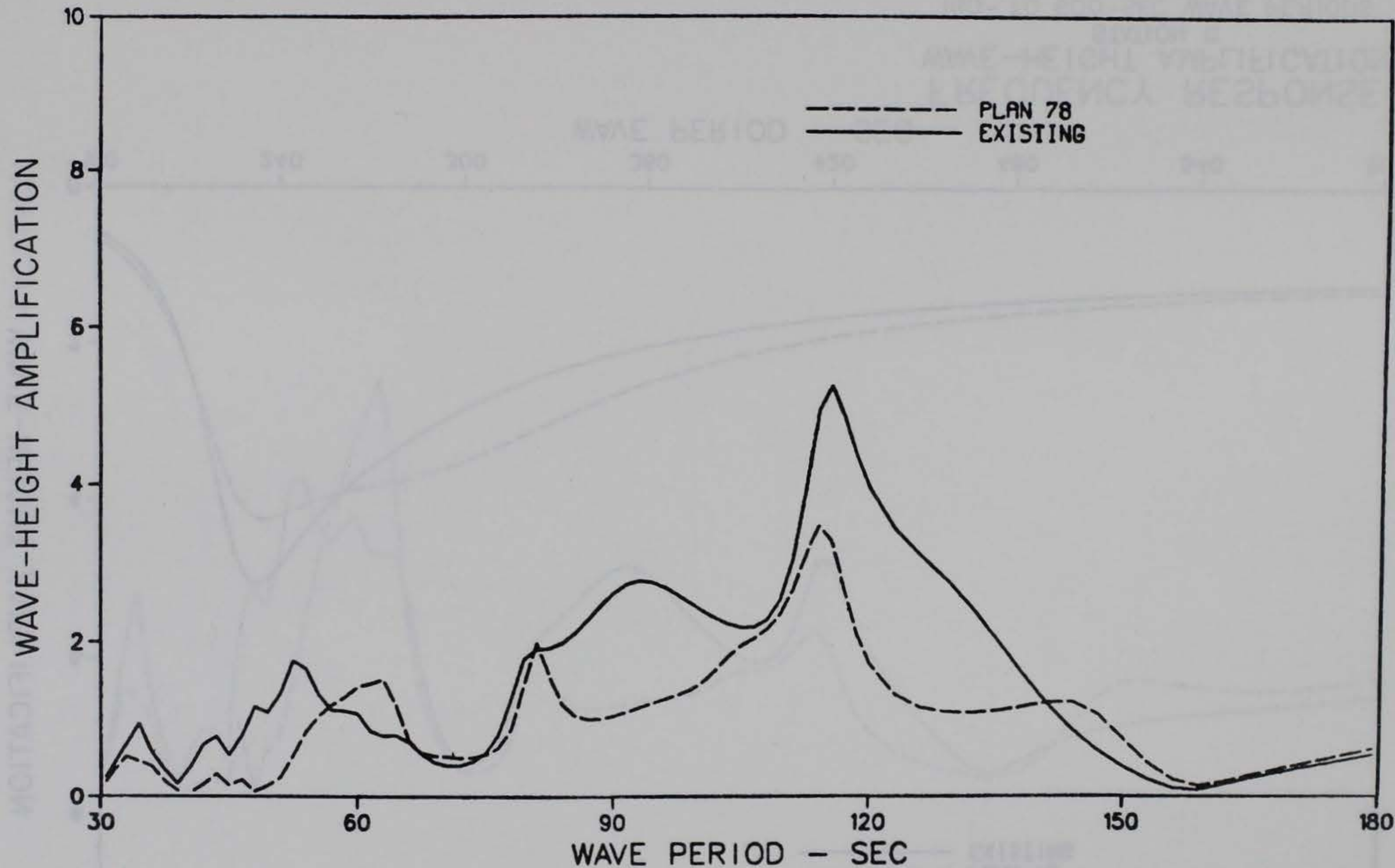
FREQUENCY RESPONSE WAVE-HEIGHT AMPLIFICATION STATION 11 30- TO 180-SEC WAVE PERIODS
