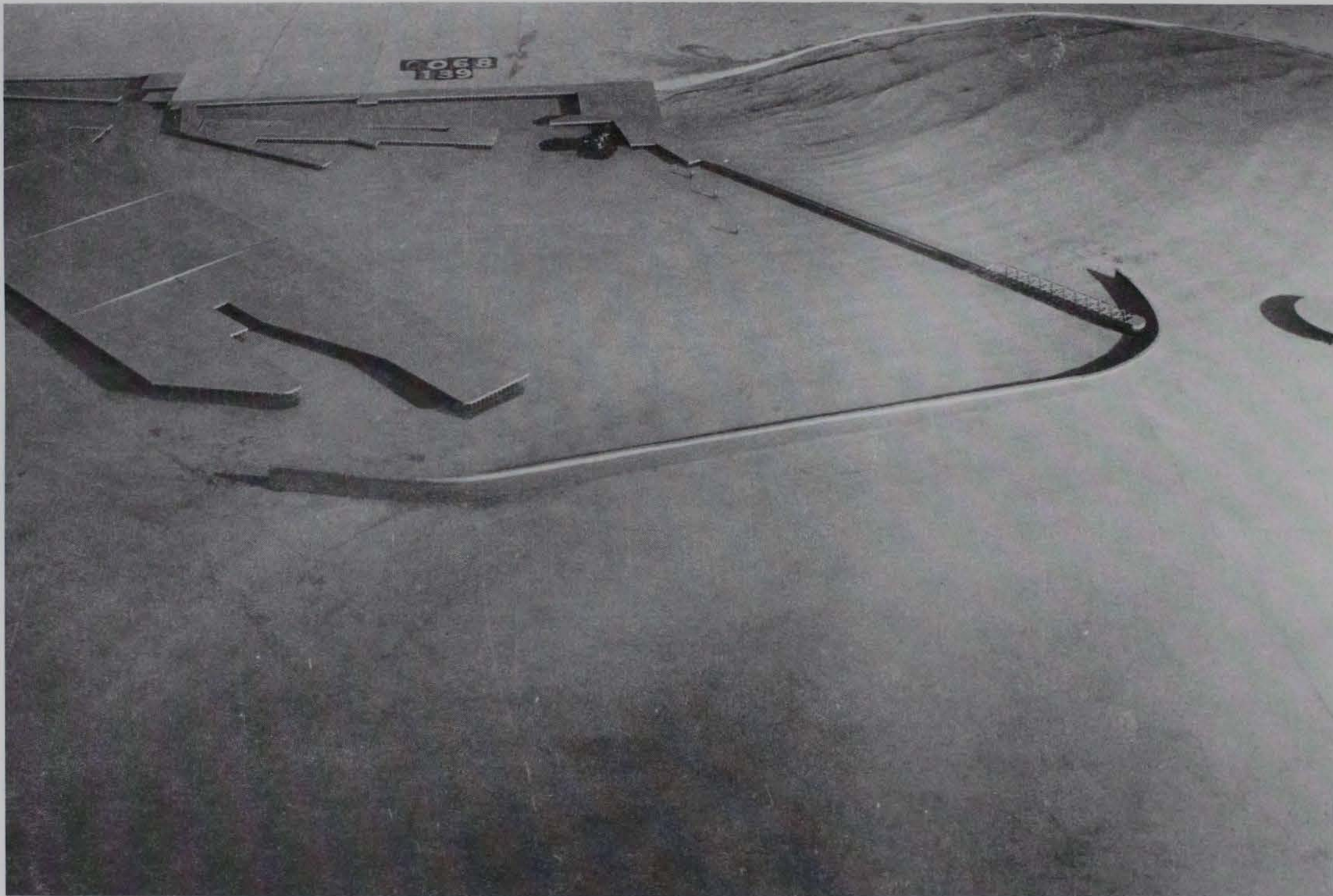
Photo 53. Typical wave patterns for Plan 22; 10-sec, 2-ft waves from west-northwest; +5.7 ft swl
