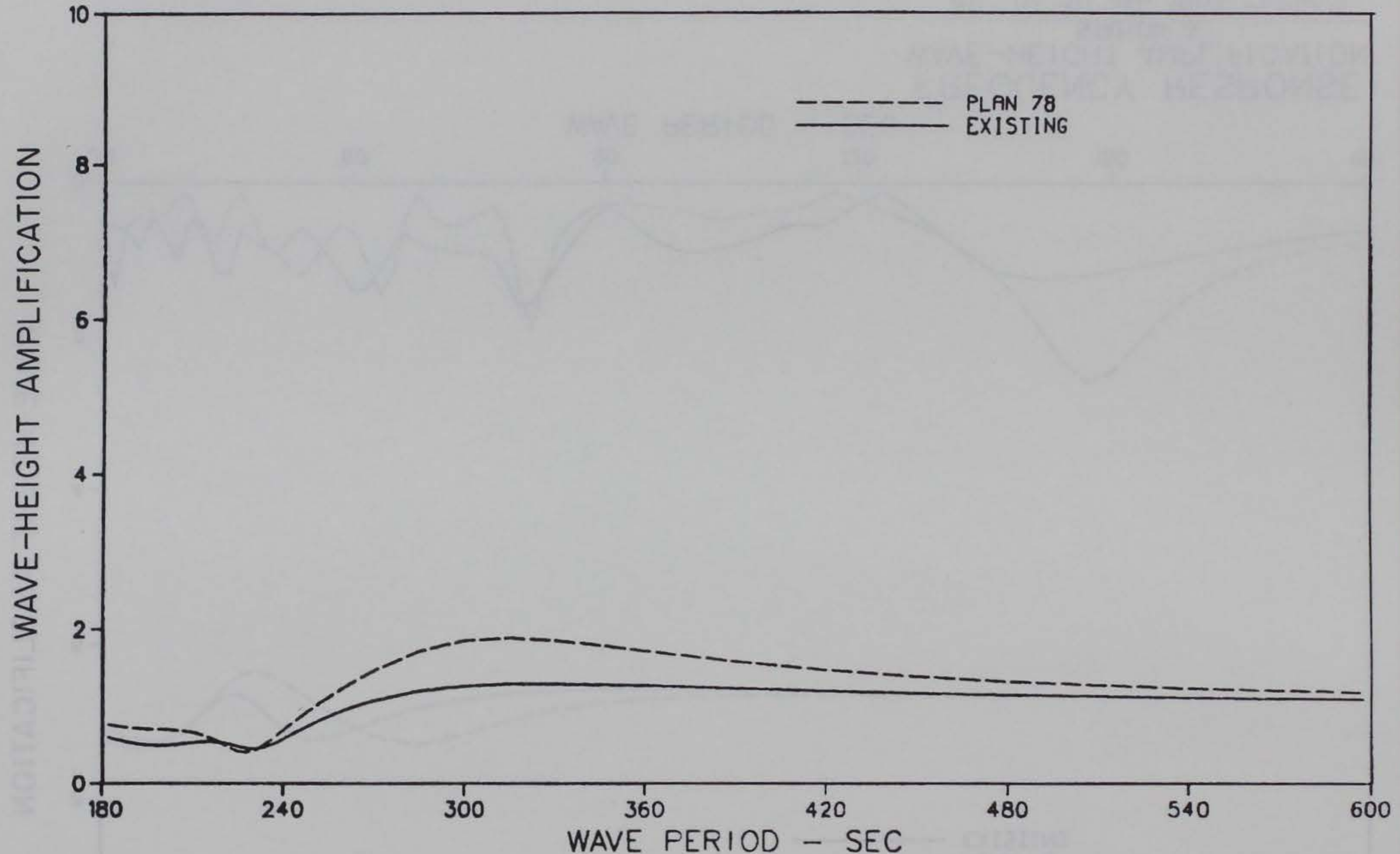
FREQUENCY RESPONSE WAVE-HEIGHT AMPLIFICATION STATION 3 180- TO 600-SEC WAVE PERIODS
