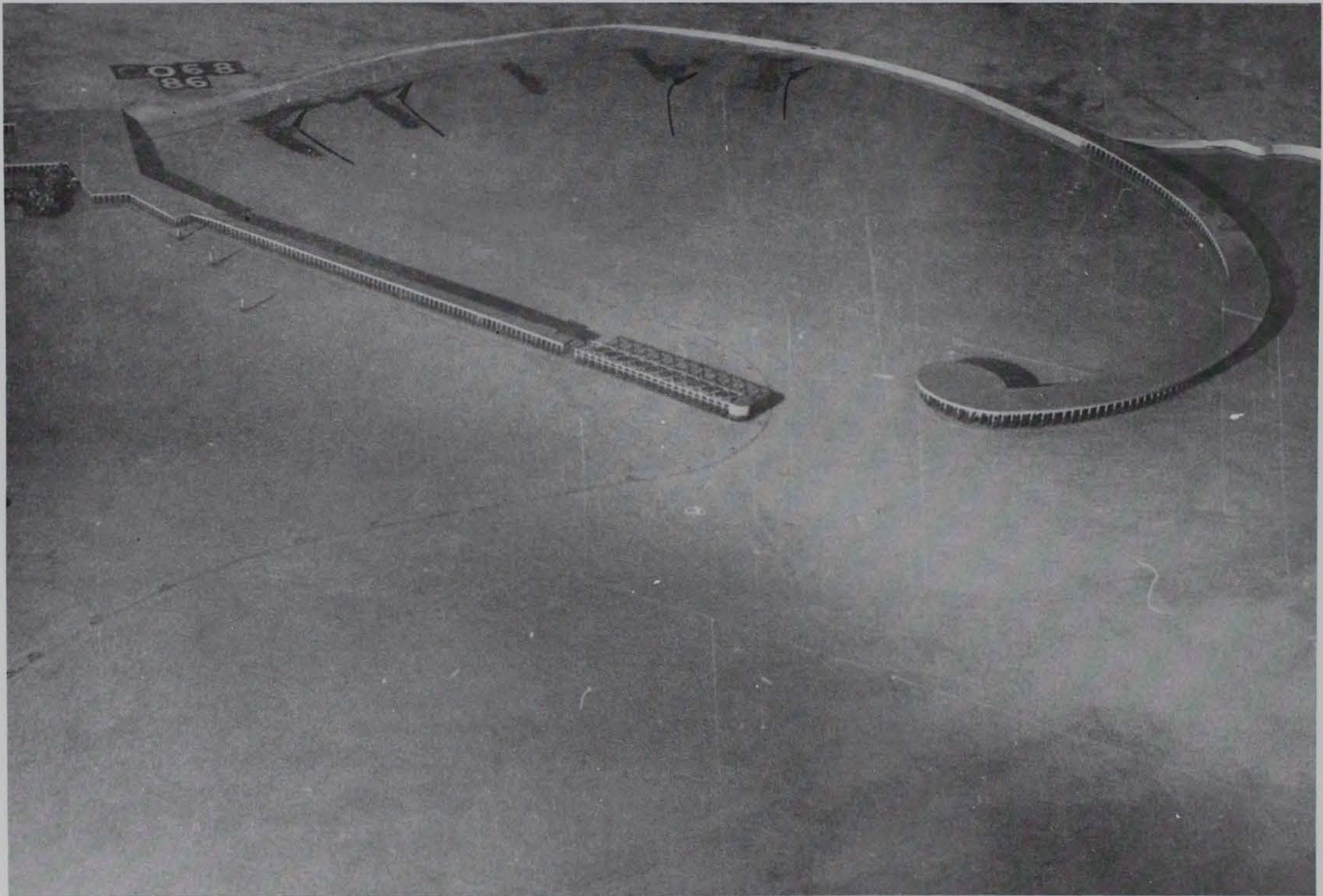
Photo 15. General movement of tracer material for existing conditions; 3.9-sec, 3.3-ft waves from northeast; 0.0-ft swl
