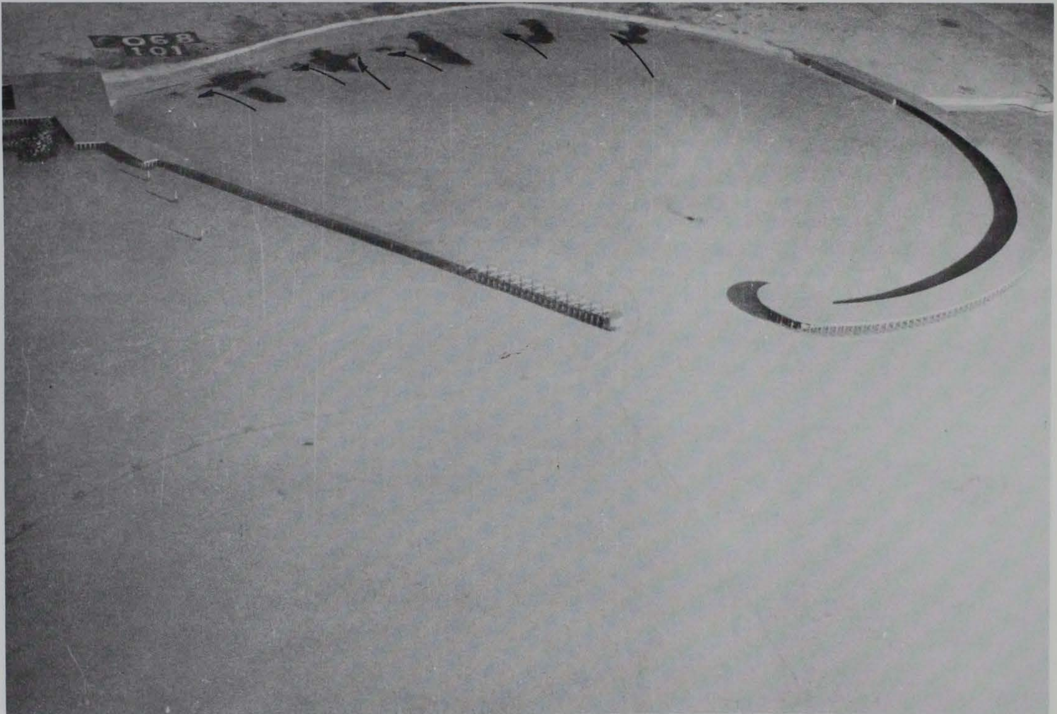
Photo 23. General movement of tracer material for existing conditions; 3.8-sec, 4.1-ft waves from northwest; 0.0-ft swl
