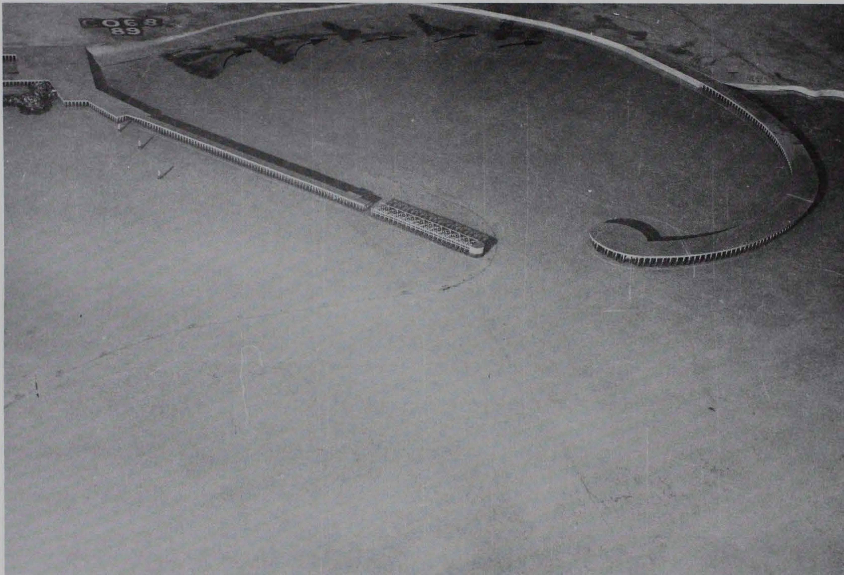
Photo 17. General movement of tracer material for existing conditions; 4.2-sec, 4.8-ft waves from north-northeast; 0.0-ft swl
