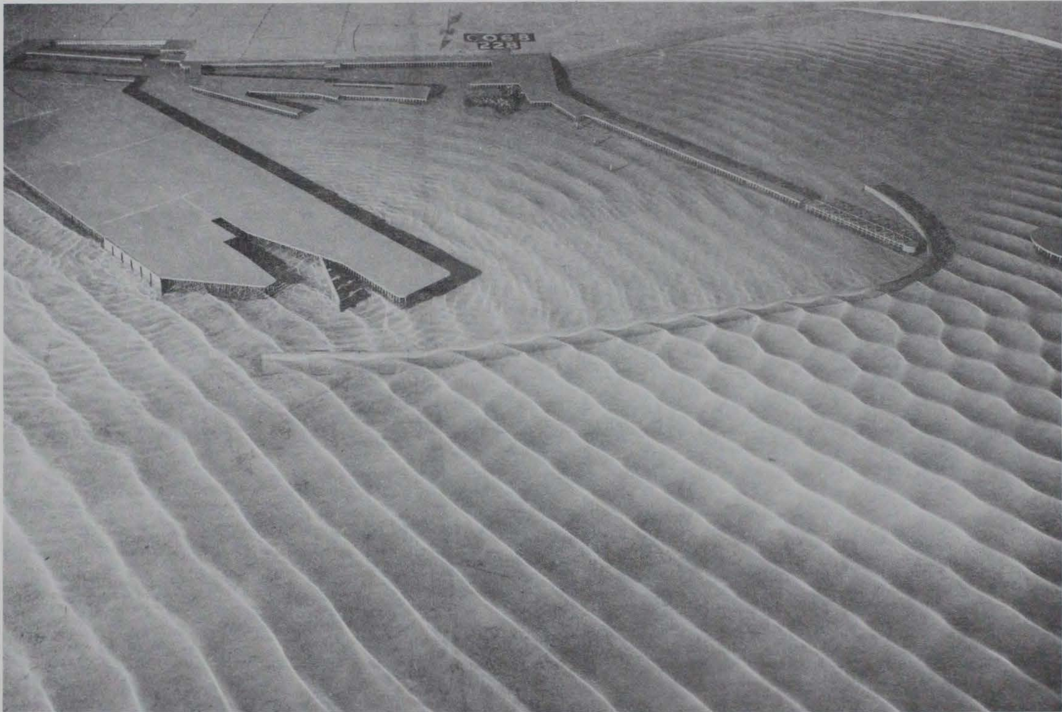
Photo 144. Typical wave patterns for Plan 84; 3.9-sec, 3.3-ft waves from northeast; 0.0-ft swl
