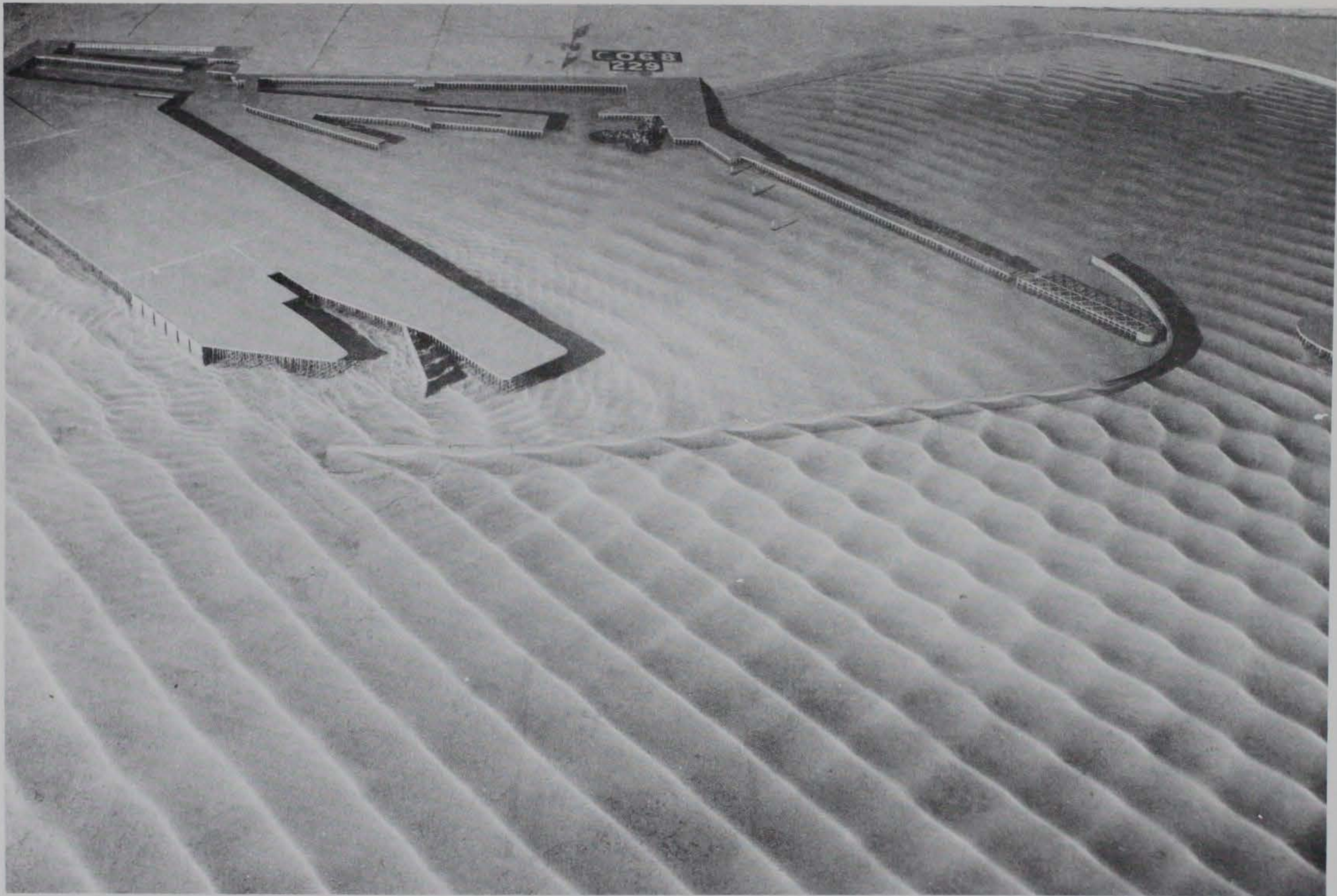
Photo 143. Typical wave patterns for Plan 83; 3.9-sec, 3.3-ft waves from northeast; 0.0-ft swl
