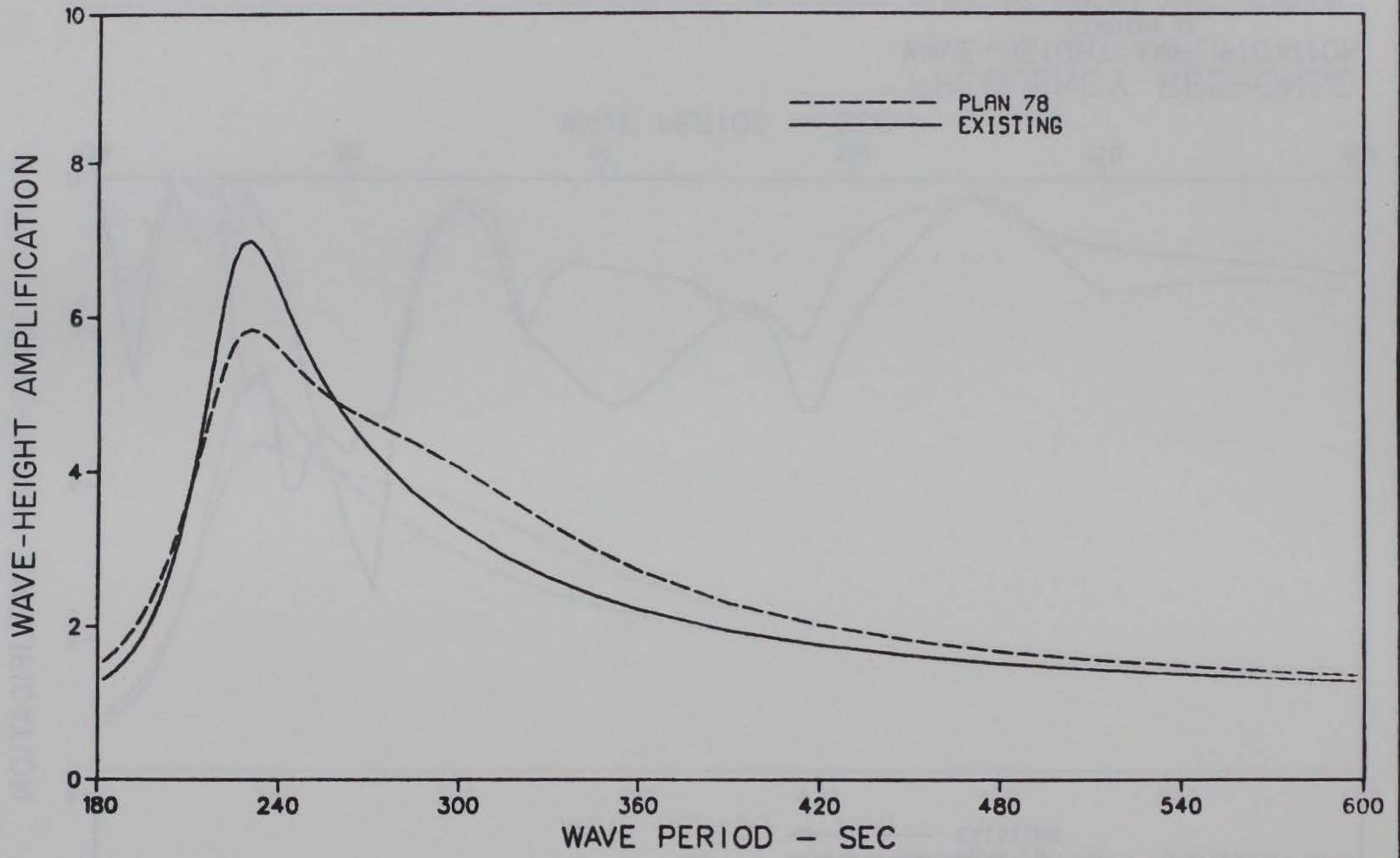
FREQUENCY RESPONSE WAVE-HEIGHT AMPLIFICATION STATION 12 180- TO 600-SEC WAVE PERIODS
