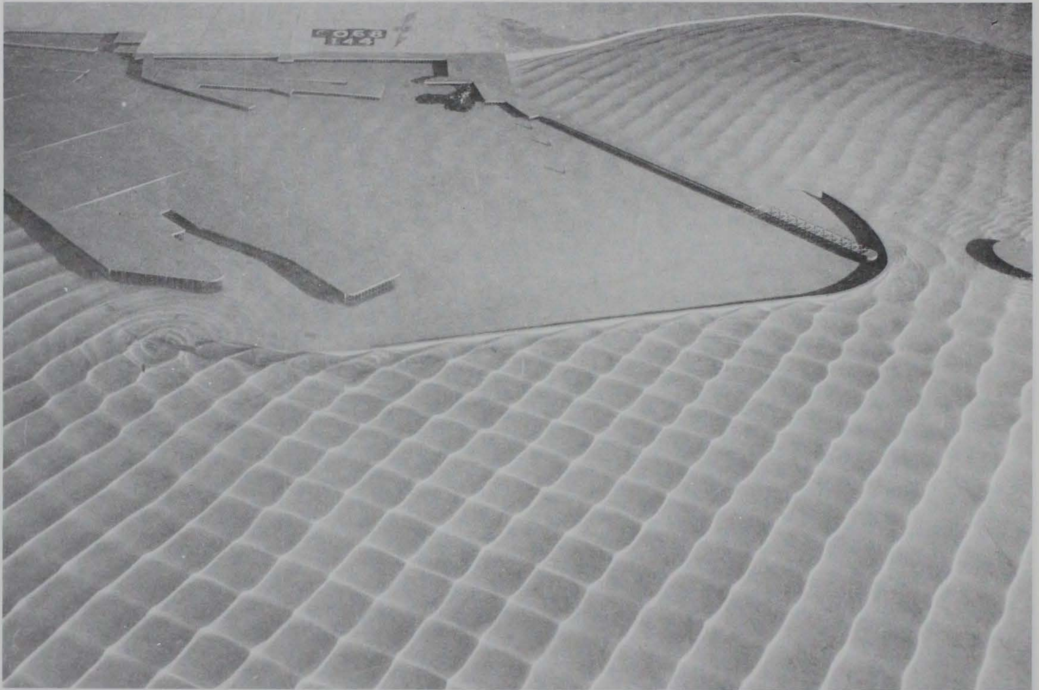
Photo 82. Typical wave patterns for Plan 38; 3.6-sec, 3.4-ft waves from west-northwest; +5.7 ft swl
