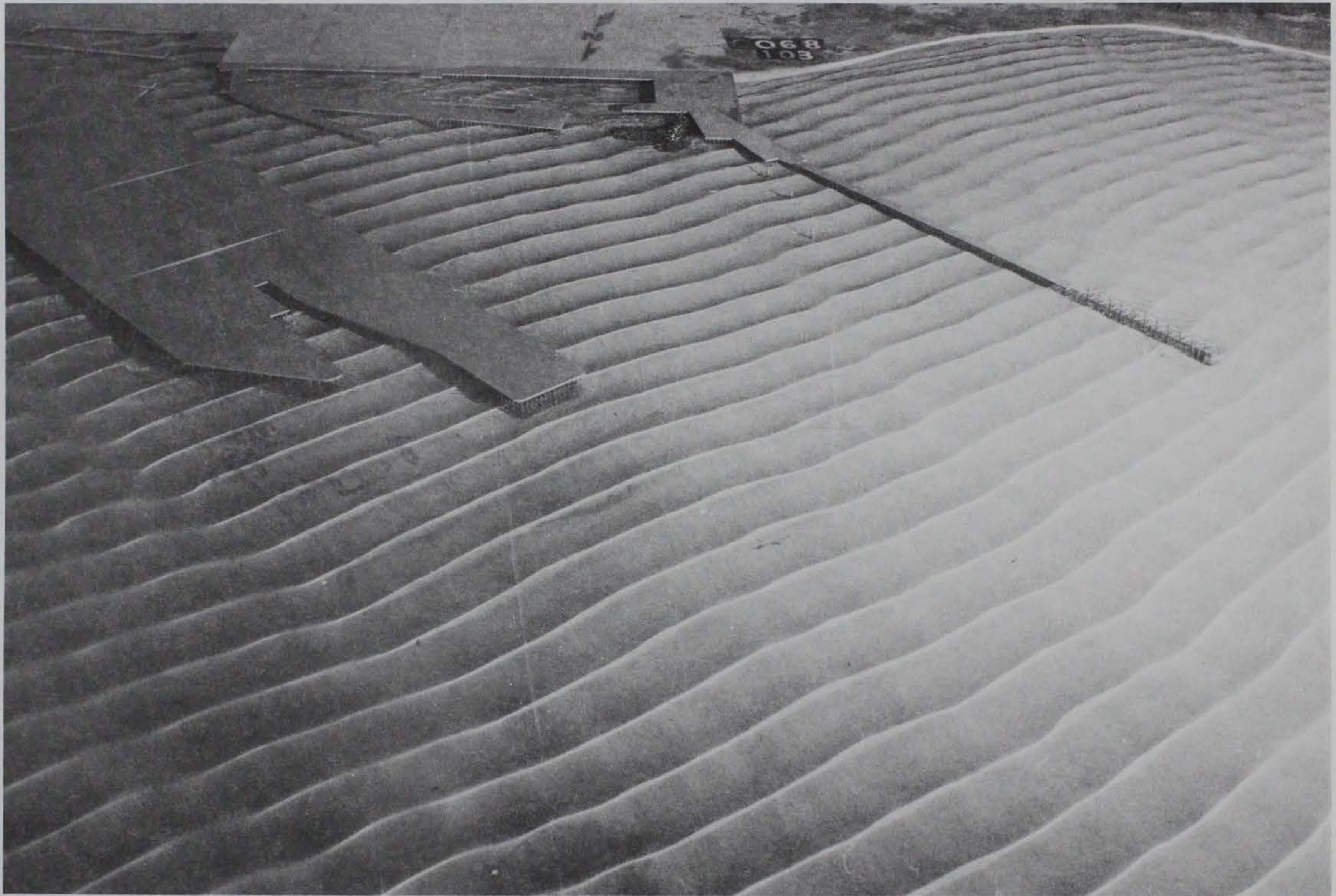
Photo 10. Typical wave patterns for existing conditions; 3.8-sec, 4.1-ft waves from northwest; +5.7 ft swl
