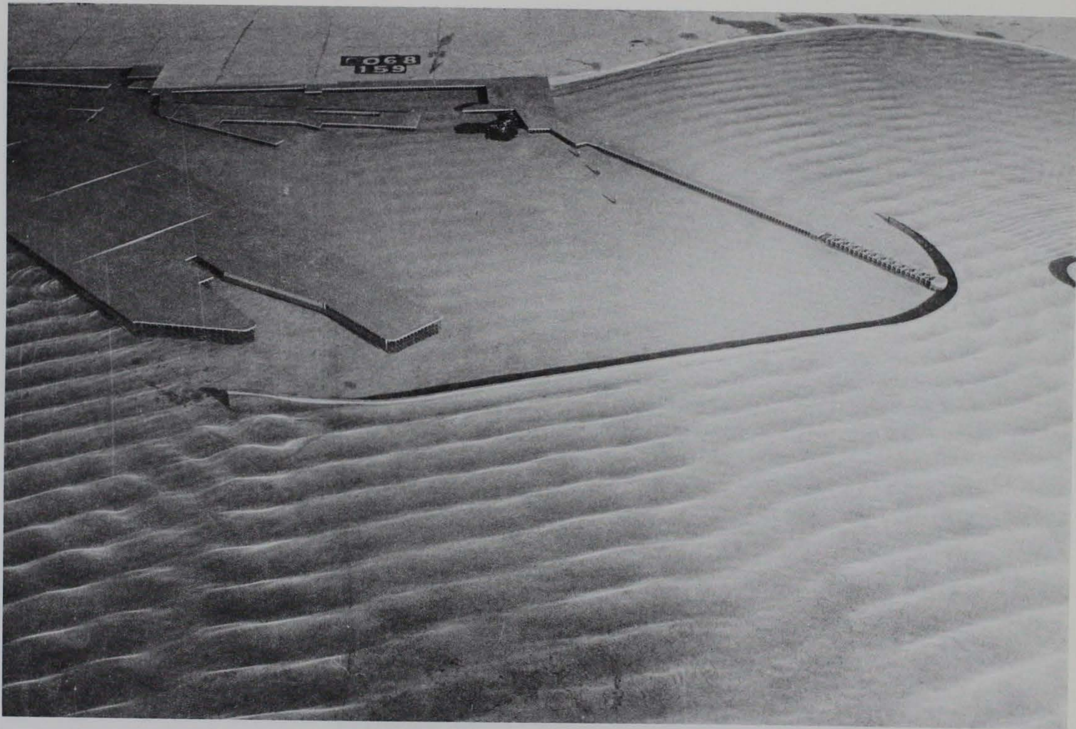
Photo 77. Typical wave patterns for Plan 38; 3.6-sec, 2-ft waves from north-northwest; +5.7 ft swl
