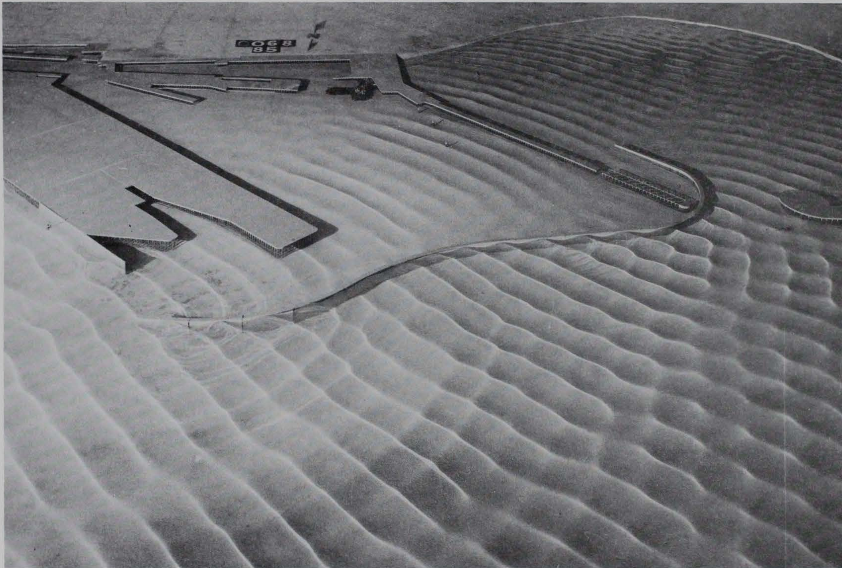
Photo 49. Typical wave patterns for Plan 18; 3.9-sec, 3.3-ft waves from northeast; +5.7 ft swl
