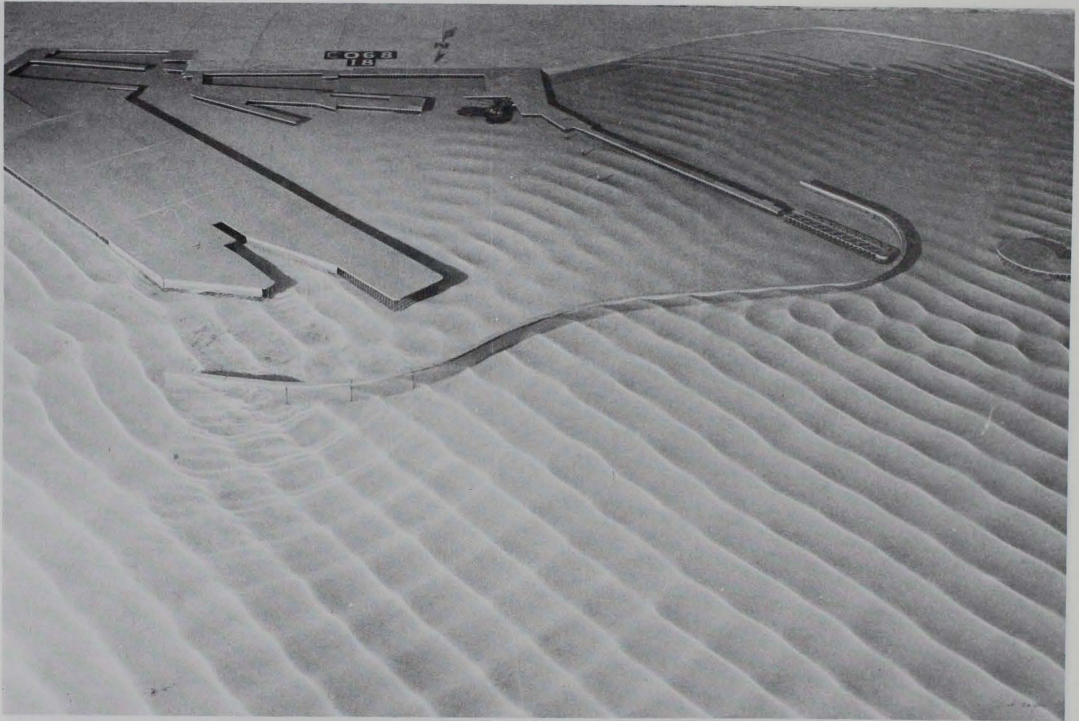
Photo 43. Typical wave patterns for Plan 12; 3.9-sec, 3.3-ft waves from northeast; +5.7 ft swl
