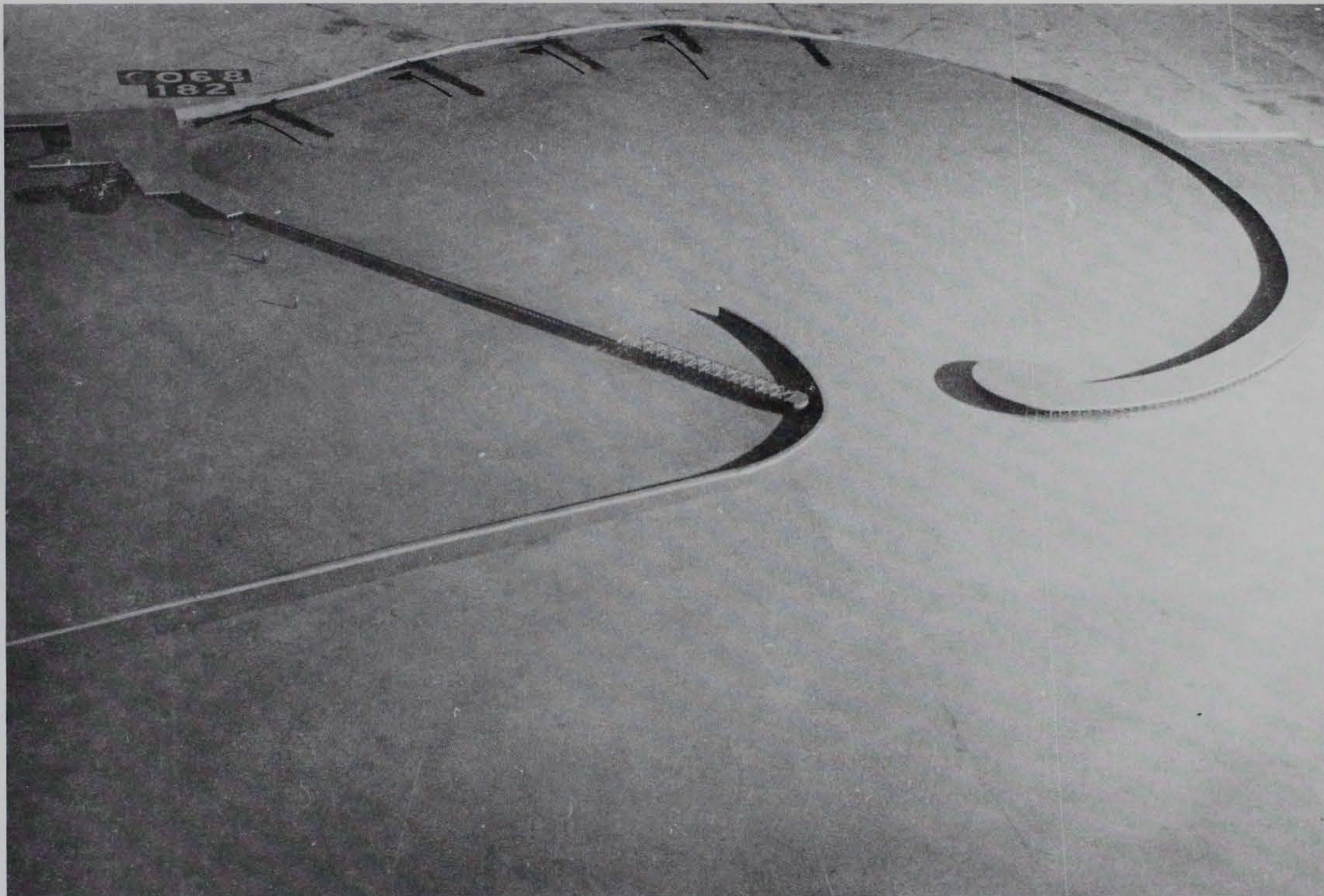
Photo 97. General movement of tracer material for Plan 38; 3.6-sec, 3.4-ft waves from west-northwest; +5.7 ft swl
