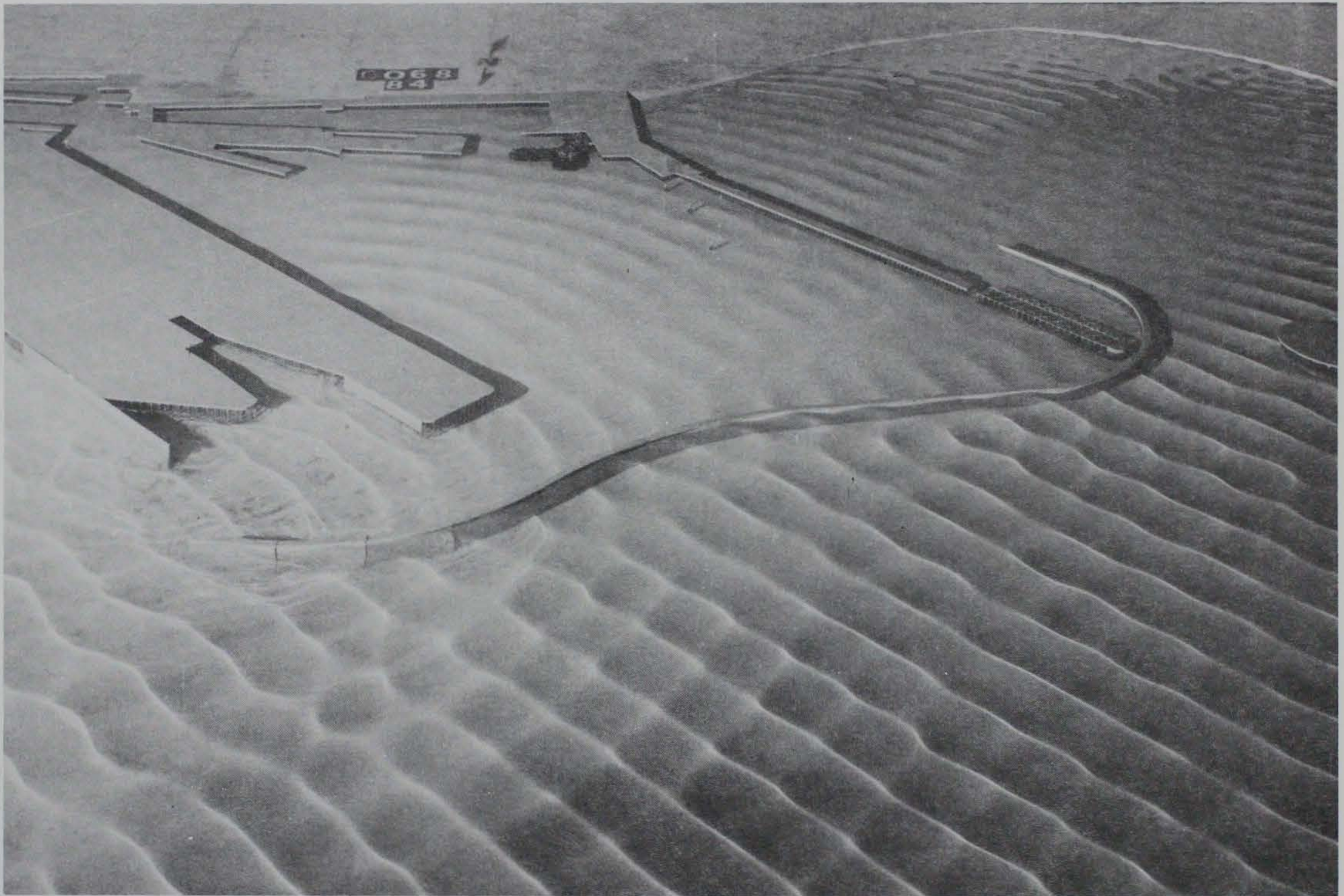
Photo 50. Typical wave patterns for Plan 19; 3.9-sec, 3.3-ft waves from northeast; +5.7 ft swl
