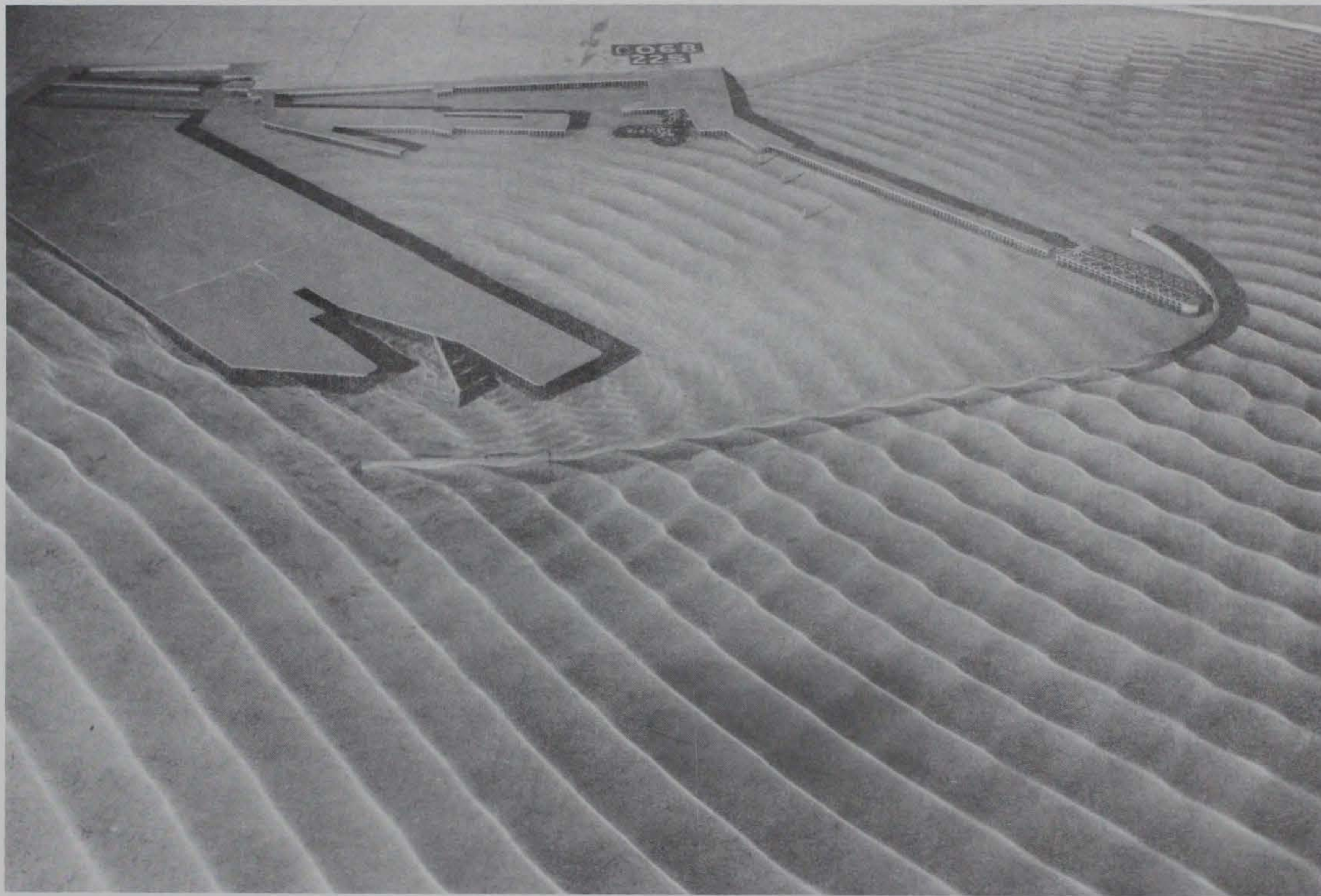
Photo 140. Typical wave patterns for Plan 80; 3.9-sec, 3.3-ft waves from northeast; 0.0-ft swl
