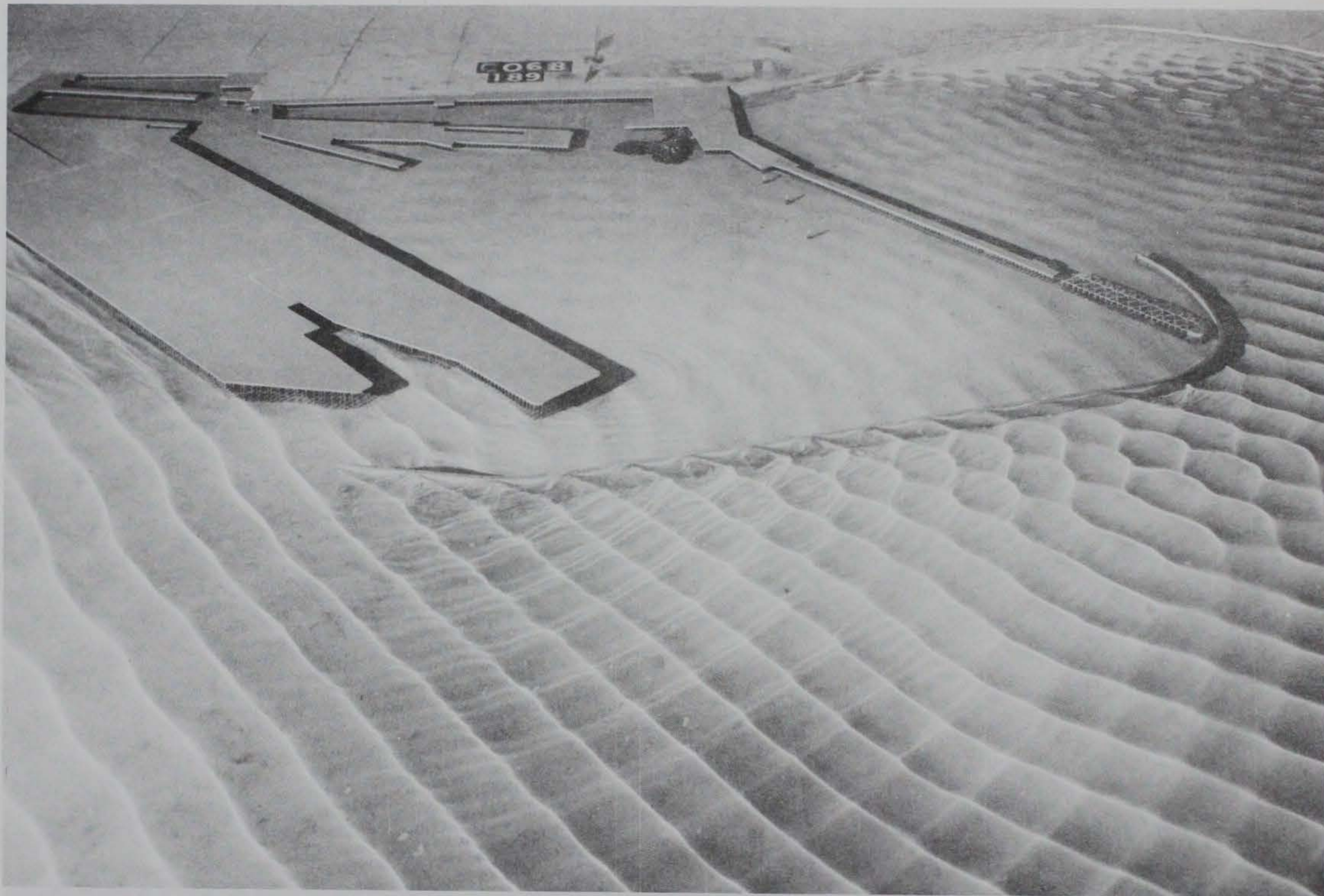
Photo 106. Typical wave patterns for Plan 45; 3.9-sec, 3.3-ft waves from northeast; +5.7 ft swl
