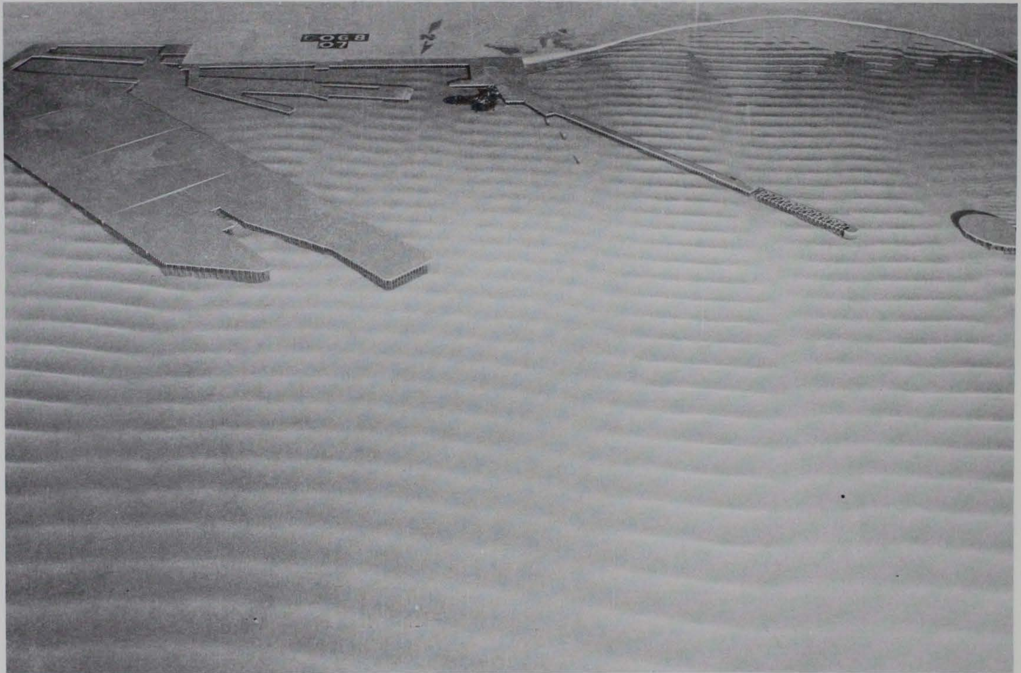
Photo 5. Typical wave patterns for existing conditions; 3.6-sec, 2-ft waves from north; +5.7 ft swl
