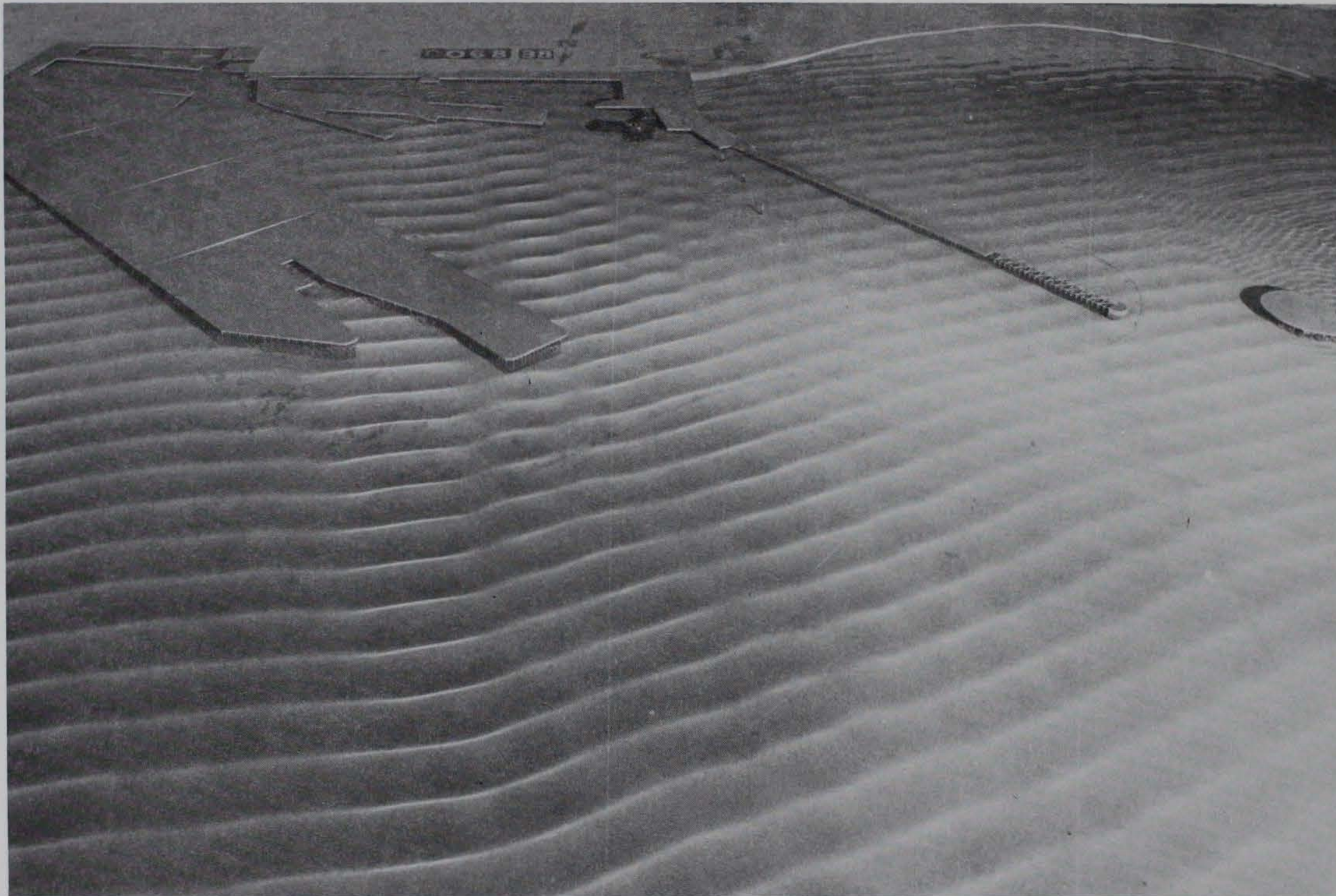
Photo 7. Typical wave patterns for existing conditions; 3.6-sec, 2-ft waves from north-northwest; +5.7 ft swl
