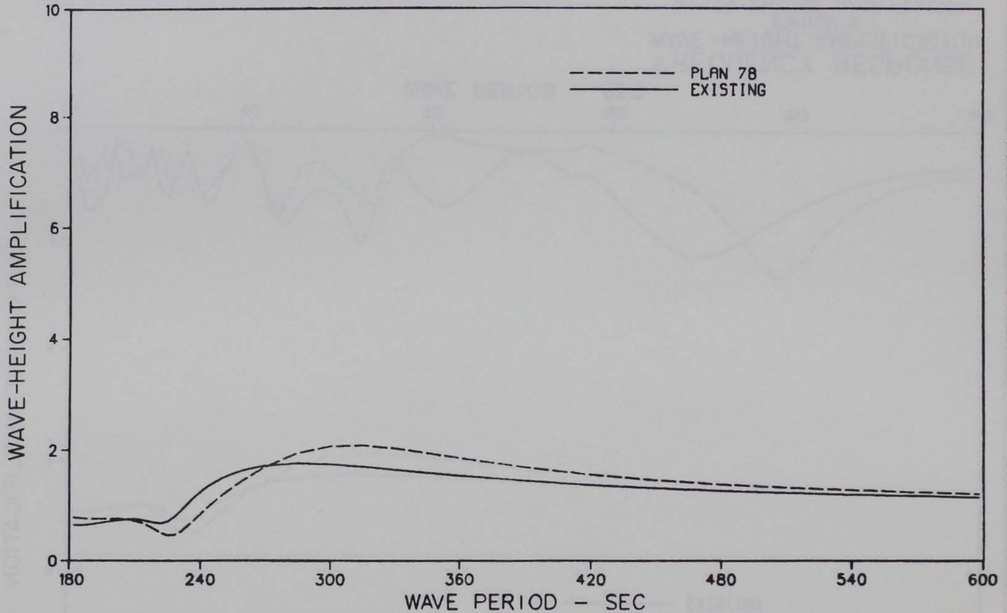
FREQUENCY RESPONSE WAVE-HEIGHT AMPLIFICATION STATION 9 180- TO 600-SEC WAVE PERIODS
