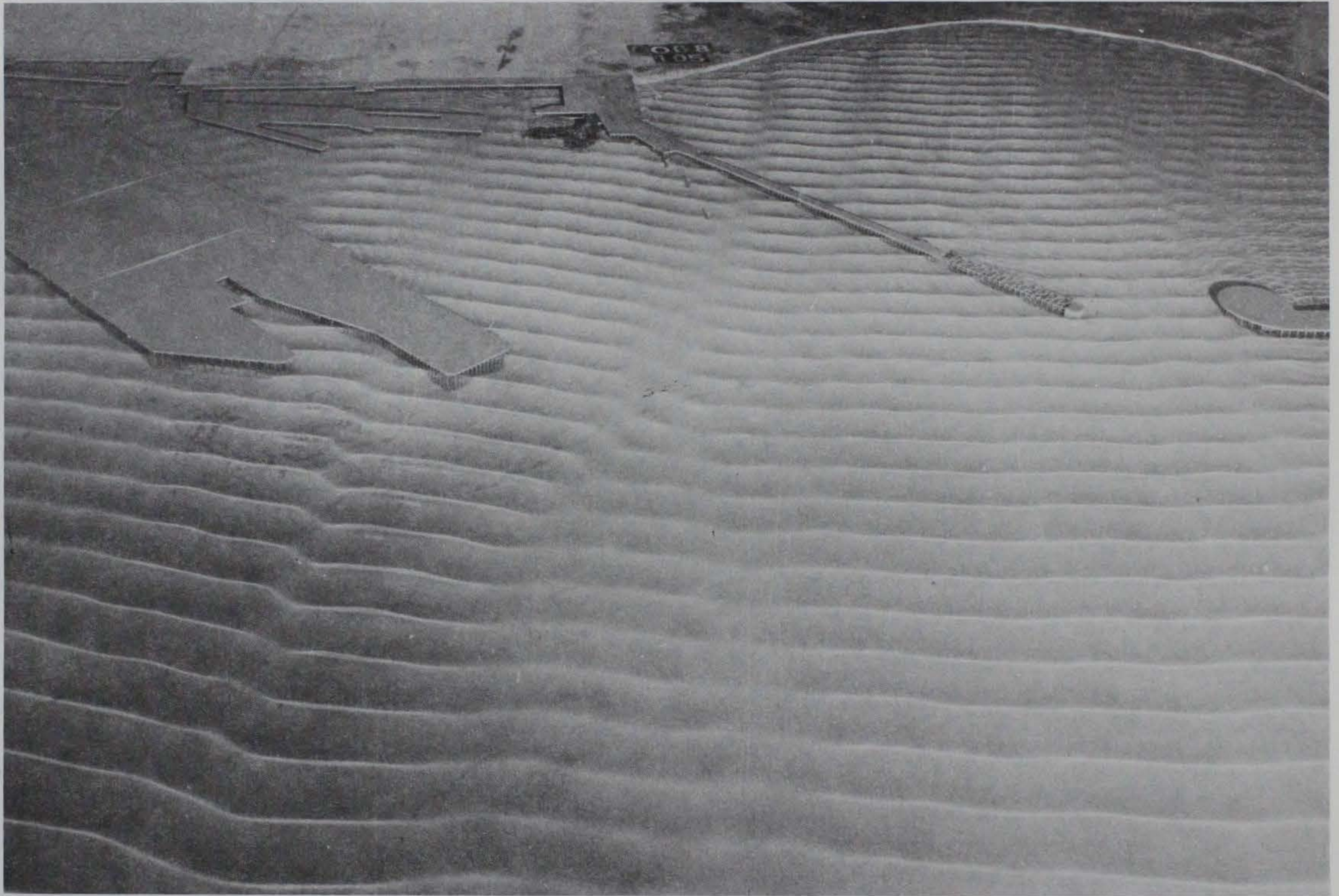
Photo 6. Typical wave patterns for existing conditions; 3.6-sec, 3.1-ft waves from north; +5.7 ft swl
