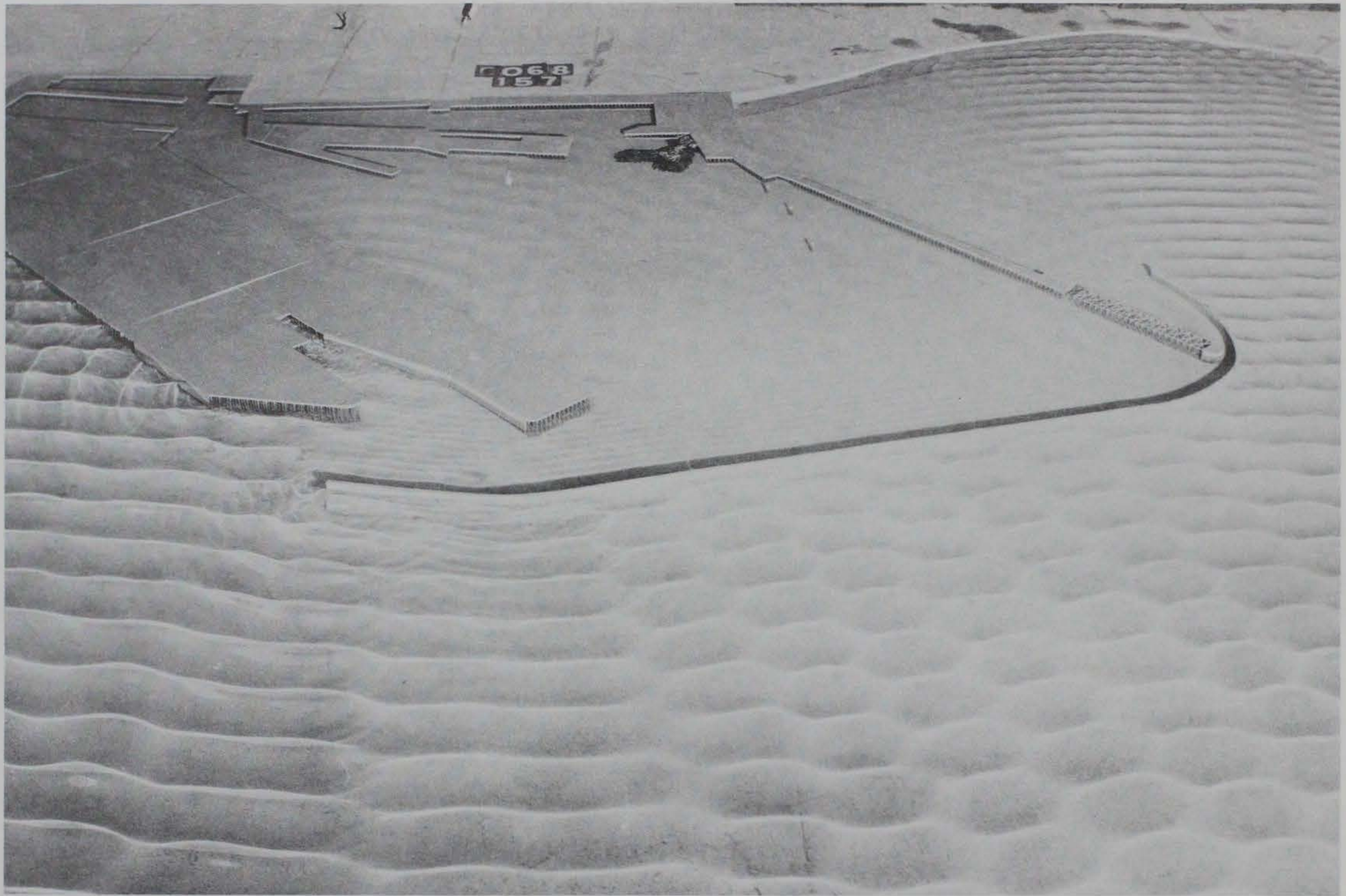
Photo 76. Typical wave patterns for Plan 38; 3.6-sec, 3.1-ft waves from north; +5.7 ft swl
