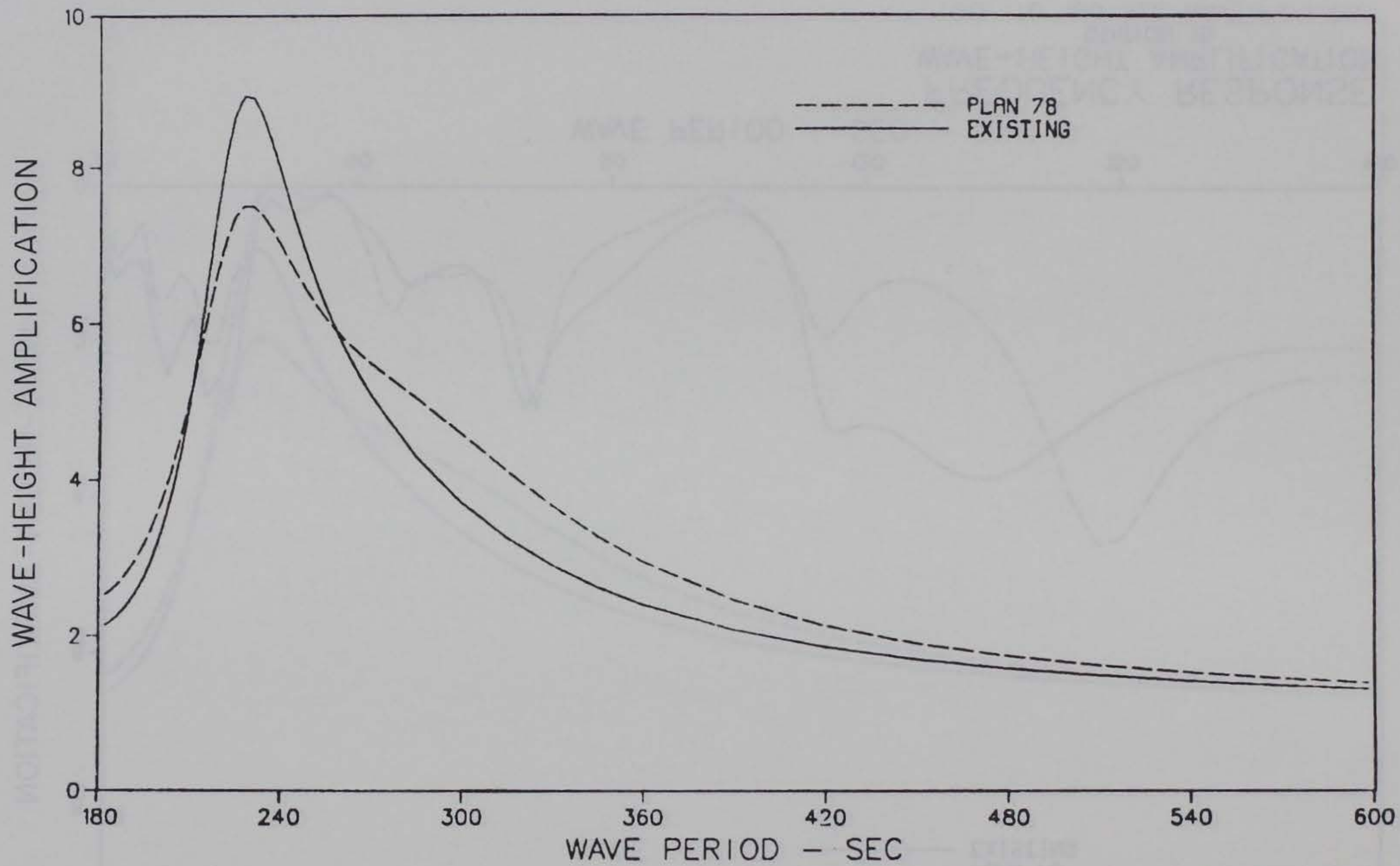
FREQUENCY RESPONSE WAVE-HEIGHT AMPLIFICATION STATION 15 180- TO 600- SEC WAVE PERIODS
