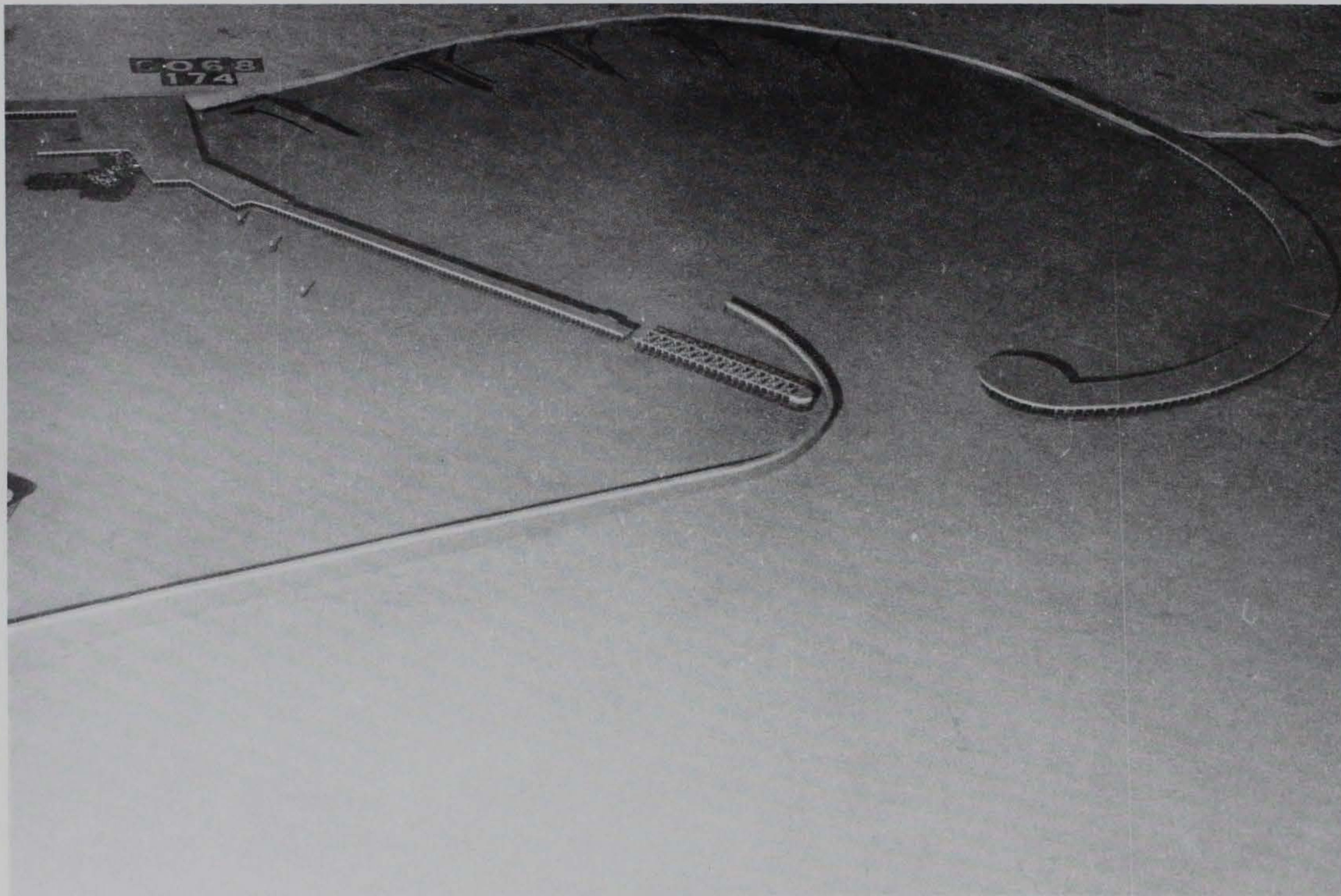
Photo 89. General movement of tracer material for Plan 38; 4.2-sec, 4.8-ft waves from north-northeast; +5.7 ft swl
