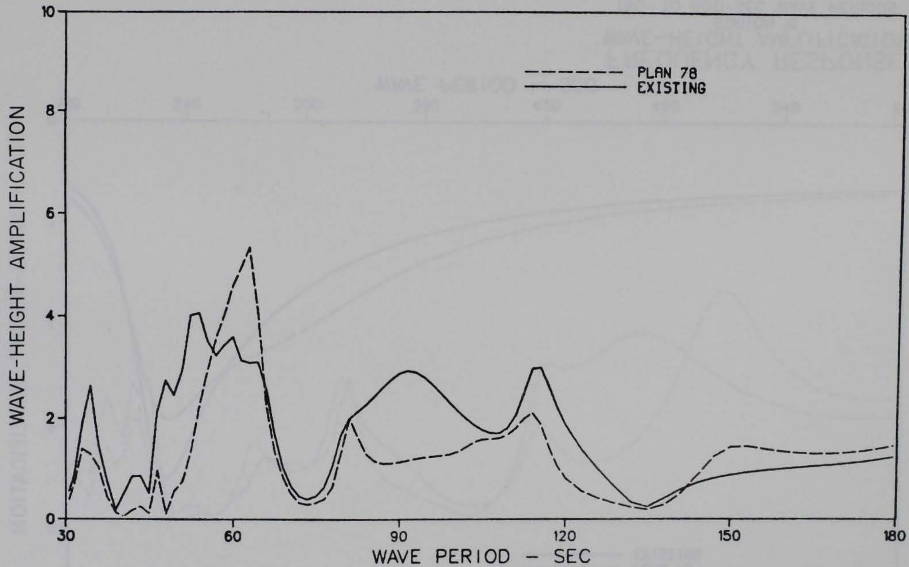
FREQUENCY RESPONSE WAVE-HEIGHT AMPLIFICATION STATION 12 30- TO 180-SEC WAVE PERIODS
