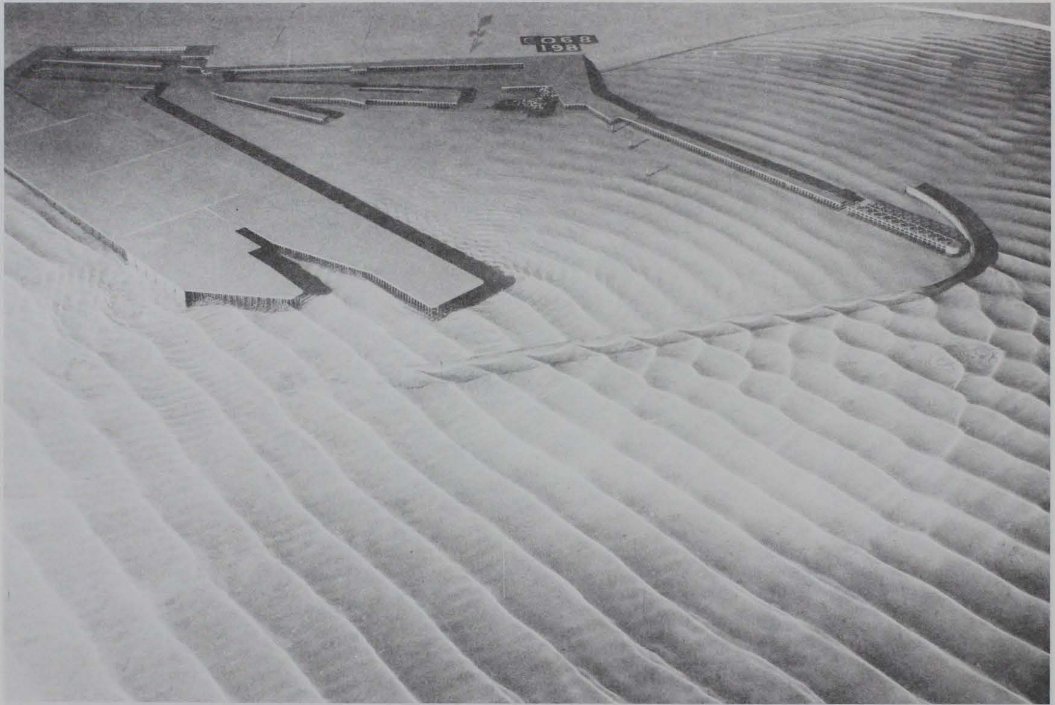
Photo 134. Typical wave patterns for Plan 74; 3.9-sec, 3.3-ft waves from northeast; 0.0-ft swl
