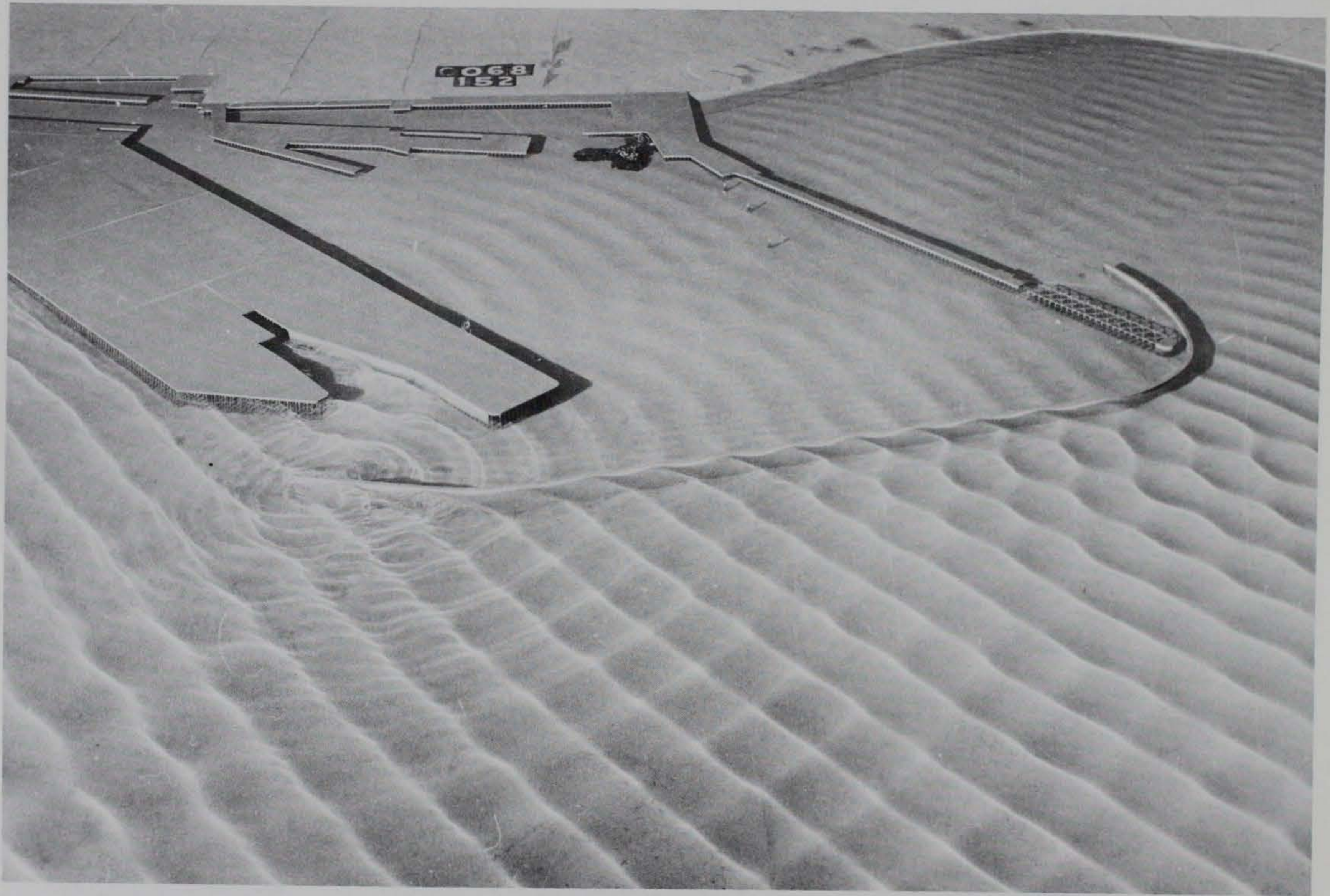
Photo 71. Typical wave patterns for Plan 39; 3.9-sec, 3.3-ft waves from northeast; +5.7 ft swl
