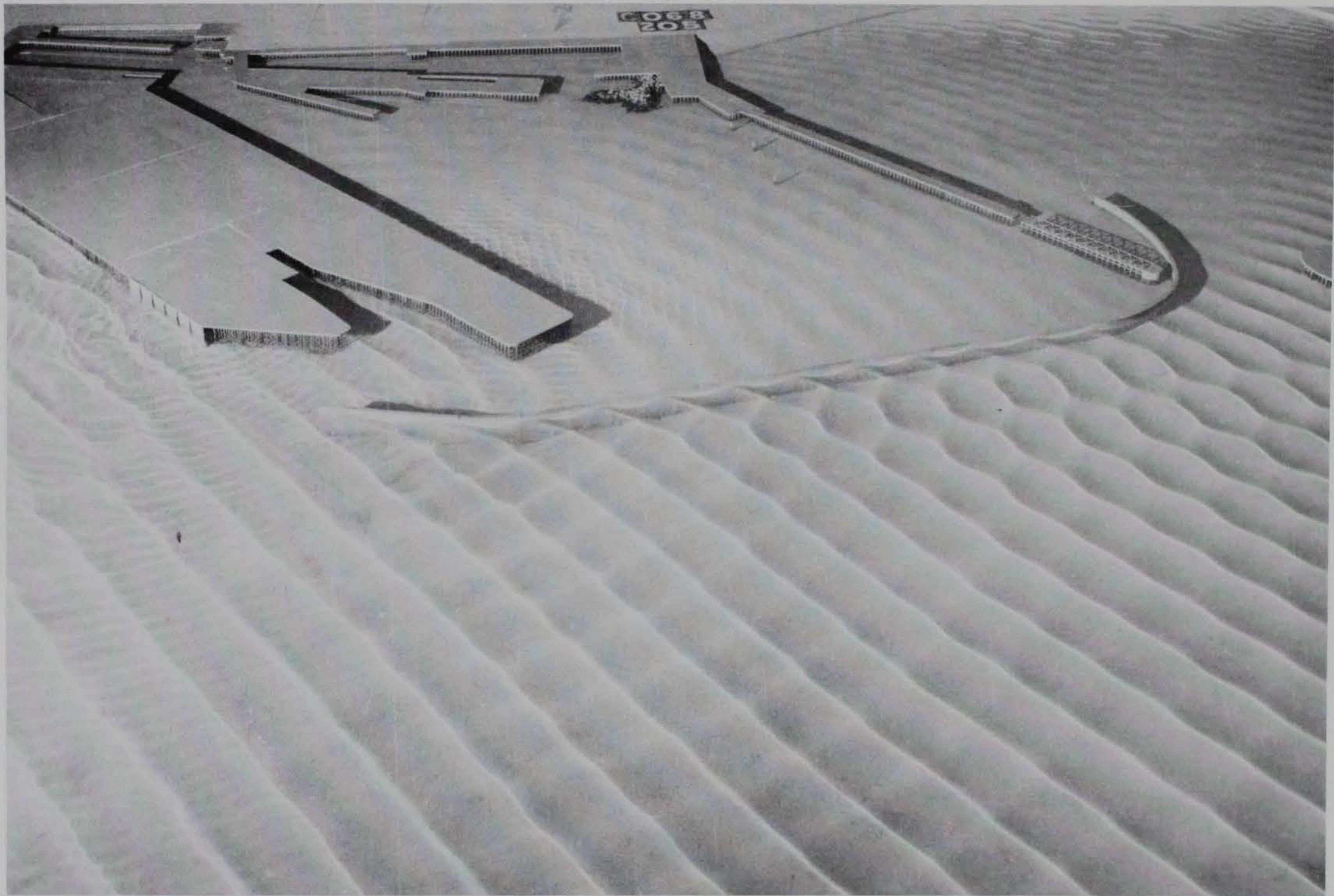
Photo 121. Typical wave patterns for Plan 61; 3.9-sec, 3.3-ft waves from northeast; 0.0-ft swl
