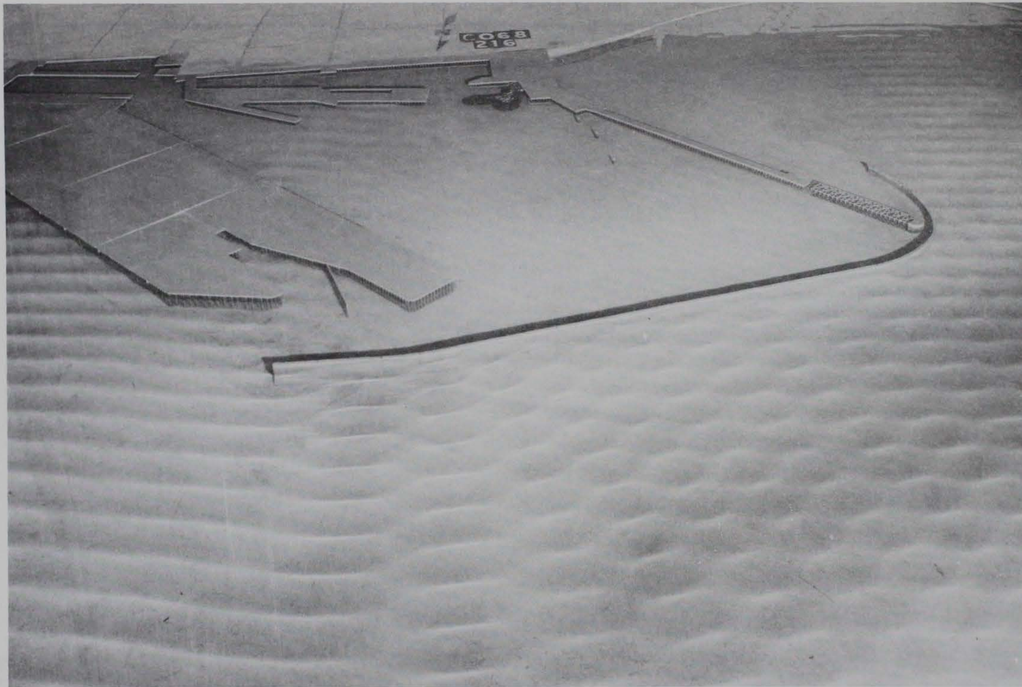
Photo 155. Typical wave patterns for Plan 78; 3.6-sec, 2.0-ft waves from north; +5.7 ft swl
