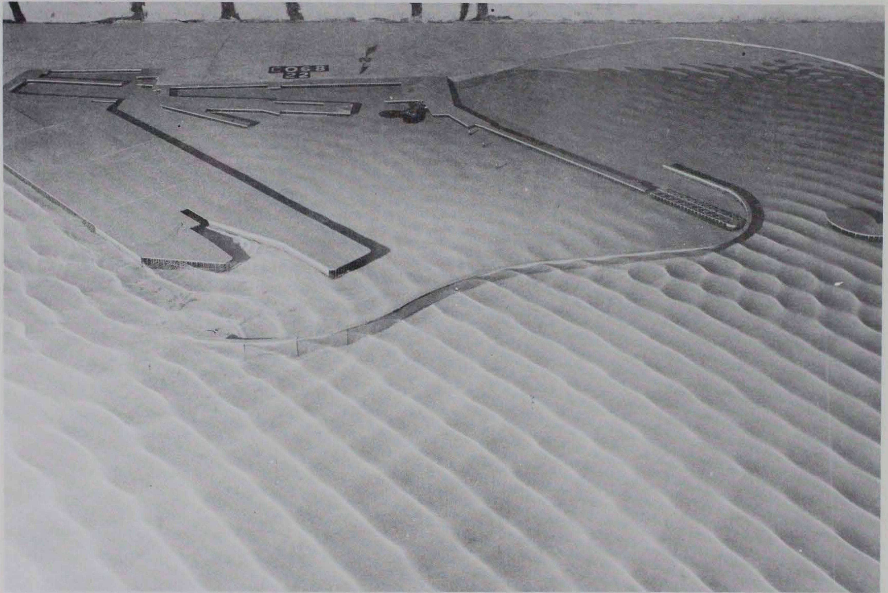
Photo 47. Typical wave patterns for Plan 16; 3.9-sec, 3.3-ft waves from northeast; +5.7 ft swl
