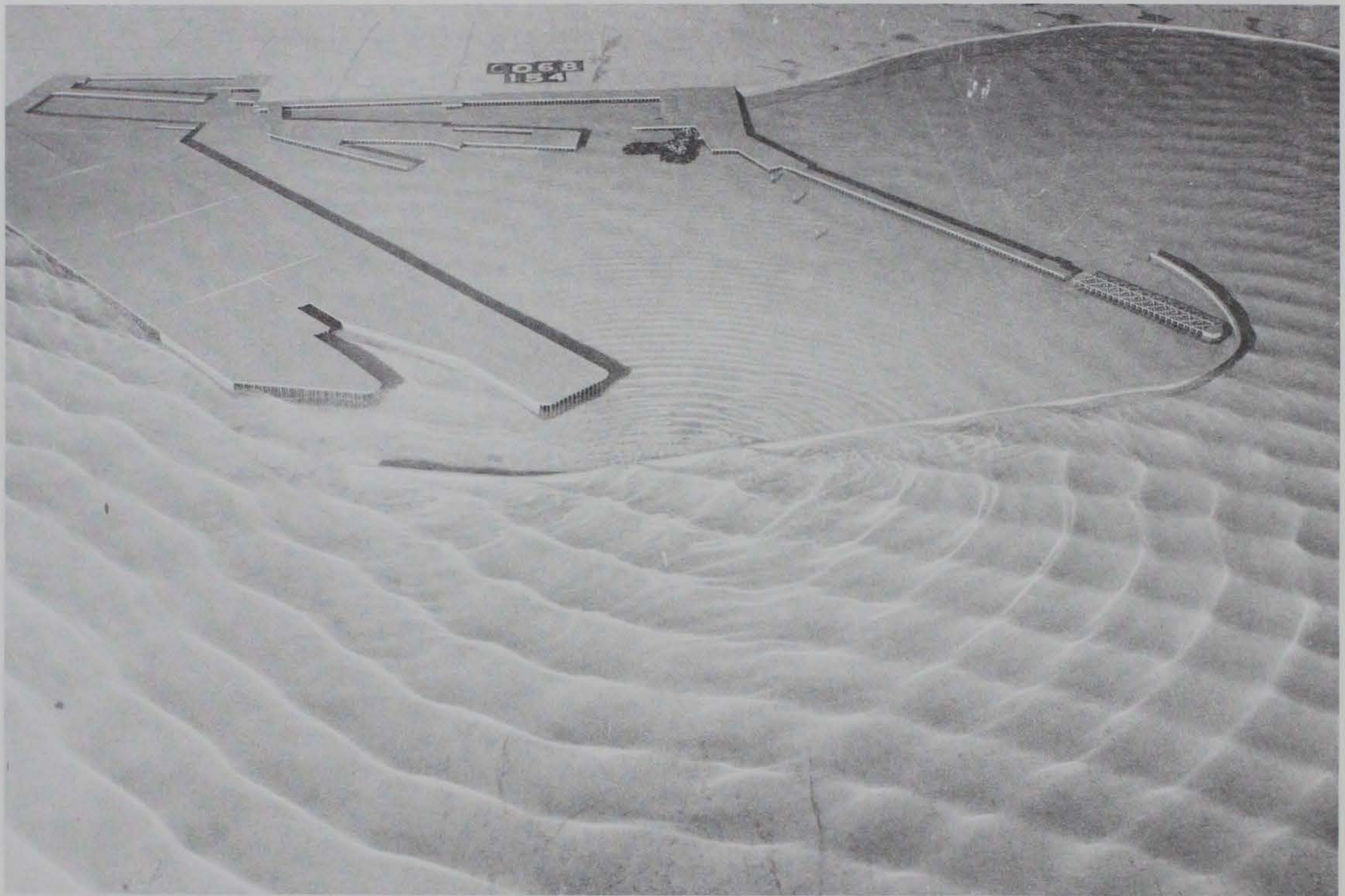
Photo 74. Typical wave patterns for Plan 38; 4.2-sec, 4.8-ft waves from north-northeast; +5.7 ft swl
