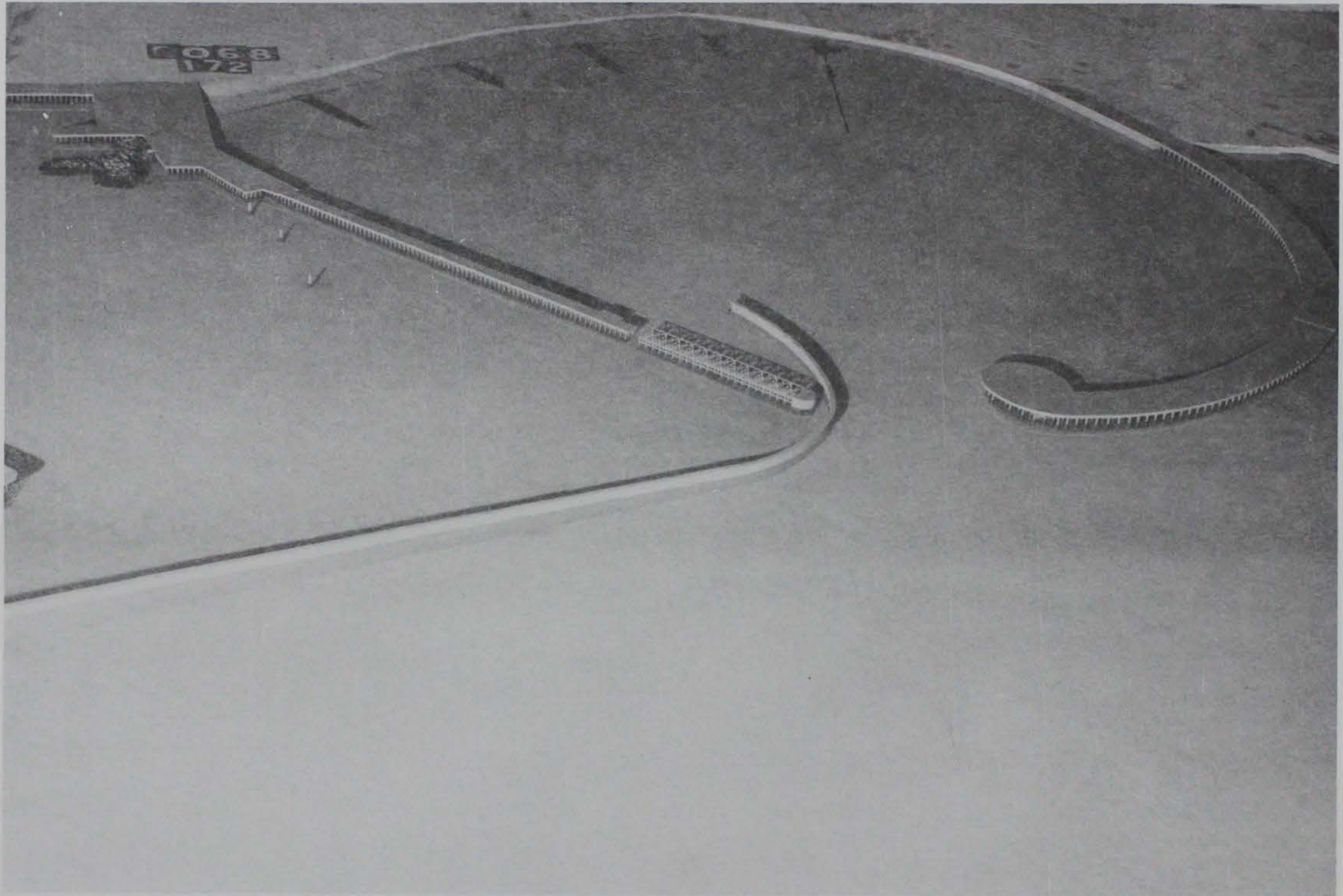
Photo 88. General movement of tracer material for Plan 38; 4.2-sec, 4.8-ft waves from north-northeast; 0.0-ft swl
