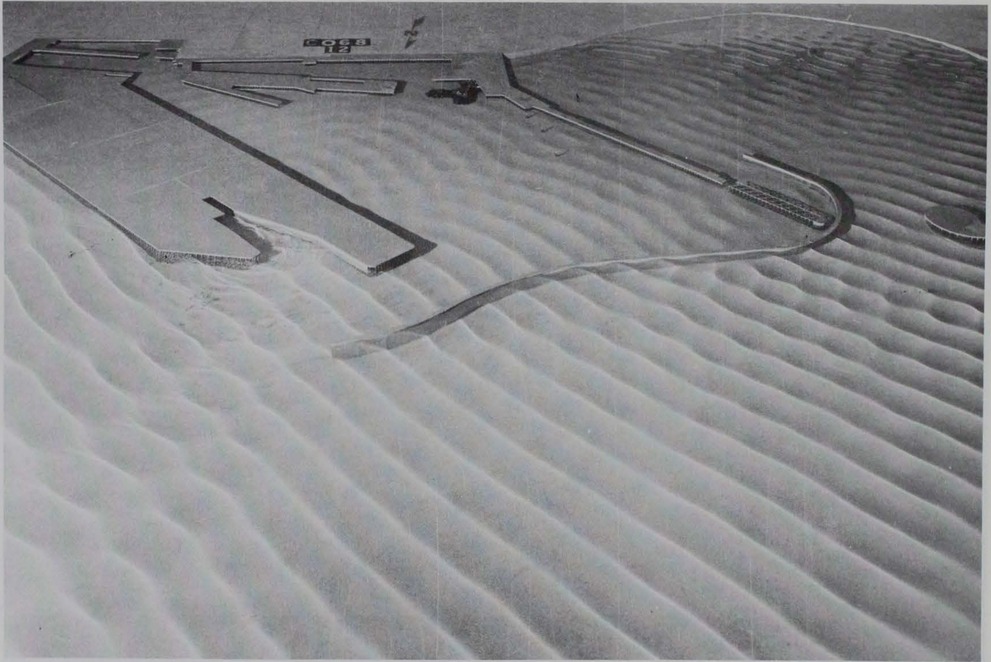
Photo 37. Typical wave patterns for Plan 6; 3.9-sec, 3.3-ft waves from northeast; +5.7 ft swl
