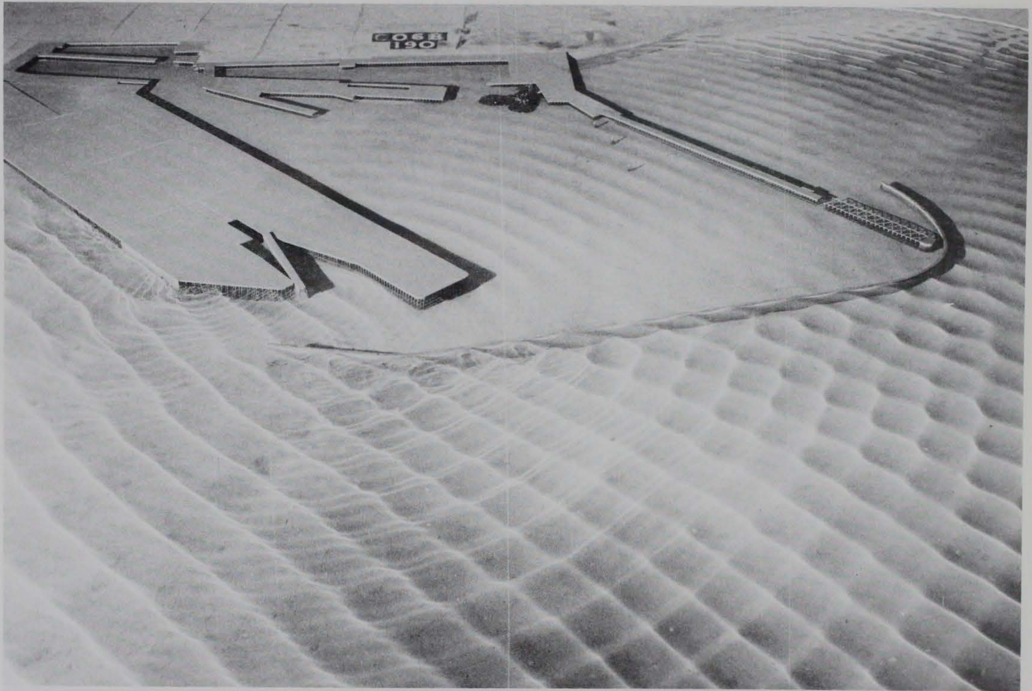
Photo 111. Typical wave patterns for Plan 51; 3.9-sec, 3.3-ft waves from northeast; +5.7 ft swl
