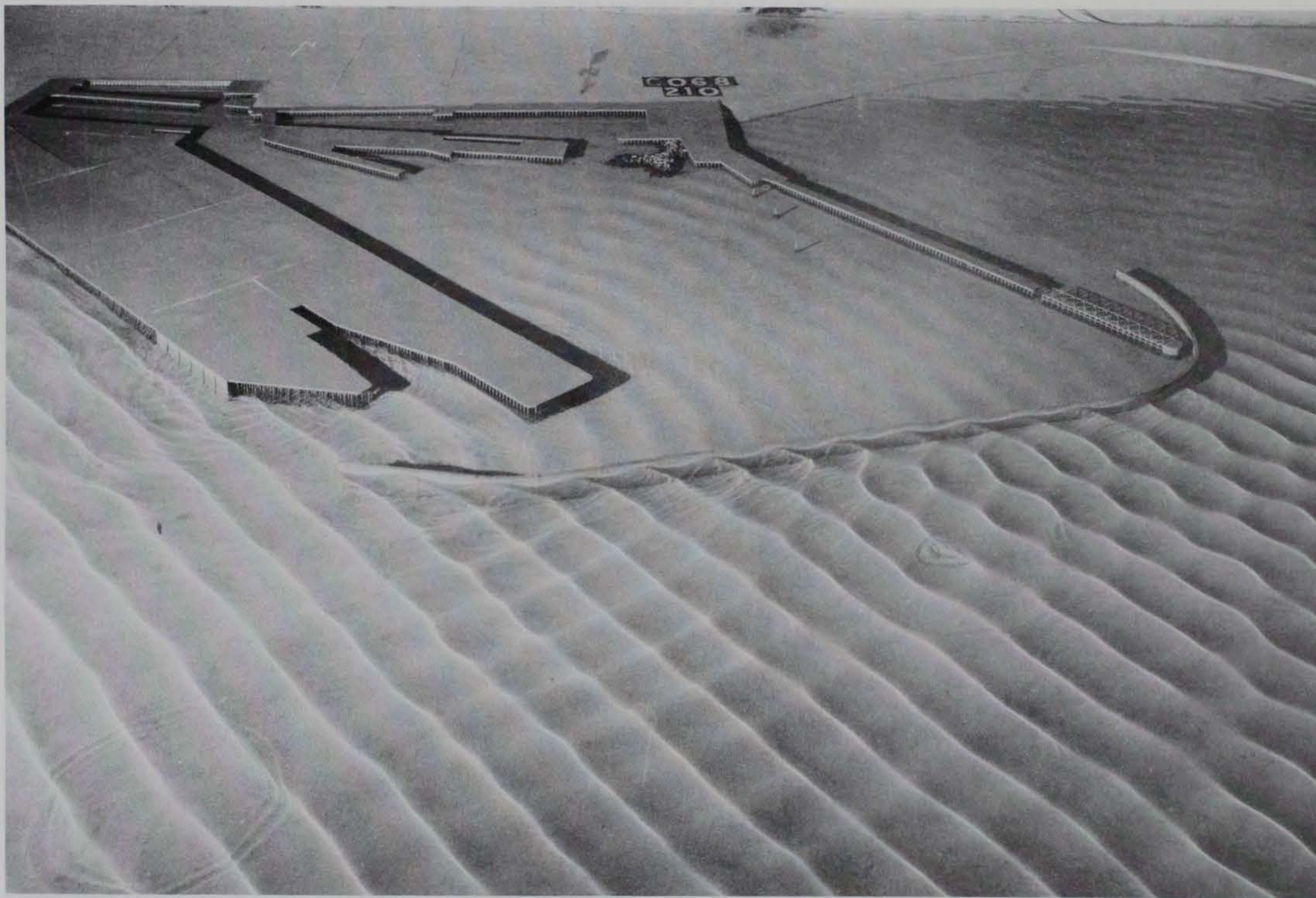
Photo 117. Typical wave patterns for Plan 57; 3.9-sec, 3.3-ft waves from northeast; 0.0-ft swl
