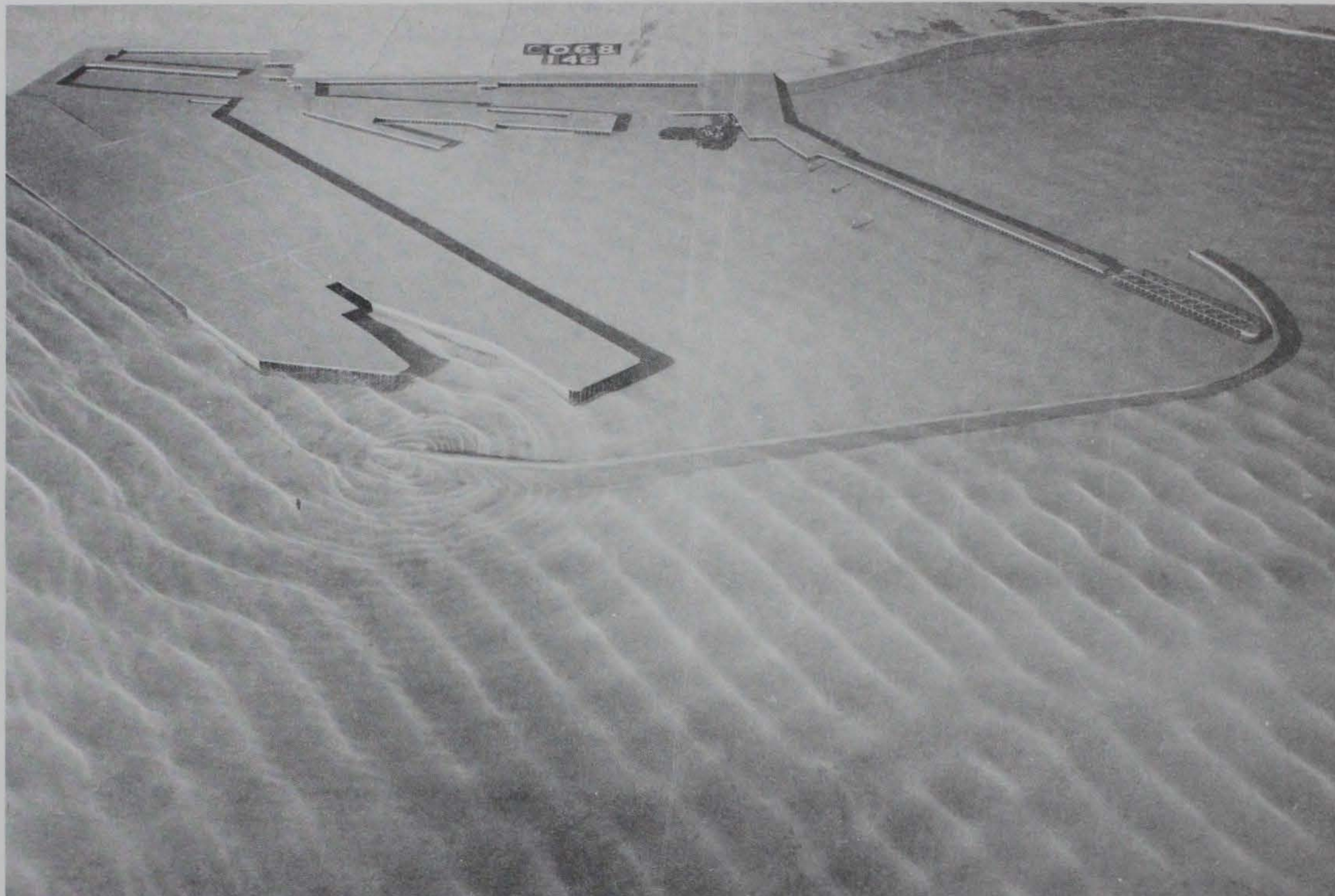
Photo 72. Typical wave patterns for Plan 38; 3.6-sec, 2-ft waves from northeast; +5.7 ft swl
