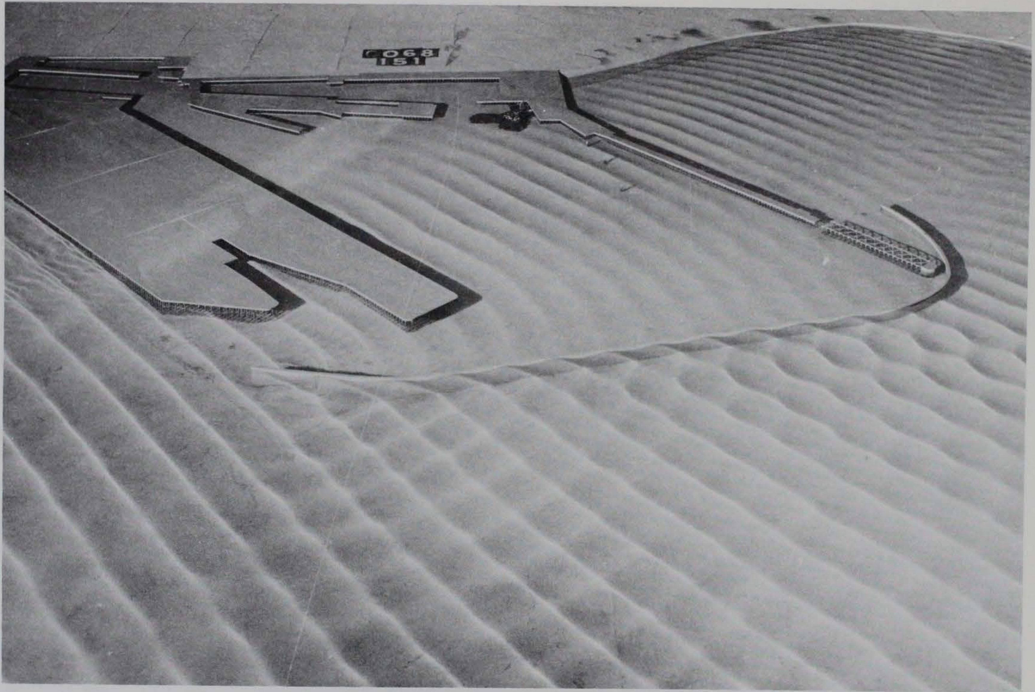
Photo 65. Typical wave patterns for Plan 23; 3.9-sec, 3.3-ft waves from northeast; +5.7 ft swl
