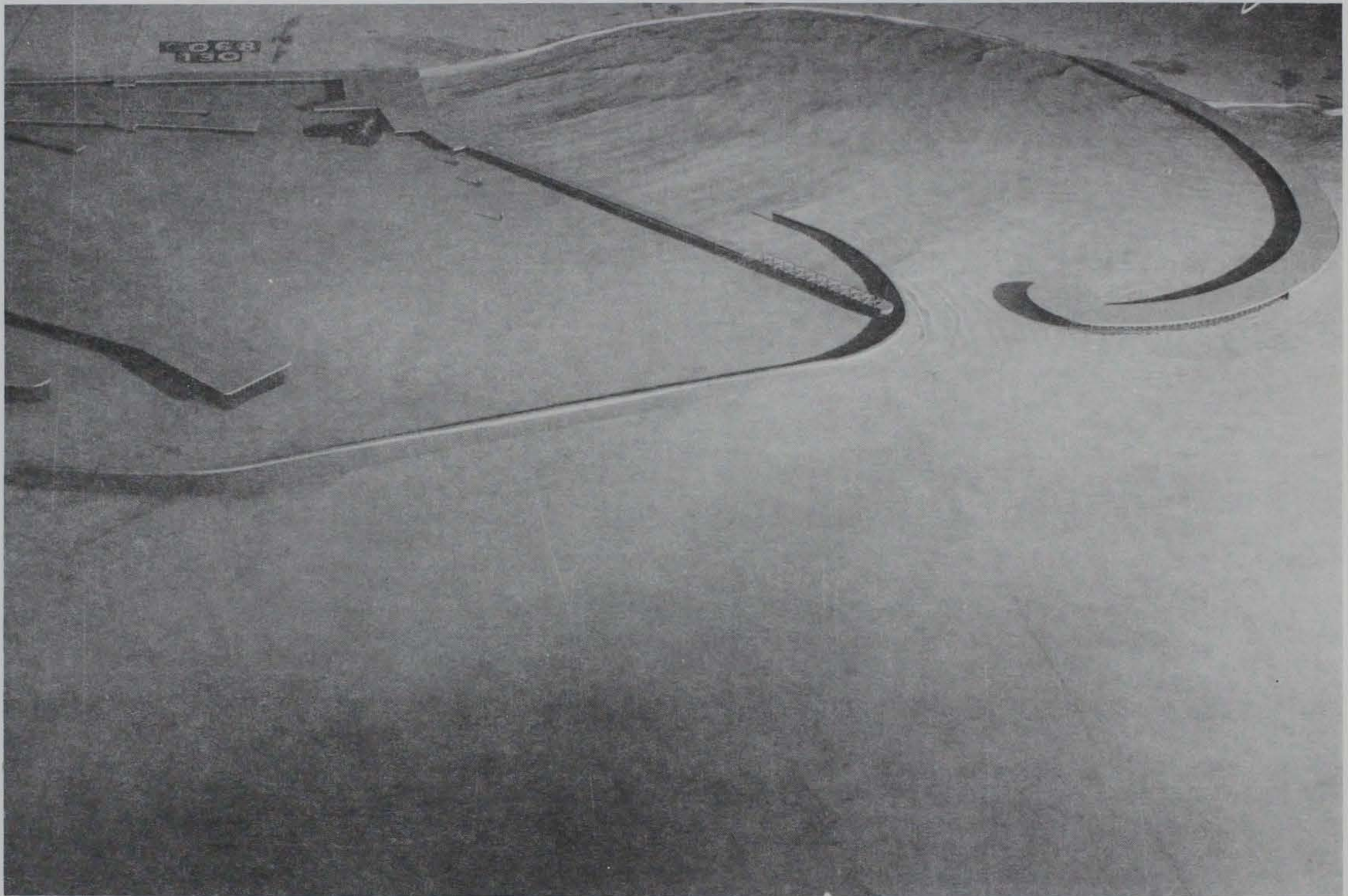
Photo 62. Typical wave patterns for Plan 31; 10-sec, 3-ft waves from west-northwest; +5.7 ft swl
