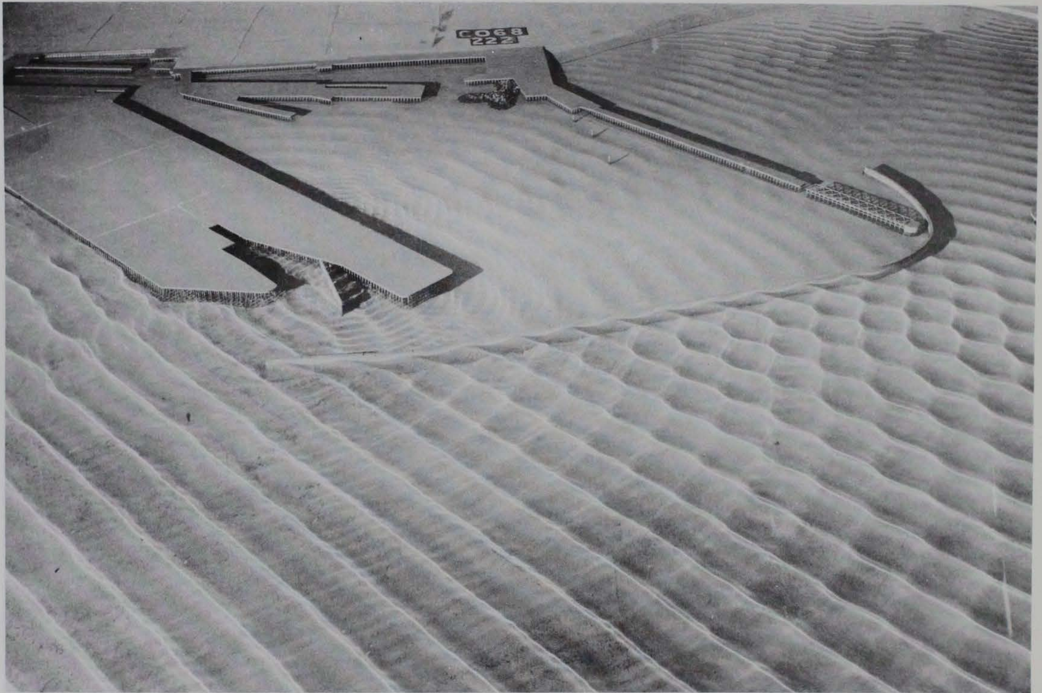
Photo 137. Typical wave patterns for Plan 77; 3.9-sec, 3.3-ft waves from northeast; 0.0-ft swl
