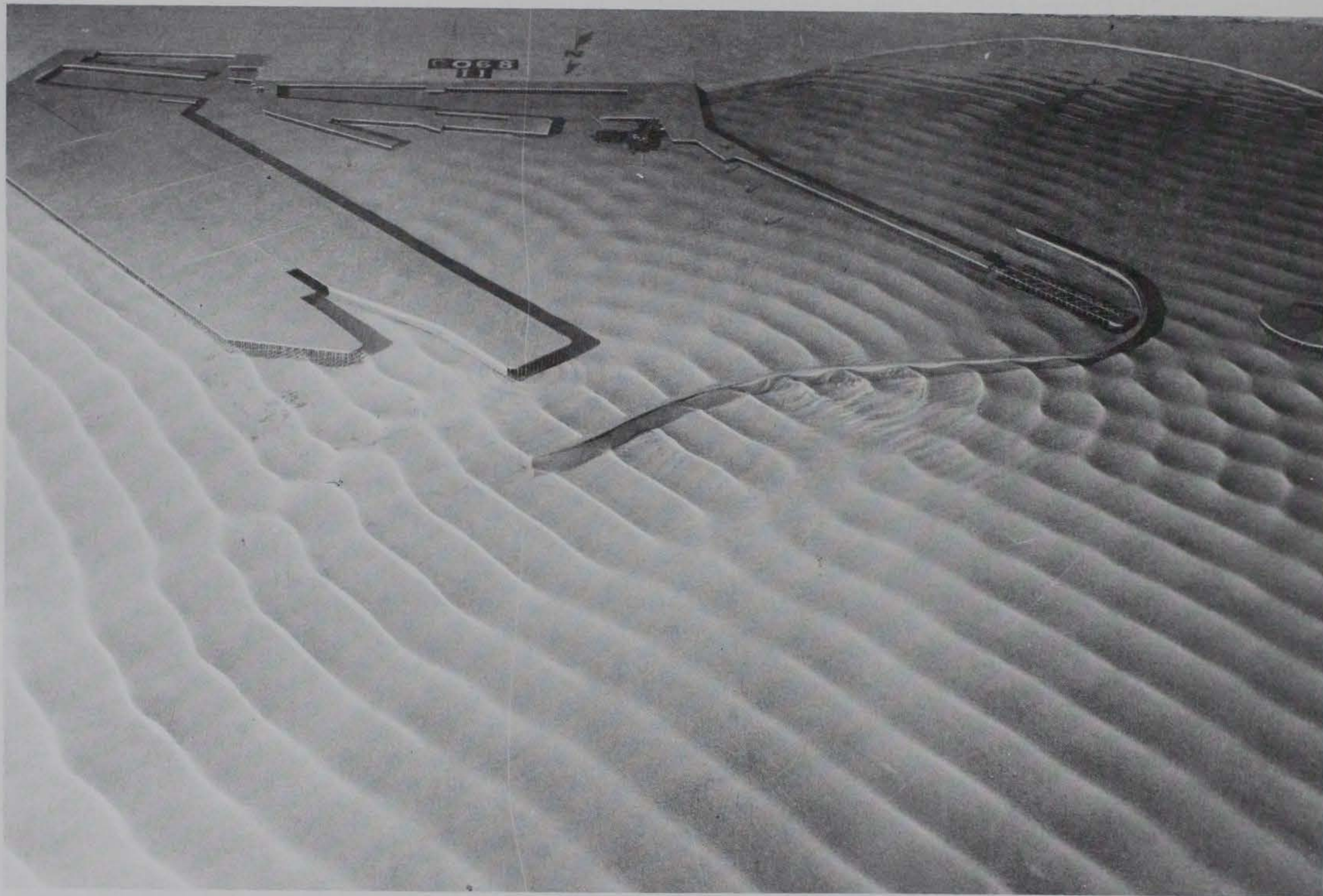
Photo 31. Typical wave patterns for Plan 1; 3.9-sec, 3.3-ft waves from northeast; +5.7 ft swl
