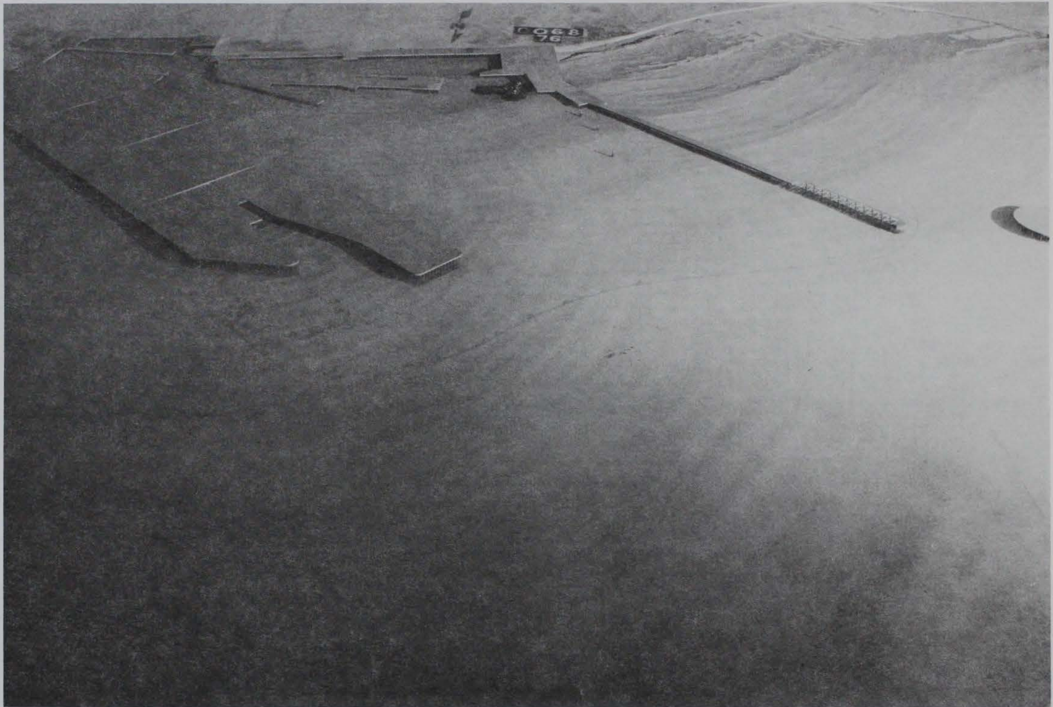
Photo 14. Typical wave patterns for existing conditions; 10-sec, 3-ft waves from west-northwest; +5.7 ft swl
