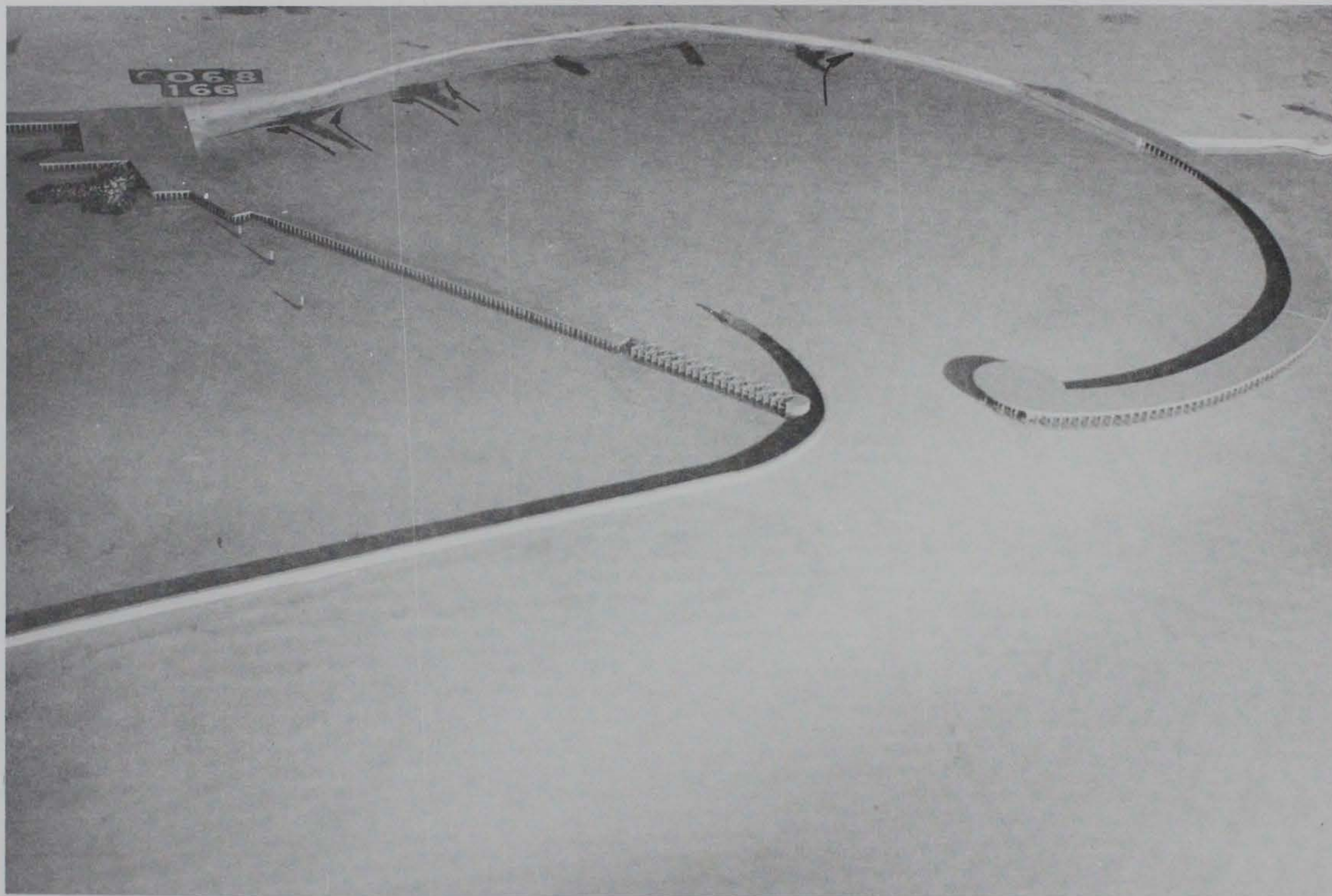
Photo 92. General movement of tracer material for Plan 38; 3.6-sec, 3.3-ft waves from north-northwest; 0.0-ft swl
