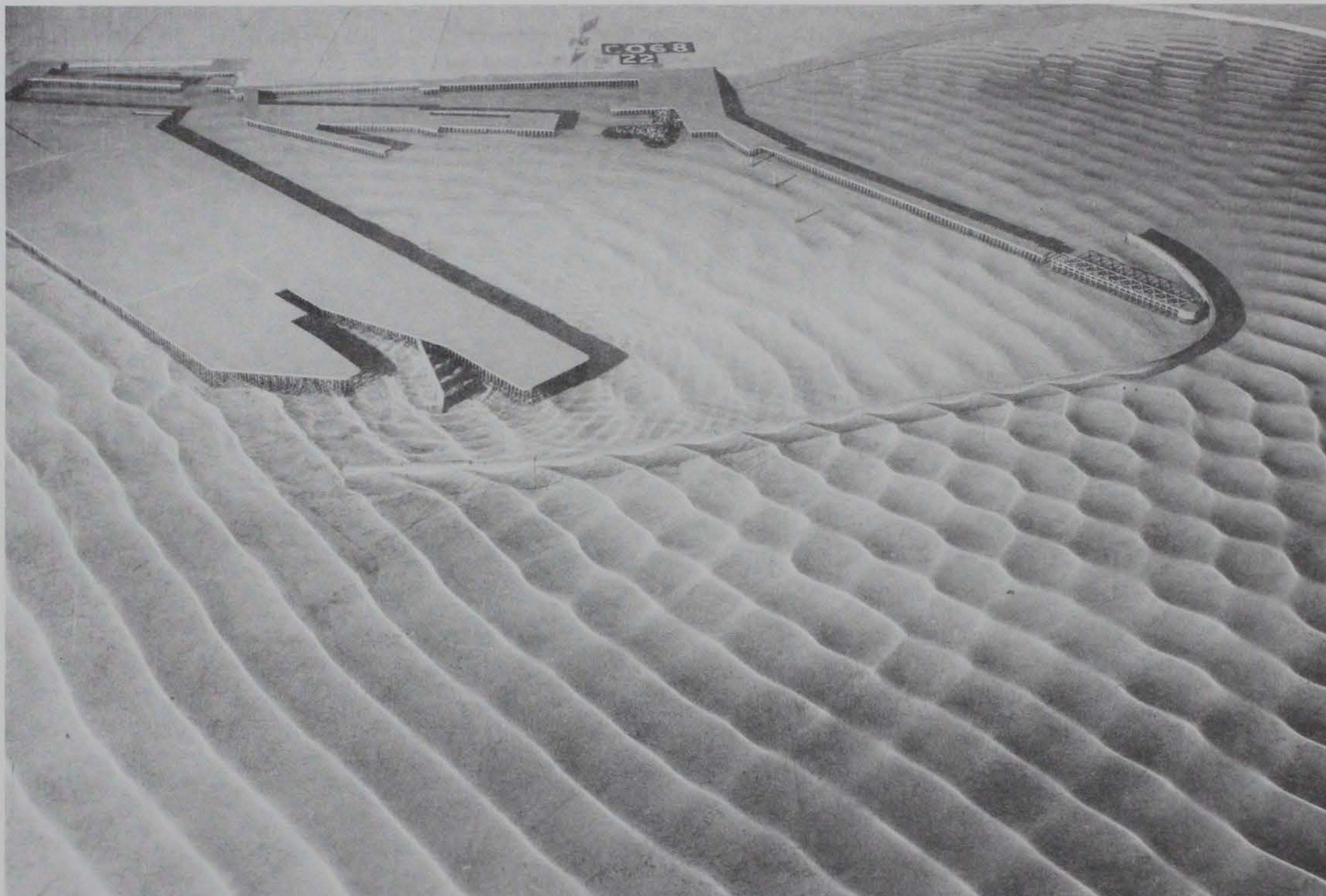
Photo 136. Typical wave patterns for Plan 76; 3.9-sec, 3.3-ft waves from northeast; 0.0-ft swl
