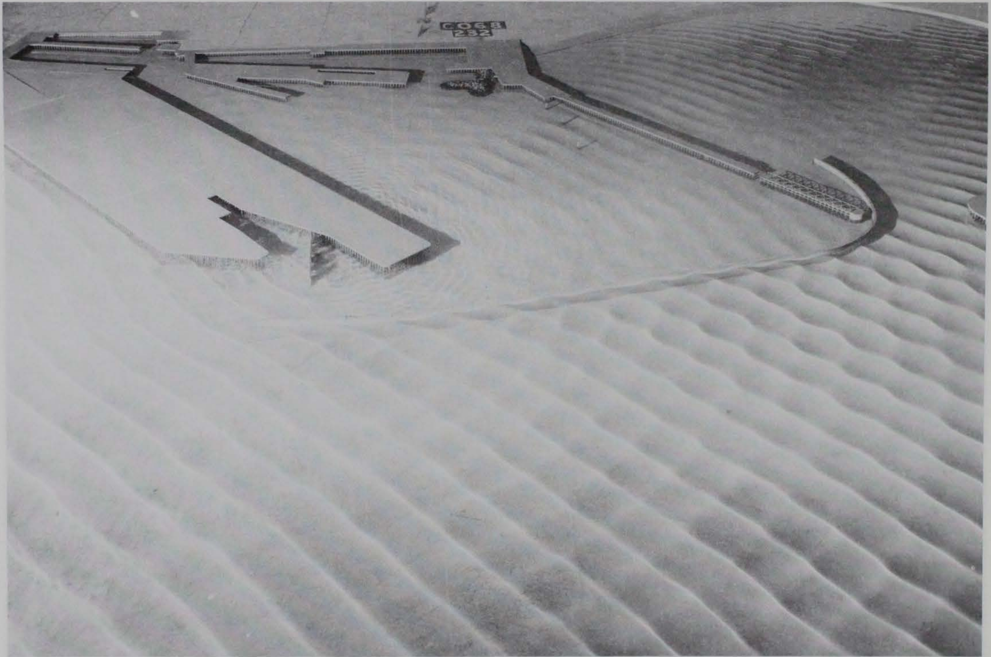
Photo 149. Typical wave patterns for Plan 89; 3.9-sec, 3.3-ft waves from northeast; 0.0-ft swl
