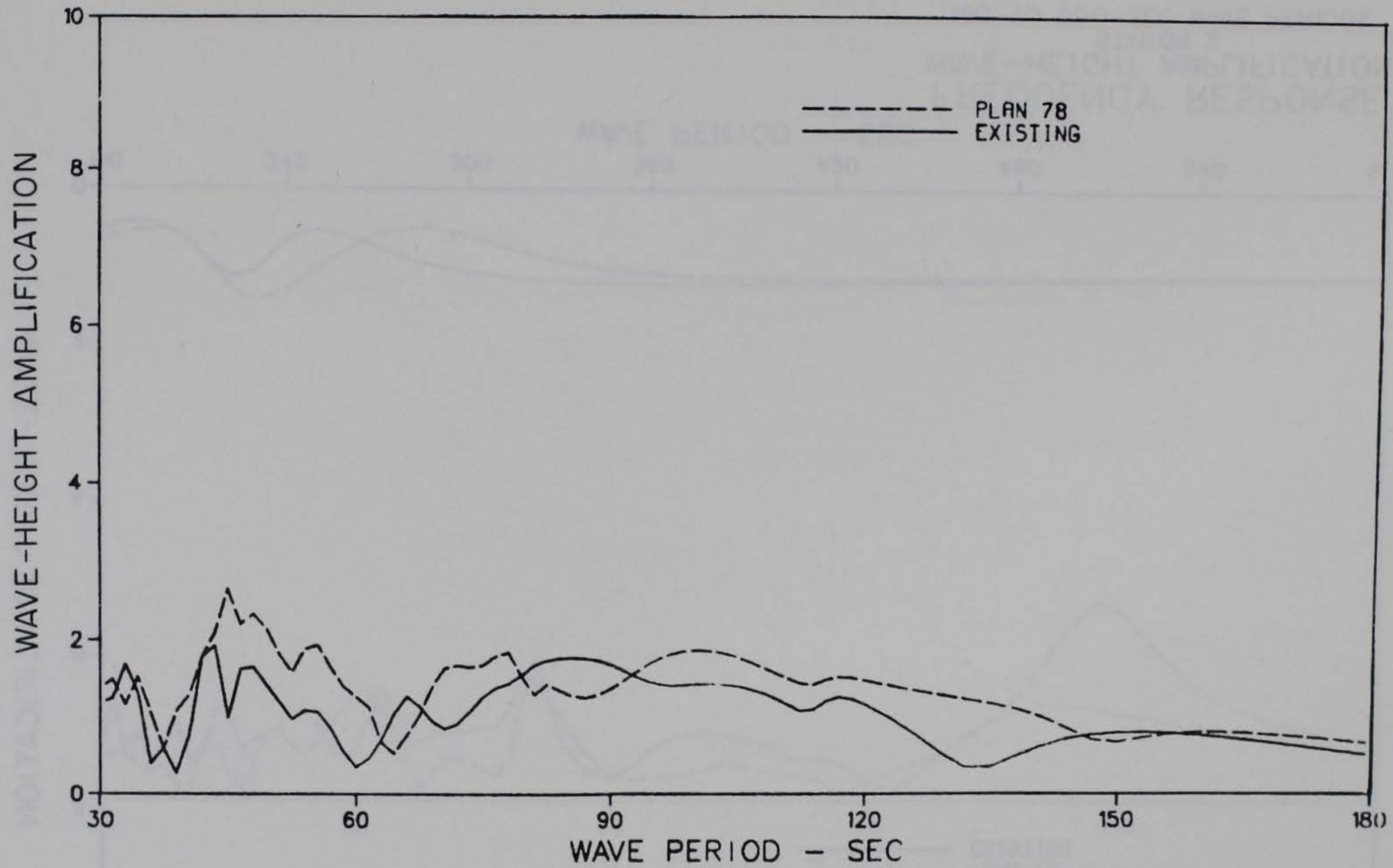
FREQUENCY RESPONSE WAVE-HEIGHT AMPLIFICATION STATION 2 30- TO 180-SEC WAVE PERIODS
