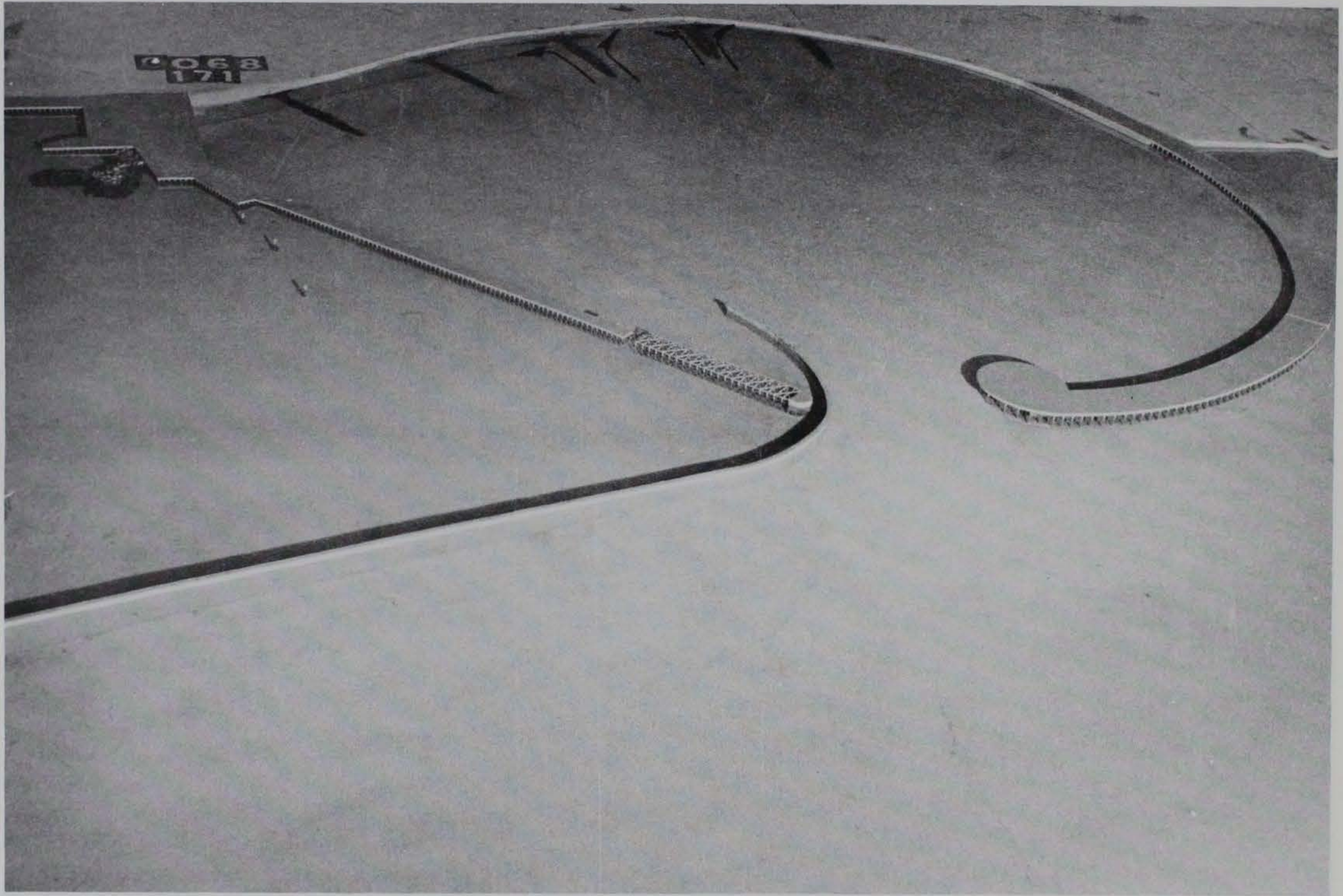
Photo 91. General movement of tracer material for Plan 38; 3.6-sec, 3.1-ft waves from north; +5.7 ft swl
