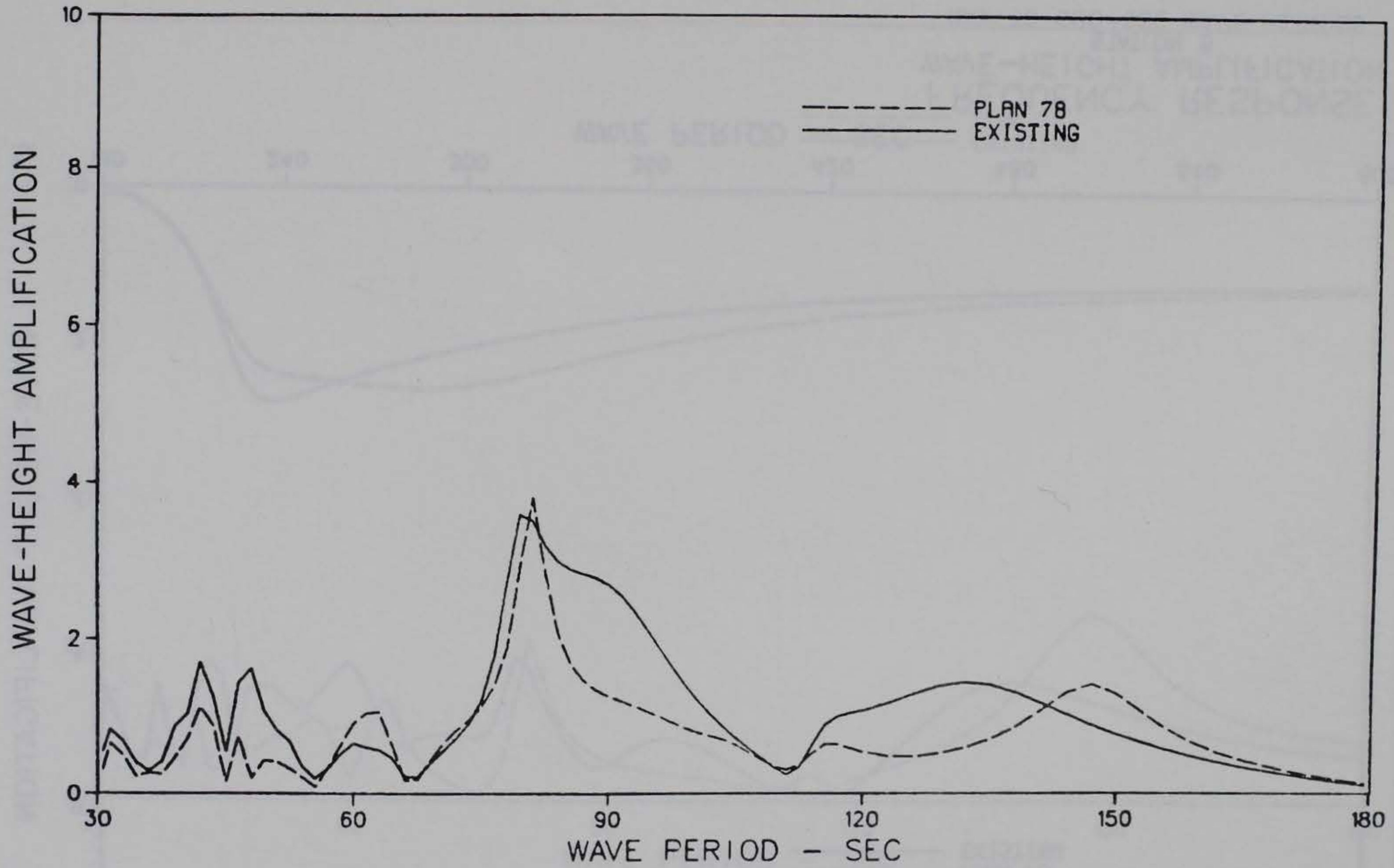
FREQUENCY RESPONSE WAVE-HEIGHT AMPLIFICATION STATION 5 30- TO 180-SEC WAVE PERIODS
