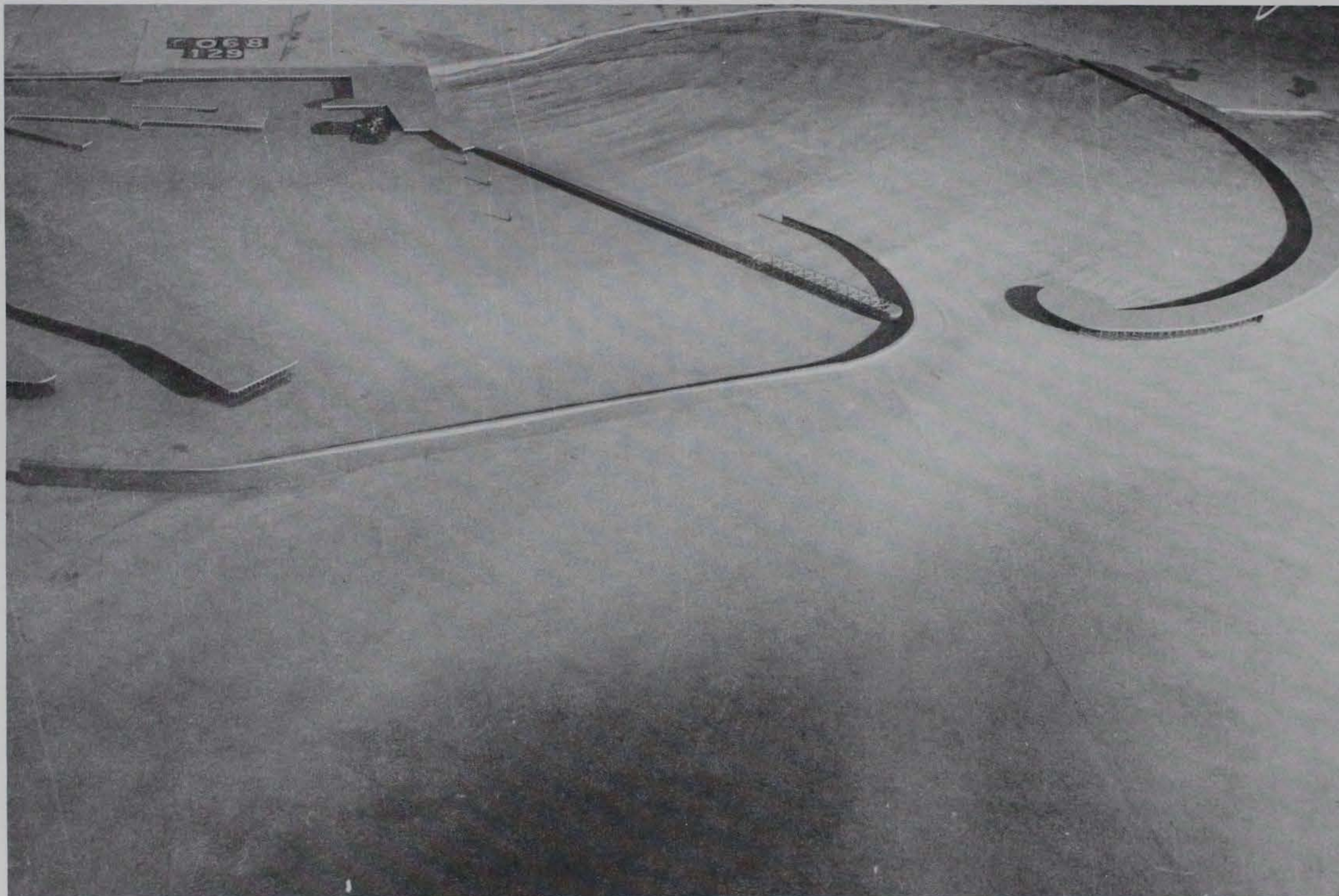
Photo 63. Typical wave patterns for Plan 32; 10-sec, 3-ft waves from west-northwest; +5.7 ft swl
