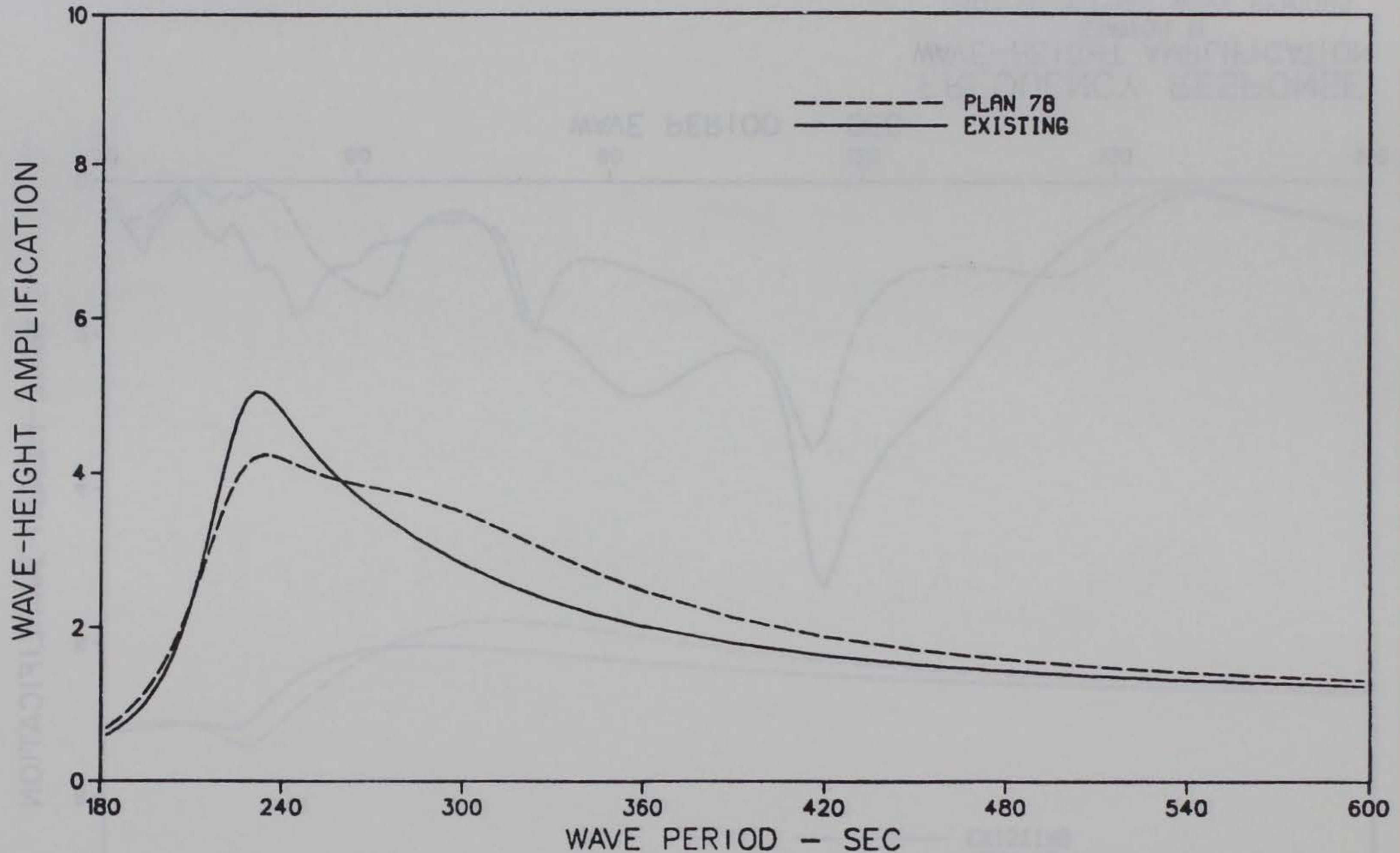
FREQUENCY RESPONSE WAVE-HEIGHT AMPLIFICATION STATION 11 180- TO 600-SEC WAVE PERIODS
