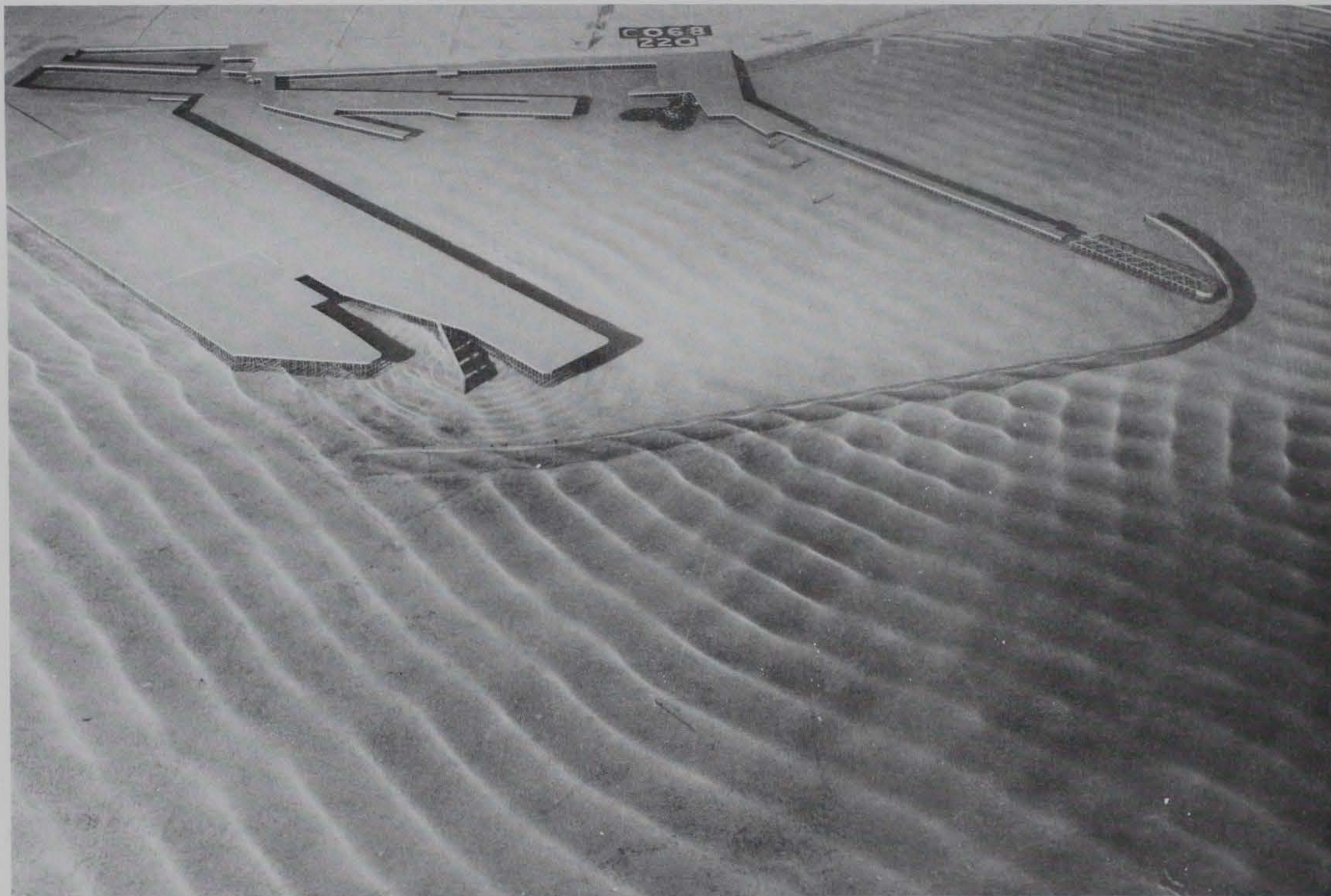
Photo 151. Typical wave patterns for Plan 78; 3.6-sec, 2.0-ft waves from northeast; +5.7 ft swl
