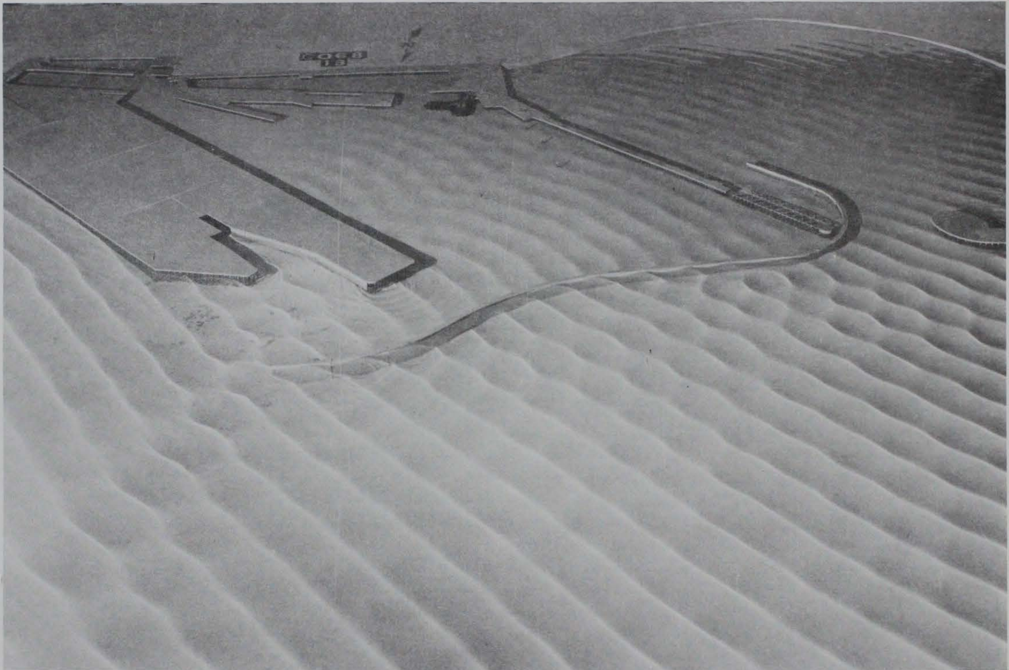
Photo 38. Typical wave patterns for Plan 7; 3.9-sec, 3.3-ft waves from northeast; +5.7 ft swl
