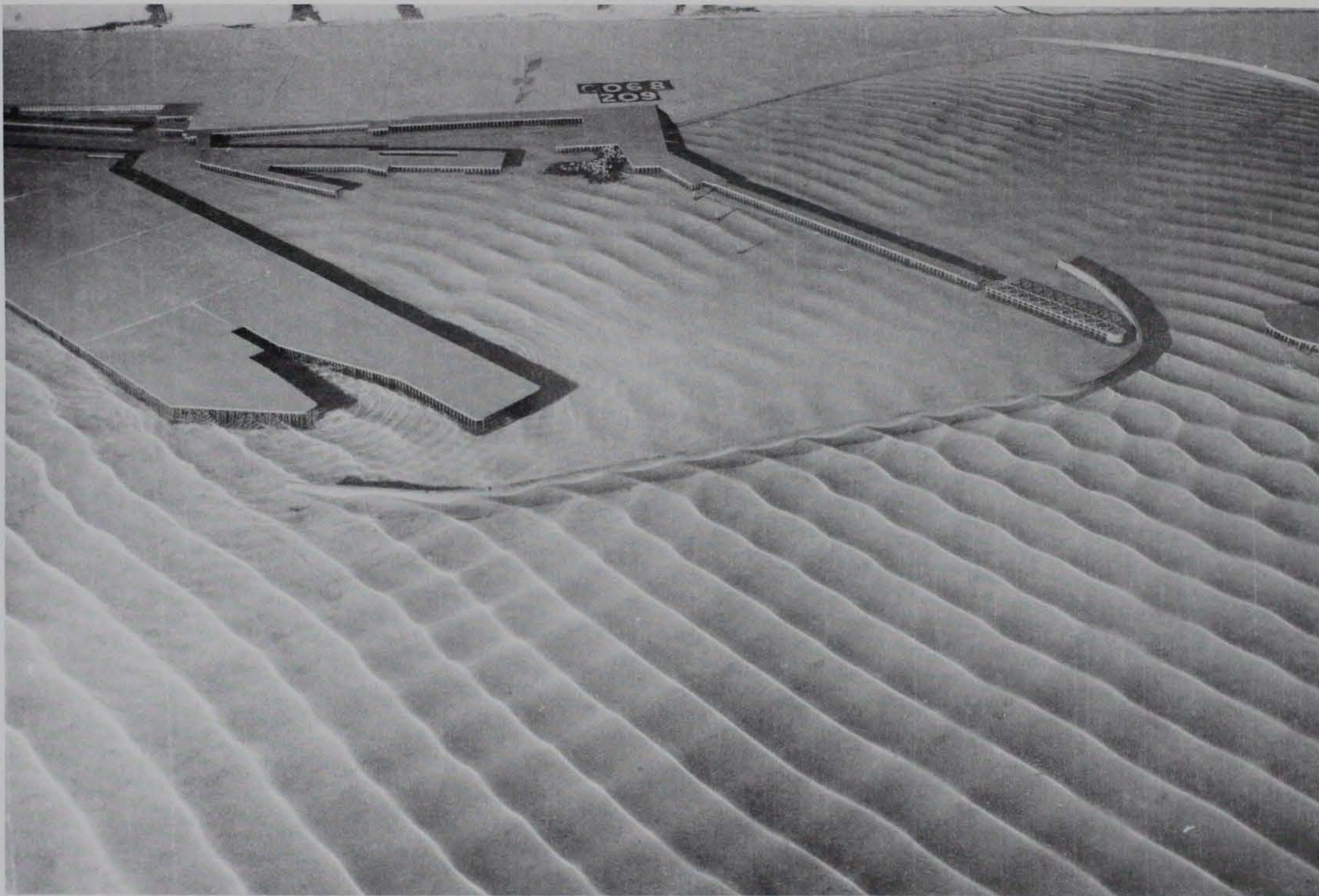
Photo 113. Typical wave patterns for Plan 53; 3.9-sec, 3.3-ft waves from northeast; 0.0-ft swl
