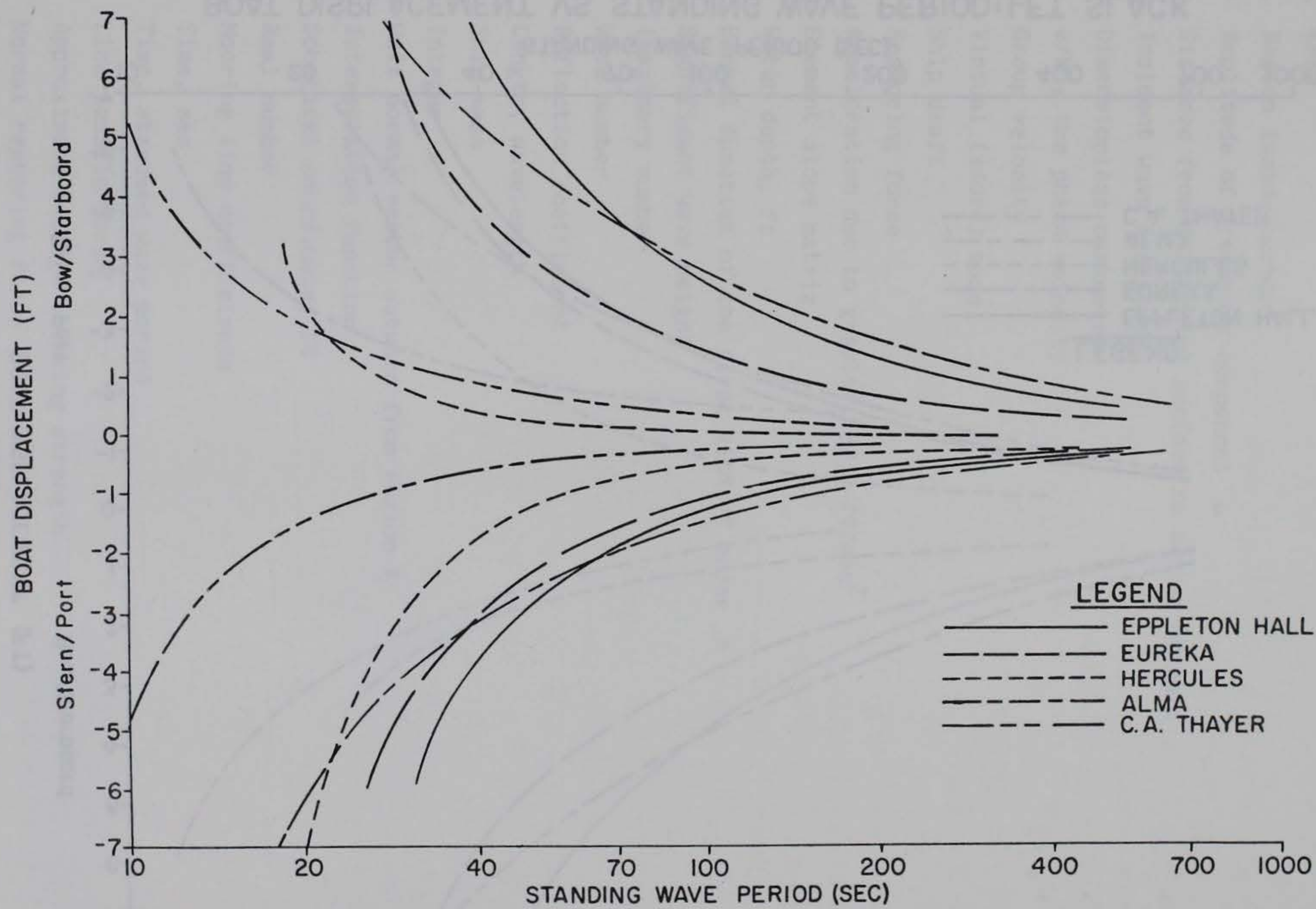
BOAT DISPLACEMENT VS. STANDING WAVE PERIOD: NO SLACK
