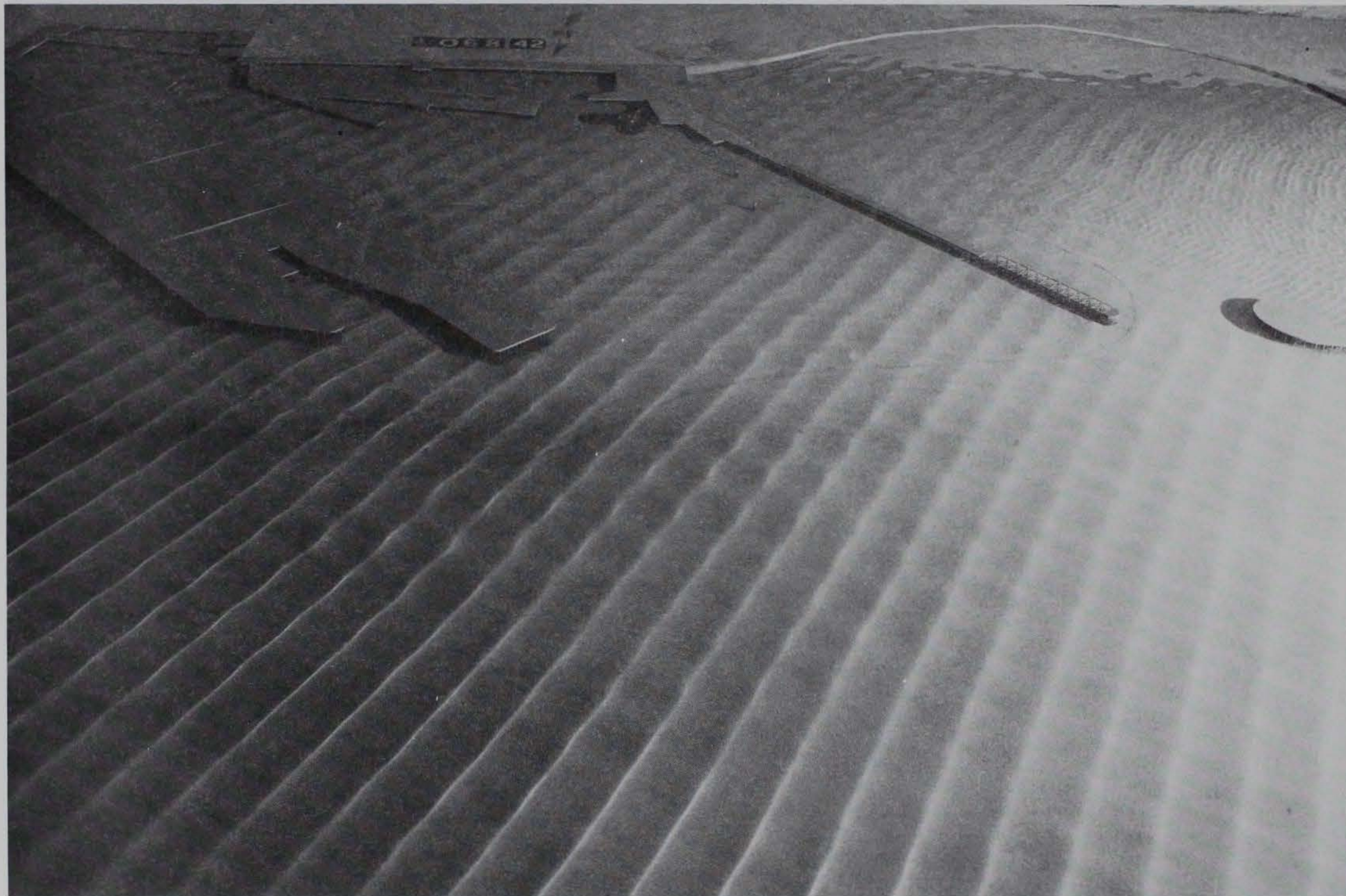
Photo 11. Typical wave patterns for existing conditions; 3.6-sec, 2-ft waves from west-northwest; +5.7 ft swl
