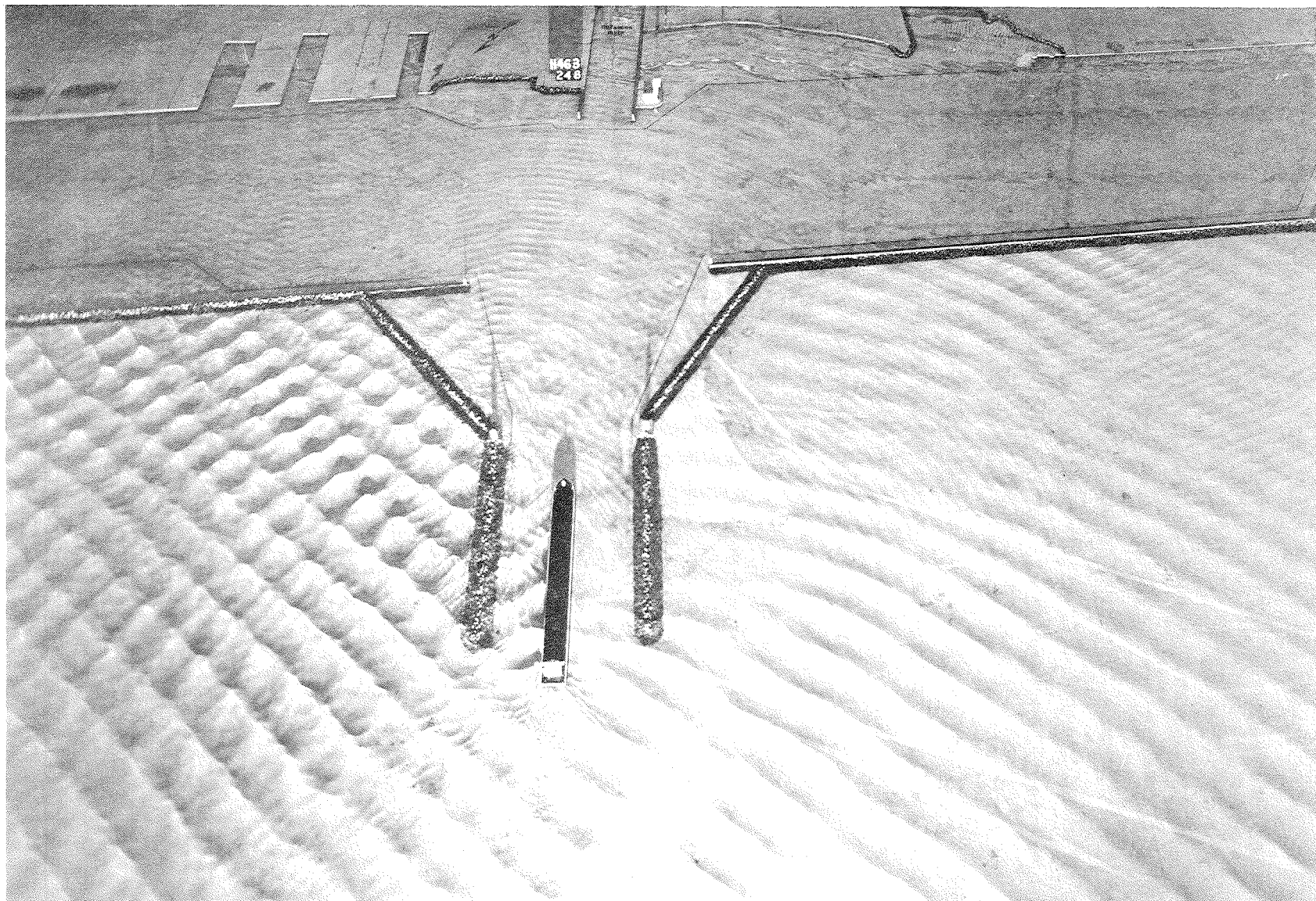
Figure 9. Three-dimensional wave basin scale model test
