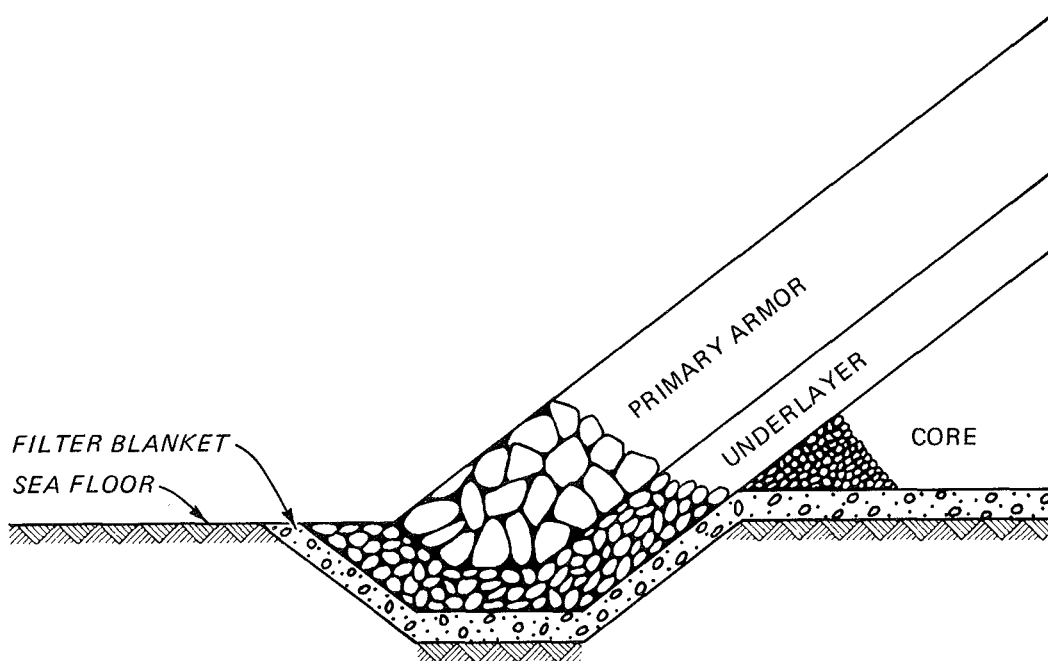
Figure 7. Typical toe trench
