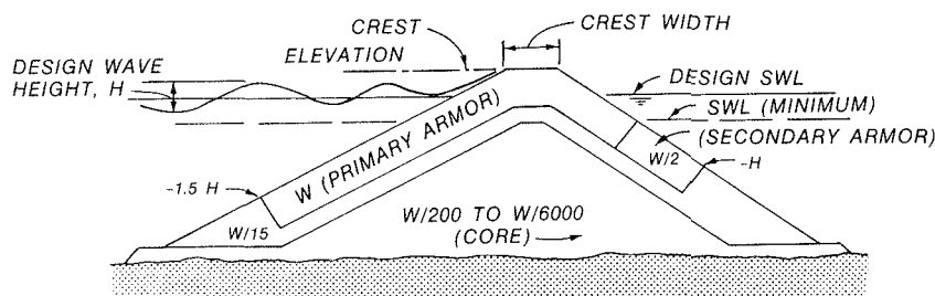
Figure 2. A typical rubble-mound breakwater cross section
