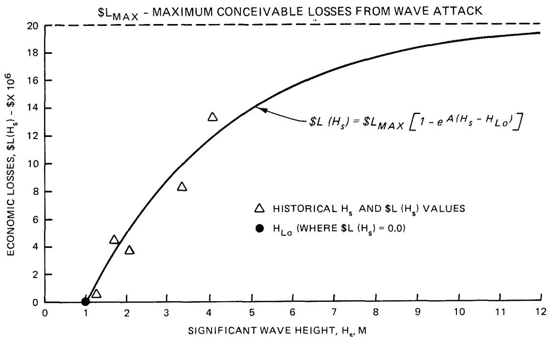
Figure 16. Economic loss function versus incident wave height
