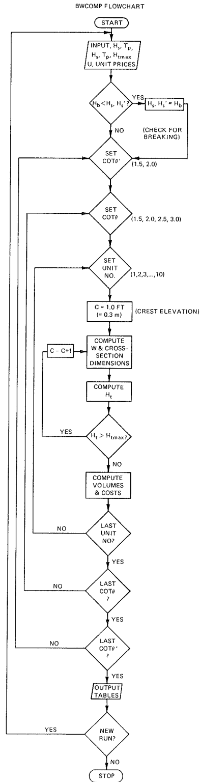
Figure B1. BWCMP flowchart
