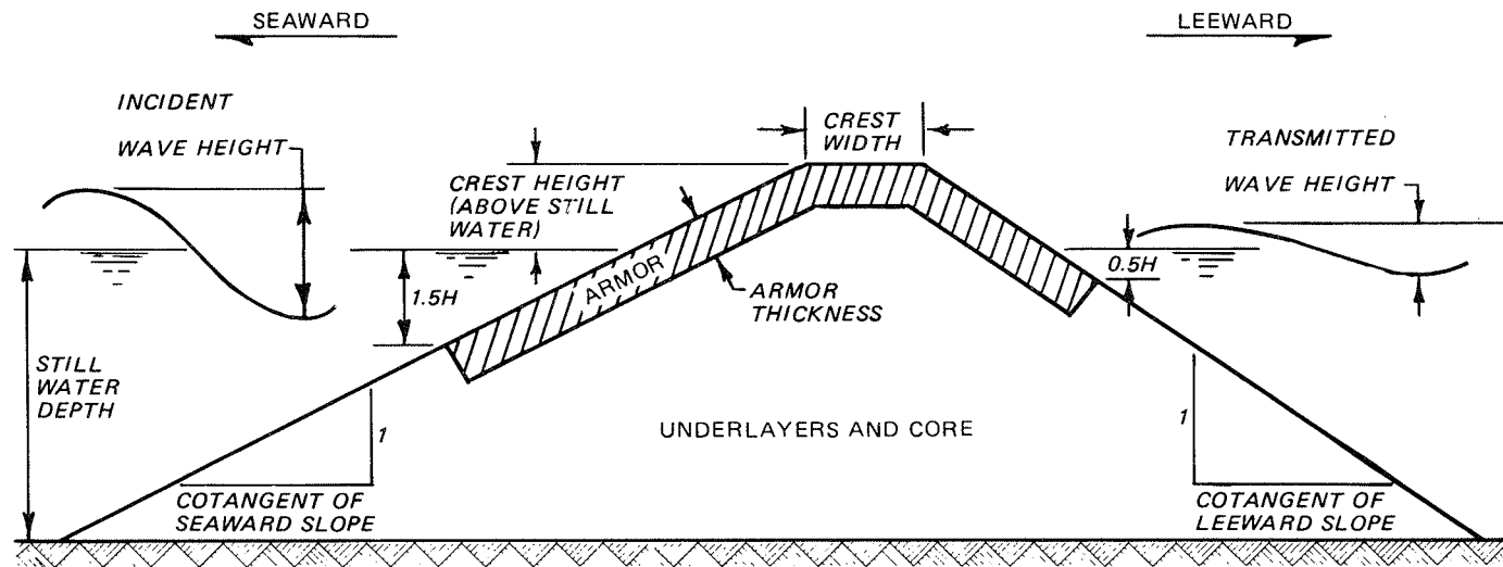
Figure 17. Parameterized cross section applied in program BWCOMP
