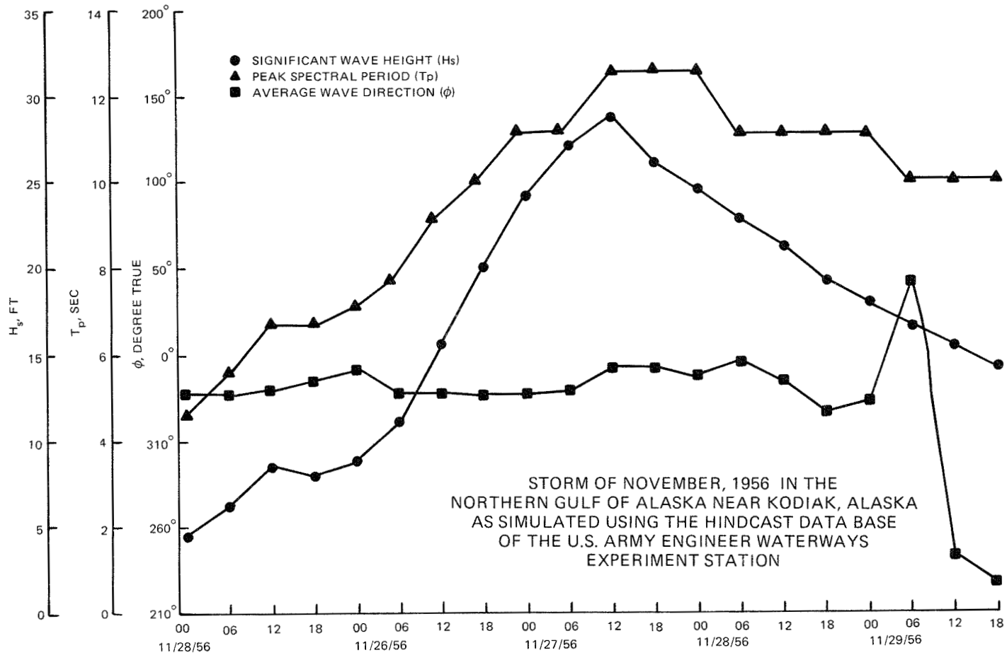
Figure 5. Typical time-history of wave parameters (To convert feet to meters, multiply by a factor of 0.3048)
