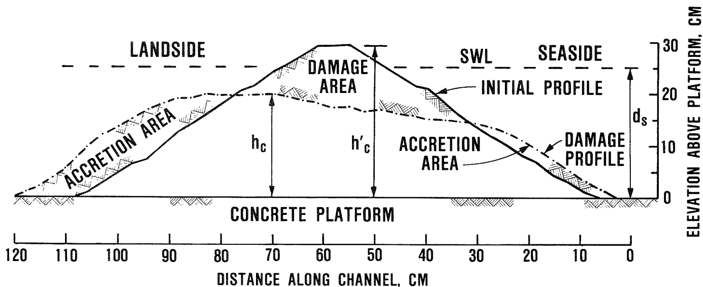
Figure 10. Definition sketch for dimensionless damage
