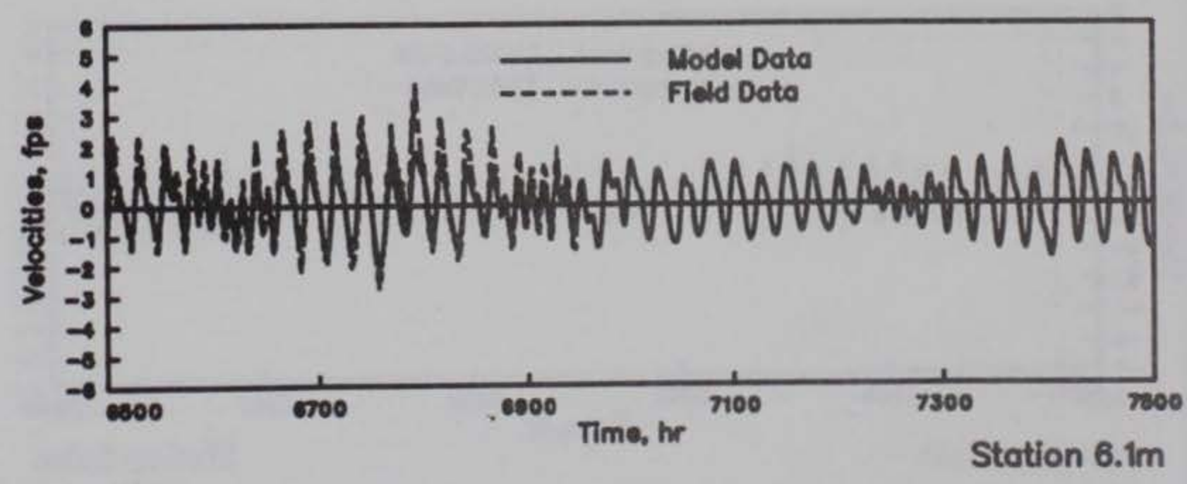
GALVESTON BAY VELOCITIES MODEL VERIFICATION STATIONS 6.0m, 6.0t, AND 6.1m HOURS 6500-7500
