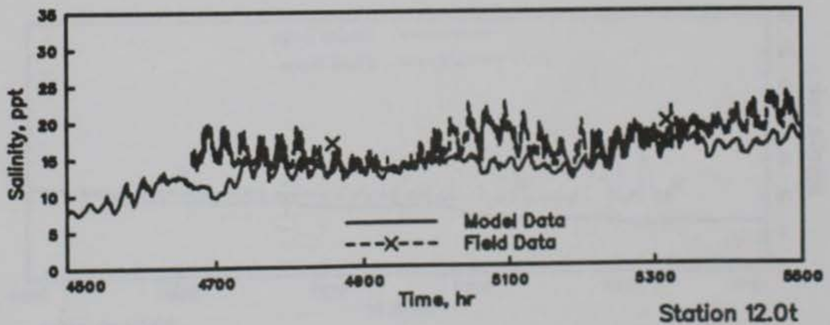
GALVESTON BAY SALINITIES MODEL VERIFICATION STATIONS 11.2, 12.0m, AND 12.0t HOURS 4500-5500
