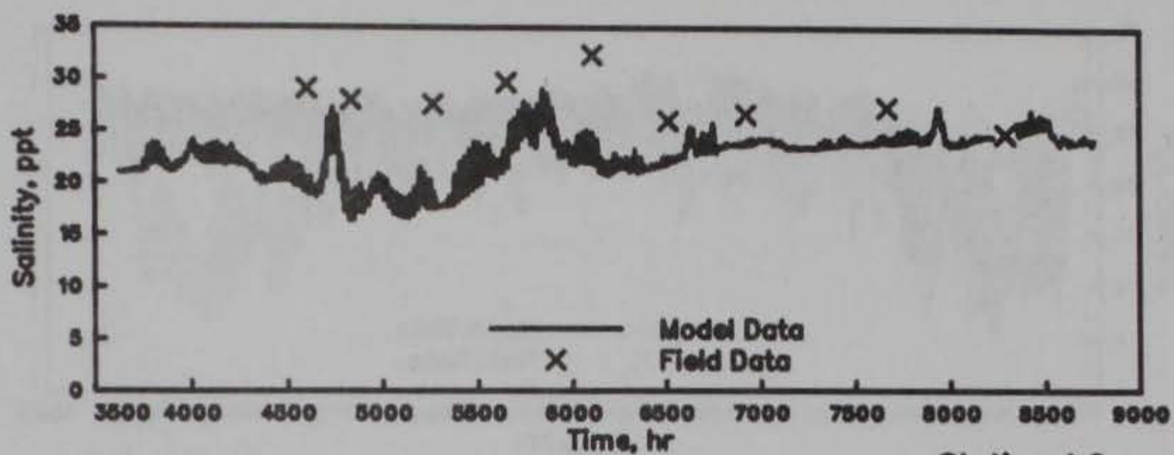
Station 4.0
