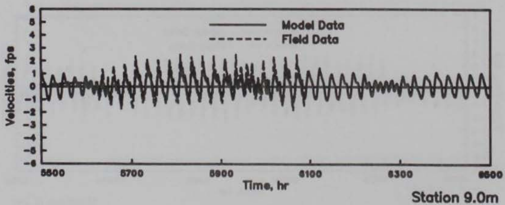
GALVESTON BAY VELOCITIES MODEL VERIFICATION STATIONS 6.1t, 8.0, AND 9.0m HOURS 5500-6500
