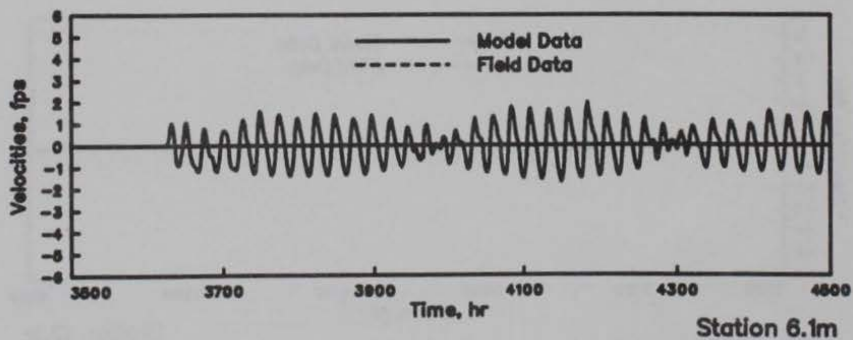
GALVESTON BAY VELOCITIES MODEL VERIFICATION STATIONS 6.0m, 6.0t, AND 6.1m HOURS 3500-4500
