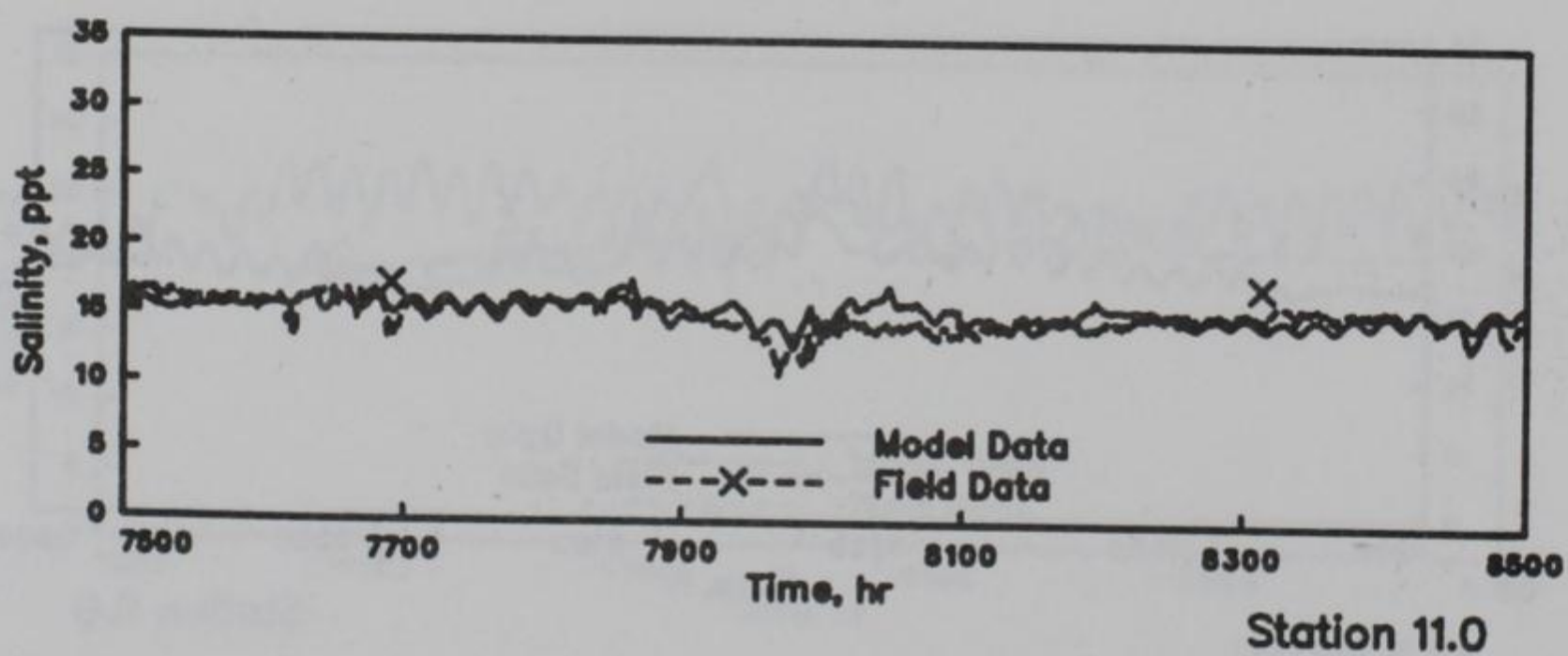
GALVESTON BAY SALINITIES MODEL VERIFICATION STATIONS 9.0m, 9.0t, AND 11.0 HOURS 7500-8500
