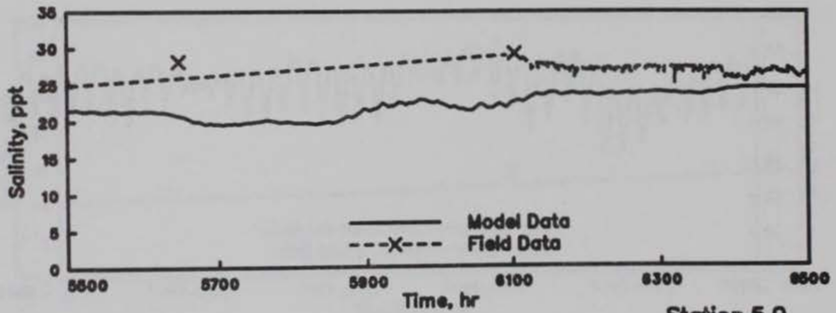
Station 5.0
