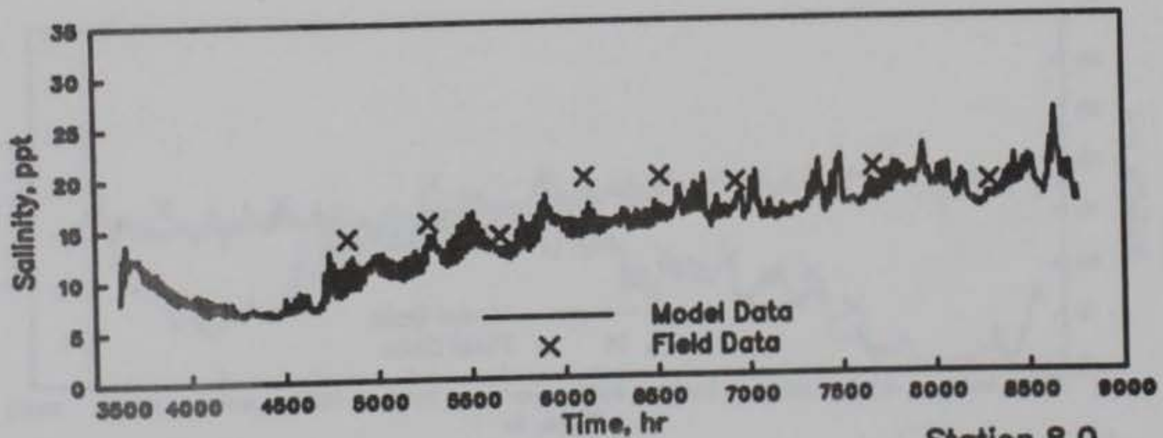
Station 8.0
