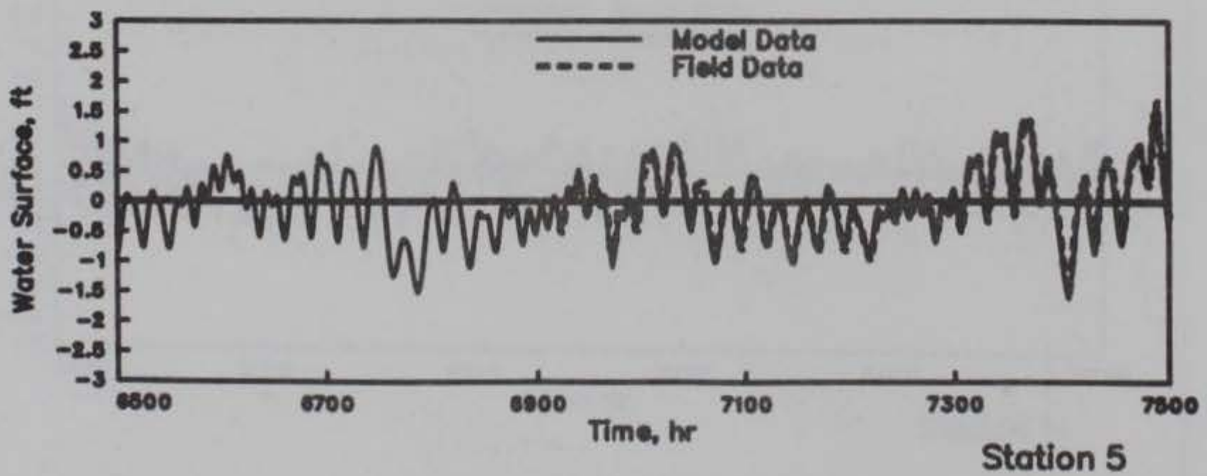
WATER-SURFACE ELEVATIONS MODEL VERIFICATION STATIONS 1, 3, AND 5 HOURS 6500-7500
