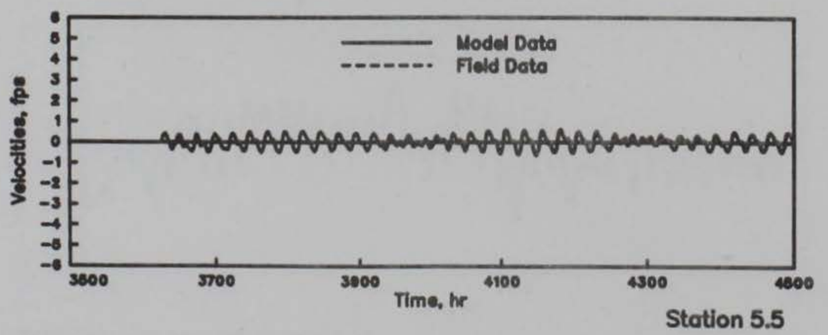
GALVESTON BAY VELOCITIES MODEL VERIFICATION STATIONS 2.0m, 2.0t, AND 5.5 HOURS 3500-4500
