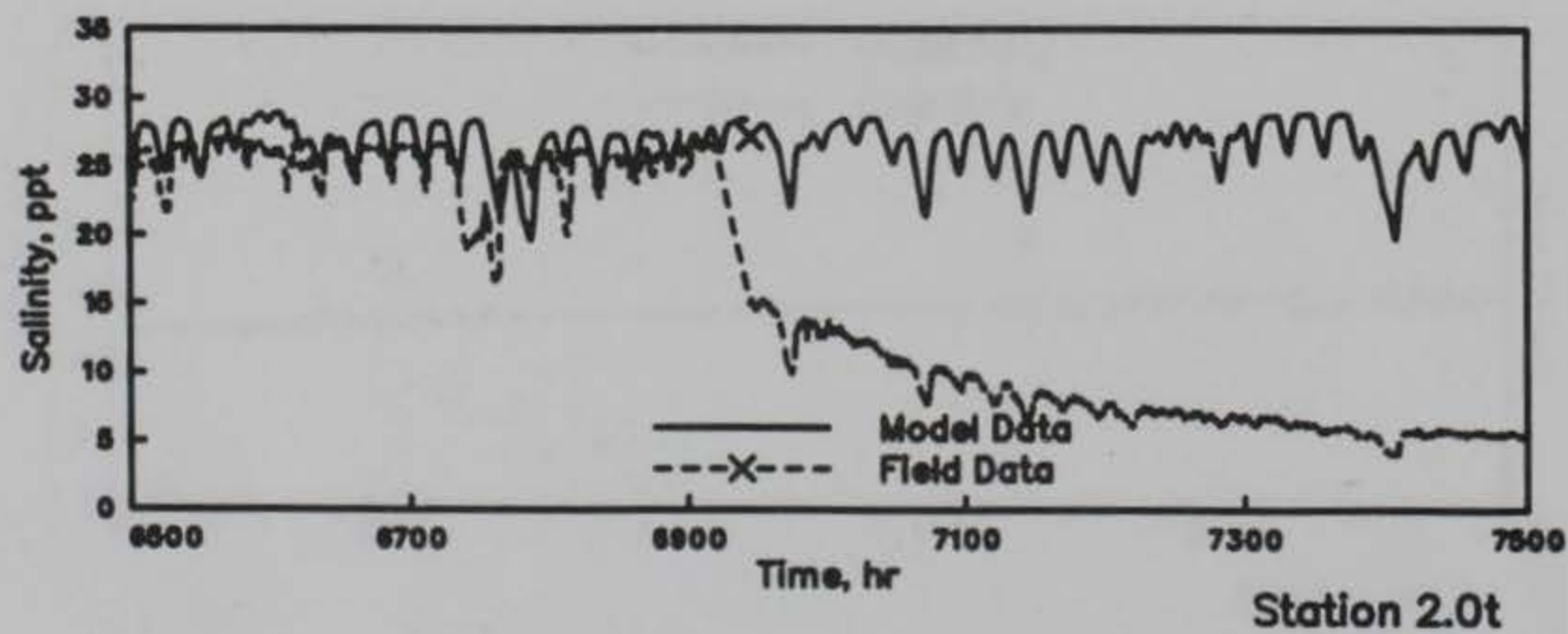
GALVESTON BAY SALINITIES MODEL VERIFICATION STATIONS 1.0, 2.0m, AND 2.0t HOURS 6500-7500
