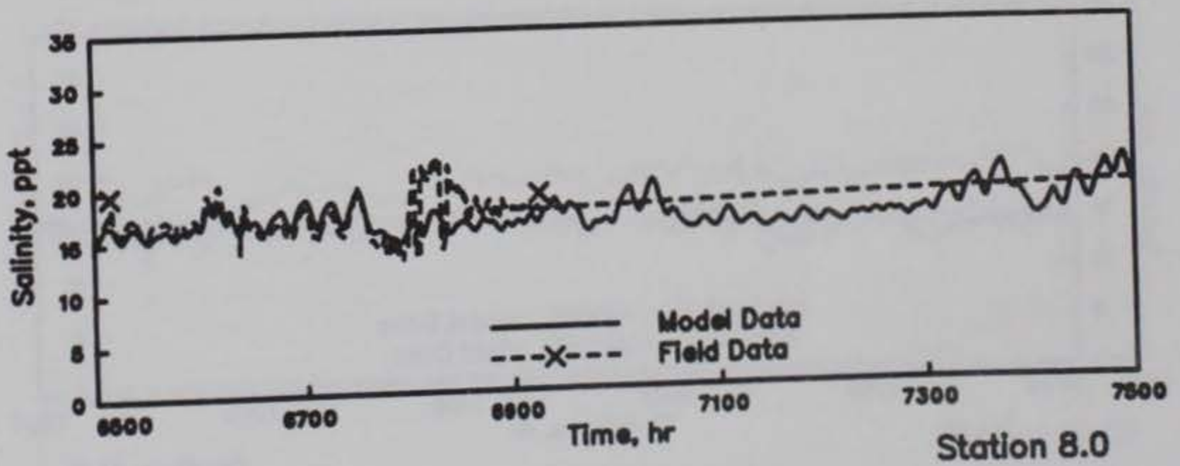
GALVESTON BAY SALINITIES MODEL VERIFICATION STATIONS 6.1t, 7.0, AND 8.0 HOURS 6500-7500
