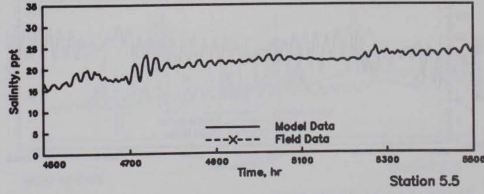
GALVESTON BAY SALINITIES MODEL VERIFICATION STATIONS 4.0, 5.0, AND 5.5 HOURS 4500-5500
