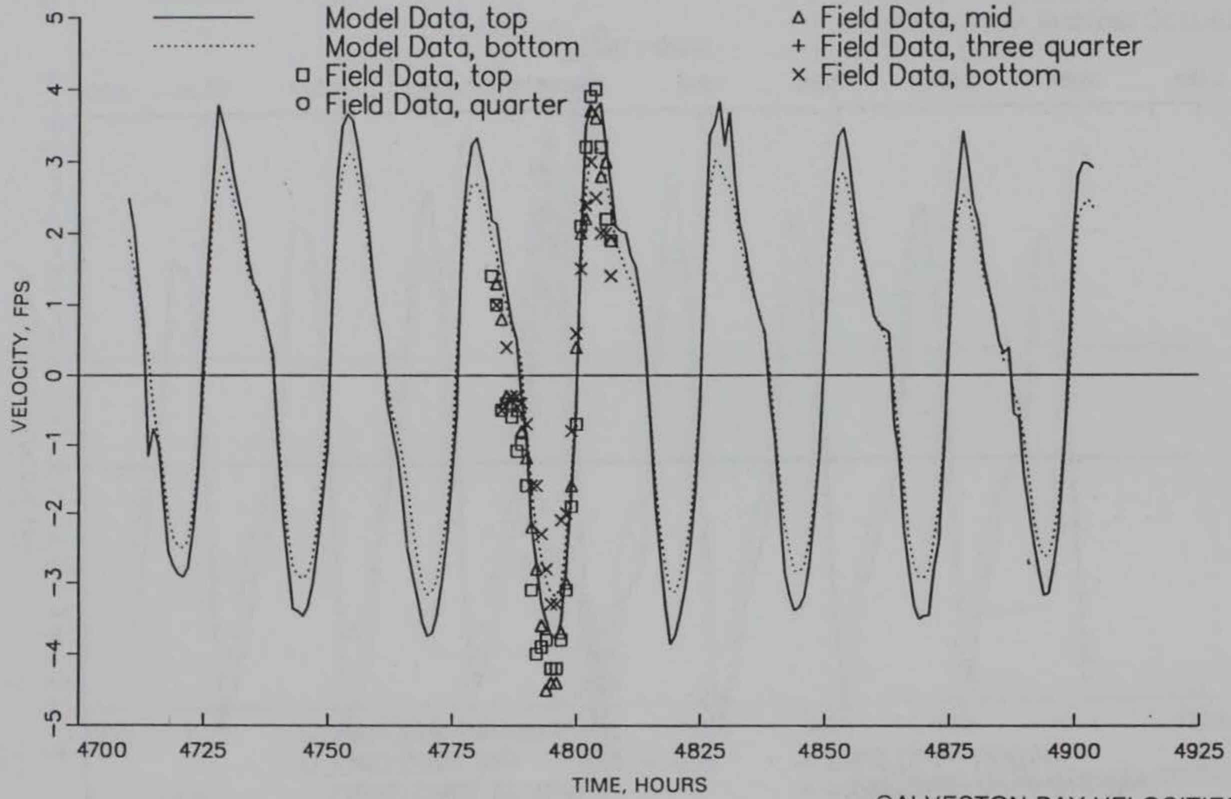
GALVESTON BAY VELOCITIES RANGE 2A
