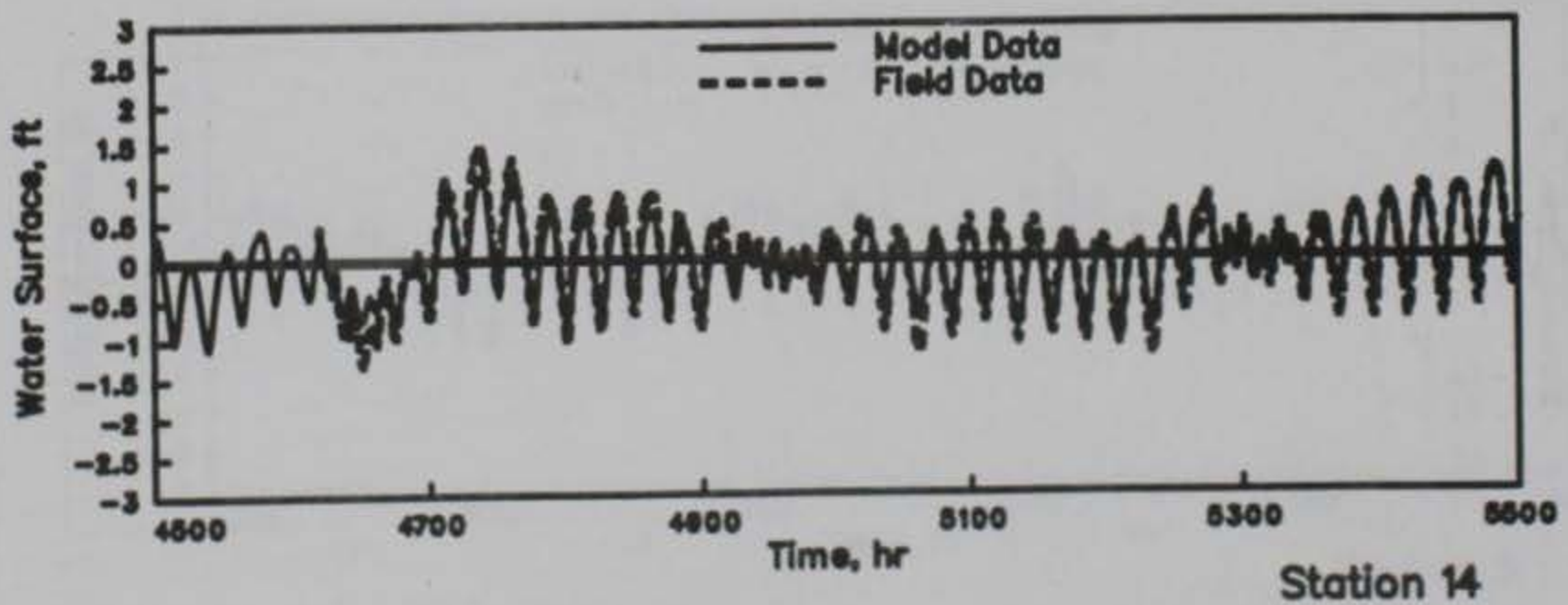
WATER-SURFACE ELEVATIONS MODEL VERIFICATION STATIONS 7, 10, AND 14 HOURS 4500-5500
