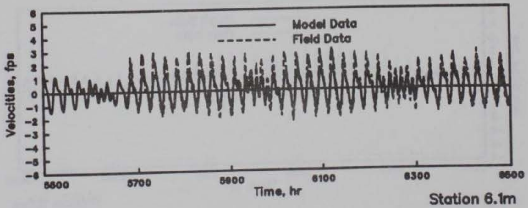
GALVESTON BAY VELOCITIES MODEL VERIFICATION STATIONS 6.0m, 6.0t, AND 6.1m HOURS 5500-6500
