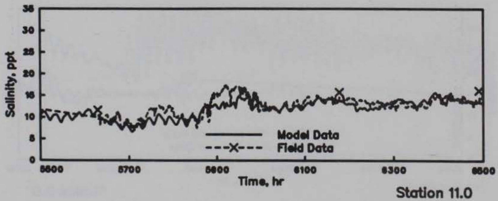
GALVESTON BAY SALINITIES MODEL VERIFICATION STATIONS 9.0m, 9.0t, AND 11.0 HOURS 5500-6500
