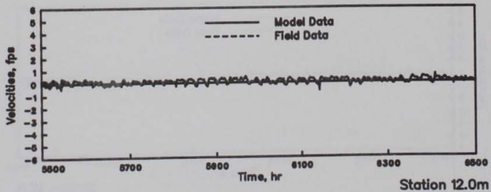
GALVESTON BAY VELOCITIES MODEL VERIFICATION STATIONS 9.0t, 11.1, AND 12.0m HOURS 5500-6500
