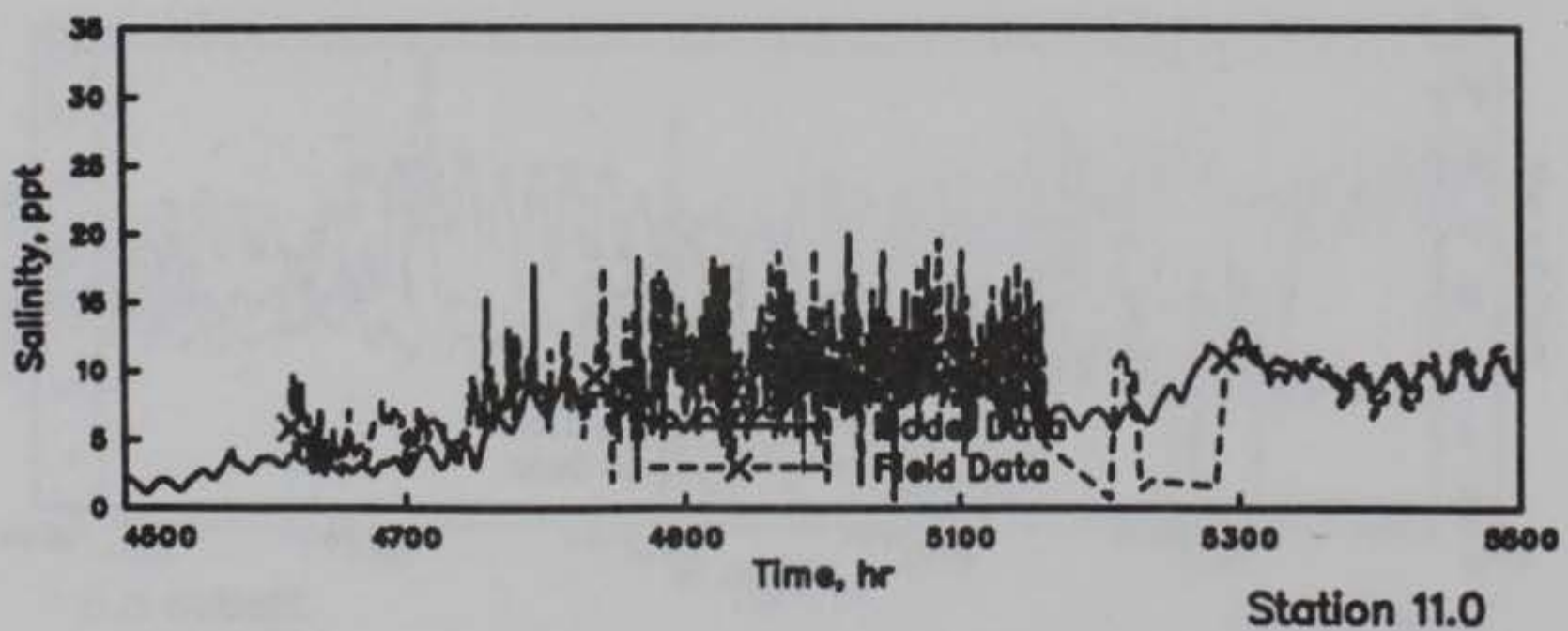
GALVESTON BAY SALINITIES MODEL VERIFICATION STATIONS 9.0m, 9.0t, AND 11.0 HOURS 4500-5500
