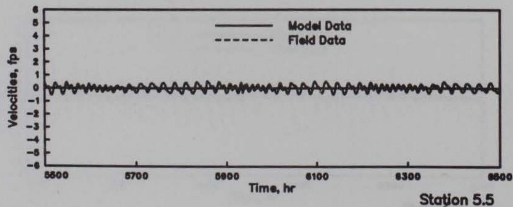
GALVESTON BAY VELOCITIES MODEL VERIFICATION STATIONS 2.0m, 2.0t, AND 5.5 HOURS 5500-6500
