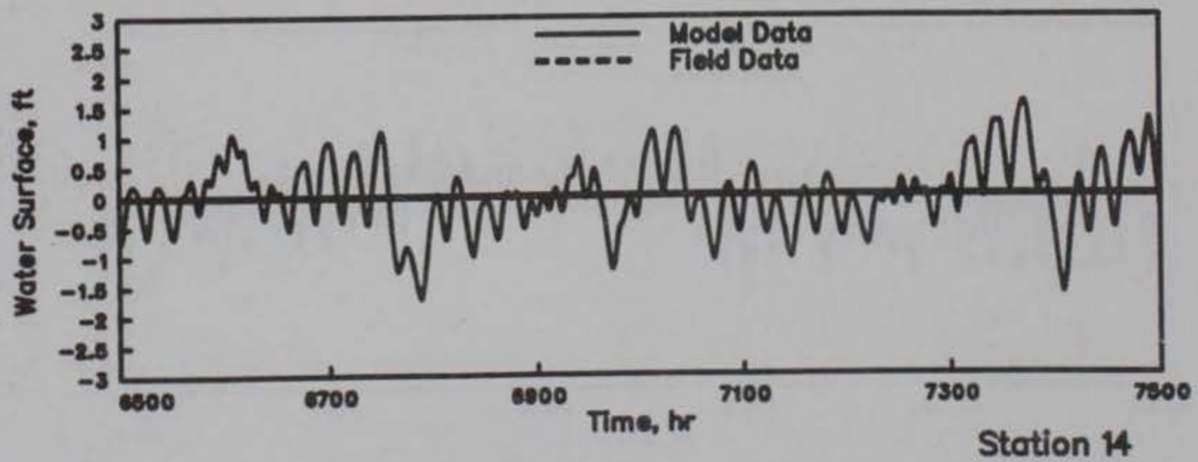
WATER-SURFACE ELEVATIONS MODEL VERIFICATION STATIONS 7, 10, AND 14 HOURS 6500-7500
