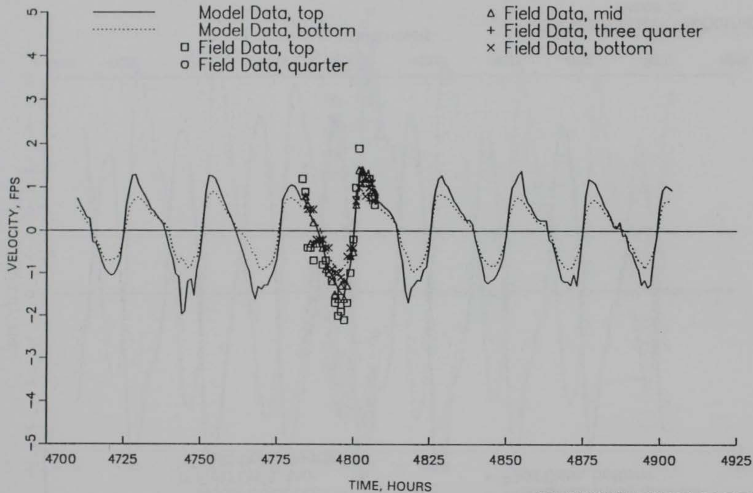
GALVESTON BAY VELOCITIES RANGE 3A
