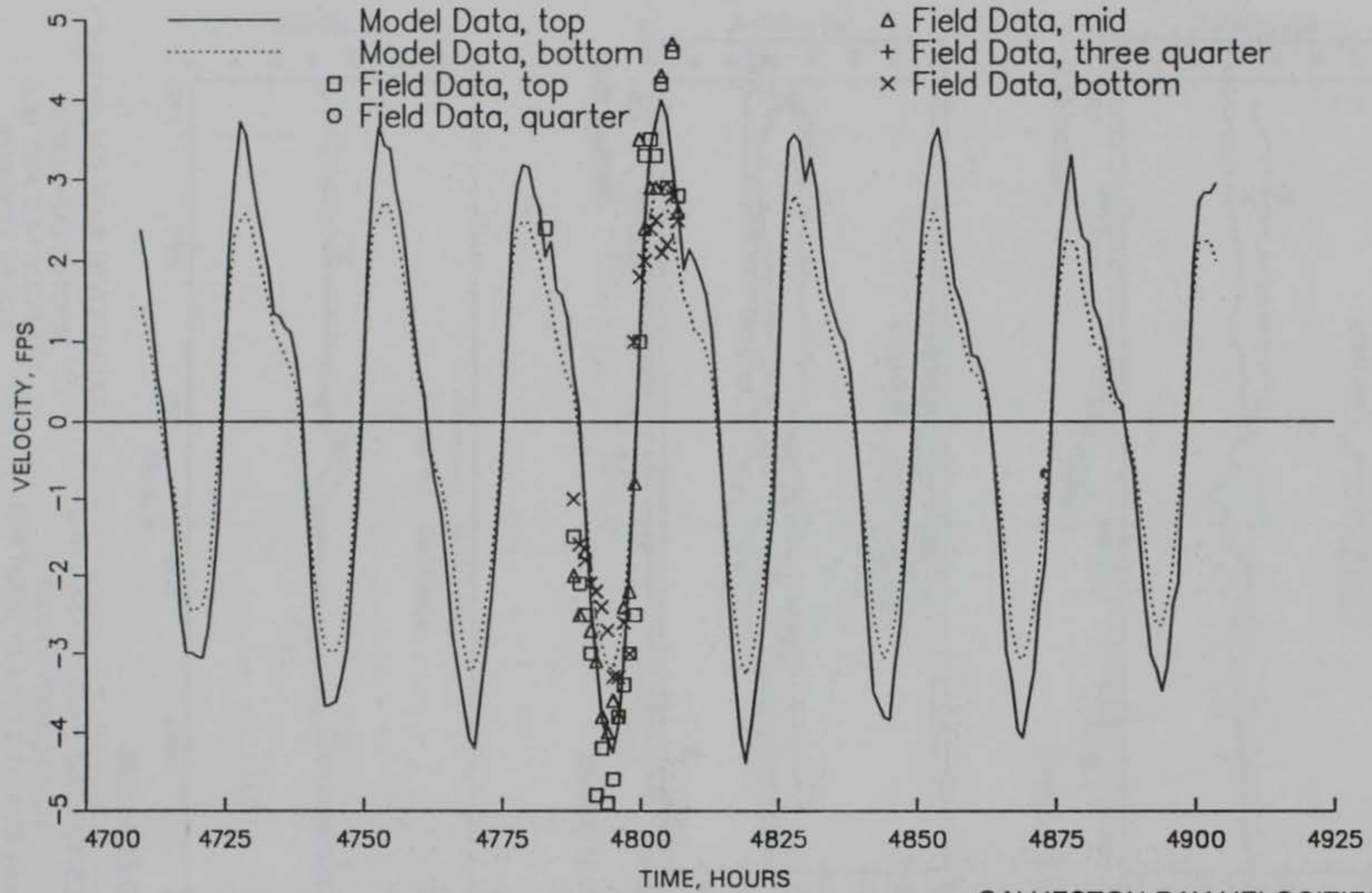
GALVESTON BAY VELOCITIES RANGE 1A
