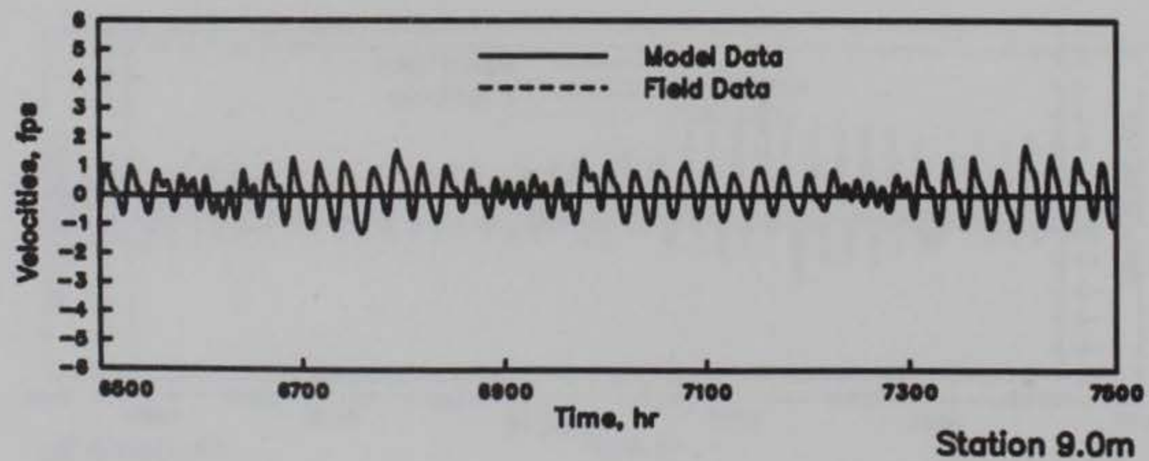
GALVESTON BAY VELOCITIES MODEL VERIFICATION STATIONS 6.1t, 8.0, AND 9.0m HOURS 6500-7500
