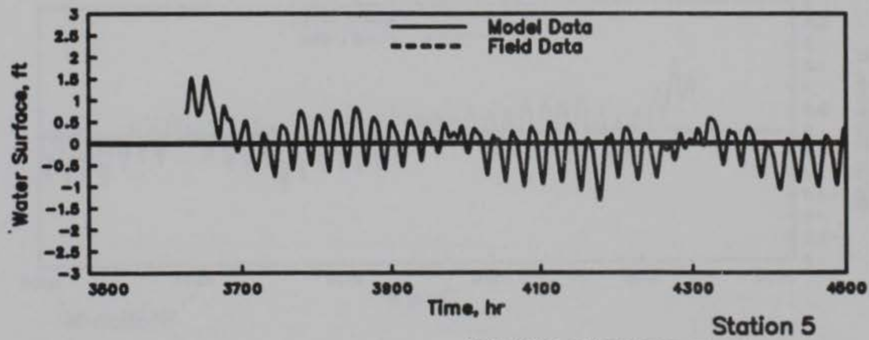
WATER-SURFACE ELEVATIONS MODEL VERIFICATION STATIONS 1, 3, AND 5 HOURS 3500-4500
