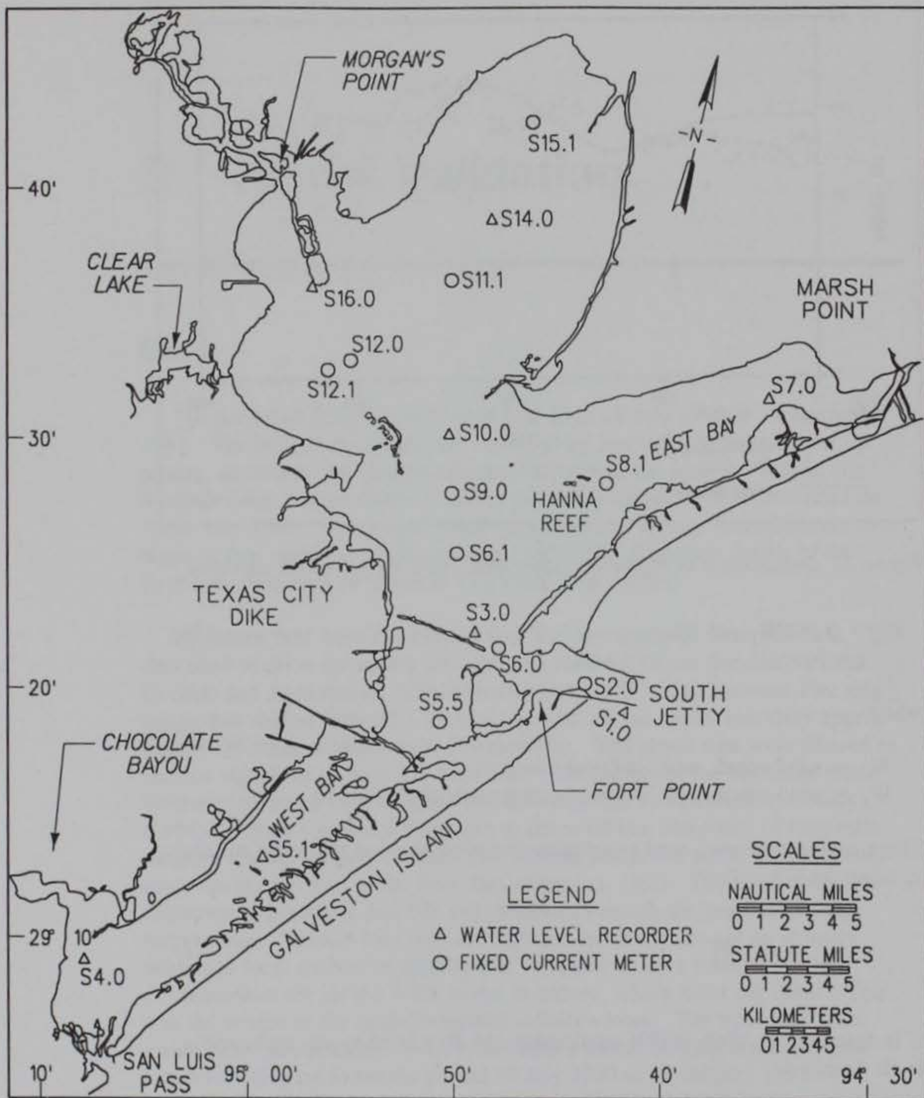
Figure 5. Basic long-term survey data collection equipment locations. (Stations S1.0, S2.0, S5.5, S6.0, S6.1, S8.1, S9.0, S11.1, S12.0 and S15.1 record salinity as well.)
