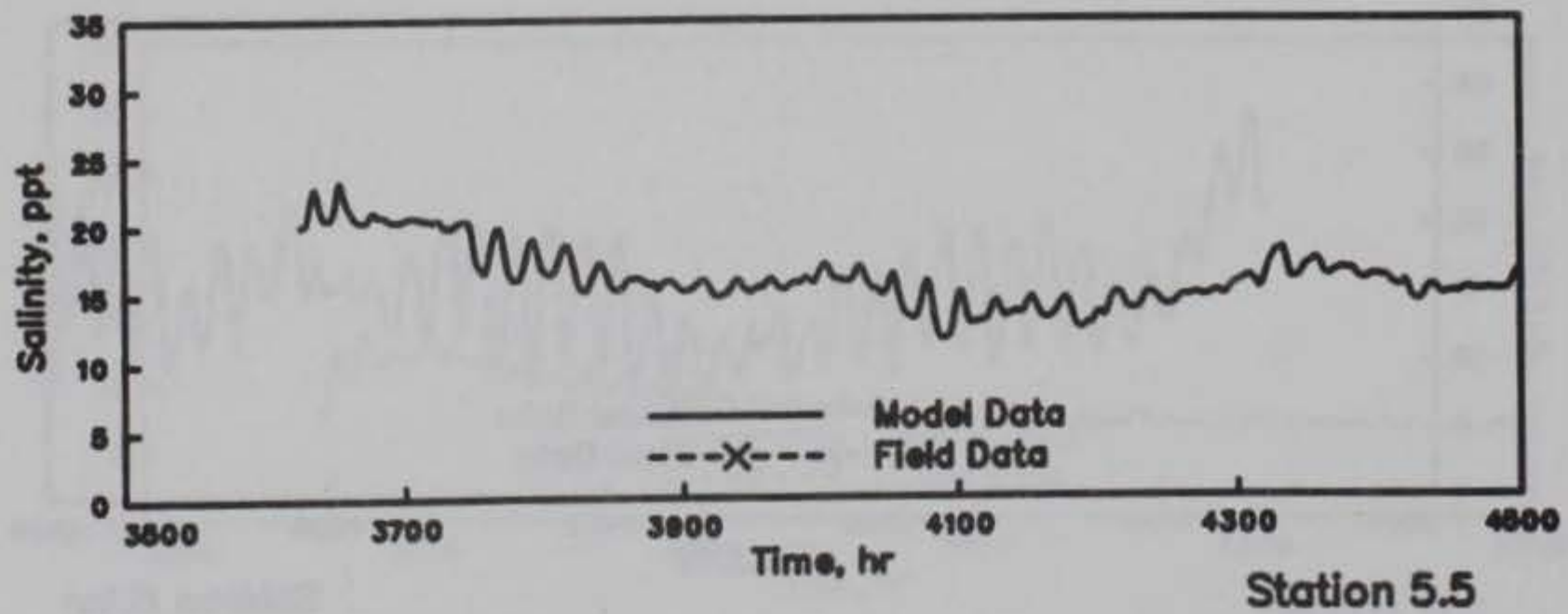
GALVESTON BAY SALINITIES MODEL VERIFICATION STATIONS 4.0, 5.0, AND 5.5 HOURS 3500-4500
