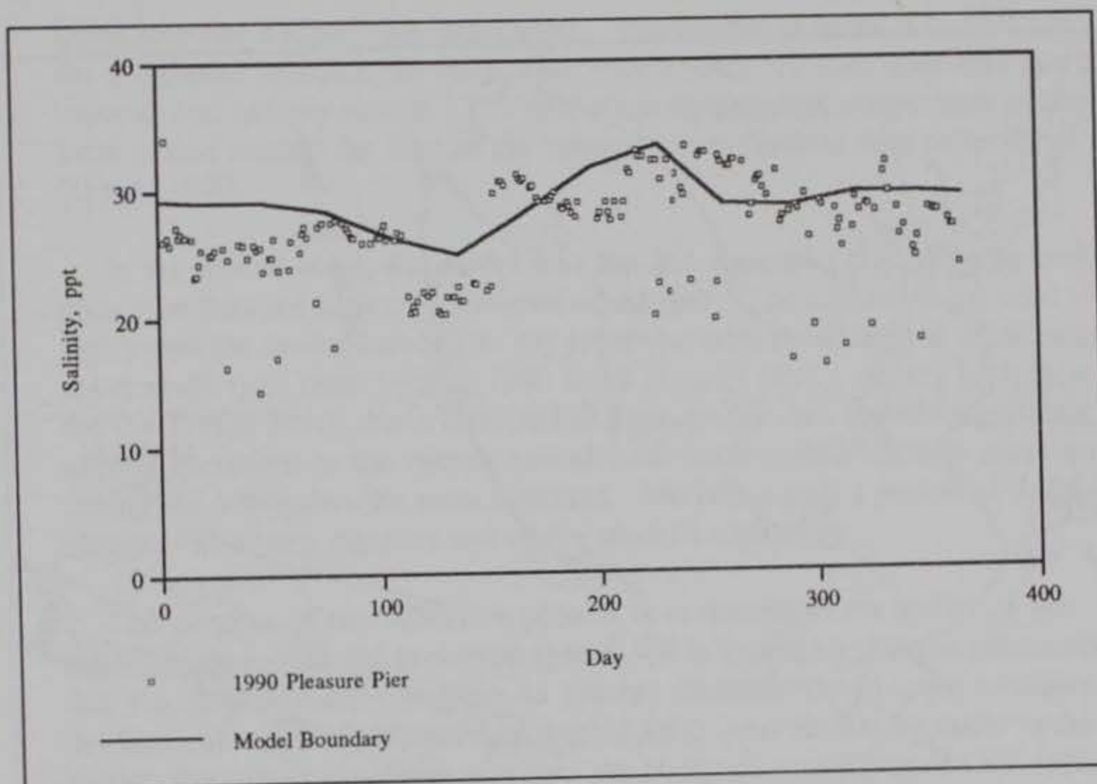
Figure 4. Comparison of model boundary and 1990 Pleasure Pier salinities
