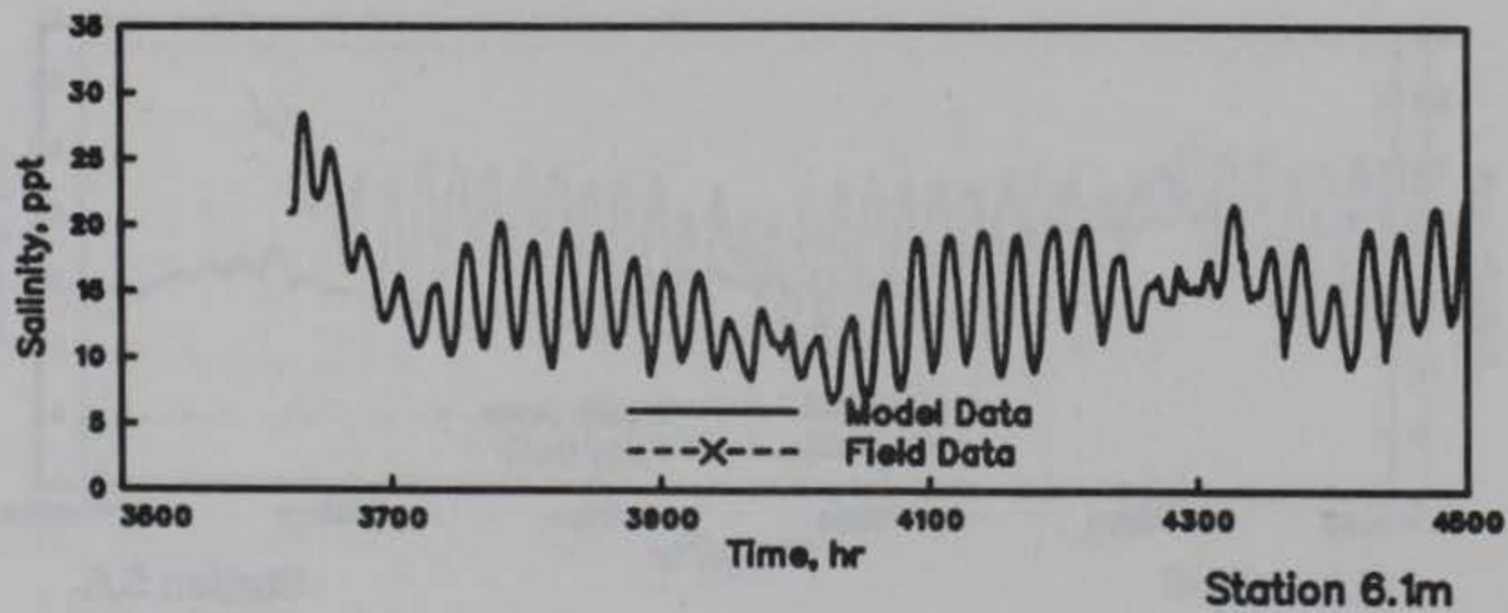
GALVESTON BAY SALINITIES MODEL VERIFICATION STATIONS 6.0m, 6.0t, AND 6.1m HOURS 3500-4500
