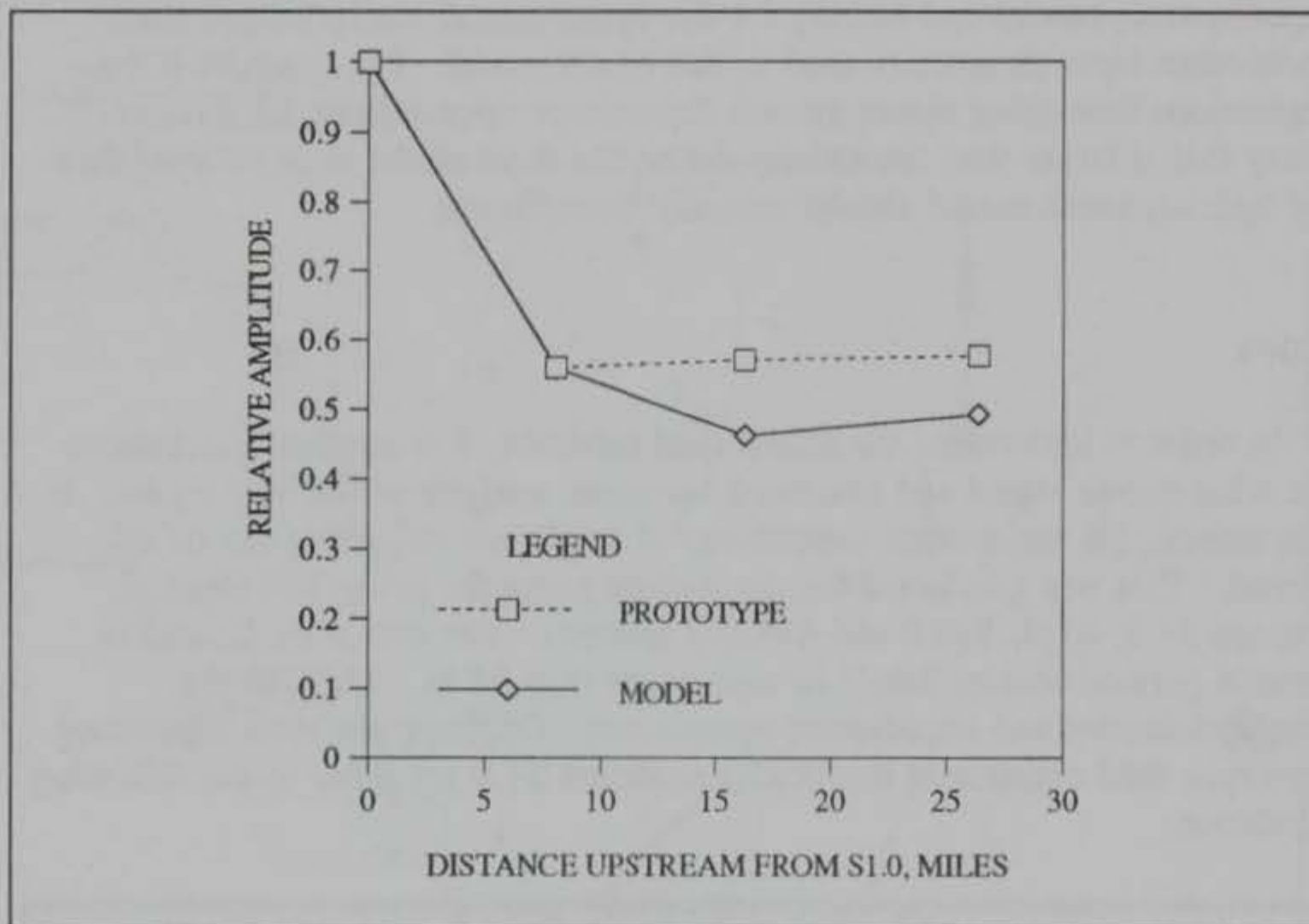
Figure 9. Model/prototype tidal amplitude comparison
