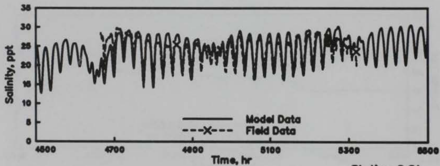
Station 6.0t
