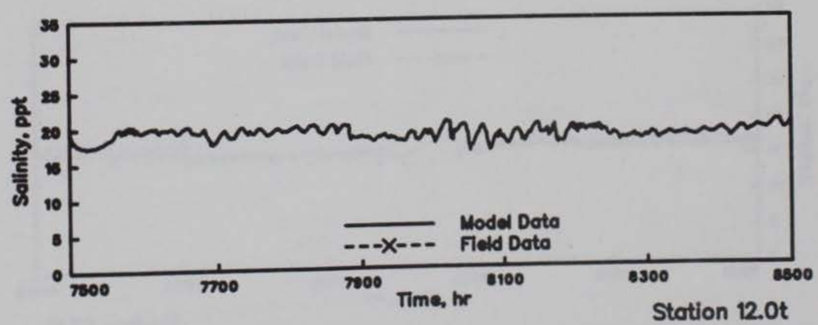
GALVESTON BAY SALINITIES MODEL VERIFICATION STATIONS 11.2, 12.0m, AND 12.0t HOURS 7500-8500
