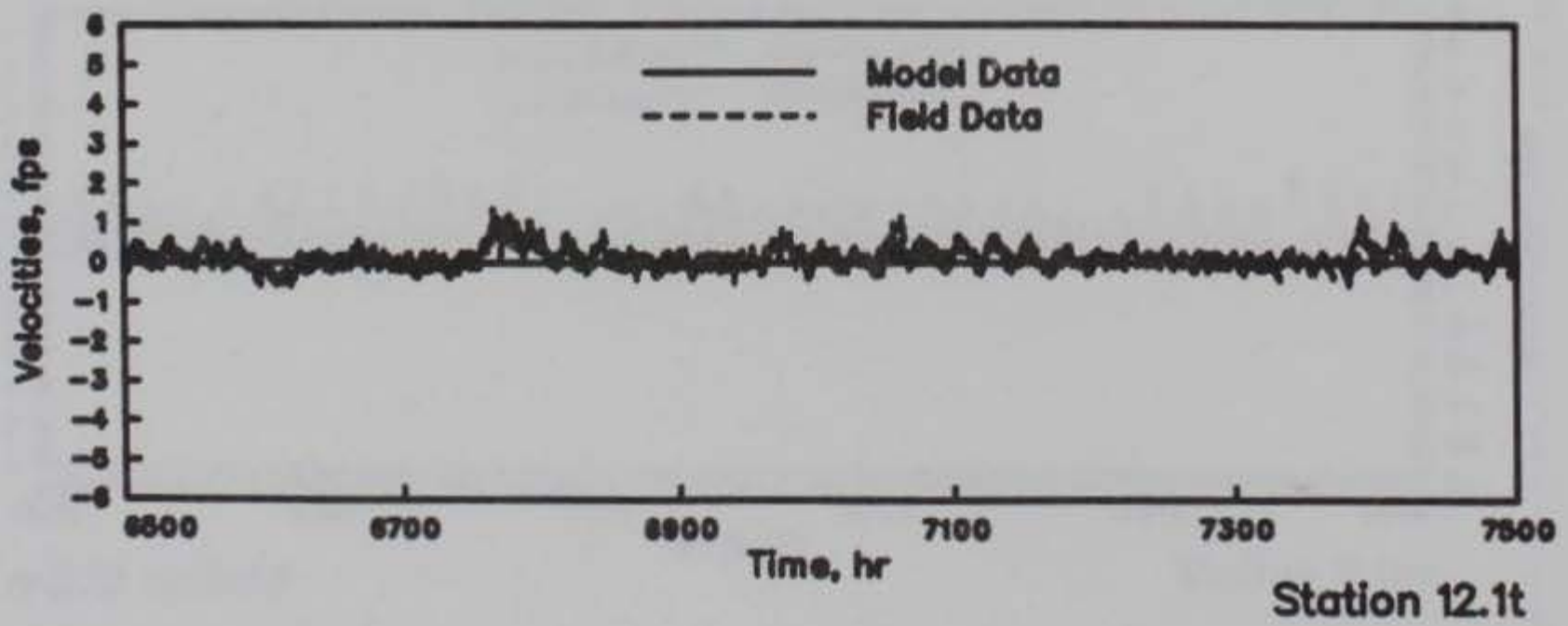
GALVESTON BAY VELOCITIES MODEL VERIFICATION STATIONS 12.0t, 12.1m, AND 12.1t HOURS 6500-7500
