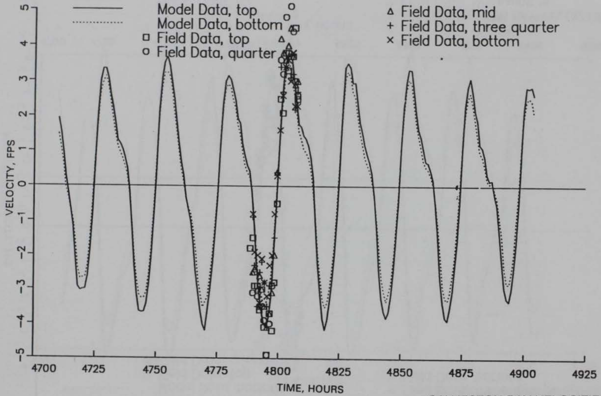
GALVESTON BAY VELOCITIES RANGE 1C
