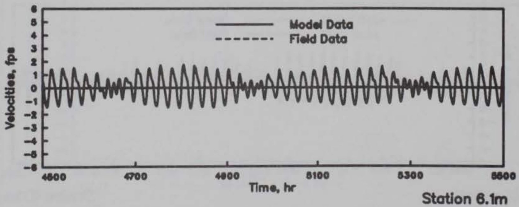
GALVESTON BAY VELOCITIES MODEL VERIFICATION STATIONS 6.0m, 6.0t, AND 6.1m HOURS 4500-5500
