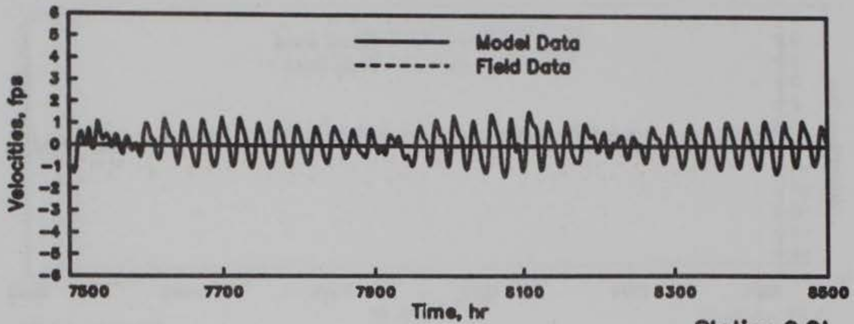
Station 9.0t
