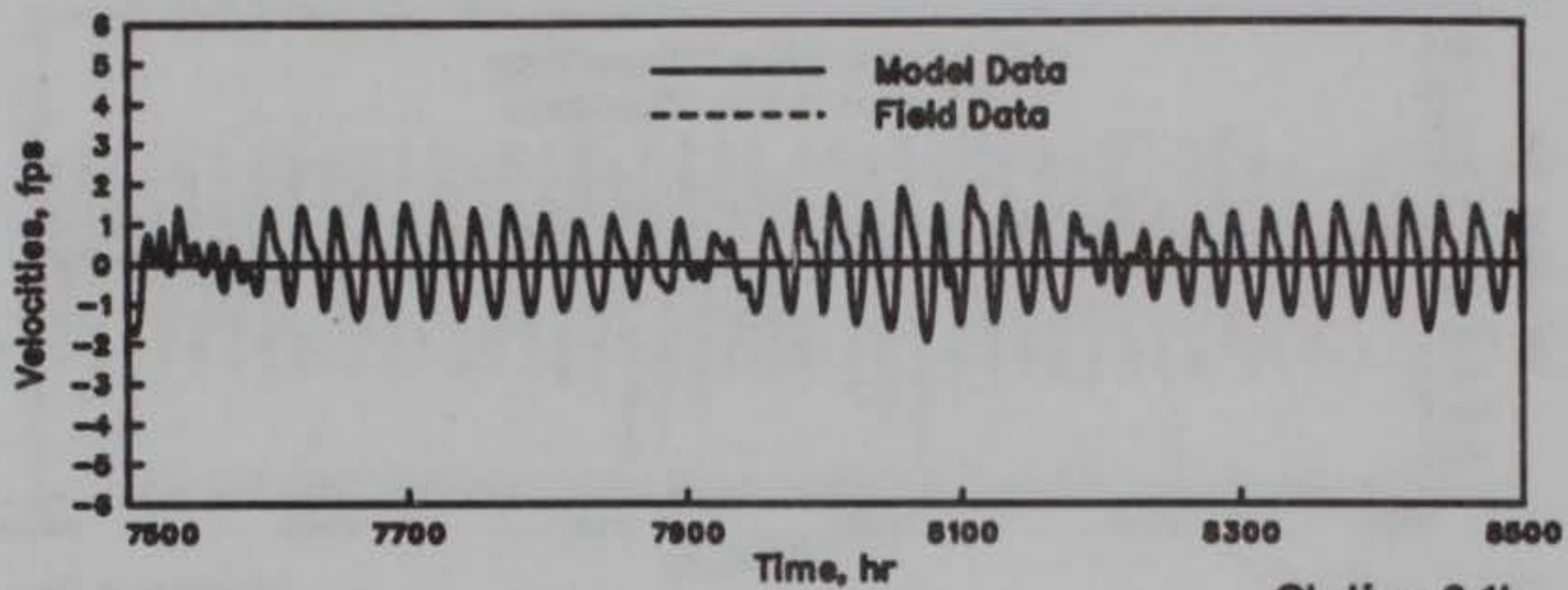
Station 6.1t
