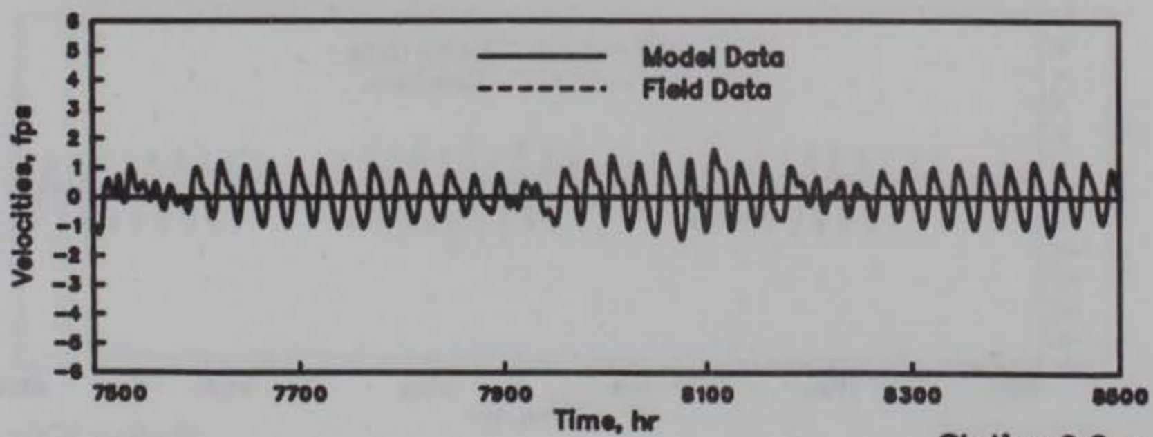
Station 9.0m
