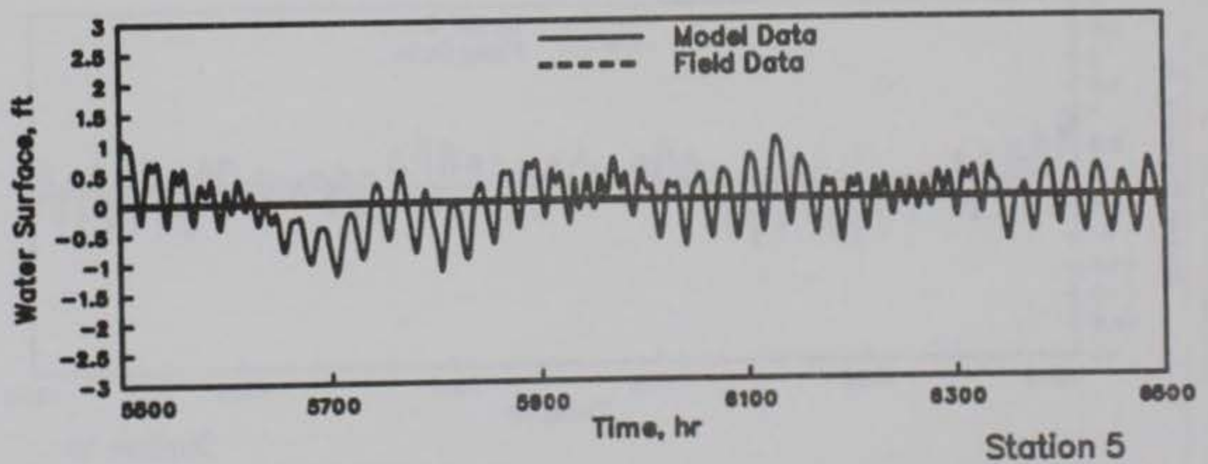
WATER-SURFACE ELEVATIONS MODEL VERIFICATION STATIONS 1, 3, AND 5 HOURS 5500-6500
