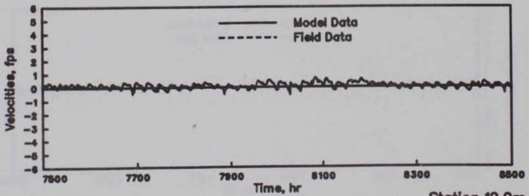
Station 12.0m
