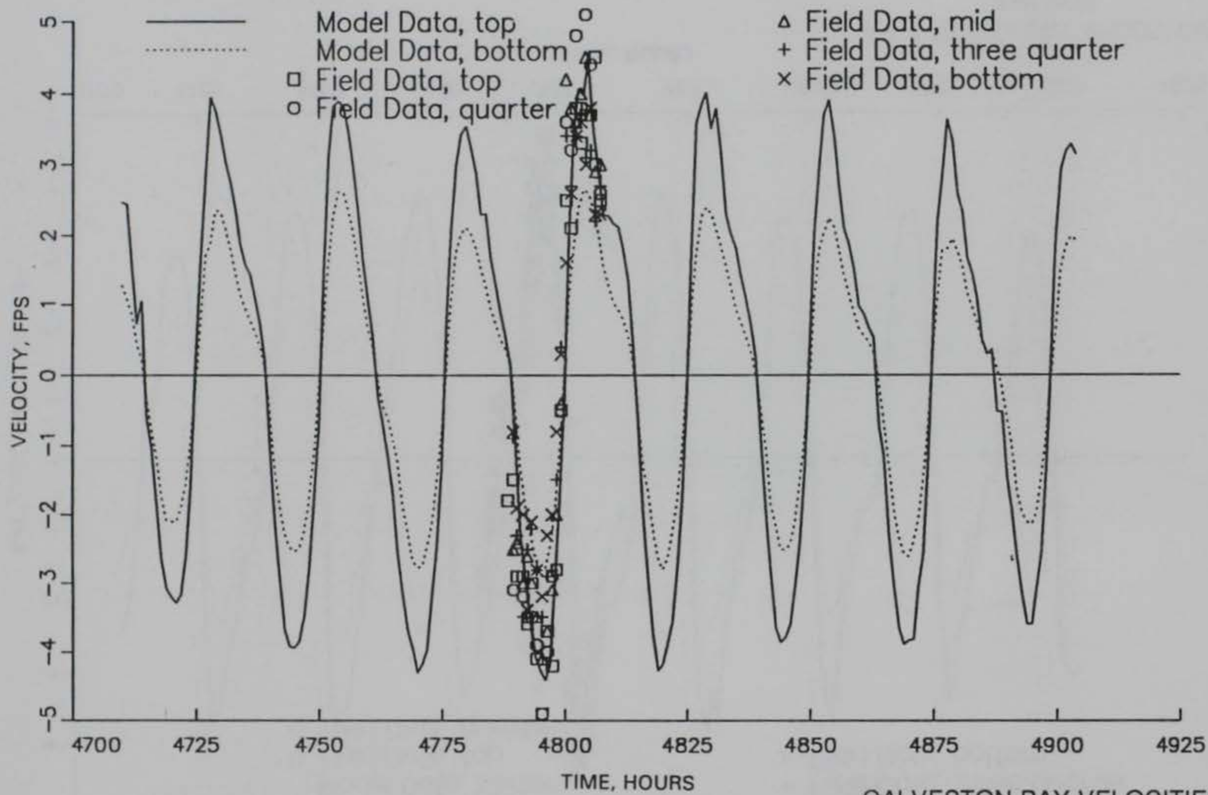
GALVESTON BAY VELOCITIES RANGE 2C
