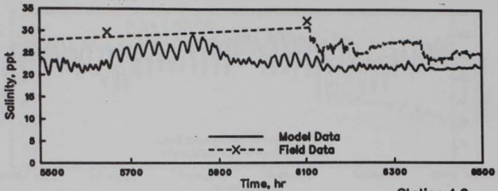
Station 4.0
