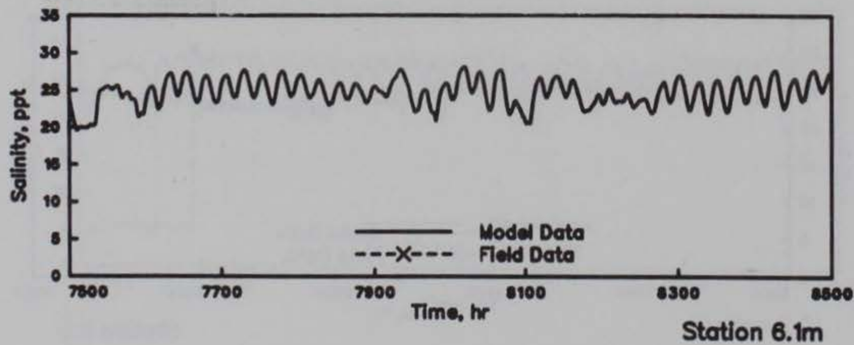
GALVESTON BAY SALINITIES MODEL VERIFICATION STATIONS 6.0m, 6.0t, AND 6.1m HOURS 7500-8500
