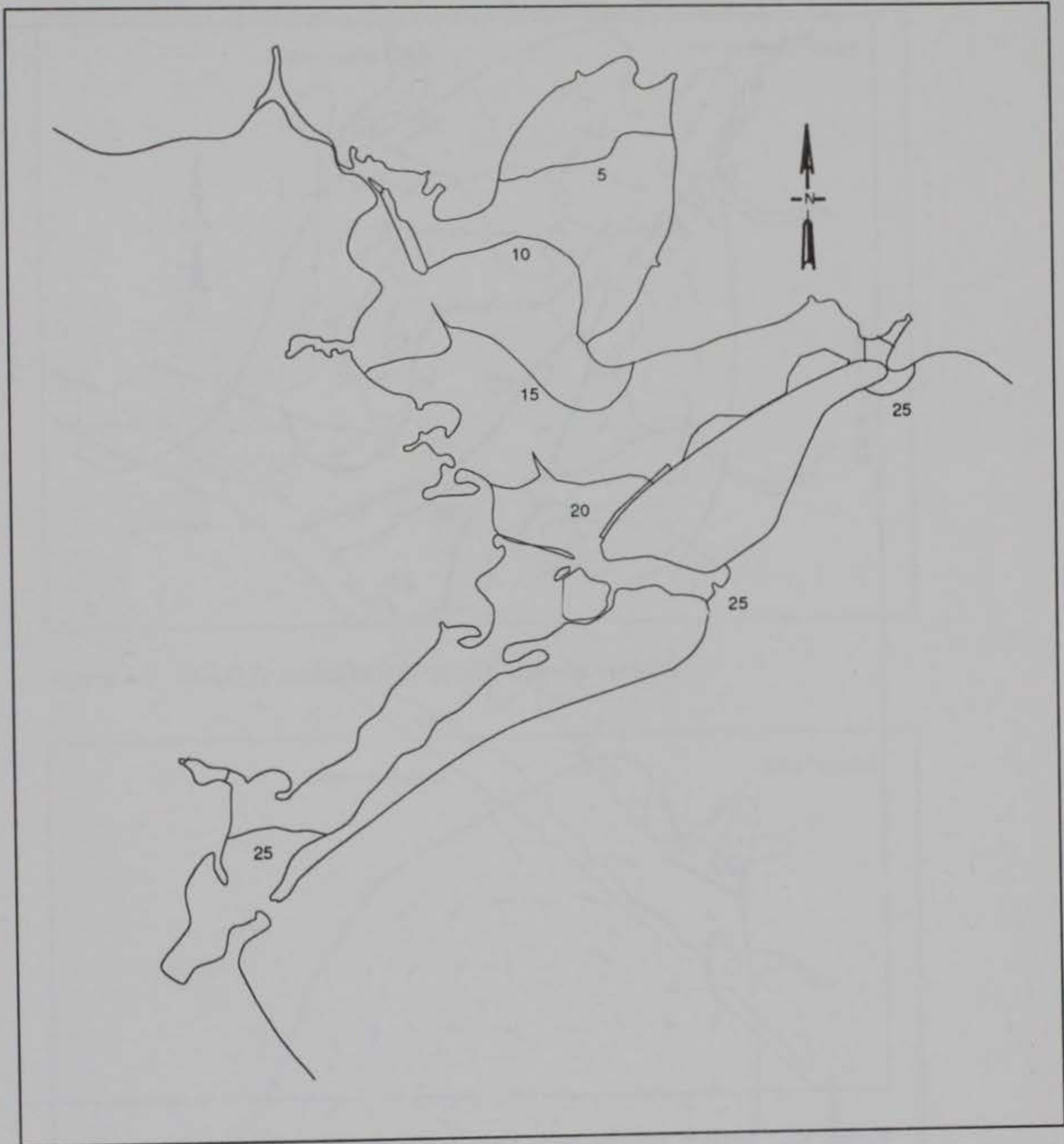
Figure 12. Isohaline plots, BASE versus Phase I bathymetry, low freshwater inflow, existing hydrology, bottom salinity
