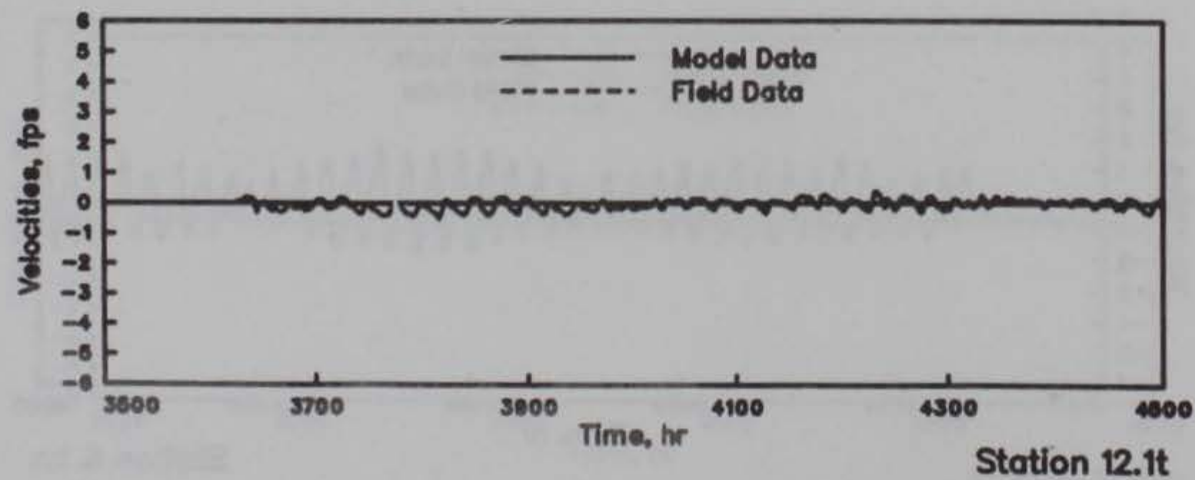
GALVESTON BAY VELOCITIES MODEL VERIFICATION STATIONS 12.0t, 12.1m, AND 12.1t HOURS 3500-4500
