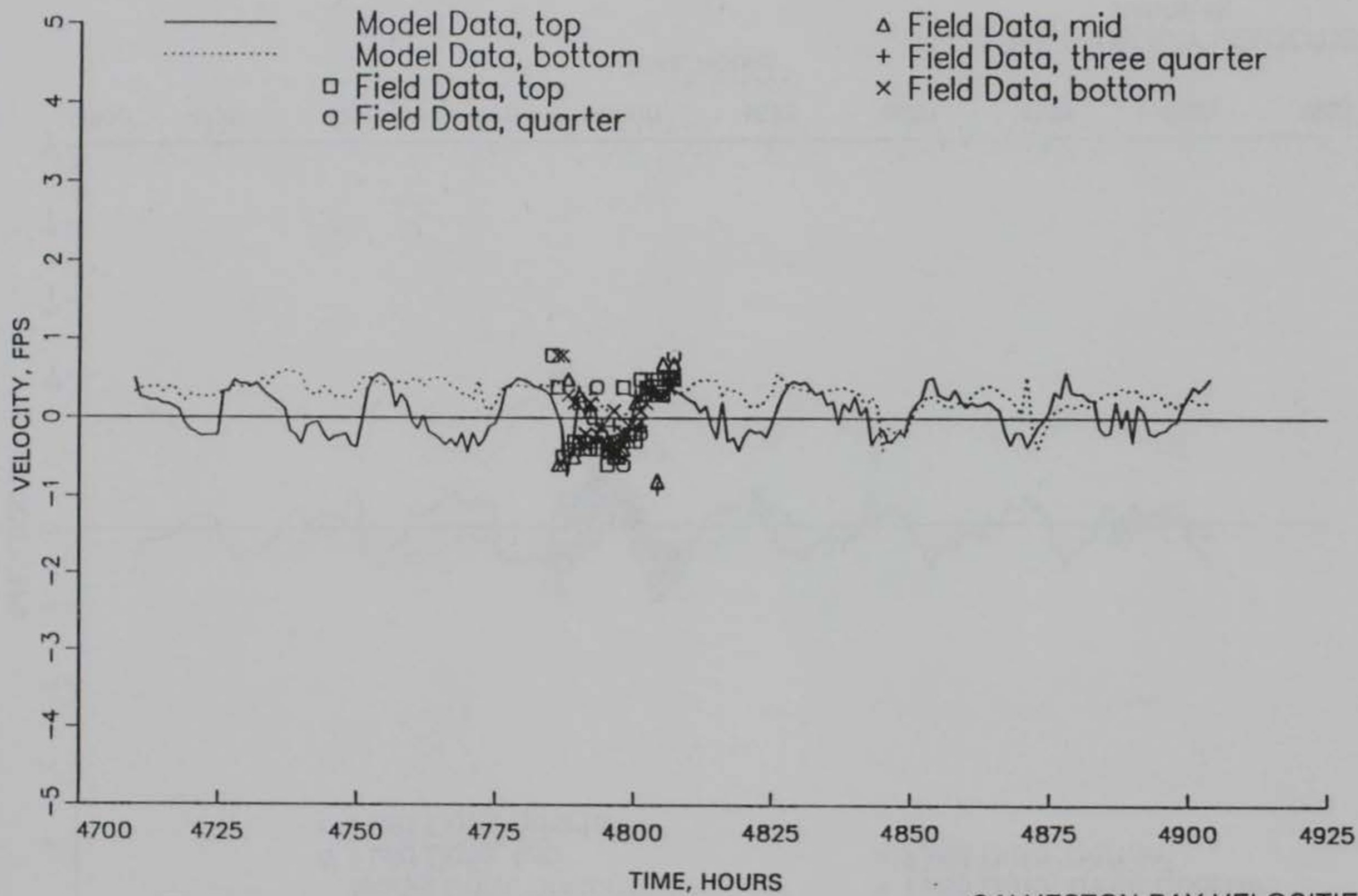
GALVESTON BAY VELOCITIES RANGE 4C
