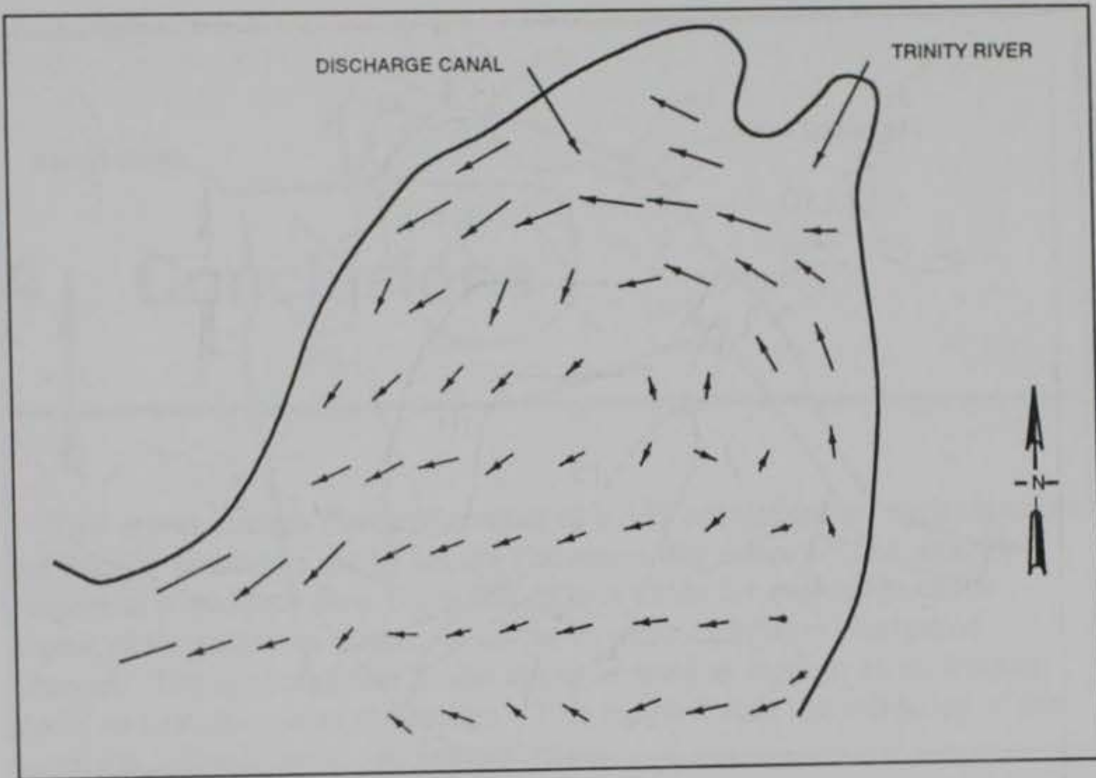
Figure 14. Monthly average May model surface velocity
