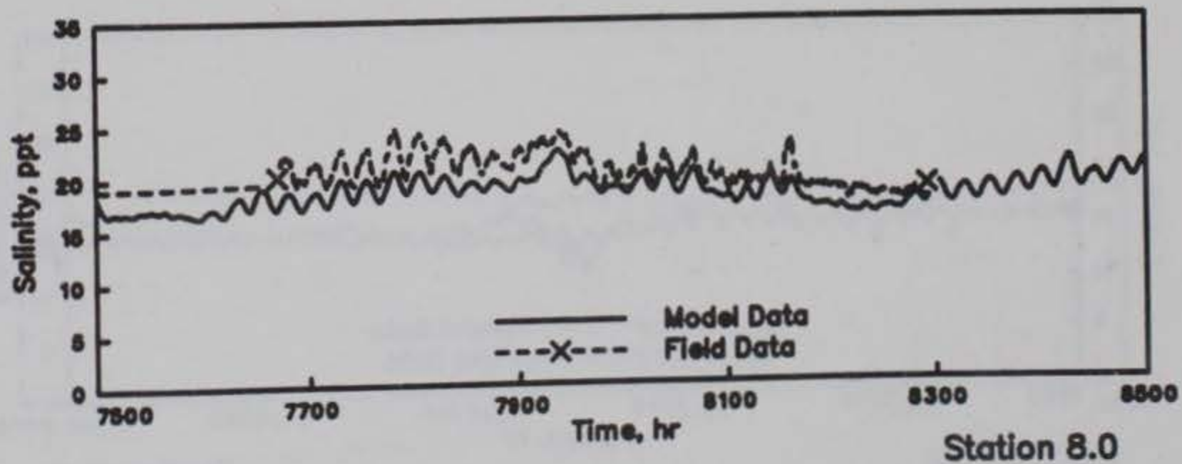
GALVESTON BAY SALINITIES MODEL VERIFICATION STATIONS 6.1t, 7.0, AND 8.0 HOURS 7500-8500
