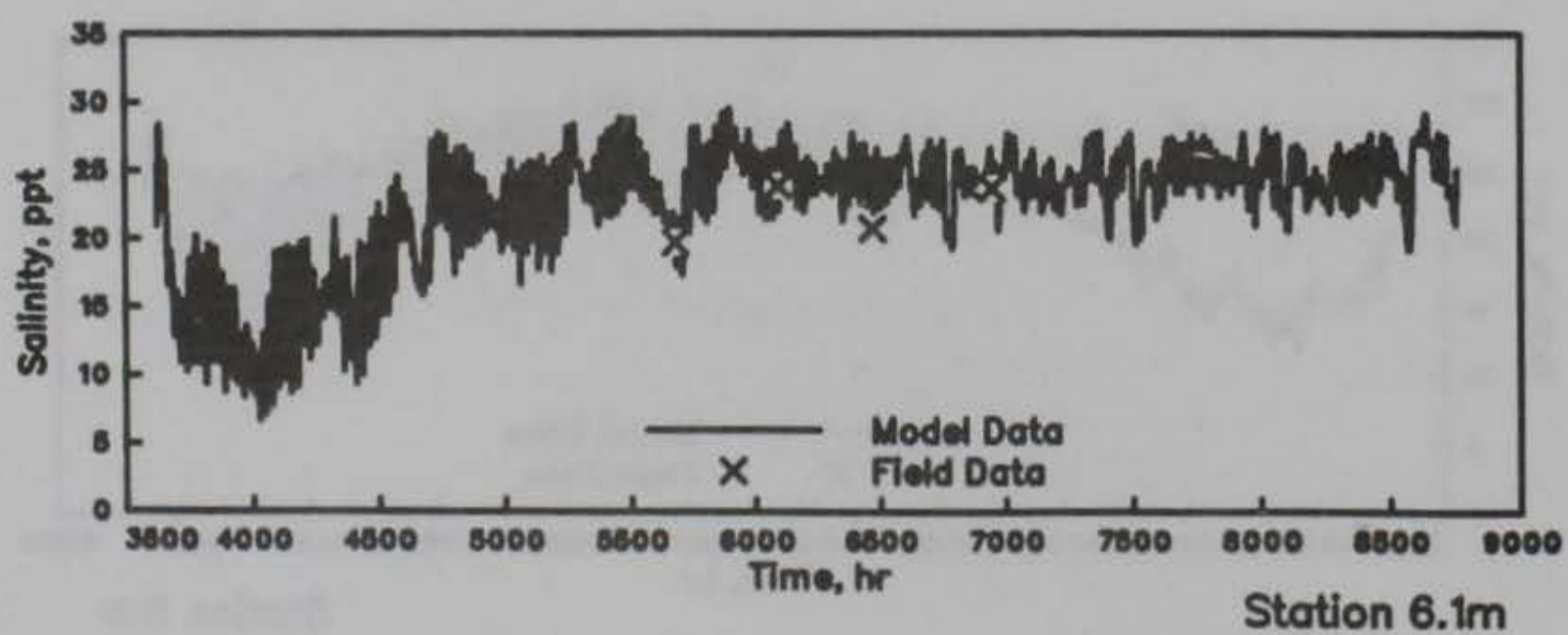
GALVESTON BAY SALINITIES, MODEL VERIFICATION STATIONS 6.0m, 6.0t, AND 6.1m HOURS 3500-9000
