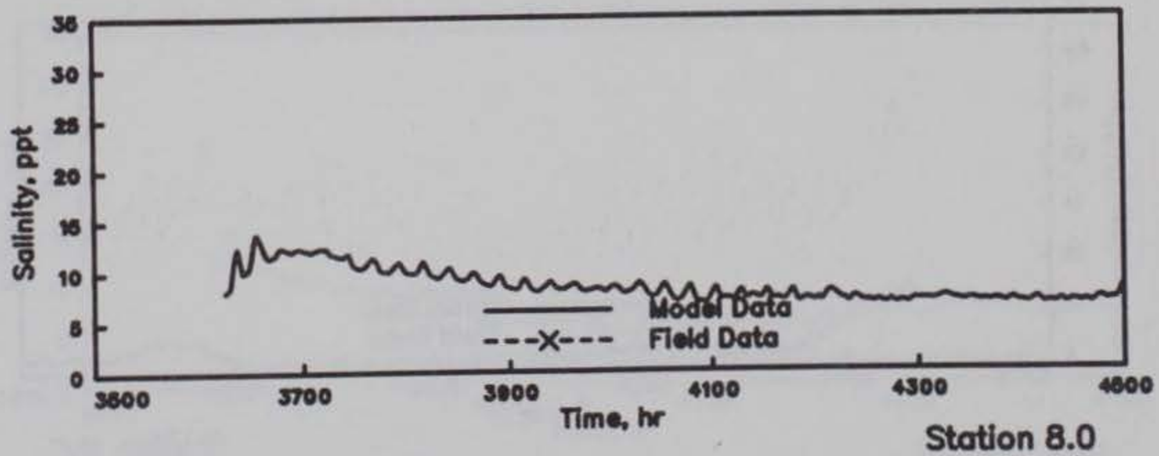
GALVESTON BAY SALINITIES MODEL VERIFICATION STATIONS 6.1t, 7.0, AND 8.0 HOURS 3500-4500
