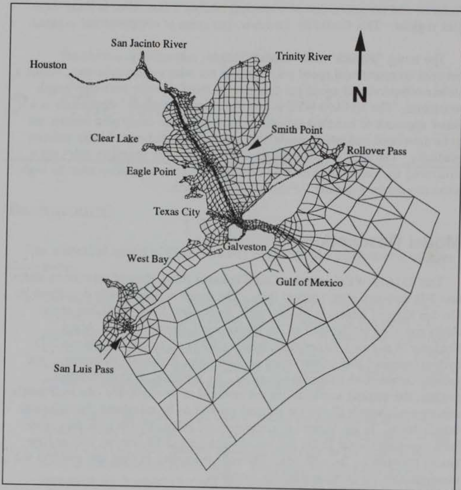
Figure 2. Mesh representing existing conditions
