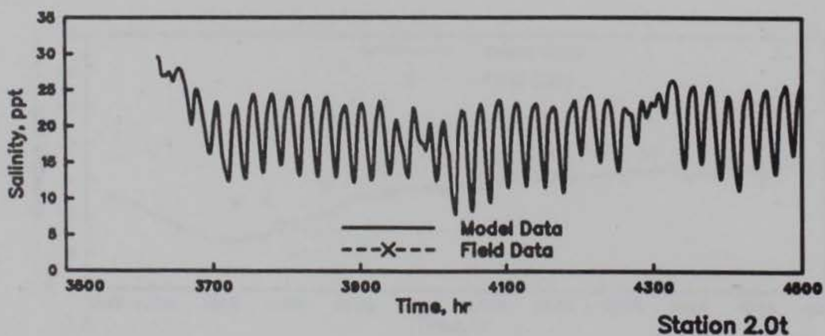
GALVESTON BAY SALINITIES MODEL VERIFICATION STATIONS 1.0, 2.0m, AND 2.0t HOURS 3500-4500
