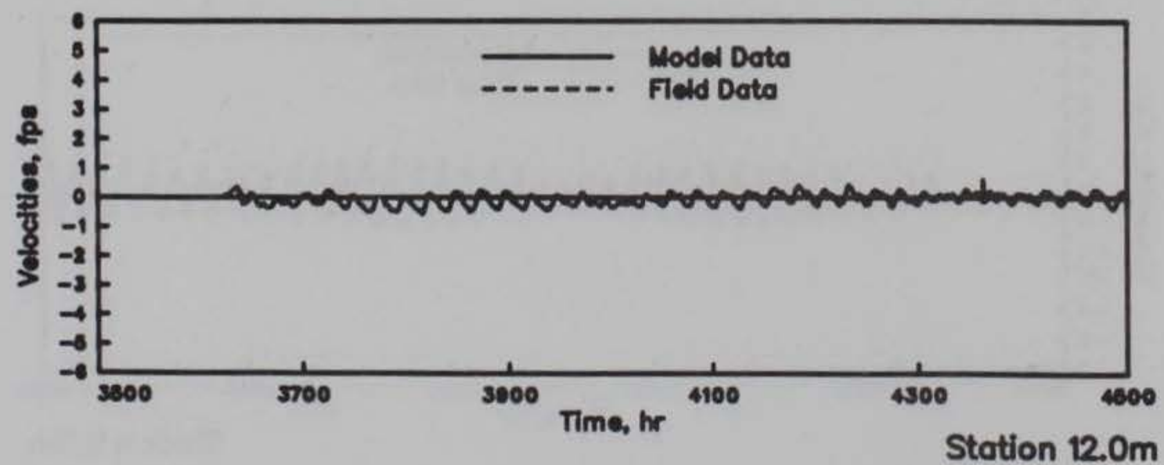
GALVESTON BAY VELOCITIES MODEL VERIFICATION STATIONS 9.0t, 11.1, AND 12.0m HOURS 3500-4500
