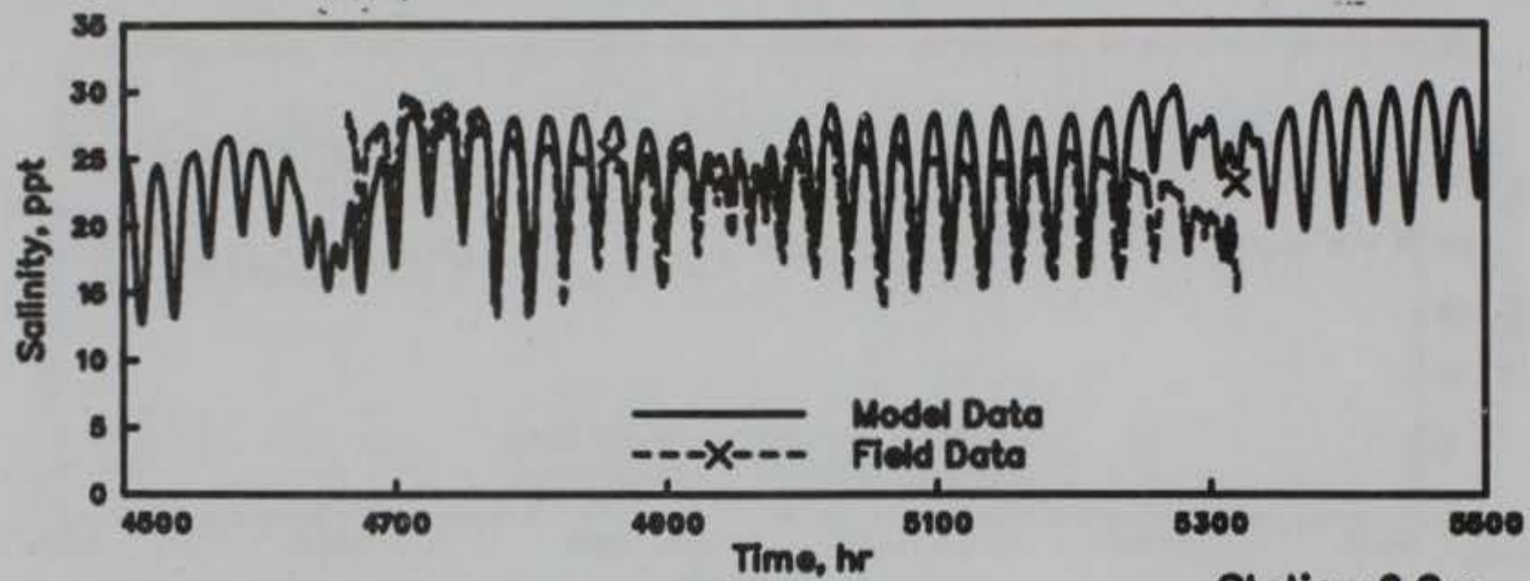
Station 6.0m
