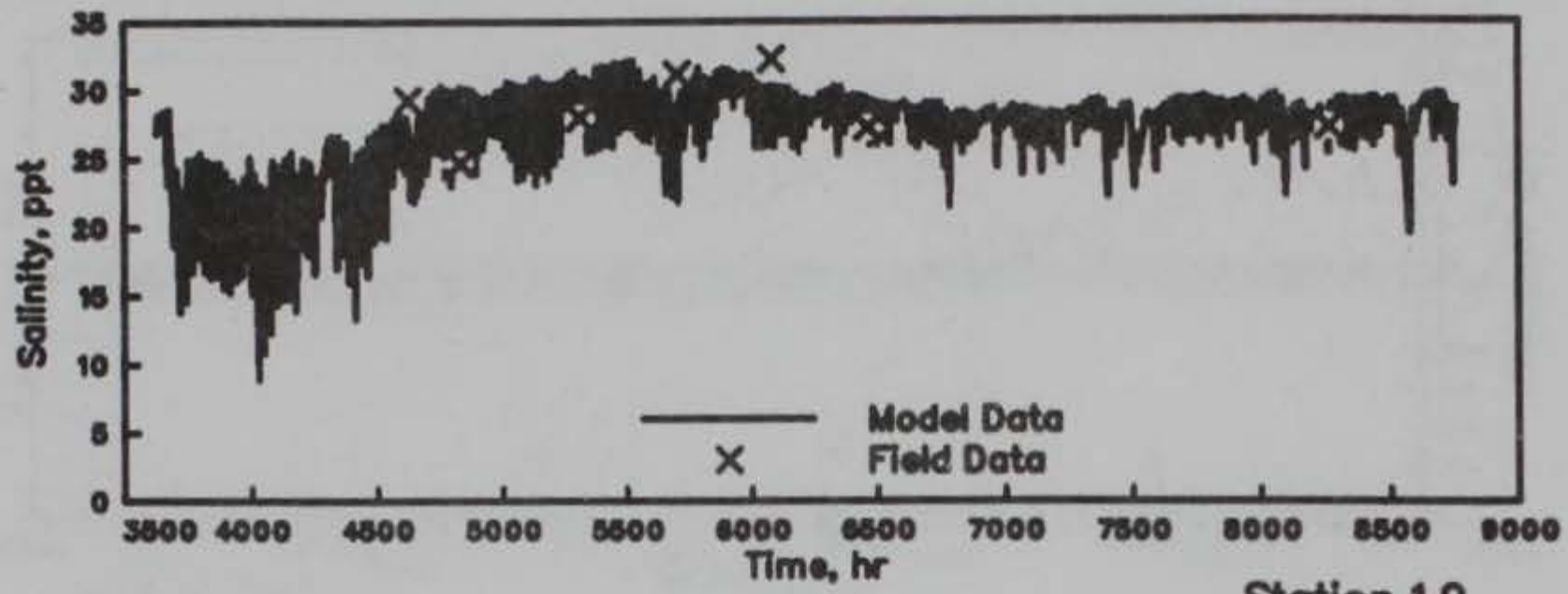
Station 1.0
