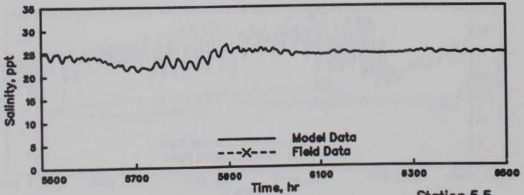
Station 5.5
