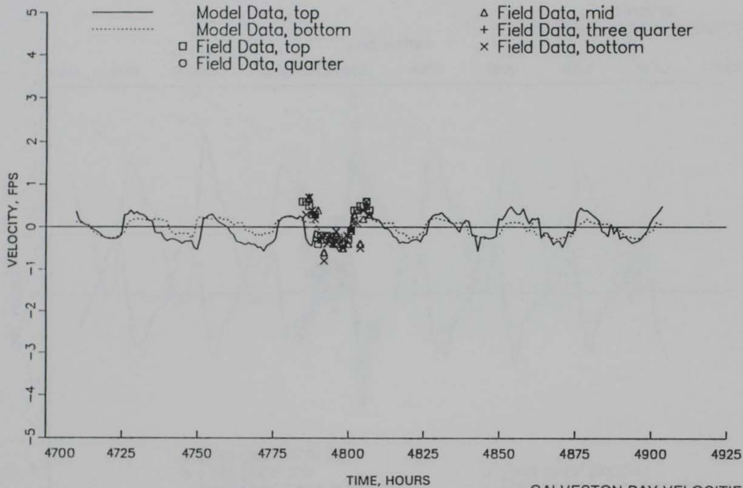
GALVESTON BAY VELOCITIES RANGE 4A
