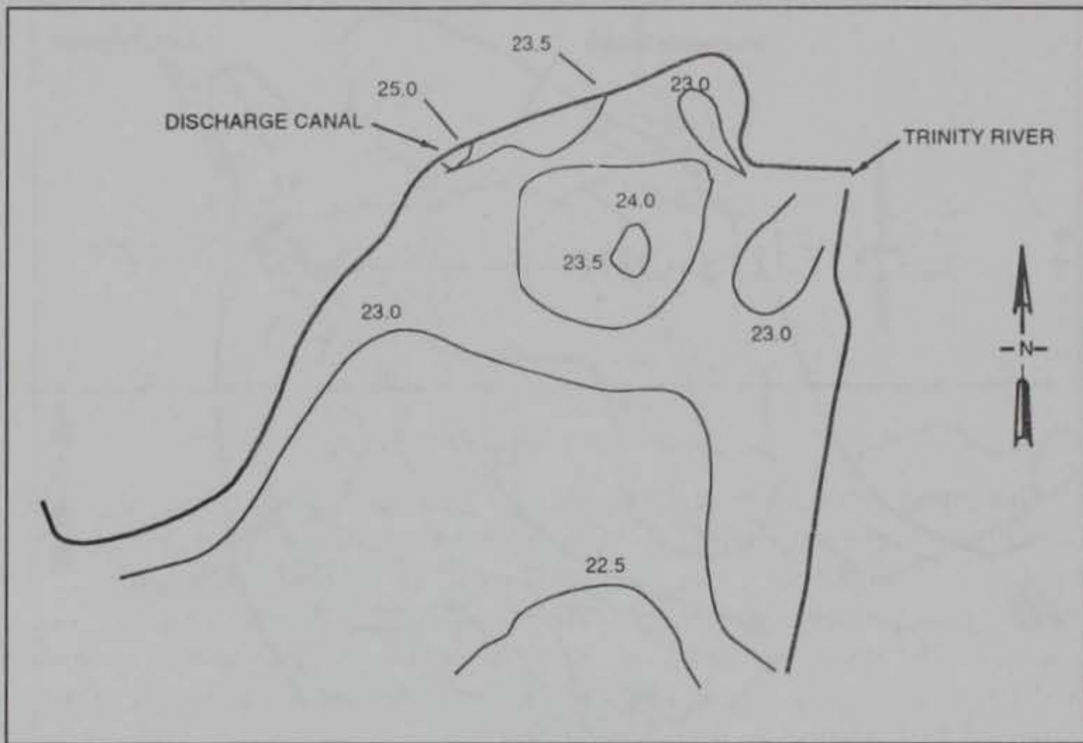
Figure 16. Temperature isohalines ( ^{\circ}\text{C} ) (from NASA 1971), May 1971
