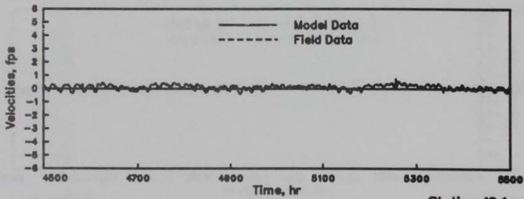
Station 12.1m
