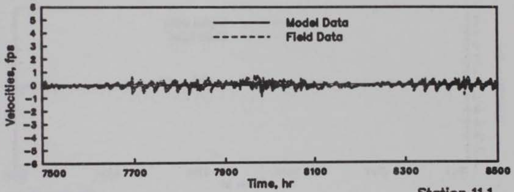
Station 11.1
