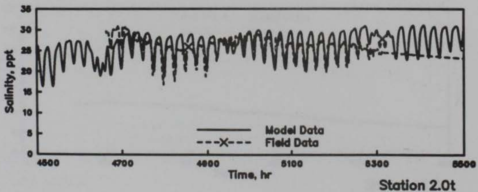
GALVESTON BAY SALINITIES MODEL VERIFICATION STATIONS 1.0, 2.0m, AND 2.0t HOURS 4500-5500
