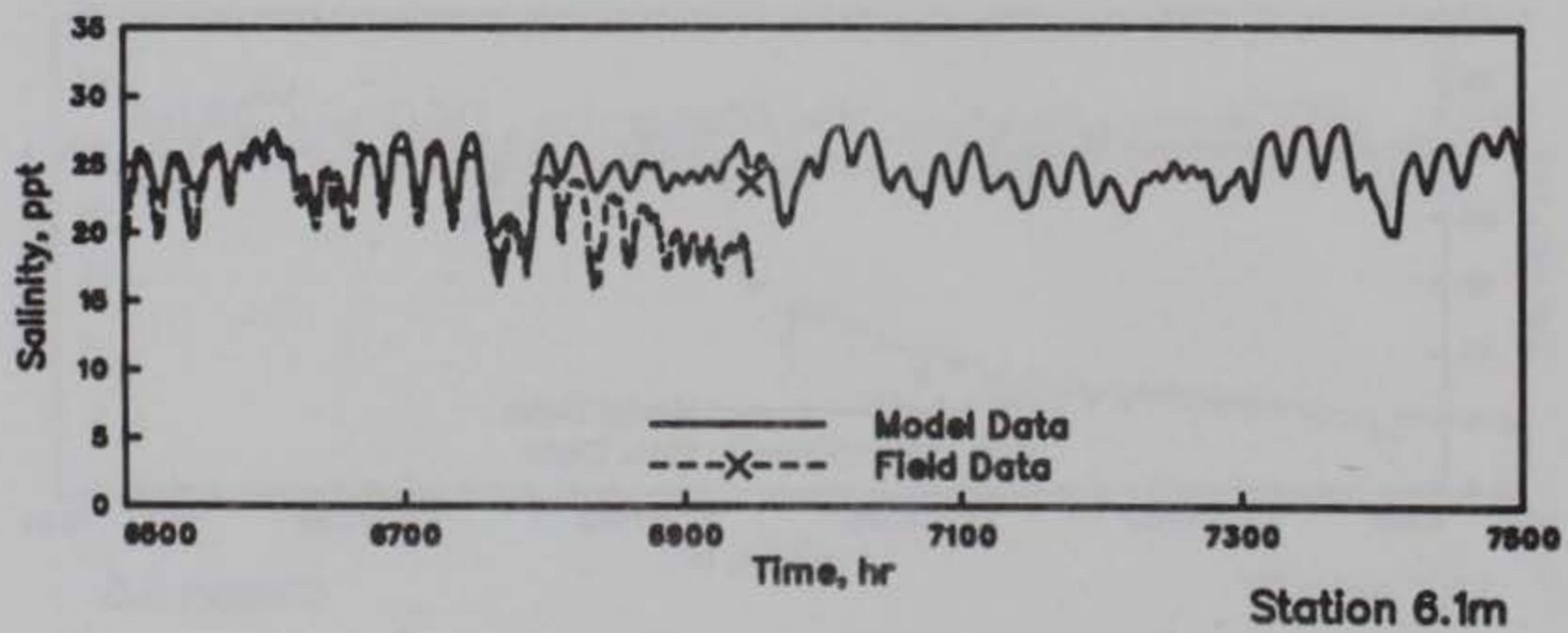
GALVESTON BAY SALINITIES MODEL VERIFICATION STATIONS 6.0m, 6.0t, AND 6.1m HOURS 6500-7500
