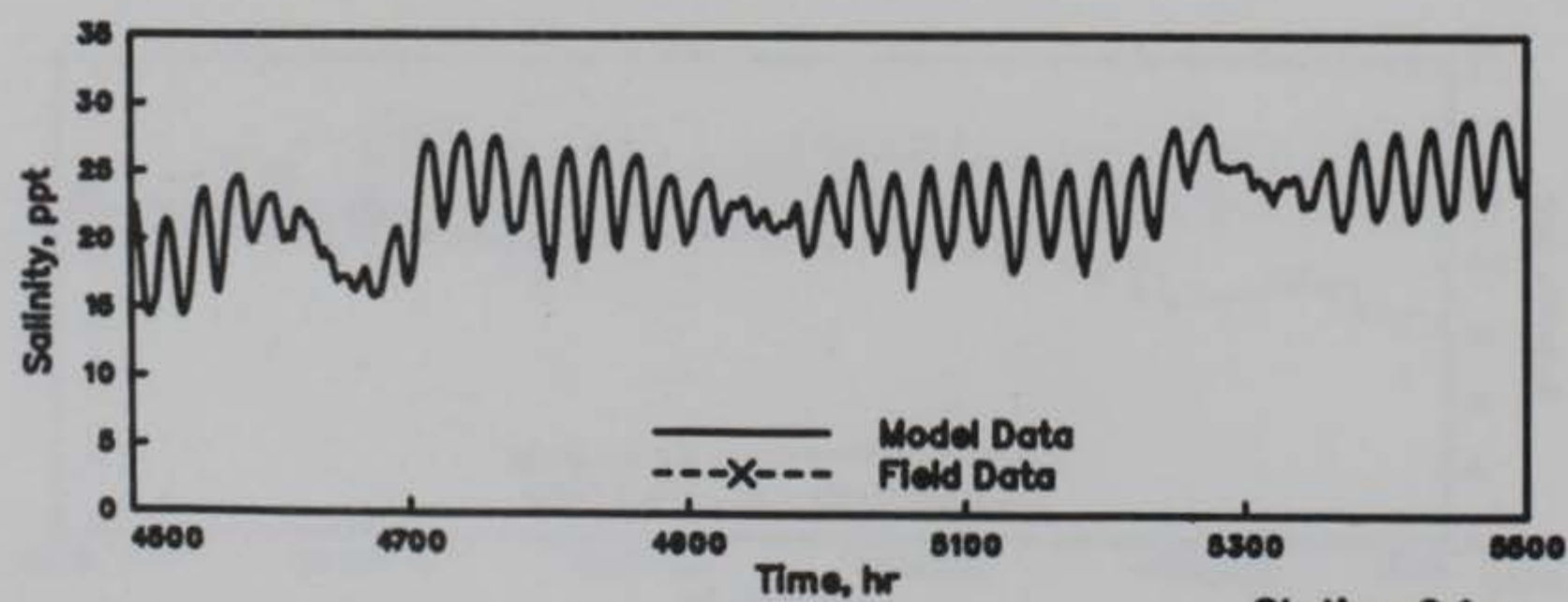
Station 6.1m
