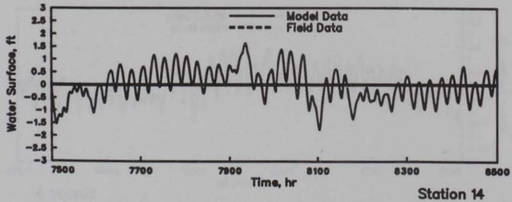
WATER-SURFACE ELEVATIONS MODEL VERIFICATION STATIONS 7, 10, AND 14 HOURS 7500-8500
