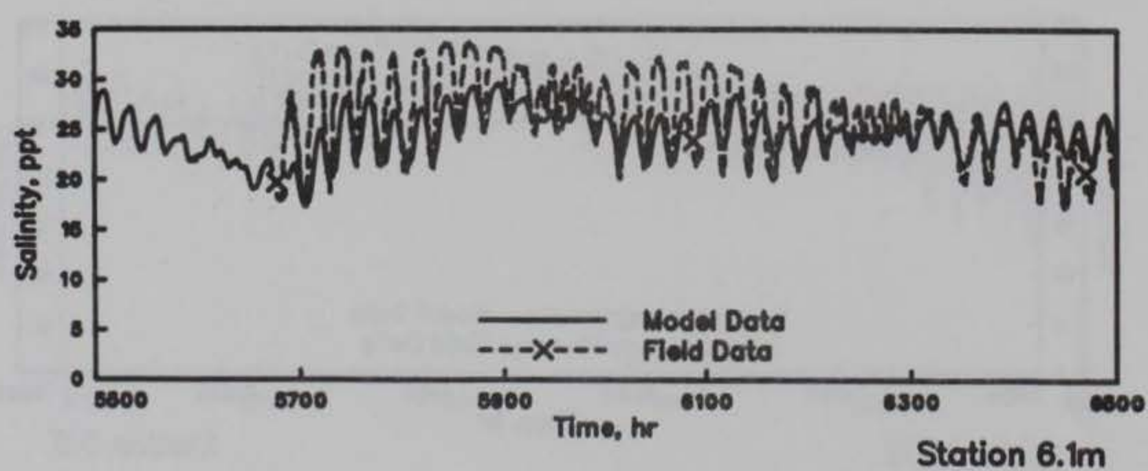
GALVESTON BAY SALINITIES MODEL VERIFICATION STATIONS 6.0m, 6.0t, AND 6.1m HOURS 5500-6500
