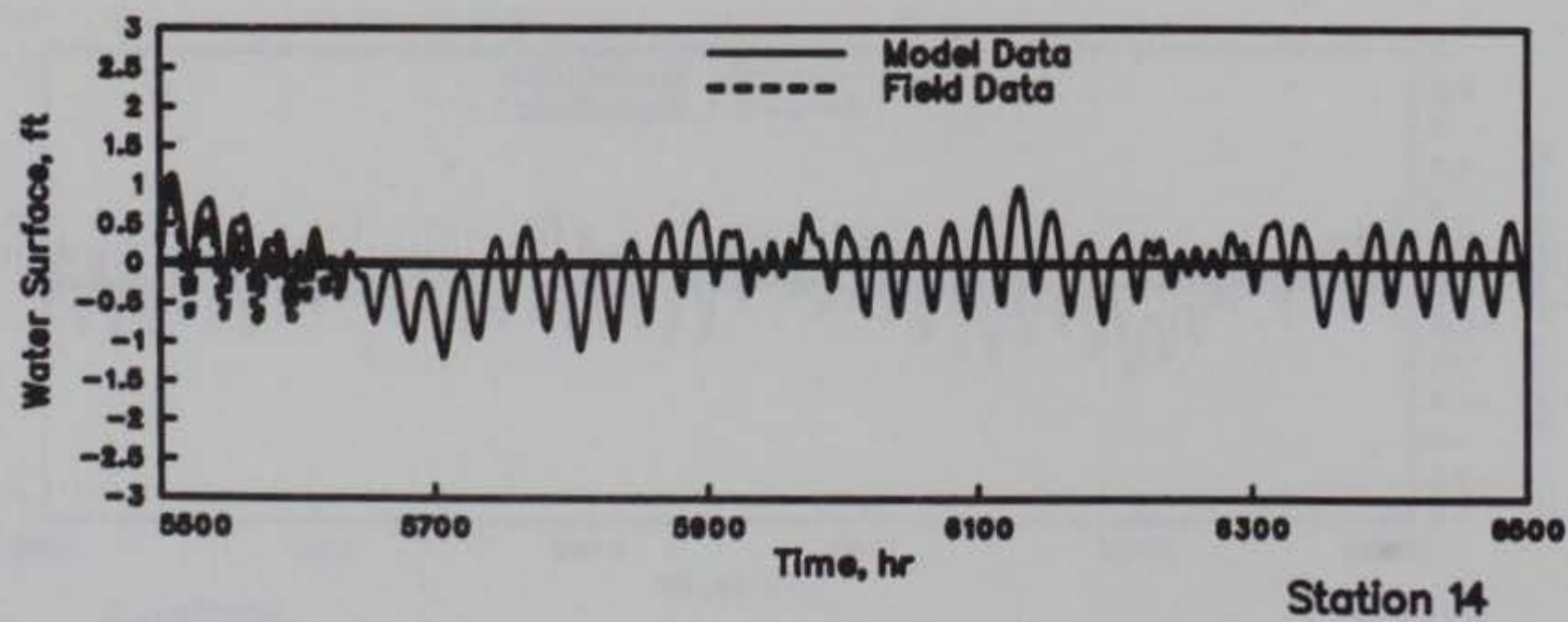
WATER-SURFACE ELEVATIONS MODEL VERIFICATION STATIONS 7, 10, AND 14 HOURS 5500-6500
