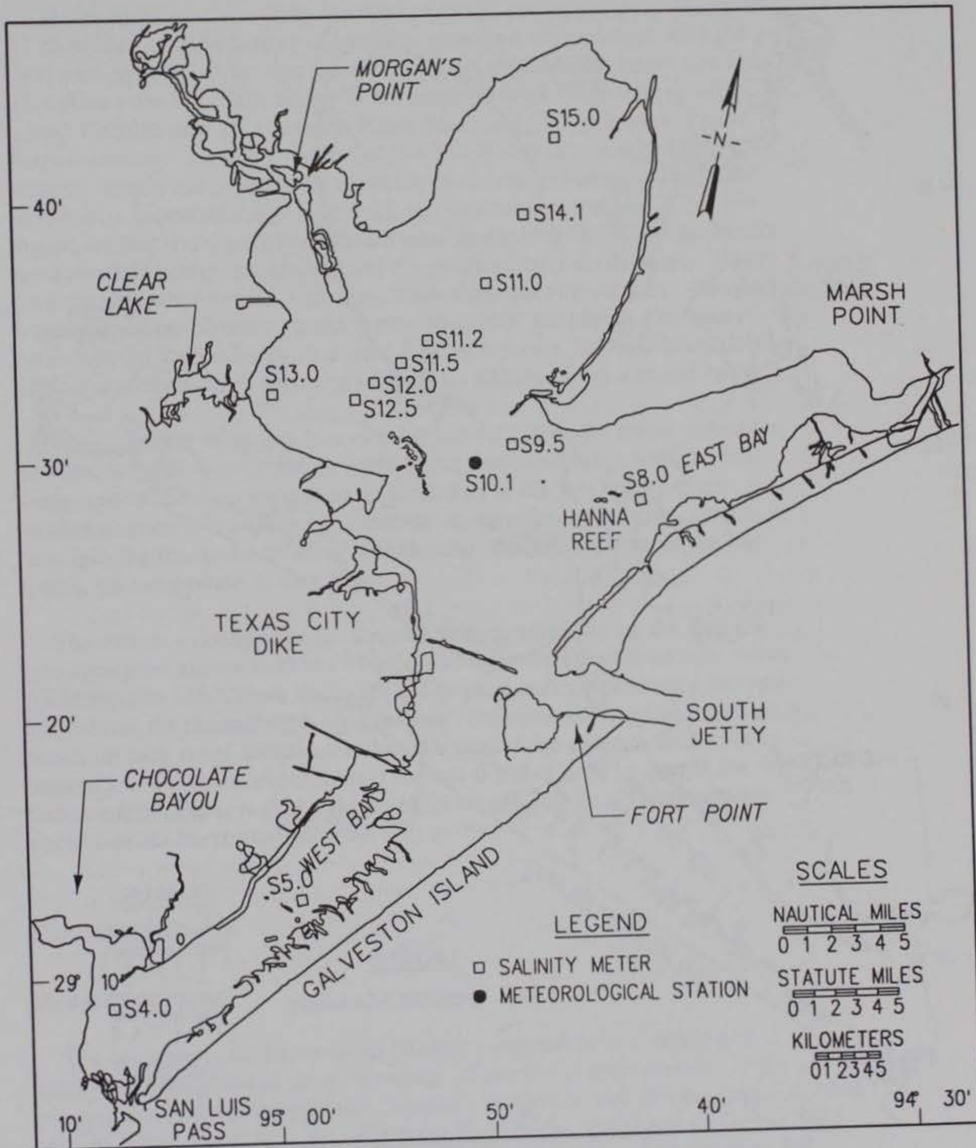
Figure 6. Supplementary long-term data collection equipment locations
