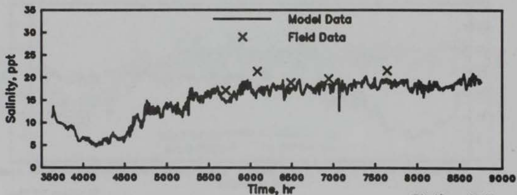
Station 12.1t
