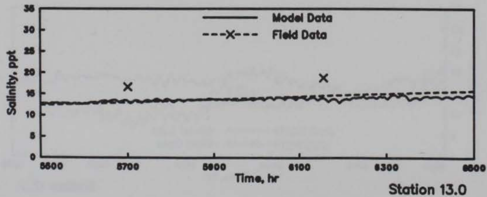
GALVESTON BAY SALINITIES MODEL VERIFICATION STATIONS 12.1m, 12.1t, AND 13.0 HOURS 5500-6500
