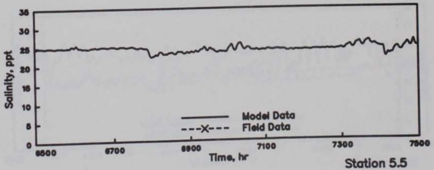
GALVESTON BAY SALINITIES MODEL VERIFICATION STATIONS 4.0, 5.0, AND 5.5 HOURS 6500-7500
