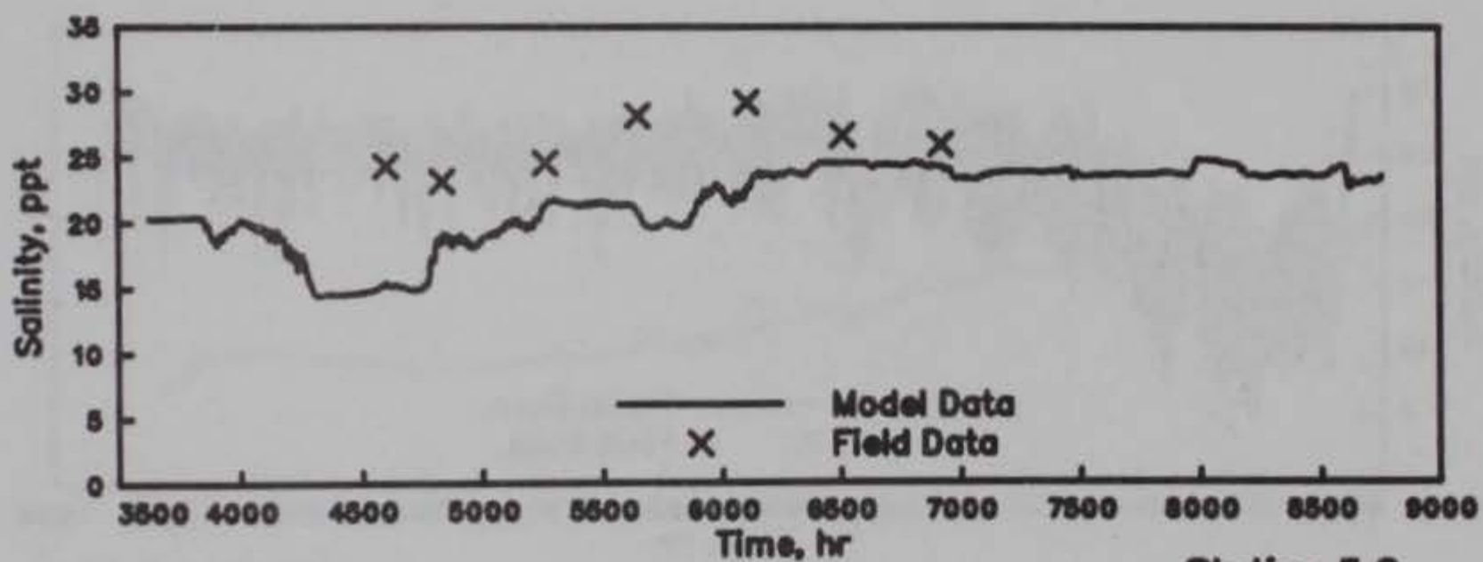
Station 5.0
