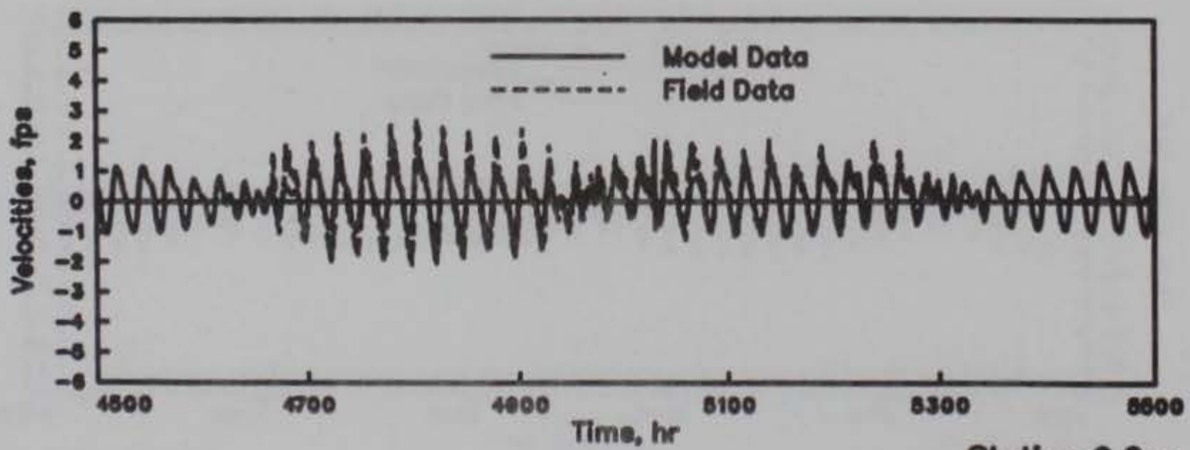
Station 9.0m
