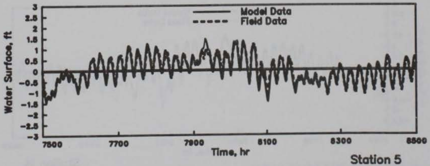
WATER-SURFACE ELEVATIONS MODEL VERIFICATION STATIONS 1, 3, AND 5 HOURS 7500-8500
