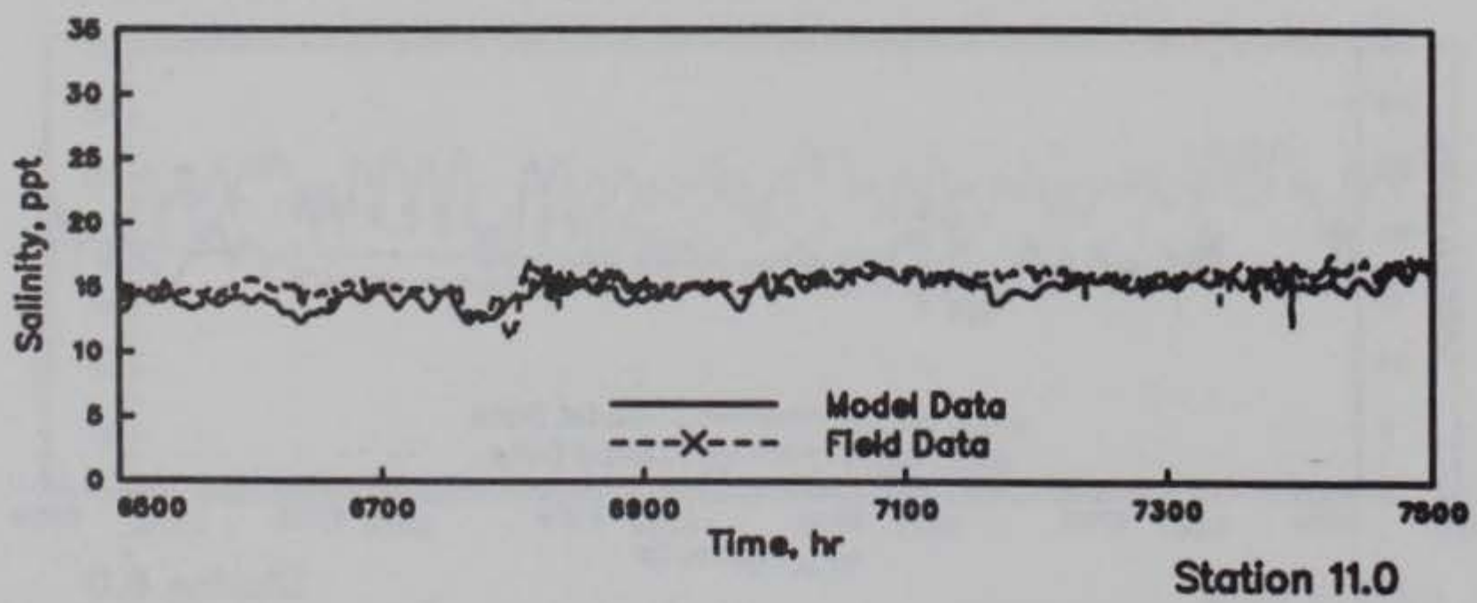
GALVESTON BAY SALINITIES MODEL VERIFICATION STATIONS 9.0m, 9.0t, AND 11.0 HOURS 6500-7500
