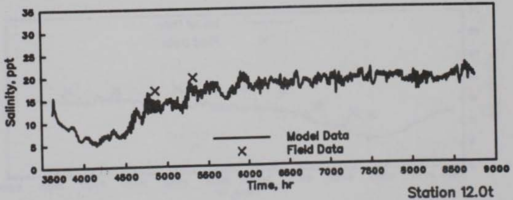
GALVESTON BAY SALINITIES MODEL VERIFICATION STATIONS 11.2, 12.0m, AND 12.0t HOURS 3500-9000
