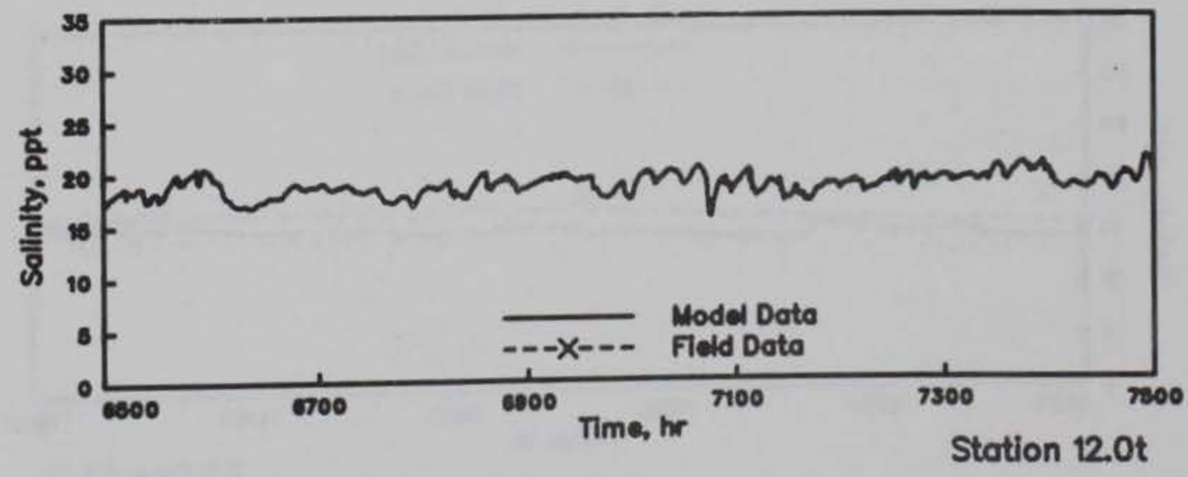
GALVESTON BAY SALINITIES MODEL VERIFICATION STATIONS 11.2, 12.0m, AND 12.0t HOURS 6500-7500
