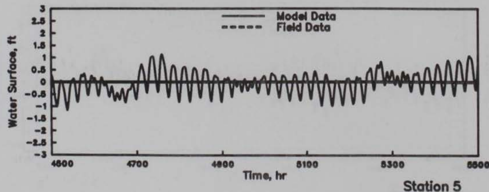
WATER-SURFACE ELEVATIONS MODEL VERIFICATION STATIONS 1, 3, AND 5 HOURS 4500-5500
