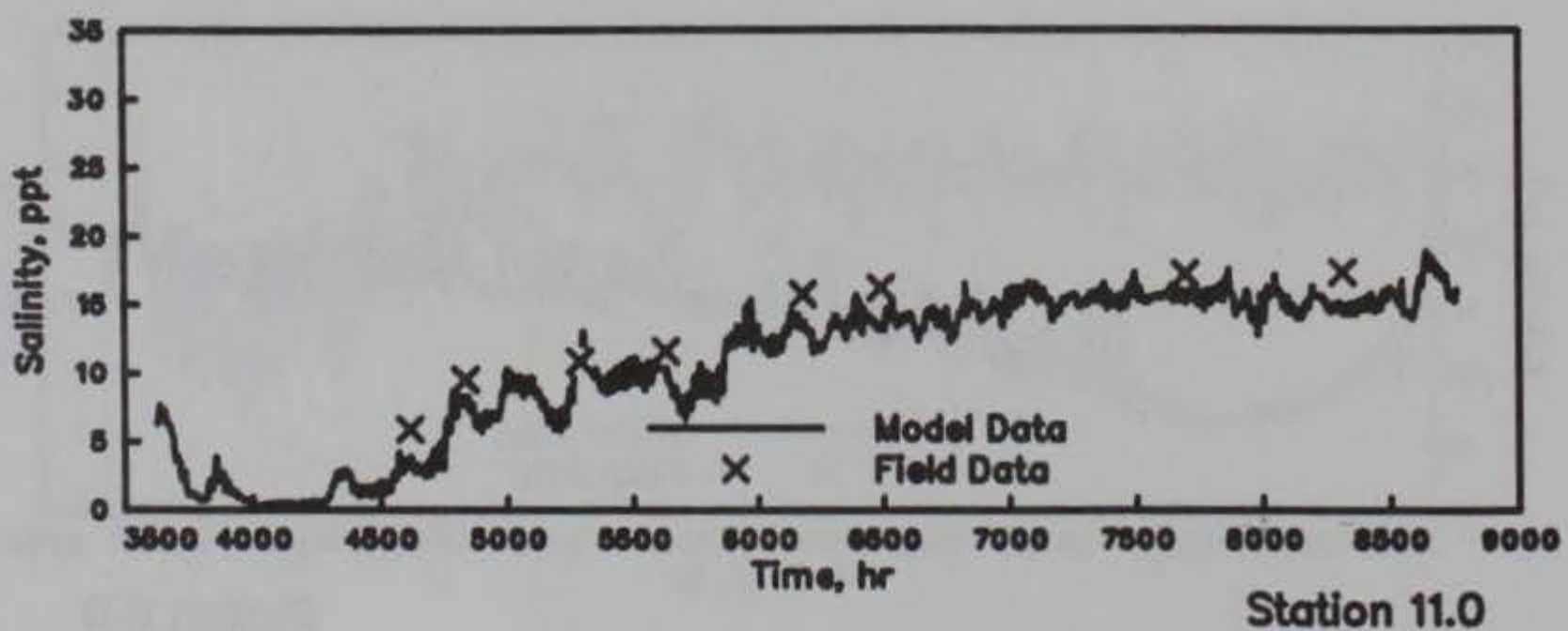
GALVESTON BAY SALINITIES MODEL VERIFICATION STATIONS 9.0m, 9.0t, AND 11.0 HOURS 3500-9000
