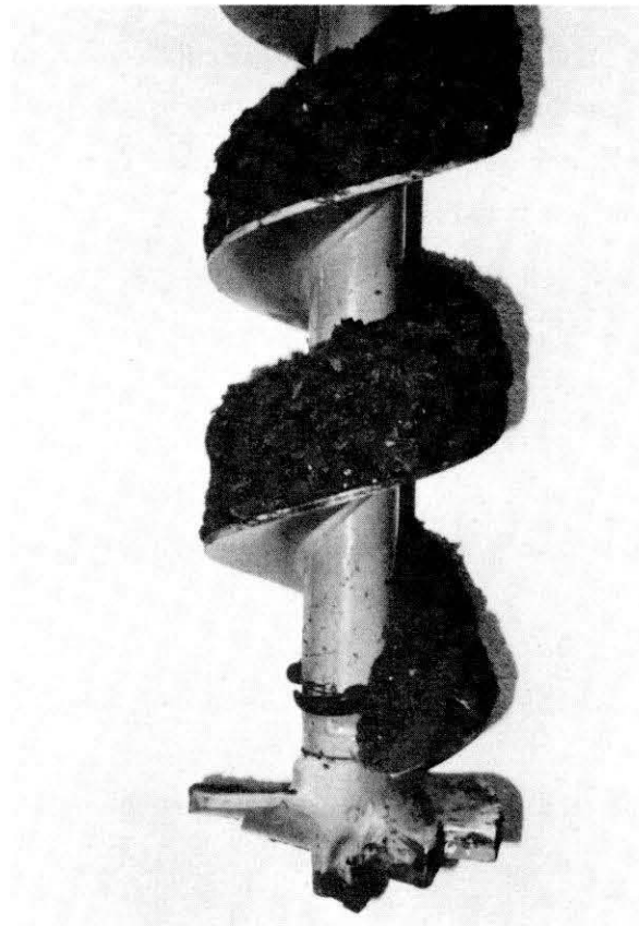
Figure 11. Cuttings remaining on the flight of the 9.5-in. auger after a period of rotation at 90 rpm.
