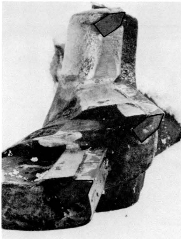
Figure 6. The 9.5-in. bit with minor modifications, including changing the carbides and some minor hand grinding to improve the relief angles.
