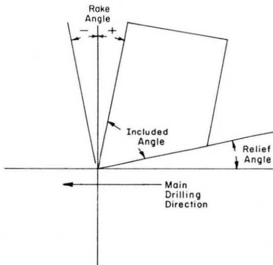
Figure 4. Carbide cutter showing the tool angles discussed in the text.
