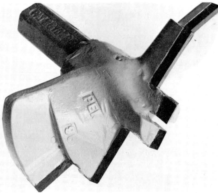
Figure 7. The 9.5-in. bit after modification, which included milling new carbide insert pockets and some grinding to streamline the cutting flow paths.
