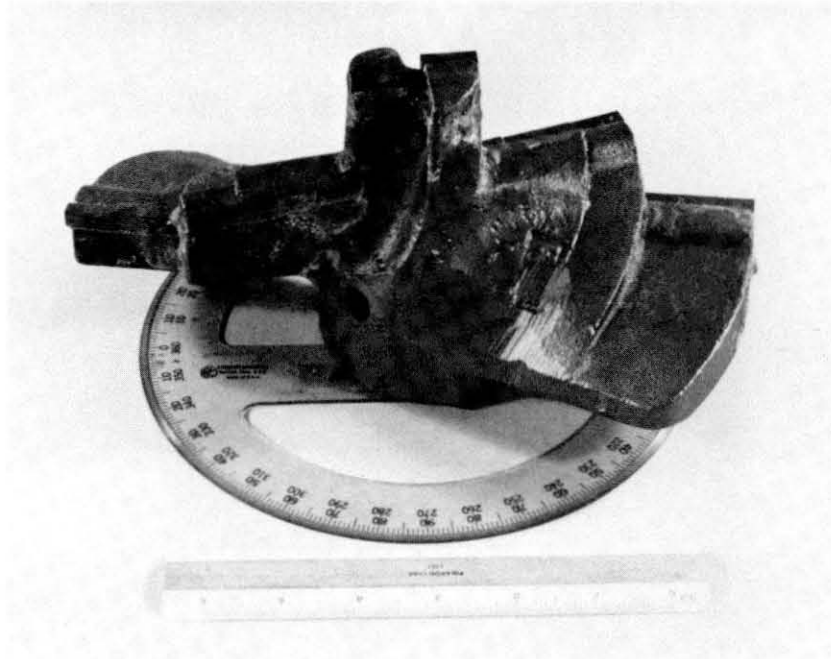
Figure 2. A Pengo Corporation TCH series 9.5-in.-diameter two-wing drag bit with step configuration and pilot.
