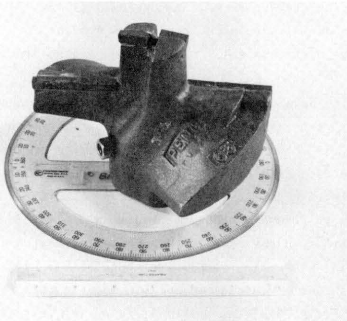
Figure 1. A Pengo Corporation TCH series 6.5-in.-diameter two-wing drag bit with pilot.
