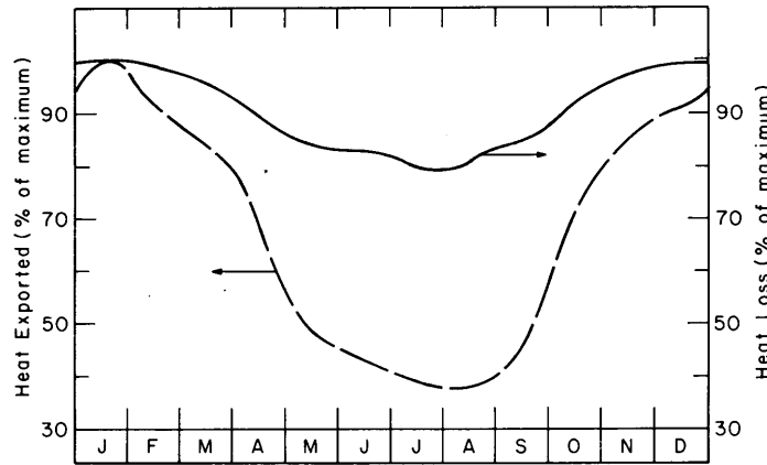
Figure 7. Normalized heat export and heat loss for 1978.
