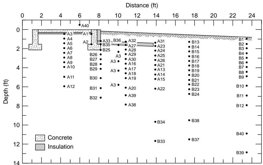
Figure 5. Location of temperature sensors.
