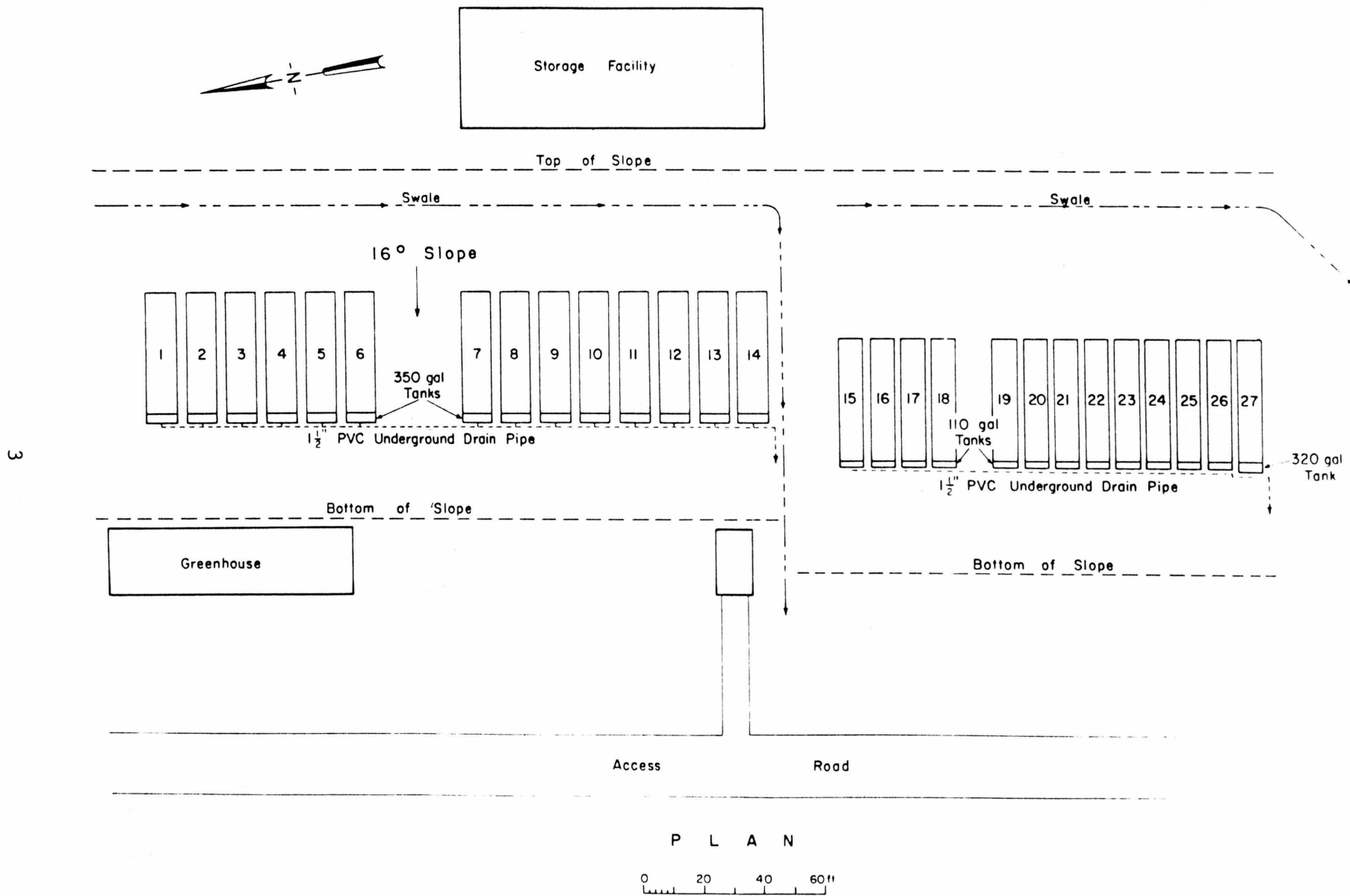
Figure 1. Plan of the 1975-76 stabilization study.
