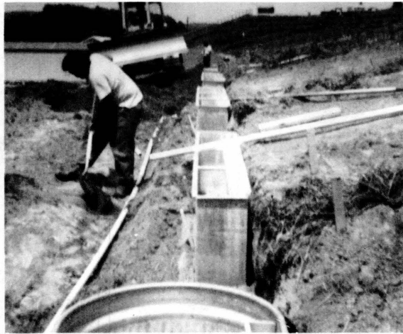
Figure 19. Replacing the sedimentation tanks with underdrains.
