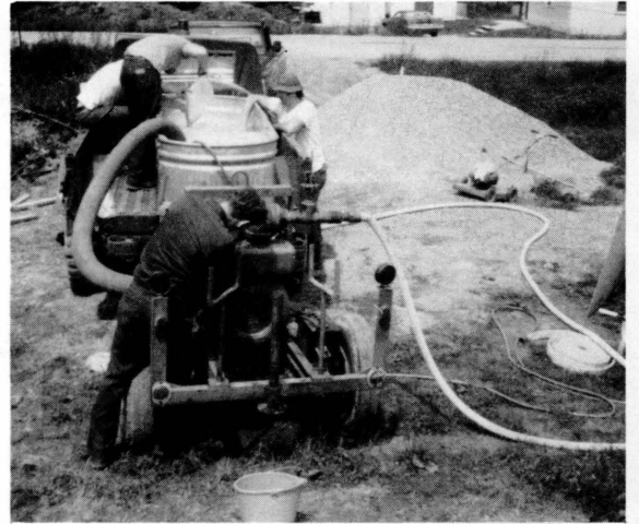
Figure 11. CRREL's homemade hydromulcher.
