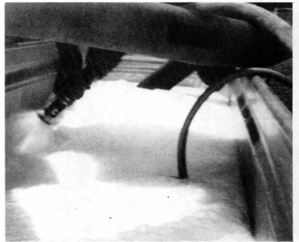
Figure 13. Mixing Curasol in hydromulcher.
