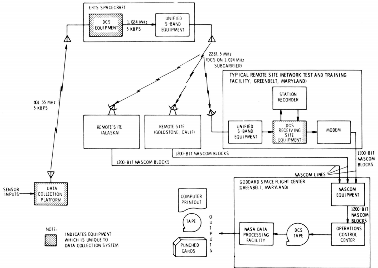
Figure 11a. LANDSAT-1 data collection system.
