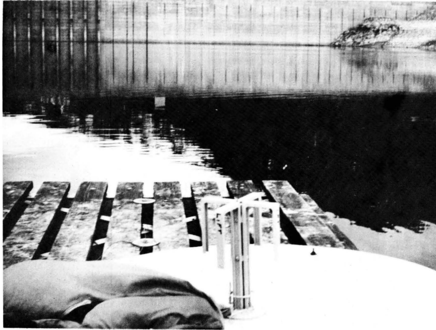
Figure 17. Floating DCP antenna and platform on Lake Koocanusa, Montana.
