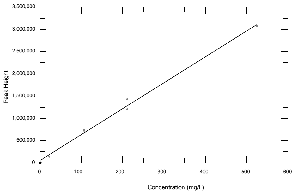
Figure 6. Initial calibration curve for the analysis of phenol by HPLC-UV.
