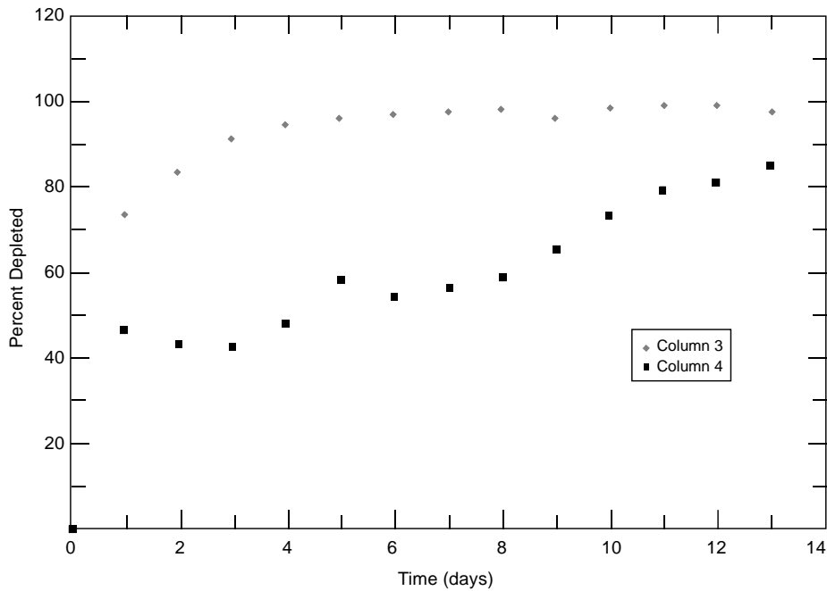
Figure 11. Remediation curve for TCE in water for round 2, columns 3 and 4.
