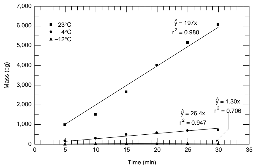
Figure 6. Mass of TNT vapor collected on polyacrylate SPME fiber at different temperatures.
