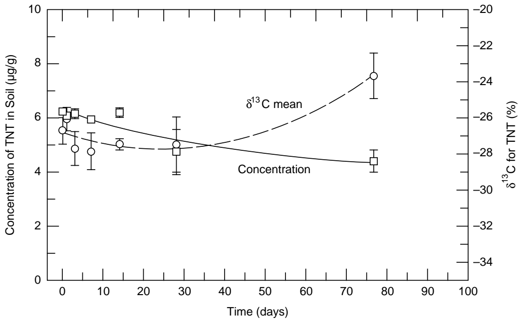
Figure 7. Concentration of TNT extracted from the soil and the \delta^{13}\text{C} value for extractable TNT over time for the experiment using LAAP soil.
