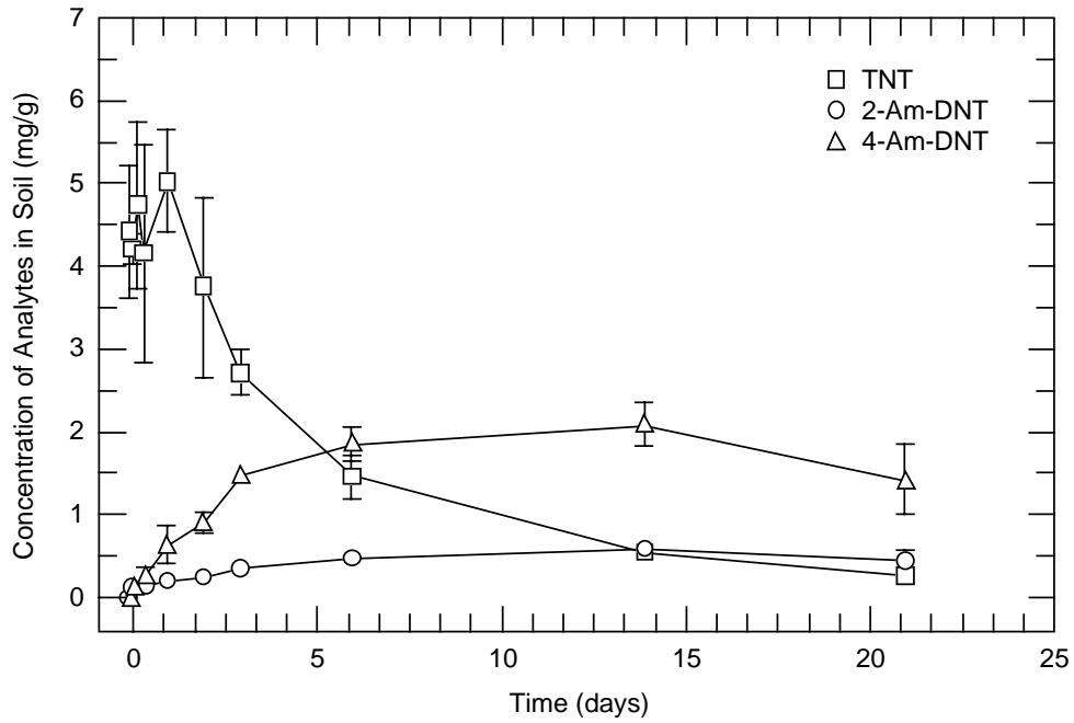
Figure 3. Concentration of TNT, 2ADNT, and 4ADNT over time for the experiment using Charlton soil.
