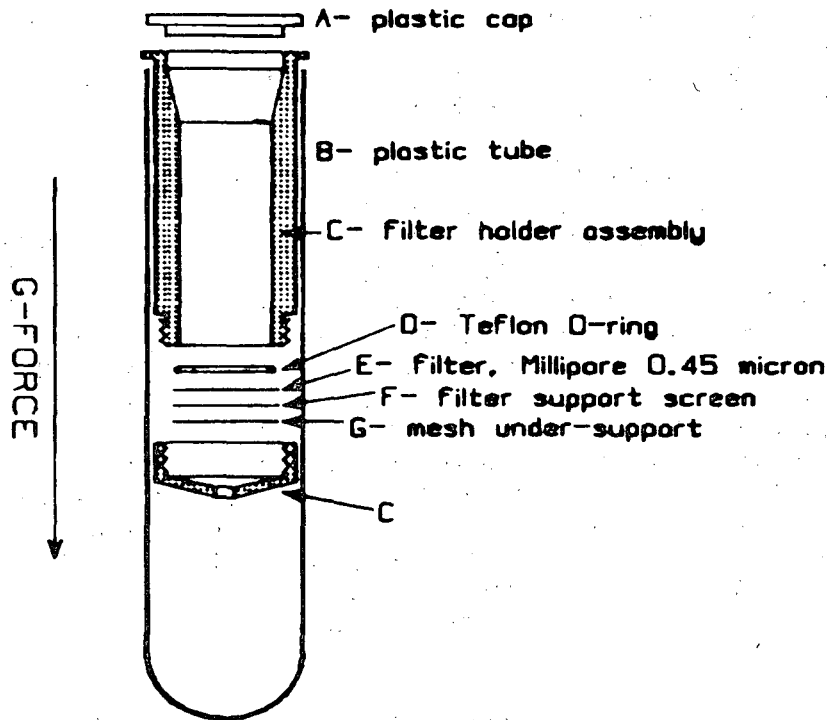
Figure 4. Filtering centrifuge apparatus.
