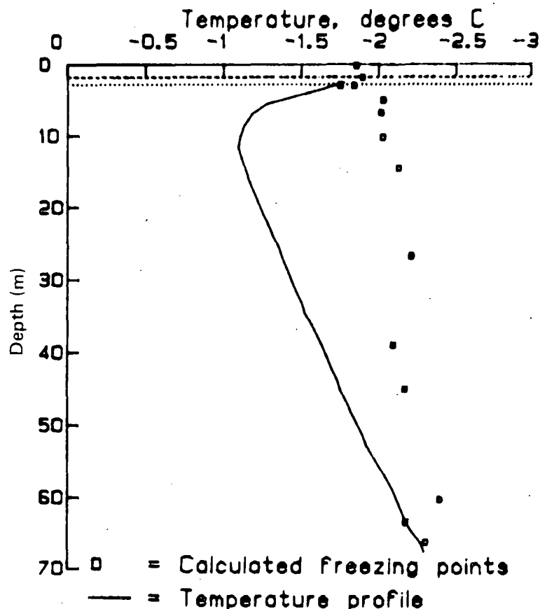
Figure 13. Temperature and calculated freezing points as a function of depth for borehole PB7 (Temperature data courtesy of B.V. Marshall and Dr. A.H. Lachenbruch, U.S.G.S.).
