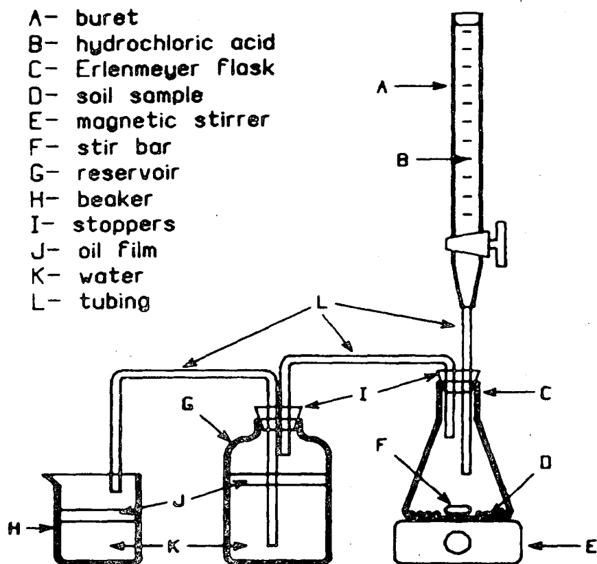
Figure 5. Apparatus used for calcium carbonate determinations.
