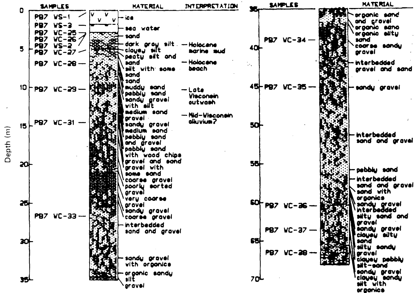
Figure 8. Preliminary log of borehole PB7 (Courtesy of Dr. D.M. Hopkins, and Roger Hartz, U.S.G.S.).
