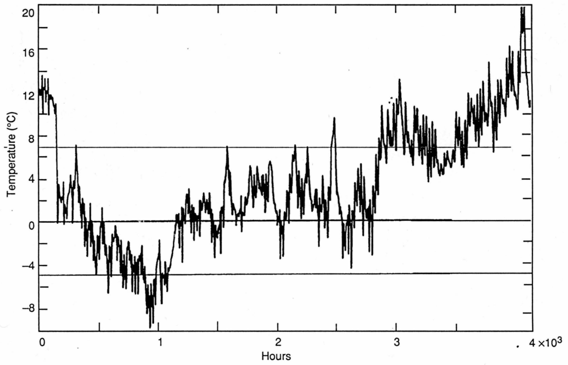
A6. Pavement temperature at 20.3 cm below upper surface.
