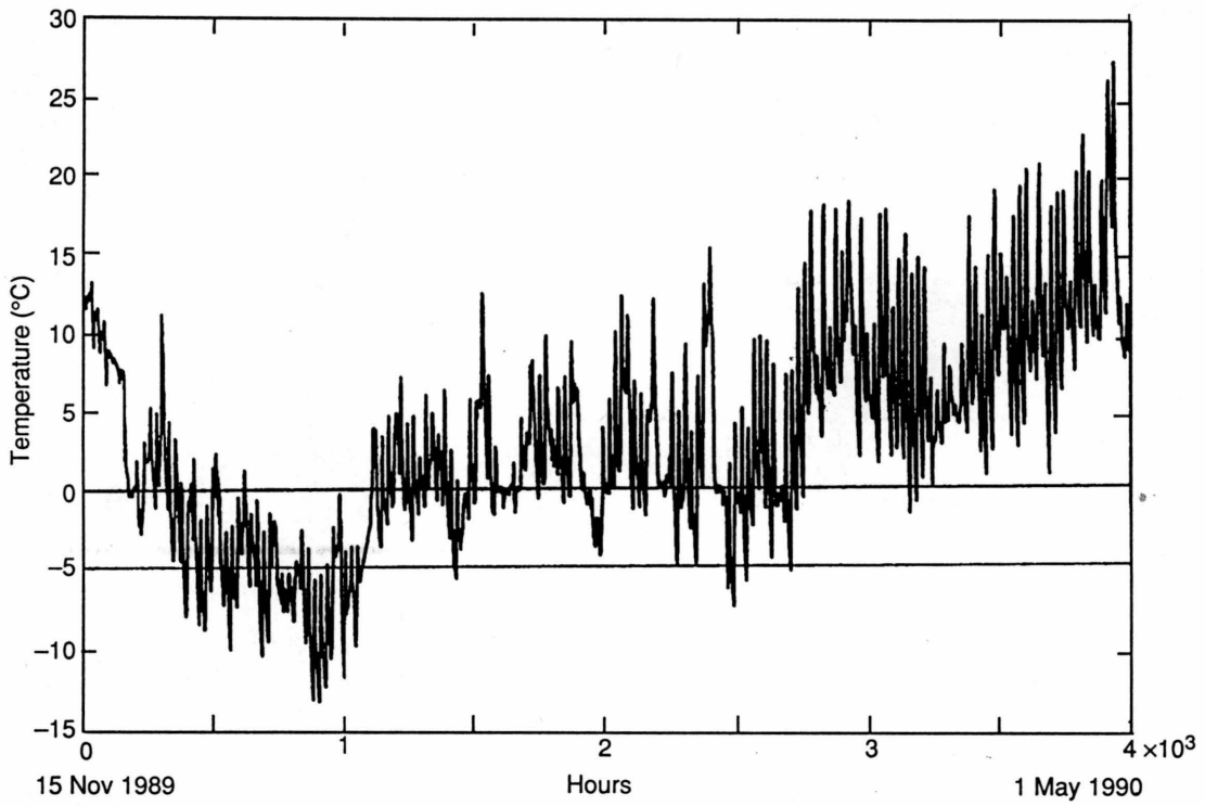
A2. RCC surface temperature.
