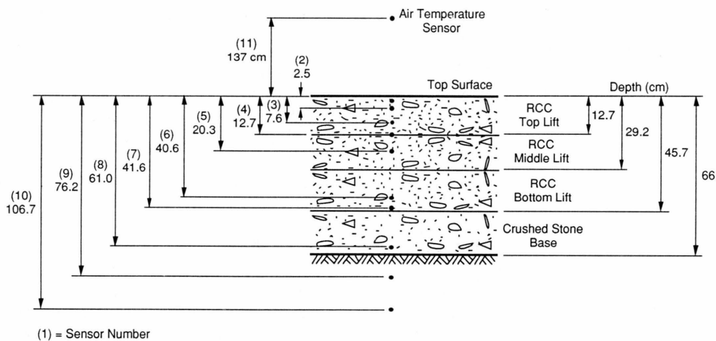
Figure 3. Thermocouple location.
