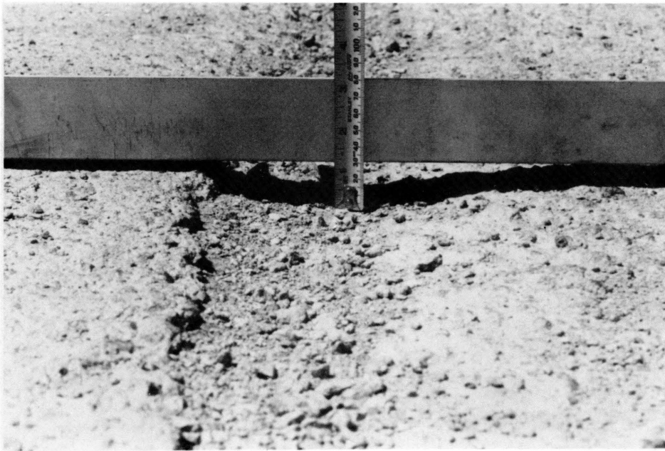
Figure 6. Loose pavement material at the vicinity of cold joints after one year of pavement service.
