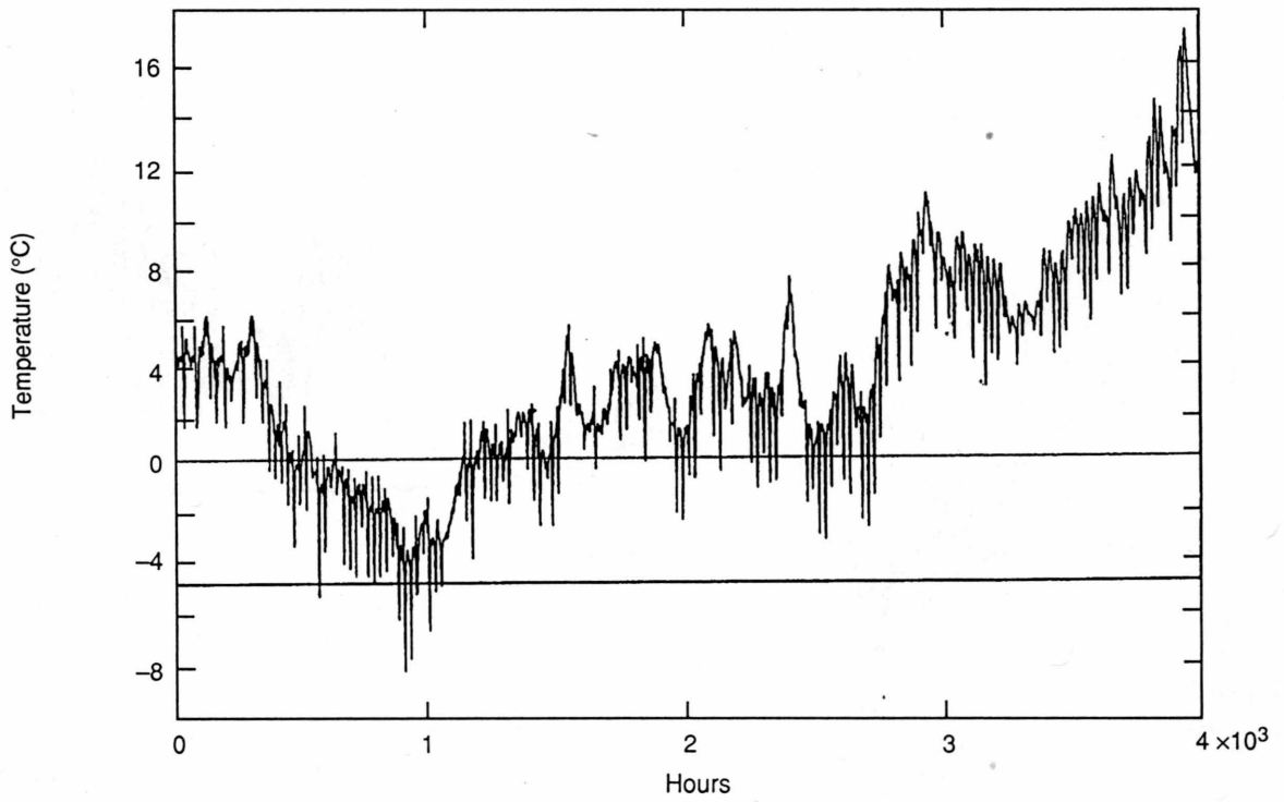
A7. Pavement temperature at 40.6 cm below upper surface.
