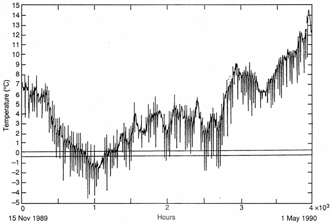
A9. Temperature at the crushed-stone base course.
