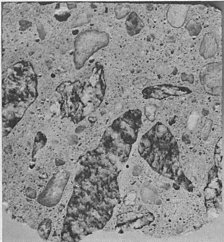
Photograph 1. Sawed and ground surface of concrete core II between 3.8 and 4.2 ft, about 1X. Several pieces of the black and white granite gneiss coarse aggregate show reaction rims believed to be due to alkali-silica reaction.
