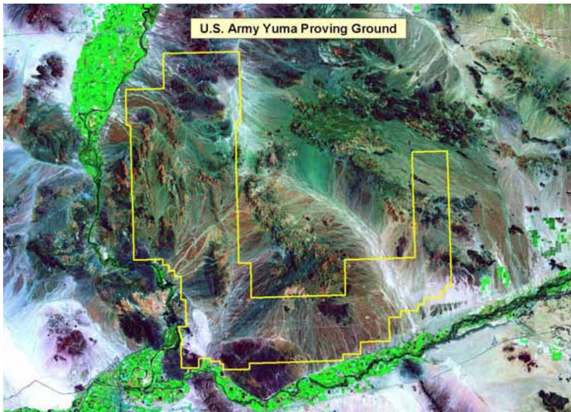
Figure 20. Landsat Thematic Mapper 7, 4, 2, color composite image of the Yuma Proving Ground.
