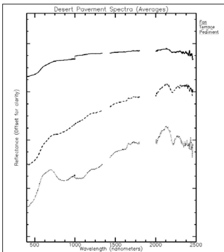
Figure 33. Field Spectra of desert pavement surfaces. With spectral contributions of eolian dust a constant, spectral variations in the 2000- to 2500-nm region show lithologic information. Reflectance (y-axis) is offset for clarity.
