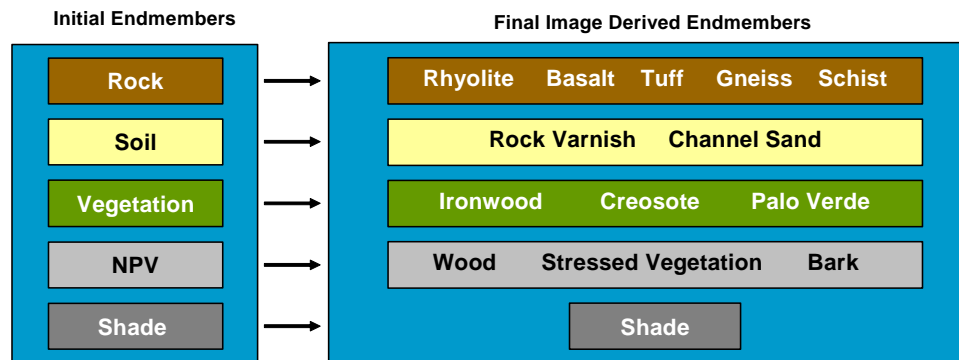
Figure 46. Initial and final image endmember extraction process.
