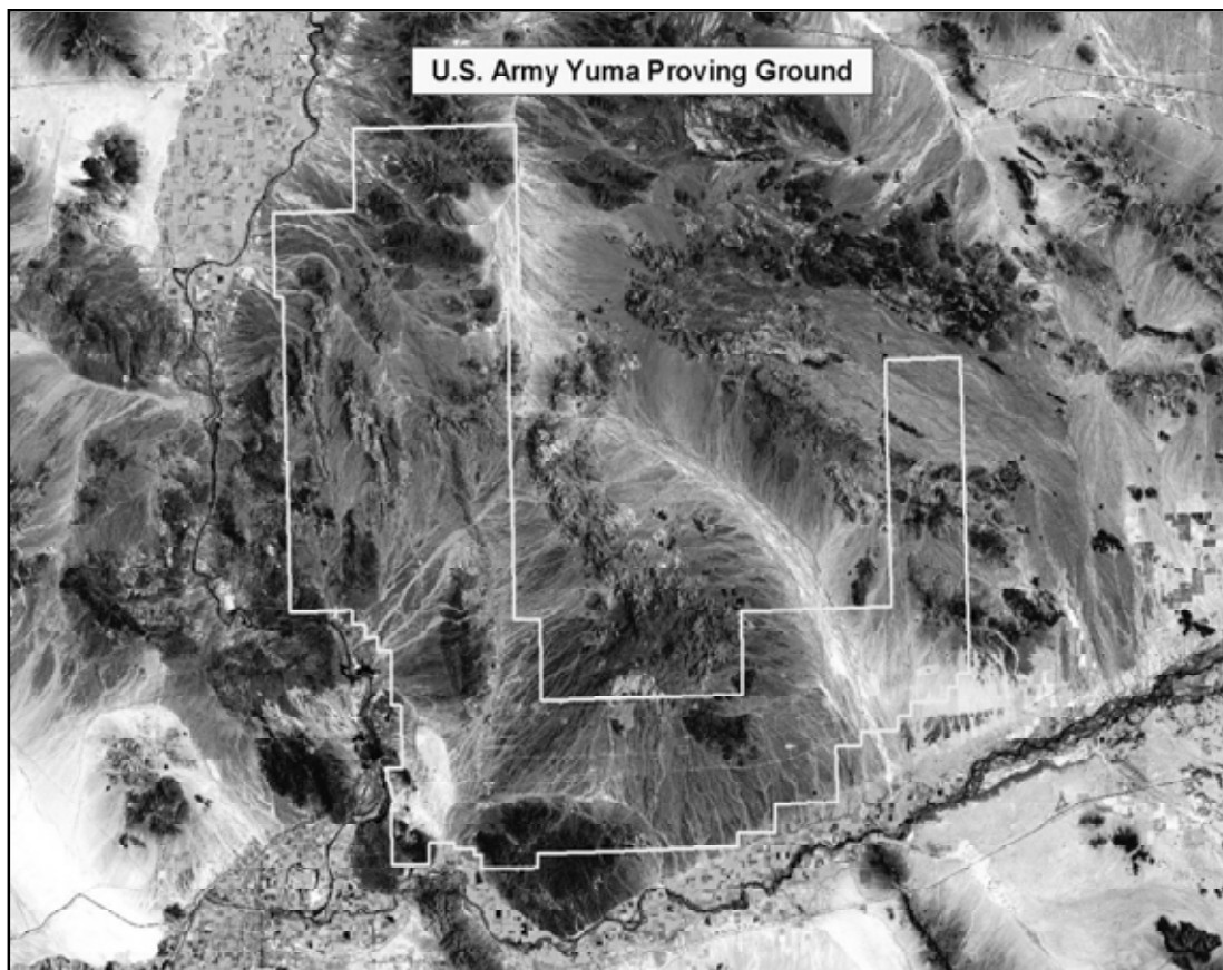
Figure 1. Landsat Thematic Mapper image of the Yuma Proving Ground. This image is centered on geographic coordinates N 33°11' 00", W 114°7' 32".
