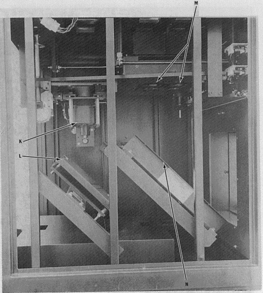
Figure 6. Viewer/Projector Internal View
