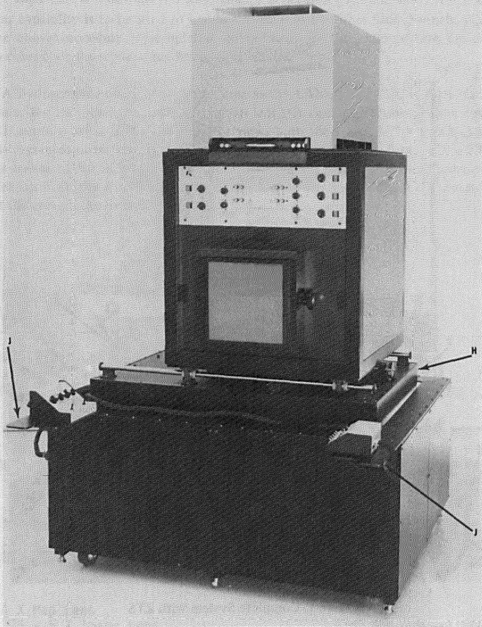
Figure 2. Viewer Projector and Base
