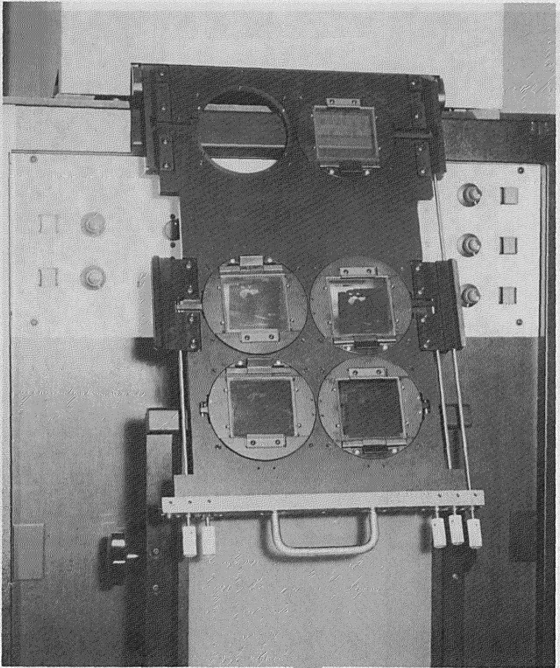
Figure 8. Theta Plate with Photographic Images
