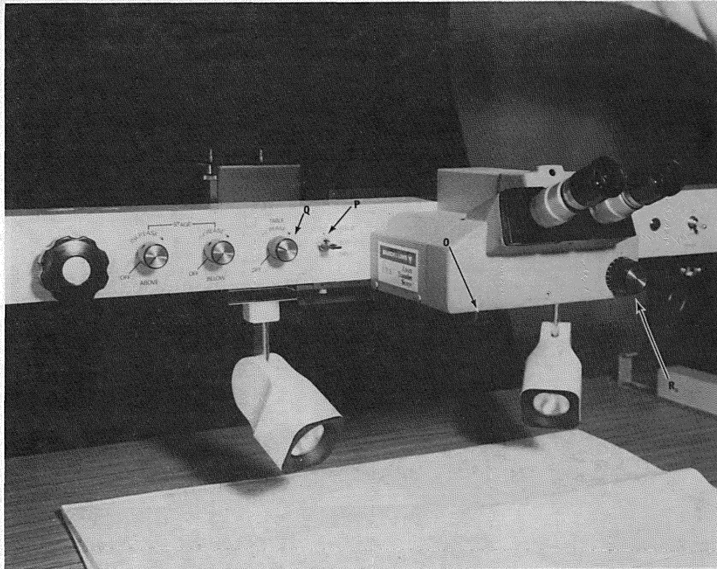
Figure 11. ZTS Stereo Viewing and Controls
