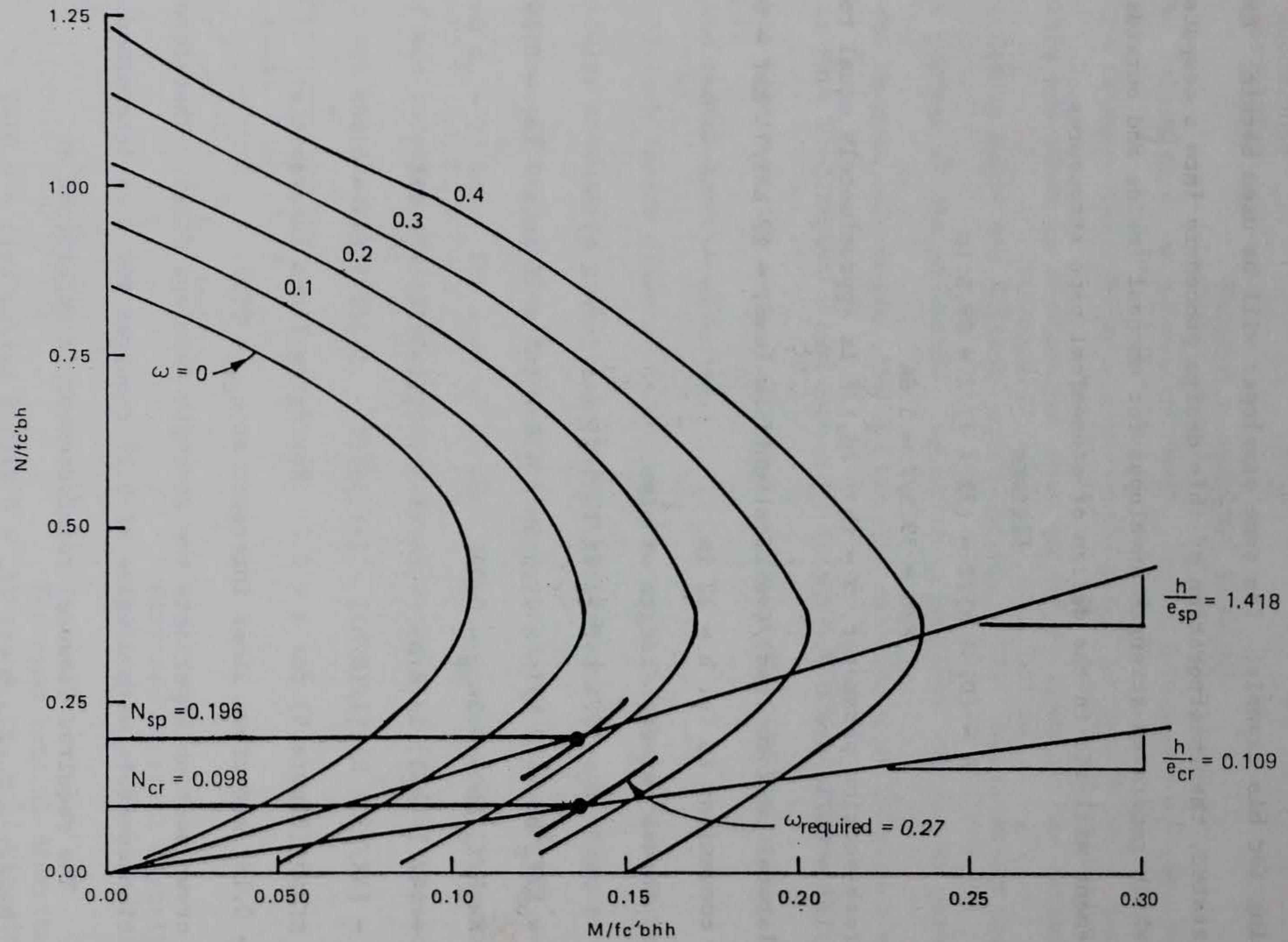
Figure 5. Strength Envelopes for \gamma = 0.7
