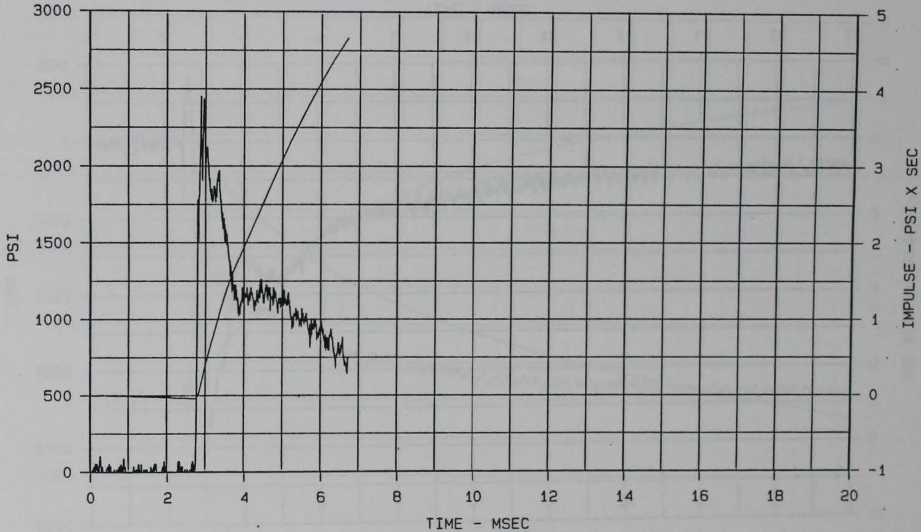
Figure 78. Soil stress wave form measured by gage SEV-3, 20 msec duration, MCBI Gage Validation Test 1
