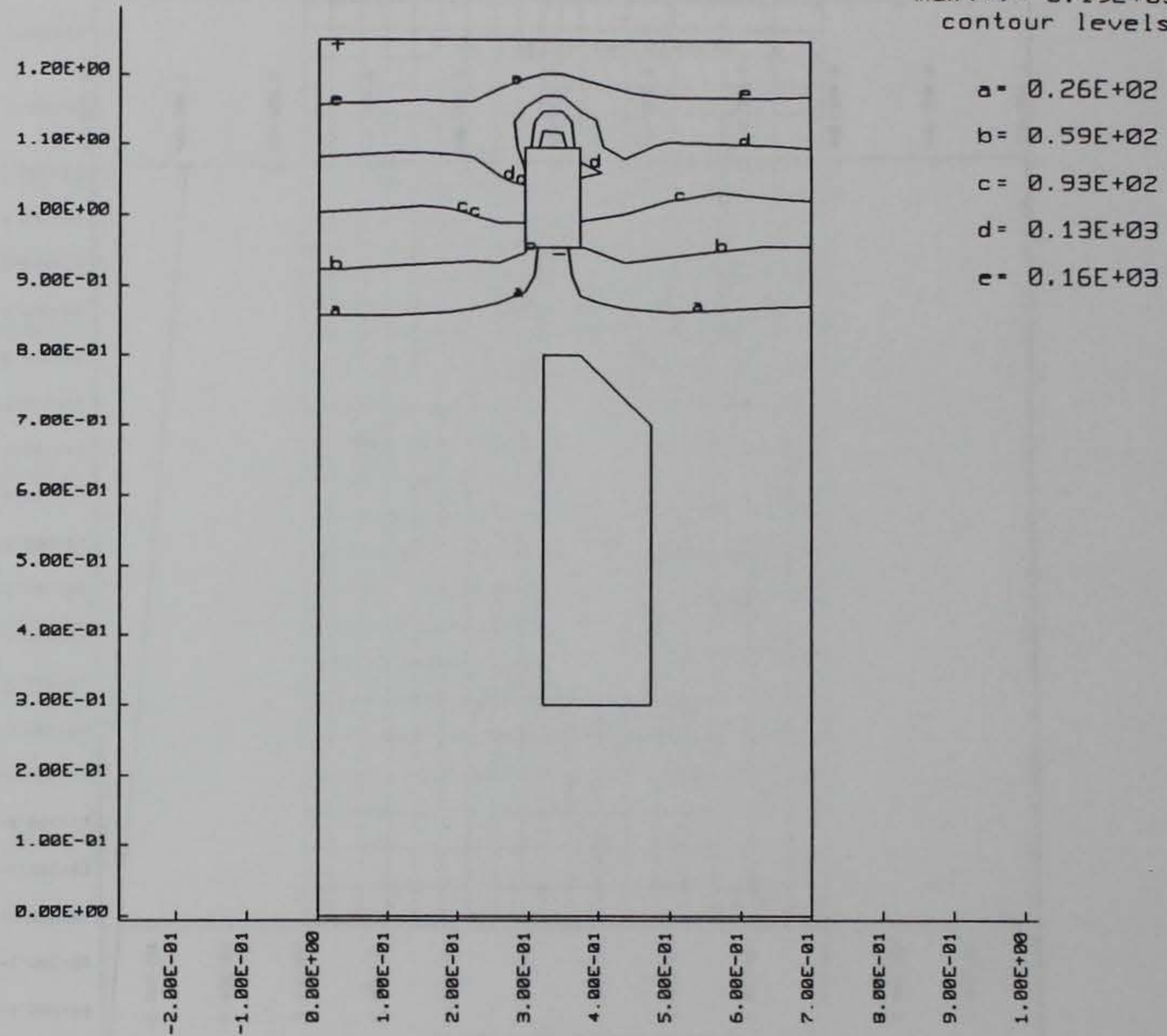
Figure 44. Axial stress contours inside the MCBI gage at 2 \mu sec after zero-time, as calculated by DYNA2D
