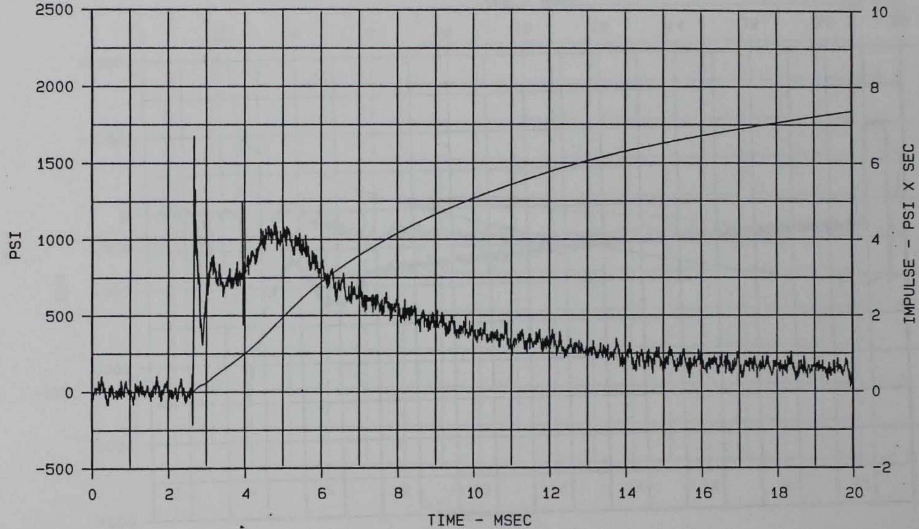
Figure 77. Soil stress wave form measured by gage SEV-2, 20 msec duration, MCBI Gage Validation Test 1
