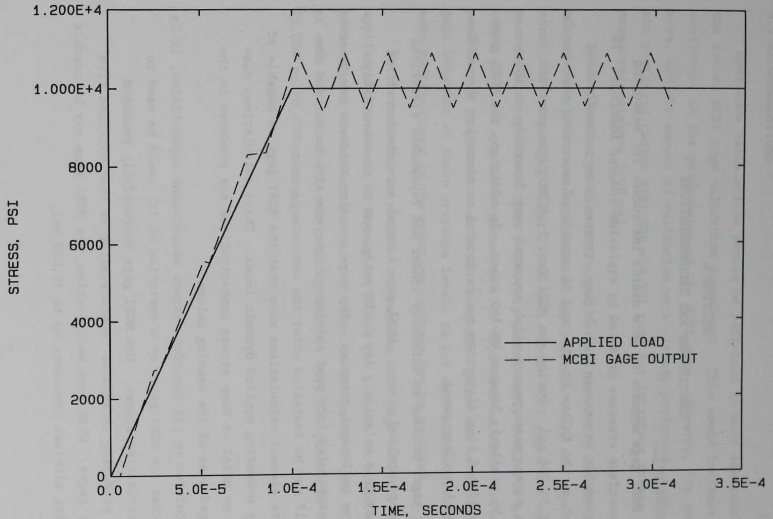
Figure 55. Comparison of calculated MCBI gage output versus applied stress loading curve
