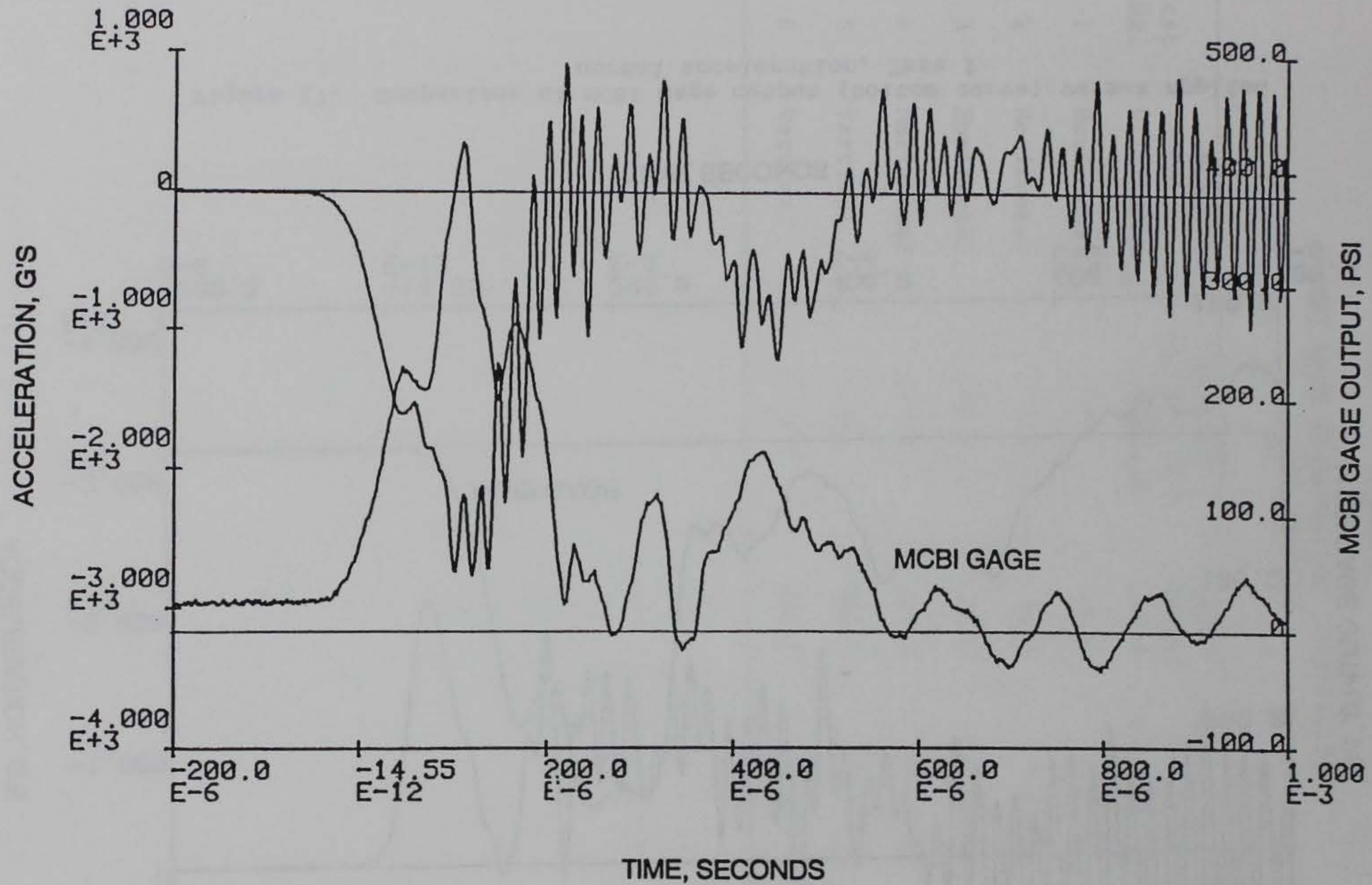
Figure 18. Comparison of MCBI gage output (bottom curve) versus applied normal acceleration, Test 2
