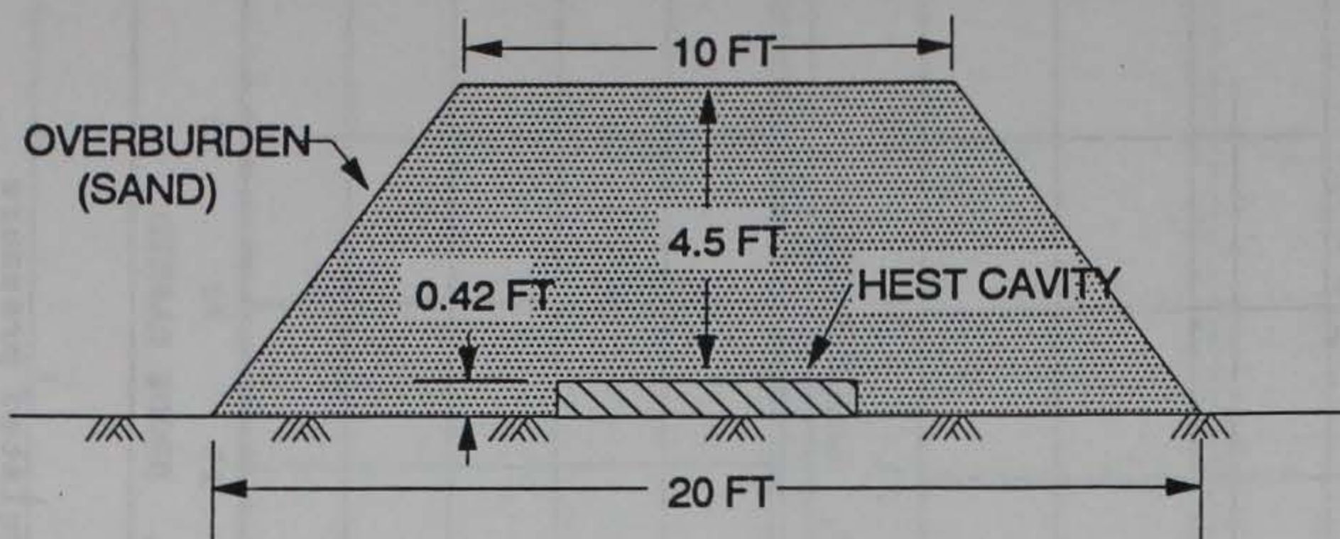
CHARGE/OVERBURDEN CONFIGURATION
