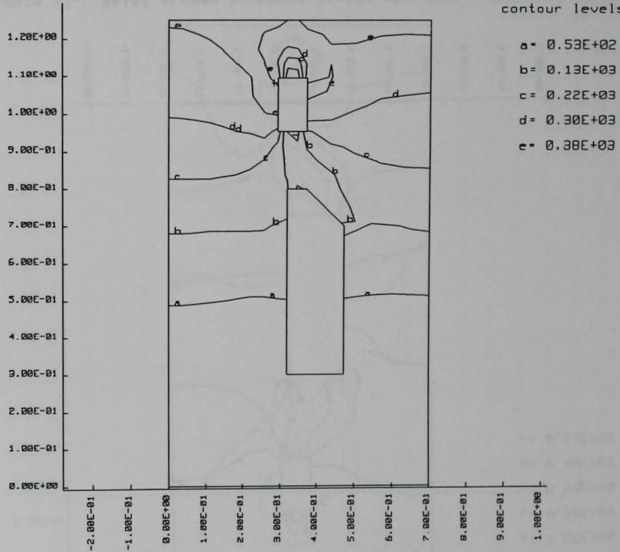
Figure 45. Axial stress contours inside the MCBI gage at 4 \mu sec after zero-time, as calculated by DYNA2D
