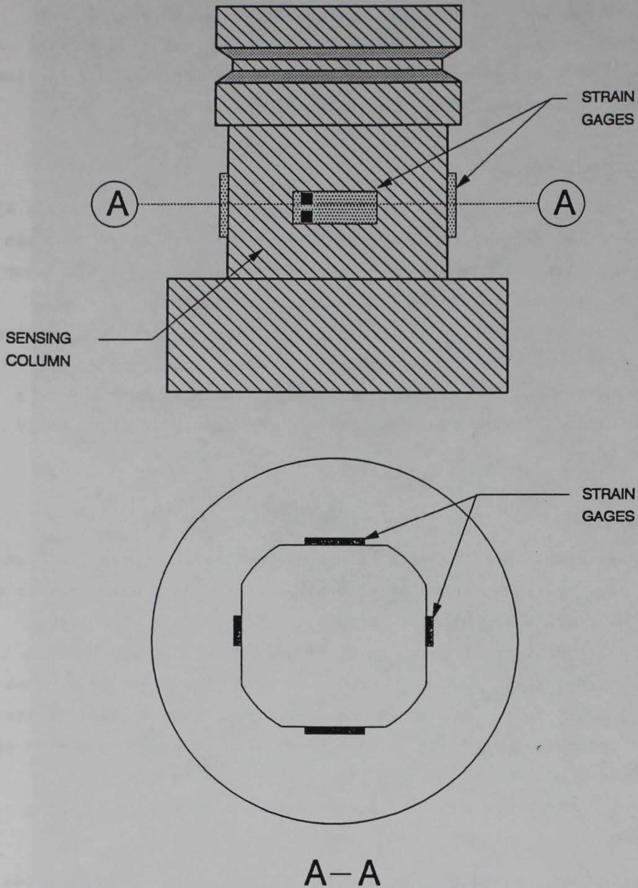
Figure 4. Location of strain gages on sensing column
