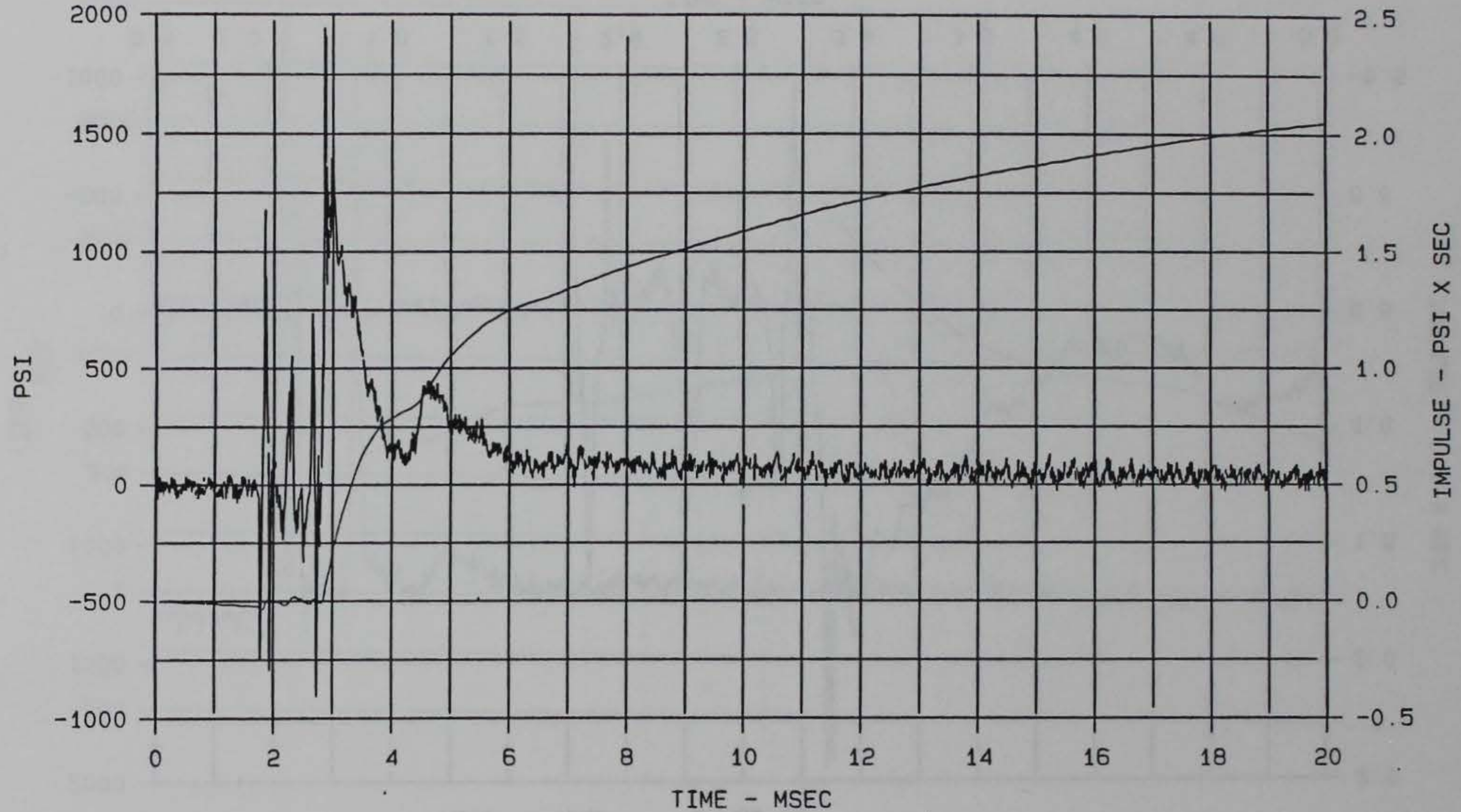
Figure 73. Interface stress wave form measured by gage MCBI-1, 20 msec duration, MCBI Gage Validation Test 1
