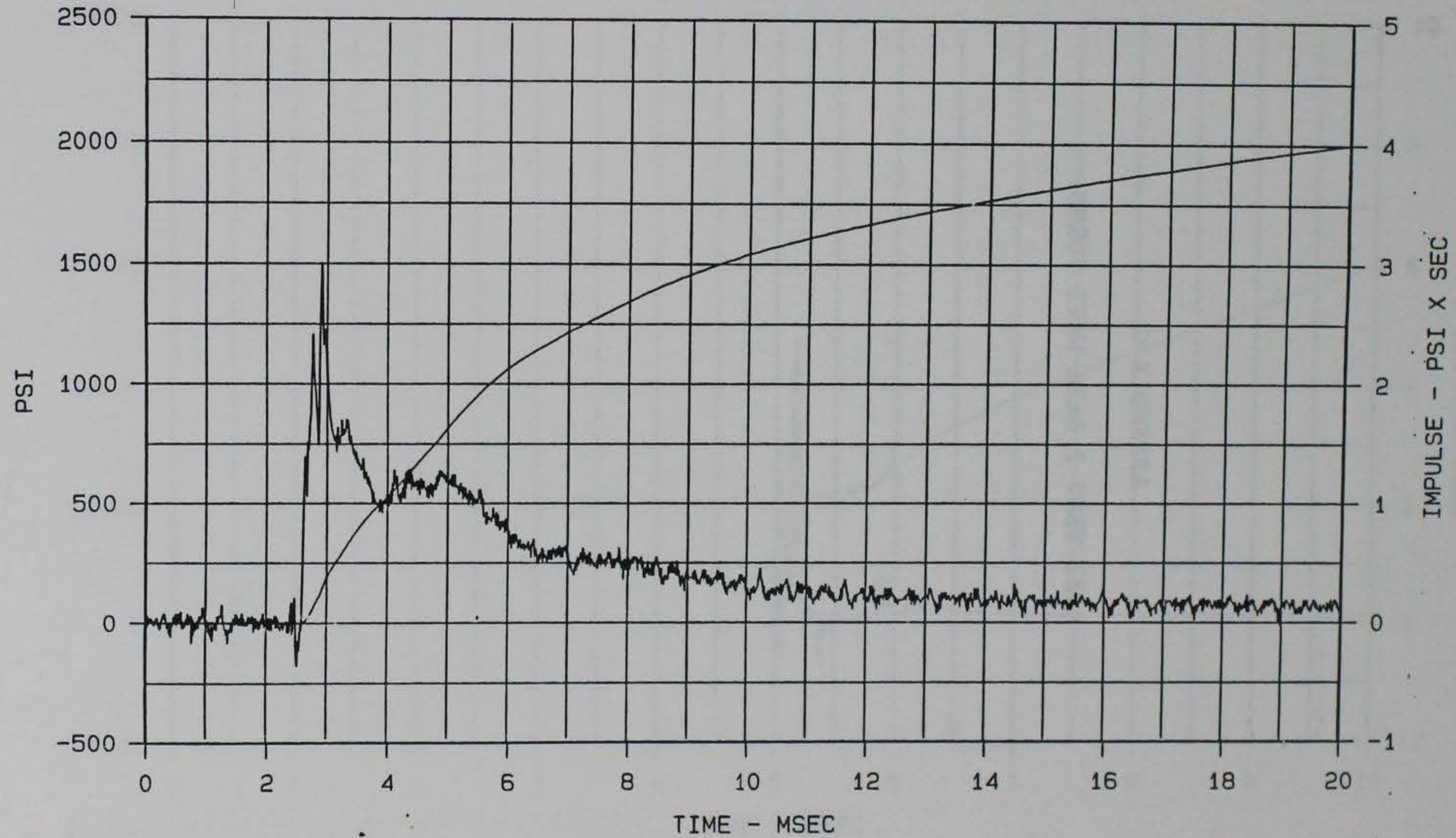
Figure 80. Soil stress wave form measured by gage SEH-2, 20 msec duration, MCBI Gage Validation Test 1
