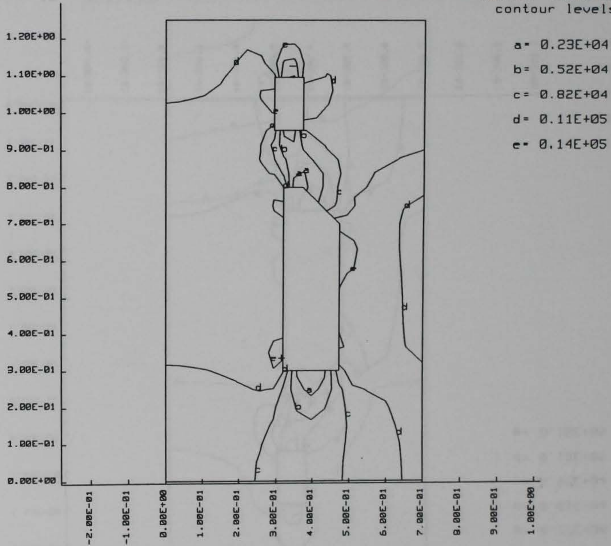
Figure 48. Axial stress contours inside the MCBI gage at 0.2 msec after zero-time, as calculated by DYNA2D
