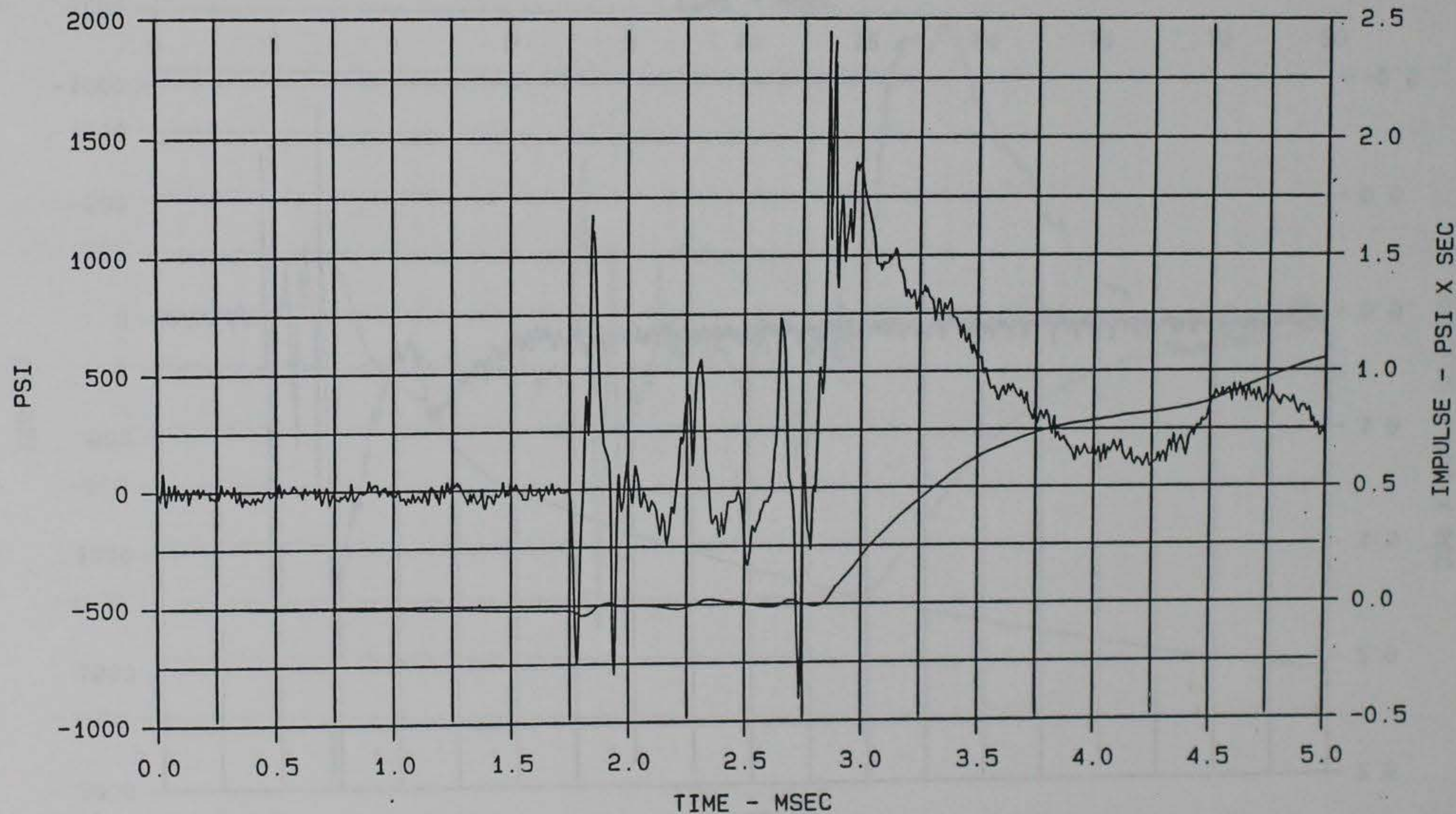
Figure 72. Interface stress wave form measured by gage MCBI-1, 5 msec duration, MCBI Gage Validation Test 1
