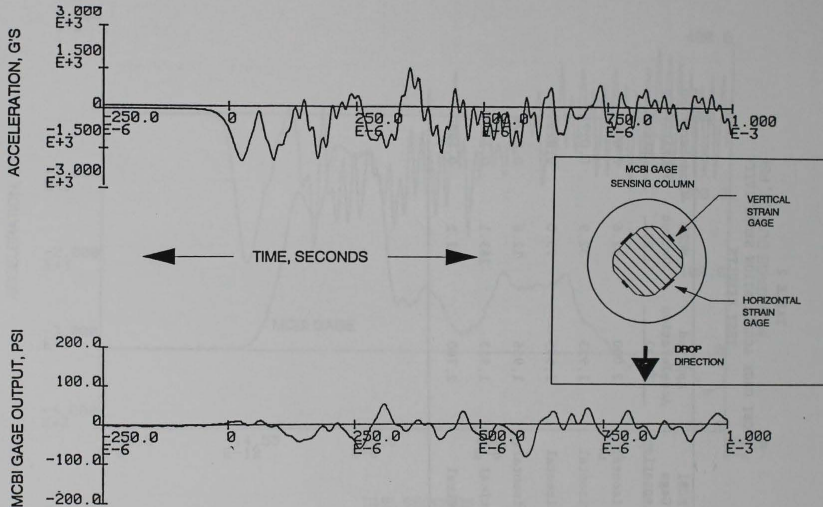
Figure 16. Comparison of MCBI gage output (bottom curve) versus applied lateral acceleration. The MCBI gage is positioned so that the transverse strain gages are 45 degrees from the vertical
