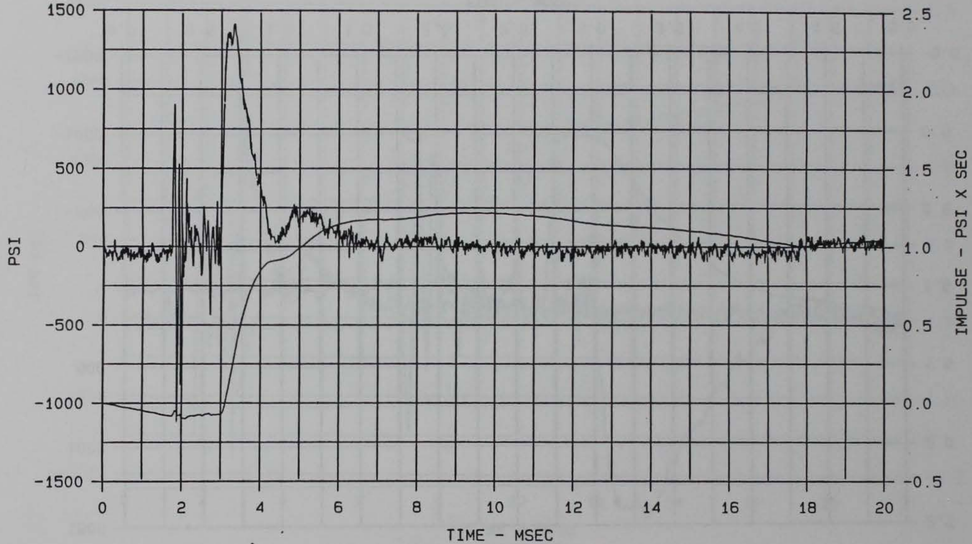
Figure 75. Interface stress wave form measured by gage MCBI-2, 20 msec duration, MCBI Gage Validation Test 1
