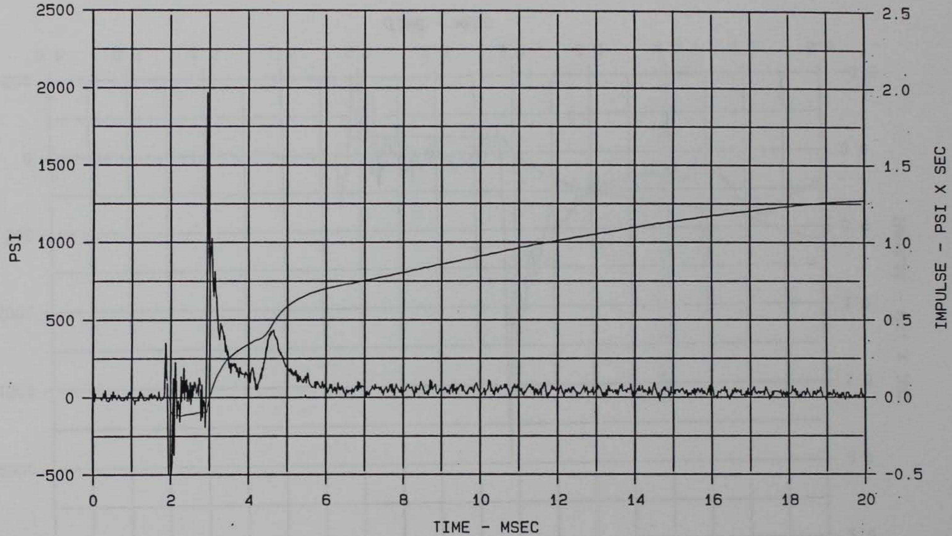
Figure 69. Interface stress wave form measured by gage VM-1, 20 msec duration, MCBI Gage Validation Test 1
