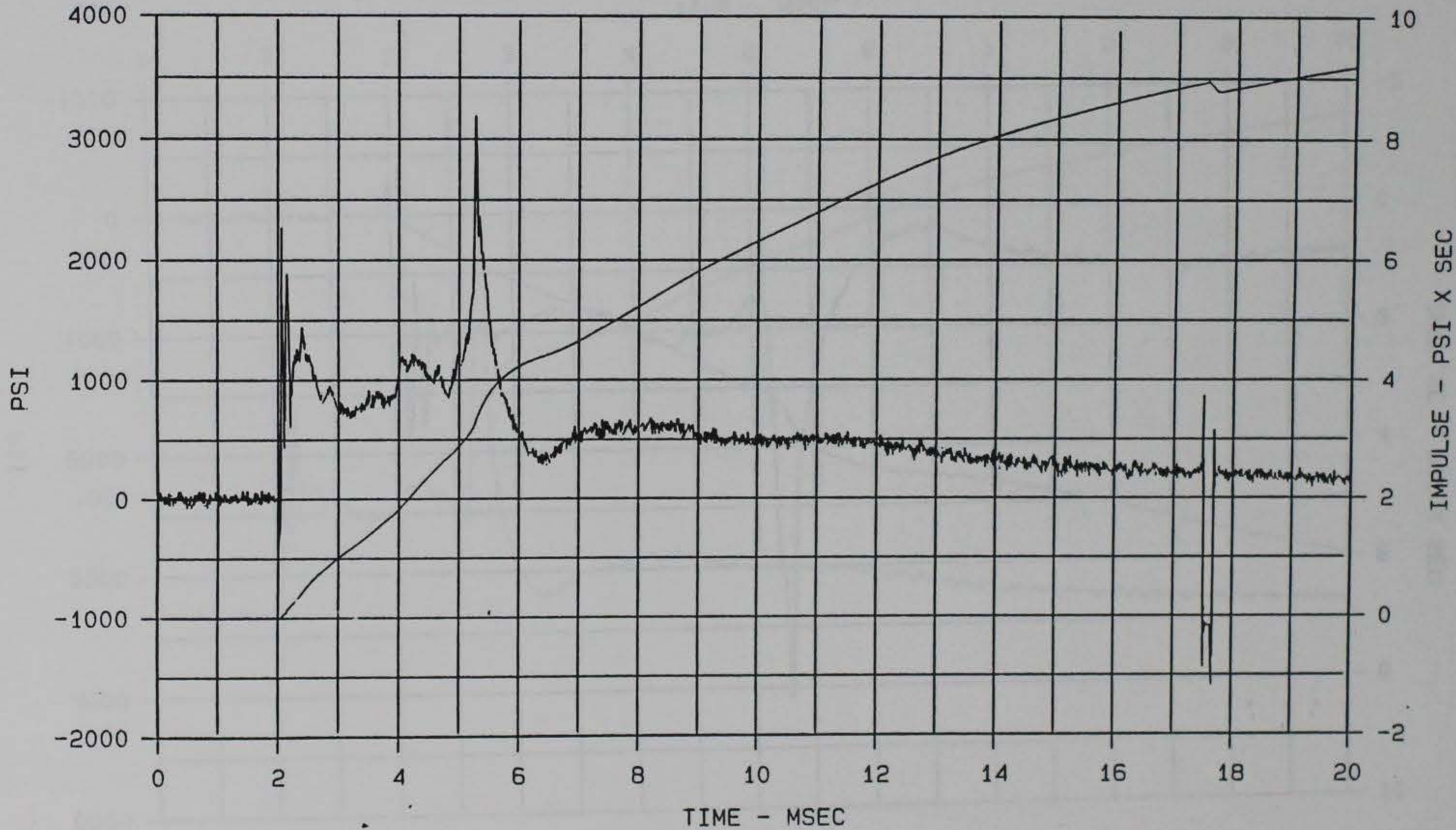
Figure 89. Soil stress wave form measured by gage SEV-2, 20 msec duration, MCBI Gage Validation Test 2
