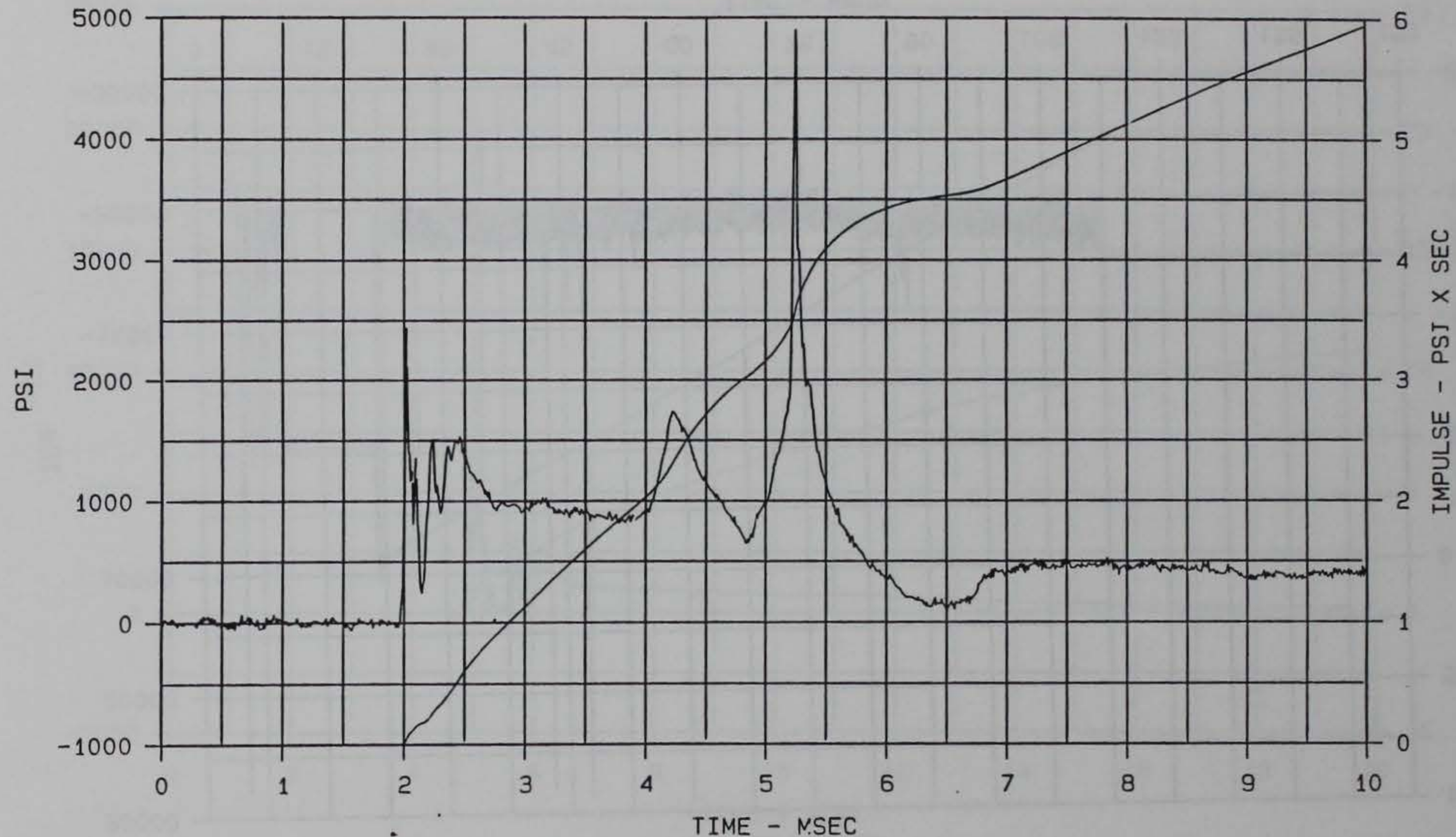
Figure 86. Soil stress wave form measured by gage SEV-1, 10 msec duration, MCBI Gage Validation Test 2
