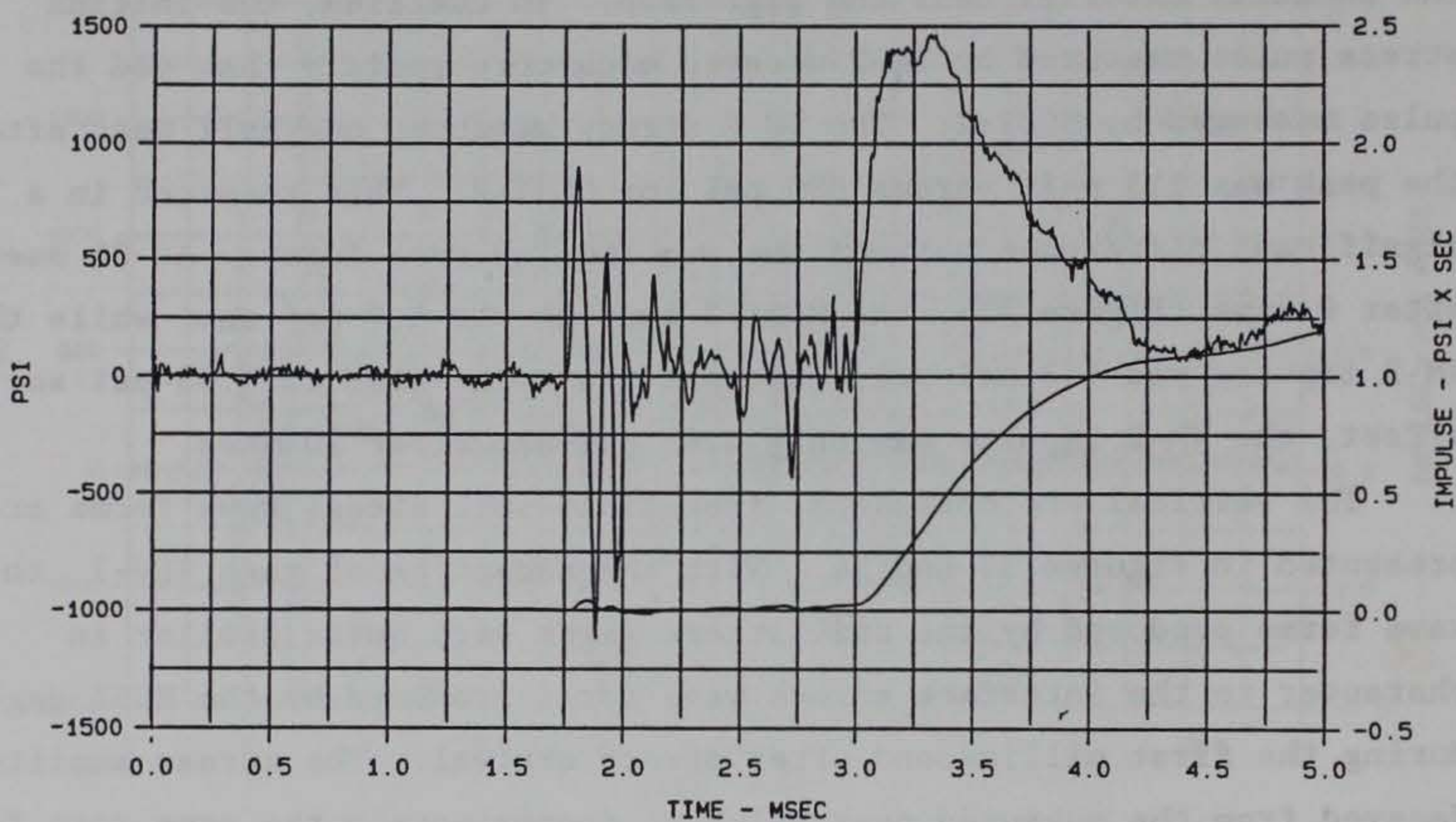
Figure 31. Comparison of MCBI-2 (bottom) and Kulite VM-2 interface stress records, 5 msec duration, MCBI Gage Validation Test 1
