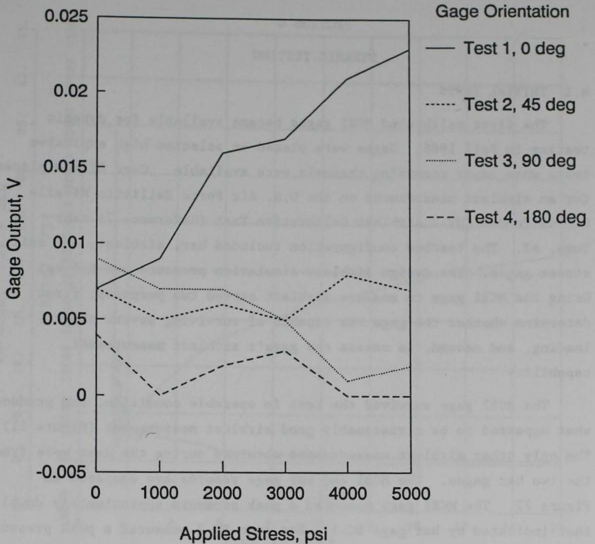
Figure 20. Lateral stress sensitivity test results. Test 1 was conducted with a longitudinal strain gage facing toward the applied stress; other orientations are relative to that of Test 1
