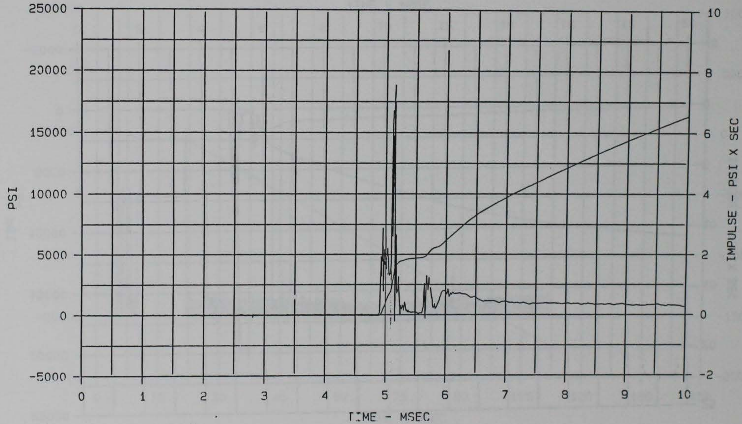
Figure 83. Interface stress wave form measured by gage MCBI-2, 10 msec duration, MCBI Gage Validation Test 2
