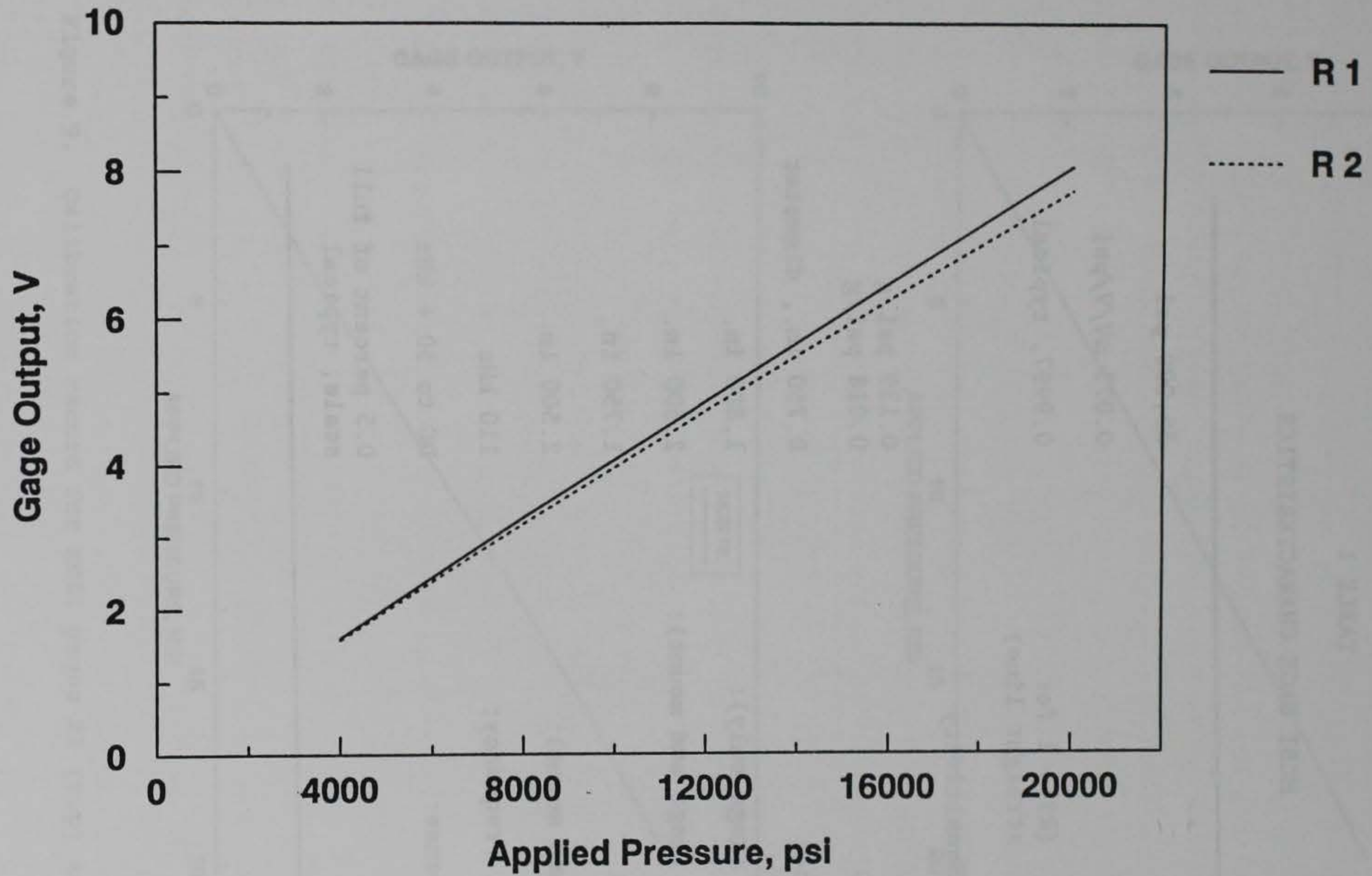
Figure 8. Pressure/output curves for MCBI prototype gages R1 and R2
