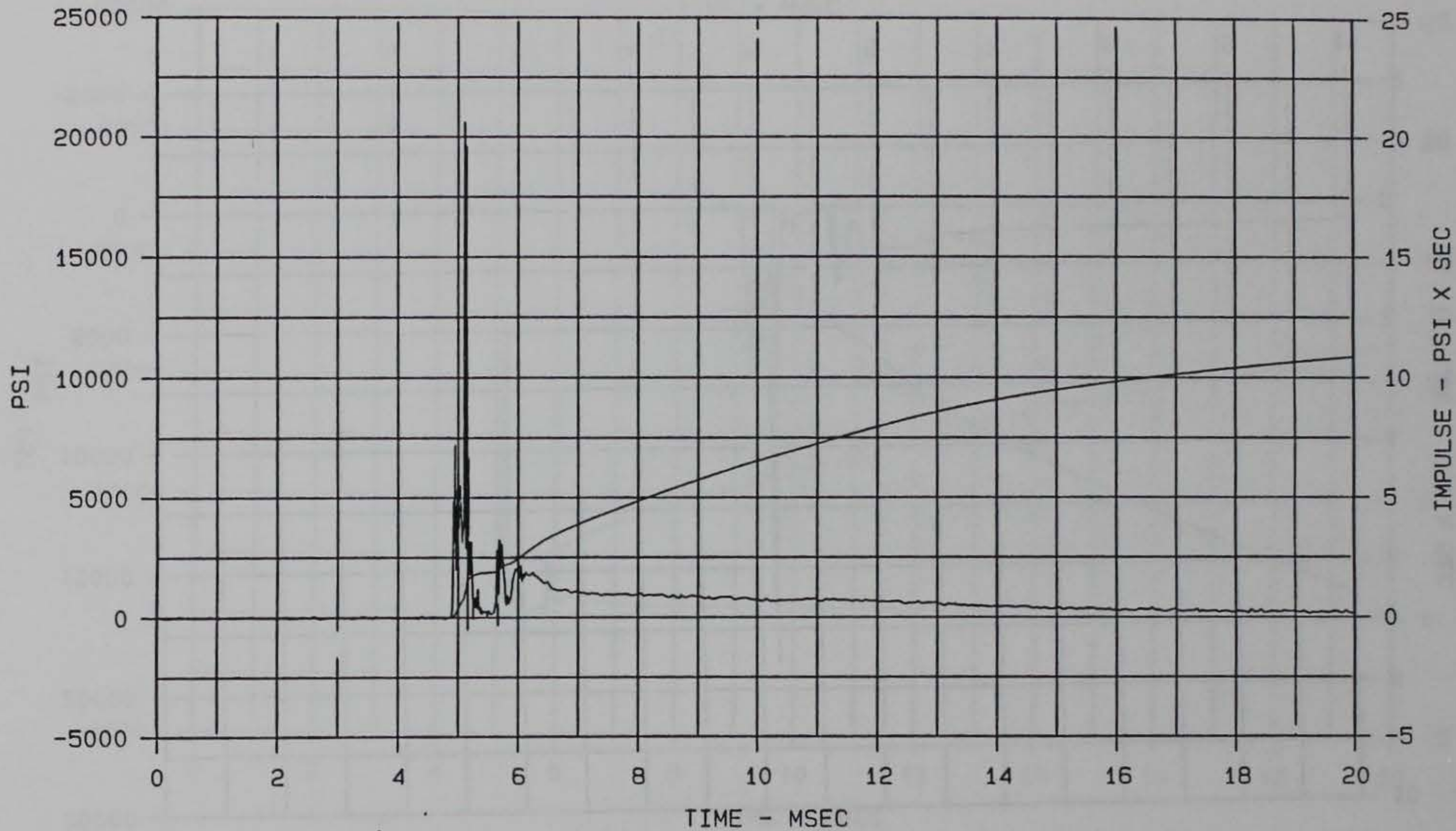
Figure 84. Interface stress wave form measured by gage MCBI-2, 20 msec duration, MCBI Gage Validation Test 2
