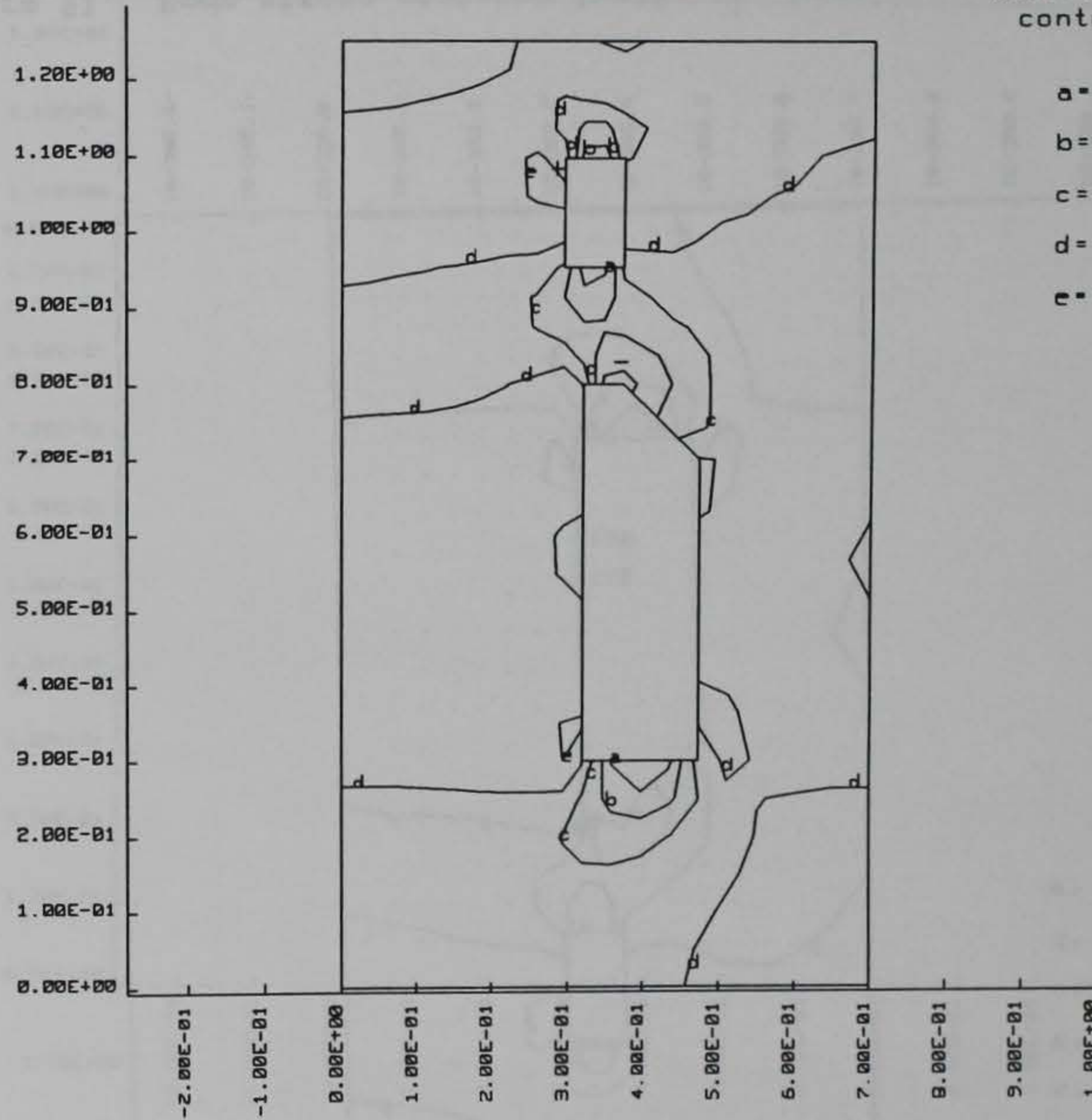
Figure 50. Hoop stress contours inside the MCBI gage at 0.2 msec after zero-time, as calculated by DYNA2D
