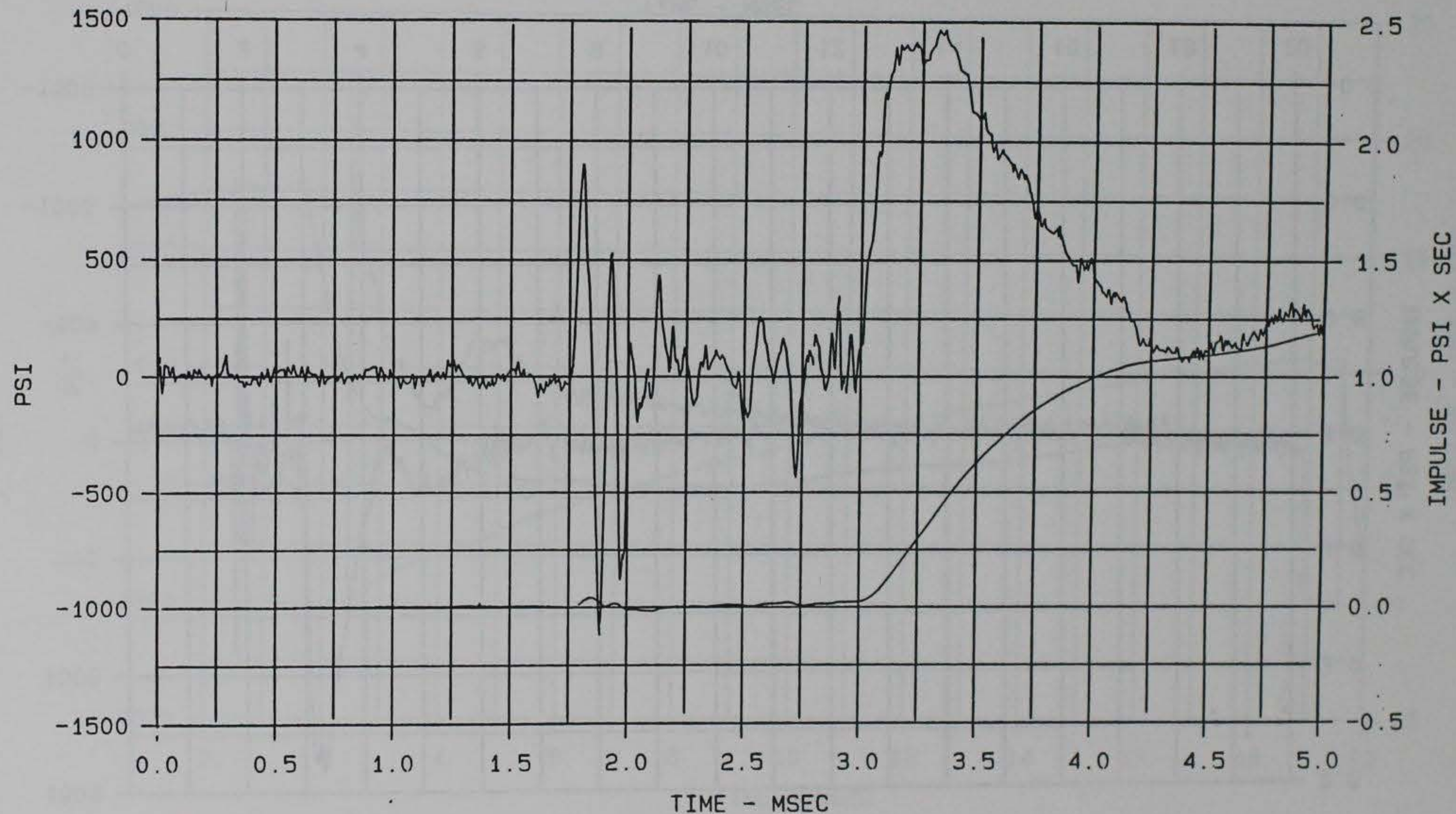
Figure 74. Interface stress wave form measured by gage MCBI-2, 5 msec duration, MCBI Gage Validation Test 1
