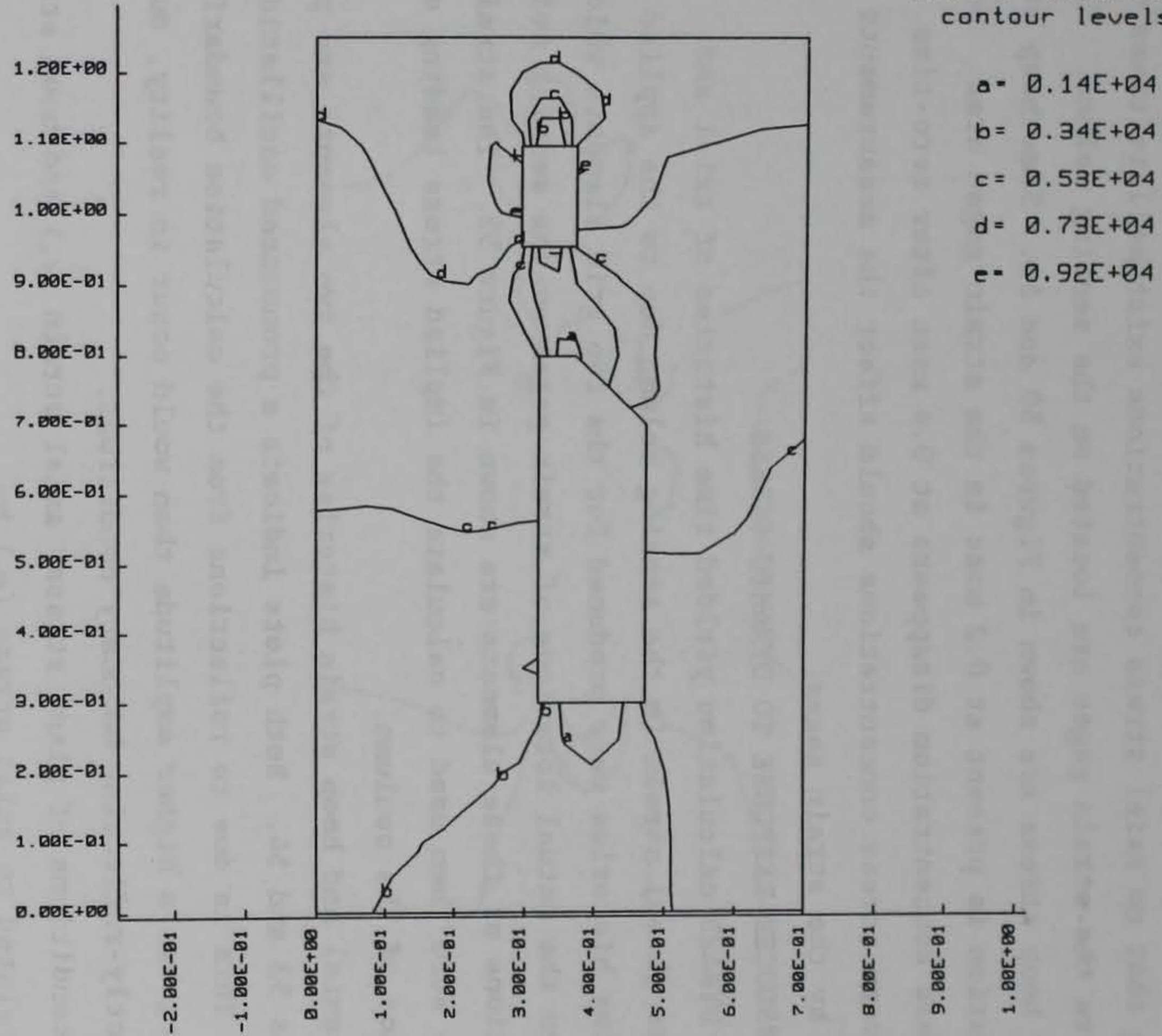
Figure 47. Axial stress contours inside the MCBI gage at 8 \mu sec after zero-time, as calculated by DYNA2D
