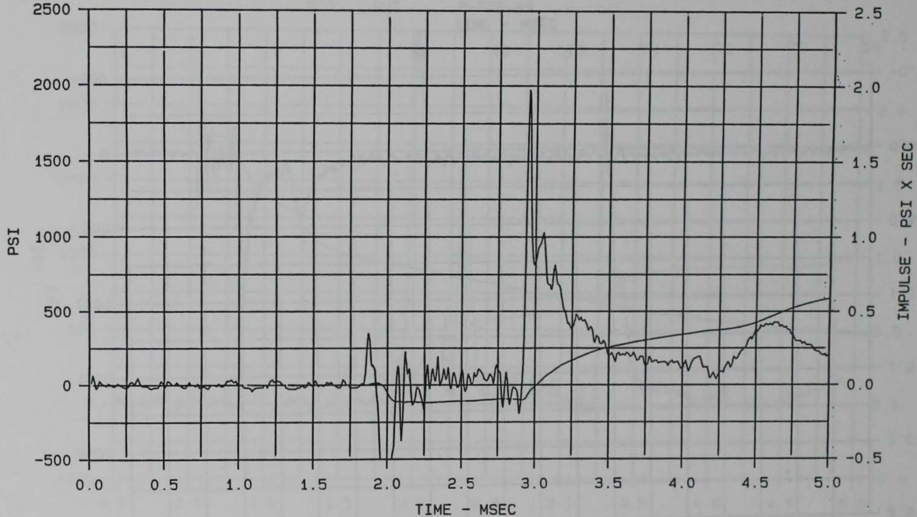
Figure 68. Interface stress wave form measured by gage VM-1, 5 msec duration, MCBI Gage Validation Test 1
