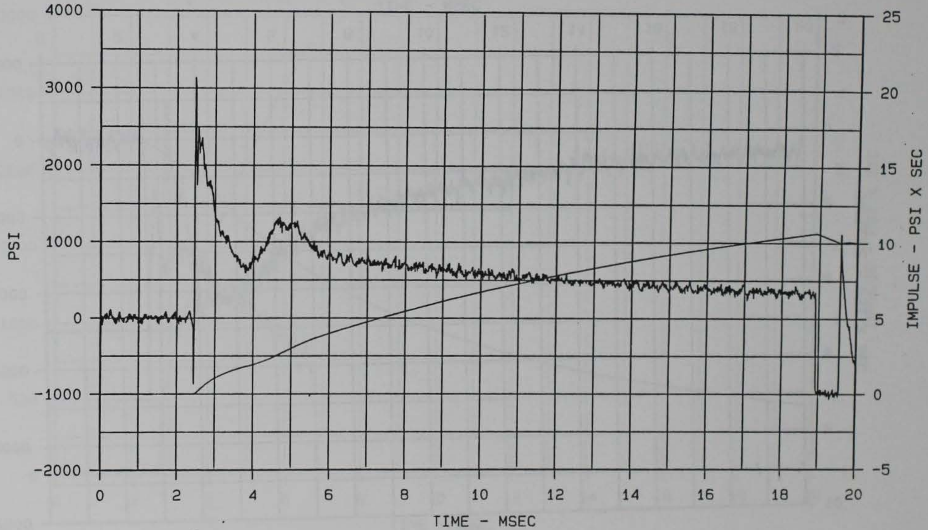
Figure 76. Soil stress wave form measured by gage SEV-1, 20 msec duration, MCBI Gage Validation Test 1
