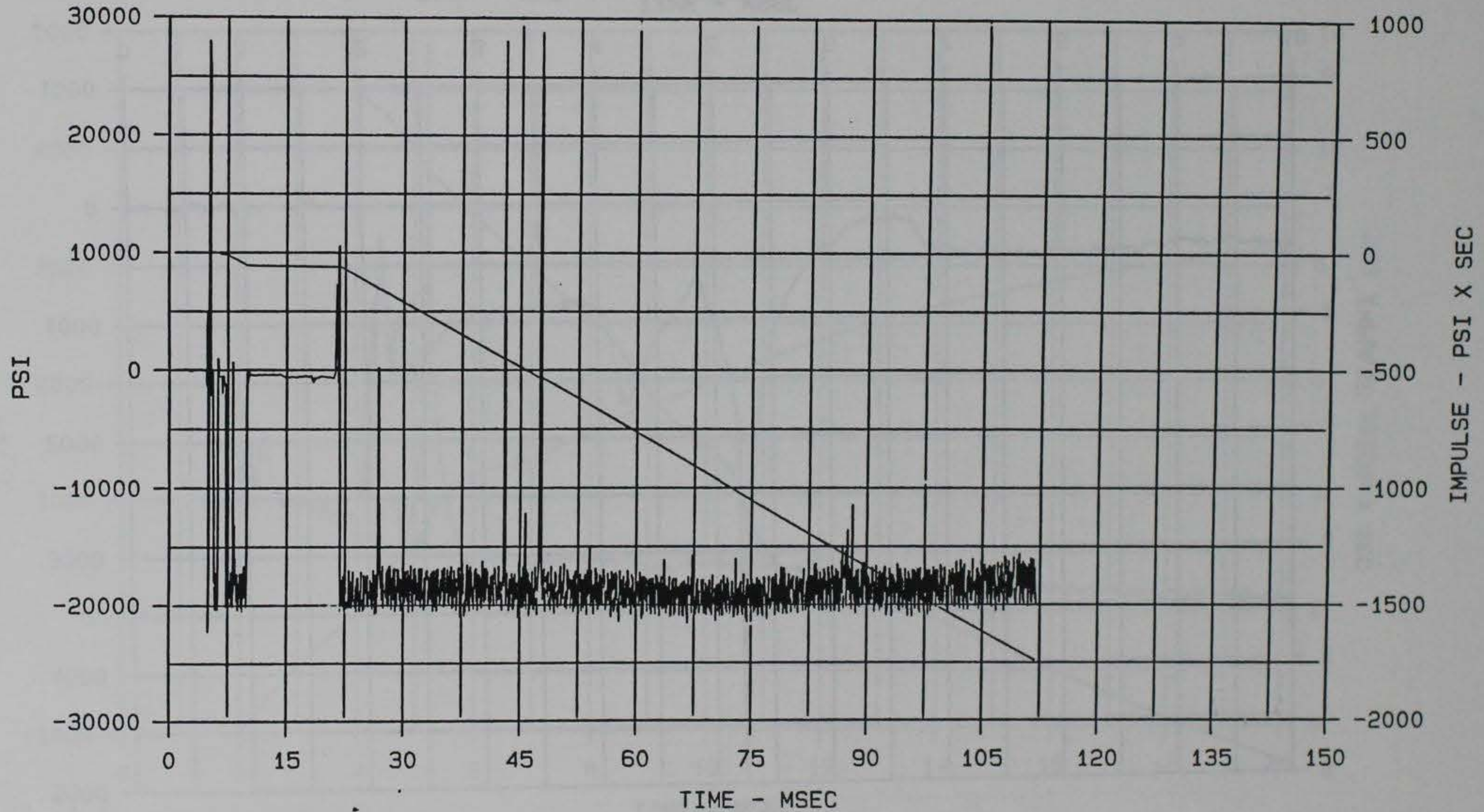
Figure 85. Interface stress wave form measured by gage MCBI-3, 150 msec duration, MCBI Gage Validation Test 2
