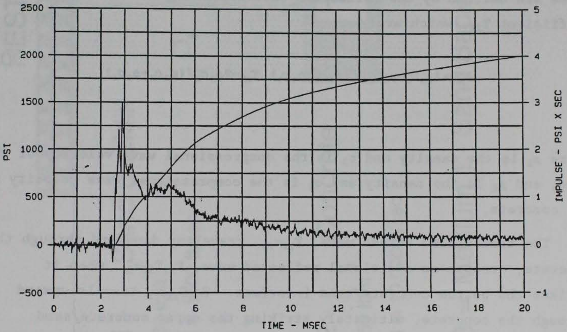
Figure 34. Horizontal soil stress wave forms, MCBI Gage Validation Test 1
