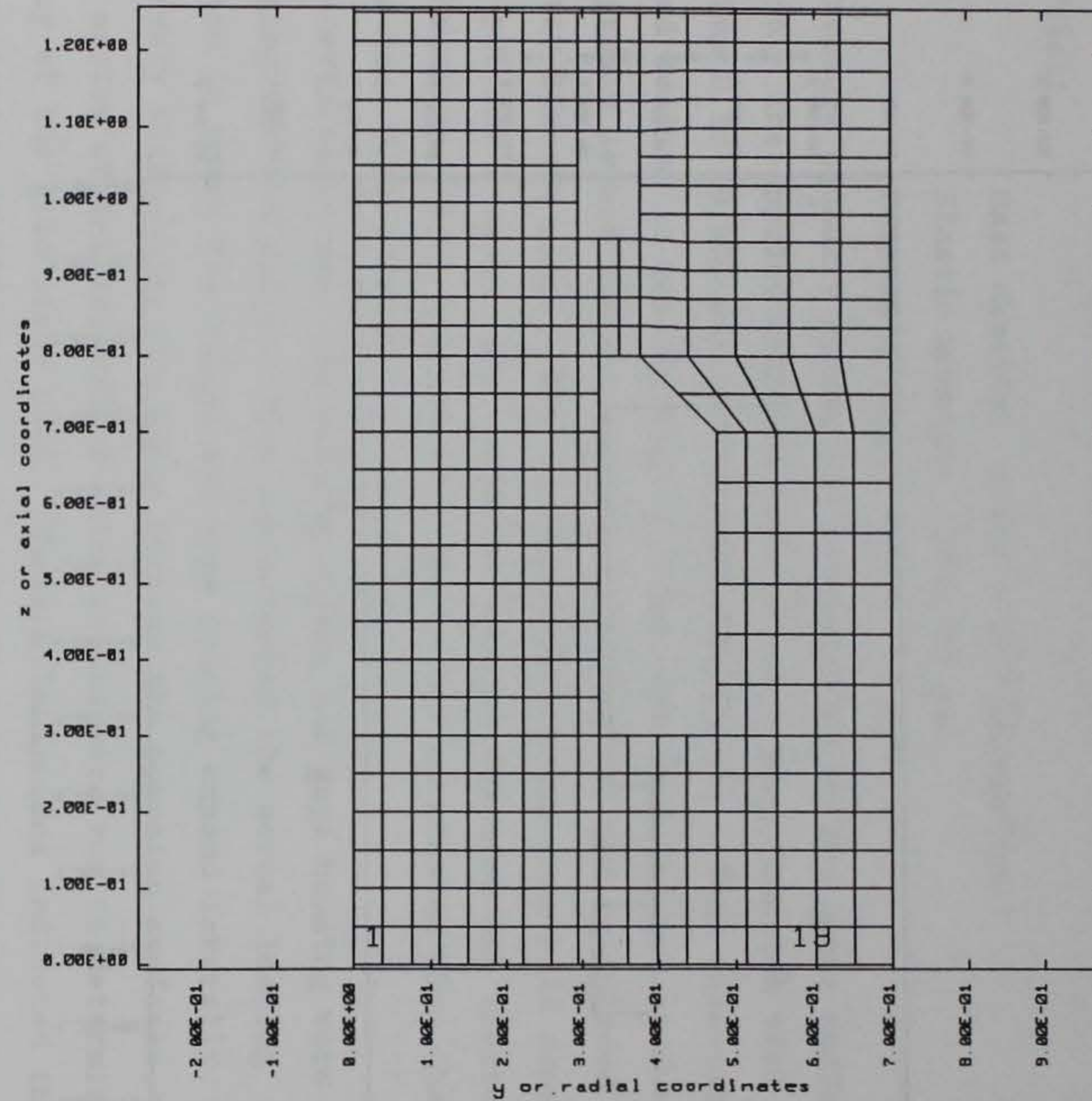
Figure 42. Finite element mesh of the MCBI gage generated by MAZE
