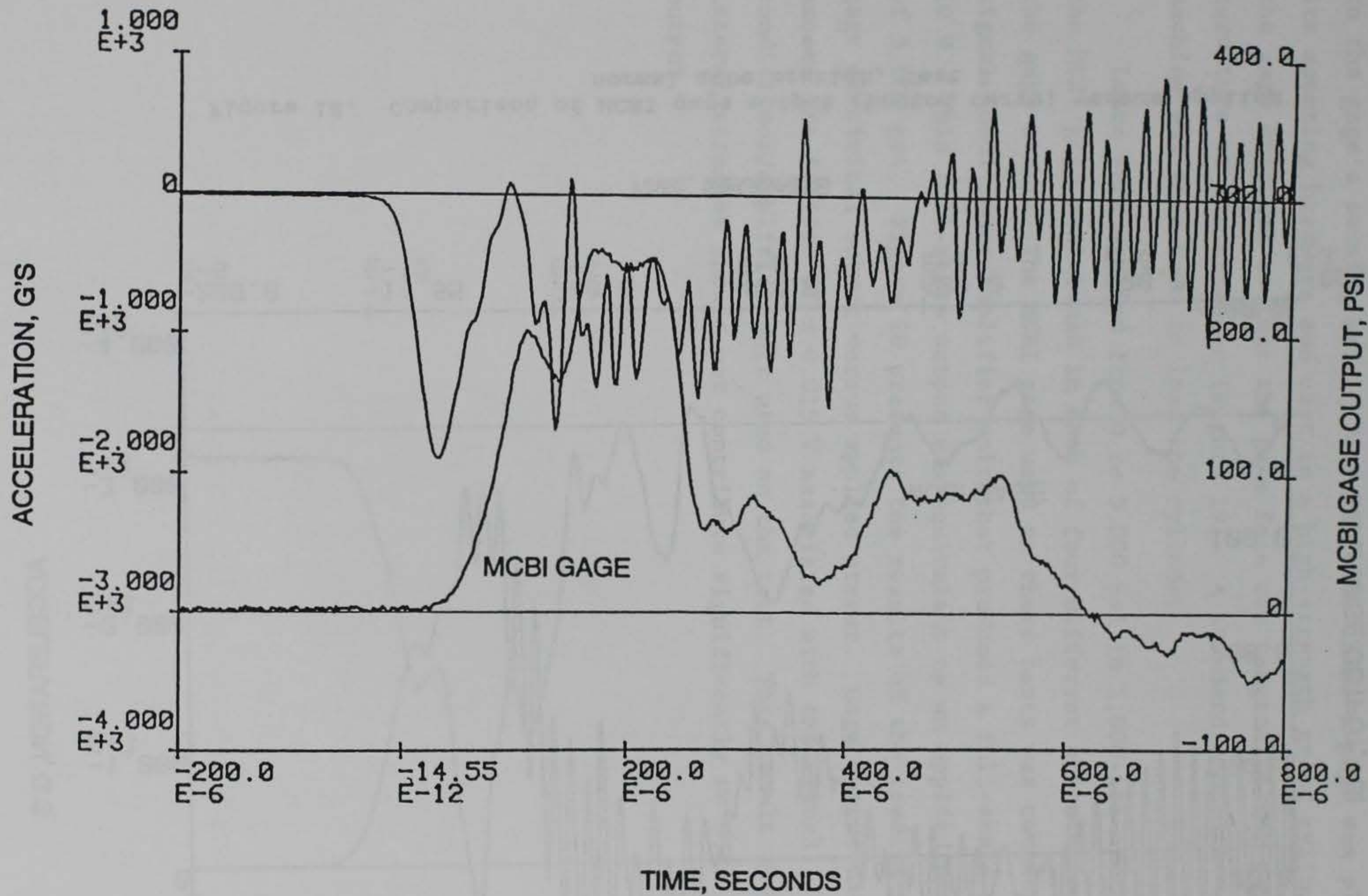
Figure 17. Comparison of MCBI gage output (bottom curve) versus applied normal acceleration, Test 1
