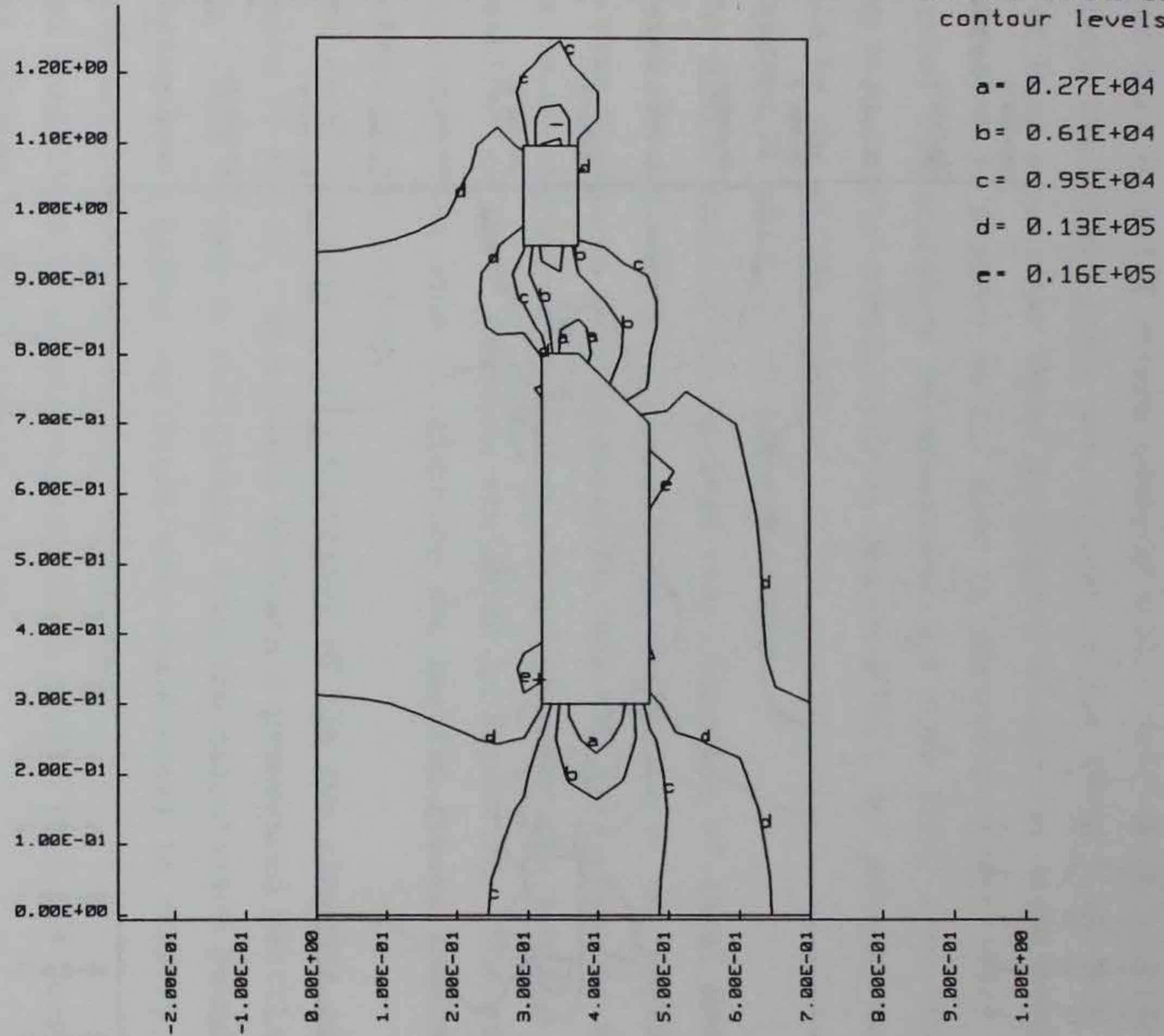
Figure 49. Axial stress contours inside the MCBI gage at 0.4 msec after zero-time, as calculated by DYNA2D
