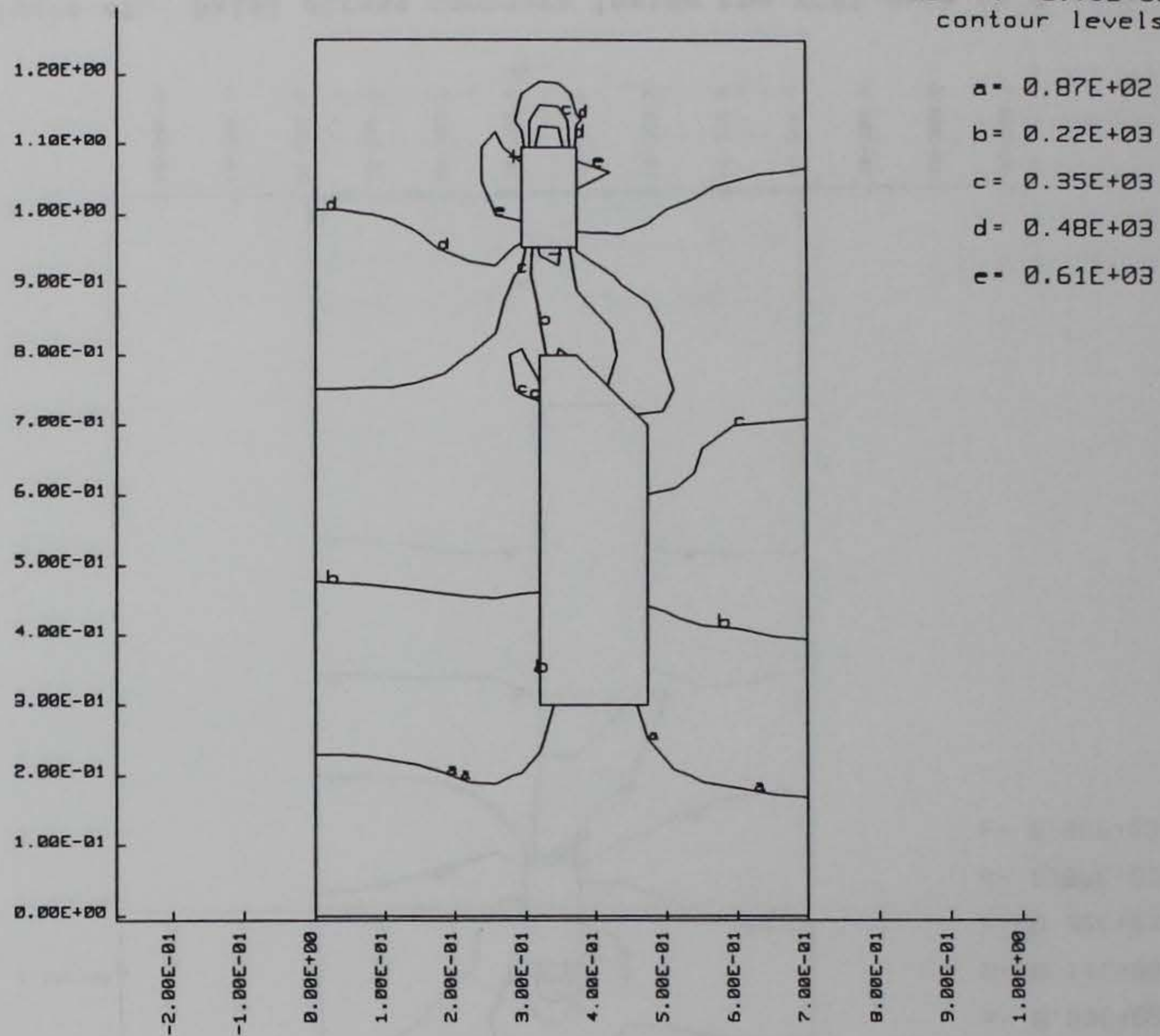
Figure 46. Axial stress contours inside the MCBI gage at 6 \mu sec after zero-time, as calculated by DYNA2D
