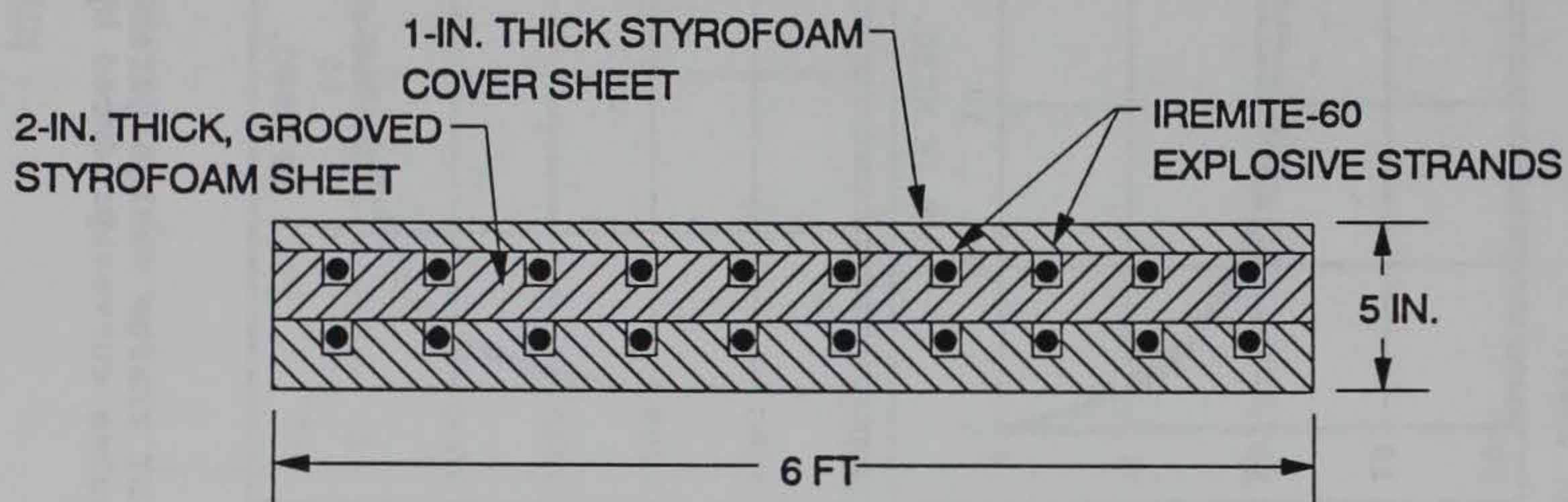
HEST CAVITY CROSS-SECTION
