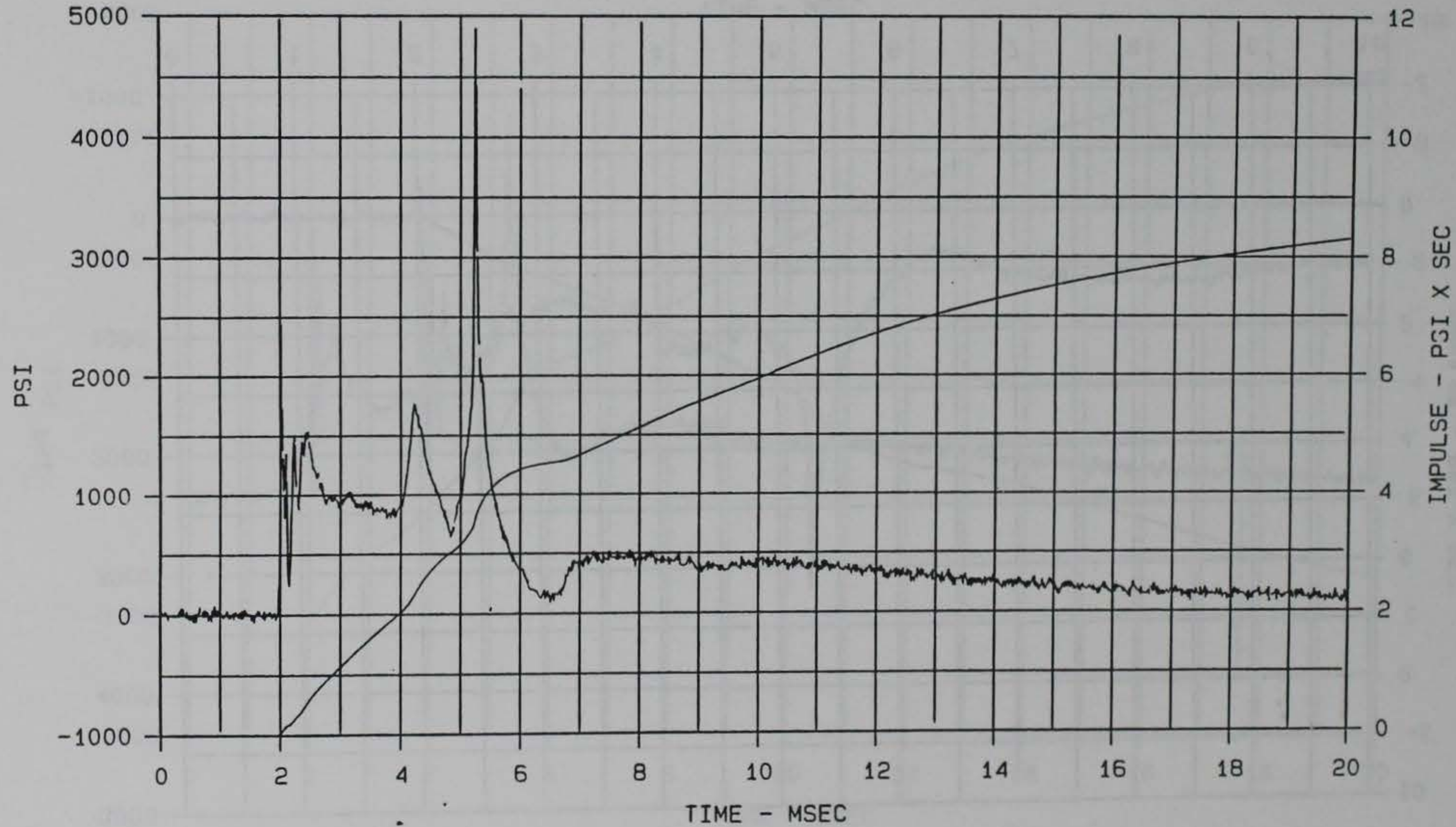
Figure 87. Soil stress wave form measured by gage SEV-1, 20 msec duration, MCBI Gage Validation Test 2
