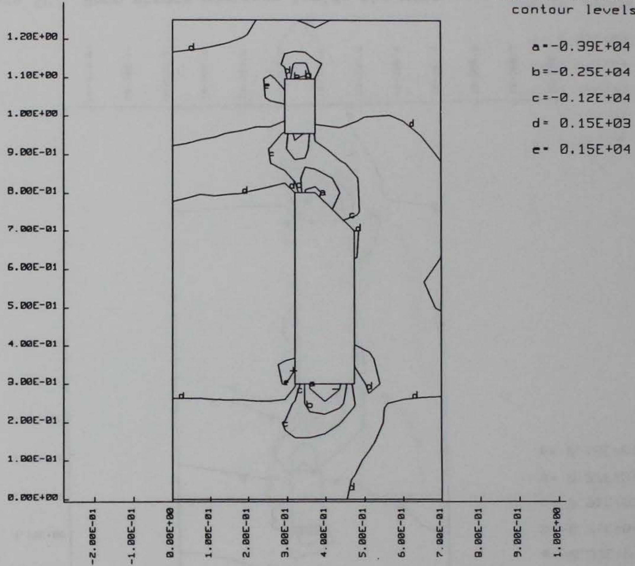
Figure 51. Hoop stress contours inside the MCBI gage at 0.4 msec after zero-time, as calculated by DYNA2D
