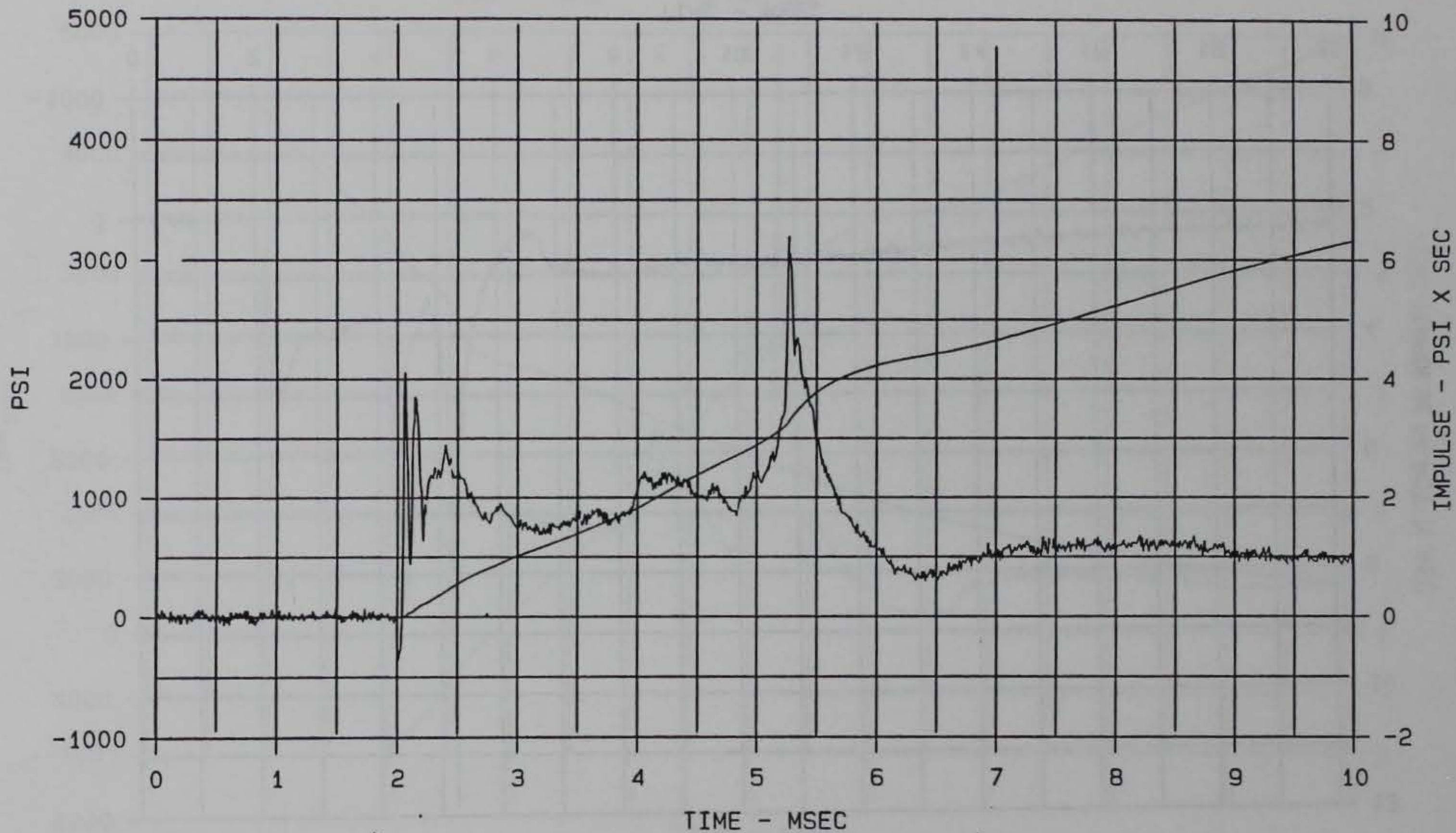
Figure 88. Soil stress wave form measured by gage SEV-2, 10 msec duration, MCBI Gage Validation Test 2
