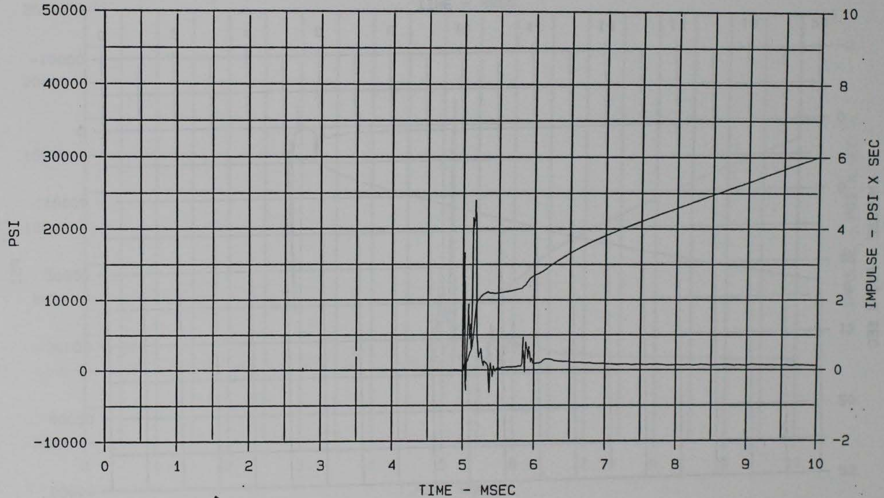
Figure 81. Interface stress wave form measured by gage MCBI-1, 10 msec duration, MCBI Gage Validation Test 2
