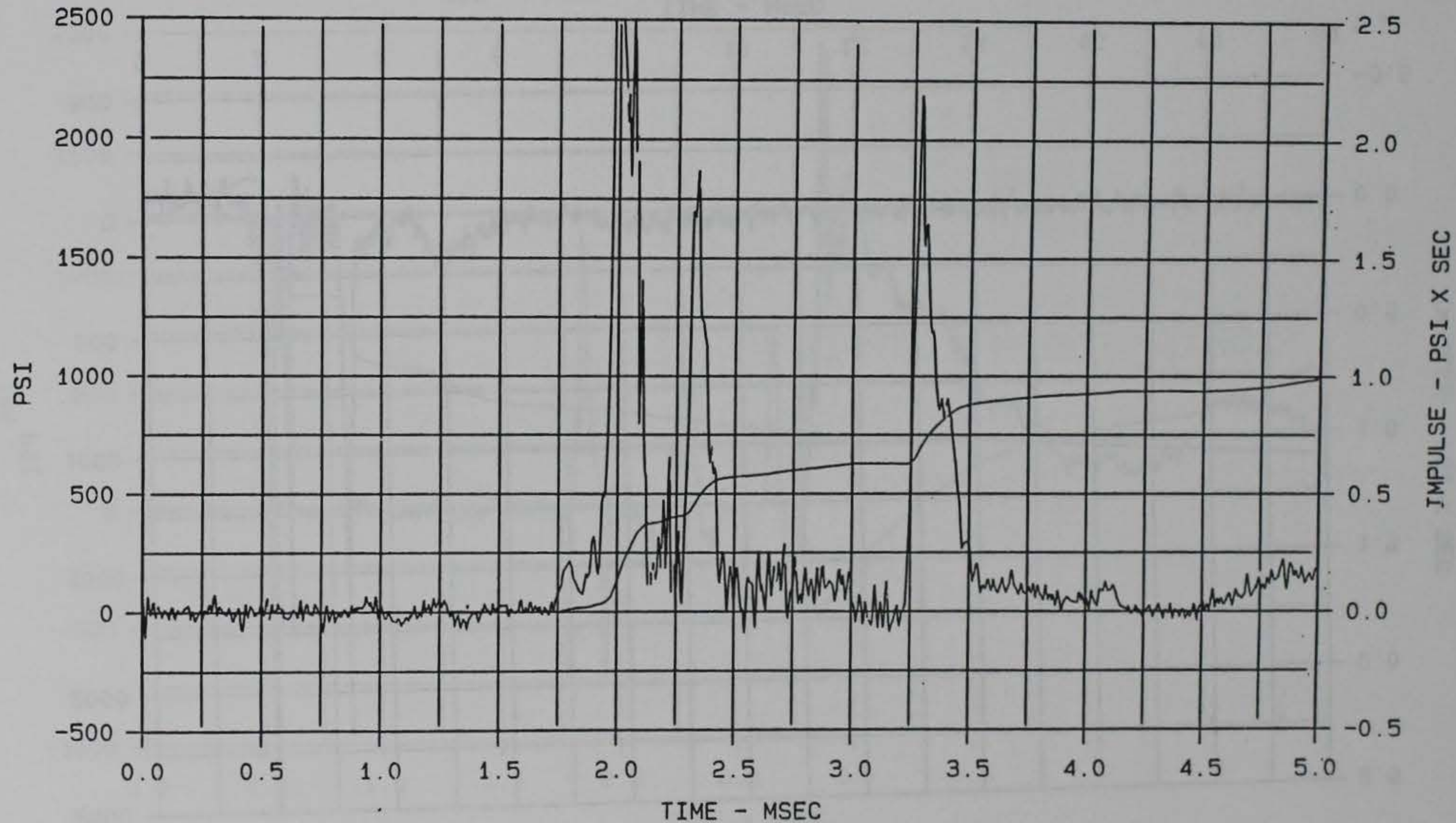
Figure 70. Interface stress wave form measured by gage VM-2, 5 msec duration, MCBI Gage Validation Test 1
