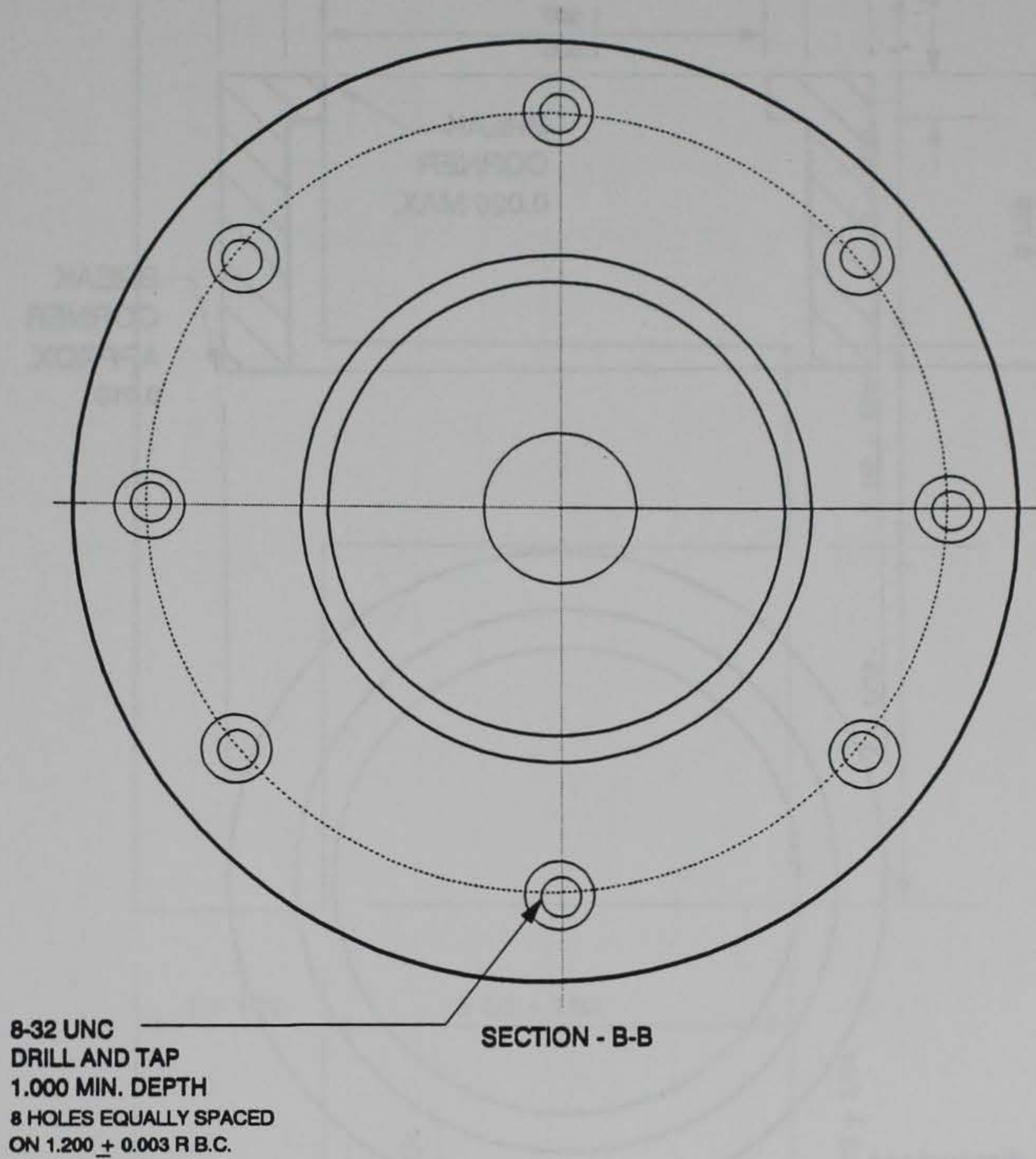
Figure 65. Top view of MCBI gage clamping ring
