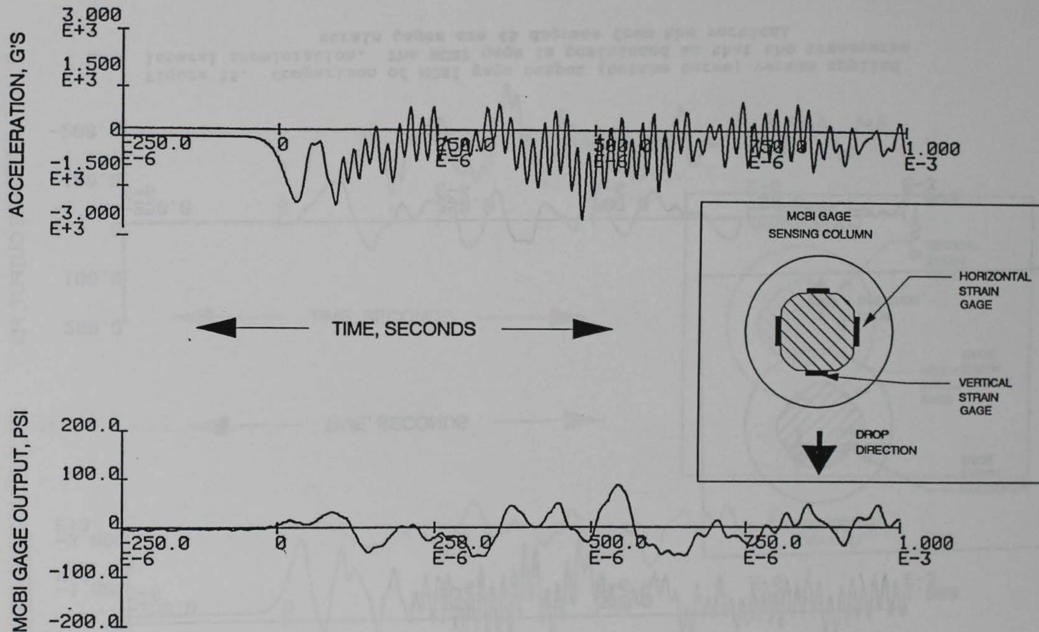
Figure 14. Comparison of MCBI gage output (bottom curve) versus applied lateral acceleration. The MCBI gage is positioned so that the transverse strain gages are horizontally oriented
