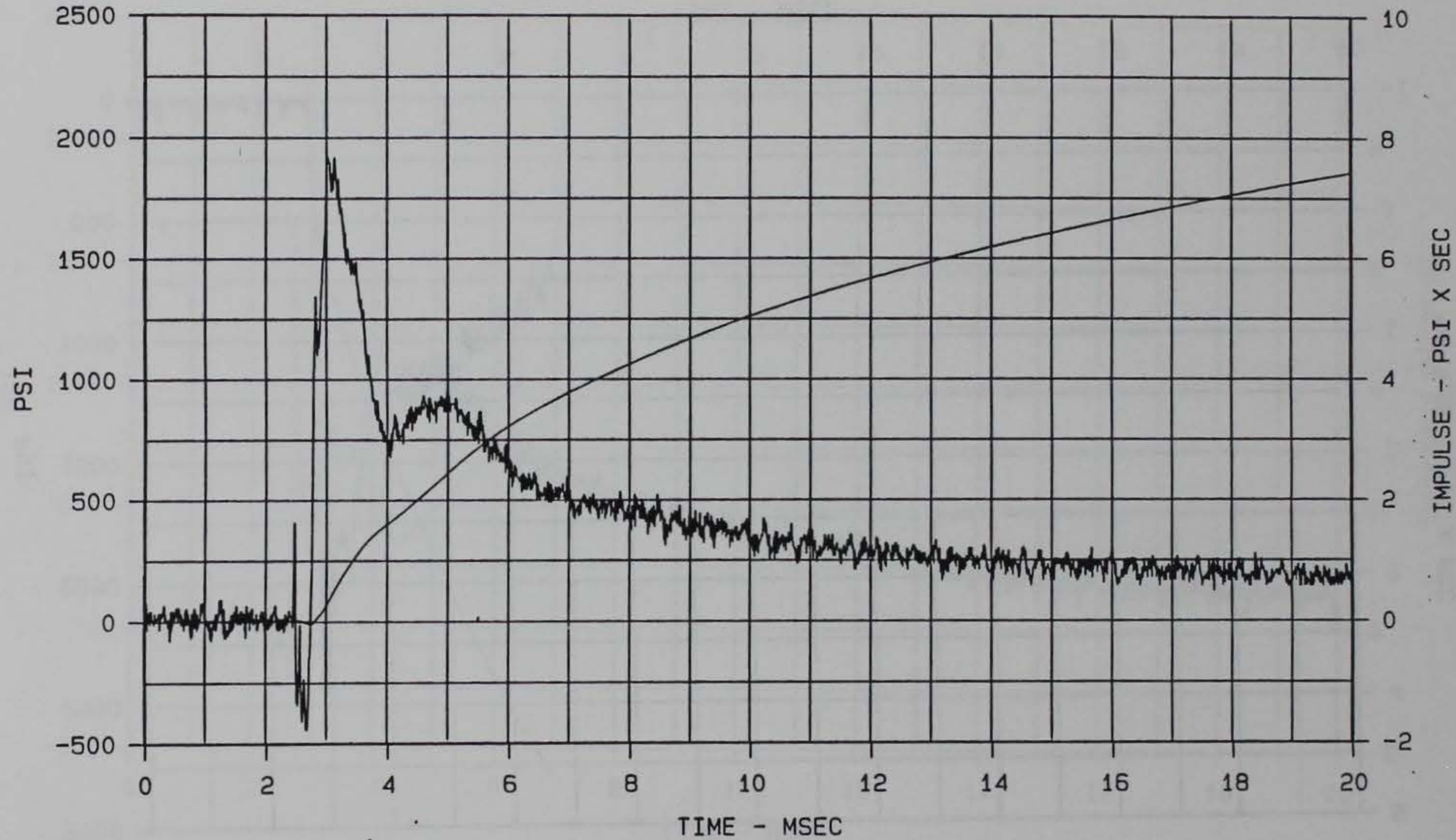
Figure 79. Soil stress wave form measured by gage SEH-1, 20 msec duration, MCBI Gage Validation Test 1
