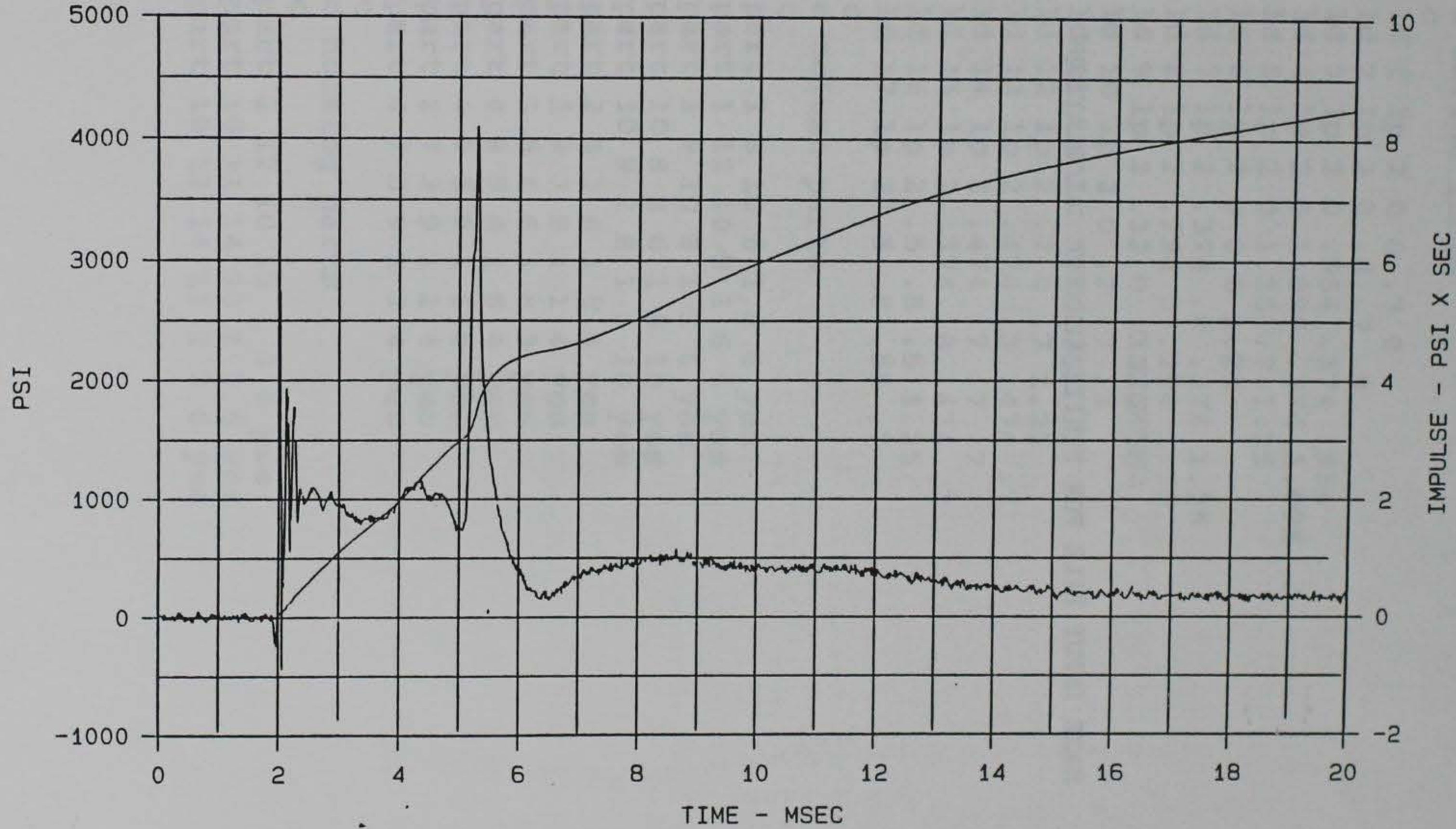
Figure 91. Soil stress wave form measured by gage SEV-3, 20 msec duration, MCBI Gage Validation Test 2
