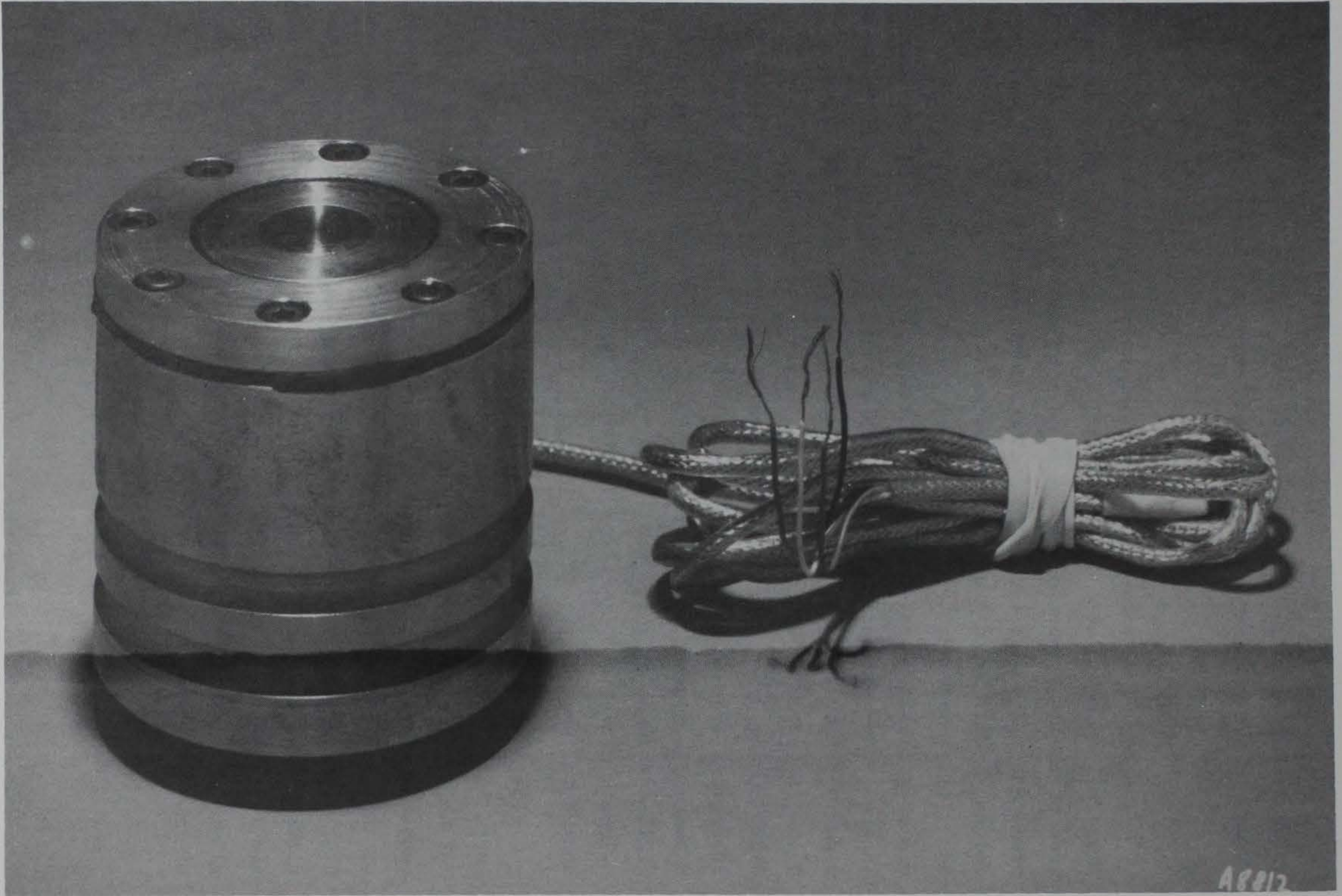
Figure 3. Fully assembled MCBI gage and mount
