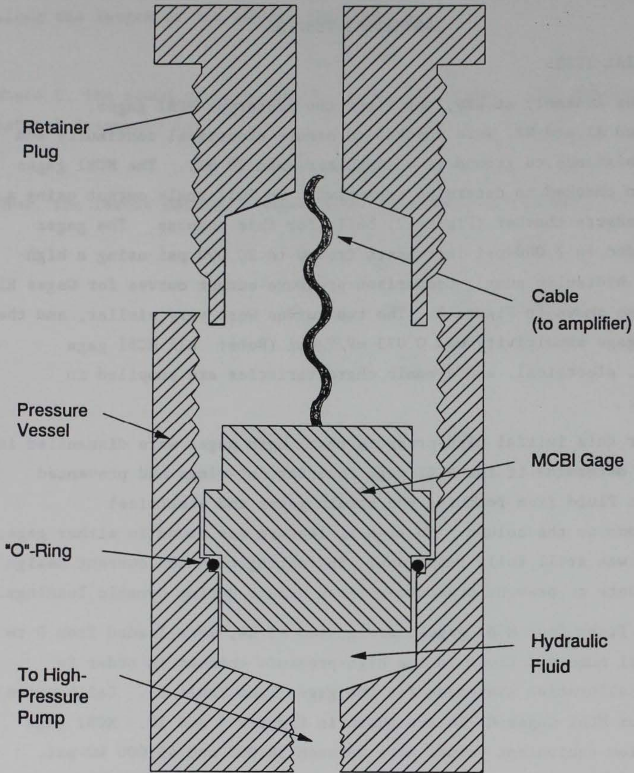
Figure 7. MCBI gage calibration vessel
