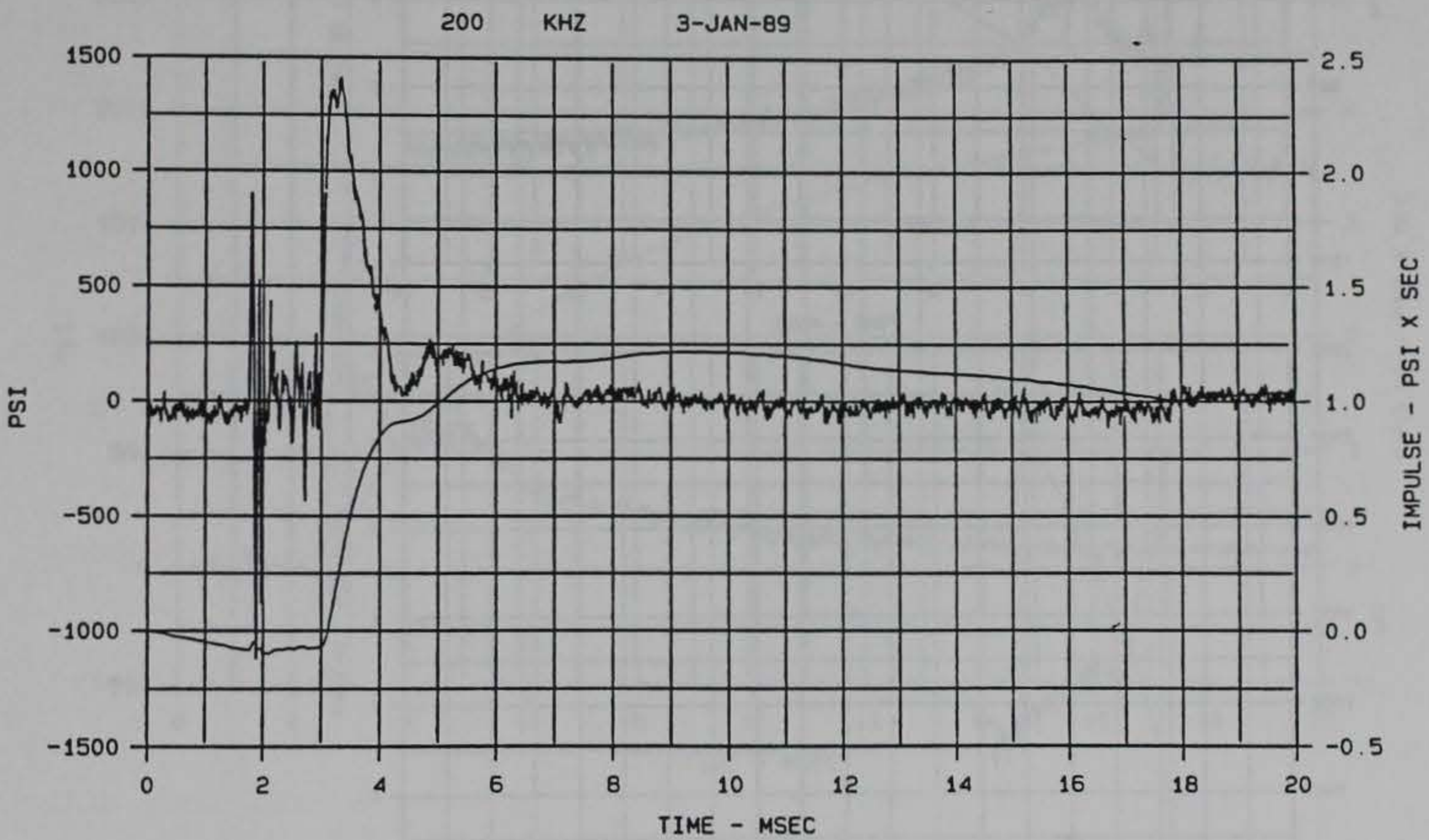
Figure 32. Comparison of MCBI-2 (bottom) and Kulite VM-2 interface stress records, 20 msec duration, MCBI Gage Validation Test 1
