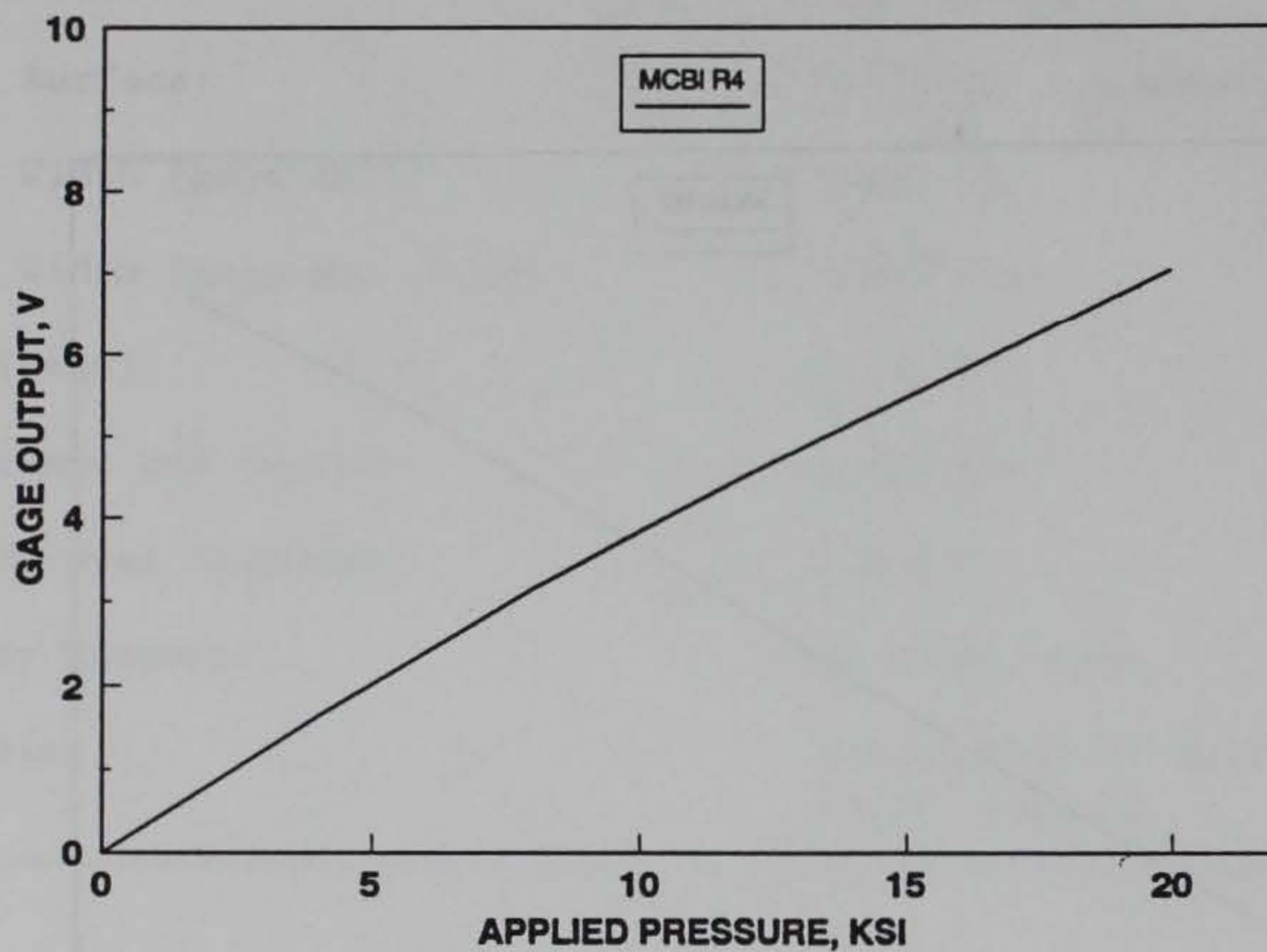
Figure 10. Calibration record for MCBI gages R3 (top) and R4
