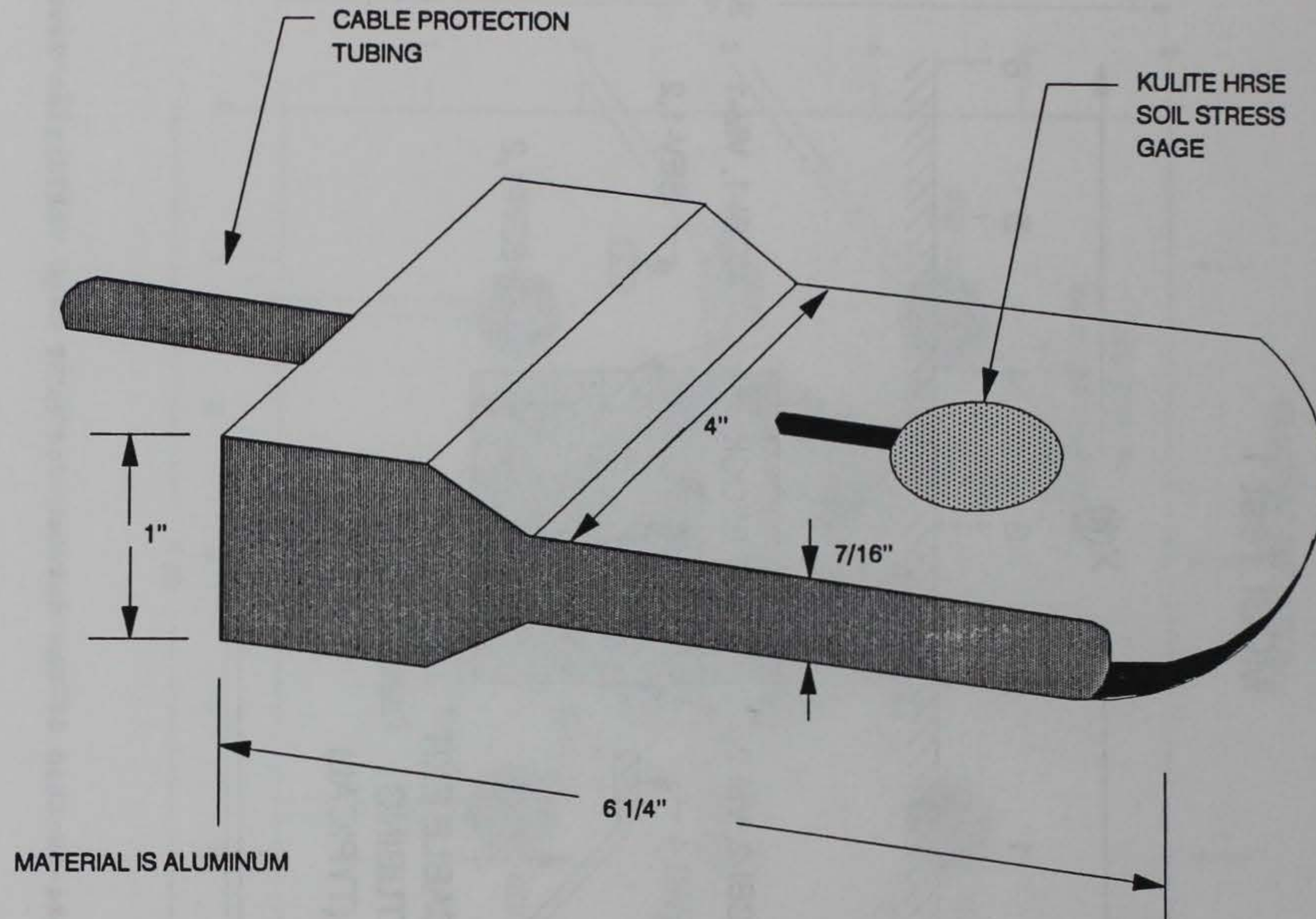
Figure 28. Kulite high-range soil stress gage and WES-designed "paddle" mount
