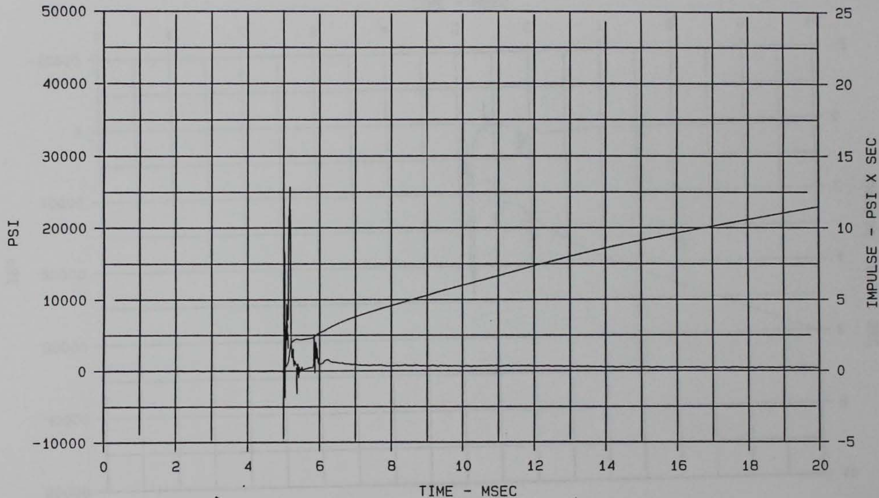
Figure 82. Interface stress wave form measured by gage MCBI-1, 20 msec duration, MCBI Gage Validation Test 2
