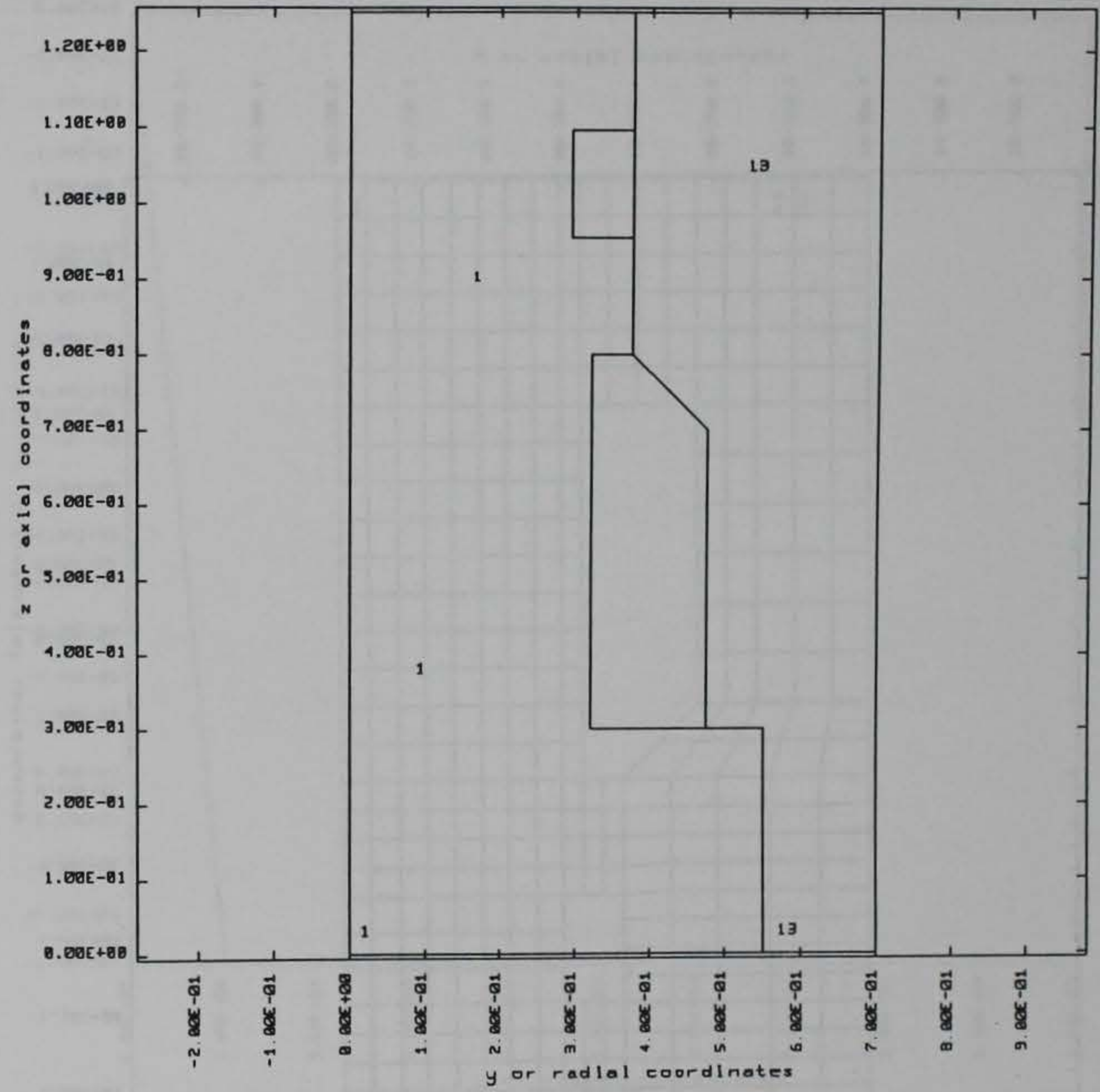
Figure 41. MCBI gage parts modeled using DYNA2D
