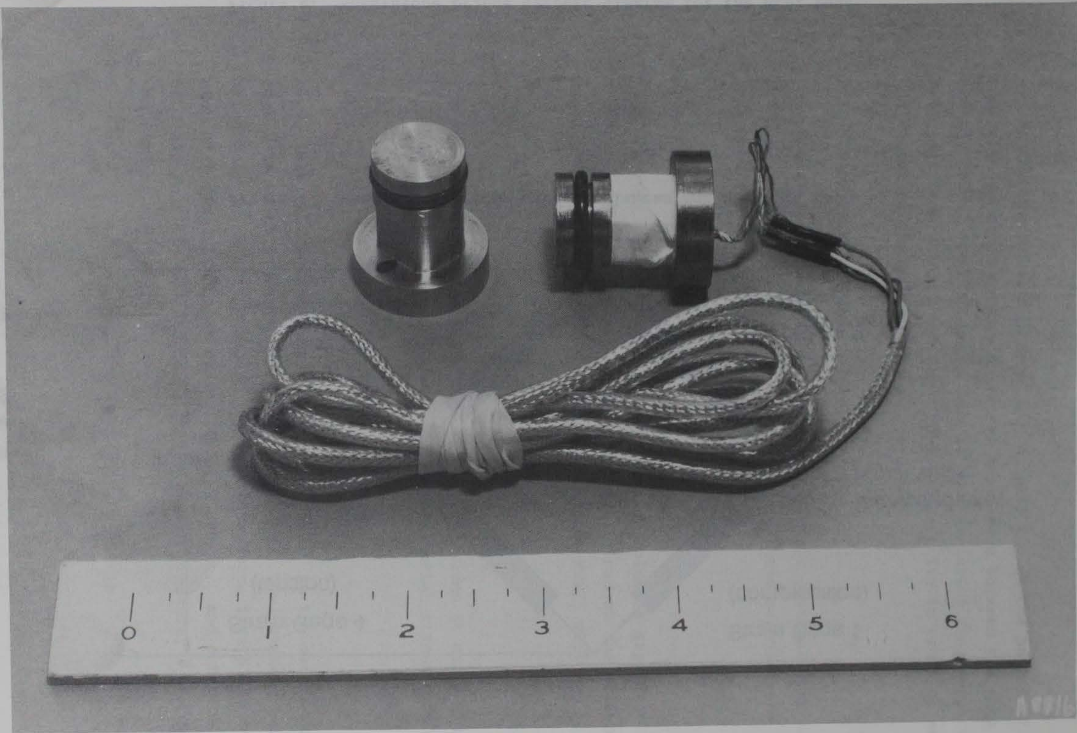
Figure 5. Sensing column before (left) and after strain gaging
