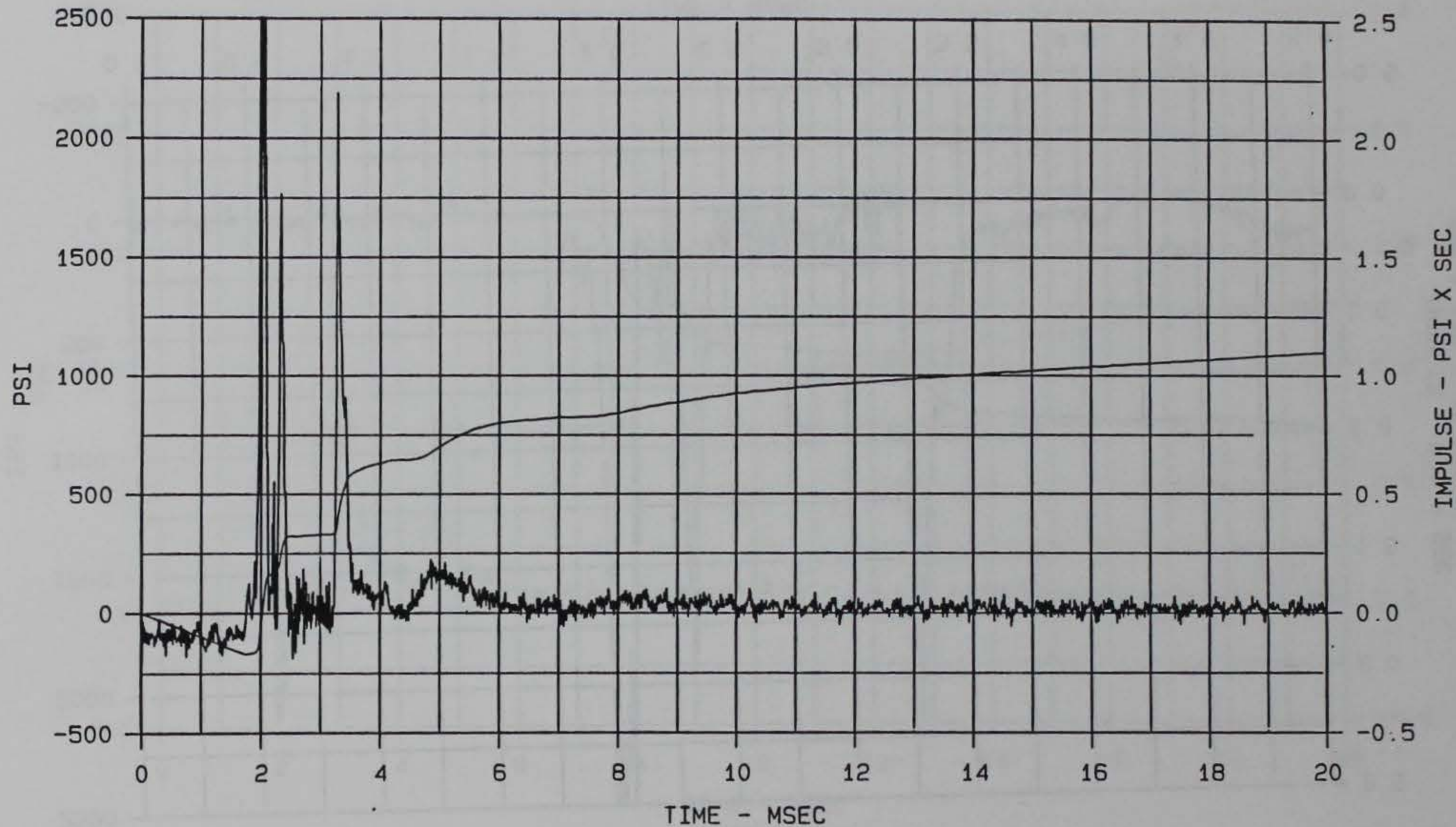
Figure 71. Interface stress wave form measured by gage VM-2, 20 msec duration, MCBI Gage Validation Test 1
