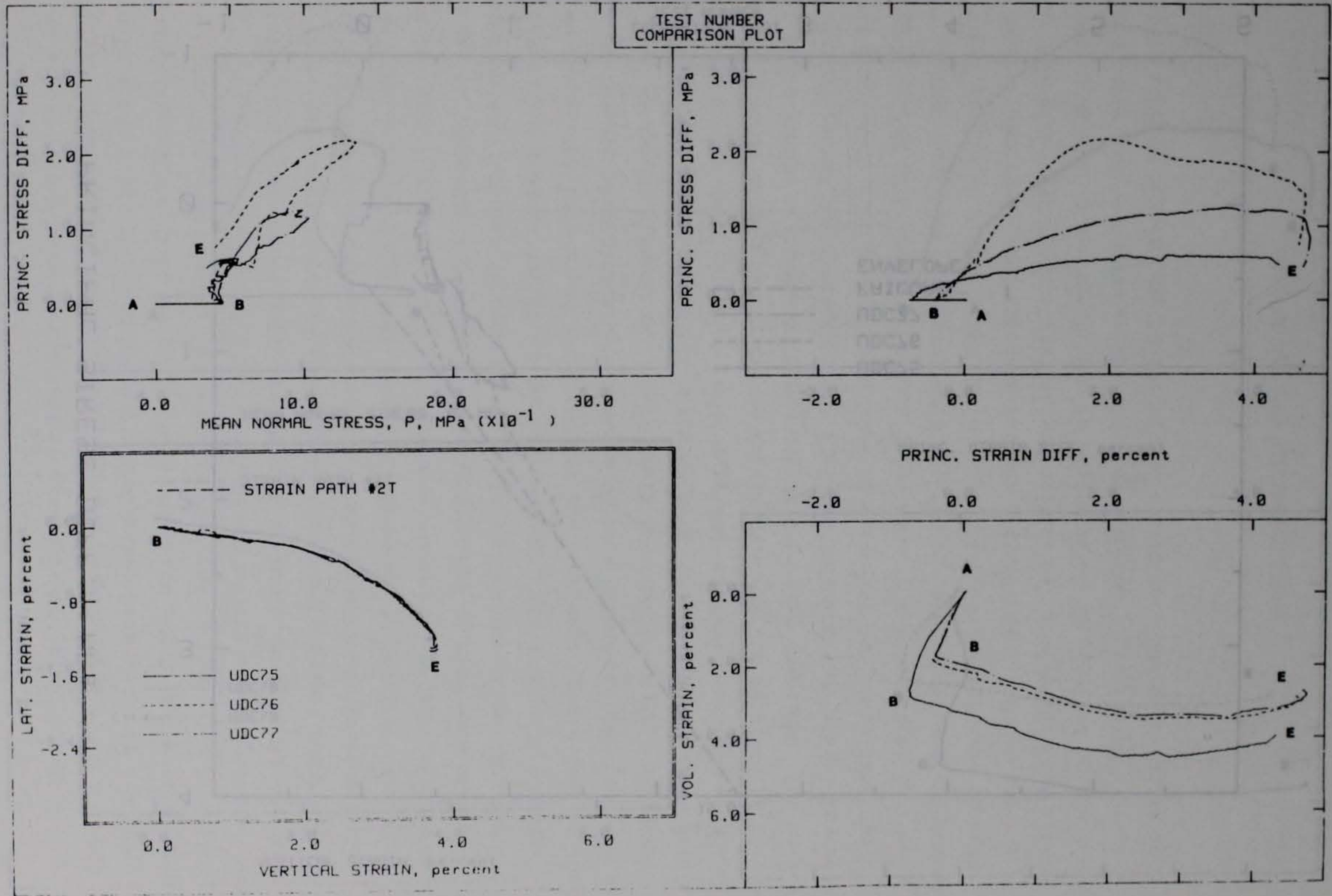
Figure 3.37. Strain path 2T test results at 0.41-MPa prestress.
