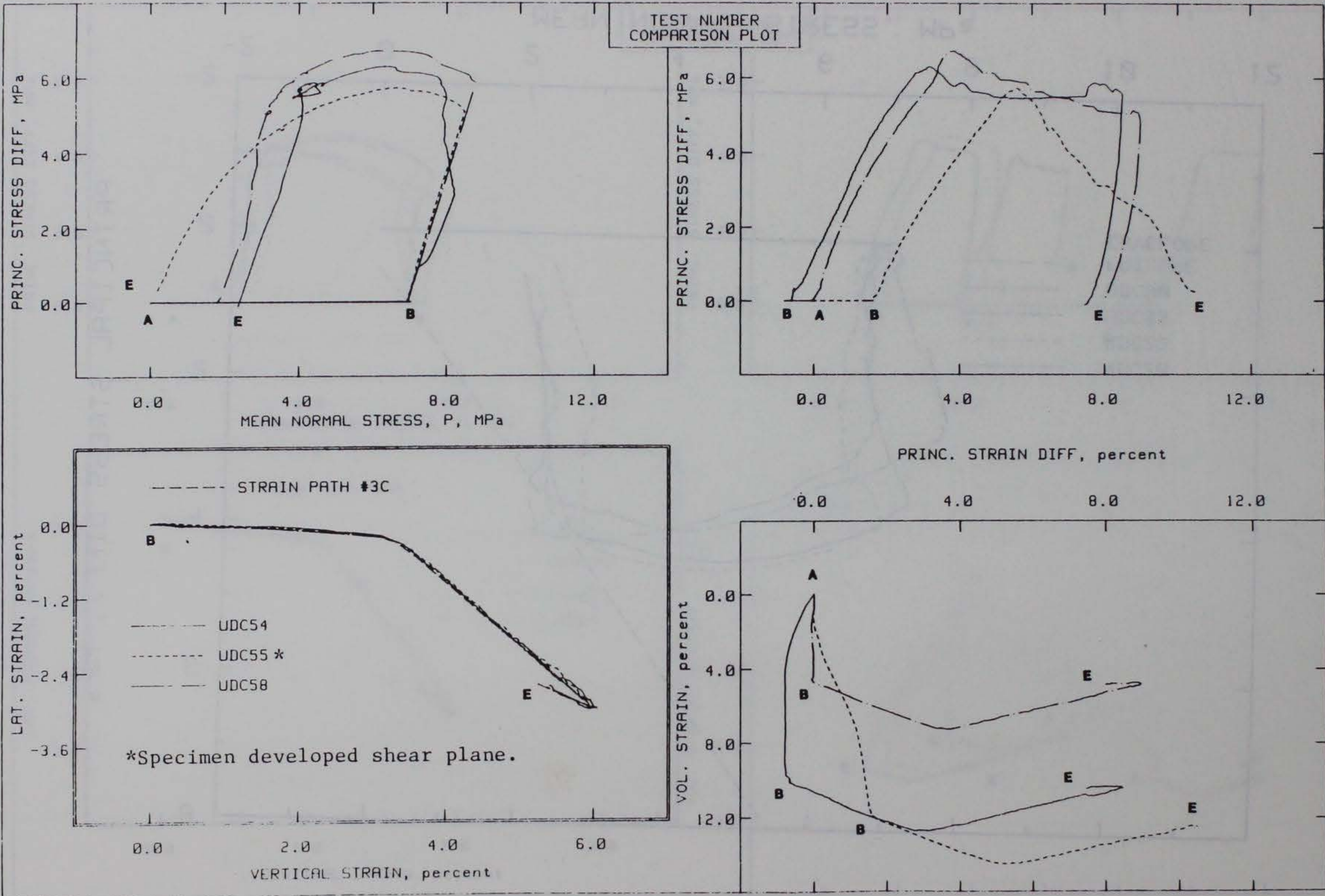
Figure 3.24. Strain path 3C test results from undisturbed specimens.
