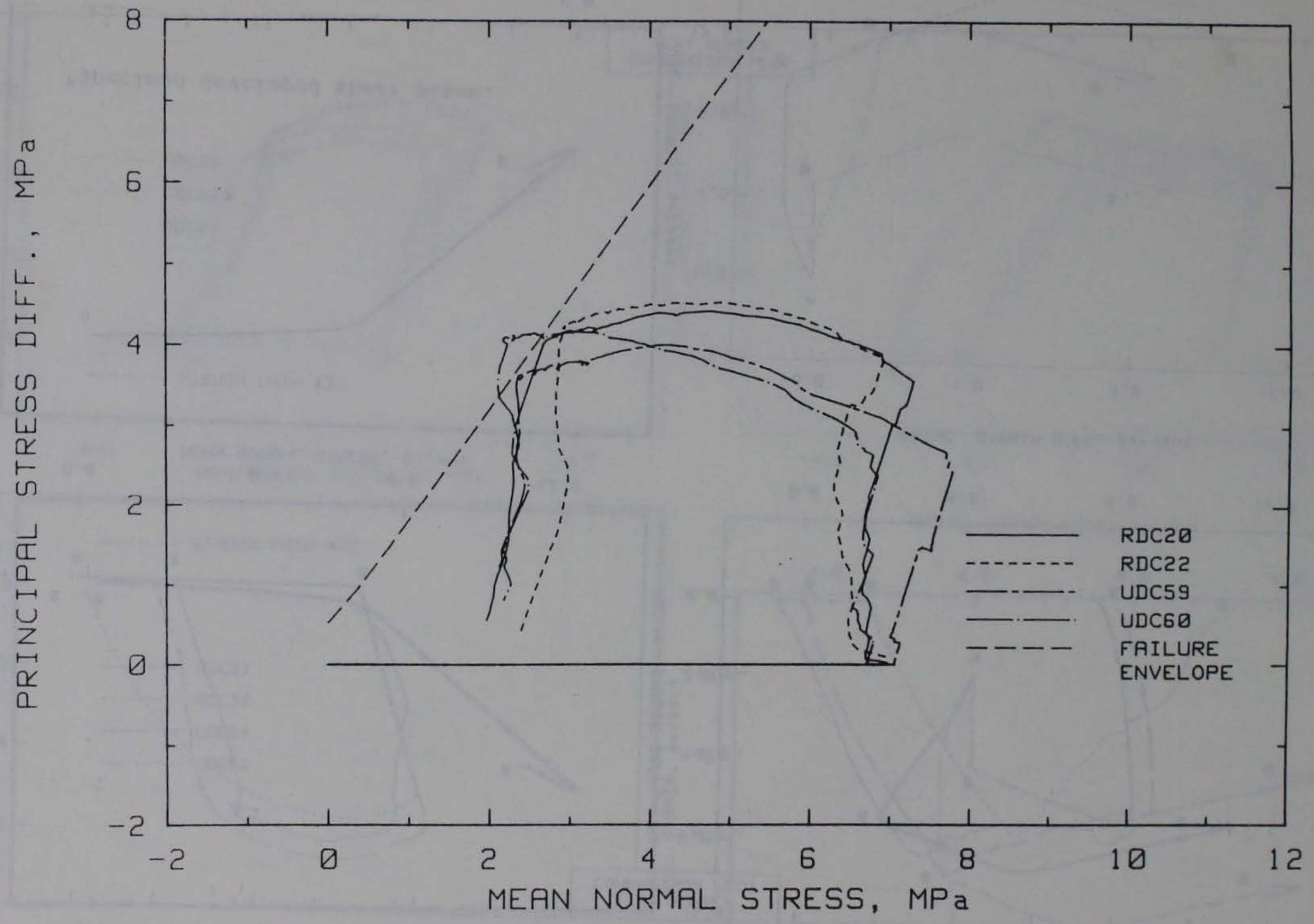
Figure 3.23. Stress paths from remolded and undisturbed specimens following SP3A.
