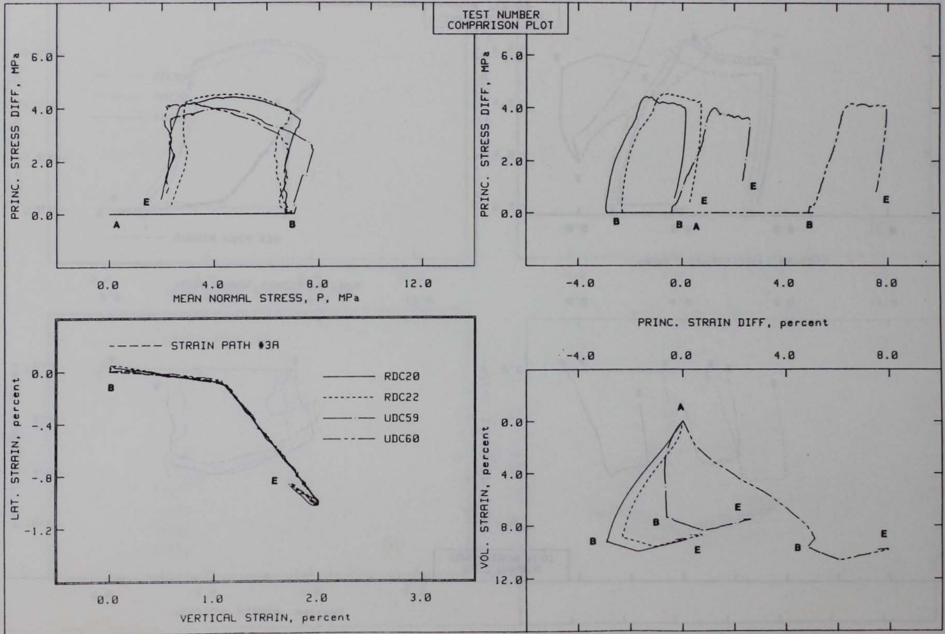
Figure 3.22. Comparison of strain path data from remolded and undisturbed specimens following SP3A.
