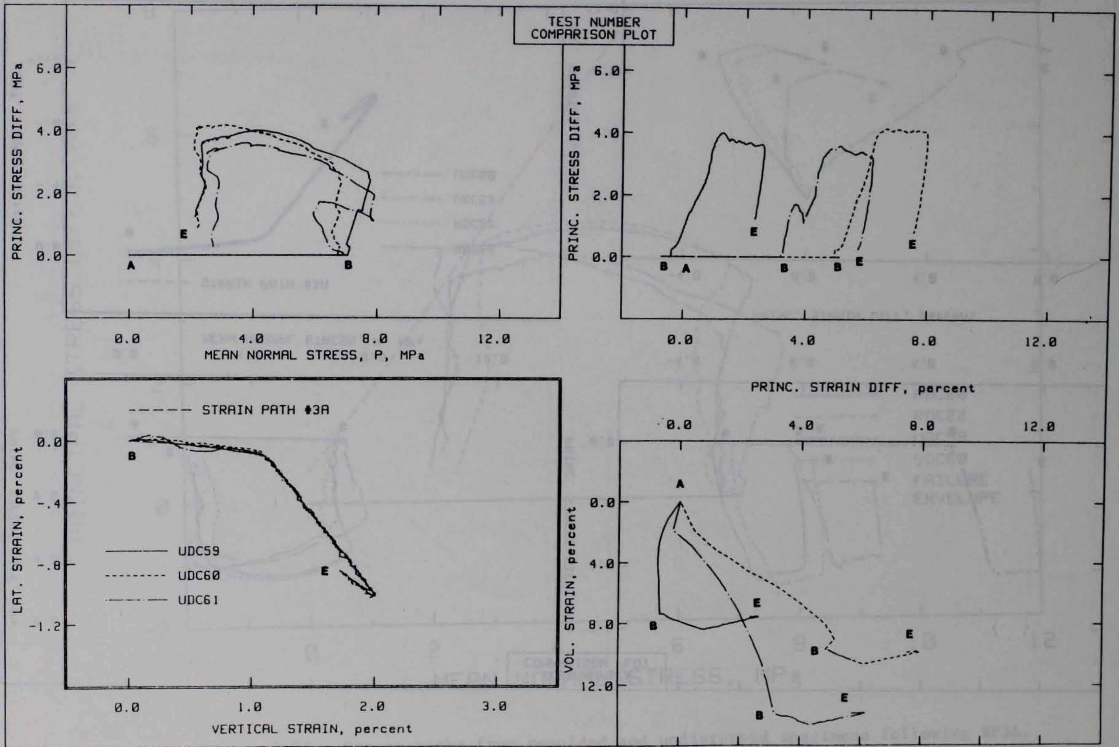
Figure 3.21. Strain path 3A test results from undisturbed specimens.
