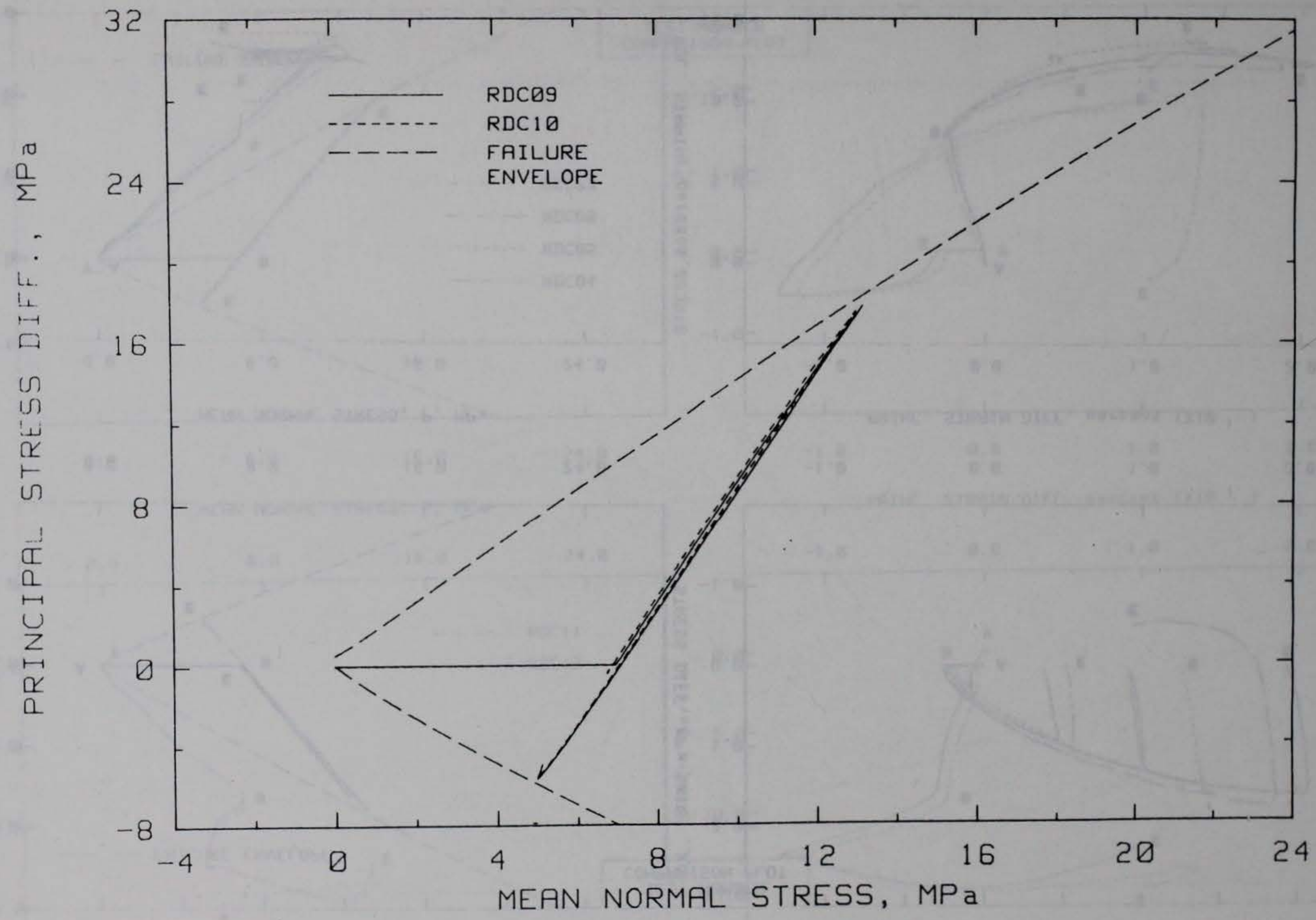
Figure 3.5. Stress paths from combined CTC/RTE tests.
