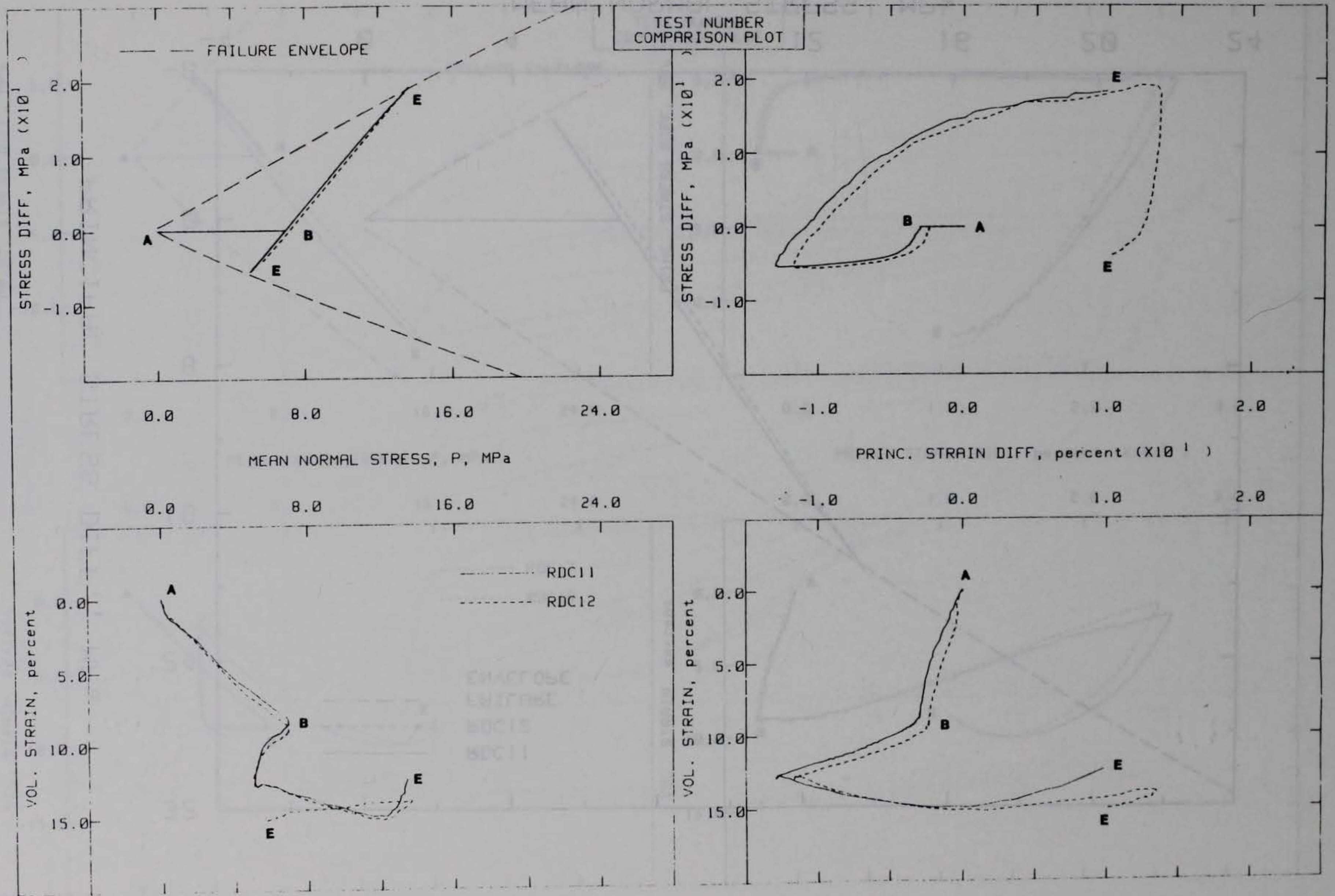
Figure 3.7. Combined RTE/CTC test results.
