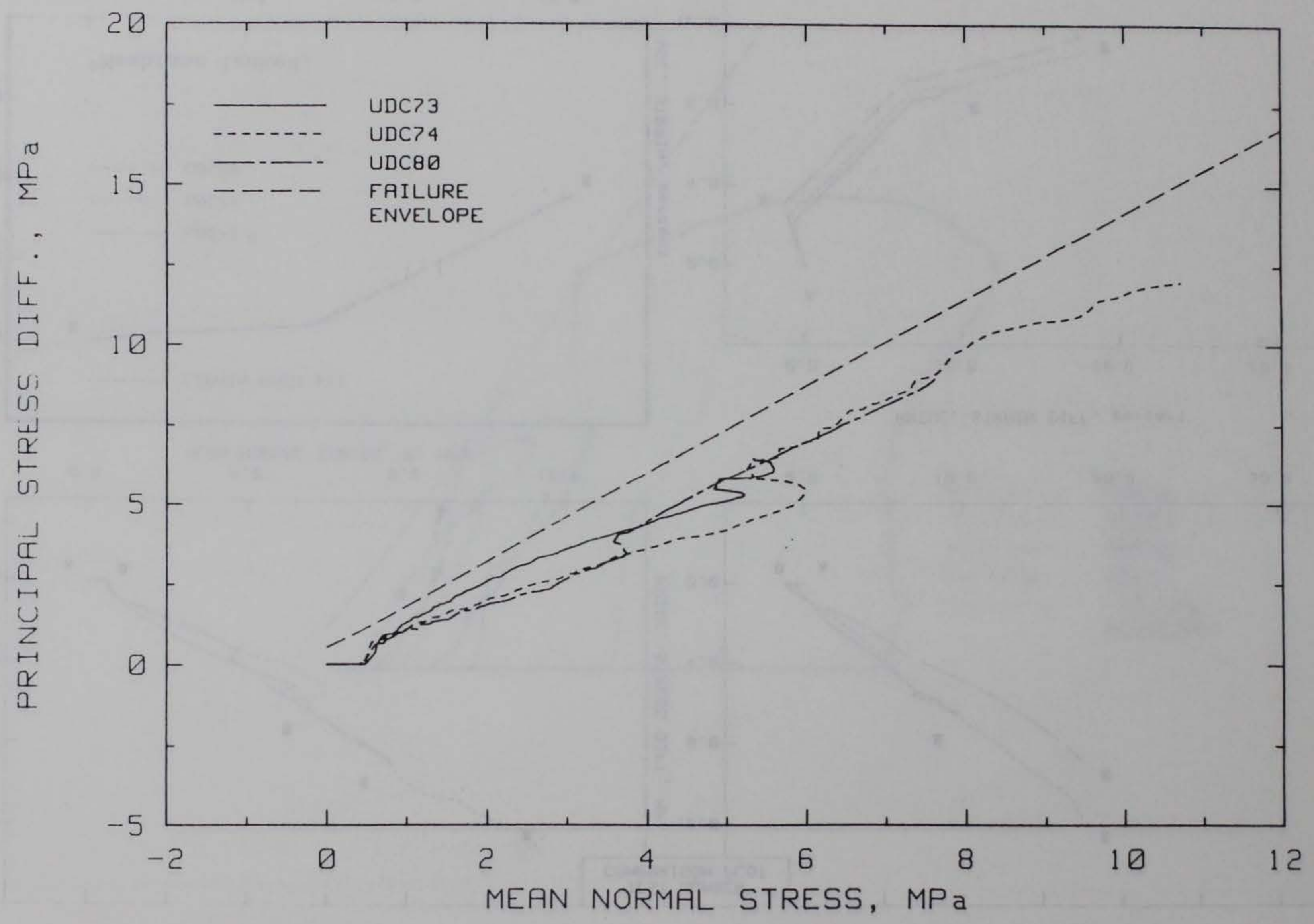
Figure 3.36. Stress paths from tests following SPIT.
