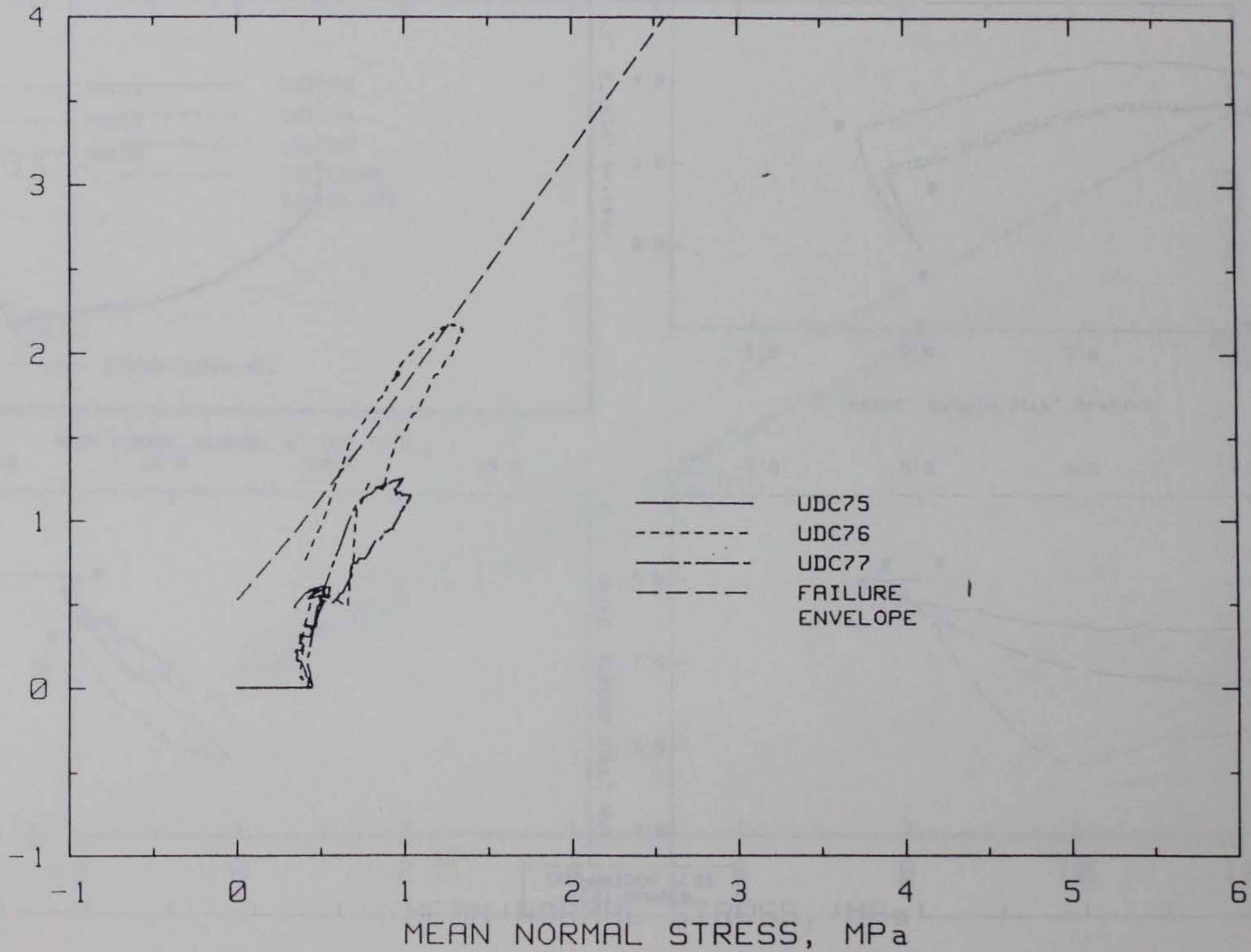
Figure 3.38. Stress paths from tests following SP2T at 0.41-MPa prestress.
