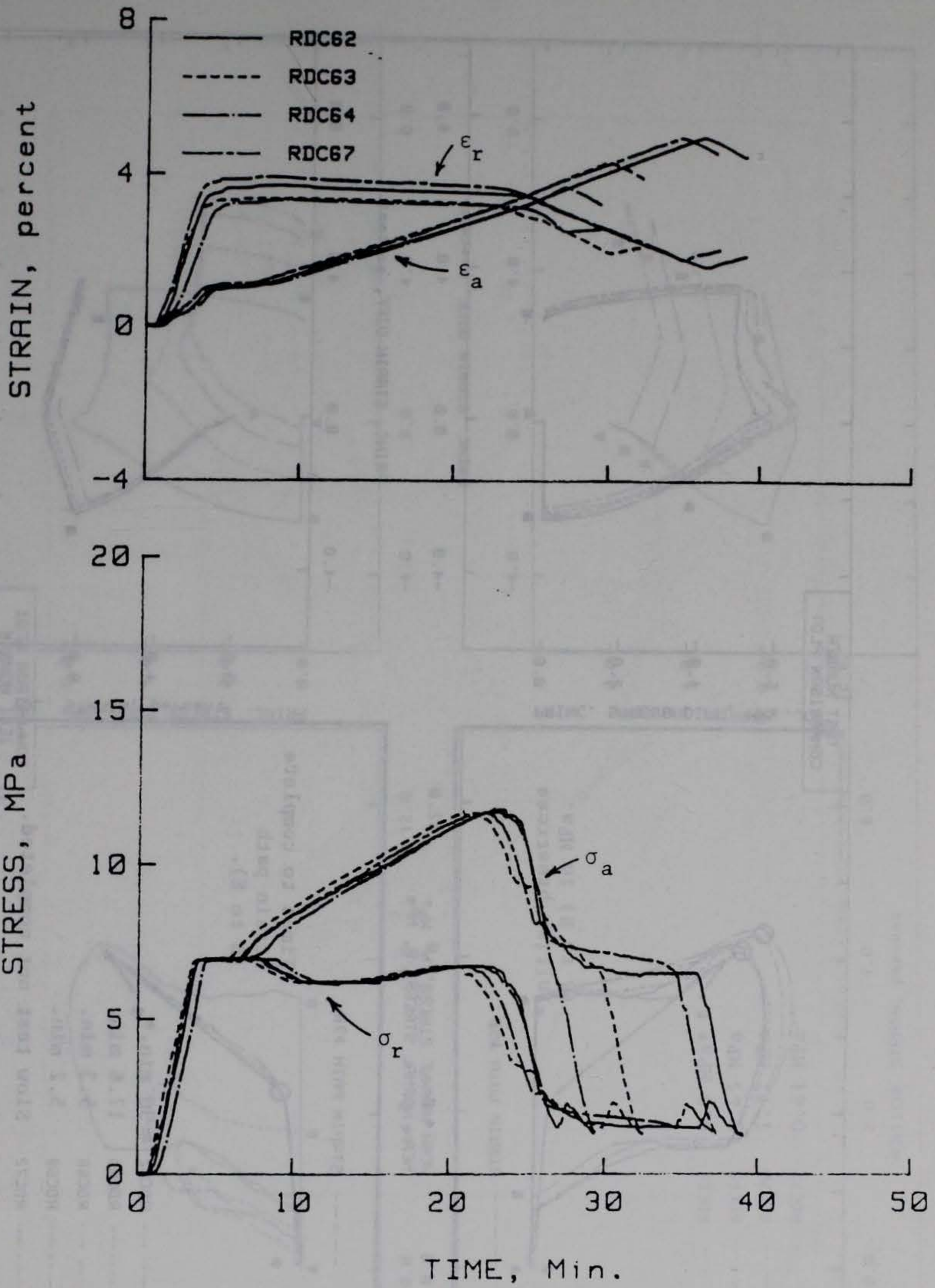
Figure 3.31. Stress-strain-time histories for reverse strain-path tests.
