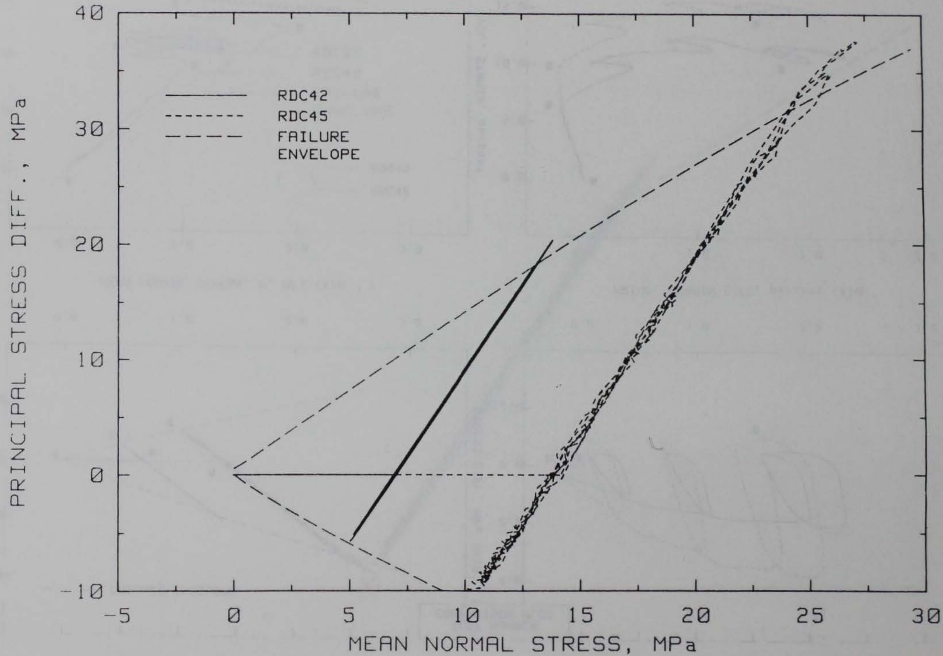
Figure 3.14. Stress paths from unload-reload CTC/RTE tests at 6.9 and 13.8 MPa.
