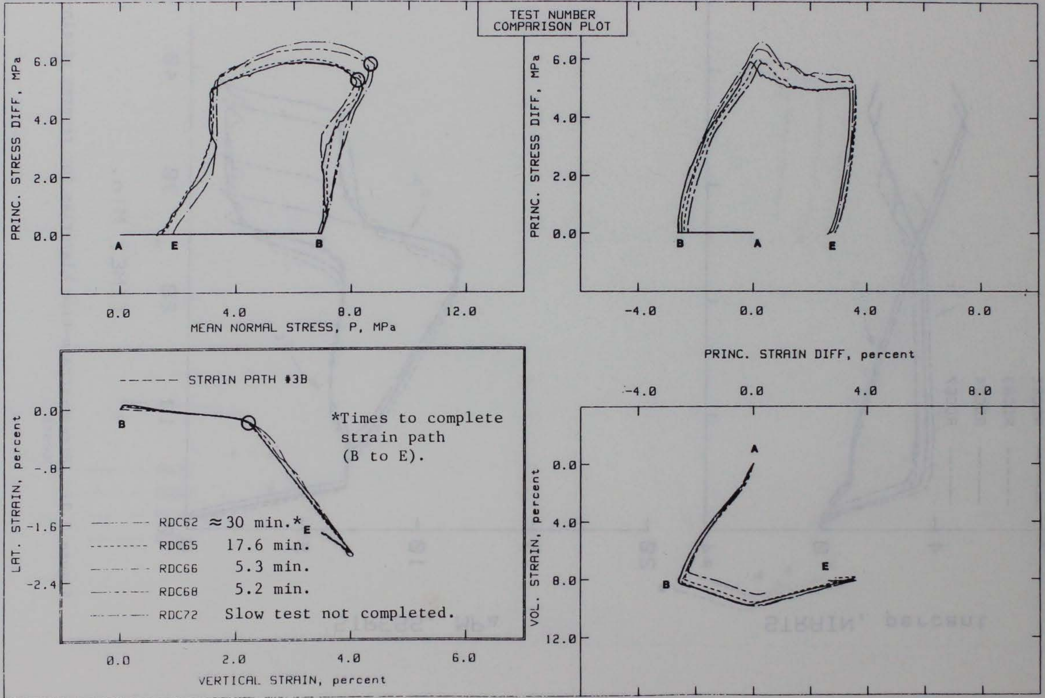
Figure 3.32. Strain-rate test results.
