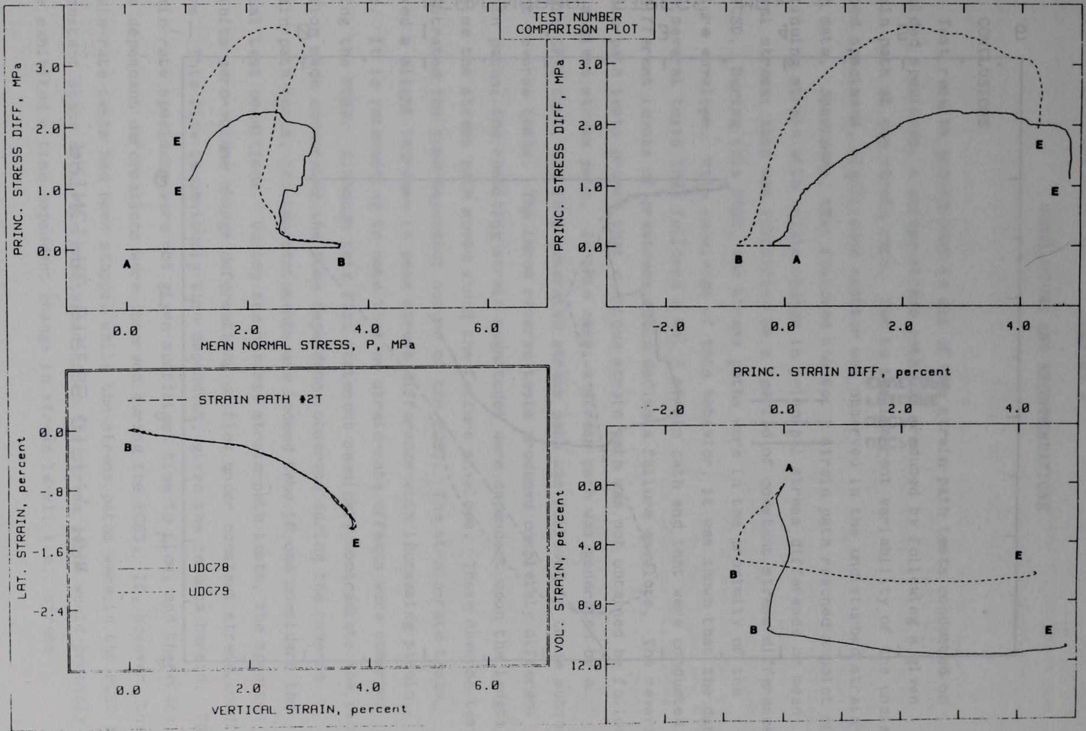
Figure 3.39. Strain path 2T test results at 3.45-MPa prestress.
