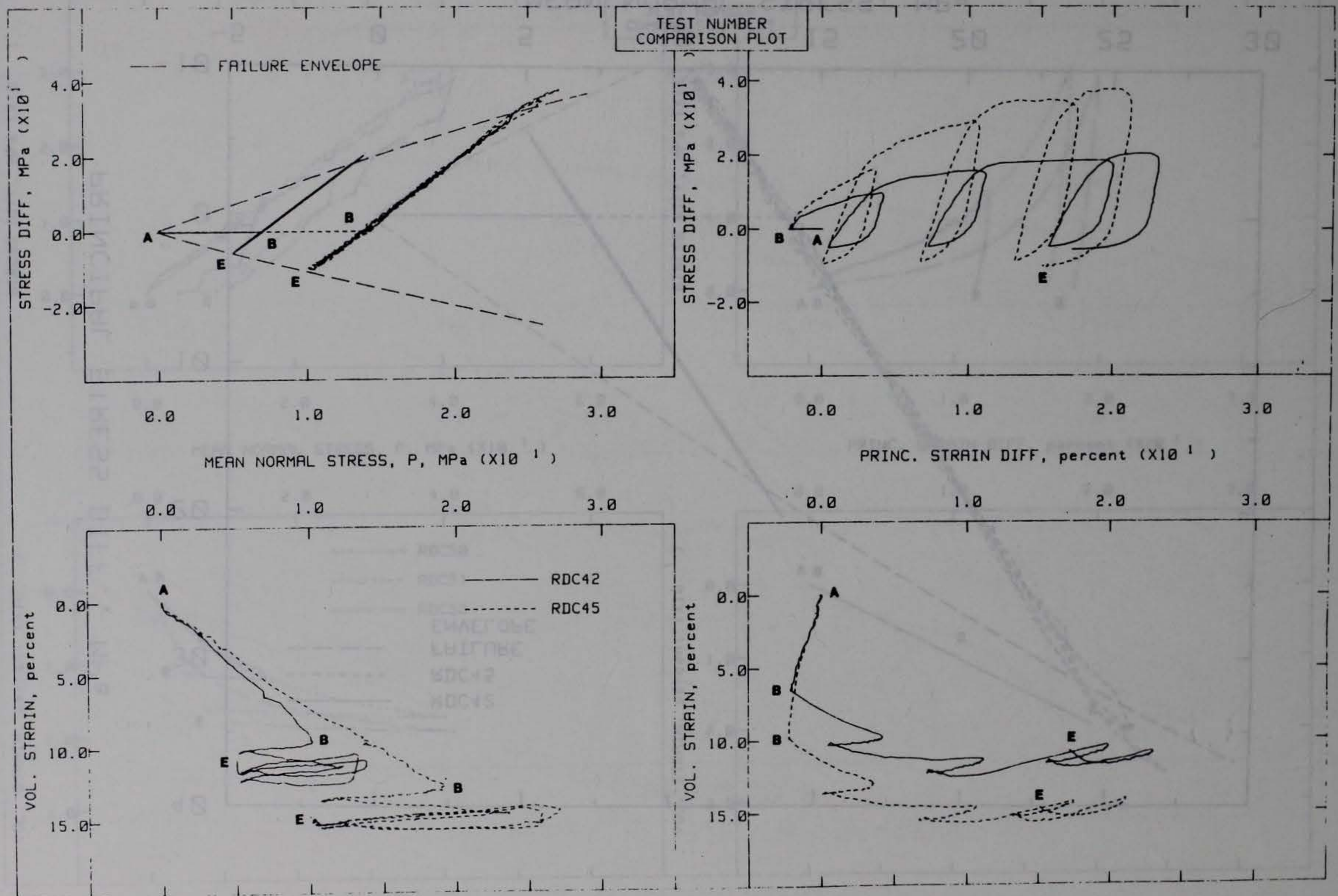
Figure 3.13. Comparison of unload-reload CTC/RTE tests at 6.9 and 13.8 MPa.
