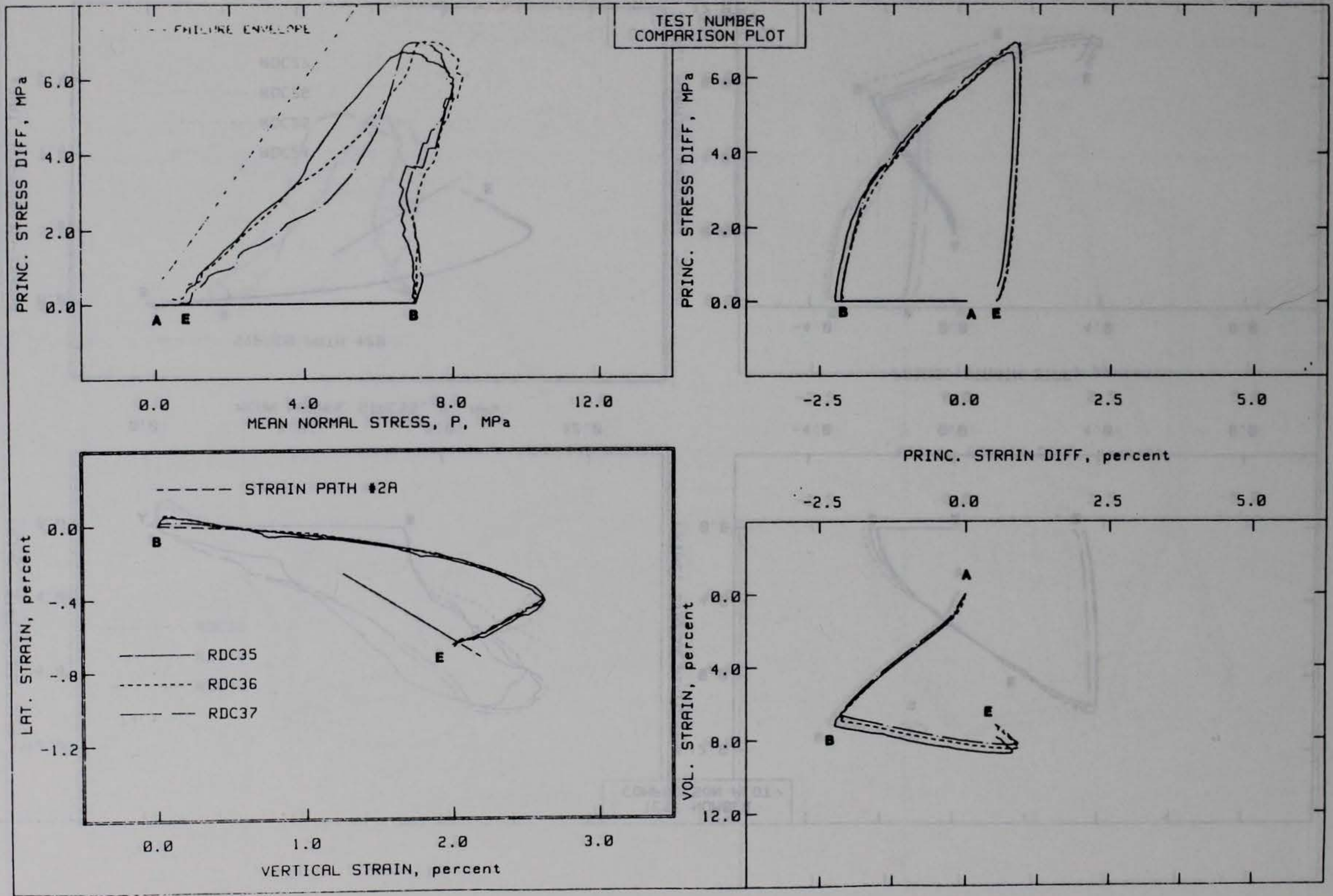
Figure 3.27. Strain path 2A test results.
