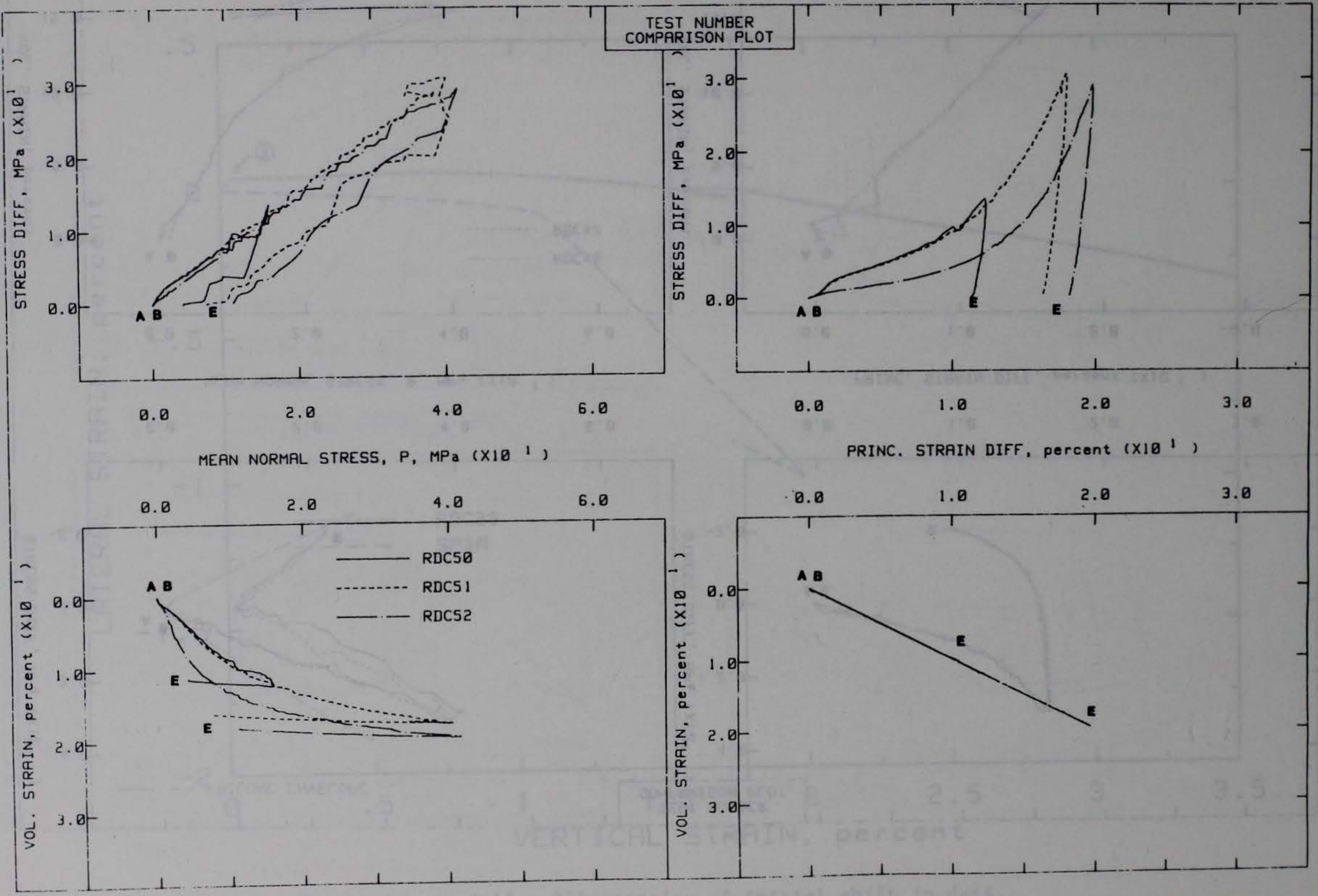
Figure 3.15. UX/K 0 test results.
