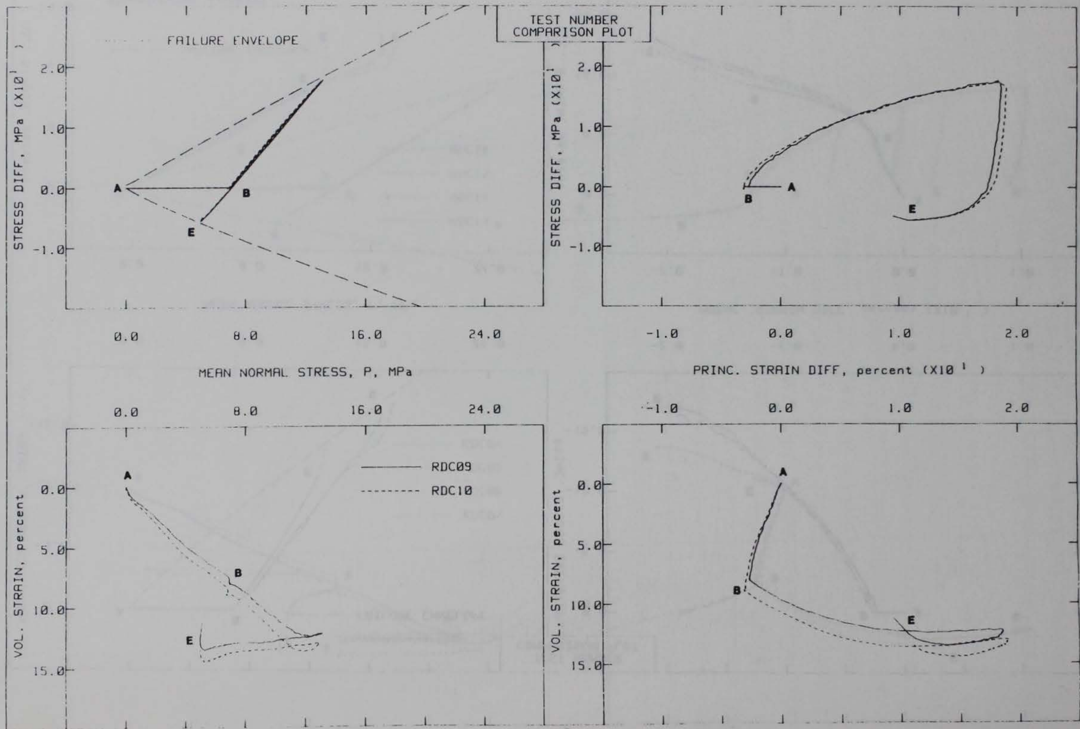
Figure 3.4. Combined CTC/RTE test results.
