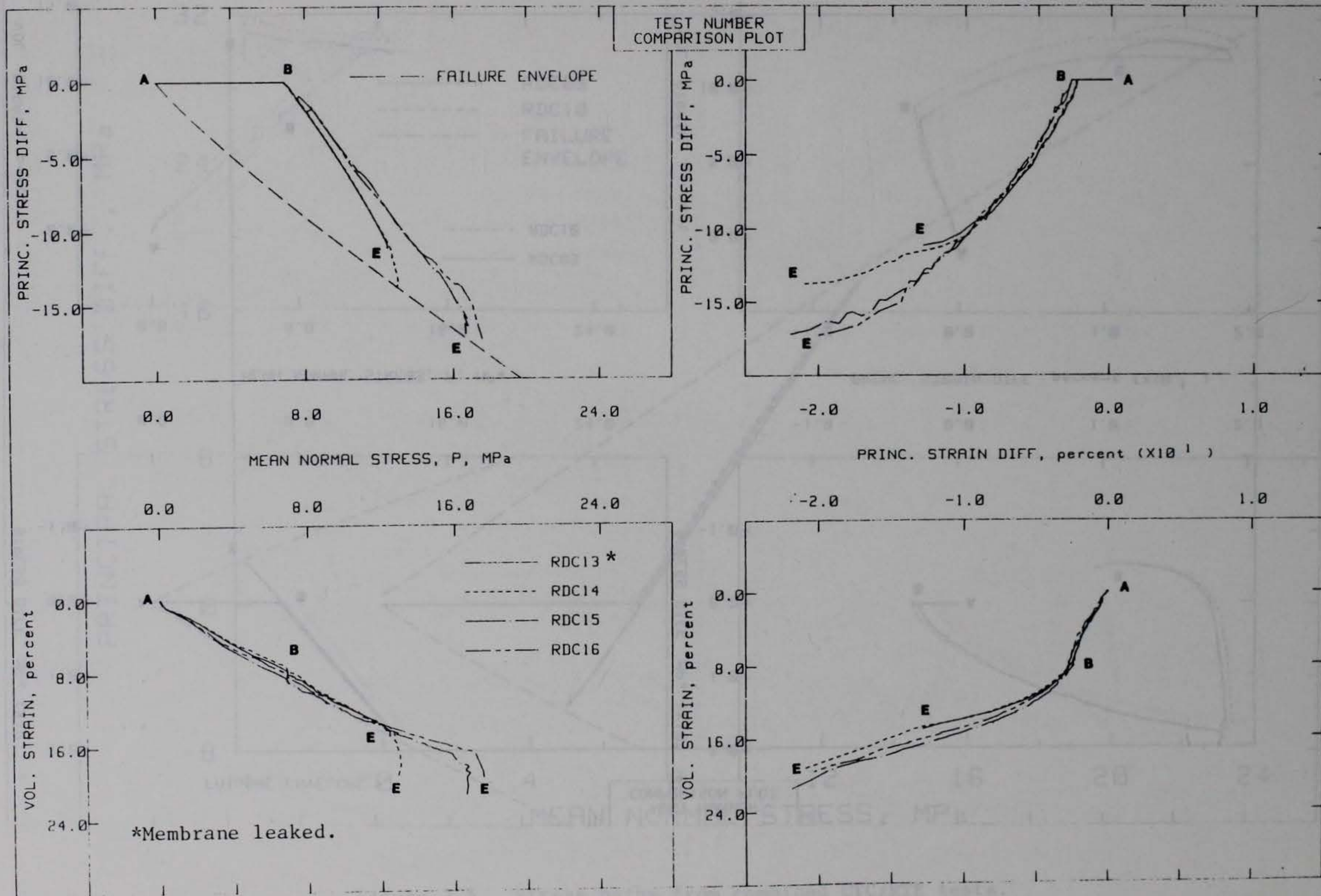
Figure 3.3. CTE test results.
