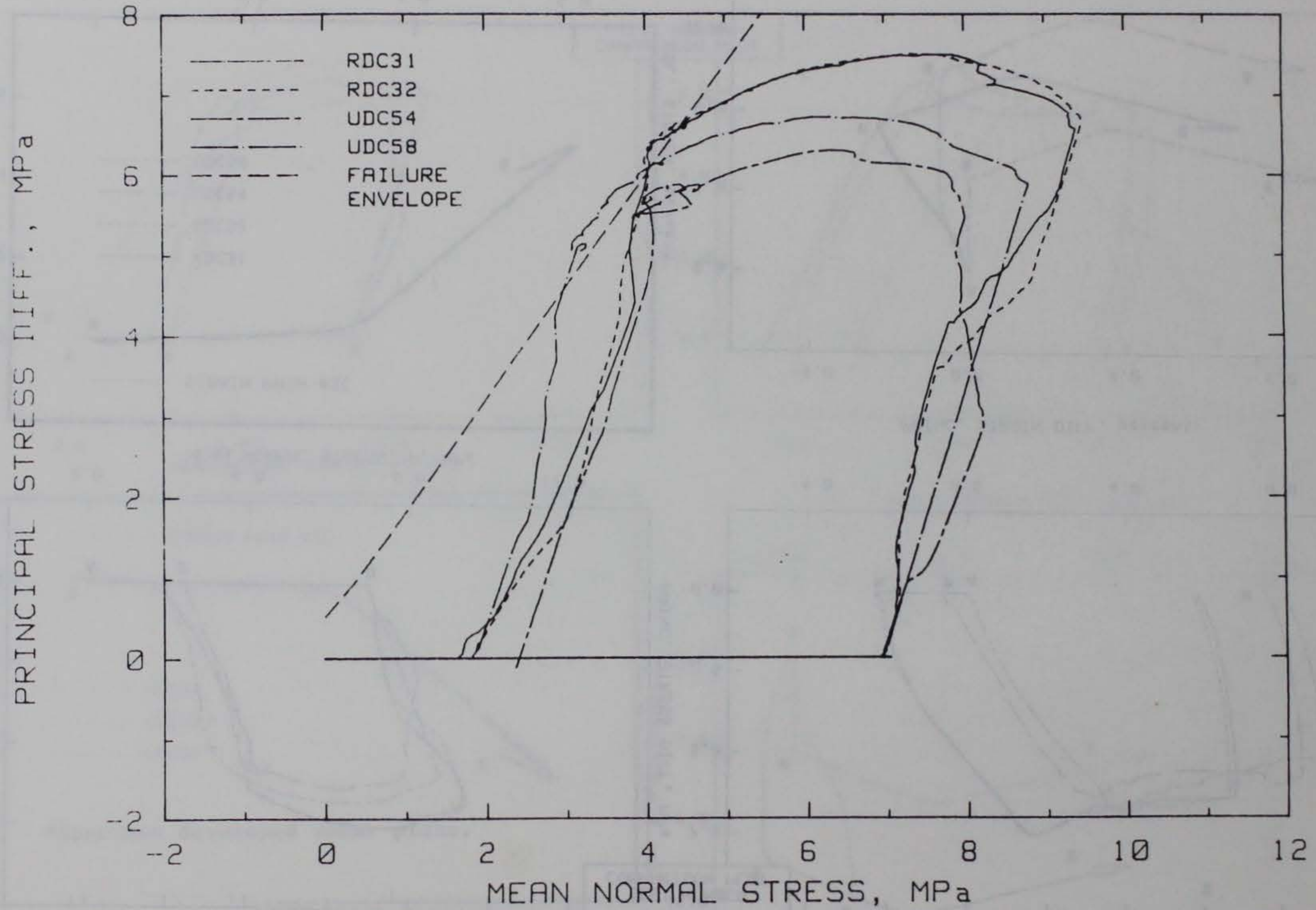
Figure 3.26. Stress paths from remolded and undisturbed specimens following SP3C.
