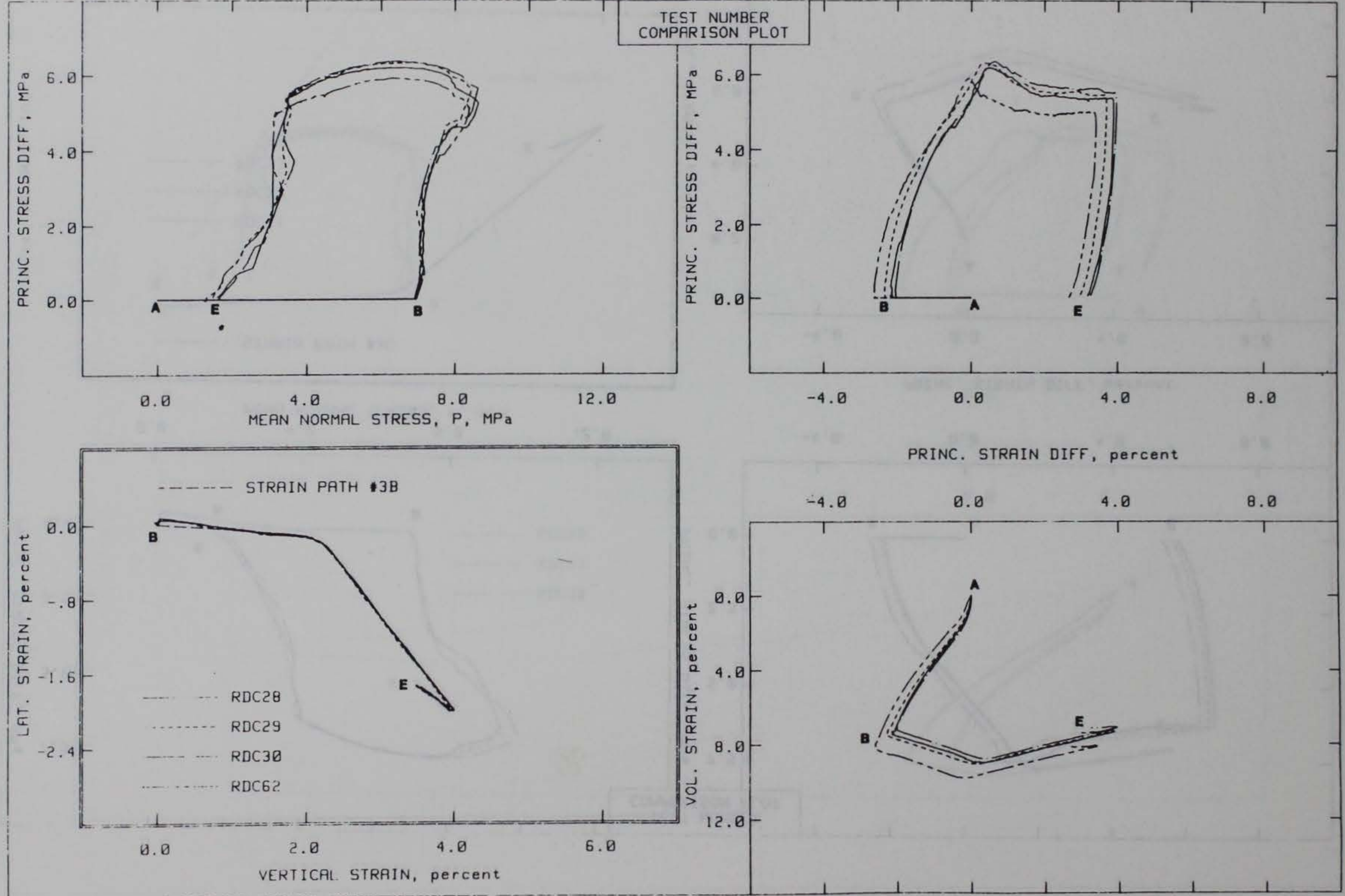
Figure 3.20. Strain path 3B test results from remolded specimens.
