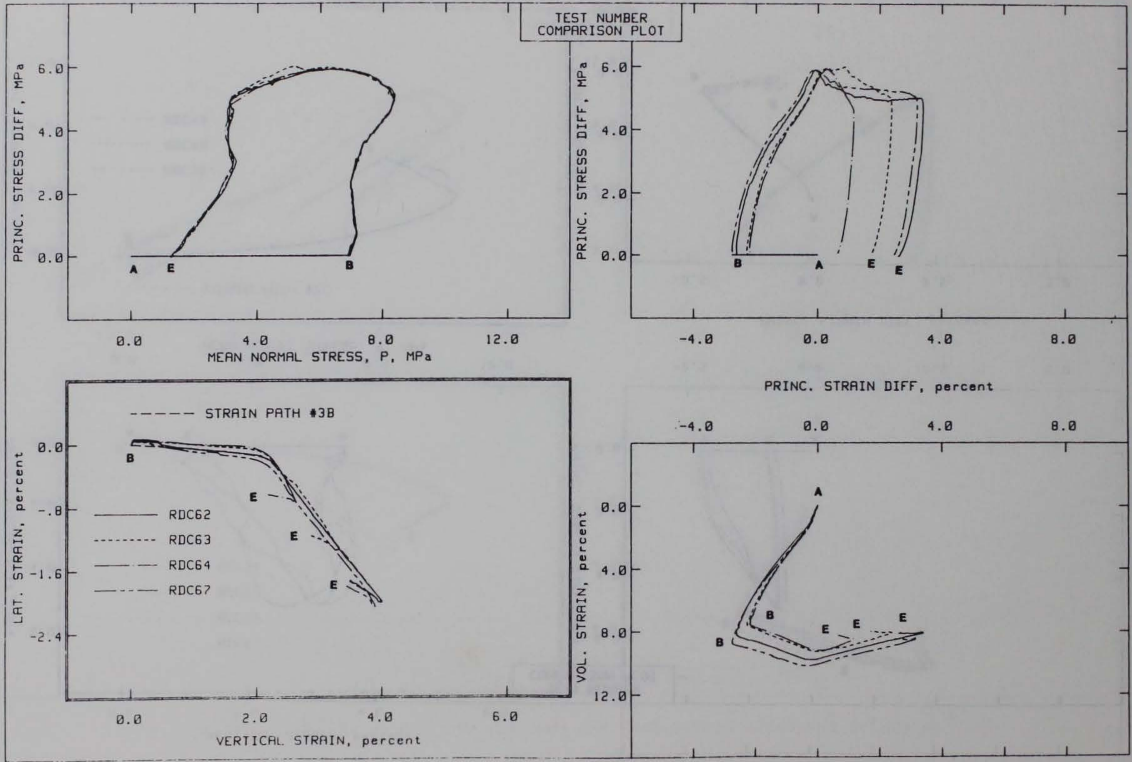
Figure 3.30. Reverse strain path test results.
