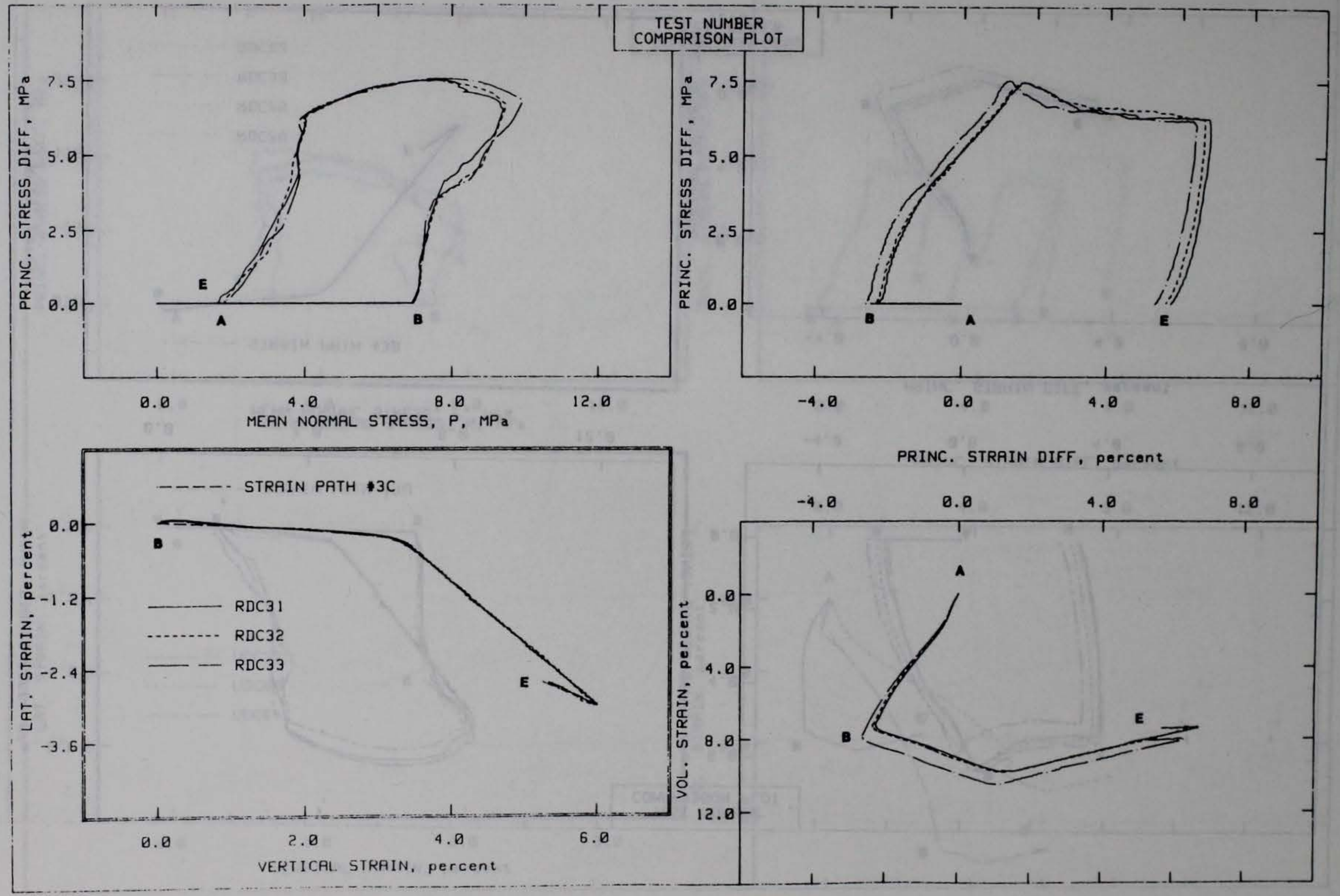
Figure 3.19. Strain path 3C test results from remolded specimens.
