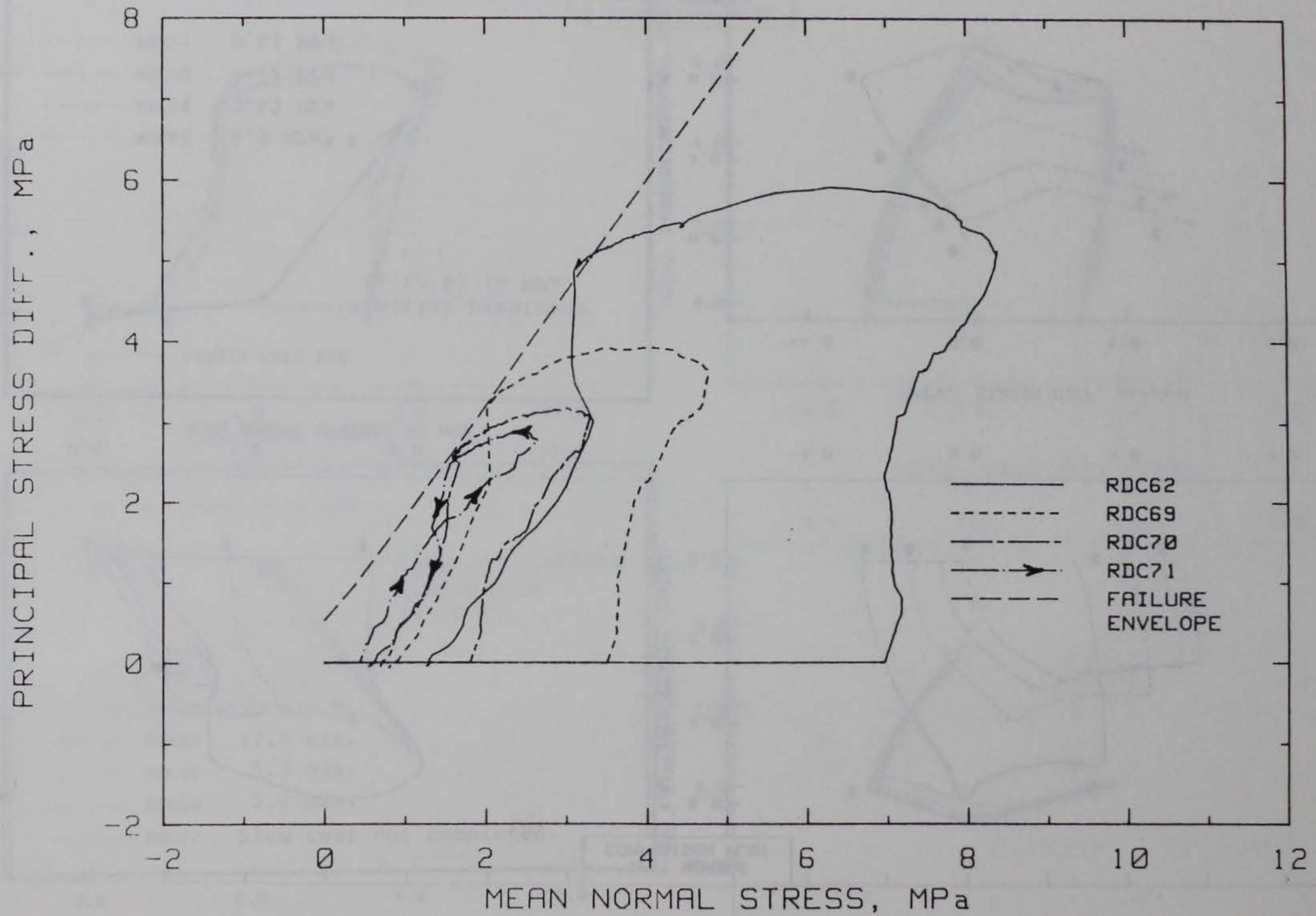
Figure 3.34. Stress paths from strain path tests at different levels of prestress.
