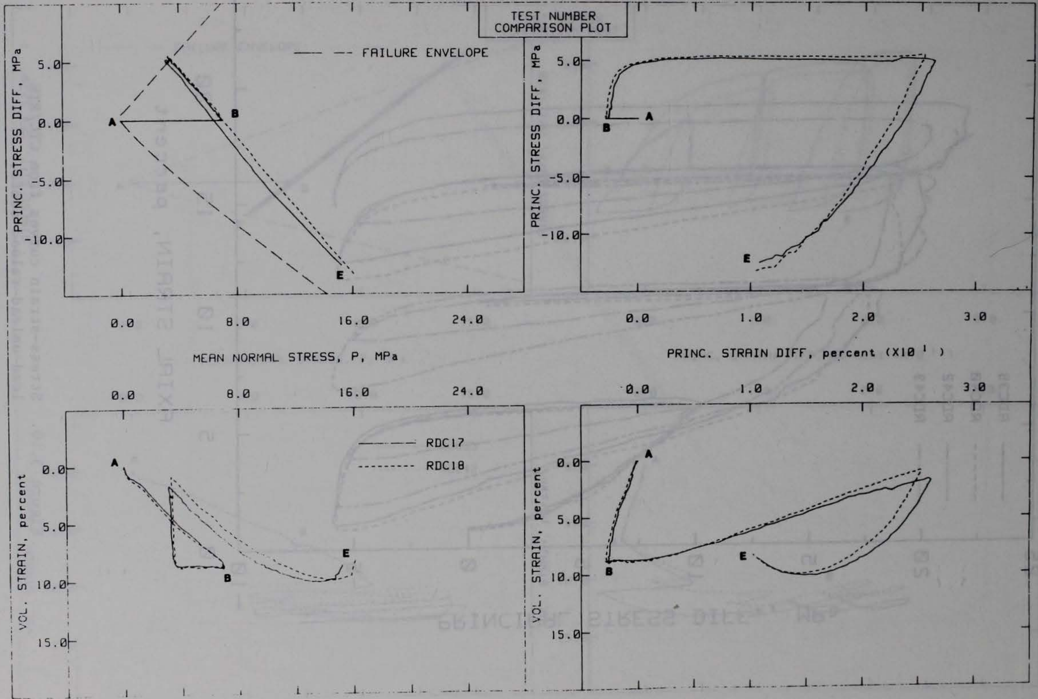
Figure 3.9. Combined RTC/CTE test results.
