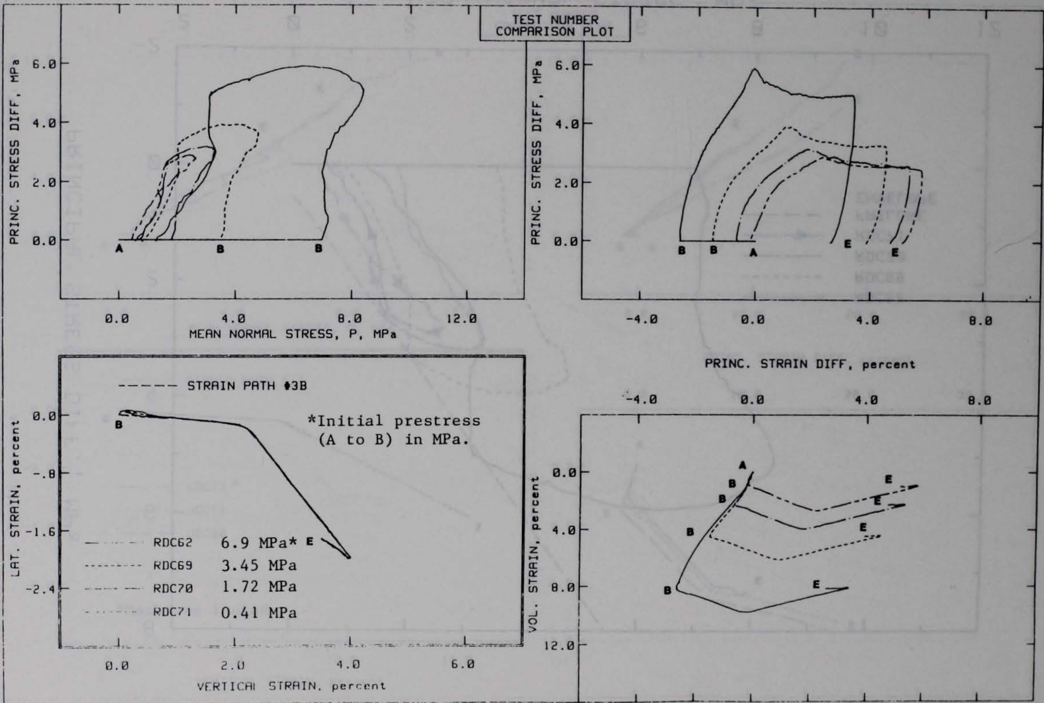
Figure 3.33. Effects of different levels of prestress.
