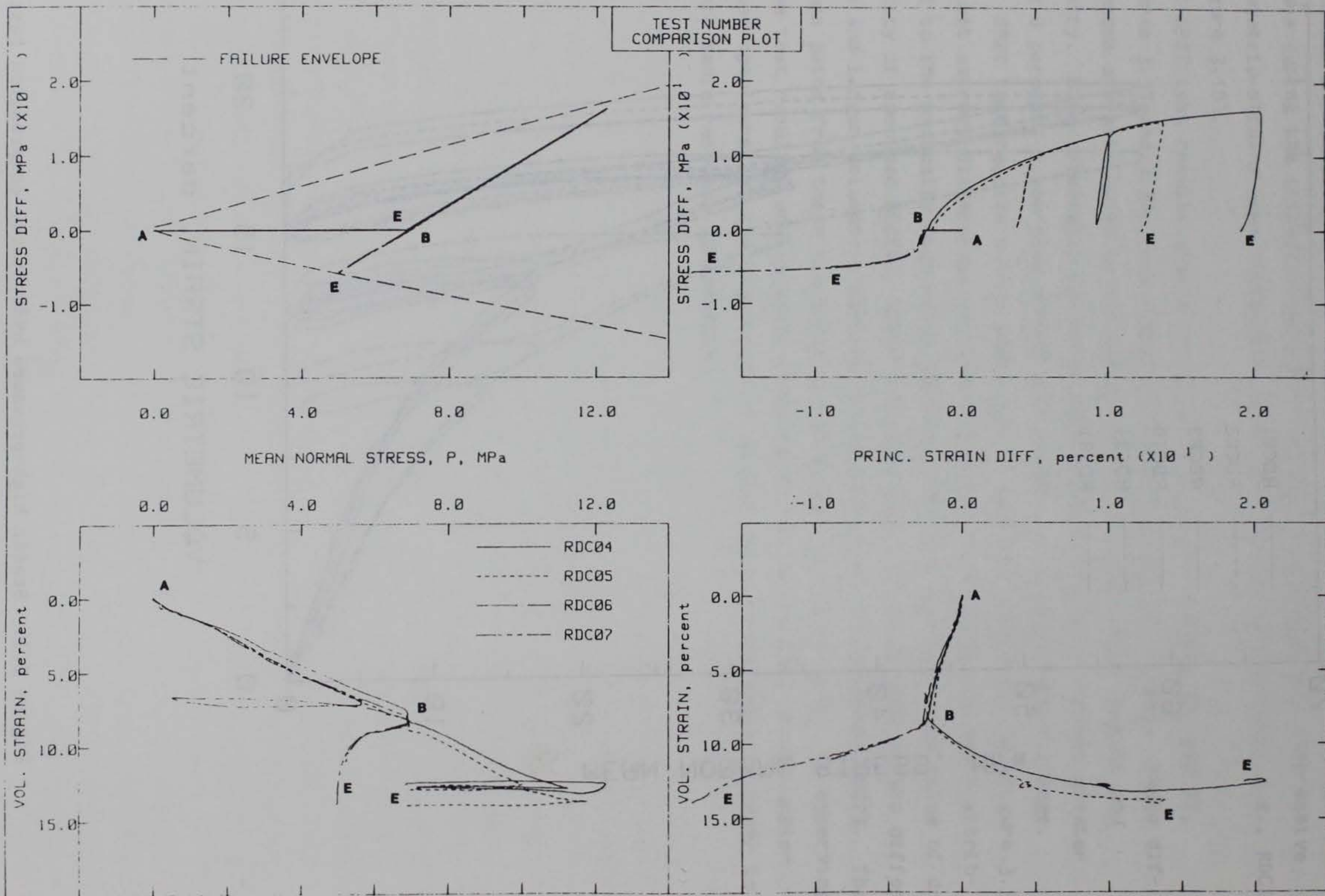
Figure 3.2. CTC and RTE test results.
