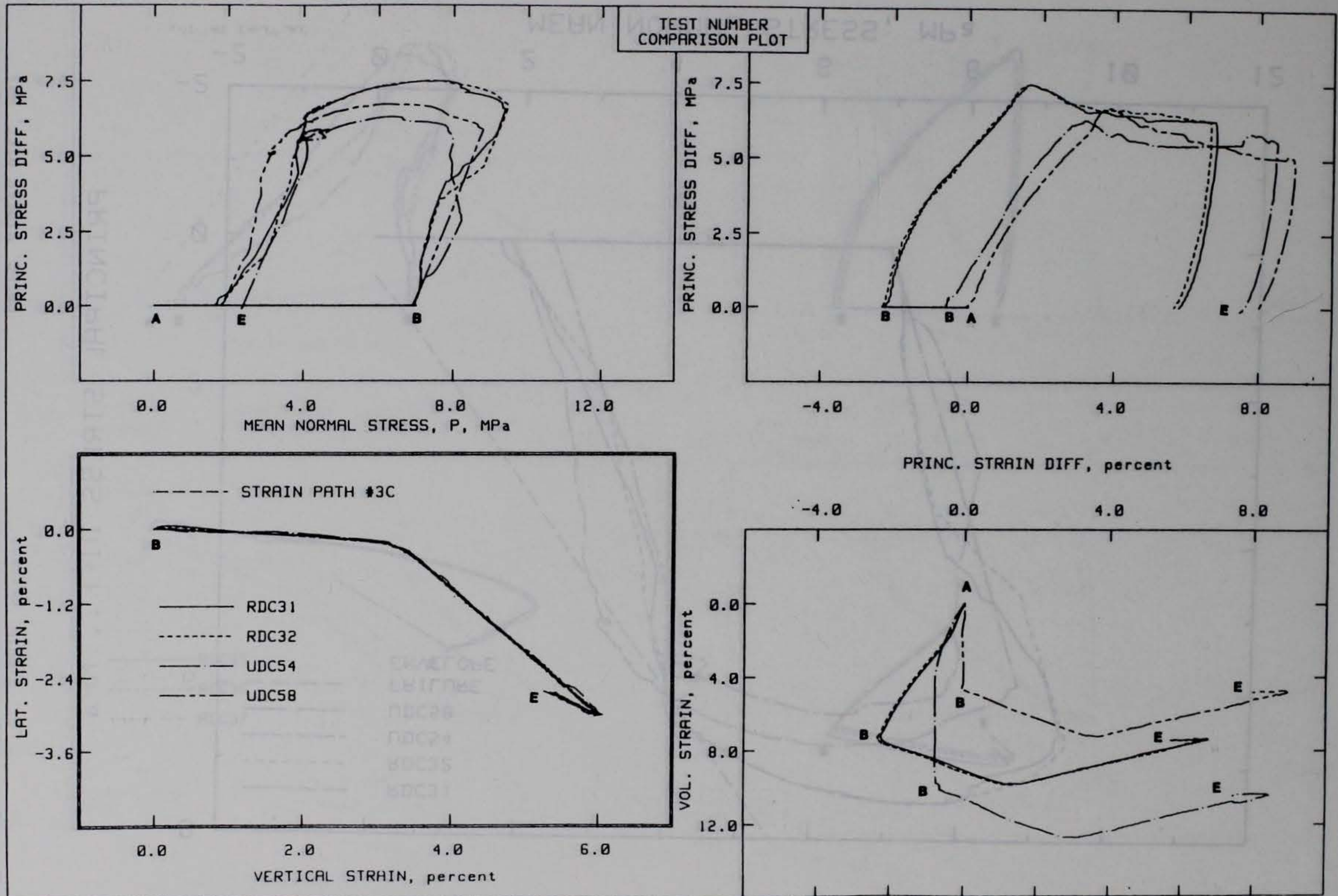
Figure 3.25. Comparison of strain path data from remolded and undisturbed specimens following SP3C.
