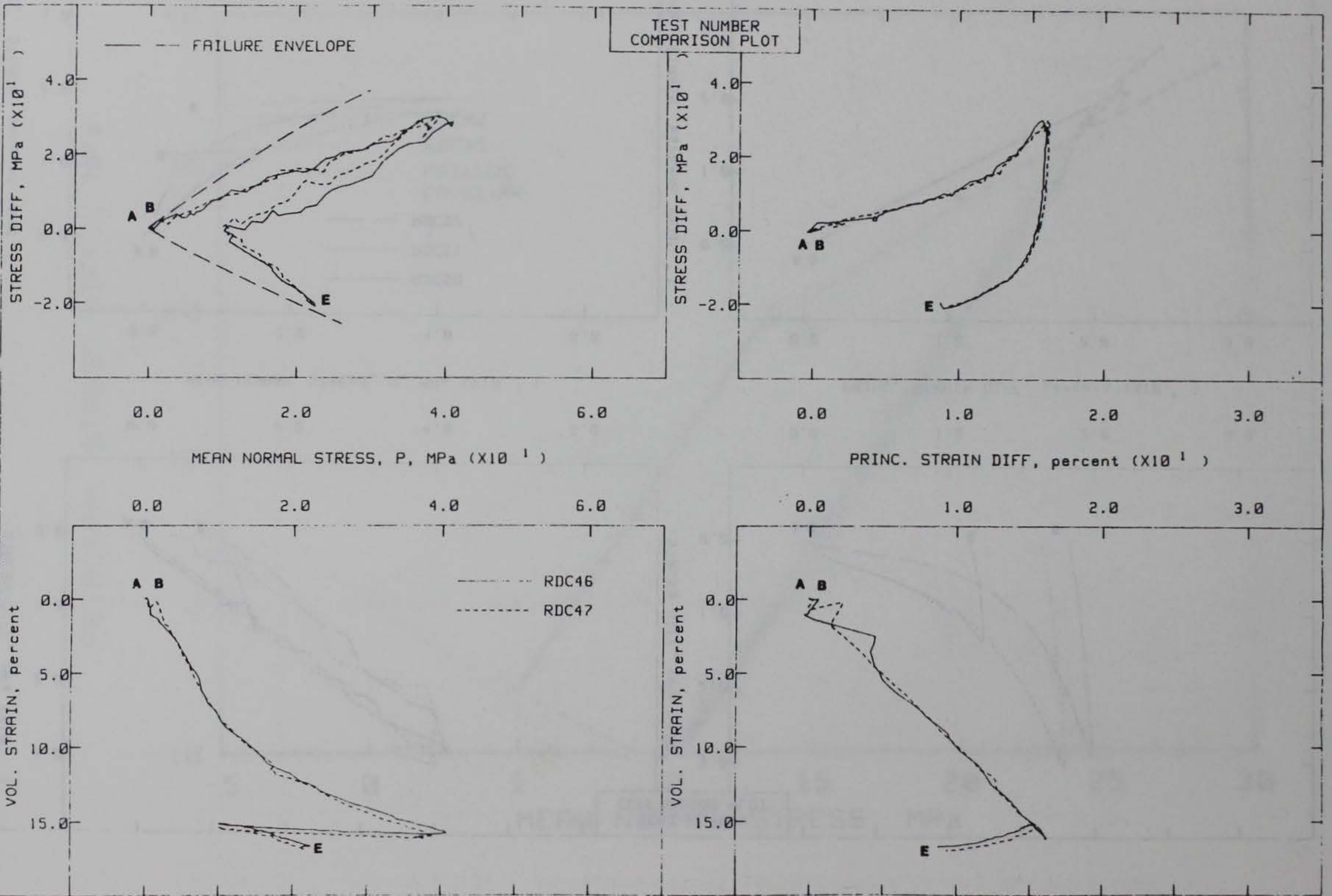
Figure 3.16. K_0/CTE test results.
