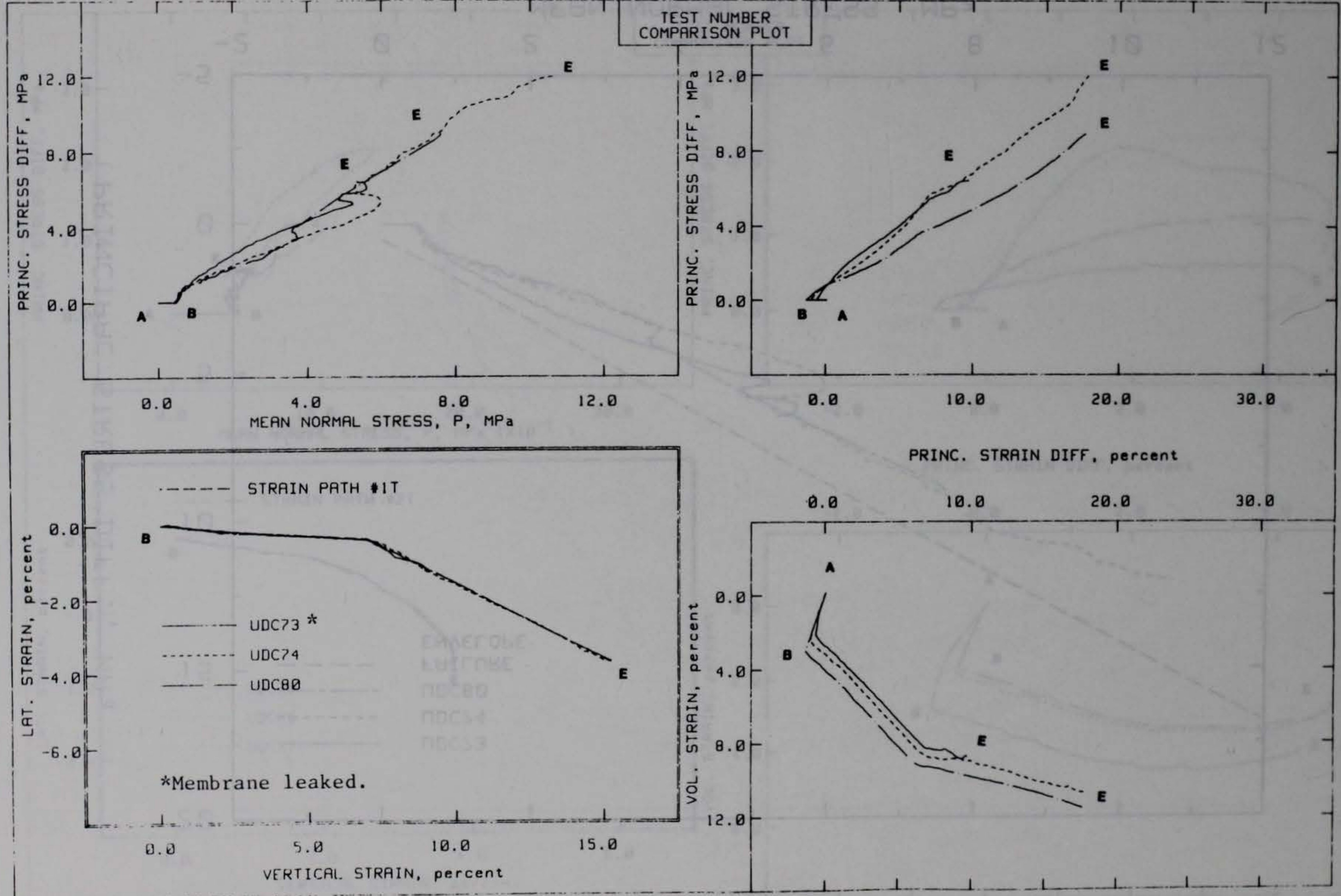
Figure 3.35. Strain path 1T test results.
