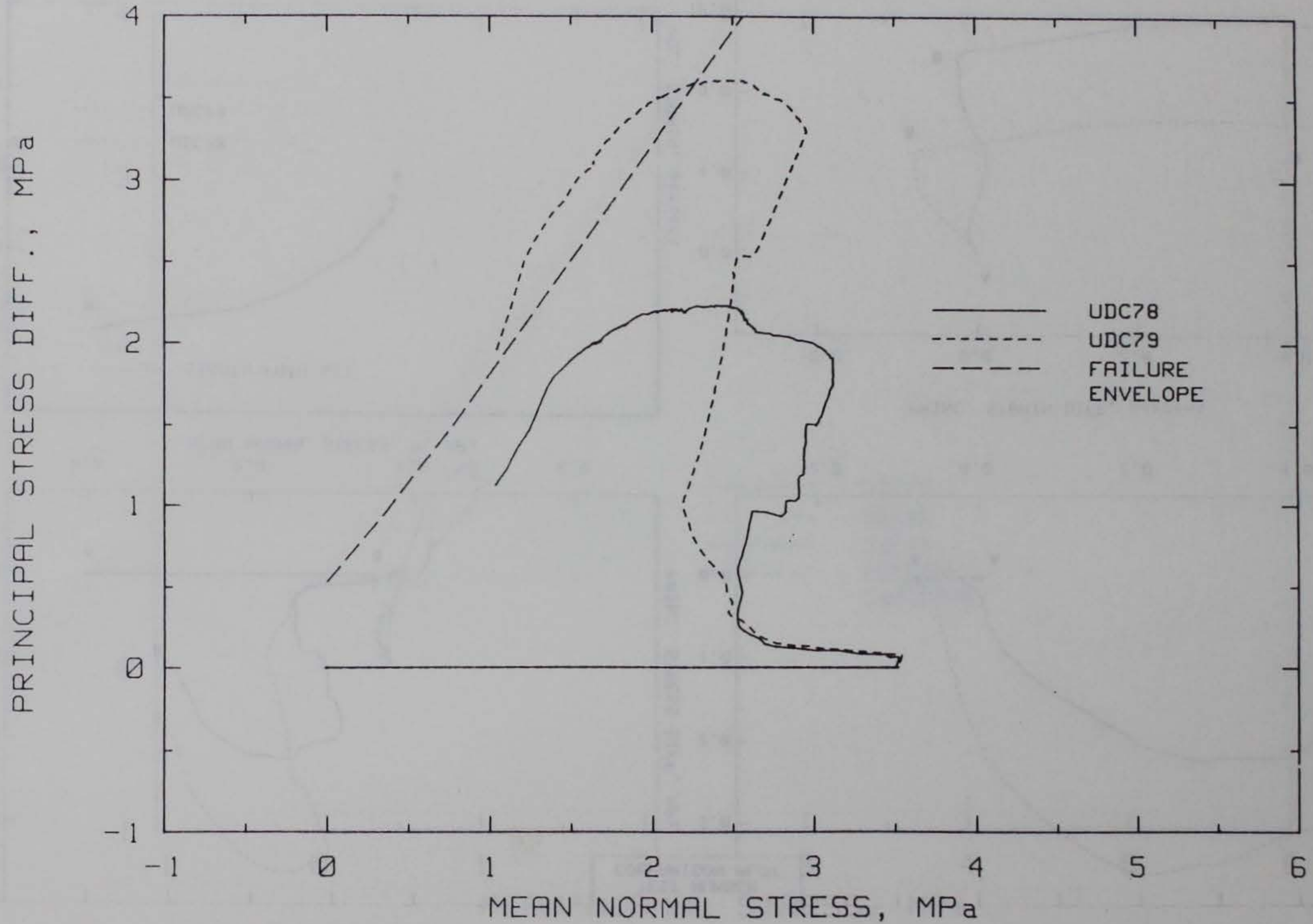
Figure 3.40. Stress paths from tests following SP2T at 3.45-MPa prestress.
