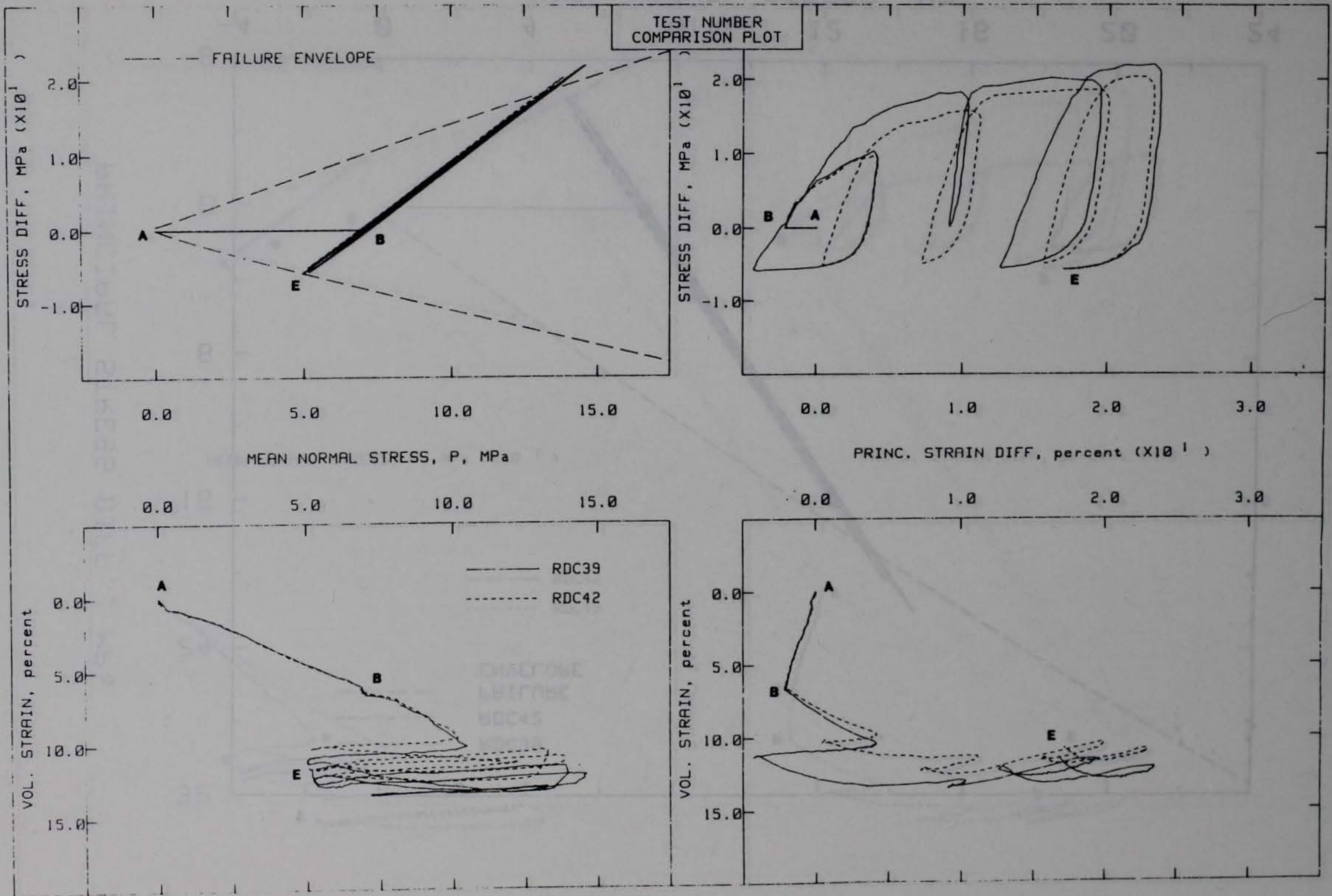
Figure 3.11. Multiple unload-reload CTC/RTE test results at 6.9 MPa prestress.
