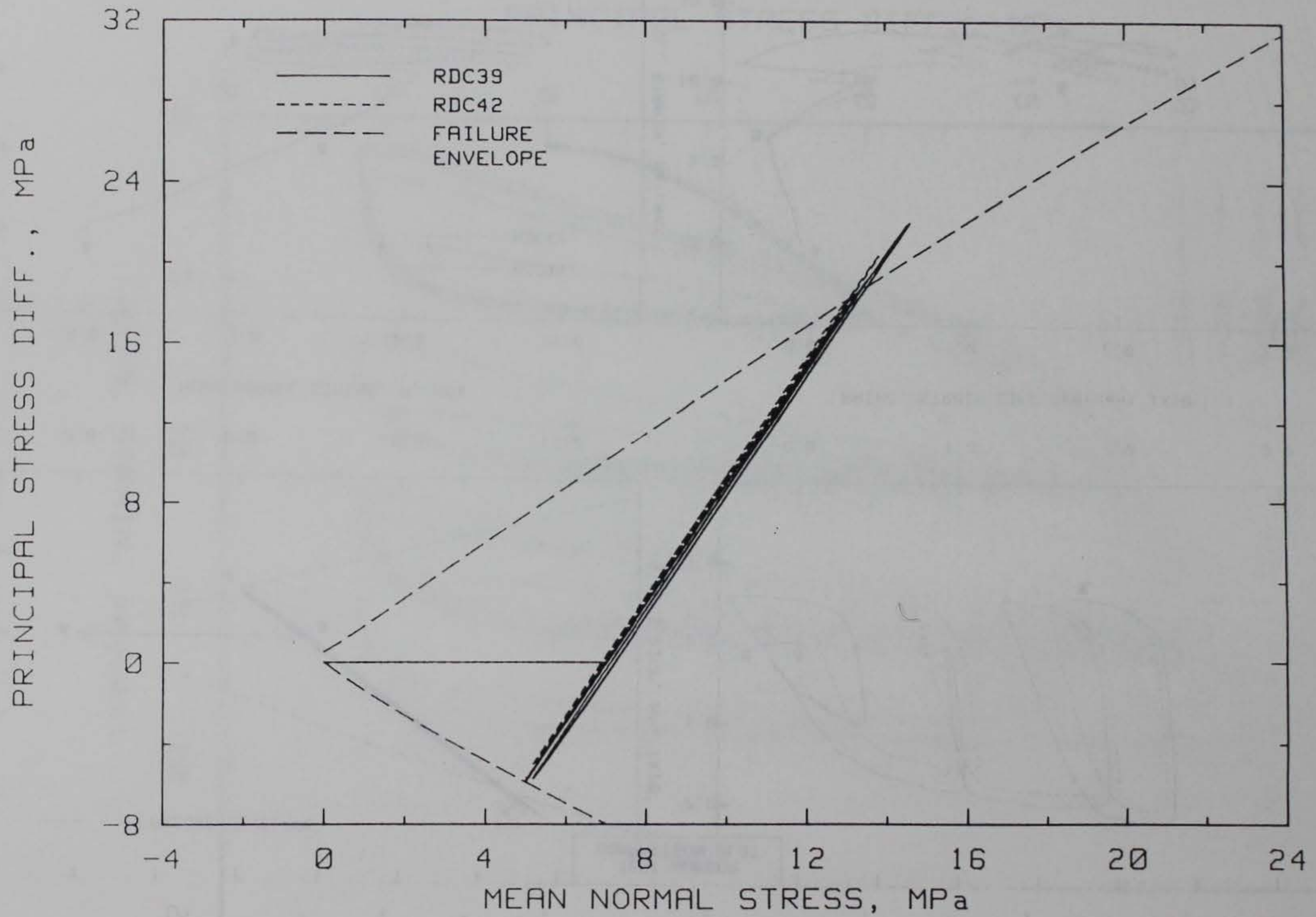
Figure 3.12. Stress paths from unload-reload CTC/RTE tests at 6.9 MPa prestress.
