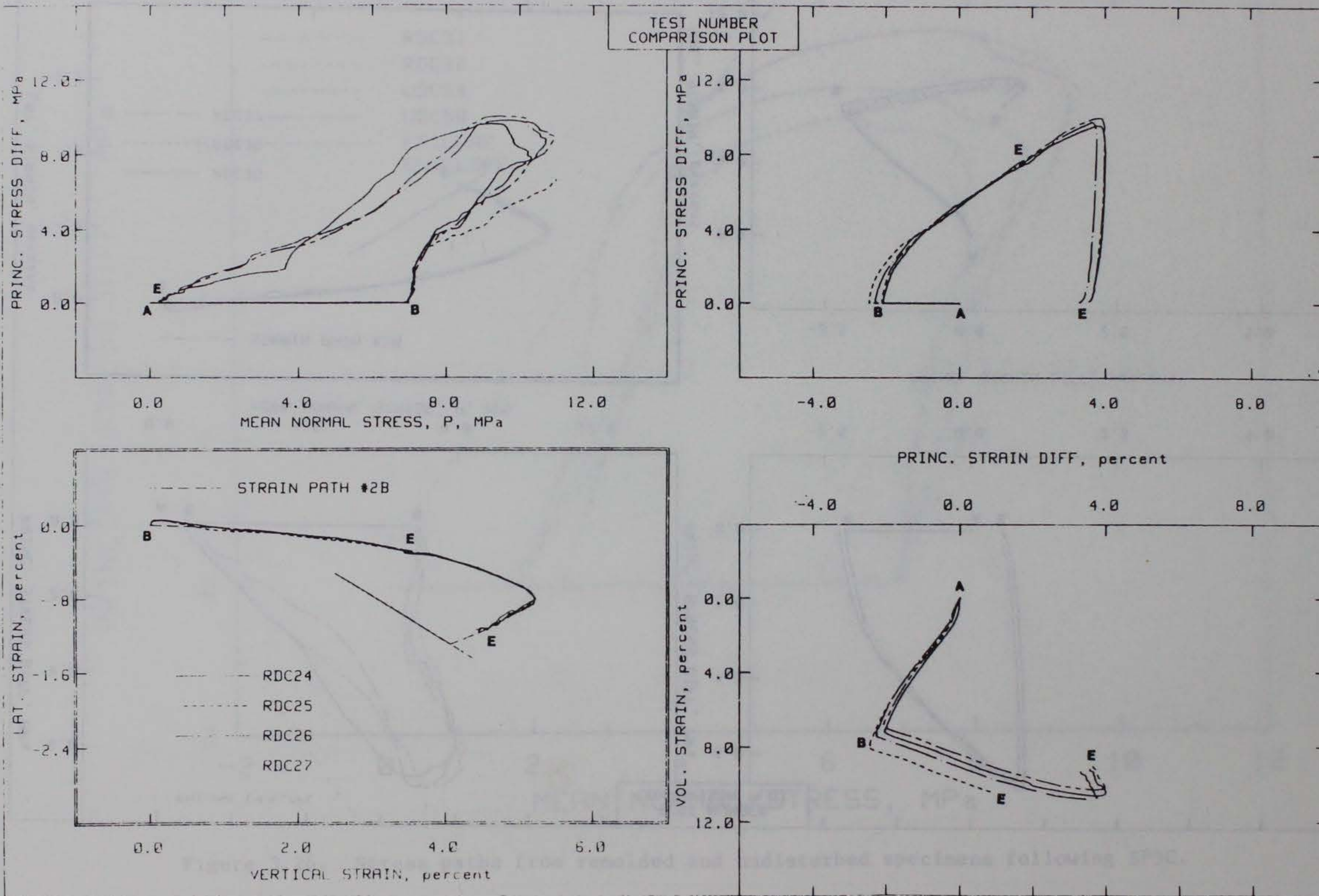
Figure 3.28. Strain path 2B test results.
