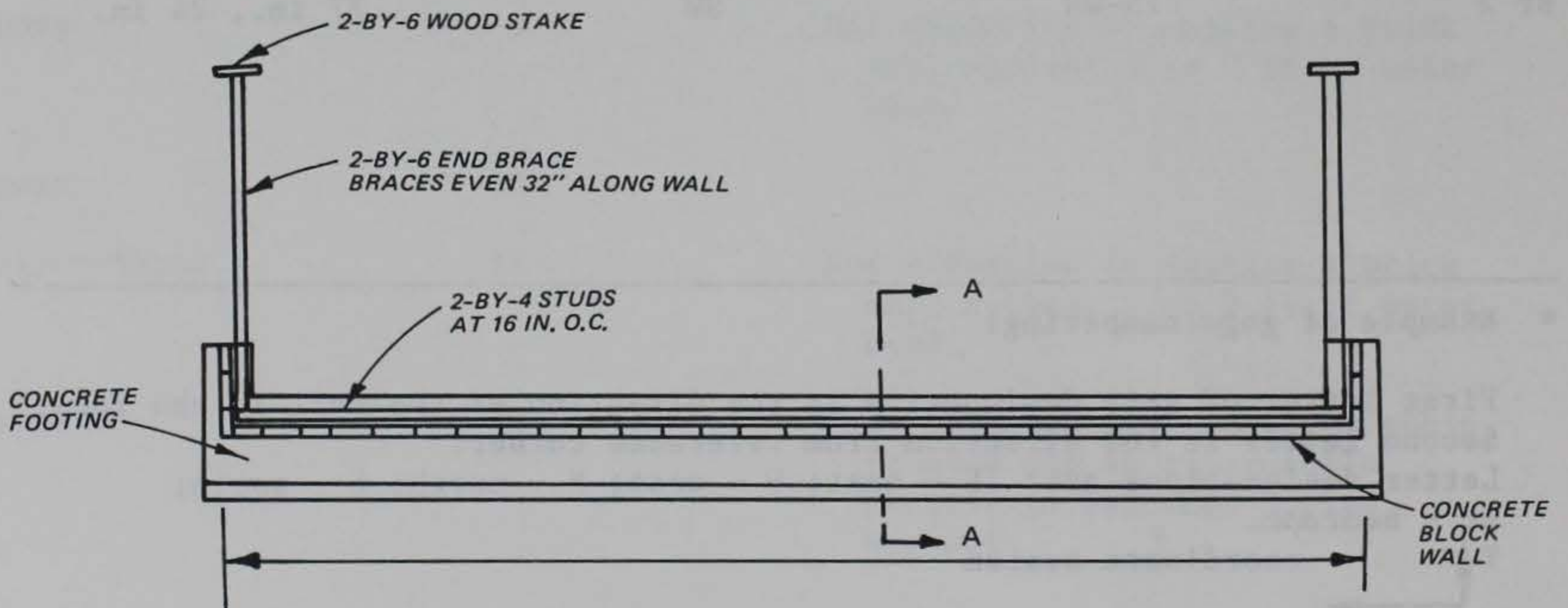
Figure 1. Concrete block wall plan and section
