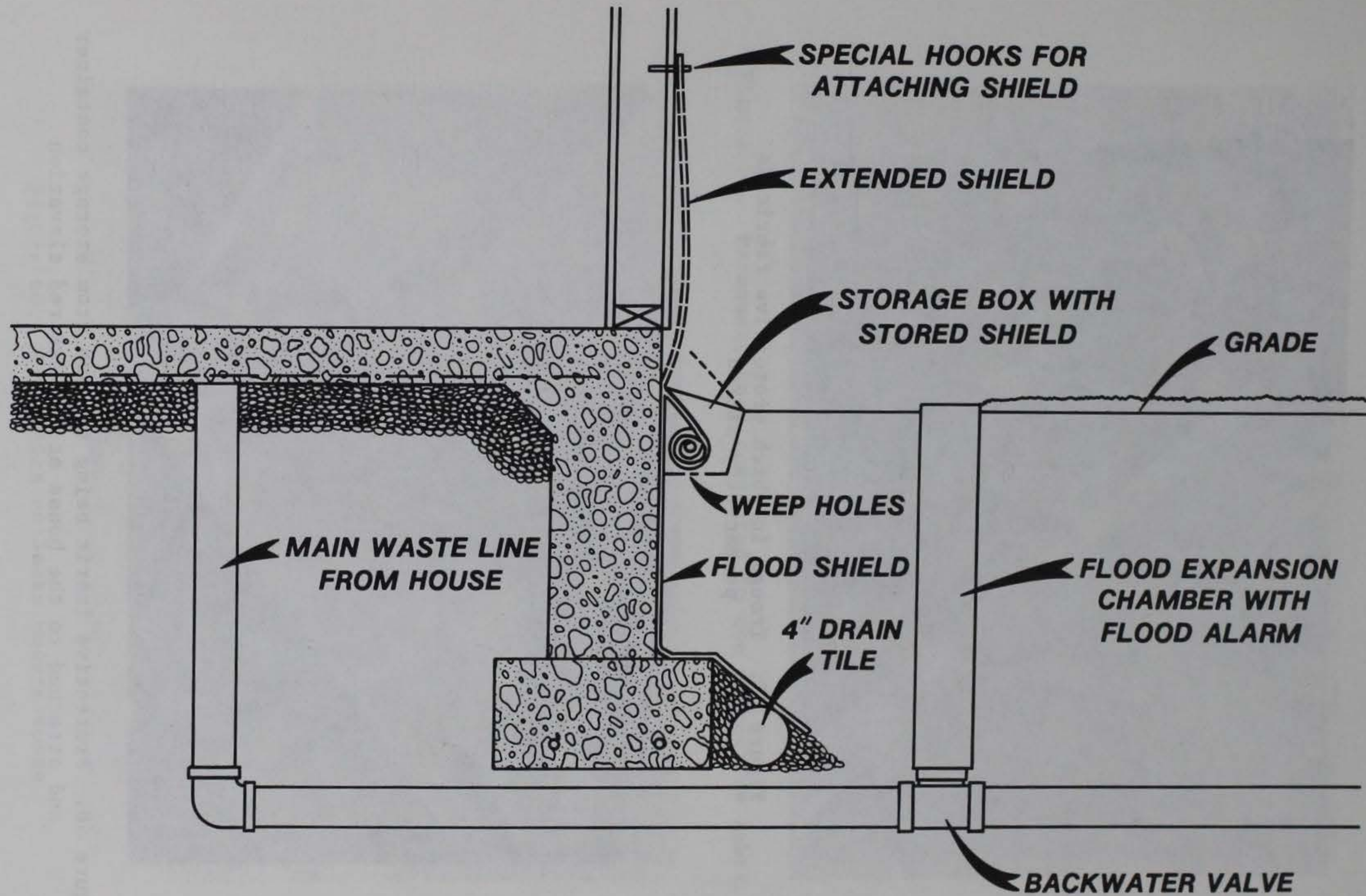
Figure 56. Schematic of embedded fabric and drainage system making up the installed flood shield
