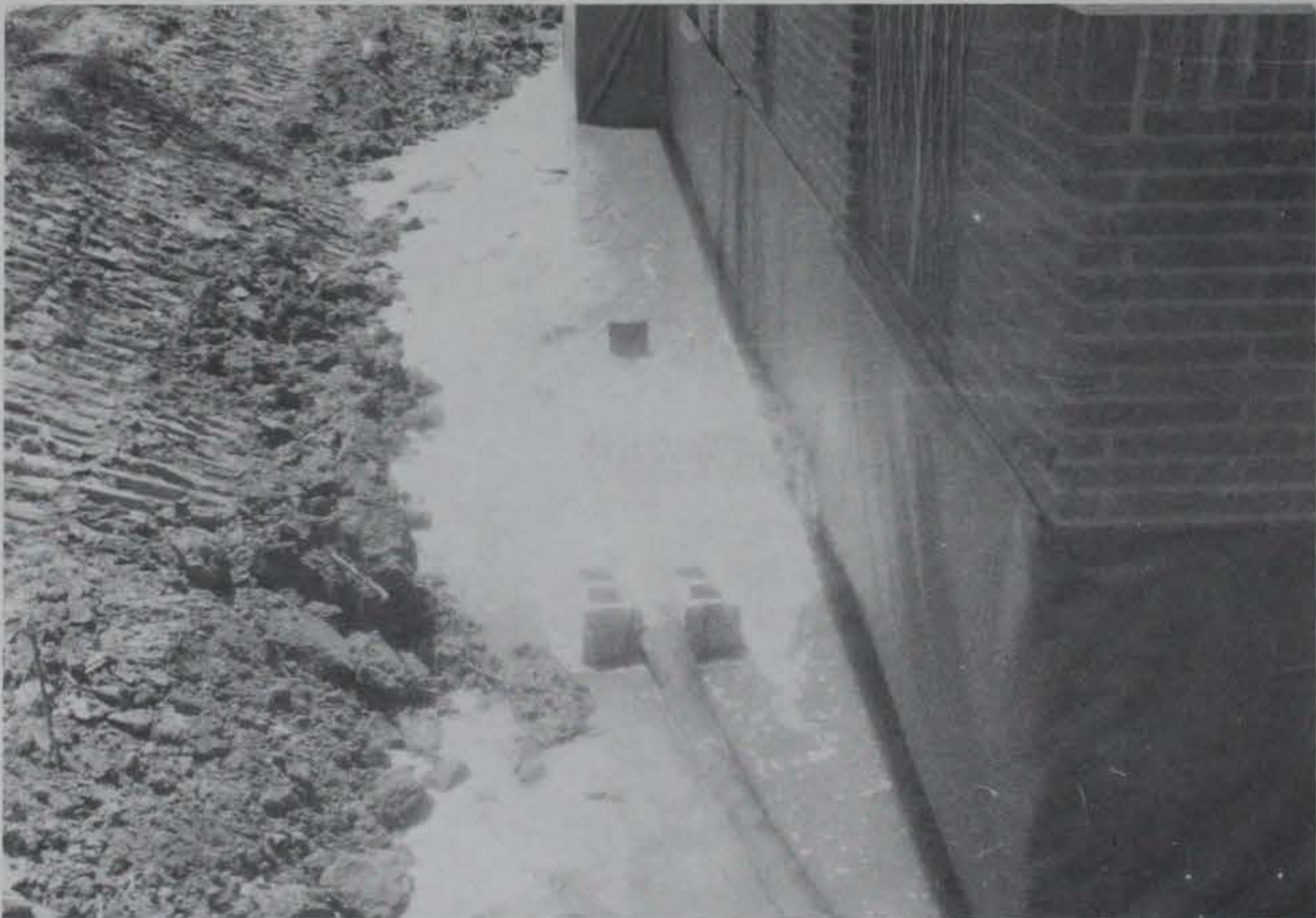
Figure 62. Beginning of water being pumped between flood shield and dike
