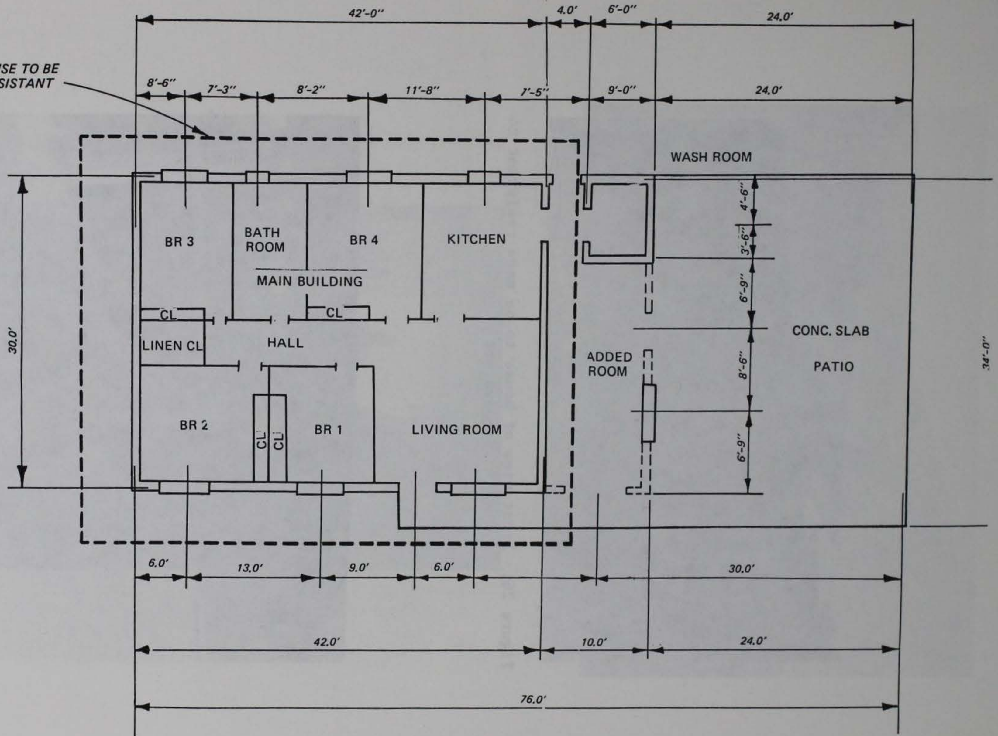
Figure 25. Floor plan of test house
