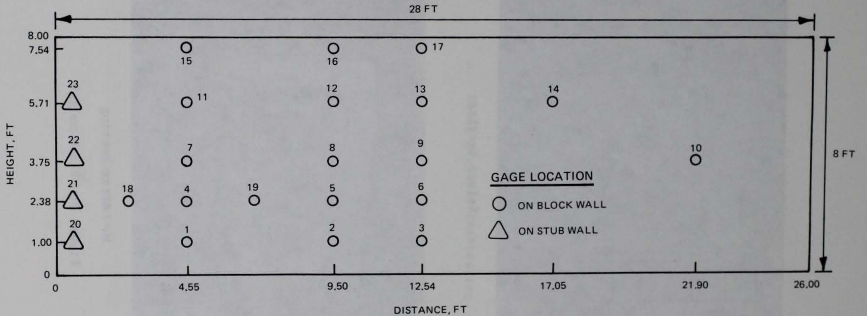
Figure 2. LVDT deflection gage locations
