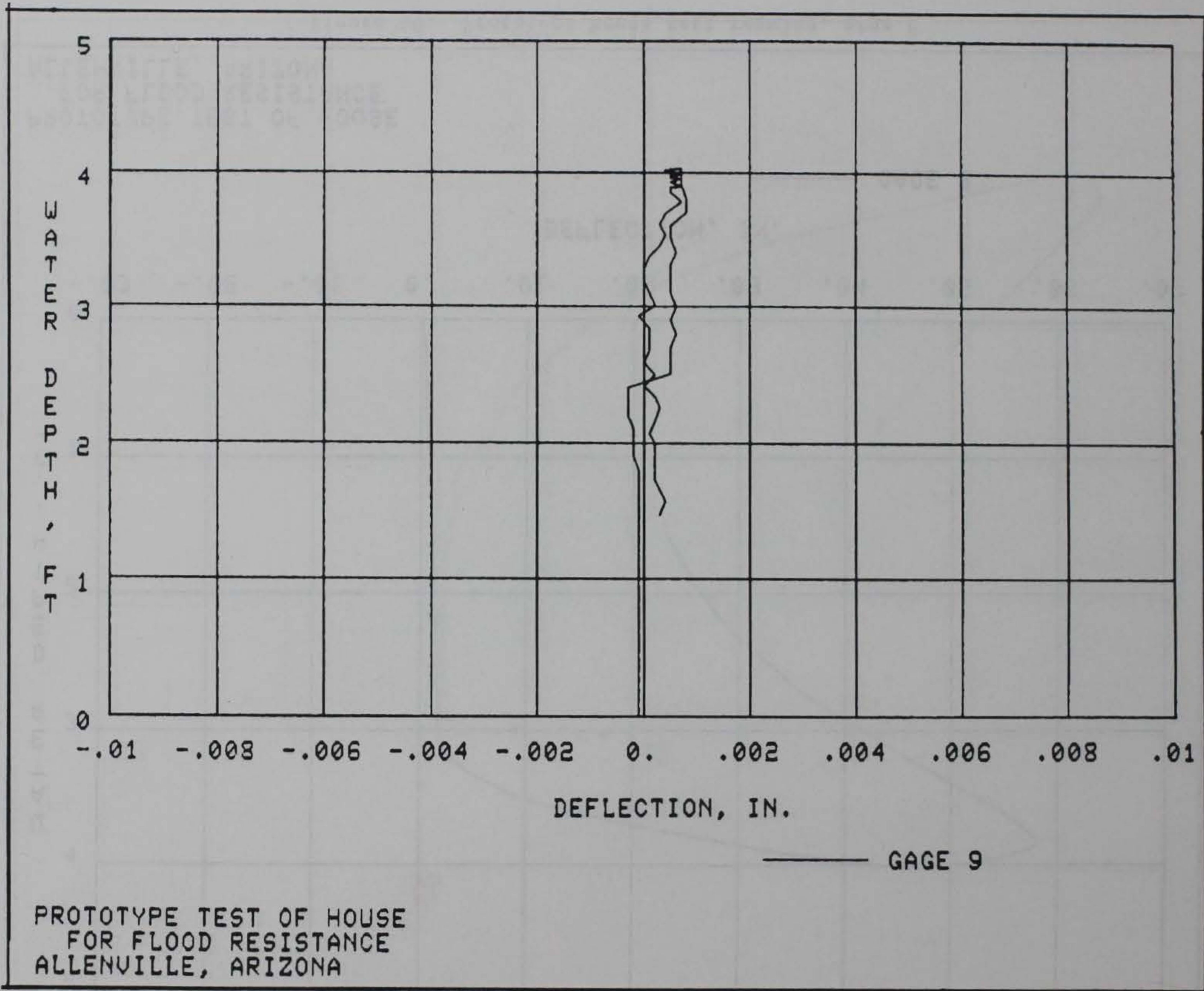
Figure 41. Prototype house test results, gage 9
