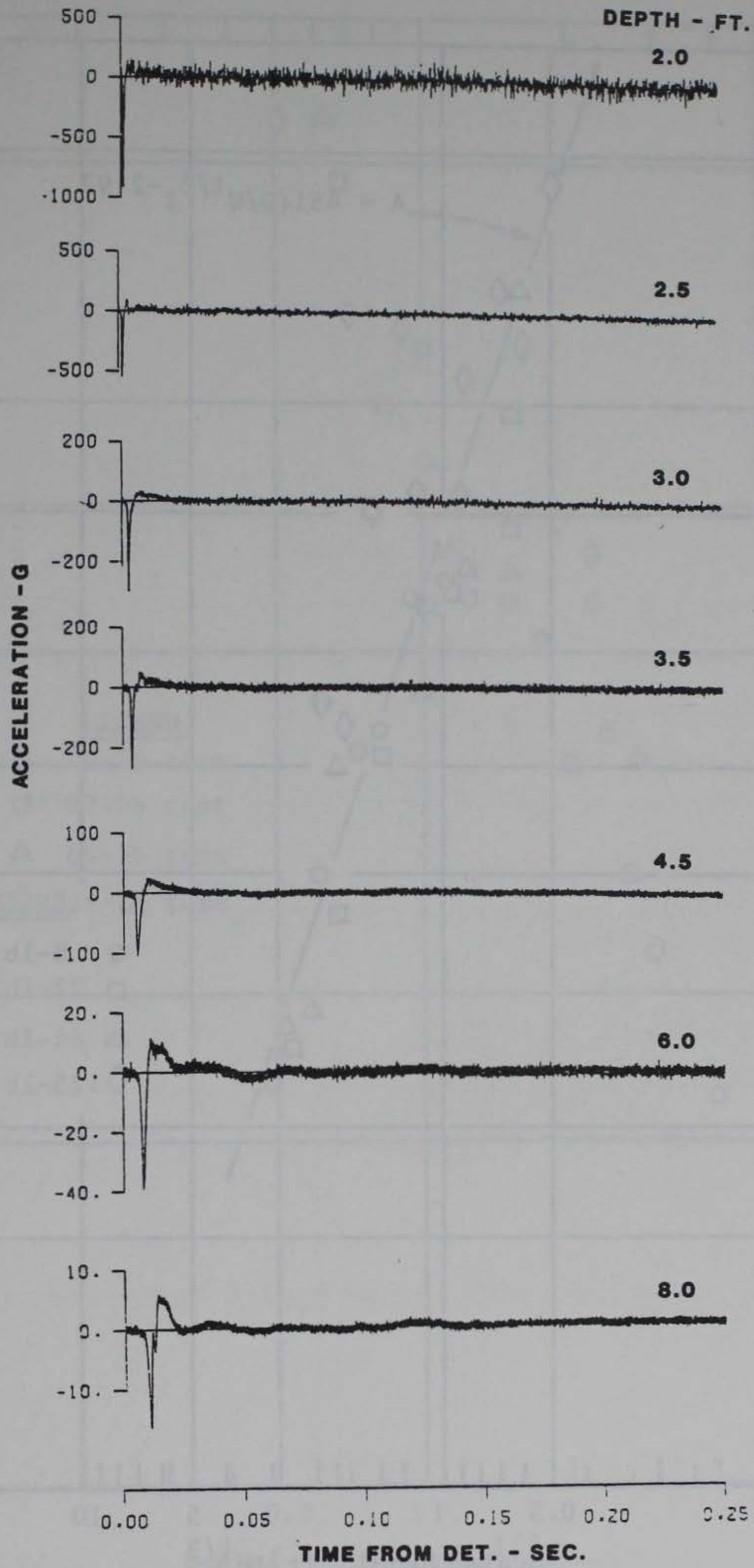
Figure 3.4. Acceleration time-histories, 27-pound rubble shield test.
