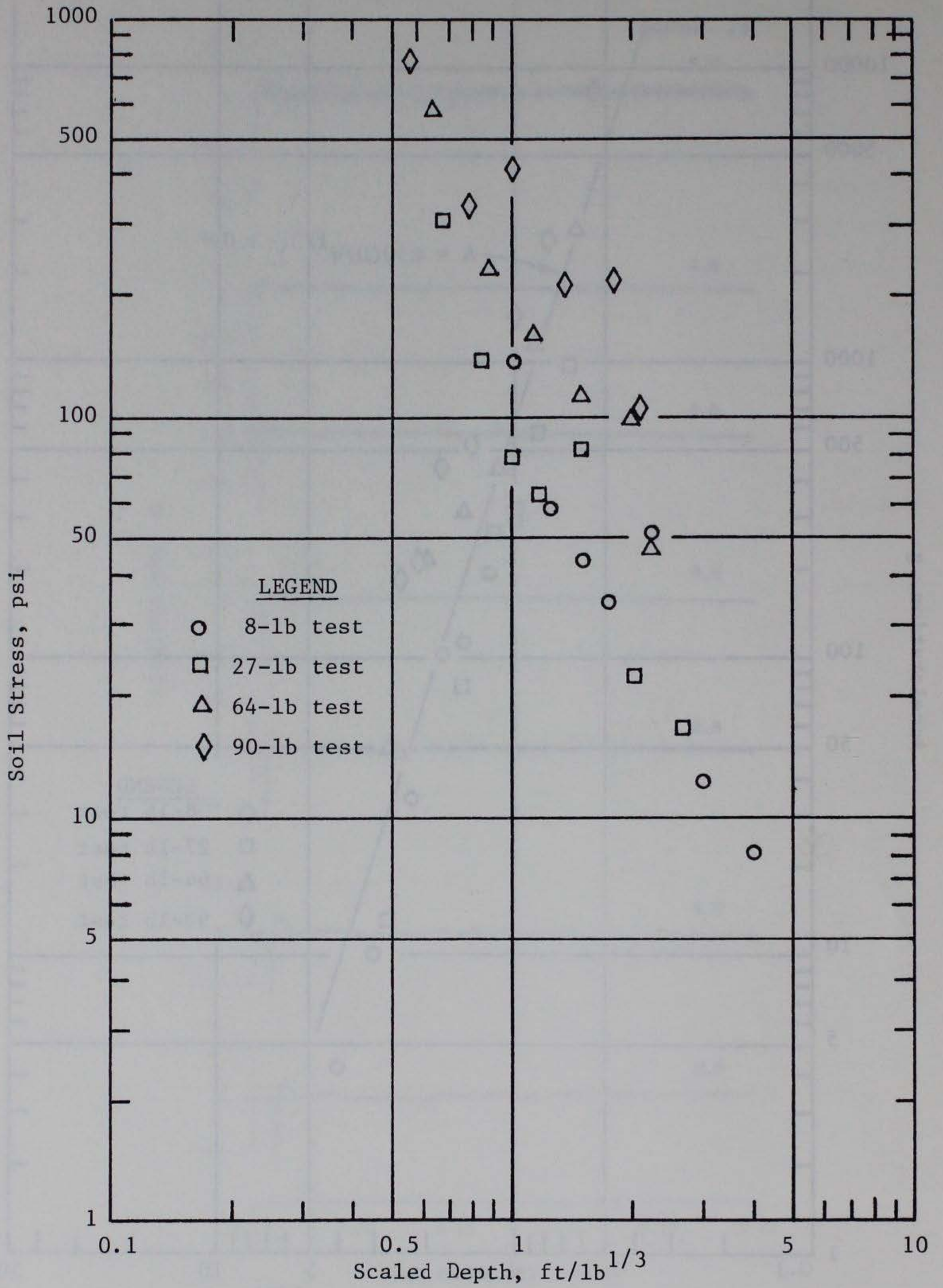
Figure 3.3. Peak stress versus scaled depth, control tests.
