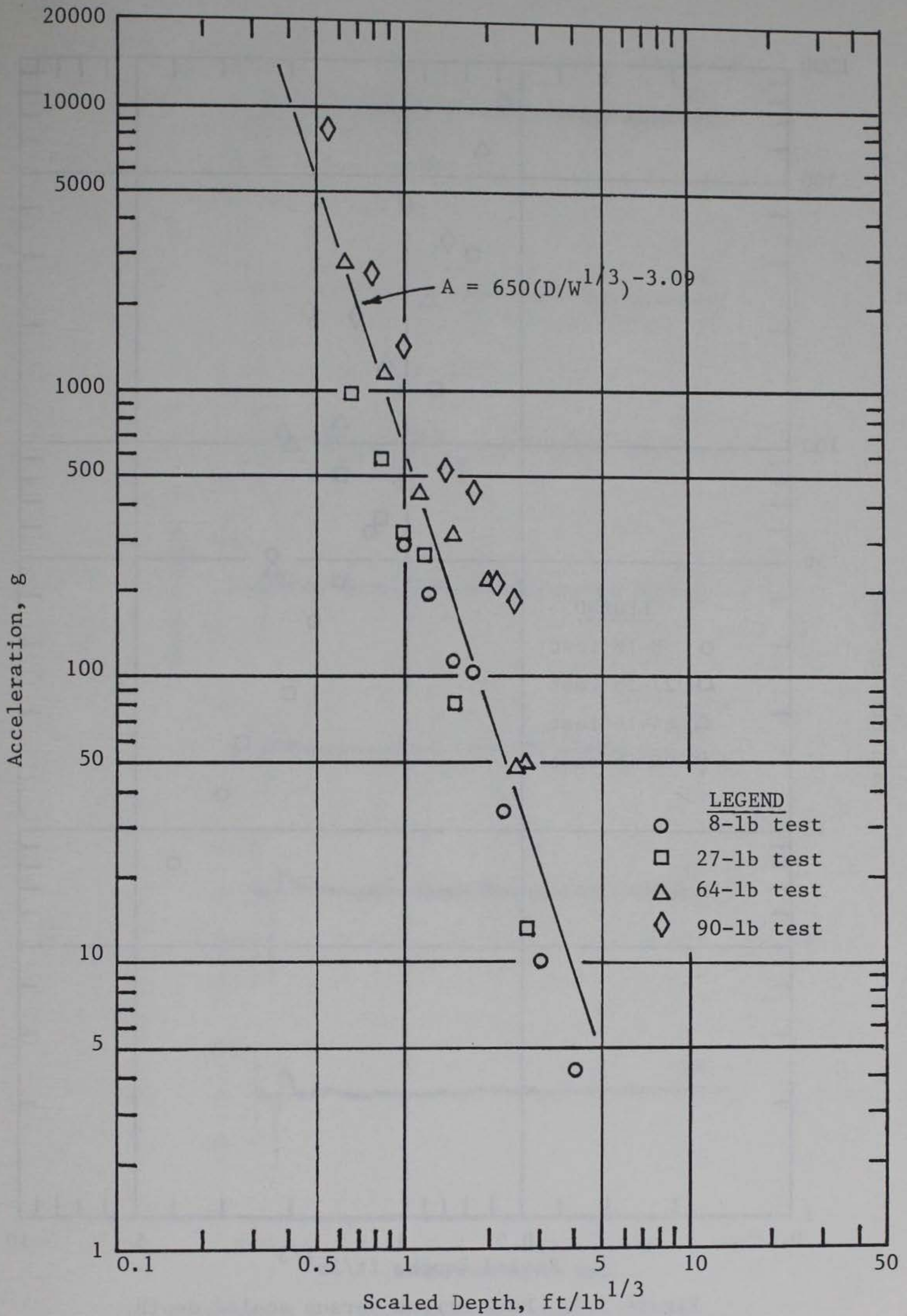
Figure 3.2. Peak acceleration versus scaled depth, control tests.
