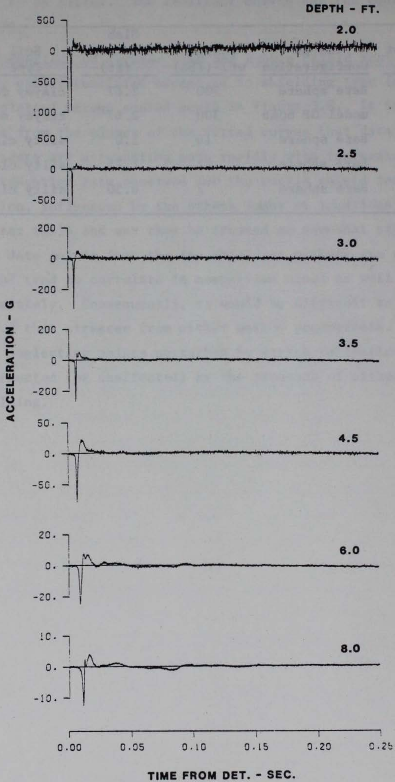
Figure 3.1. Acceleration time-histories, 27-pound control test.
