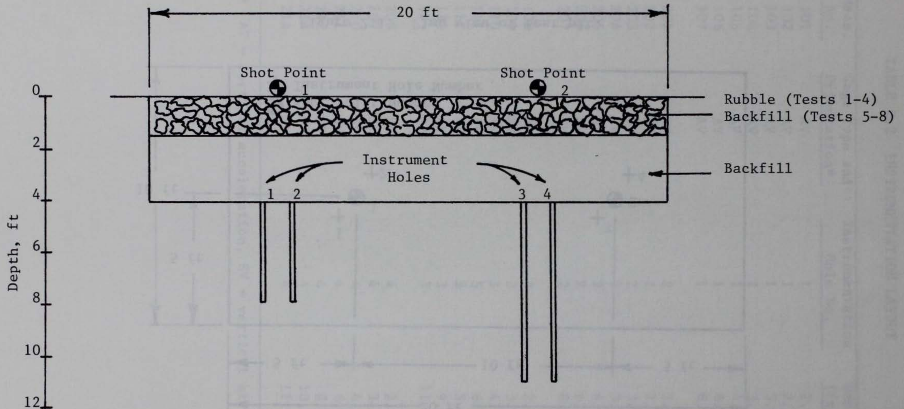
Figure 2.2. Cross section of test pit.
