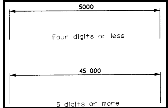
Figure 16. Proper dimension presentations for metric measurements with four or more digits
