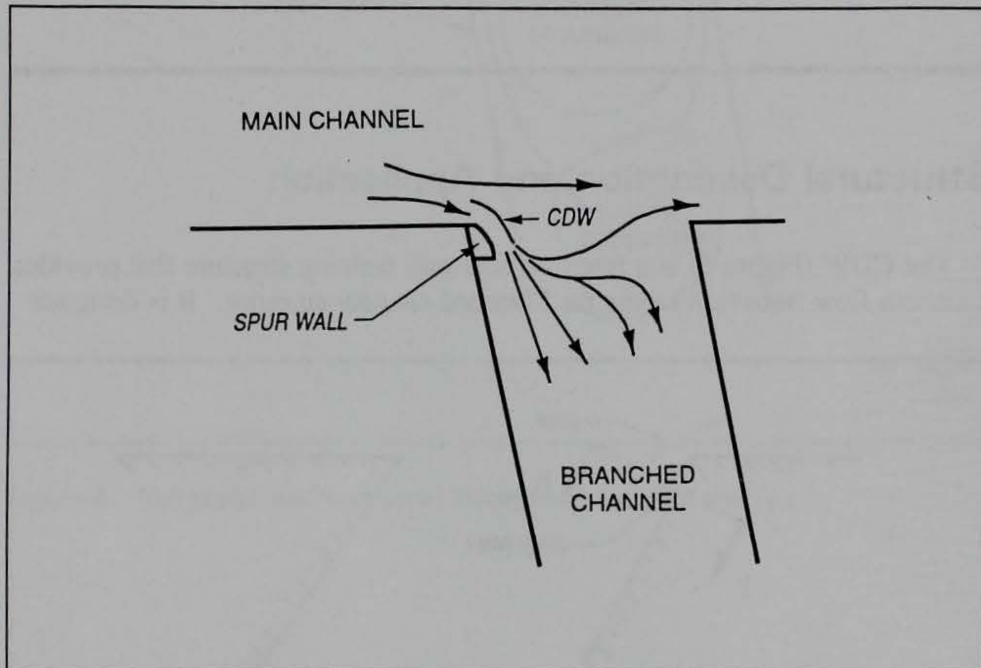
Figure 6. CDW principle of operation
