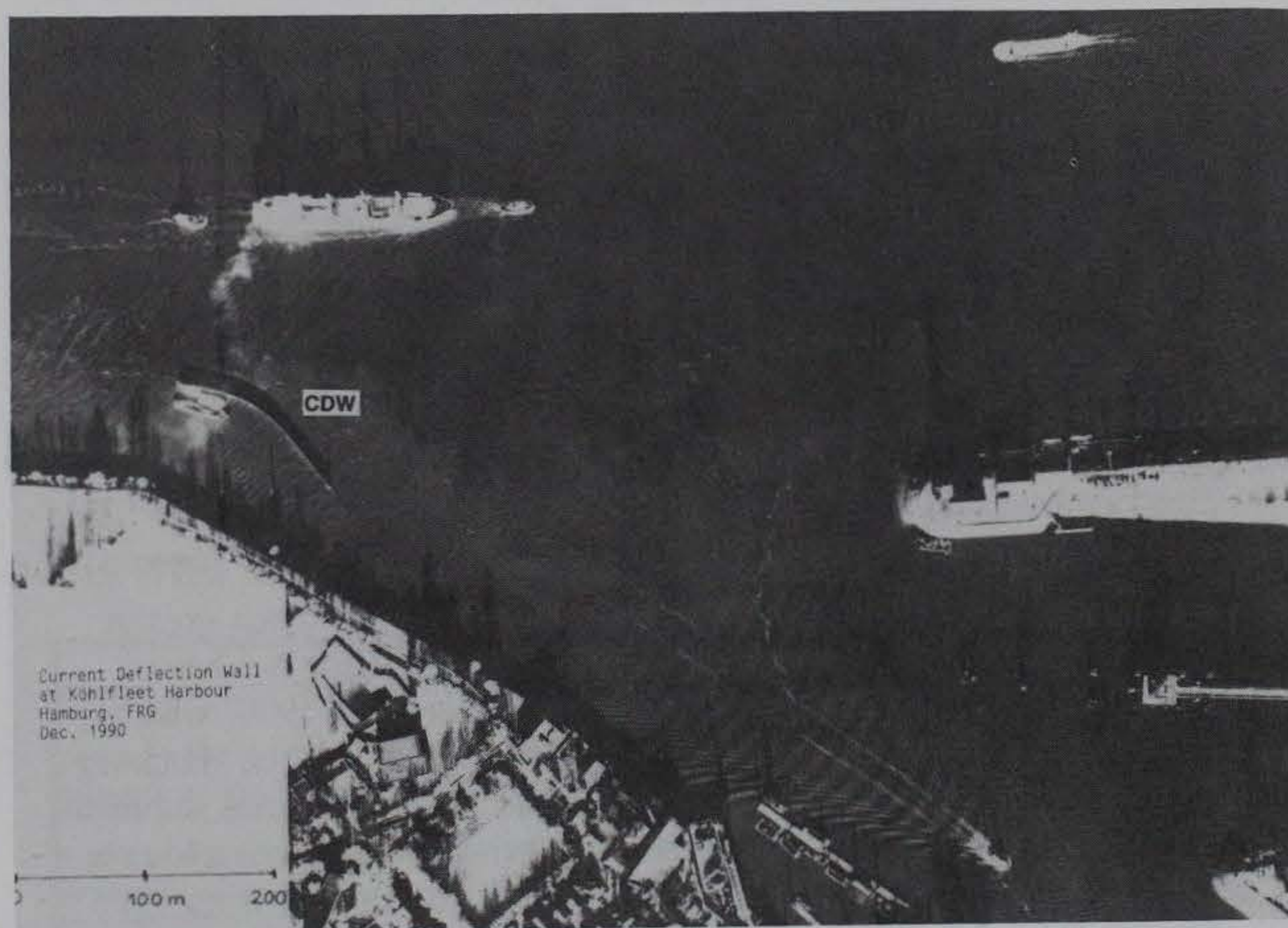
Figure 8. Aerial view of CDW prototype in Kohl fleet Harbor, Port of Hamburg, Germany (courtesy of Dr. Robert Kirby, Ravensrodd Consultants, Ltd.)
