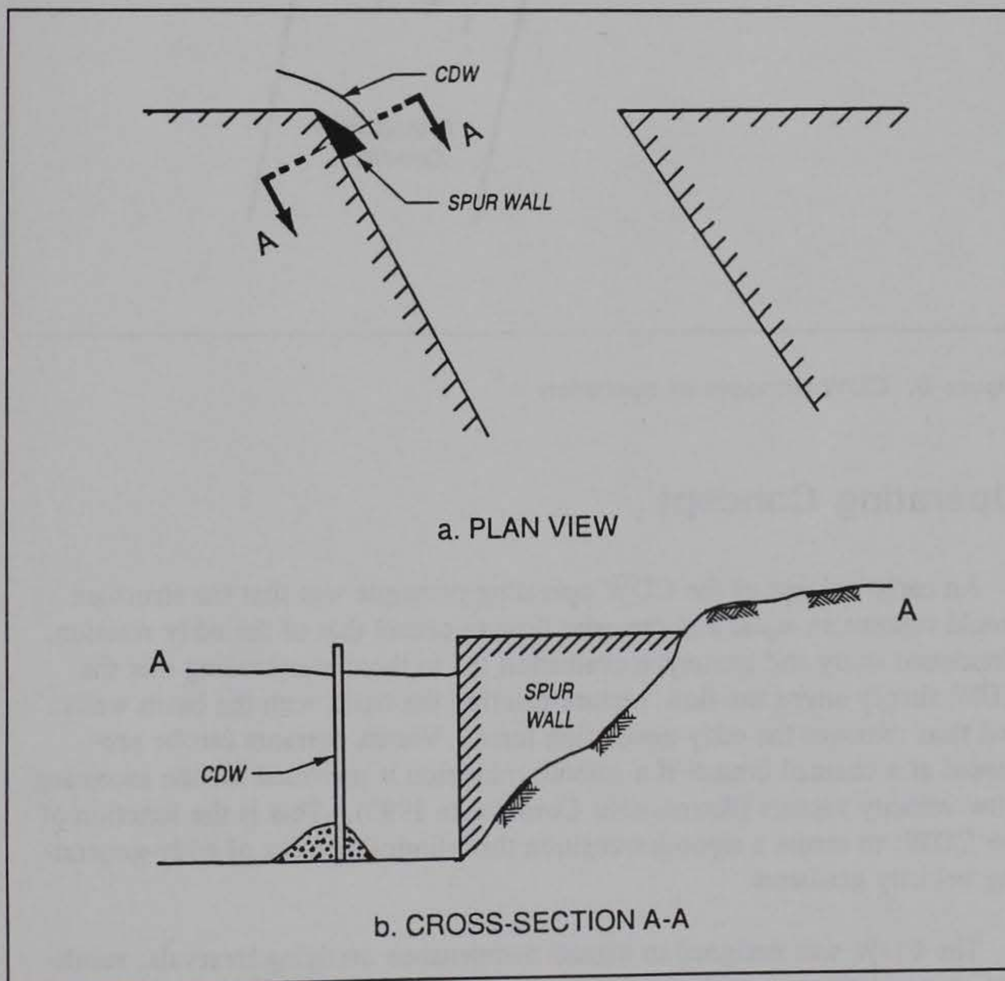
Figure 5. Plan and cross-sectional CDW schematics
