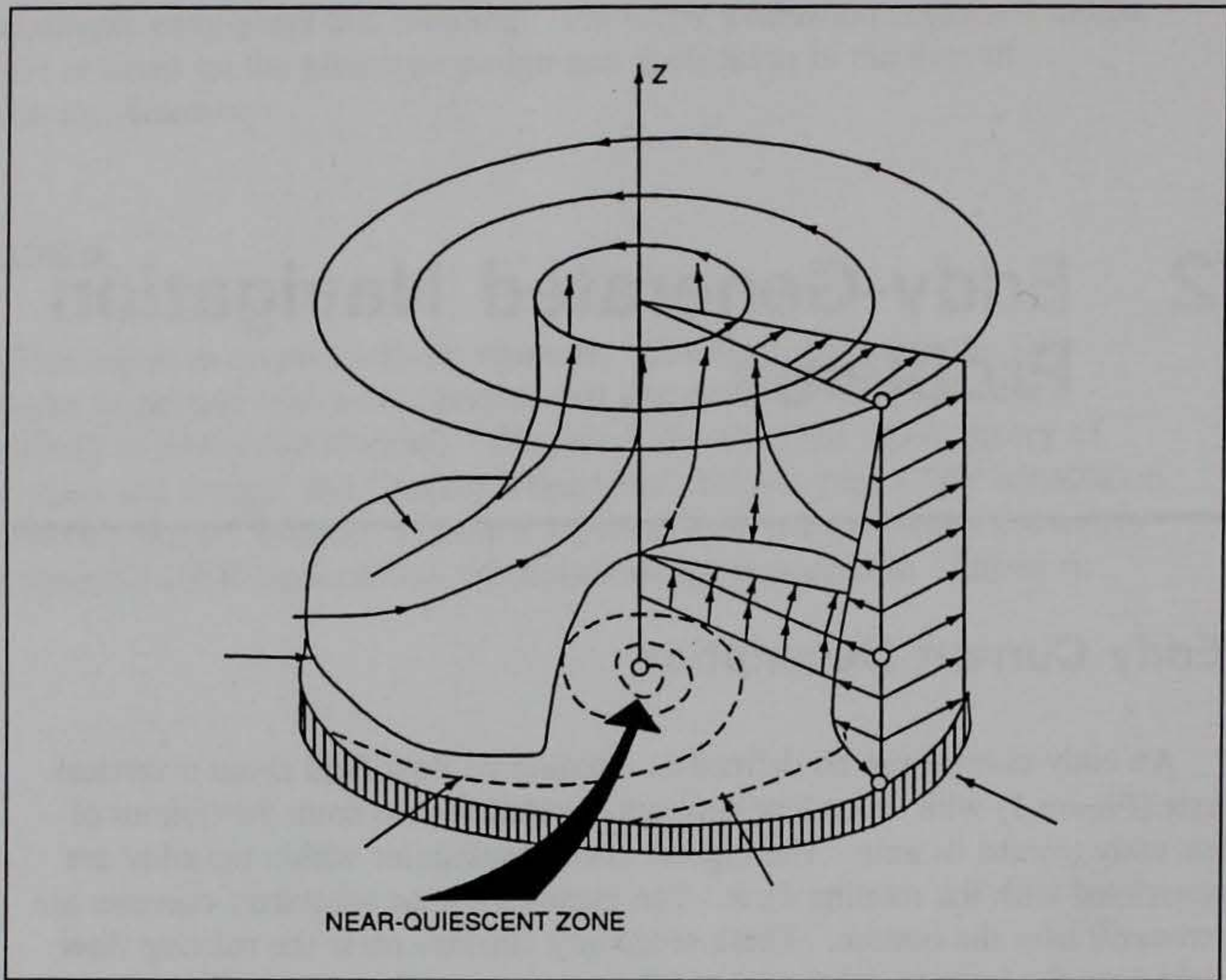
Figure 1. Eddy current patterns and relative velocity distributions
