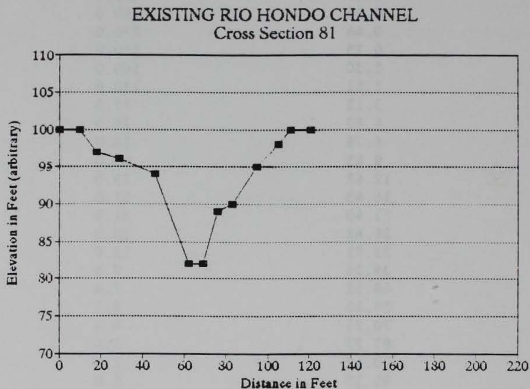
Figure 14. Existing Rio Hondo channel at cross section 81
