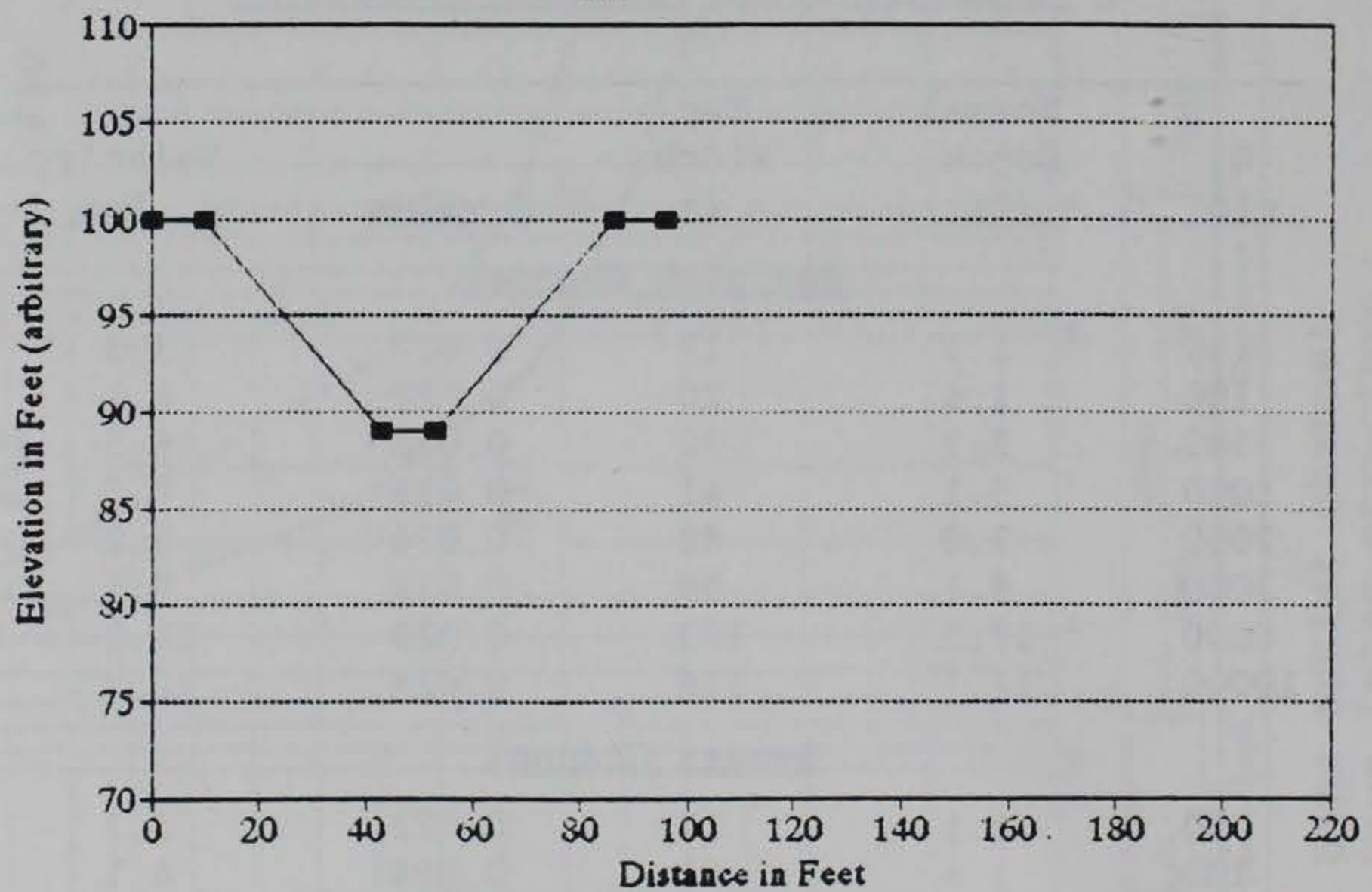
Figure A1. Existing-slope project approach and bypass channel cross sections
