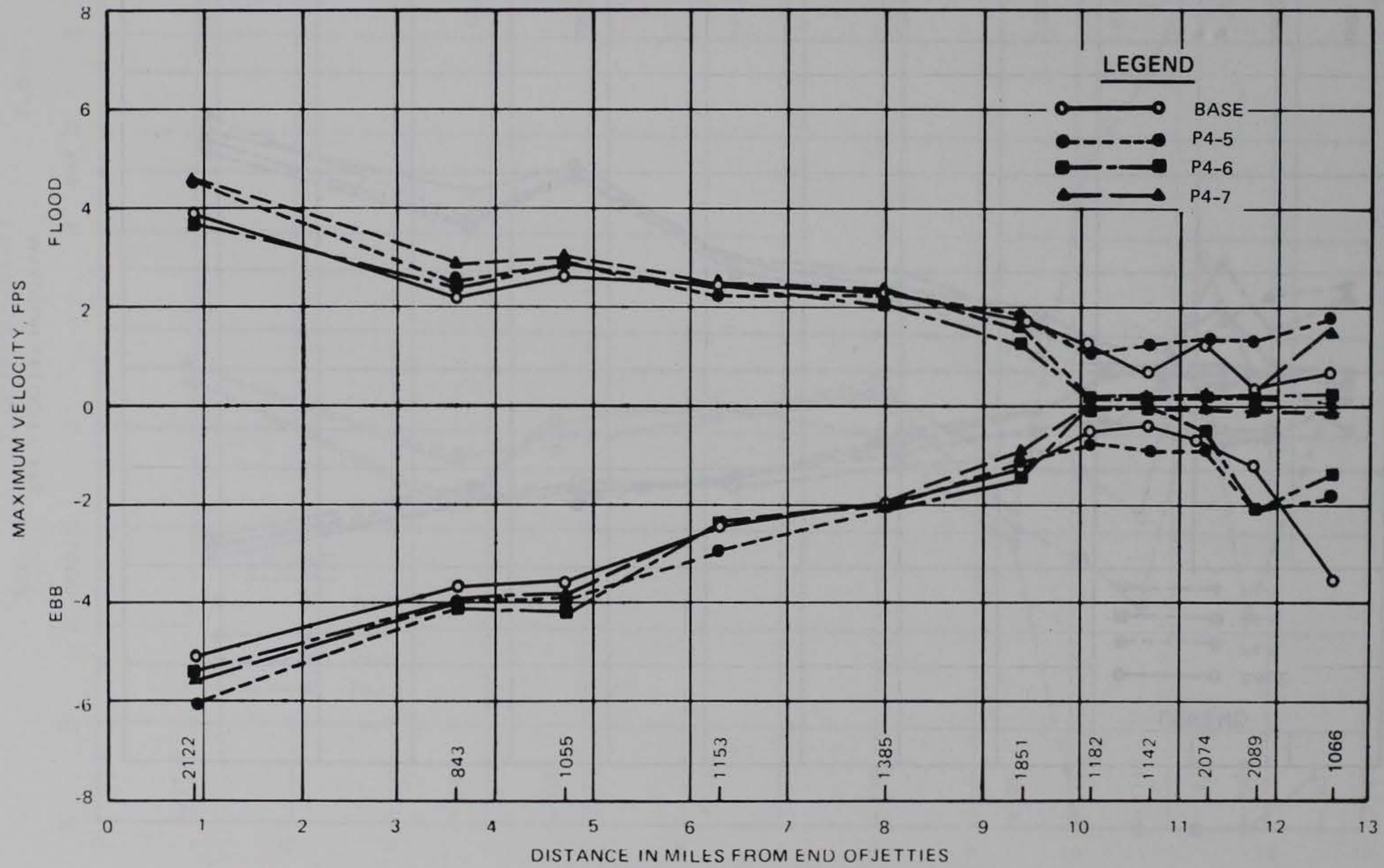
Figure 15. Effects of plans P4-8, P4-9, and P4-10 on flow predominance - surface
