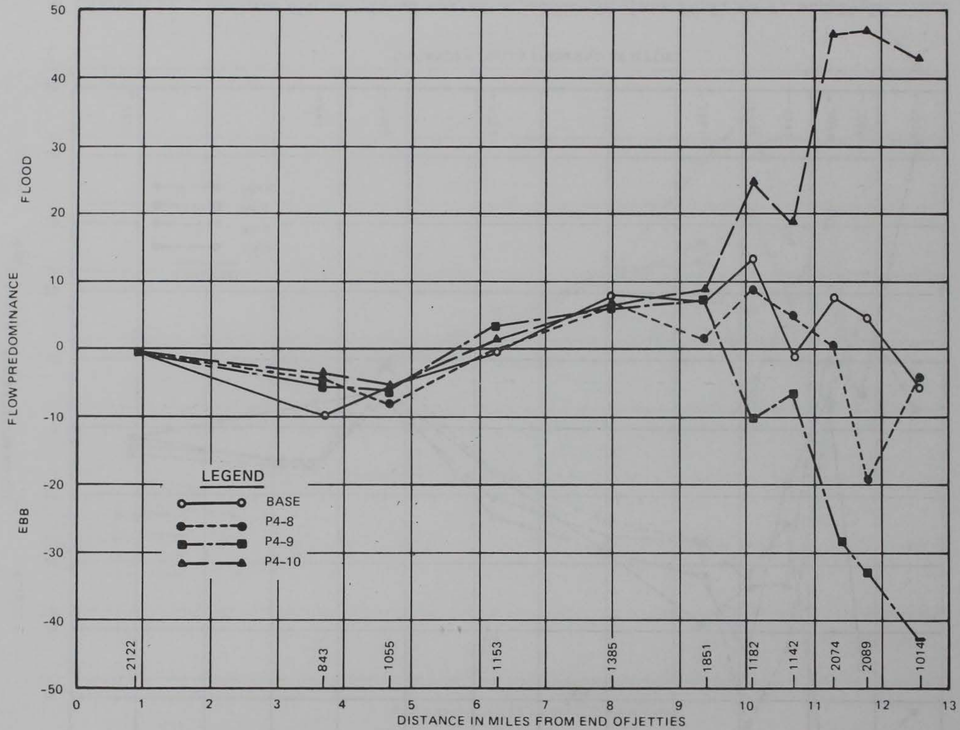
Figure 20. Maximum ebb and flood currents, bottom plans P4-8, P4-9, and P4-10
