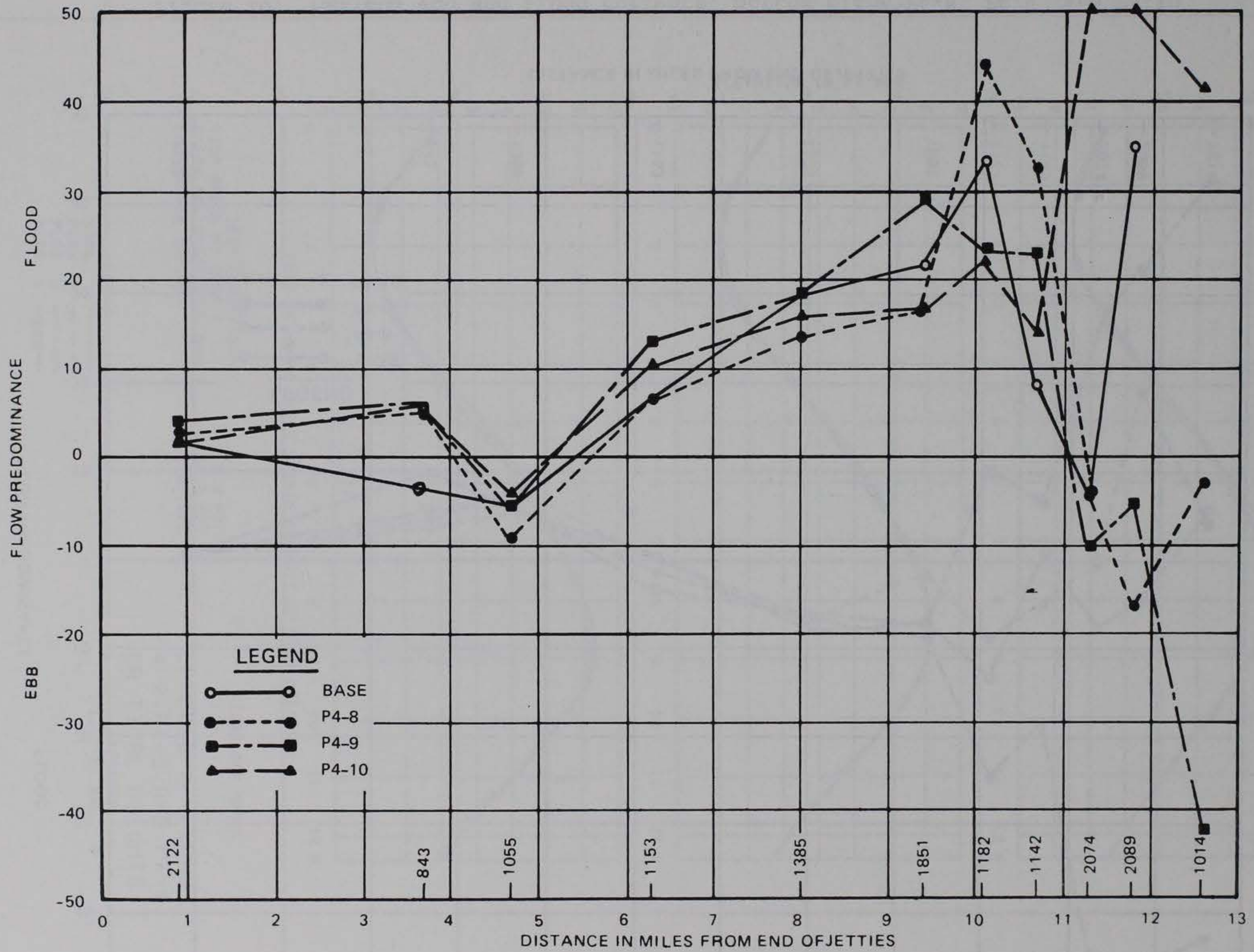
Figure 19. Maximum ebb and flood currents, middepth plans P4-8, P4-9, and P4-10
