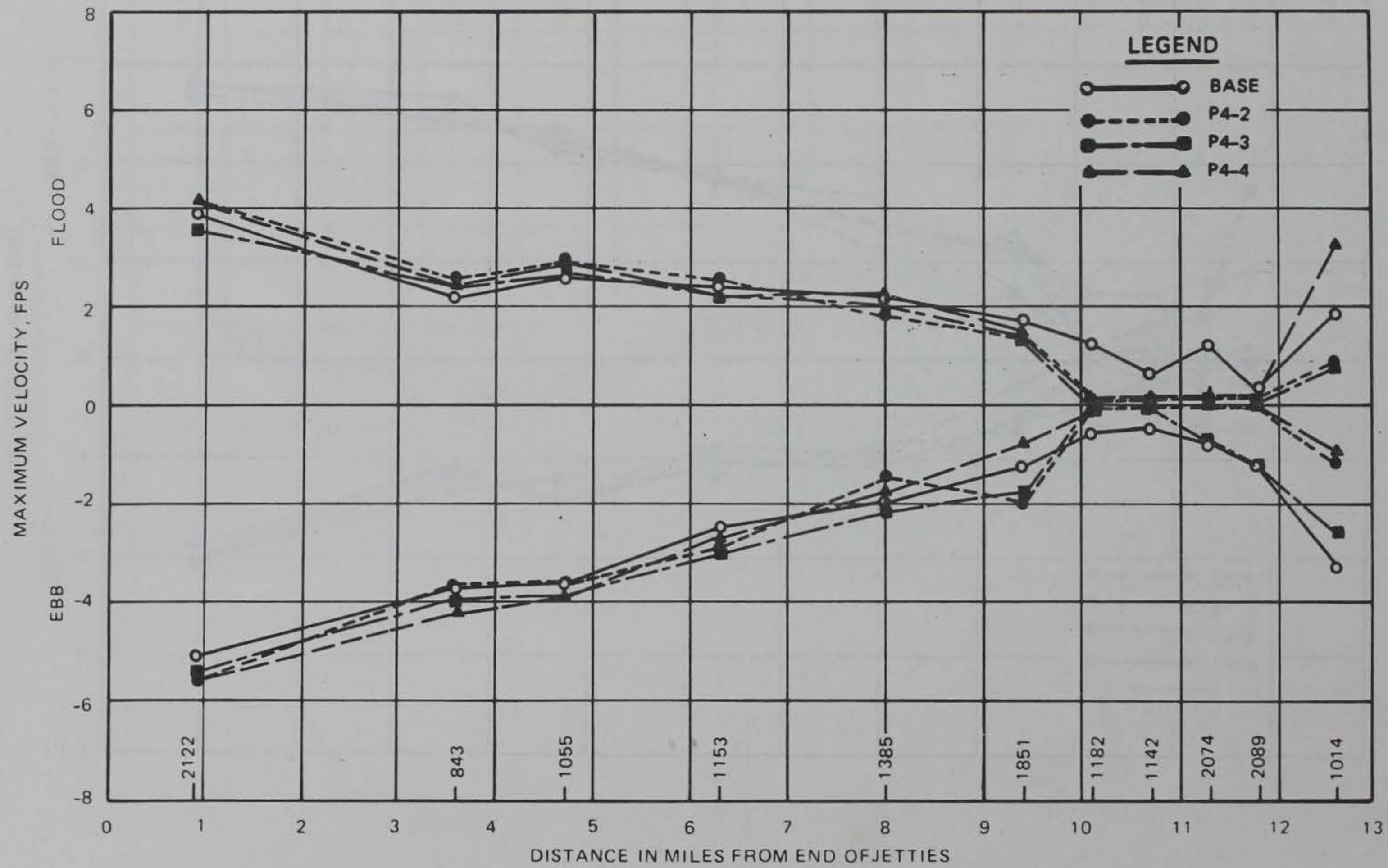
Figure 8. Maximum ebb and flood currents - bottom plans P4-2, P4-3, and P4-4
