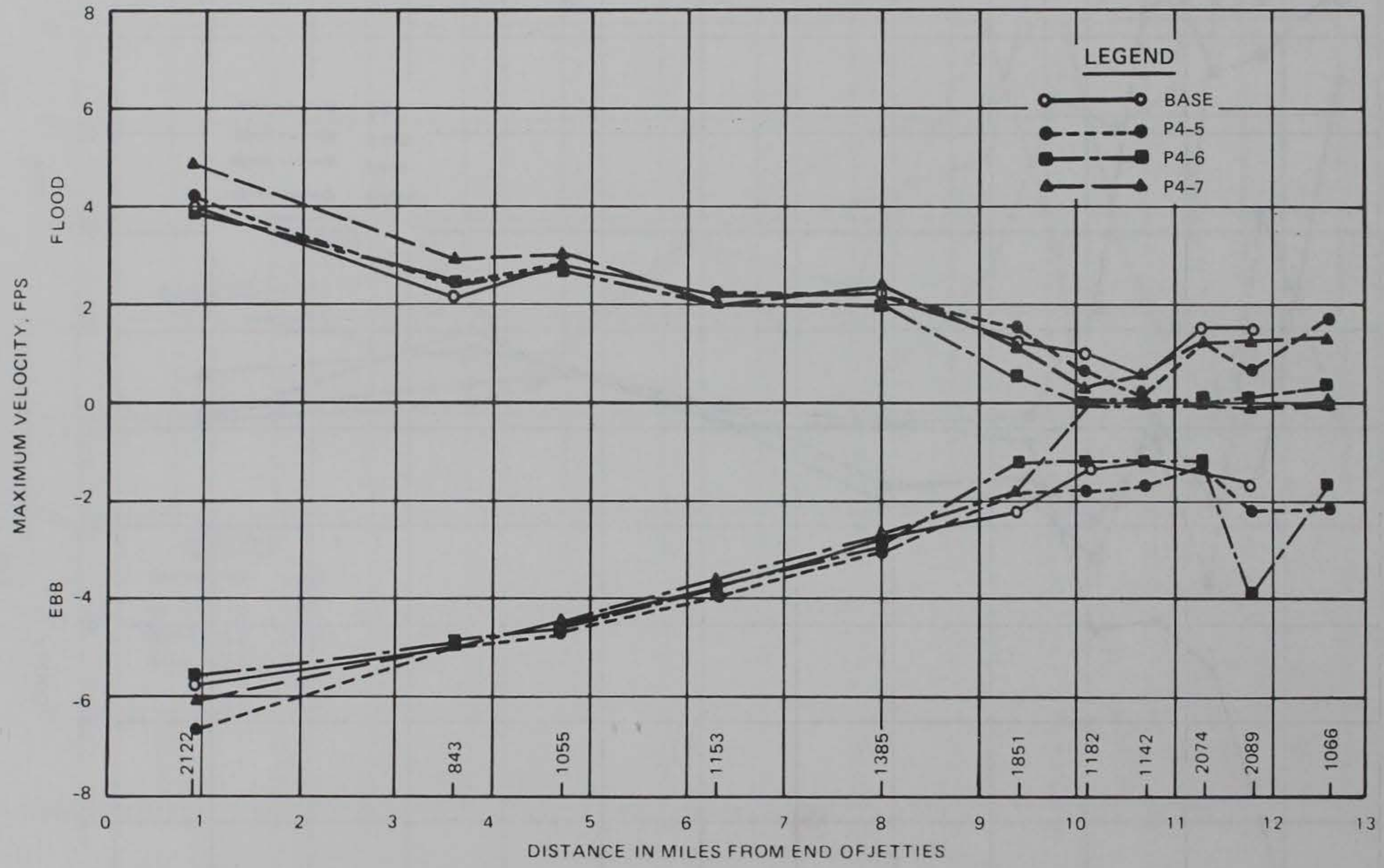
Figure 14. Maximum ebb and flood currents - bottom plans P4-5, P4-6, and P4-7
