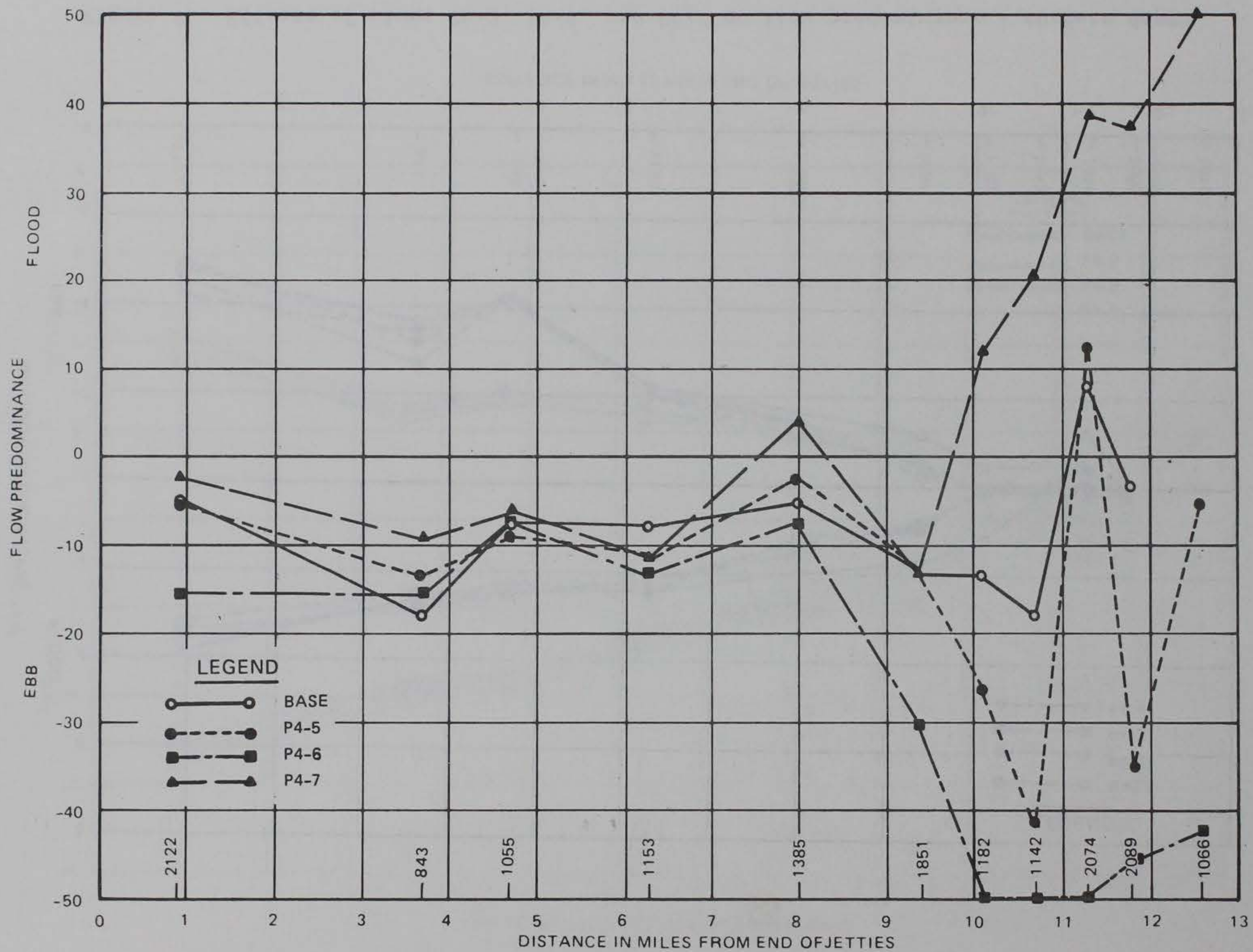
Figure 10. Effects of plans P4-5, P4-6, and P4-7 on flow predominance - middepth
