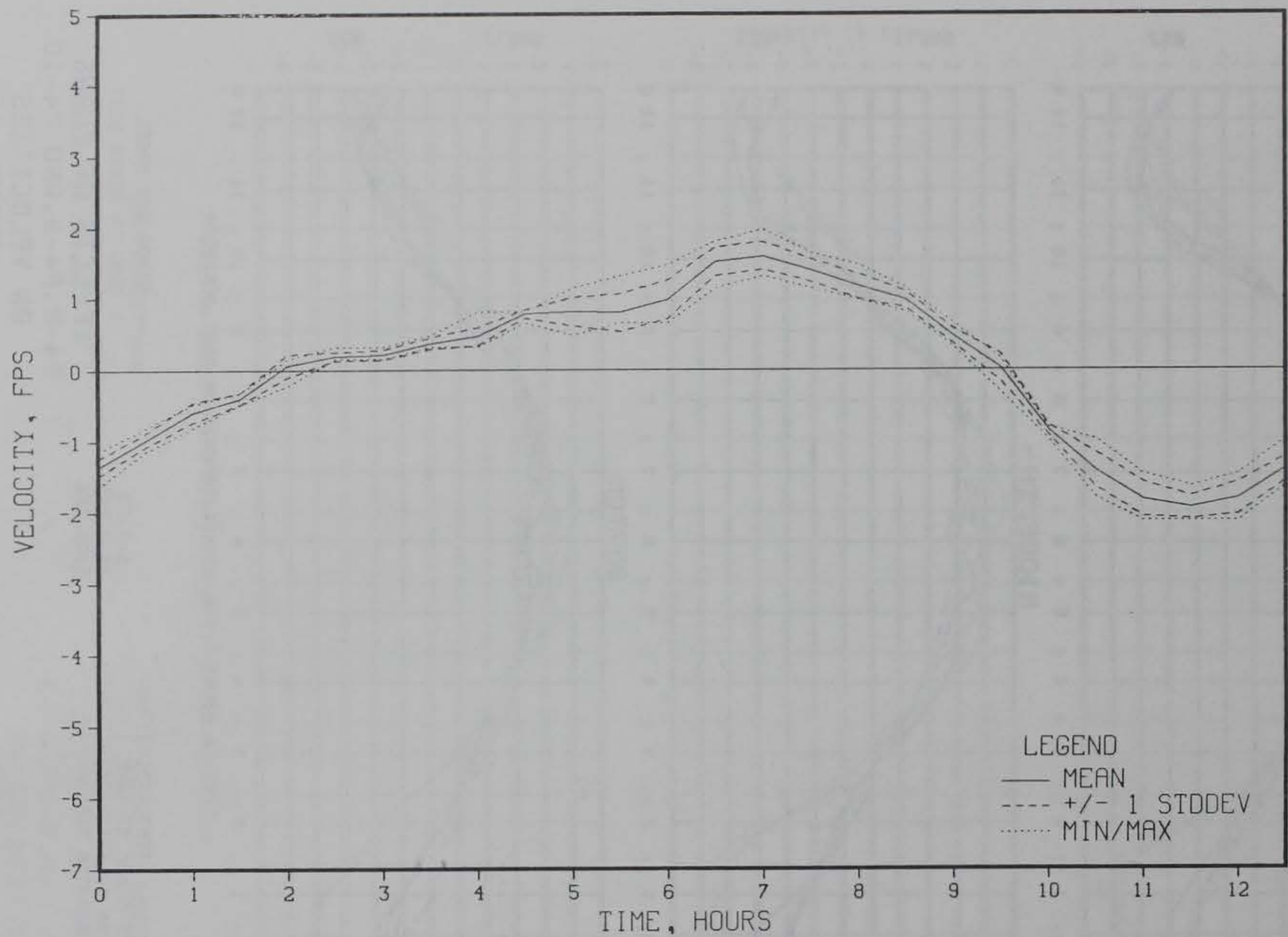
KINGS BAY REPEATABILITY ANALYSIS STATION 60
