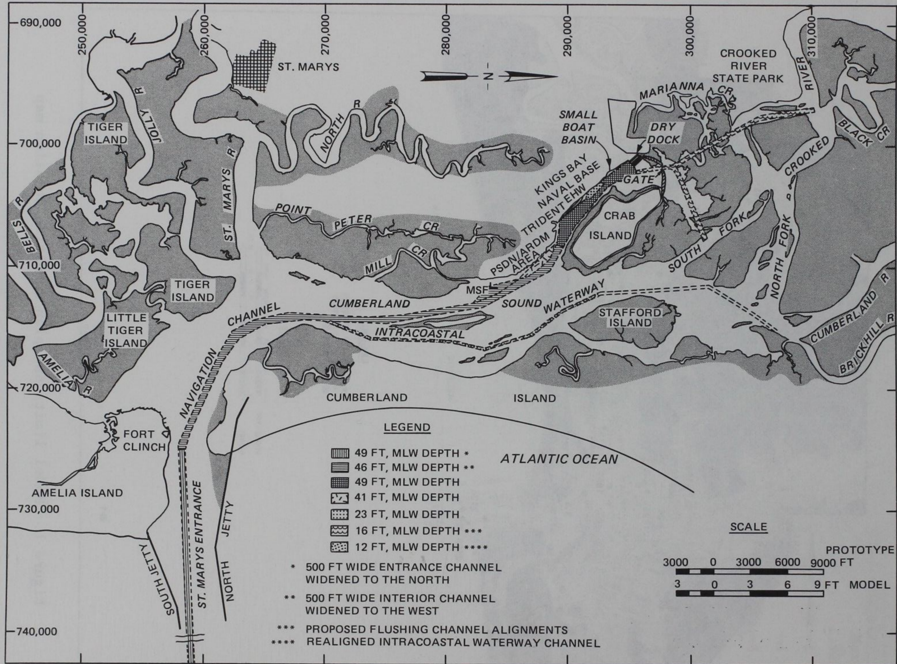
Figure 2. Elements of remedial measure plans
