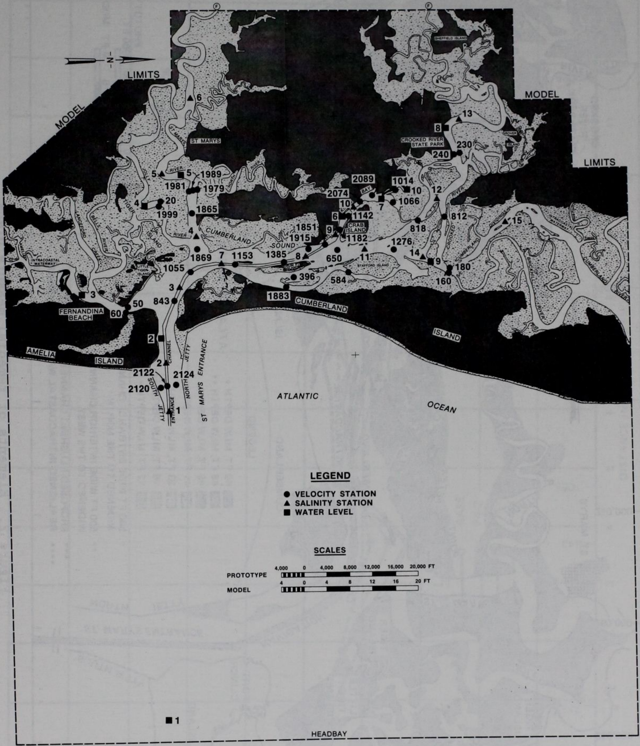
Figure 1. Model limits and plan condition location map
