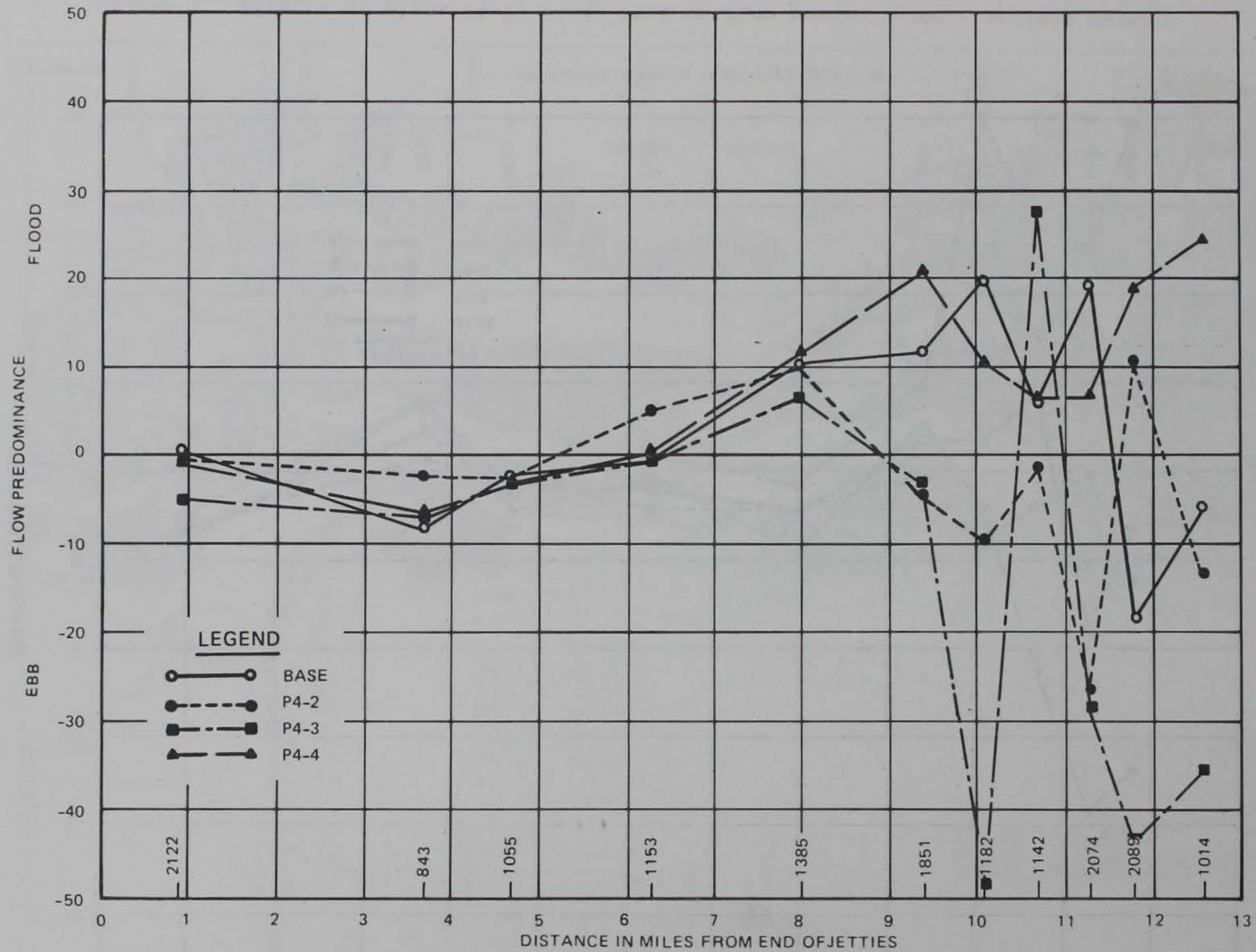
Figure 4. Effects of plans P4-2, P4-3, and P4-4 on flow predominance - middepth
