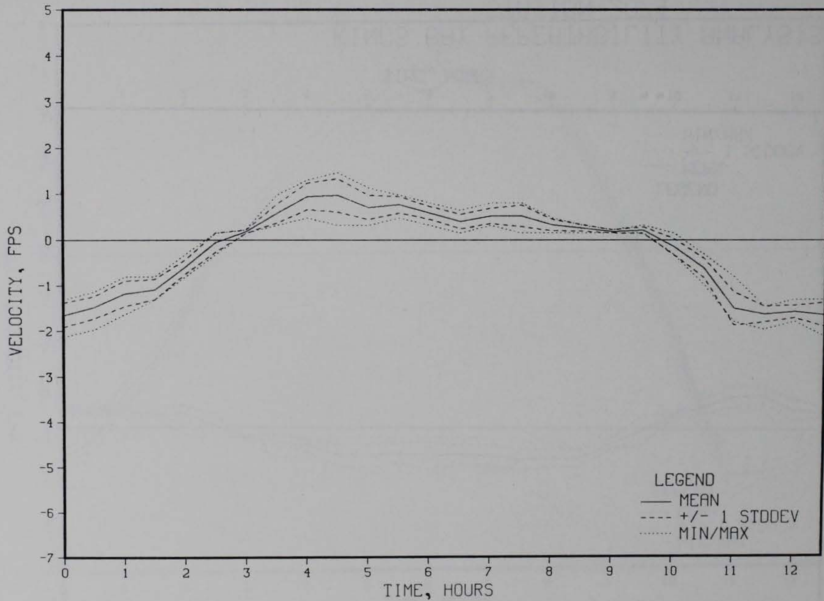
KINGS BAY REPEATABILITY ANALYSIS STATION 1999
