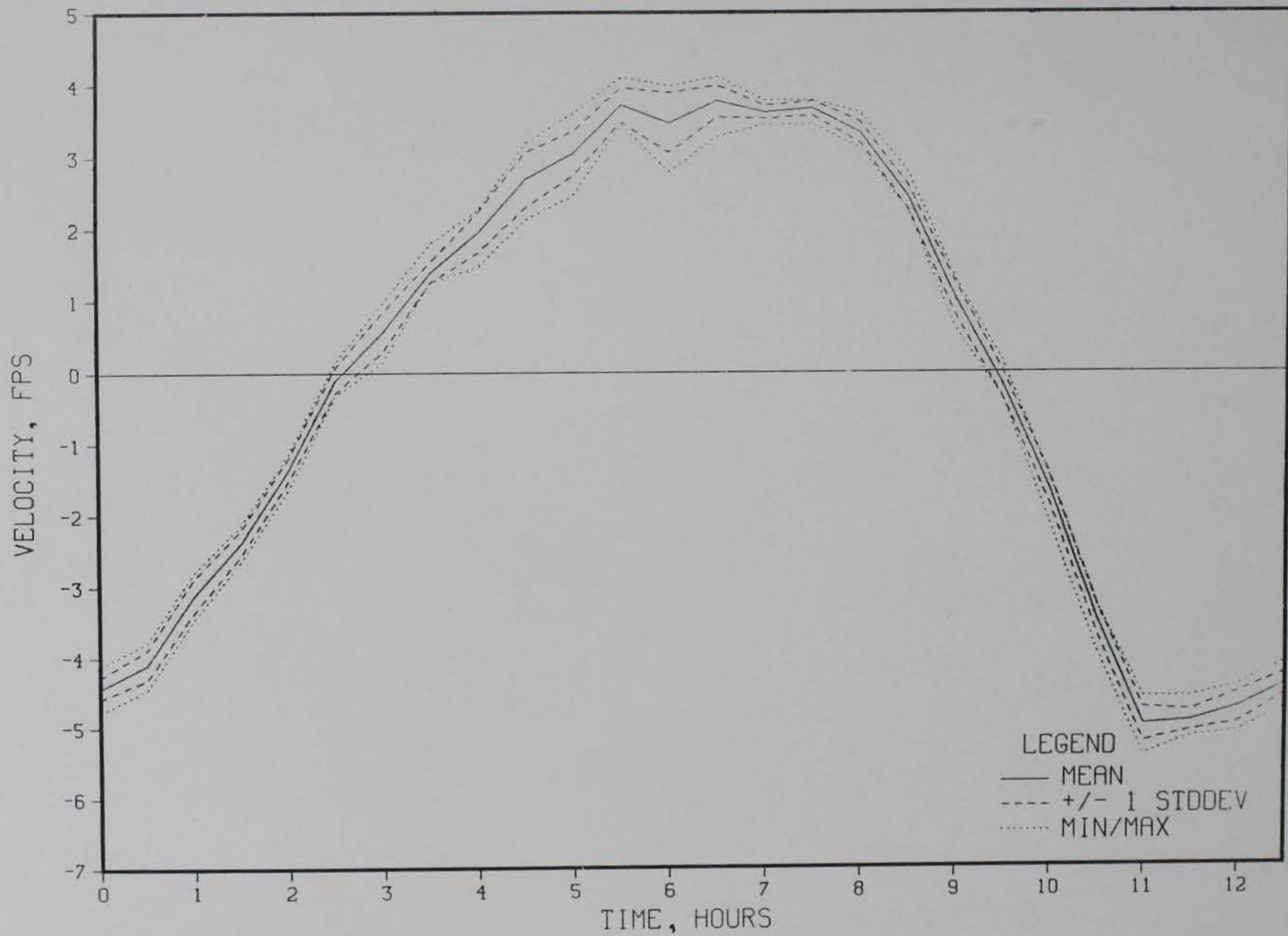
KINGS BAY REPEATABILITY ANALYSIS STATION 2122
