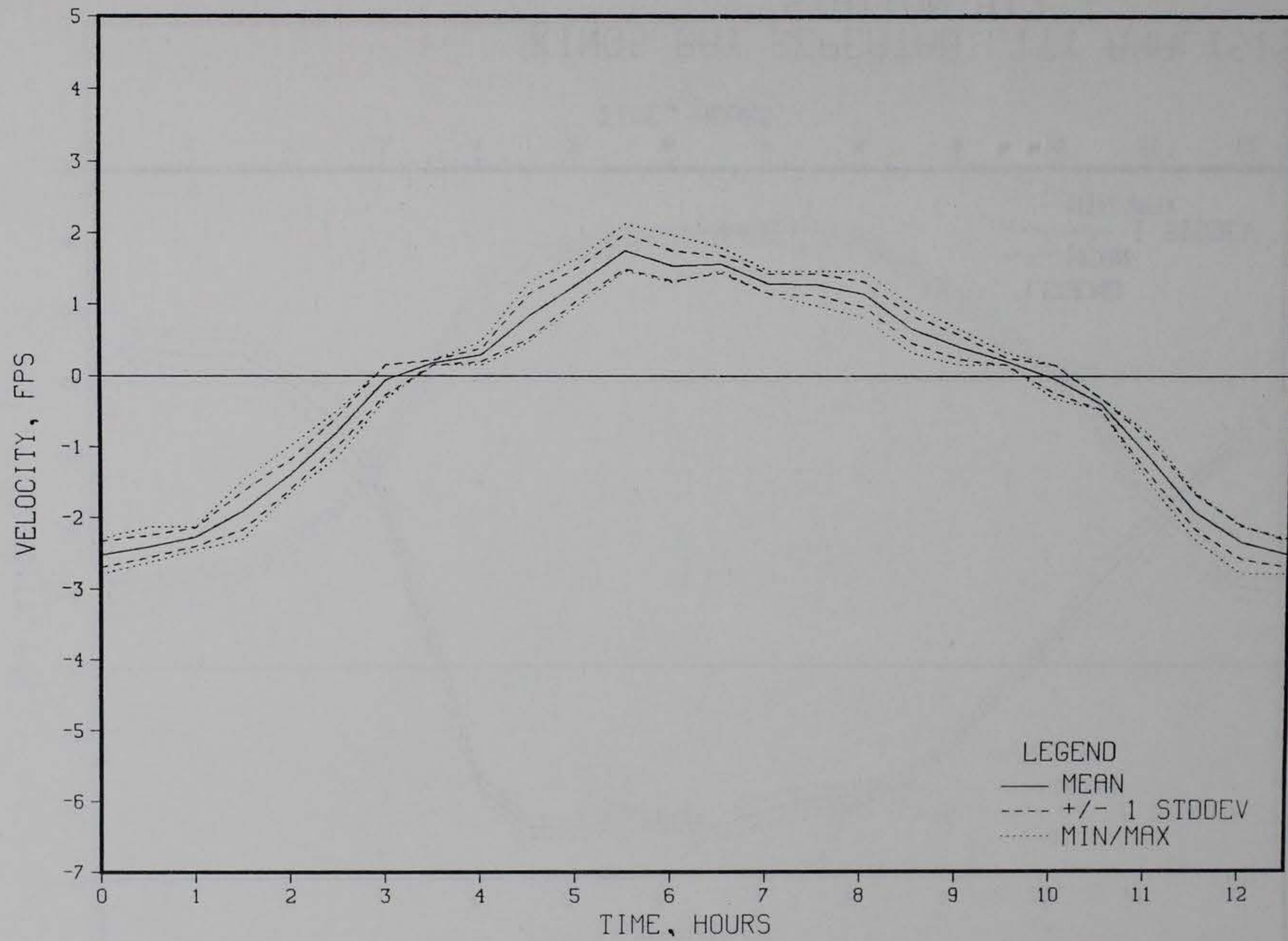
KINGS BAY REPEATABILITY ANALYSIS STATION 650
