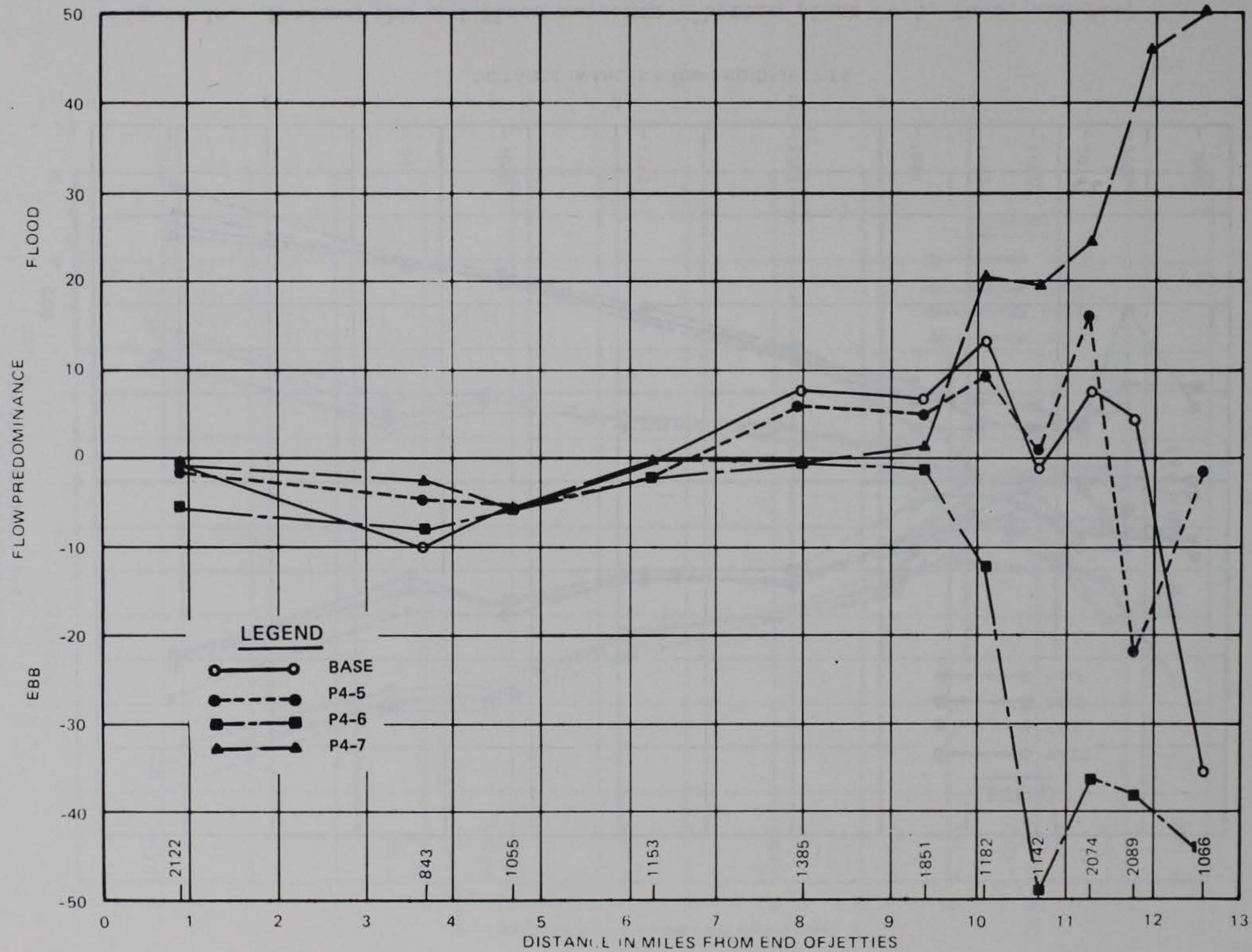
Figure 13. Maximum ebb and flood currents - middepth plans P4-5, P4-6, and P4-7
