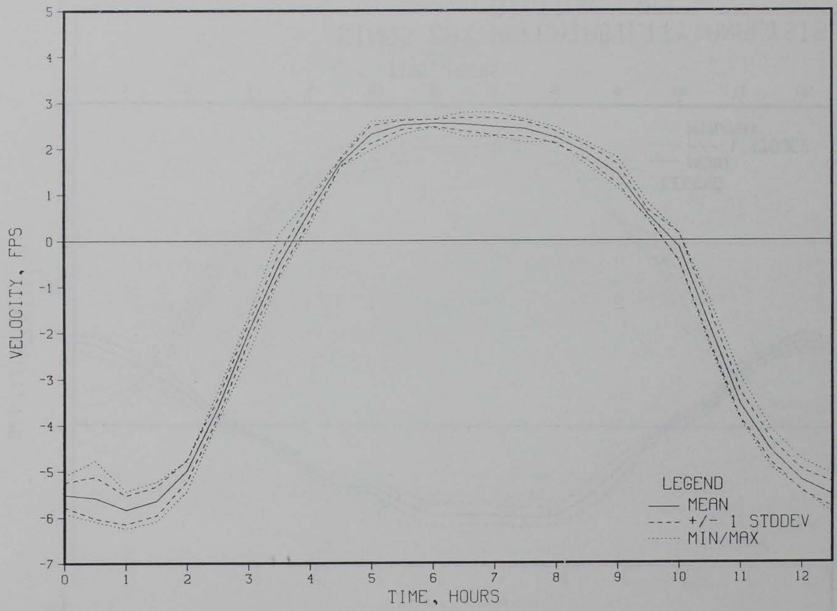
KINGS BAY REPEATABILITY ANALYSIS STATION 1989
