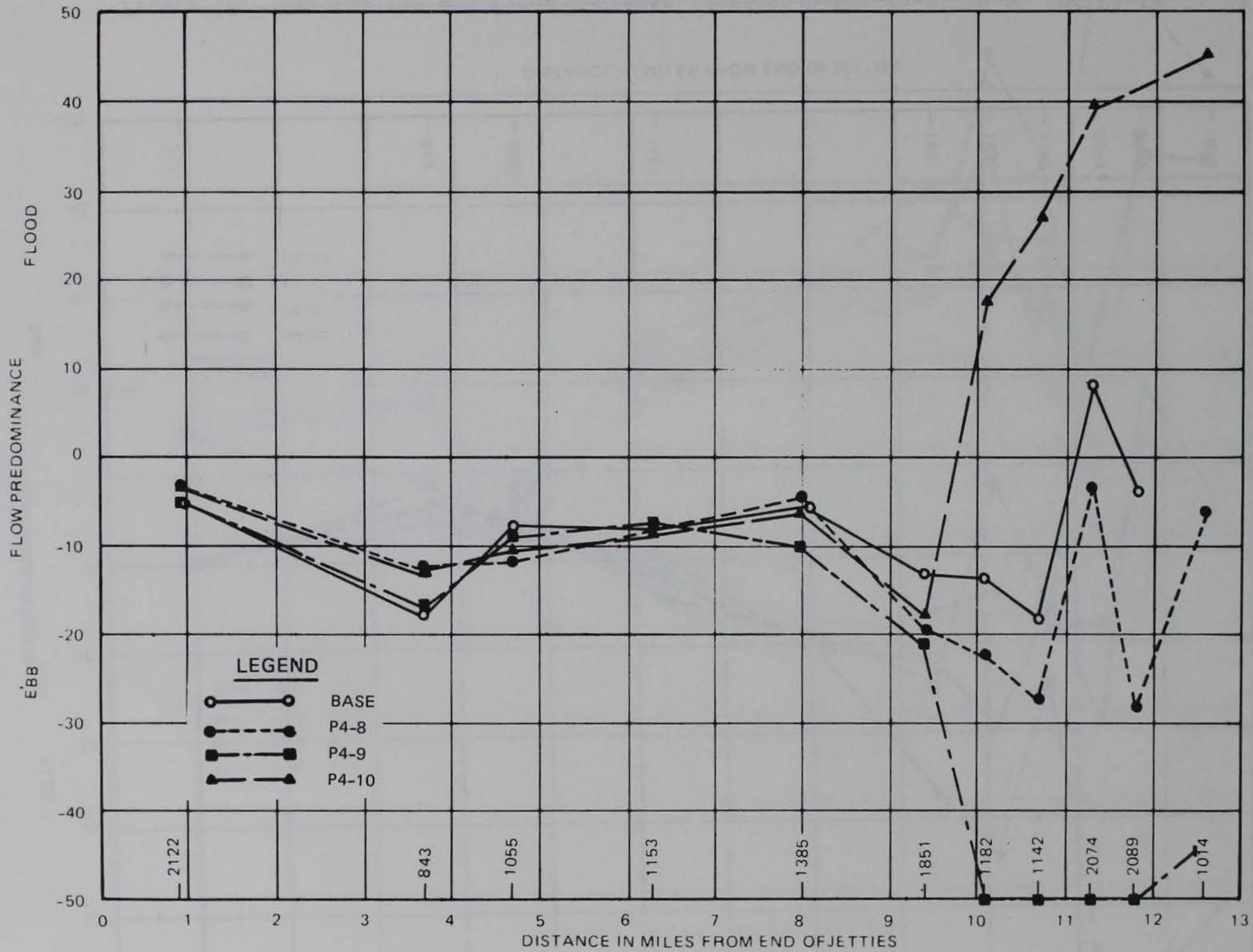
Figure 17. Effects of plans P4-8, P4-9, and P4-10 on flow predominance - bottom
