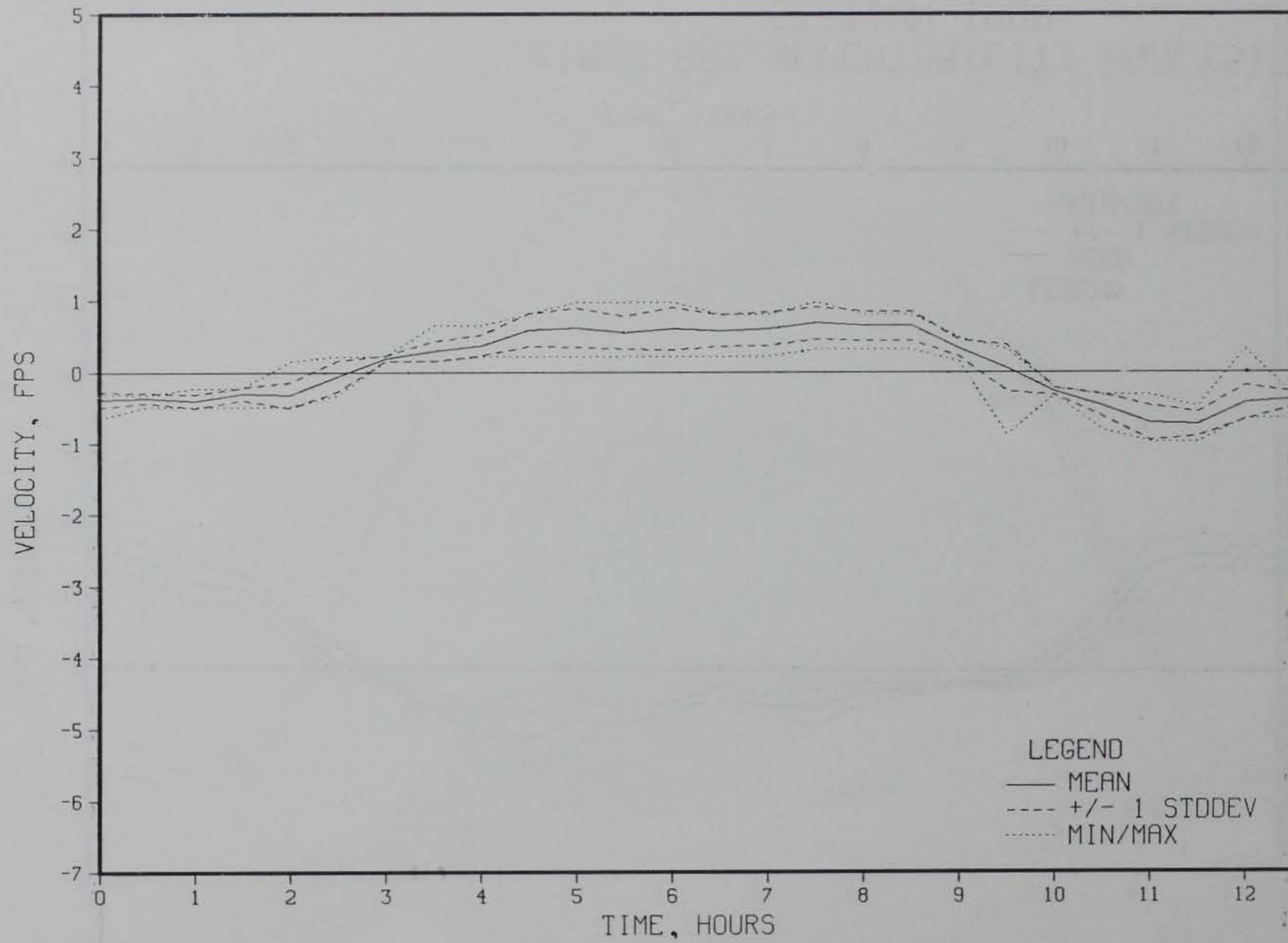
KINGS BAY REPEATABILITY ANALYSIS STATION 2074
