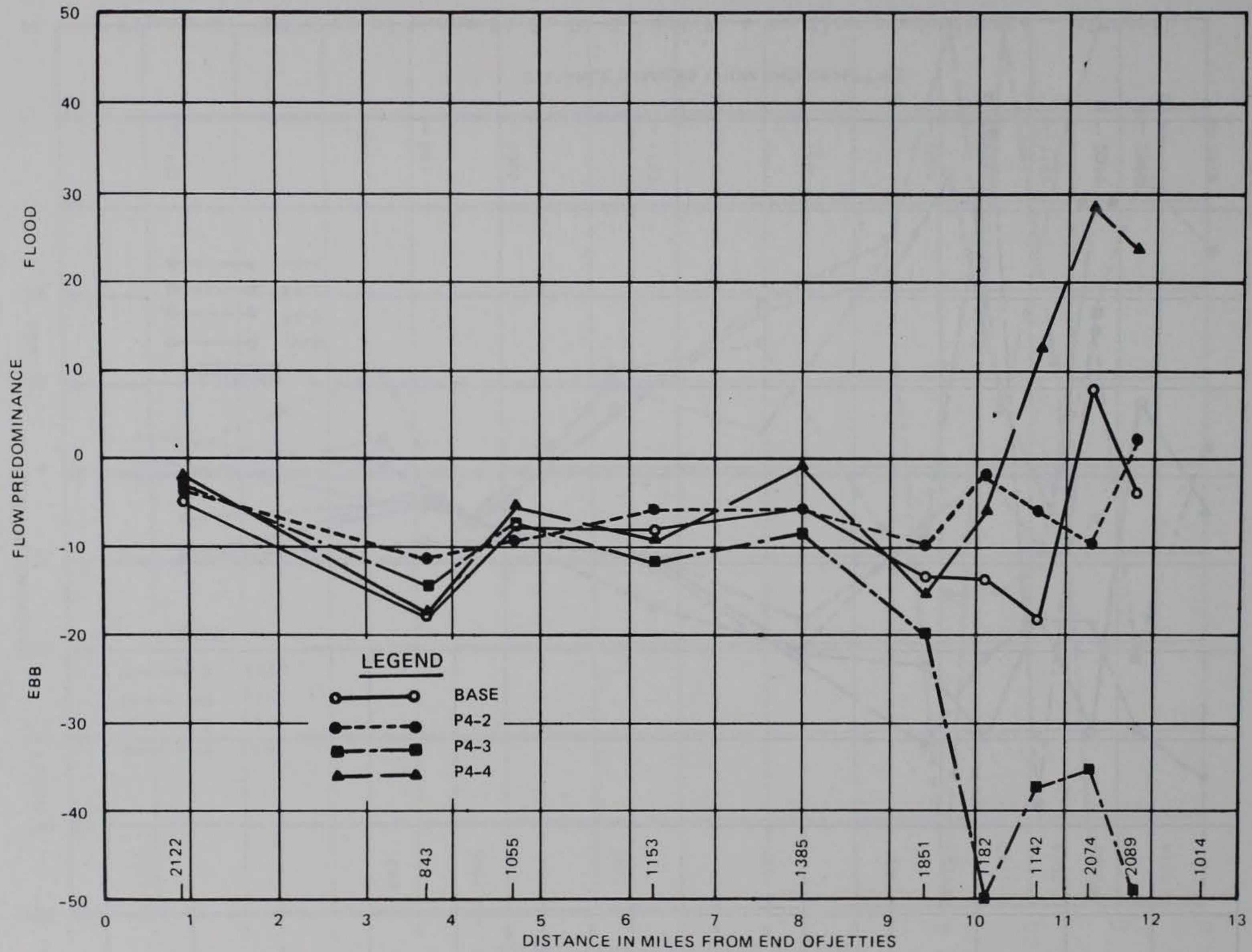
Figure 3. Effects of plans P4-2, P4-3, P4-4 on flow predominance - surface depth
