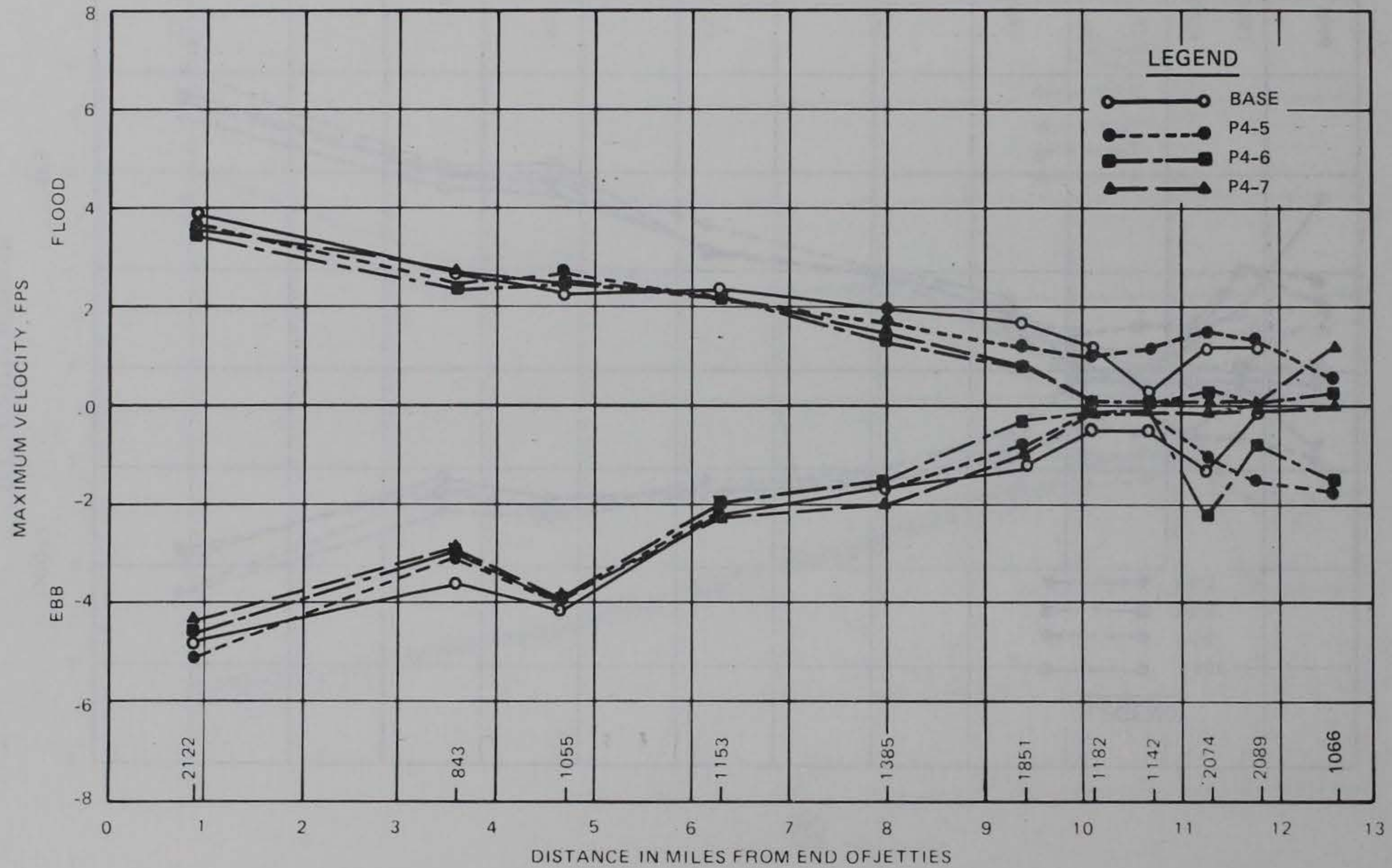
Figure 16. Effects of plans P4-8, P4-9, and P4-10 on flow predominance - middepth
