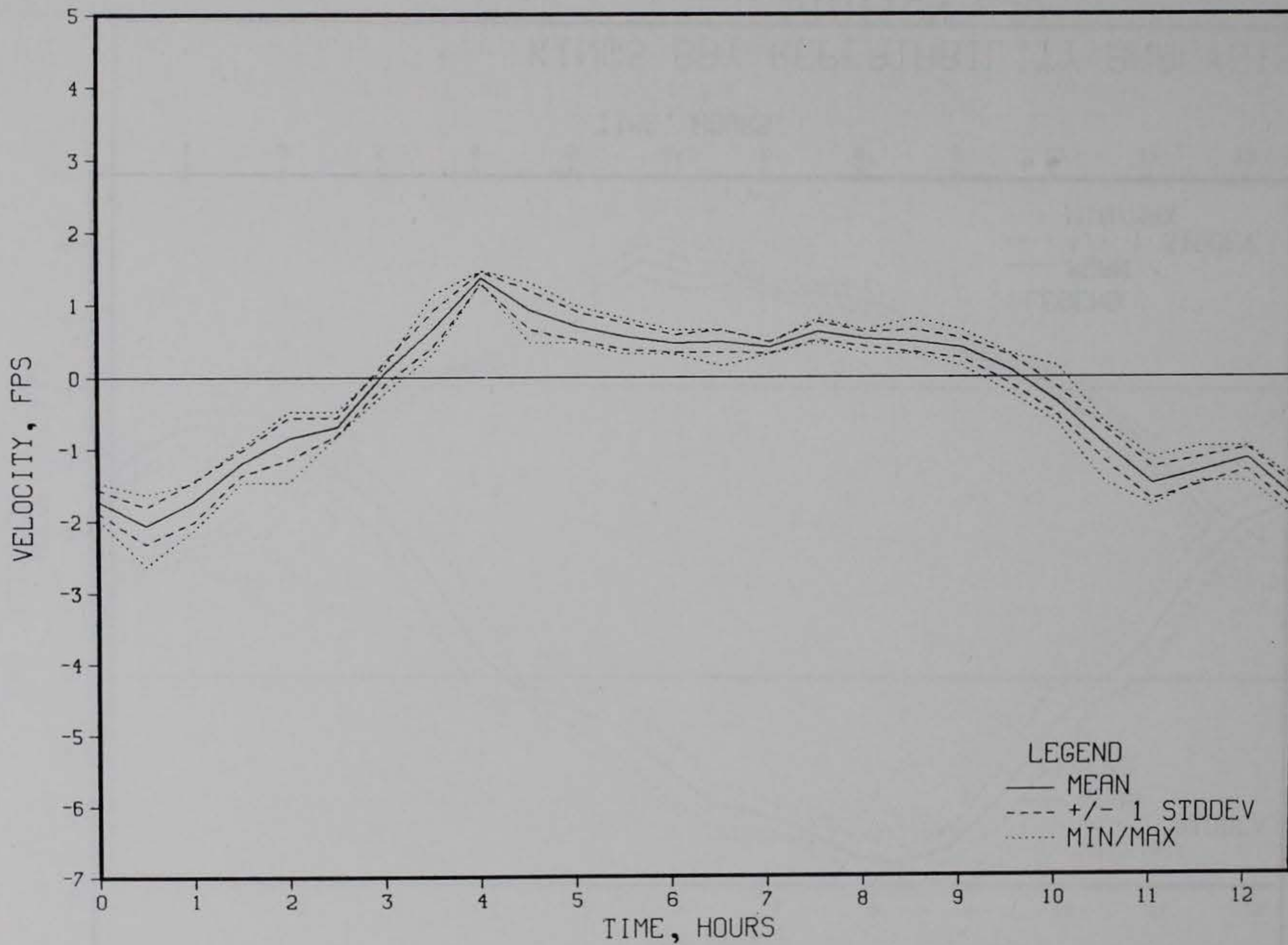
KINGS BAY REPEATABILITY ANALYSIS STATION 160
