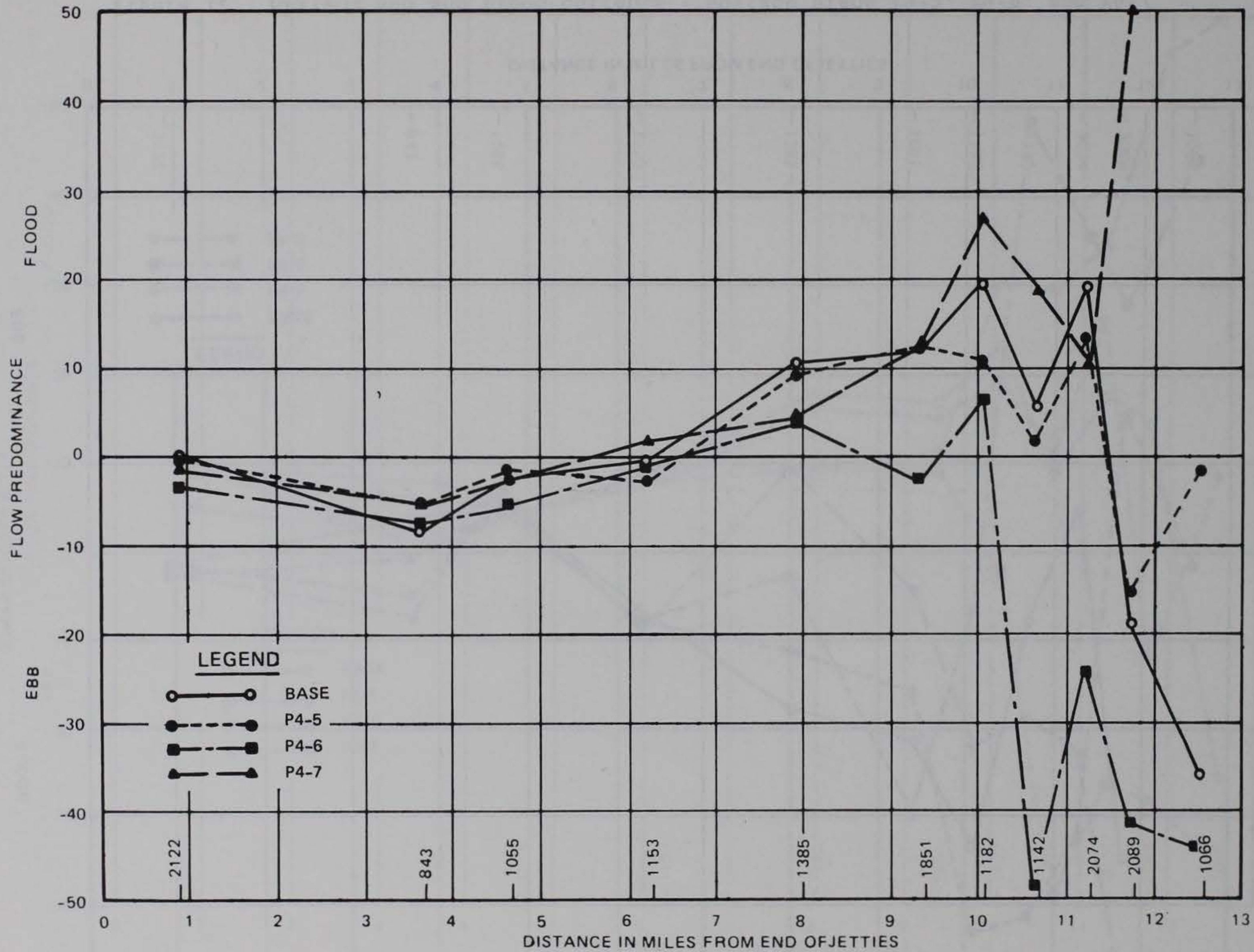
Figure 11. Effects of plans P4-5, P4-6, and P4-7 on flow predominance - bottom depth
