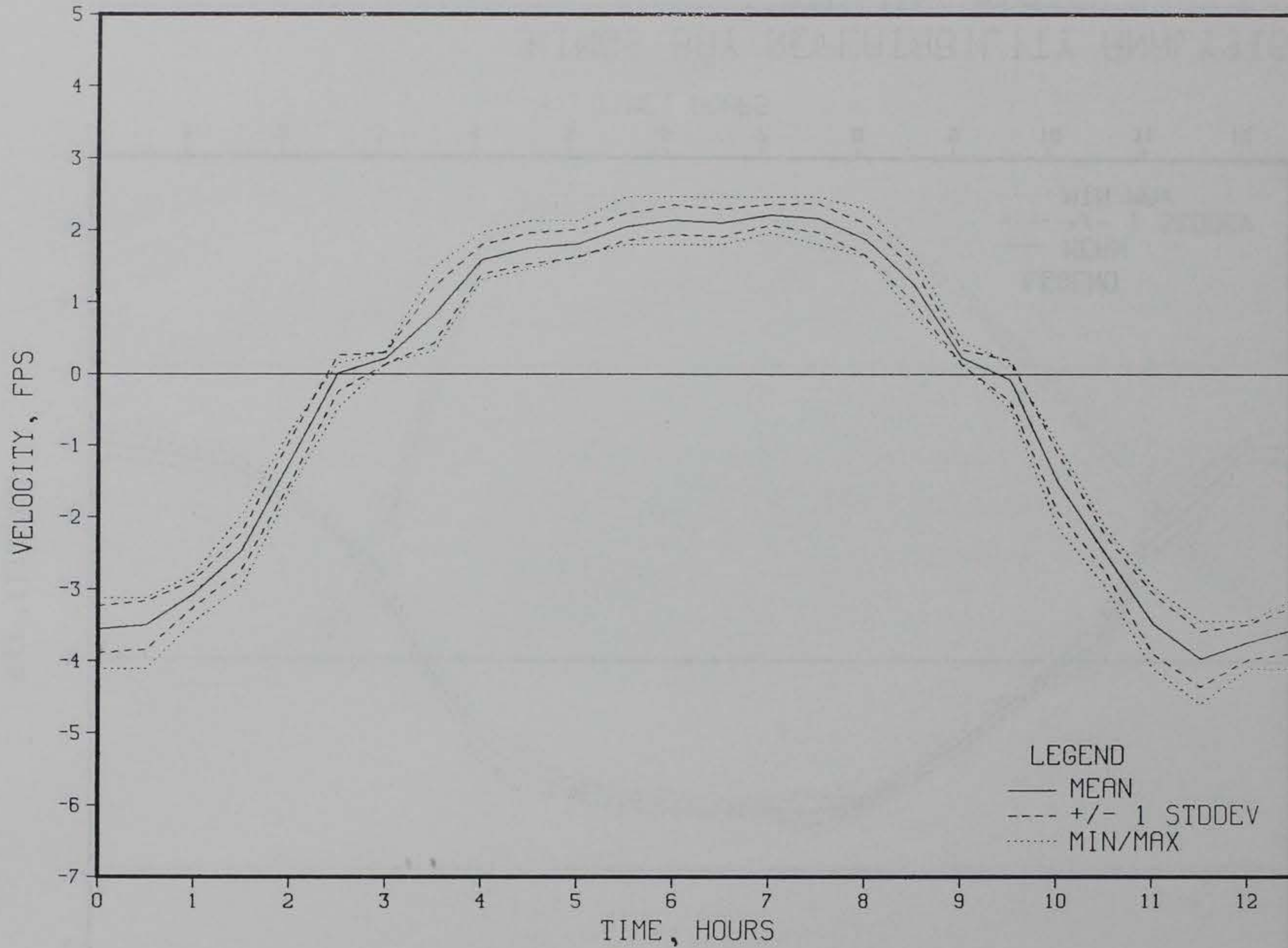
KINGS BAY REPEATABILITY ANALYSIS STATION 843
