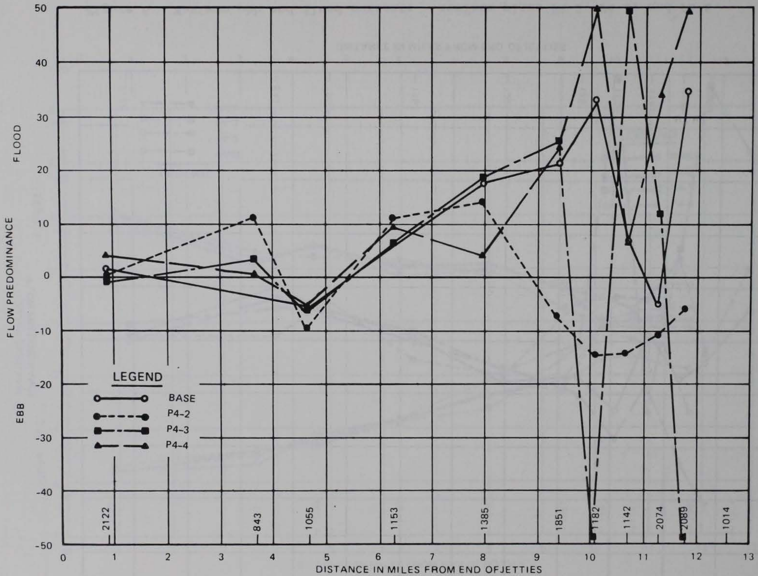
Figure 5. Effects of plans P4-2, P4-3, and P4-4 on flow predominance - bottom depth
