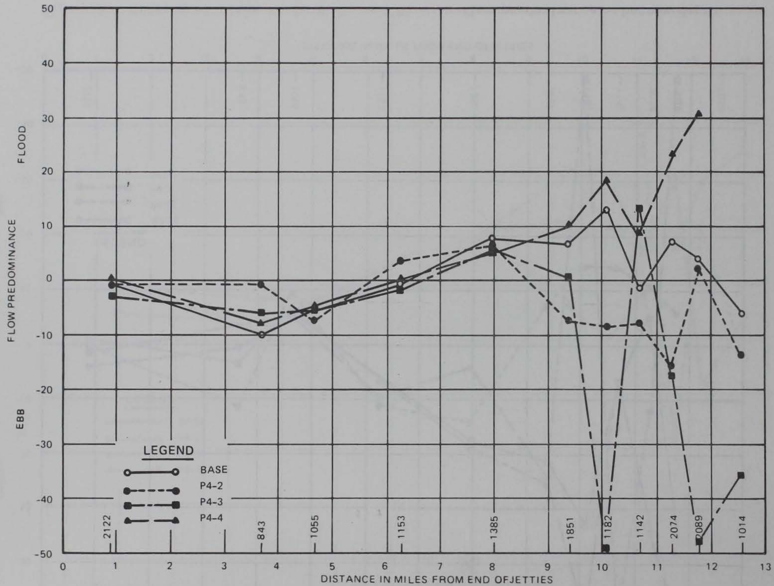
Figure 6. Maximum ebb and flood currents - surface plans P4-2, P4-3, and P4-4
