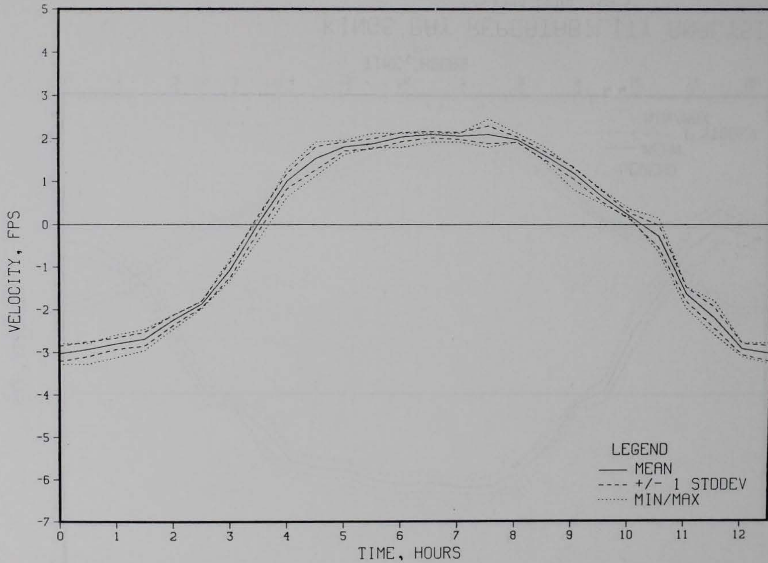
KINGS BAY REPEATABILITY ANALYSIS STATION 818
