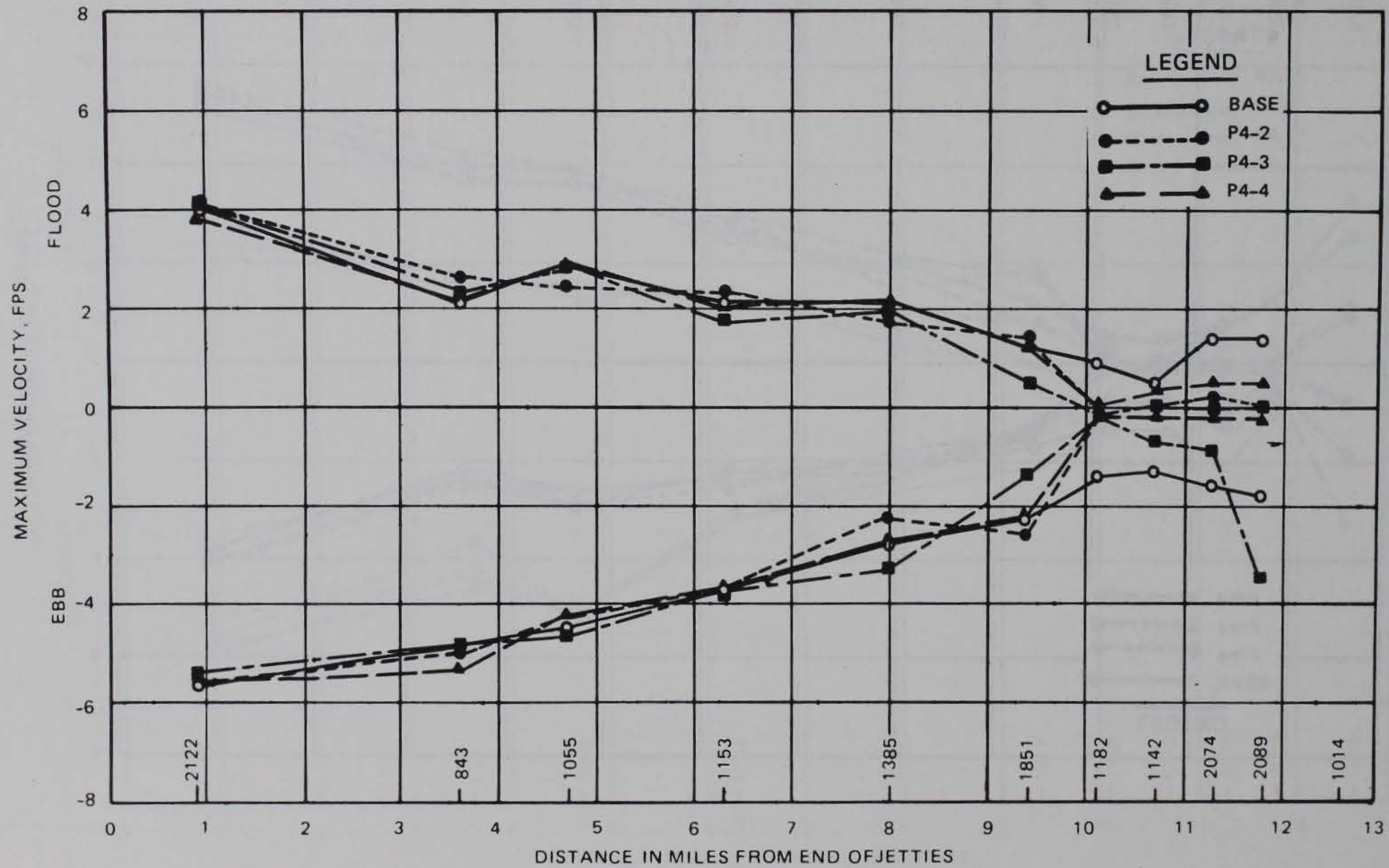
Figure 7. Maximum ebb and flood currents - middepth plans P4-2, P4-3, and P4-4
