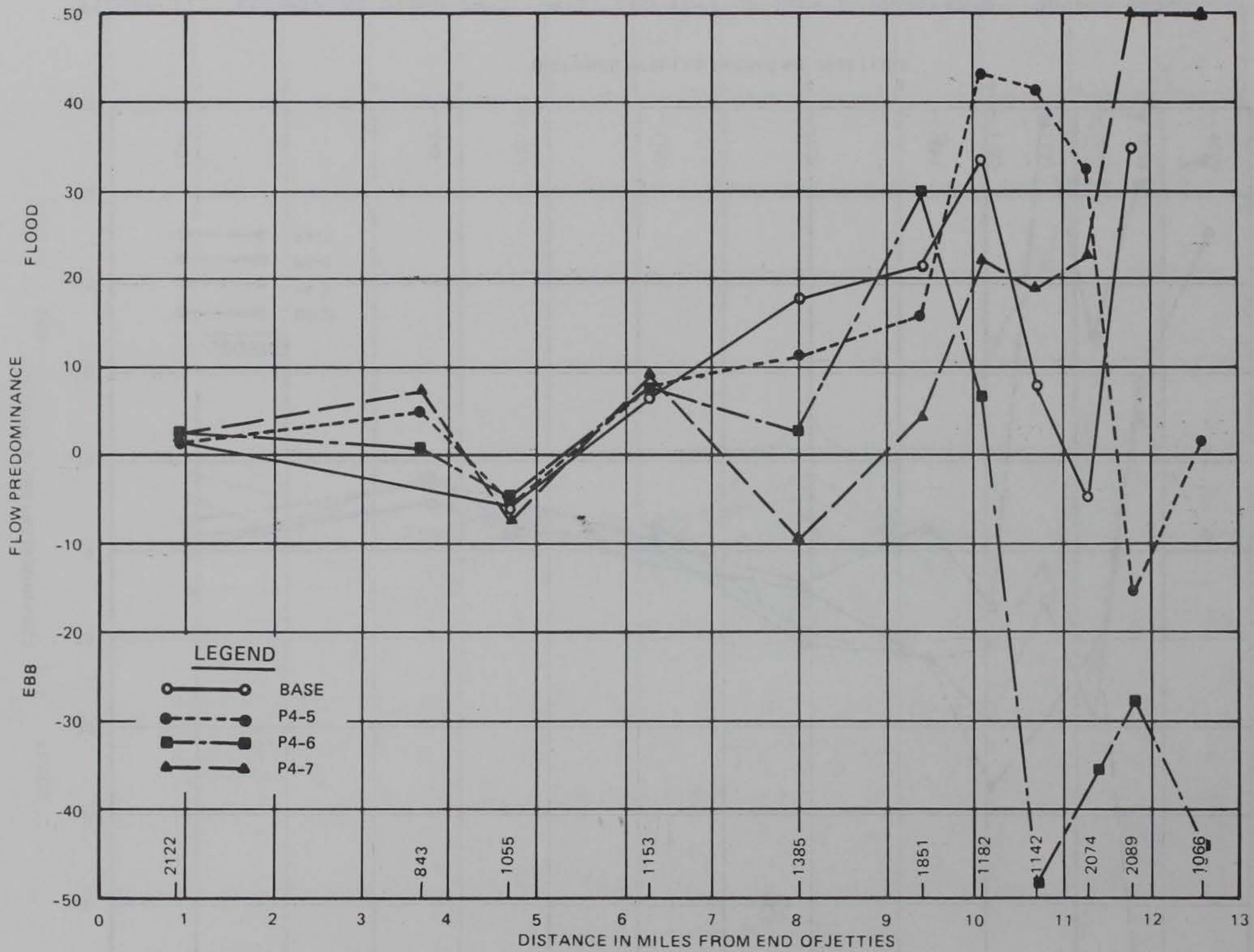
Figure 12. Maximum ebb and flood currents - surface plans P4-5, P4-6, and P4-7
