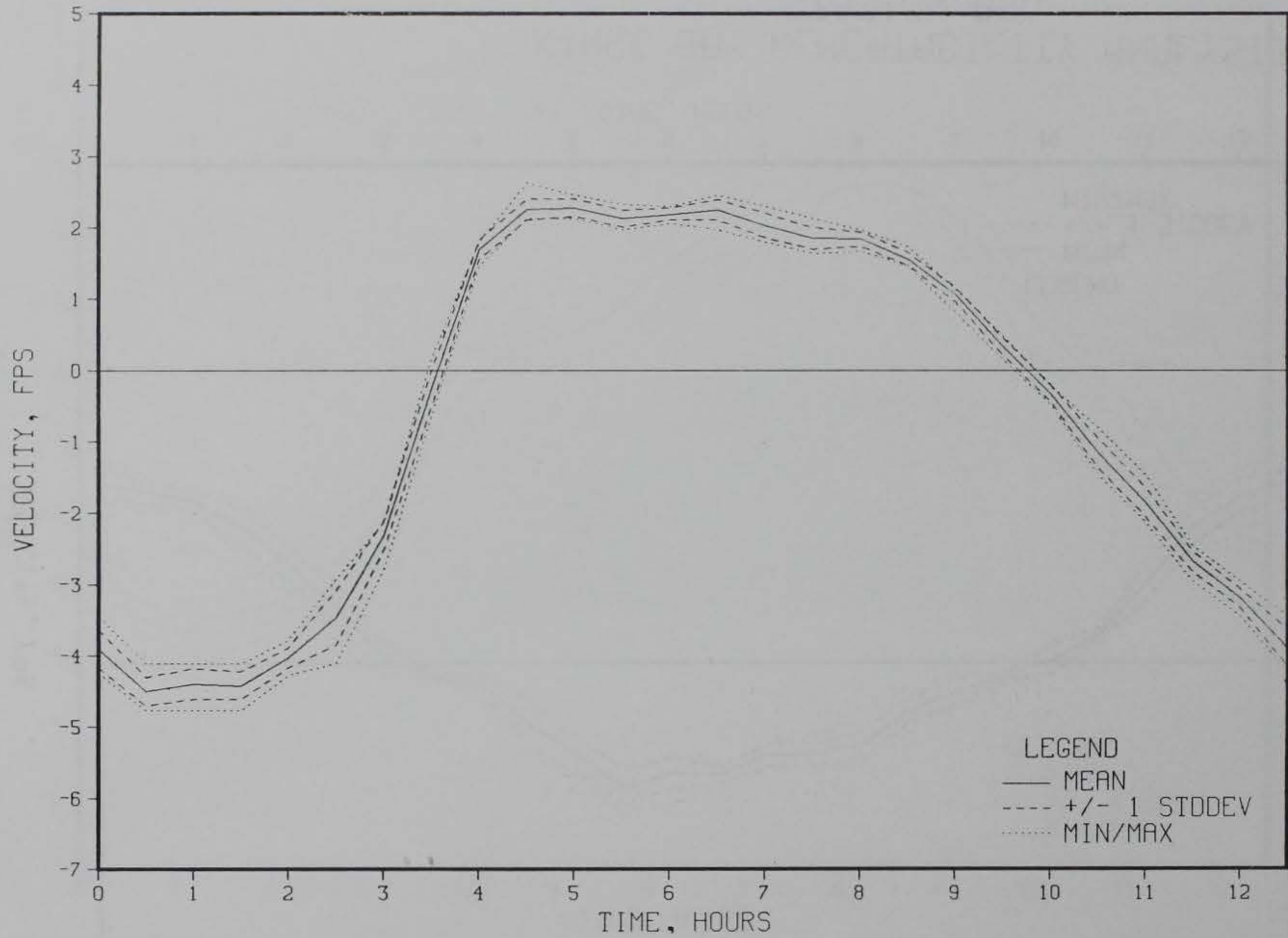
KINGS BAY REPEATABILITY ANALYSIS STATION 812
