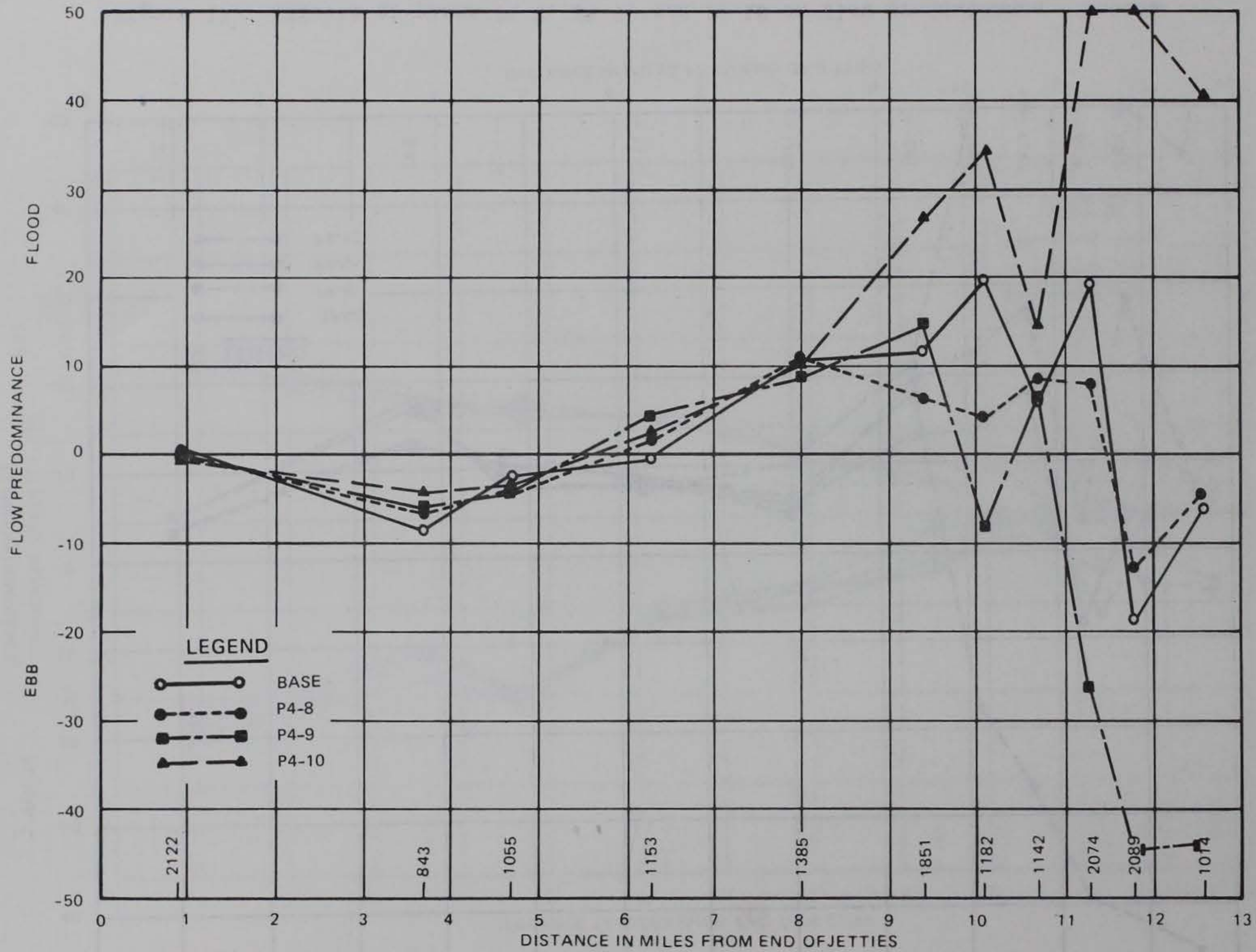
Figure 18. Maximum ebb and flood currents, surface plans P4-8, P4-9, and P4-10
